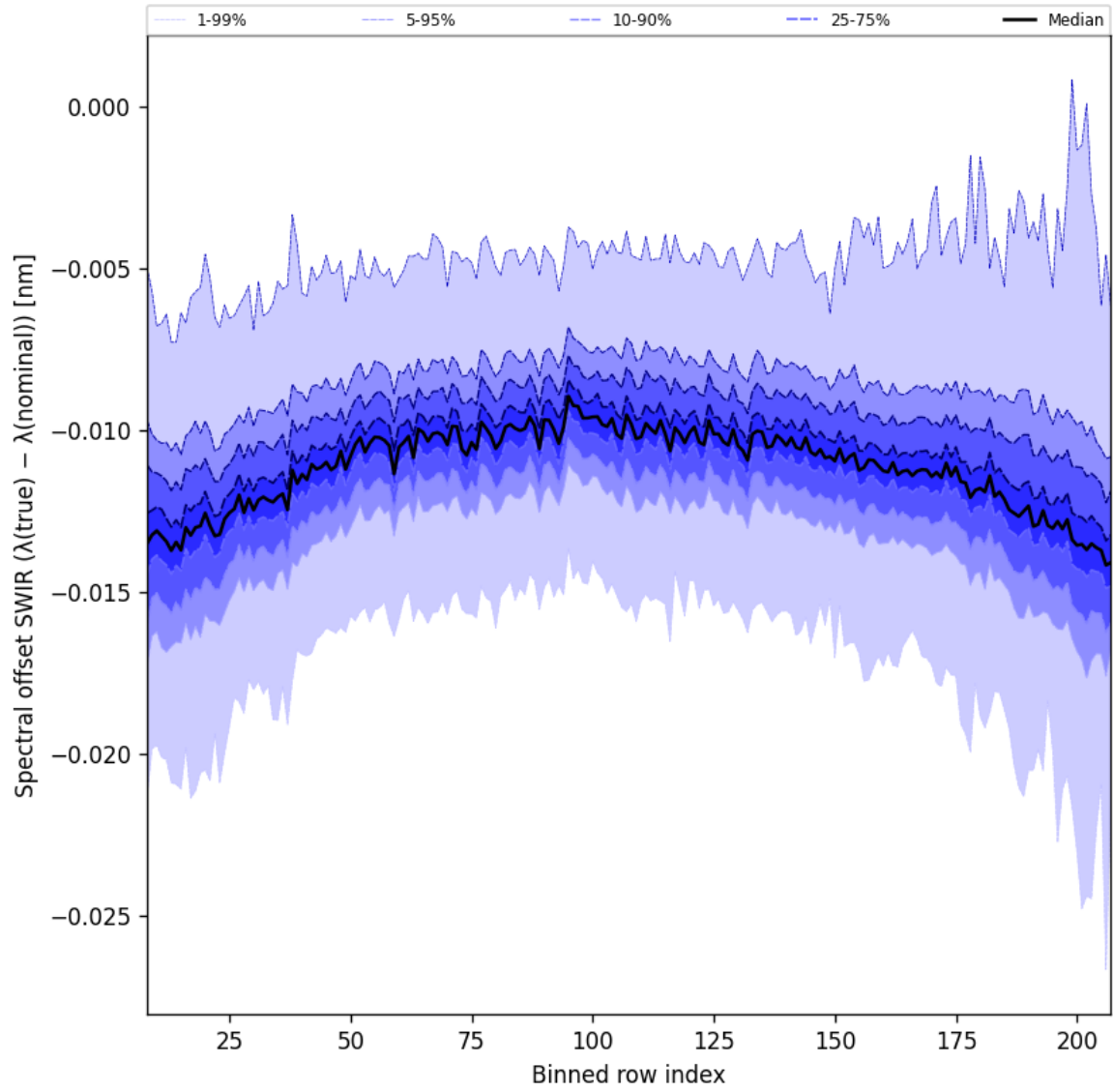
Figure 38: Along track statistics of “Spectral offset SWIR ( \lambda_{\text{true}} - \lambda_{\text{nominal}} )” for 2025-01-23 to 2025-01-24
