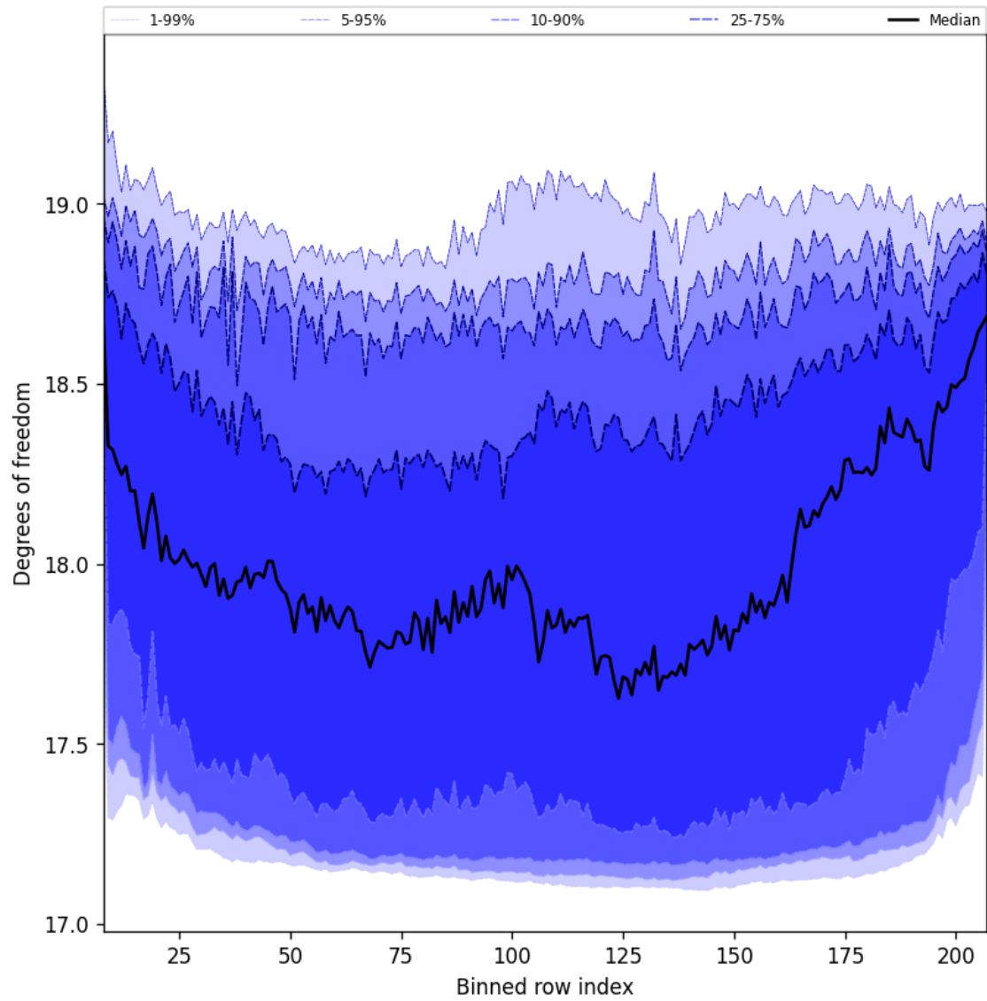
Figure 41: Along track statistics of “Degrees of freedom” for 2025-01-23 to 2025-01-24
