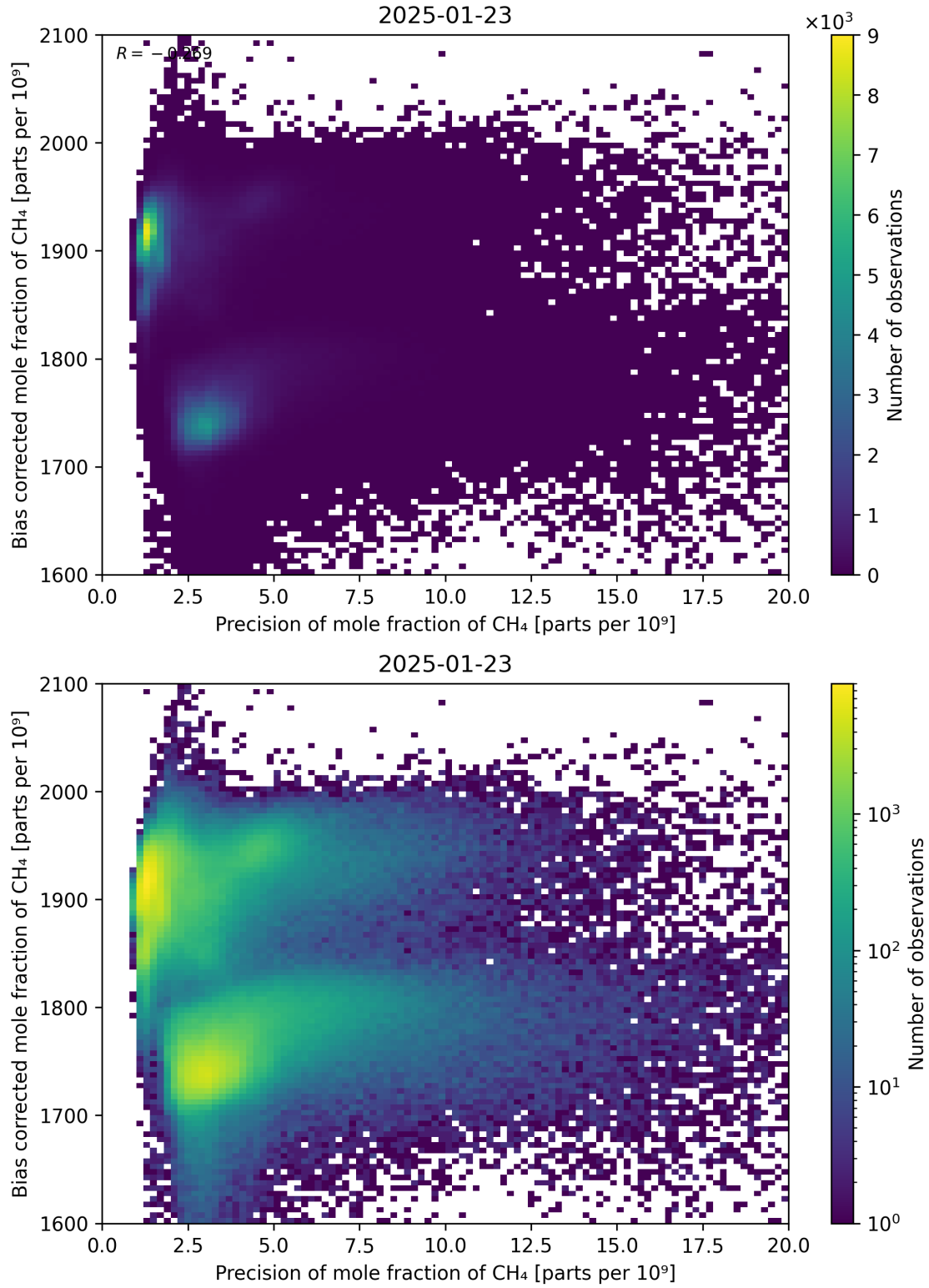
Figure 82: Scatter density plot of “Precision of mole fraction of CH 4 ” against “Bias corrected mole fraction of CH 4 ” for 2025-01-23 to 2025-01-24.
