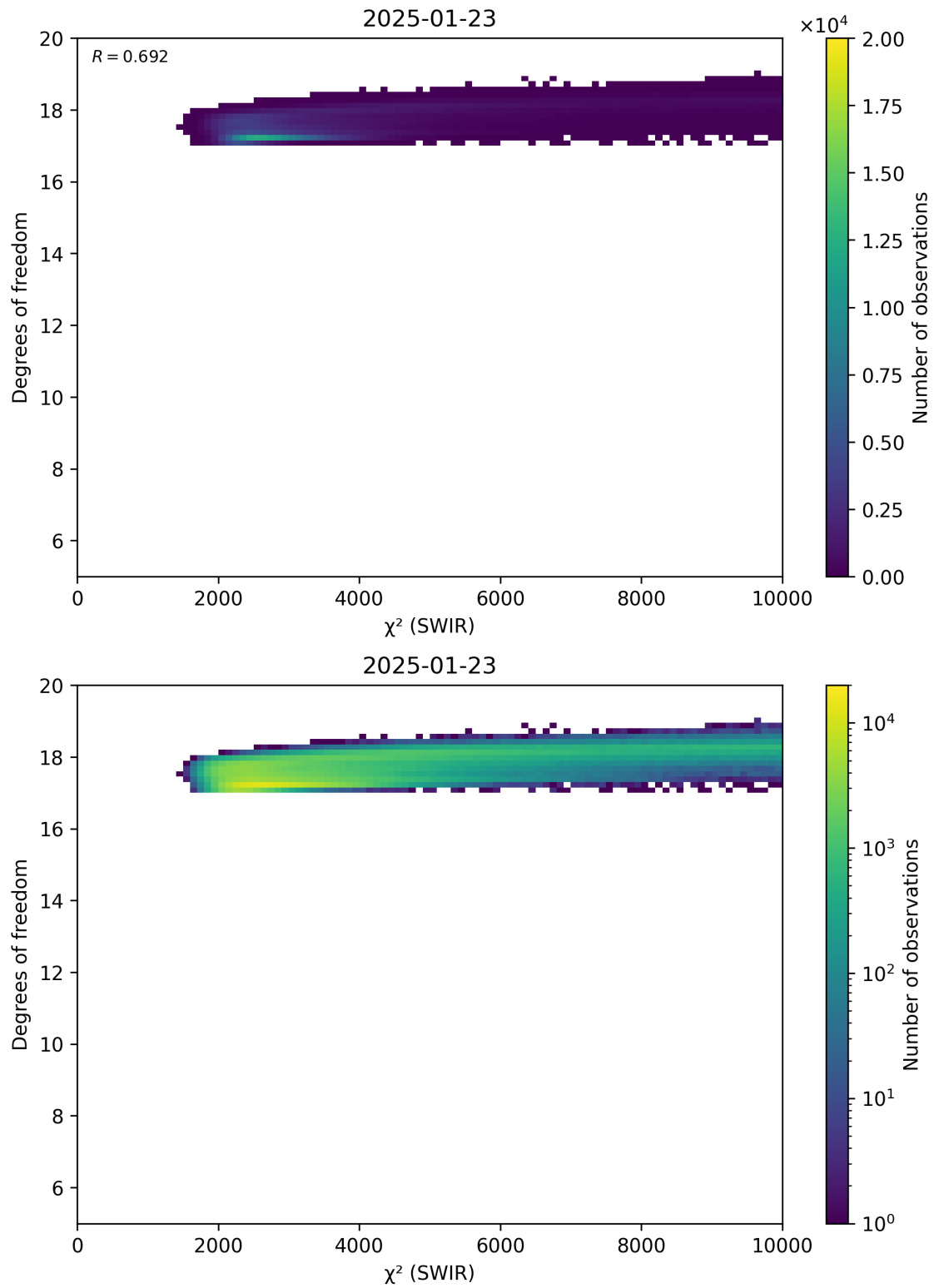
Figure 48: Scatter density plot of “ \chi^2 (SWIR)” against “Degrees of freedom” for 2025-01-23 to 2025-01-24.
