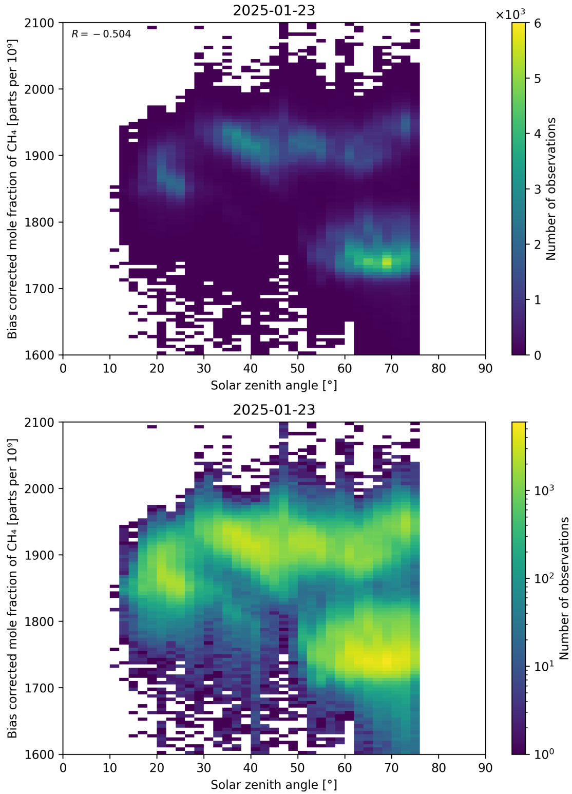
Figure 100: Scatter density plot of “Solar zenith angle” against “Bias corrected mole fraction of CH 4 ” for 2025-01-23 to 2025-01-24.
