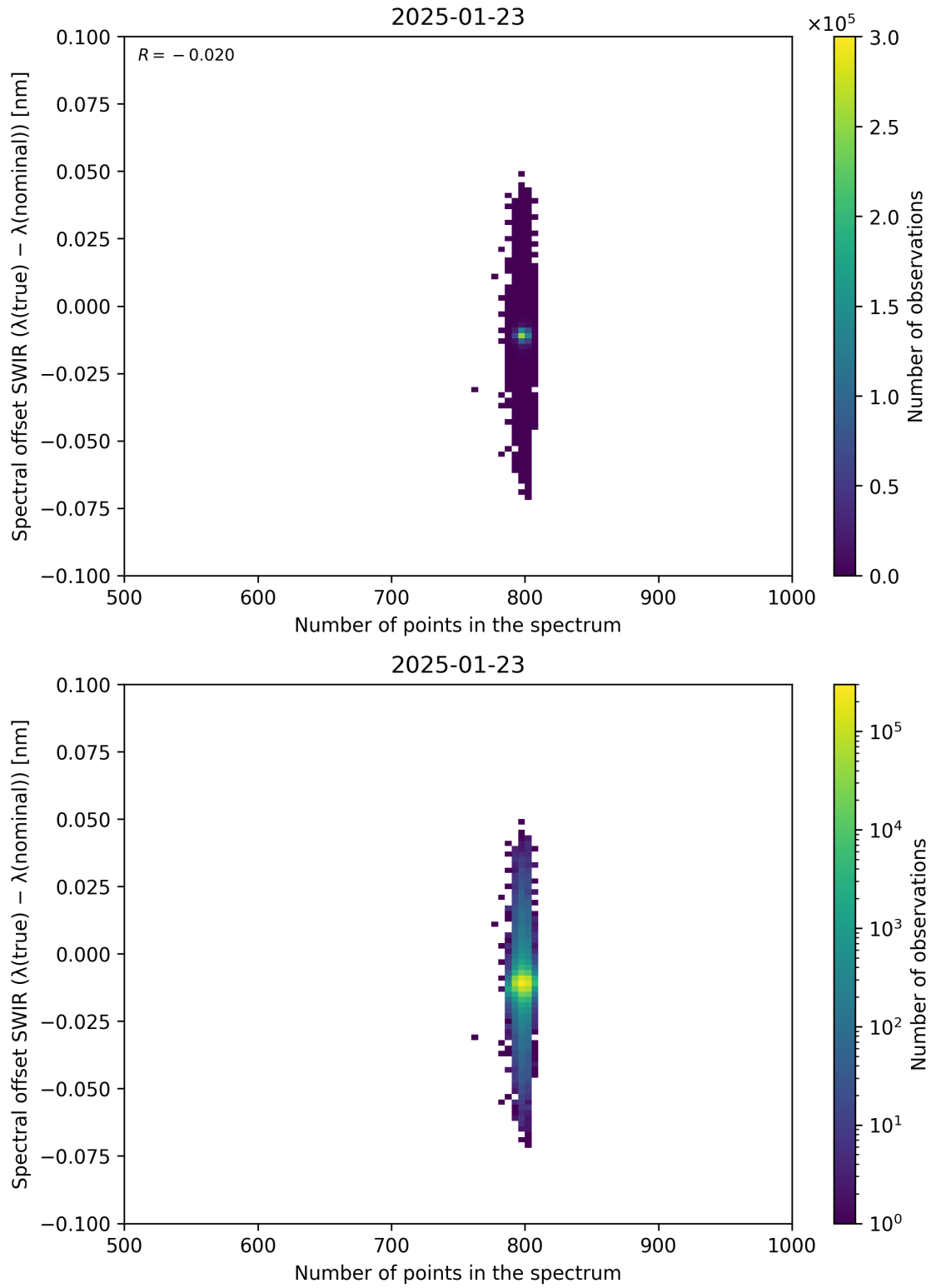
Figure 93: Scatter density plot of “Number of points in the spectrum” against “Spectral offset SWIR ( \lambda_{\text{true}} - \lambda_{\text{nominal}} )” for 2025-01-23 to 2025-01-24.
