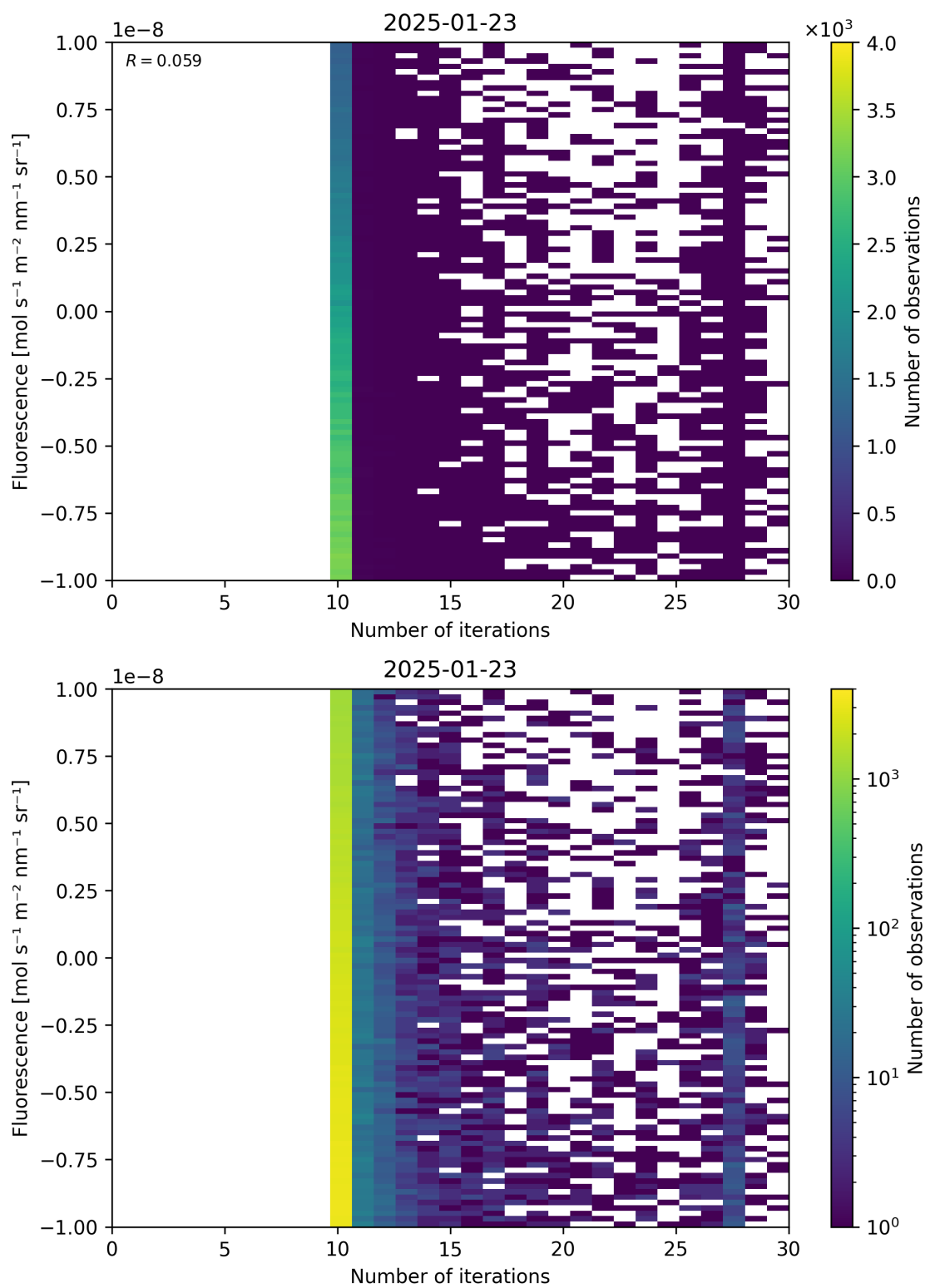
Figure 87: Scatter density plot of “Number of iterations” against “Fluorescence” for 2025-01-23 to 2025-01-24.
