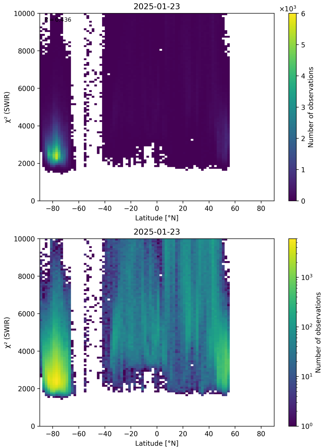
Figure 54: Scatter density plot of “Latitude” against “ \chi^2 (SWIR)” for 2025-01-23 to 2025-01-24.
