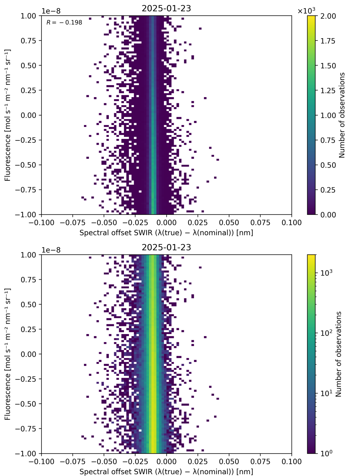
Figure 120: Scatter density plot of “Spectral offset SWIR ( \lambda_{\text{true}} - \lambda_{\text{nominal}} )” against “Fluorescence” for 2025-01-23 to 2025-01-24.
