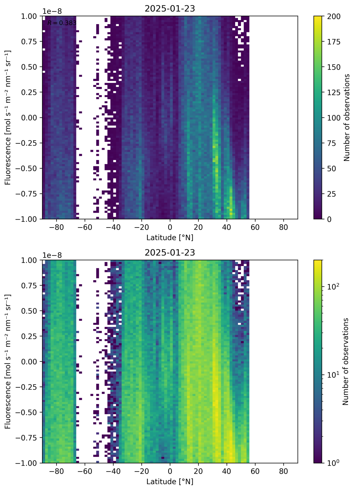
Figure 56: Scatter density plot of “Latitude” against “Fluorescence” for 2025-01-23 to 2025-01-24.
