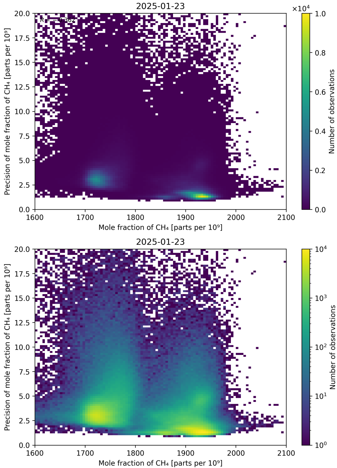
Figure 75: Scatter density plot of “Mole fraction of CH 4 ” against “Precision of mole fraction of CH 4 ” for 2025-01-23 to 2025-01-24.
