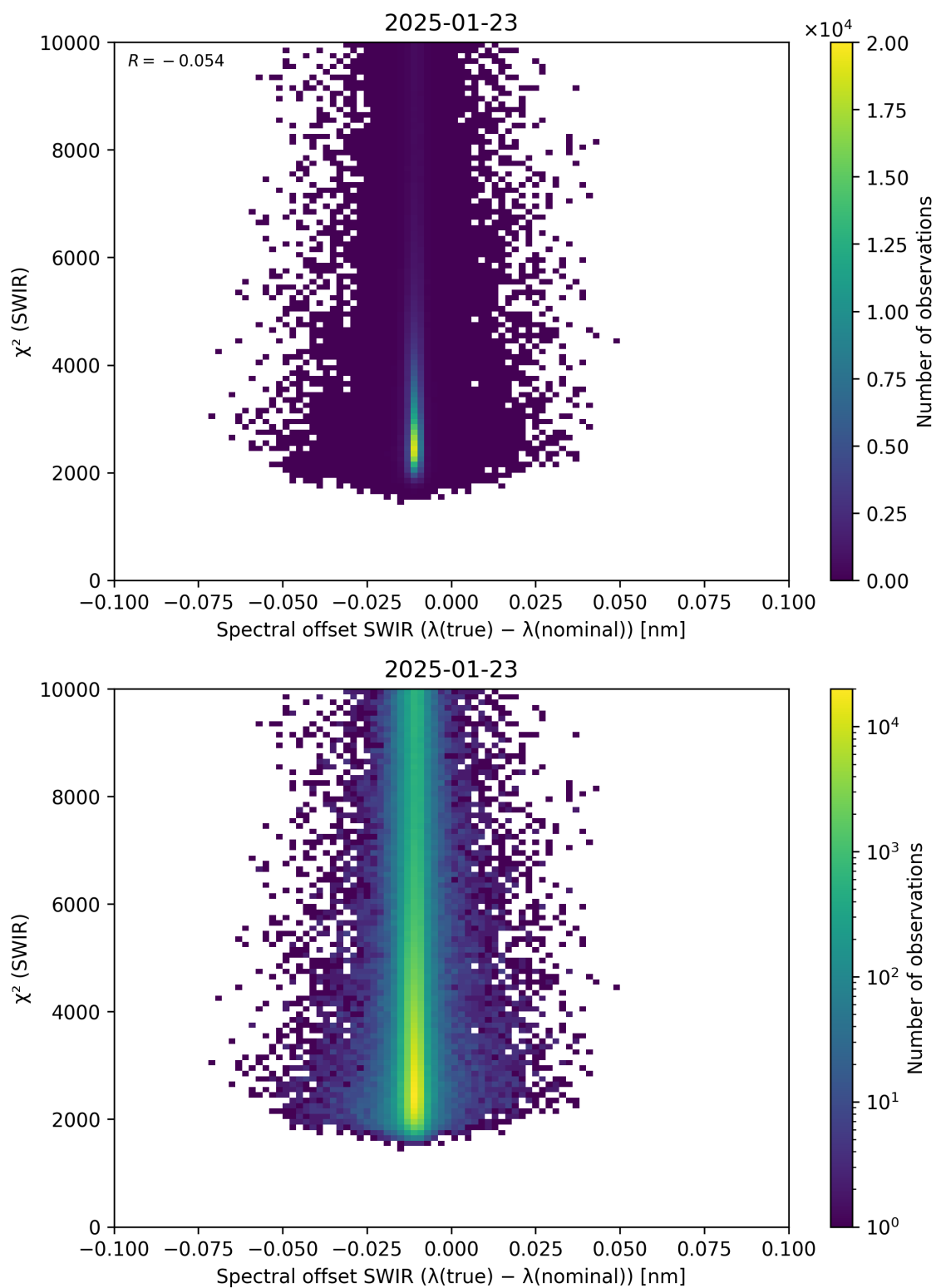
Figure 118: Scatter density plot of “Spectral offset SWIR ( \lambda_{\text{true}} - \lambda_{\text{nominal}} )” against “ \chi^2 (SWIR)” for 2025-01-23 to 2025-01-24.
