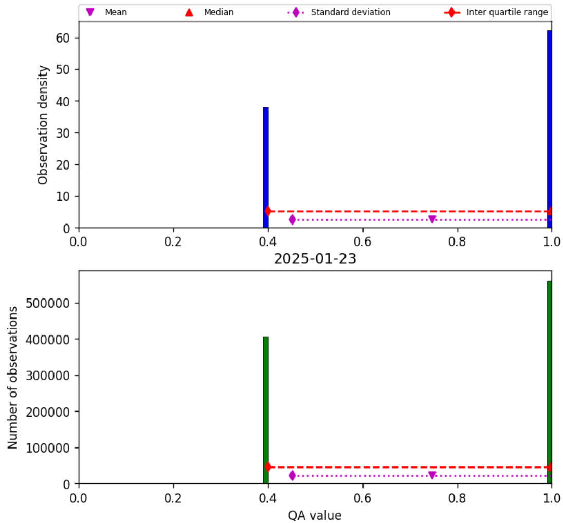
Figure 22: Histogram of “QA value” for 2025-01-23 to 2025-01-24
