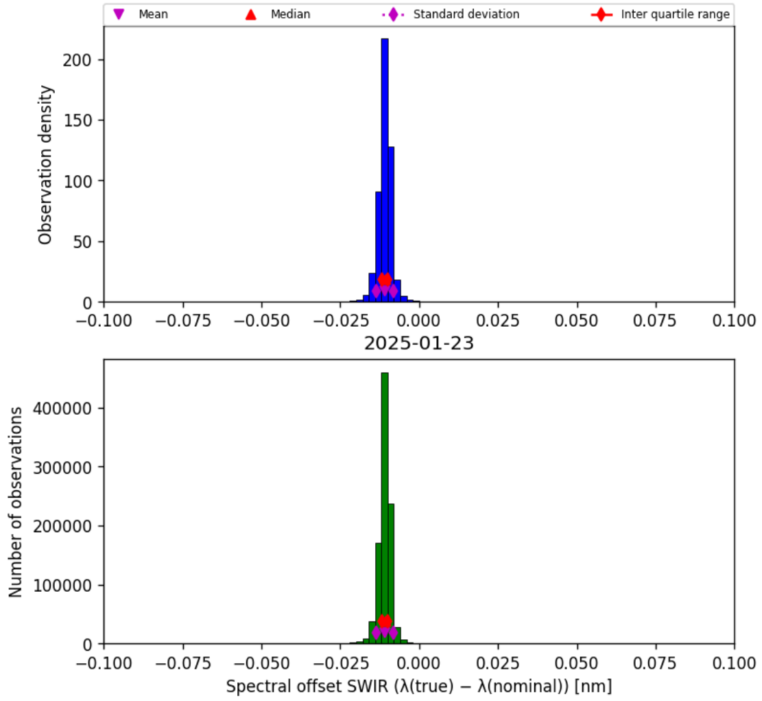
Figure 27: Histogram of “Spectral offset SWIR ( \lambda_{\text{true}} - \lambda_{\text{nominal}} )” for 2025-01-23 to 2025-01-24
