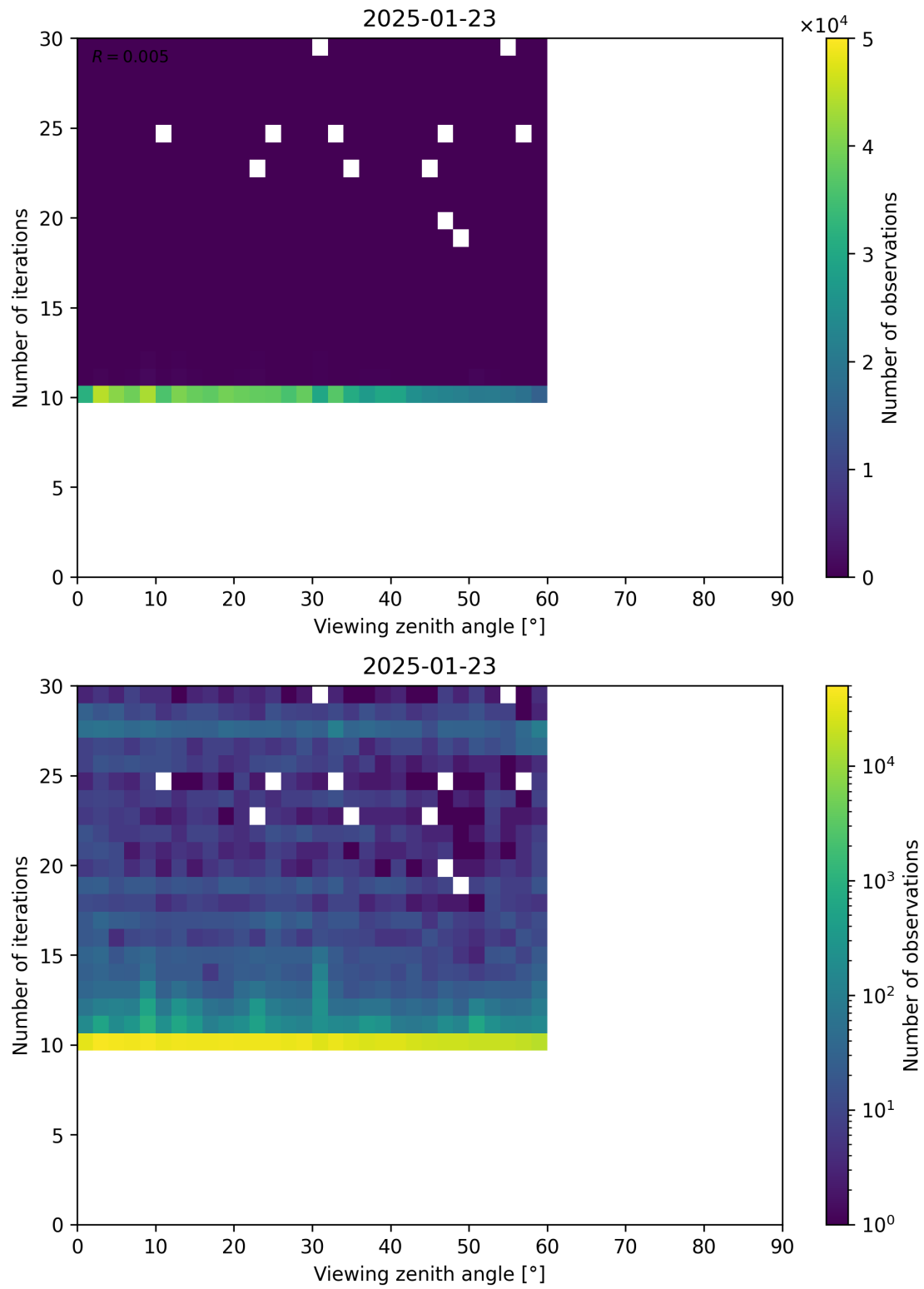
Figure 113: Scatter density plot of “Viewing zenith angle” against “Number of iterations” for 2025-01-23 to 2025-01-24.
