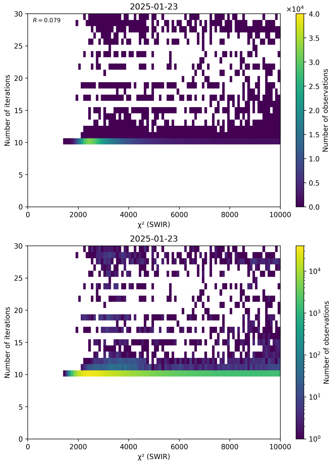
Figure 50: Scatter density plot of “ \chi^2 (SWIR)” against “Number of iterations” for 2025-01-23 to 2025-01-24.
