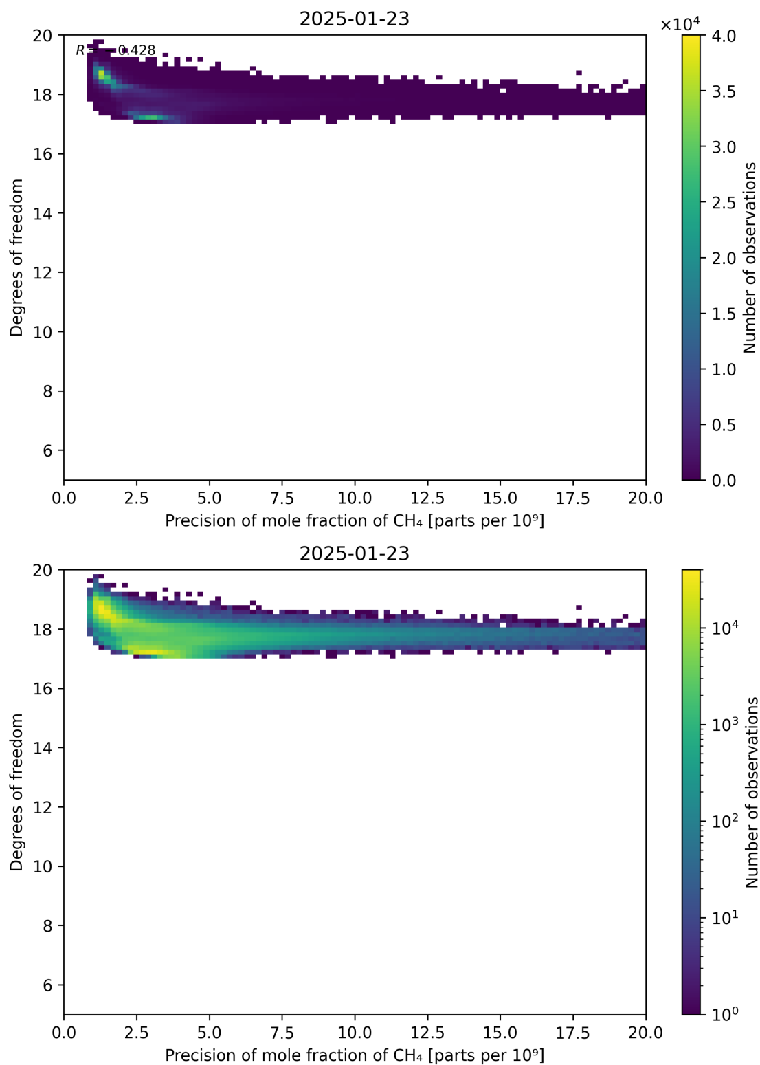
Figure 80: Scatter density plot of “Precision of mole fraction of CH 4 ” against “Degrees of freedom” for 2025-01-23 to 2025-01-24.
