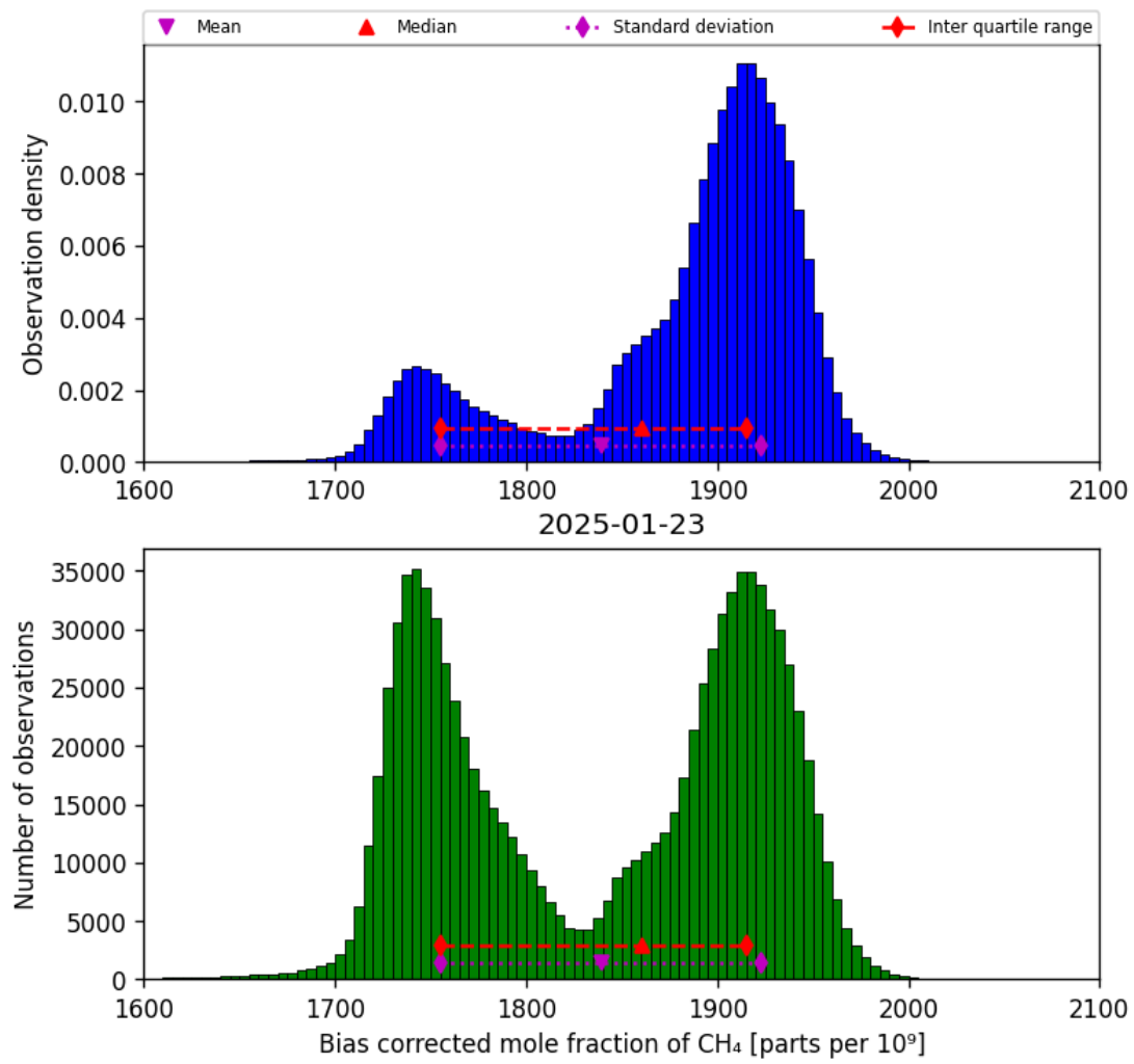
Figure 25: Histogram of “Bias corrected mole fraction of CH 4 ” for 2025-01-23 to 2025-01-24
