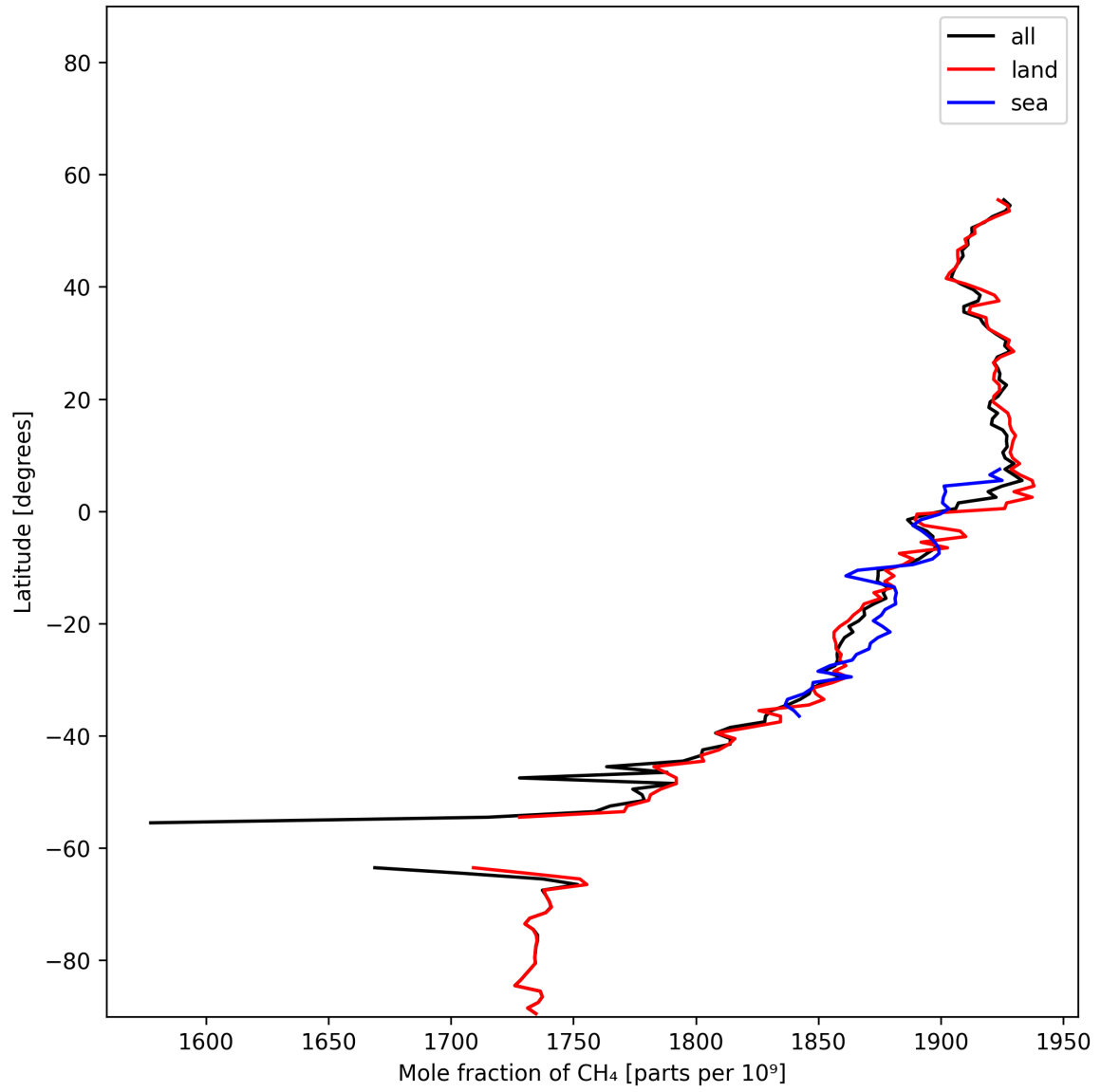
Figure 12: Zonal average of “Mole fraction of \text{CH}_4 ” for 2025-01-23 to 2025-01-24.
