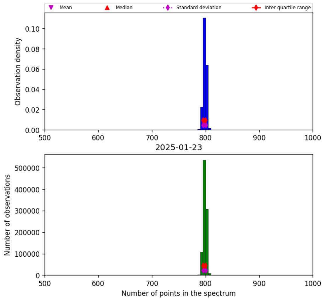
Figure 26: Histogram of “Number of points in the spectrum” for 2025-01-23 to 2025-01-24
