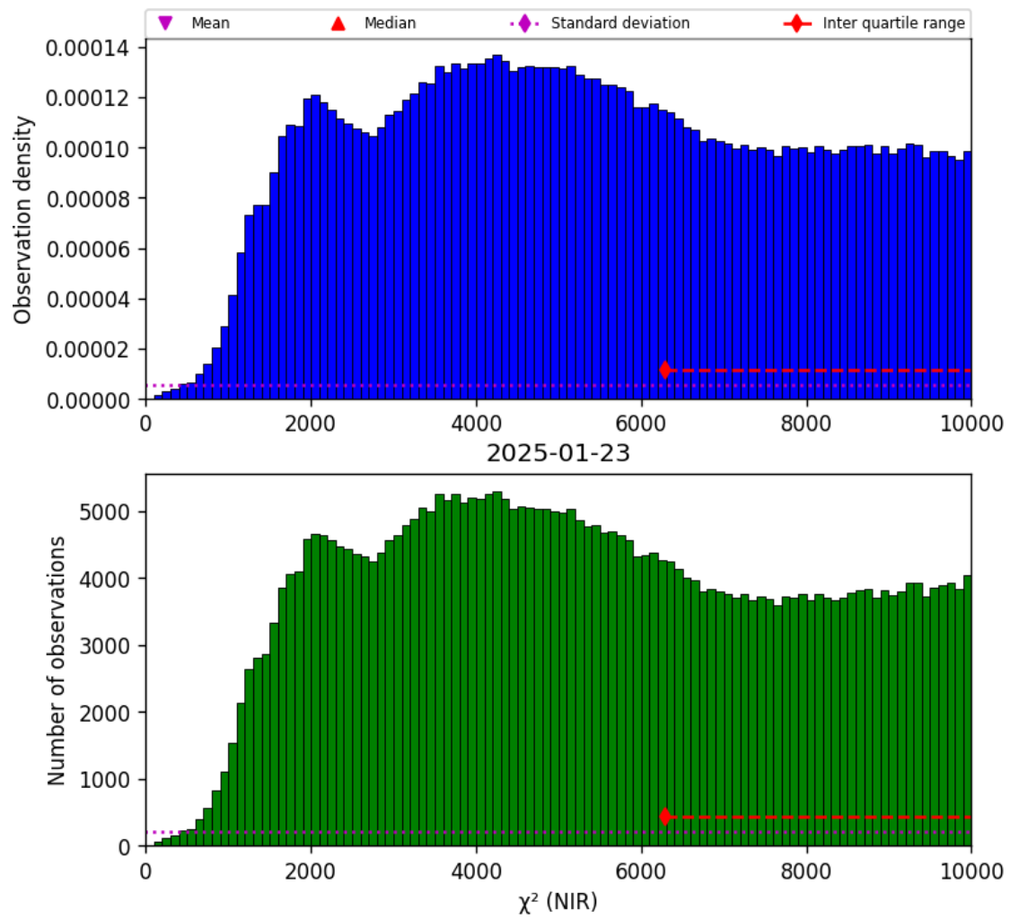
Figure 29: Histogram of “ \chi^2 (NIR)” for 2025-01-23 to 2025-01-24
