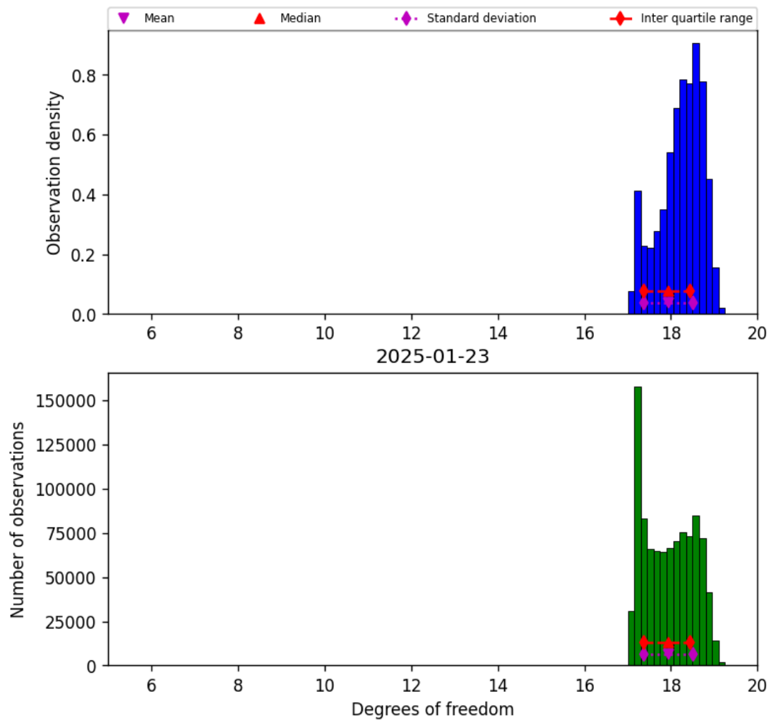
Figure 30: Histogram of “Degrees of freedom” for 2025-01-23 to 2025-01-24
