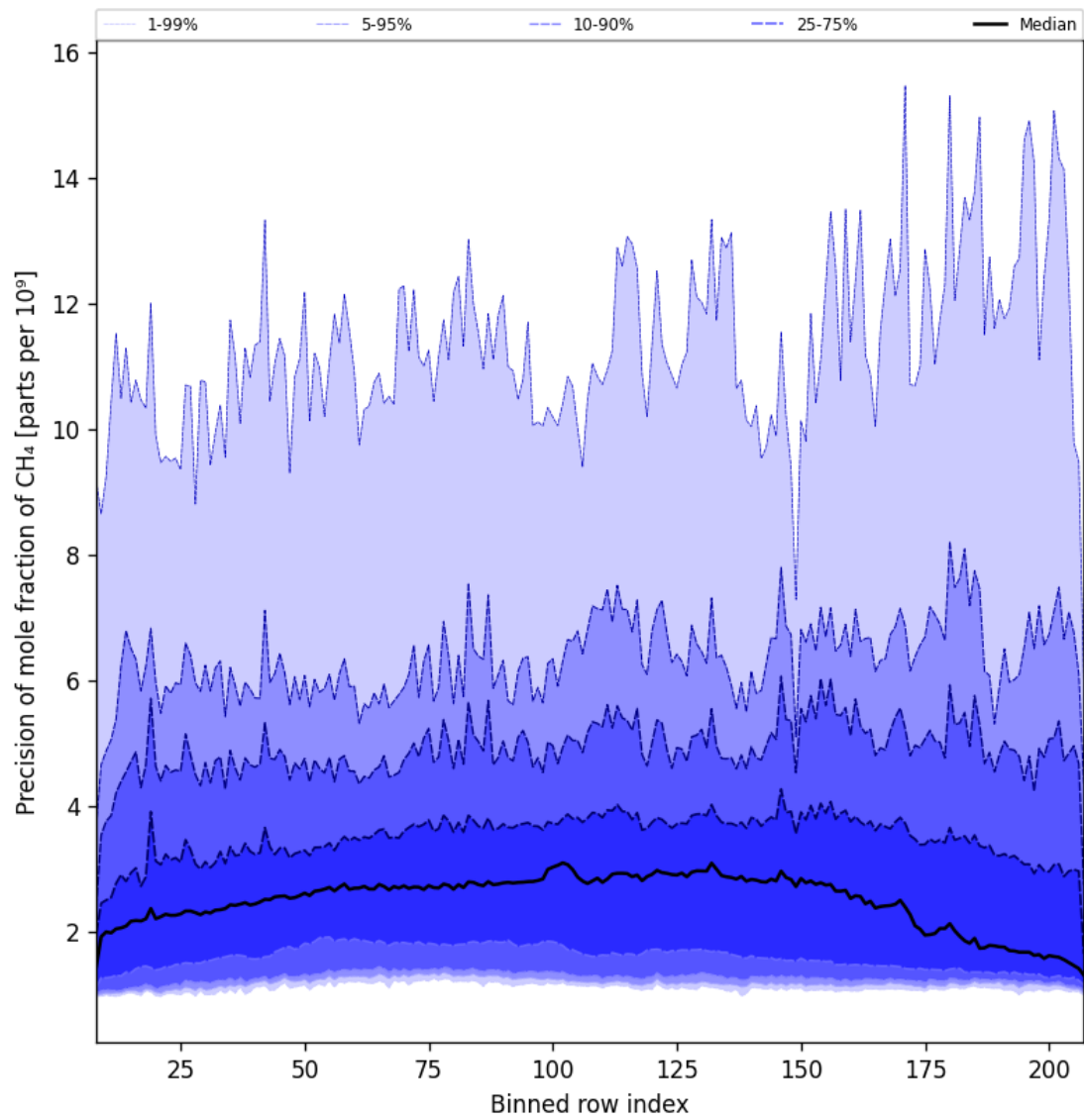
Figure 35: Along track statistics of “Precision of mole fraction of CH 4 ” for 2025-01-23 to 2025-01-24
