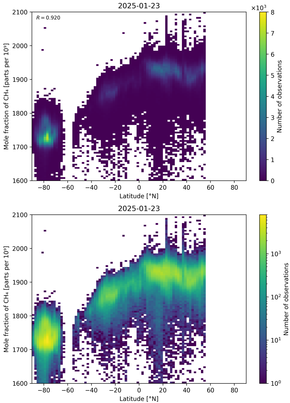
Figure 57: Scatter density plot of “Latitude” against “Mole fraction of CH 4 ” for 2025-01-23 to 2025-01-24.
