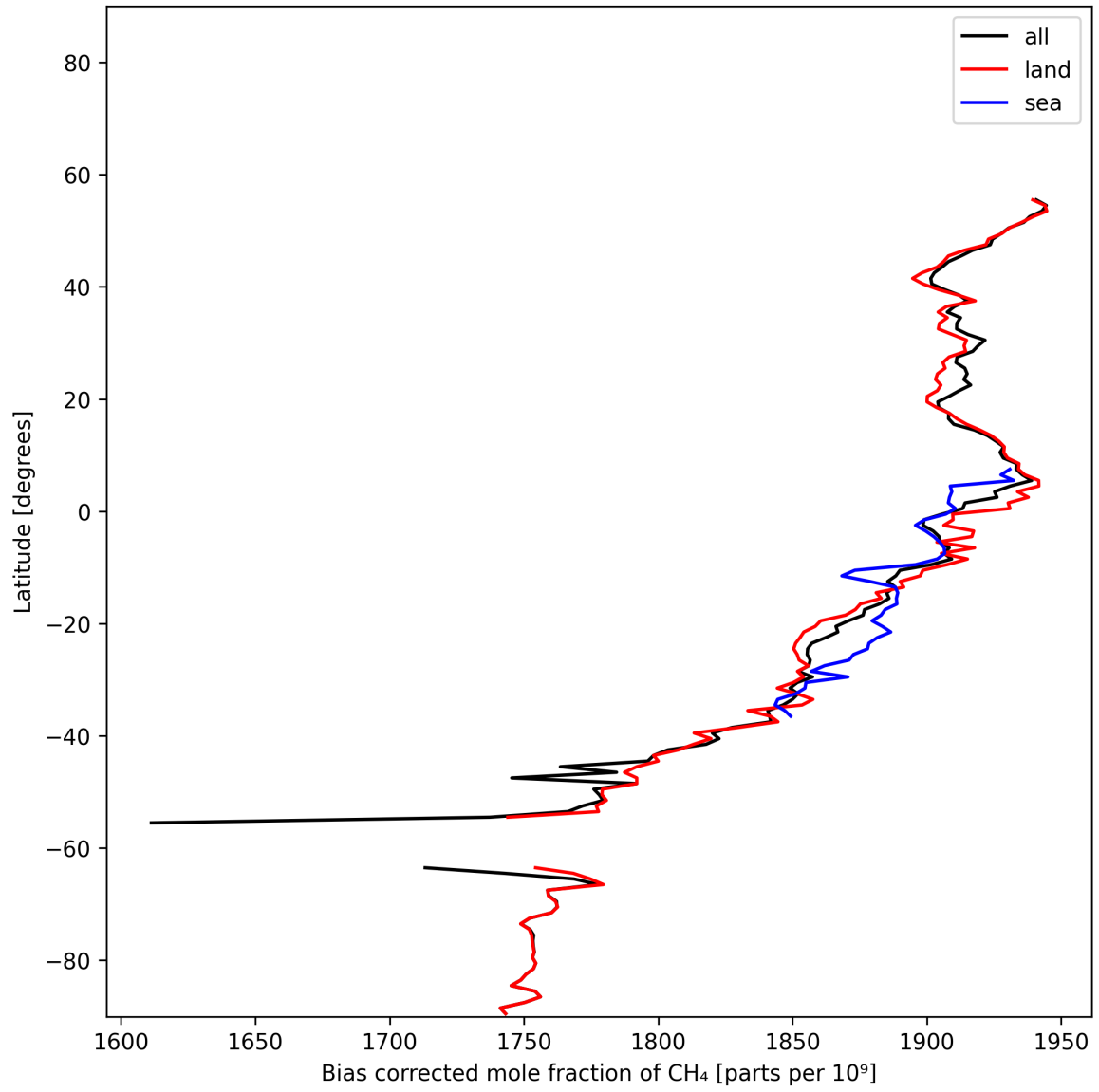
Figure 14: Zonal average of “Bias corrected mole fraction of CH 4 ” for 2025-01-23 to 2025-01-24.
