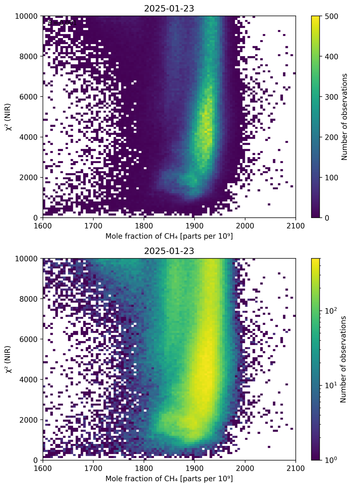
Figure 70: Scatter density plot of “Mole fraction of CH 4 ” against “ \chi^2 (NIR)” for 2025-01-23 to 2025-01-24.
