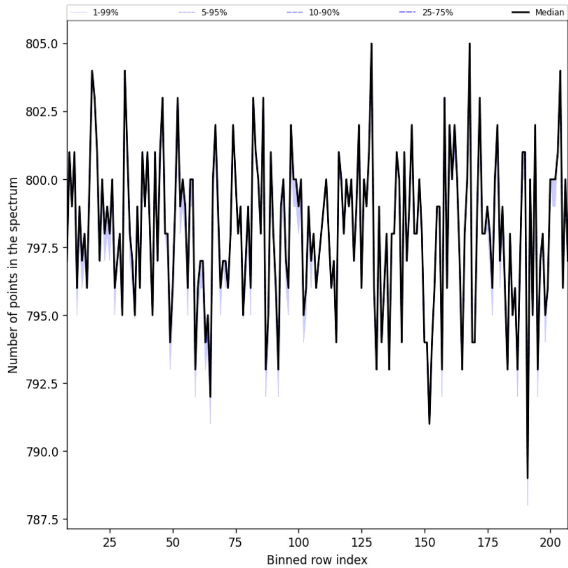
Figure 37: Along track statistics of “Number of points in the spectrum” for 2025-01-23 to 2025-01-24
