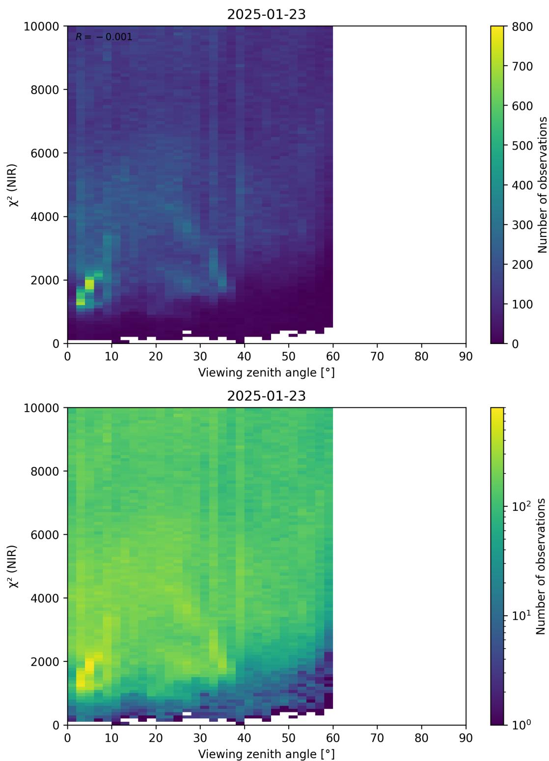
Figure 105: Scatter density plot of “Viewing zenith angle” against “ \chi^2 (NIR)” for 2025-01-23 to 2025-01-24.
