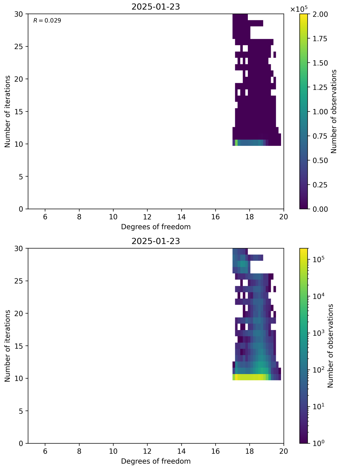
Figure 52: Scatter density plot of “Degrees of freedom” against “Number of iterations” for 2025-01-23 to 2025-01-24.
