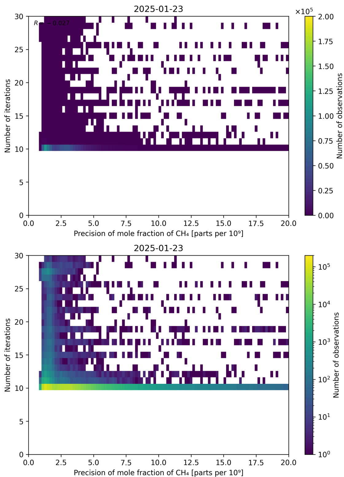
Figure 83: Scatter density plot of “Precision of mole fraction of CH 4 ” against “Number of iterations” for 2025-01-23 to 2025-01-24.
