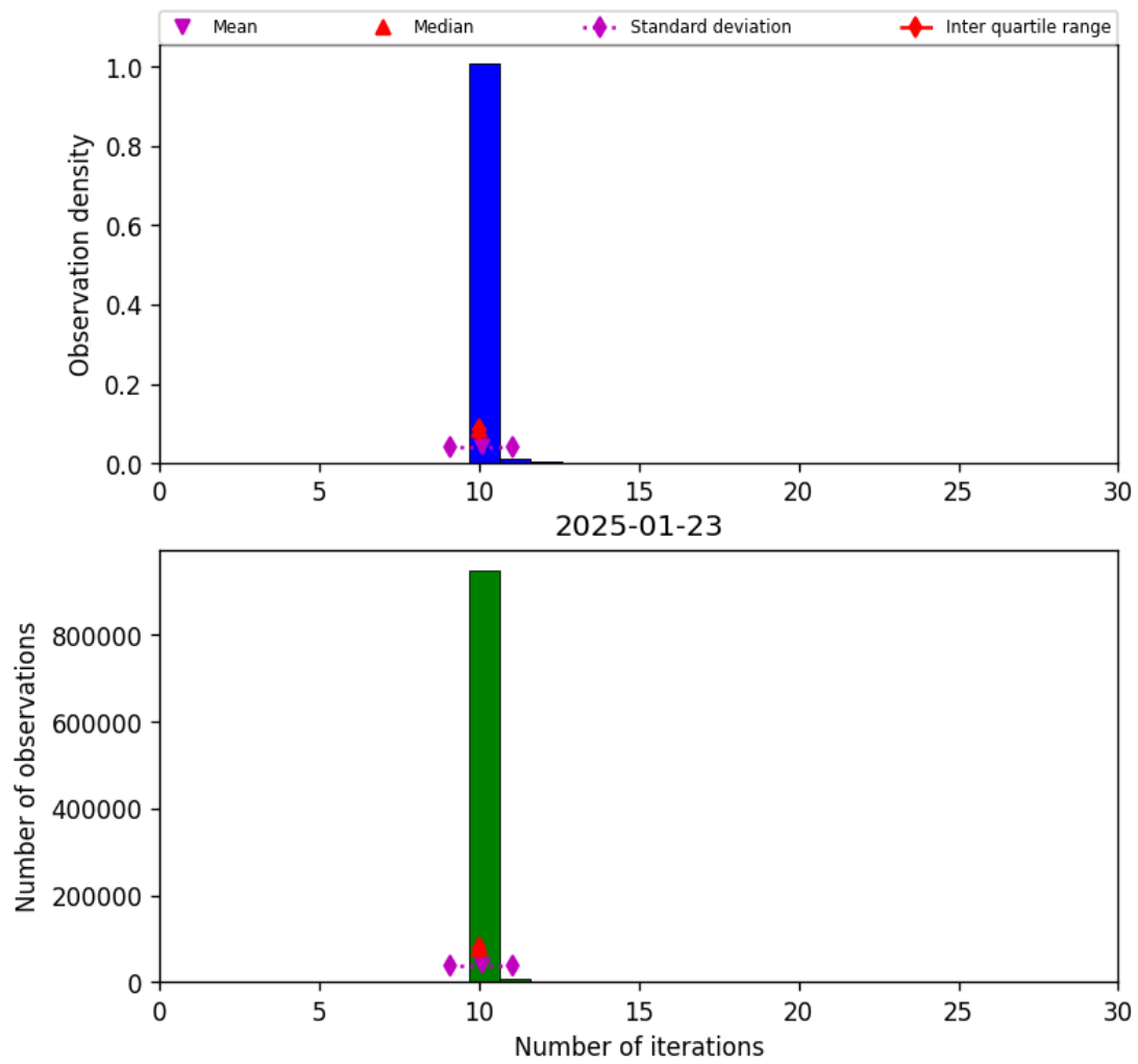
Figure 31: Histogram of “Number of iterations” for 2025-01-23 to 2025-01-24
