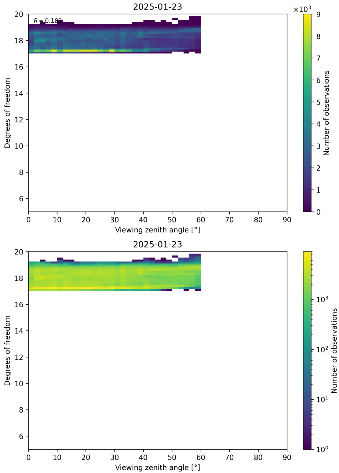
Figure 107: Scatter density plot of “Viewing zenith angle” against “Degrees of freedom” for 2025-01-23 to 2025-01-24.
