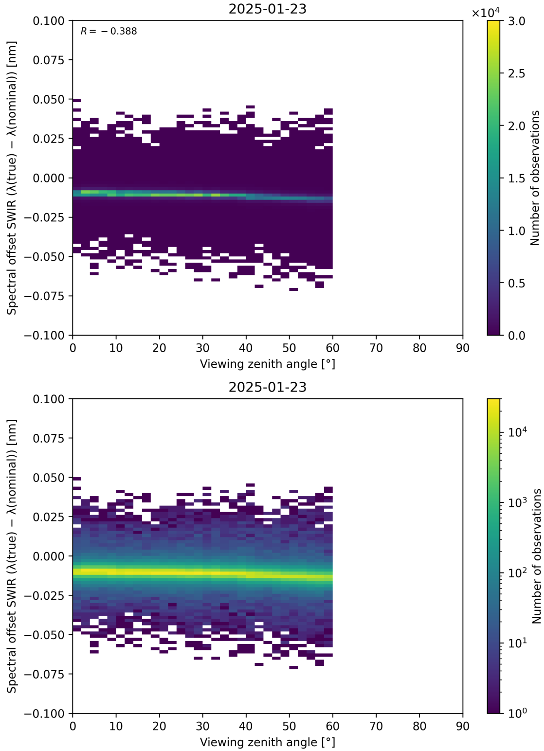
Figure 116: Scatter density plot of “Viewing zenith angle” against “Spectral offset SWIR ( \lambda_{\text{true}} - \lambda_{\text{nominal}} )” for 2025-01-23 to 2025-01-24.
