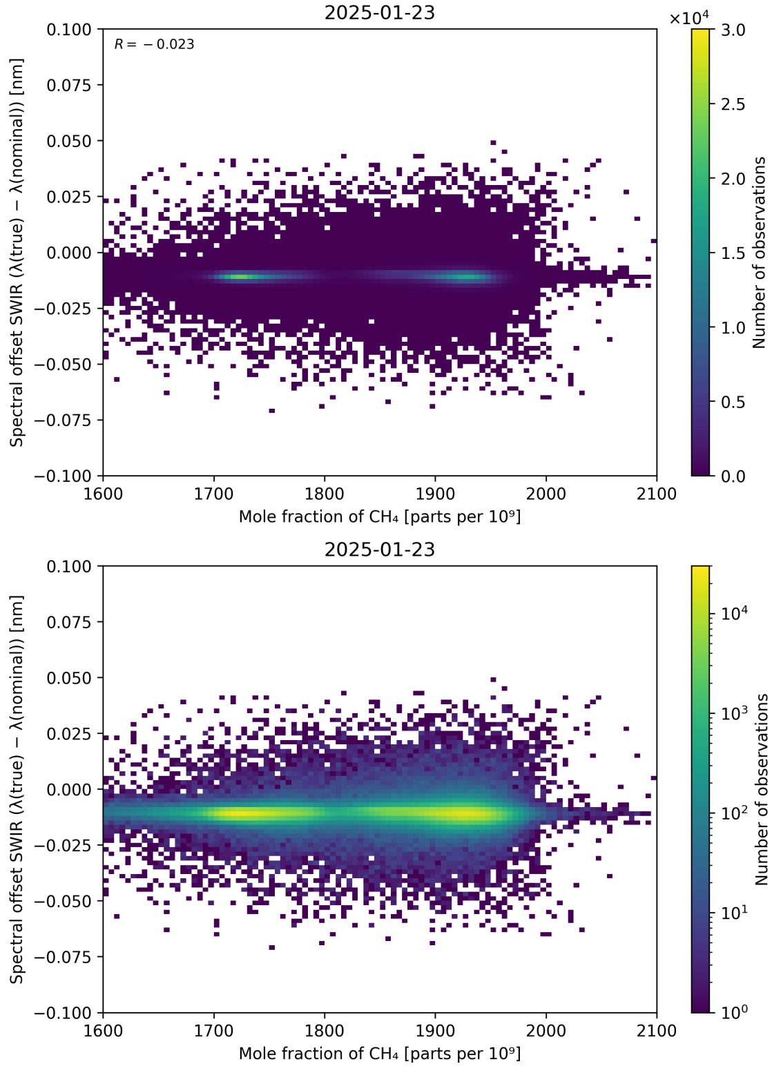
Figure 86: Scatter density plot of “Mole fraction of CH 4 ” against “Spectral offset SWIR ( \lambda_{\text{true}} - \lambda_{\text{nominal}} )” for 2025-01-23 to 2025-01-24.
