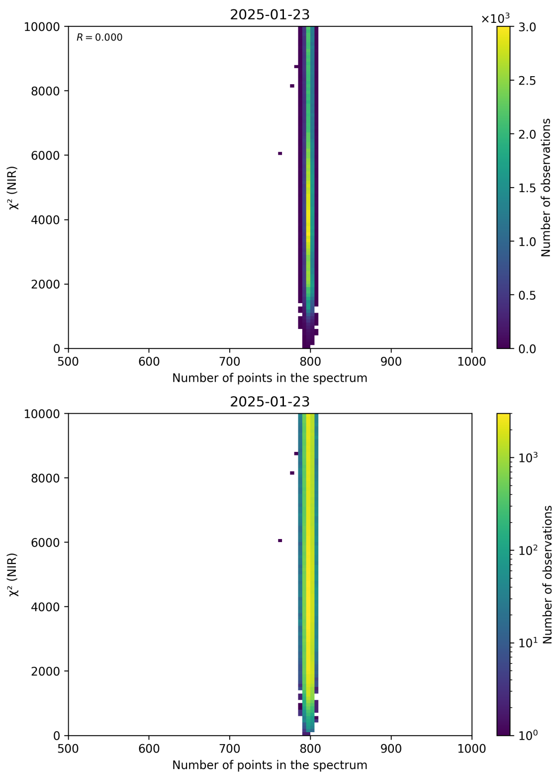
Figure 88: Scatter density plot of “Number of points in the spectrum” against “ \chi^2 (NIR)” for 2025-01-23 to 2025-01-24.
