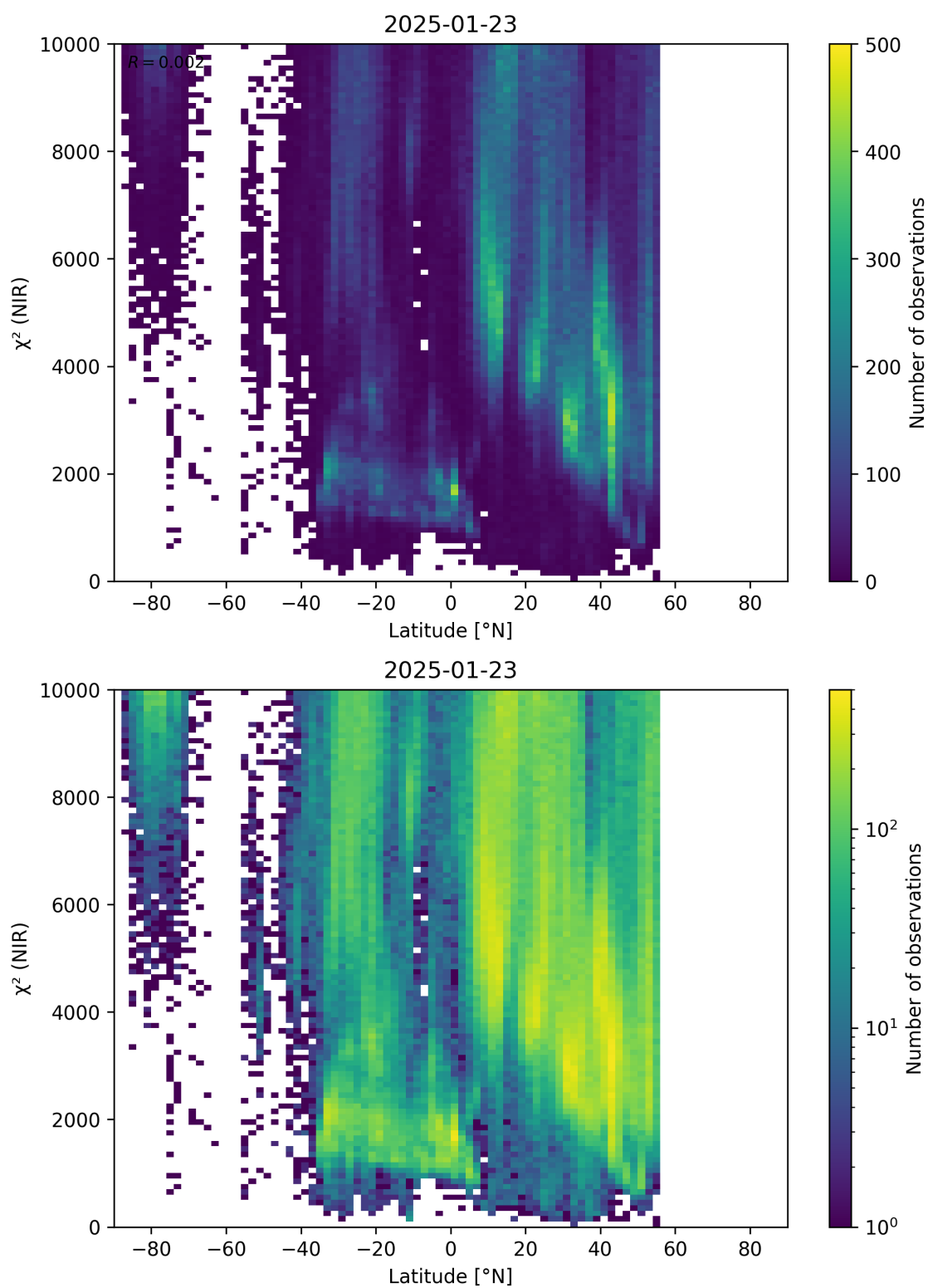
Figure 53: Scatter density plot of “Latitude” against “ \chi^2 (NIR)” for 2025-01-23 to 2025-01-24.
