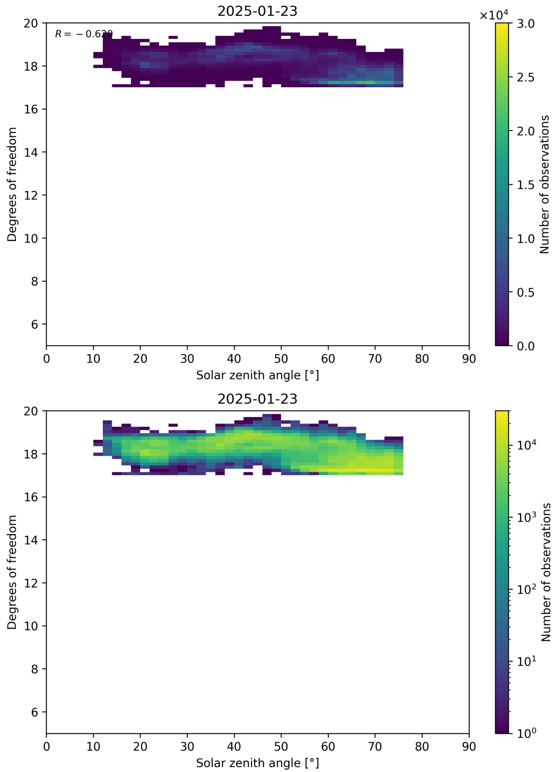
Figure 96: Scatter density plot of “Solar zenith angle” against “Degrees of freedom” for 2025-01-23 to 2025-01-24.
