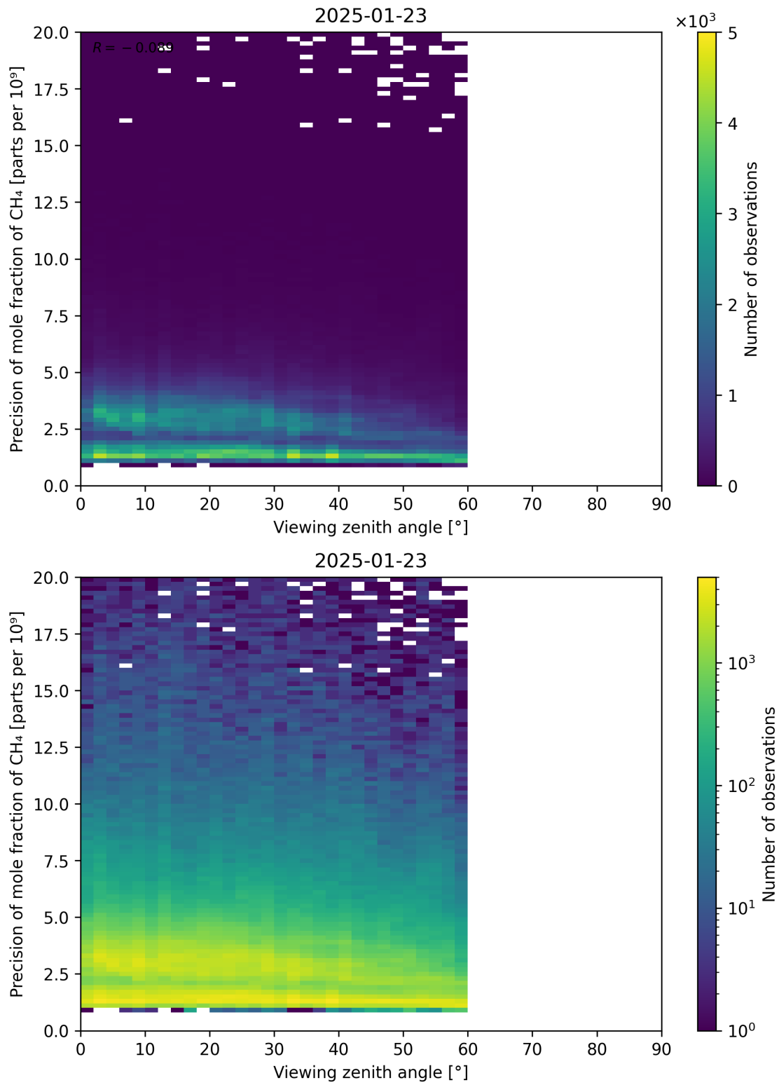
Figure 112: Scatter density plot of “Viewing zenith angle” against “Precision of mole fraction of CH 4 ” for 2025-01-23 to 2025-01-24.
