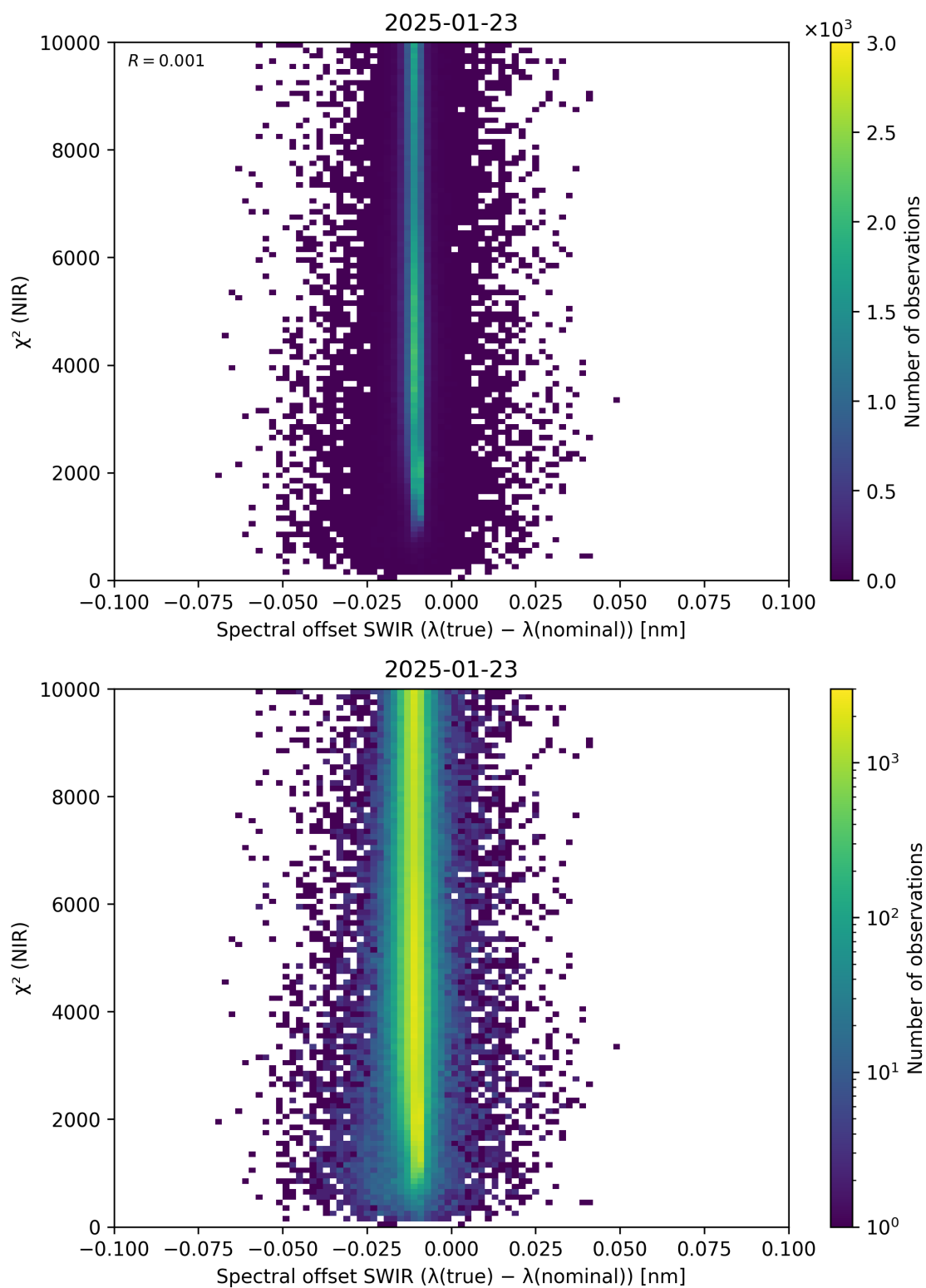
Figure 117: Scatter density plot of “Spectral offset SWIR ( \lambda_{\text{true}} - \lambda_{\text{nominal}} )” against “ \chi^2 (NIR)” for 2025-01-23 to 2025-01-24.
