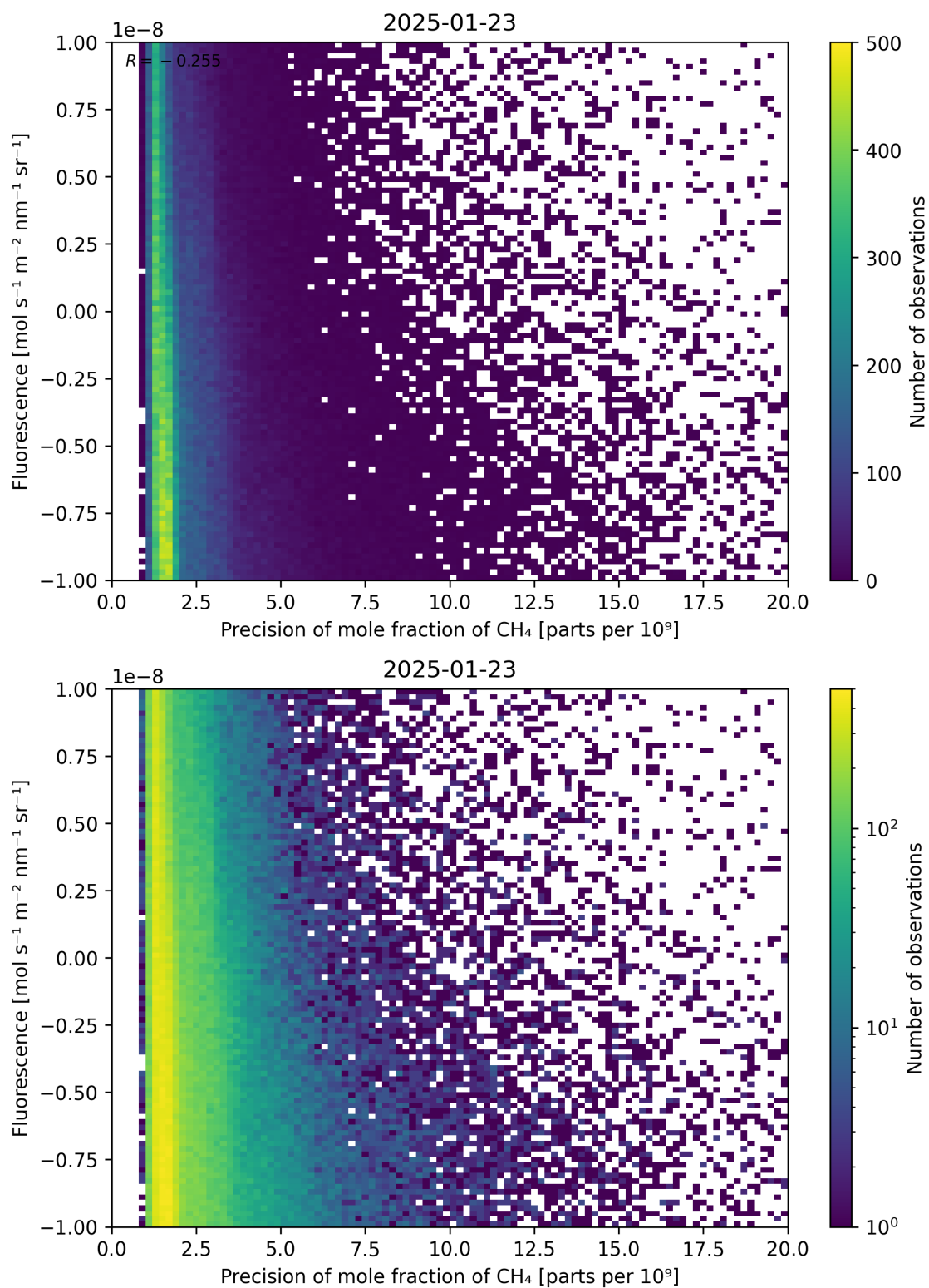
Figure 81: Scatter density plot of “Precision of mole fraction of CH 4 ” against “Fluorescence” for 2025-01-23 to 2025-01-24.
