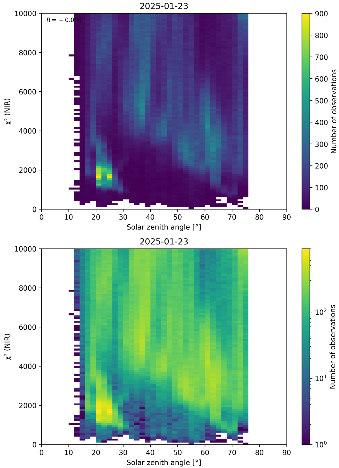
Figure 94: Scatter density plot of “Solar zenith angle” against “ \chi^2 (NIR)” for 2025-01-23 to 2025-01-24.
