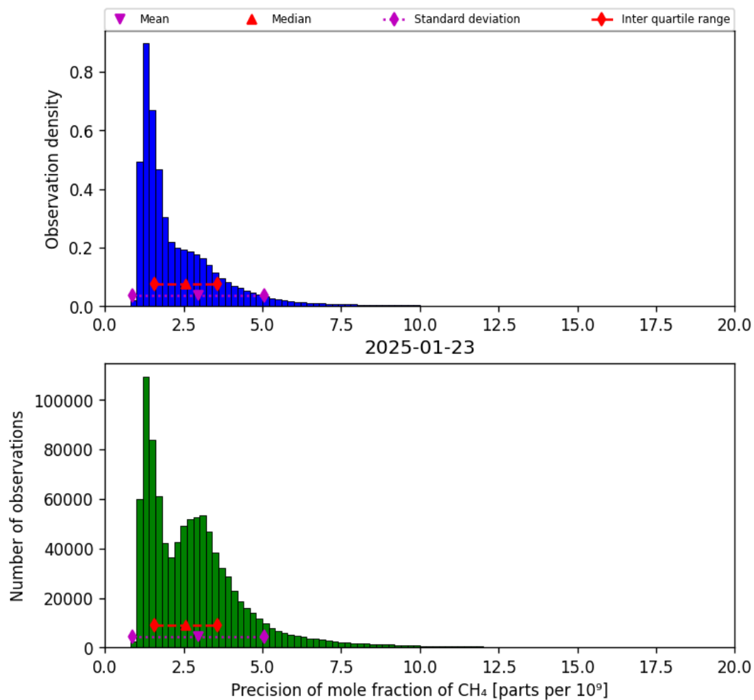
Figure 24: Histogram of “Precision of mole fraction of CH 4 ” for 2025-01-23 to 2025-01-24
