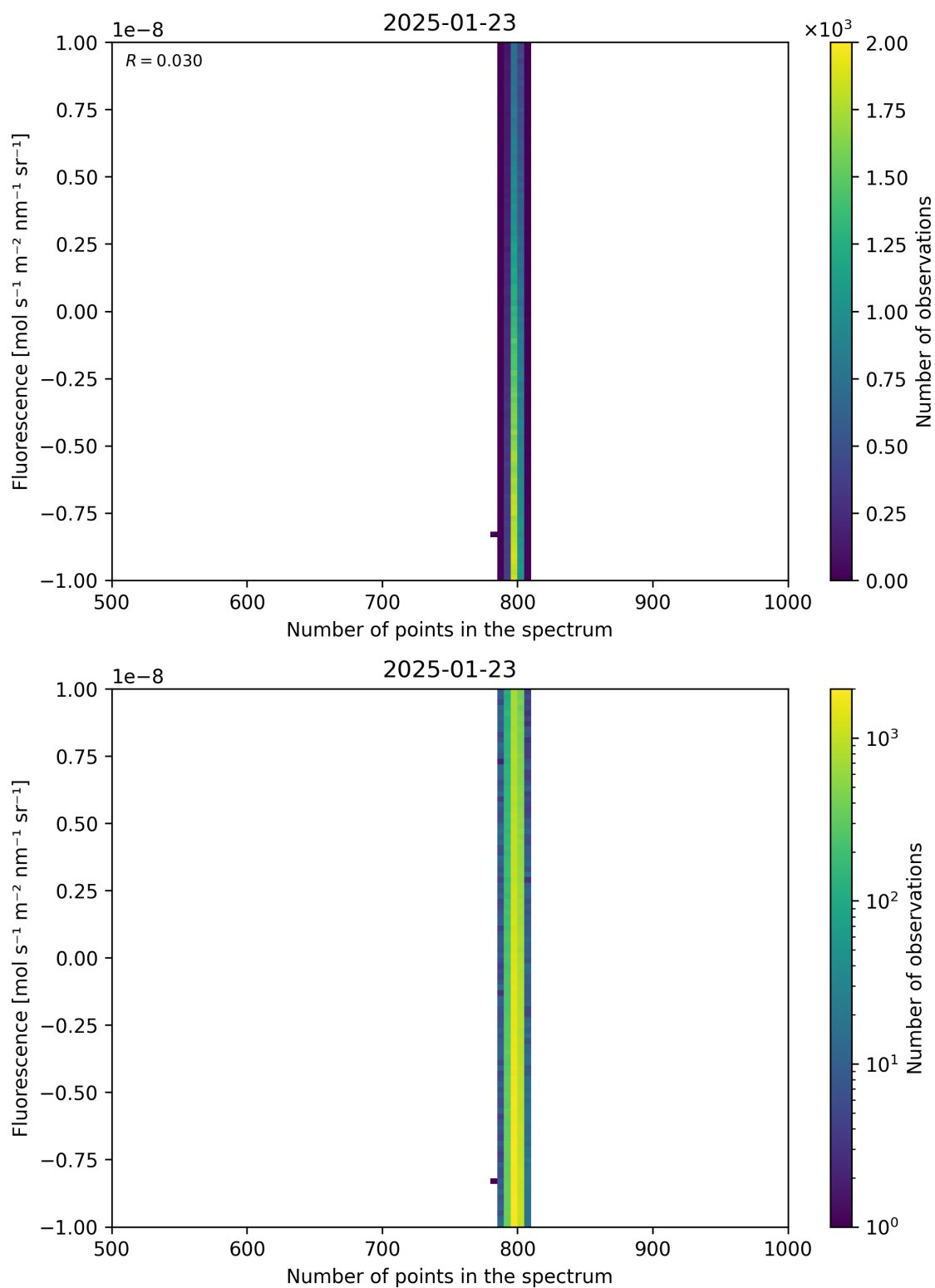
Figure 91: Scatter density plot of “Number of points in the spectrum” against “Fluorescence” for 2025-01-23 to 2025-01-24.
