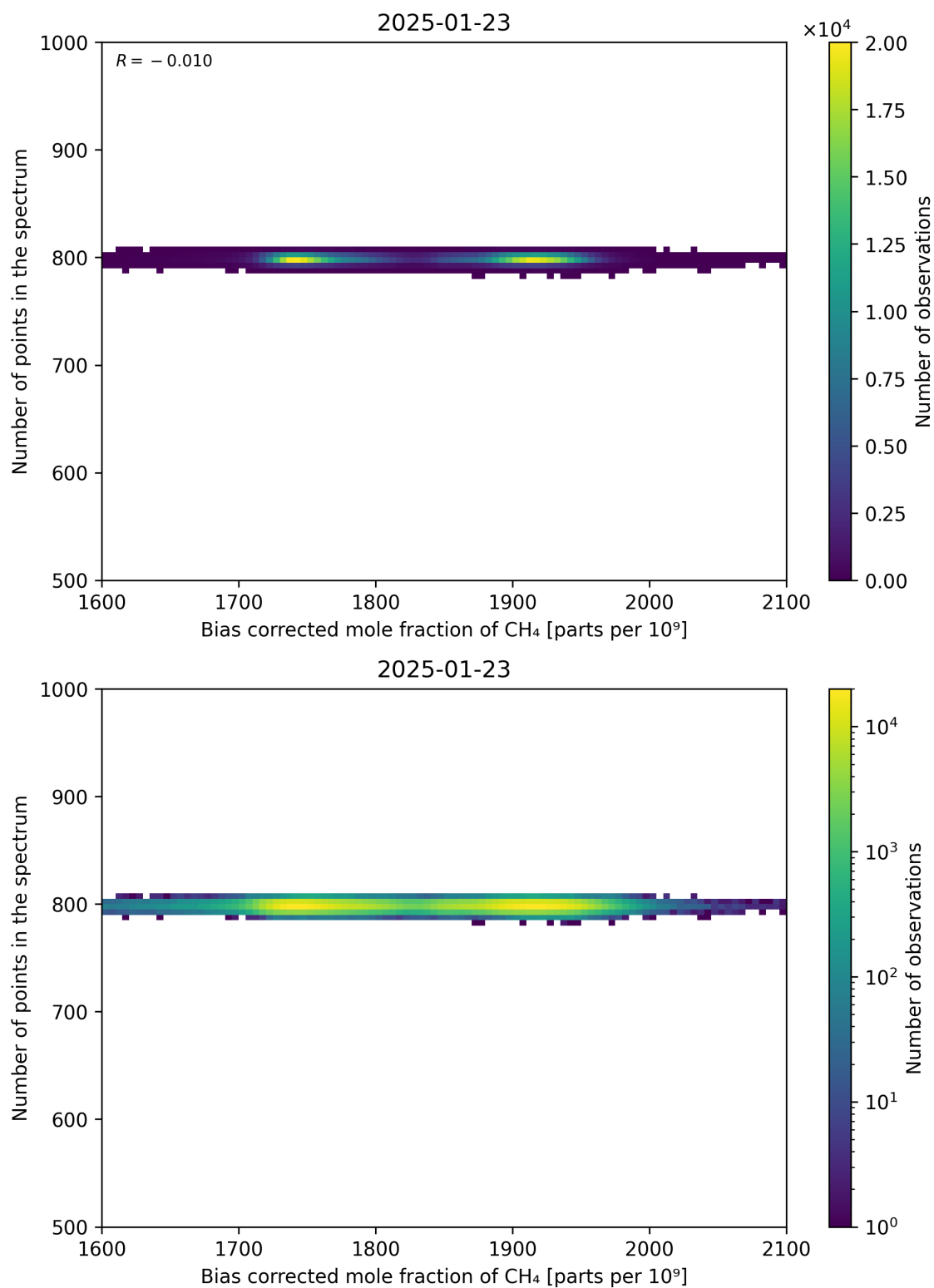
Figure 68: Scatter density plot of “Bias corrected mole fraction of CH 4 ” against “Number of points in the spectrum” for 2025-01-23 to 2025-01-24.
