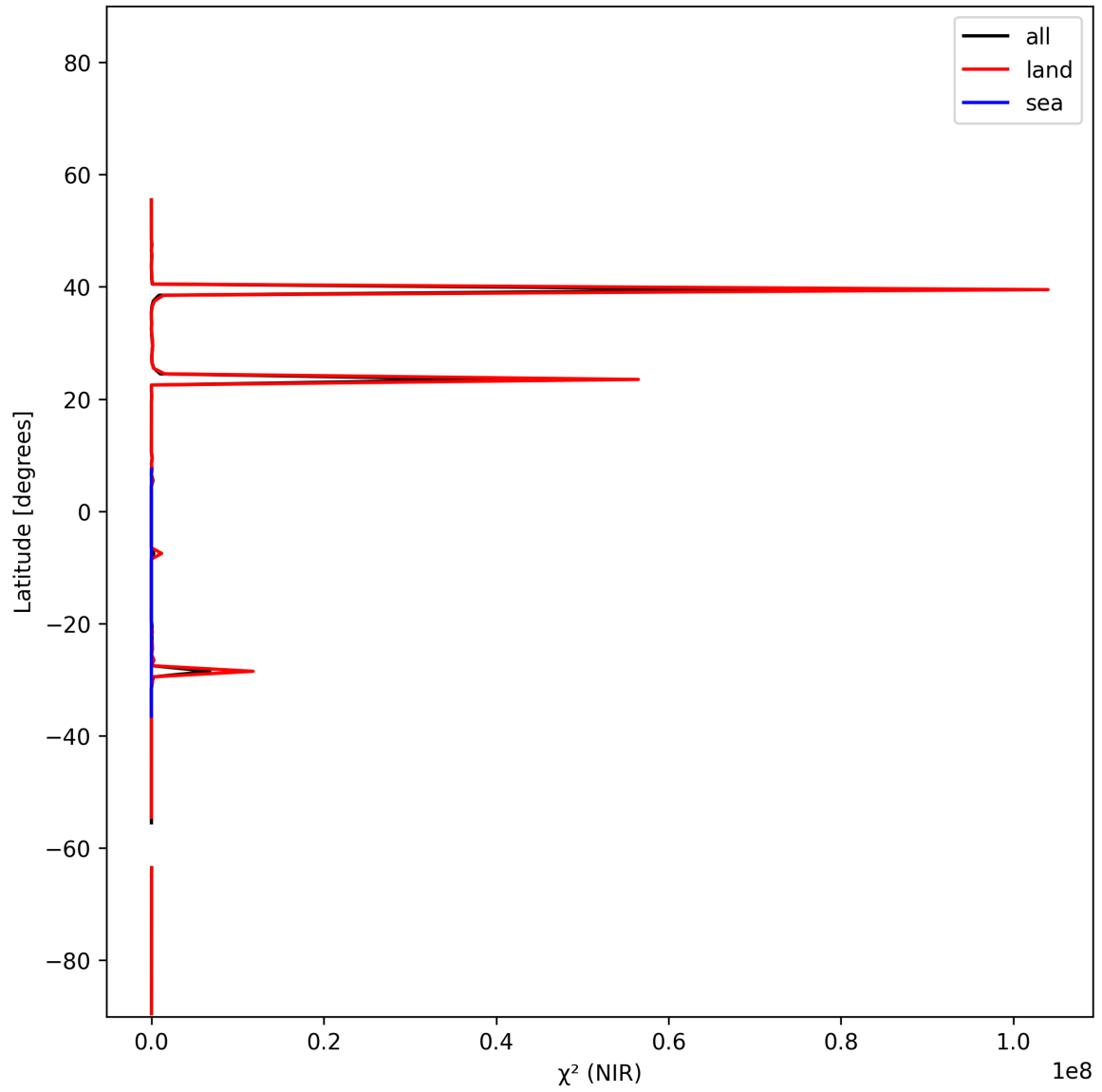
Figure 18: Zonal average of “ \chi^2 (NIR)” for 2025-01-23 to 2025-01-24.
