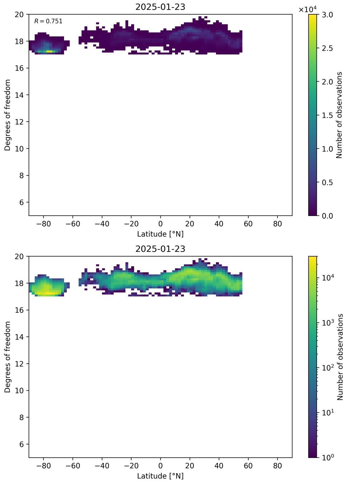
Figure 55: Scatter density plot of “Latitude” against “Degrees of freedom” for 2025-01-23 to 2025-01-24.
