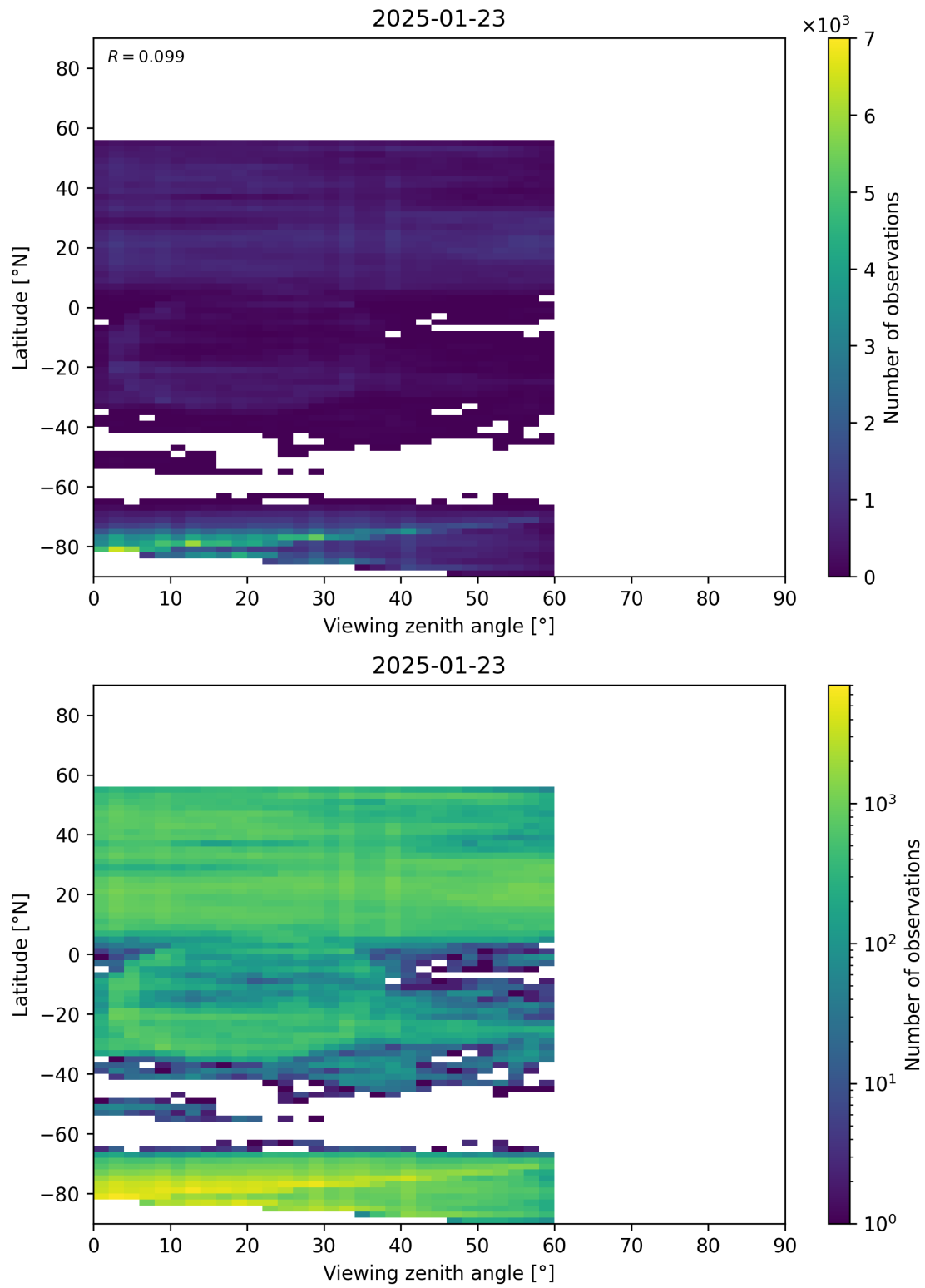
Figure 109: Scatter density plot of “Viewing zenith angle” against “Latitude” for 2025-01-23 to 2025-01-24.
