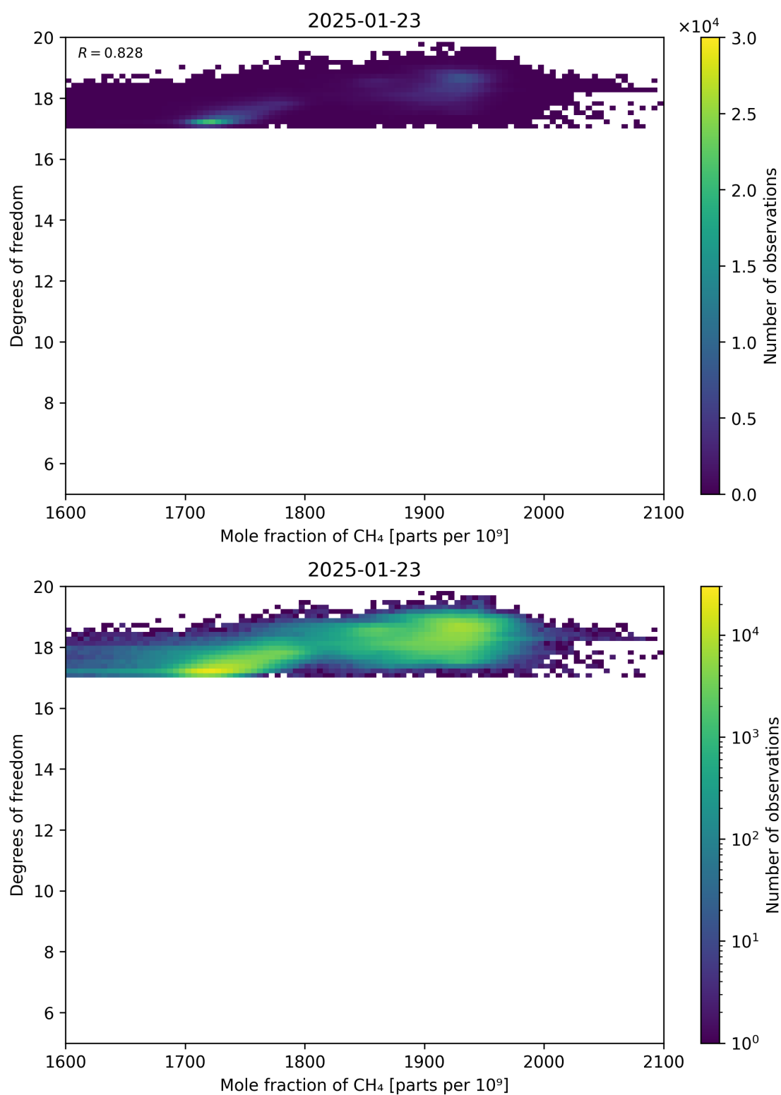
Figure 72: Scatter density plot of “Mole fraction of CH 4 ” against “Degrees of freedom” for 2025-01-23 to 2025-01-24.
