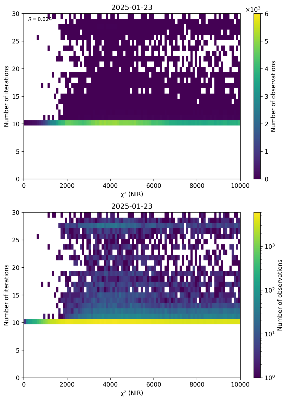
Figure 46: Scatter density plot of “ \chi^2 (NIR)” against “Number of iterations” for 2025-01-23 to 2025-01-24.
