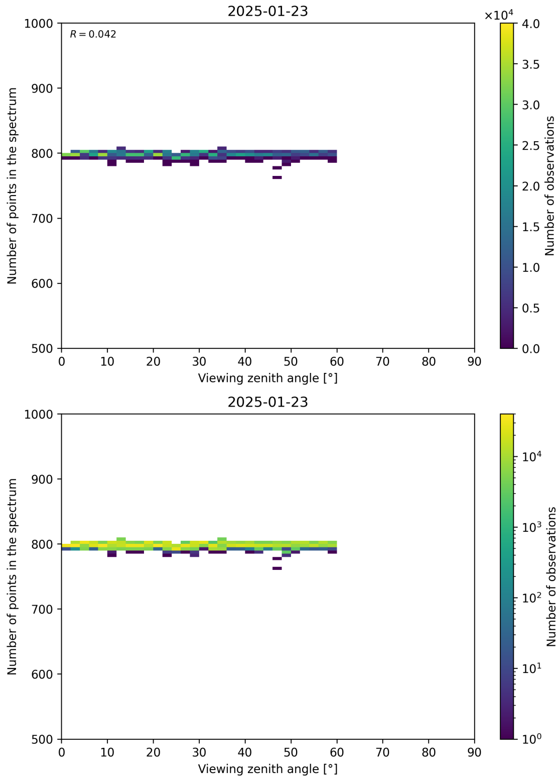
Figure 114: Scatter density plot of “Viewing zenith angle” against “Number of points in the spectrum” for 2025-01-23 to 2025-01-24.
