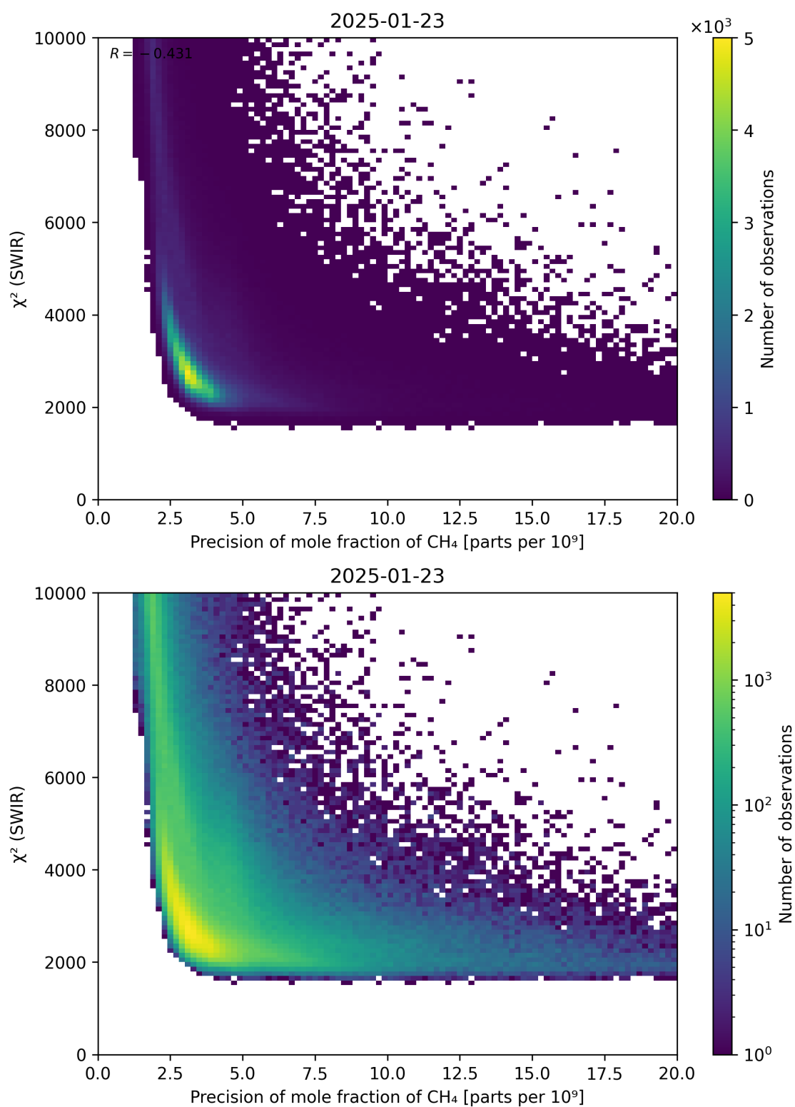
Figure 79: Scatter density plot of “Precision of mole fraction of \text{CH}_4 ” against “ \chi^2 (SWIR)” for 2025-01-23 to 2025-01-24.
