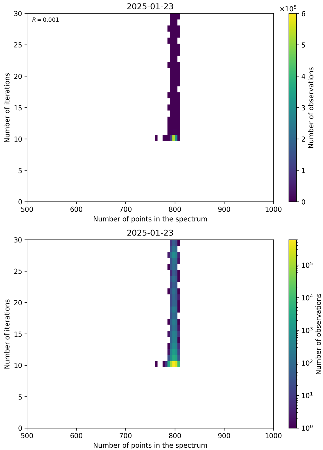
Figure 92: Scatter density plot of “Number of points in the spectrum” against “Number of iterations” for 2025-01-23 to 2025-01-24.
