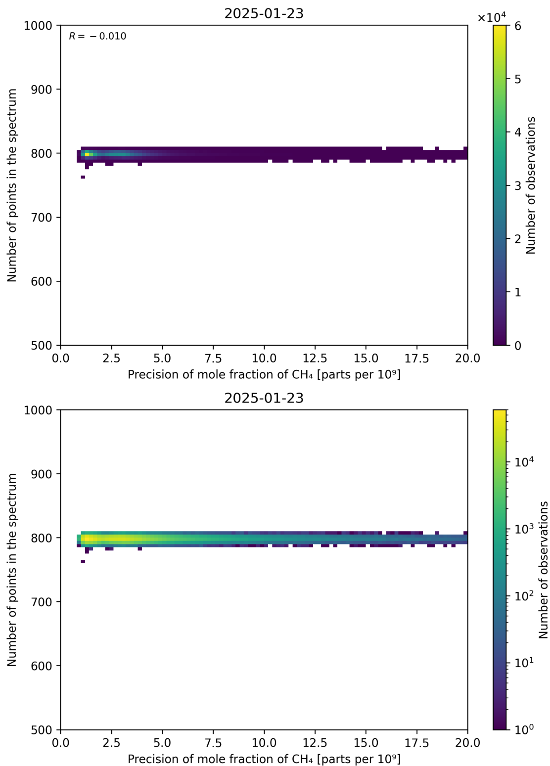
Figure 84: Scatter density plot of “Precision of mole fraction of CH 4 ” against “Number of points in the spectrum” for 2025-01-23 to 2025-01-24.
