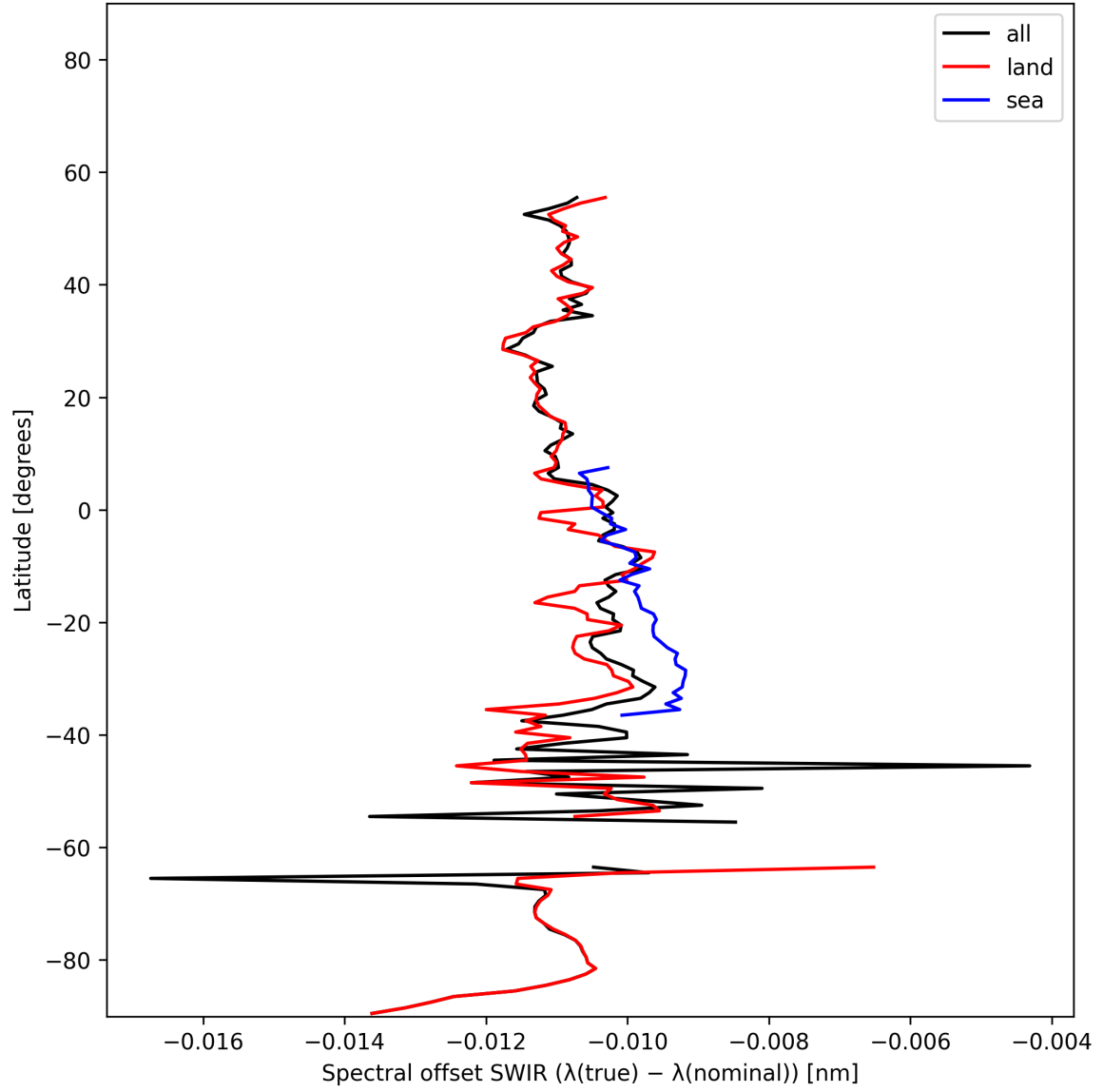
Figure 16: Zonal average of “Spectral offset SWIR ( \lambda_{\text{true}} - \lambda_{\text{nominal}} )” for 2025-01-23 to 2025-01-24.
