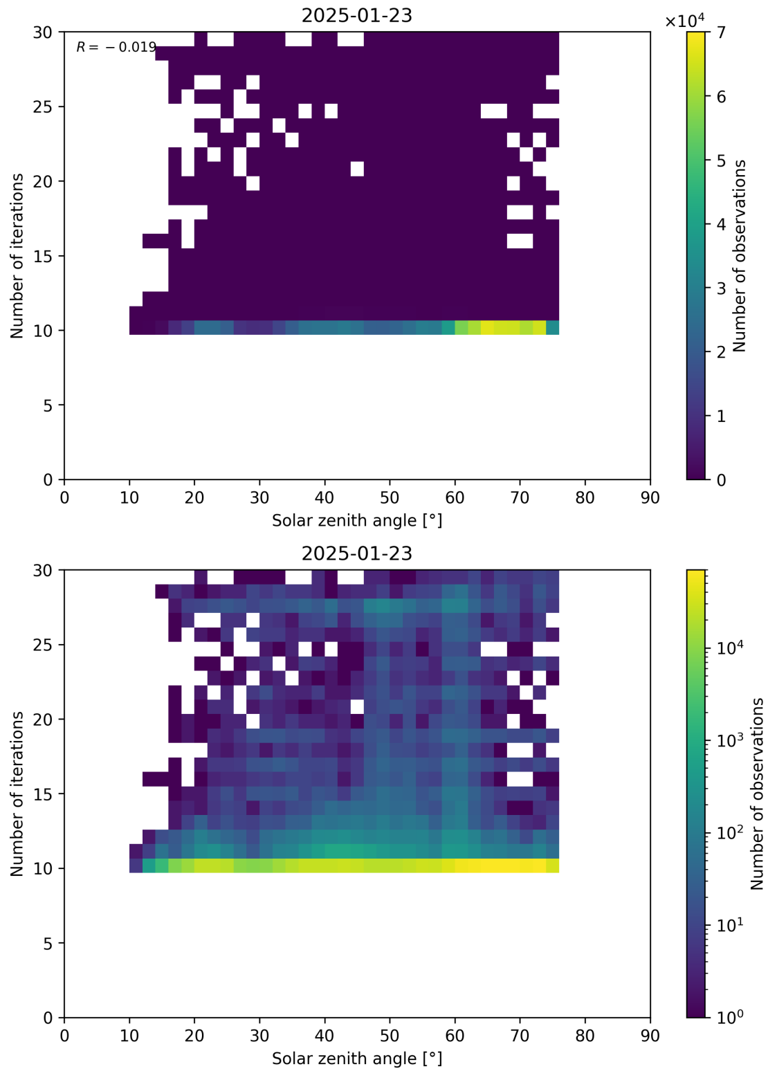
Figure 102: Scatter density plot of “Solar zenith angle” against “Number of iterations” for 2025-01-23 to 2025-01-24.
