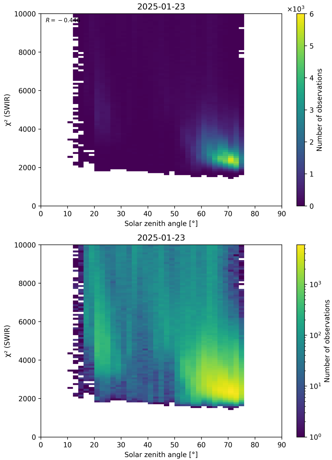
Figure 95: Scatter density plot of “Solar zenith angle” against “ \chi^2 (SWIR)” for 2025-01-23 to 2025-01-24.
