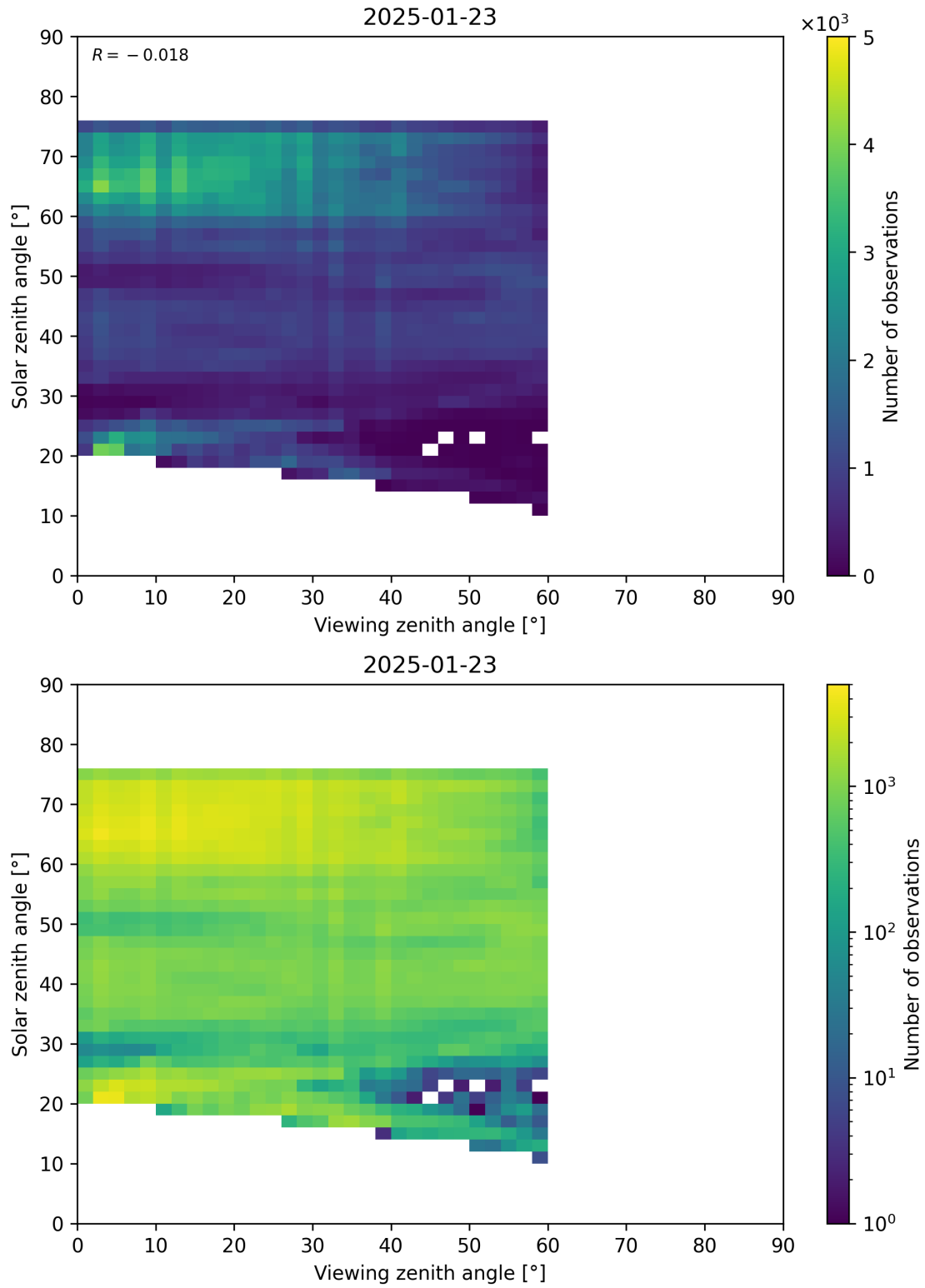
Figure 115: Scatter density plot of “Viewing zenith angle” against “Solar zenith angle” for 2025-01-23 to 2025-01-24.
