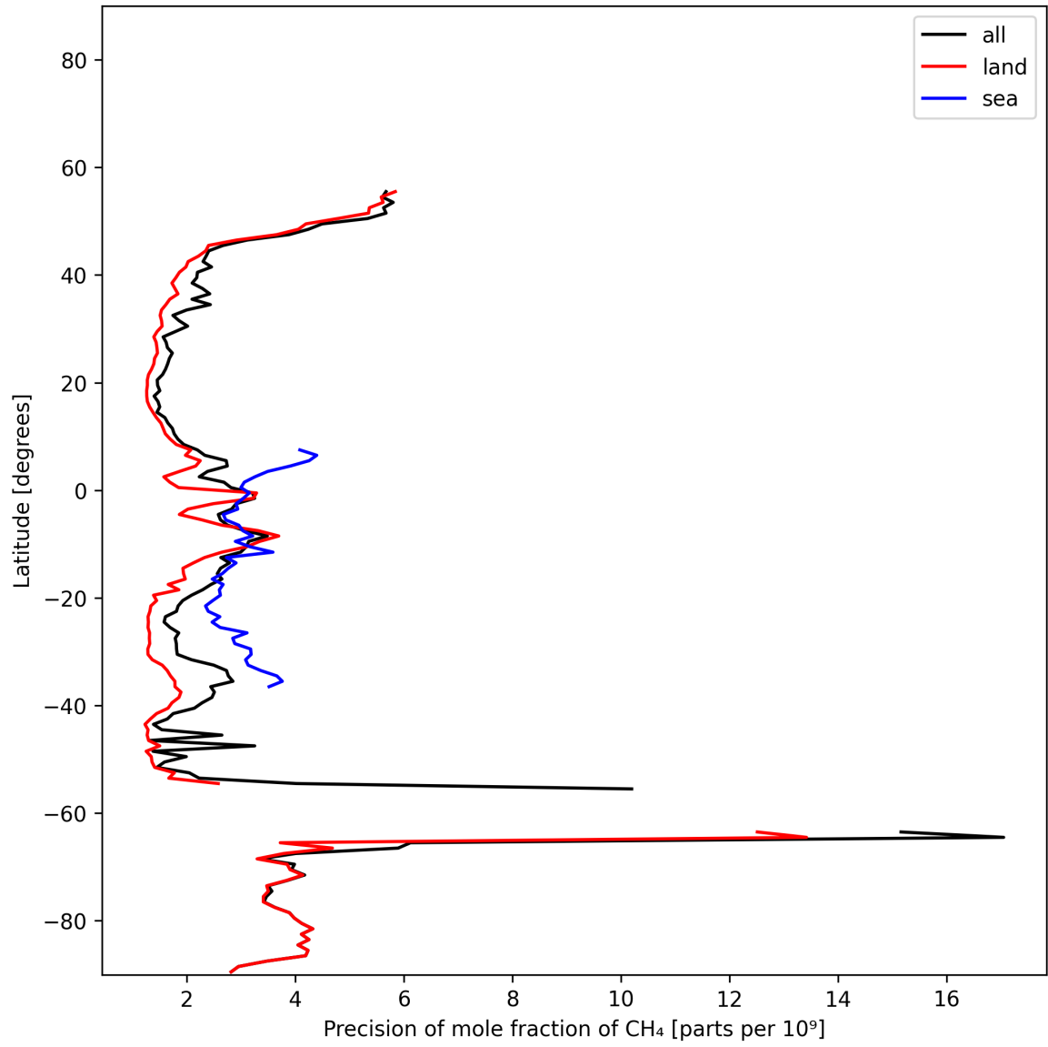
Figure 13: Zonal average of “Precision of mole fraction of CH 4 ” for 2025-01-23 to 2025-01-24.
