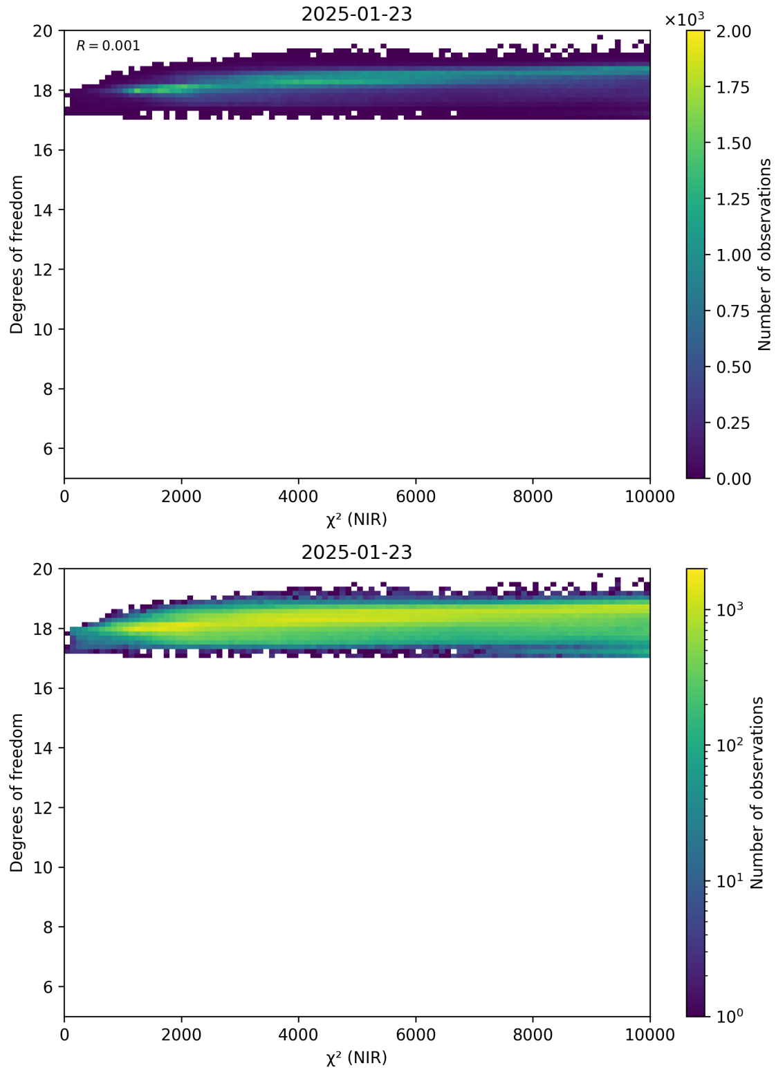
Figure 44: Scatter density plot of “ \chi^2 (NIR)” against “Degrees of freedom” for 2025-01-23 to 2025-01-24.
