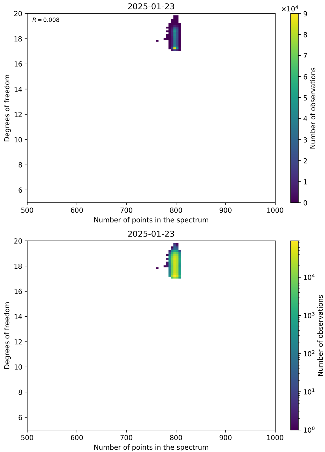
Figure 90: Scatter density plot of “Number of points in the spectrum” against “Degrees of freedom” for 2025-01-23 to 2025-01-24.
