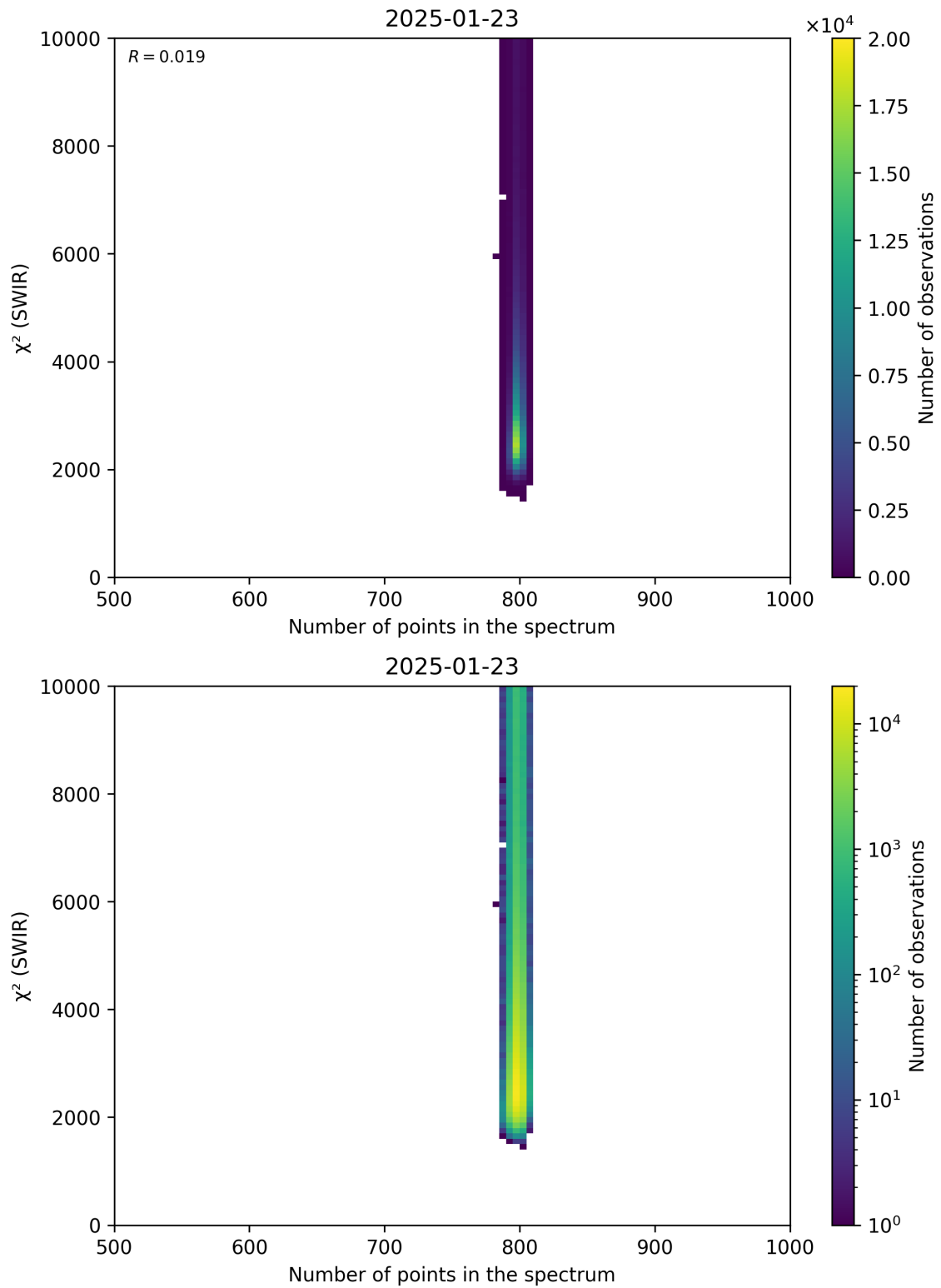
Figure 89: Scatter density plot of “Number of points in the spectrum” against “ \chi^2 (SWIR)” for 2025-01-23 to 2025-01-24.
