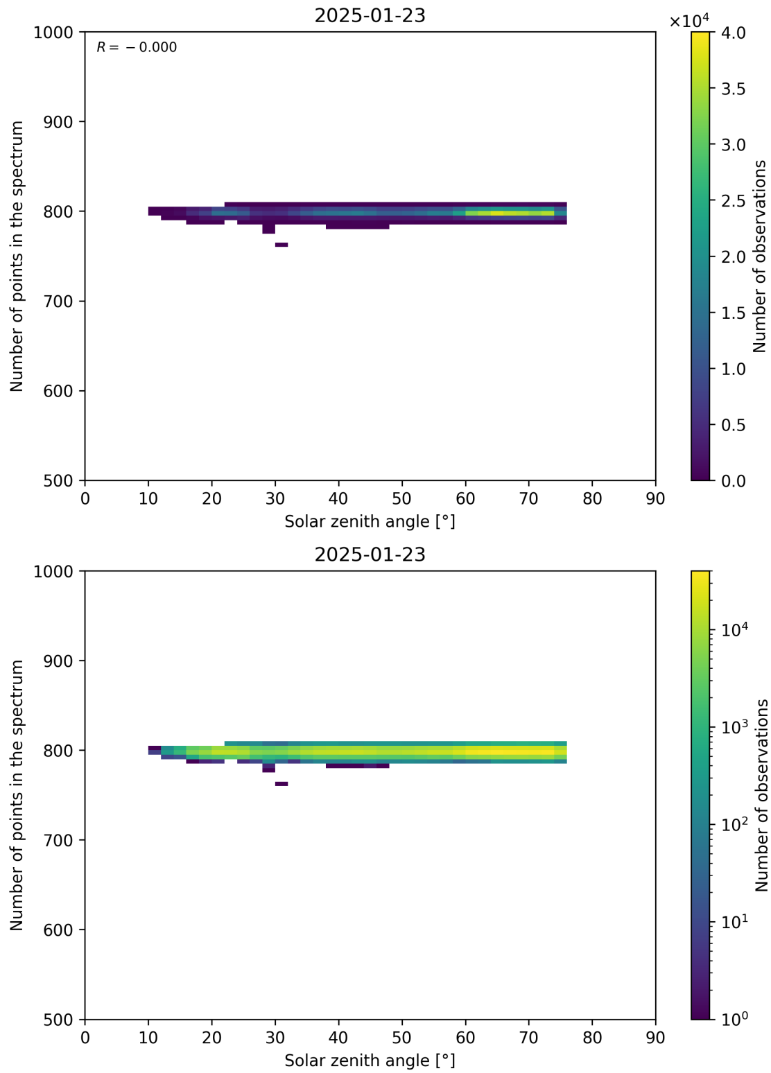
Figure 103: Scatter density plot of “Solar zenith angle” against “Number of points in the spectrum” for 2025-01-23 to 2025-01-24.
