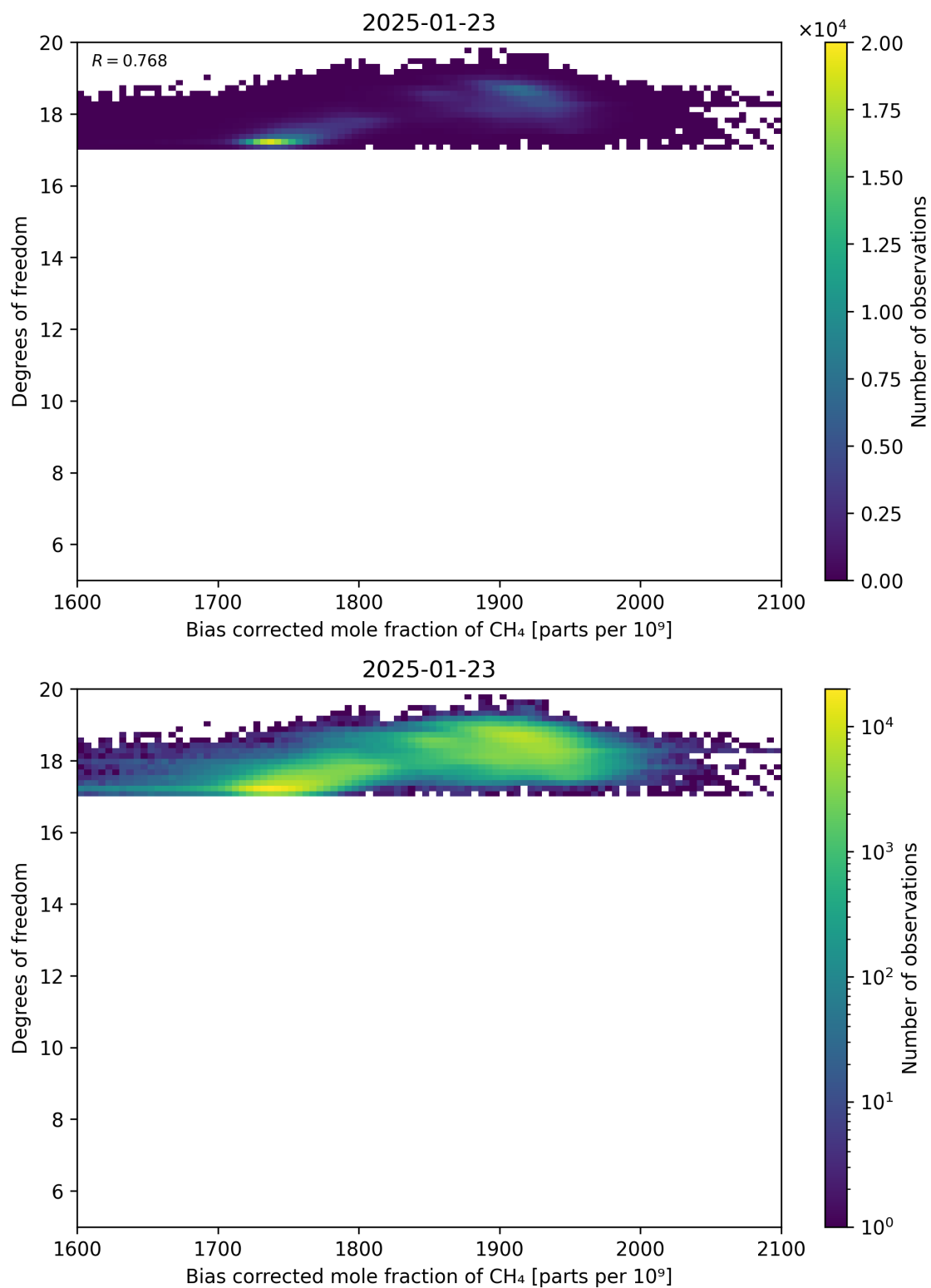
Figure 65: Scatter density plot of “Bias corrected mole fraction of CH 4 ” against “Degrees of freedom” for 2025-01-23 to 2025-01-24.
