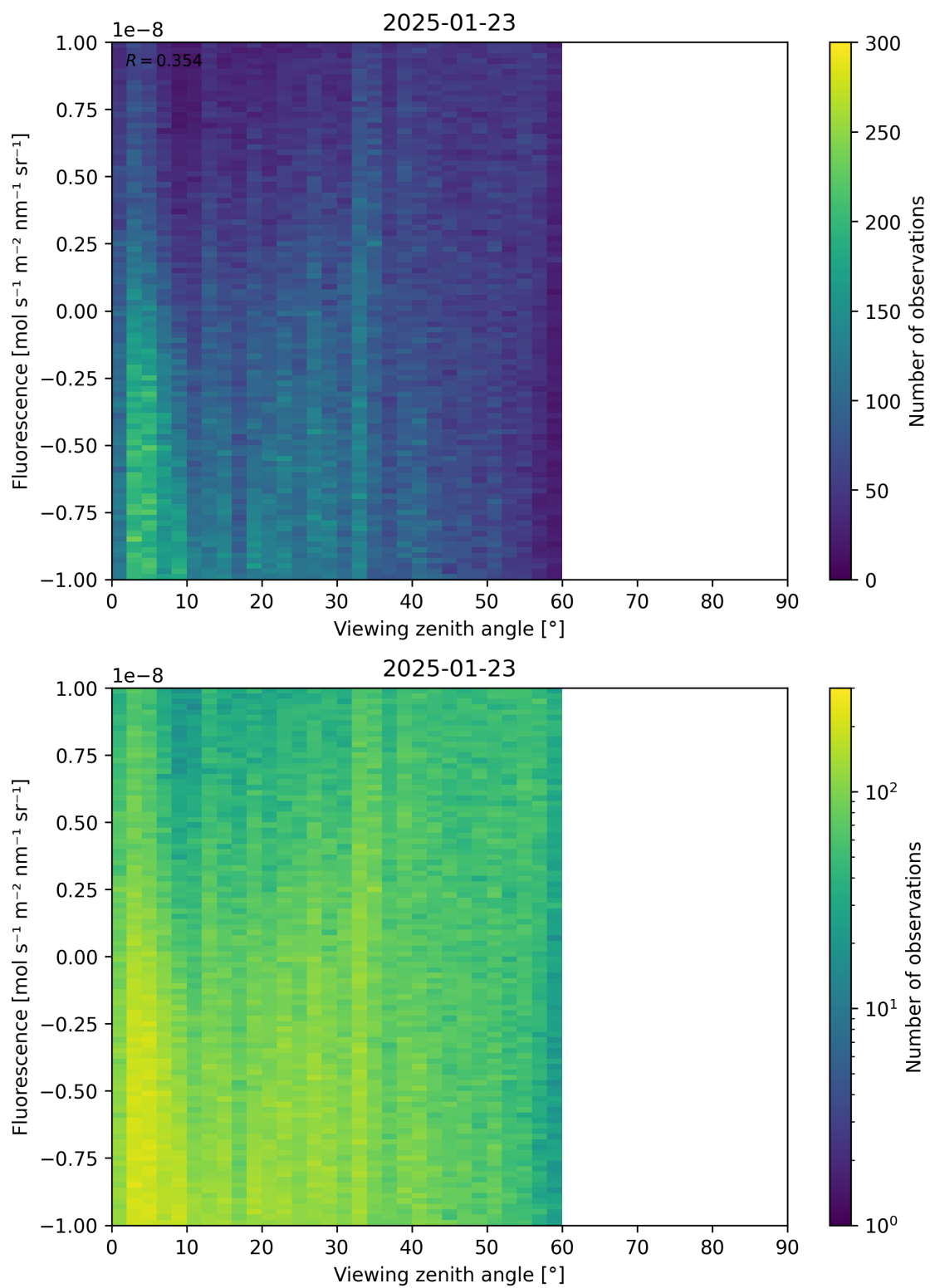
Figure 108: Scatter density plot of “Viewing zenith angle” against “Fluorescence” for 2025-01-23 to 2025-01-24.
