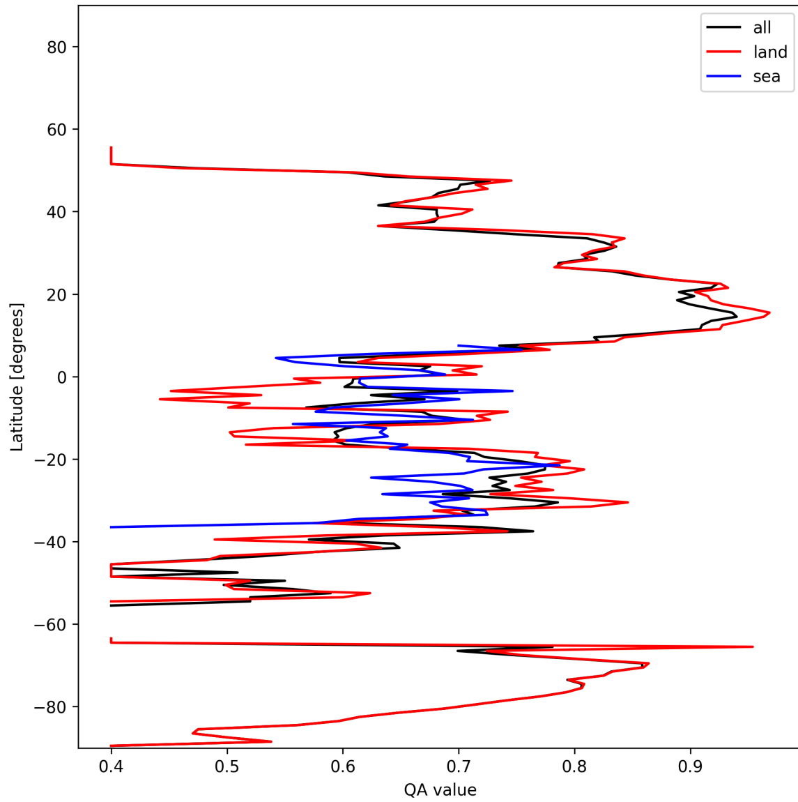
Figure 11: Zonal average of “QA value” for 2025-01-23 to 2025-01-24.
