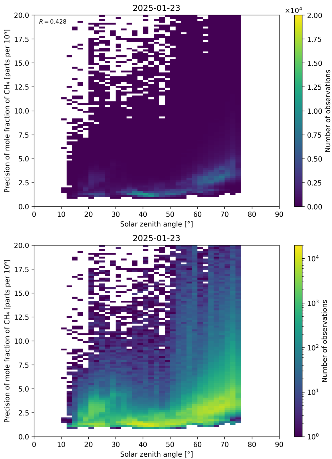
Figure 101: Scatter density plot of “Solar zenith angle” against “Precision of mole fraction of CH 4 ” for 2025-01-23 to 2025-01-24.
