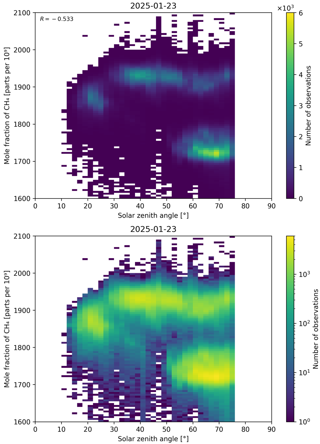
Figure 99: Scatter density plot of “Solar zenith angle” against “Mole fraction of CH 4 ” for 2025-01-23 to 2025-01-24.
