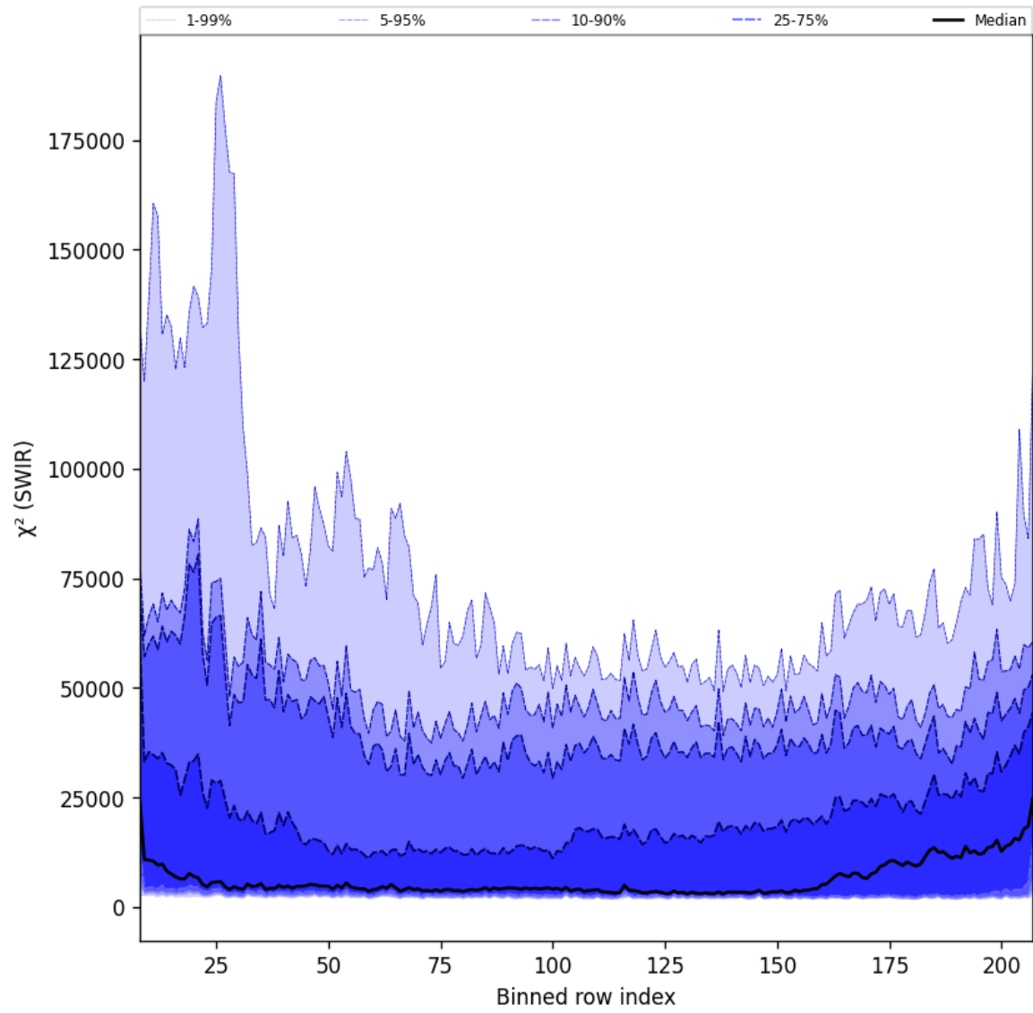
Figure 39: Along track statistics of “ \chi^2 (SWIR)” for 2025-01-23 to 2025-01-24
