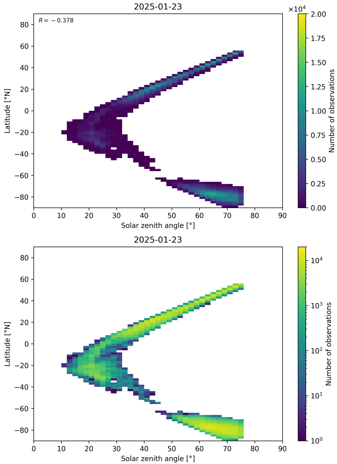
Figure 98: Scatter density plot of “Solar zenith angle” against “Latitude” for 2025-01-23 to 2025-01-24.
