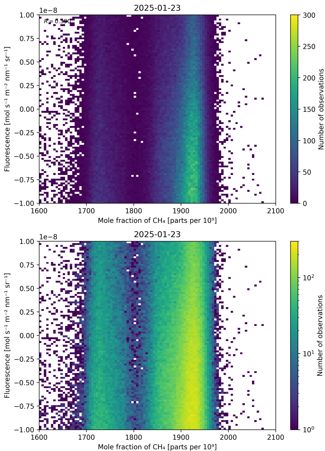
Figure 73: Scatter density plot of “Mole fraction of \text{CH}_4 ” against “Fluorescence” for 2025-01-23 to 2025-01-24.
