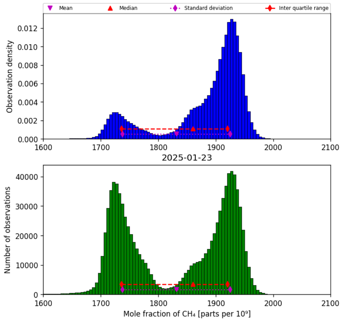
Figure 23: Histogram of “Mole fraction of CH 4 ” for 2025-01-23 to 2025-01-24
