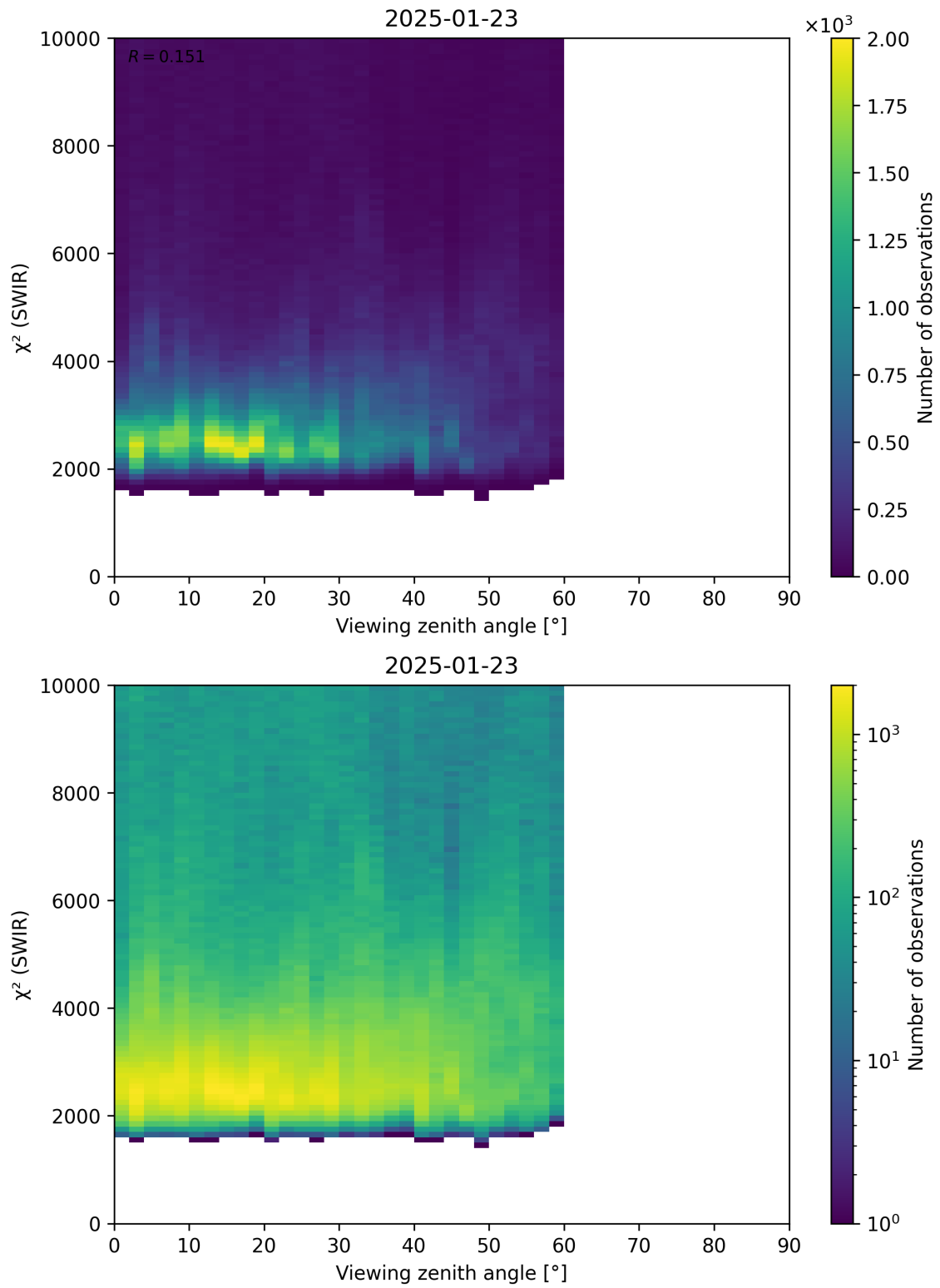
Figure 106: Scatter density plot of “Viewing zenith angle” against “ \chi^2 (SWIR)” for 2025-01-23 to 2025-01-24.
