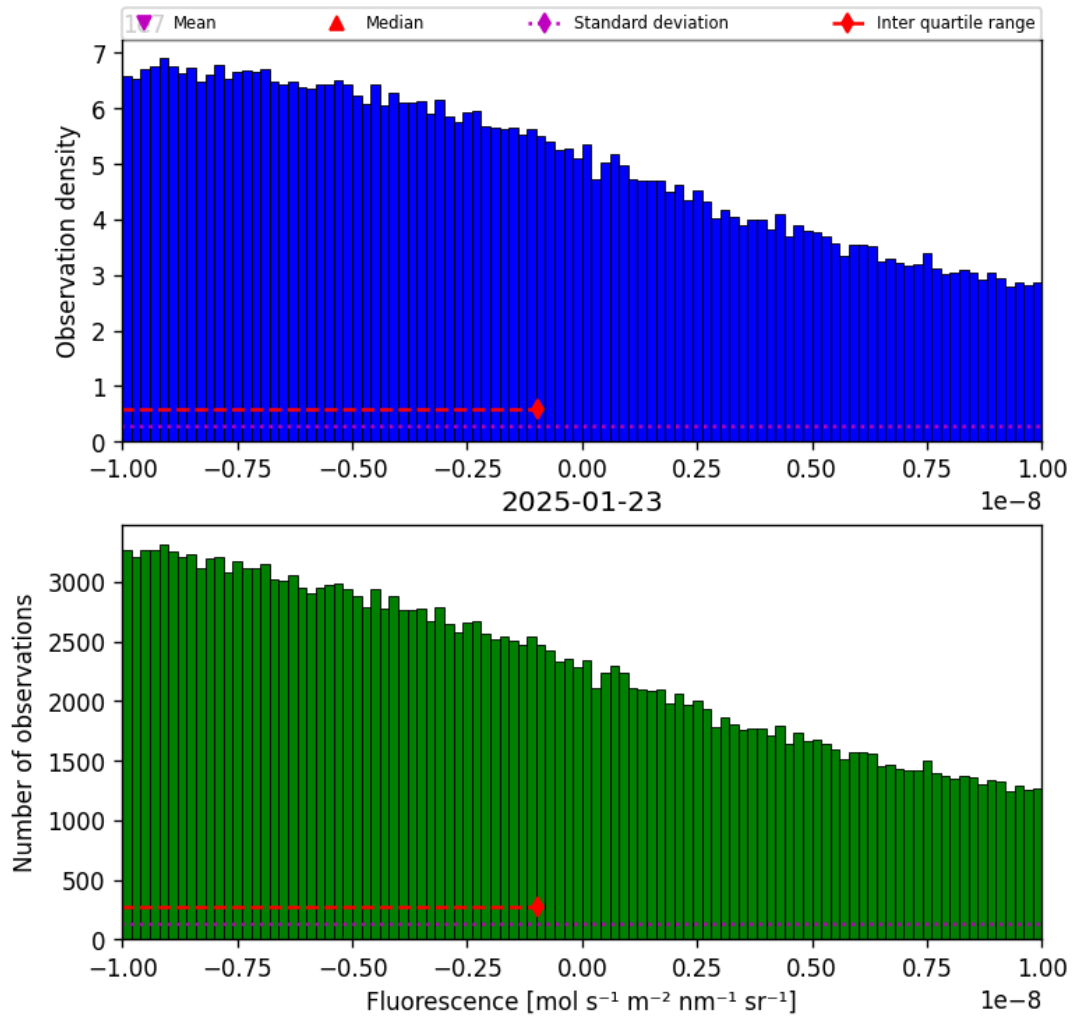
Figure 32: Histogram of “Fluorescence” for 2025-01-23 to 2025-01-24
