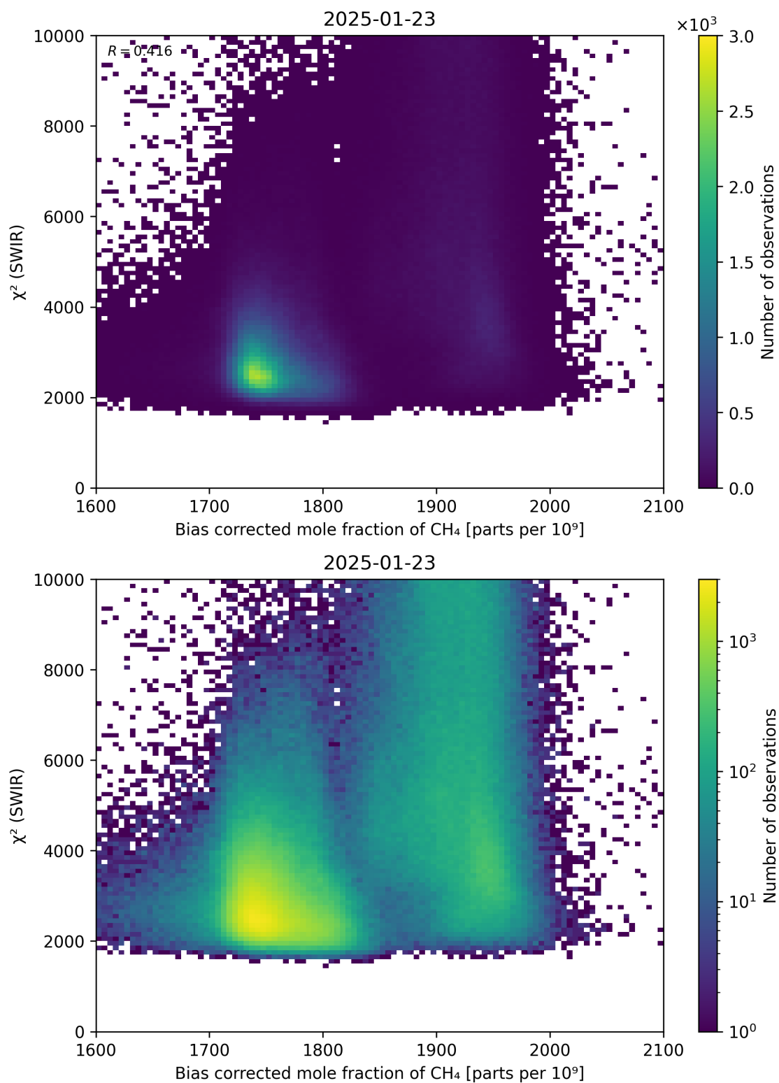
Figure 64: Scatter density plot of “Bias corrected mole fraction of \text{CH}_4 ” against “ \chi^2 (SWIR)” for 2025-01-23 to 2025-01-24.
