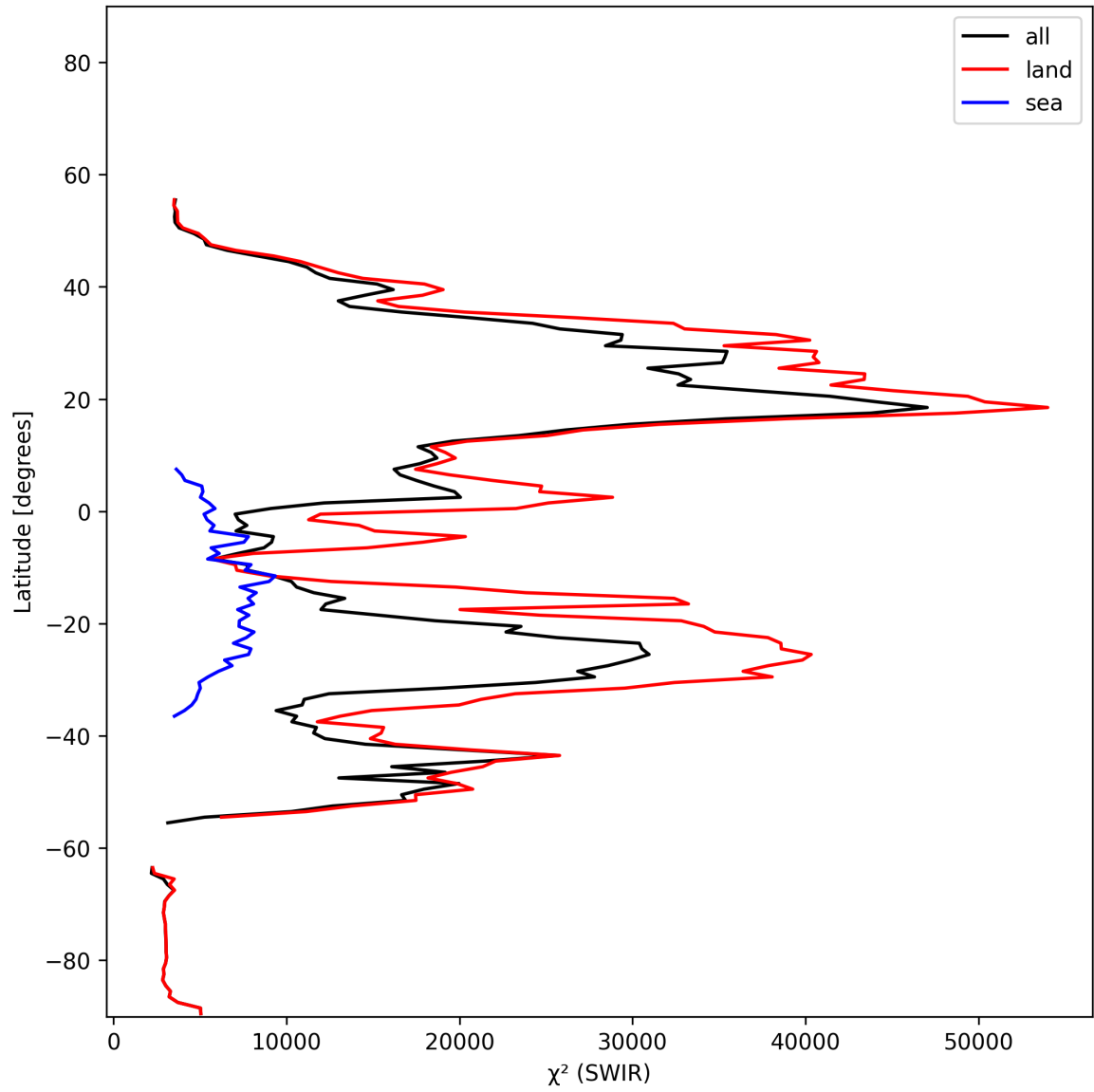
Figure 17: Zonal average of “ \chi^2 (SWIR)” for 2025-01-23 to 2025-01-24.
