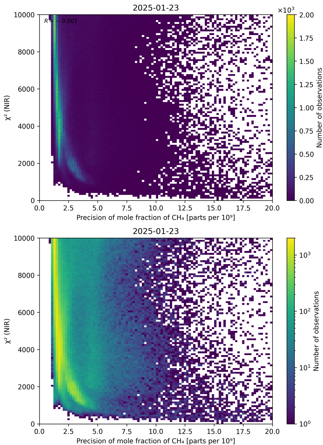
Figure 78: Scatter density plot of “Precision of mole fraction of CH 4 ” against “ \chi^2 (NIR)” for 2025-01-23 to 2025-01-24.
