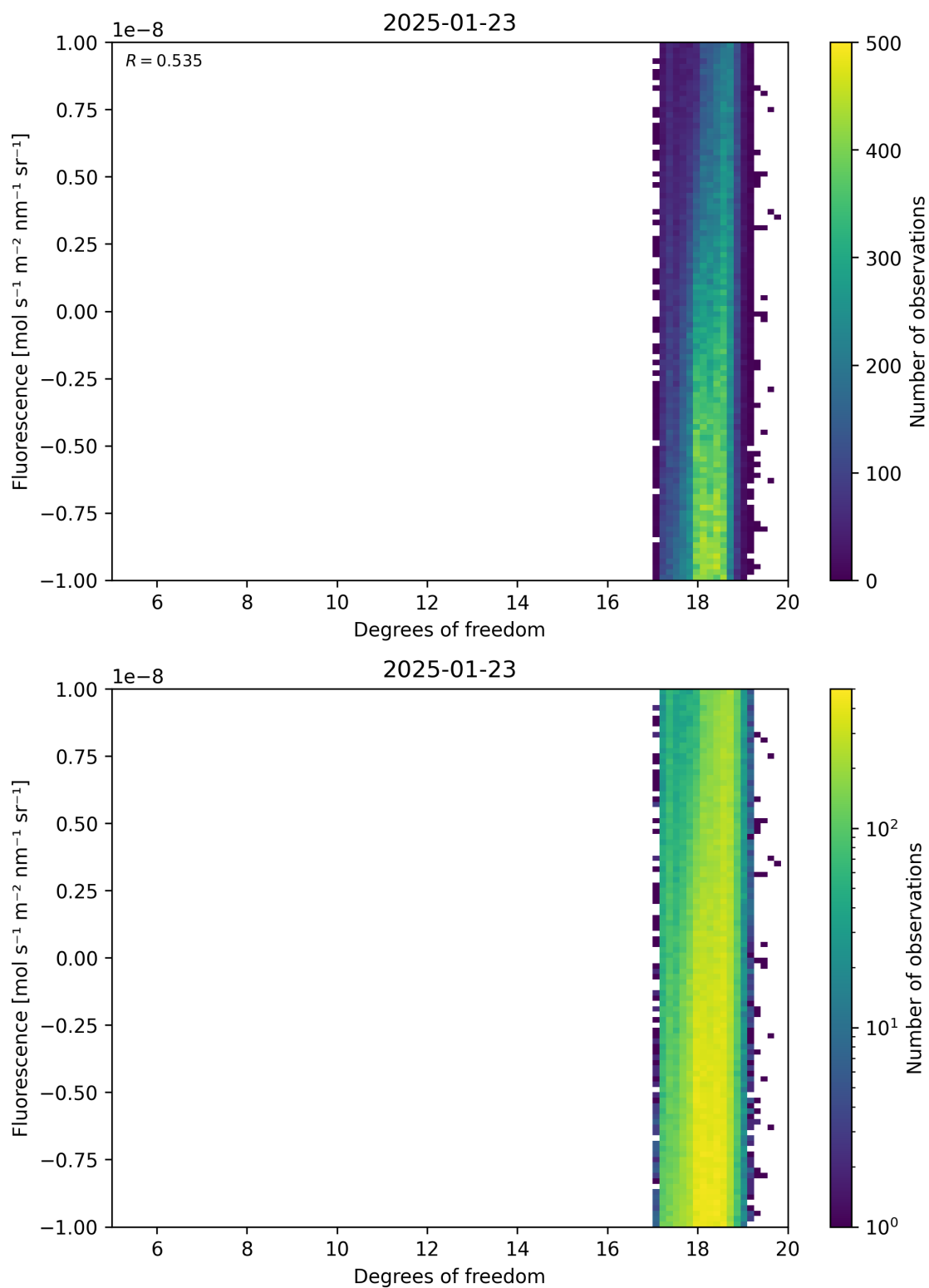
Figure 51: Scatter density plot of “Degrees of freedom” against “Fluorescence” for 2025-01-23 to 2025-01-24.
