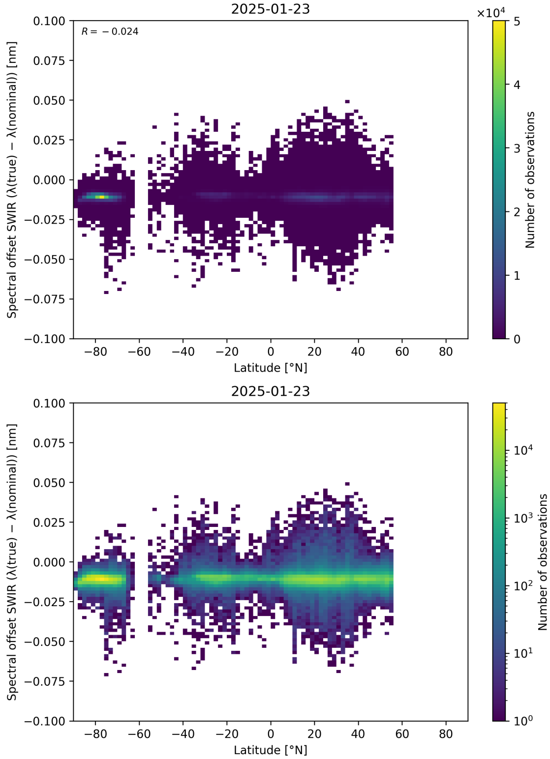
Figure 62: Scatter density plot of “Latitude” against “Spectral offset SWIR ( \lambda_{\text{true}} - \lambda_{\text{nominal}} )” for 2025-01-23 to 2025-01-24.
