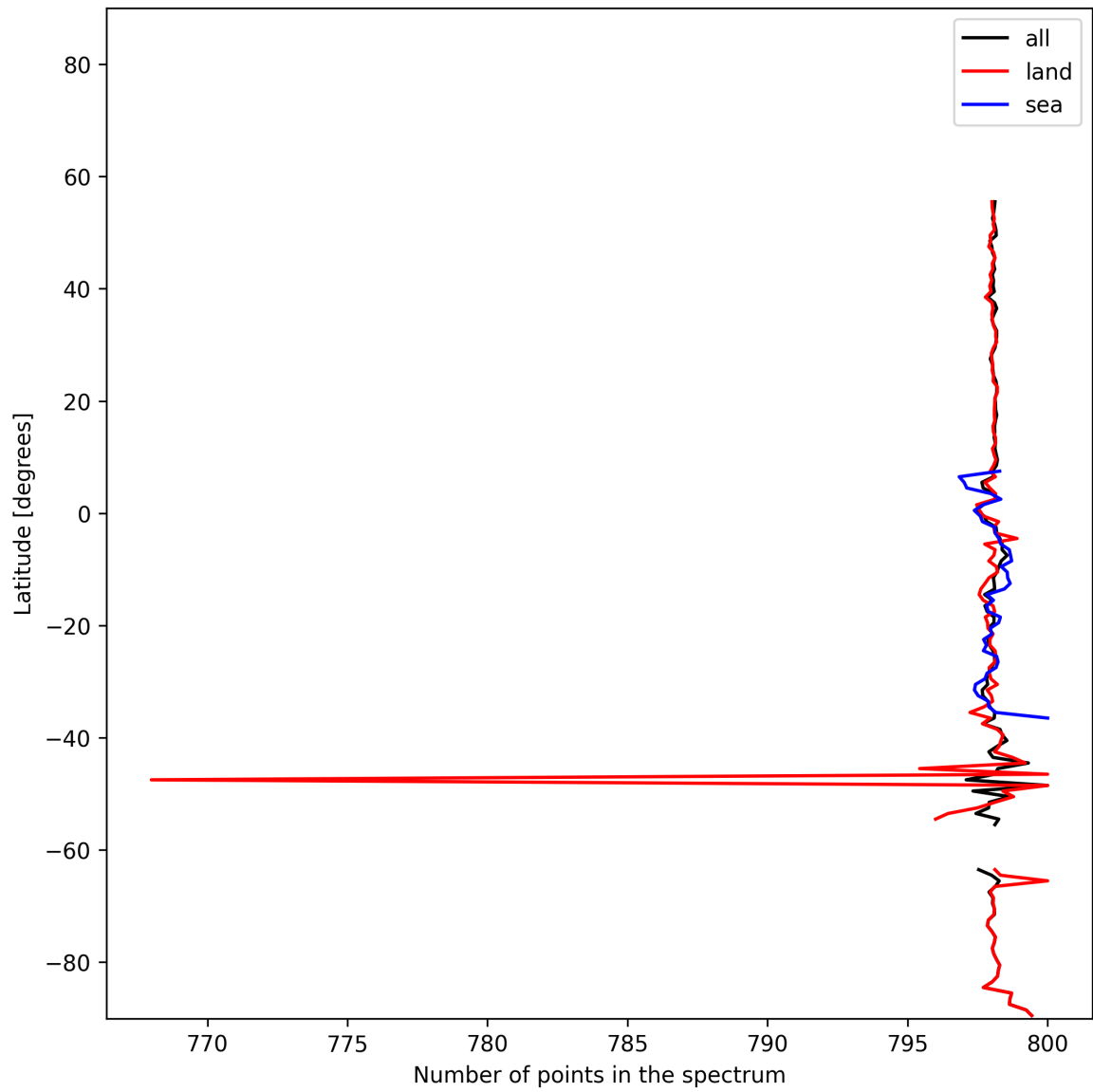
Figure 15: Zonal average of “Number of points in the spectrum” for 2025-01-23 to 2025-01-24.
