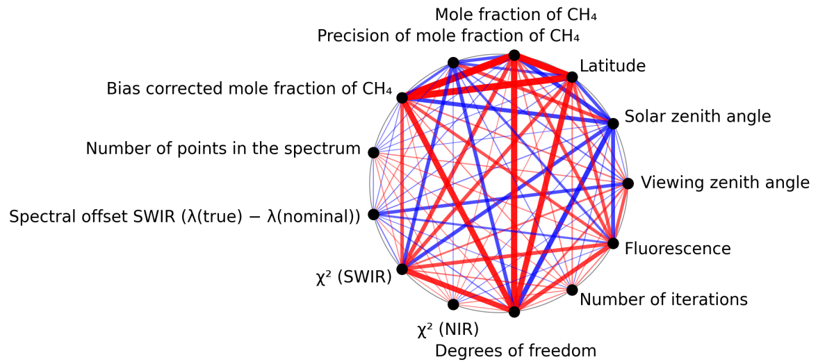
Figure 1: Map of correlation graph for 2025-01-23 to 2025-01-24.
