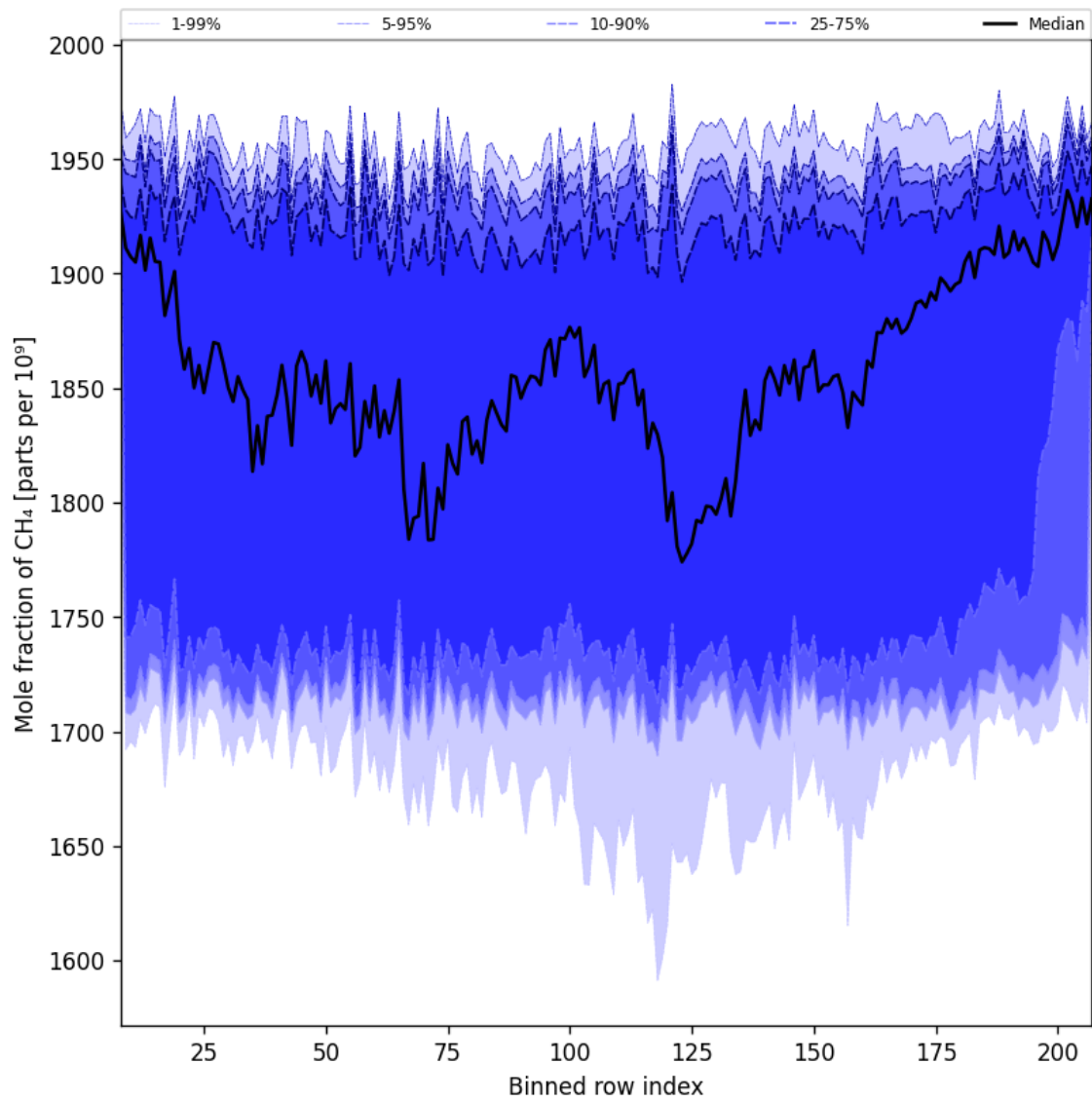
Figure 34: Along track statistics of “Mole fraction of CH 4 ” for 2025-01-23 to 2025-01-24
