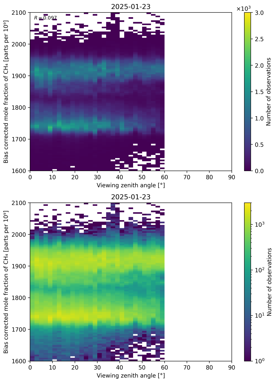
Figure 111: Scatter density plot of “Viewing zenith angle” against “Bias corrected mole fraction of CH 4 ” for 2025-01-23 to 2025-01-24.
