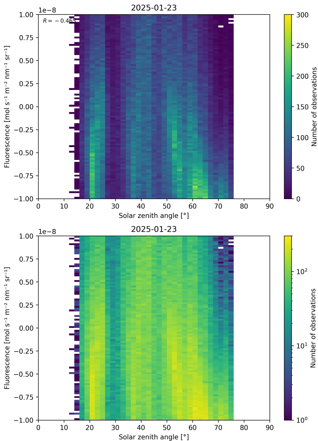
Figure 97: Scatter density plot of “Solar zenith angle” against “Fluorescence” for 2025-01-23 to 2025-01-24.
