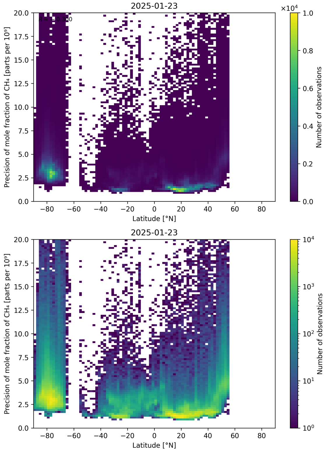
Figure 59: Scatter density plot of “Latitude” against “Precision of mole fraction of CH 4 ” for 2025-01-23 to 2025-01-24.
