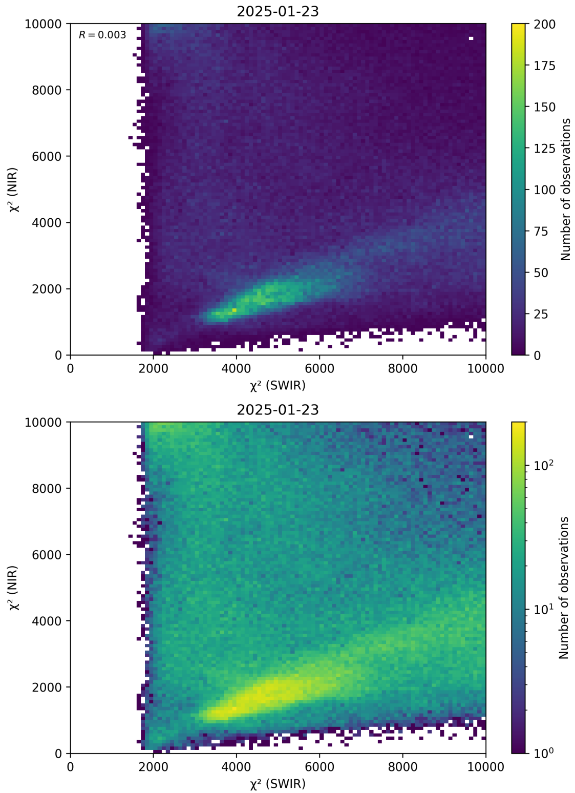
Figure 47: Scatter density plot of “ \chi^2 (SWIR)” against “ \chi^2 (NIR)” for 2025-01-23 to 2025-01-24.
