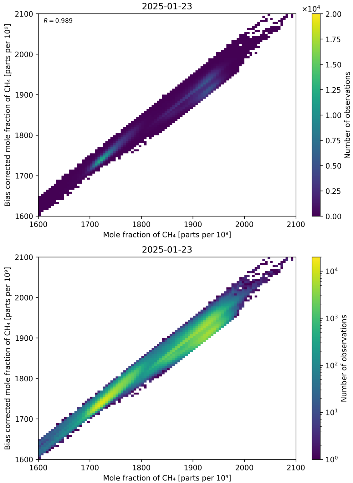
Figure 74: Scatter density plot of “Mole fraction of CH 4 ” against “Bias corrected mole fraction of CH 4 ” for 2025-01-23 to 2025-01-24.
