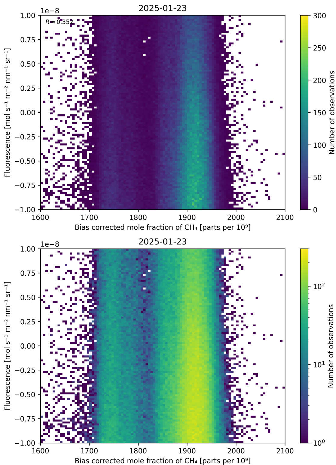
Figure 66: Scatter density plot of “Bias corrected mole fraction of \text{CH}_4 ” against “Fluorescence” for 2025-01-23 to 2025-01-24.
