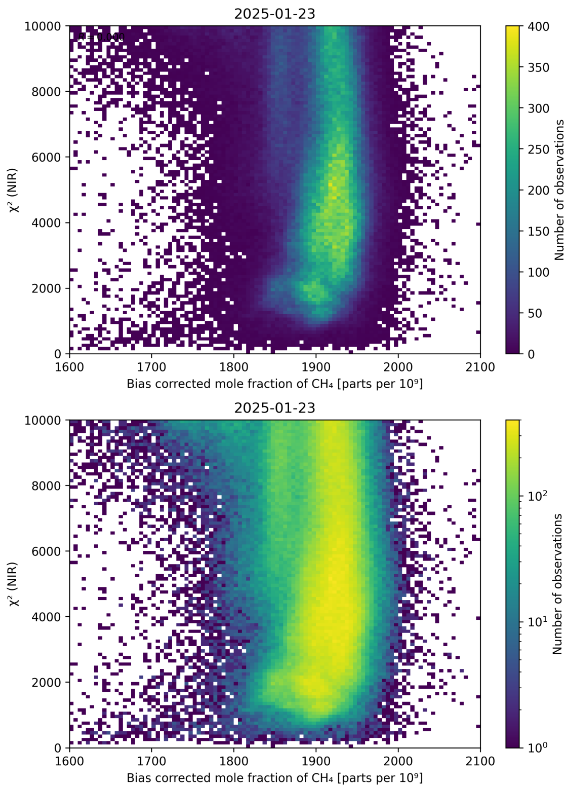
Figure 63: Scatter density plot of “Bias corrected mole fraction of CH 4 ” against “ \chi^2 (NIR)” for 2025-01-23 to 2025-01-24.
