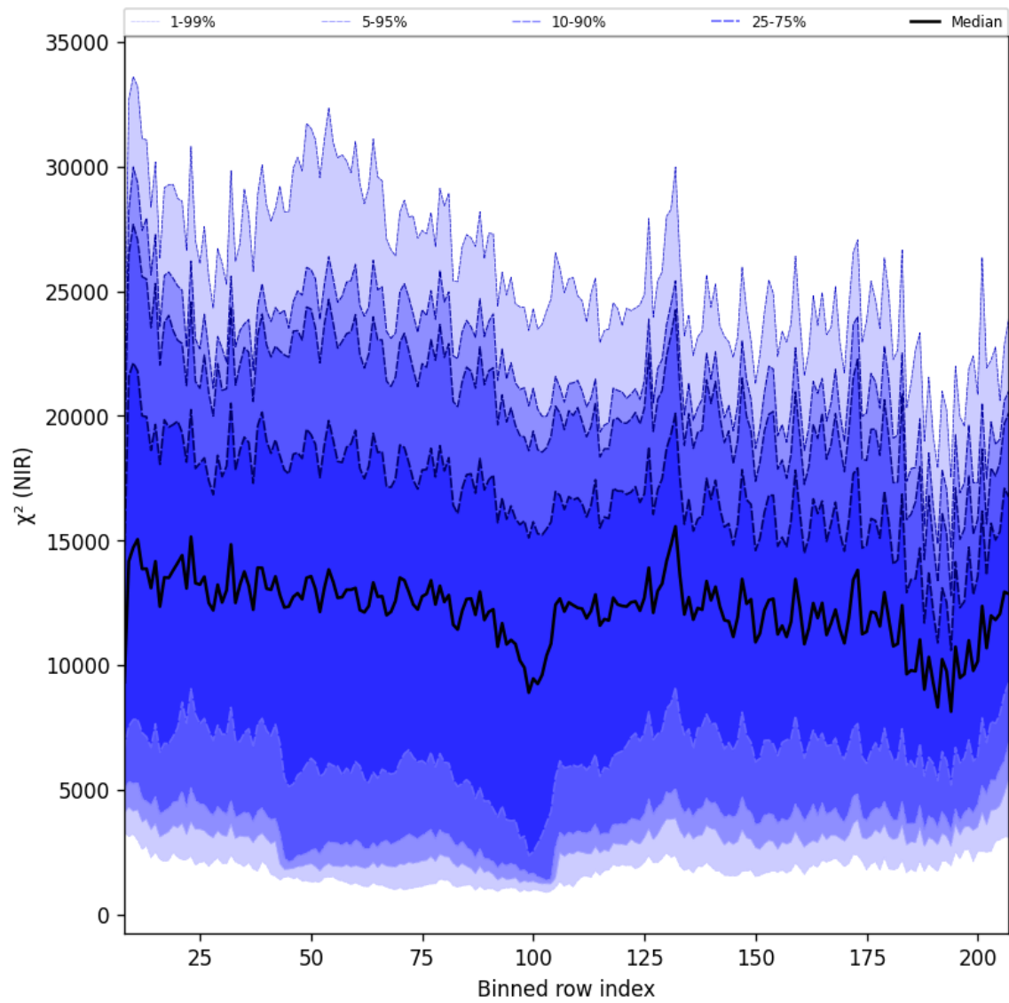
Figure 40: Along track statistics of “ \chi^2 (NIR)” for 2025-01-23 to 2025-01-24
