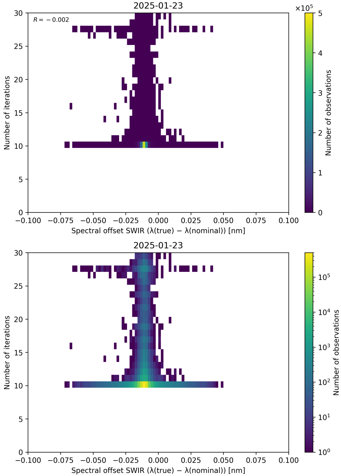
Figure 121: Scatter density plot of “Spectral offset SWIR ( \lambda_{\text{true}} - \lambda_{\text{nominal}} )” against “Number of iterations” for 2025-01-23 to 2025-01-24.
