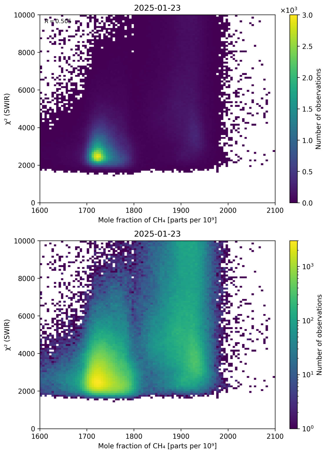
Figure 71: Scatter density plot of “Mole fraction of \text{CH}_4 ” against “ \chi^2 (SWIR)” for 2025-01-23 to 2025-01-24.
