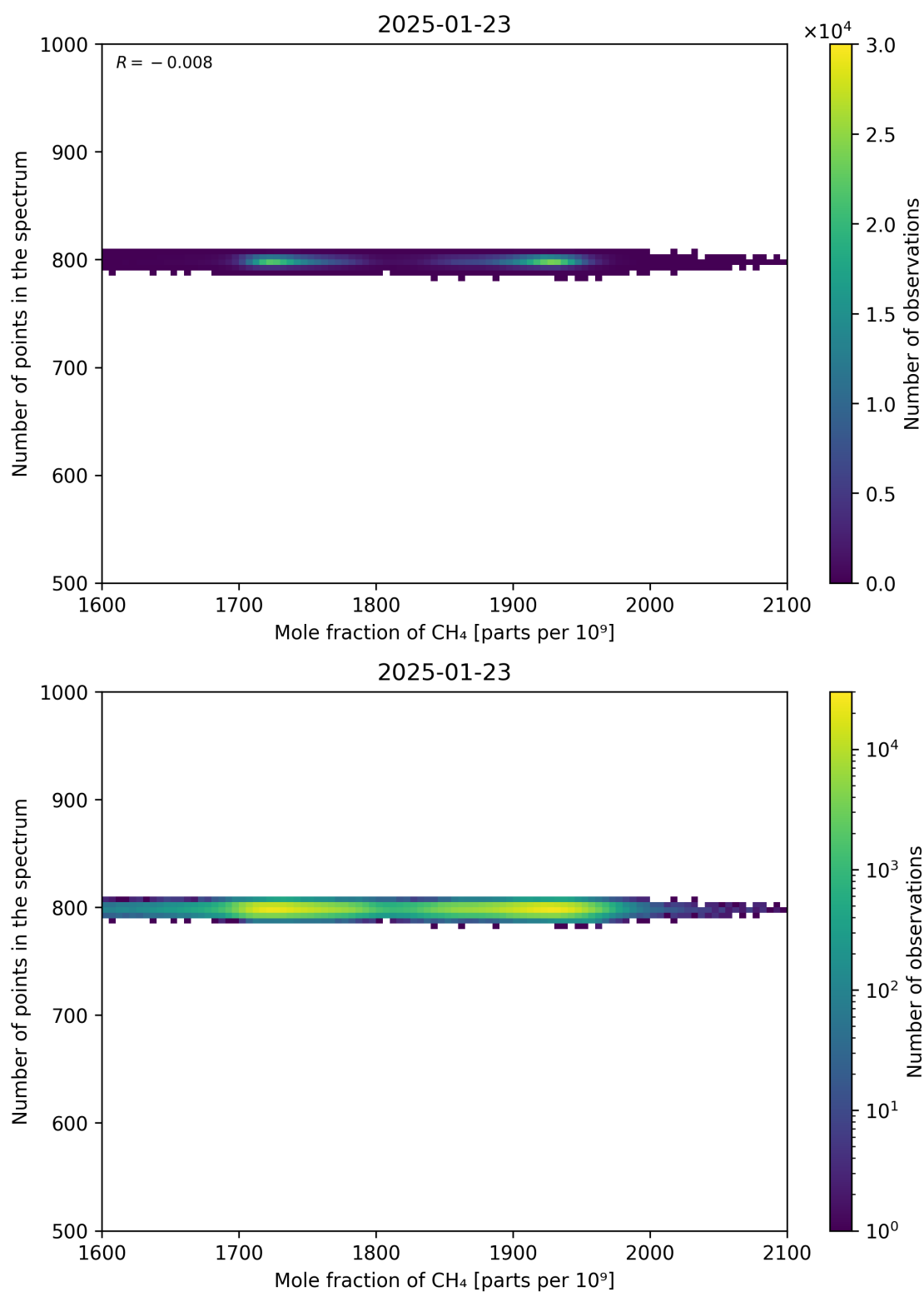
Figure 77: Scatter density plot of “Mole fraction of CH 4 ” against “Number of points in the spectrum” for 2025-01-23 to 2025-01-24.
