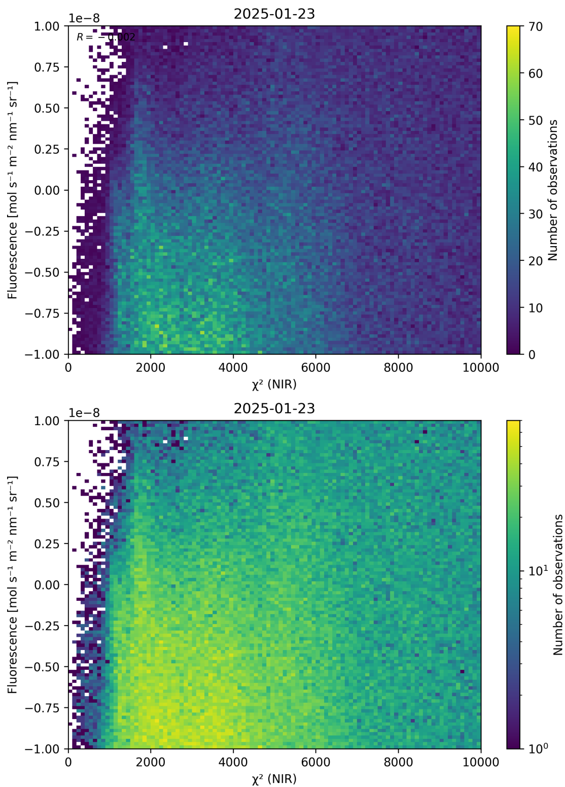
Figure 45: Scatter density plot of “ \chi^2 (NIR)” against “Fluorescence” for 2025-01-23 to 2025-01-24.
