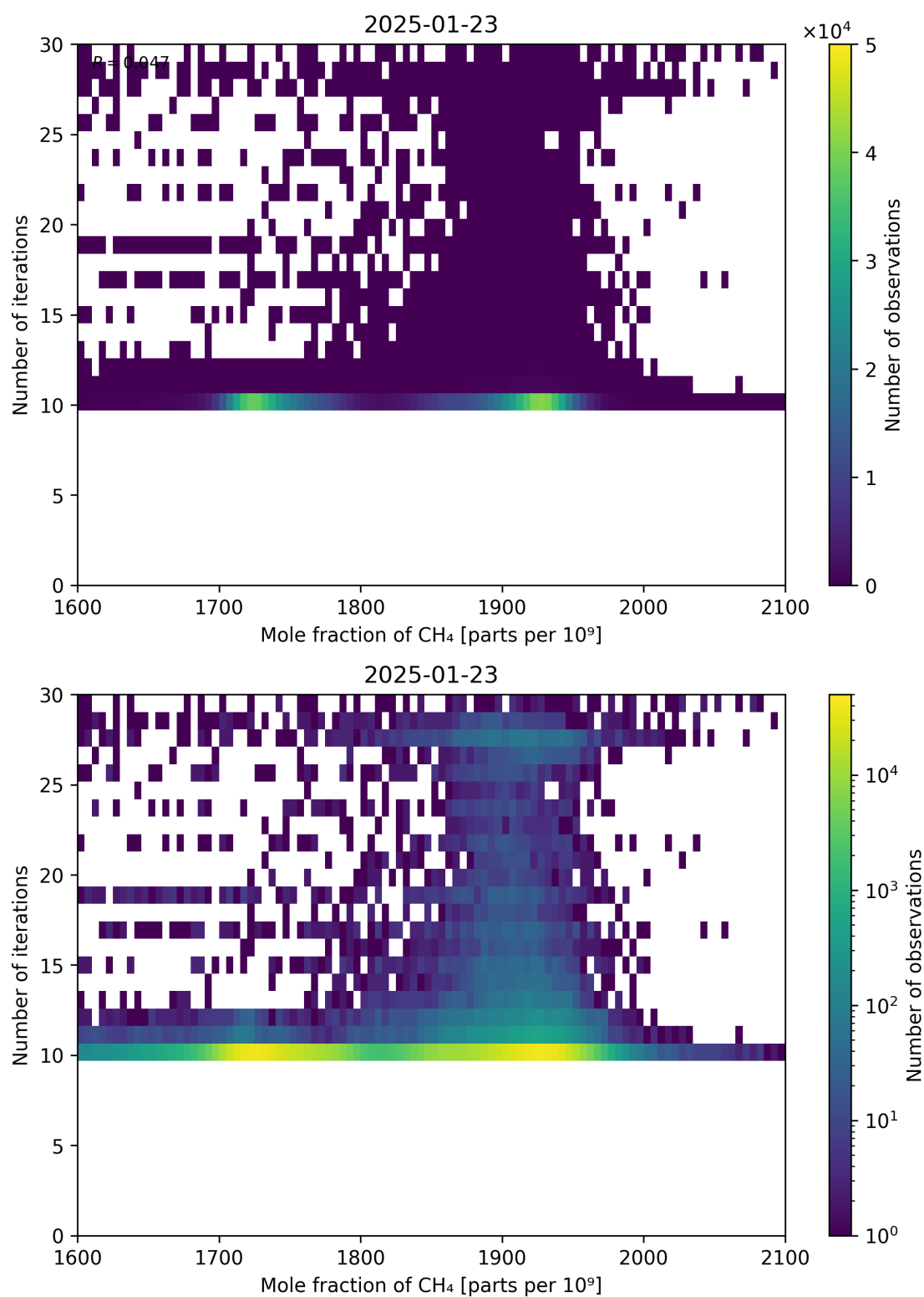
Figure 76: Scatter density plot of “Mole fraction of CH 4 ” against “Number of iterations” for 2025-01-23 to 2025-01-24.
