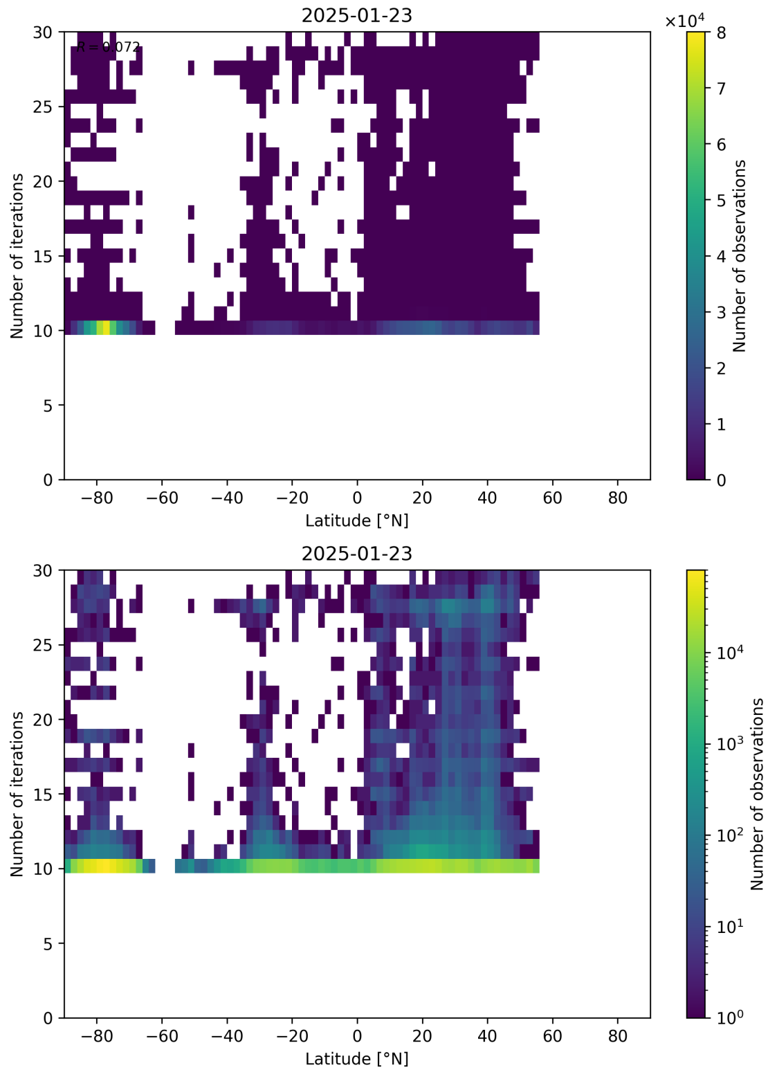
Figure 60: Scatter density plot of “Latitude” against “Number of iterations” for 2025-01-23 to 2025-01-24.
