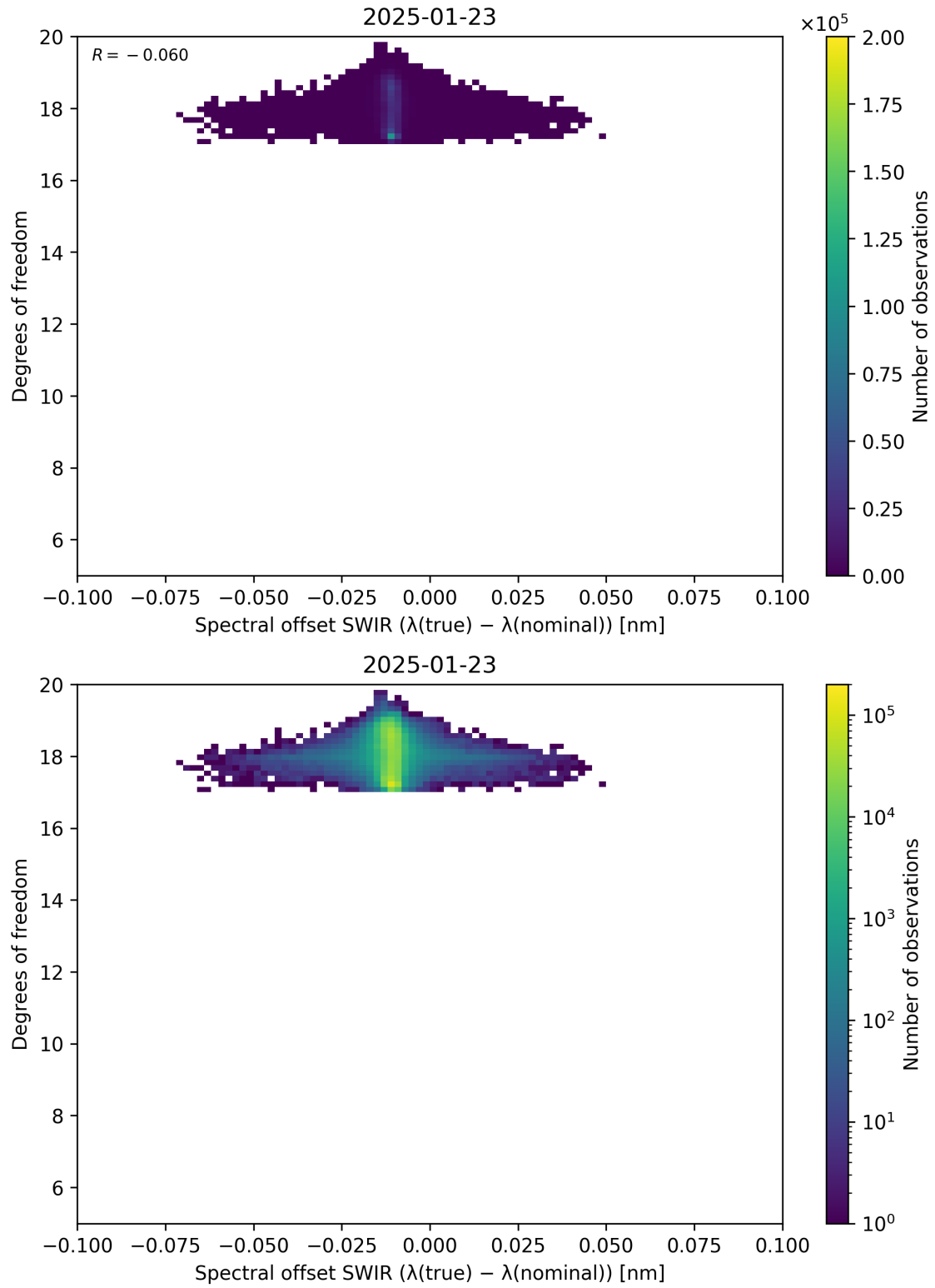
Figure 119: Scatter density plot of “Spectral offset SWIR ( \lambda_{\text{true}} - \lambda_{\text{nominal}} )” against “Degrees of freedom” for 2025-01-23 to 2025-01-24.
