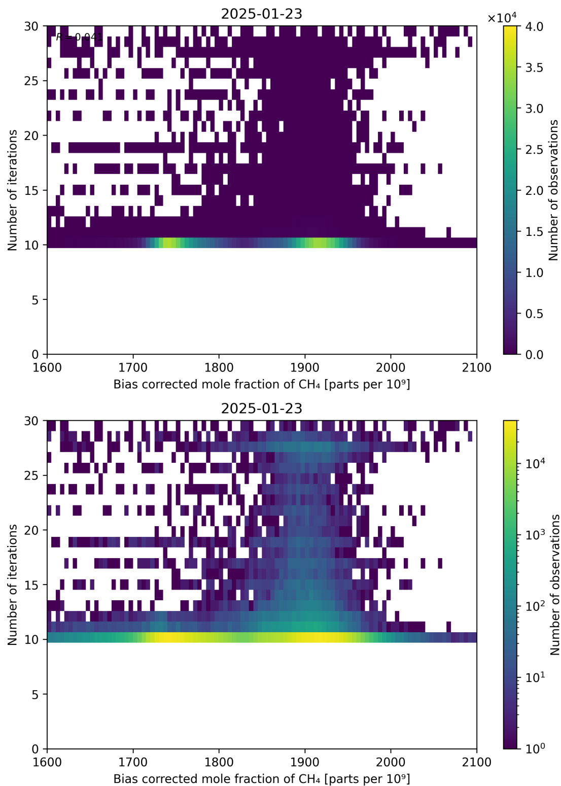
Figure 67: Scatter density plot of “Bias corrected mole fraction of CH 4 ” against “Number of iterations” for 2025-01-23 to 2025-01-24.
