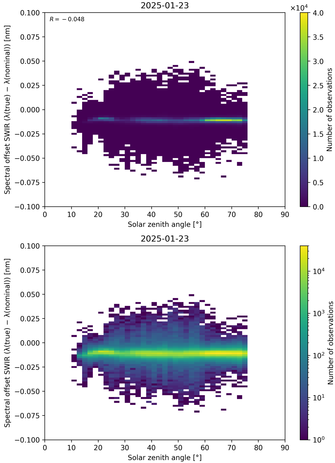
Figure 104: Scatter density plot of “Solar zenith angle” against “Spectral offset SWIR ( \lambda_{\text{true}} - \lambda_{\text{nominal}} )” for 2025-01-23 to 2025-01-24.
