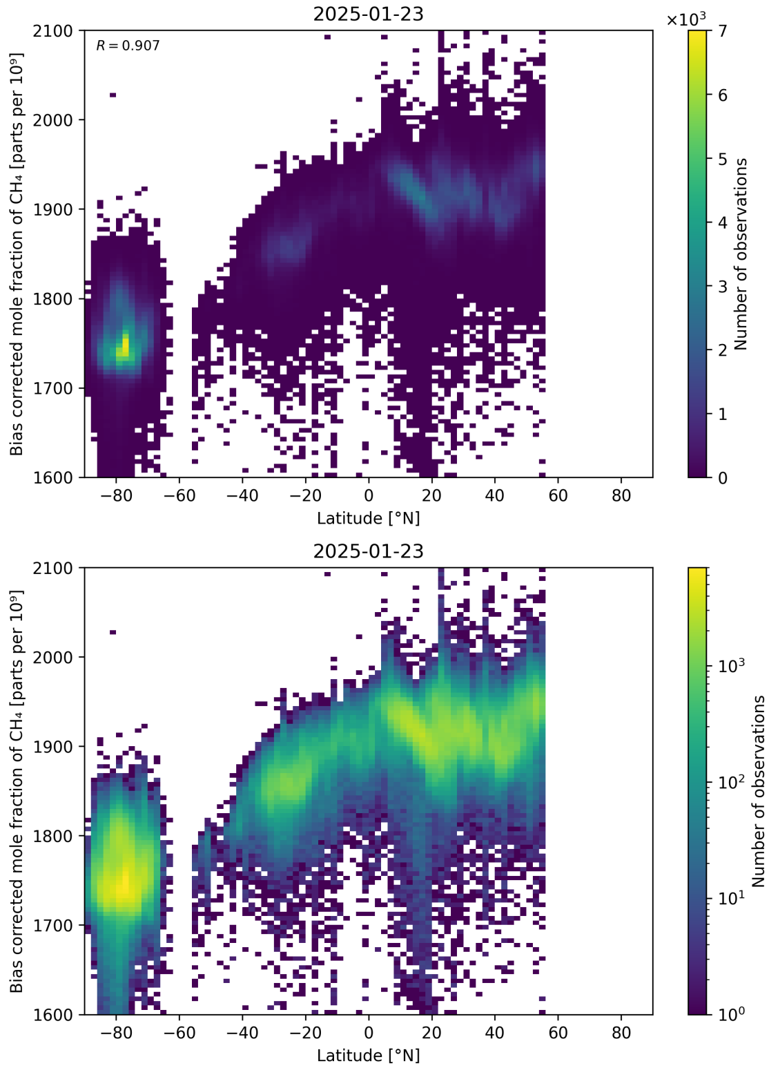
Figure 58: Scatter density plot of “Latitude” against “Bias corrected mole fraction of CH 4 ” for 2025-01-23 to 2025-01-24.
