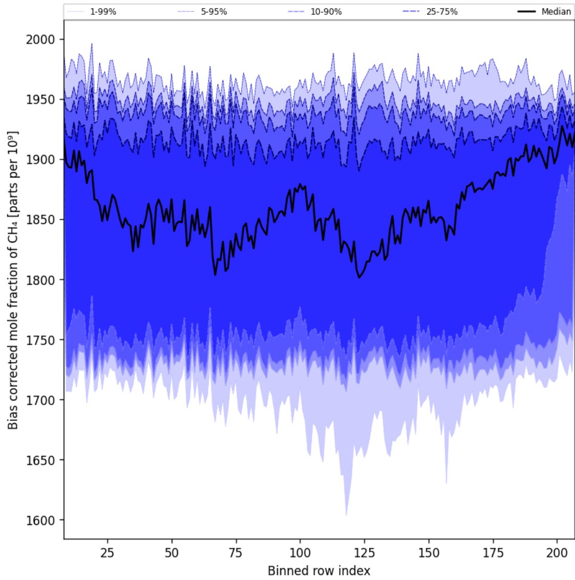
Figure 36: Along track statistics of “Bias corrected mole fraction of CH 4 ” for 2025-01-23 to 2025-01-24
