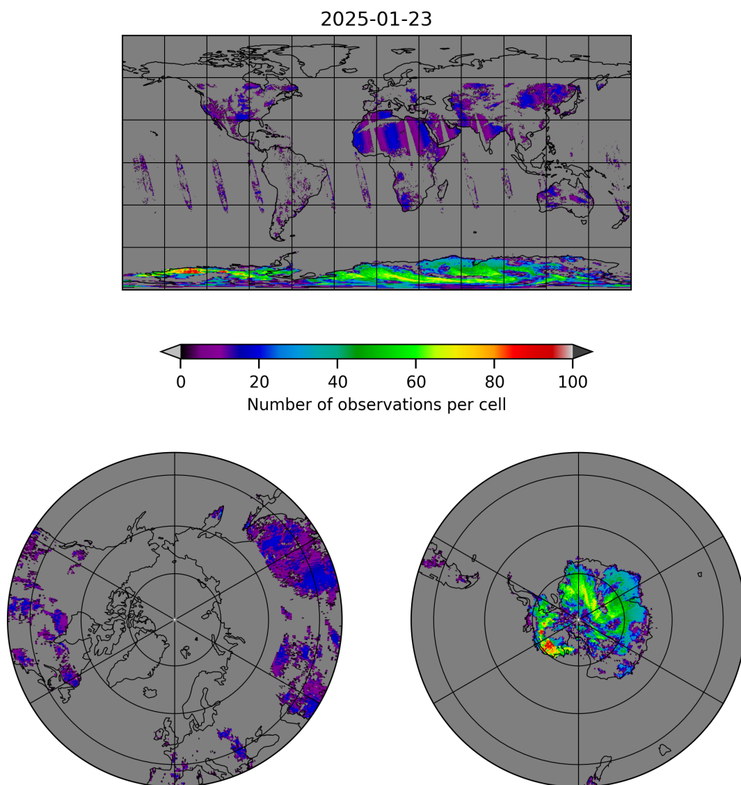
Figure 10: Map of the number of observations for 2025-01-23 to 2025-01-24
