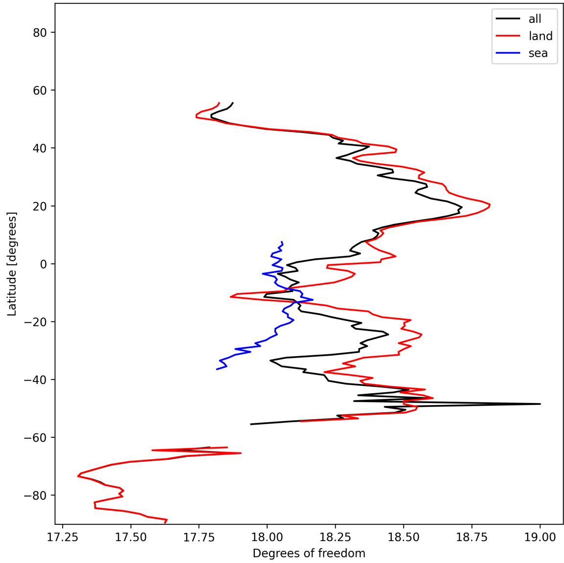
Figure 19: Zonal average of “Degrees of freedom” for 2025-01-23 to 2025-01-24.
