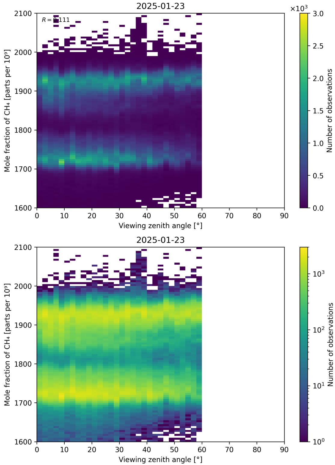
Figure 110: Scatter density plot of “Viewing zenith angle” against “Mole fraction of CH 4 ” for 2025-01-23 to 2025-01-24.
