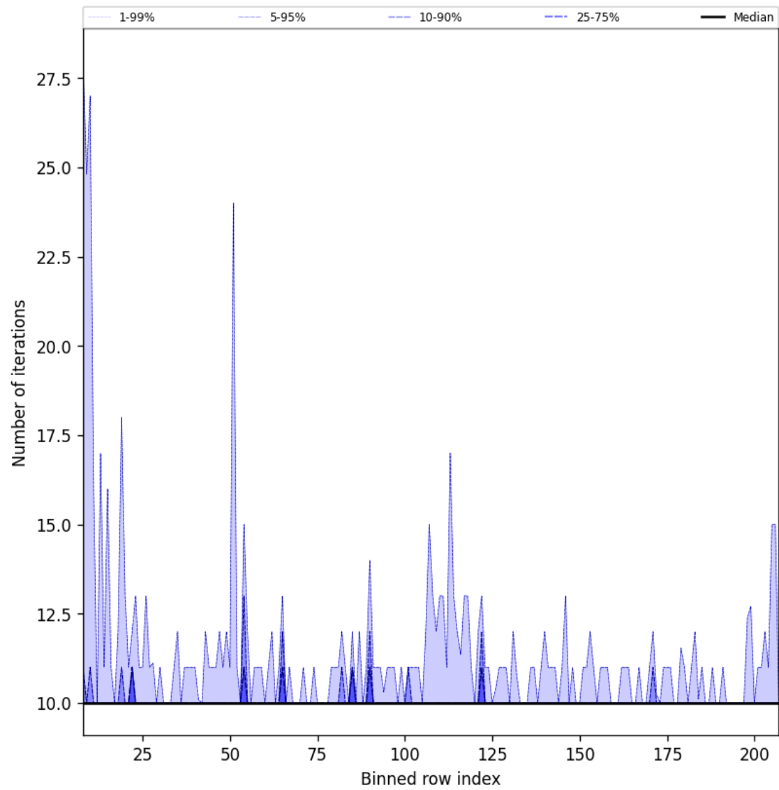
Figure 42: Along track statistics of “Number of iterations” for 2025-01-23 to 2025-01-24
