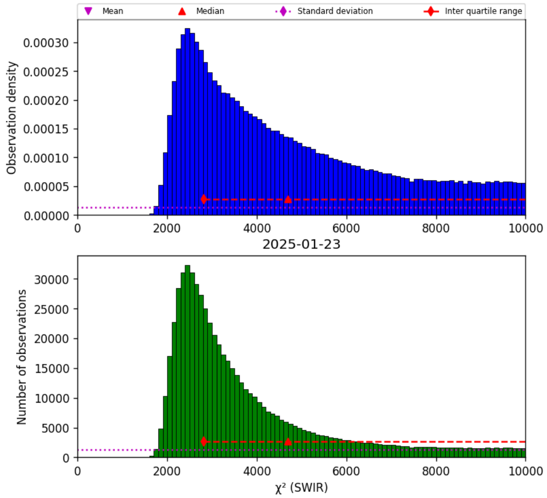
Figure 28: Histogram of “ \chi^2 (SWIR)” for 2025-01-23 to 2025-01-24
