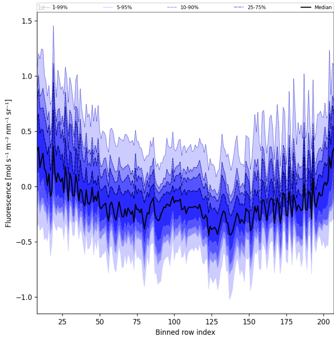
Figure 43: Along track statistics of “Fluorescence” for 2025-01-23 to 2025-01-24
