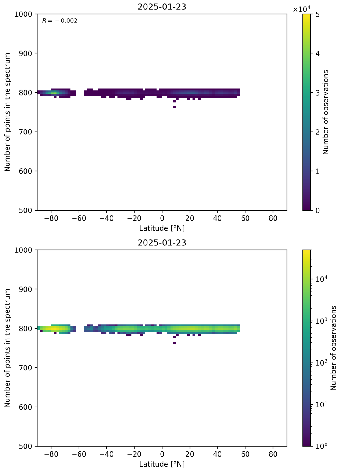
Figure 61: Scatter density plot of “Latitude” against “Number of points in the spectrum” for 2025-01-23 to 2025-01-24.
