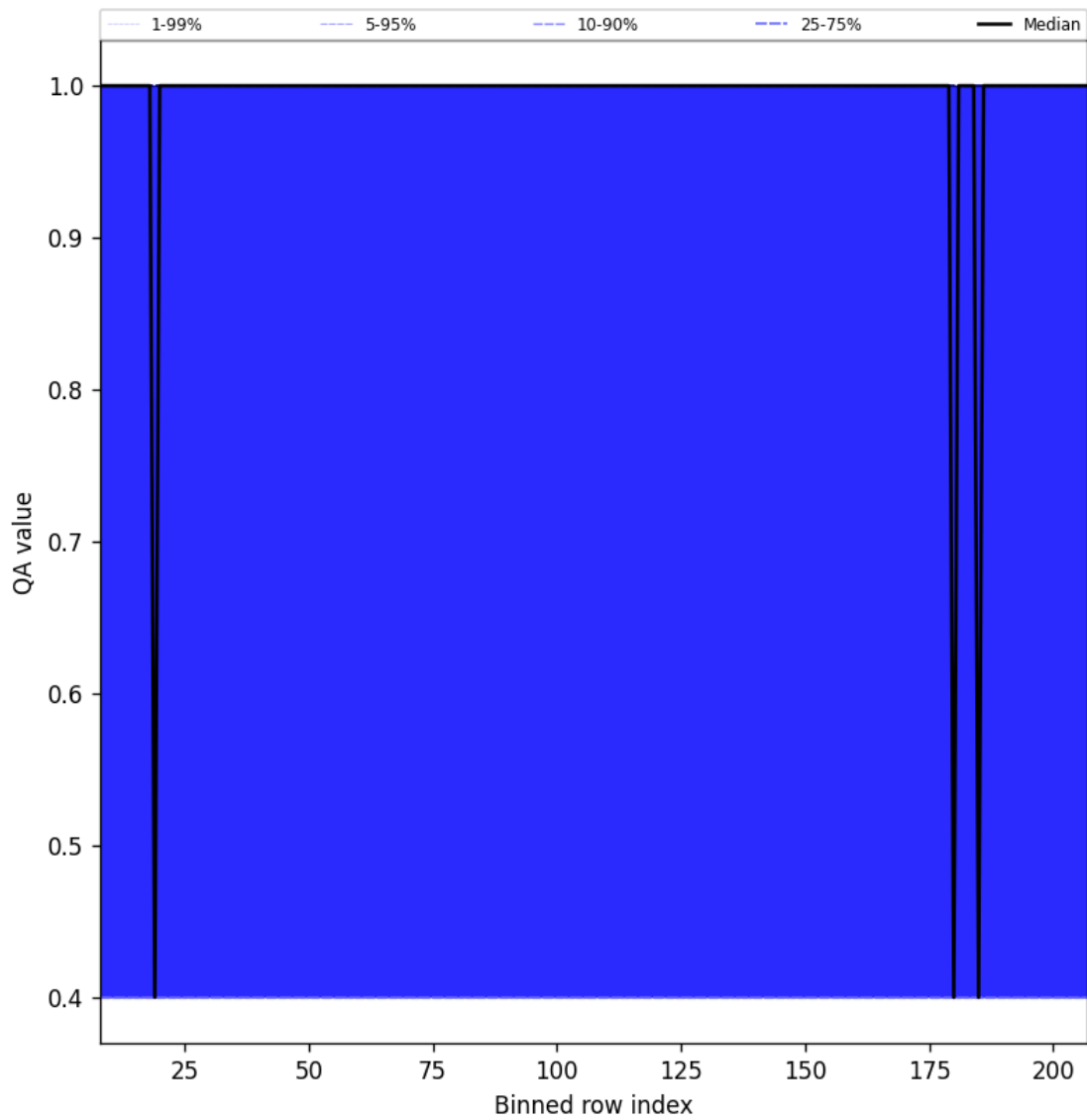
Figure 33: Along track statistics of “QA value” for 2025-01-23 to 2025-01-24
