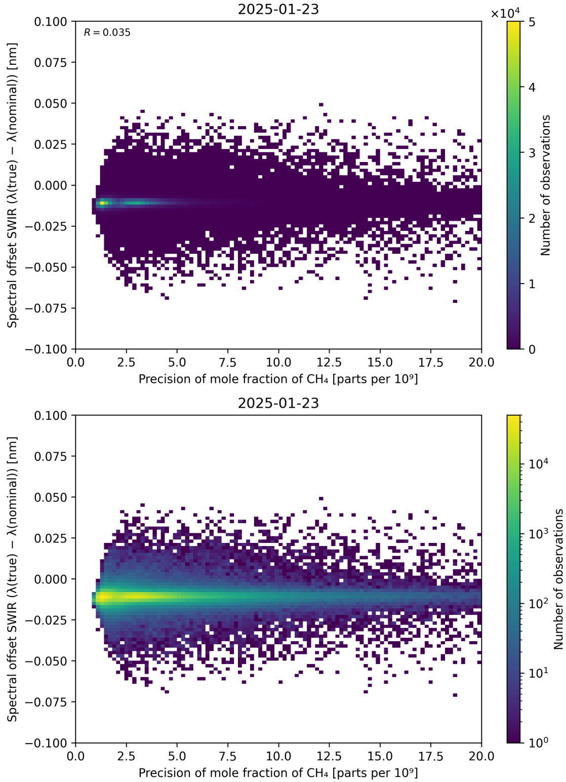
Figure 85: Scatter density plot of “Precision of mole fraction of \text{CH}_4 ” against “Spectral offset SWIR ( \lambda_{\text{true}} - \lambda_{\text{nominal}} )” for 2025-01-23 to 2025-01-24.
