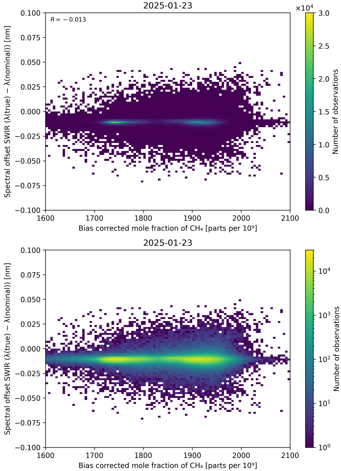
Figure 69: Scatter density plot of “Bias corrected mole fraction of \text{CH}_4 ” against “Spectral offset SWIR ( \lambda_{\text{true}} - \lambda_{\text{nominal}} )” for 2025-01-23 to 2025-01-24.
