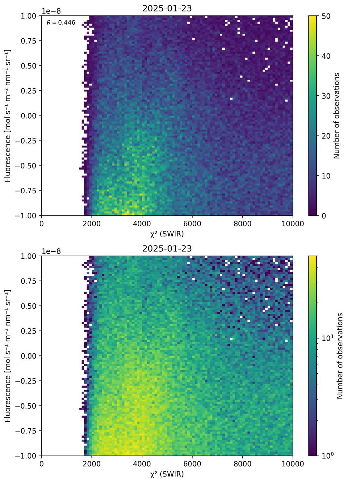
Figure 49: Scatter density plot of “ \chi^2 (SWIR)” against “Fluorescence” for 2025-01-23 to 2025-01-24.
