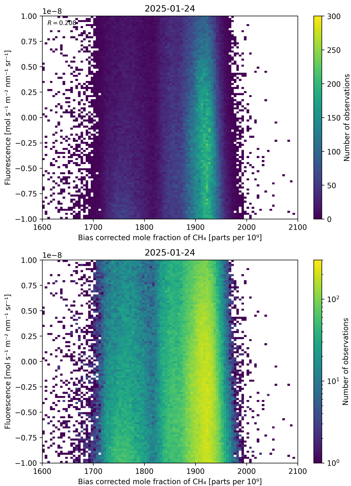
Figure 66: Scatter density plot of “Bias corrected mole fraction of \text{CH}_4 ” against “Fluorescence” for 2025-01-23 to 2025-01-25.
