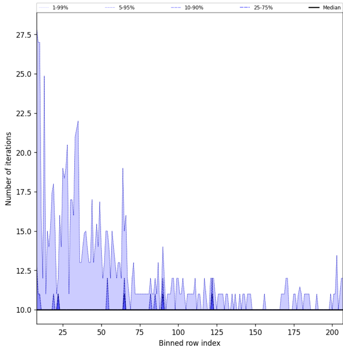
Figure 42: Along track statistics of “Number of iterations” for 2025-01-23 to 2025-01-25
