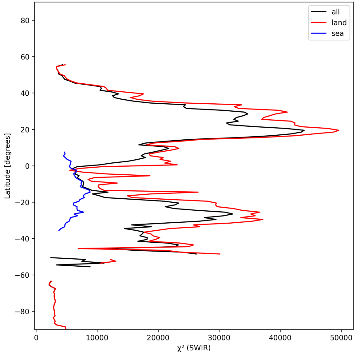
Figure 17: Zonal average of “ \chi^2 (SWIR)” for 2025-01-23 to 2025-01-25.
