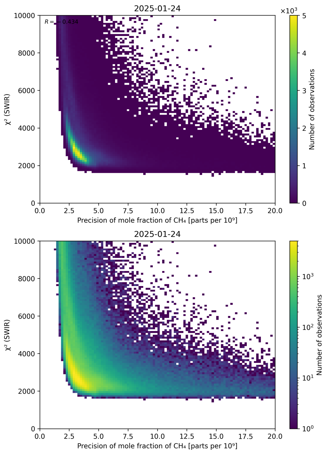
Figure 79: Scatter density plot of “Precision of mole fraction of \text{CH}_4 ” against “ \chi^2 (SWIR)” for 2025-01-23 to 2025-01-25.
