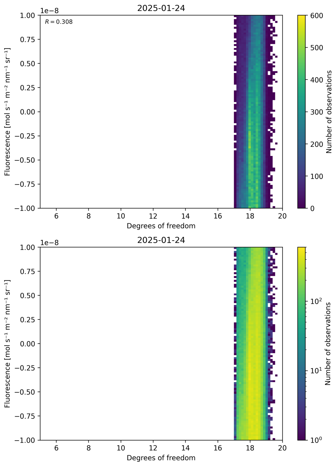
Figure 51: Scatter density plot of “Degrees of freedom” against “Fluorescence” for 2025-01-23 to 2025-01-25.
