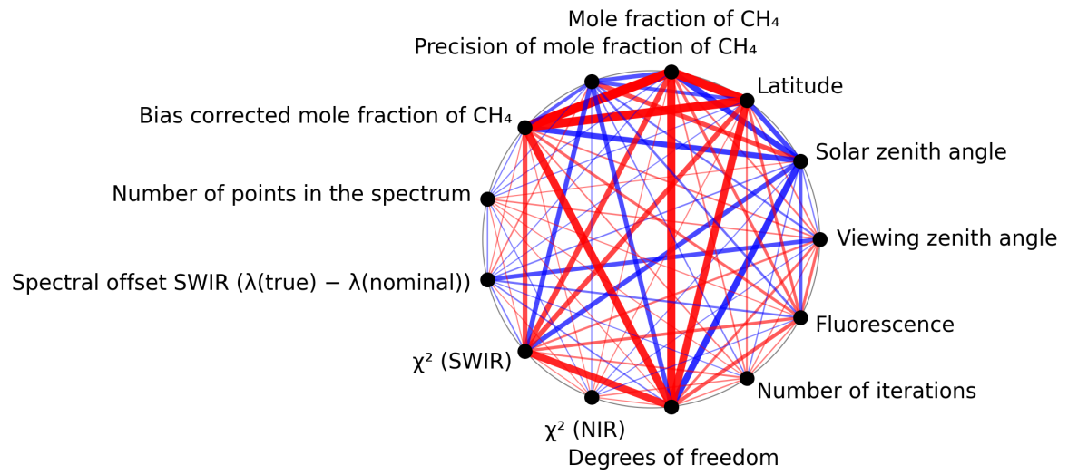
Figure 1: Map of correlation graph for 2025-01-23 to 2025-01-25.
