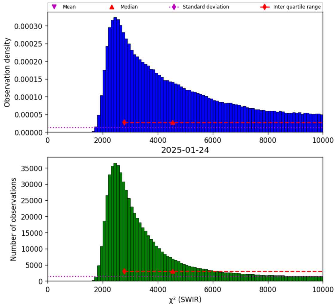
Figure 28: Histogram of “ \chi^2 (SWIR)” for 2025-01-23 to 2025-01-25
