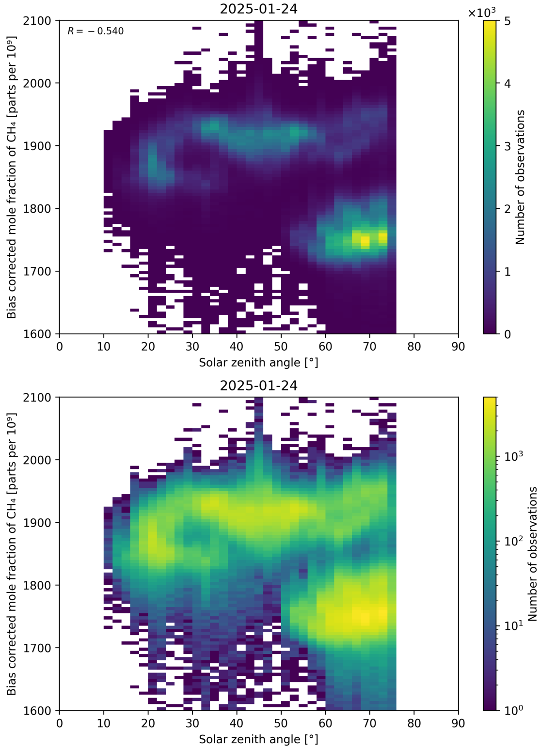
Figure 100: Scatter density plot of “Solar zenith angle” against “Bias corrected mole fraction of \text{CH}_4 ” for 2025-01-23 to 2025-01-25.
