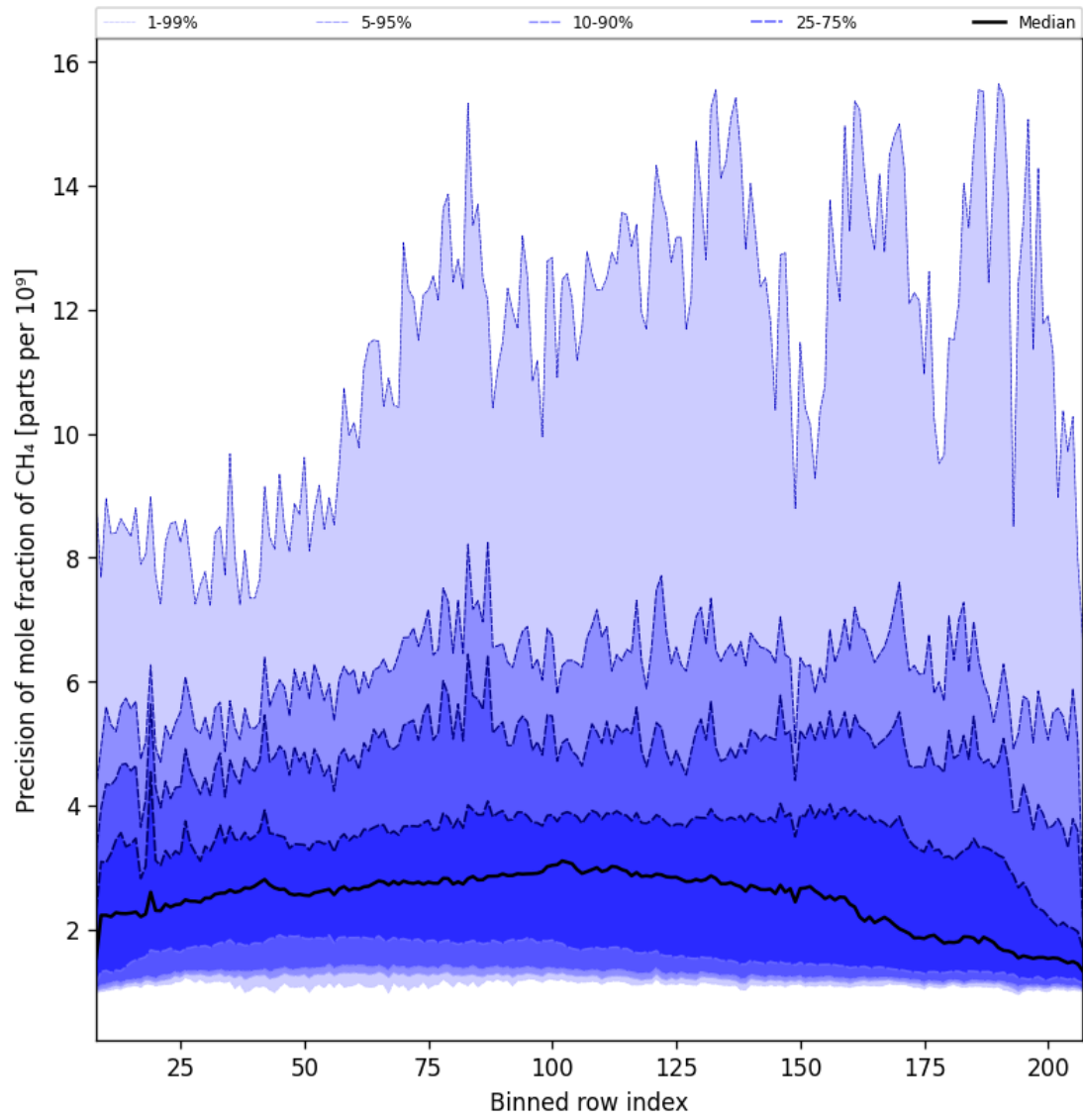
Figure 35: Along track statistics of “Precision of mole fraction of CH 4 ” for 2025-01-23 to 2025-01-25
