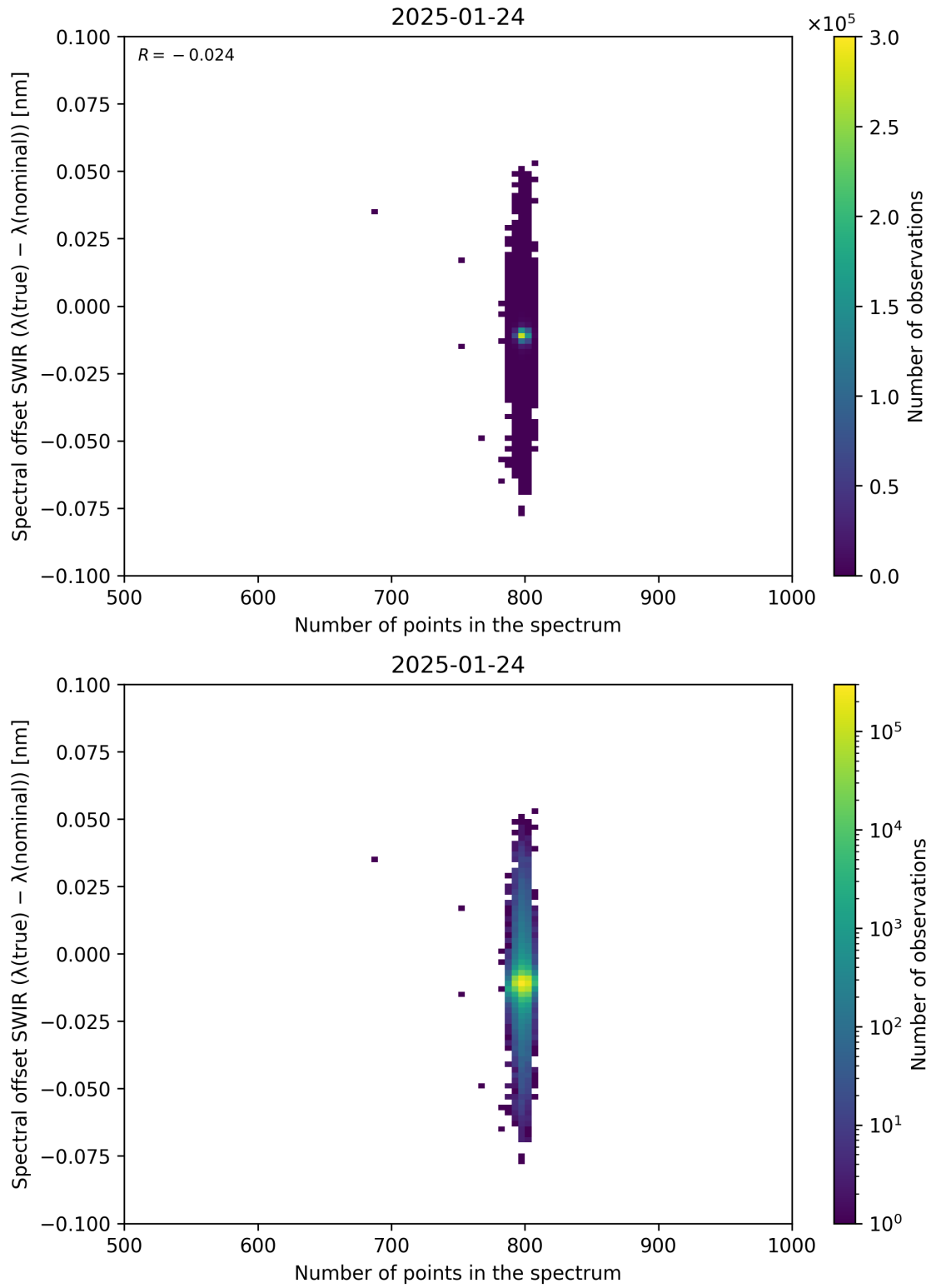
Figure 93: Scatter density plot of “Number of points in the spectrum” against “Spectral offset SWIR ( \lambda_{\text{true}} - \lambda_{\text{nominal}} )” for 2025-01-23 to 2025-01-25.
