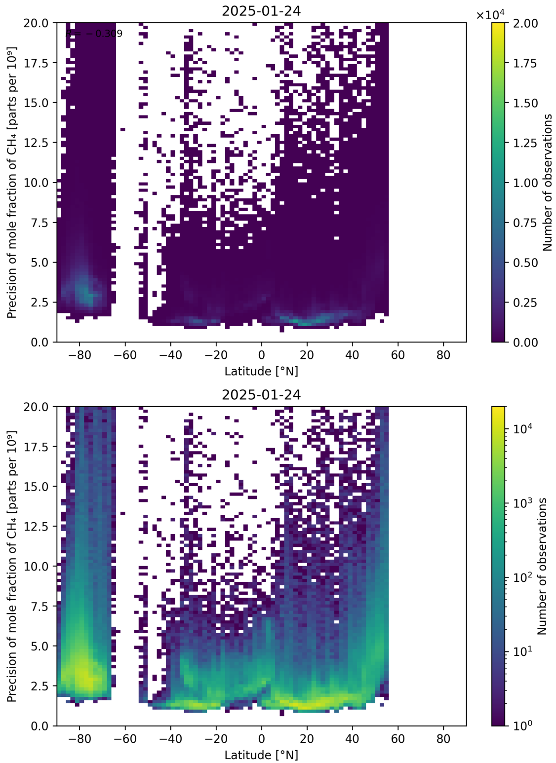
Figure 59: Scatter density plot of “Latitude” against “Precision of mole fraction of CH 4 ” for 2025-01-23 to 2025-01-25.
