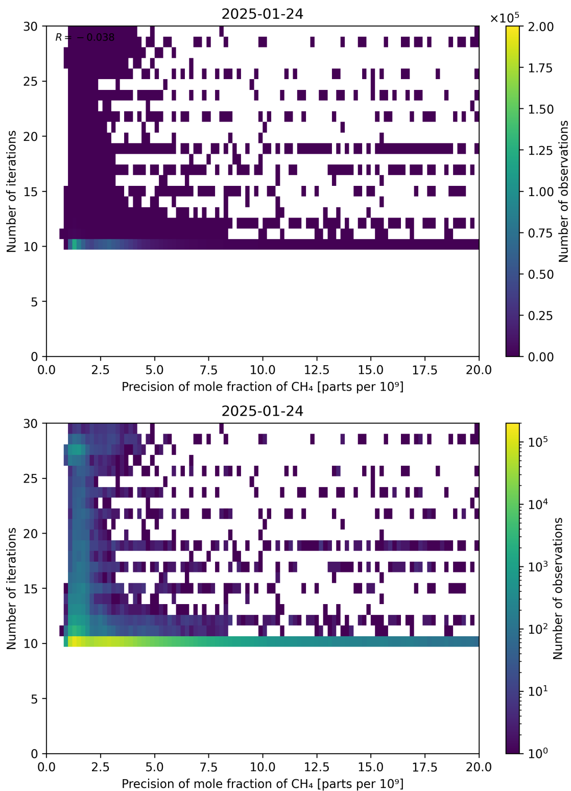
Figure 83: Scatter density plot of “Precision of mole fraction of CH 4 ” against “Number of iterations” for 2025-01-23 to 2025-01-25.
