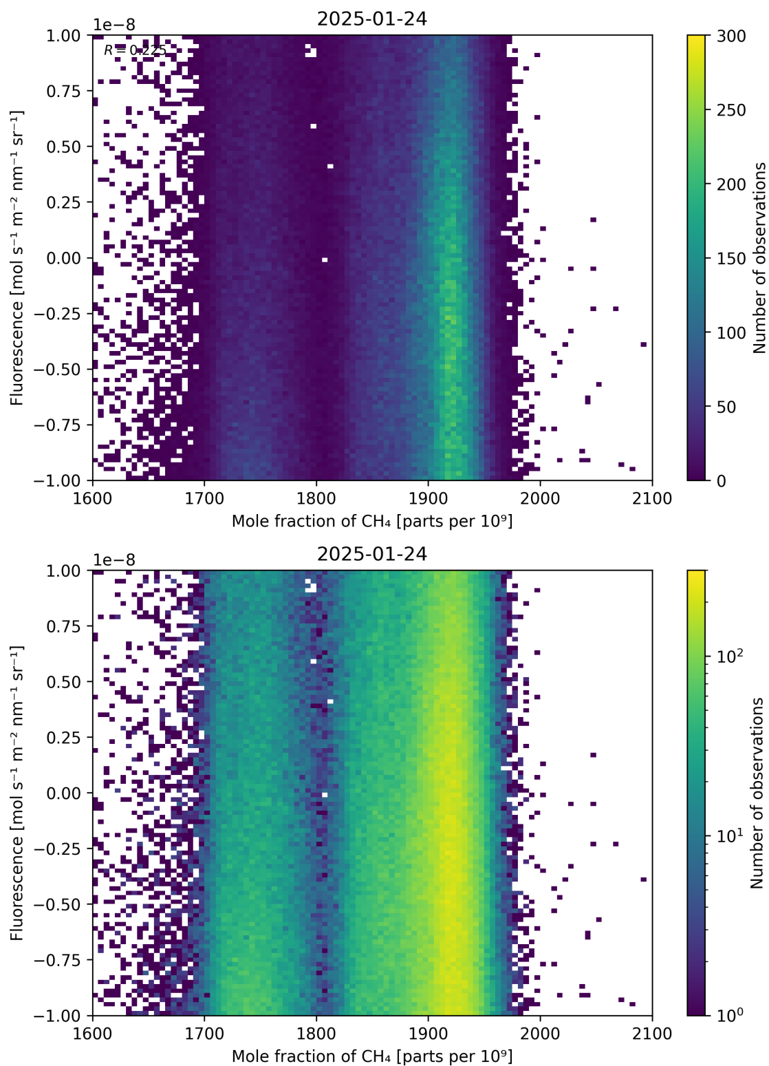
Figure 73: Scatter density plot of “Mole fraction of \text{CH}_4 ” against “Fluorescence” for 2025-01-23 to 2025-01-25.
