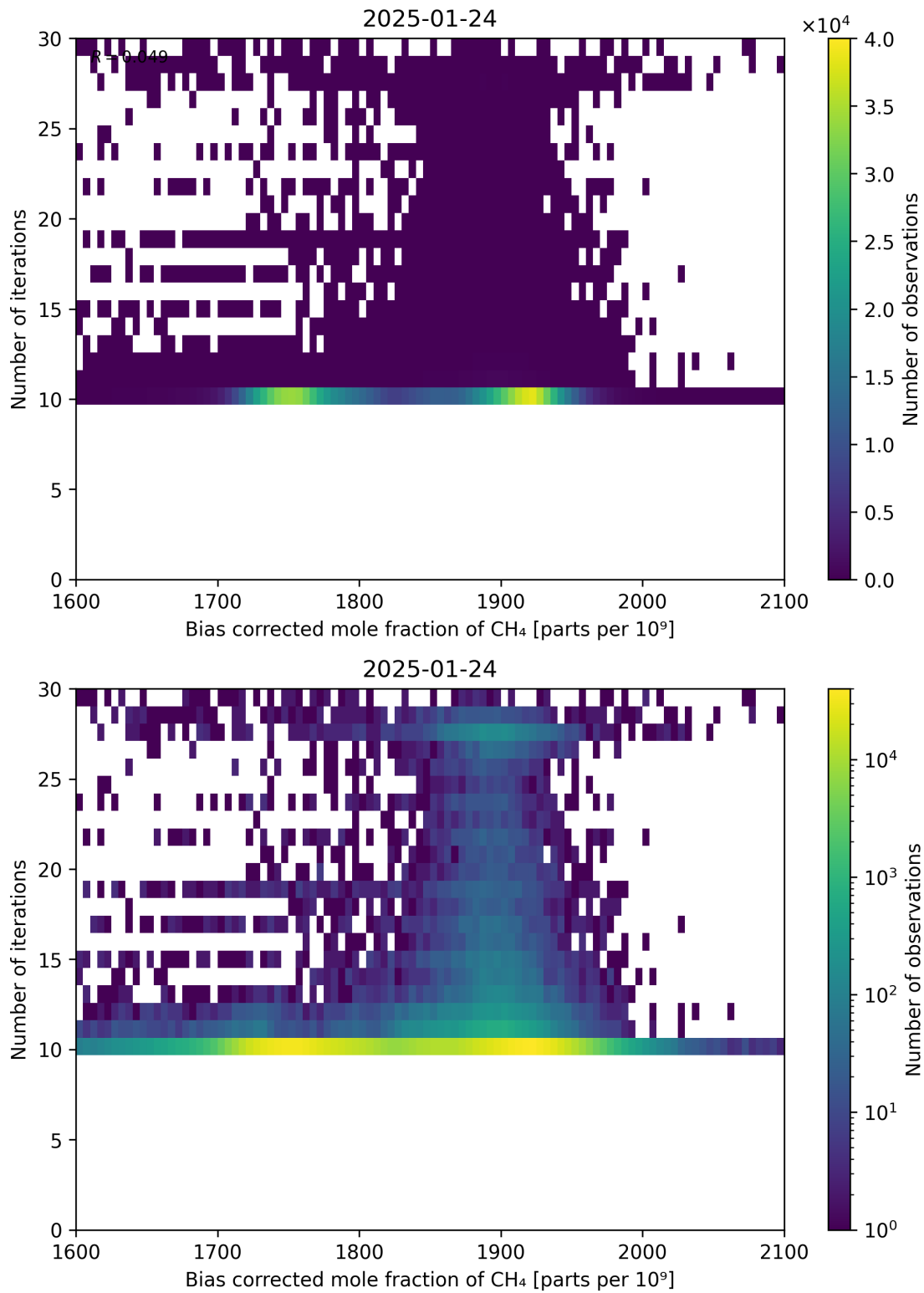
Figure 67: Scatter density plot of “Bias corrected mole fraction of CH 4 ” against “Number of iterations” for 2025-01-23 to 2025-01-25.
