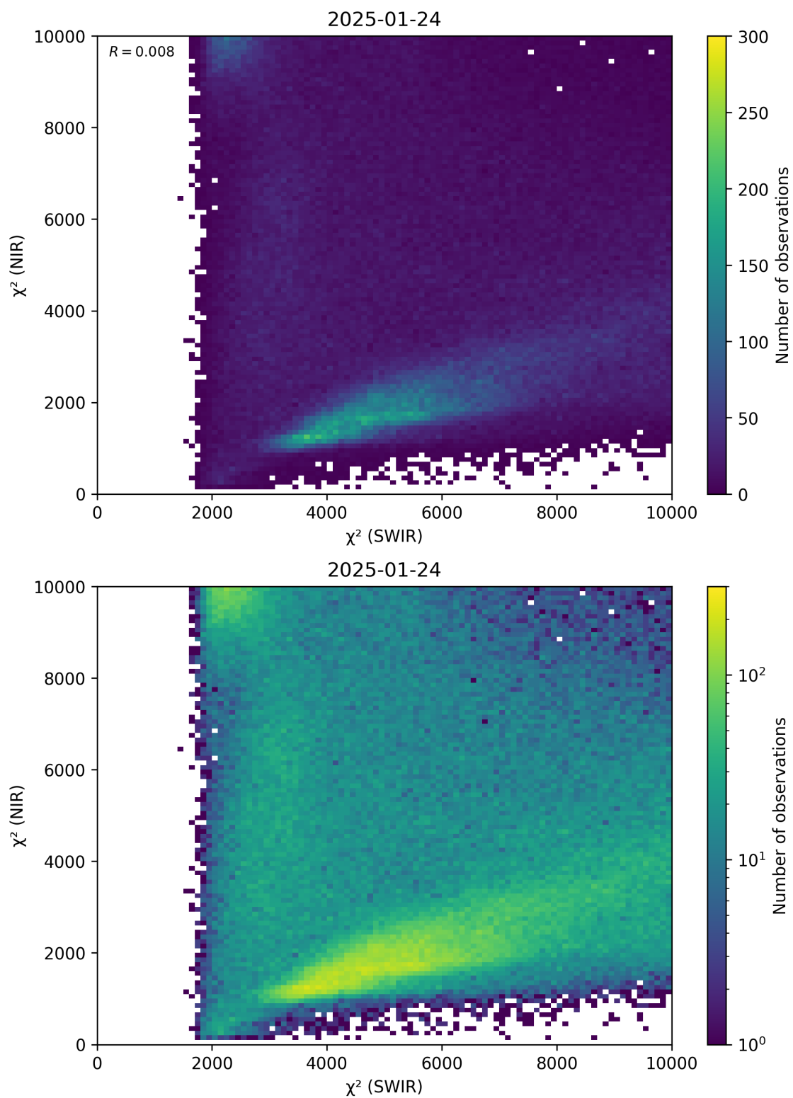
Figure 47: Scatter density plot of “ \chi^2 (SWIR)” against “ \chi^2 (NIR)” for 2025-01-23 to 2025-01-25.
