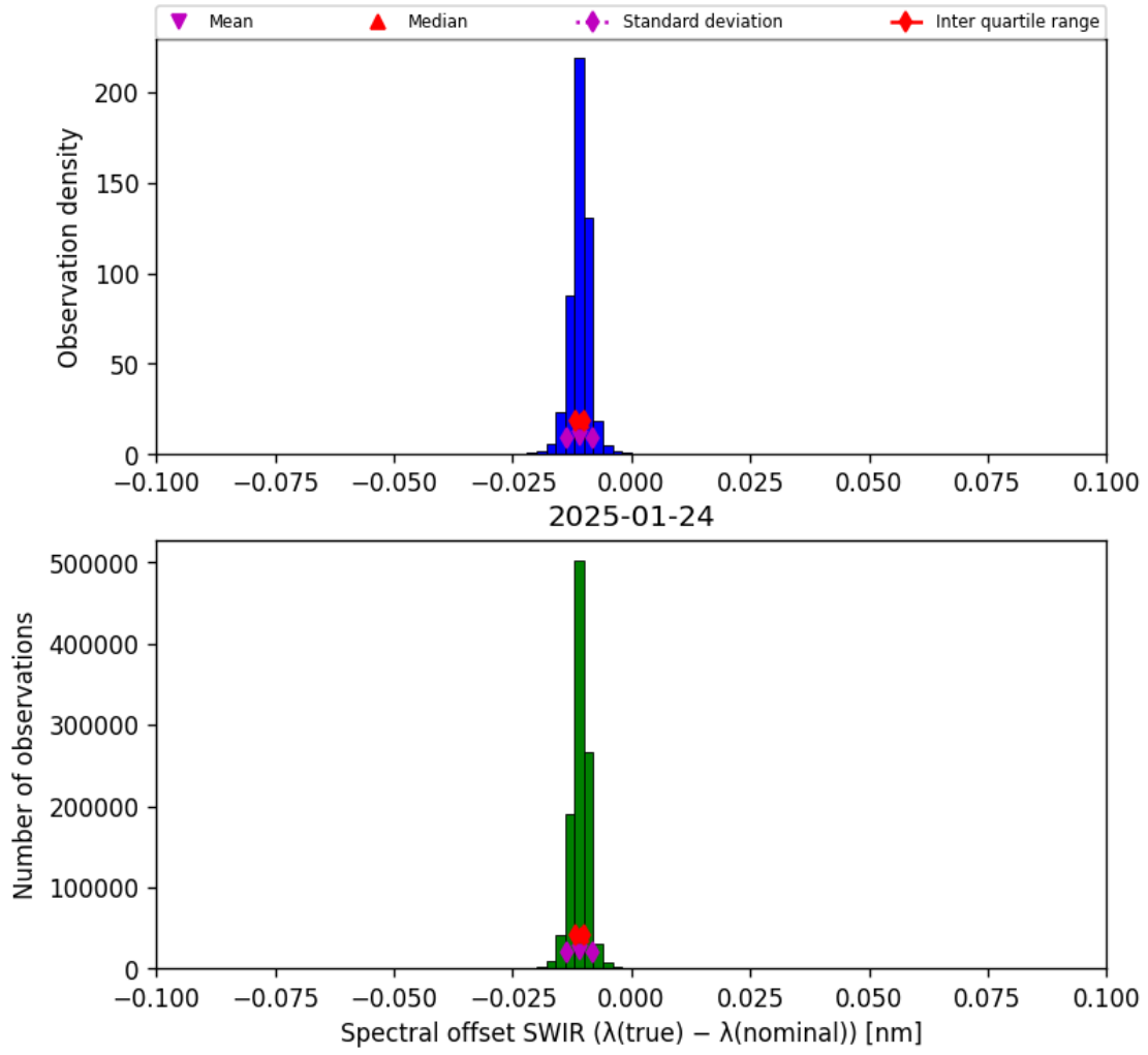
Figure 27: Histogram of “Spectral offset SWIR ( \lambda_{\text{true}} - \lambda_{\text{nominal}} )” for 2025-01-23 to 2025-01-25
