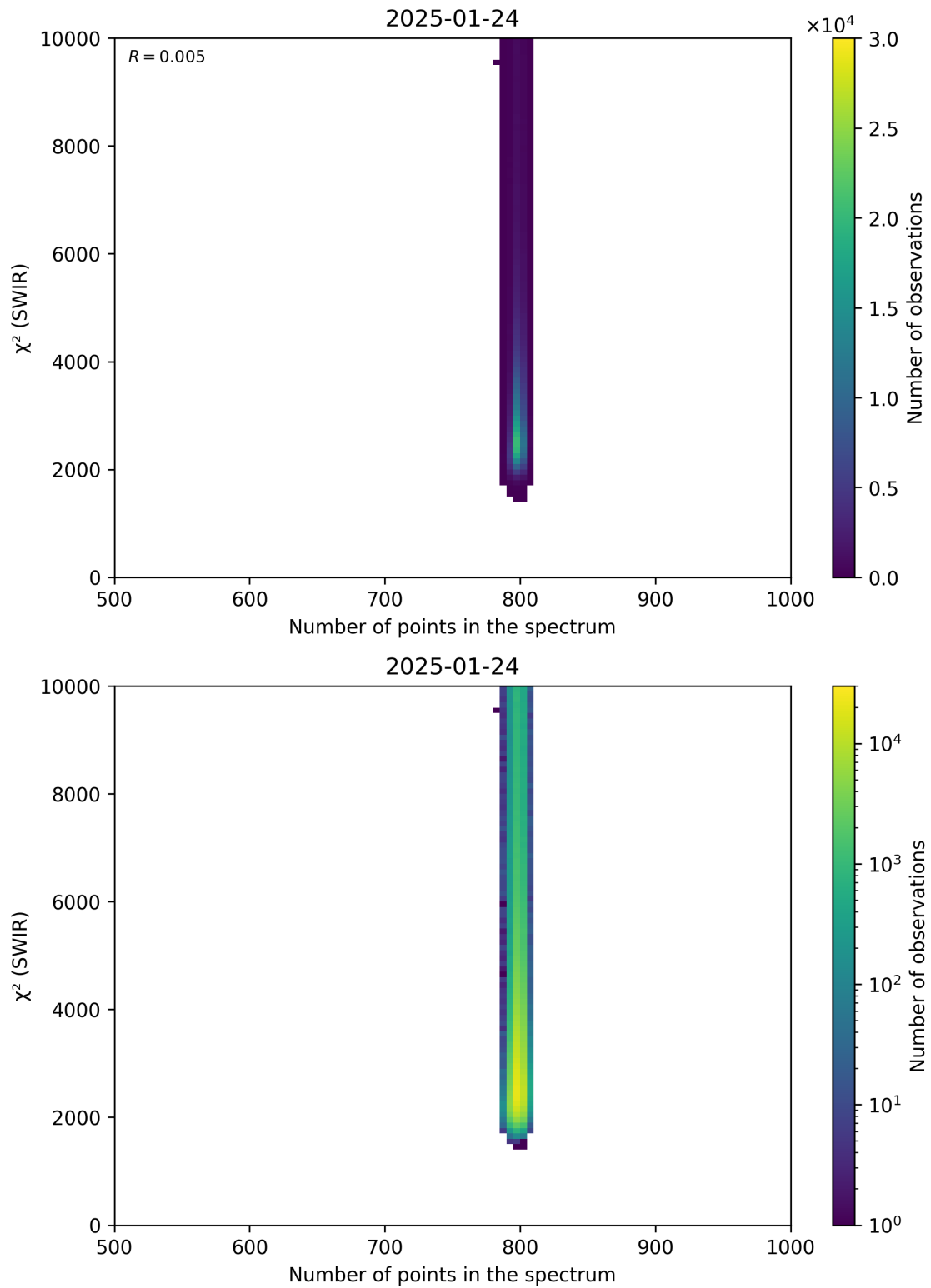
Figure 89: Scatter density plot of “Number of points in the spectrum” against “ \chi^2 (SWIR)” for 2025-01-23 to 2025-01-25.
