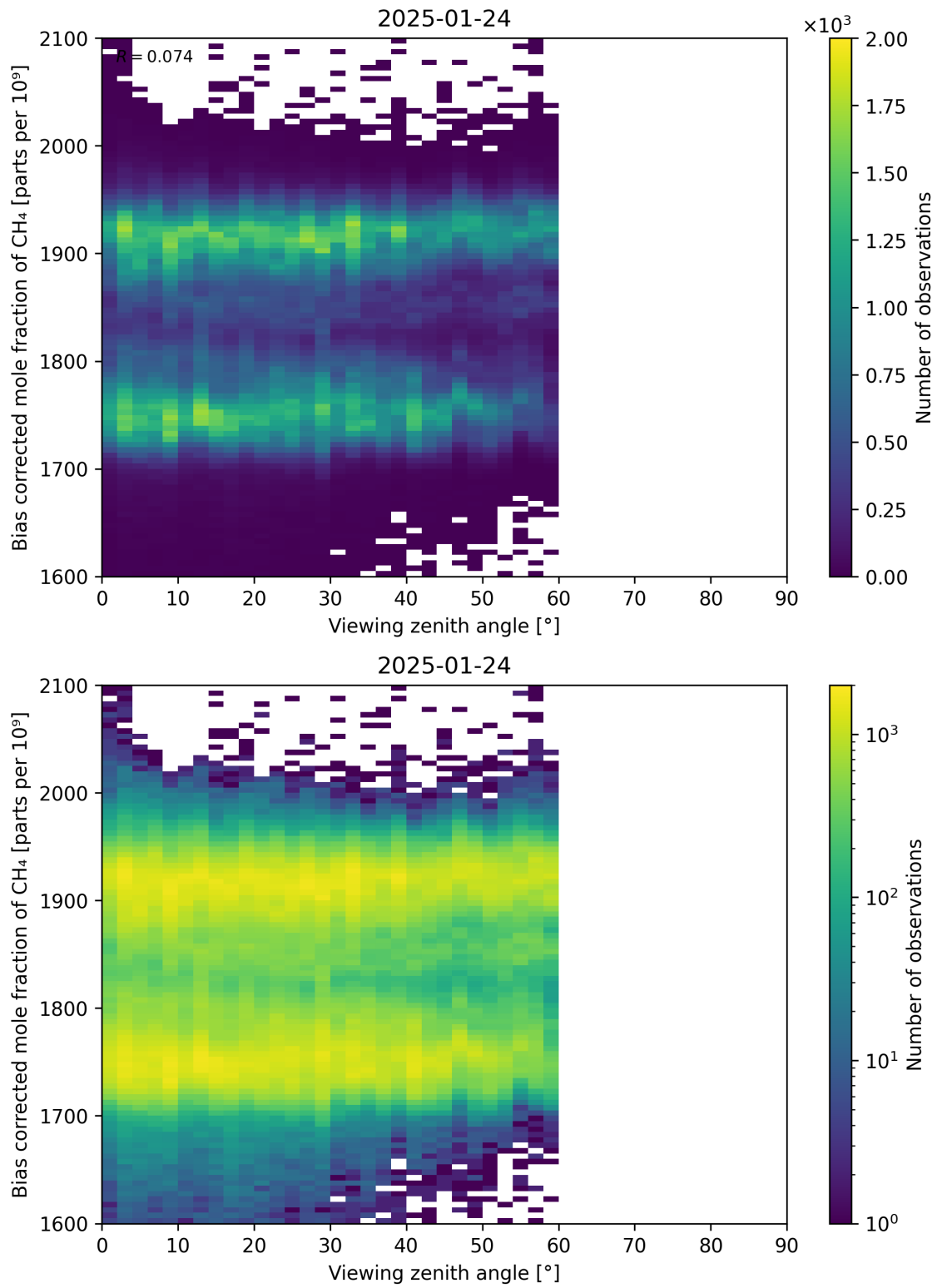
Figure 111: Scatter density plot of “Viewing zenith angle” against “Bias corrected mole fraction of CH 4 ” for 2025-01-23 to 2025-01-25.
