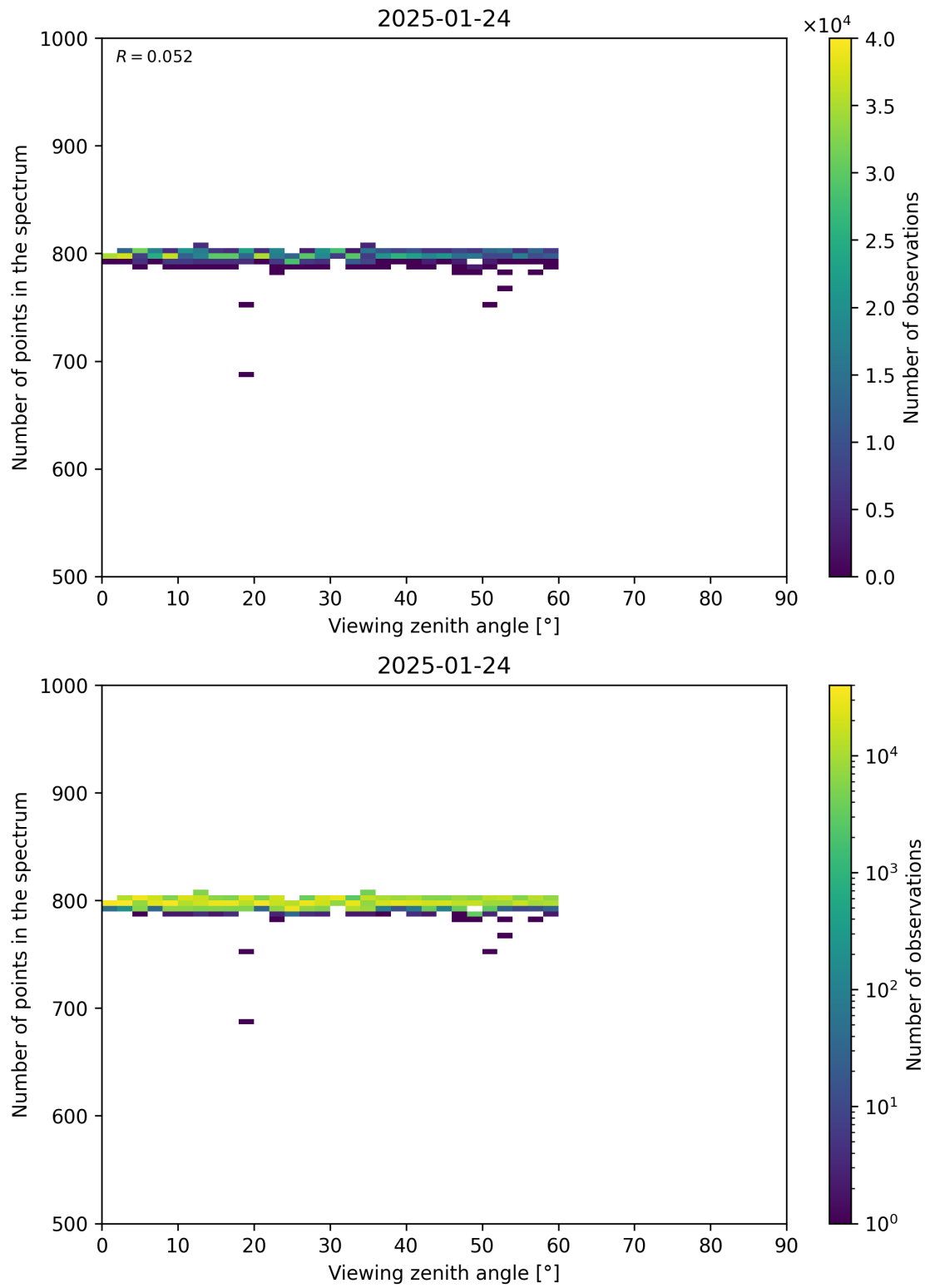
Figure 114: Scatter density plot of “Viewing zenith angle” against “Number of points in the spectrum” for 2025-01-23 to 2025-01-25.
