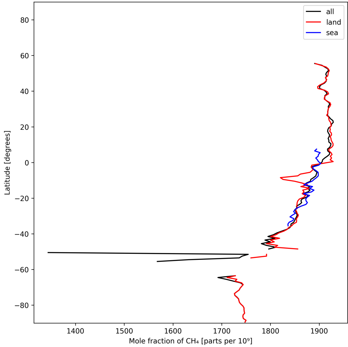
Figure 12: Zonal average of “Mole fraction of \text{CH}_4 ” for 2025-01-23 to 2025-01-25.
