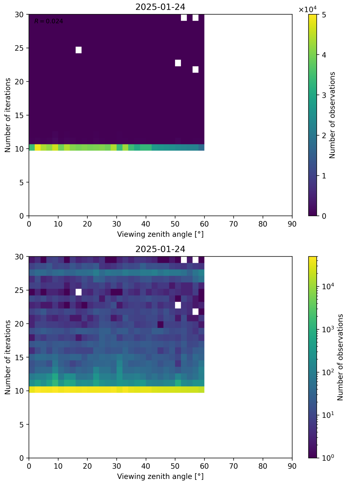
Figure 113: Scatter density plot of “Viewing zenith angle” against “Number of iterations” for 2025-01-23 to 2025-01-25.
