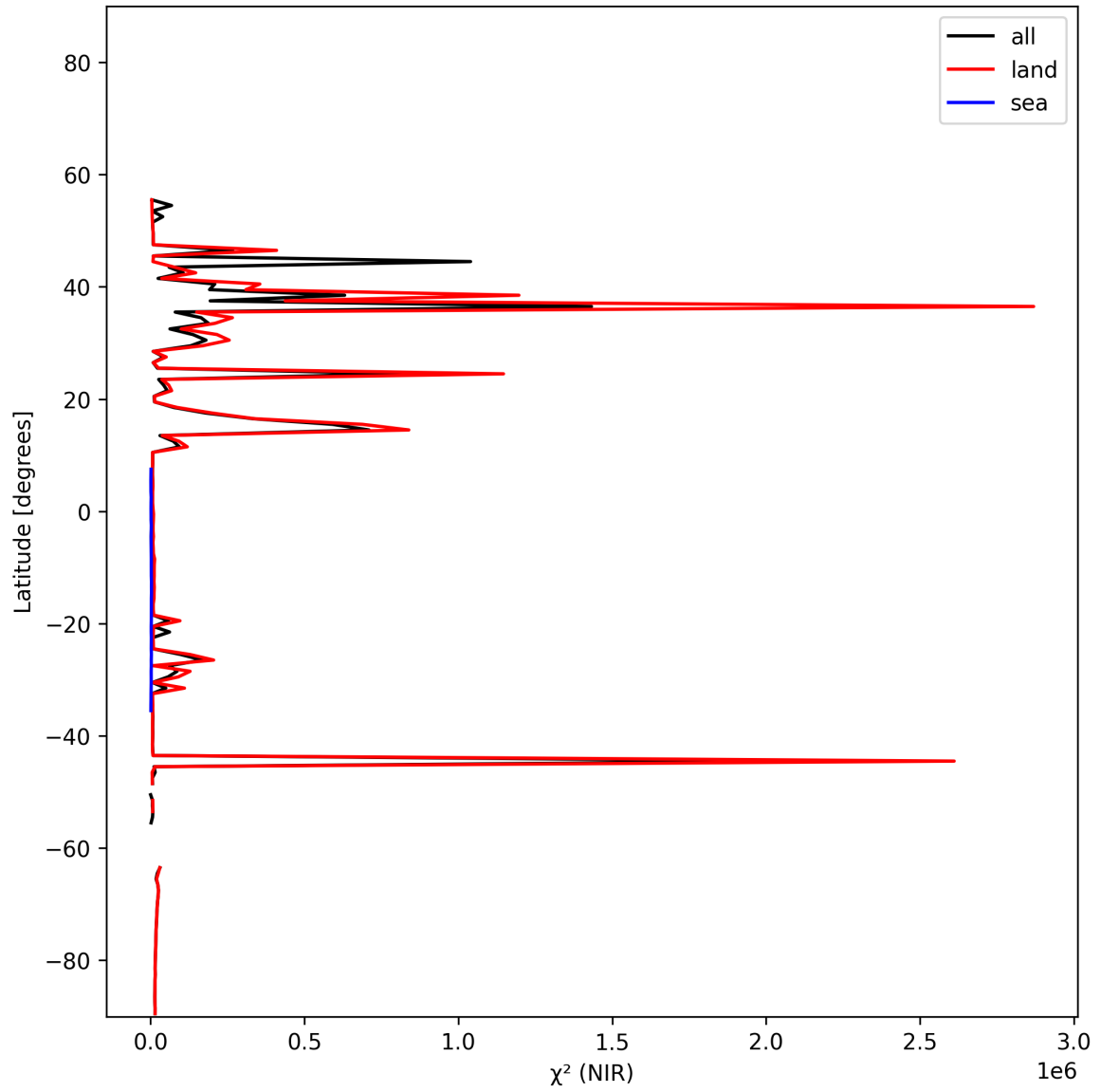
Figure 18: Zonal average of “ \chi^2 (NIR)” for 2025-01-23 to 2025-01-25.
