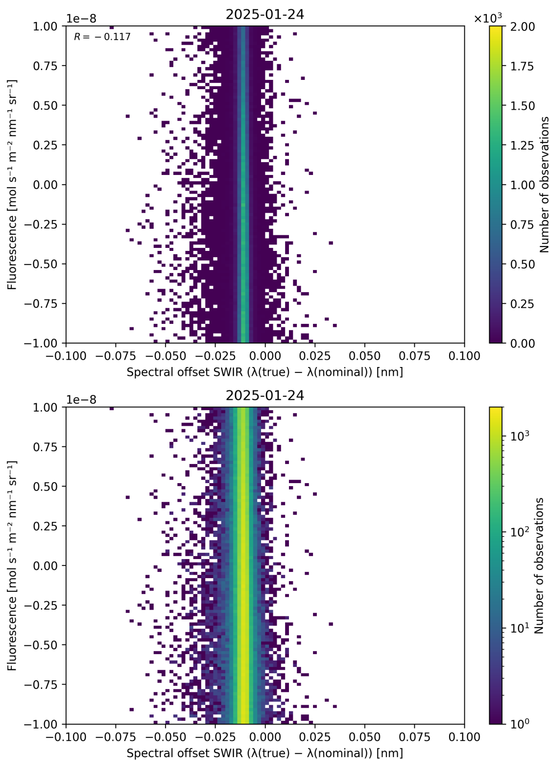
Figure 120: Scatter density plot of “Spectral offset SWIR ( \lambda_{\text{true}} - \lambda_{\text{nominal}} )” against “Fluorescence” for 2025-01-23 to 2025-01-25.
