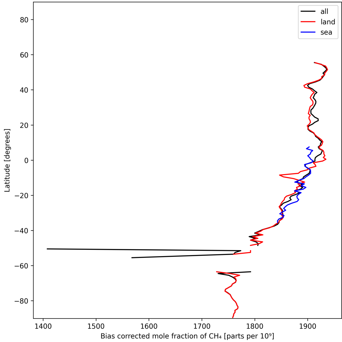
Figure 14: Zonal average of “Bias corrected mole fraction of CH 4 ” for 2025-01-23 to 2025-01-25.
