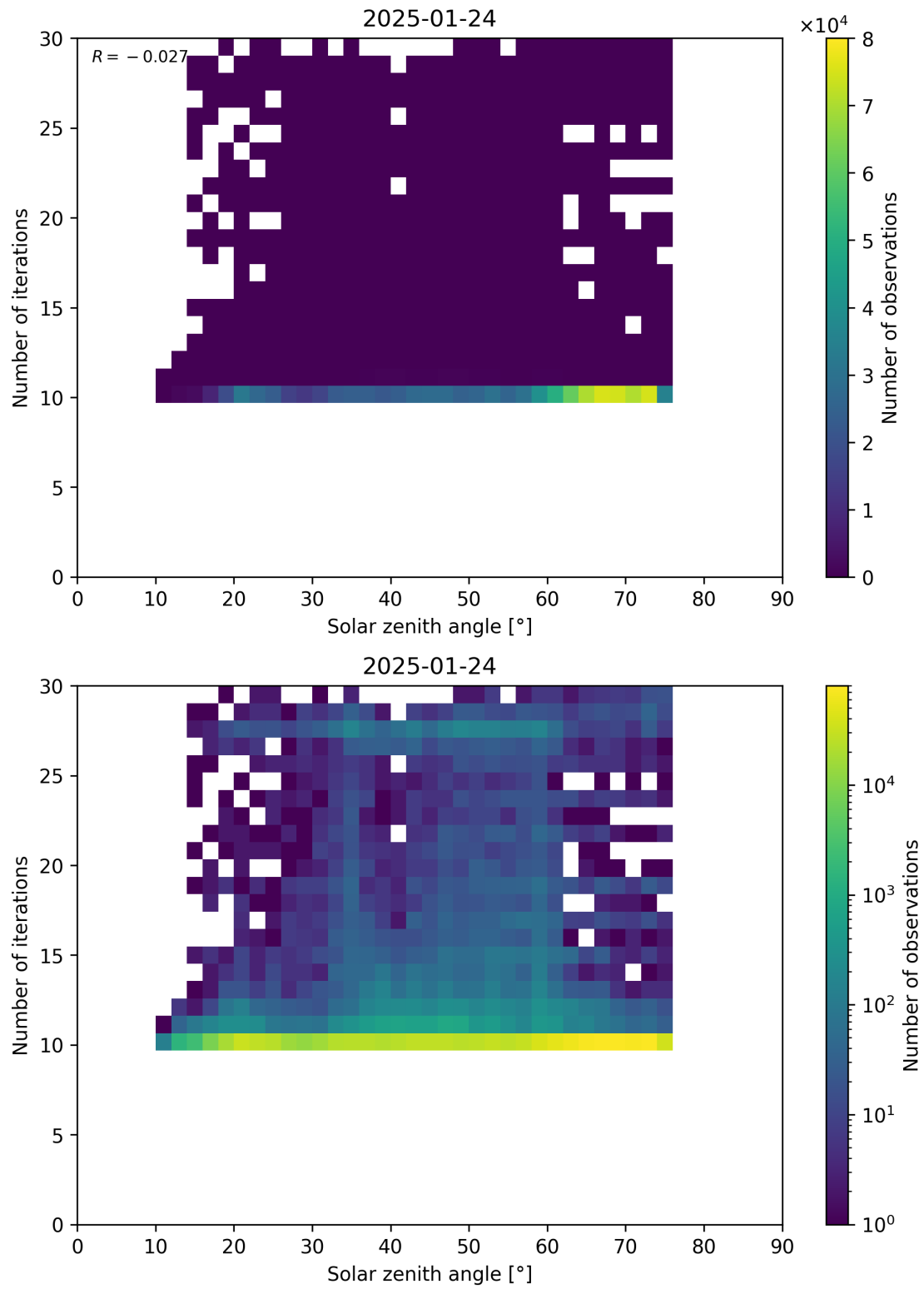
Figure 102: Scatter density plot of “Solar zenith angle” against “Number of iterations” for 2025-01-23 to 2025-01-25.
