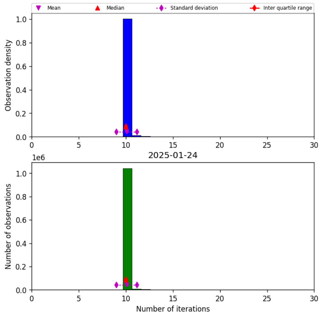
Figure 31: Histogram of "Number of iterations" for 2025-01-23 to 2025-01-25
