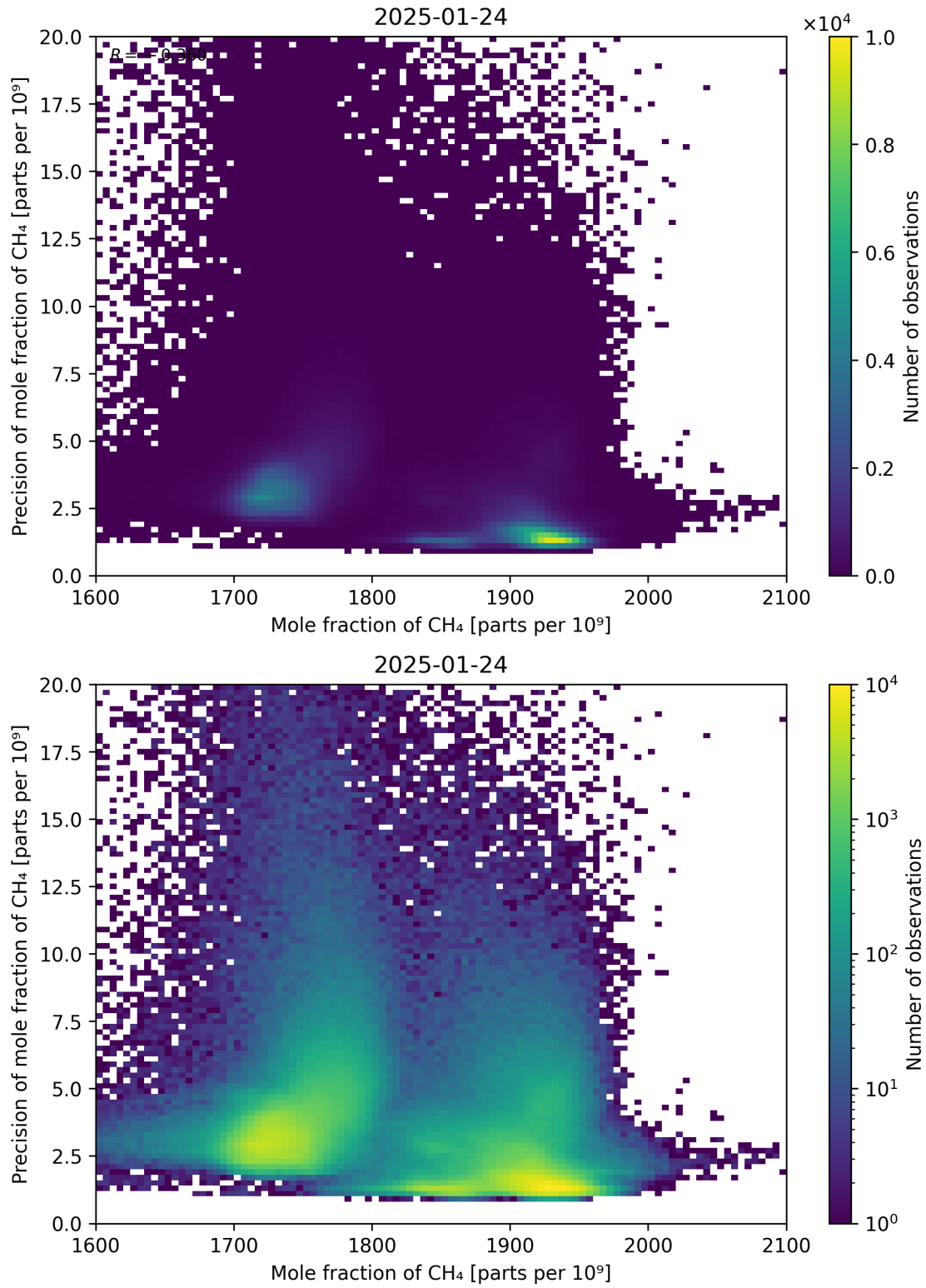
Figure 75: Scatter density plot of “Mole fraction of CH 4 ” against “Precision of mole fraction of CH 4 ” for 2025-01-23 to 2025-01-25.
