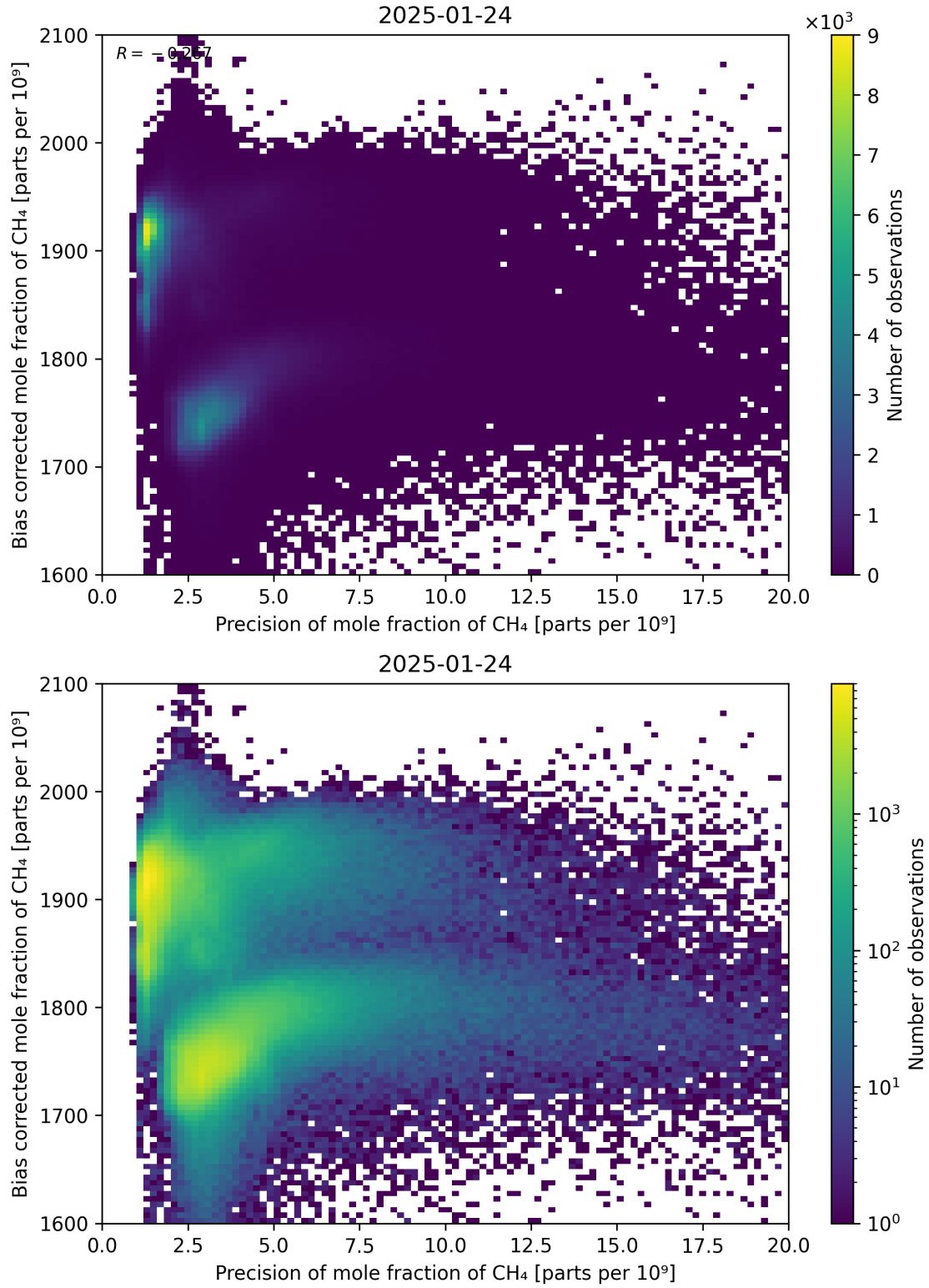
Figure 82: Scatter density plot of “Precision of mole fraction of CH 4 ” against “Bias corrected mole fraction of CH 4 ” for 2025-01-23 to 2025-01-25.
