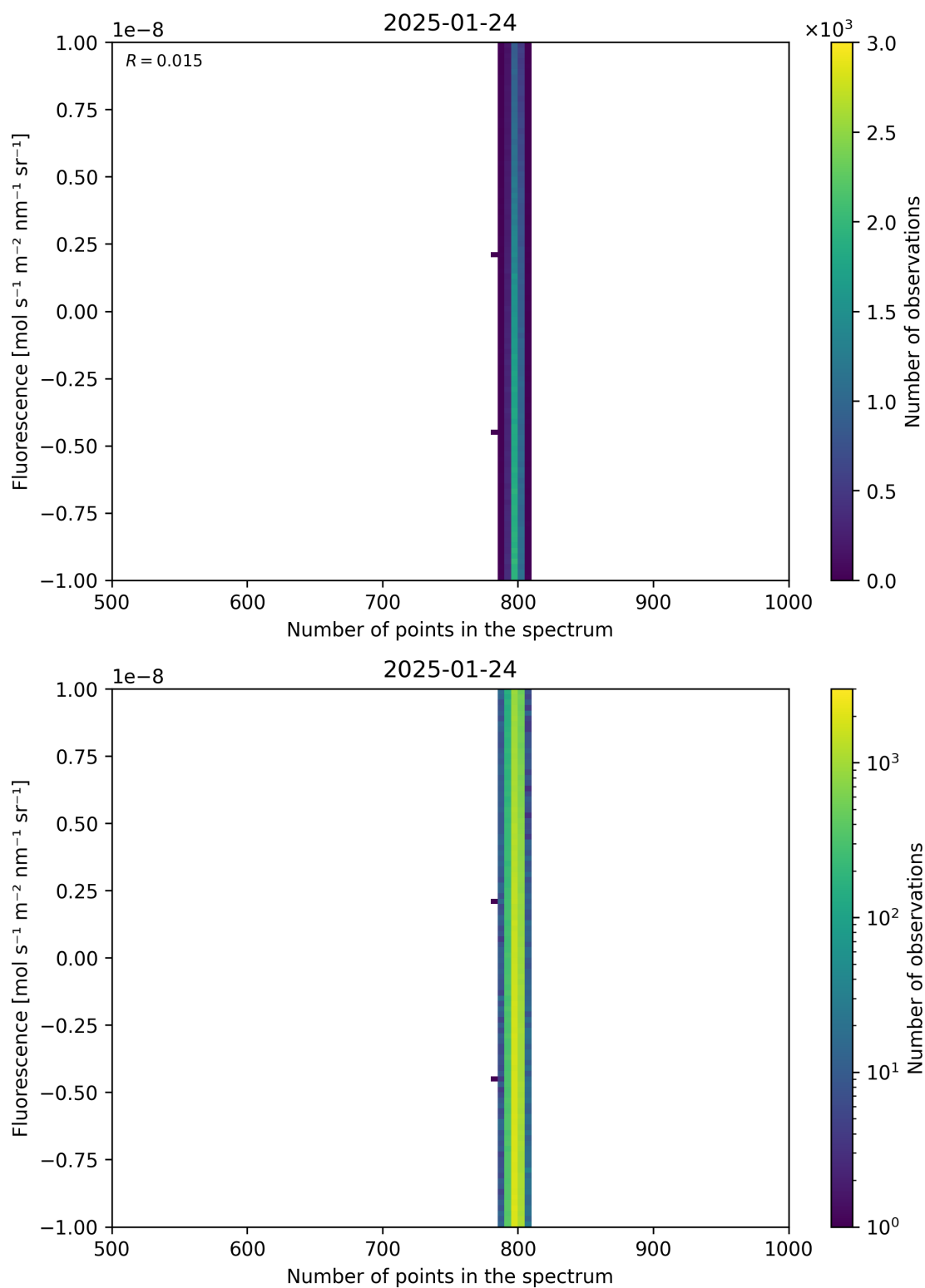
Figure 91: Scatter density plot of “Number of points in the spectrum” against “Fluorescence” for 2025-01-23 to 2025-01-25.
