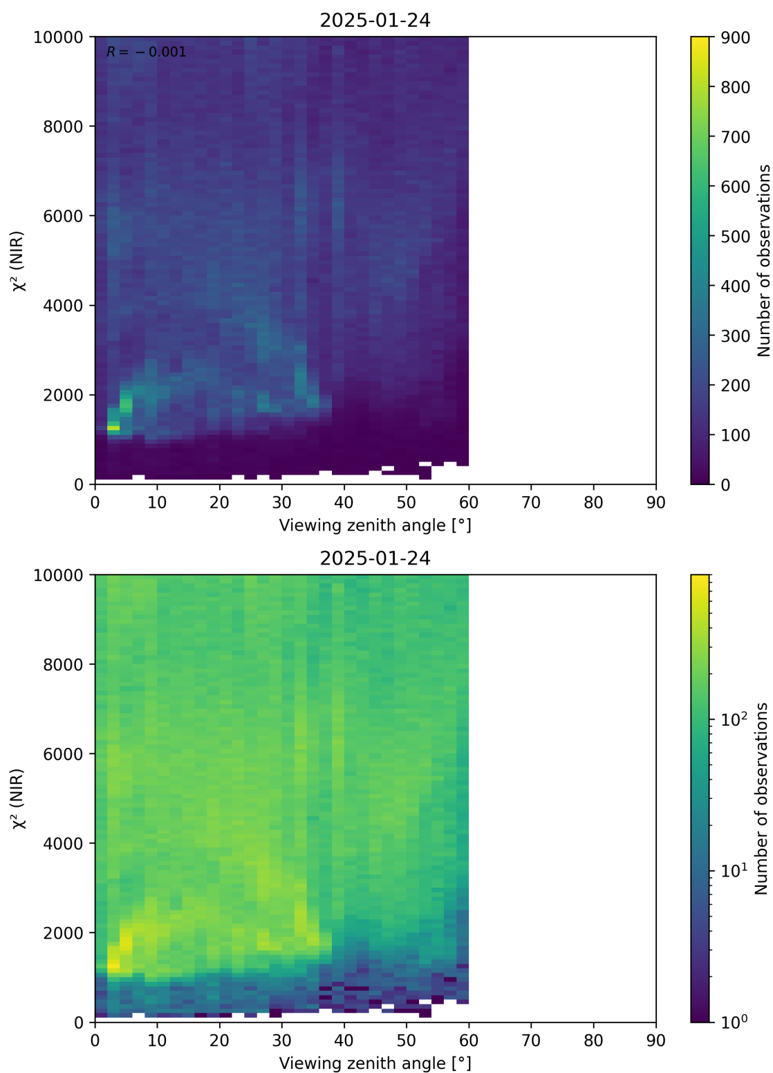
Figure 105: Scatter density plot of “Viewing zenith angle” against “ \chi^2 (NIR)” for 2025-01-23 to 2025-01-25.
