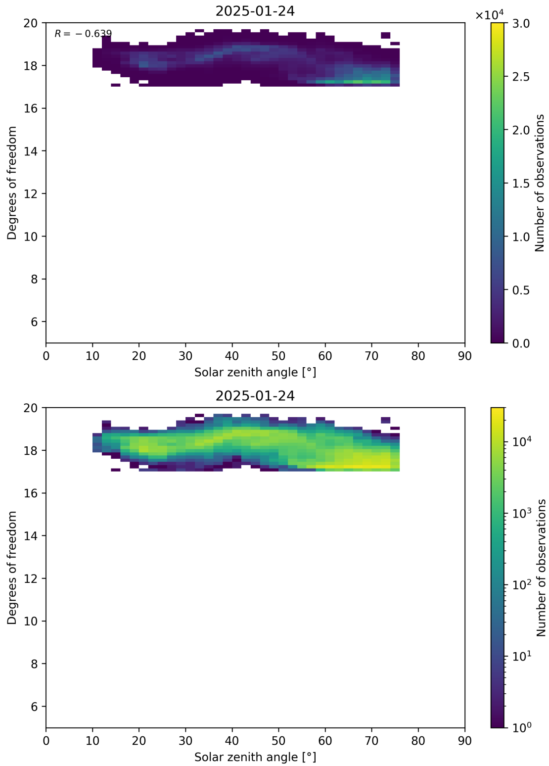
Figure 96: Scatter density plot of “Solar zenith angle” against “Degrees of freedom” for 2025-01-23 to 2025-01-25.
