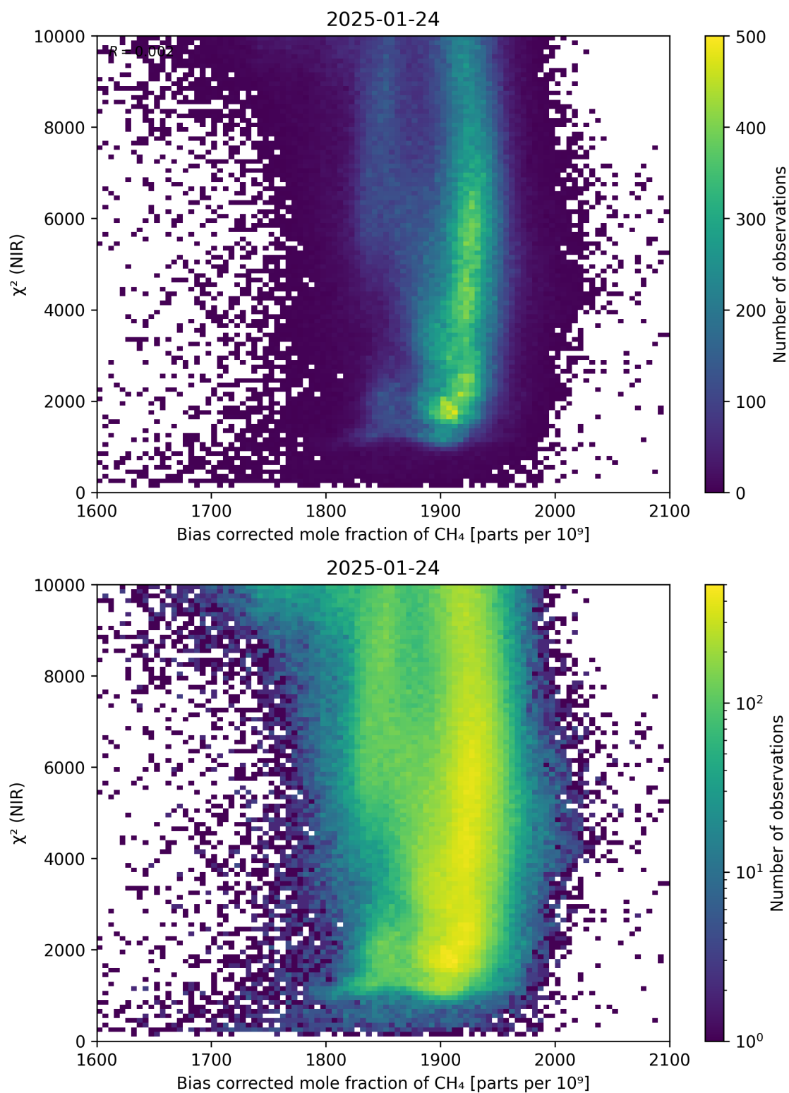
Figure 63: Scatter density plot of “Bias corrected mole fraction of \text{CH}_4 ” against “ \chi^2 (NIR)” for 2025-01-23 to 2025-01-25.
