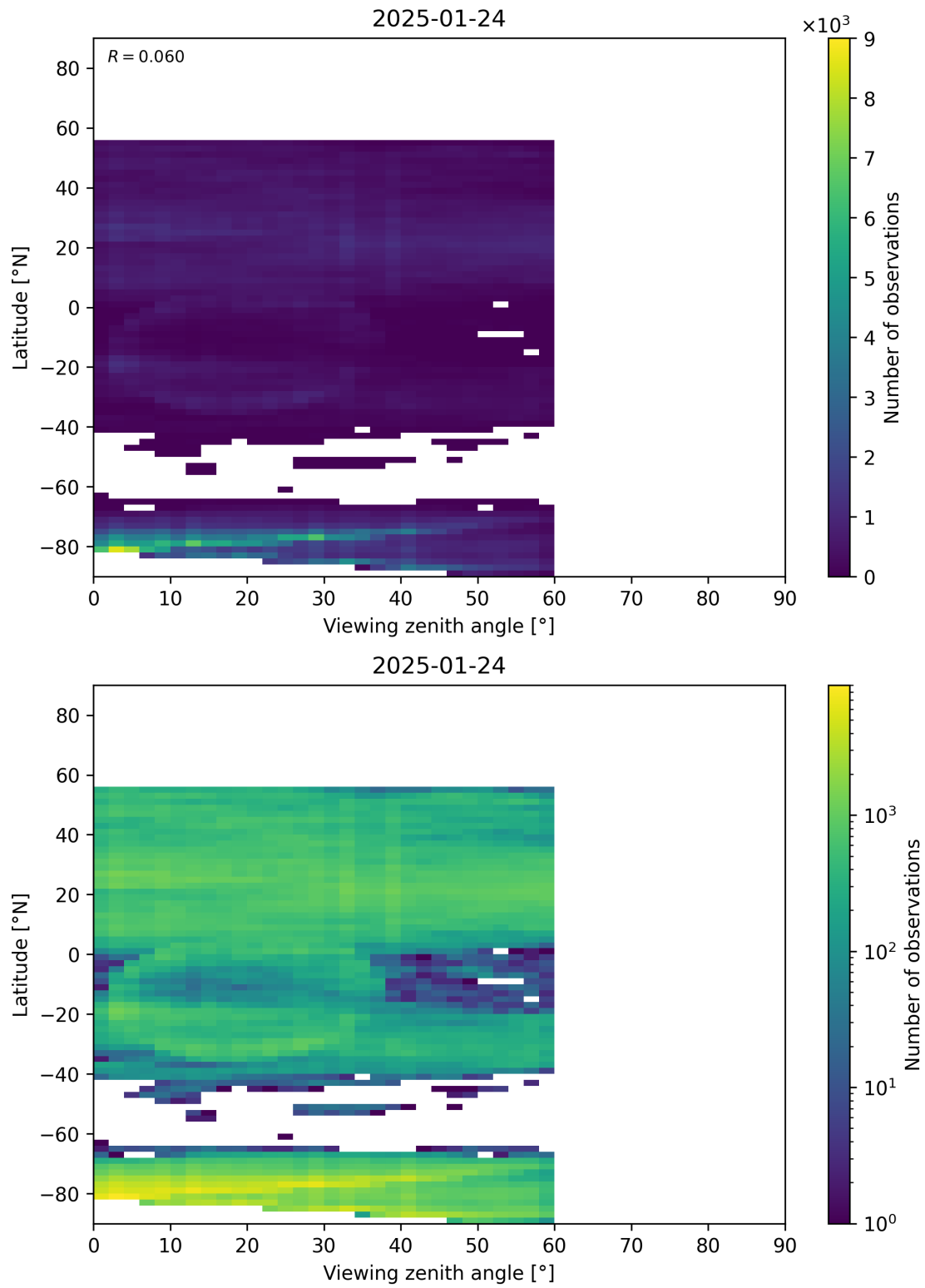
Figure 109: Scatter density plot of “Viewing zenith angle” against “Latitude” for 2025-01-23 to 2025-01-25.
