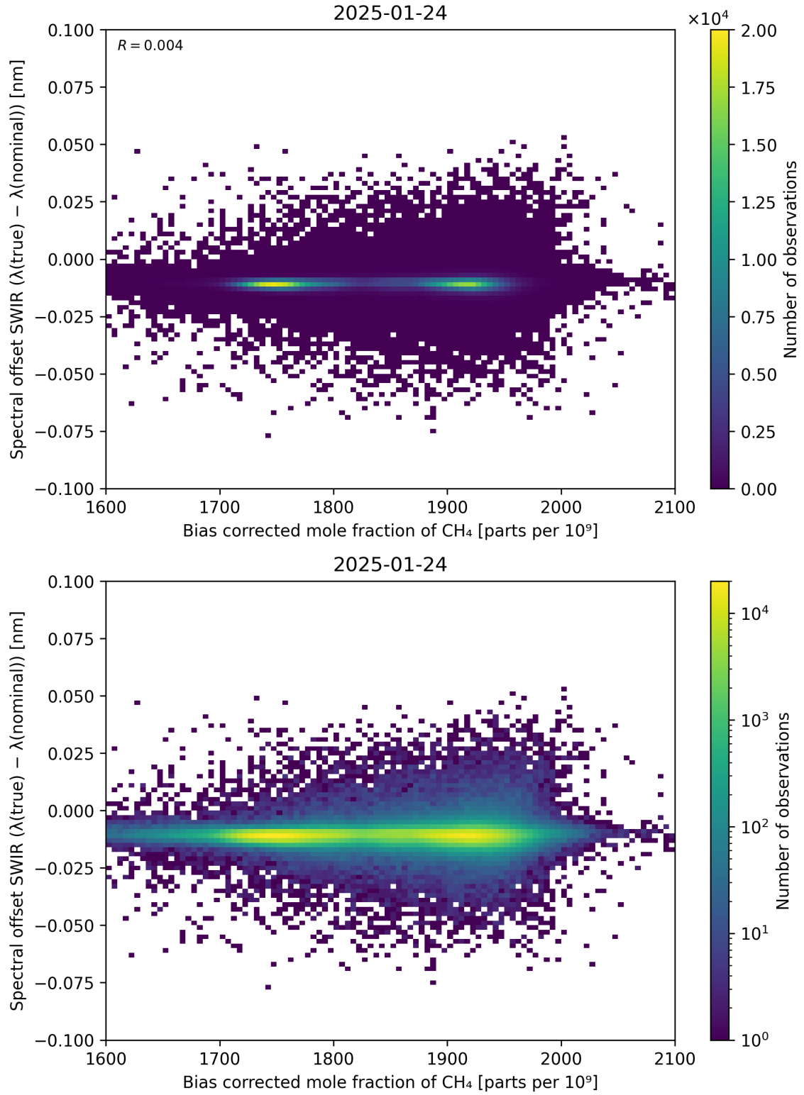
Figure 69: Scatter density plot of “Bias corrected mole fraction of \text{CH}_4 ” against “Spectral offset SWIR ( \lambda_{\text{true}} - \lambda_{\text{nominal}} )” for 2025-01-23 to 2025-01-25.
