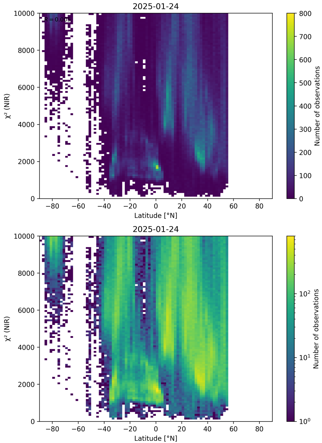
Figure 53: Scatter density plot of “Latitude” against “ \chi^2 (NIR)” for 2025-01-23 to 2025-01-25.
