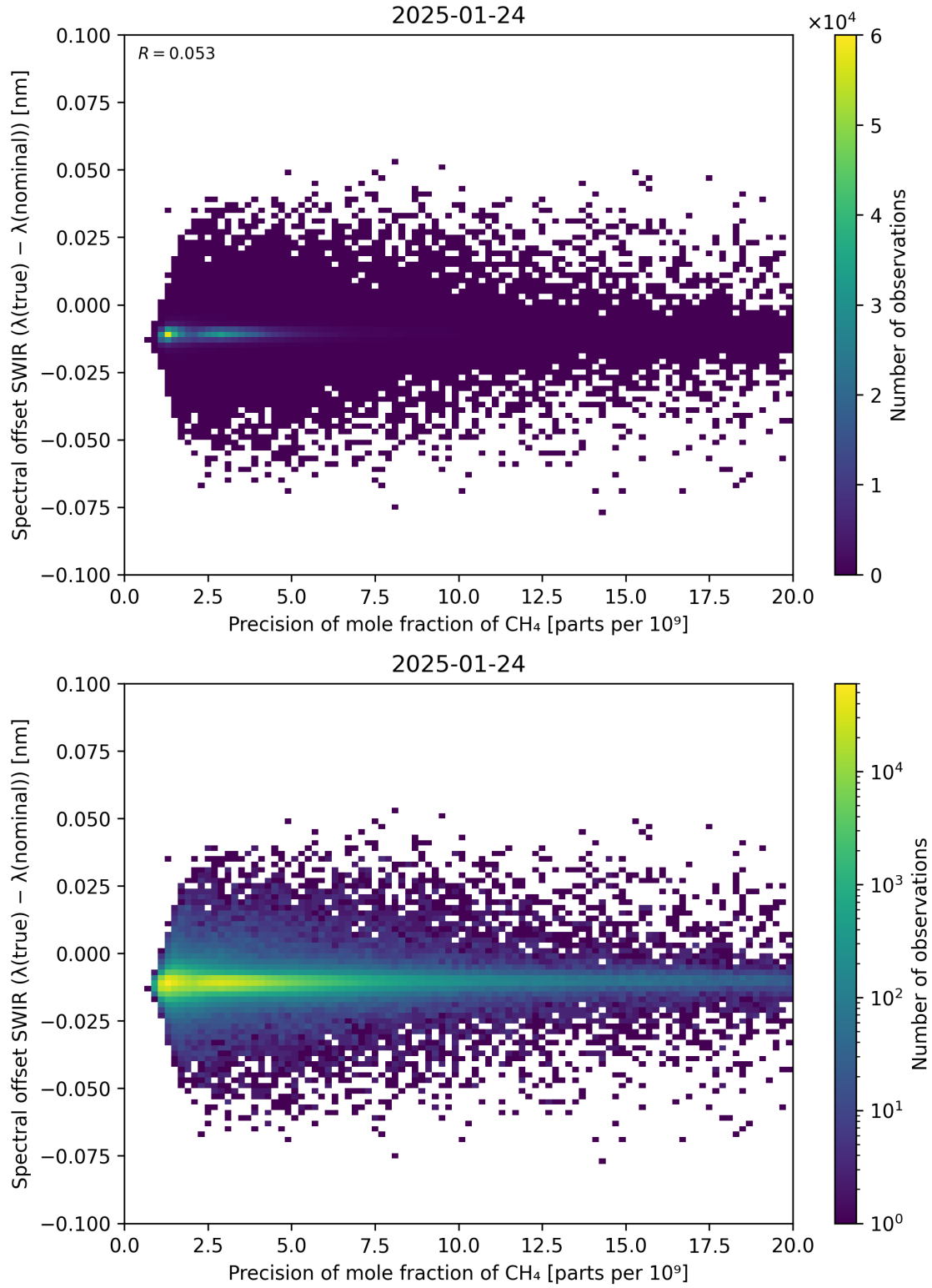
Figure 85: Scatter density plot of “Precision of mole fraction of CH 4 ” against “Spectral offset SWIR ( \lambda_{\text{true}} - \lambda_{\text{nominal}} )” for 2025-01-23 to 2025-01-25.
