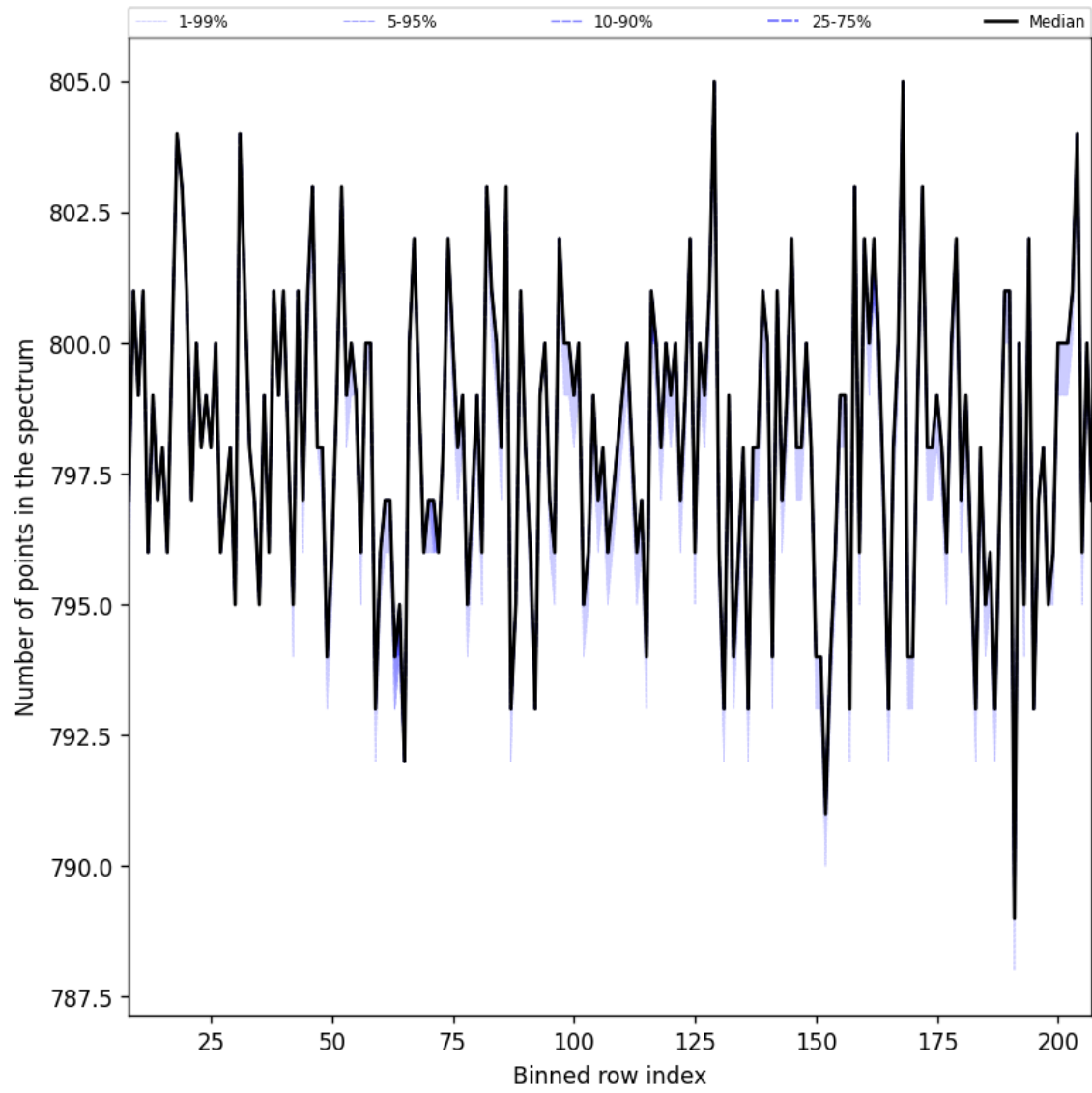
Figure 37: Along track statistics of “Number of points in the spectrum” for 2025-01-23 to 2025-01-25
