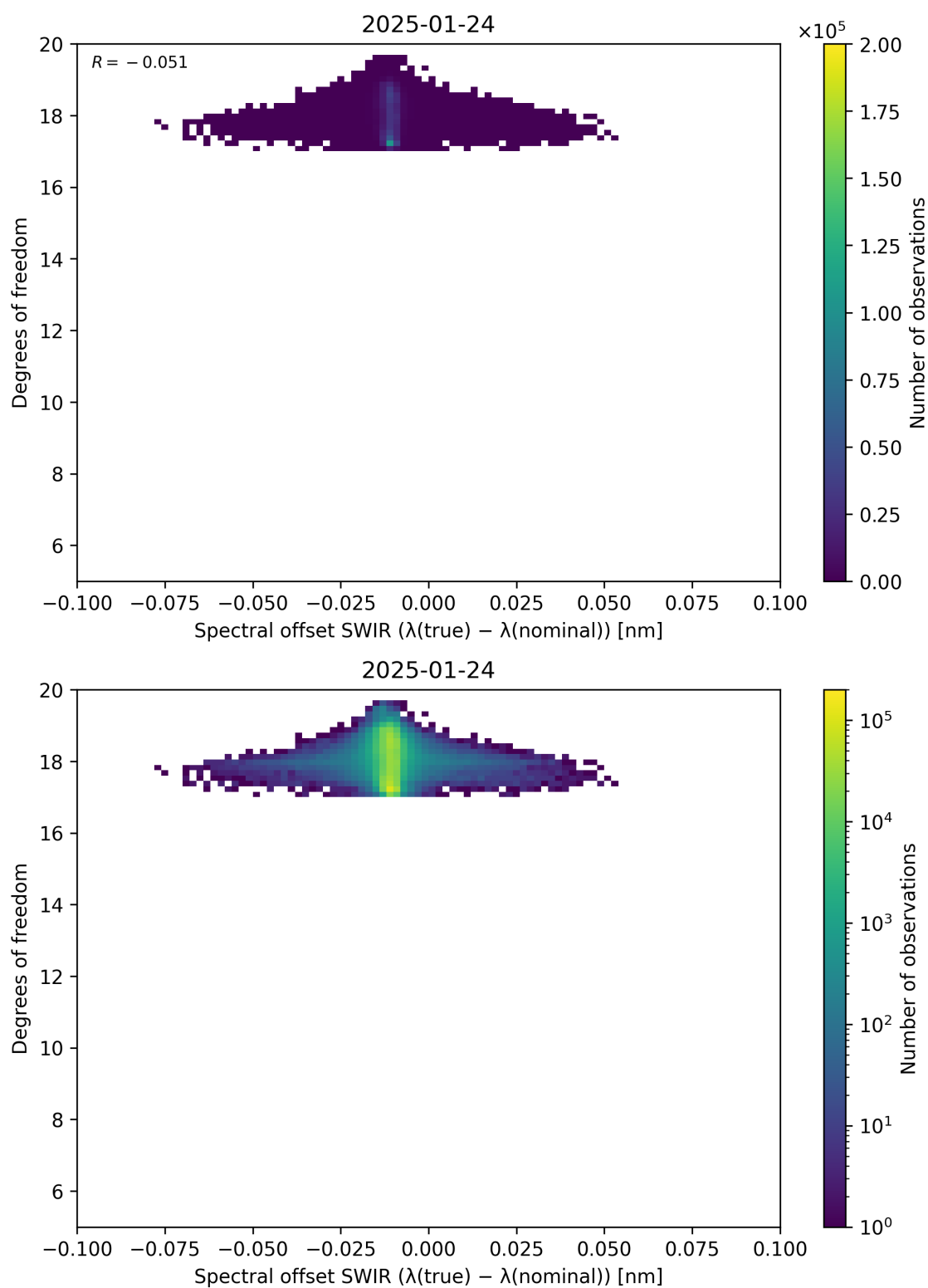
Figure 119: Scatter density plot of “Spectral offset SWIR ( \lambda_{\text{true}} - \lambda_{\text{nominal}} )” against “Degrees of freedom” for 2025-01-23 to 2025-01-25.
