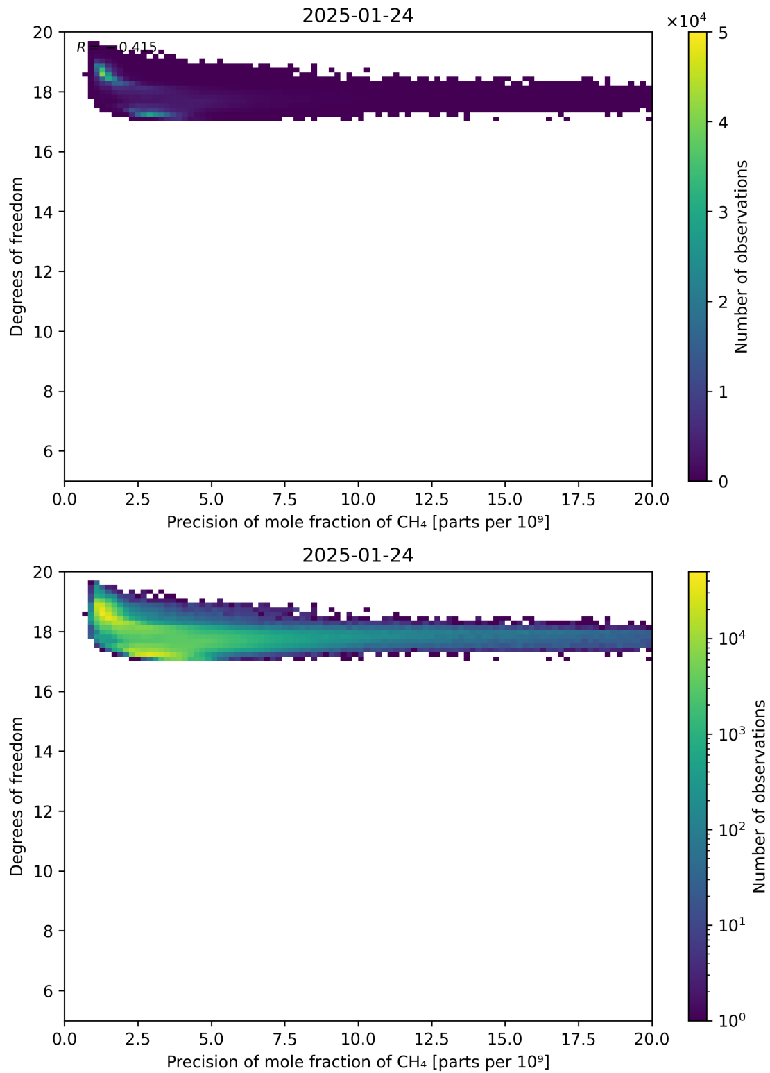
Figure 80: Scatter density plot of “Precision of mole fraction of CH 4 ” against “Degrees of freedom” for 2025-01-23 to 2025-01-25.
