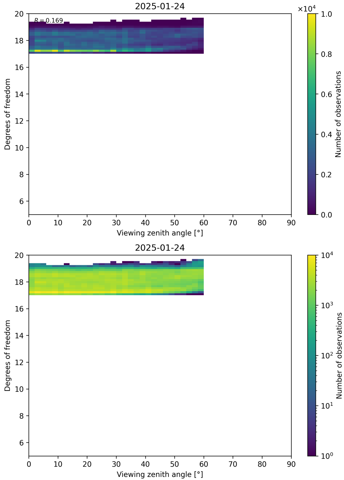
Figure 107: Scatter density plot of “Viewing zenith angle” against “Degrees of freedom” for 2025-01-23 to 2025-01-25.
