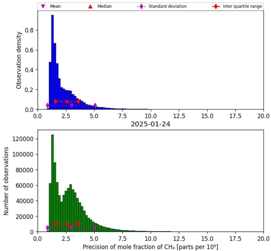
Figure 24: Histogram of “Precision of mole fraction of CH 4 ” for 2025-01-23 to 2025-01-25
