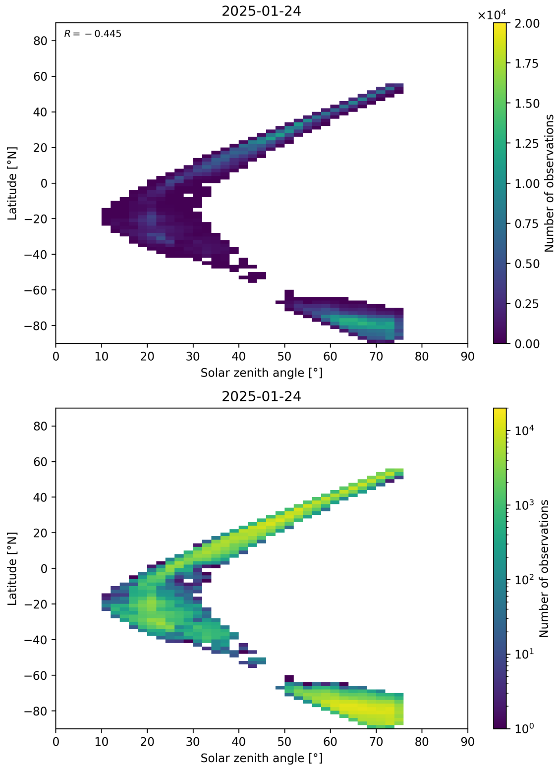
Figure 98: Scatter density plot of “Solar zenith angle” against “Latitude” for 2025-01-23 to 2025-01-25.
