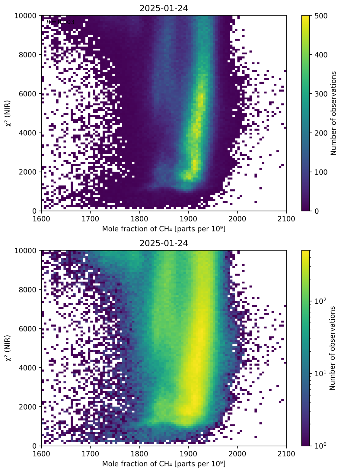
Figure 70: Scatter density plot of “Mole fraction of CH 4 ” against “ \chi^2 (NIR)” for 2025-01-23 to 2025-01-25.
