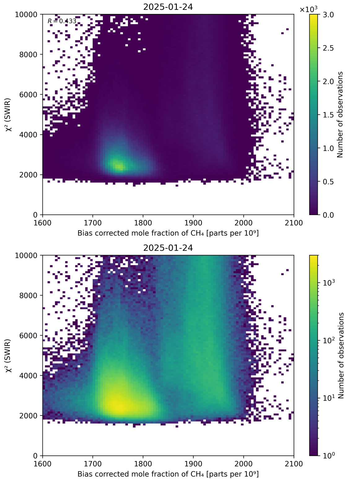
Figure 64: Scatter density plot of “Bias corrected mole fraction of \text{CH}_4 ” against “ \chi^2 (SWIR)” for 2025-01-23 to 2025-01-25.
