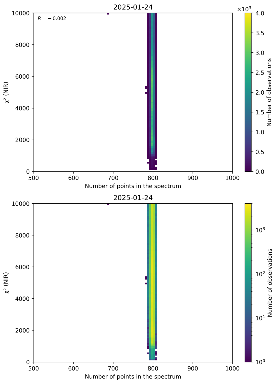
Figure 88: Scatter density plot of “Number of points in the spectrum” against “ \chi^2 (NIR)” for 2025-01-23 to 2025-01-25.
