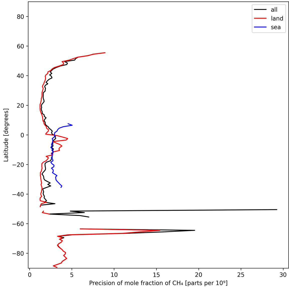
Figure 13: Zonal average of “Precision of mole fraction of CH 4 ” for 2025-01-23 to 2025-01-25.
