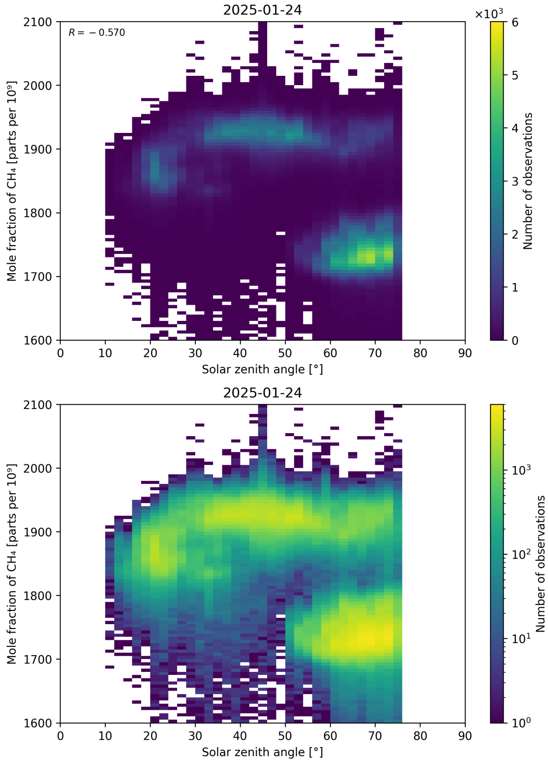
Figure 99: Scatter density plot of “Solar zenith angle” against “Mole fraction of CH 4 ” for 2025-01-23 to 2025-01-25.
