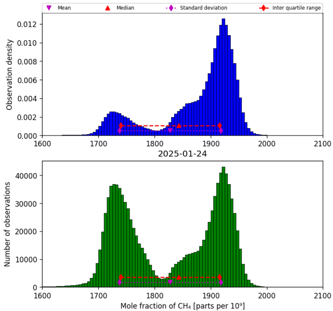
Figure 23: Histogram of “Mole fraction of CH 4 ” for 2025-01-23 to 2025-01-25
