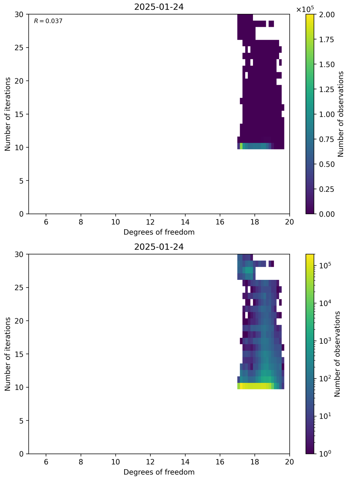
Figure 52: Scatter density plot of “Degrees of freedom” against “Number of iterations” for 2025-01-23 to 2025-01-25.
