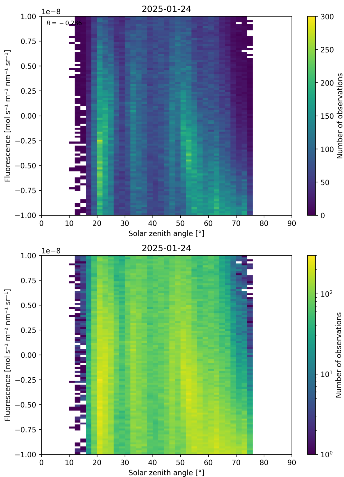
Figure 97: Scatter density plot of “Solar zenith angle” against “Fluorescence” for 2025-01-23 to 2025-01-25.
