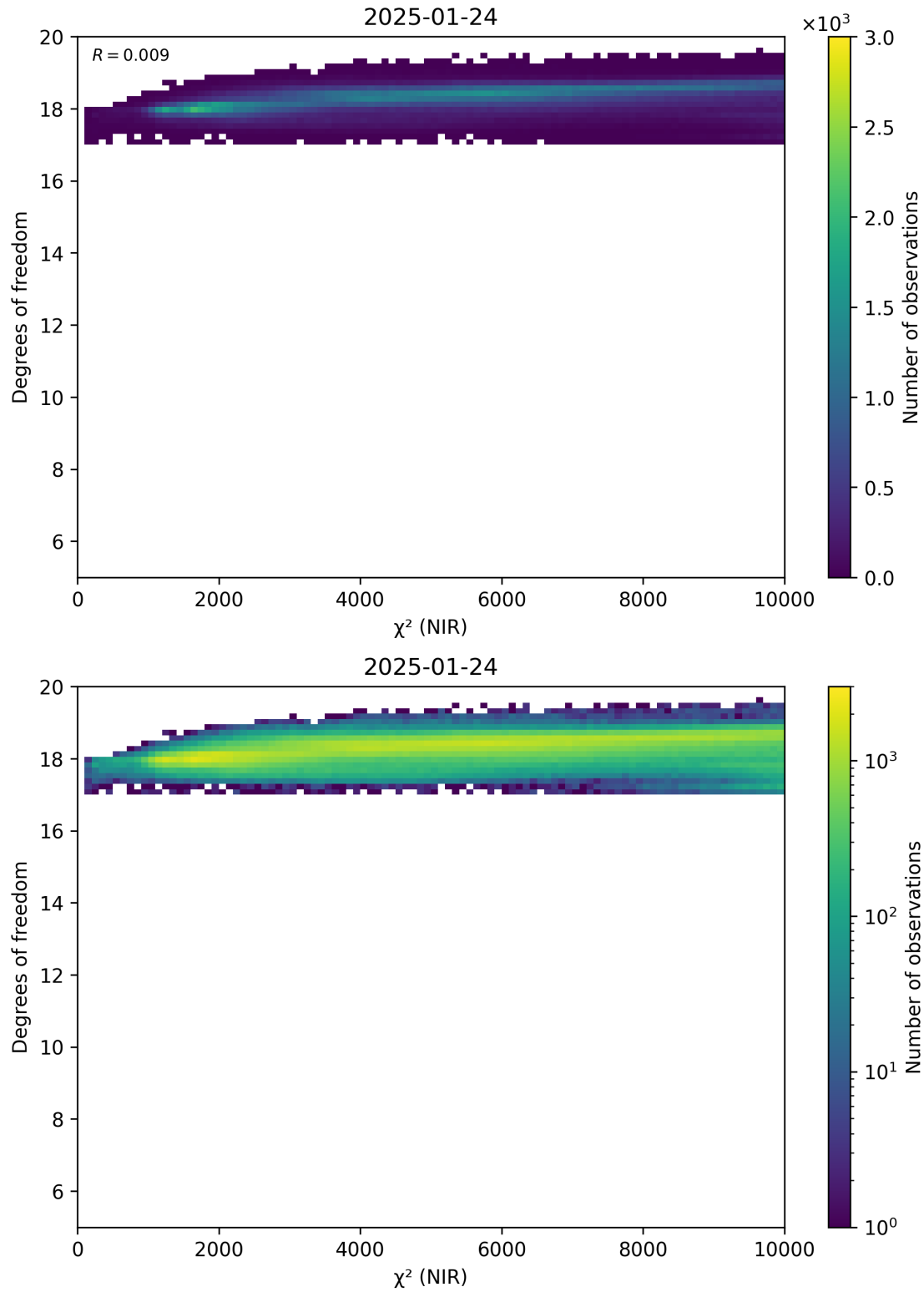
Figure 44: Scatter density plot of “ \chi^2 (NIR)” against “Degrees of freedom” for 2025-01-23 to 2025-01-25.
