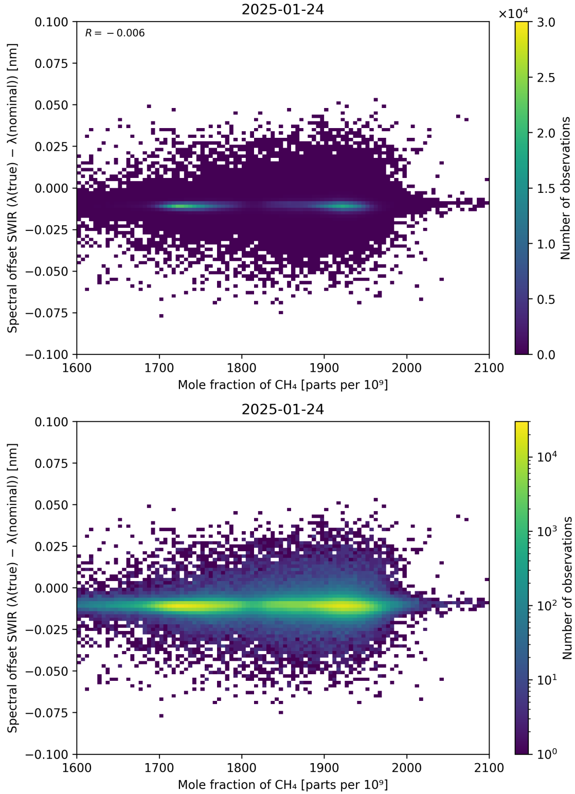
Figure 86: Scatter density plot of “Mole fraction of \text{CH}_4 ” against “Spectral offset SWIR ( \lambda_{\text{true}} - \lambda_{\text{nominal}} )” for 2025-01-23 to 2025-01-25.
