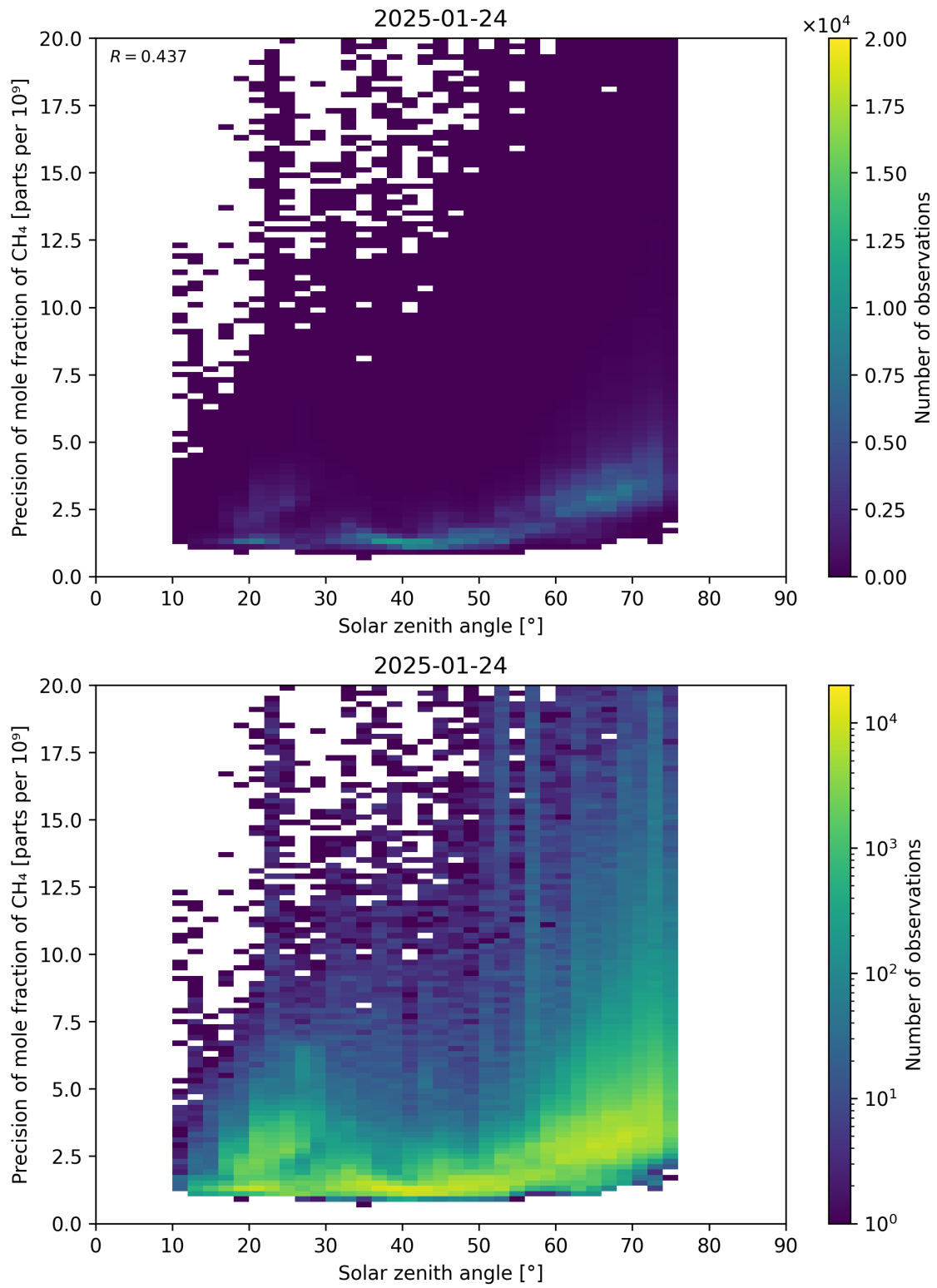
Figure 101: Scatter density plot of “Solar zenith angle” against “Precision of mole fraction of CH 4 ” for 2025-01-23 to 2025-01-25.
