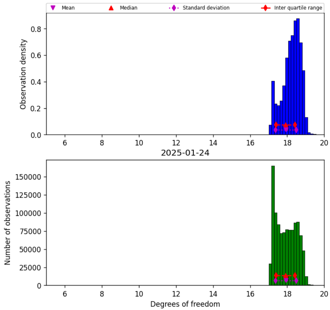
Figure 30: Histogram of “Degrees of freedom” for 2025-01-23 to 2025-01-25
