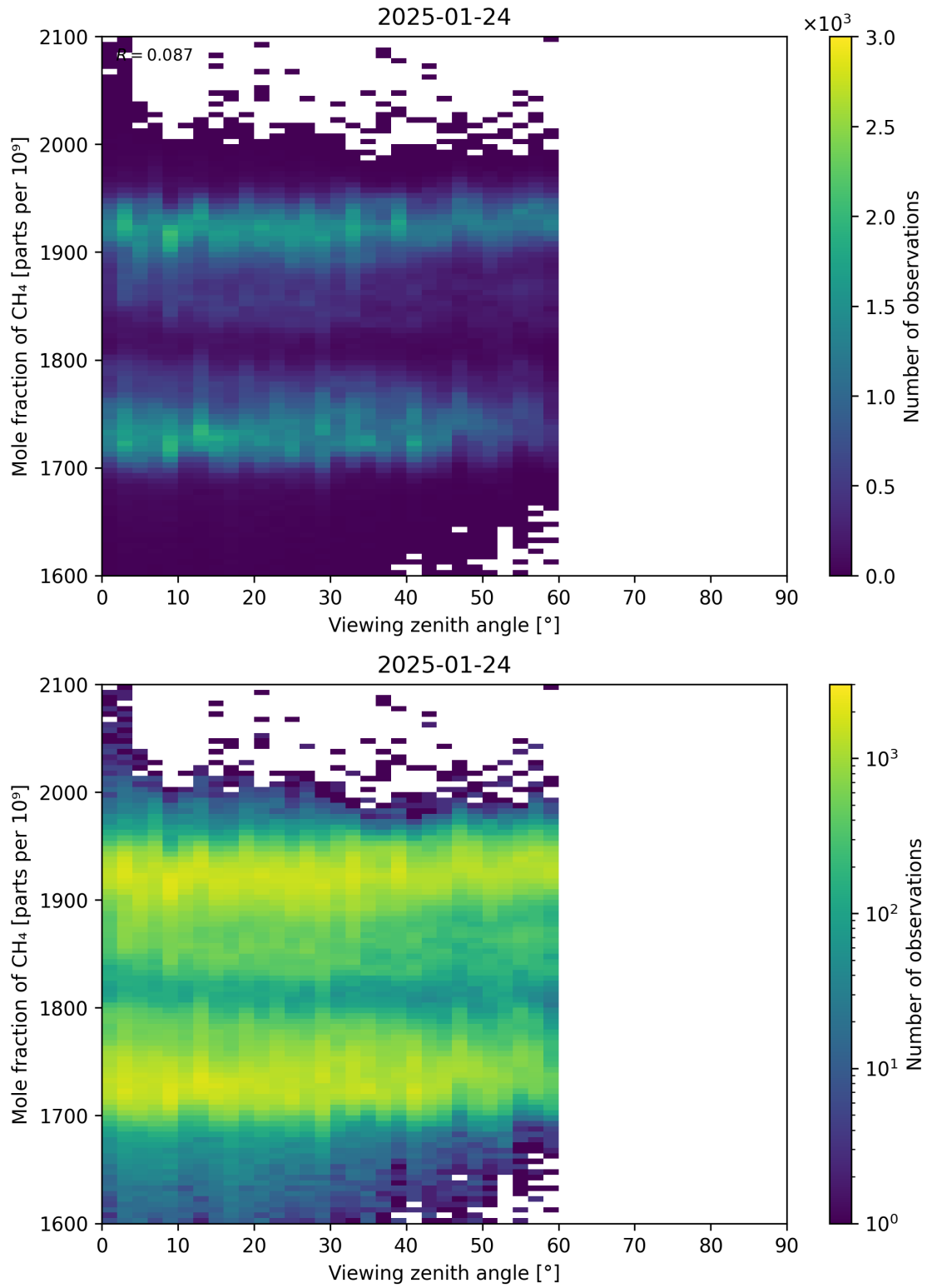
Figure 110: Scatter density plot of “Viewing zenith angle” against “Mole fraction of \text{CH}_4 ” for 2025-01-23 to 2025-01-25.
