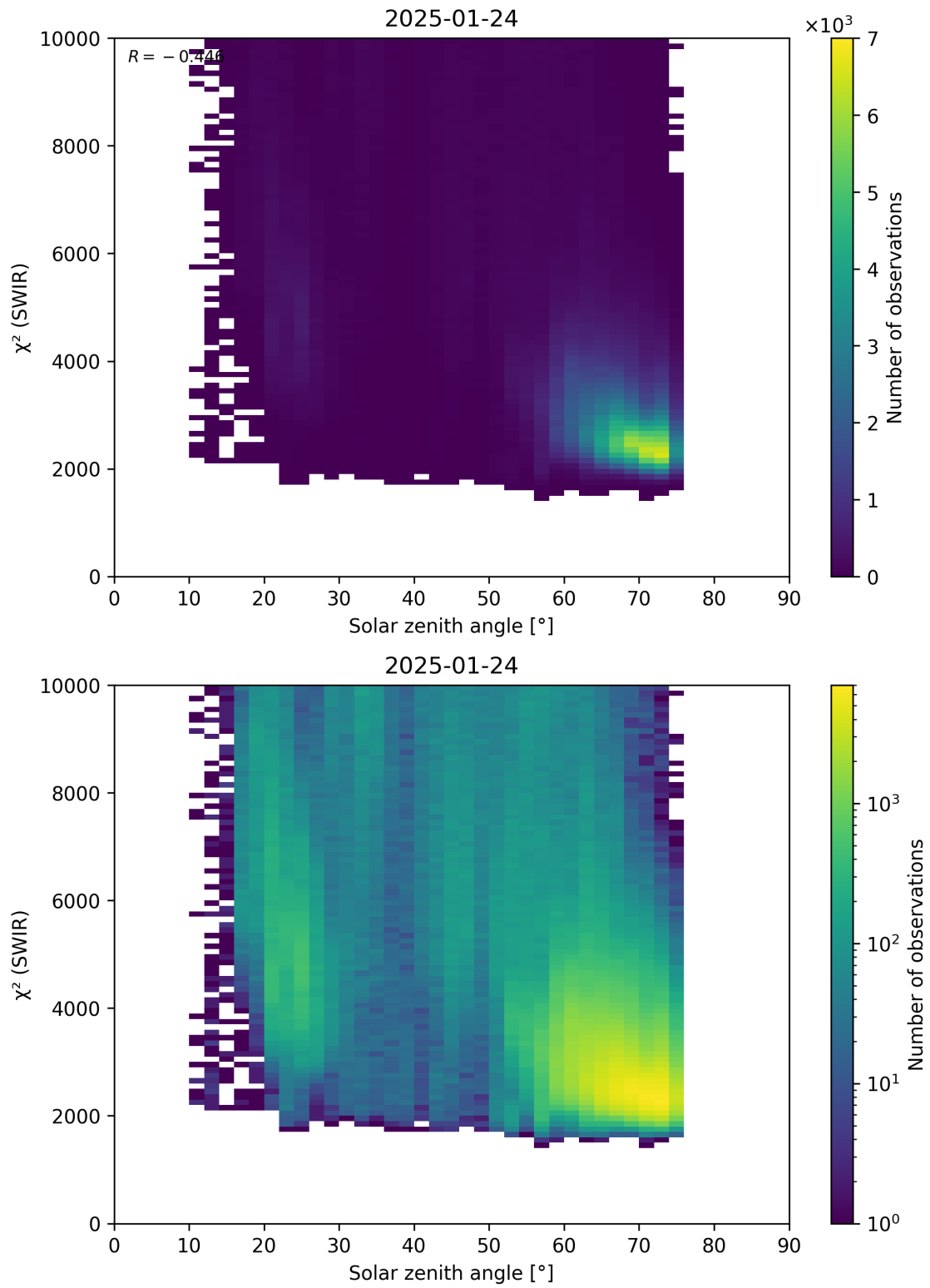
Figure 95: Scatter density plot of “Solar zenith angle” against “ \chi^2 (SWIR)” for 2025-01-23 to 2025-01-25.
