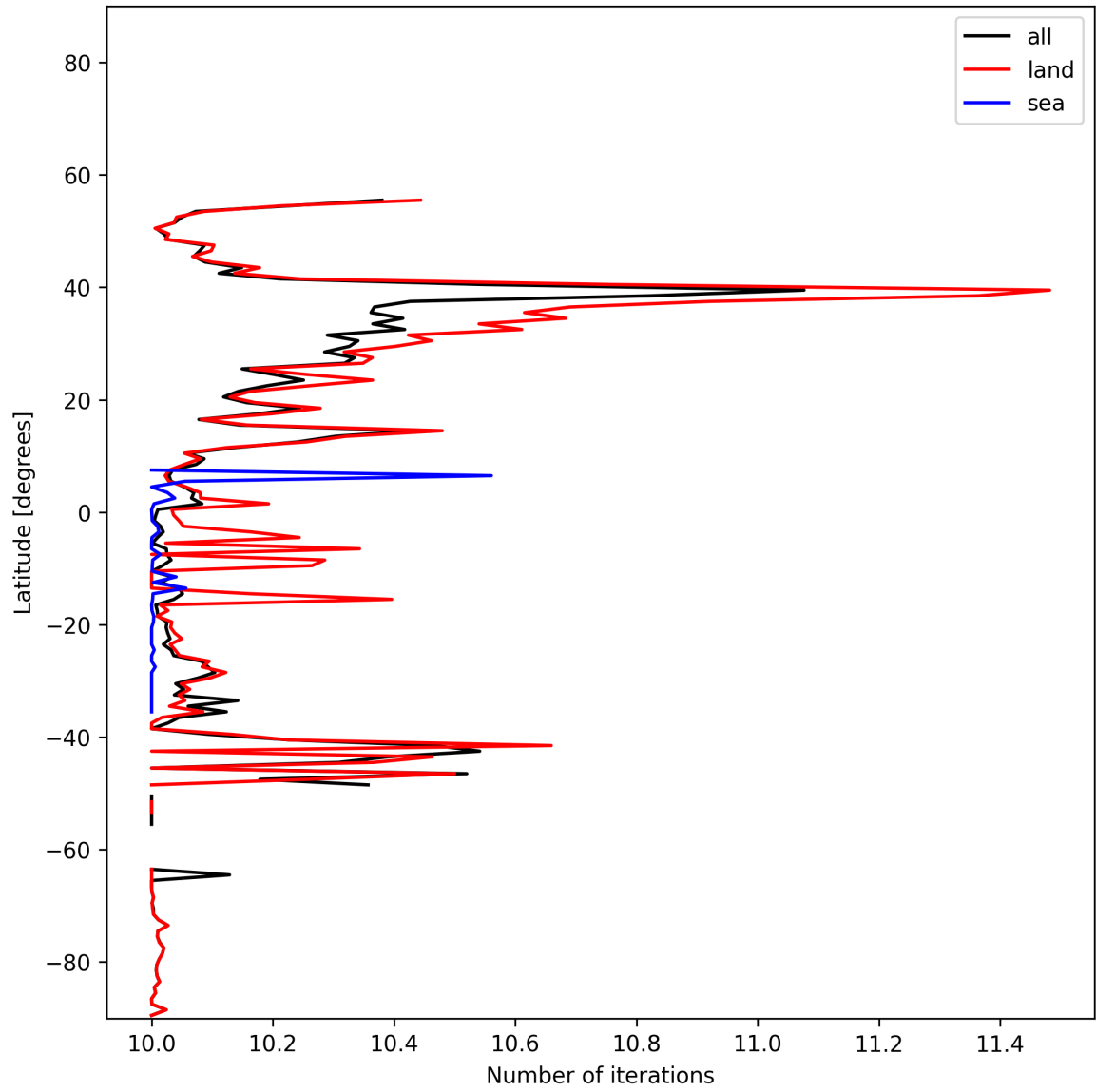
Figure 20: Zonal average of “Number of iterations” for 2025-01-23 to 2025-01-25.
