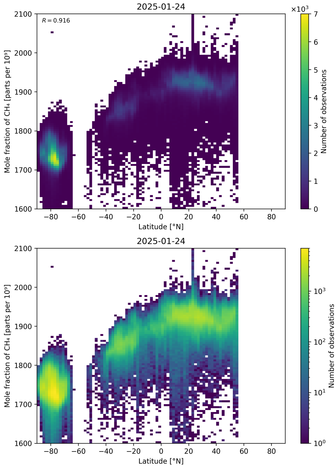
Figure 57: Scatter density plot of “Latitude” against “Mole fraction of CH 4 ” for 2025-01-23 to 2025-01-25.
