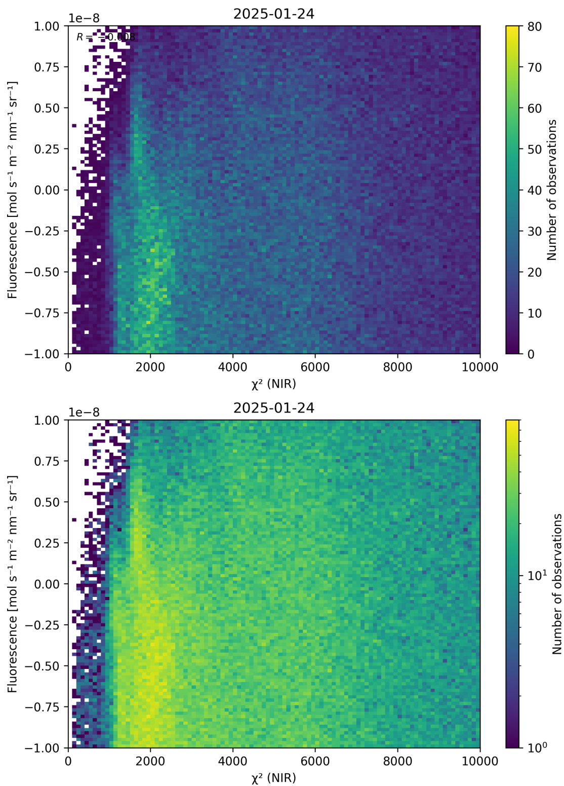
Figure 45: Scatter density plot of “ \chi^2 (NIR)” against “Fluorescence” for 2025-01-23 to 2025-01-25.
