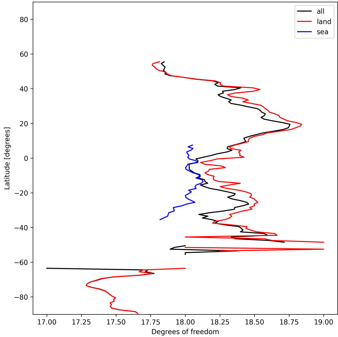
Figure 19: Zonal average of “Degrees of freedom” for 2025-01-23 to 2025-01-25.
