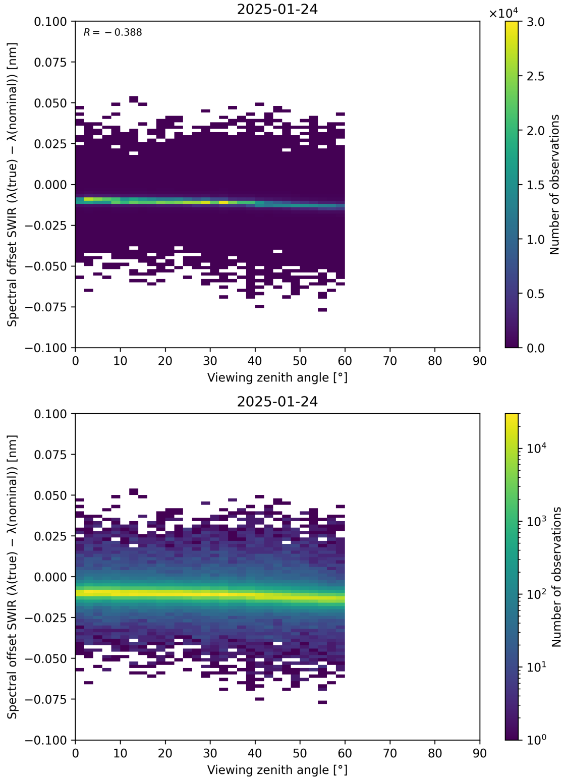
Figure 116: Scatter density plot of “Viewing zenith angle” against “Spectral offset SWIR ( \lambda_{\text{true}} - \lambda_{\text{nominal}} )” for 2025-01-23 to 2025-01-25.
