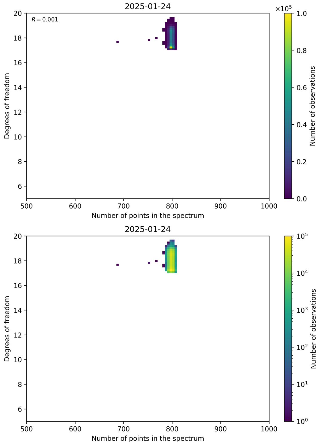
Figure 90: Scatter density plot of “Number of points in the spectrum” against “Degrees of freedom” for 2025-01-23 to 2025-01-25.
