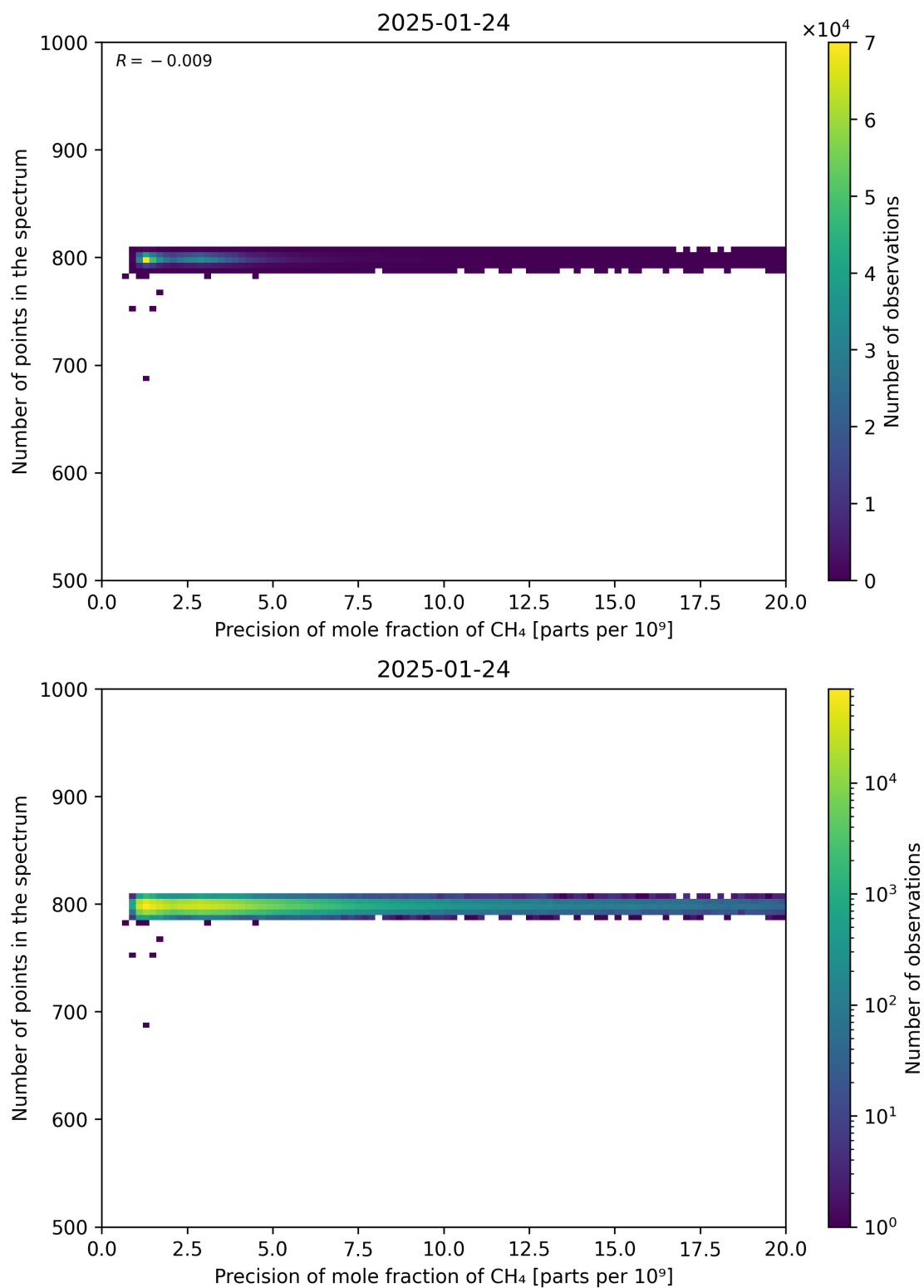
Figure 84: Scatter density plot of “Precision of mole fraction of CH 4 ” against “Number of points in the spectrum” for 2025-01-23 to 2025-01-25.
