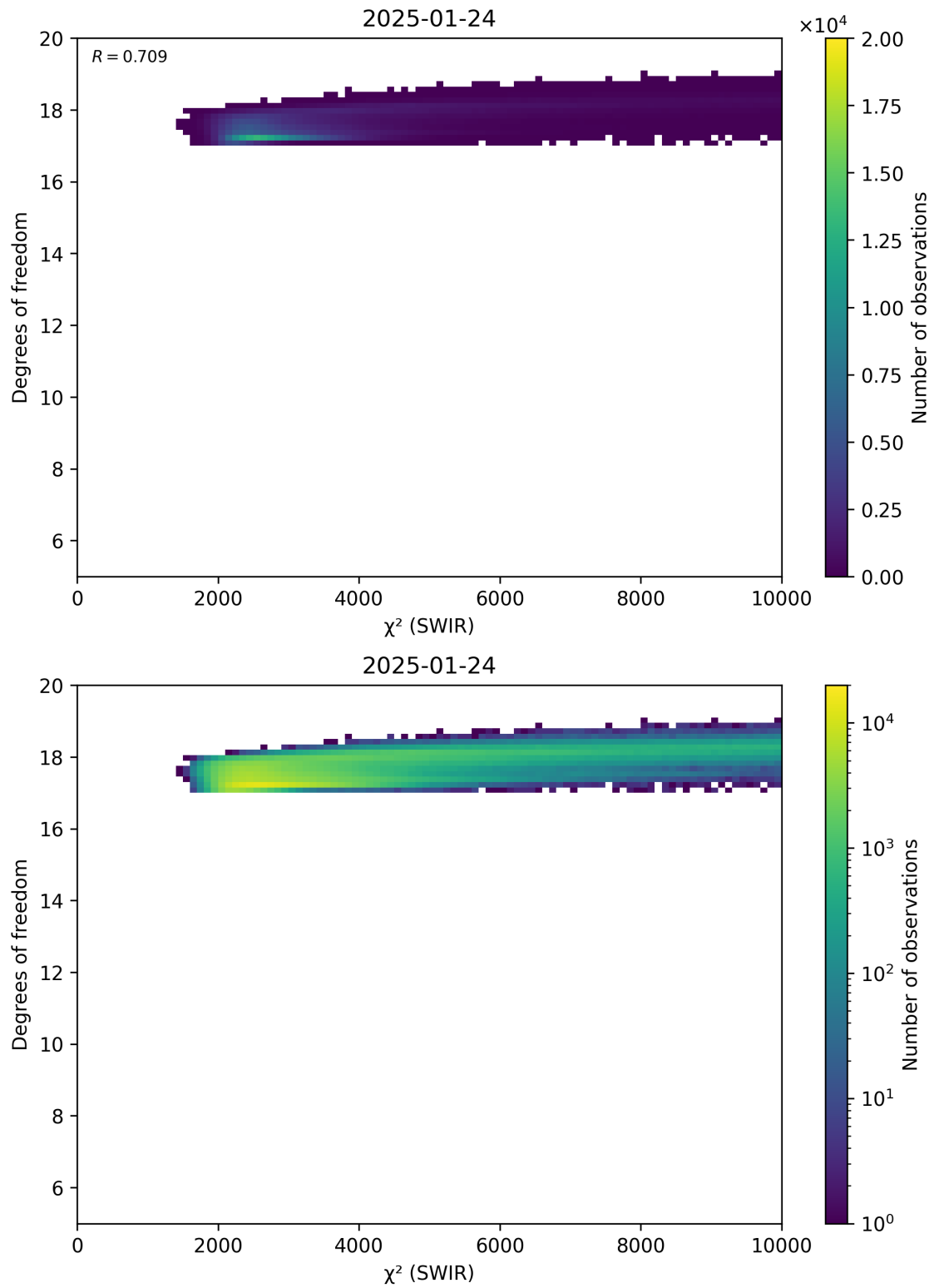
Figure 48: Scatter density plot of “ \chi^2 (SWIR)” against “Degrees of freedom” for 2025-01-23 to 2025-01-25.
