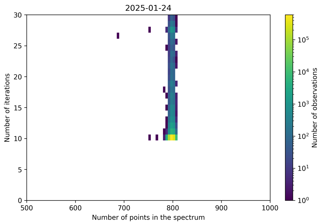
Figure 92: Scatter density plot of “Number of points in the spectrum” against “Number of iterations” for 2025-01-23 to 2025-01-25.
