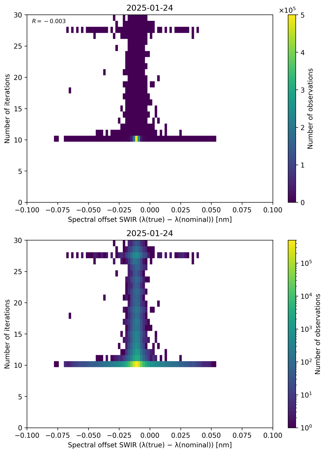
Figure 121: Scatter density plot of “Spectral offset SWIR ( \lambda_{\text{true}} - \lambda_{\text{nominal}} )” against “Number of iterations” for 2025-01-23 to 2025-01-25.
