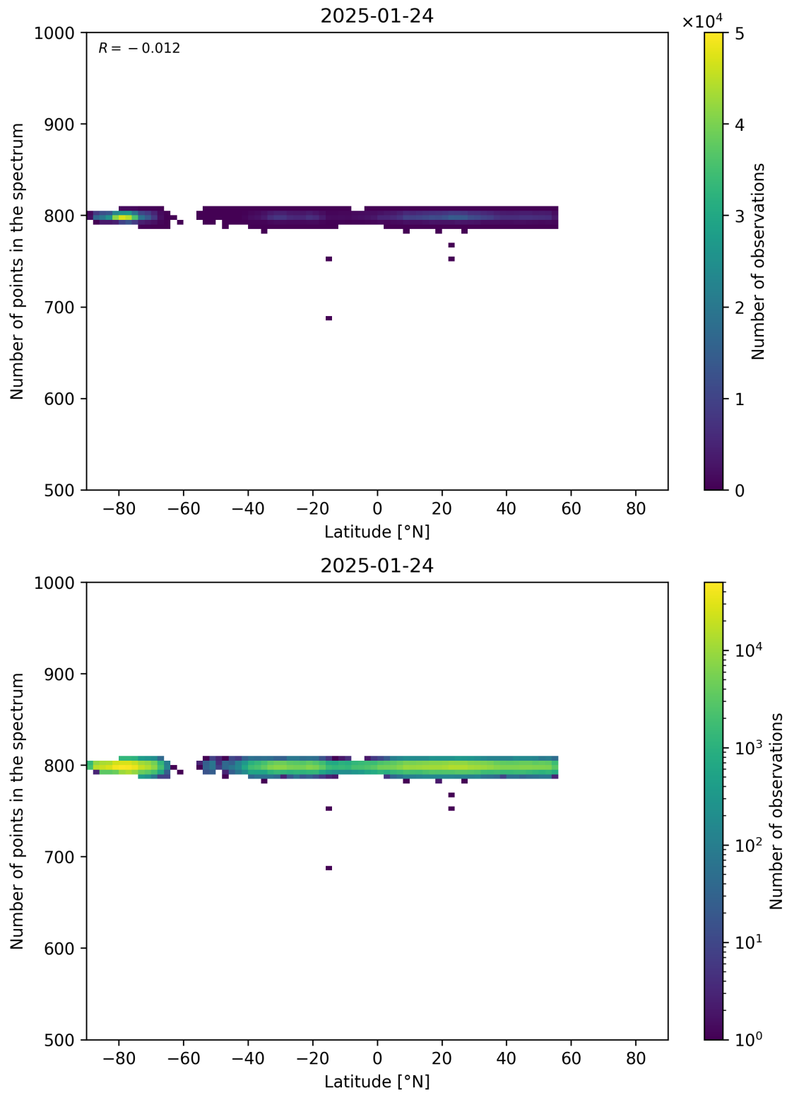
Figure 61: Scatter density plot of “Latitude” against “Number of points in the spectrum” for 2025-01-23 to 2025-01-25.
