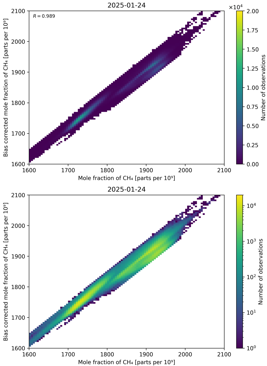
Figure 74: Scatter density plot of “Mole fraction of CH 4 ” against “Bias corrected mole fraction of CH 4 ” for 2025-01-23 to 2025-01-25.
