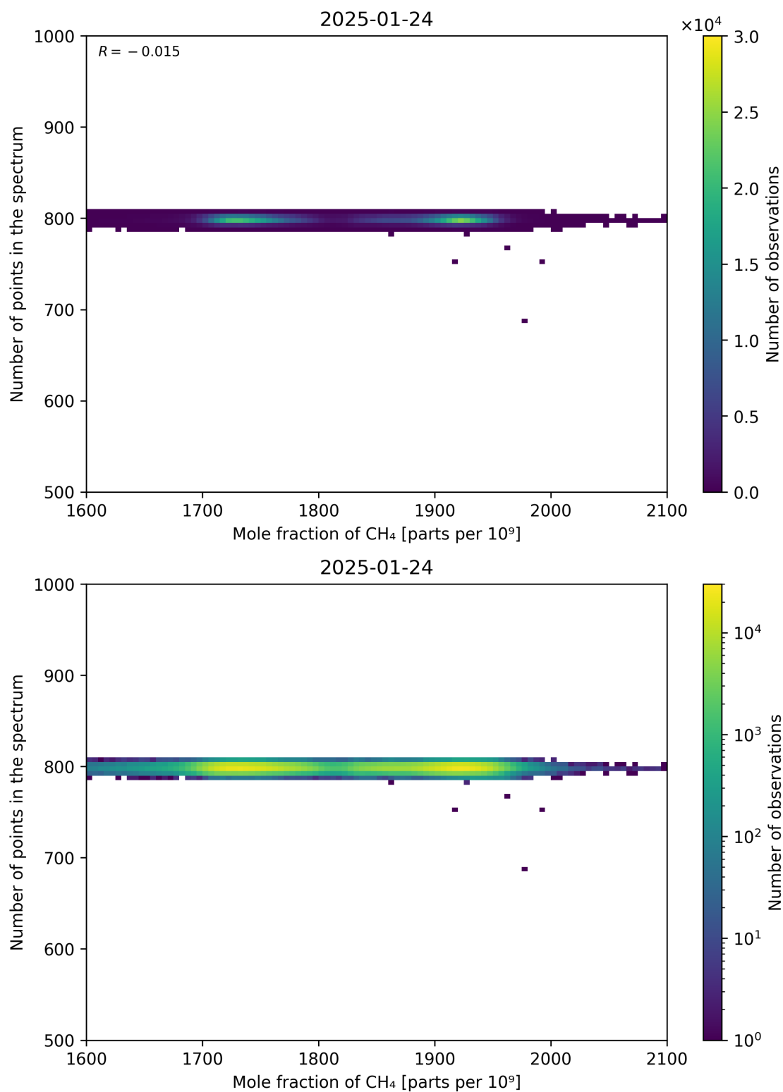
Figure 77: Scatter density plot of “Mole fraction of CH 4 ” against “Number of points in the spectrum” for 2025-01-23 to 2025-01-25.
