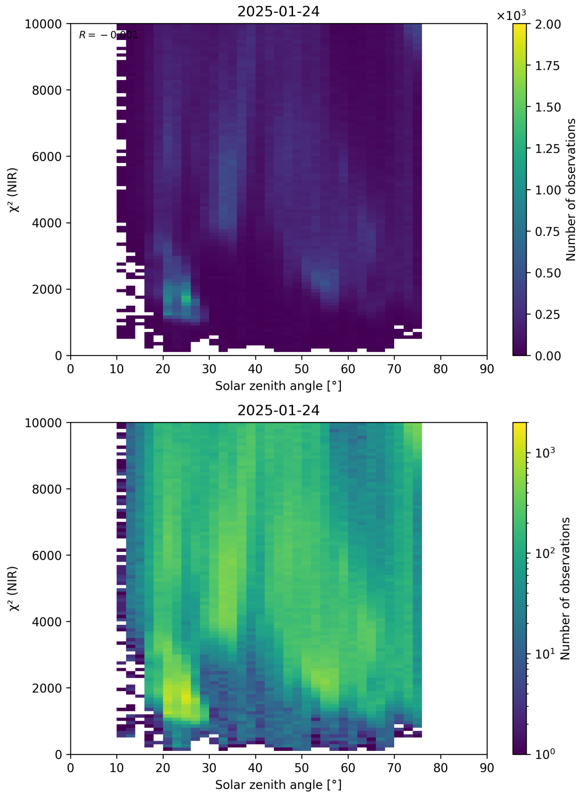
Figure 94: Scatter density plot of “Solar zenith angle” against “ \chi^2 (NIR)” for 2025-01-23 to 2025-01-25.
