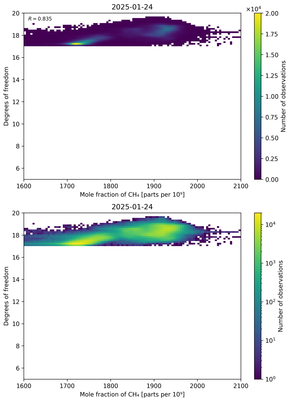
Figure 72: Scatter density plot of “Mole fraction of CH 4 ” against “Degrees of freedom” for 2025-01-23 to 2025-01-25.
