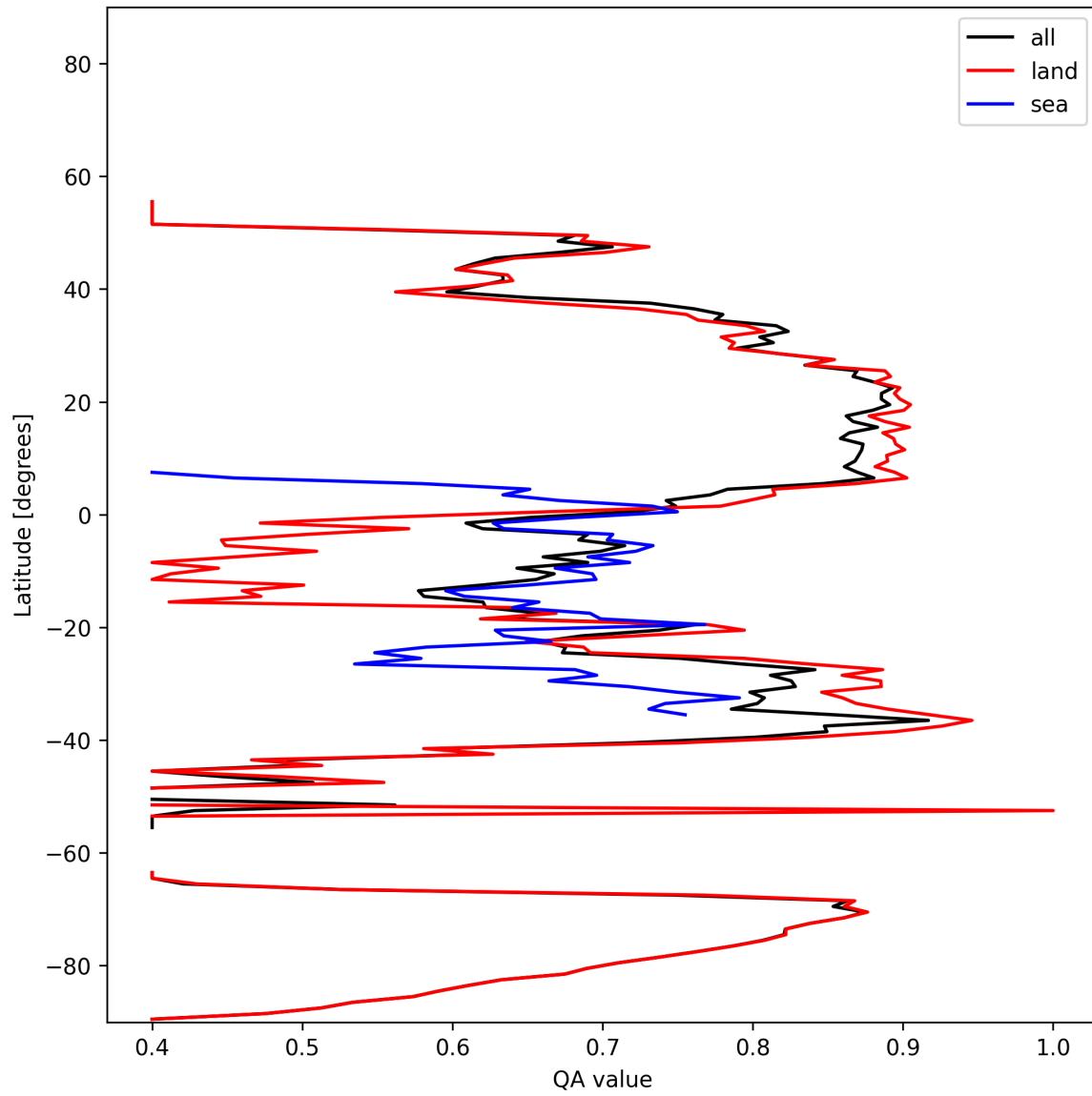
Figure 11: Zonal average of “QA value” for 2025-01-23 to 2025-01-25.
