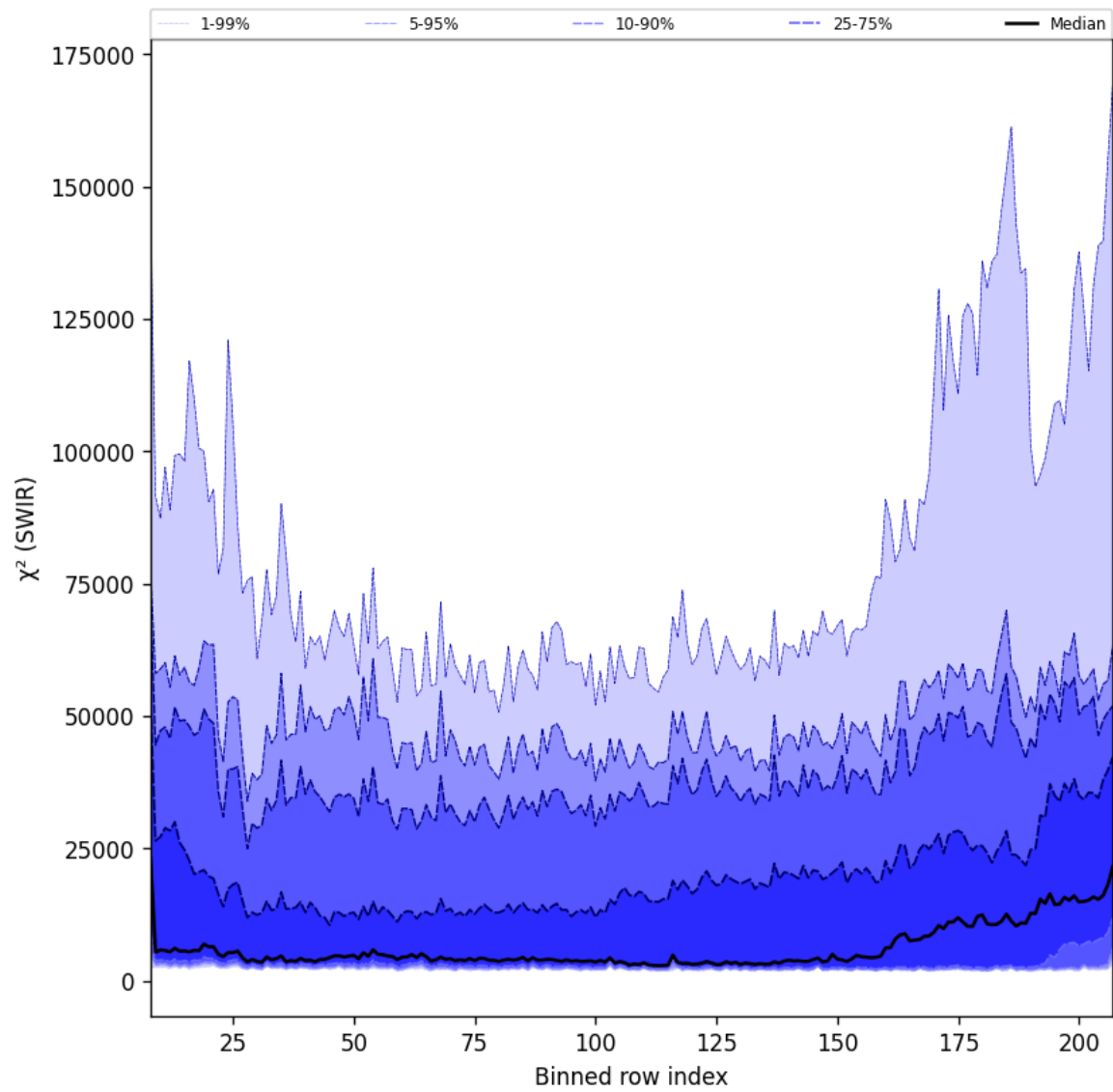
Figure 39: Along track statistics of “ \chi^2 (SWIR)” for 2025-01-23 to 2025-01-25
