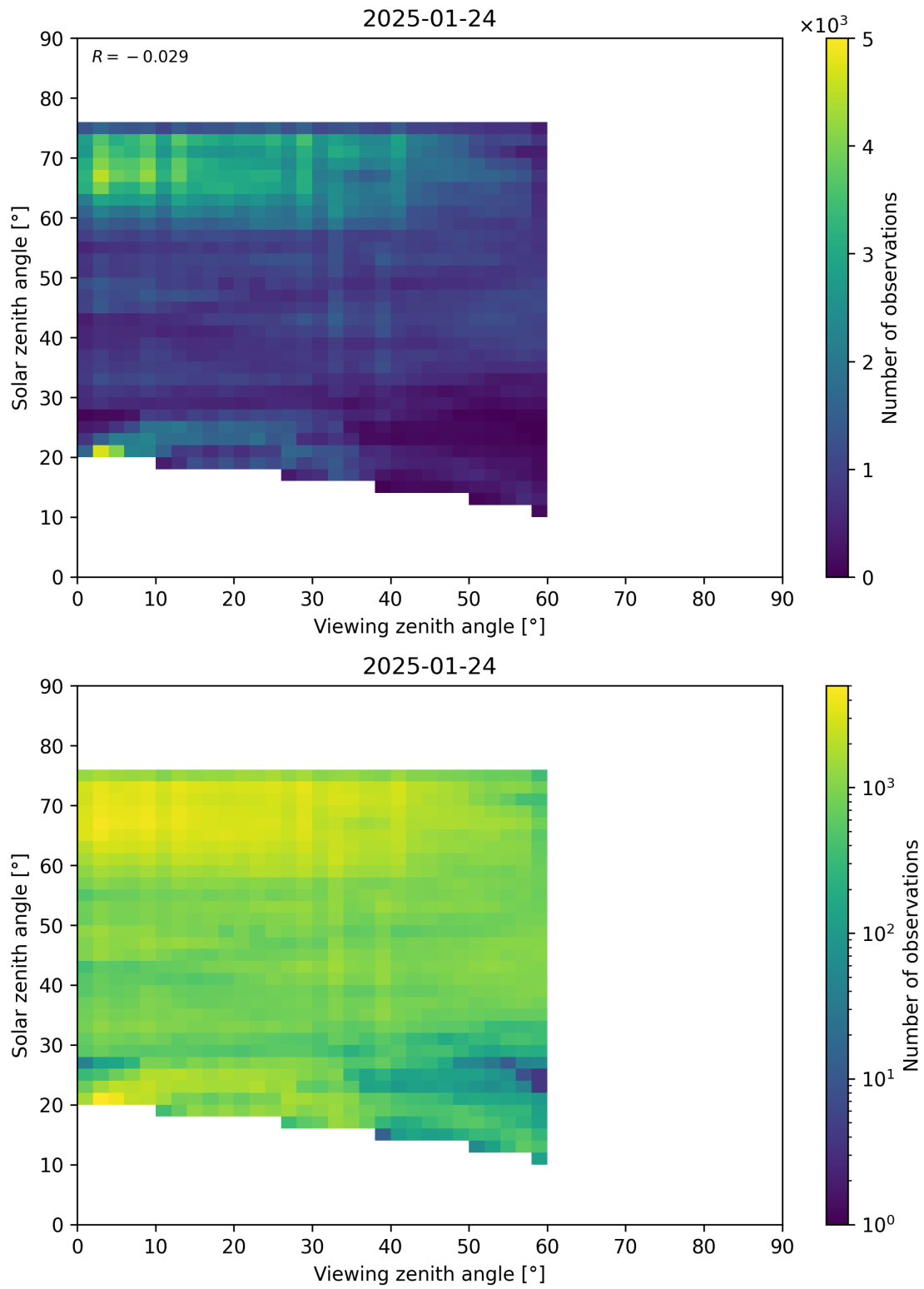
Figure 115: Scatter density plot of “Viewing zenith angle” against “Solar zenith angle” for 2025-01-23 to 2025-01-25.
