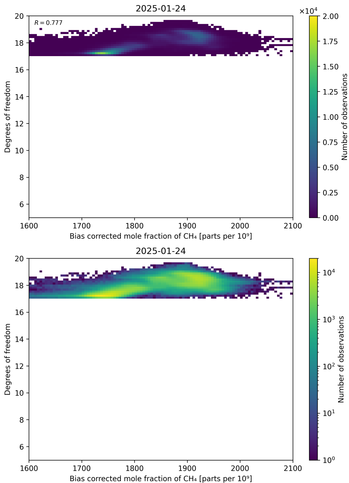
Figure 65: Scatter density plot of “Bias corrected mole fraction of CH 4 ” against “Degrees of freedom” for 2025-01-23 to 2025-01-25.
