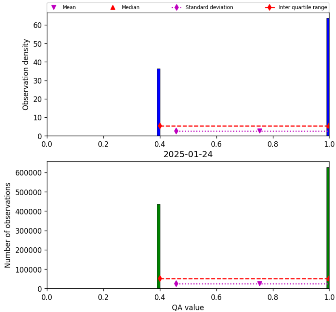
Figure 22: Histogram of “QA value” for 2025-01-23 to 2025-01-25
