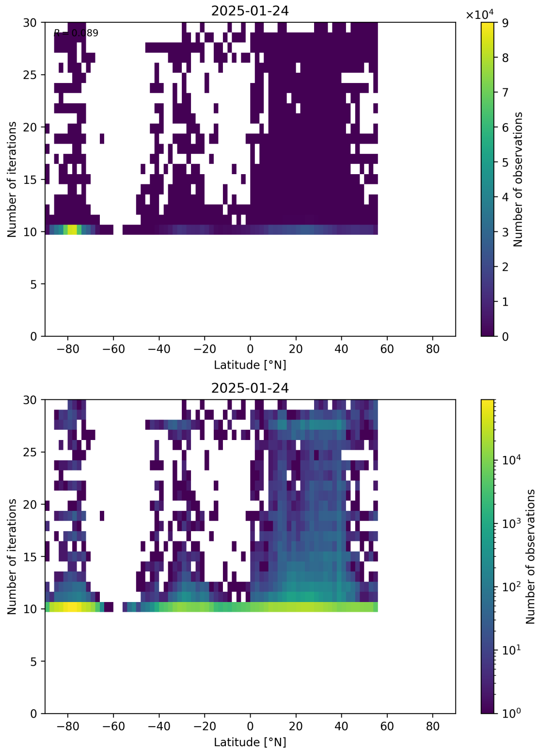
Figure 60: Scatter density plot of “Latitude” against “Number of iterations” for 2025-01-23 to 2025-01-25.
