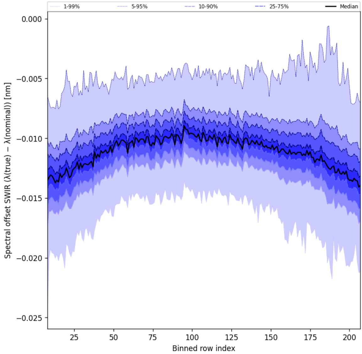
Figure 38: Along track statistics of “Spectral offset SWIR ( \lambda_{\text{true}} - \lambda_{\text{nominal}} )” for 2025-01-23 to 2025-01-25
