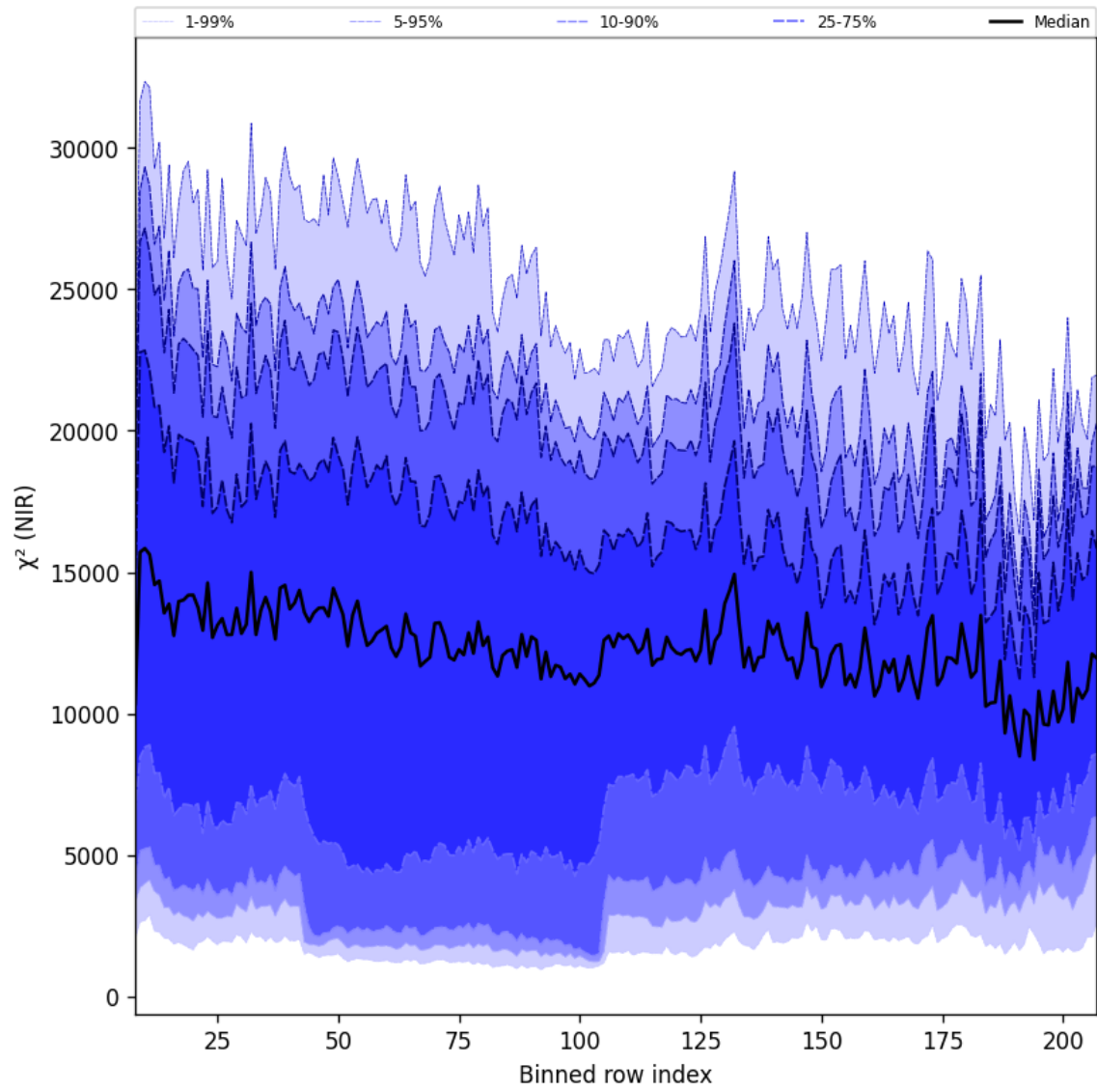
Figure 40: Along track statistics of “ \chi^2 (NIR)” for 2025-01-23 to 2025-01-25
