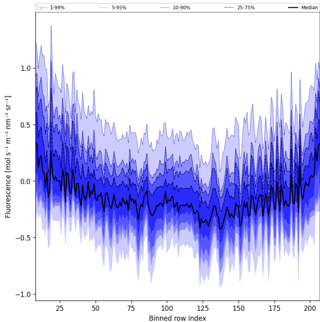
Figure 43: Along track statistics of “Fluorescence” for 2025-01-23 to 2025-01-25
