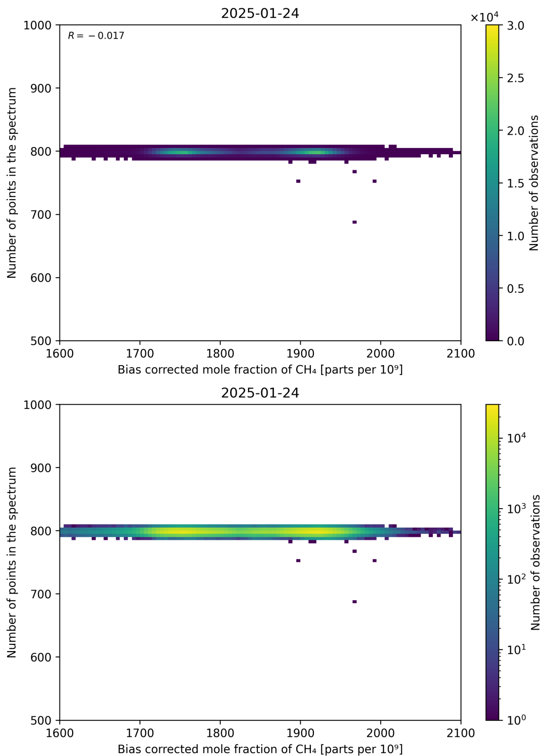
Figure 68: Scatter density plot of “Bias corrected mole fraction of CH 4 ” against “Number of points in the spectrum” for 2025-01-23 to 2025-01-25.
