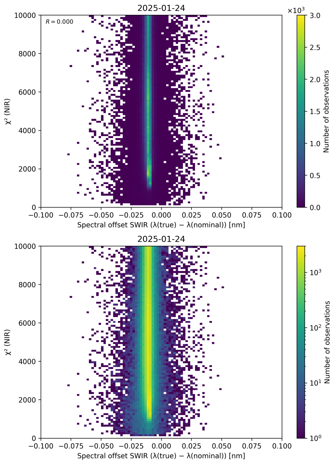
Figure 117: Scatter density plot of “Spectral offset SWIR ( \lambda_{\text{true}} - \lambda_{\text{nominal}} )” against “ \chi^2 (NIR)” for 2025-01-23 to 2025-01-25.
