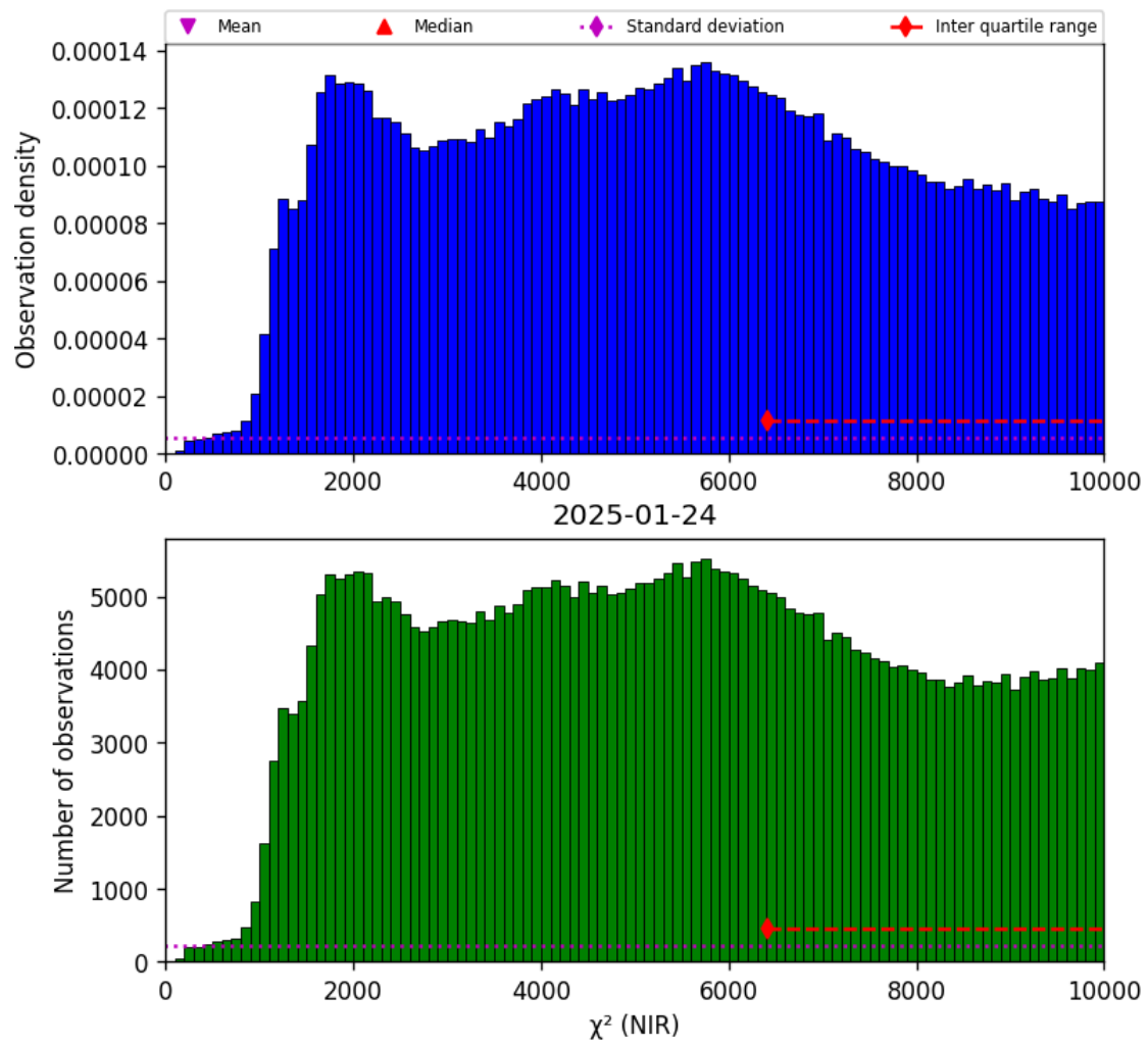
Figure 29: Histogram of “ \chi^2 (NIR)” for 2025-01-23 to 2025-01-25
