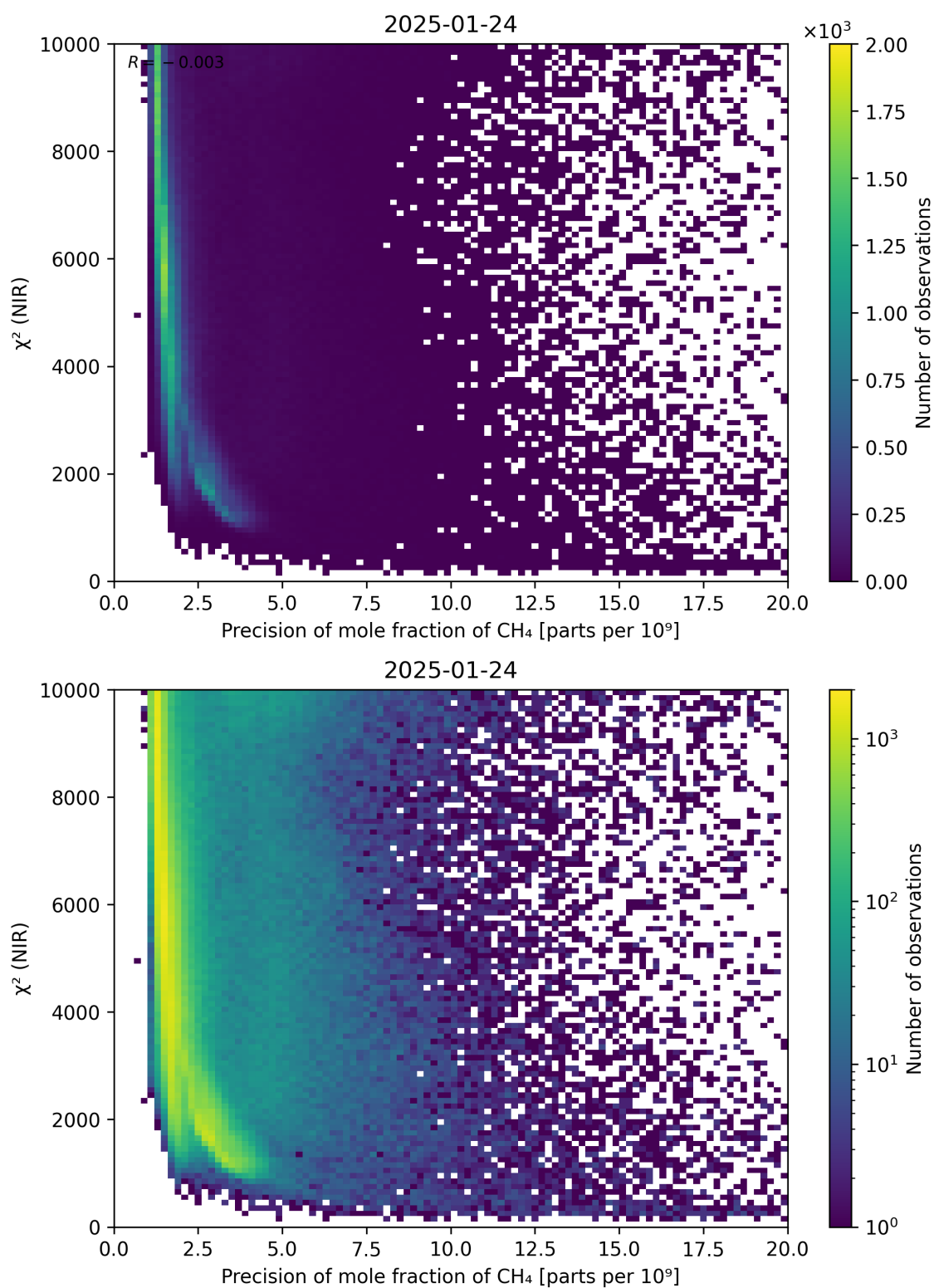
Figure 78: Scatter density plot of “Precision of mole fraction of CH 4 ” against “ \chi^2 (NIR)” for 2025-01-23 to 2025-01-25.
