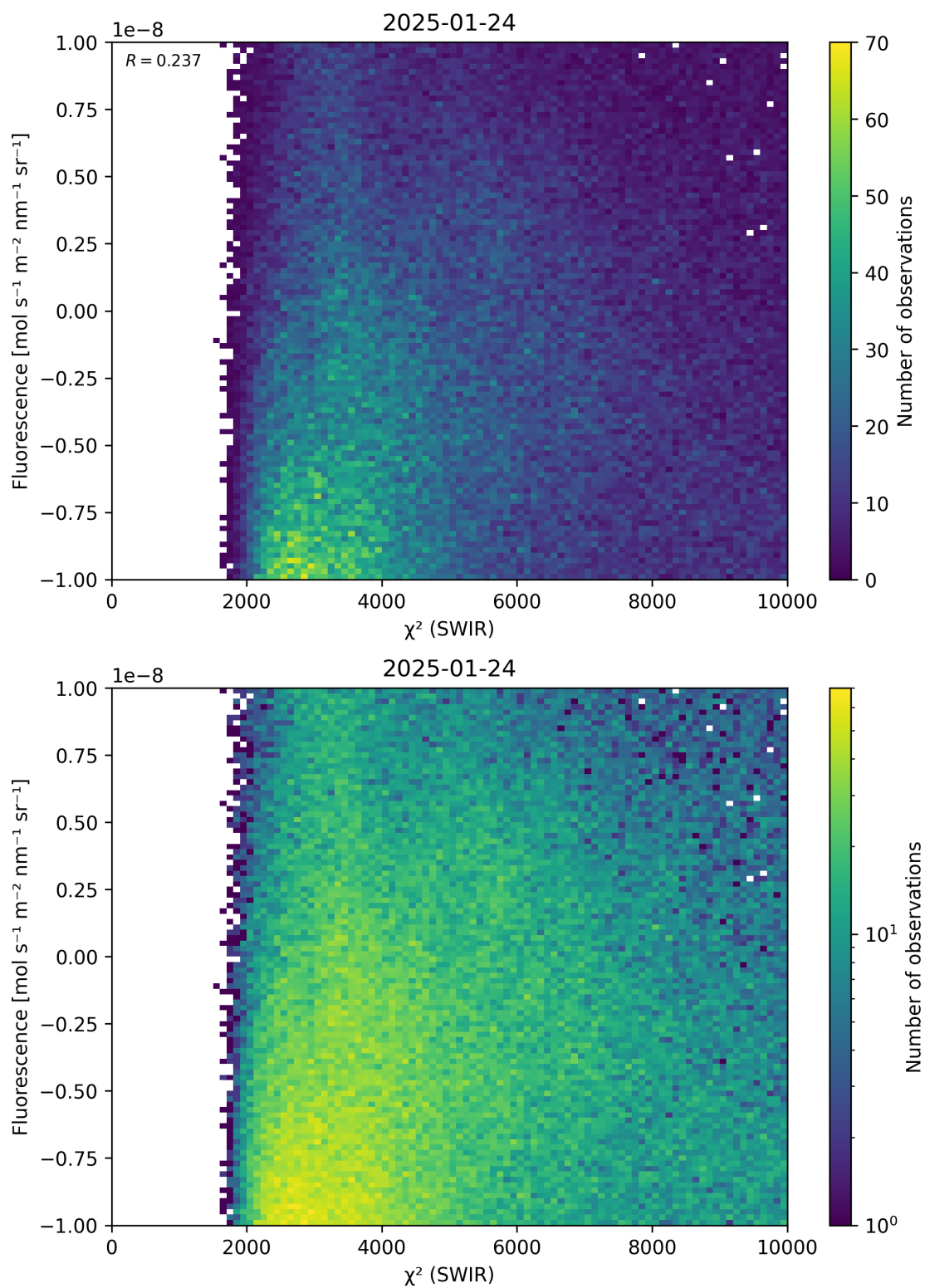
Figure 49: Scatter density plot of “ \chi^2 (SWIR)” against “Fluorescence” for 2025-01-23 to 2025-01-25.
