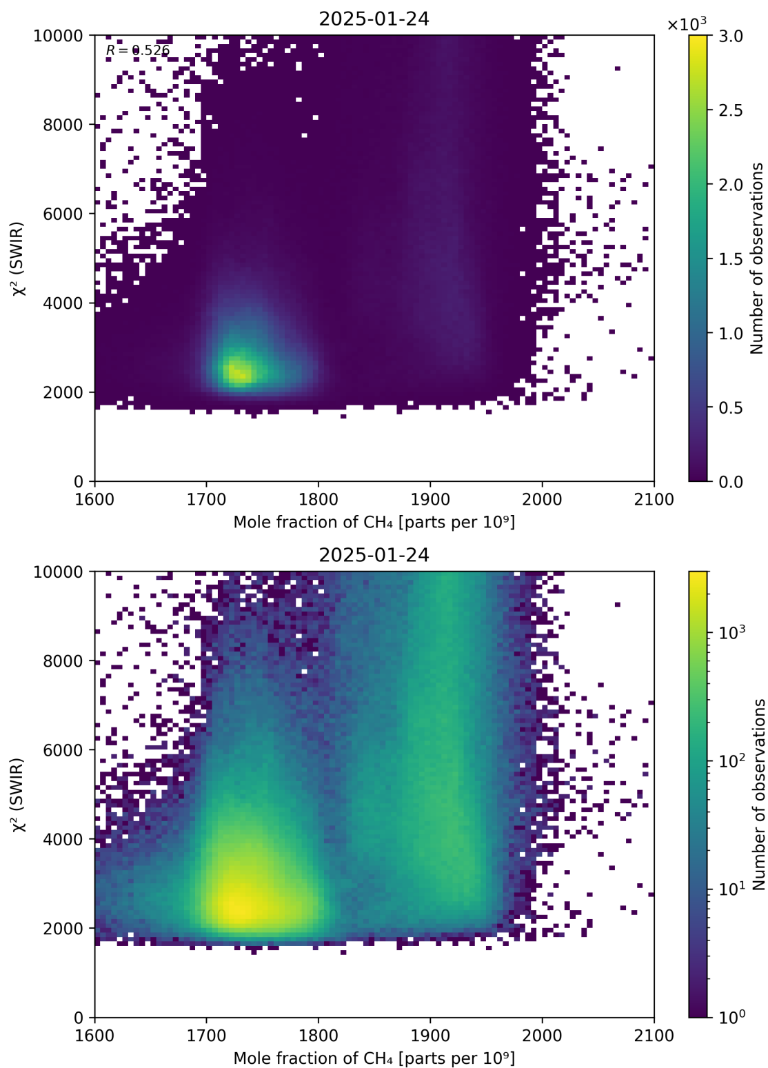
Figure 71: Scatter density plot of “Mole fraction of \text{CH}_4 ” against “ \chi^2 (SWIR)” for 2025-01-23 to 2025-01-25.
