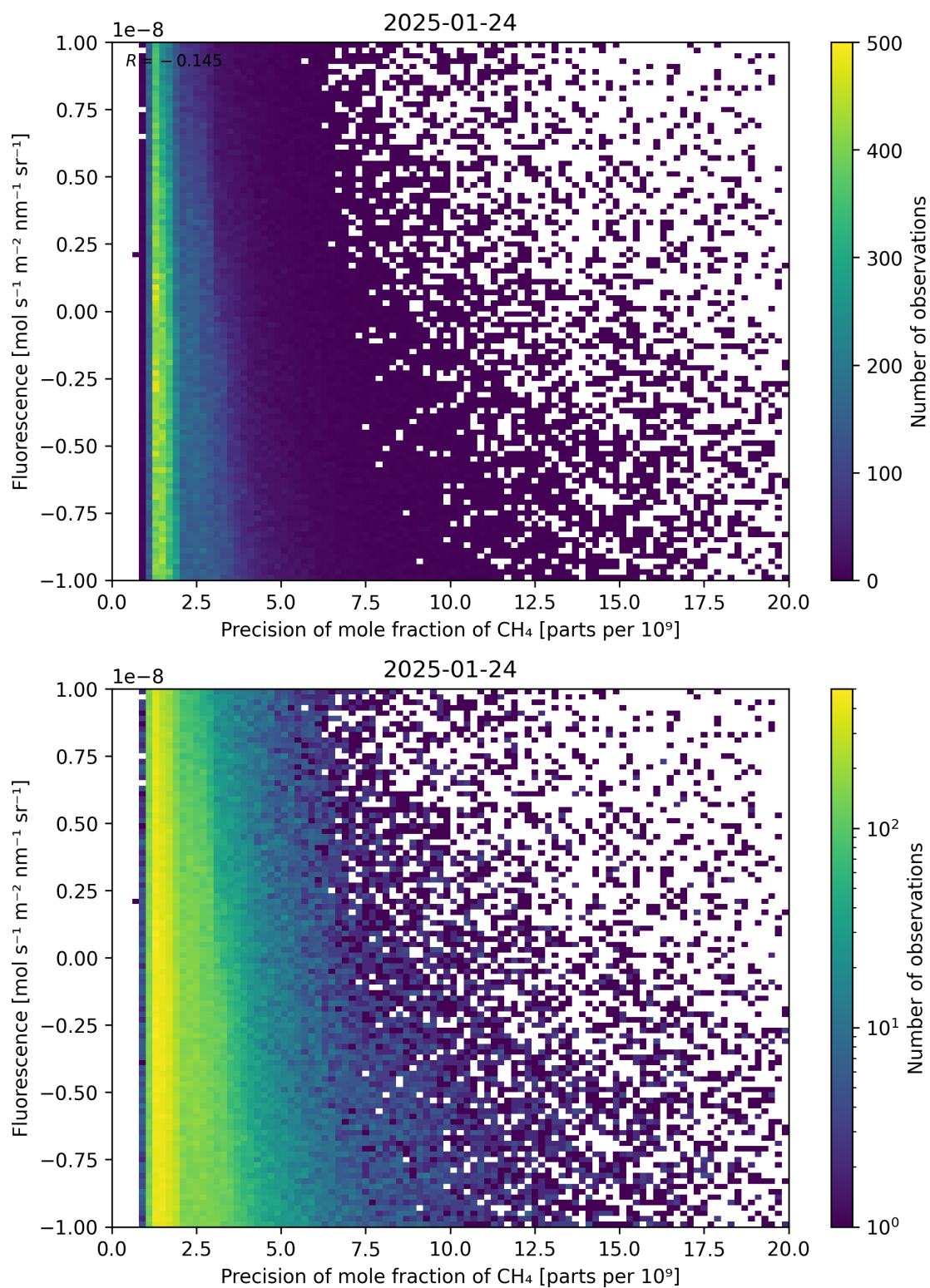
Figure 81: Scatter density plot of “Precision of mole fraction of \text{CH}_4 ” against “Fluorescence” for 2025-01-23 to 2025-01-25.
