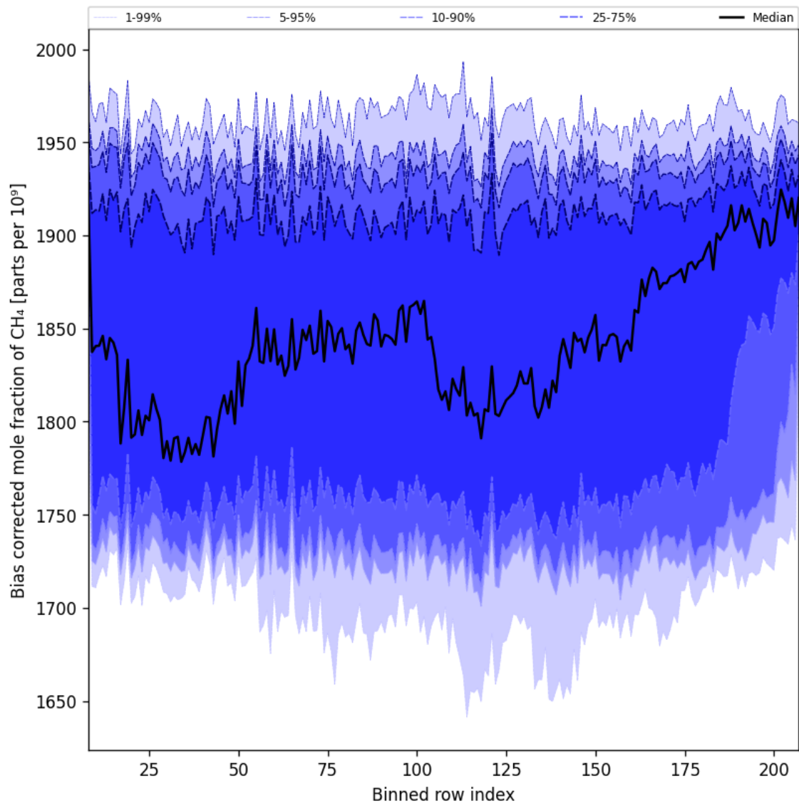
Figure 36: Along track statistics of “Bias corrected mole fraction of CH 4 ” for 2025-01-23 to 2025-01-25
