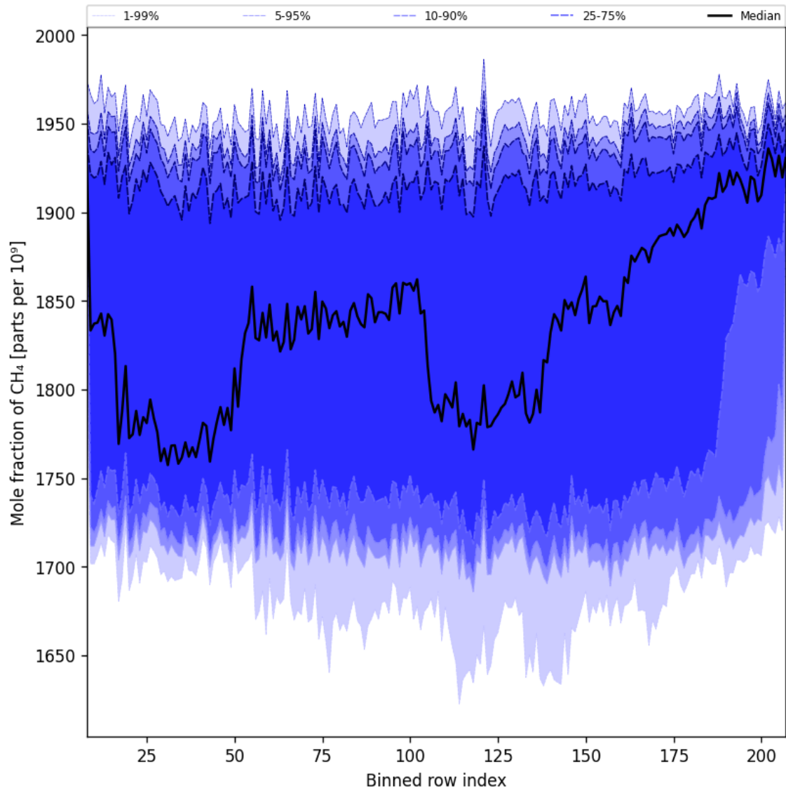
Figure 34: Along track statistics of “Mole fraction of CH 4 ” for 2025-01-23 to 2025-01-25
