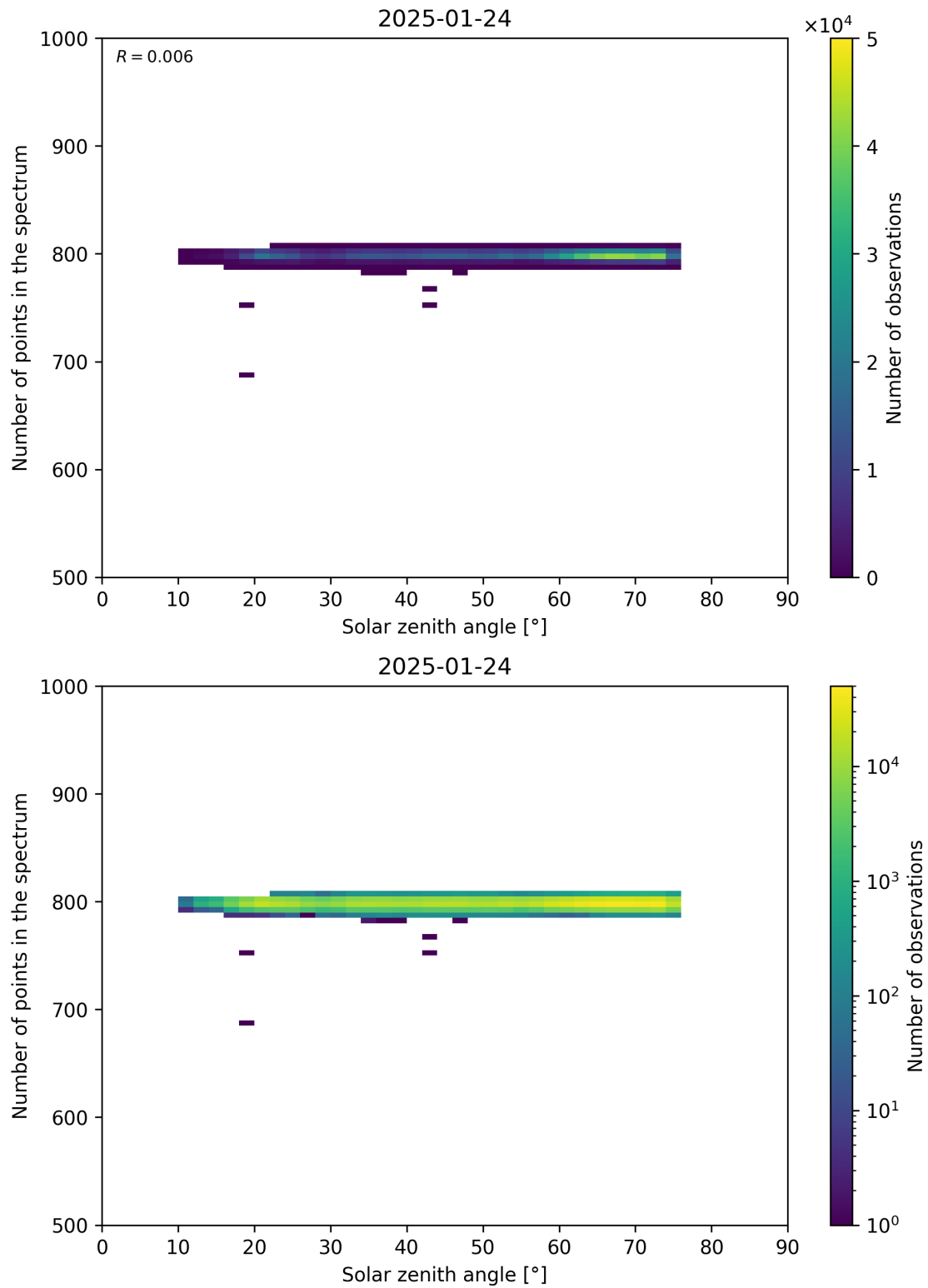
Figure 103: Scatter density plot of “Solar zenith angle” against “Number of points in the spectrum” for 2025-01-23 to 2025-01-25.
