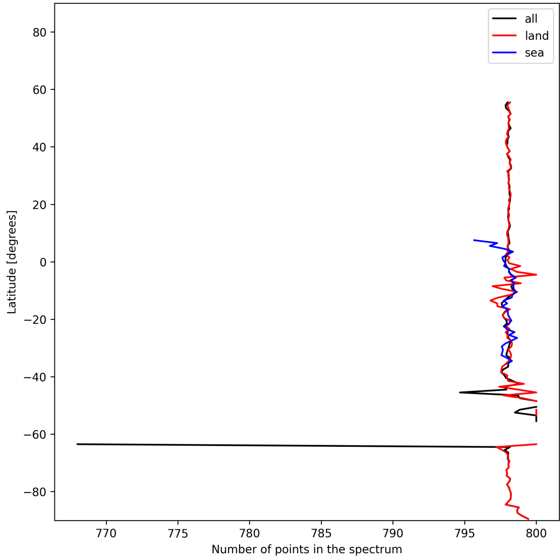
Figure 15: Zonal average of “Number of points in the spectrum” for 2025-01-23 to 2025-01-25.
