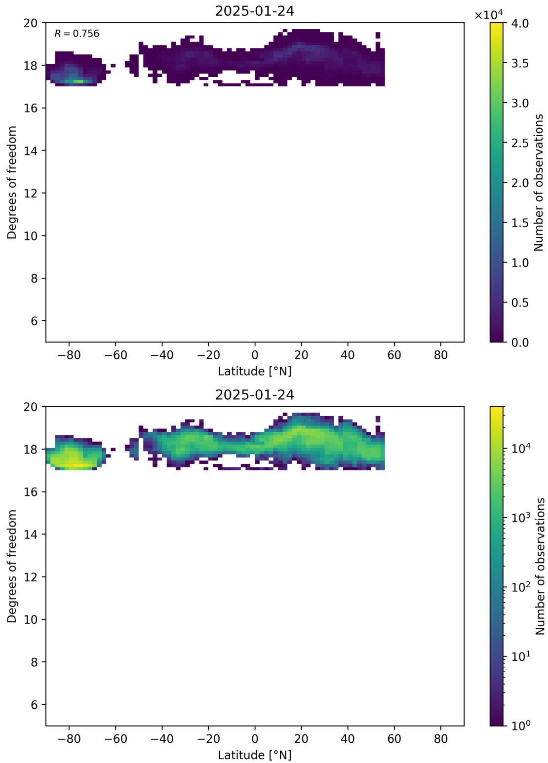
Figure 55: Scatter density plot of “Latitude” against “Degrees of freedom” for 2025-01-23 to 2025-01-25.
