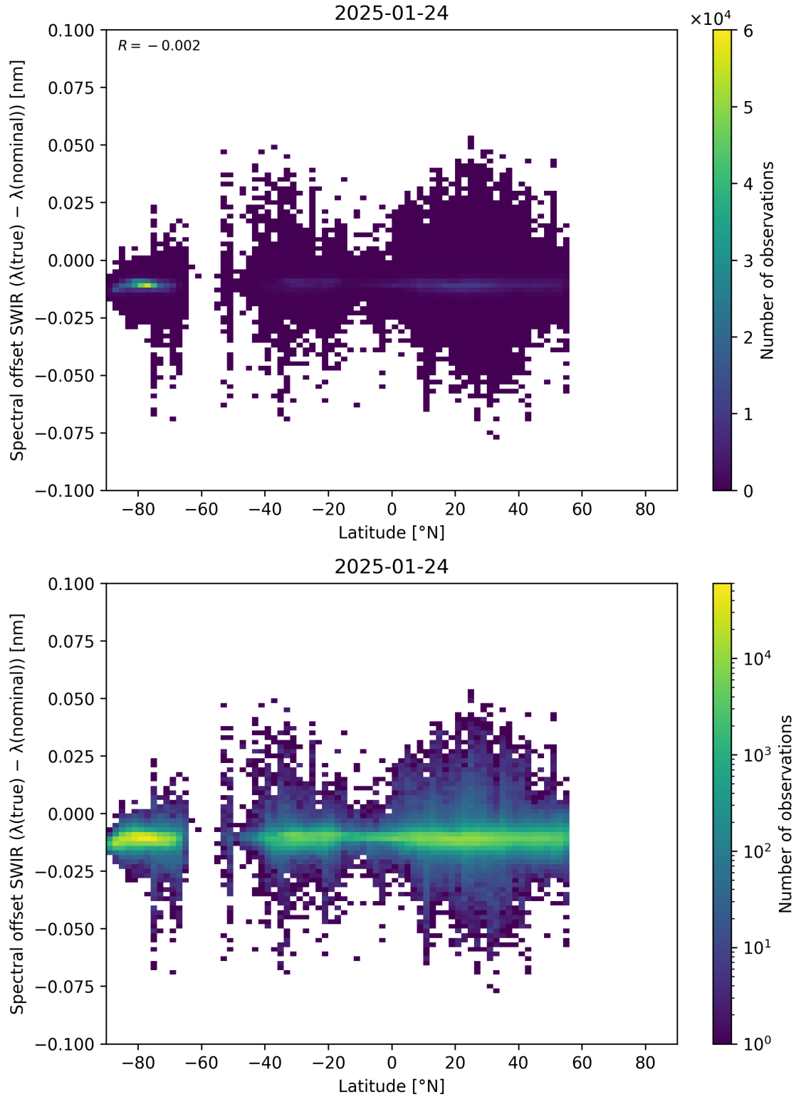
Figure 62: Scatter density plot of “Latitude” against “Spectral offset SWIR ( \lambda_{\text{true}} - \lambda_{\text{nominal}} )” for 2025-01-23 to 2025-01-25.
