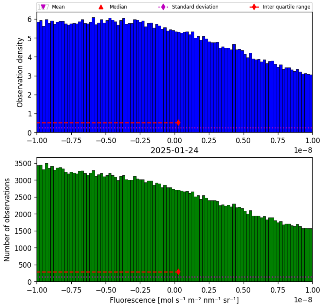
Figure 32: Histogram of “Fluorescence” for 2025-01-23 to 2025-01-25
