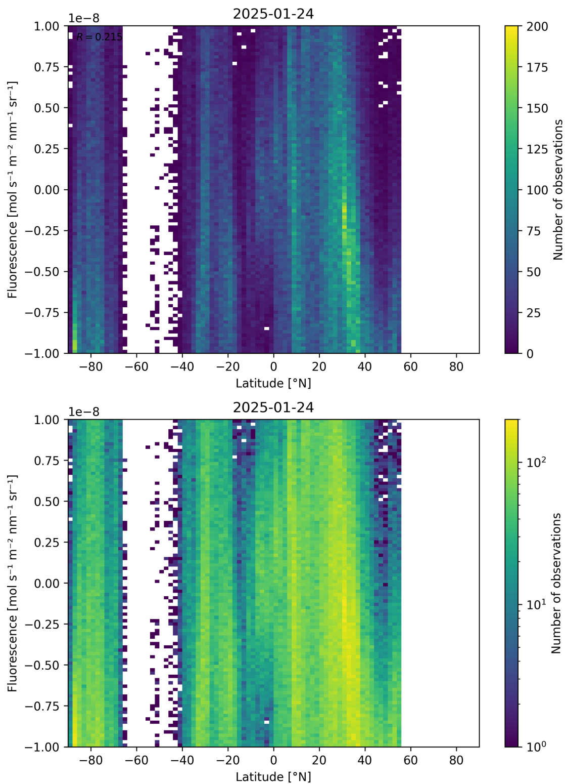
Figure 56: Scatter density plot of “Latitude” against “Fluorescence” for 2025-01-23 to 2025-01-25.
