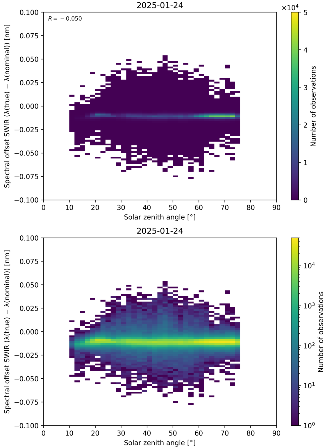
Figure 104: Scatter density plot of “Solar zenith angle” against “Spectral offset SWIR ( \lambda_{\text{true}} - \lambda_{\text{nominal}} )” for 2025-01-23 to 2025-01-25.
