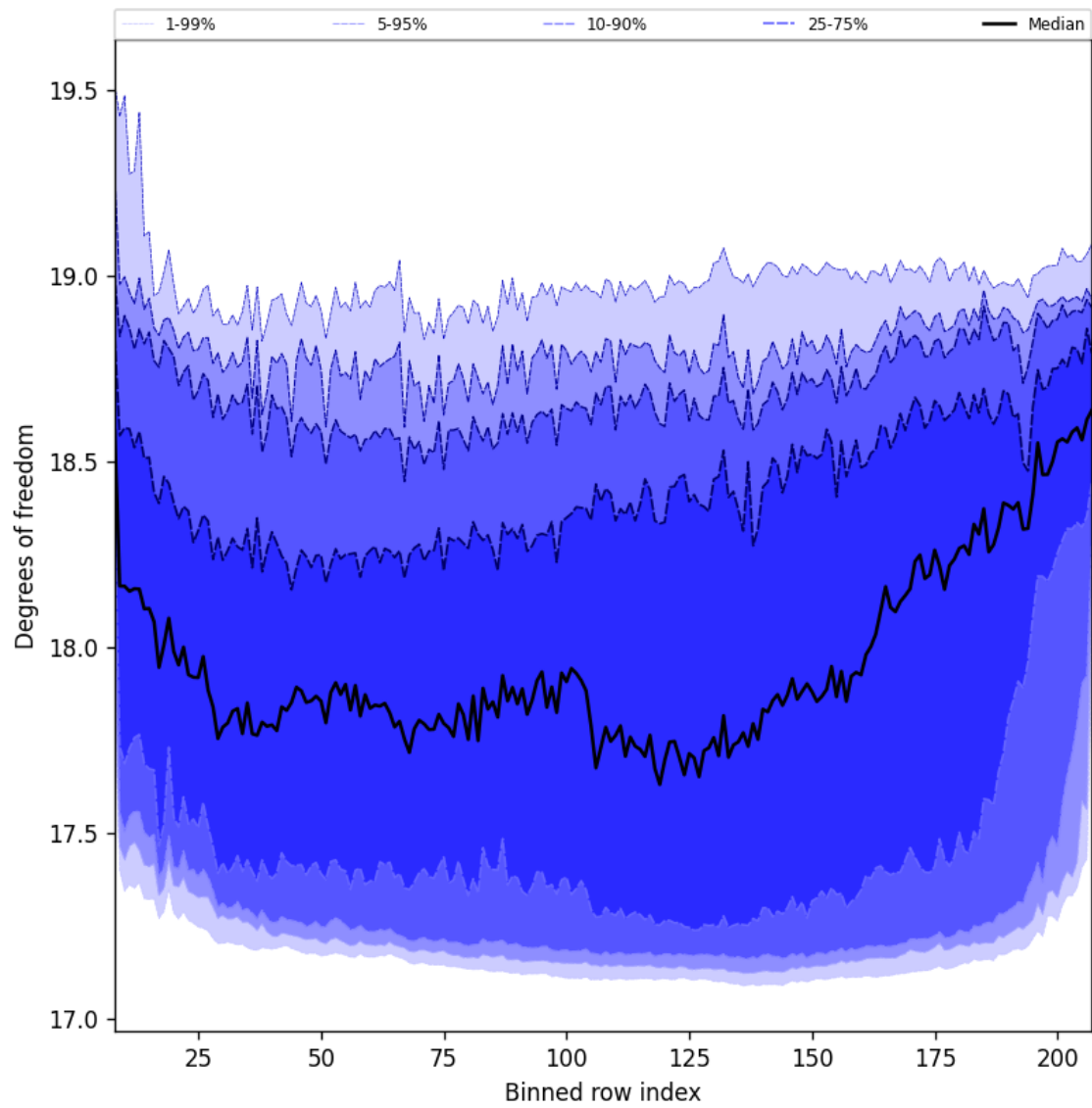
Figure 41: Along track statistics of “Degrees of freedom” for 2025-01-23 to 2025-01-25
