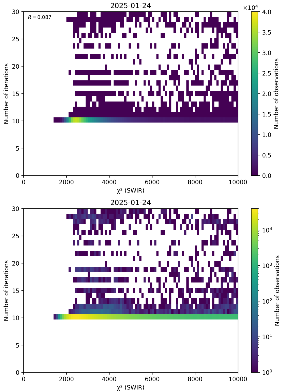
Figure 50: Scatter density plot of “ \chi^2 (SWIR)” against “Number of iterations” for 2025-01-23 to 2025-01-25.
