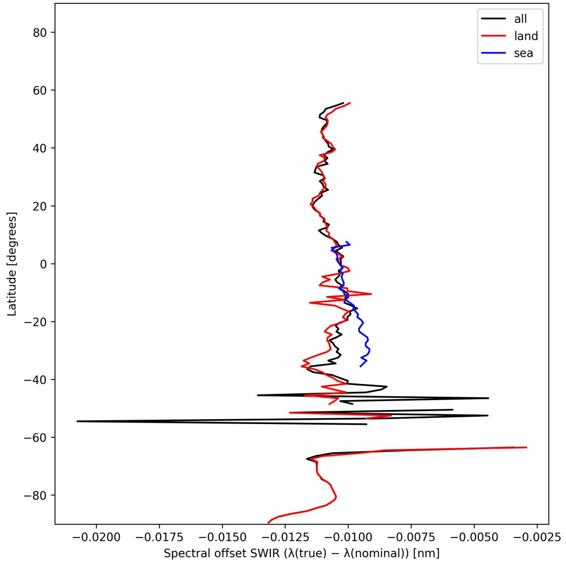
Figure 16: Zonal average of “Spectral offset SWIR ( \lambda_{\text{true}} - \lambda_{\text{nominal}} )” for 2025-01-23 to 2025-01-25.
