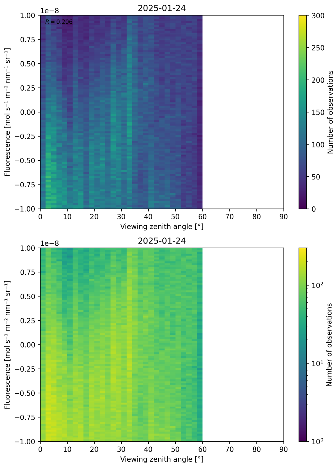
Figure 108: Scatter density plot of “Viewing zenith angle” against “Fluorescence” for 2025-01-23 to 2025-01-25.
