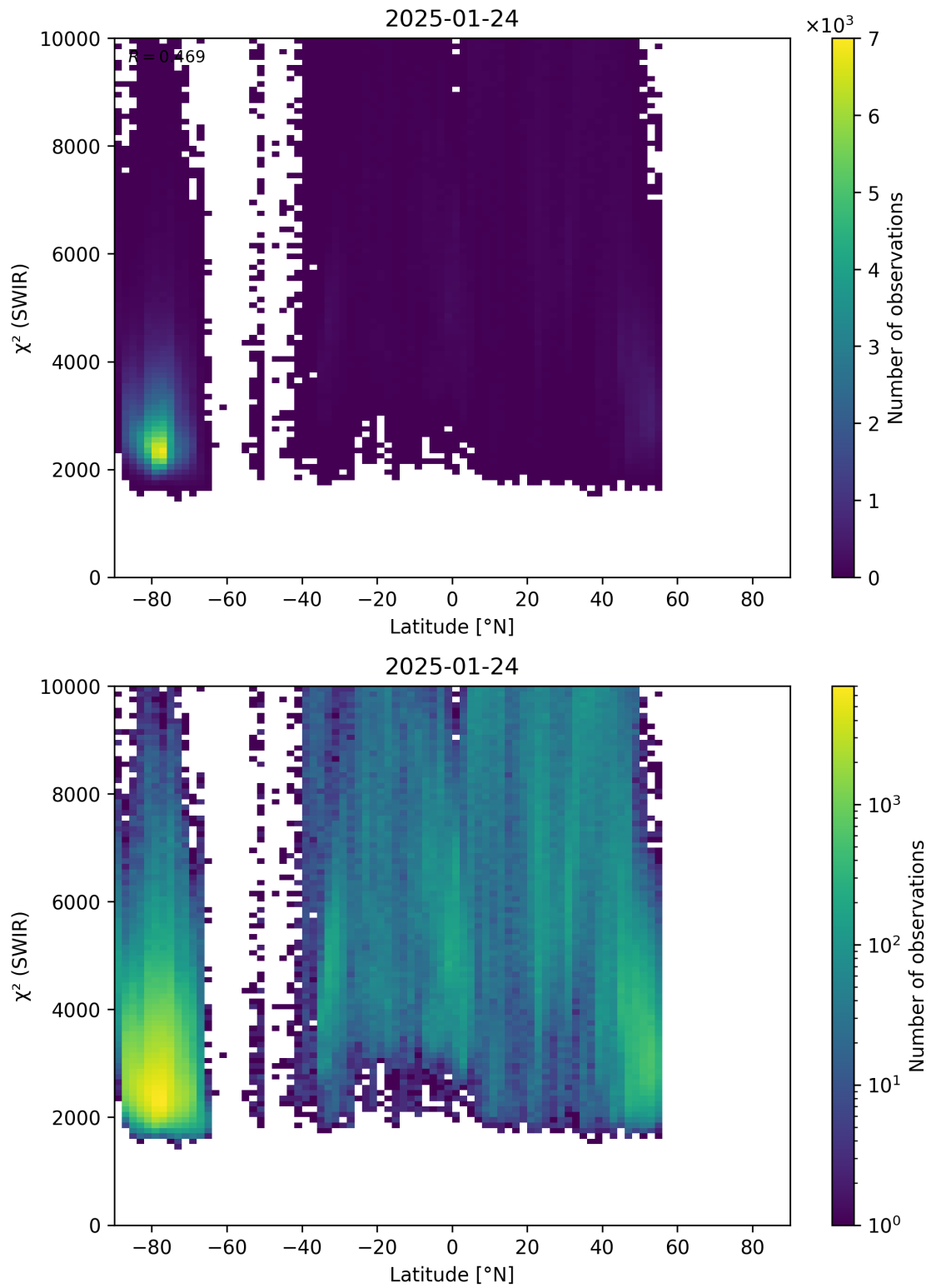
Figure 54: Scatter density plot of “Latitude” against “ \chi^2 (SWIR)” for 2025-01-23 to 2025-01-25.
