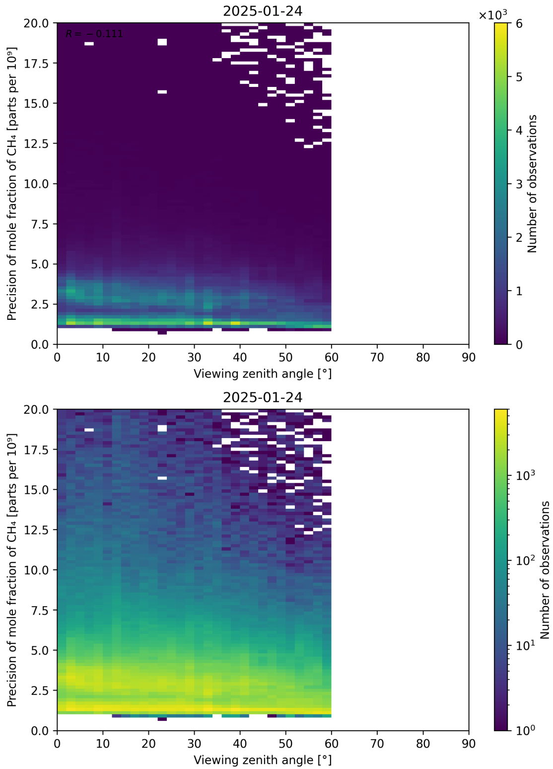
Figure 112: Scatter density plot of “Viewing zenith angle” against “Precision of mole fraction of \text{CH}_4 ” for 2025-01-23 to 2025-01-25.
