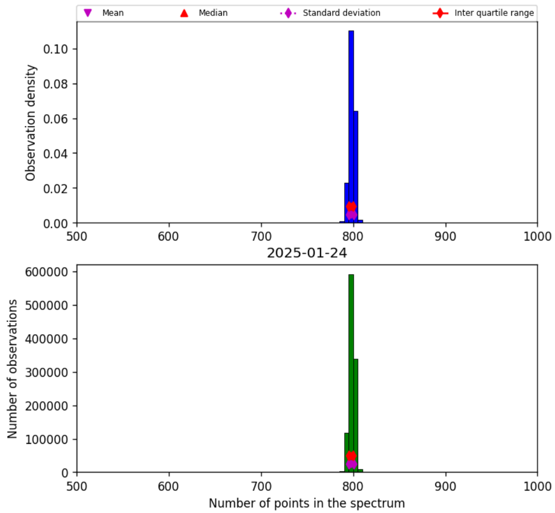
Figure 26: Histogram of “Number of points in the spectrum” for 2025-01-23 to 2025-01-25
