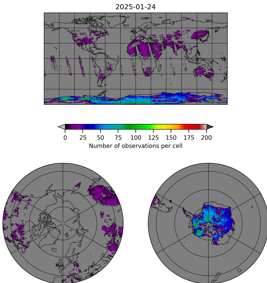
Figure 10: Map of the number of observations for 2025-01-23 to 2025-01-25
