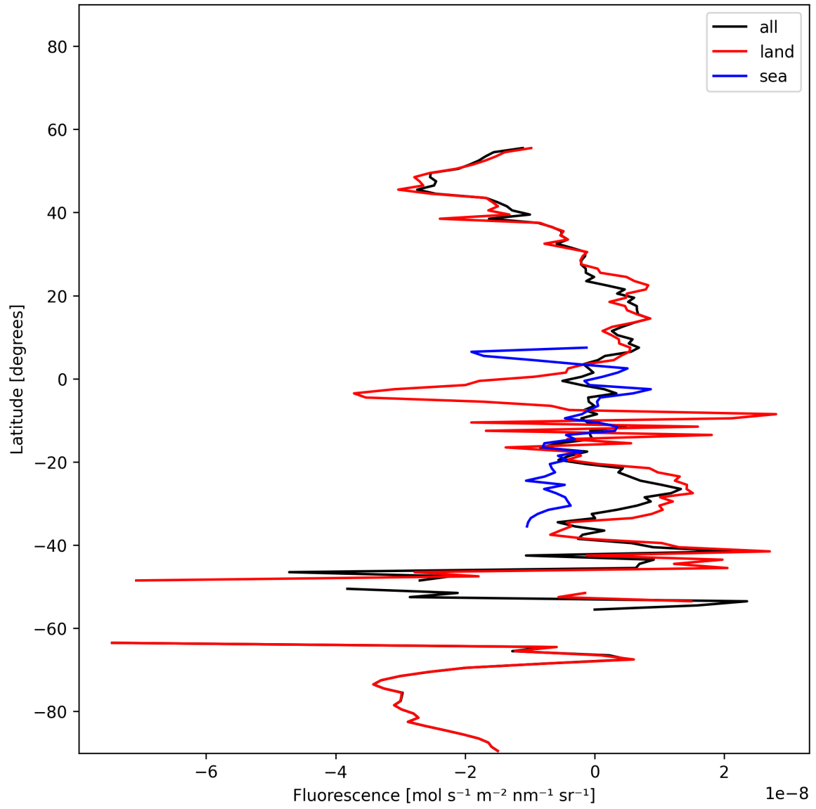
Figure 21: Zonal average of “Fluorescence” for 2025-01-23 to 2025-01-25.
