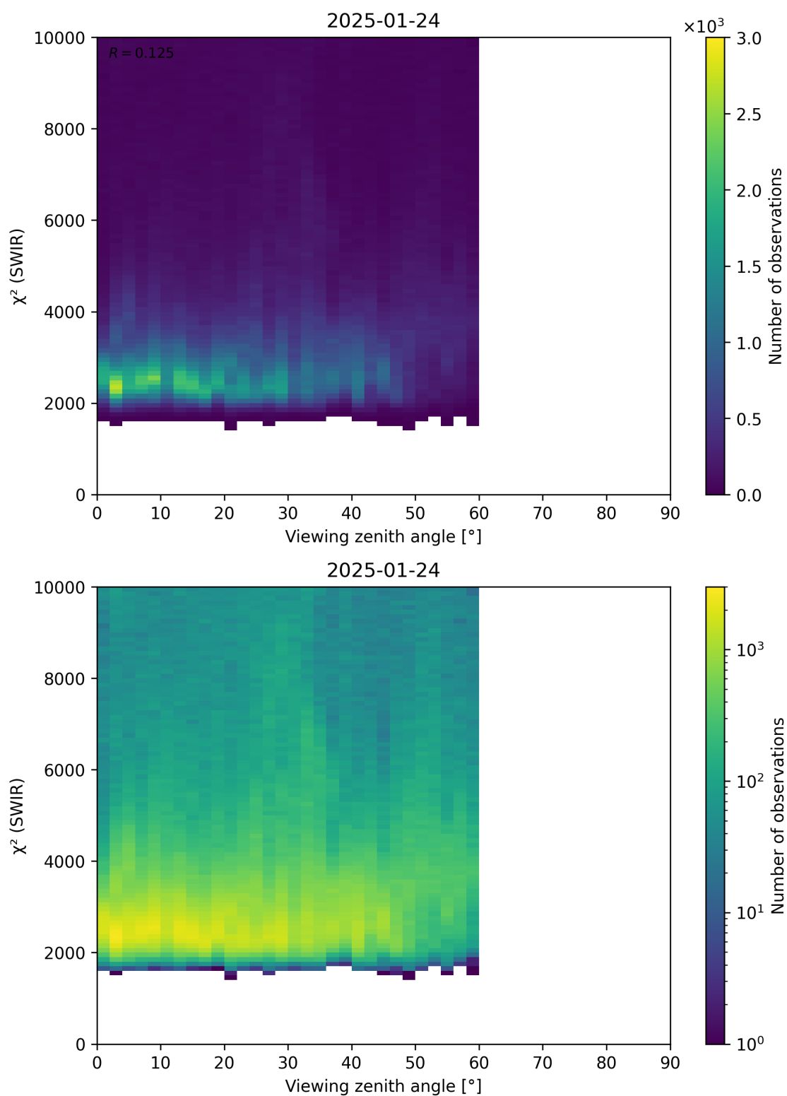
Figure 106: Scatter density plot of “Viewing zenith angle” against “ \chi^2 (SWIR)” for 2025-01-23 to 2025-01-25.
