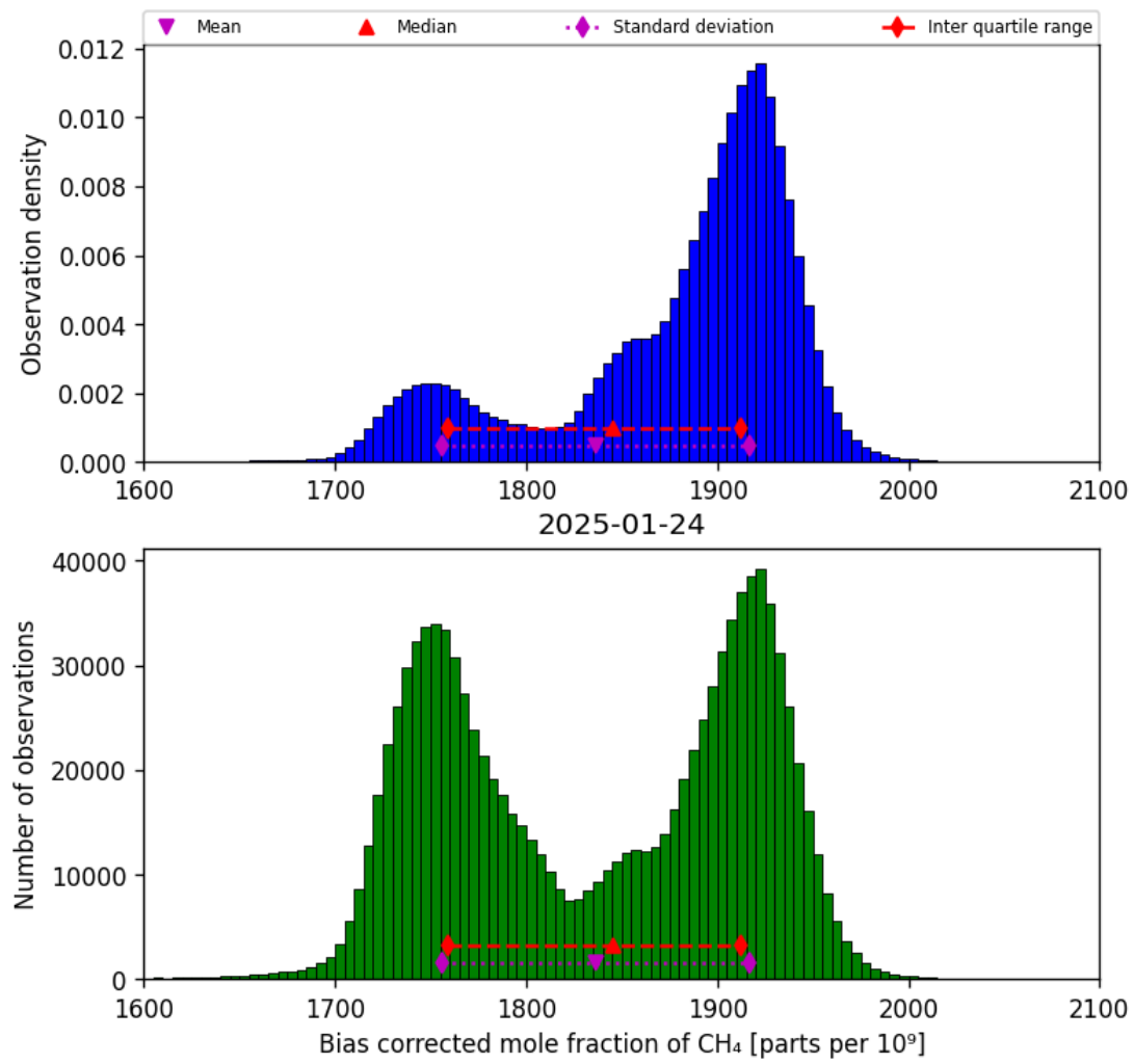
Figure 25: Histogram of “Bias corrected mole fraction of CH 4 ” for 2025-01-23 to 2025-01-25
