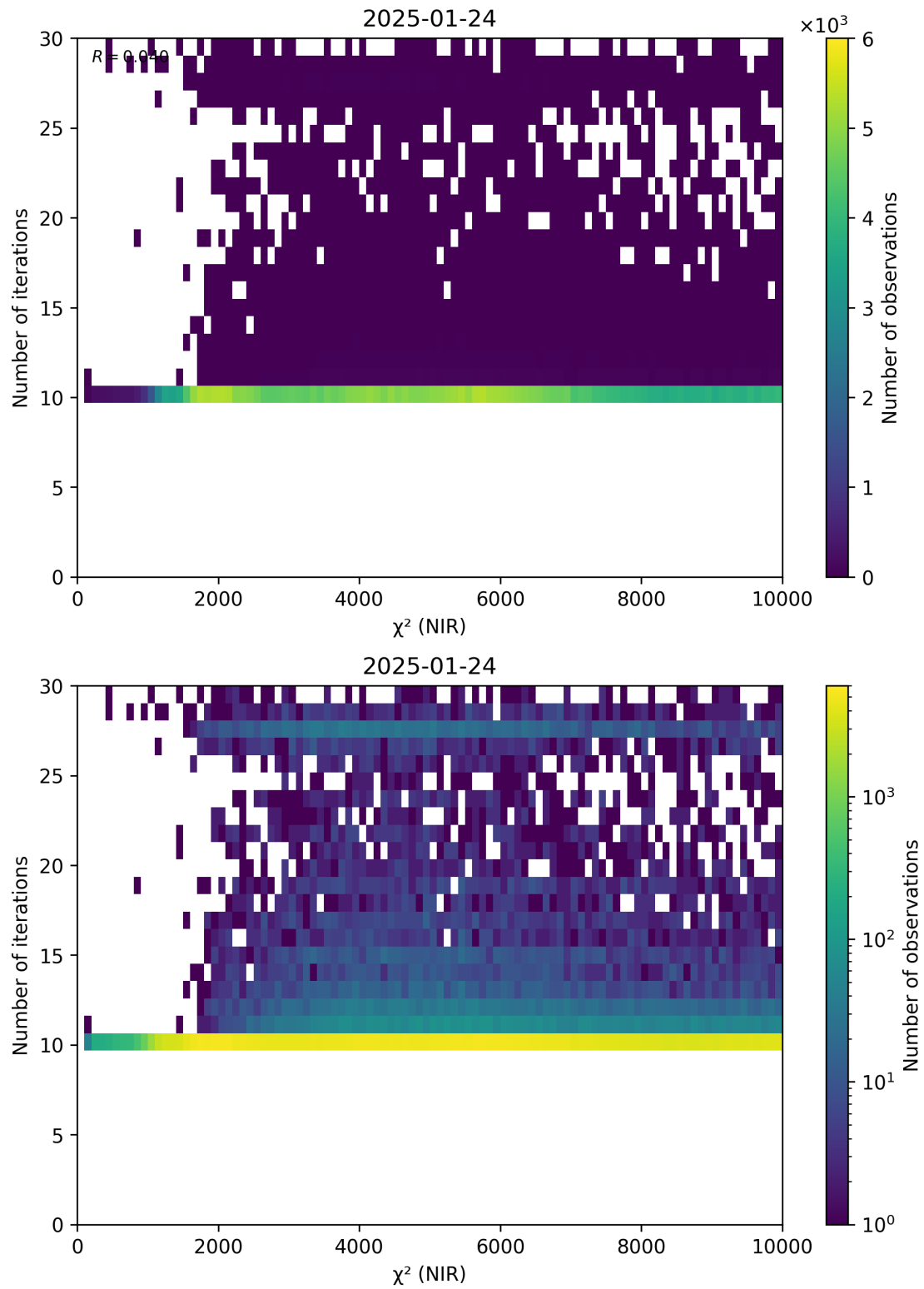
Figure 46: Scatter density plot of “ \chi^2 (NIR)” against “Number of iterations” for 2025-01-23 to 2025-01-25.
