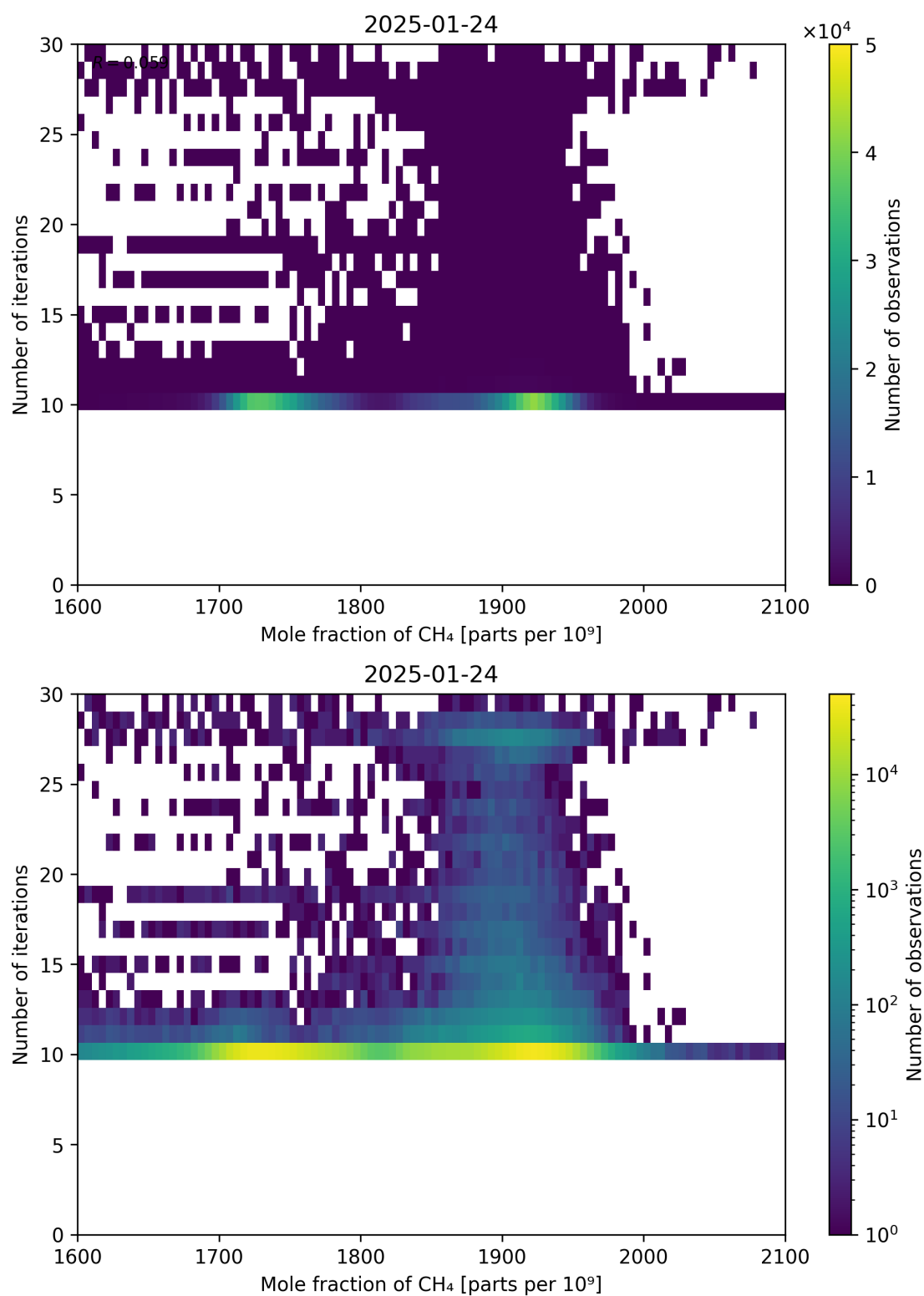
Figure 76: Scatter density plot of “Mole fraction of CH 4 ” against “Number of iterations” for 2025-01-23 to 2025-01-25.
