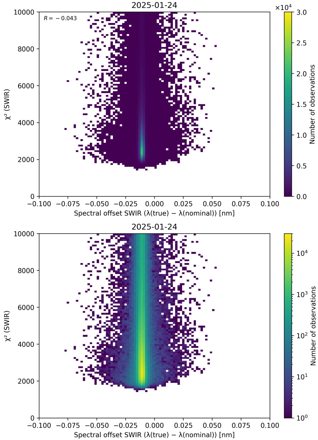
Figure 118: Scatter density plot of “Spectral offset SWIR ( \lambda_{\text{true}} - \lambda_{\text{nominal}} )” against “ \chi^2 (SWIR)” for 2025-01-23 to 2025-01-25.
