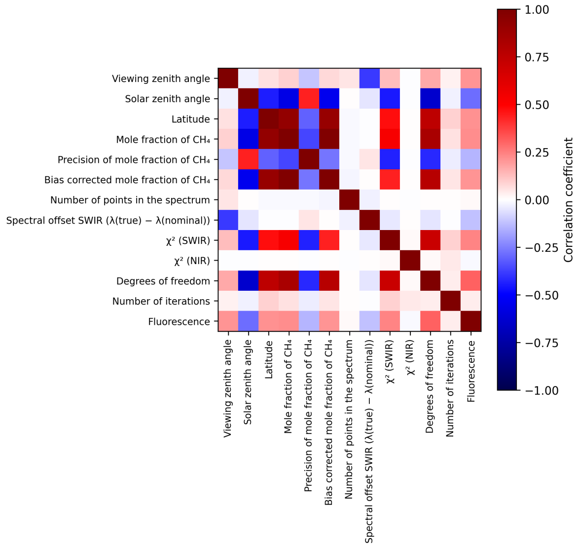
Figure 2: Map of correlation matrix for 2025-01-23 to 2025-01-25.
