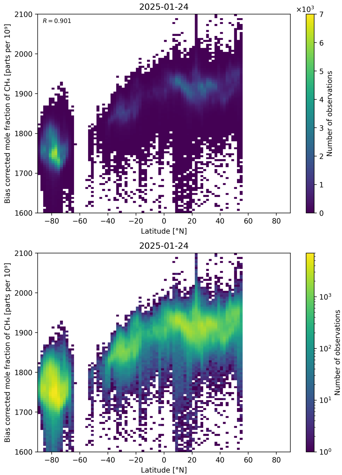
Figure 58: Scatter density plot of “Latitude” against “Bias corrected mole fraction of CH 4 ” for 2025-01-23 to 2025-01-25.
