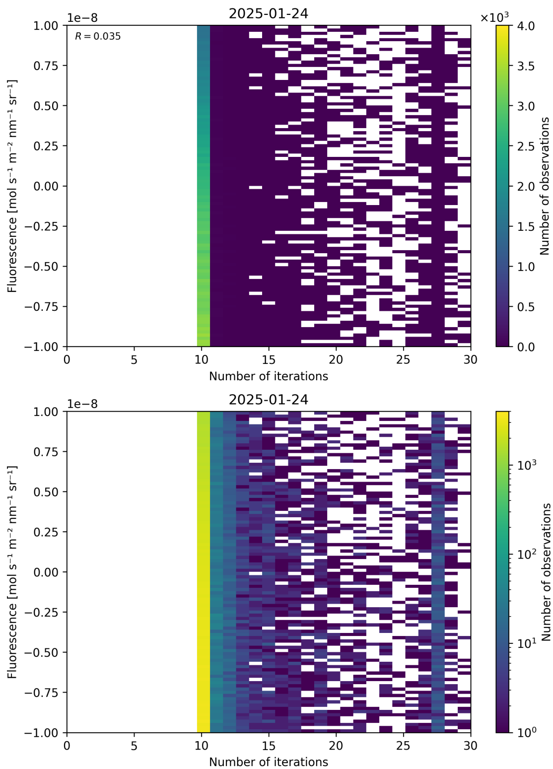
Figure 87: Scatter density plot of “Number of iterations” against “Fluorescence” for 2025-01-23 to 2025-01-25.
