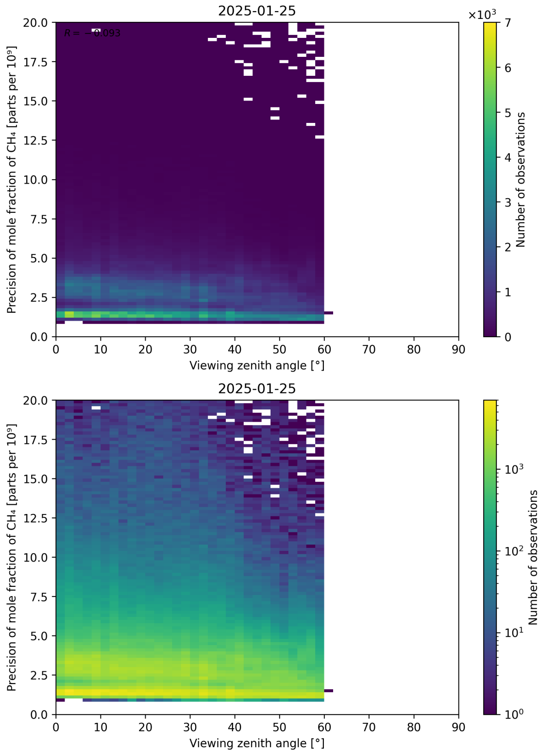
Figure 112: Scatter density plot of “Viewing zenith angle” against “Precision of mole fraction of CH 4 ” for 2025-01-24 to 2025-01-26.
