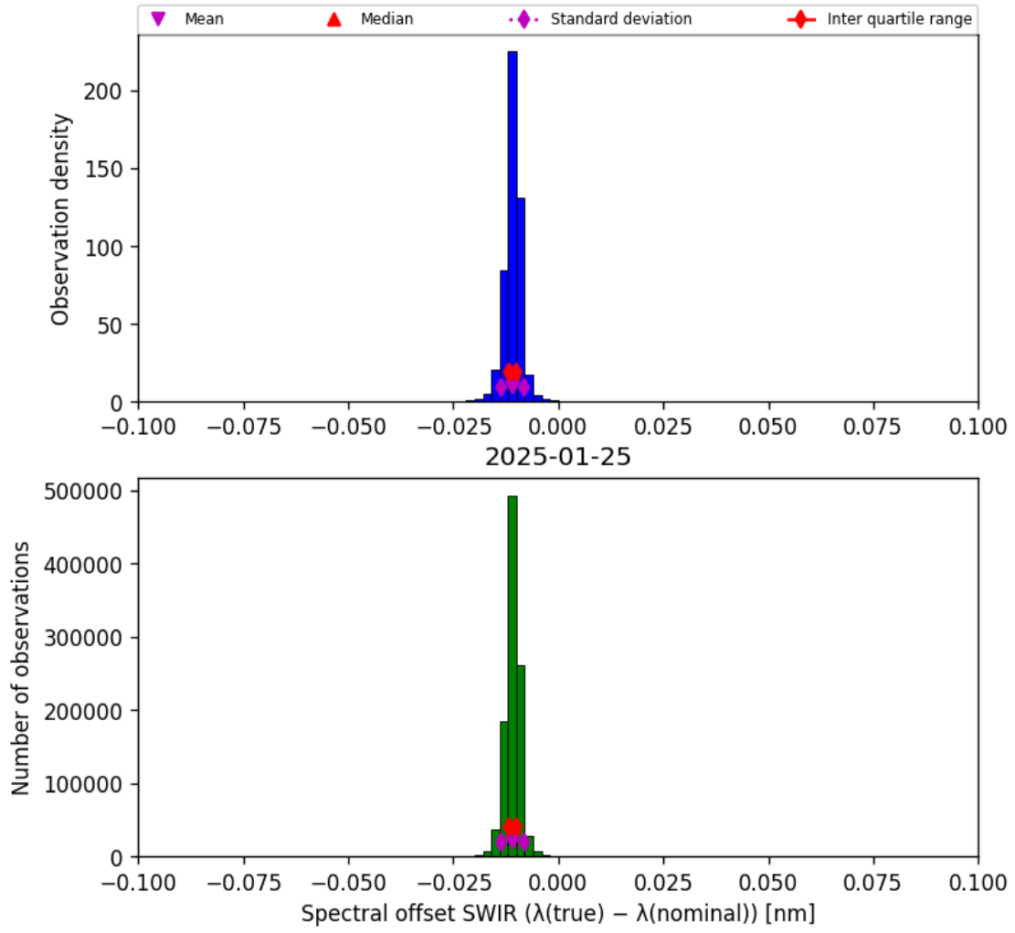
Figure 27: Histogram of “Spectral offset SWIR ( \lambda_{\text{true}} - \lambda_{\text{nominal}} )” for 2025-01-24 to 2025-01-26
