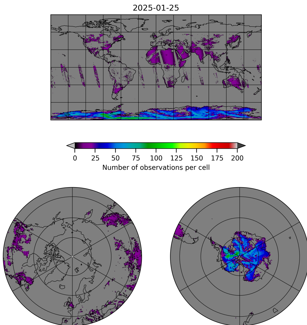
Figure 10: Map of the number of observations for 2025-01-24 to 2025-01-26
