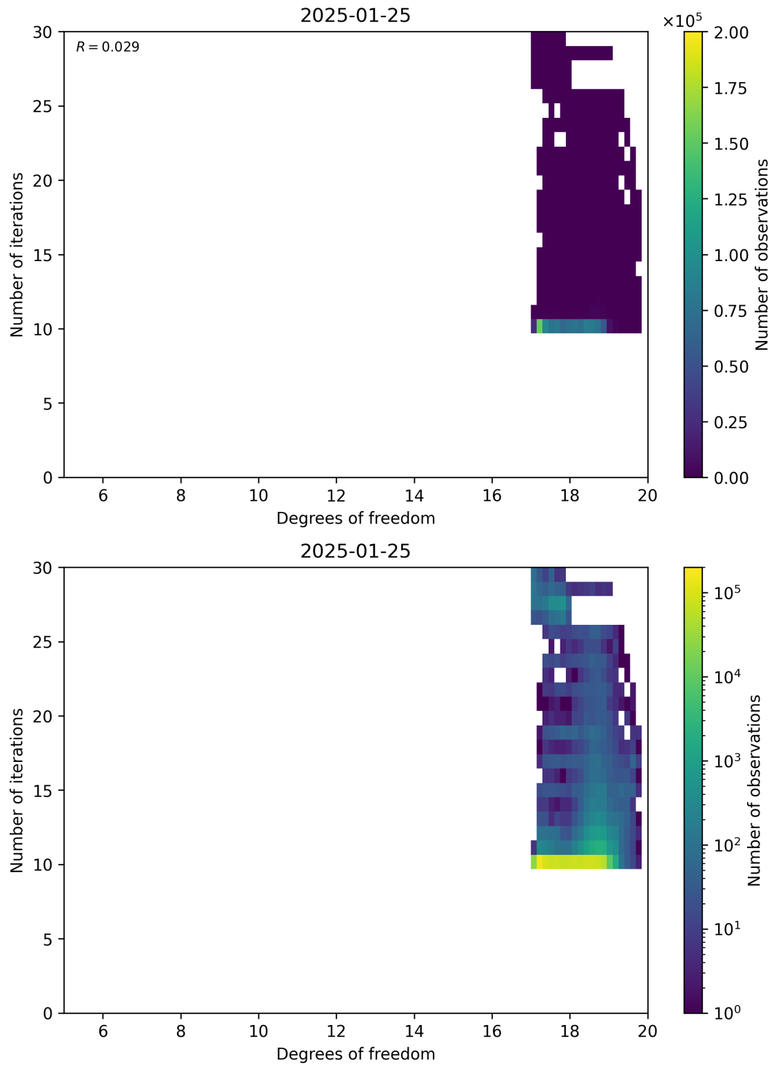
Figure 52: Scatter density plot of “Degrees of freedom” against “Number of iterations” for 2025-01-24 to 2025-01-26.
