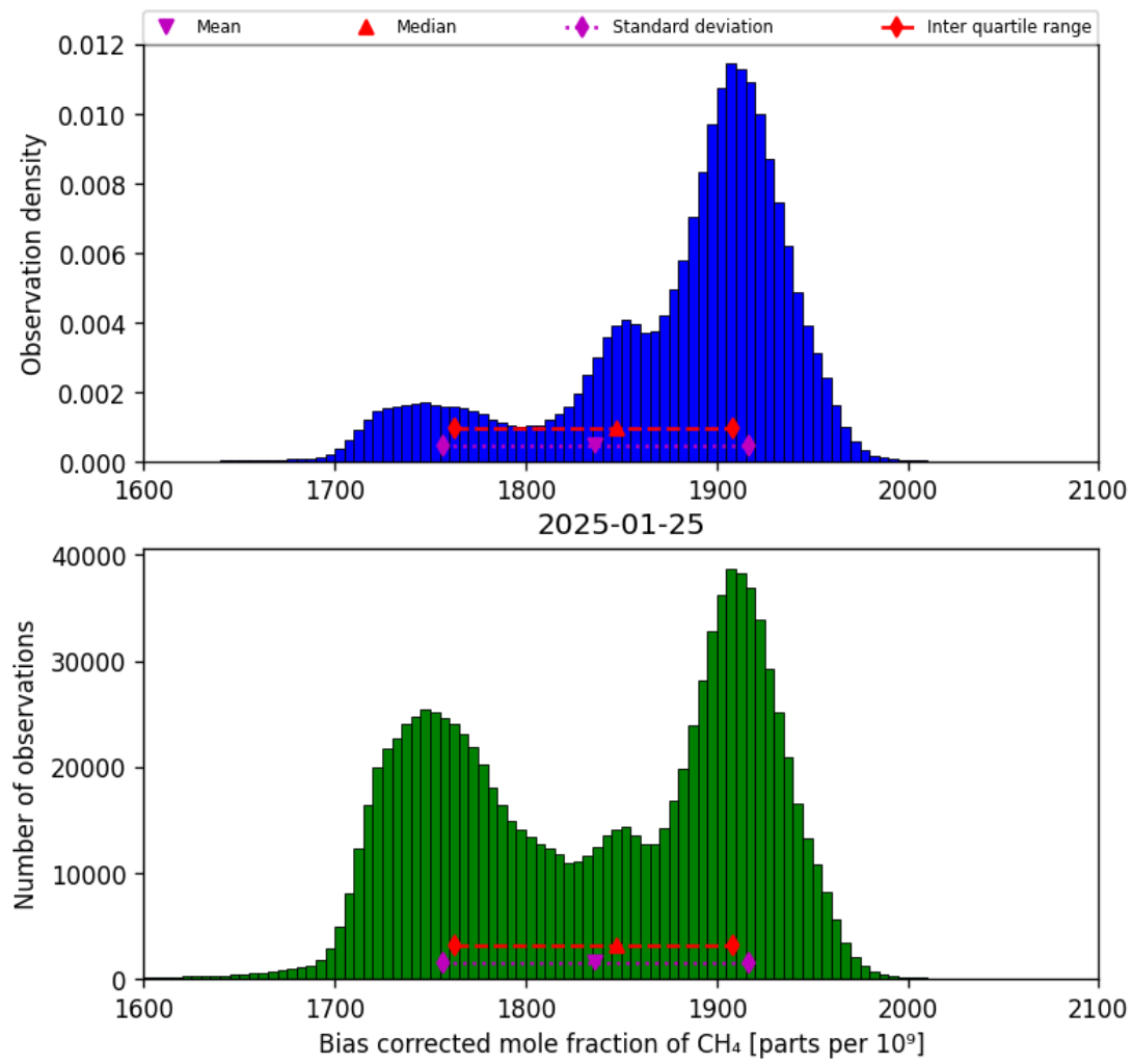
Figure 25: Histogram of “Bias corrected mole fraction of CH 4 ” for 2025-01-24 to 2025-01-26
