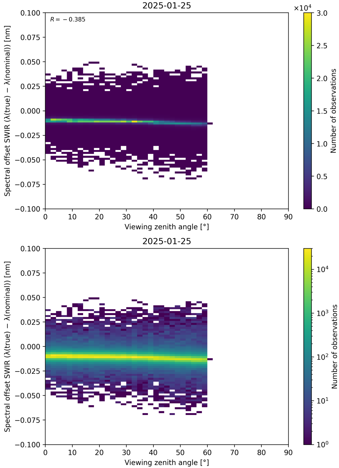
Figure 116: Scatter density plot of “Viewing zenith angle” against “Spectral offset SWIR ( \lambda_{\text{true}} - \lambda_{\text{nominal}} )” for 2025-01-24 to 2025-01-26.
