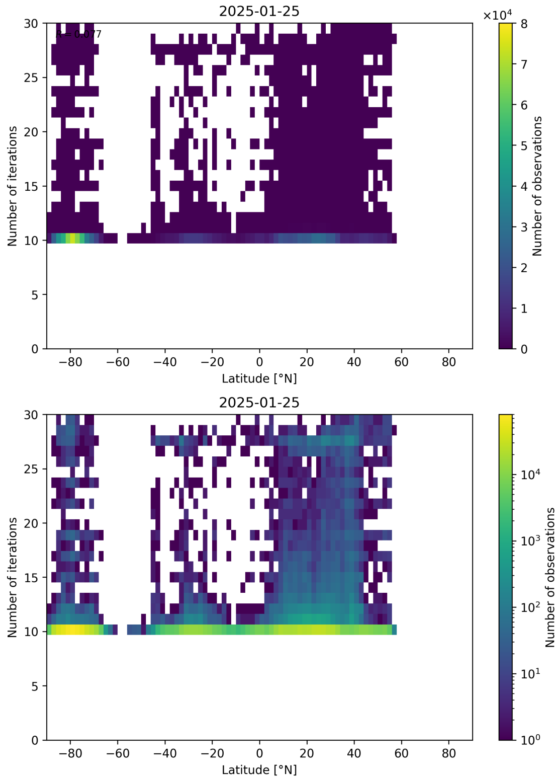
Figure 60: Scatter density plot of “Latitude” against “Number of iterations” for 2025-01-24 to 2025-01-26.
