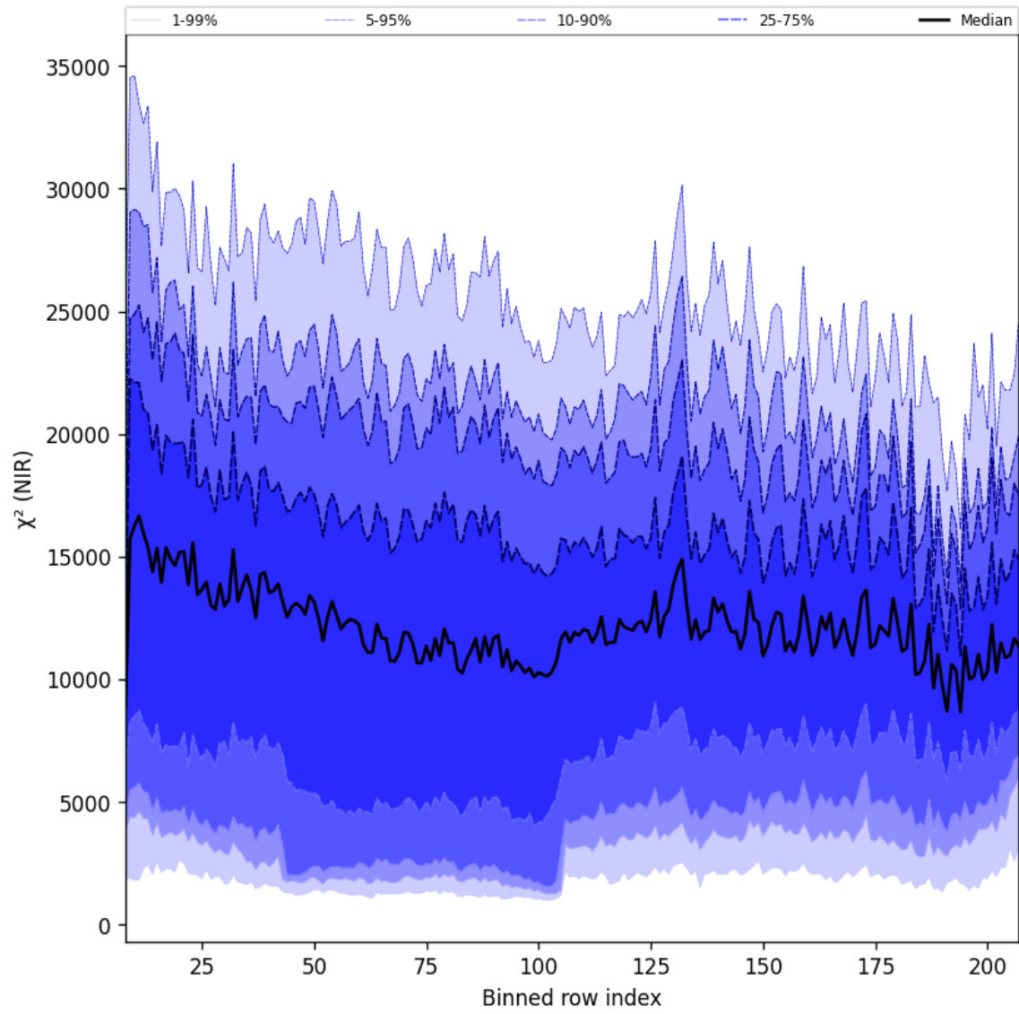
Figure 40: Along track statistics of “ \chi^2 (NIR)” for 2025-01-24 to 2025-01-26
