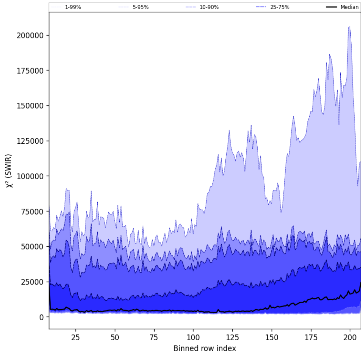
Figure 39: Along track statistics of “ \chi^2 (SWIR)” for 2025-01-24 to 2025-01-26
