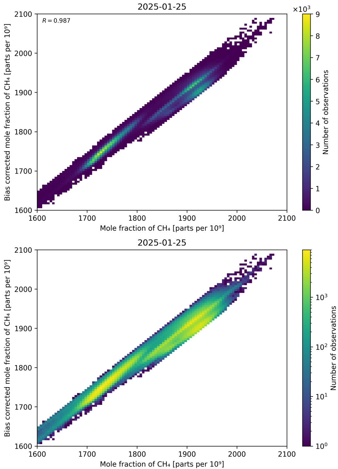
Figure 74: Scatter density plot of “Mole fraction of CH 4 ” against “Bias corrected mole fraction of CH 4 ” for 2025-01-24 to 2025-01-26.
