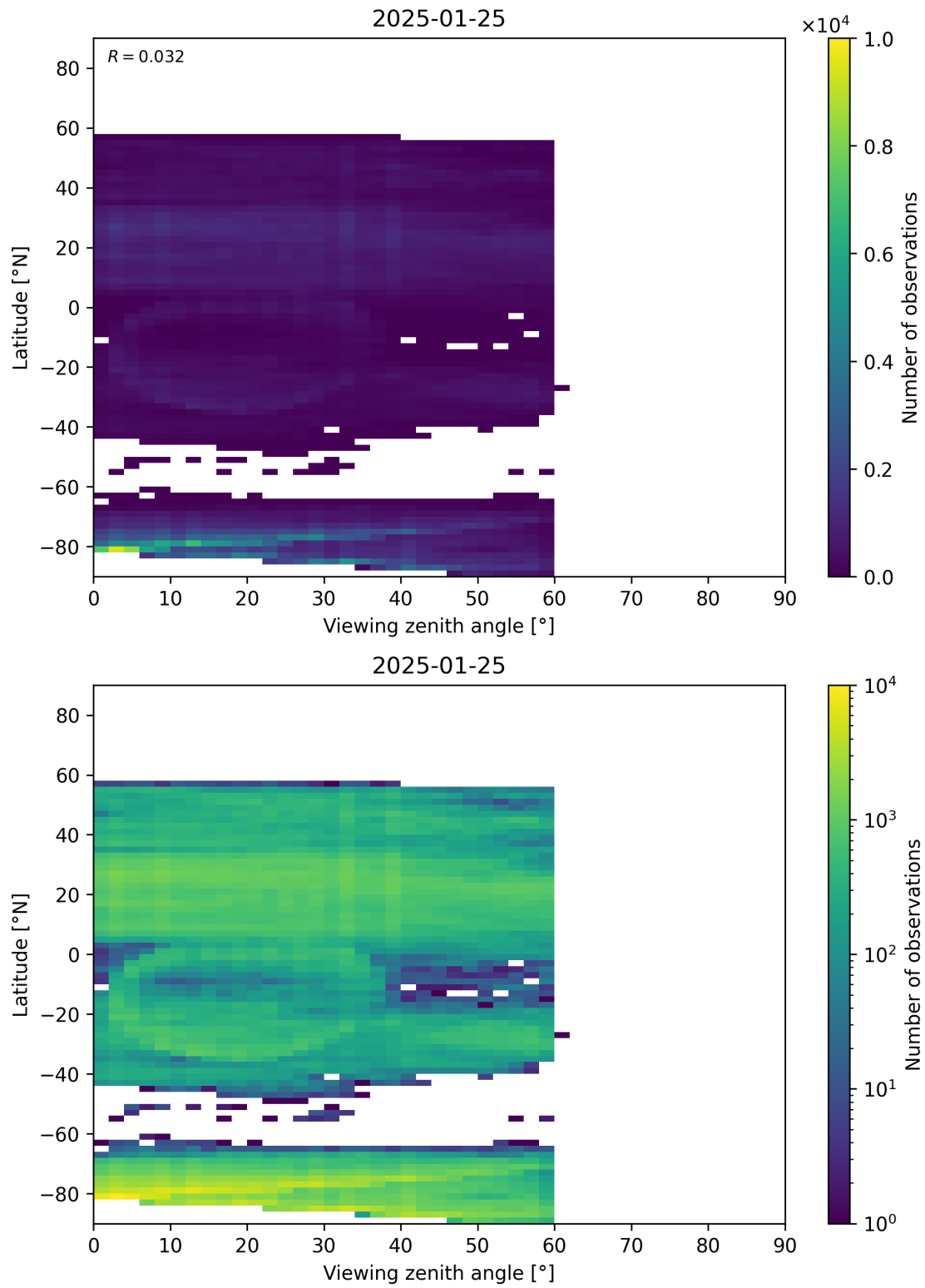
Figure 109: Scatter density plot of “Viewing zenith angle” against “Latitude” for 2025-01-24 to 2025-01-26.
