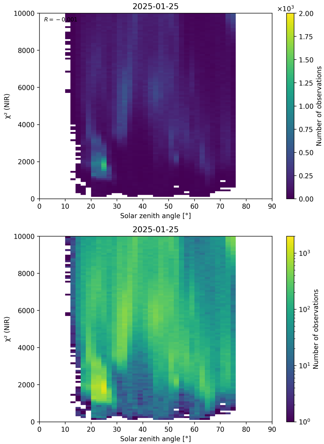
Figure 94: Scatter density plot of “Solar zenith angle” against “ \chi^2 (NIR)” for 2025-01-24 to 2025-01-26.
