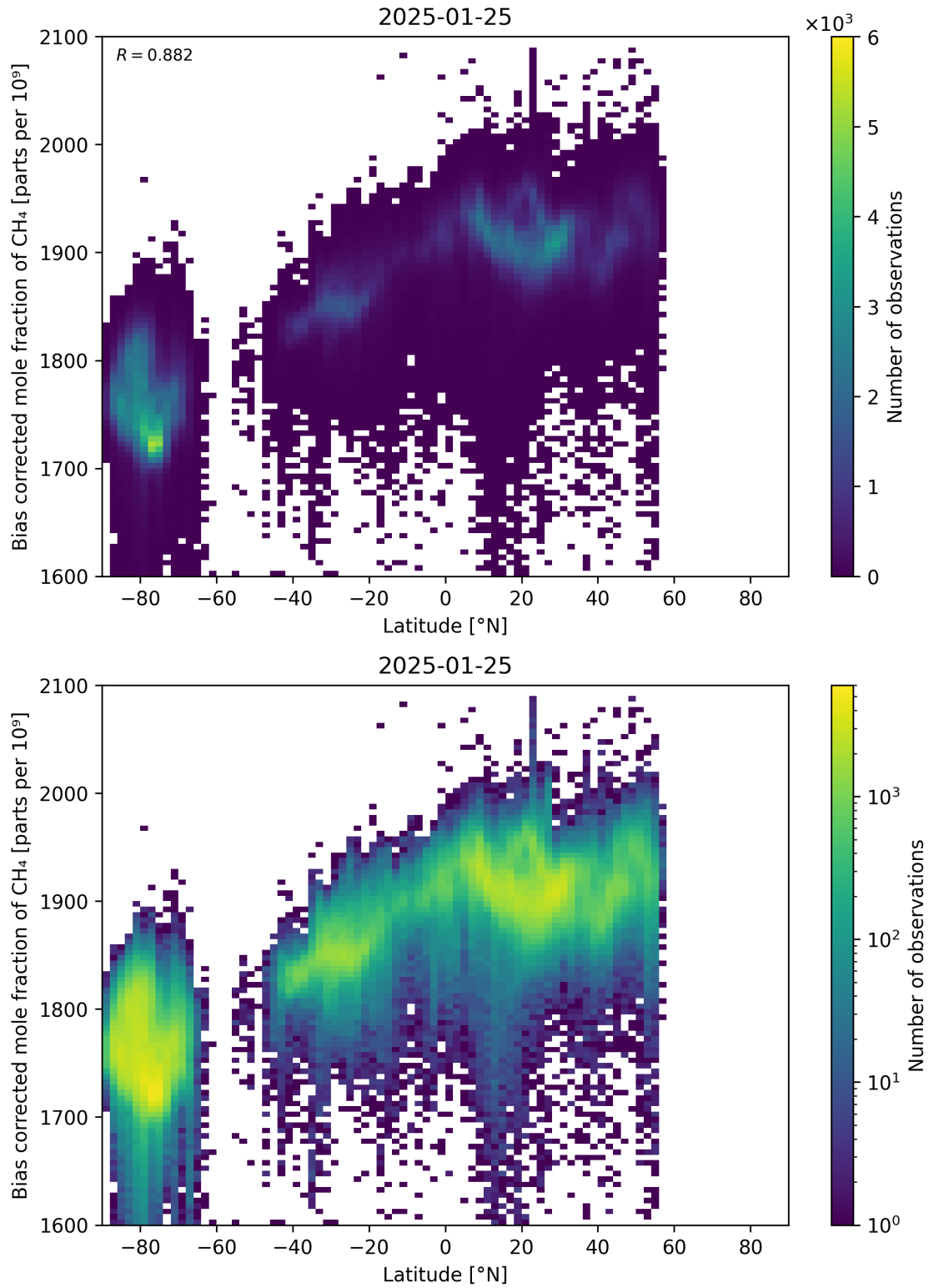
Figure 58: Scatter density plot of “Latitude” against “Bias corrected mole fraction of \text{CH}_4 ” for 2025-01-24 to 2025-01-26.
