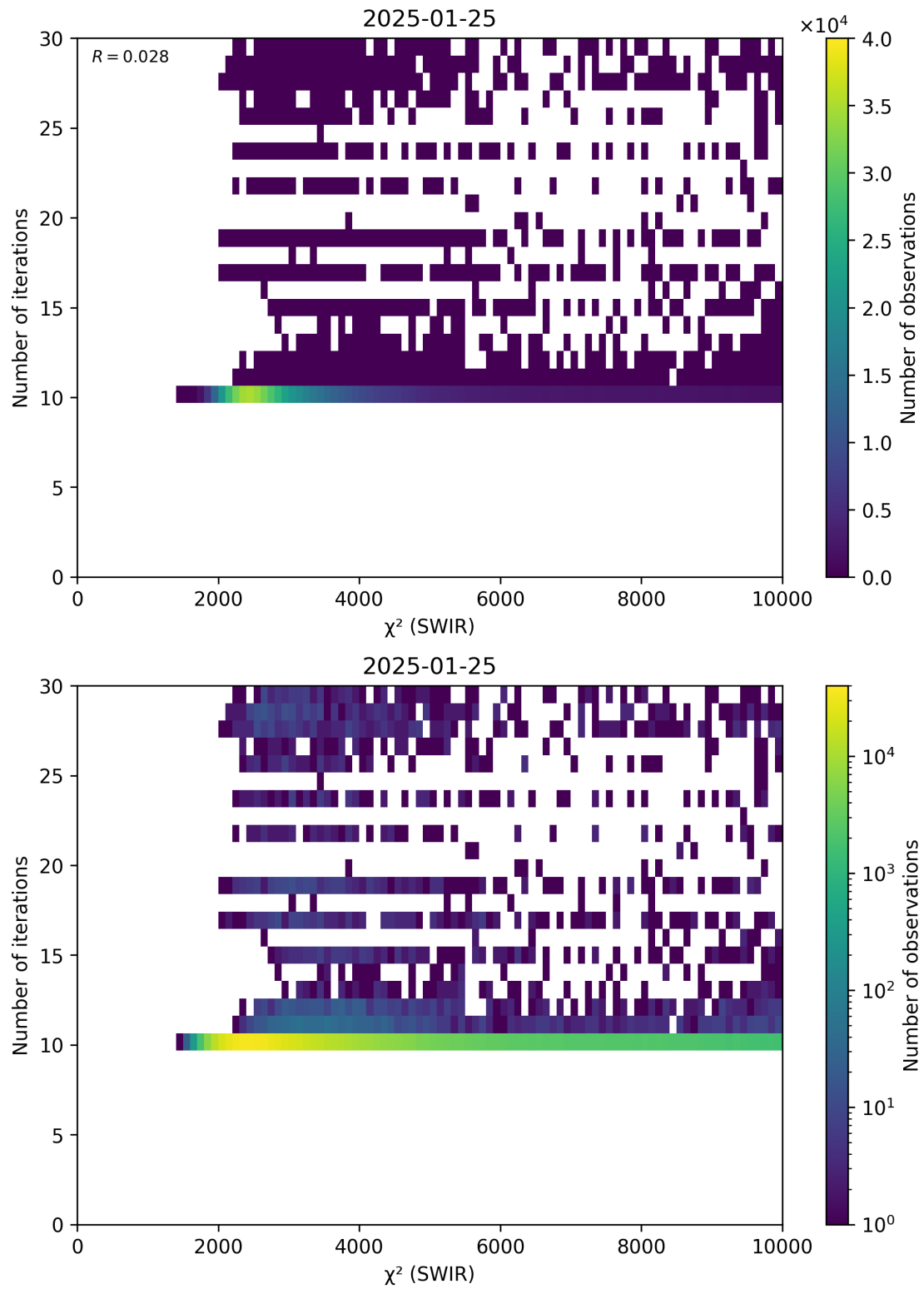
Figure 50: Scatter density plot of “ \chi^2 (SWIR)” against “Number of iterations” for 2025-01-24 to 2025-01-26.
