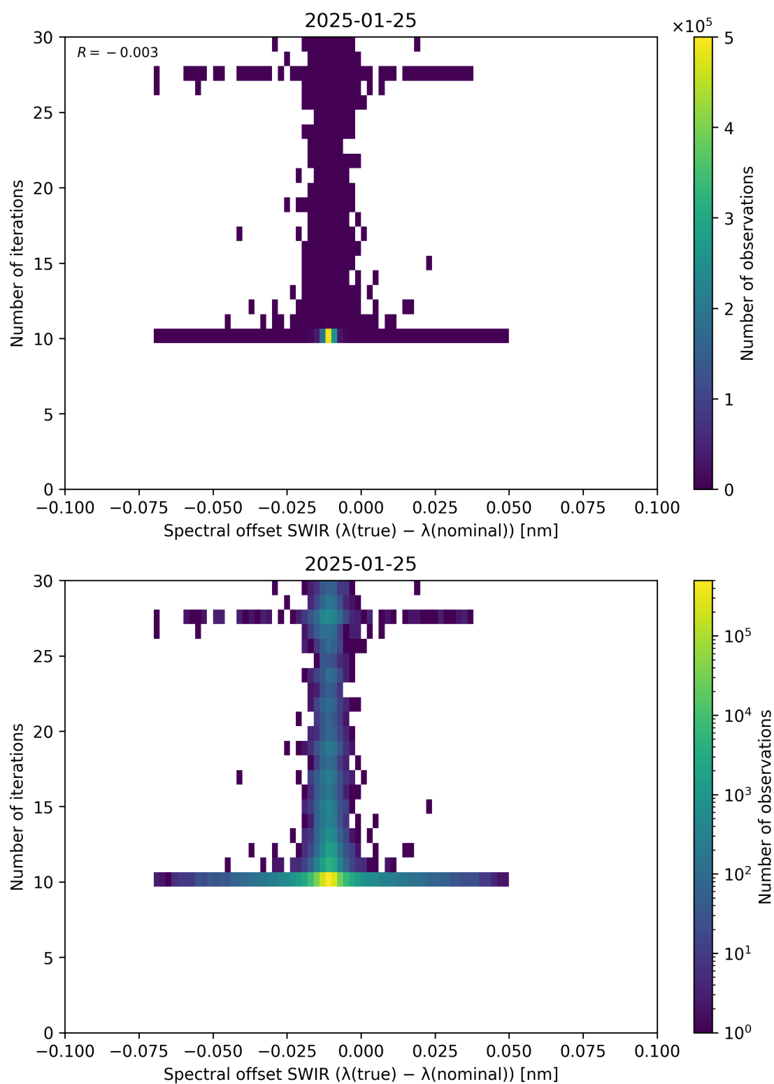
Figure 121: Scatter density plot of “Spectral offset SWIR ( \lambda_{\text{true}} - \lambda_{\text{nominal}} )” against “Number of iterations” for 2025-01-24 to 2025-01-26.
