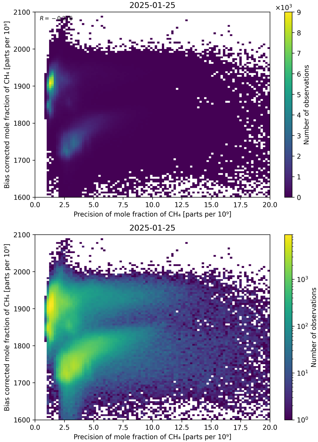
Figure 82: Scatter density plot of “Precision of mole fraction of CH 4 ” against “Bias corrected mole fraction of CH 4 ” for 2025-01-24 to 2025-01-26.
