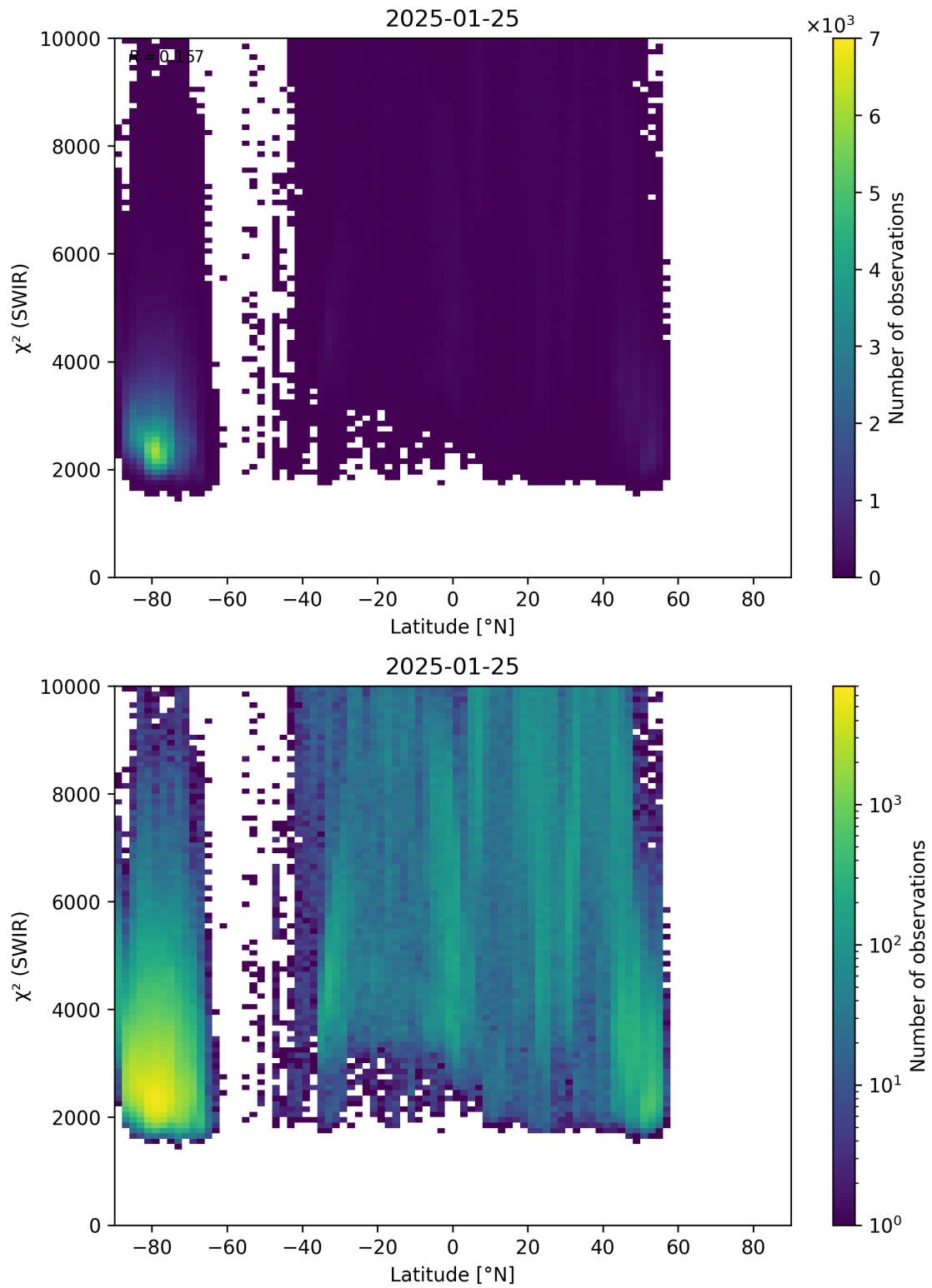
Figure 54: Scatter density plot of “Latitude” against “ \chi^2 (SWIR)” for 2025-01-24 to 2025-01-26.
