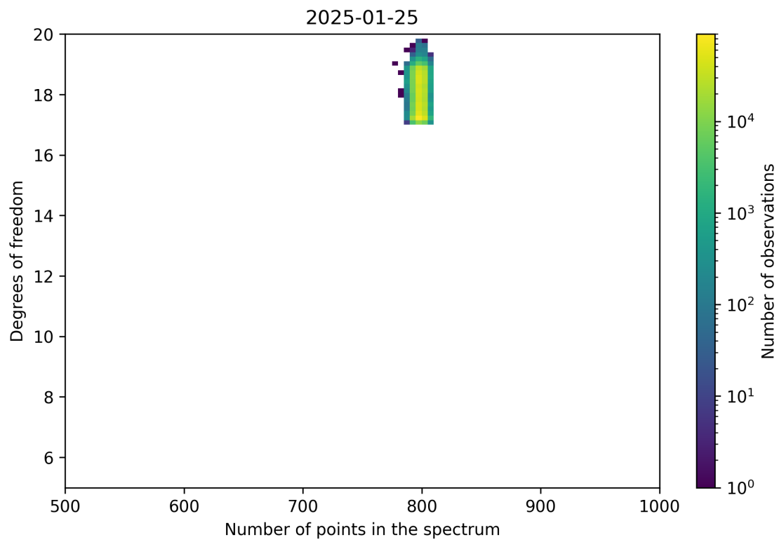
Figure 90: Scatter density plot of “Number of points in the spectrum” against “Degrees of freedom” for 2025-01-24 to 2025-01-26.
