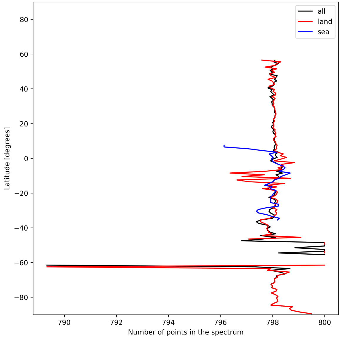
Figure 15: Zonal average of “Number of points in the spectrum” for 2025-01-24 to 2025-01-26.
