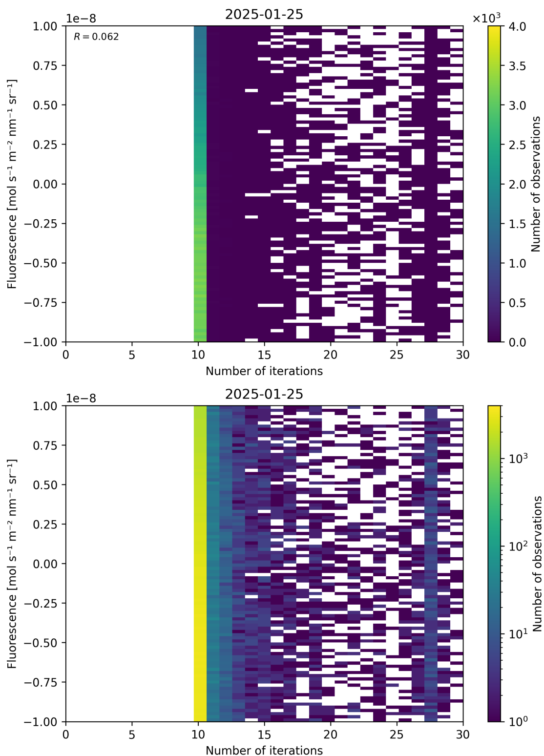
Figure 87: Scatter density plot of “Number of iterations” against “Fluorescence” for 2025-01-24 to 2025-01-26.
