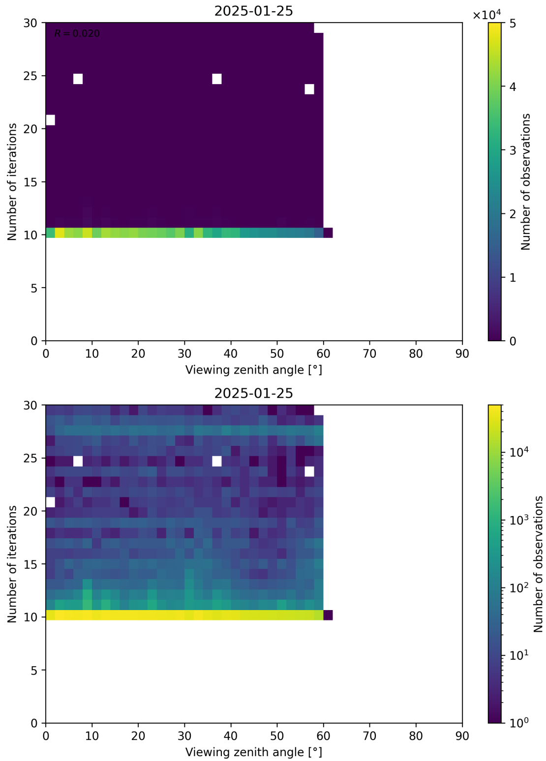
Figure 113: Scatter density plot of “Viewing zenith angle” against “Number of iterations” for 2025-01-24 to 2025-01-26.
