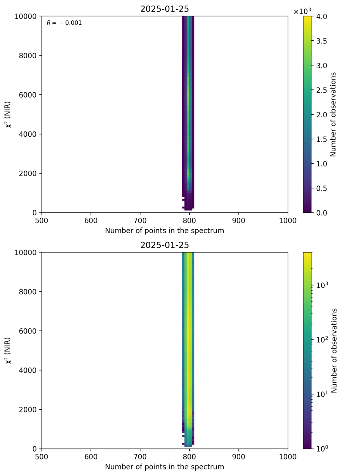
Figure 88: Scatter density plot of “Number of points in the spectrum” against “ \chi^2 (NIR)” for 2025-01-24 to 2025-01-26.
