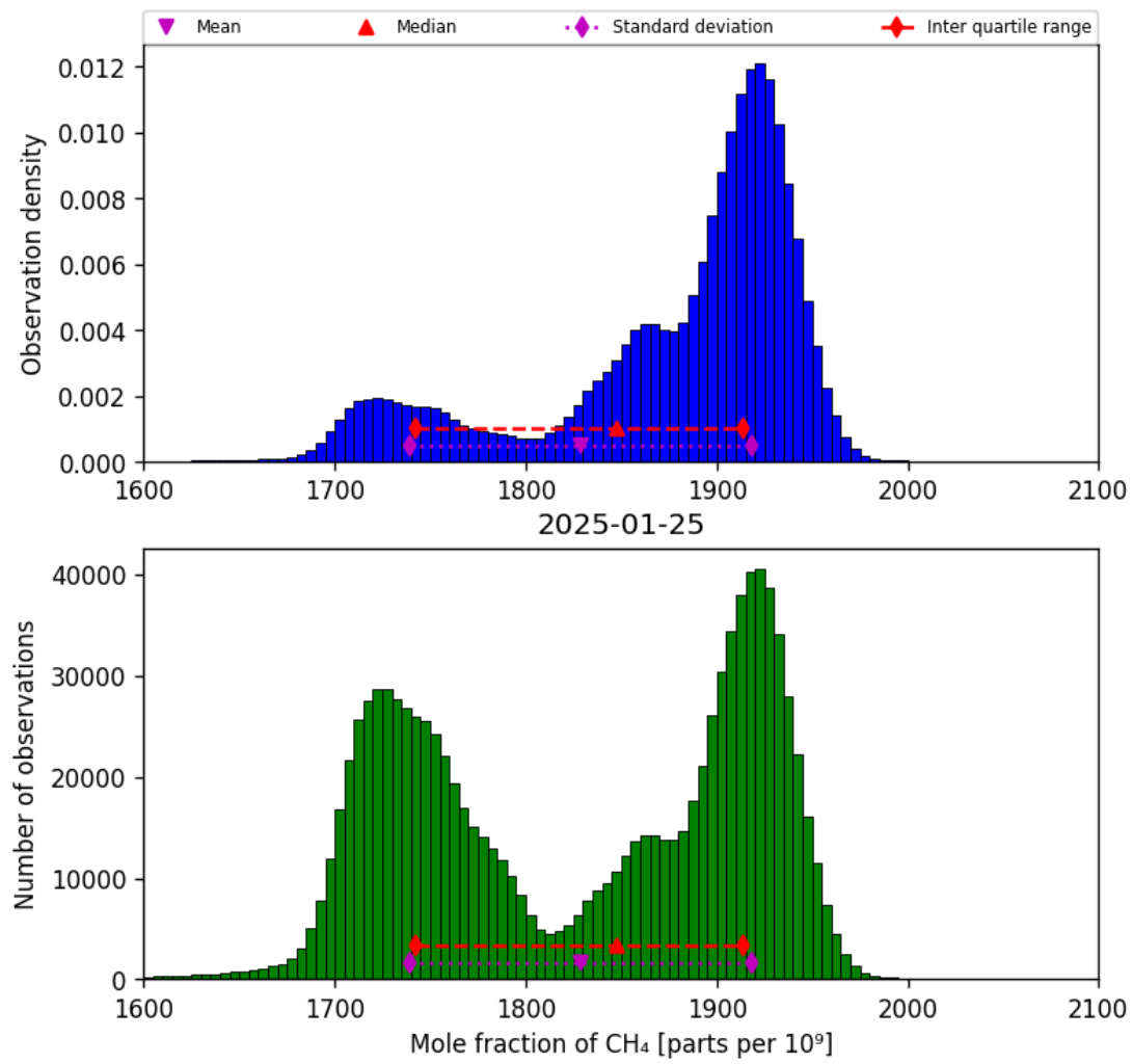
Figure 23: Histogram of “Mole fraction of CH 4 ” for 2025-01-24 to 2025-01-26
