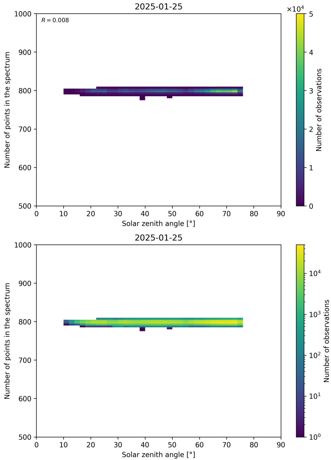
Figure 103: Scatter density plot of “Solar zenith angle” against “Number of points in the spectrum” for 2025-01-24 to 2025-01-26.
