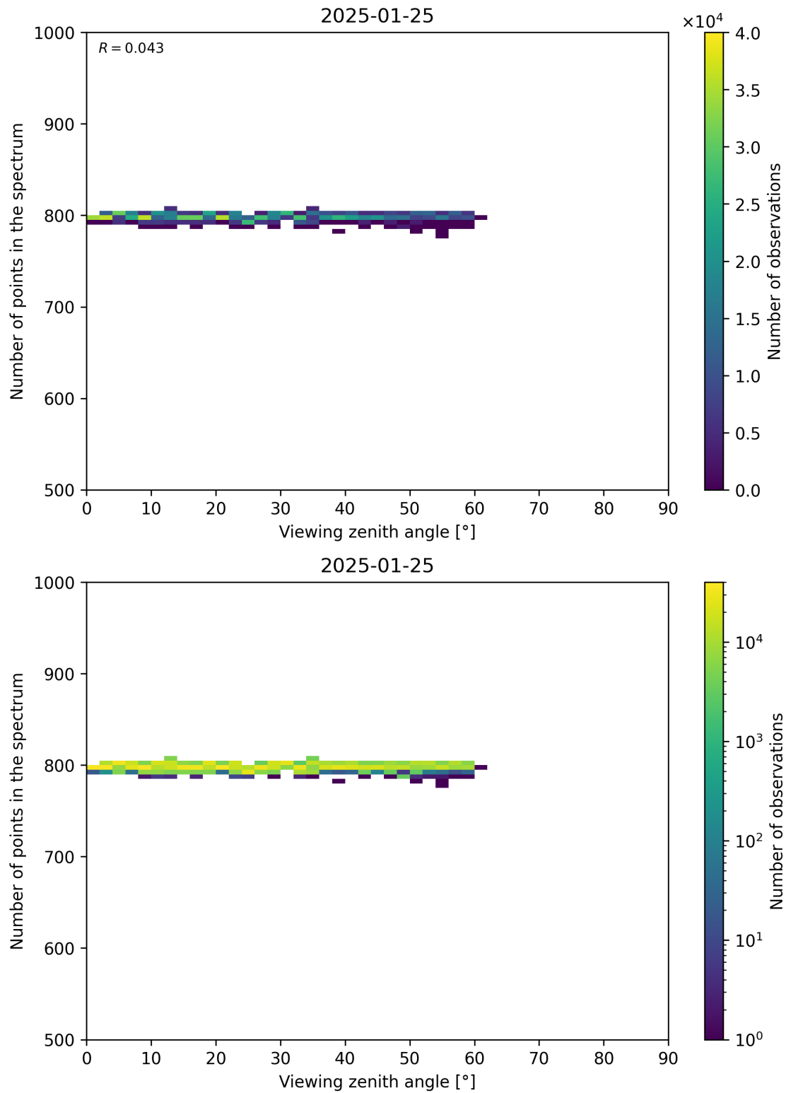
Figure 114: Scatter density plot of “Viewing zenith angle” against “Number of points in the spectrum” for 2025-01-24 to 2025-01-26.
