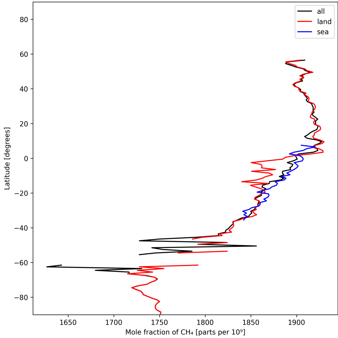
Figure 12: Zonal average of “Mole fraction of CH 4 ” for 2025-01-24 to 2025-01-26.
