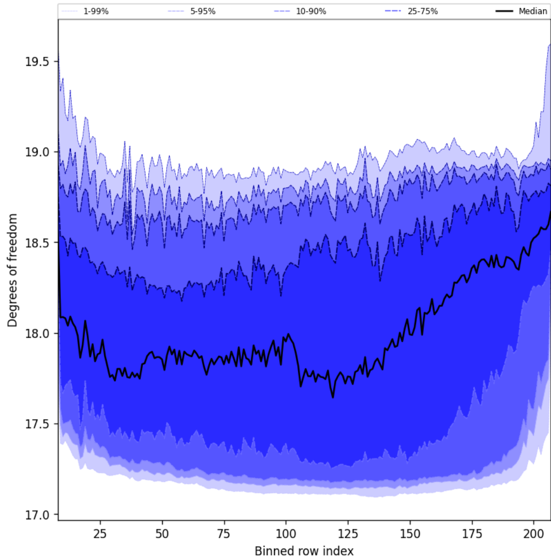
Figure 41: Along track statistics of “Degrees of freedom” for 2025-01-24 to 2025-01-26
