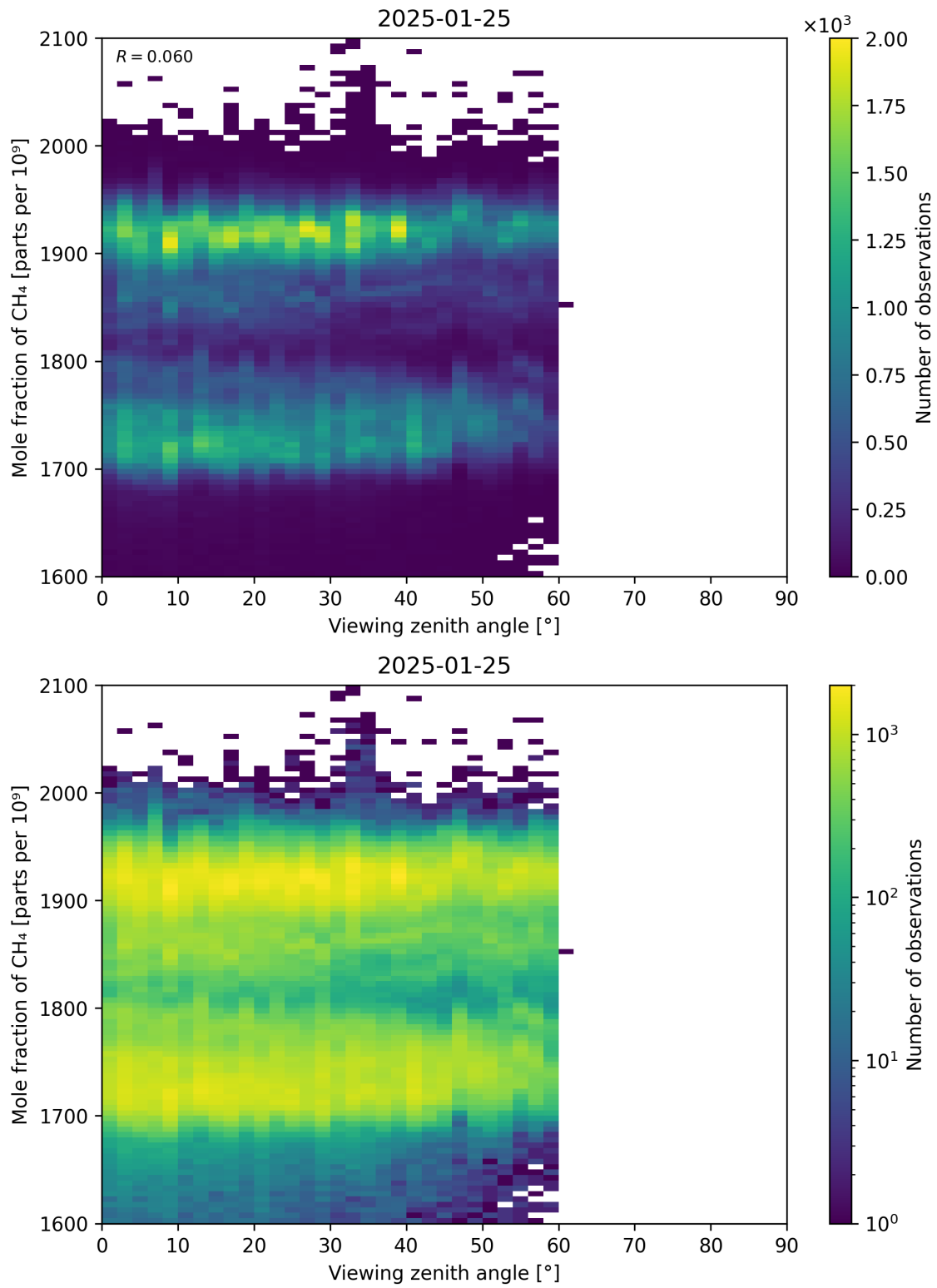
Figure 110: Scatter density plot of “Viewing zenith angle” against “Mole fraction of \text{CH}_4 ” for 2025-01-24 to 2025-01-26.
