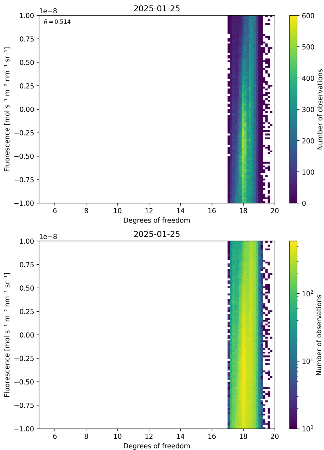
Figure 51: Scatter density plot of “Degrees of freedom” against “Fluorescence” for 2025-01-24 to 2025-01-26.
