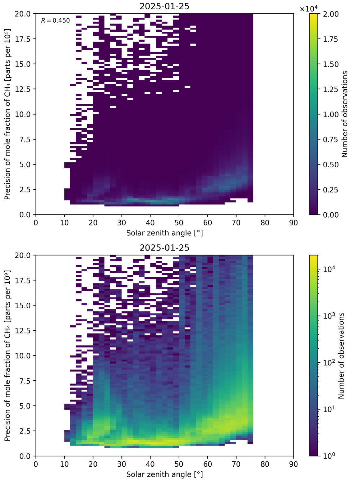
Figure 101: Scatter density plot of “Solar zenith angle” against “Precision of mole fraction of CH 4 ” for 2025-01-24 to 2025-01-26.
