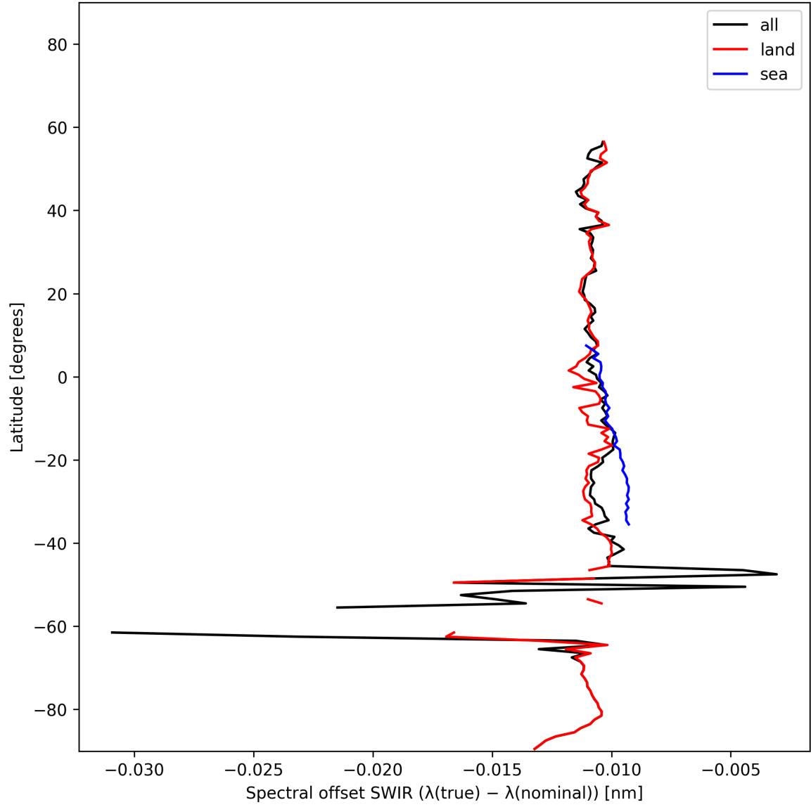
Figure 16: Zonal average of “Spectral offset SWIR ( \lambda_{\text{true}} - \lambda_{\text{nominal}} )” for 2025-01-24 to 2025-01-26.
