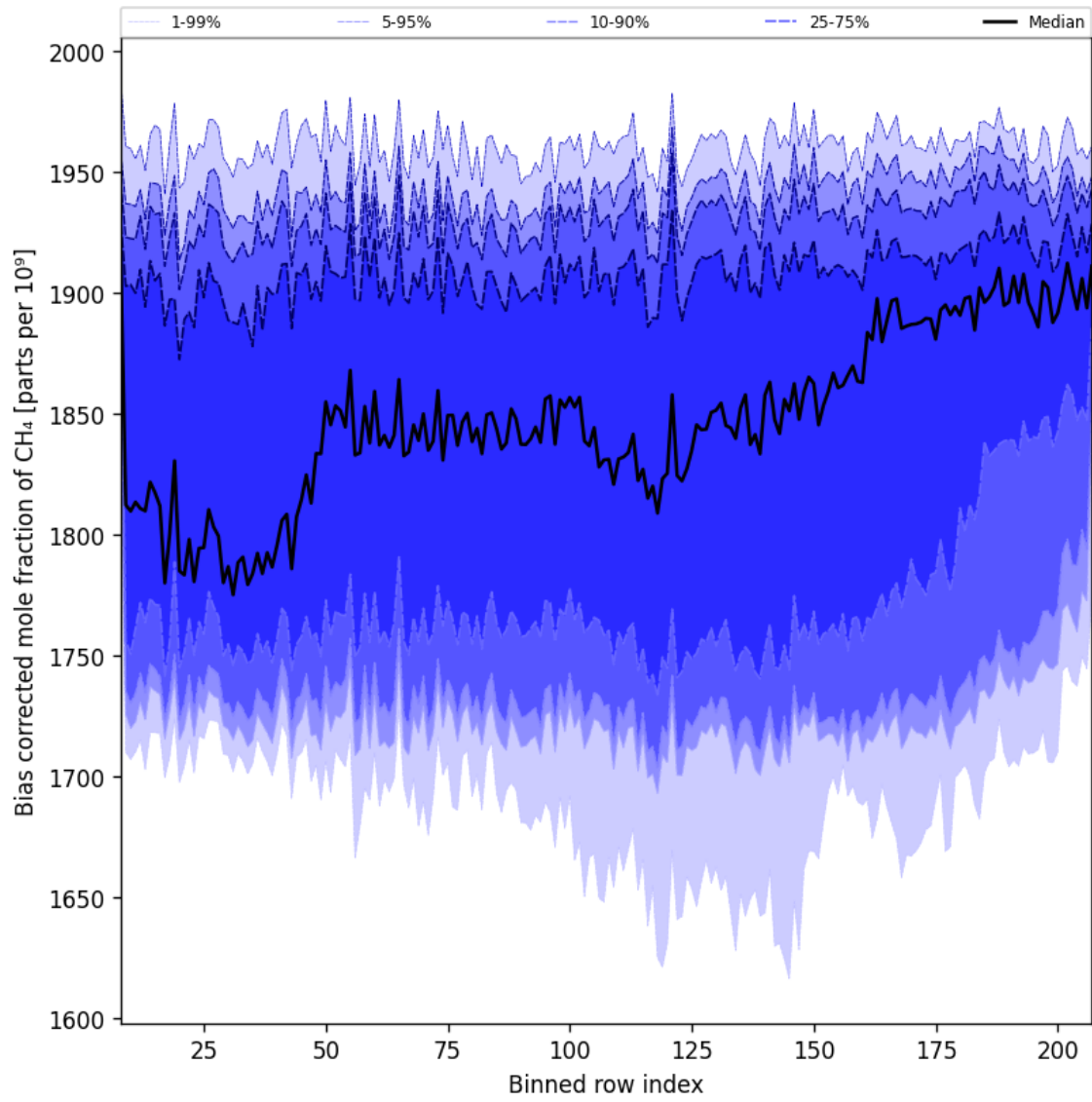
Figure 36: Along track statistics of “Bias corrected mole fraction of CH 4 ” for 2025-01-24 to 2025-01-26
