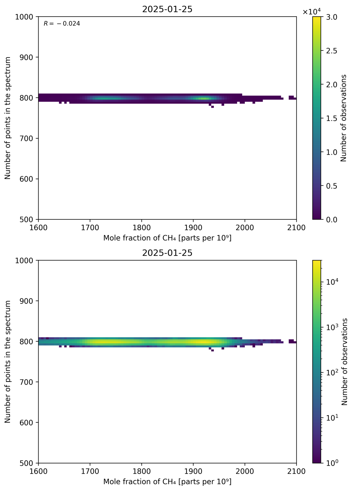
Figure 77: Scatter density plot of “Mole fraction of CH 4 ” against “Number of points in the spectrum” for 2025-01-24 to 2025-01-26.
