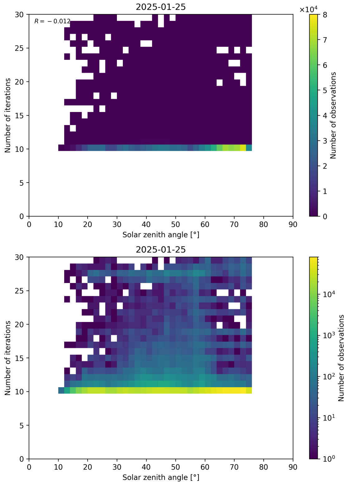
Figure 102: Scatter density plot of “Solar zenith angle” against “Number of iterations” for 2025-01-24 to 2025-01-26.
