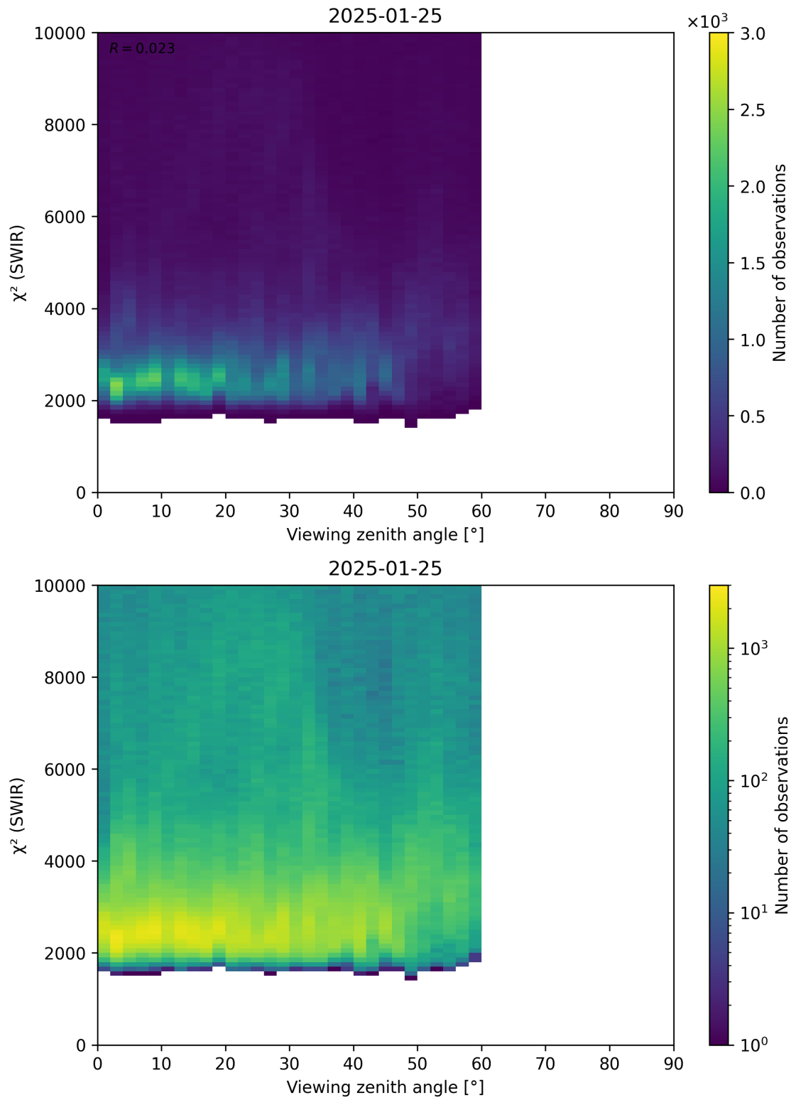
Figure 106: Scatter density plot of “Viewing zenith angle” against “ \chi^2 (SWIR)” for 2025-01-24 to 2025-01-26.
