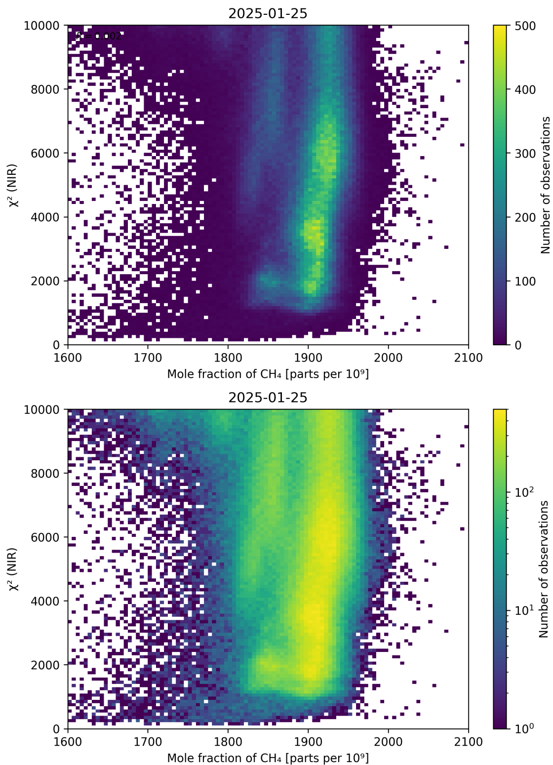
Figure 70: Scatter density plot of “Mole fraction of CH 4 ” against “ \chi^2 (NIR)” for 2025-01-24 to 2025-01-26.
