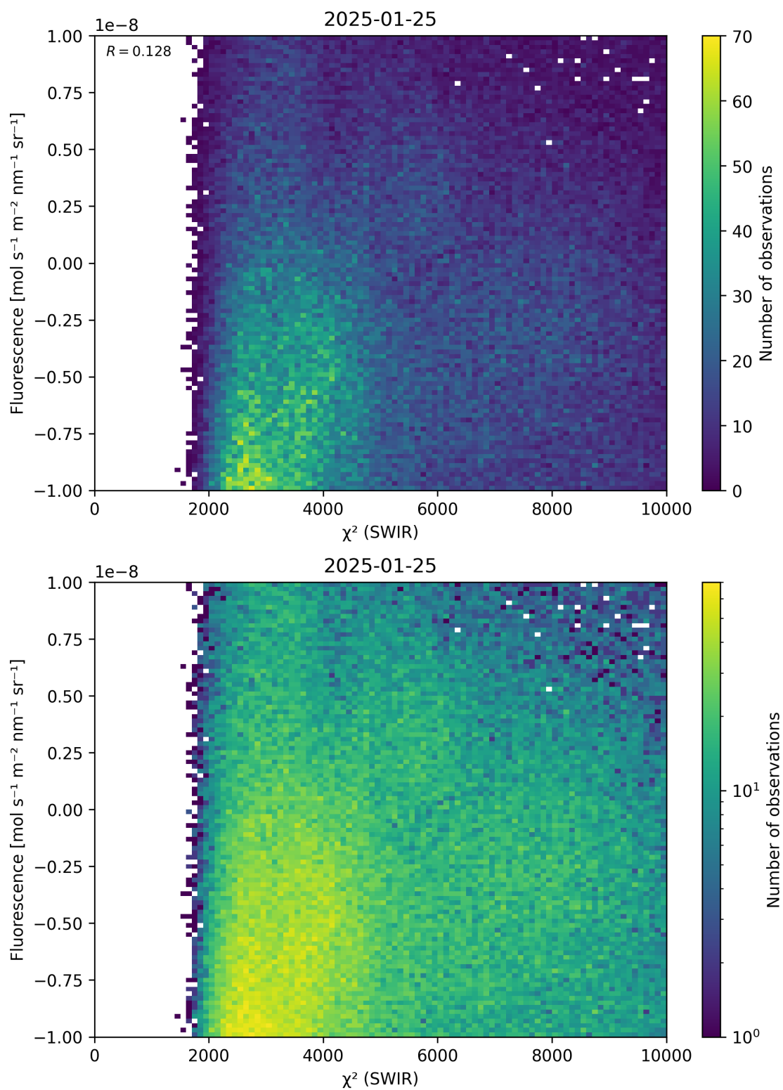
Figure 49: Scatter density plot of “ \chi^2 (SWIR)” against “Fluorescence” for 2025-01-24 to 2025-01-26.
