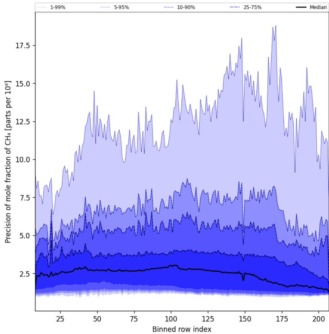
Figure 35: Along track statistics of “Precision of mole fraction of CH 4 ” for 2025-01-24 to 2025-01-26
