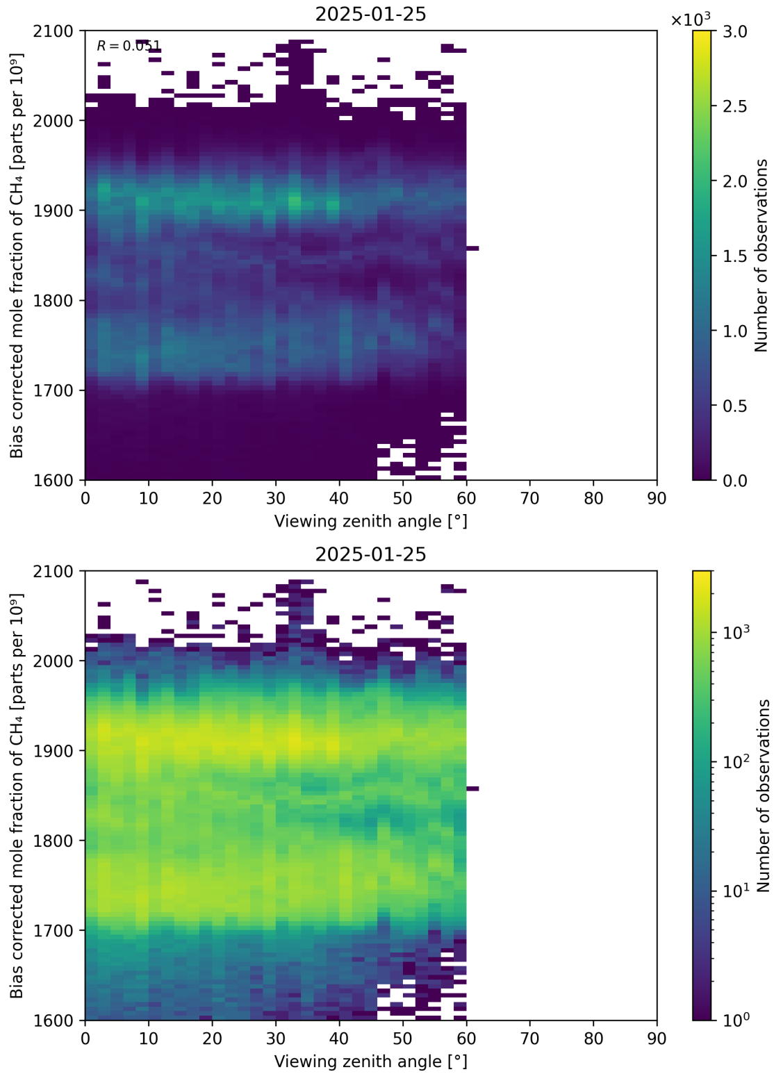
Figure 111: Scatter density plot of “Viewing zenith angle” against “Bias corrected mole fraction of CH 4 ” for 2025-01-24 to 2025-01-26.
