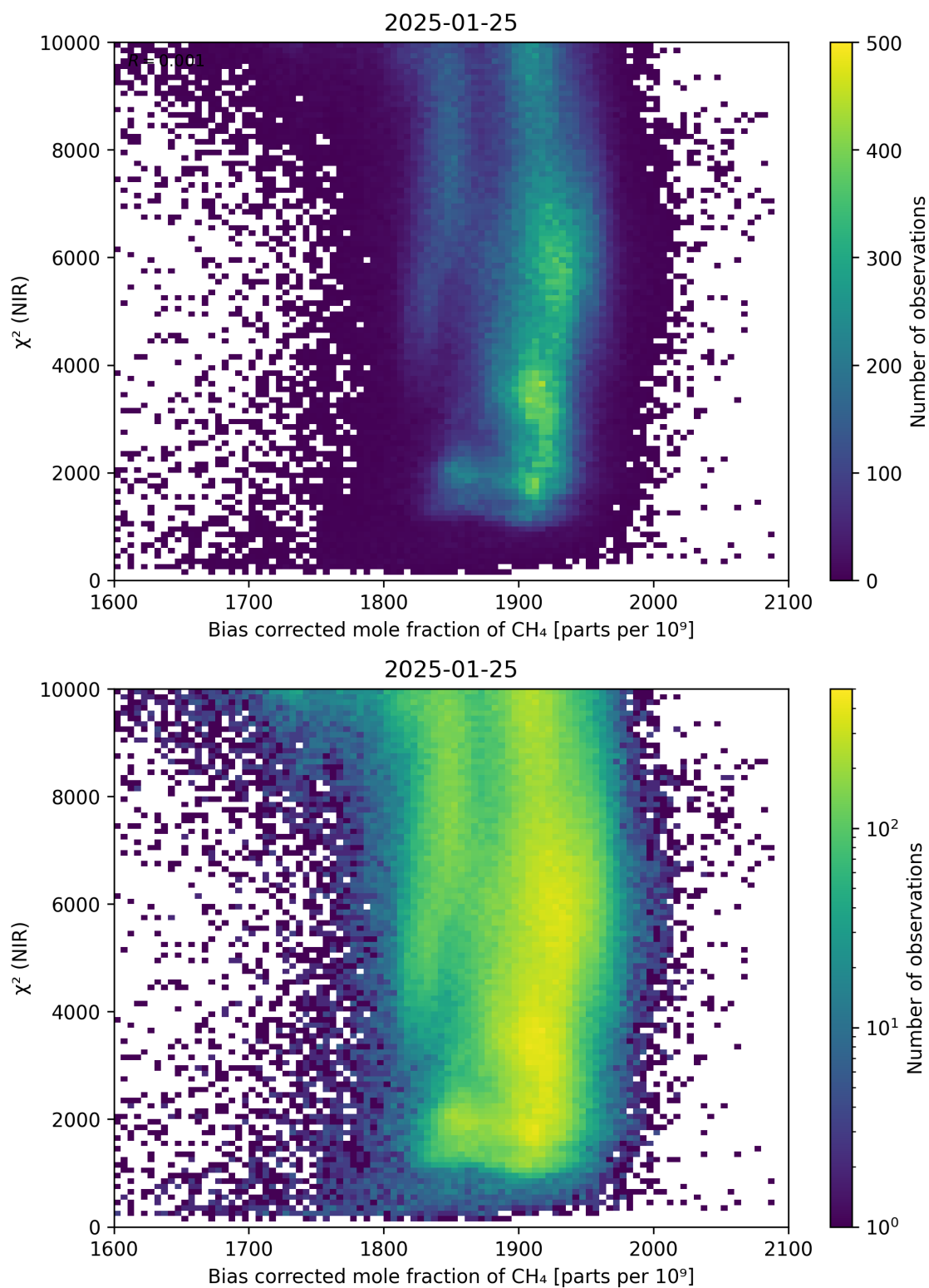
Figure 63: Scatter density plot of “Bias corrected mole fraction of \text{CH}_4 ” against “ \chi^2 (NIR)” for 2025-01-24 to 2025-01-26.
