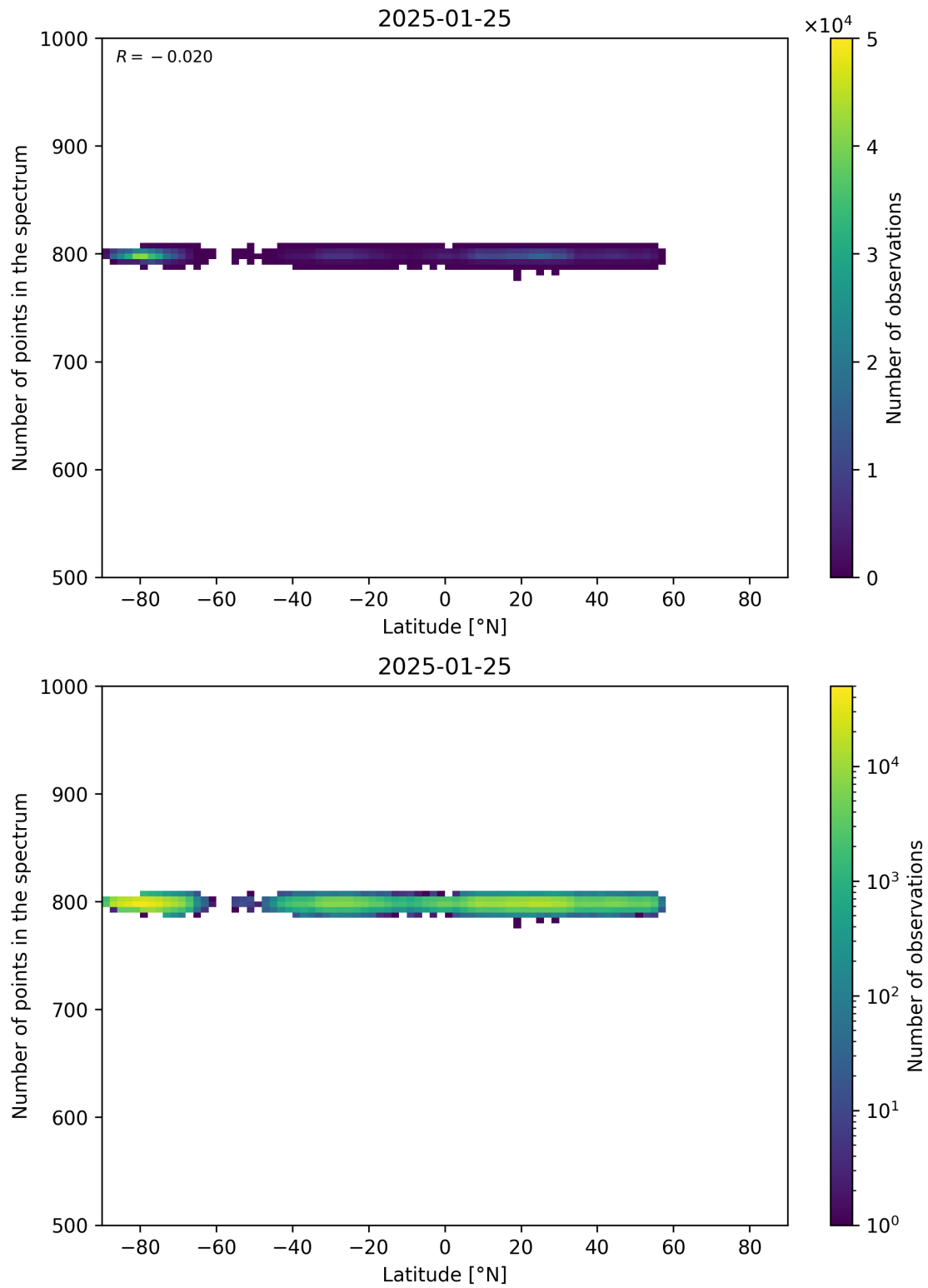
Figure 61: Scatter density plot of “Latitude” against “Number of points in the spectrum” for 2025-01-24 to 2025-01-26.
