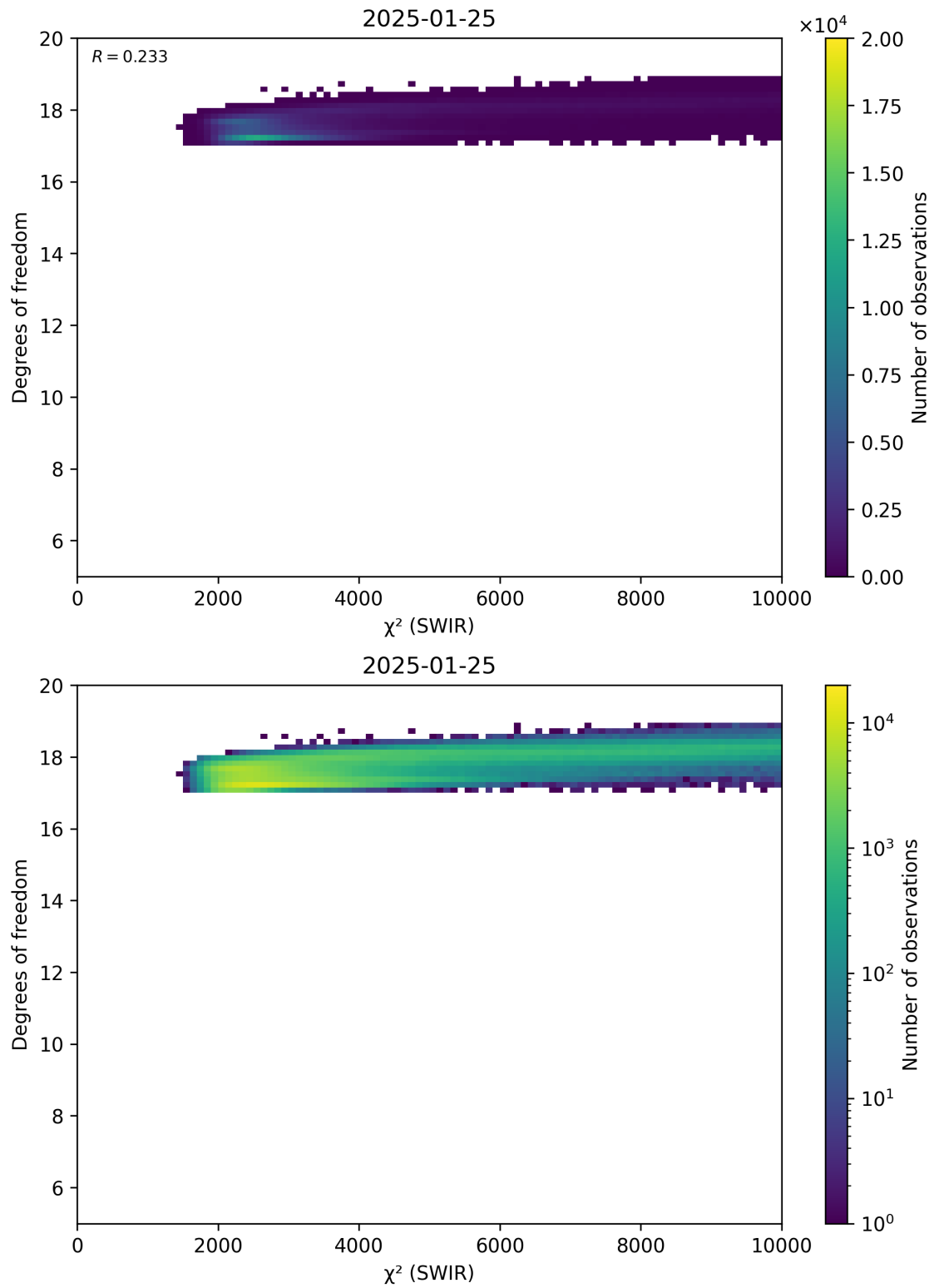
Figure 48: Scatter density plot of “ \chi^2 (SWIR)” against “Degrees of freedom” for 2025-01-24 to 2025-01-26.
