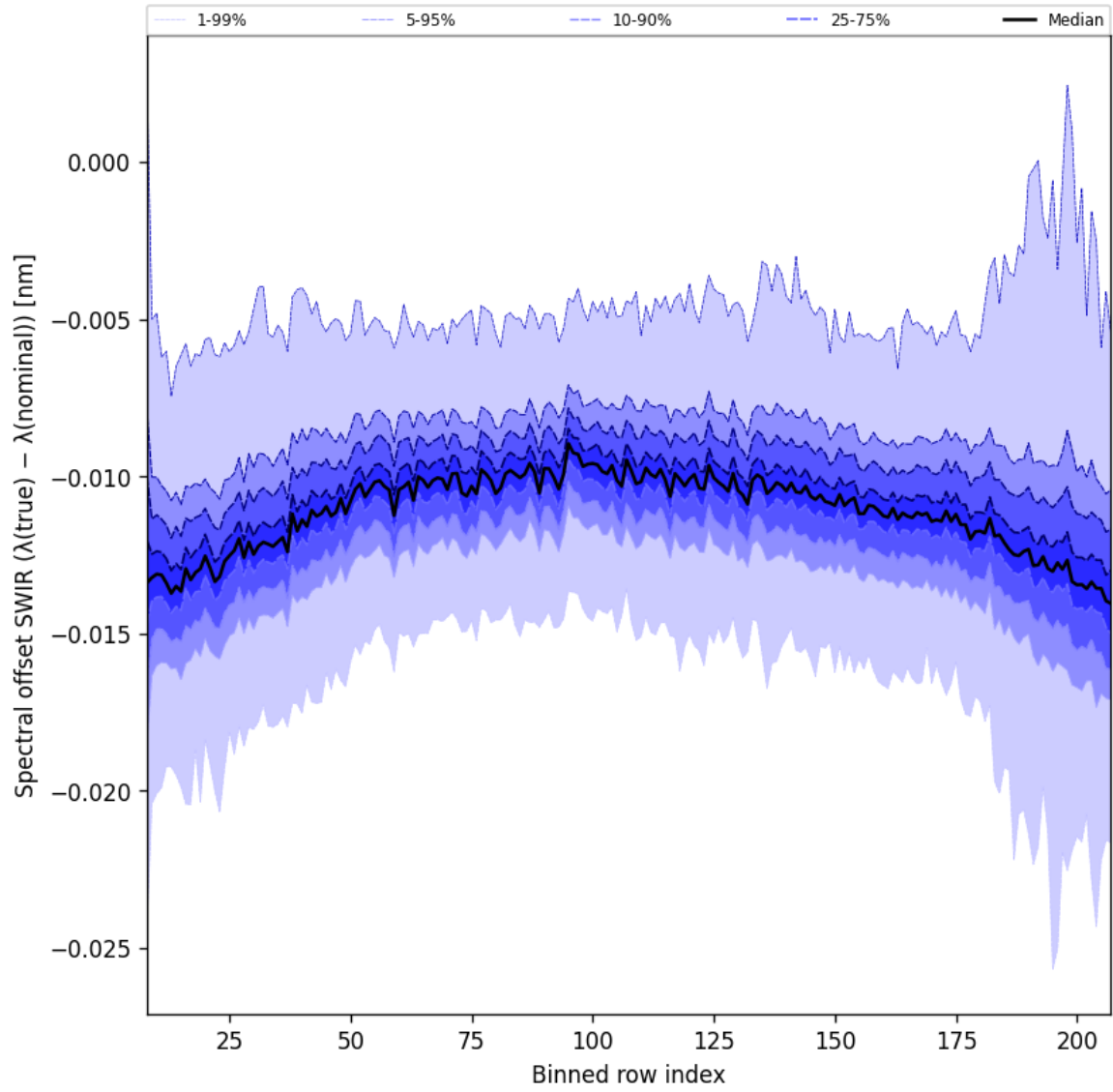
Figure 38: Along track statistics of “Spectral offset SWIR ( \lambda_{\text{true}} - \lambda_{\text{nominal}} )” for 2025-01-24 to 2025-01-26
