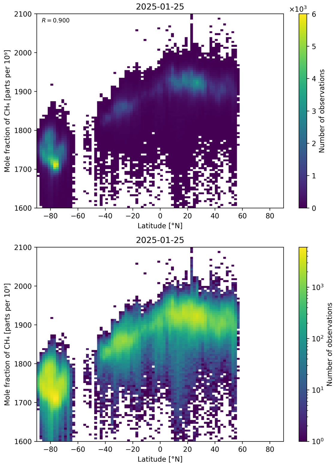
Figure 57: Scatter density plot of “Latitude” against “Mole fraction of CH 4 ” for 2025-01-24 to 2025-01-26.
