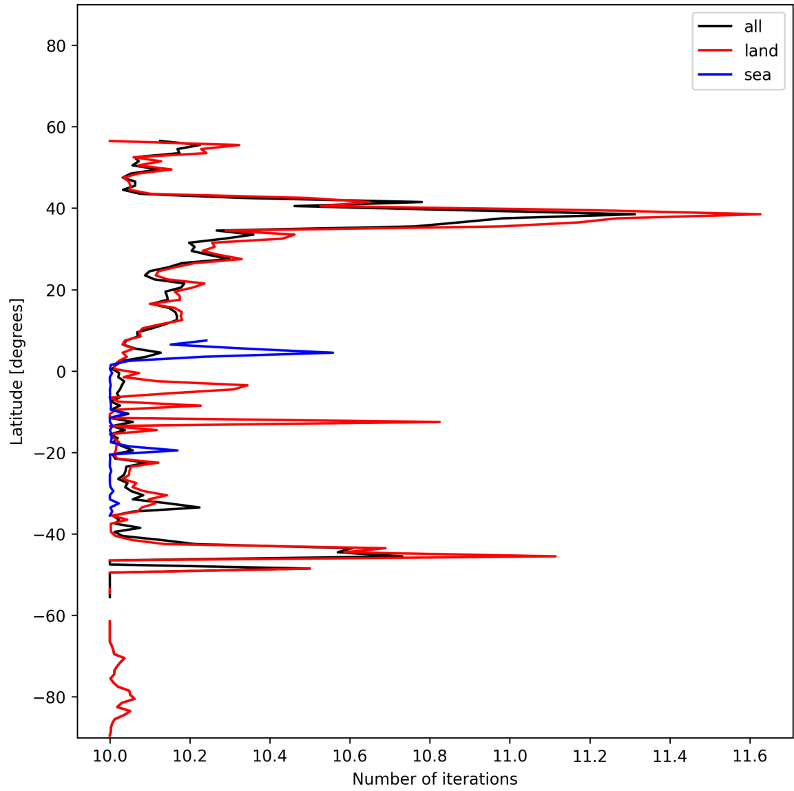
Figure 20: Zonal average of “Number of iterations” for 2025-01-24 to 2025-01-26.
