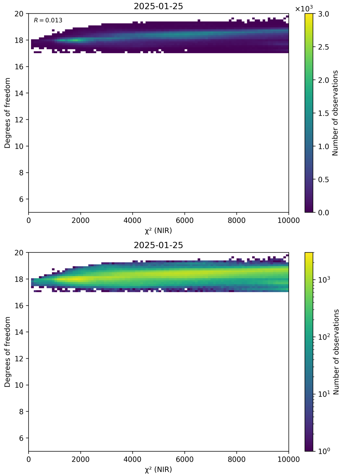
Figure 44: Scatter density plot of “ \chi^2 (NIR)” against “Degrees of freedom” for 2025-01-24 to 2025-01-26.
