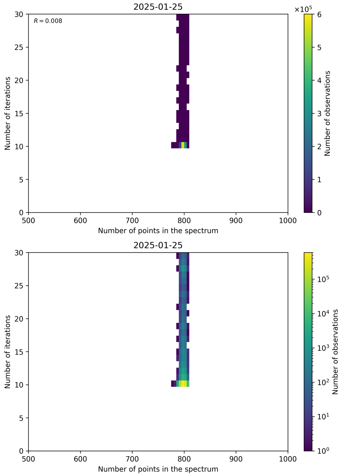
Figure 92: Scatter density plot of “Number of points in the spectrum” against “Number of iterations” for 2025-01-24 to 2025-01-26.
