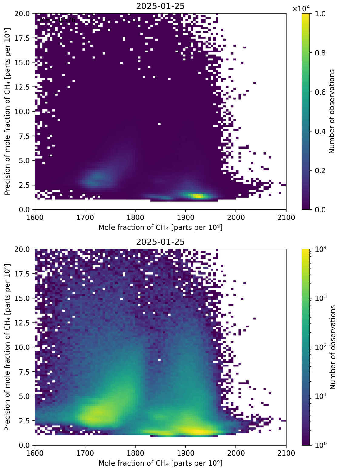
Figure 75: Scatter density plot of “Mole fraction of CH 4 ” against “Precision of mole fraction of CH 4 ” for 2025-01-24 to 2025-01-26.
