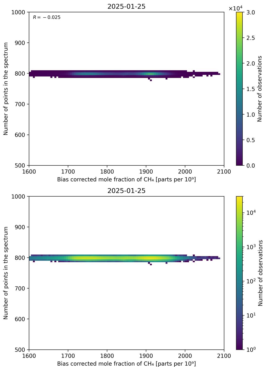
Figure 68: Scatter density plot of “Bias corrected mole fraction of CH 4 ” against “Number of points in the spectrum” for 2025-01-24 to 2025-01-26.
