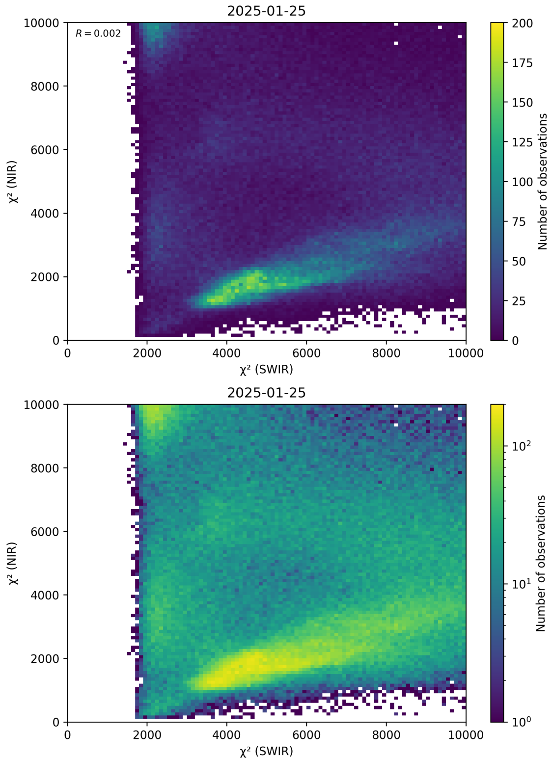
Figure 47: Scatter density plot of “ \chi^2 (SWIR)” against “ \chi^2 (NIR)” for 2025-01-24 to 2025-01-26.
