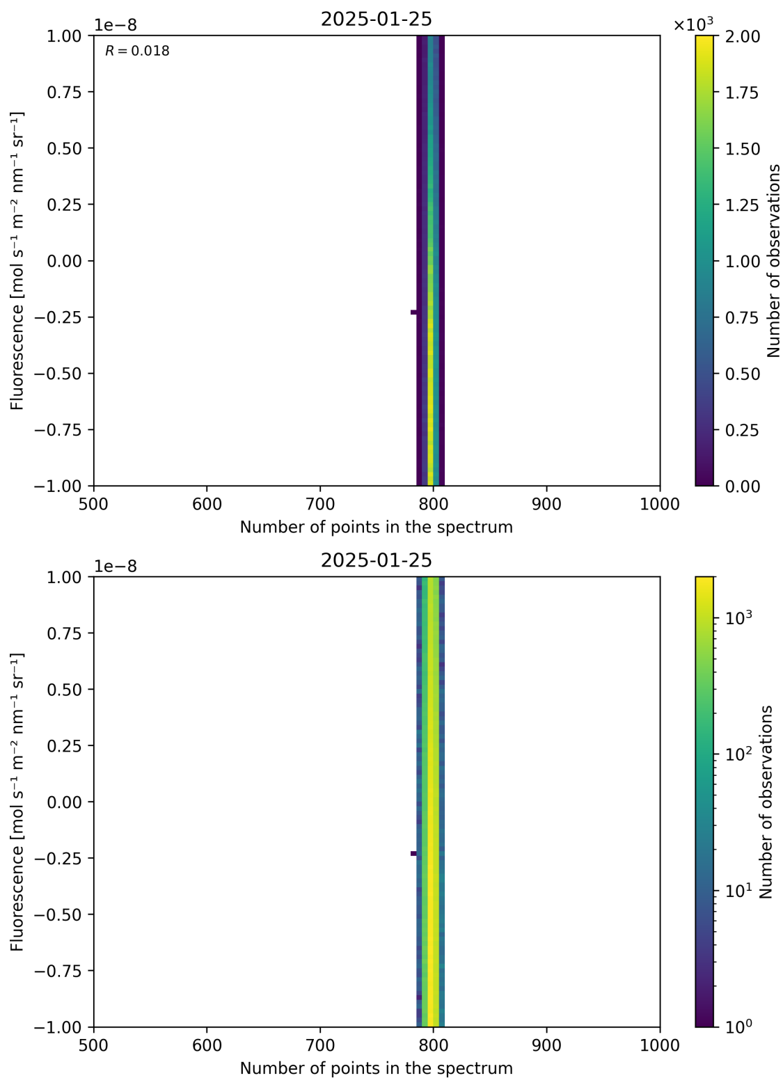
Figure 91: Scatter density plot of “Number of points in the spectrum” against “Fluorescence” for 2025-01-24 to 2025-01-26.
