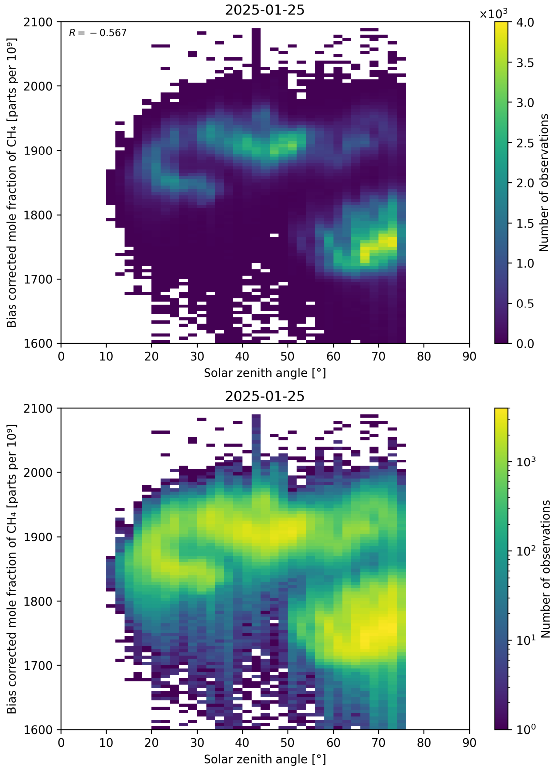
Figure 100: Scatter density plot of “Solar zenith angle” against “Bias corrected mole fraction of CH 4 ” for 2025-01-24 to 2025-01-26.
