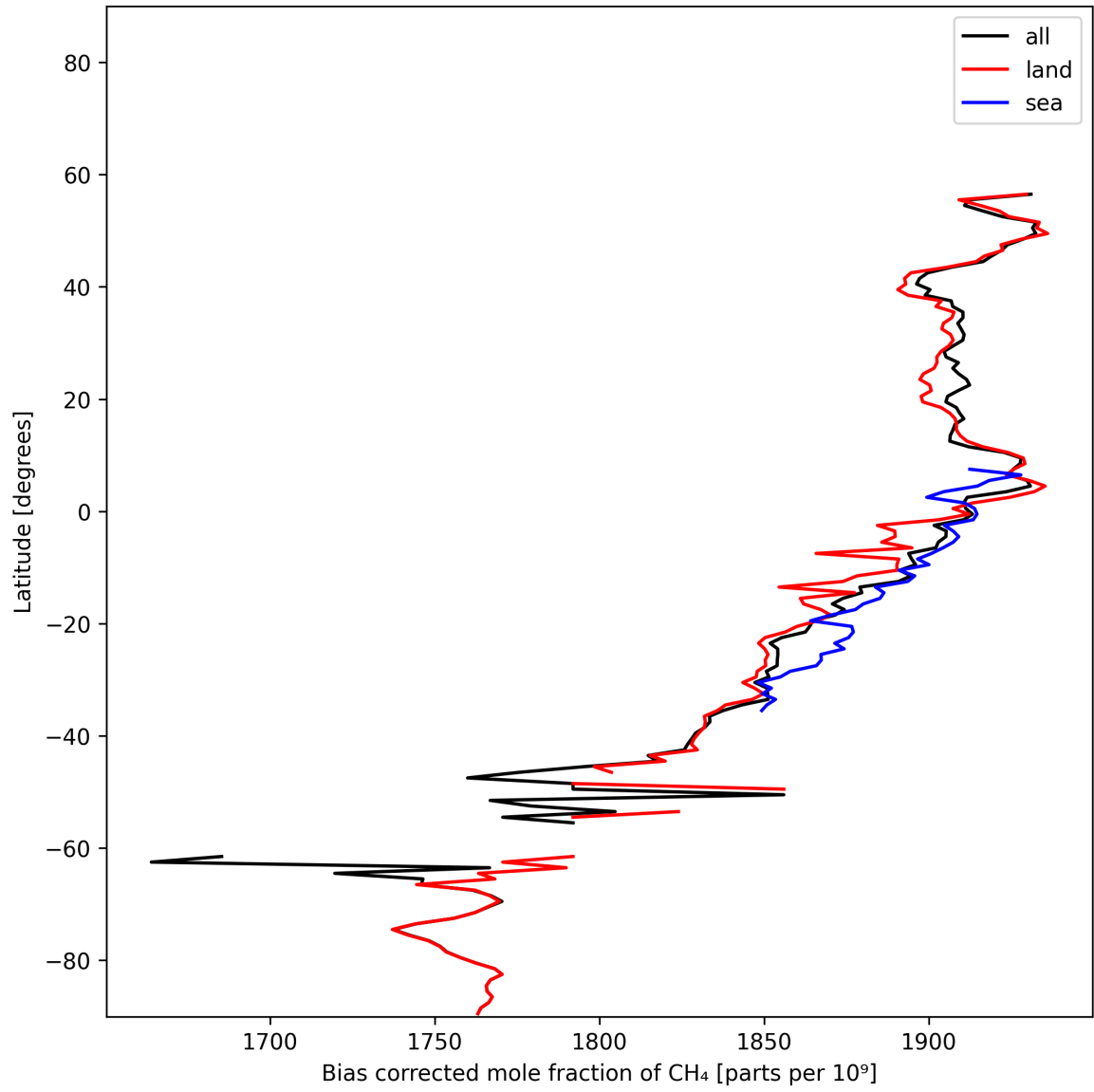
Figure 14: Zonal average of “Bias corrected mole fraction of CH 4 ” for 2025-01-24 to 2025-01-26.
