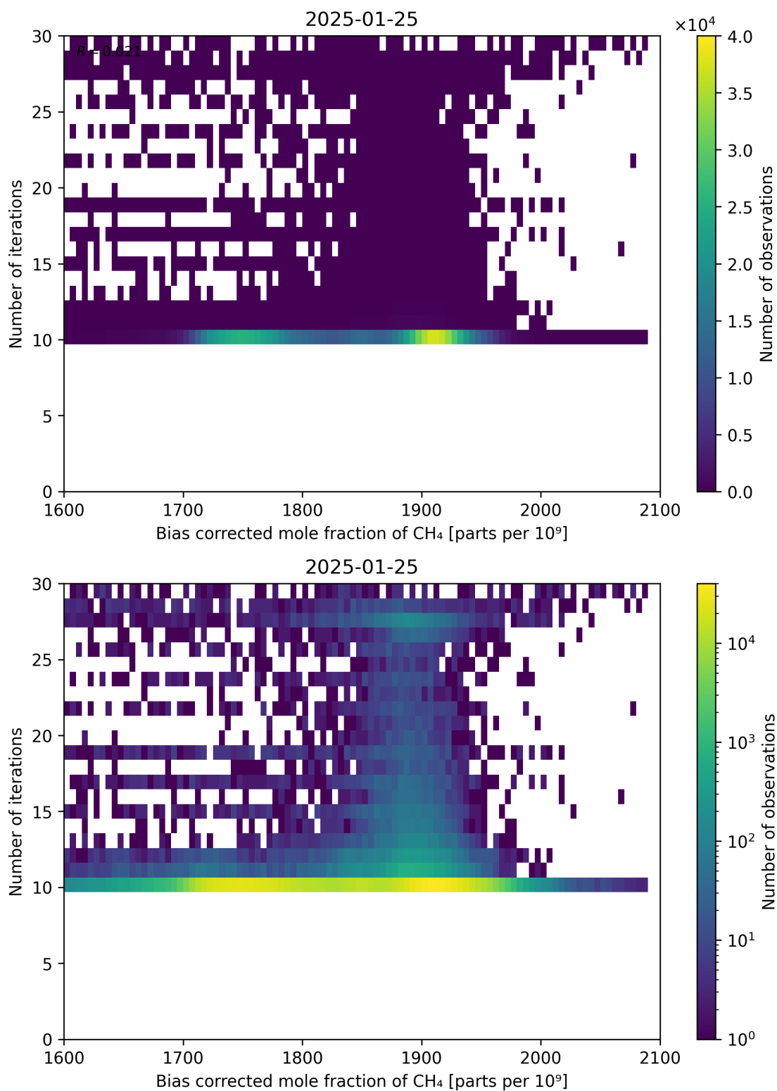
Figure 67: Scatter density plot of “Bias corrected mole fraction of \text{CH}_4 ” against “Number of iterations” for 2025-01-24 to 2025-01-26.
