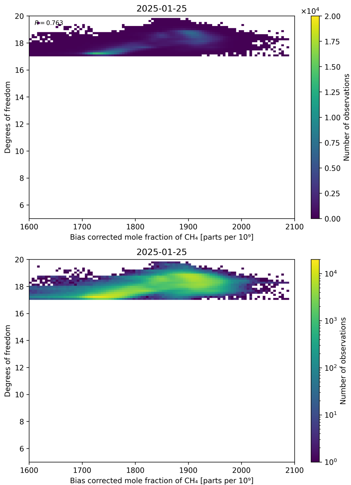
Figure 65: Scatter density plot of “Bias corrected mole fraction of CH 4 ” against “Degrees of freedom” for 2025-01-24 to 2025-01-26.
