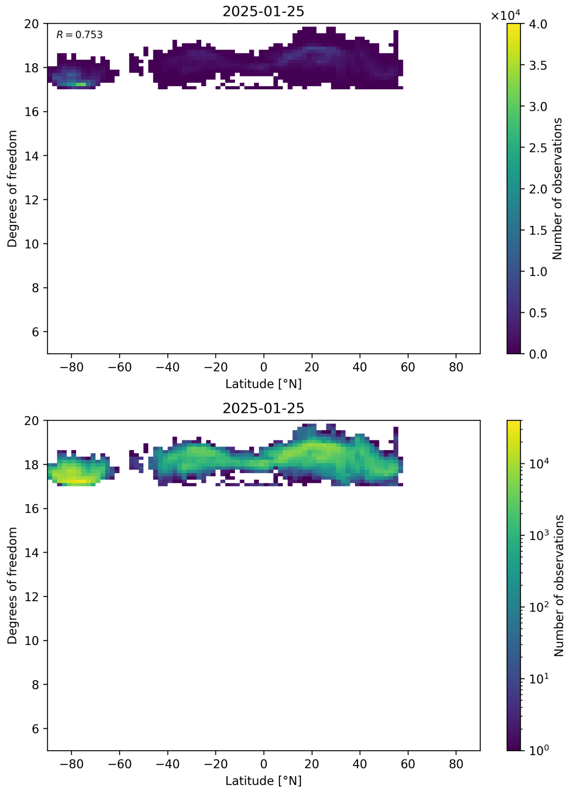
Figure 55: Scatter density plot of “Latitude” against “Degrees of freedom” for 2025-01-24 to 2025-01-26.
