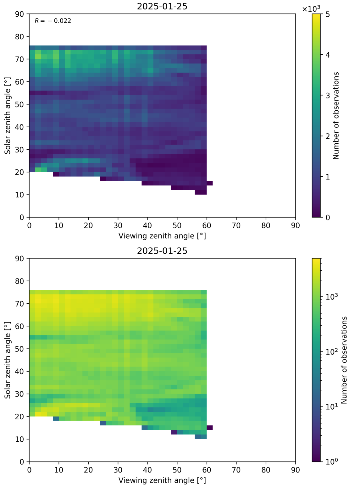
Figure 115: Scatter density plot of “Viewing zenith angle” against “Solar zenith angle” for 2025-01-24 to 2025-01-26.
