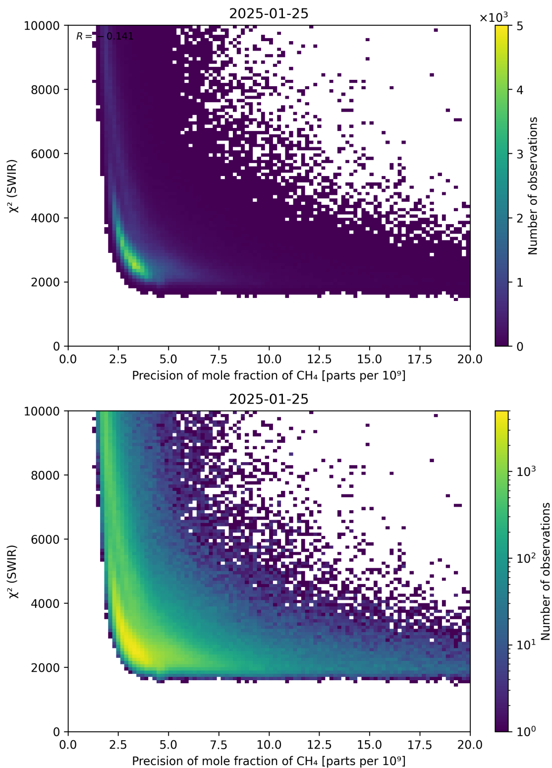
Figure 79: Scatter density plot of “Precision of mole fraction of CH 4 ” against “ \chi^2 (SWIR)” for 2025-01-24 to 2025-01-26.
