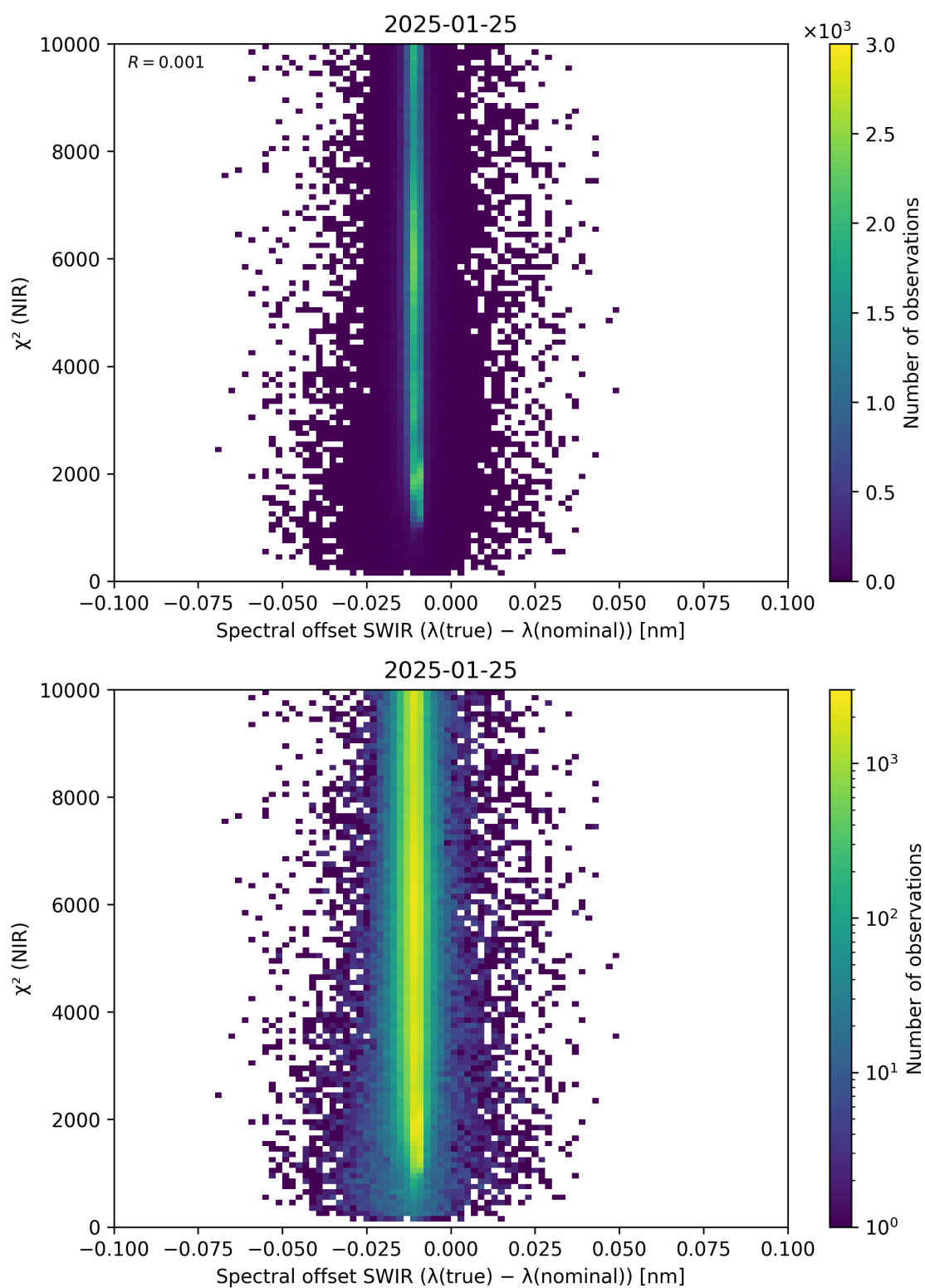
Figure 117: Scatter density plot of “Spectral offset SWIR ( \lambda_{\text{true}} - \lambda_{\text{nominal}} )” against “ \chi^2 (NIR)” for 2025-01-24 to 2025-01-26.
