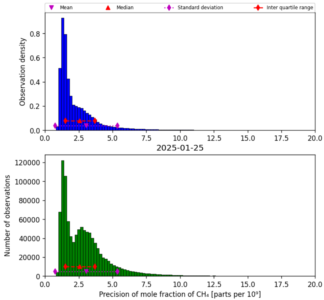
Figure 24: Histogram of “Precision of mole fraction of CH 4 ” for 2025-01-24 to 2025-01-26
