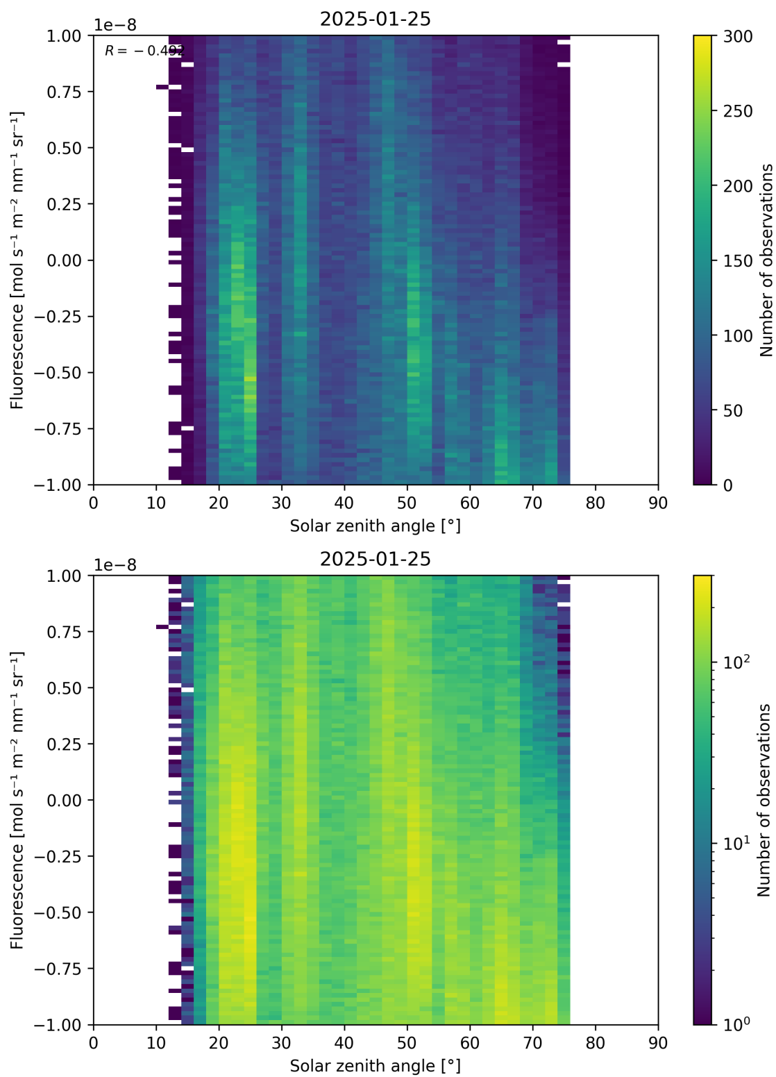
Figure 97: Scatter density plot of “Solar zenith angle” against “Fluorescence” for 2025-01-24 to 2025-01-26.
