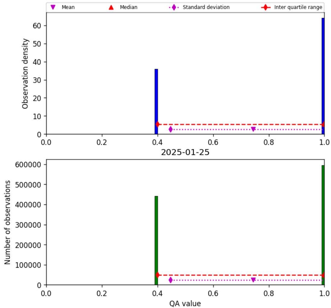
Figure 22: Histogram of “QA value” for 2025-01-24 to 2025-01-26
