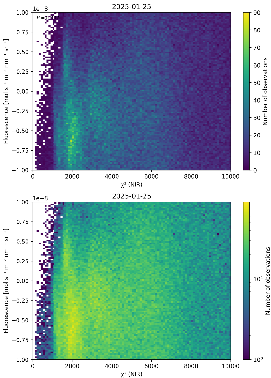
Figure 45: Scatter density plot of “ \chi^2 (NIR)” against “Fluorescence” for 2025-01-24 to 2025-01-26.
