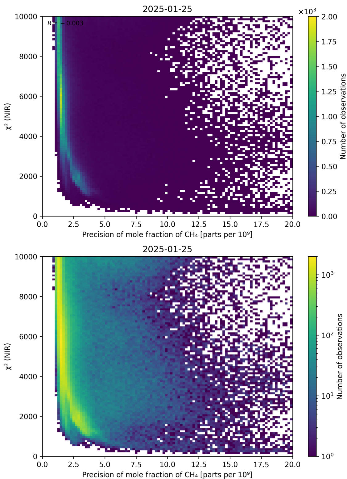
Figure 78: Scatter density plot of “Precision of mole fraction of CH 4 ” against “ \chi^2 (NIR)” for 2025-01-24 to 2025-01-26.
