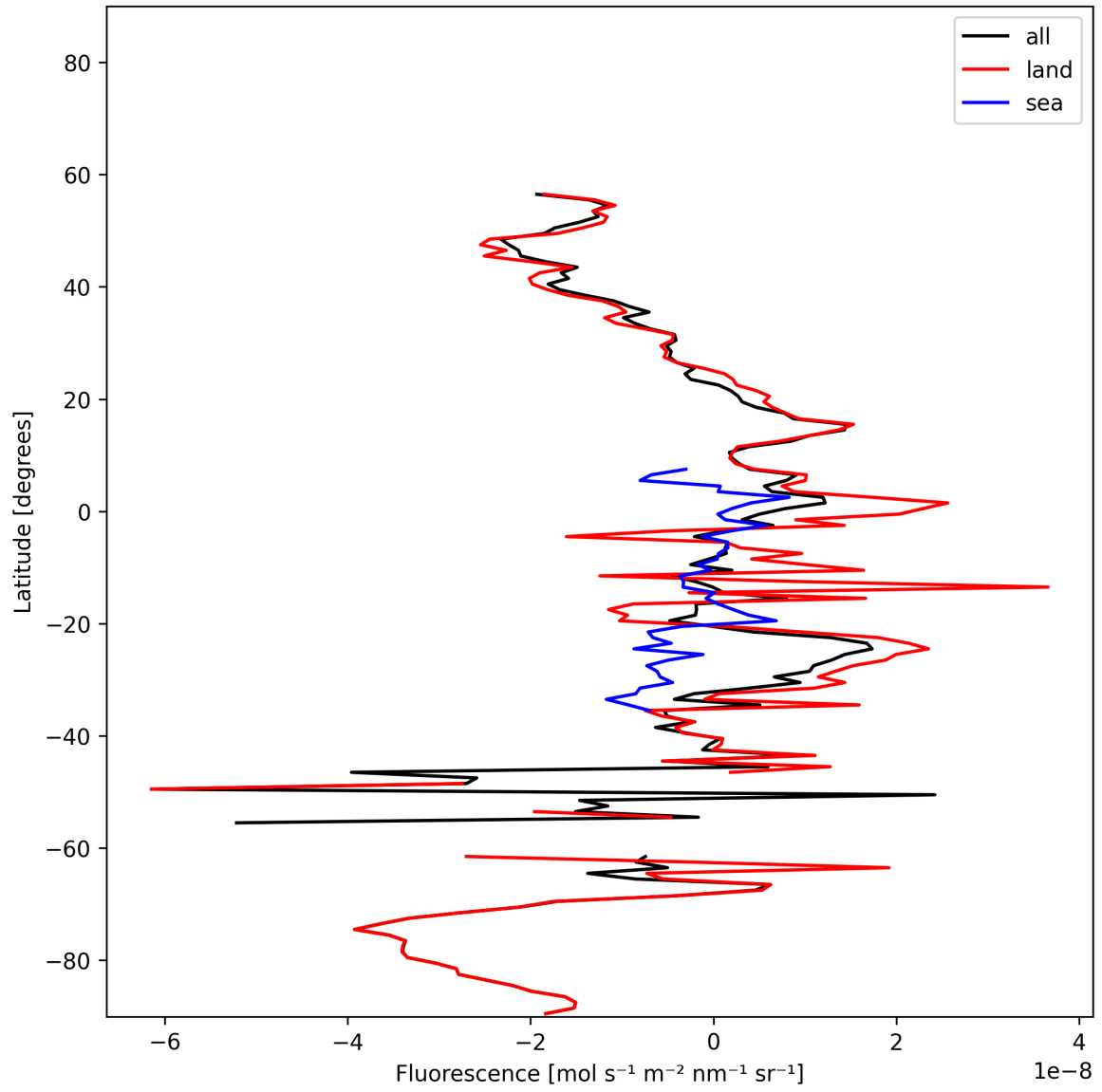
Figure 21: Zonal average of “Fluorescence” for 2025-01-24 to 2025-01-26.
