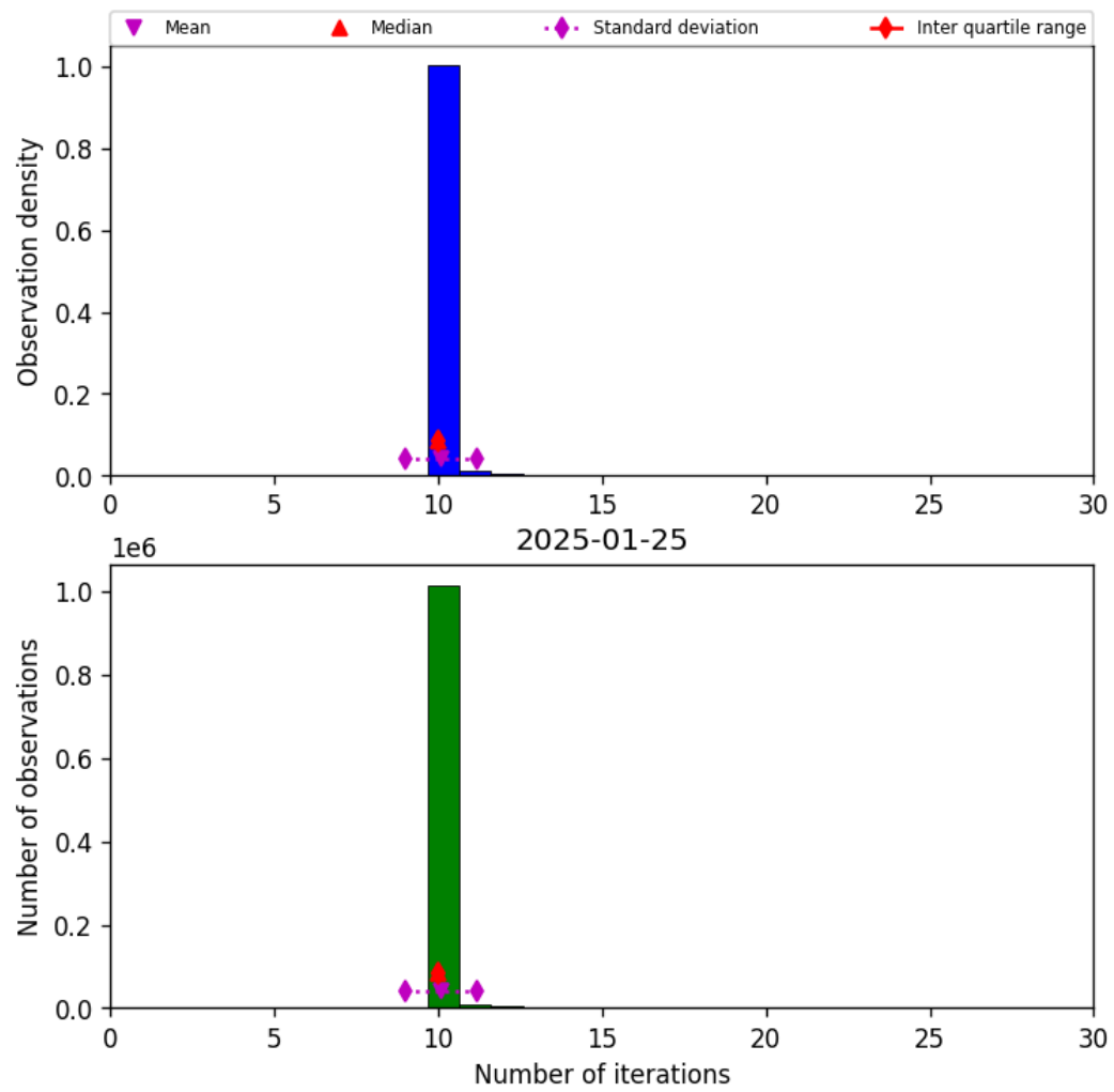
Figure 31: Histogram of “Number of iterations” for 2025-01-24 to 2025-01-26
