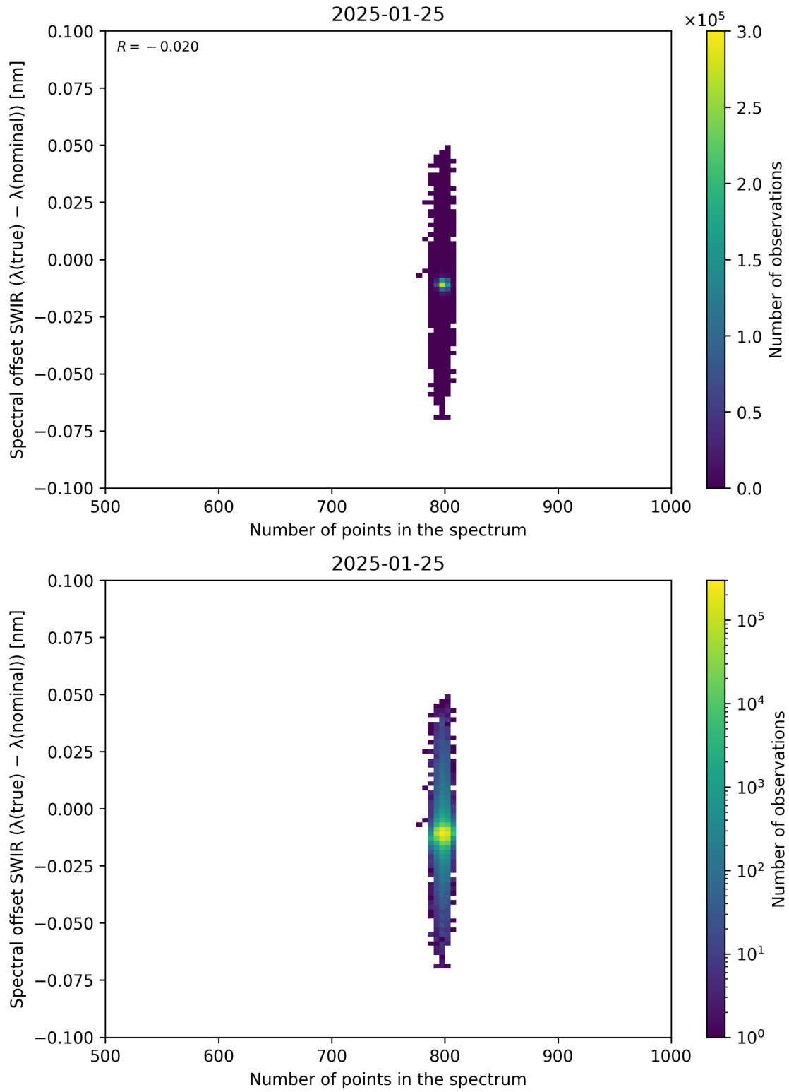
Figure 93: Scatter density plot of “Number of points in the spectrum” against “Spectral offset SWIR ( \lambda_{\text{true}} - \lambda_{\text{nominal}} )” for 2025-01-24 to 2025-01-26.
