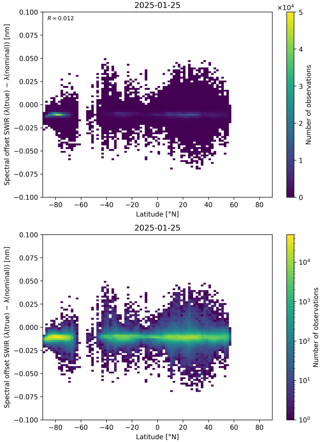
Figure 62: Scatter density plot of “Latitude” against “Spectral offset SWIR ( \lambda_{\text{true}} - \lambda_{\text{nominal}} )” for 2025-01-24 to 2025-01-26.
