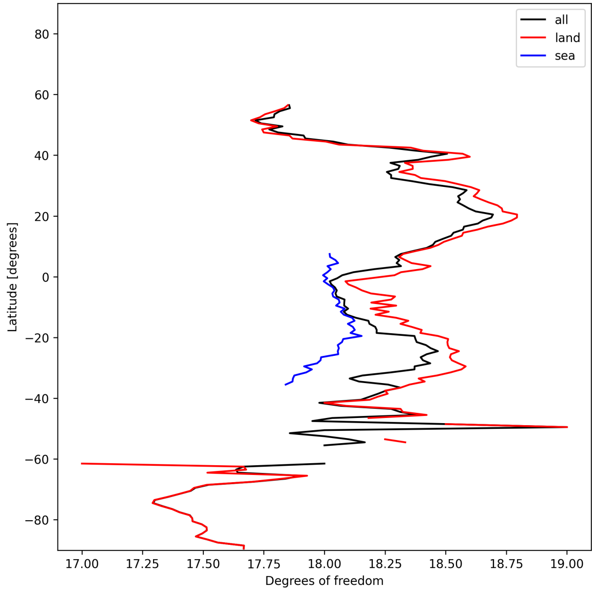
Figure 19: Zonal average of “Degrees of freedom” for 2025-01-24 to 2025-01-26.
