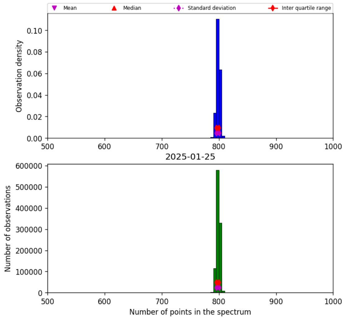
Figure 26: Histogram of “Number of points in the spectrum” for 2025-01-24 to 2025-01-26
