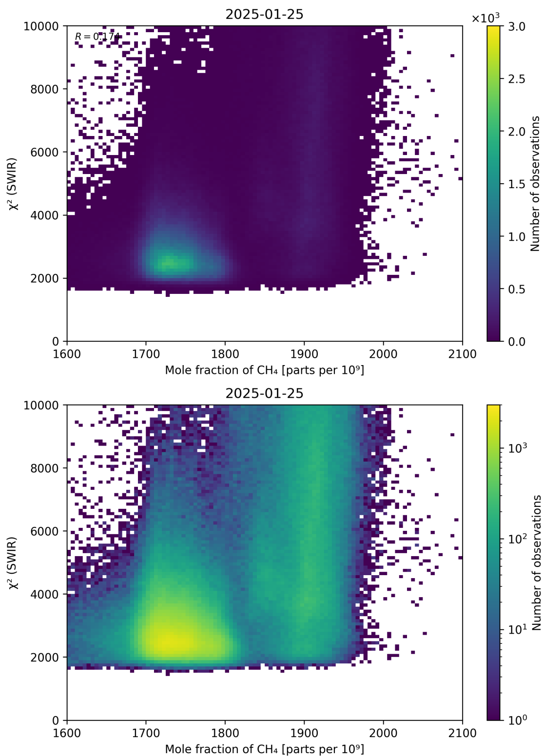
Figure 71: Scatter density plot of “Mole fraction of \text{CH}_4 ” against “ \chi^2 (SWIR)” for 2025-01-24 to 2025-01-26.
