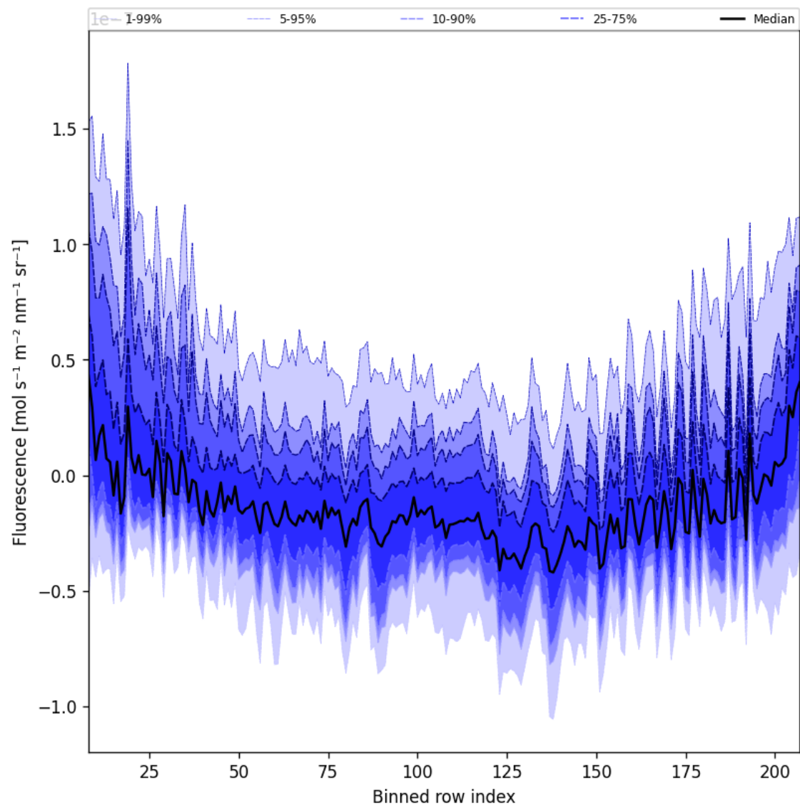
Figure 43: Along track statistics of “Fluorescence” for 2025-01-24 to 2025-01-26
