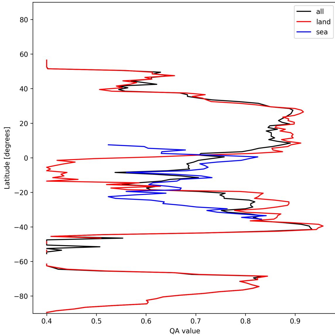
Figure 11: Zonal average of “QA value” for 2025-01-24 to 2025-01-26.
