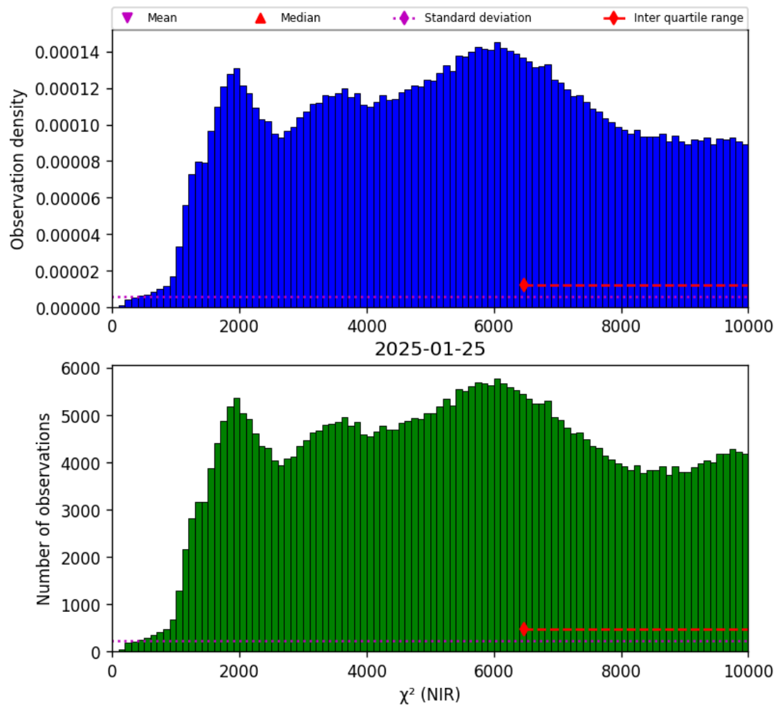
Figure 29: Histogram of “ \chi^2 (NIR)” for 2025-01-24 to 2025-01-26
