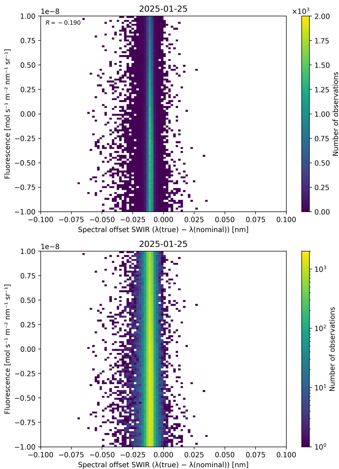
Figure 120: Scatter density plot of “Spectral offset SWIR ( \lambda_{\text{true}} - \lambda_{\text{nominal}} )” against “Fluorescence” for 2025-01-24 to 2025-01-26.
