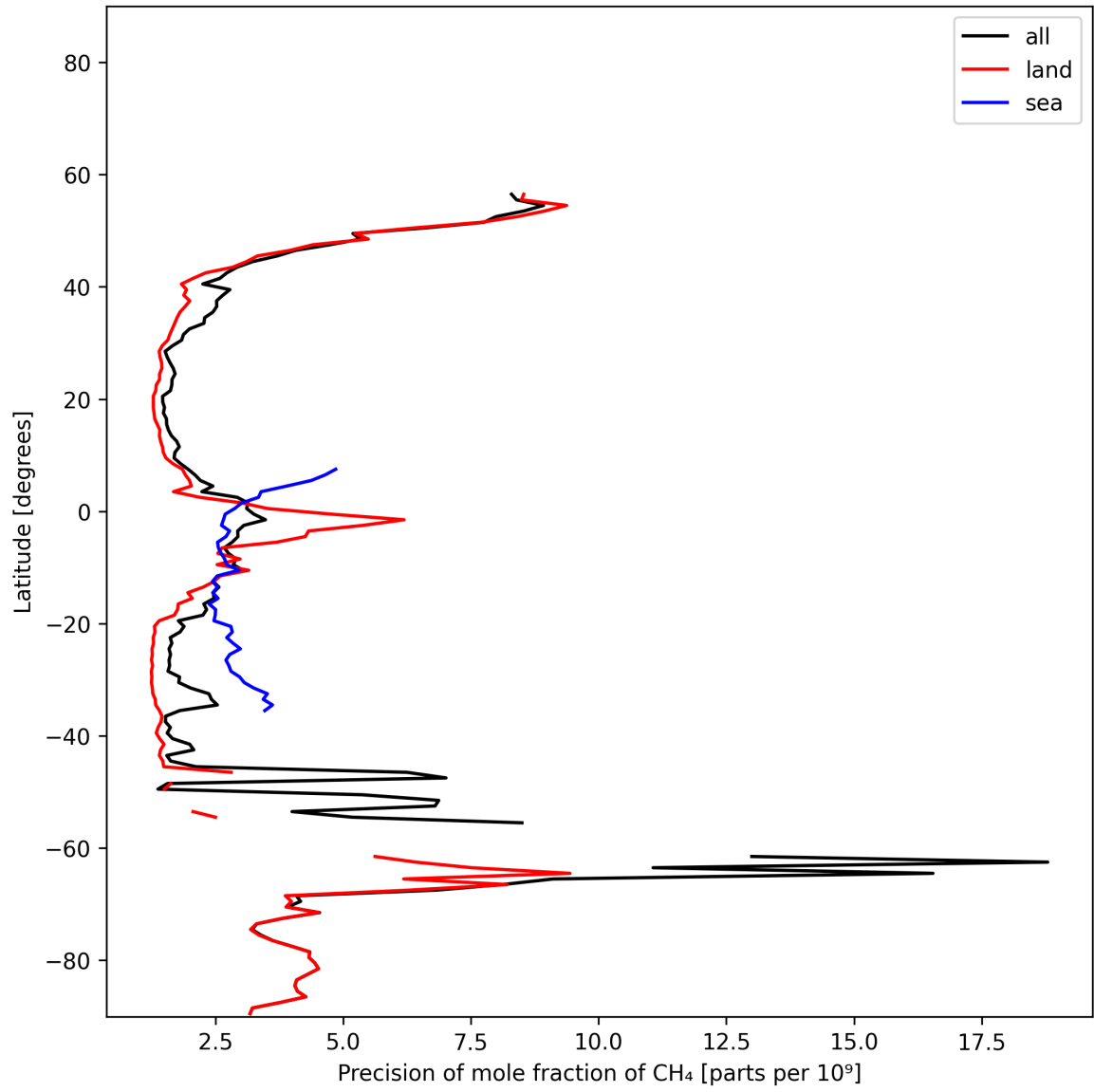
Figure 13: Zonal average of “Precision of mole fraction of CH 4 ” for 2025-01-24 to 2025-01-26.
