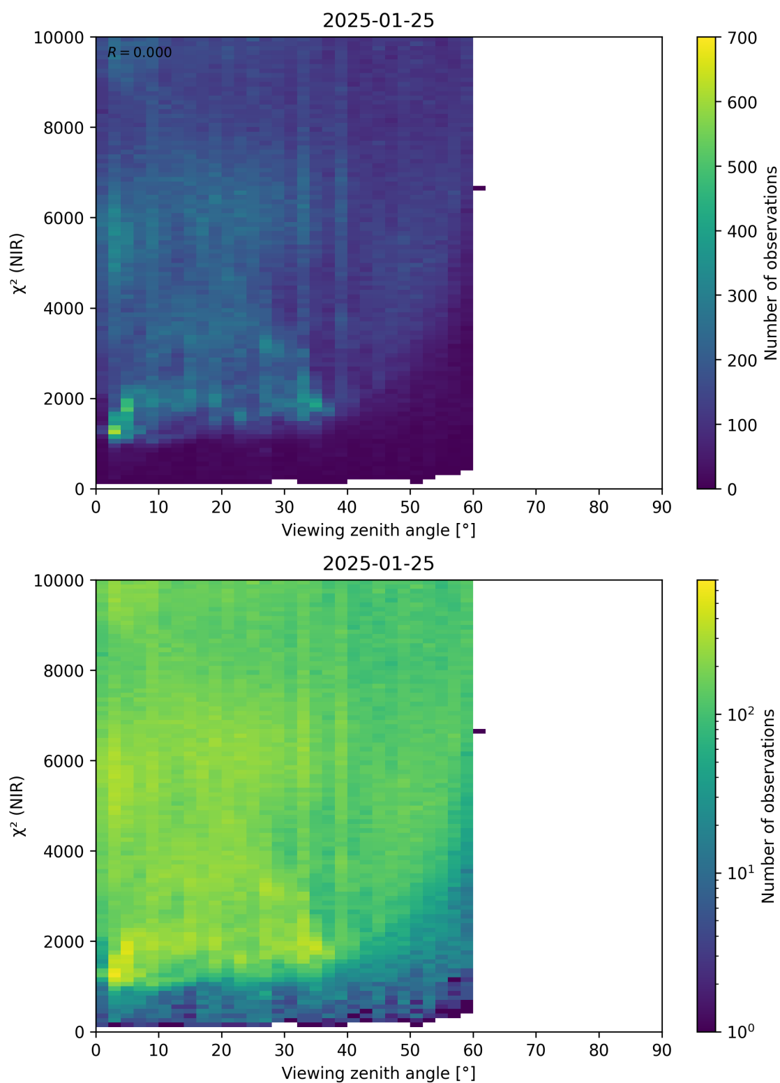
Figure 105: Scatter density plot of “Viewing zenith angle” against “ \chi^2 (NIR)” for 2025-01-24 to 2025-01-26.
