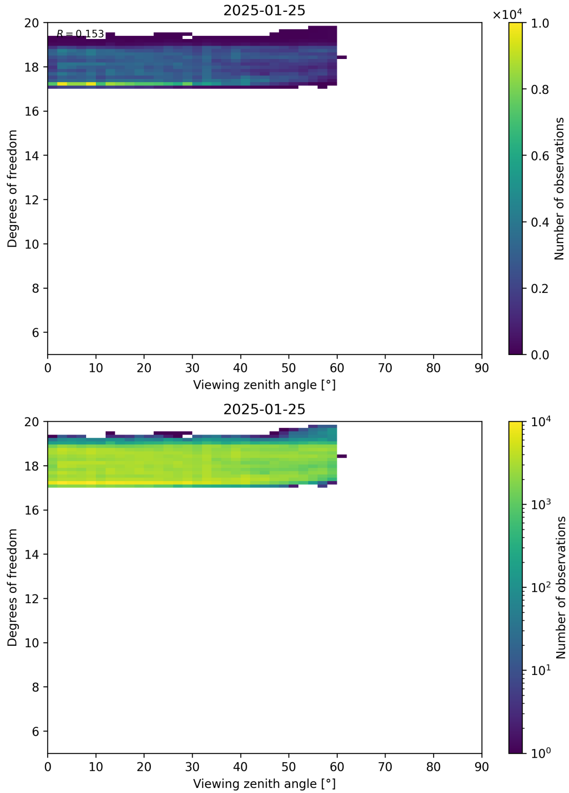
Figure 107: Scatter density plot of “Viewing zenith angle” against “Degrees of freedom” for 2025-01-24 to 2025-01-26.
