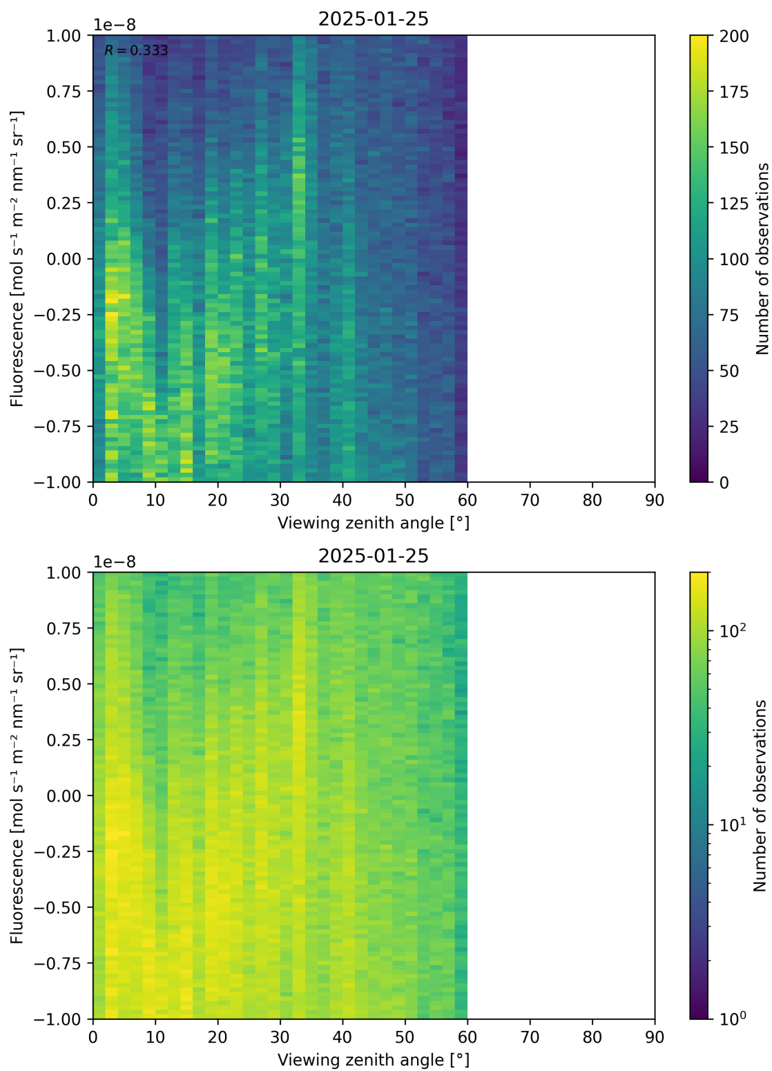
Figure 108: Scatter density plot of “Viewing zenith angle” against “Fluorescence” for 2025-01-24 to 2025-01-26.
