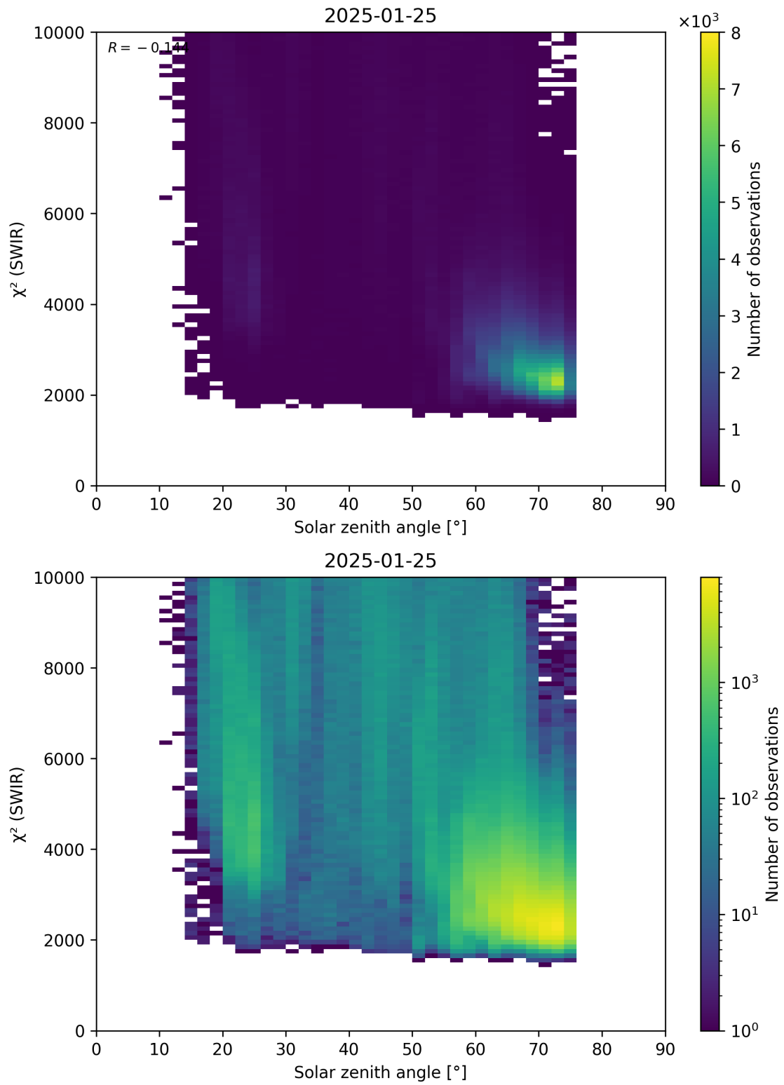
Figure 95: Scatter density plot of “Solar zenith angle” against “ \chi^2 (SWIR)” for 2025-01-24 to 2025-01-26.
