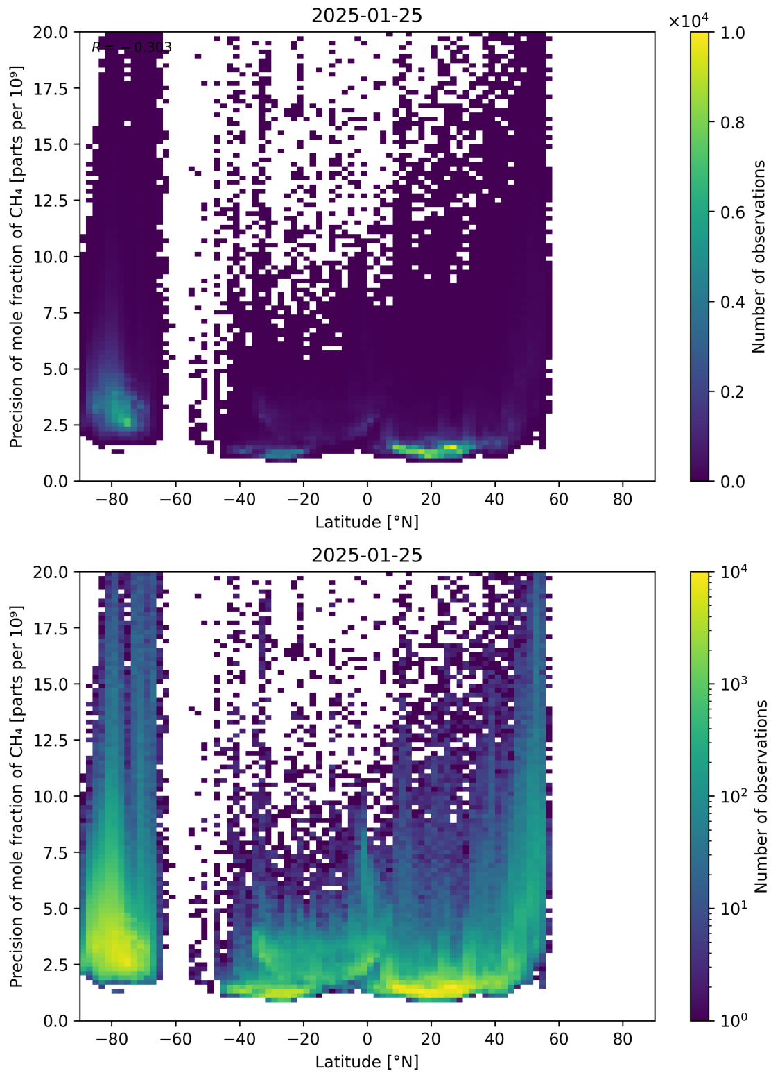
Figure 59: Scatter density plot of “Latitude” against “Precision of mole fraction of CH 4 ” for 2025-01-24 to 2025-01-26.
