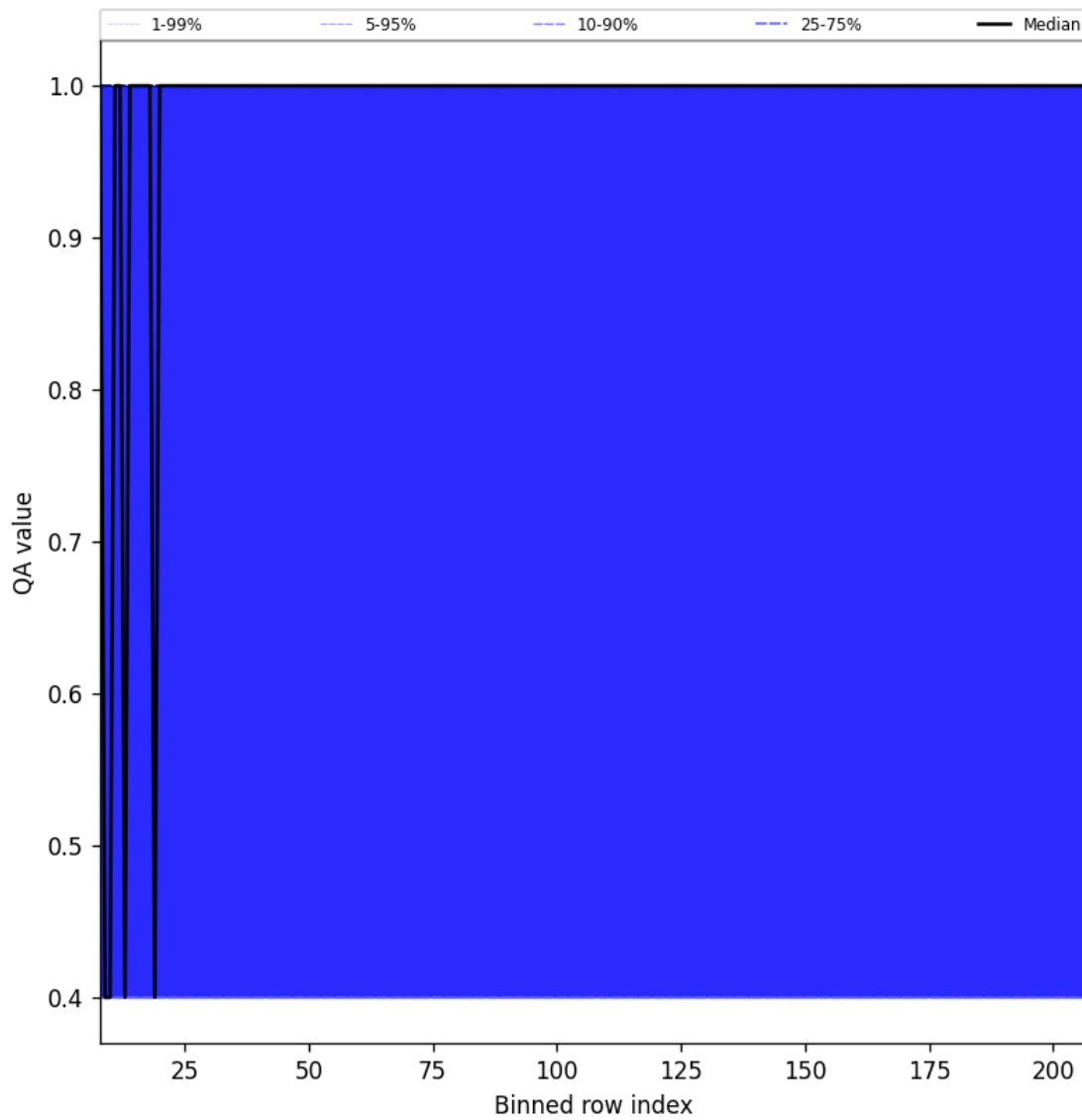
Figure 33: Along track statistics of “QA value” for 2025-01-24 to 2025-01-26
