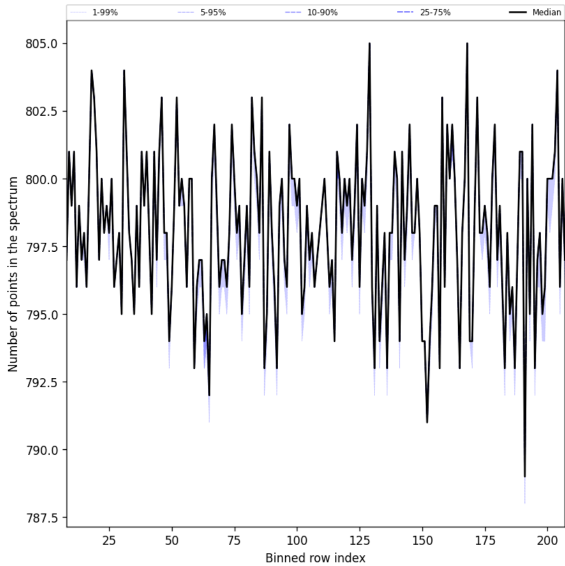
Figure 37: Along track statistics of “Number of points in the spectrum” for 2025-01-24 to 2025-01-26
