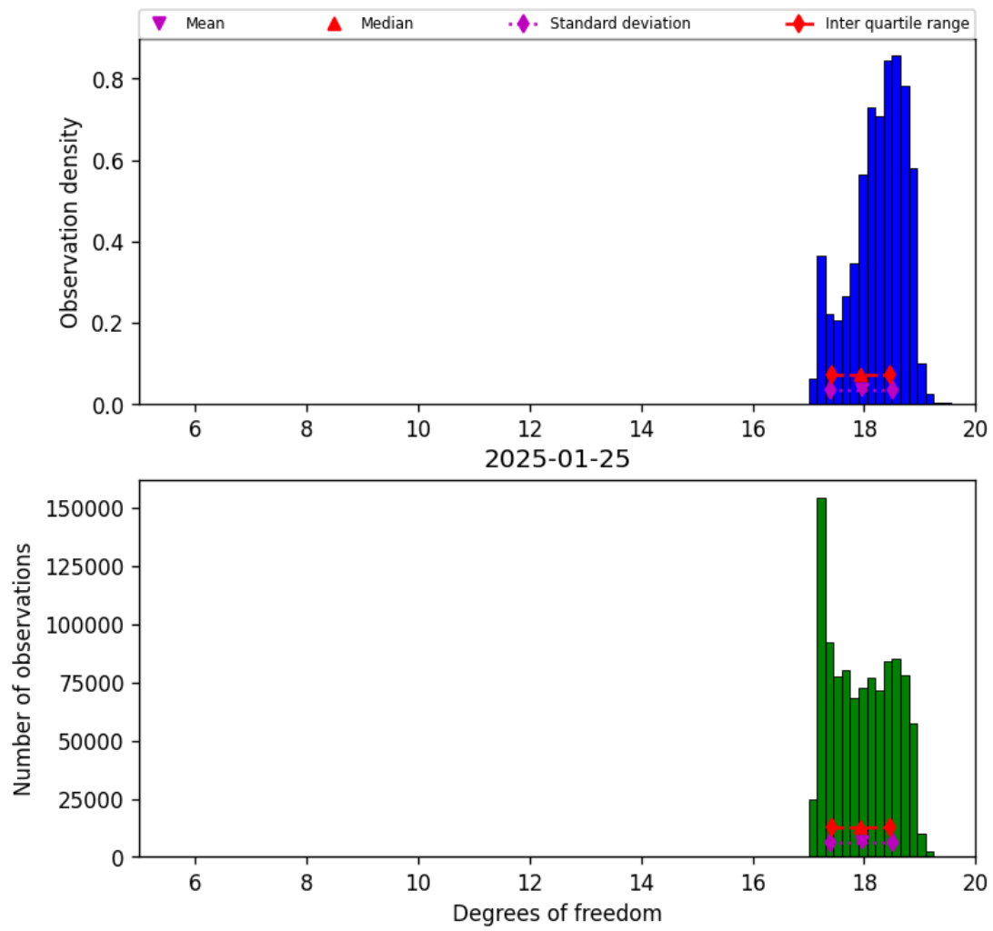
Figure 30: Histogram of "Degrees of freedom" for 2025-01-24 to 2025-01-26
