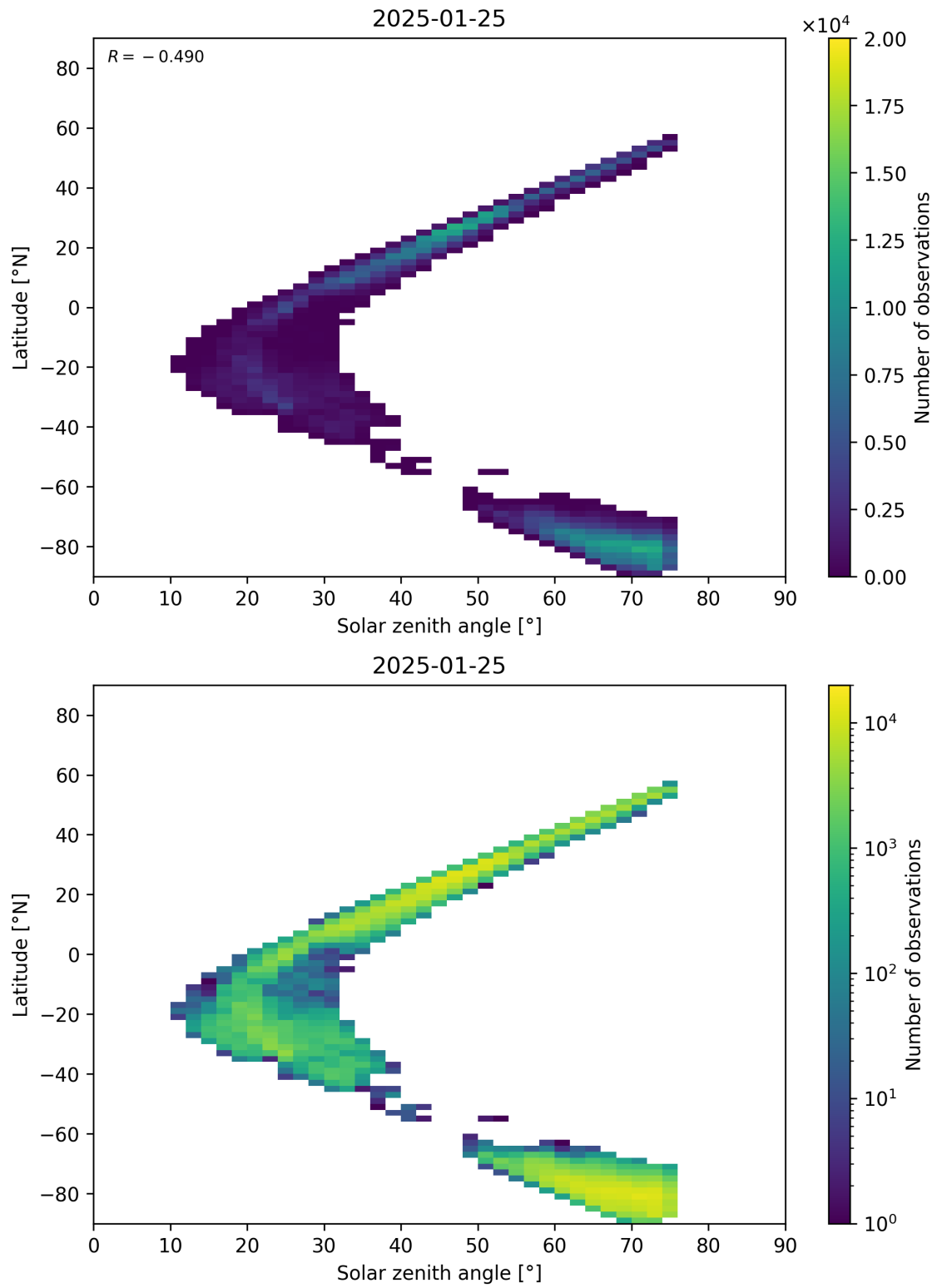
Figure 98: Scatter density plot of “Solar zenith angle” against “Latitude” for 2025-01-24 to 2025-01-26.
