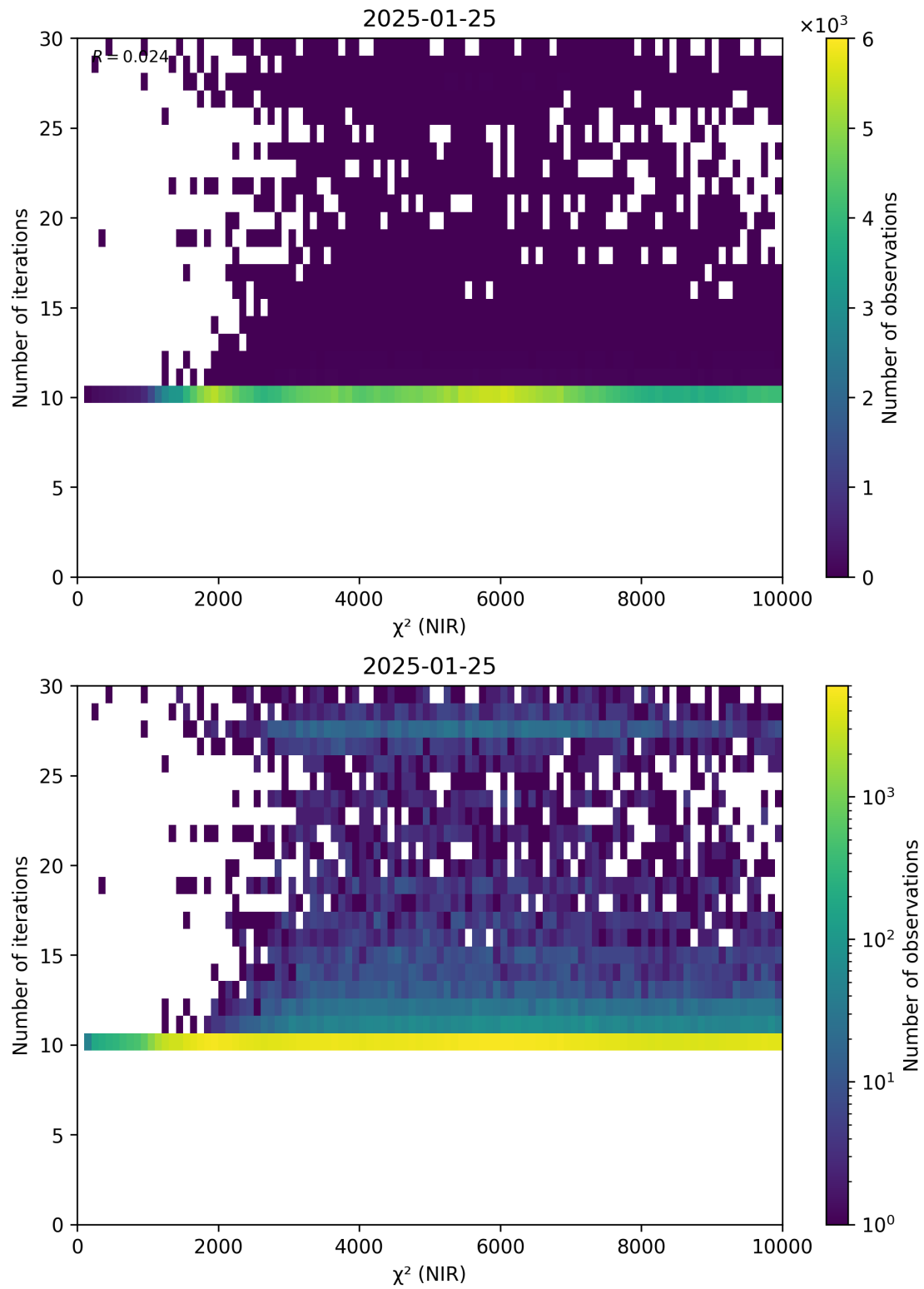
Figure 46: Scatter density plot of “ \chi^2 (NIR)” against “Number of iterations” for 2025-01-24 to 2025-01-26.
