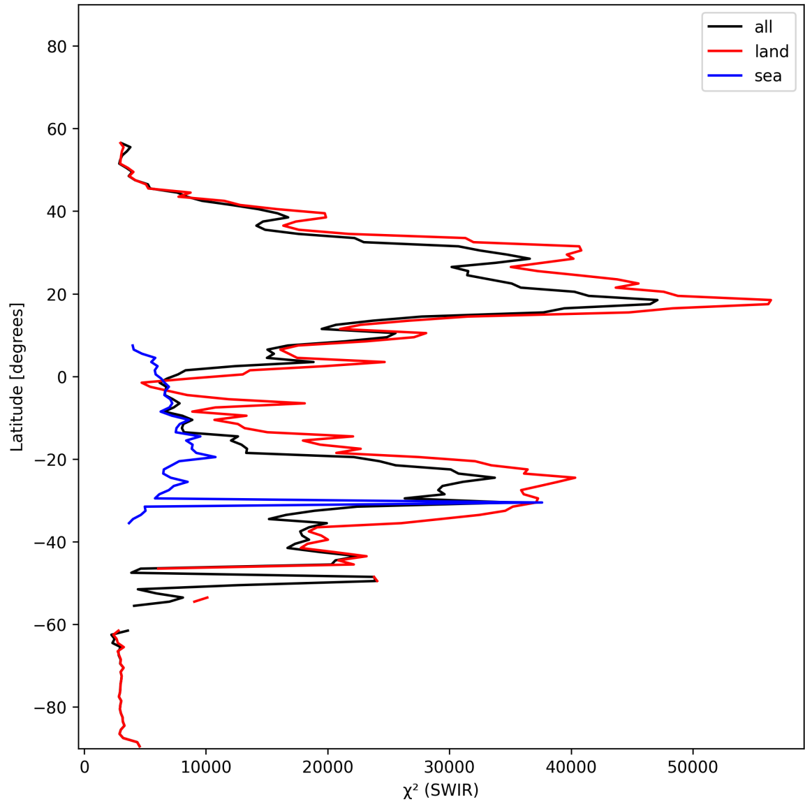
Figure 17: Zonal average of “ \chi^2 (SWIR)” for 2025-01-24 to 2025-01-26.
