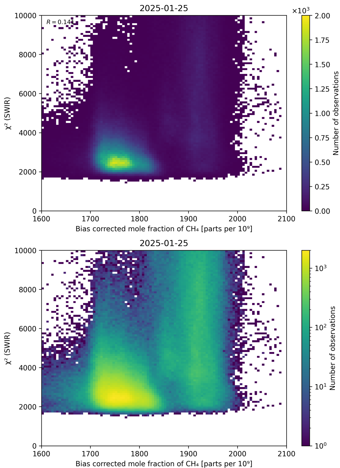
Figure 64: Scatter density plot of “Bias corrected mole fraction of \text{CH}_4 ” against “ \chi^2 (SWIR)” for 2025-01-24 to 2025-01-26.
