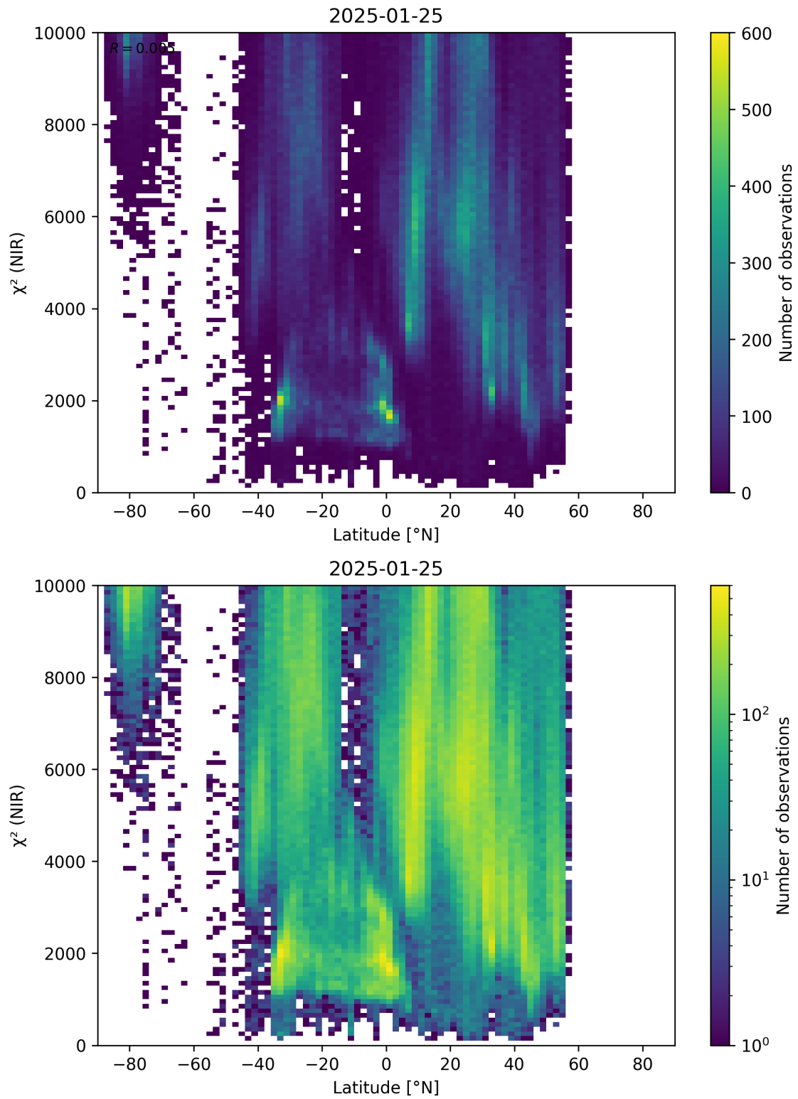
Figure 53: Scatter density plot of “Latitude” against “ \chi^2 (NIR)” for 2025-01-24 to 2025-01-26.
