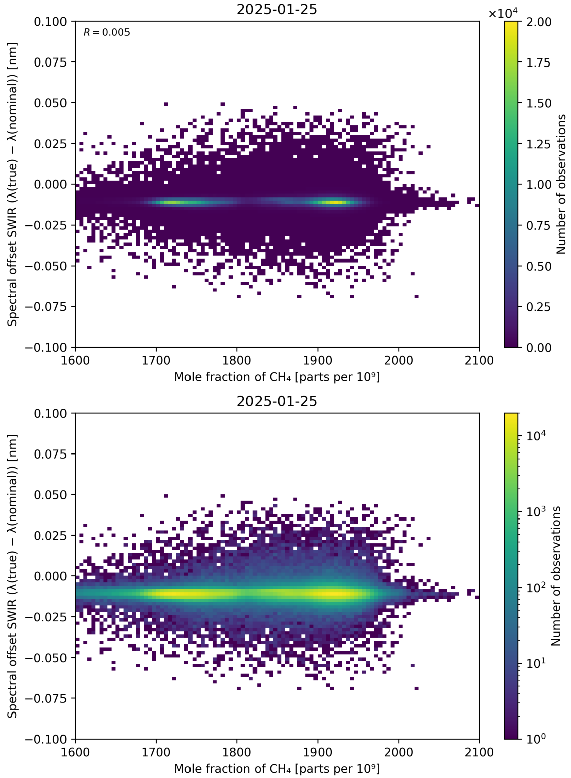
Figure 86: Scatter density plot of “Mole fraction of \text{CH}_4 ” against “Spectral offset SWIR ( \lambda_{\text{true}} - \lambda_{\text{nominal}} )” for 2025-01-24 to 2025-01-26.
