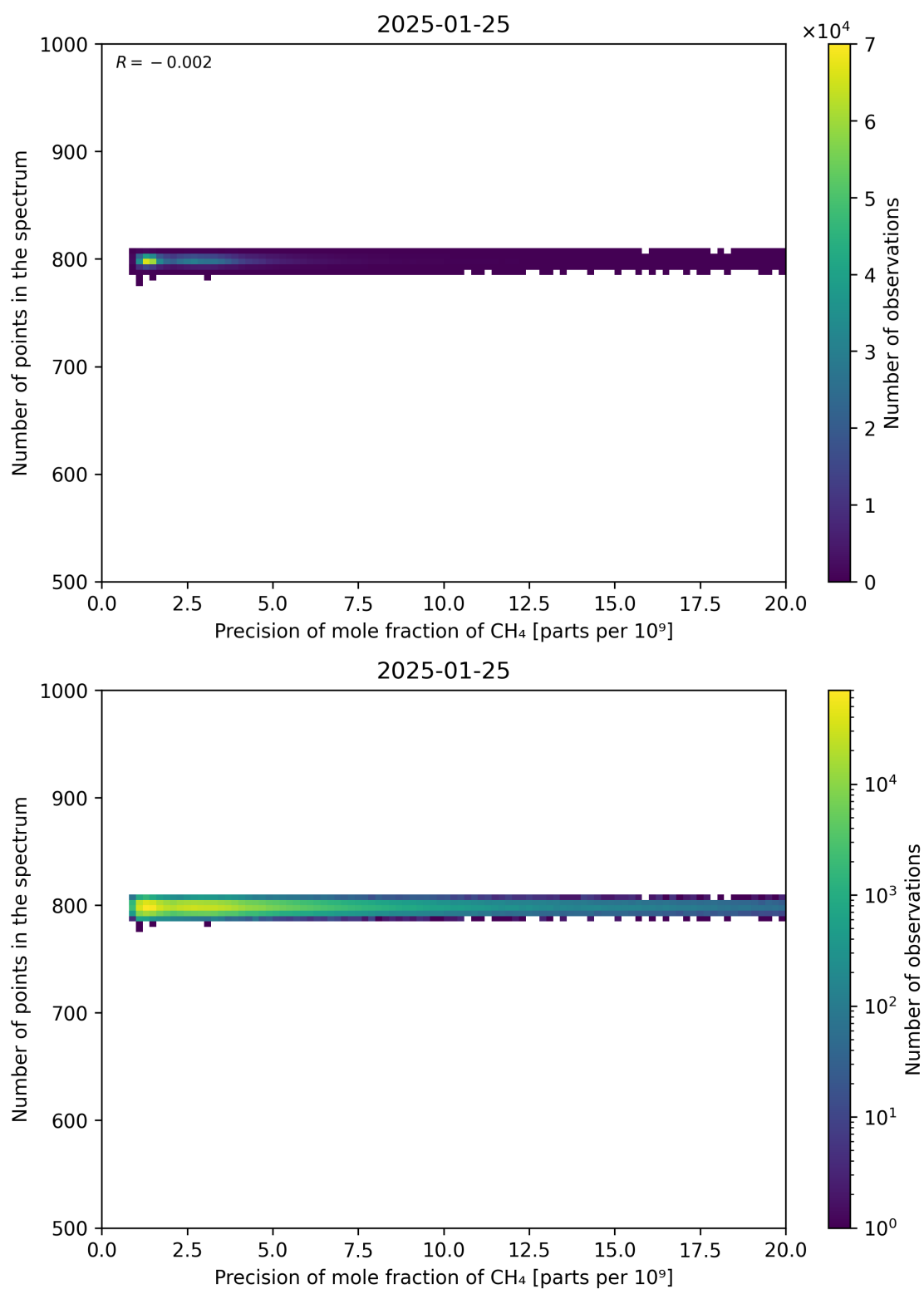
Figure 84: Scatter density plot of “Precision of mole fraction of CH 4 ” against “Number of points in the spectrum” for 2025-01-24 to 2025-01-26.
