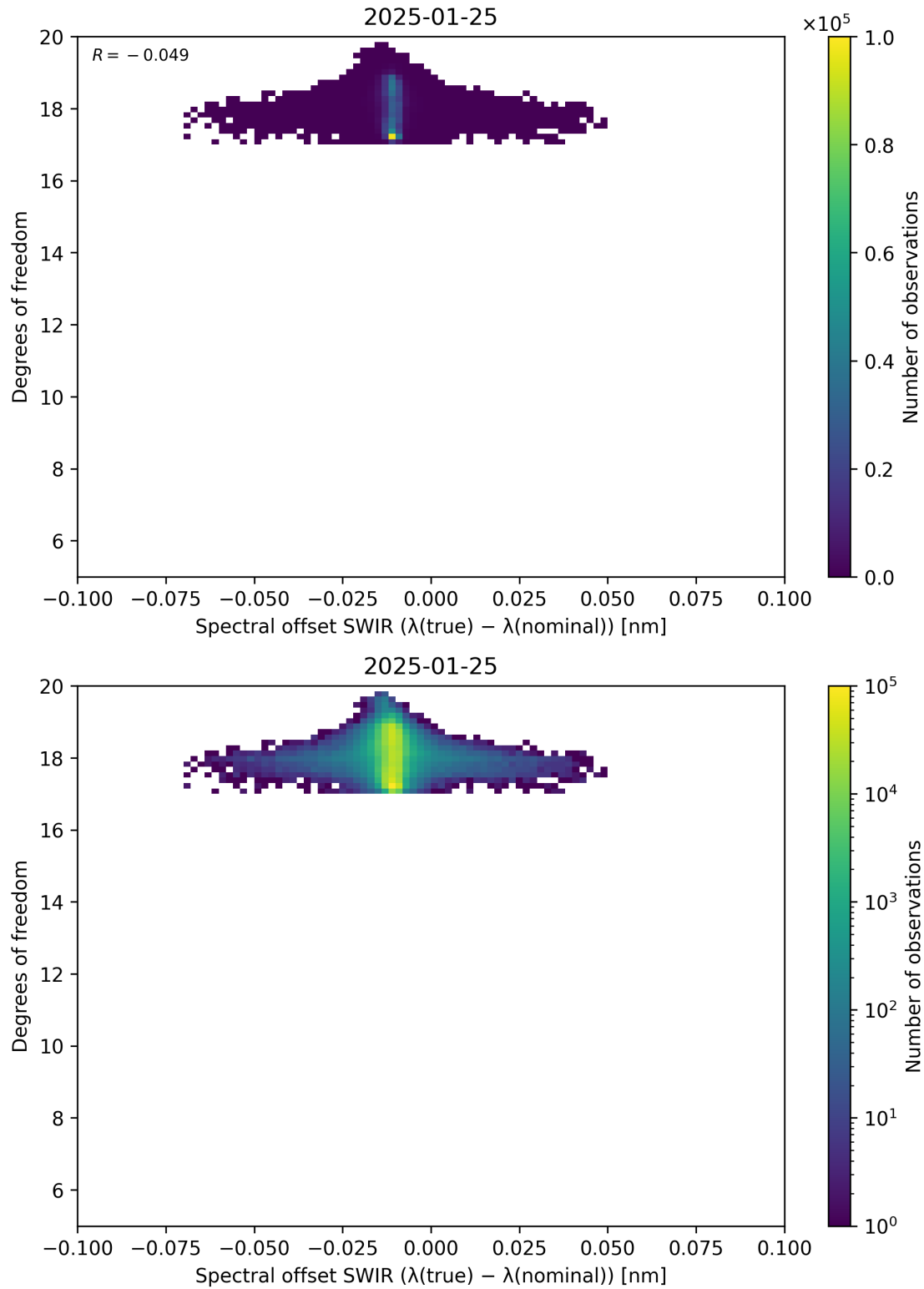
Figure 119: Scatter density plot of “Spectral offset SWIR ( \lambda_{\text{true}} - \lambda_{\text{nominal}} )” against “Degrees of freedom” for 2025-01-24 to 2025-01-26.
