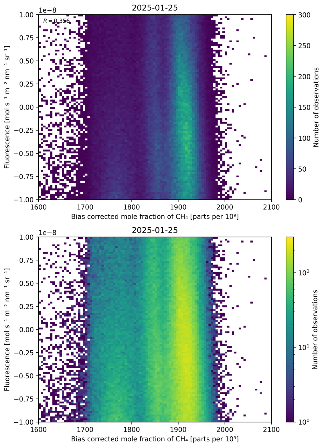
Figure 66: Scatter density plot of “Bias corrected mole fraction of CH 4 ” against “Fluorescence” for 2025-01-24 to 2025-01-26.
