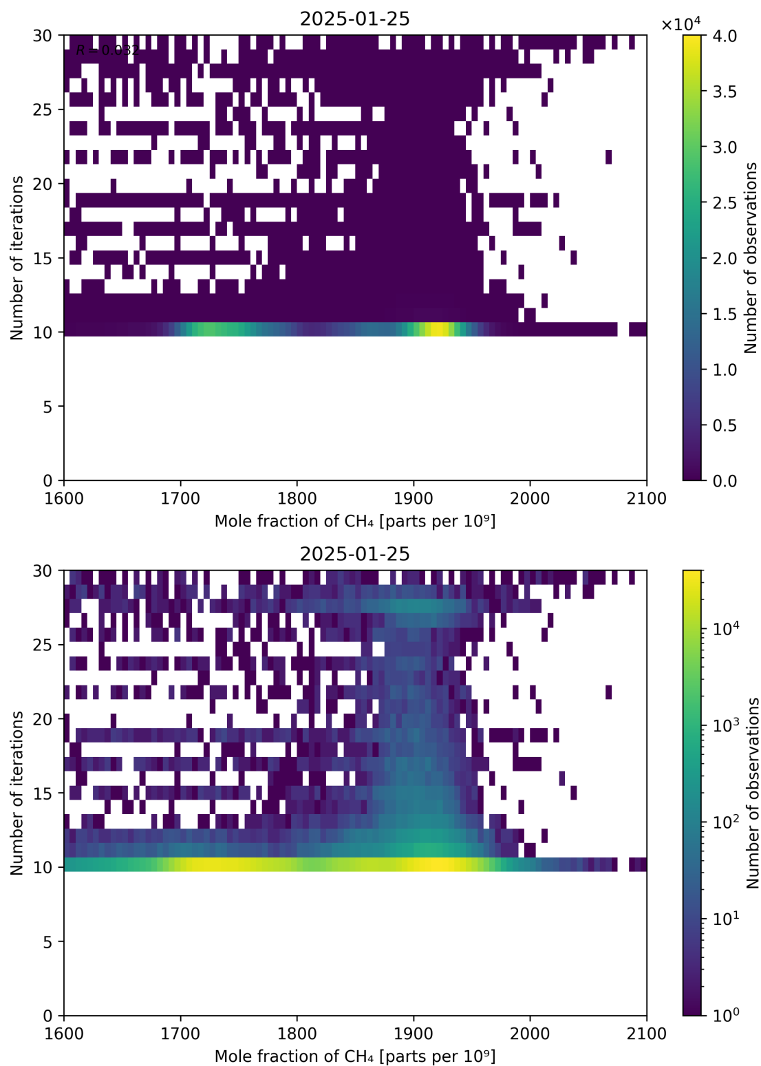
Figure 76: Scatter density plot of “Mole fraction of CH 4 ” against “Number of iterations” for 2025-01-24 to 2025-01-26.
