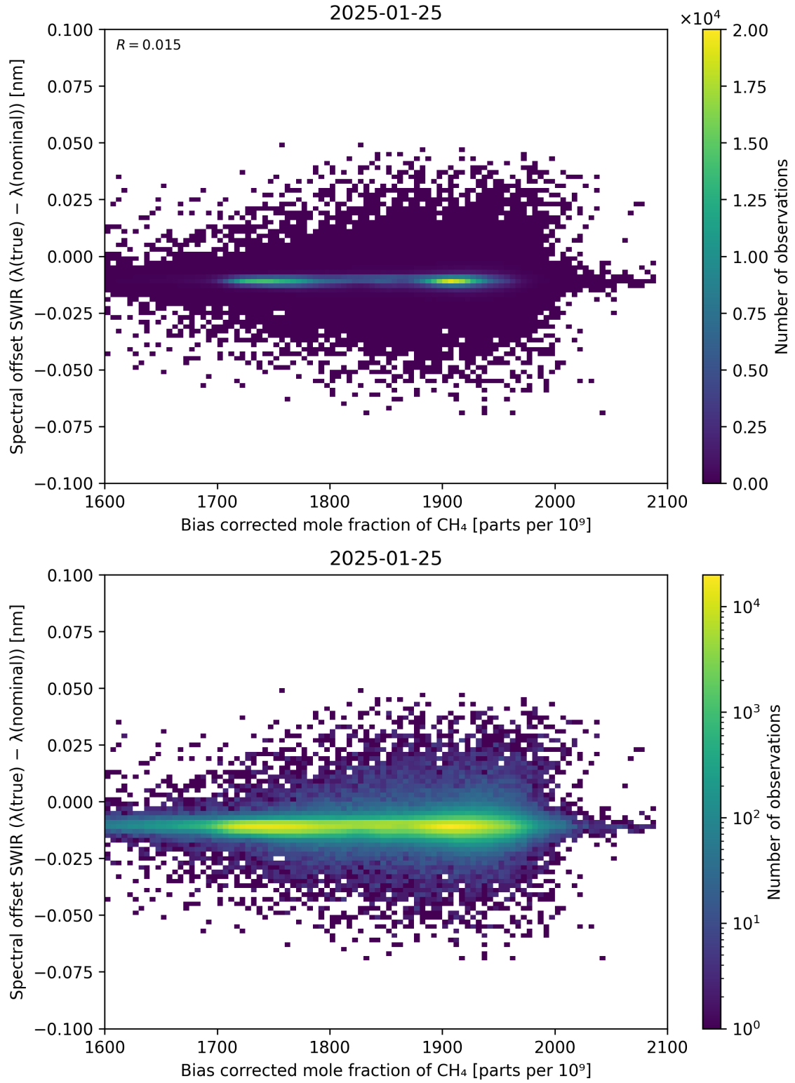
Figure 69: Scatter density plot of “Bias corrected mole fraction of \text{CH}_4 ” against “Spectral offset SWIR ( \lambda_{\text{true}} - \lambda_{\text{nominal}} )” for 2025-01-24 to 2025-01-26.
