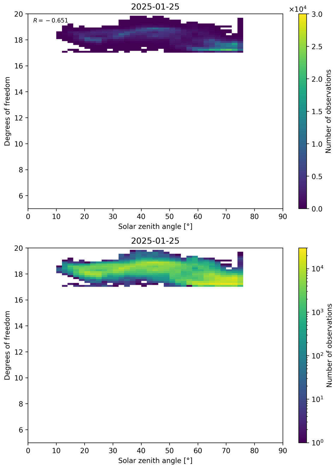
Figure 96: Scatter density plot of “Solar zenith angle” against “Degrees of freedom” for 2025-01-24 to 2025-01-26.
