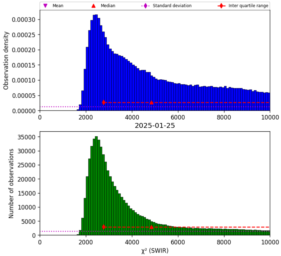
Figure 28: Histogram of “ \chi^2 (SWIR)” for 2025-01-24 to 2025-01-26
