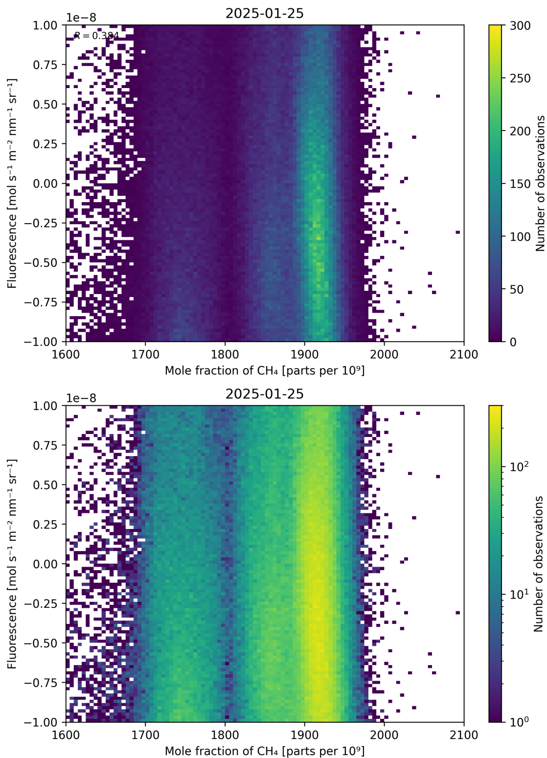
Figure 73: Scatter density plot of “Mole fraction of CH 4 ” against “Fluorescence” for 2025-01-24 to 2025-01-26.
