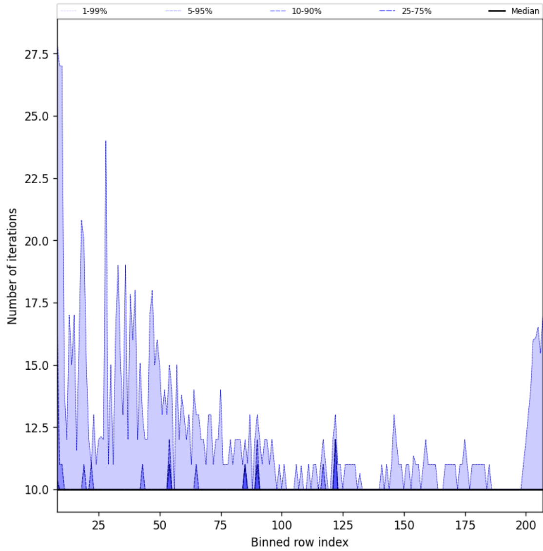
Figure 42: Along track statistics of “Number of iterations” for 2025-01-24 to 2025-01-26
