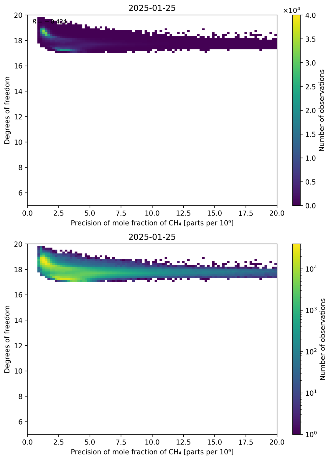
Figure 80: Scatter density plot of “Precision of mole fraction of CH 4 ” against “Degrees of freedom” for 2025-01-24 to 2025-01-26.
