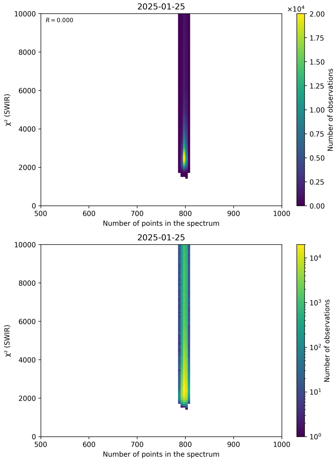
Figure 89: Scatter density plot of “Number of points in the spectrum” against “ \chi^2 (SWIR)” for 2025-01-24 to 2025-01-26.
