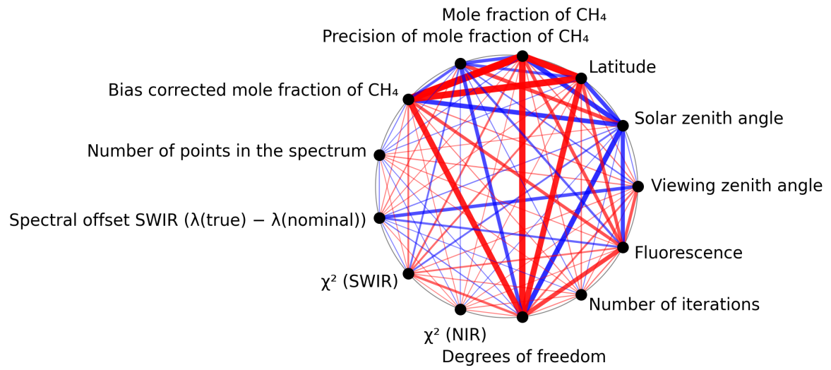
Figure 1: Map of correlation graph for 2025-01-24 to 2025-01-26.
