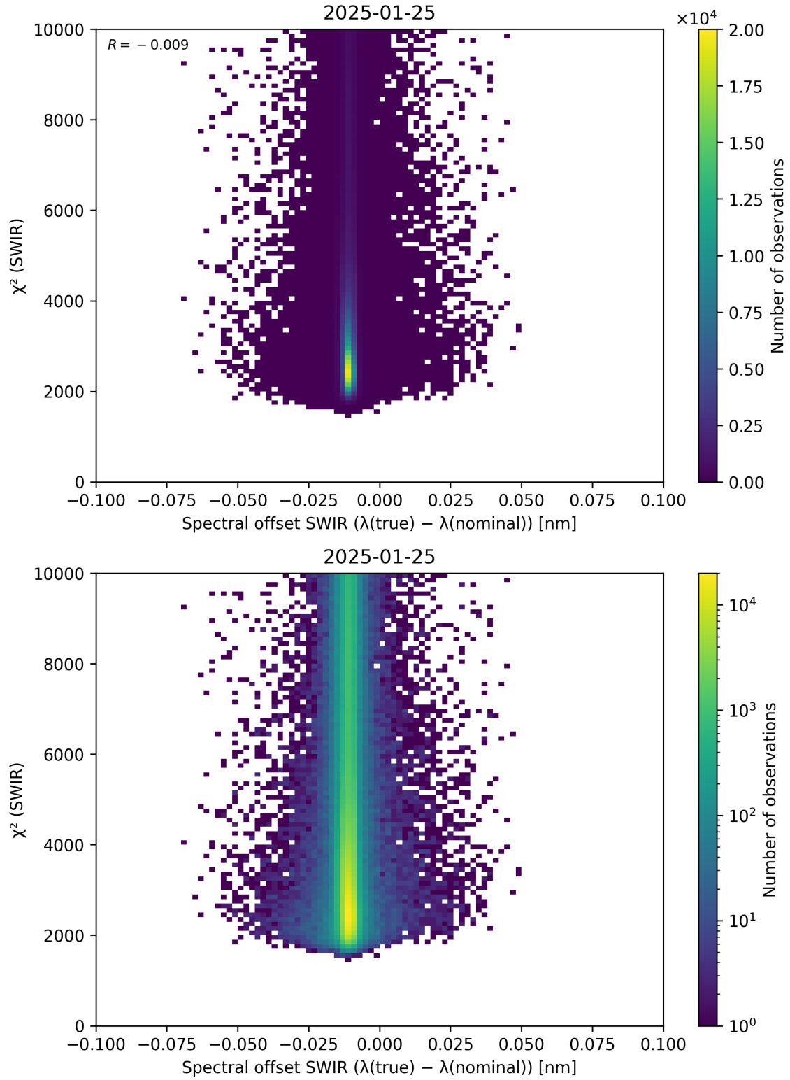
Figure 118: Scatter density plot of “Spectral offset SWIR ( \lambda_{\text{true}} - \lambda_{\text{nominal}} )” against “ \chi^2 (SWIR)” for 2025-01-24 to 2025-01-26.
