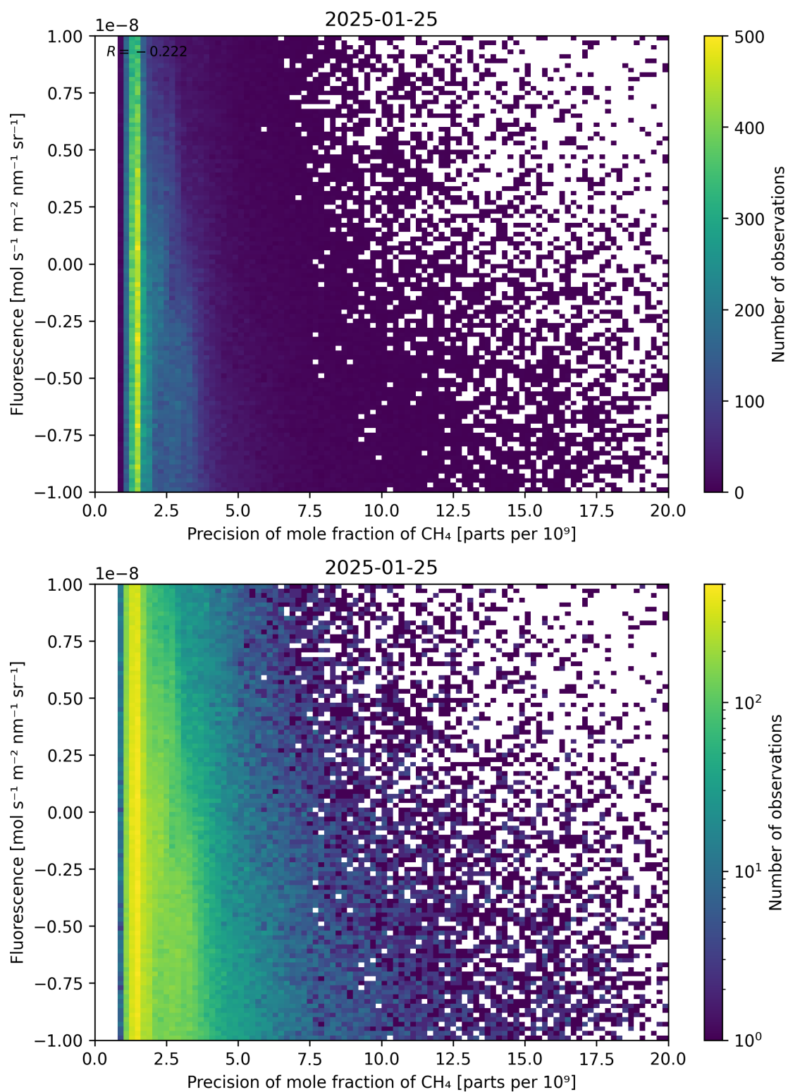
Figure 81: Scatter density plot of “Precision of mole fraction of \text{CH}_4 ” against “Fluorescence” for 2025-01-24 to 2025-01-26.
