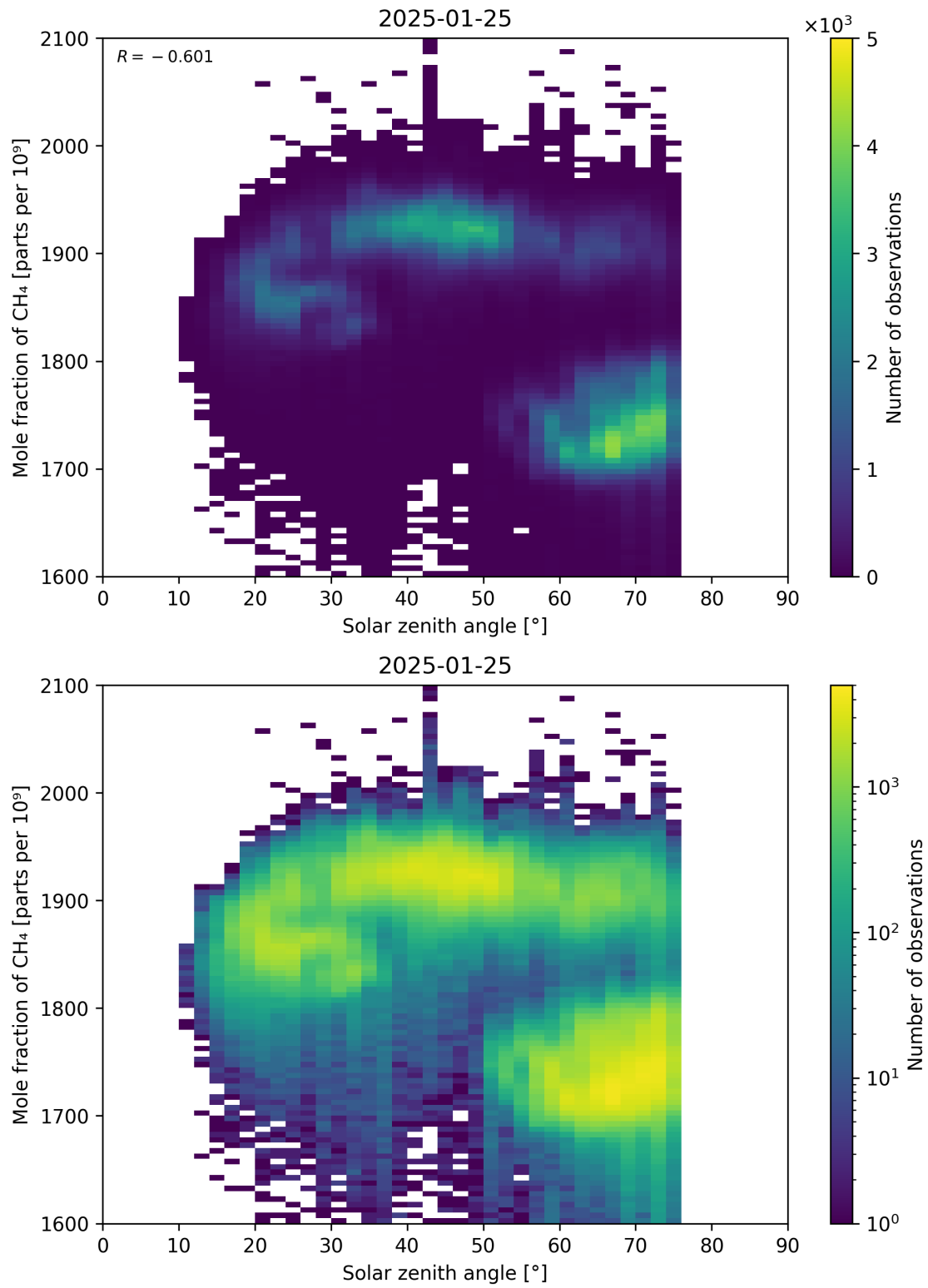
Figure 99: Scatter density plot of “Solar zenith angle” against “Mole fraction of CH 4 ” for 2025-01-24 to 2025-01-26.
