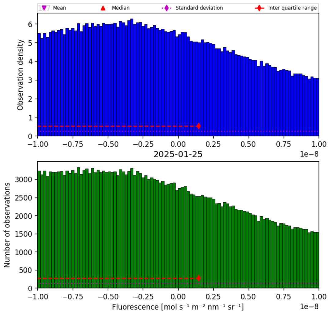
Figure 32: Histogram of “Fluorescence” for 2025-01-24 to 2025-01-26
