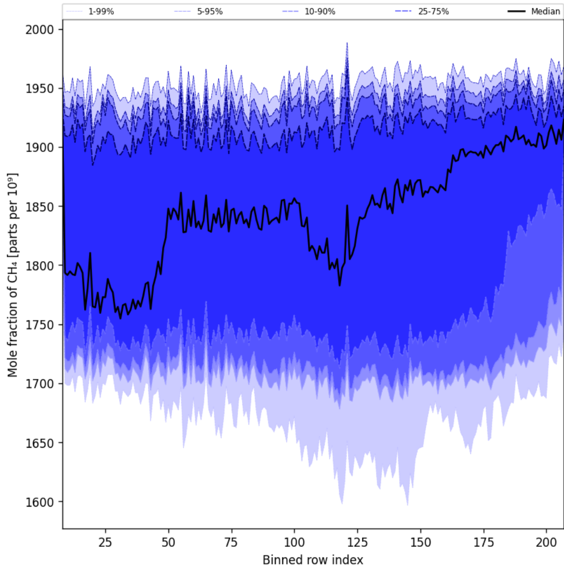
Figure 34: Along track statistics of “Mole fraction of CH 4 ” for 2025-01-24 to 2025-01-26
