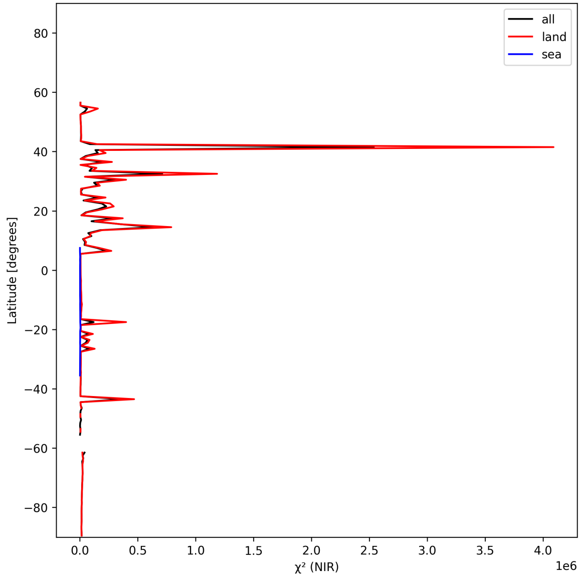
Figure 18: Zonal average of “ \chi^2 (NIR)” for 2025-01-24 to 2025-01-26.
