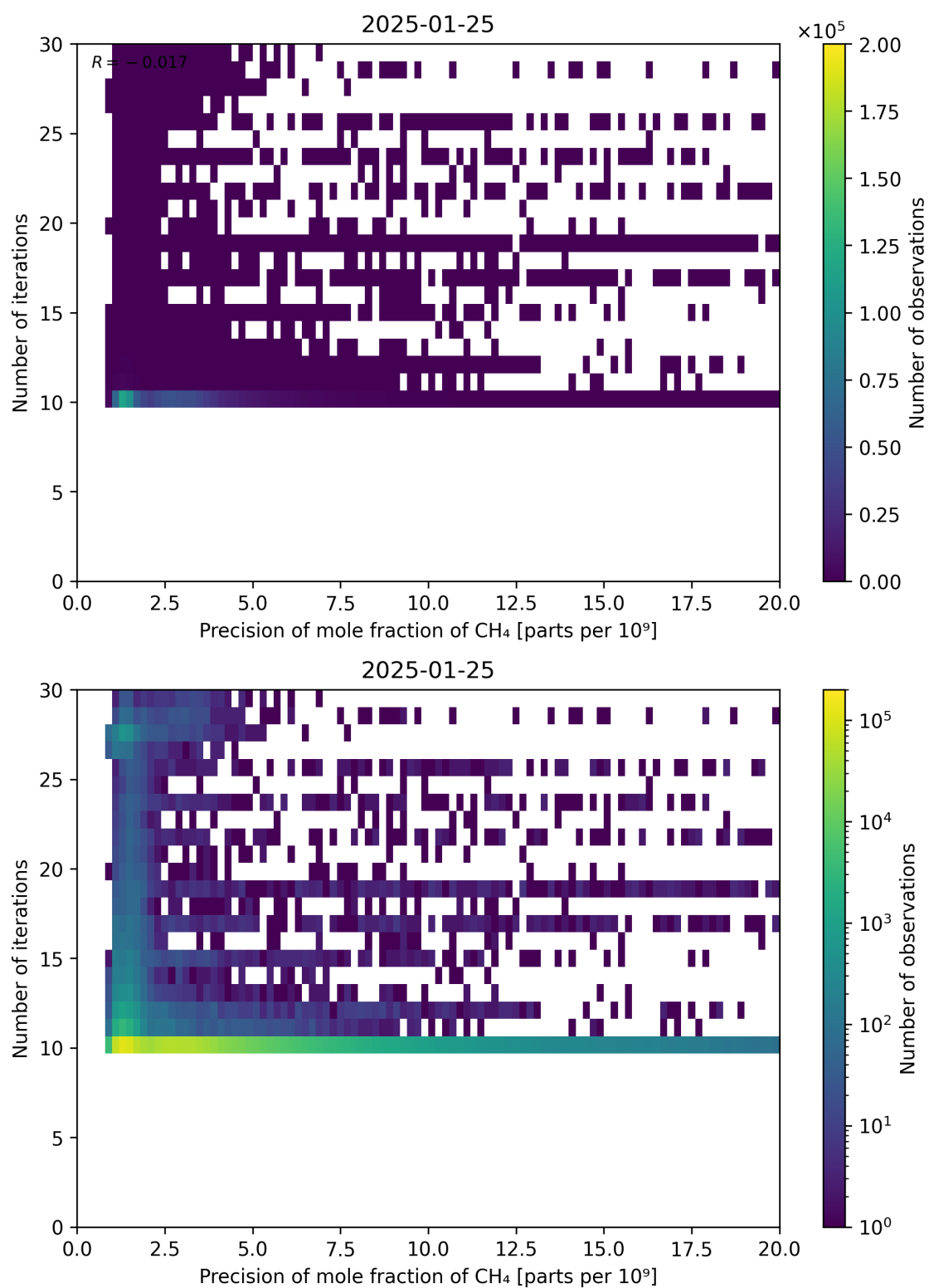
Figure 83: Scatter density plot of “Precision of mole fraction of CH 4 ” against “Number of iterations” for 2025-01-24 to 2025-01-26.
