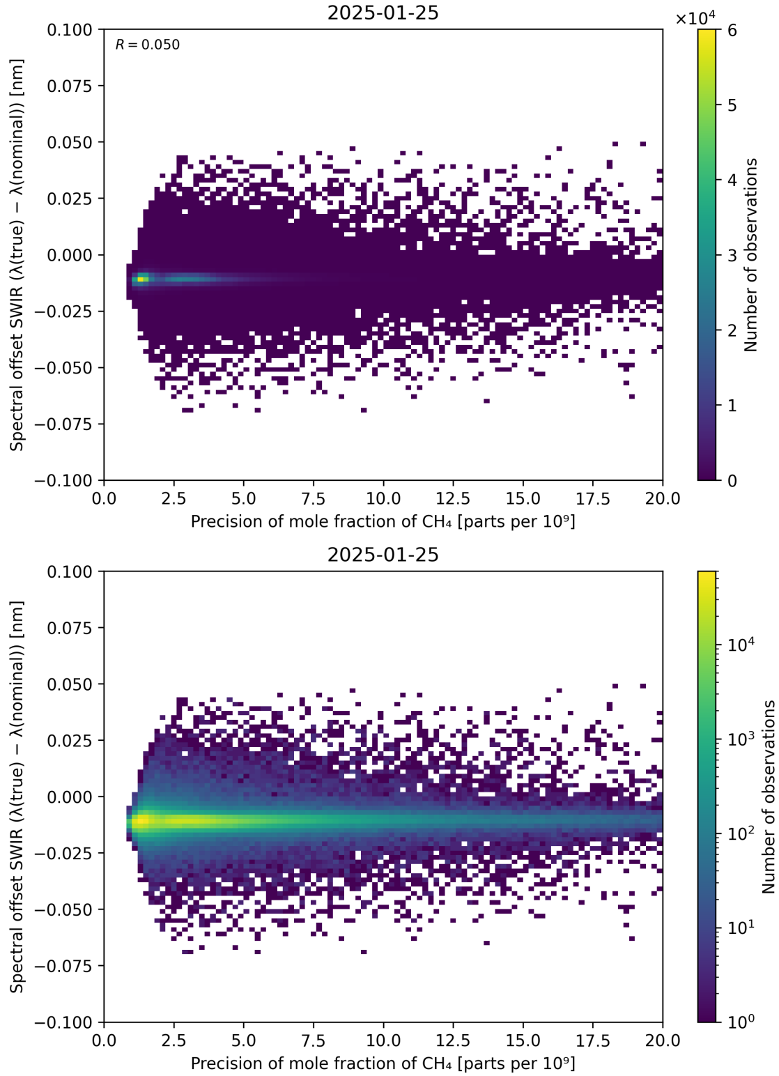
Figure 85: Scatter density plot of “Precision of mole fraction of CH 4 ” against “Spectral offset SWIR ( \lambda_{\text{true}} - \lambda_{\text{nominal}} )” for 2025-01-24 to 2025-01-26.
