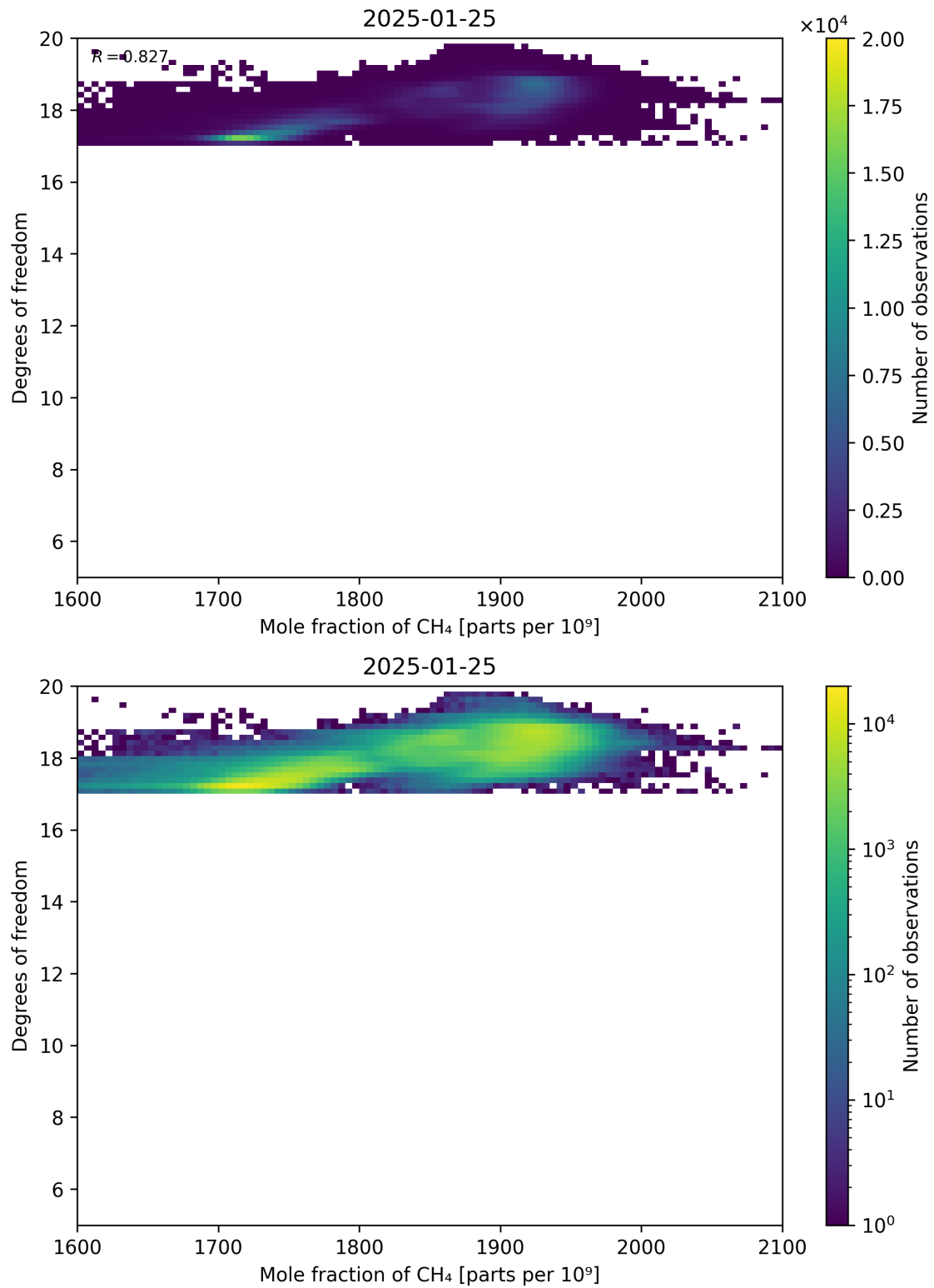
Figure 72: Scatter density plot of “Mole fraction of CH 4 ” against “Degrees of freedom” for 2025-01-24 to 2025-01-26.
