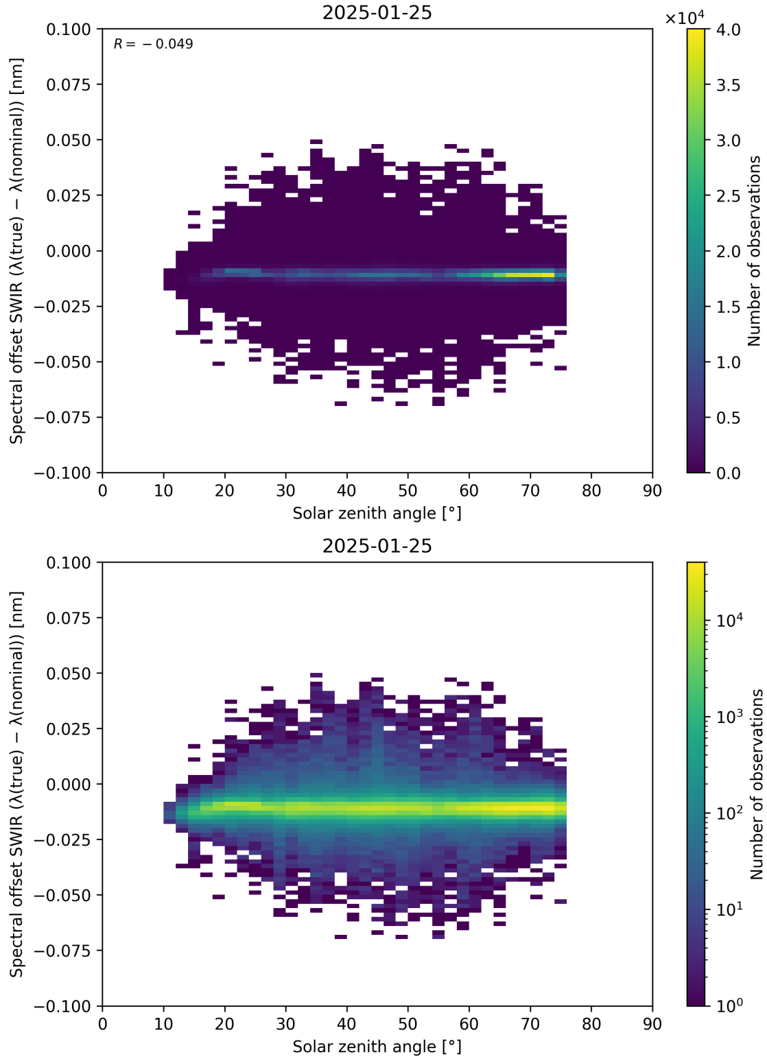
Figure 104: Scatter density plot of “Solar zenith angle” against “Spectral offset SWIR ( \lambda_{\text{true}} - \lambda_{\text{nominal}} )” for 2025-01-24 to 2025-01-26.
