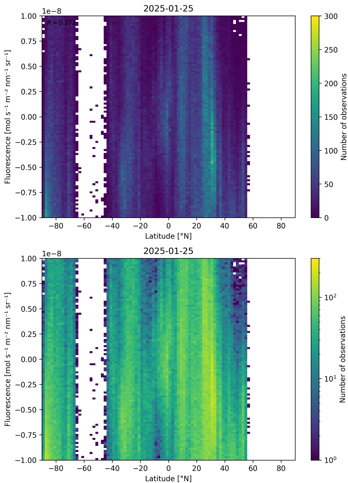
Figure 56: Scatter density plot of “Latitude” against “Fluorescence” for 2025-01-24 to 2025-01-26.
