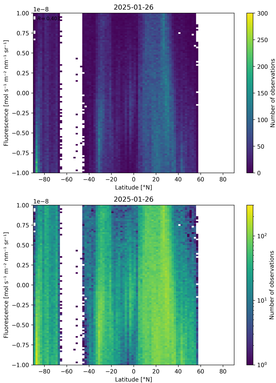
Figure 56: Scatter density plot of “Latitude” against “Fluorescence” for 2025-01-25 to 2025-01-27.
