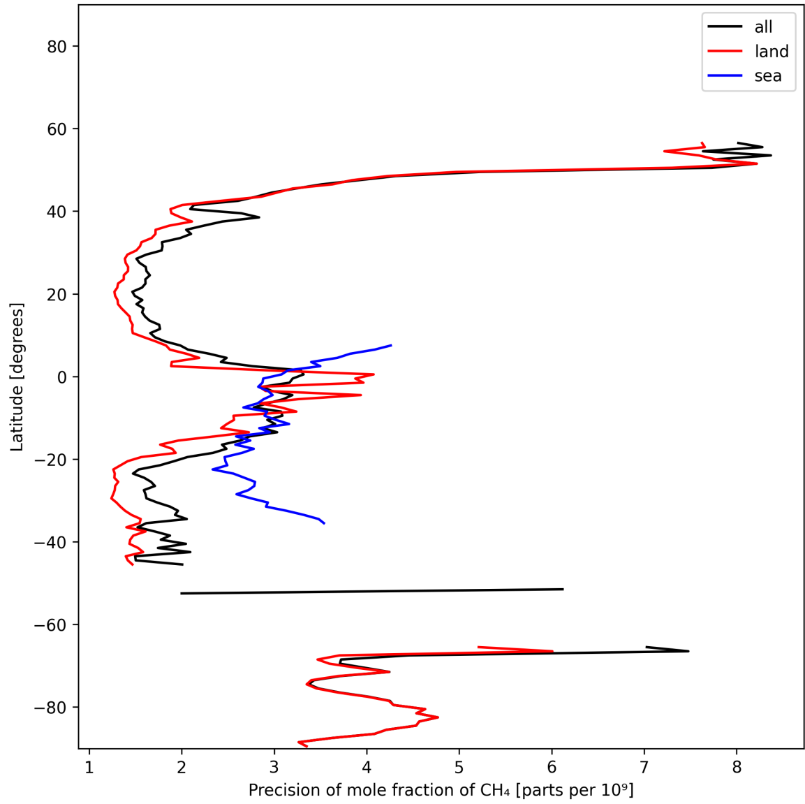
Figure 13: Zonal average of “Precision of mole fraction of CH 4 ” for 2025-01-25 to 2025-01-27.
