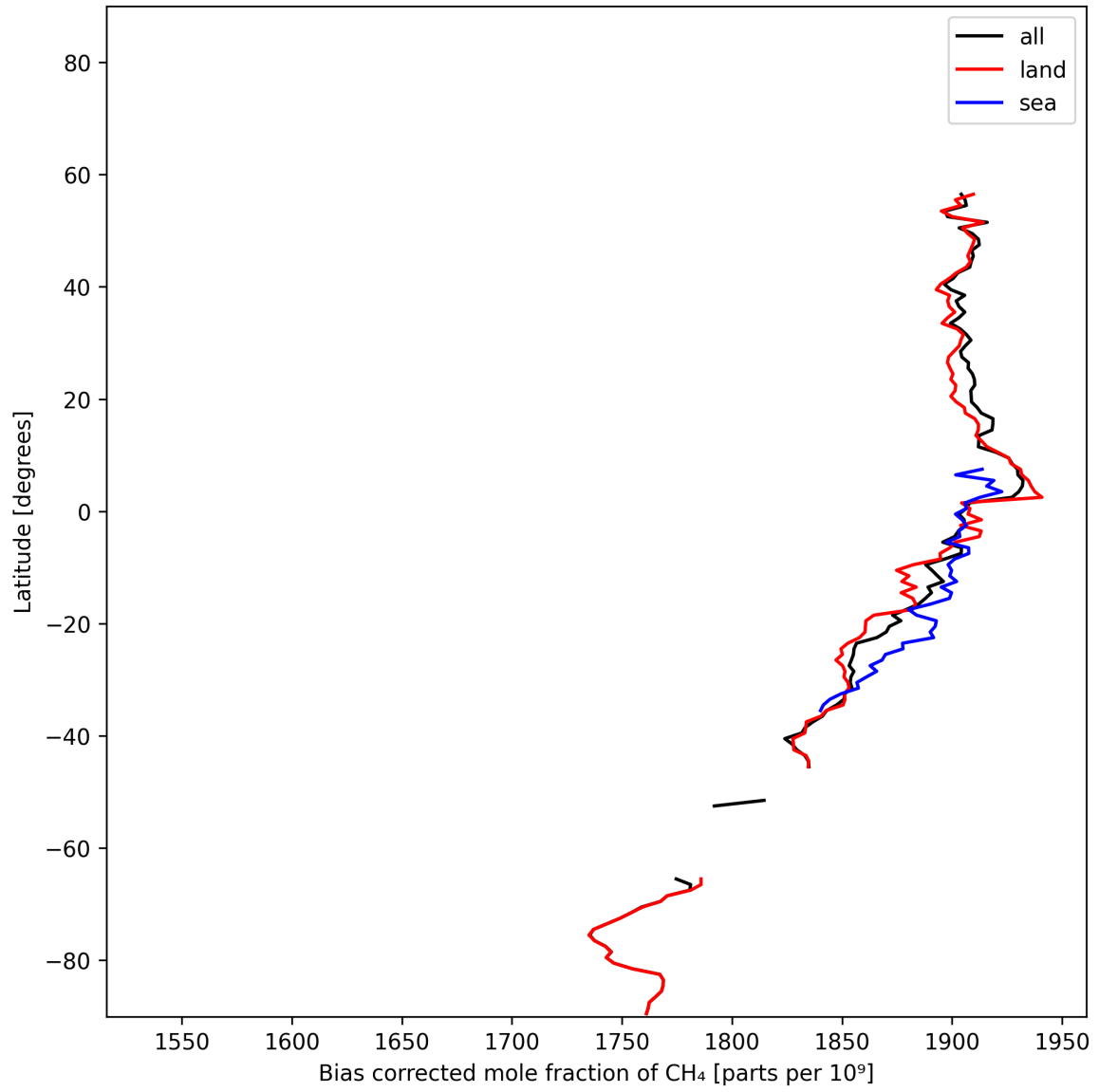
Figure 14: Zonal average of “Bias corrected mole fraction of CH 4 ” for 2025-01-25 to 2025-01-27.
