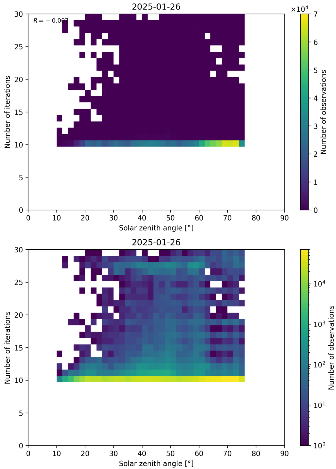
Figure 102: Scatter density plot of “Solar zenith angle” against “Number of iterations” for 2025-01-25 to 2025-01-27.
