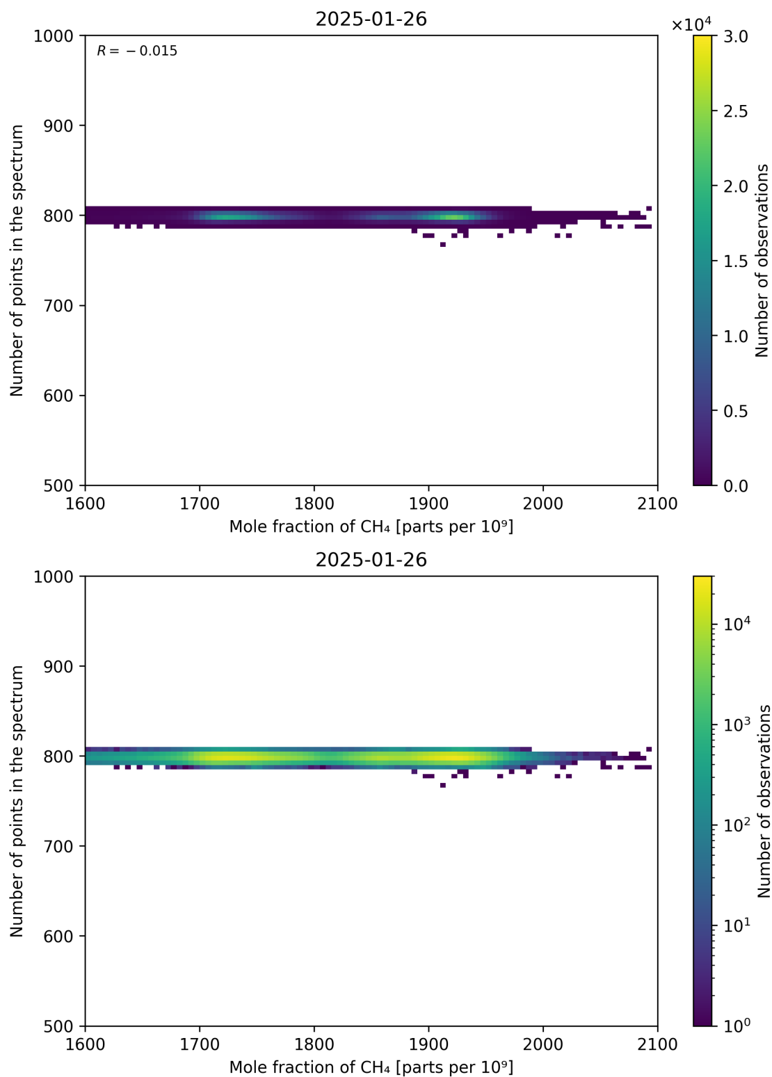
Figure 77: Scatter density plot of “Mole fraction of CH 4 ” against “Number of points in the spectrum” for 2025-01-25 to 2025-01-27.
