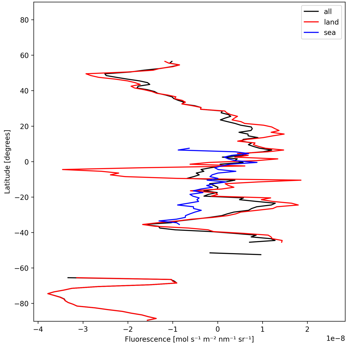
Figure 21: Zonal average of “Fluorescence” for 2025-01-25 to 2025-01-27.
