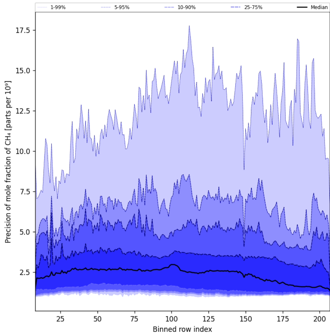
Figure 35: Along track statistics of “Precision of mole fraction of CH 4 ” for 2025-01-25 to 2025-01-27
