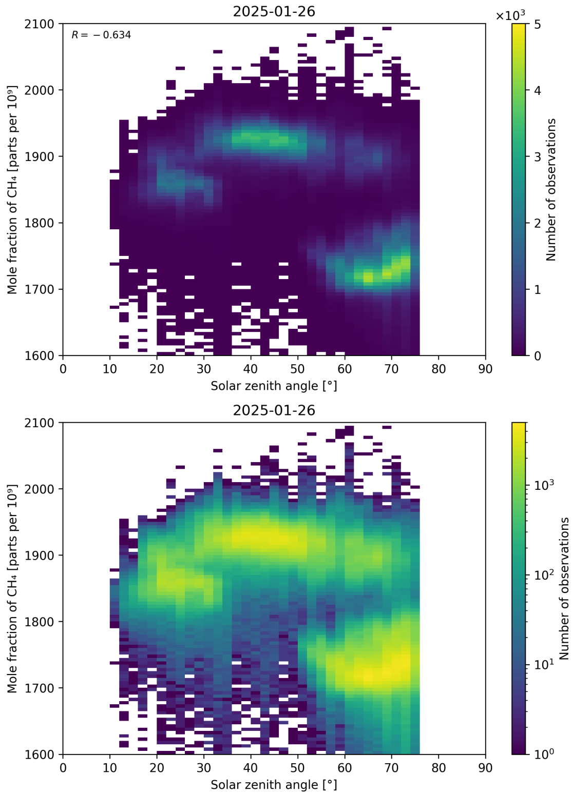
Figure 99: Scatter density plot of “Solar zenith angle” against “Mole fraction of CH 4 ” for 2025-01-25 to 2025-01-27.
