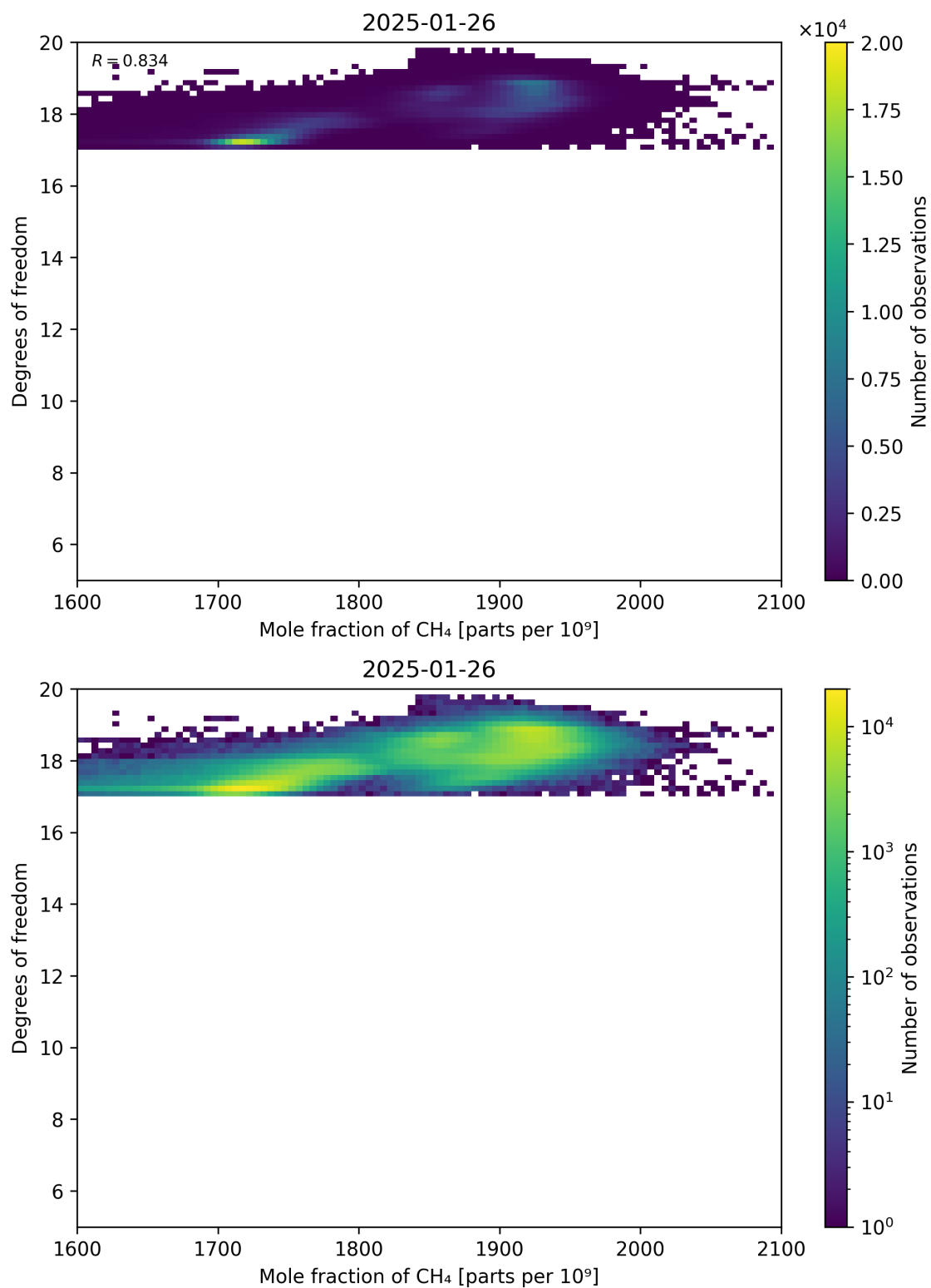
Figure 72: Scatter density plot of “Mole fraction of CH 4 ” against “Degrees of freedom” for 2025-01-25 to 2025-01-27.
