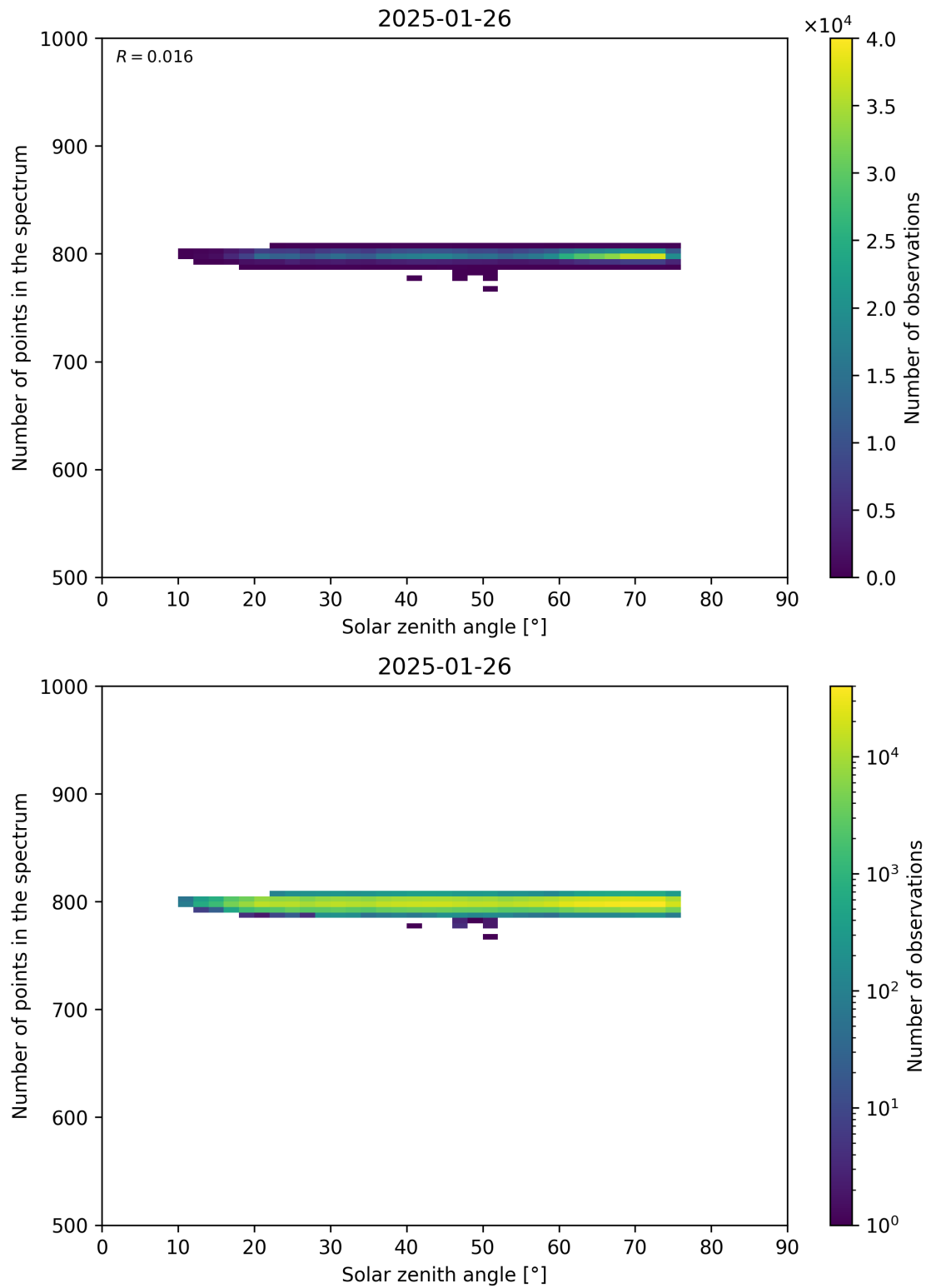
Figure 103: Scatter density plot of “Solar zenith angle” against “Number of points in the spectrum” for 2025-01-25 to 2025-01-27.
