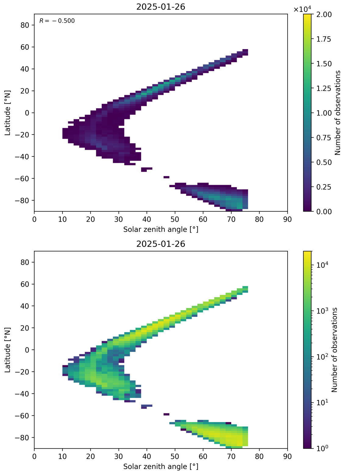
Figure 98: Scatter density plot of “Solar zenith angle” against “Latitude” for 2025-01-25 to 2025-01-27.
