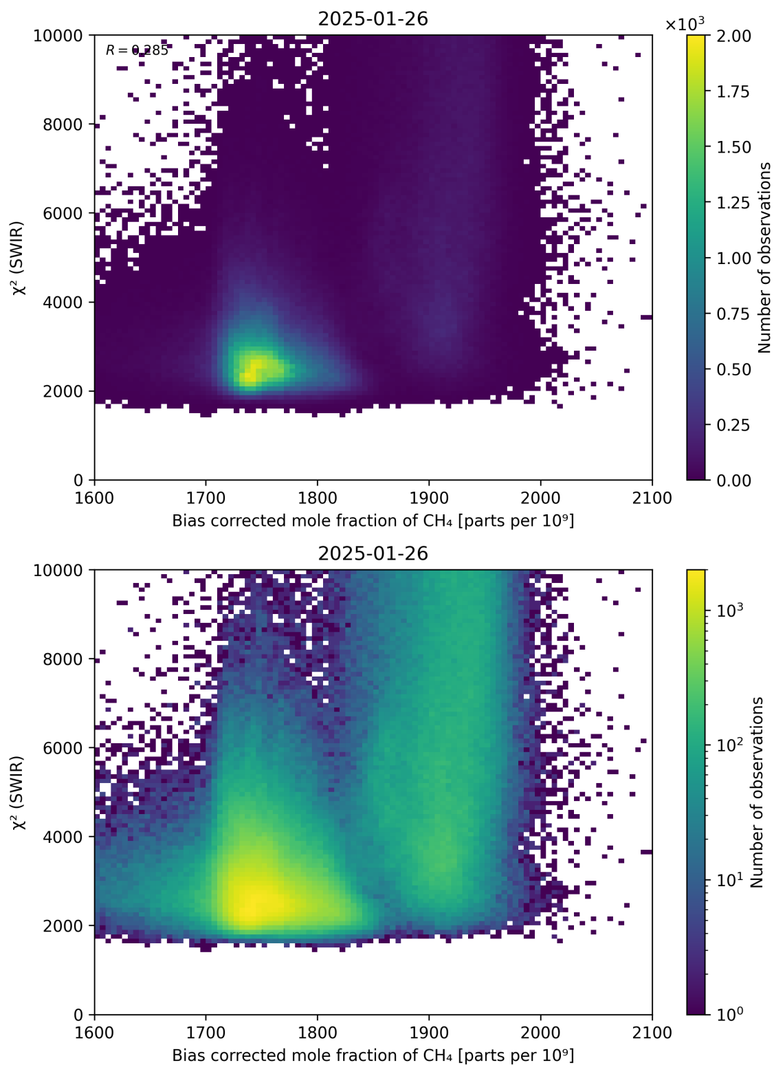
Figure 64: Scatter density plot of “Bias corrected mole fraction of \text{CH}_4 ” against “ \chi^2 (SWIR)” for 2025-01-25 to 2025-01-27.
