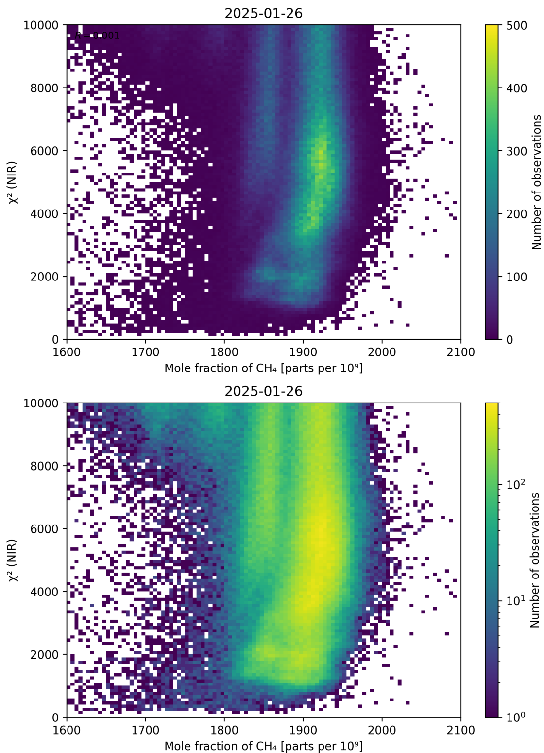
Figure 70: Scatter density plot of “Mole fraction of CH 4 ” against “ \chi^2 (NIR)” for 2025-01-25 to 2025-01-27.
