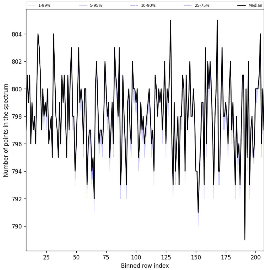
Figure 37: Along track statistics of “Number of points in the spectrum” for 2025-01-25 to 2025-01-27
