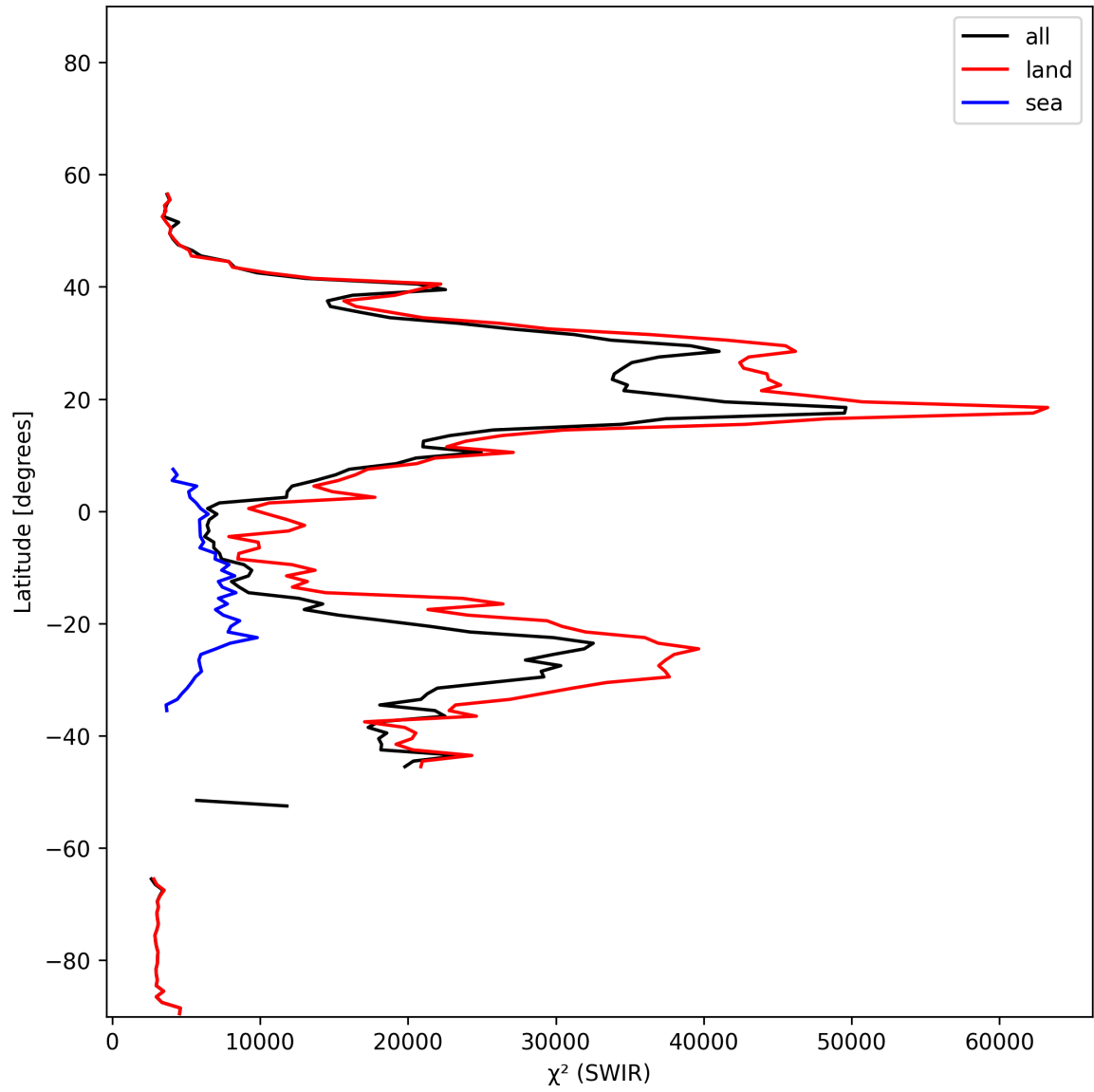
Figure 17: Zonal average of “ \chi^2 (SWIR)” for 2025-01-25 to 2025-01-27.
