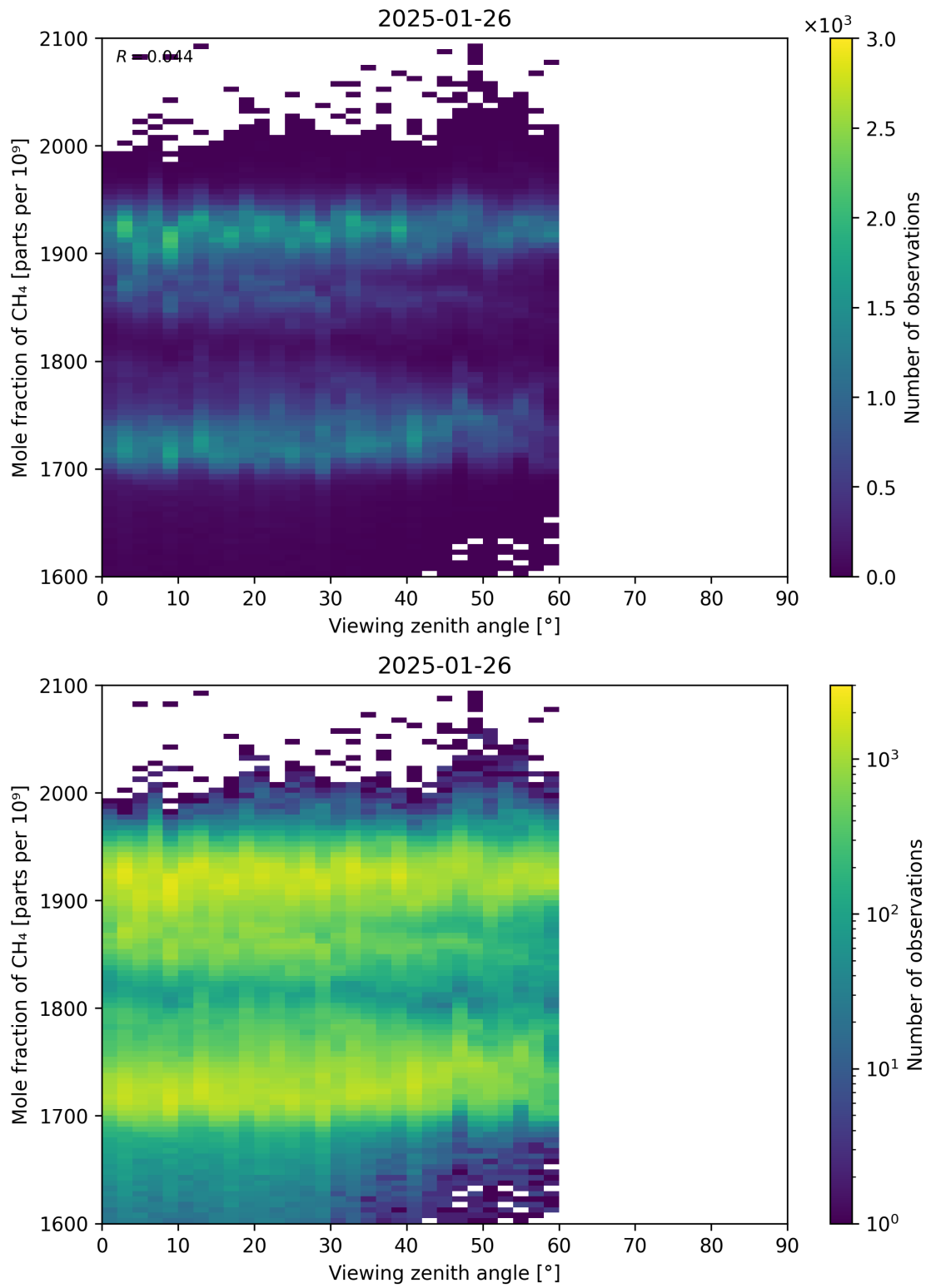
Figure 110: Scatter density plot of “Viewing zenith angle” against “Mole fraction of \text{CH}_4 ” for 2025-01-25 to 2025-01-27.
