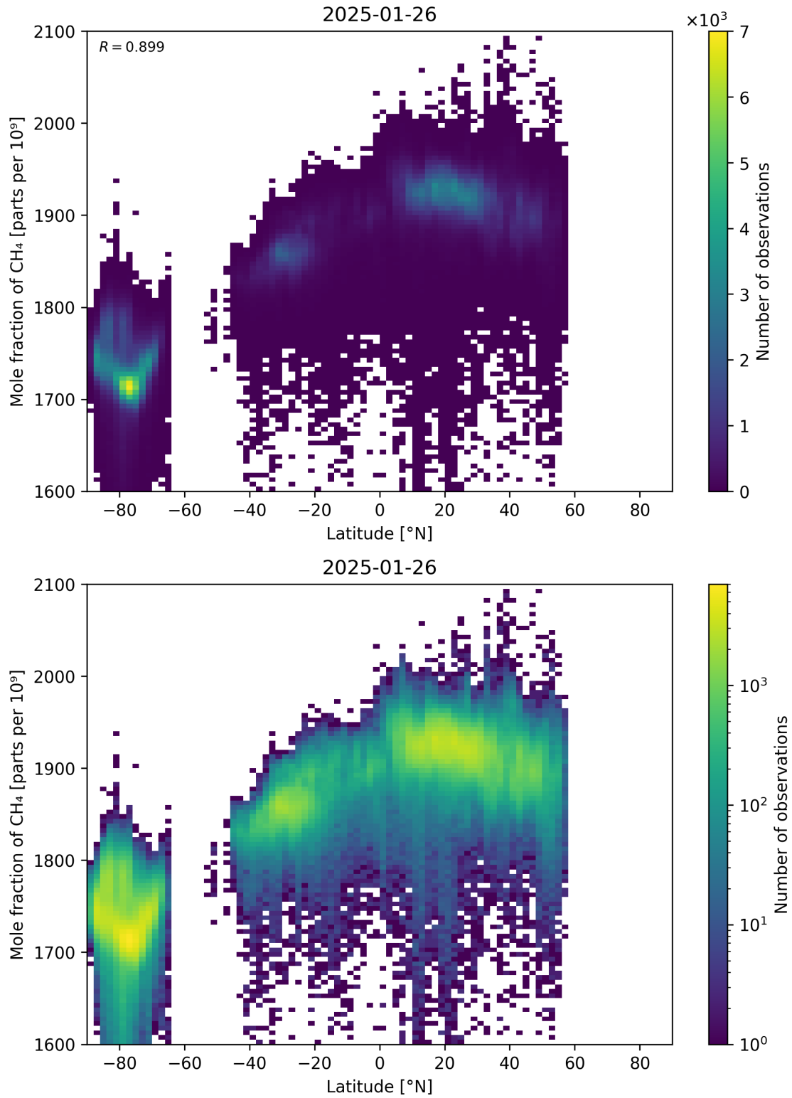
Figure 57: Scatter density plot of “Latitude” against “Mole fraction of CH 4 ” for 2025-01-25 to 2025-01-27.
