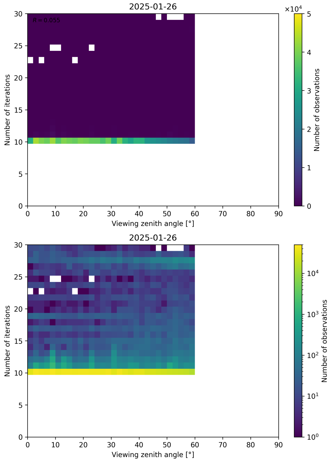
Figure 113: Scatter density plot of “Viewing zenith angle” against “Number of iterations” for 2025-01-25 to 2025-01-27.
