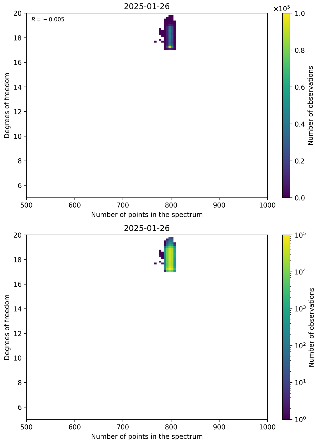
Figure 90: Scatter density plot of “Number of points in the spectrum” against “Degrees of freedom” for 2025-01-25 to 2025-01-27.
