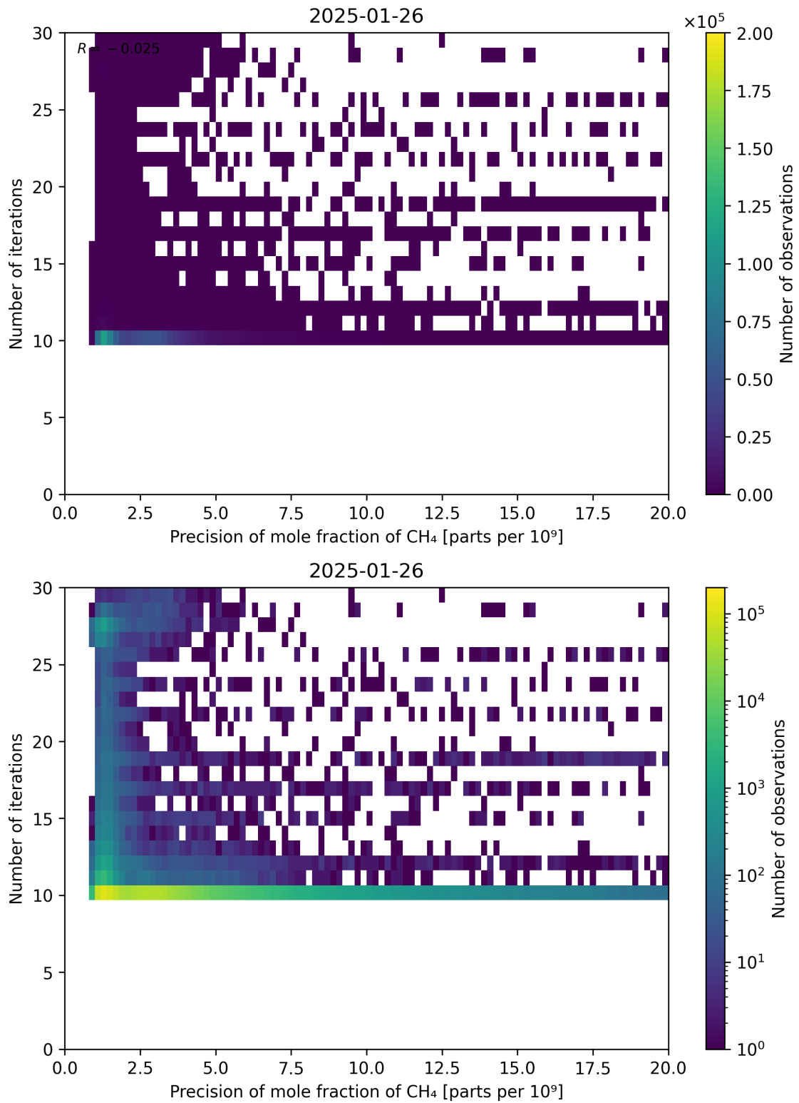
Figure 83: Scatter density plot of “Precision of mole fraction of CH 4 ” against “Number of iterations” for 2025-01-25 to 2025-01-27.
