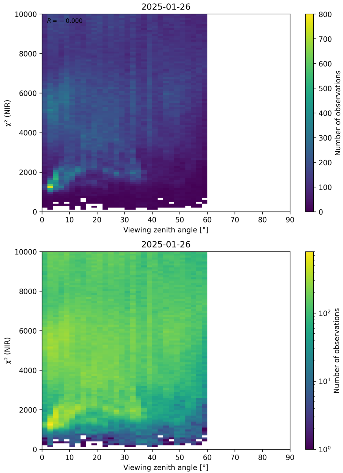
Figure 105: Scatter density plot of “Viewing zenith angle” against “ \chi^2 (NIR)” for 2025-01-25 to 2025-01-27.
