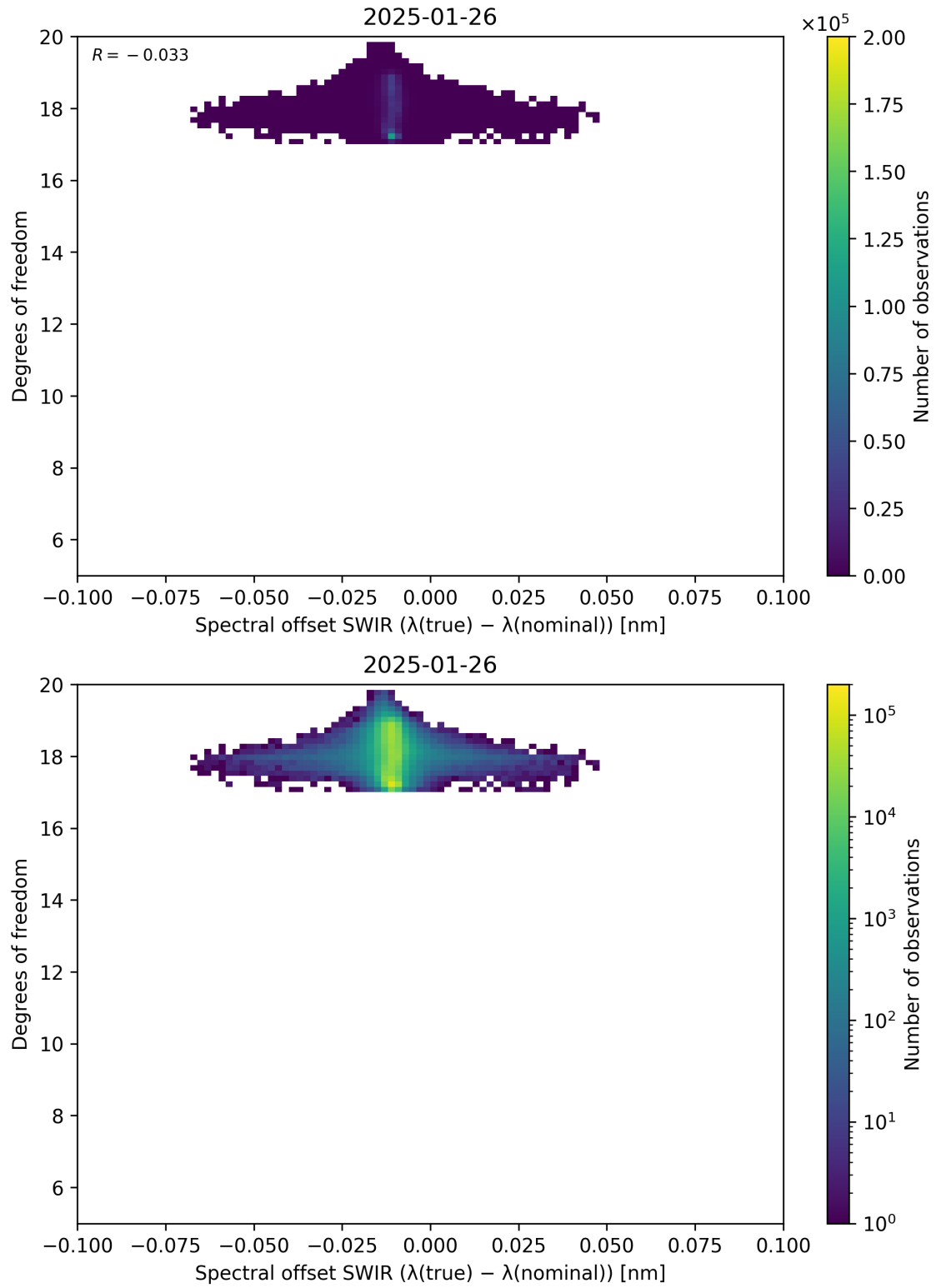
Figure 119: Scatter density plot of “Spectral offset SWIR ( \lambda_{\text{true}} - \lambda_{\text{nominal}} )” against “Degrees of freedom” for 2025-01-25 to 2025-01-27.
