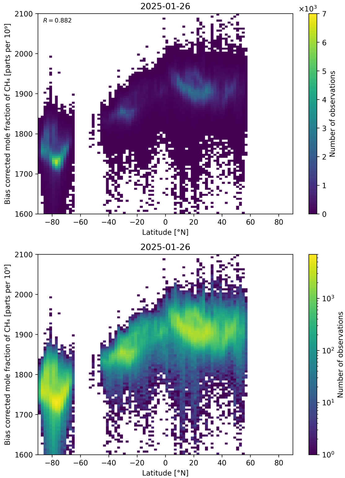
Figure 58: Scatter density plot of “Latitude” against “Bias corrected mole fraction of CH 4 ” for 2025-01-25 to 2025-01-27.
