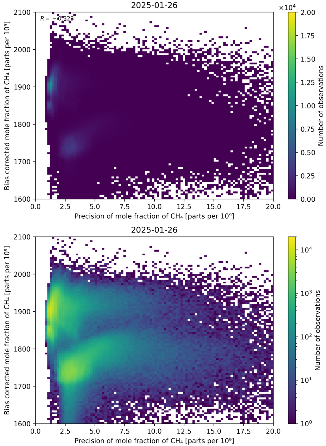
Figure 82: Scatter density plot of “Precision of mole fraction of \text{CH}_4 ” against “Bias corrected mole fraction of \text{CH}_4 ” for 2025-01-25 to 2025-01-27.
