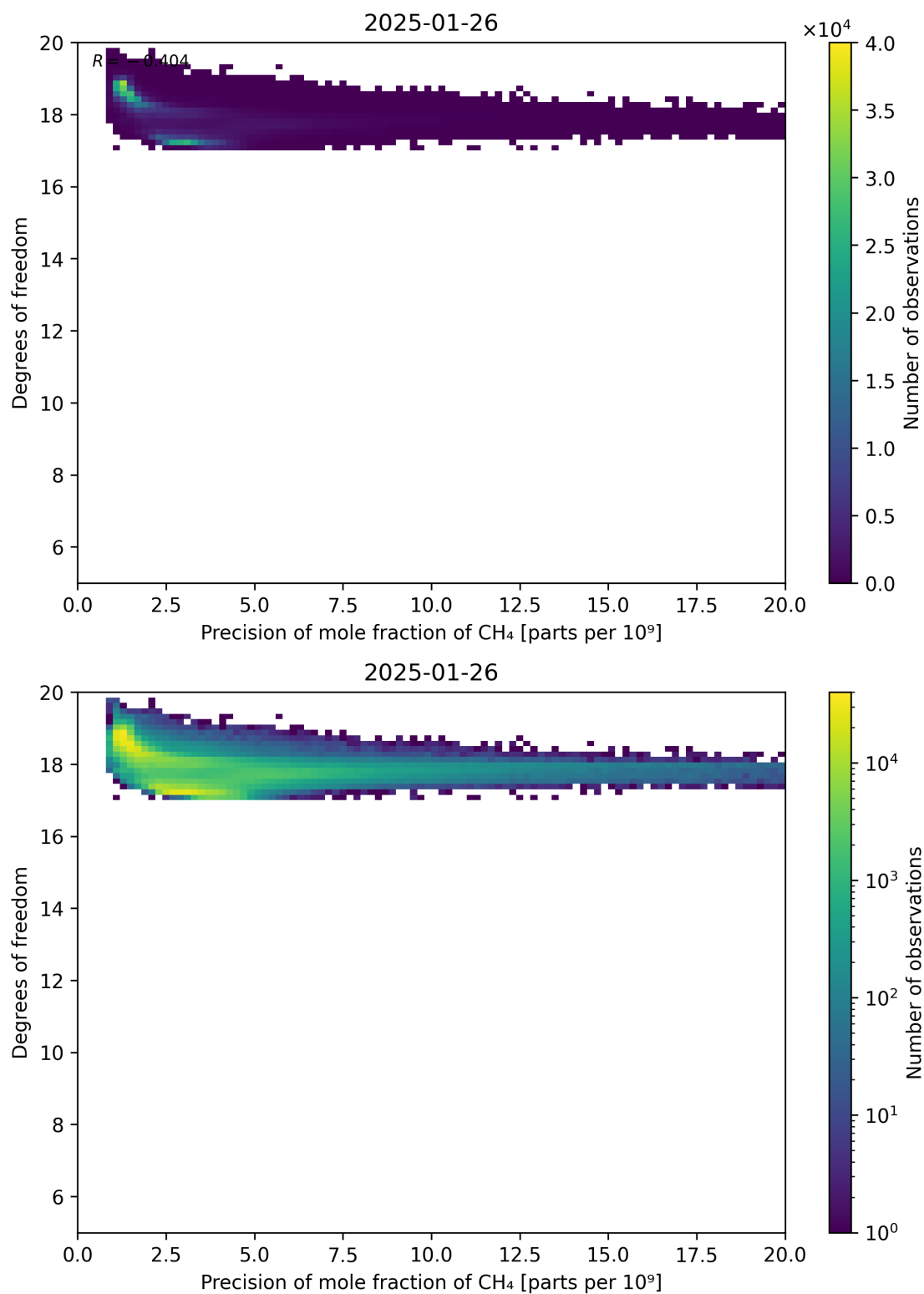
Figure 80: Scatter density plot of “Precision of mole fraction of CH 4 ” against “Degrees of freedom” for 2025-01-25 to 2025-01-27.
