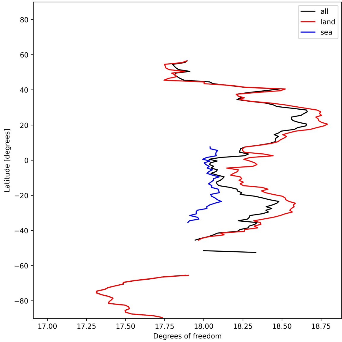
Figure 19: Zonal average of “Degrees of freedom” for 2025-01-25 to 2025-01-27.
