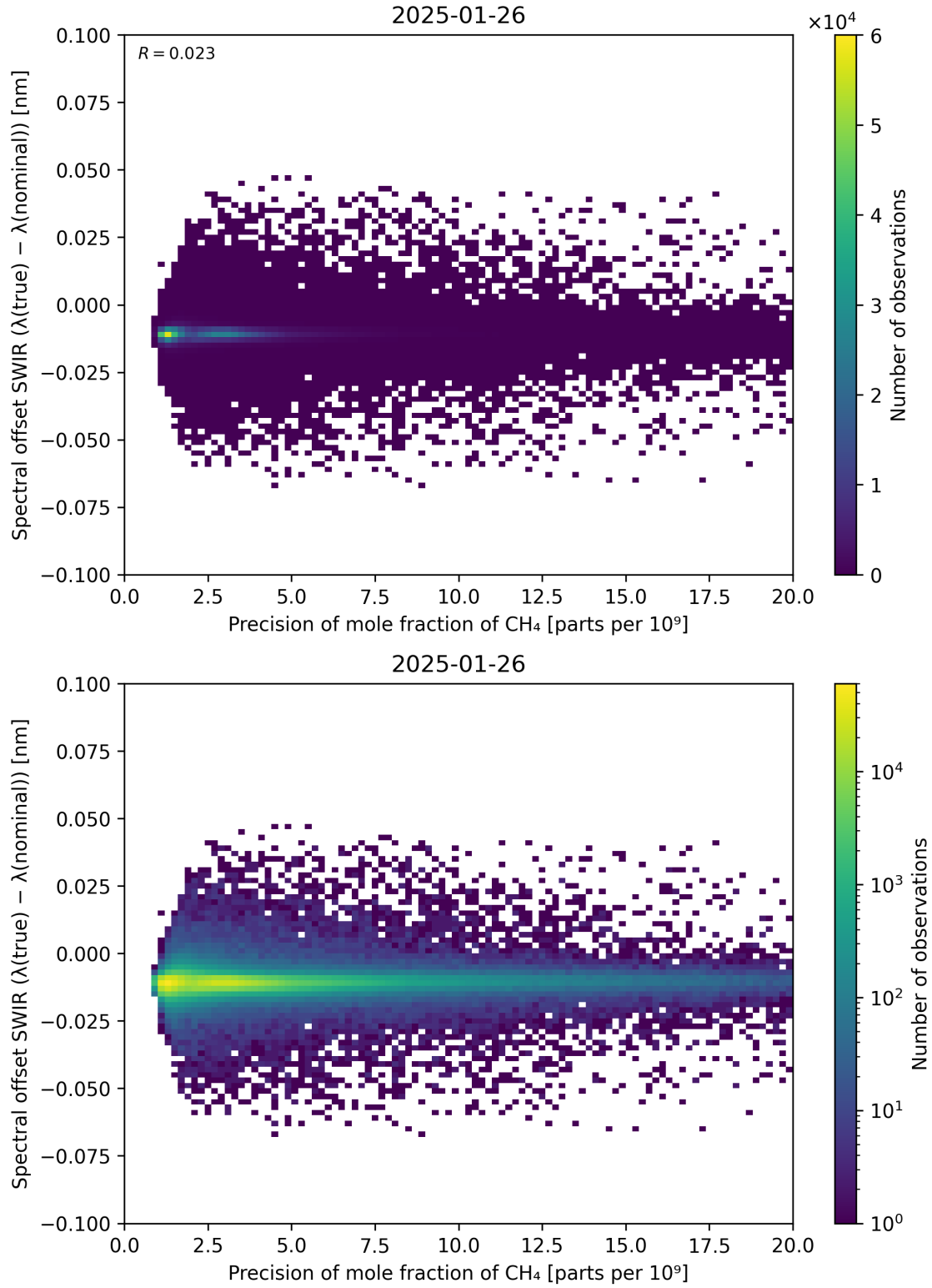
Figure 85: Scatter density plot of “Precision of mole fraction of \text{CH}_4 ” against “Spectral offset SWIR ( \lambda_{\text{true}} - \lambda_{\text{nominal}} )” for 2025-01-25 to 2025-01-27.
