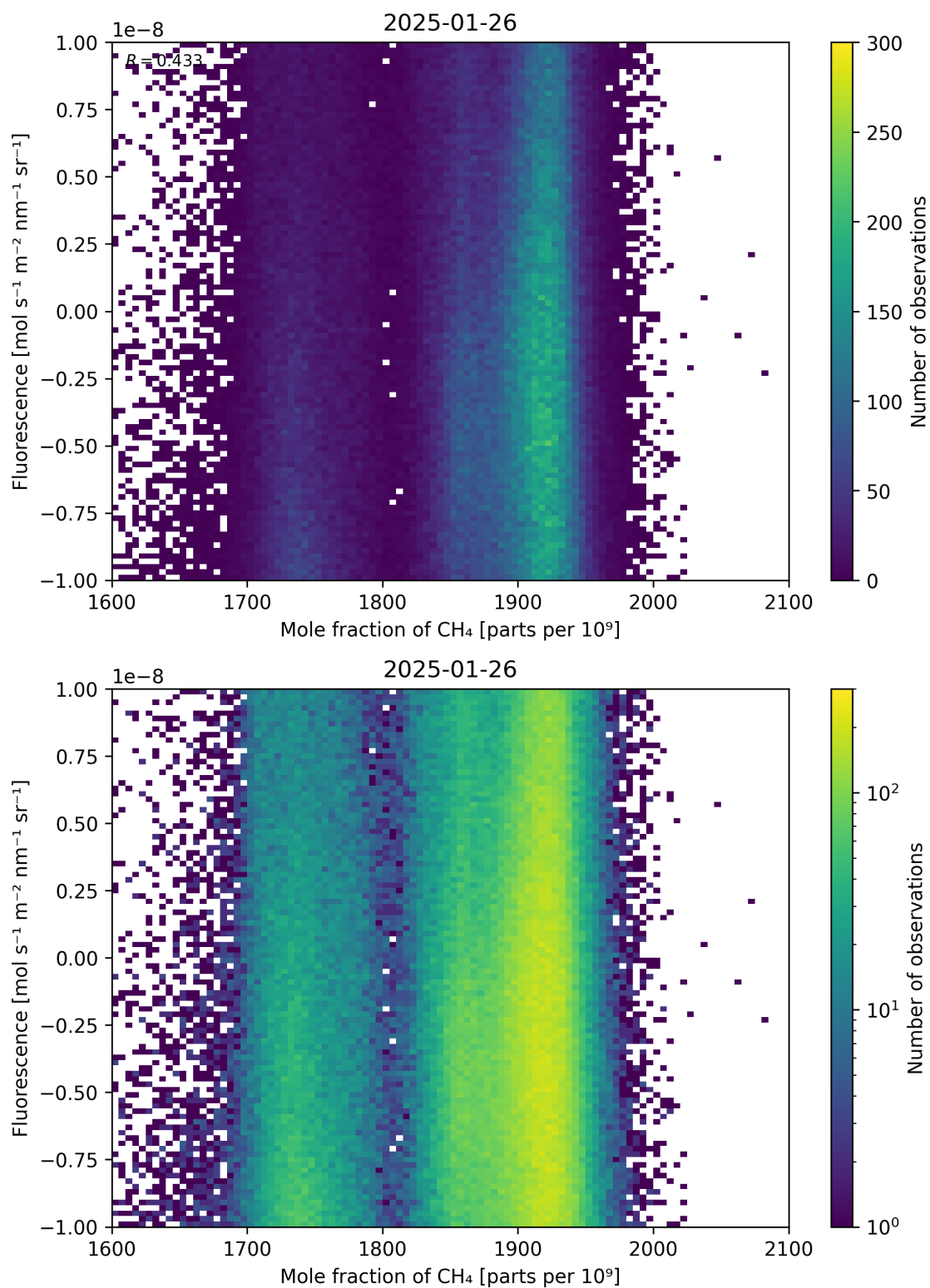
Figure 73: Scatter density plot of “Mole fraction of \text{CH}_4 ” against “Fluorescence” for 2025-01-25 to 2025-01-27.
