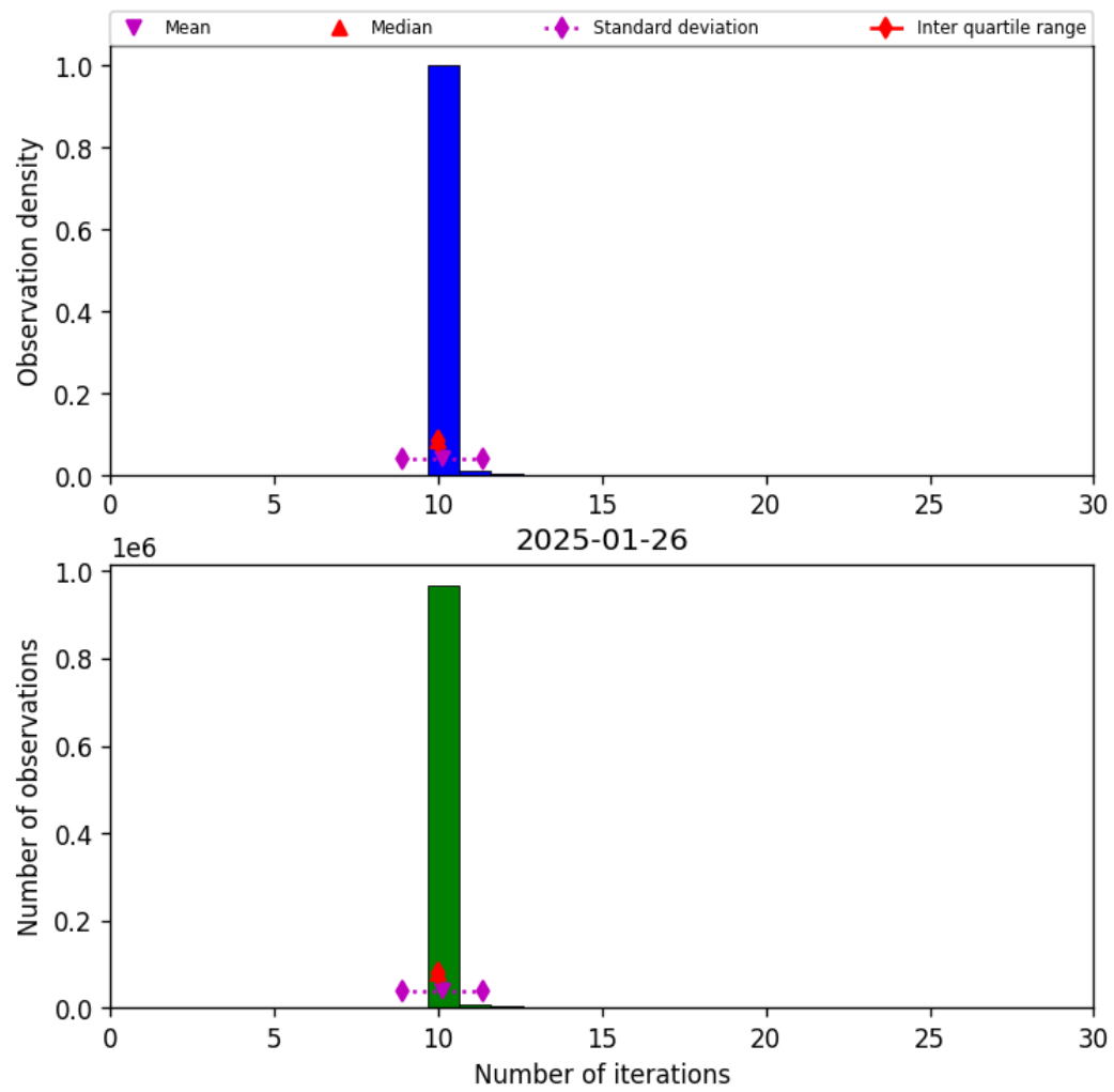
Figure 31: Histogram of “Number of iterations” for 2025-01-25 to 2025-01-27
