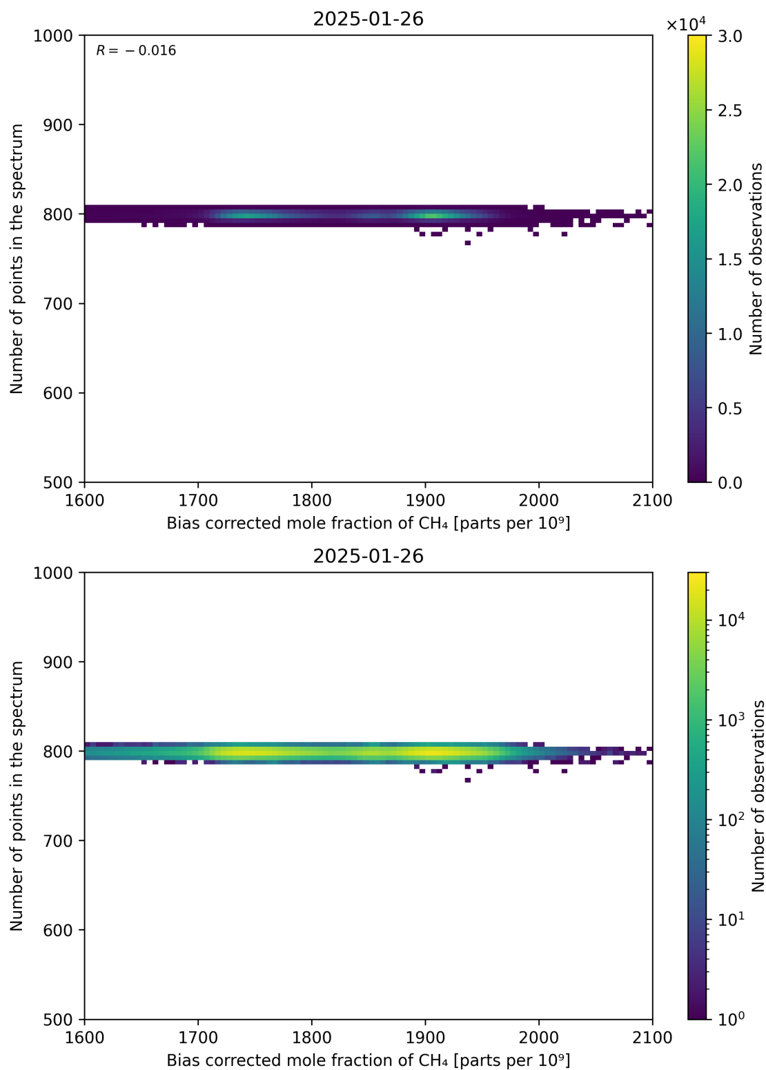
Figure 68: Scatter density plot of “Bias corrected mole fraction of CH 4 ” against “Number of points in the spectrum” for 2025-01-25 to 2025-01-27.
