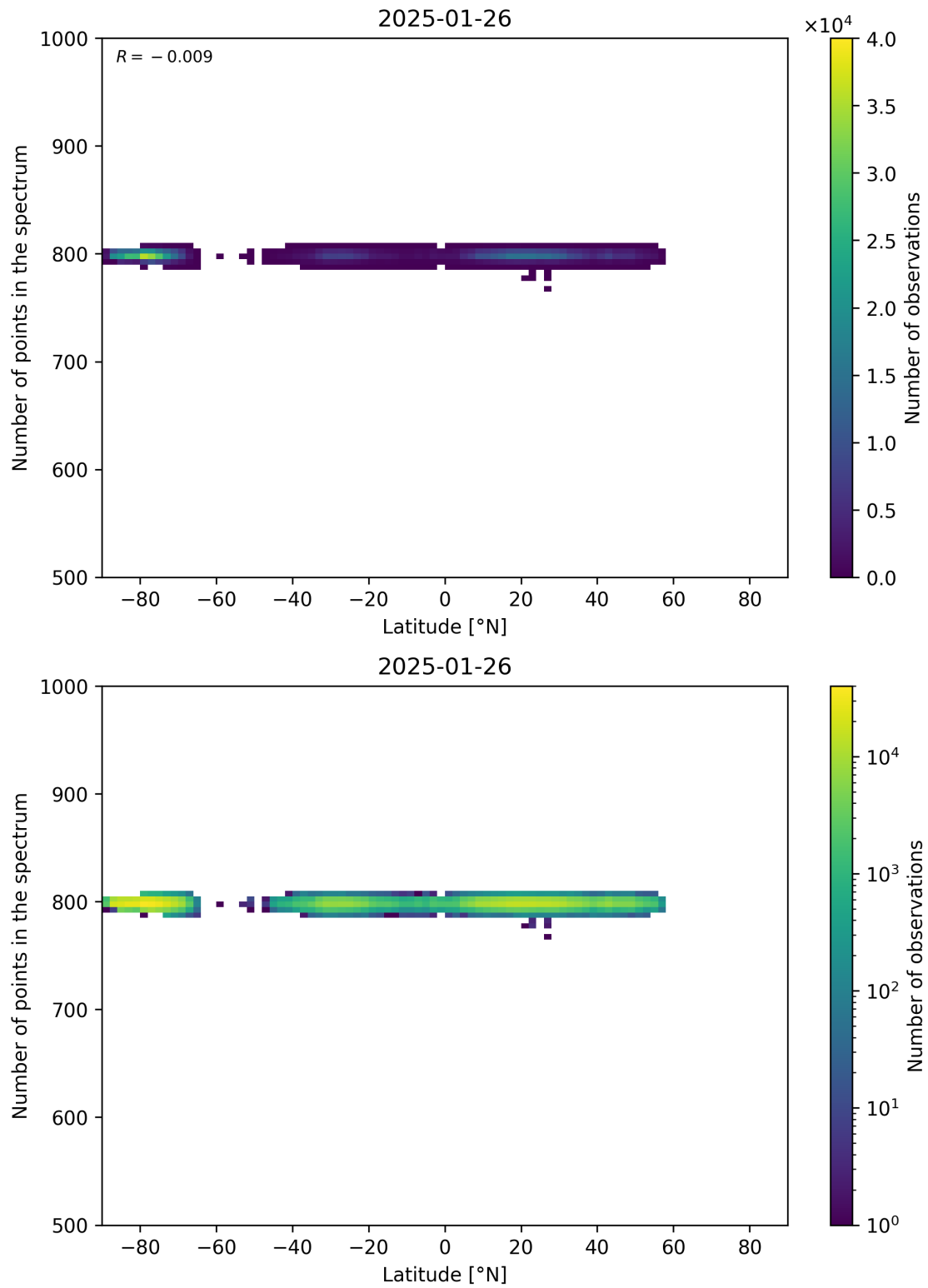
Figure 61: Scatter density plot of “Latitude” against “Number of points in the spectrum” for 2025-01-25 to 2025-01-27.
