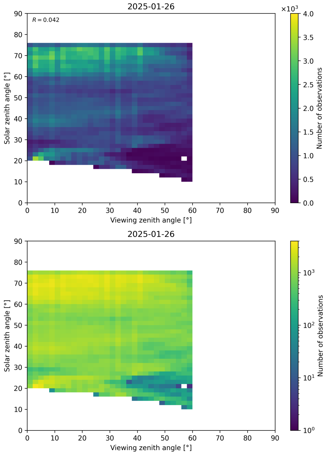
Figure 115: Scatter density plot of “Viewing zenith angle” against “Solar zenith angle” for 2025-01-25 to 2025-01-27.
