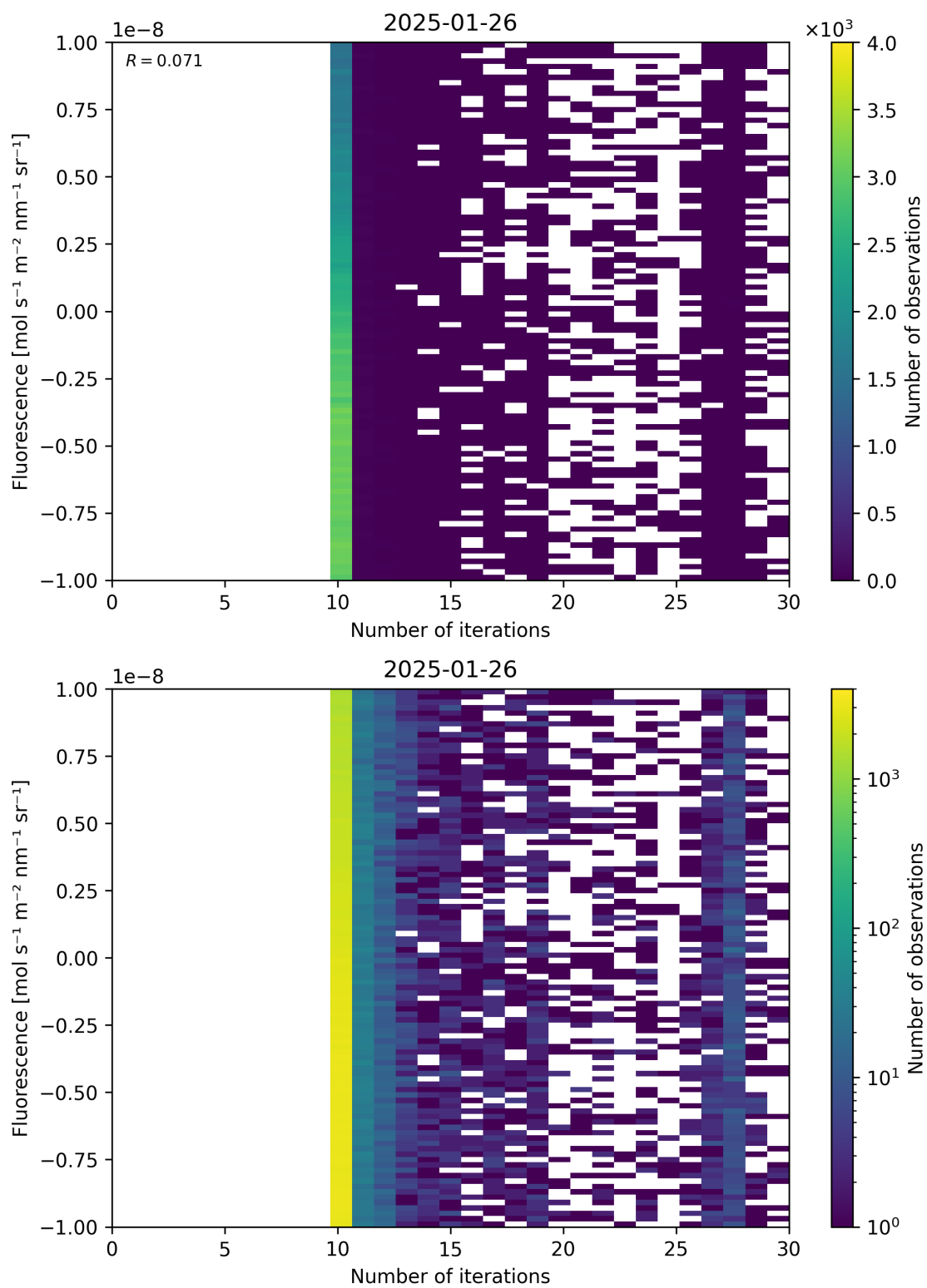
Figure 87: Scatter density plot of “Number of iterations” against “Fluorescence” for 2025-01-25 to 2025-01-27.
