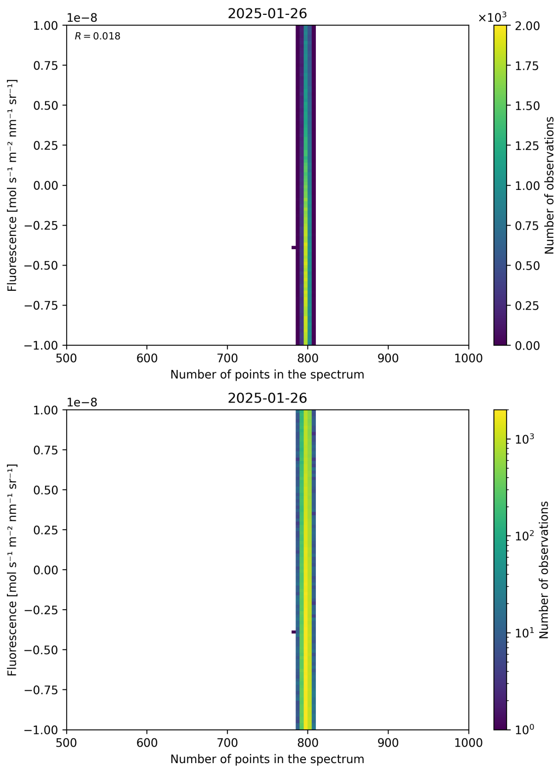
Figure 91: Scatter density plot of “Number of points in the spectrum” against “Fluorescence” for 2025-01-25 to 2025-01-27.
