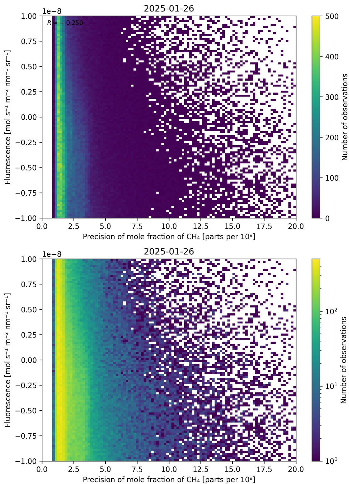
Figure 81: Scatter density plot of “Precision of mole fraction of CH 4 ” against “Fluorescence” for 2025-01-25 to 2025-01-27.
