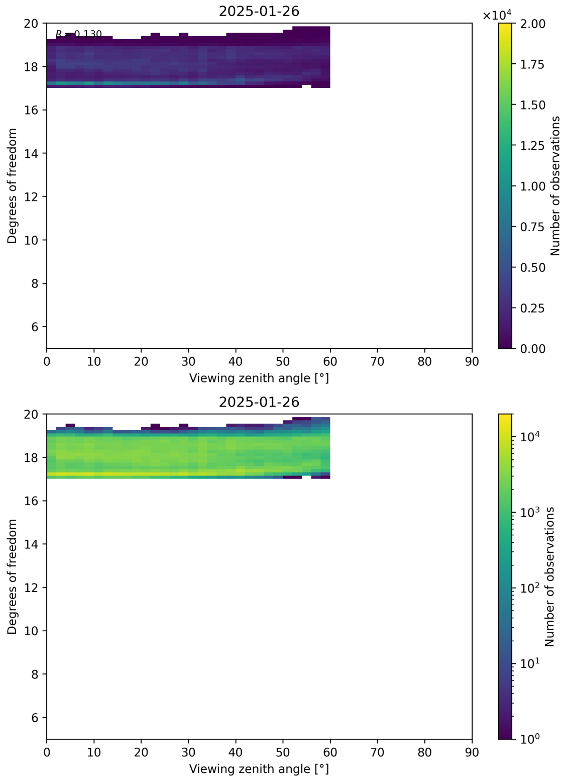
Figure 107: Scatter density plot of “Viewing zenith angle” against “Degrees of freedom” for 2025-01-25 to 2025-01-27.
