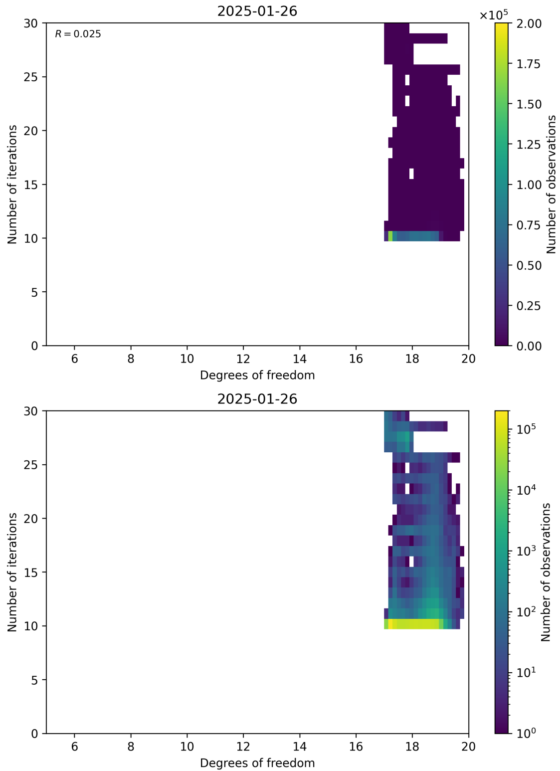
Figure 52: Scatter density plot of “Degrees of freedom” against “Number of iterations” for 2025-01-25 to 2025-01-27.
