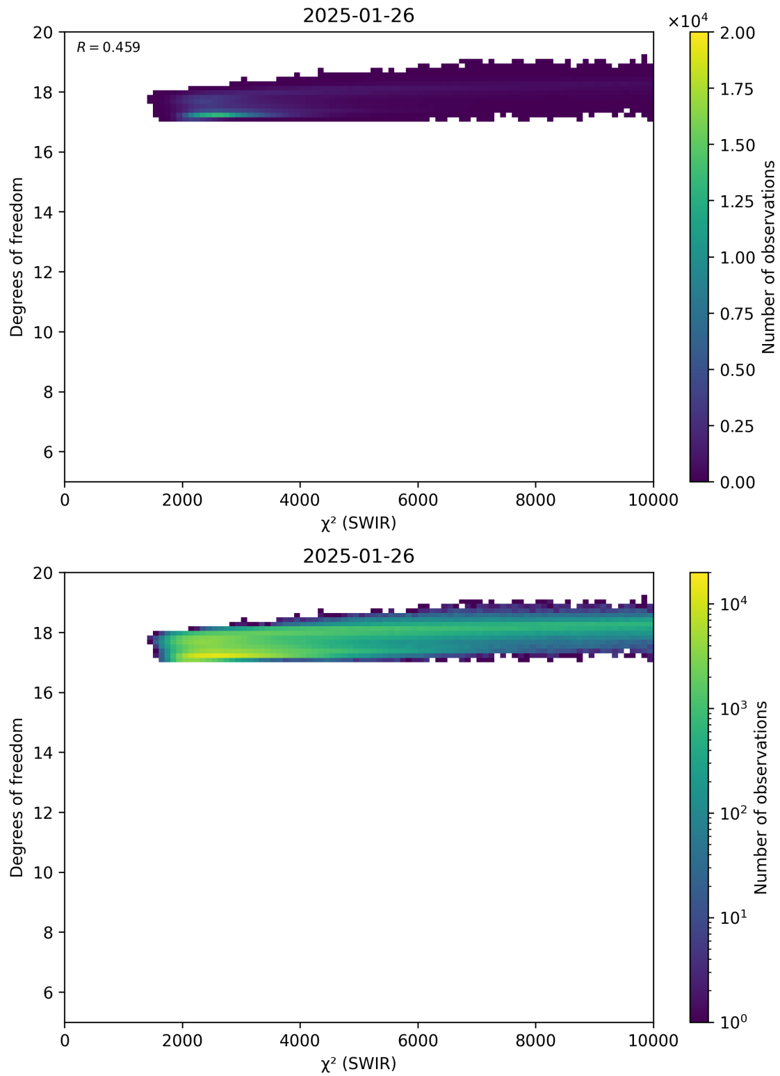
Figure 48: Scatter density plot of “ \chi^2 (SWIR)” against “Degrees of freedom” for 2025-01-25 to 2025-01-27.
