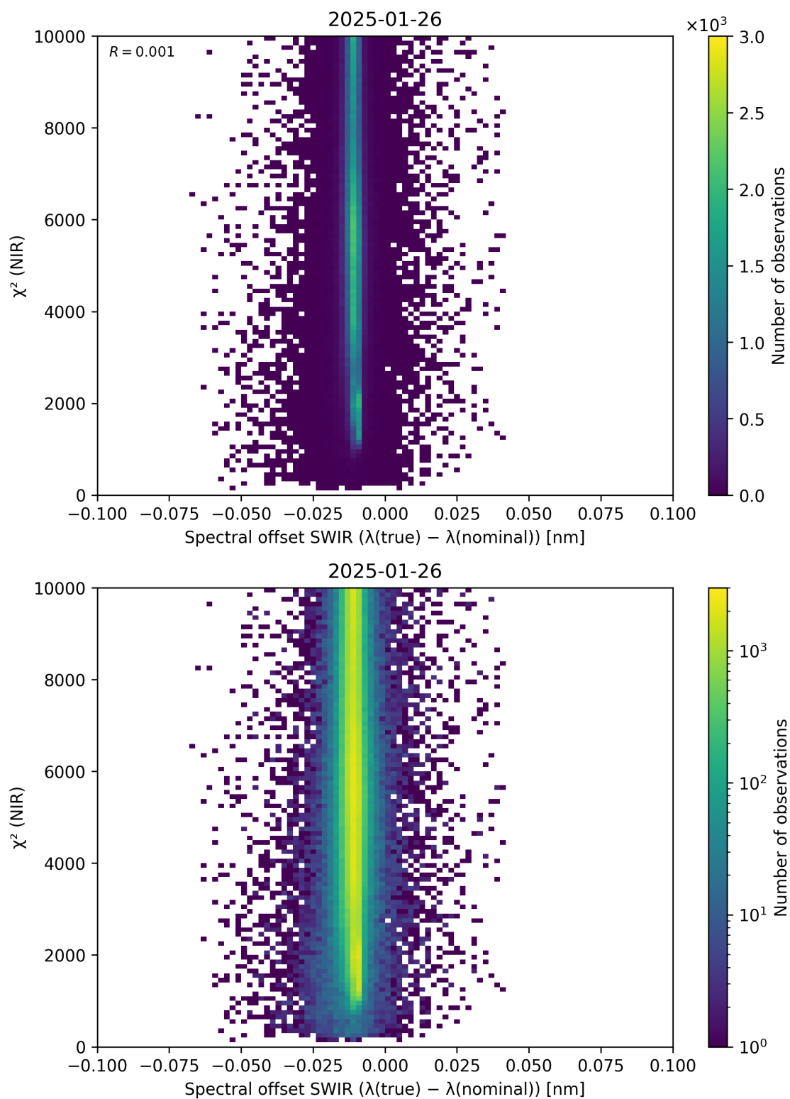
Figure 117: Scatter density plot of “Spectral offset SWIR ( \lambda_{\text{true}} - \lambda_{\text{nominal}} )” against “ \chi^2 (NIR)” for 2025-01-25 to 2025-01-27.
