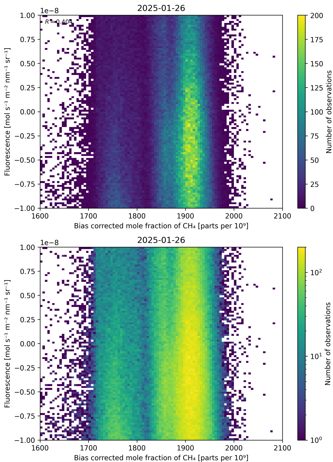
Figure 66: Scatter density plot of “Bias corrected mole fraction of \text{CH}_4 ” against “Fluorescence” for 2025-01-25 to 2025-01-27.
