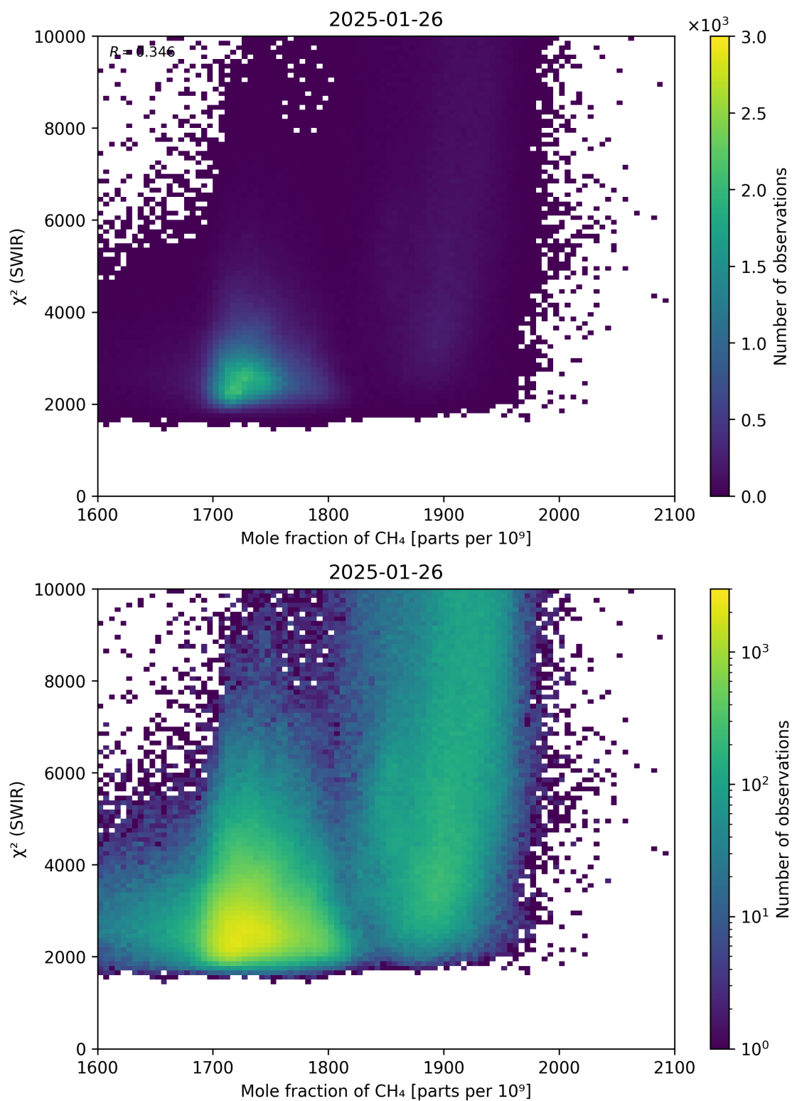
Figure 71: Scatter density plot of “Mole fraction of \text{CH}_4 ” against “ \chi^2 (SWIR)” for 2025-01-25 to 2025-01-27.
