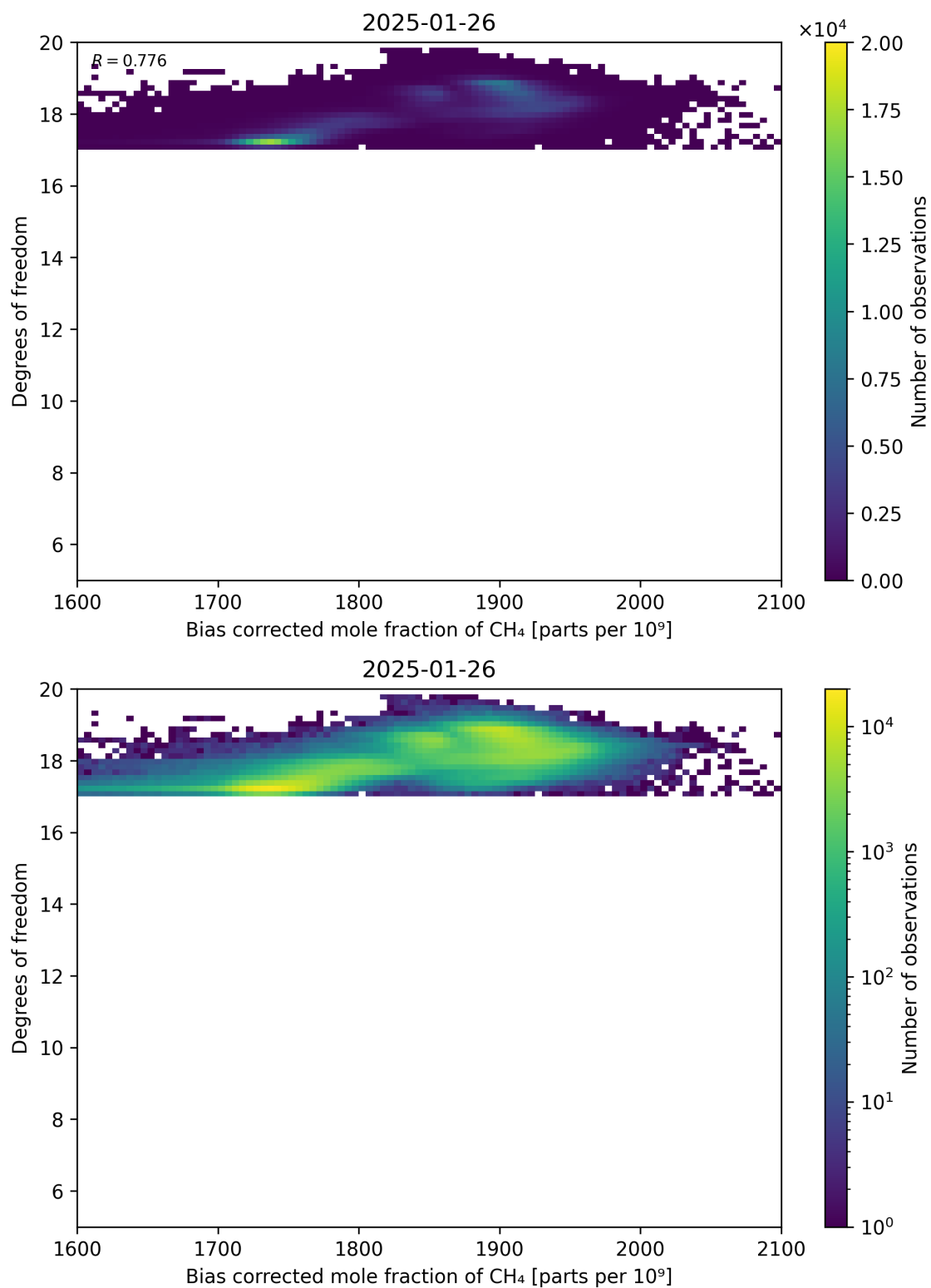
Figure 65: Scatter density plot of “Bias corrected mole fraction of CH 4 ” against “Degrees of freedom” for 2025-01-25 to 2025-01-27.
