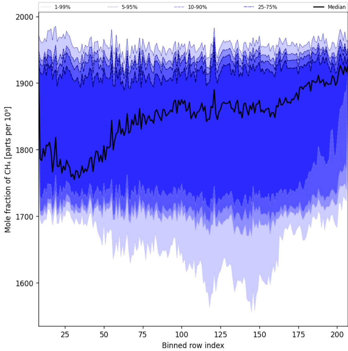
Figure 34: Along track statistics of “Mole fraction of CH 4 ” for 2025-01-25 to 2025-01-27
