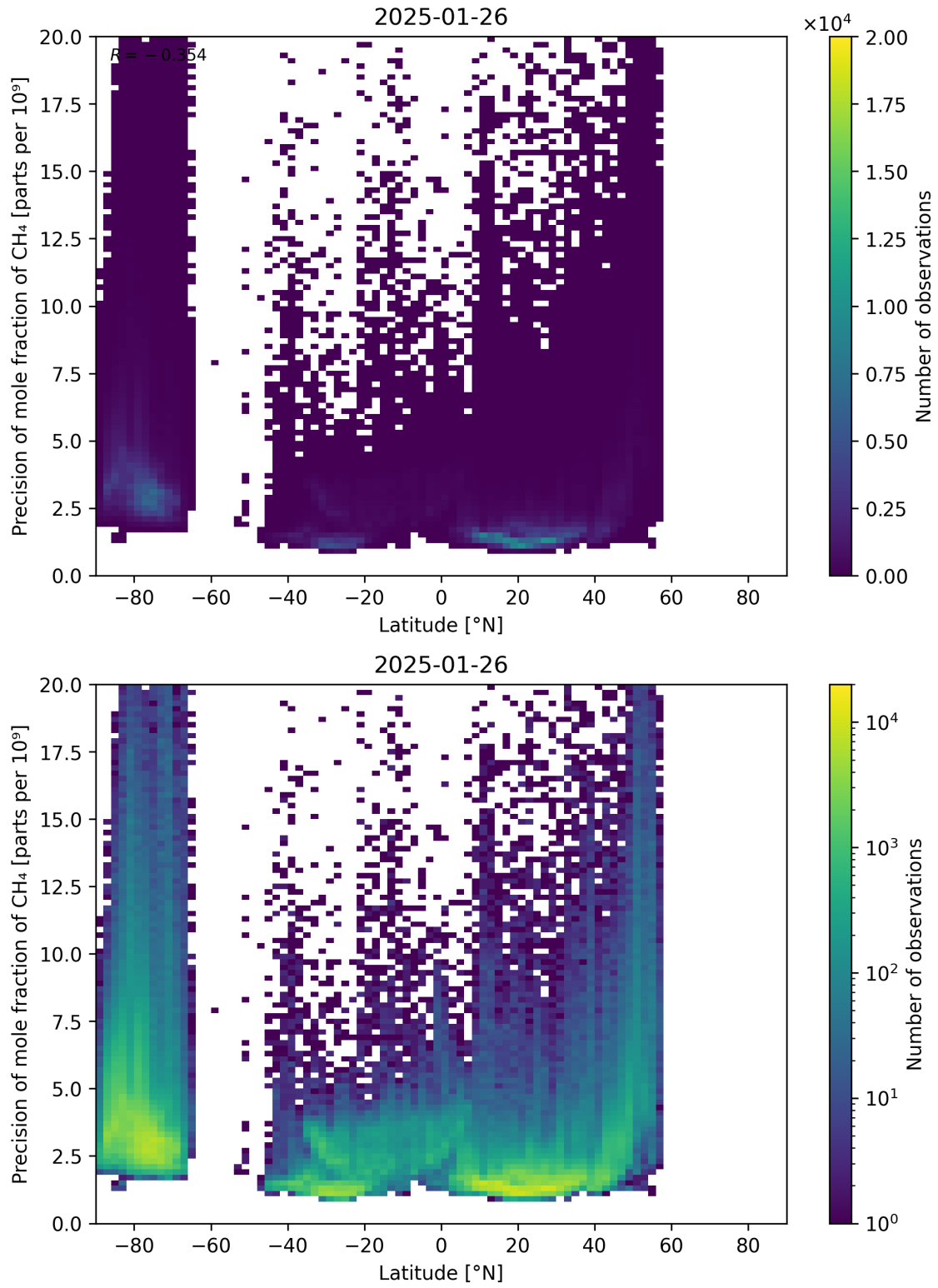
Figure 59: Scatter density plot of “Latitude” against “Precision of mole fraction of CH 4 ” for 2025-01-25 to 2025-01-27.
