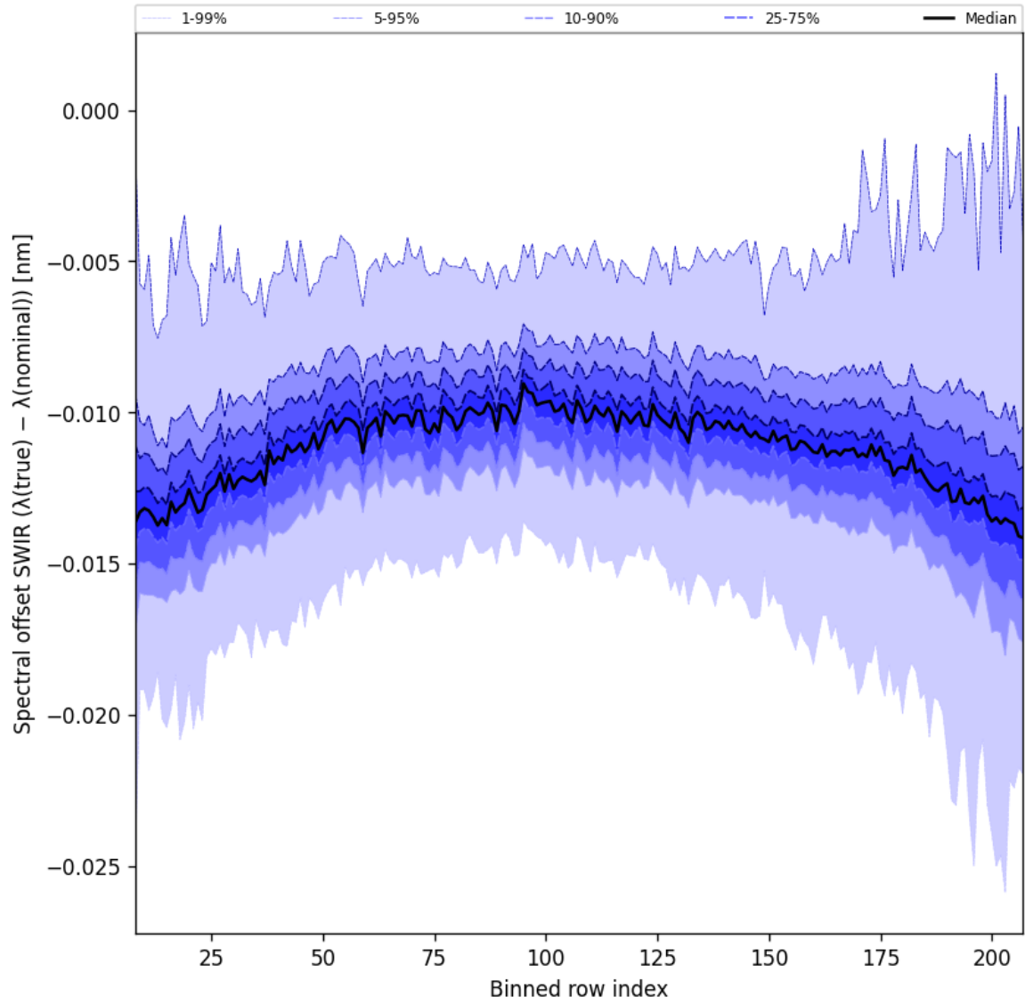
Figure 38: Along track statistics of “Spectral offset SWIR ( \lambda_{\text{true}} - \lambda_{\text{nominal}} )” for 2025-01-25 to 2025-01-27
