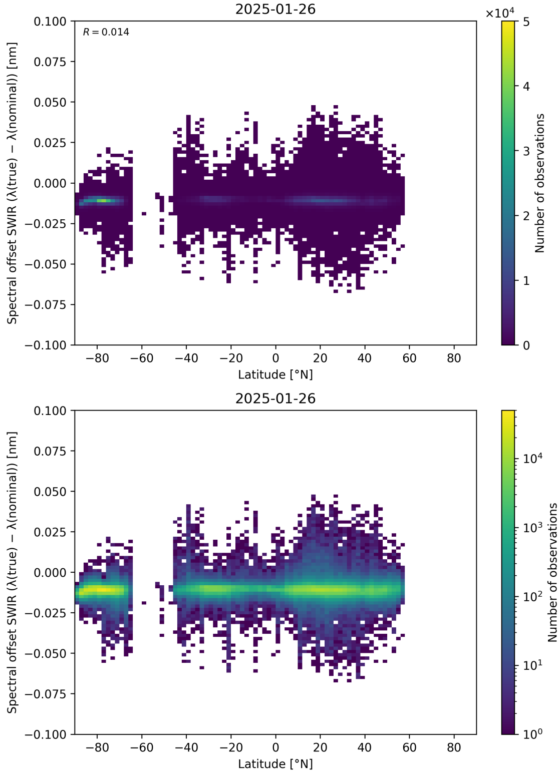
Figure 62: Scatter density plot of “Latitude” against “Spectral offset SWIR ( \lambda_{\text{true}} - \lambda_{\text{nominal}} )” for 2025-01-25 to 2025-01-27.
