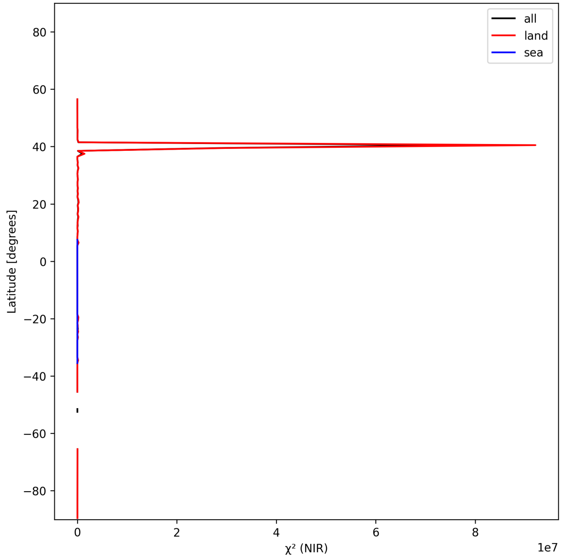
Figure 18: Zonal average of “ \chi^2 (NIR)” for 2025-01-25 to 2025-01-27.
