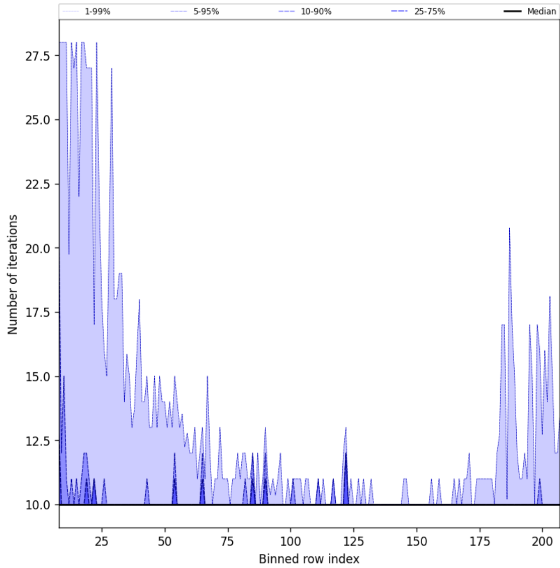
Figure 42: Along track statistics of “Number of iterations” for 2025-01-25 to 2025-01-27
