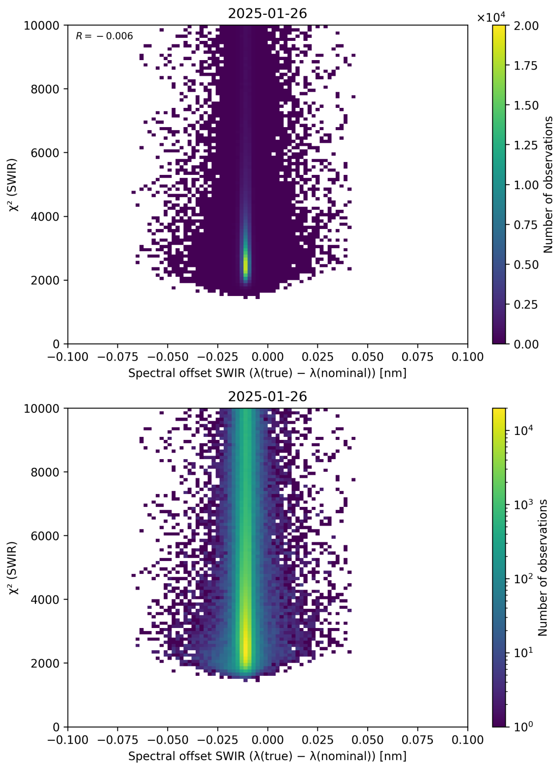
Figure 118: Scatter density plot of “Spectral offset SWIR ( \lambda_{\text{true}} - \lambda_{\text{nominal}} )” against “ \chi^2 (SWIR)” for 2025-01-25 to 2025-01-27.
