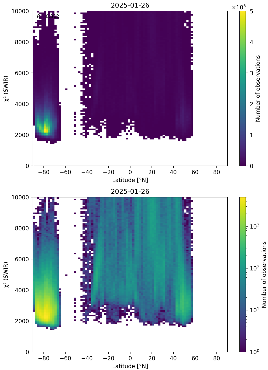
Figure 54: Scatter density plot of “Latitude” against “ \chi^2 (SWIR)” for 2025-01-25 to 2025-01-27.
