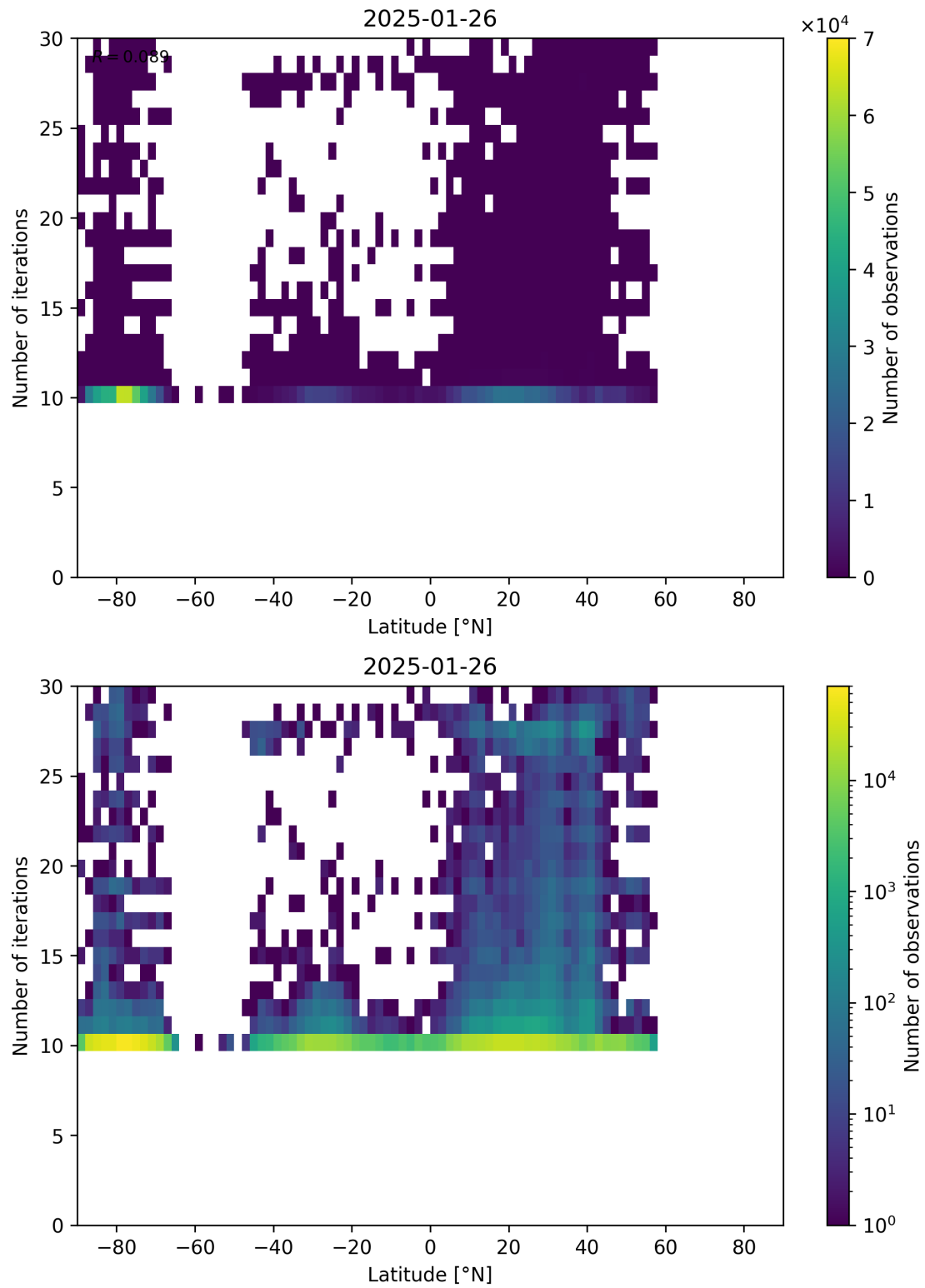
Figure 60: Scatter density plot of “Latitude” against “Number of iterations” for 2025-01-25 to 2025-01-27.
