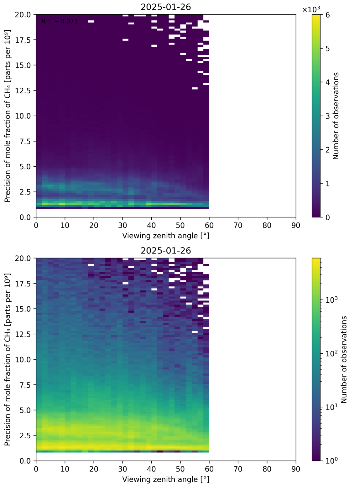
Figure 112: Scatter density plot of “Viewing zenith angle” against “Precision of mole fraction of \text{CH}_4 ” for 2025-01-25 to 2025-01-27.
