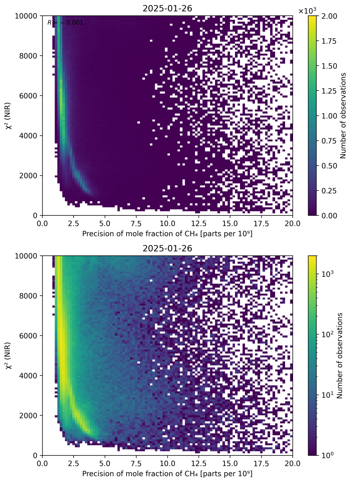
Figure 78: Scatter density plot of “Precision of mole fraction of CH 4 ” against “ \chi^2 (NIR)” for 2025-01-25 to 2025-01-27.
