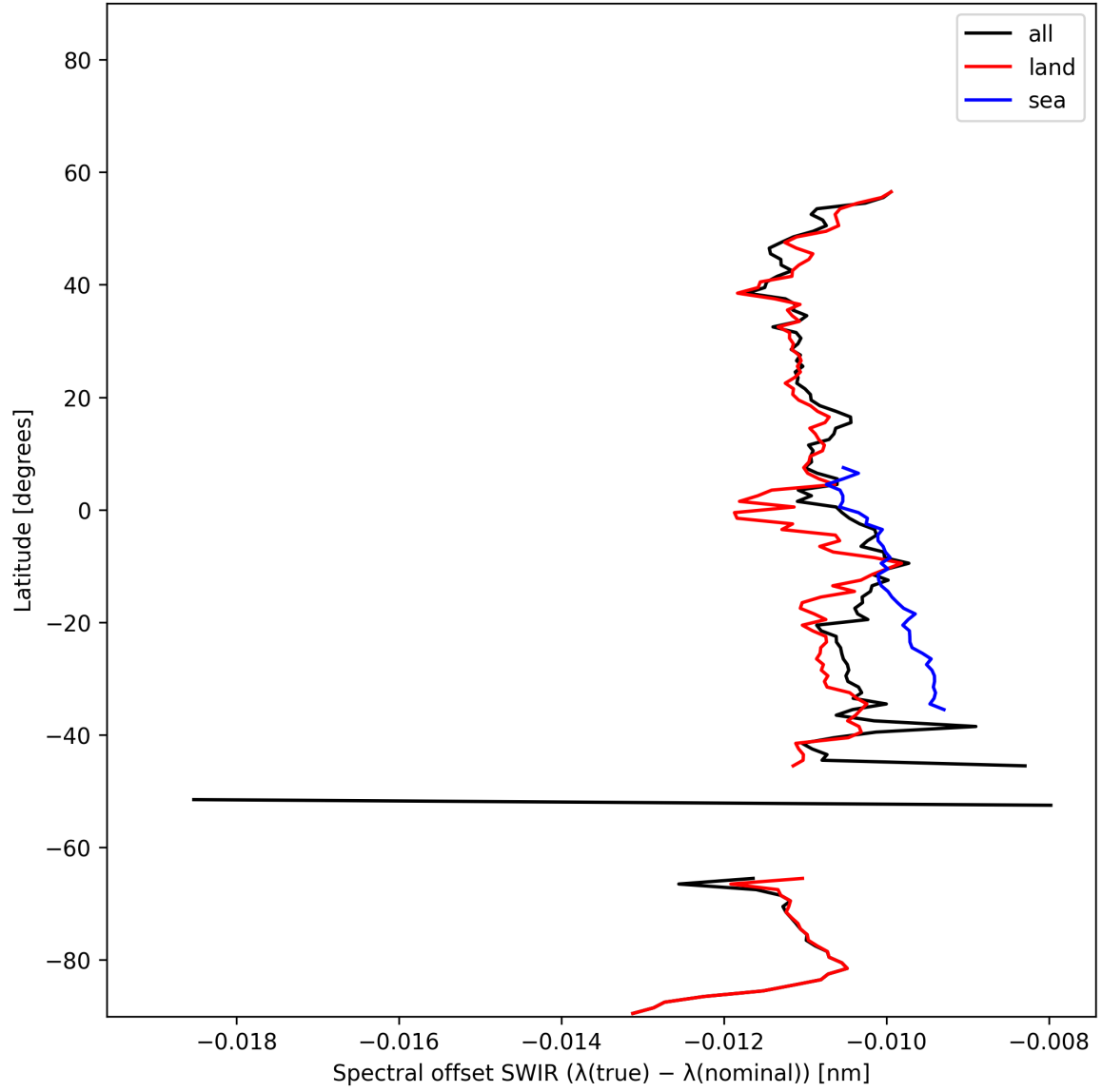
Figure 16: Zonal average of “Spectral offset SWIR ( \lambda_{\text{true}} - \lambda_{\text{nominal}} )” for 2025-01-25 to 2025-01-27.
