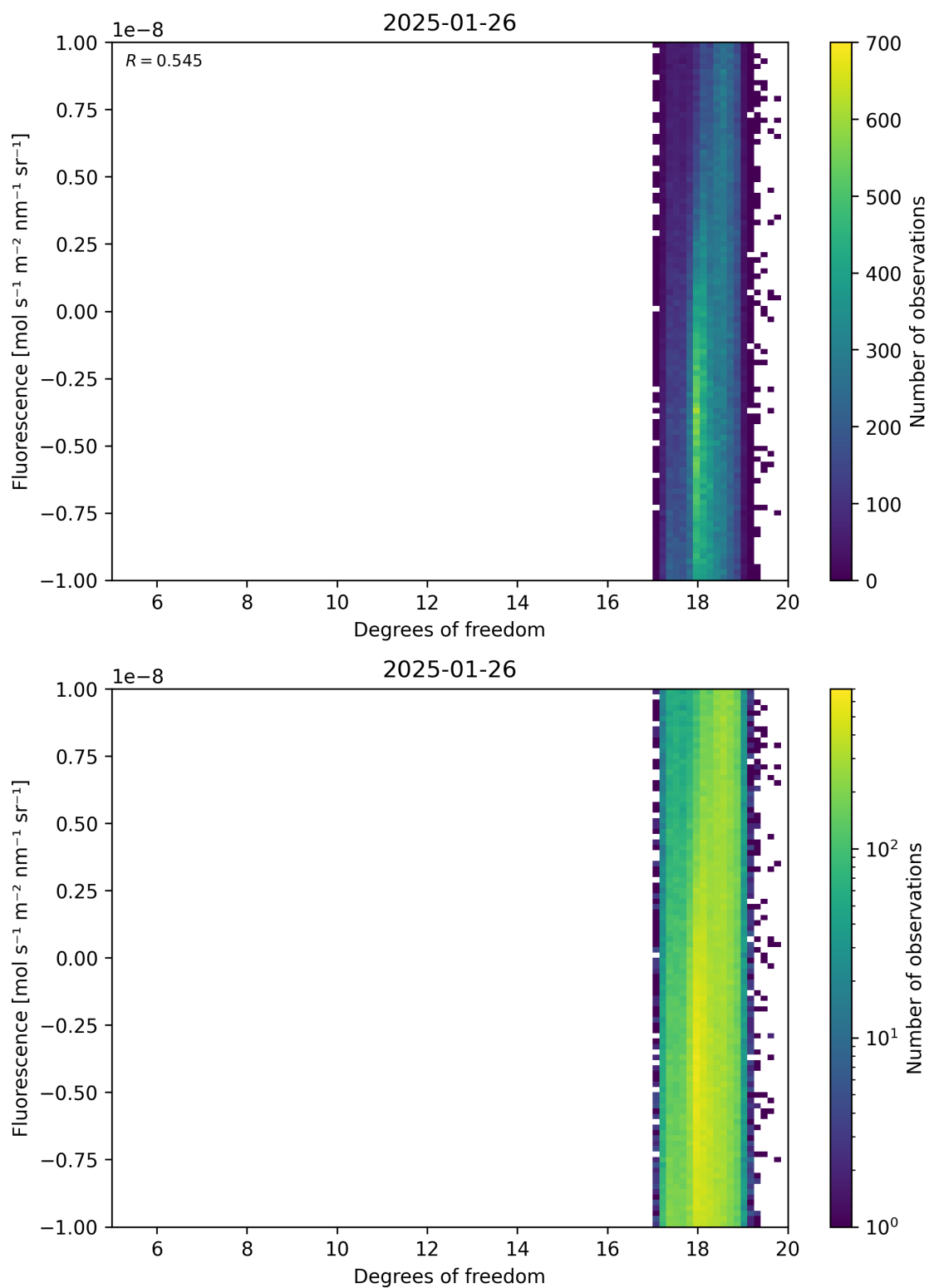
Figure 51: Scatter density plot of “Degrees of freedom” against “Fluorescence” for 2025-01-25 to 2025-01-27.
