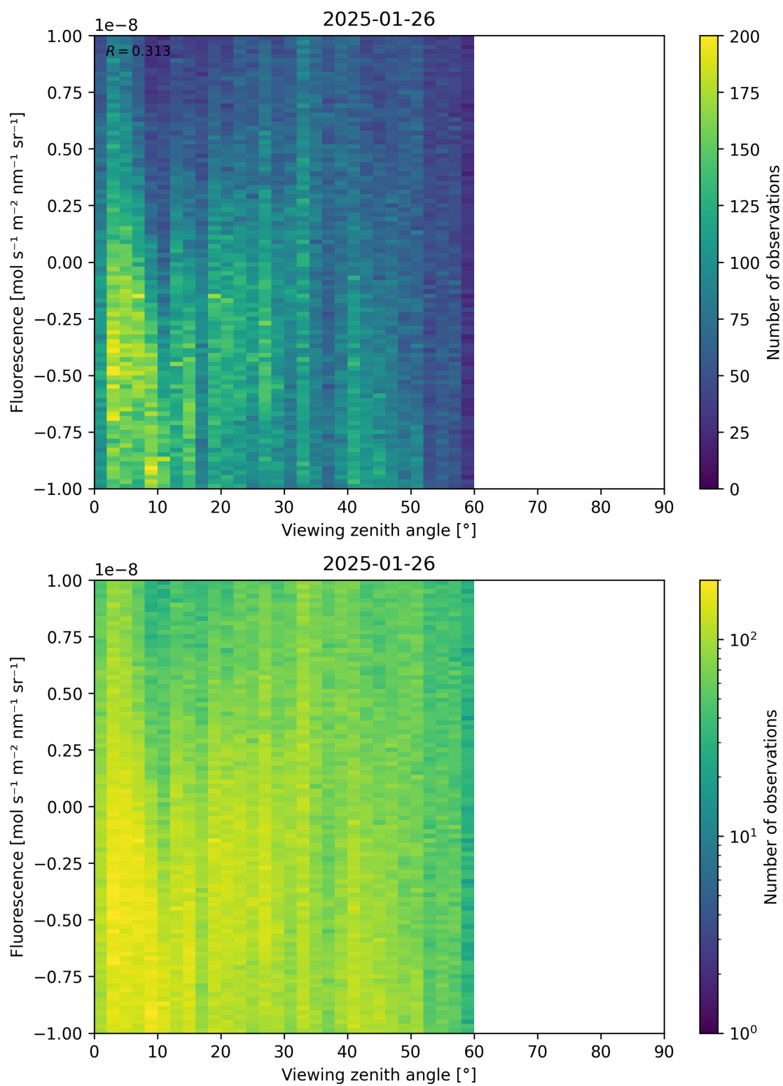
Figure 108: Scatter density plot of “Viewing zenith angle” against “Fluorescence” for 2025-01-25 to 2025-01-27.
