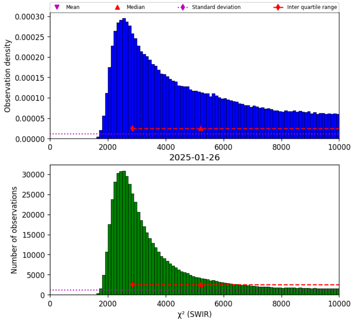
Figure 28: Histogram of “ \chi^2 (SWIR)” for 2025-01-25 to 2025-01-27
