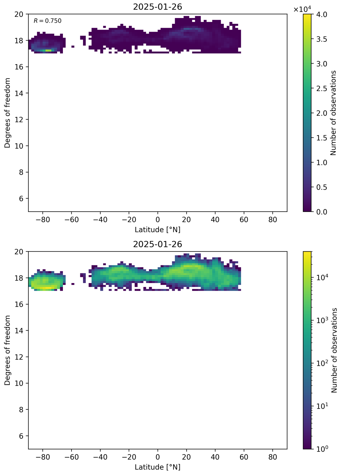
Figure 55: Scatter density plot of “Latitude” against “Degrees of freedom” for 2025-01-25 to 2025-01-27.
