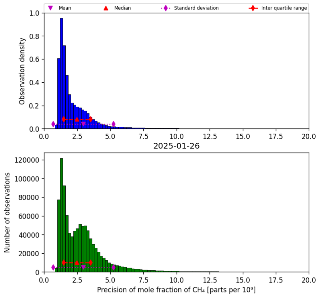
Figure 24: Histogram of “Precision of mole fraction of CH 4 ” for 2025-01-25 to 2025-01-27
