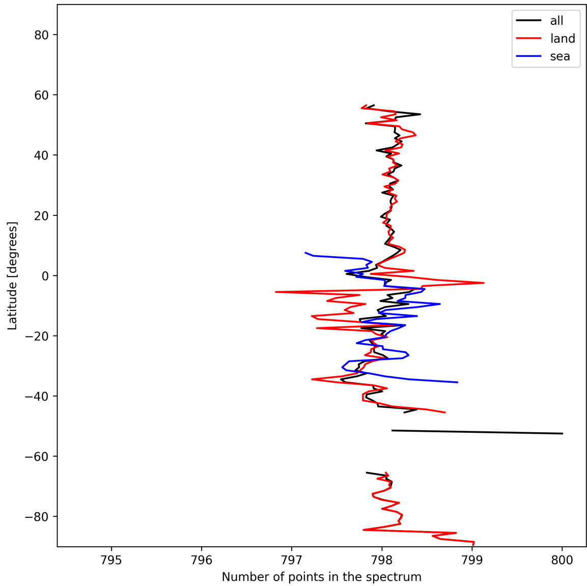
Figure 15: Zonal average of “Number of points in the spectrum” for 2025-01-25 to 2025-01-27.
