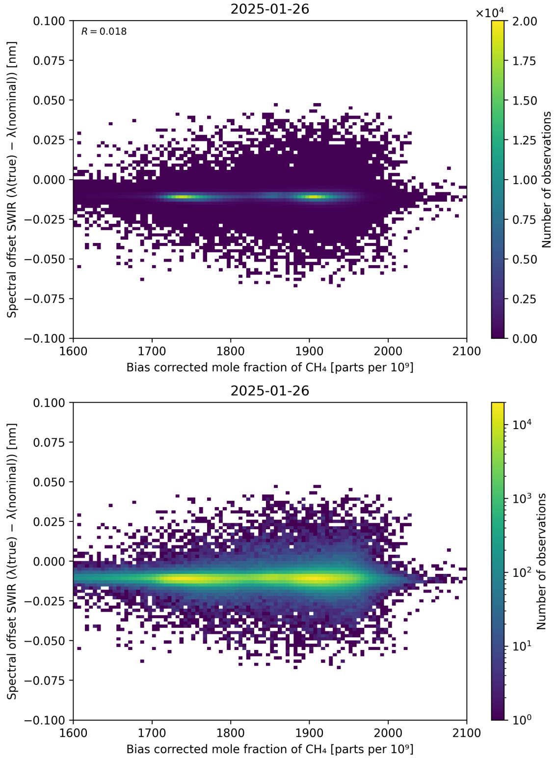
Figure 69: Scatter density plot of “Bias corrected mole fraction of \text{CH}_4 ” against “Spectral offset SWIR ( \lambda_{\text{true}} - \lambda_{\text{nominal}} )” for 2025-01-25 to 2025-01-27.
