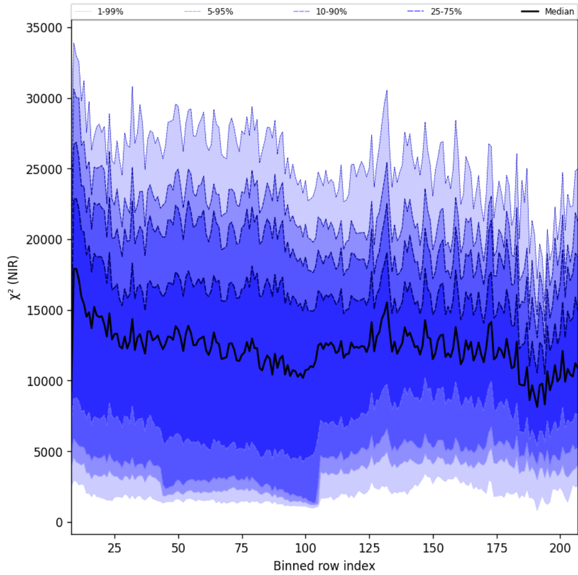
Figure 40: Along track statistics of “ \chi^2 (NIR)” for 2025-01-25 to 2025-01-27
