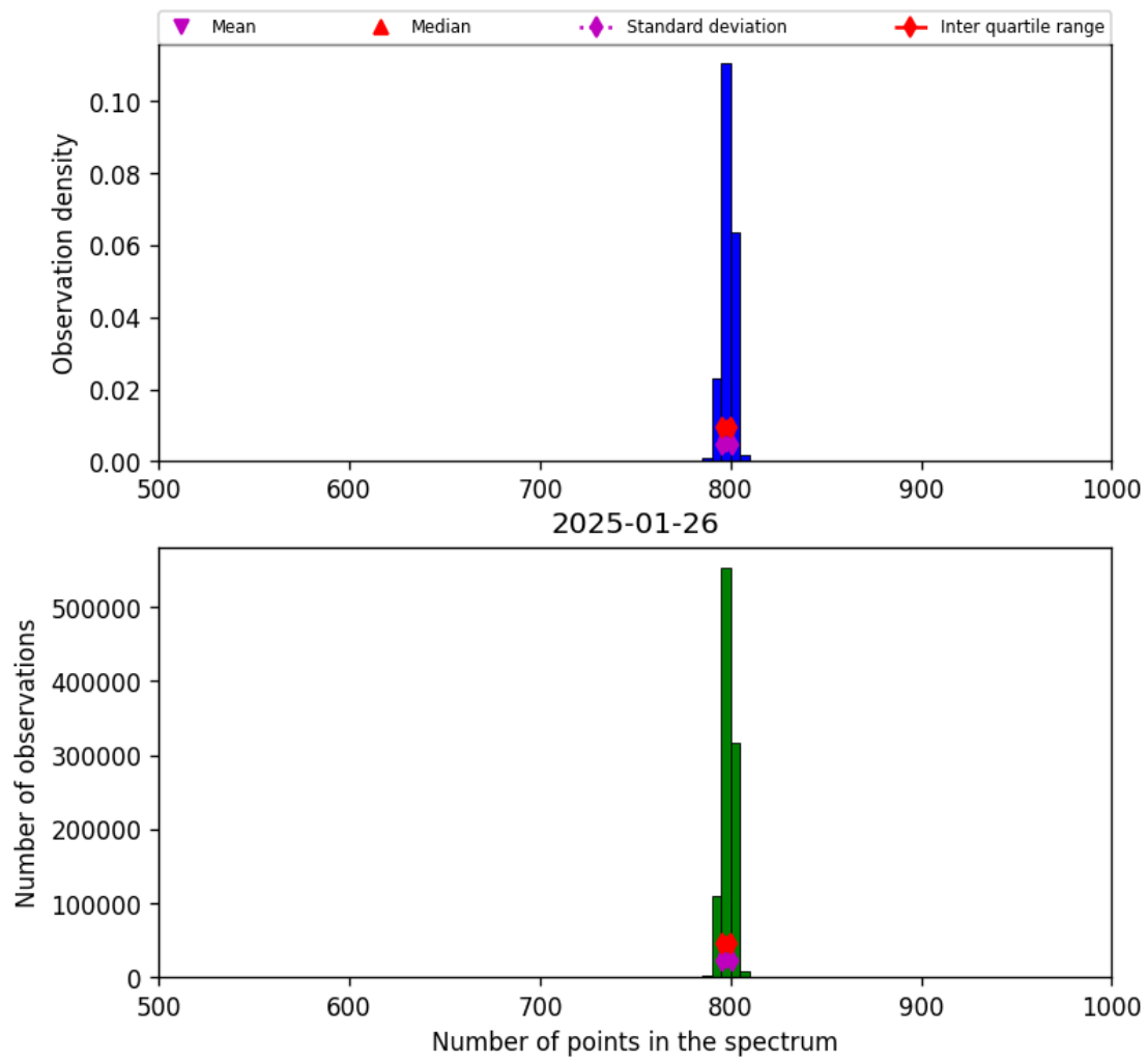
Figure 26: Histogram of “Number of points in the spectrum” for 2025-01-25 to 2025-01-27
