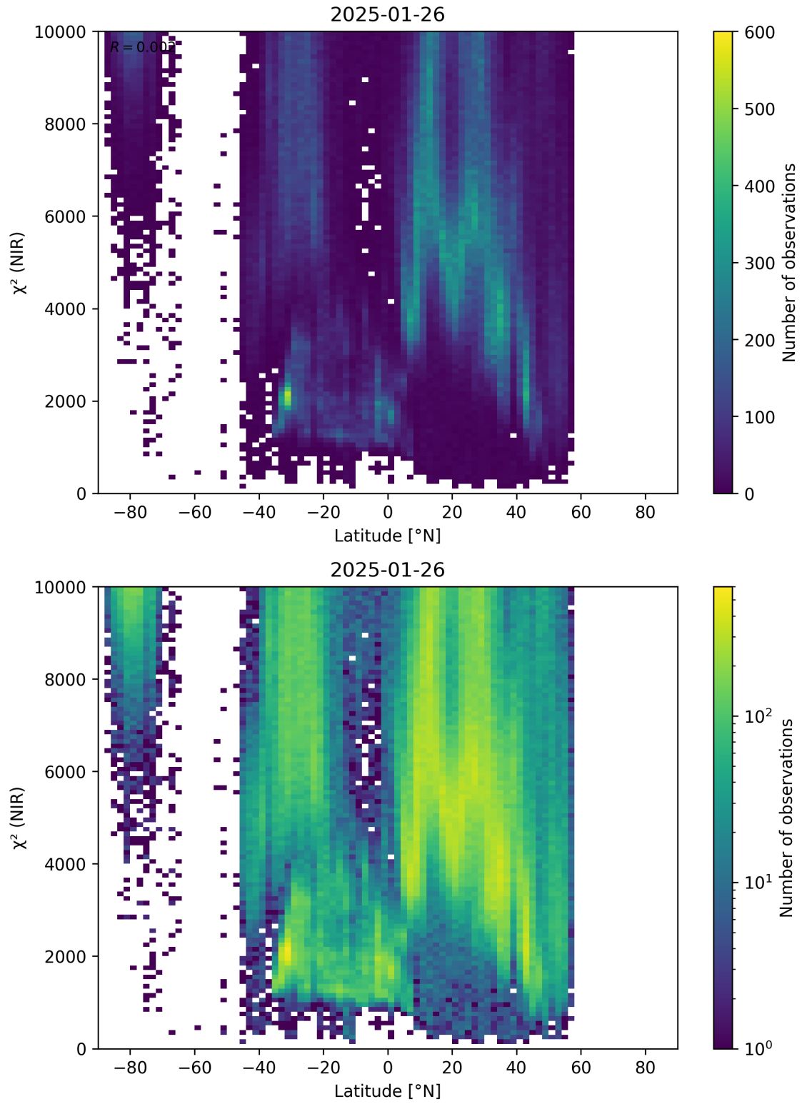
Figure 53: Scatter density plot of “Latitude” against “ \chi^2 (NIR)” for 2025-01-25 to 2025-01-27.
