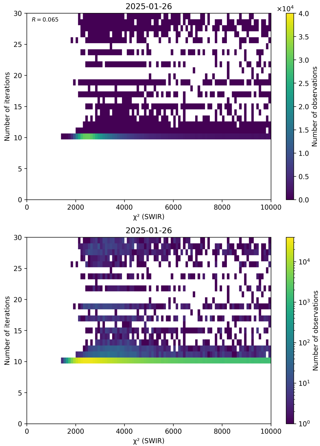
Figure 50: Scatter density plot of “ \chi^2 (SWIR)” against “Number of iterations” for 2025-01-25 to 2025-01-27.
