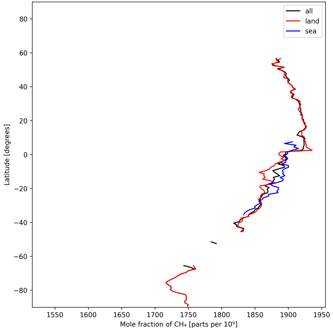
Figure 12: Zonal average of “Mole fraction of CH 4 ” for 2025-01-25 to 2025-01-27.
