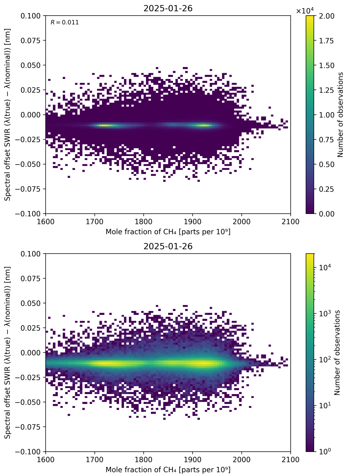
Figure 86: Scatter density plot of “Mole fraction of CH 4 ” against “Spectral offset SWIR ( \lambda_{\text{true}} - \lambda_{\text{nominal}} )” for 2025-01-25 to 2025-01-27.
