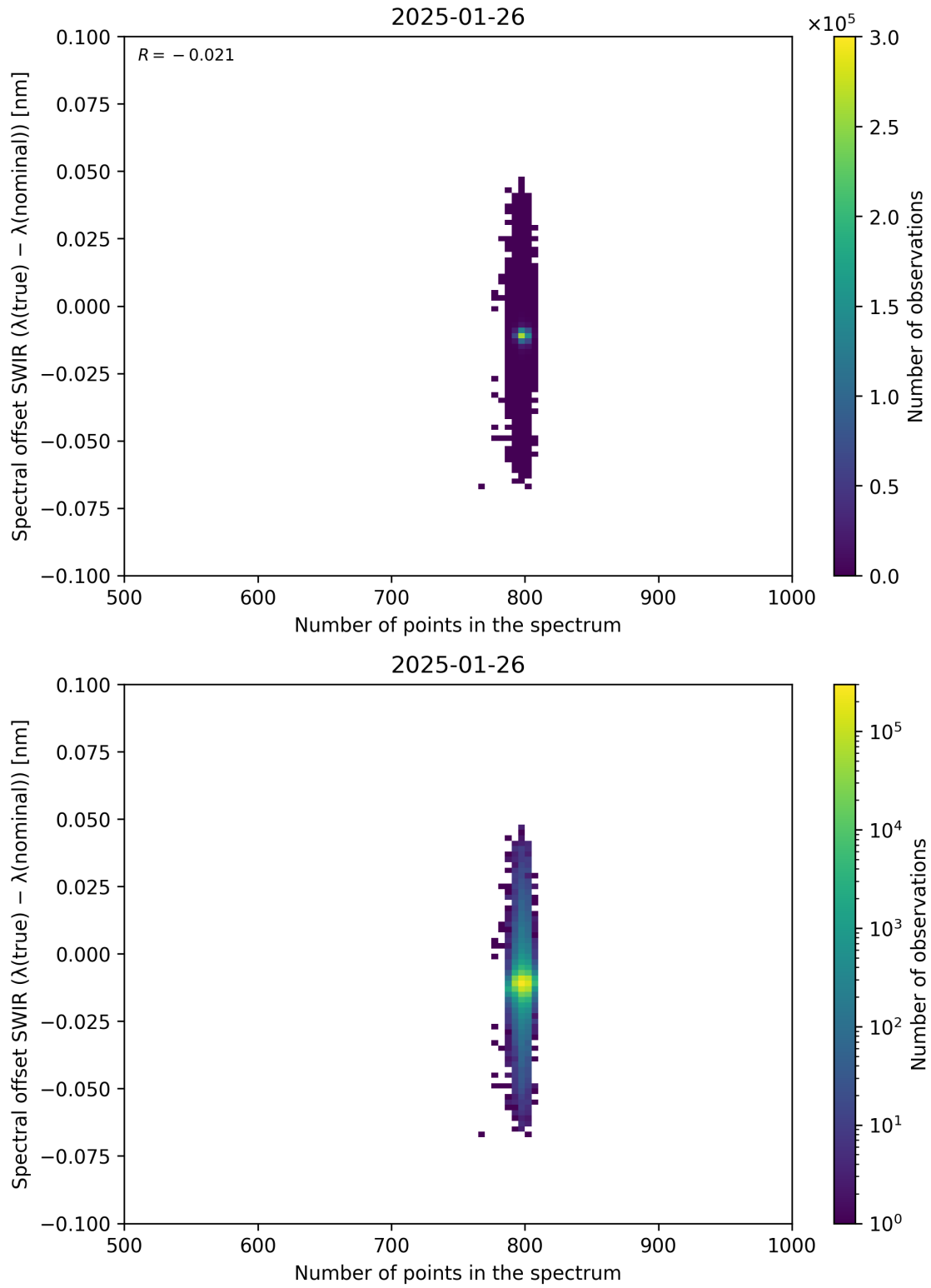
Figure 93: Scatter density plot of “Number of points in the spectrum” against “Spectral offset SWIR ( \lambda_{\text{true}} - \lambda_{\text{nominal}} )” for 2025-01-25 to 2025-01-27.
