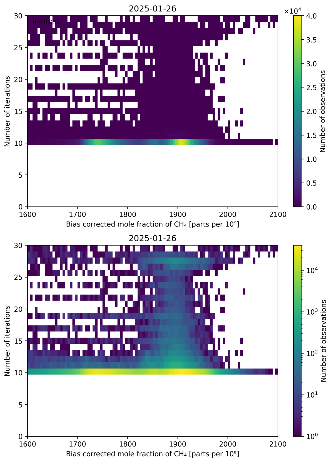
Figure 67: Scatter density plot of “Bias corrected mole fraction of \text{CH}_4 ” against “Number of iterations” for 2025-01-25 to 2025-01-27.
