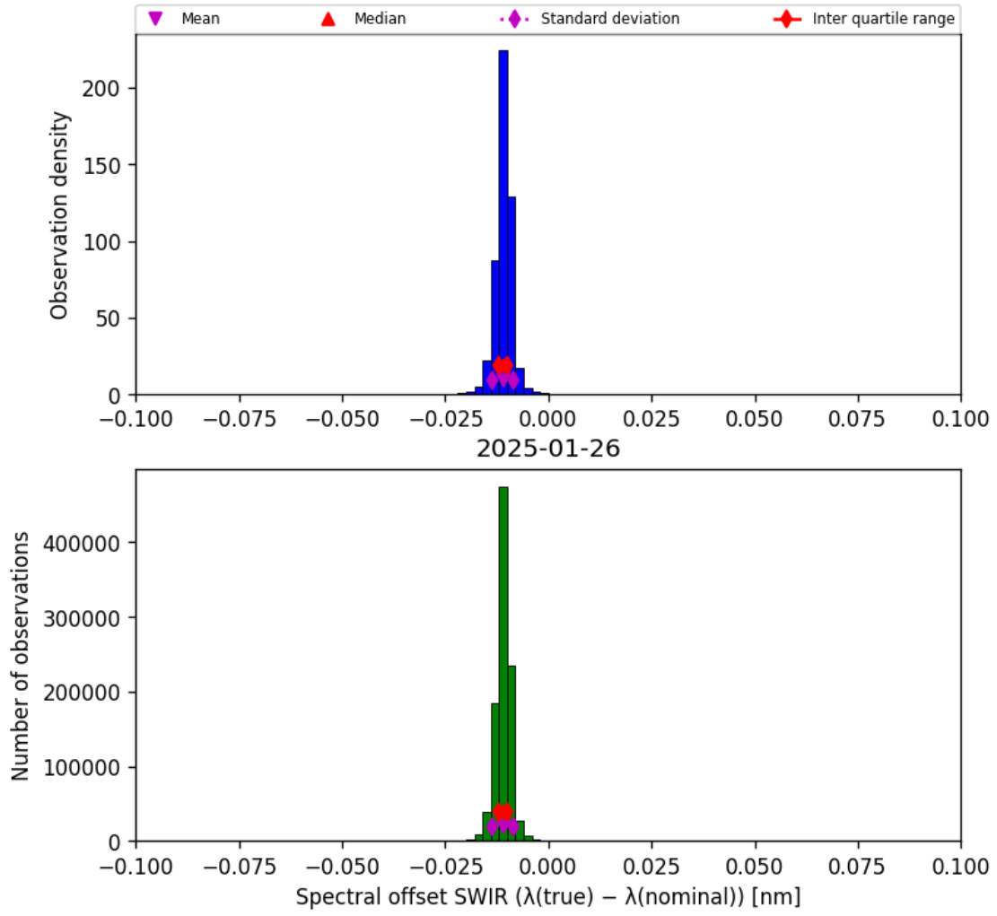
Figure 27: Histogram of “Spectral offset SWIR ( \lambda_{\text{true}} - \lambda_{\text{nominal}} )” for 2025-01-25 to 2025-01-27
