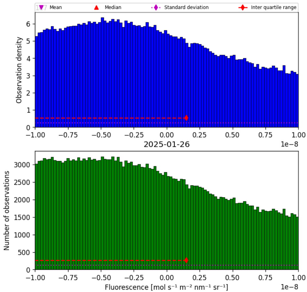
Figure 32: Histogram of “Fluorescence” for 2025-01-25 to 2025-01-27
