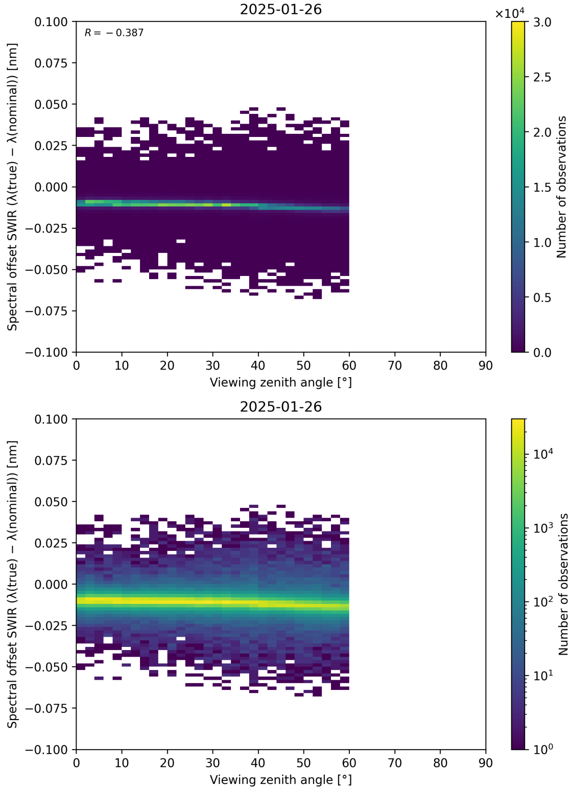
Figure 116: Scatter density plot of “Viewing zenith angle” against “Spectral offset SWIR ( \lambda_{\text{true}} - \lambda_{\text{nominal}} )” for 2025-01-25 to 2025-01-27.
