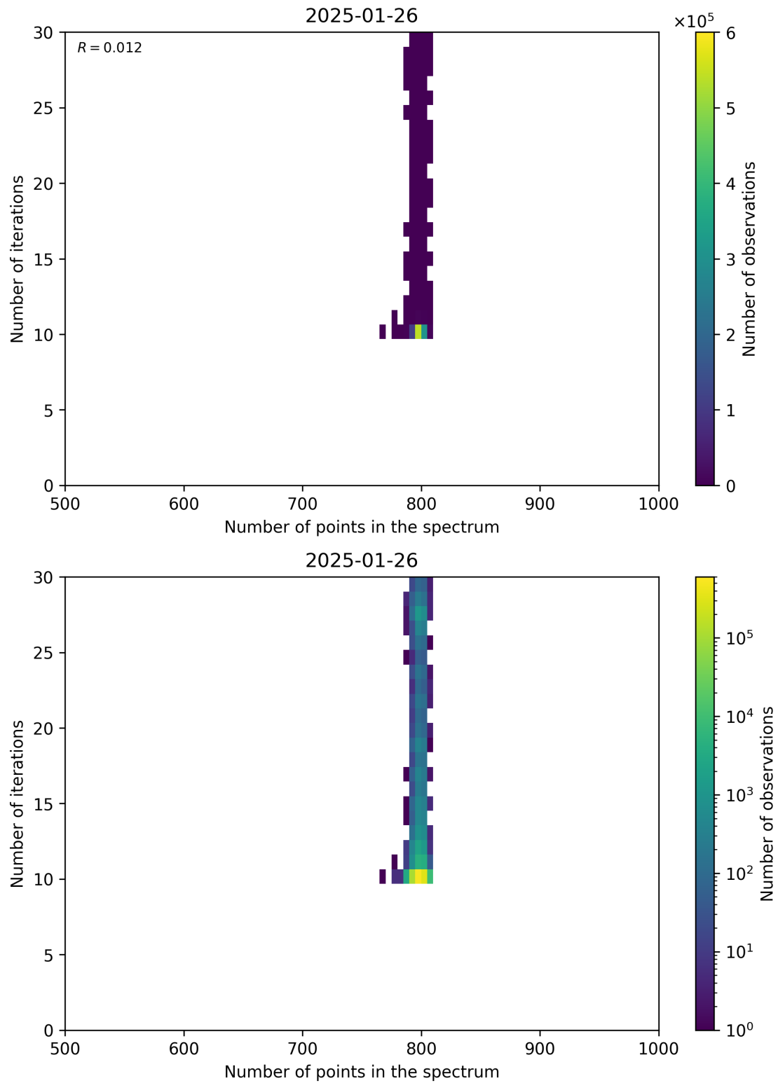
Figure 92: Scatter density plot of “Number of points in the spectrum” against “Number of iterations” for 2025-01-25 to 2025-01-27.
