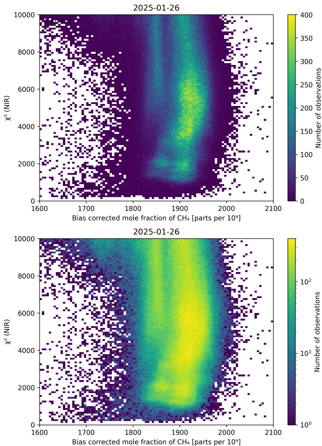
Figure 63: Scatter density plot of “Bias corrected mole fraction of \text{CH}_4 ” against “ \chi^2 (NIR)” for 2025-01-25 to 2025-01-27.
