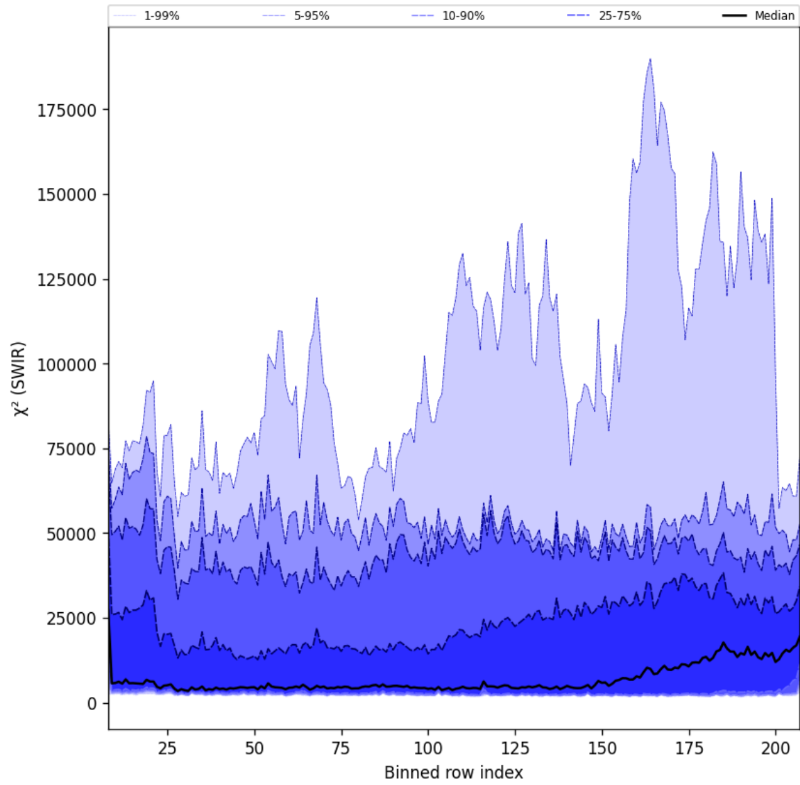
Figure 39: Along track statistics of “ \chi^2 (SWIR)” for 2025-01-25 to 2025-01-27
