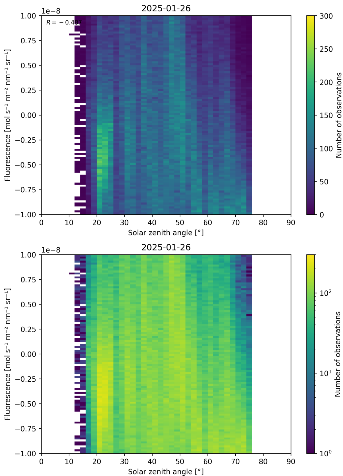
Figure 97: Scatter density plot of “Solar zenith angle” against “Fluorescence” for 2025-01-25 to 2025-01-27.
