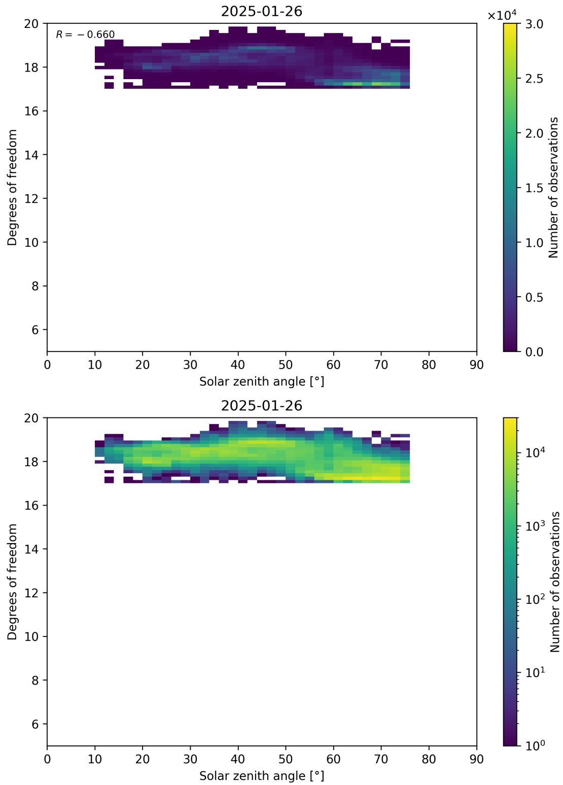
Figure 96: Scatter density plot of “Solar zenith angle” against “Degrees of freedom” for 2025-01-25 to 2025-01-27.
