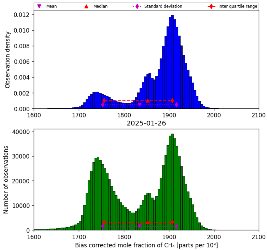
Figure 25: Histogram of “Bias corrected mole fraction of CH 4 ” for 2025-01-25 to 2025-01-27
