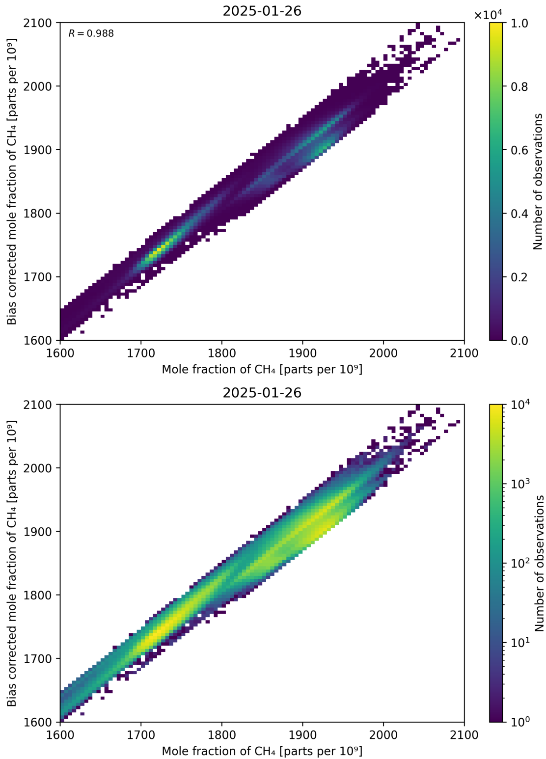
Figure 74: Scatter density plot of “Mole fraction of CH 4 ” against “Bias corrected mole fraction of CH 4 ” for 2025-01-25 to 2025-01-27.
