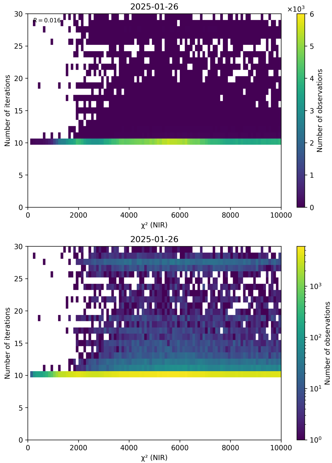
Figure 46: Scatter density plot of “ \chi^2 (NIR)” against “Number of iterations” for 2025-01-25 to 2025-01-27.
