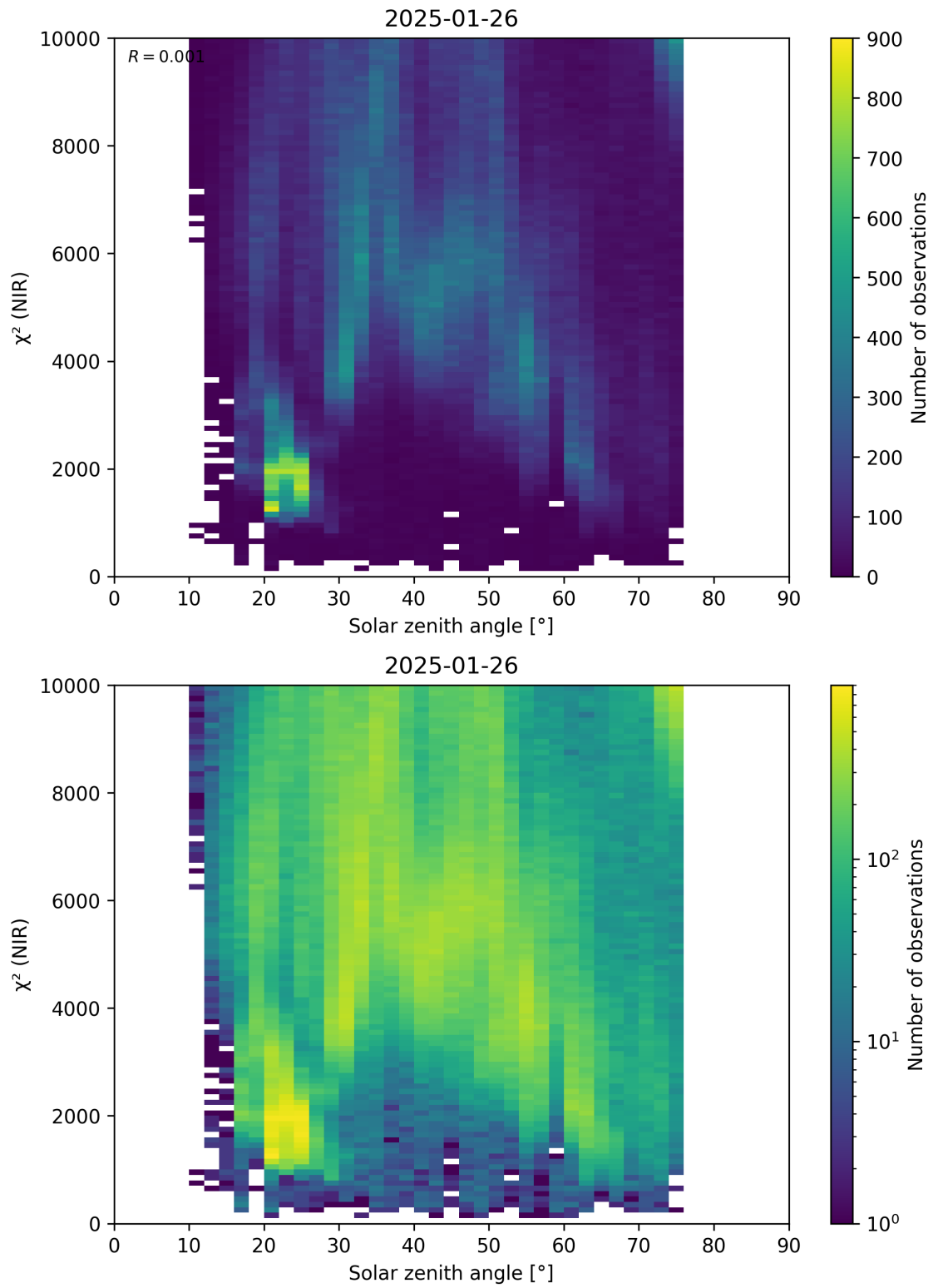
Figure 94: Scatter density plot of “Solar zenith angle” against “ \chi^2 (NIR)” for 2025-01-25 to 2025-01-27.
