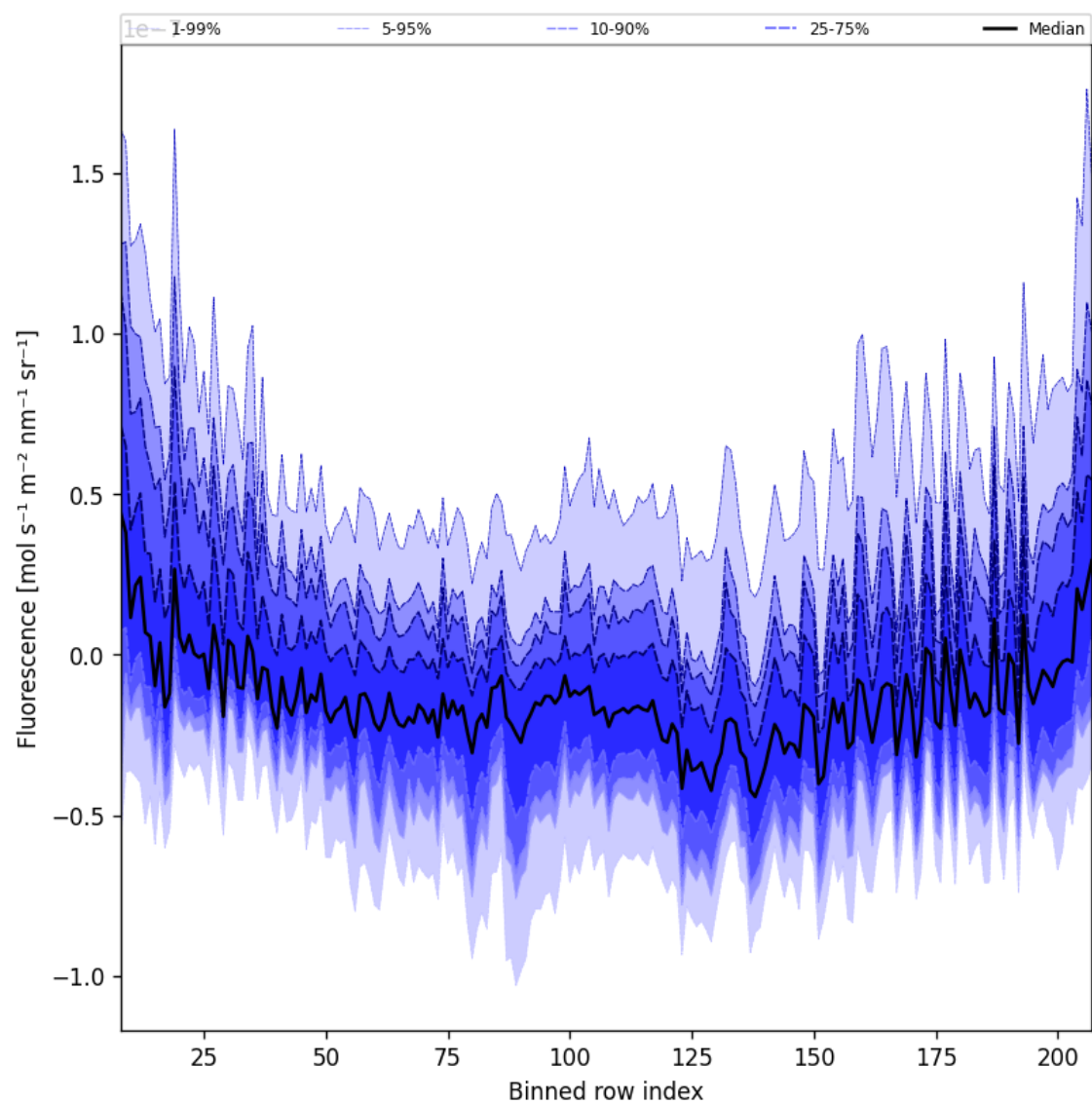
Figure 43: Along track statistics of "Fluorescence" for 2025-01-25 to 2025-01-27
