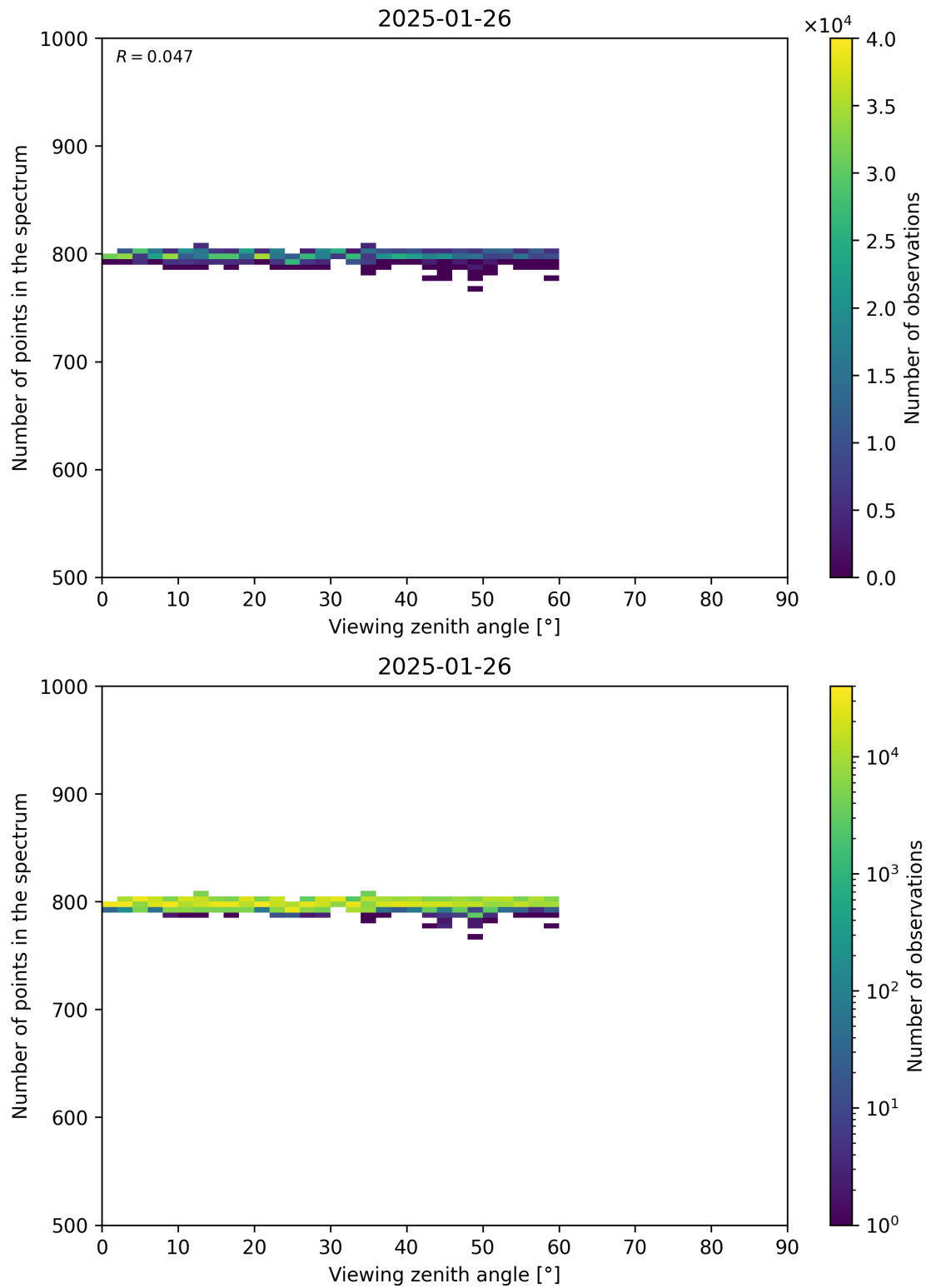
Figure 114: Scatter density plot of “Viewing zenith angle” against “Number of points in the spectrum” for 2025-01-25 to 2025-01-27.
