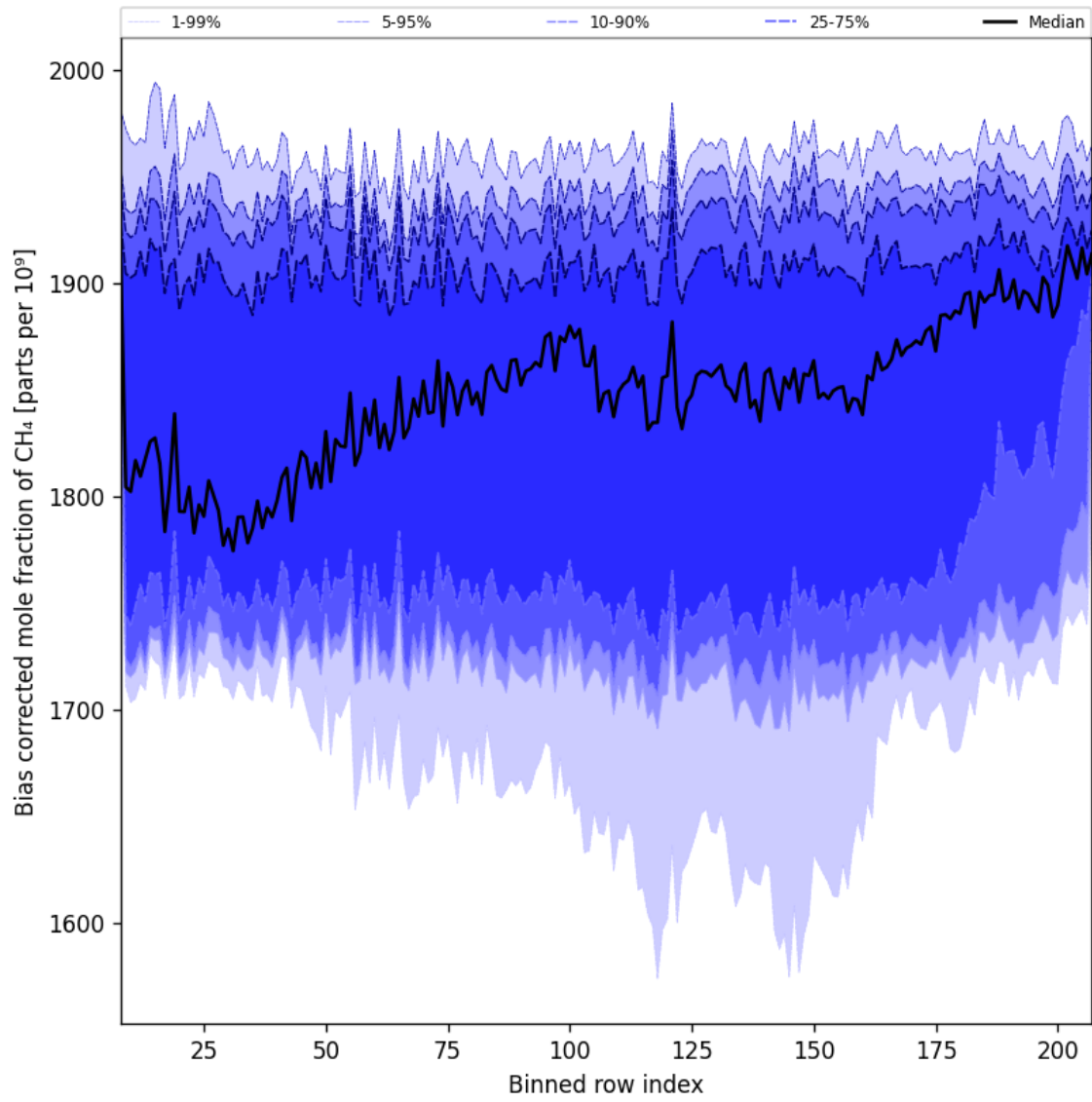
Figure 36: Along track statistics of “Bias corrected mole fraction of CH 4 ” for 2025-01-25 to 2025-01-27
