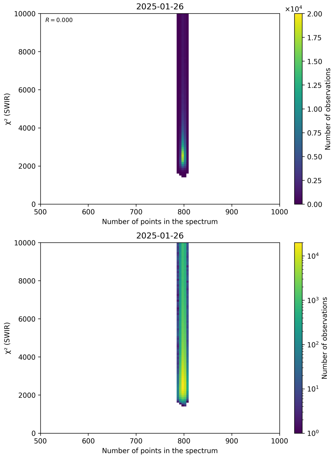
Figure 89: Scatter density plot of “Number of points in the spectrum” against “ \chi^2 (SWIR)” for 2025-01-25 to 2025-01-27.
