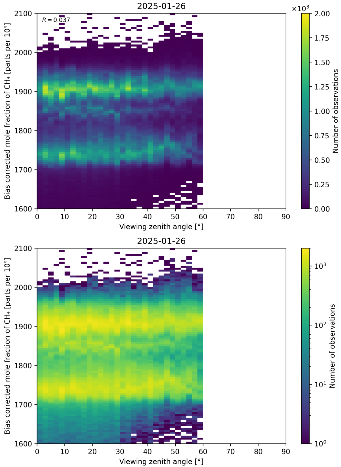
Figure 111: Scatter density plot of “Viewing zenith angle” against “Bias corrected mole fraction of CH 4 ” for 2025-01-25 to 2025-01-27.
