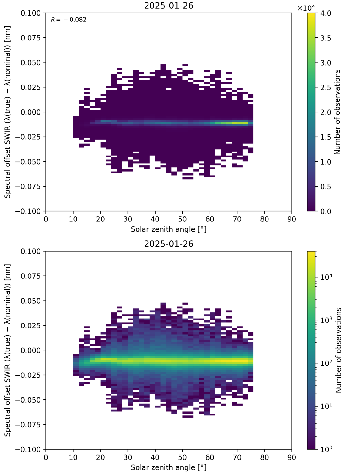
Figure 104: Scatter density plot of “Solar zenith angle” against “Spectral offset SWIR ( \lambda_{\text{true}} - \lambda_{\text{nominal}} )” for 2025-01-25 to 2025-01-27.
