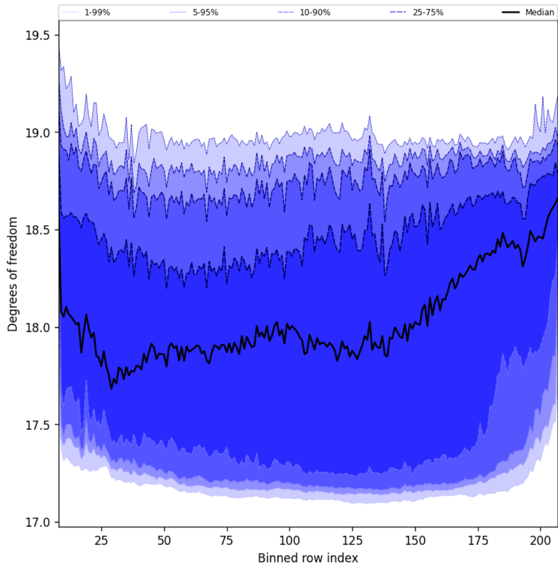
Figure 41: Along track statistics of “Degrees of freedom” for 2025-01-25 to 2025-01-27
