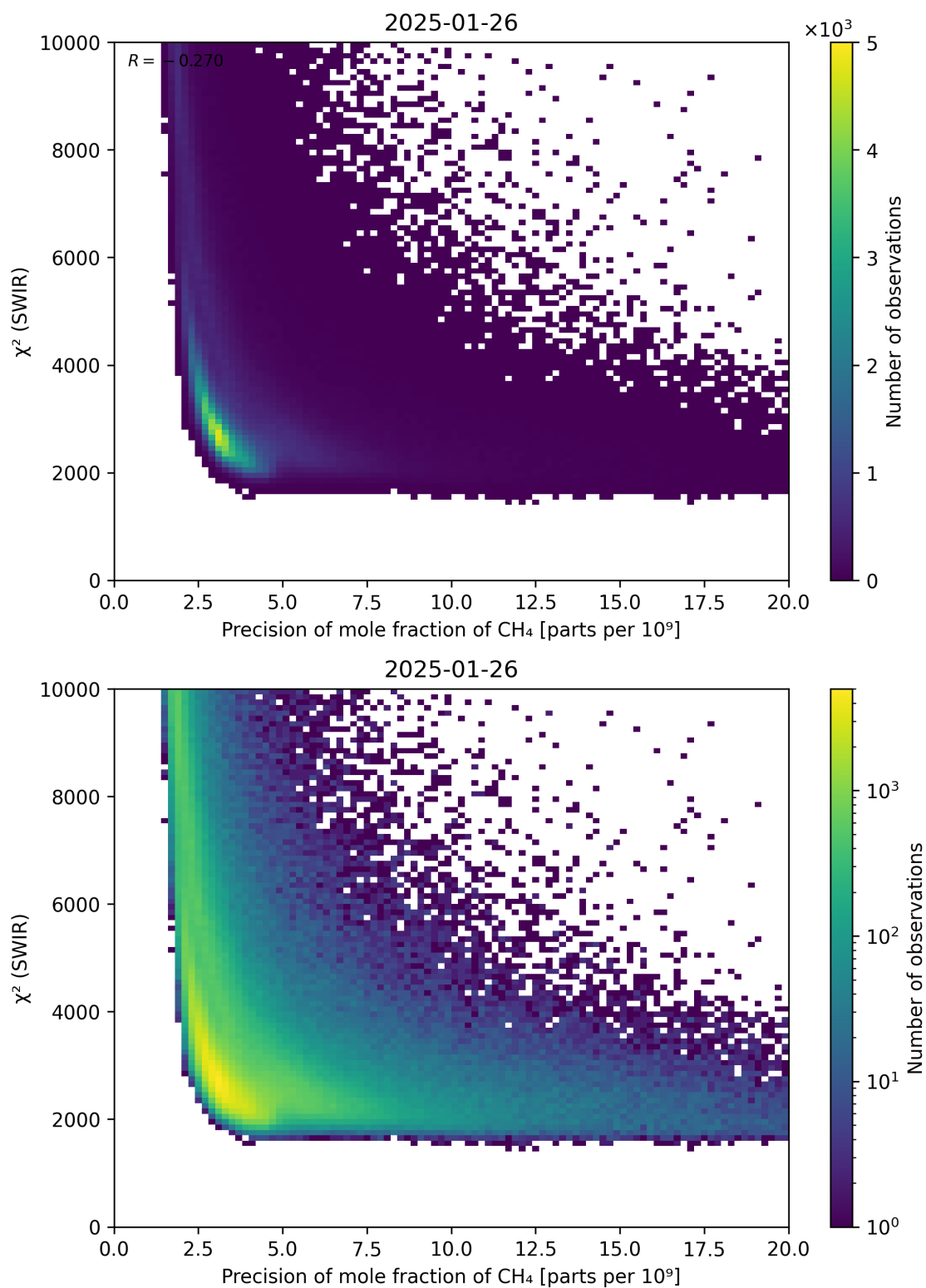
Figure 79: Scatter density plot of “Precision of mole fraction of \text{CH}_4 ” against “ \chi^2 (SWIR)” for 2025-01-25 to 2025-01-27.
