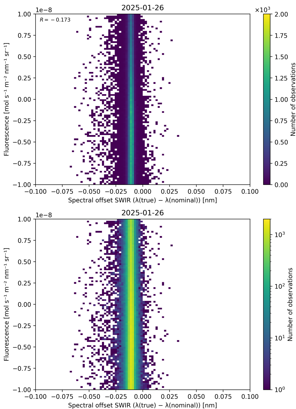
Figure 120: Scatter density plot of “Spectral offset SWIR ( \lambda_{\text{true}} - \lambda_{\text{nominal}} )” against “Fluorescence” for 2025-01-25 to 2025-01-27.
