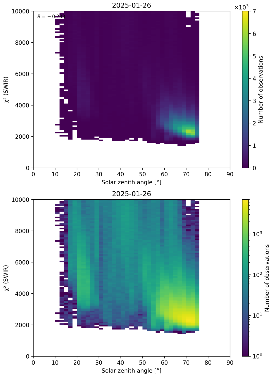
Figure 95: Scatter density plot of “Solar zenith angle” against “ \chi^2 (SWIR)” for 2025-01-25 to 2025-01-27.
