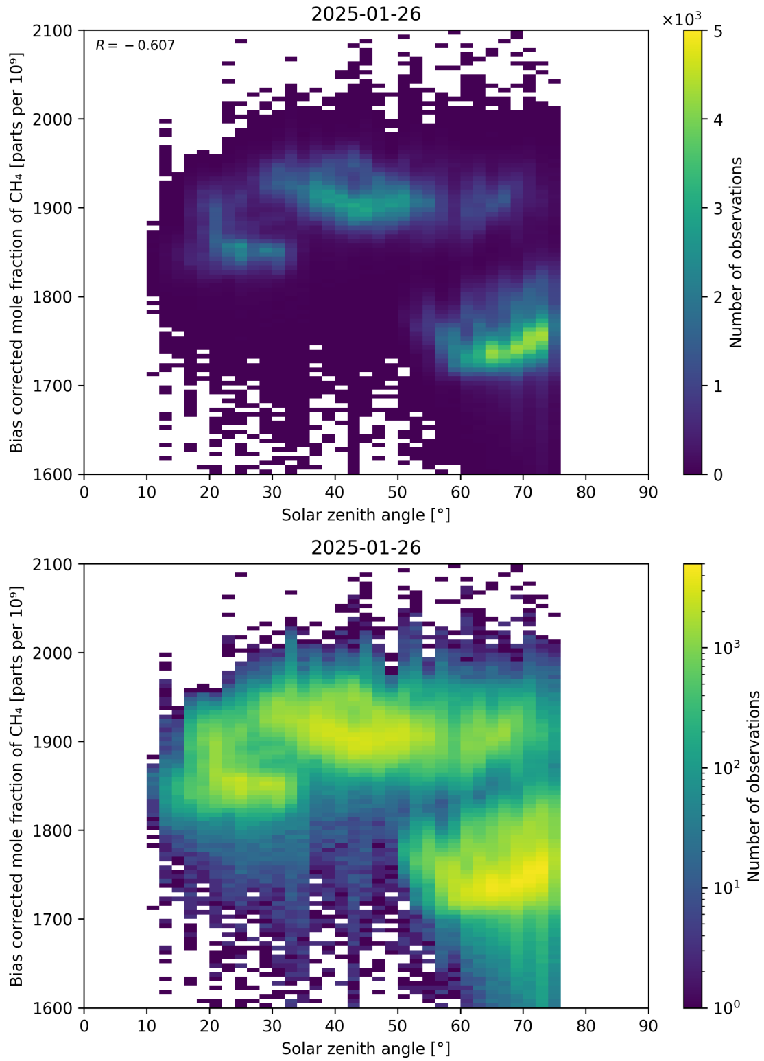
Figure 100: Scatter density plot of “Solar zenith angle” against “Bias corrected mole fraction of \text{CH}_4 ” for 2025-01-25 to 2025-01-27.
