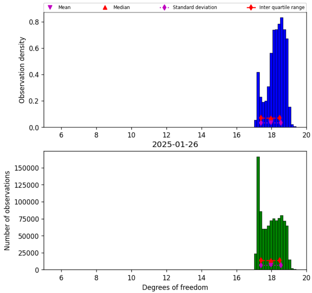
Figure 30: Histogram of “Degrees of freedom” for 2025-01-25 to 2025-01-27
