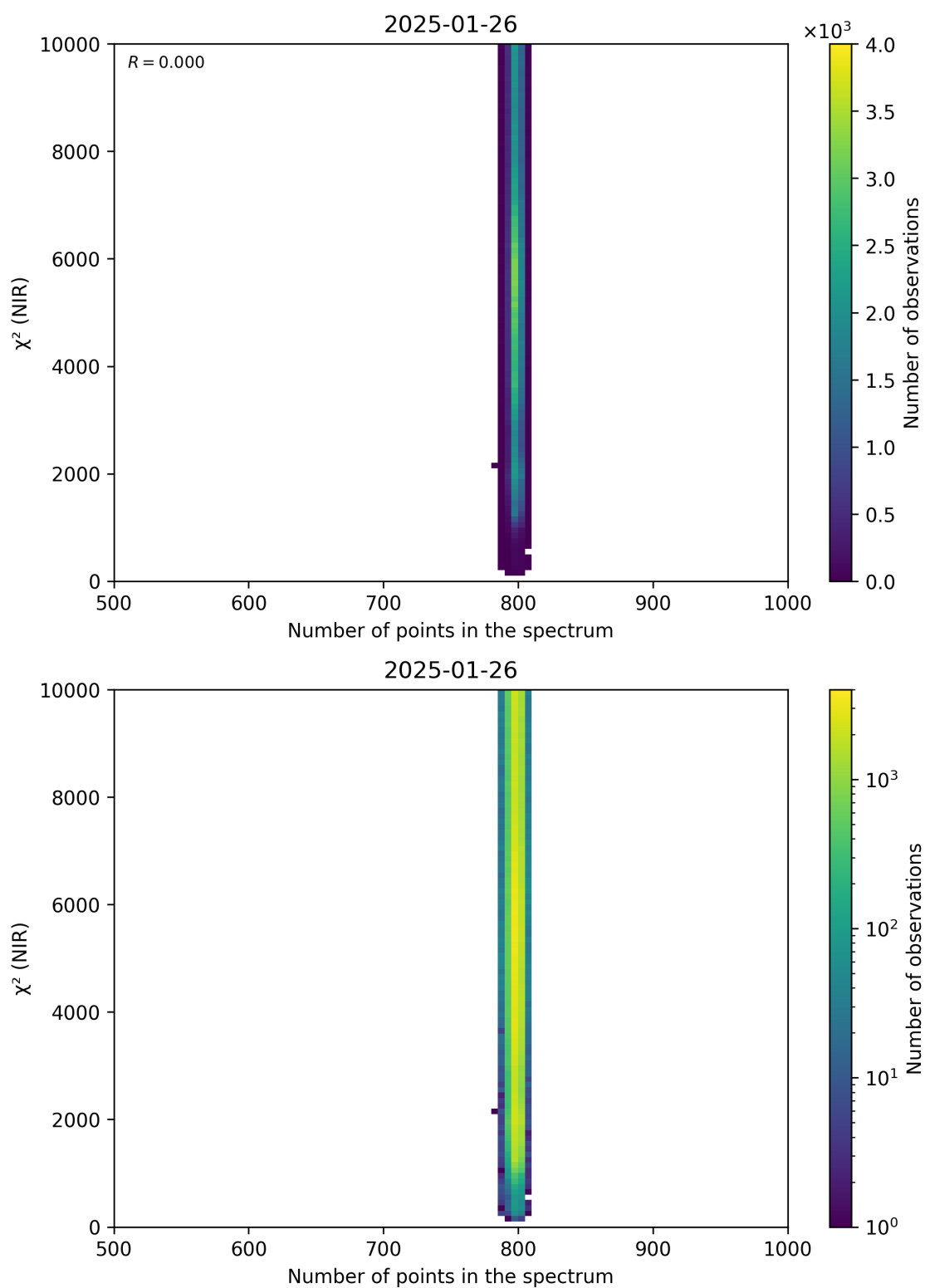
Figure 88: Scatter density plot of “Number of points in the spectrum” against “ \chi^2 (NIR)” for 2025-01-25 to 2025-01-27.
