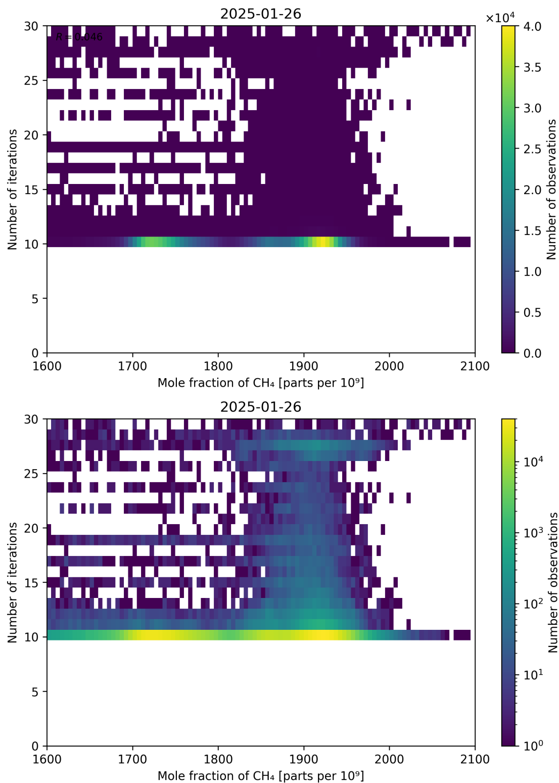
Figure 76: Scatter density plot of “Mole fraction of CH 4 ” against “Number of iterations” for 2025-01-25 to 2025-01-27.
