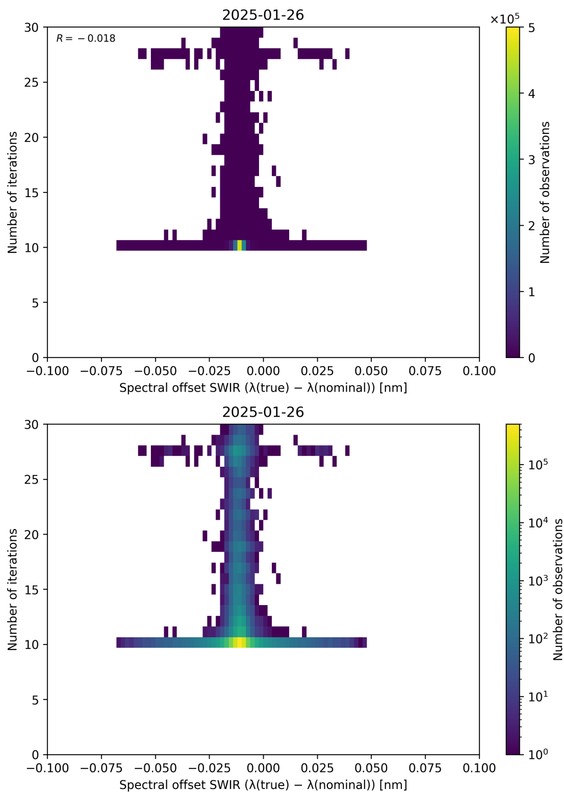
Figure 121: Scatter density plot of “Spectral offset SWIR ( \lambda_{\text{true}} - \lambda_{\text{nominal}} )” against “Number of iterations” for 2025-01-25 to 2025-01-27.
