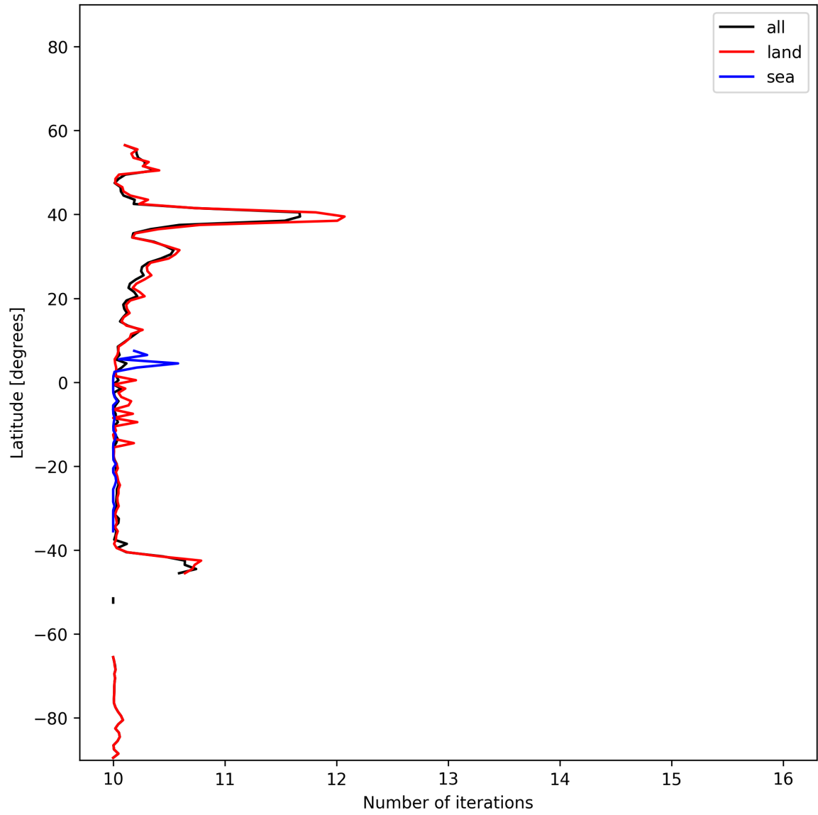
Figure 20: Zonal average of “Number of iterations” for 2025-01-25 to 2025-01-27.
