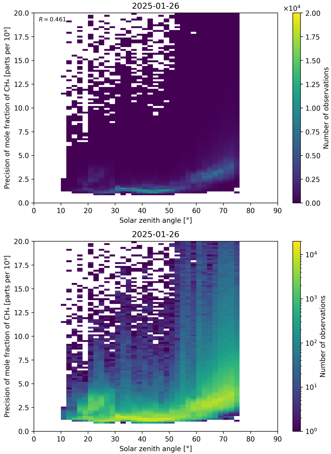
Figure 101: Scatter density plot of “Solar zenith angle” against “Precision of mole fraction of CH 4 ” for 2025-01-25 to 2025-01-27.
