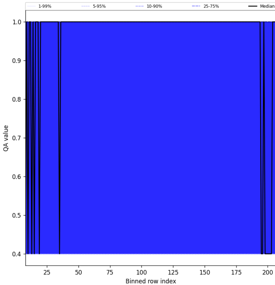
Figure 33: Along track statistics of “QA value” for 2025-01-25 to 2025-01-27
