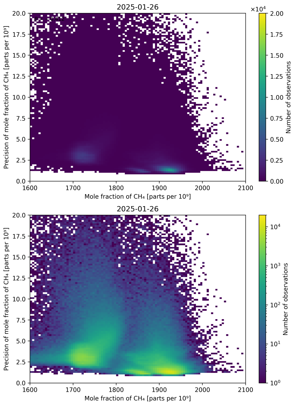
Figure 75: Scatter density plot of “Mole fraction of CH 4 ” against “Precision of mole fraction of CH 4 ” for 2025-01-25 to 2025-01-27.
