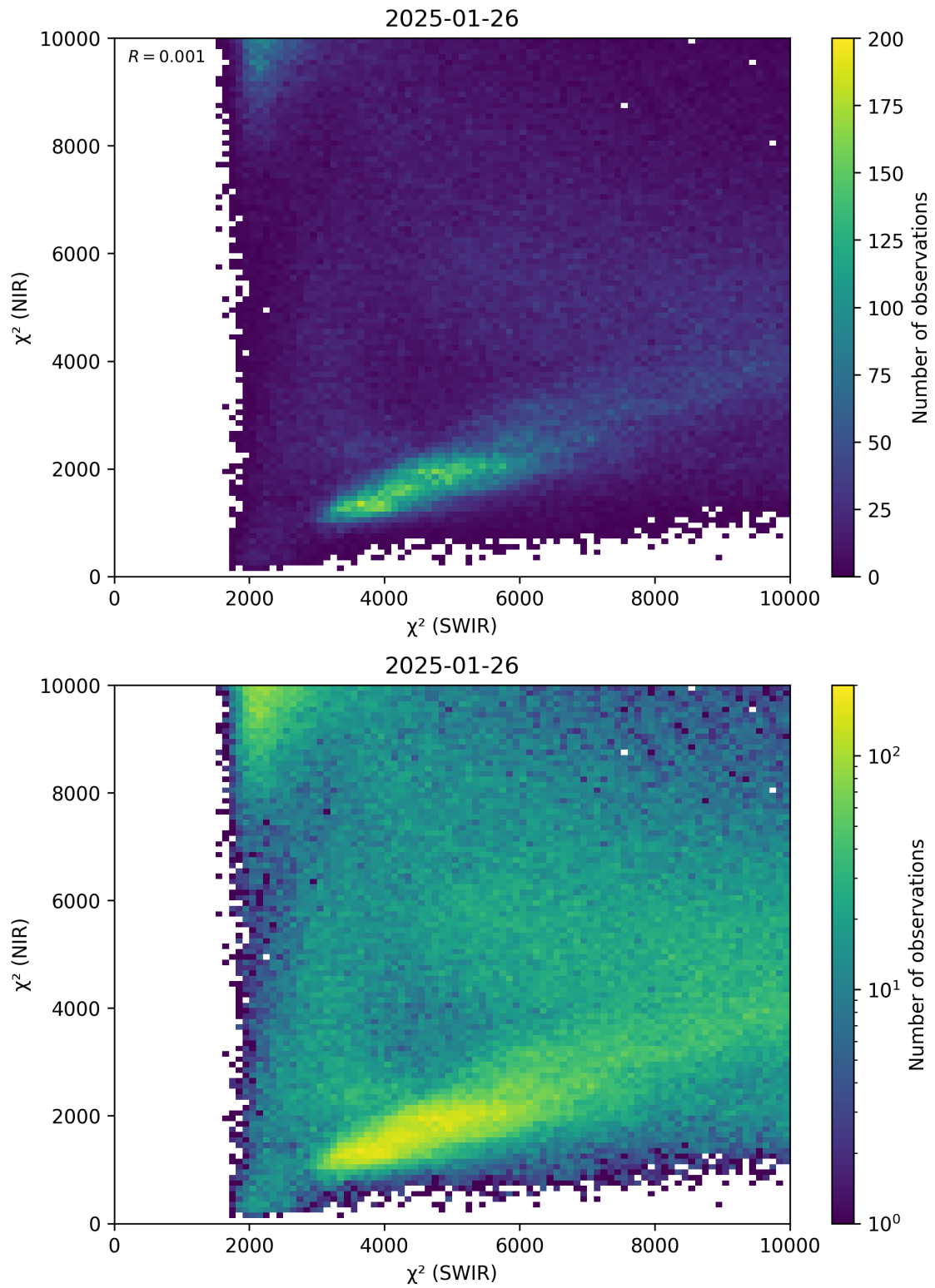
Figure 47: Scatter density plot of “ \chi^2 (SWIR)” against “ \chi^2 (NIR)” for 2025-01-25 to 2025-01-27.
