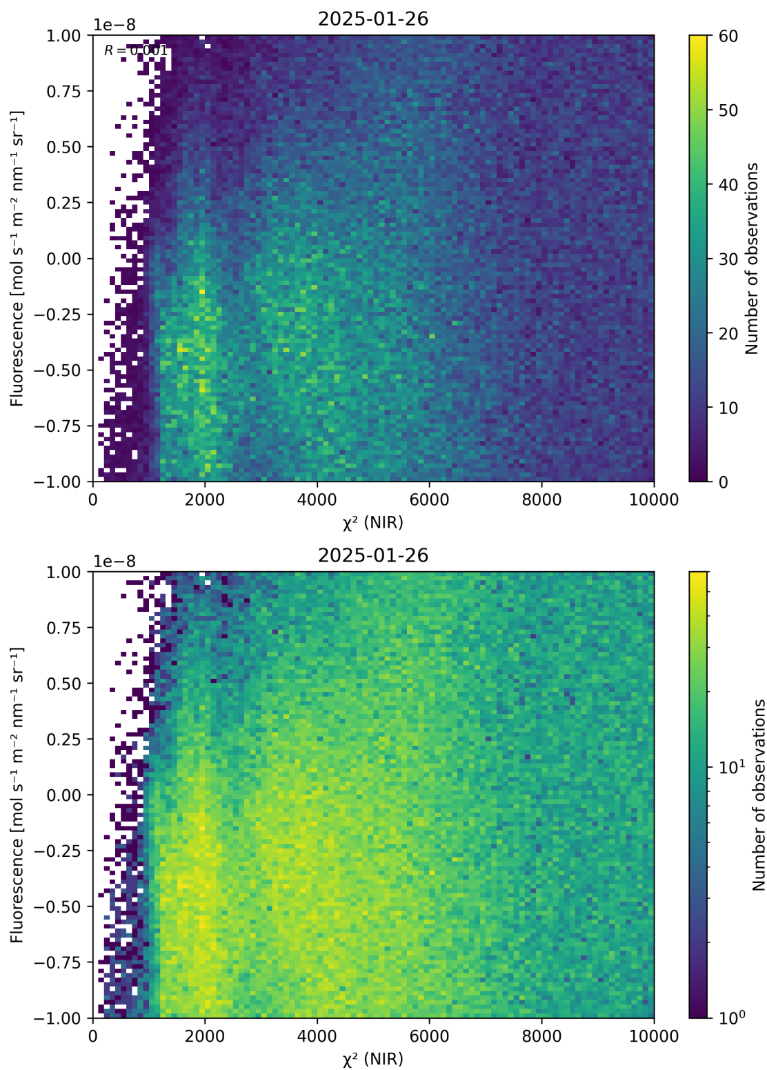
Figure 45: Scatter density plot of “ \chi^2 (NIR)” against “Fluorescence” for 2025-01-25 to 2025-01-27.
