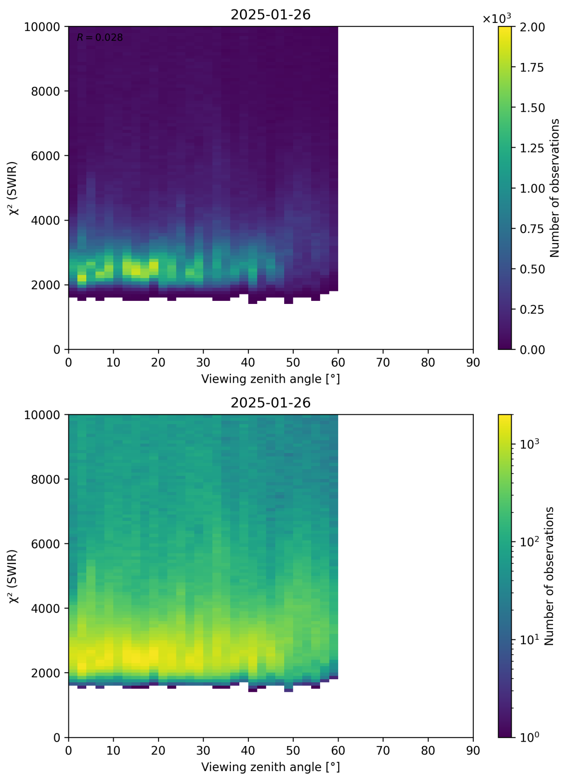
Figure 106: Scatter density plot of “Viewing zenith angle” against “ \chi^2 (SWIR)” for 2025-01-25 to 2025-01-27.
