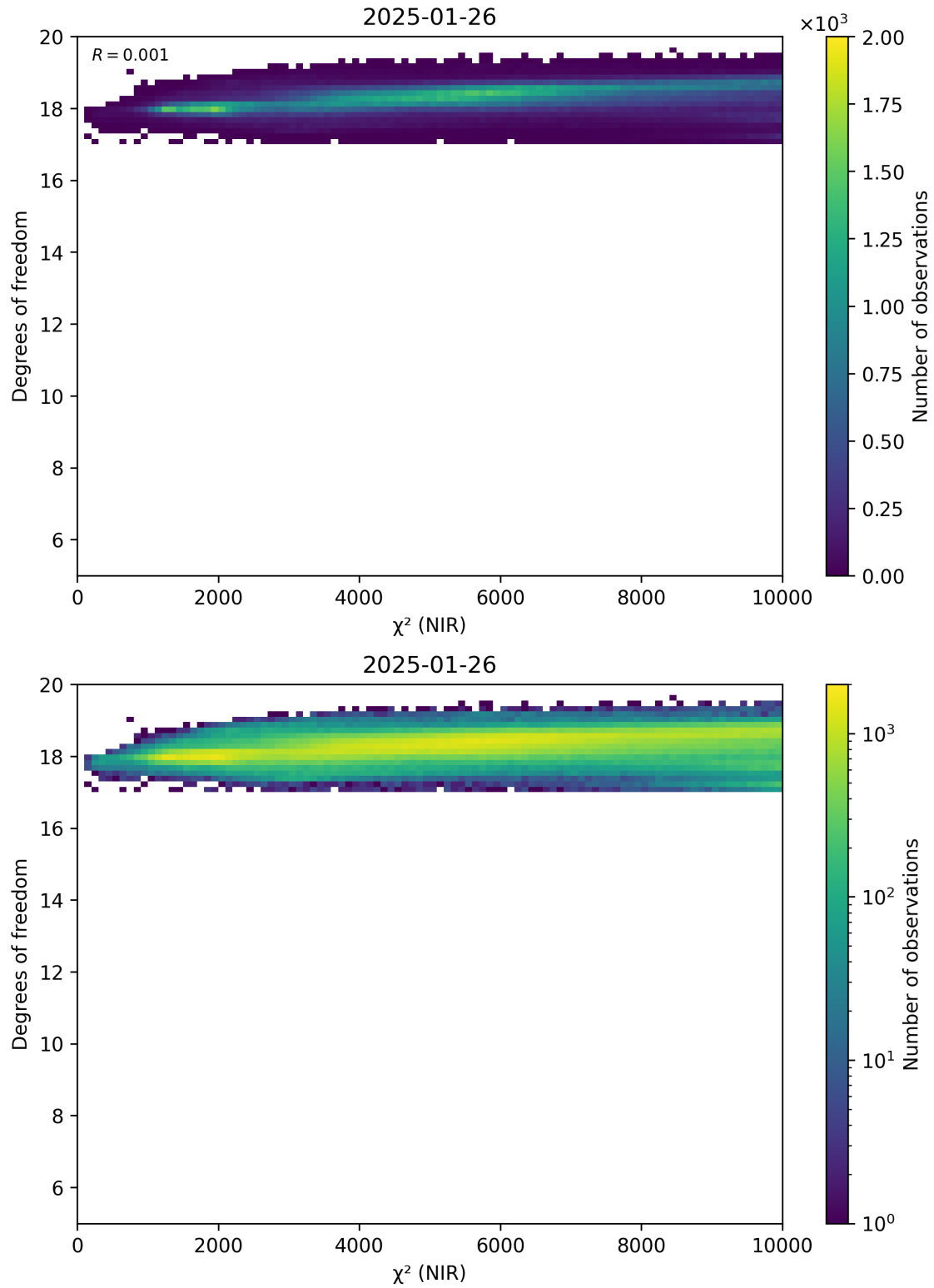
Figure 44: Scatter density plot of “ \chi^2 (NIR)” against “Degrees of freedom” for 2025-01-25 to 2025-01-27.
