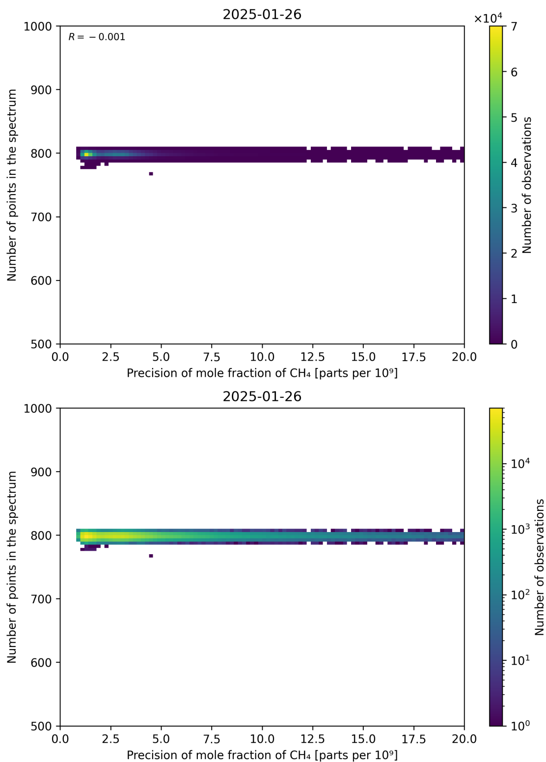
Figure 84: Scatter density plot of “Precision of mole fraction of CH 4 ” against “Number of points in the spectrum” for 2025-01-25 to 2025-01-27.
