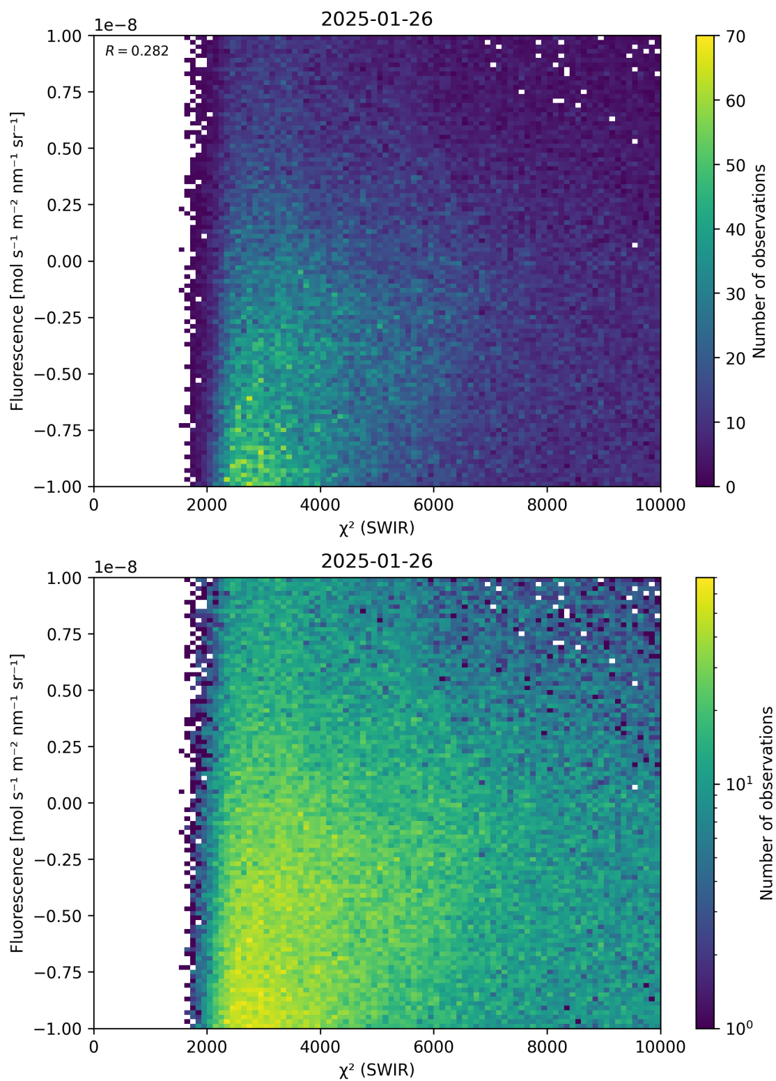
Figure 49: Scatter density plot of “ \chi^2 (SWIR)” against “Fluorescence” for 2025-01-25 to 2025-01-27.
