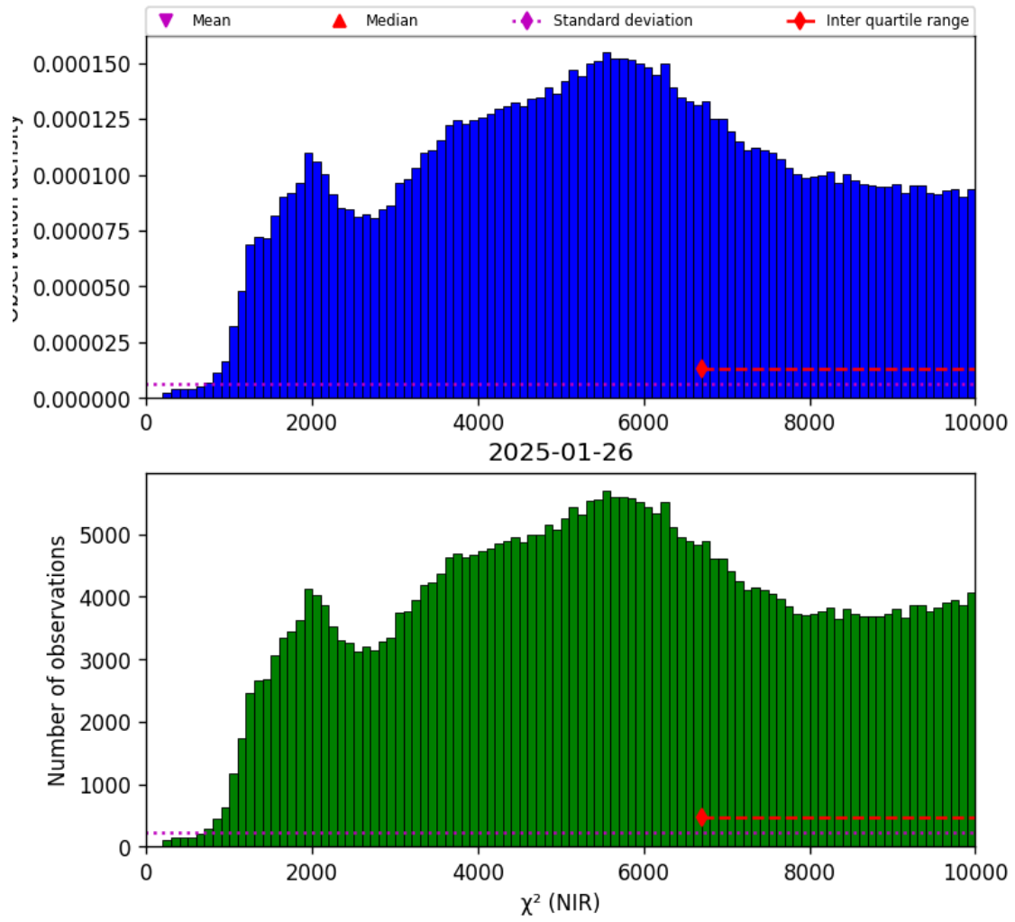
Figure 29: Histogram of “ \chi^2 (NIR)” for 2025-01-25 to 2025-01-27
