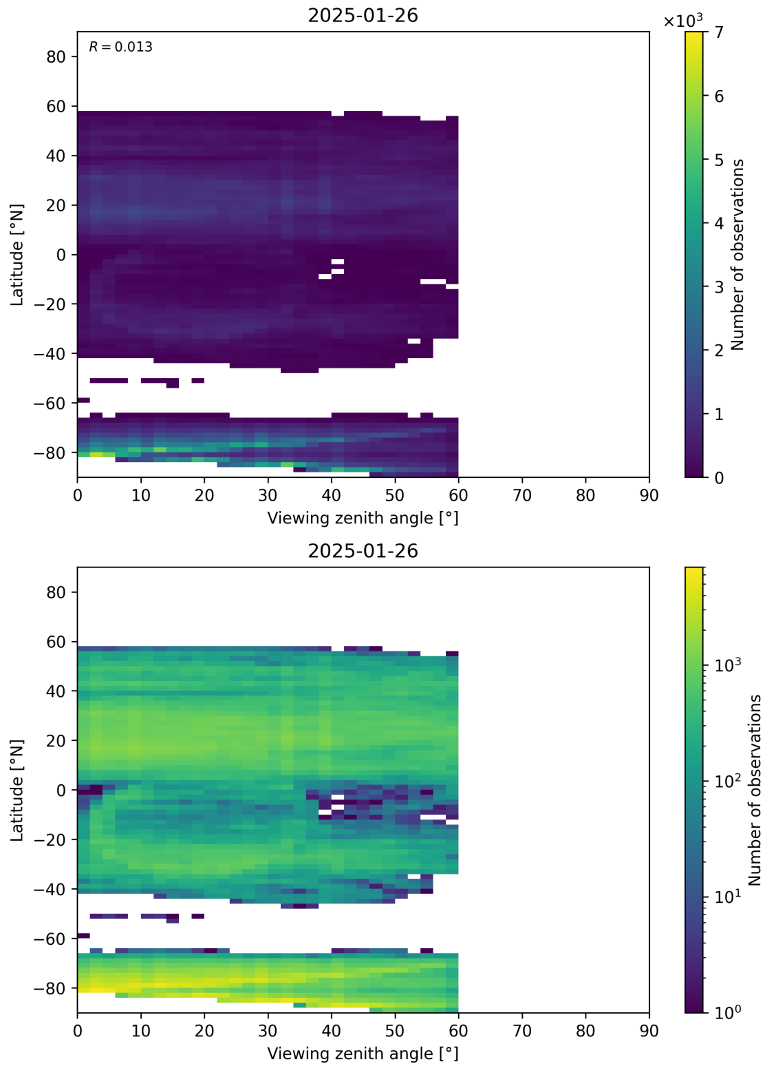
Figure 109: Scatter density plot of “Viewing zenith angle” against “Latitude” for 2025-01-25 to 2025-01-27.
