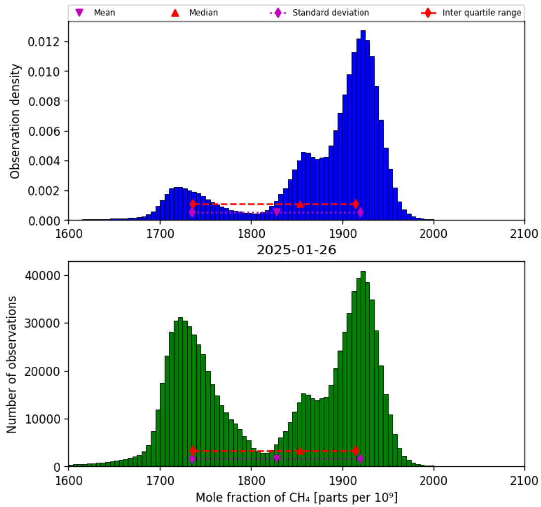
Figure 23: Histogram of “Mole fraction of CH 4 ” for 2025-01-25 to 2025-01-27
