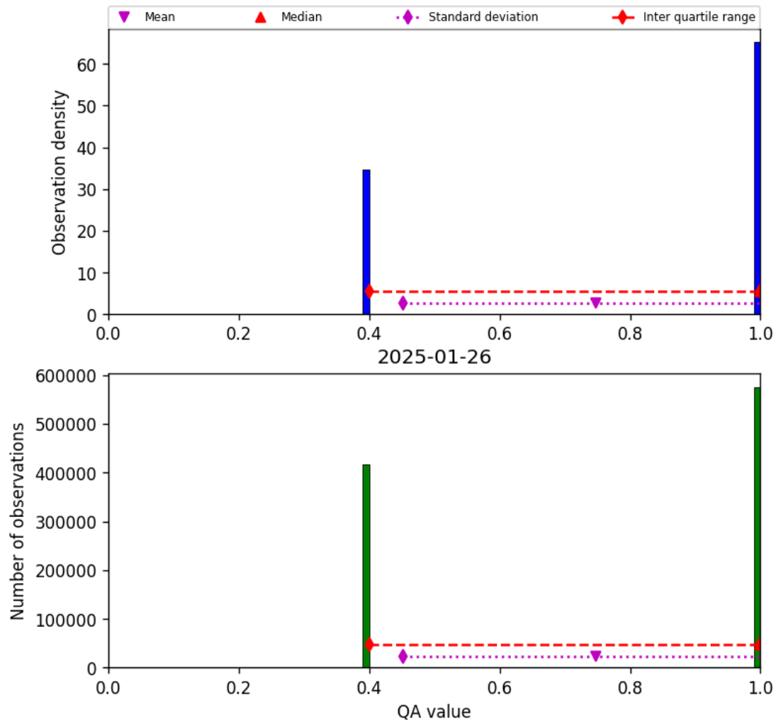
Figure 22: Histogram of “QA value” for 2025-01-25 to 2025-01-27
