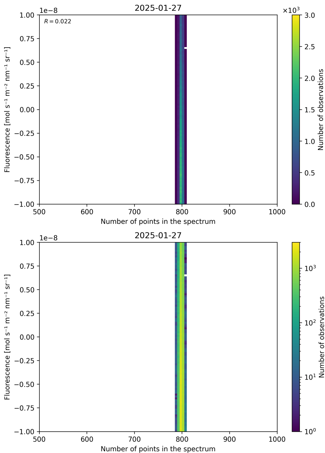
Figure 91: Scatter density plot of “Number of points in the spectrum” against “Fluorescence” for 2025-01-26 to 2025-01-28.
