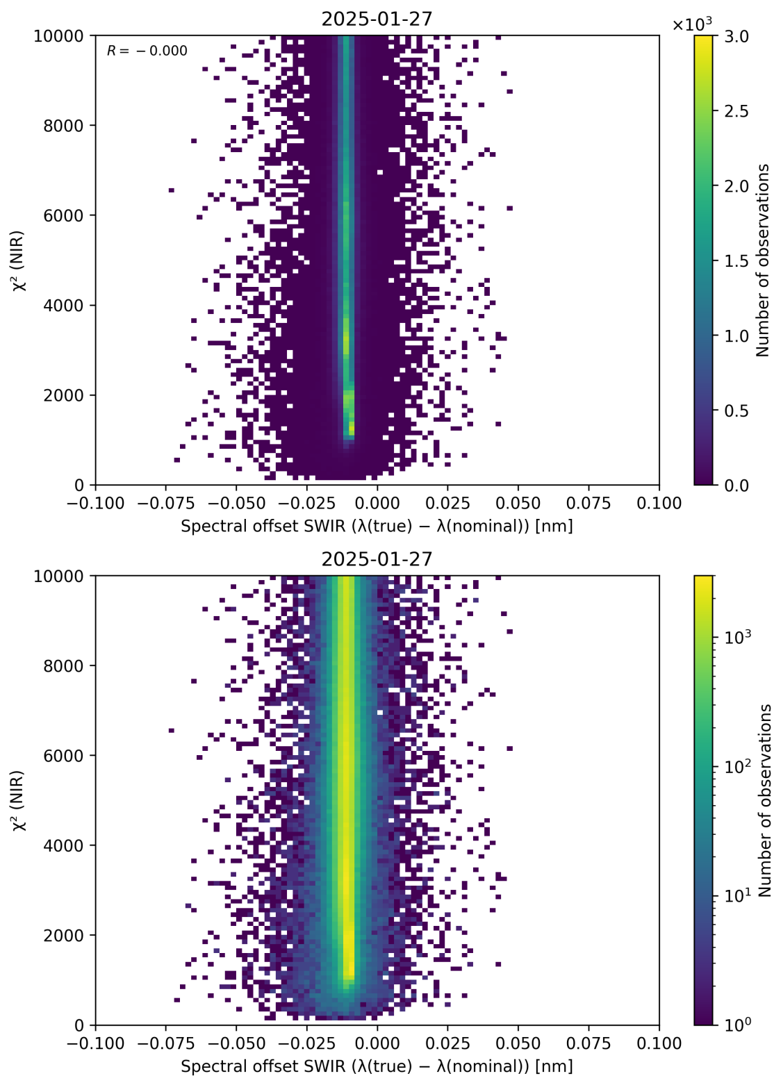
Figure 117: Scatter density plot of “Spectral offset SWIR ( \lambda_{\text{true}} - \lambda_{\text{nominal}} )” against “ \chi^2 (NIR)” for 2025-01-26 to 2025-01-28.
