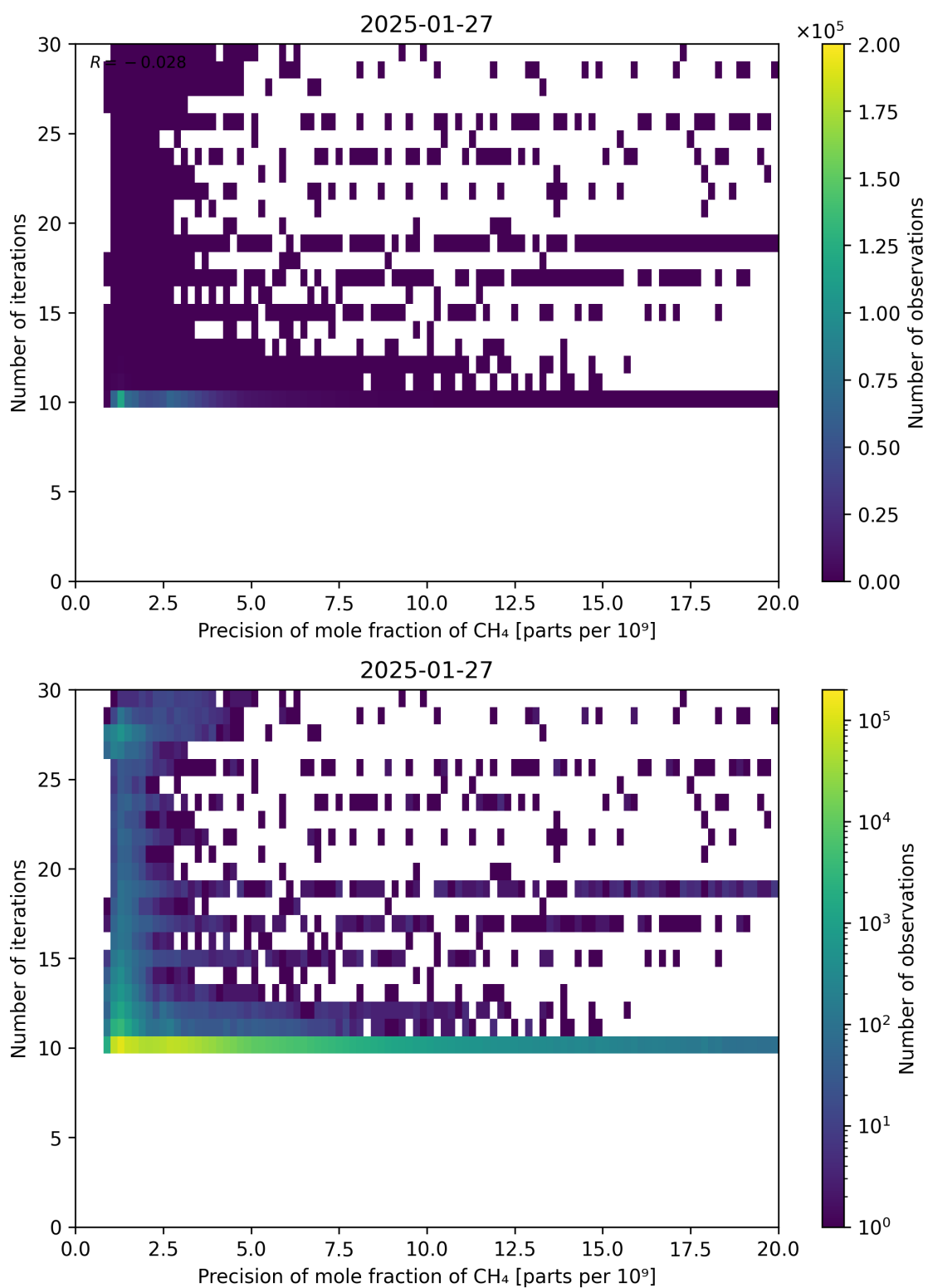
Figure 83: Scatter density plot of “Precision of mole fraction of CH 4 ” against “Number of iterations” for 2025-01-26 to 2025-01-28.
