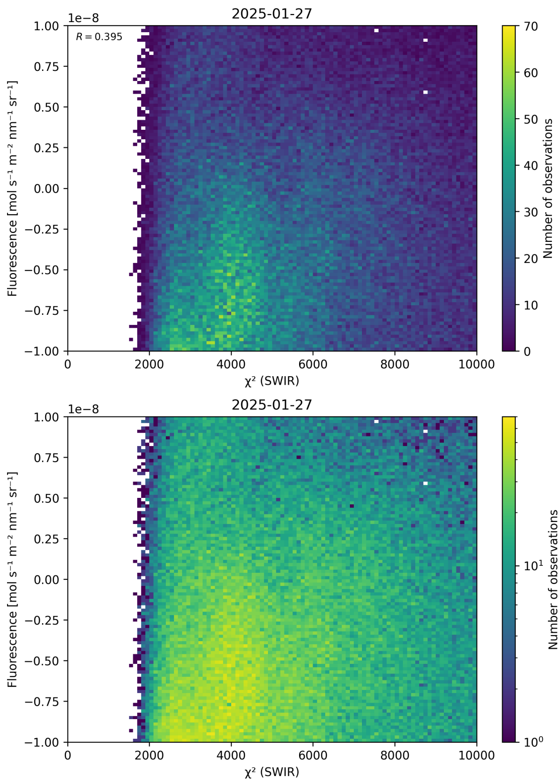
Figure 49: Scatter density plot of “ \chi^2 (SWIR)” against “Fluorescence” for 2025-01-26 to 2025-01-28.
