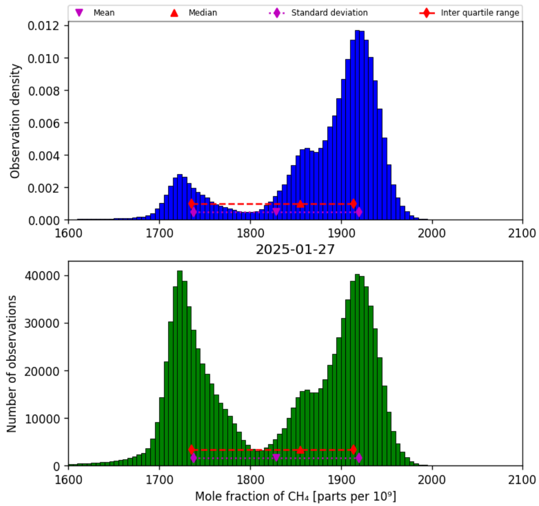
Figure 23: Histogram of “Mole fraction of CH 4 ” for 2025-01-26 to 2025-01-28
