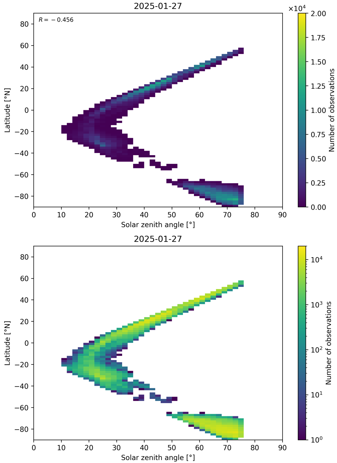
Figure 98: Scatter density plot of “Solar zenith angle” against “Latitude” for 2025-01-26 to 2025-01-28.
