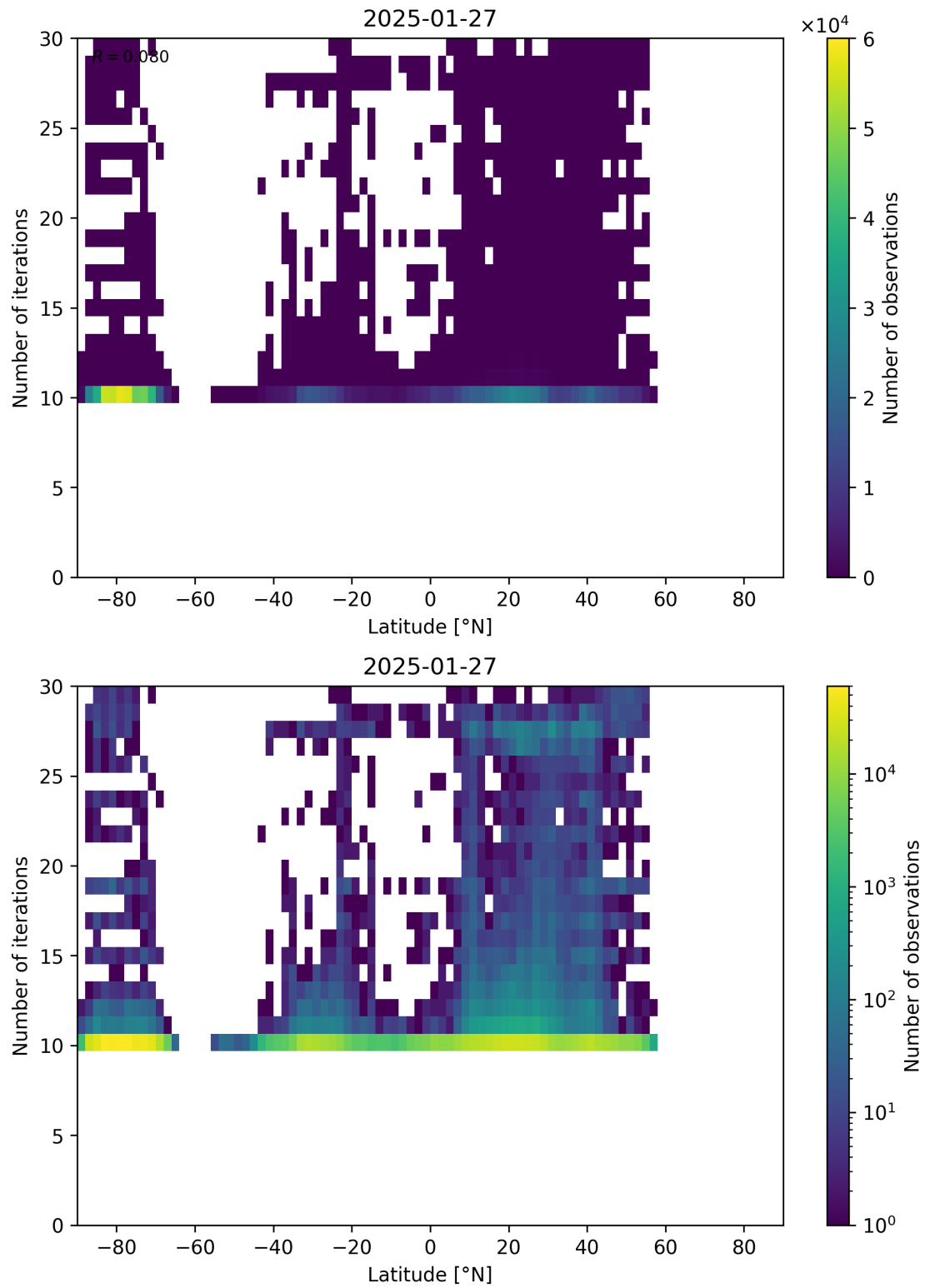
Figure 60: Scatter density plot of “Latitude” against “Number of iterations” for 2025-01-26 to 2025-01-28.
