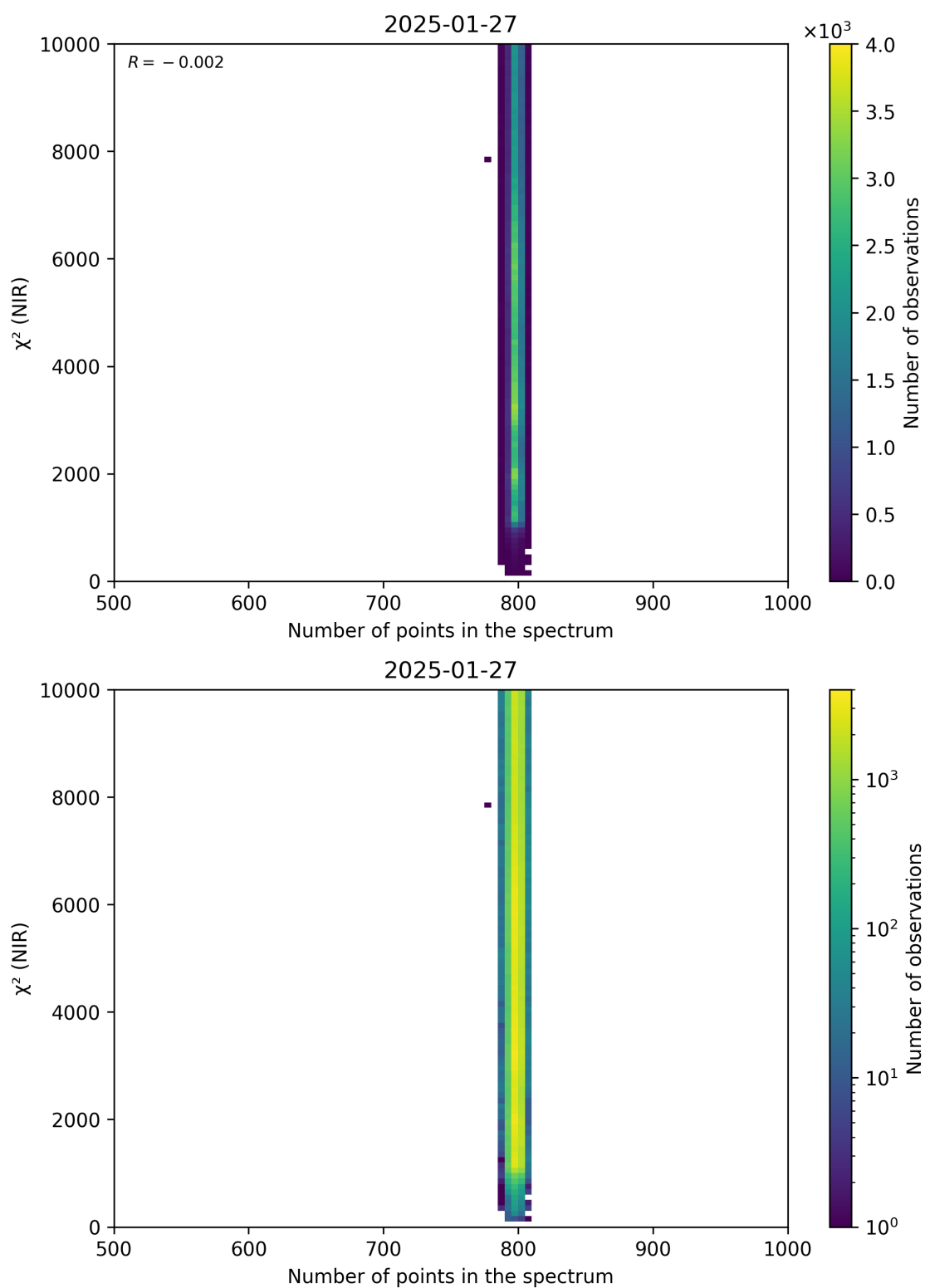
Figure 88: Scatter density plot of “Number of points in the spectrum” against “ \chi^2 (NIR)” for 2025-01-26 to 2025-01-28.
