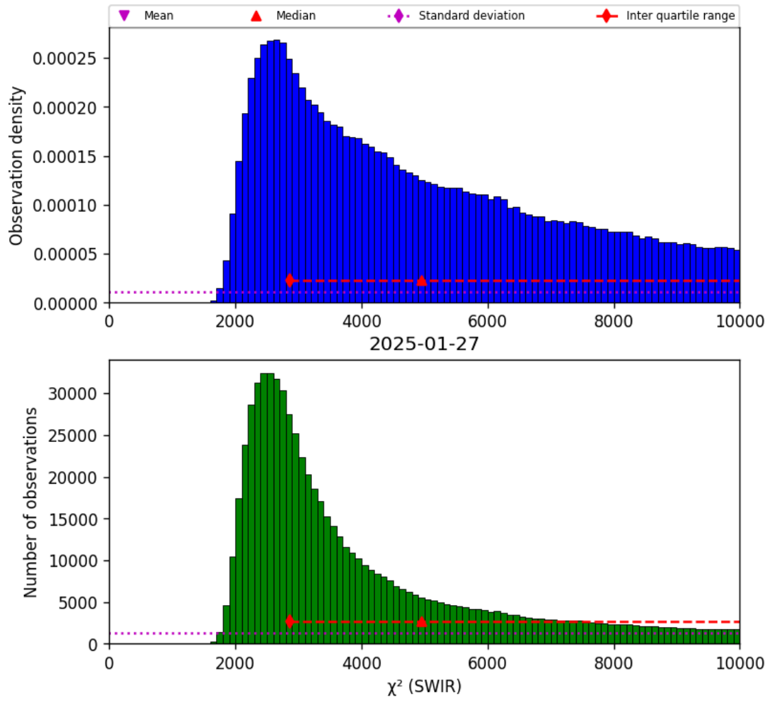
Figure 28: Histogram of “ \chi^2 (SWIR)” for 2025-01-26 to 2025-01-28
