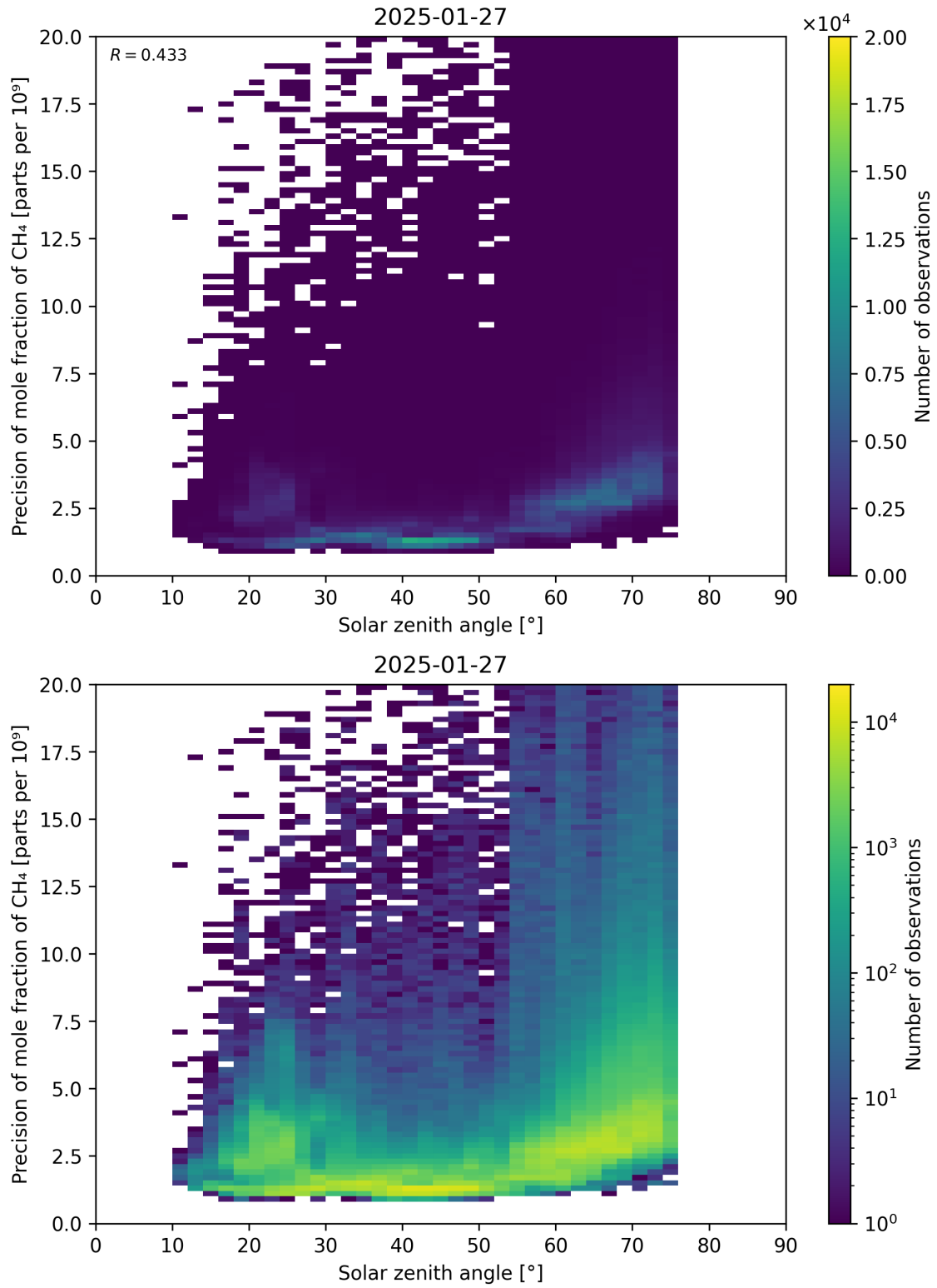
Figure 101: Scatter density plot of “Solar zenith angle” against “Precision of mole fraction of \text{CH}_4 ” for 2025-01-26 to 2025-01-28.
