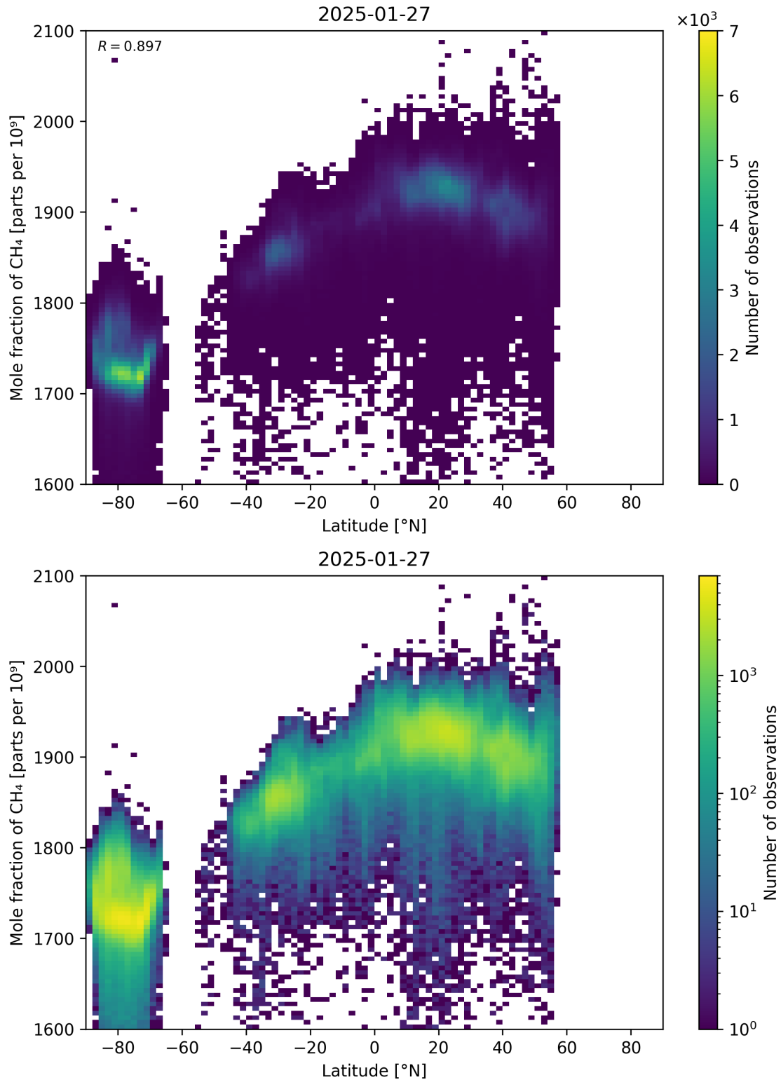
Figure 57: Scatter density plot of “Latitude” against “Mole fraction of CH 4 ” for 2025-01-26 to 2025-01-28.
