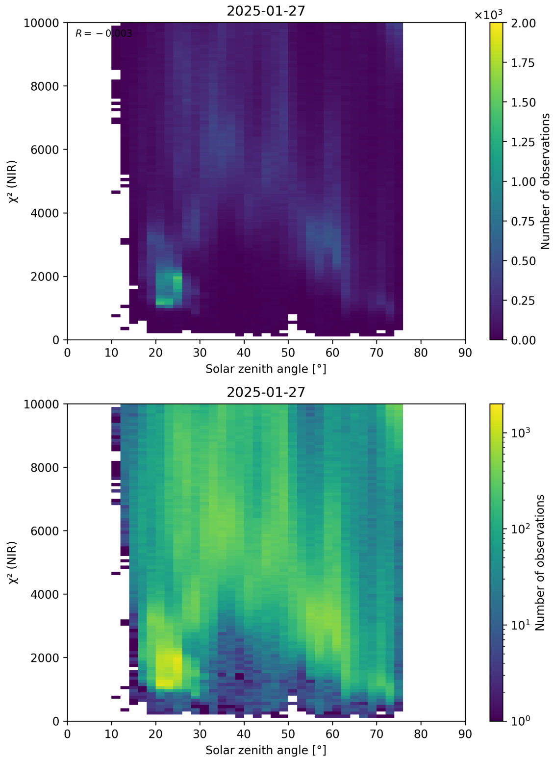
Figure 94: Scatter density plot of “Solar zenith angle” against “ \chi^2 (NIR)” for 2025-01-26 to 2025-01-28.
