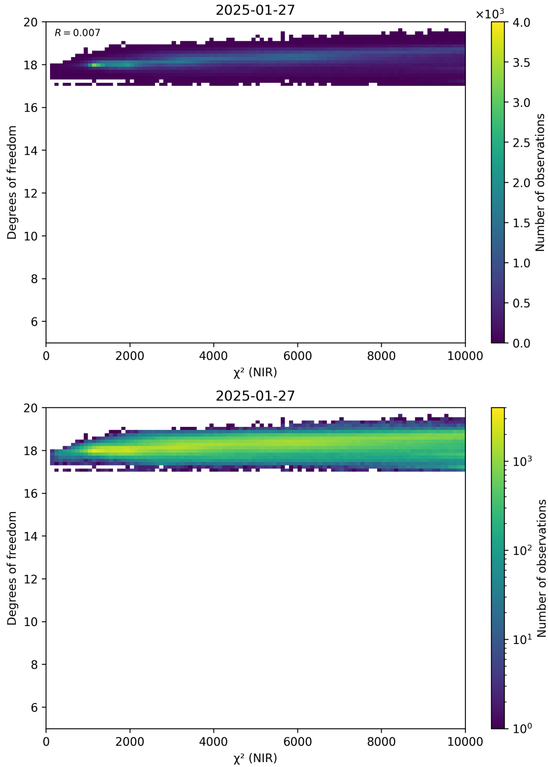
Figure 44: Scatter density plot of “ \chi^2 (NIR)” against “Degrees of freedom” for 2025-01-26 to 2025-01-28.
