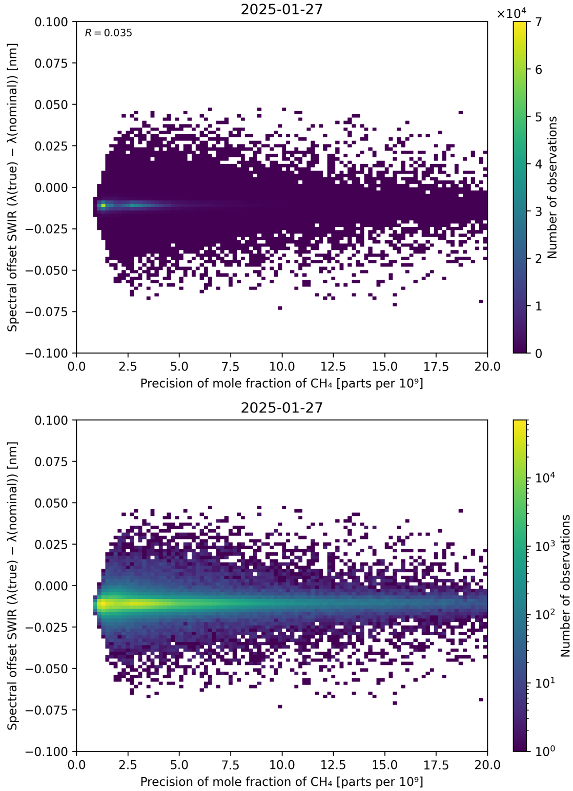
Figure 85: Scatter density plot of “Precision of mole fraction of \text{CH}_4 ” against “Spectral offset SWIR ( \lambda_{\text{true}} - \lambda_{\text{nominal}} )” for 2025-01-26 to 2025-01-28.
