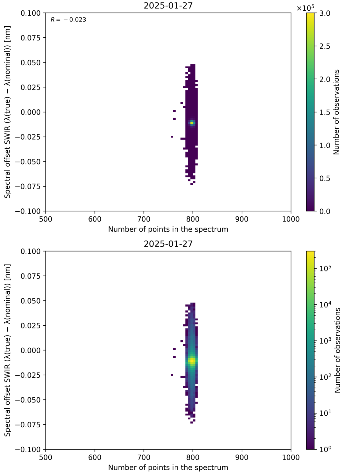
Figure 93: Scatter density plot of “Number of points in the spectrum” against “Spectral offset SWIR ( \lambda_{\text{true}} - \lambda_{\text{nominal}} )” for 2025-01-26 to 2025-01-28.
