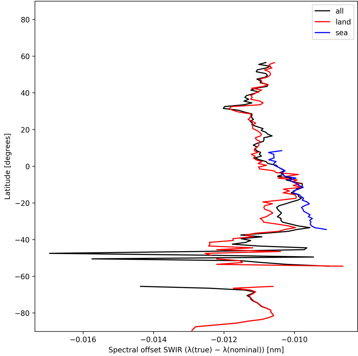
Figure 16: Zonal average of “Spectral offset SWIR ( \lambda_{\text{true}} - \lambda_{\text{nominal}} )” for 2025-01-26 to 2025-01-28.
