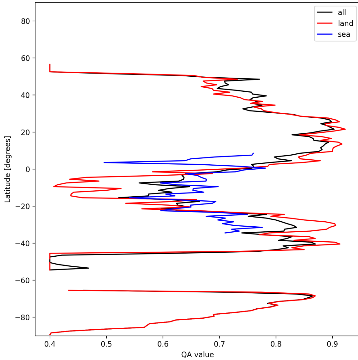
Figure 11: Zonal average of “QA value” for 2025-01-26 to 2025-01-28.
