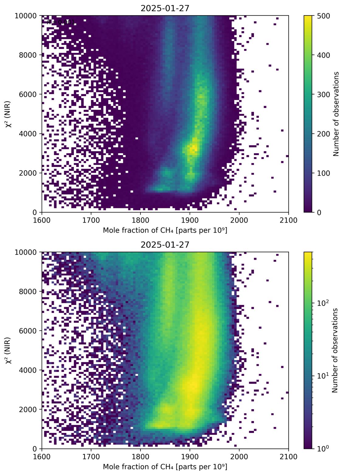
Figure 70: Scatter density plot of “Mole fraction of \text{CH}_4 ” against “ \chi^2 (NIR)” for 2025-01-26 to 2025-01-28.
