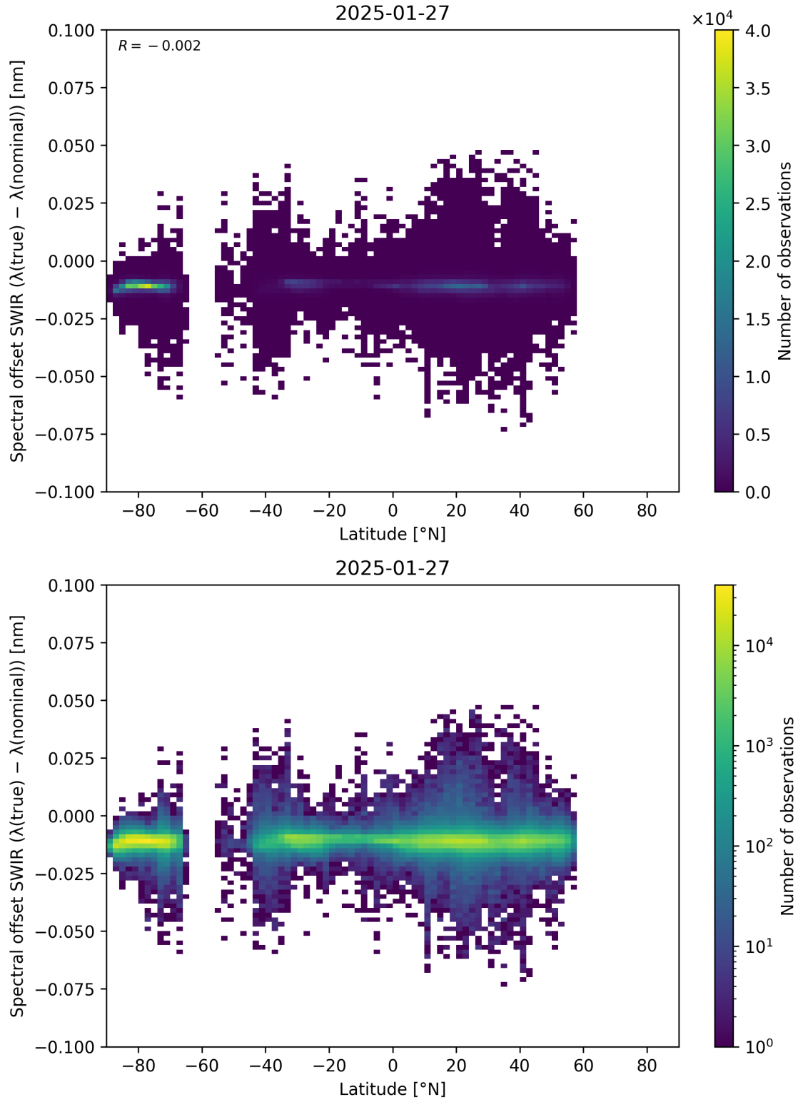
Figure 62: Scatter density plot of “Latitude” against “Spectral offset SWIR ( \lambda_{\text{true}} - \lambda_{\text{nominal}} )” for 2025-01-26 to 2025-01-28.
