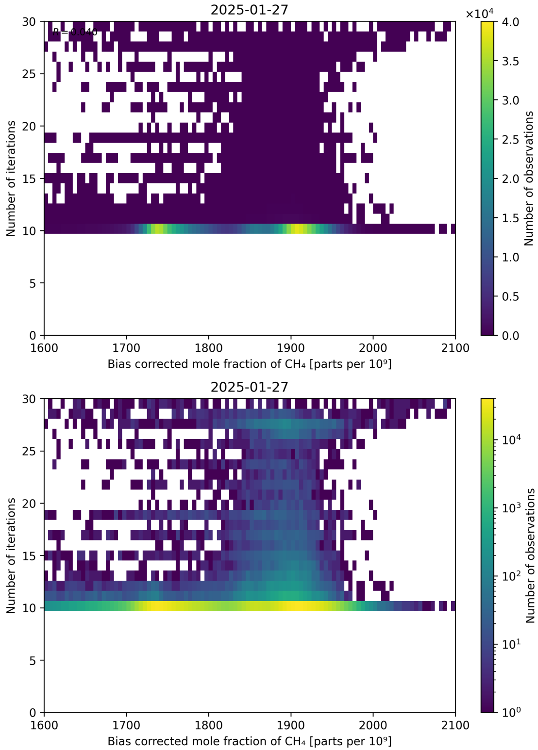
Figure 67: Scatter density plot of “Bias corrected mole fraction of \text{CH}_4 ” against “Number of iterations” for 2025-01-26 to 2025-01-28.
