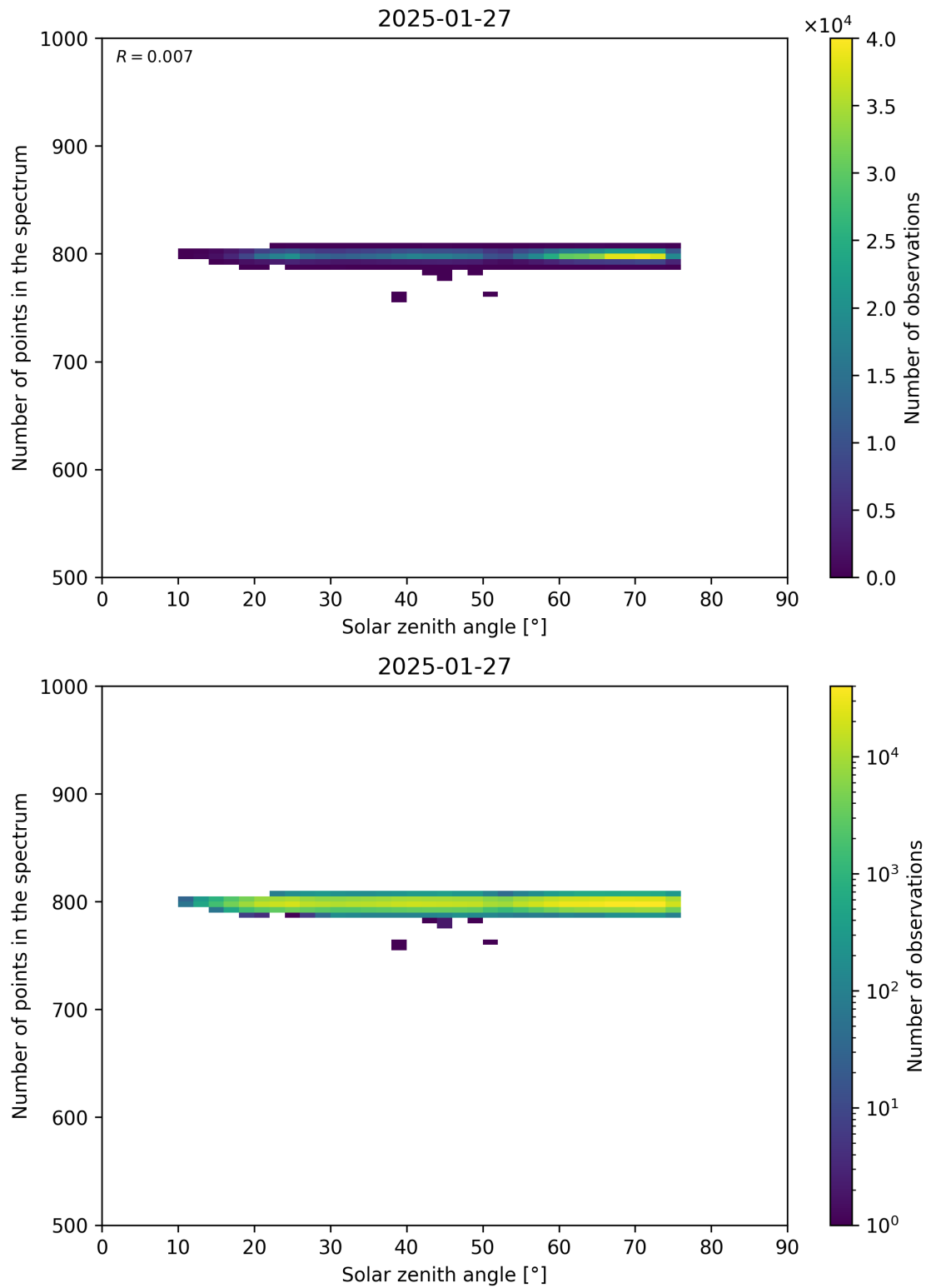
Figure 103: Scatter density plot of “Solar zenith angle” against “Number of points in the spectrum” for 2025-01-26 to 2025-01-28.
