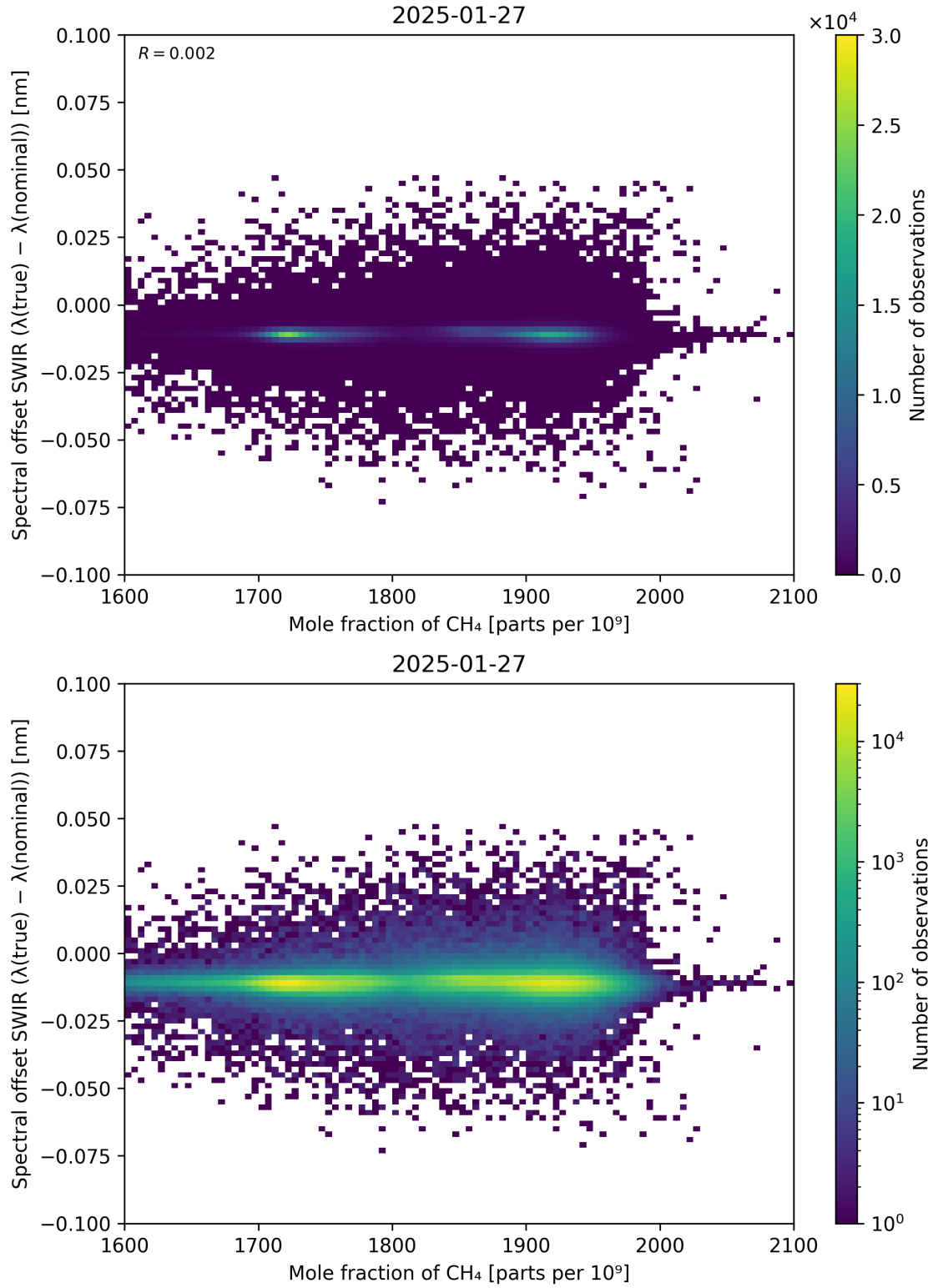
Figure 86: Scatter density plot of “Mole fraction of \text{CH}_4 ” against “Spectral offset SWIR ( \lambda_{\text{true}} - \lambda_{\text{nominal}} )” for 2025-01-26 to 2025-01-28.
