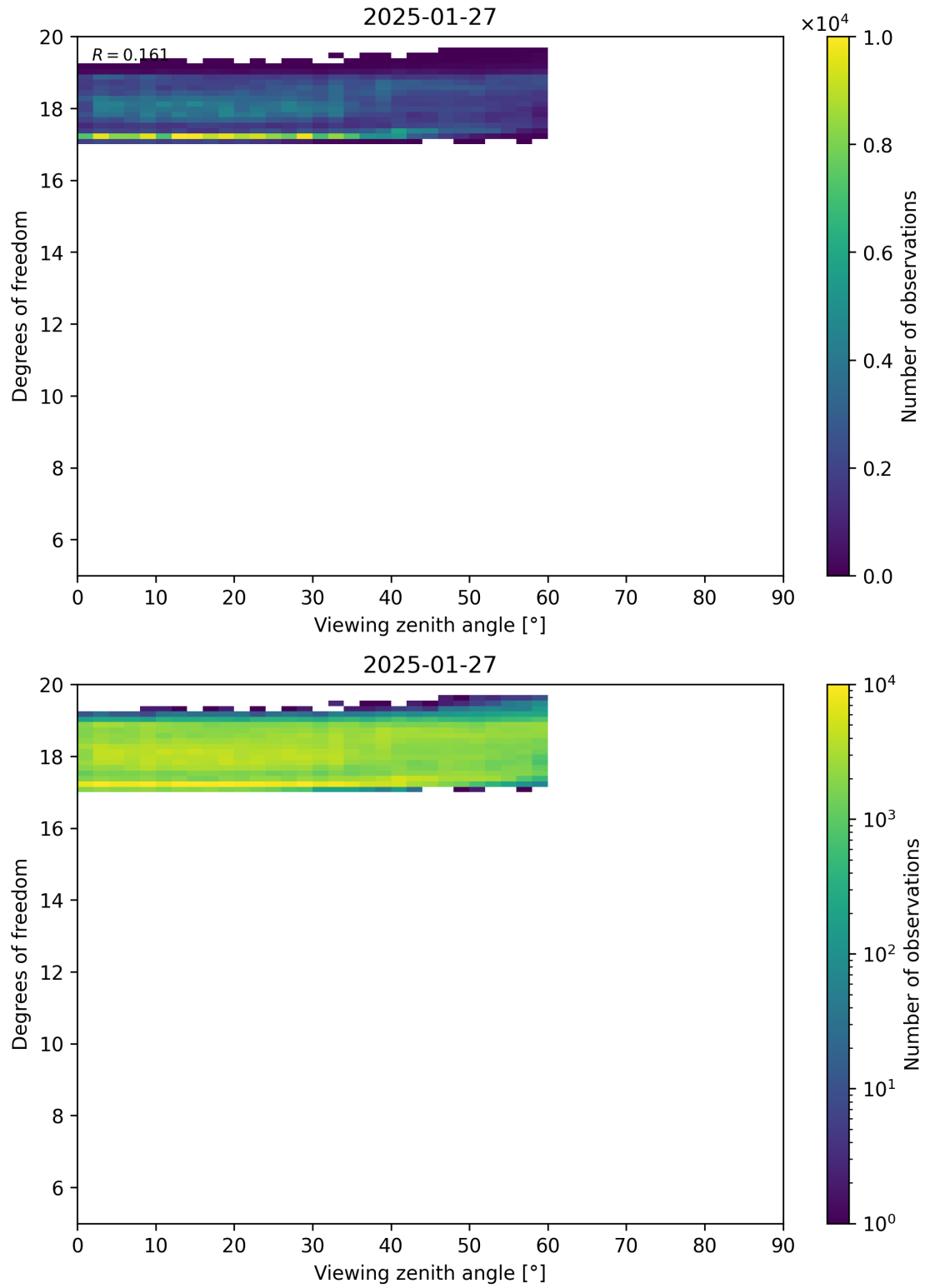
Figure 107: Scatter density plot of “Viewing zenith angle” against “Degrees of freedom” for 2025-01-26 to 2025-01-28.
