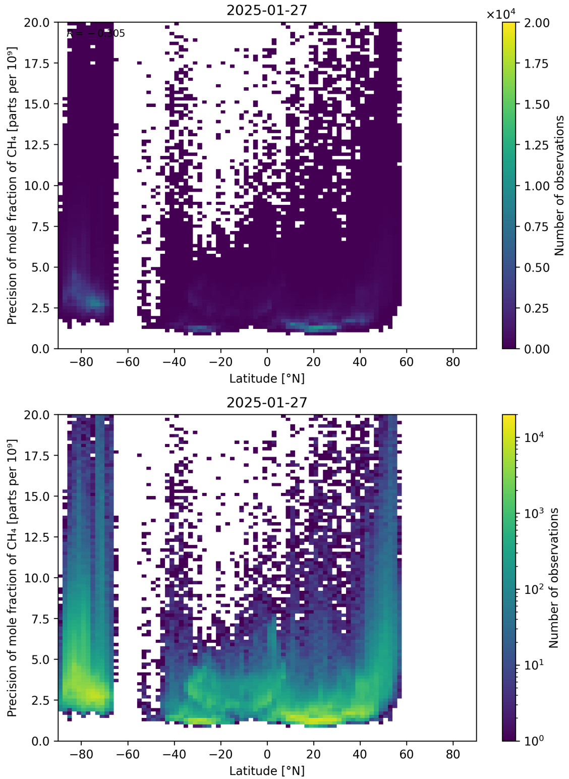
Figure 59: Scatter density plot of “Latitude” against “Precision of mole fraction of CH 4 ” for 2025-01-26 to 2025-01-28.
