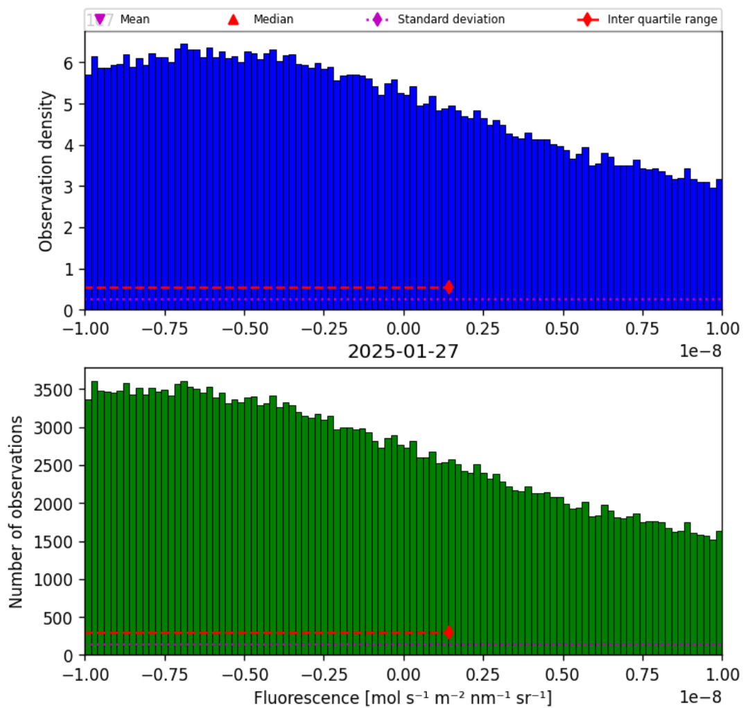
Figure 32: Histogram of “Fluorescence” for 2025-01-26 to 2025-01-28
