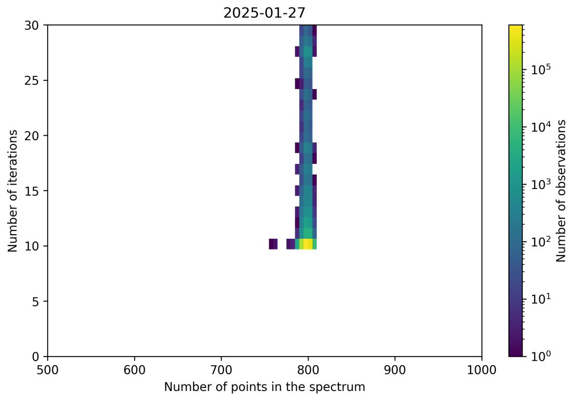
Figure 92: Scatter density plot of “Number of points in the spectrum” against “Number of iterations” for 2025-01-26 to 2025-01-28.
