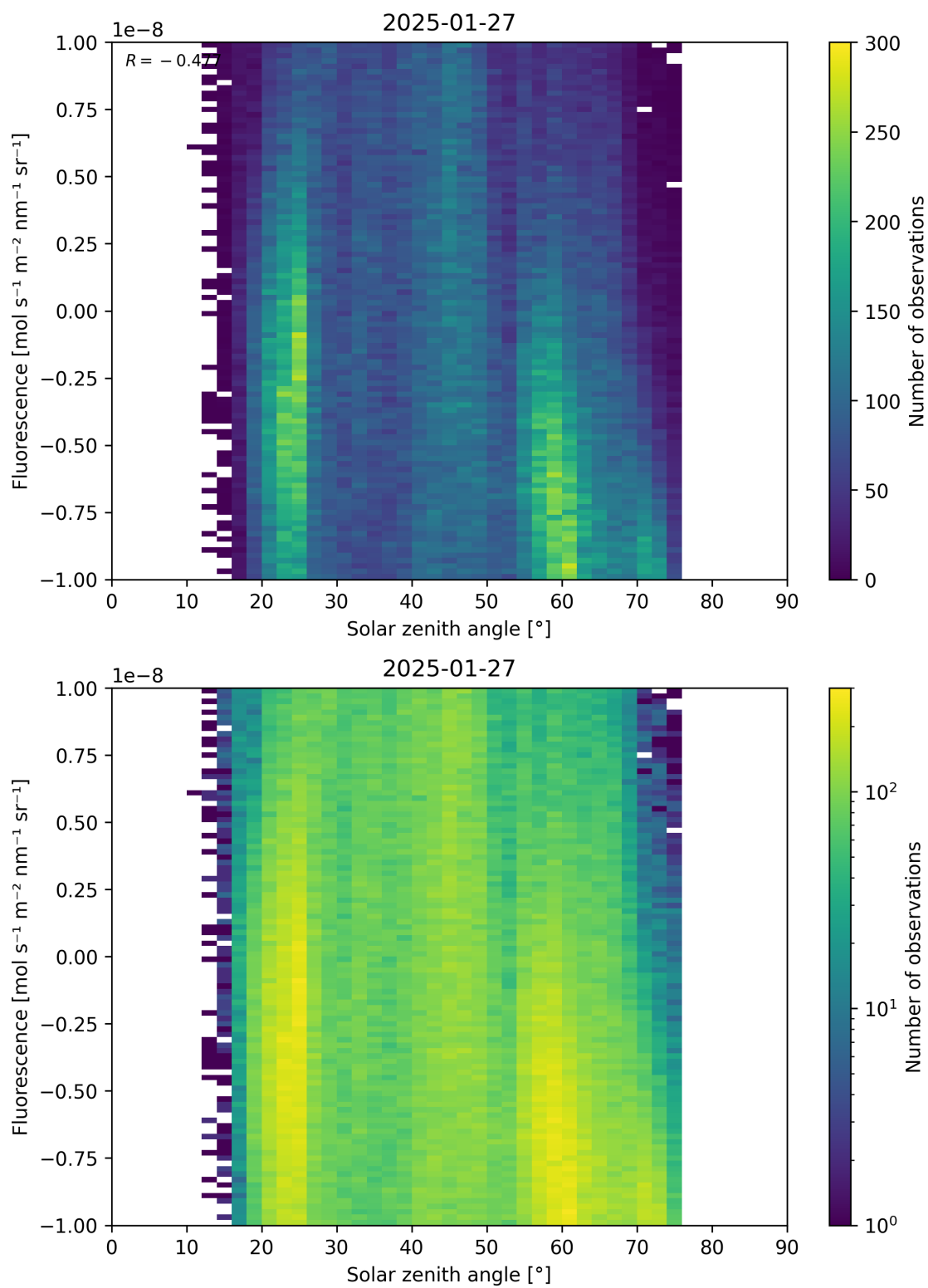
Figure 97: Scatter density plot of “Solar zenith angle” against “Fluorescence” for 2025-01-26 to 2025-01-28.
