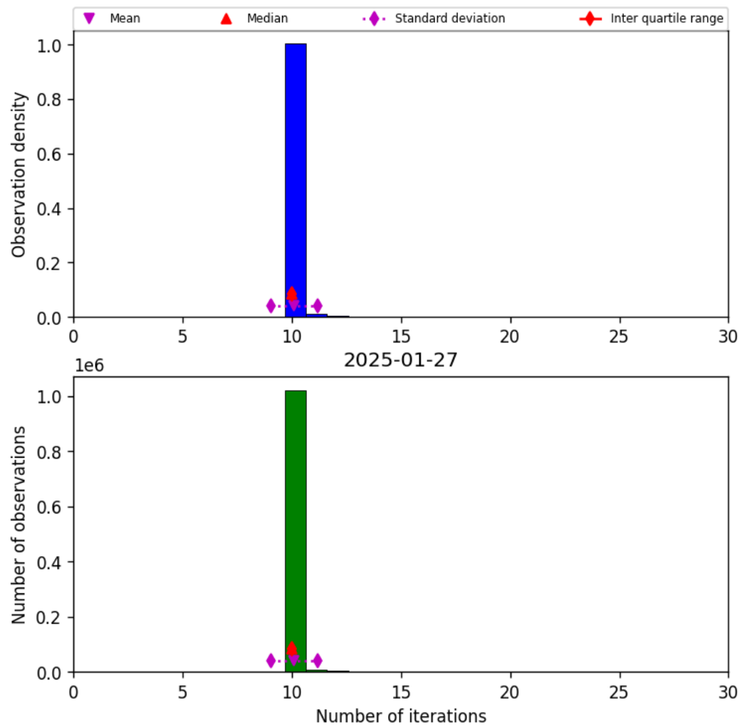
Figure 31: Histogram of "Number of iterations" for 2025-01-26 to 2025-01-28
