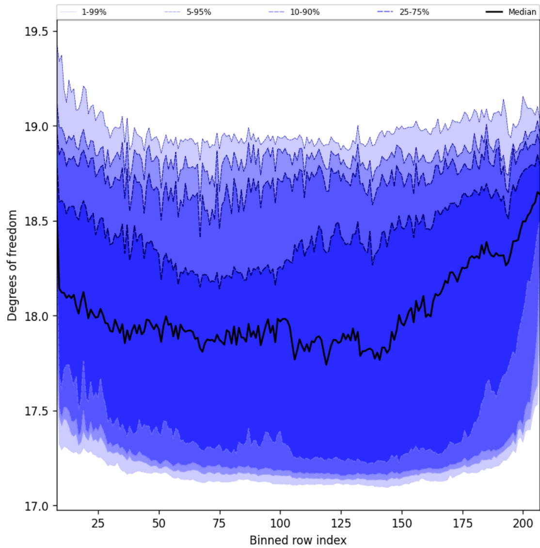
Figure 41: Along track statistics of “Degrees of freedom” for 2025-01-26 to 2025-01-28
