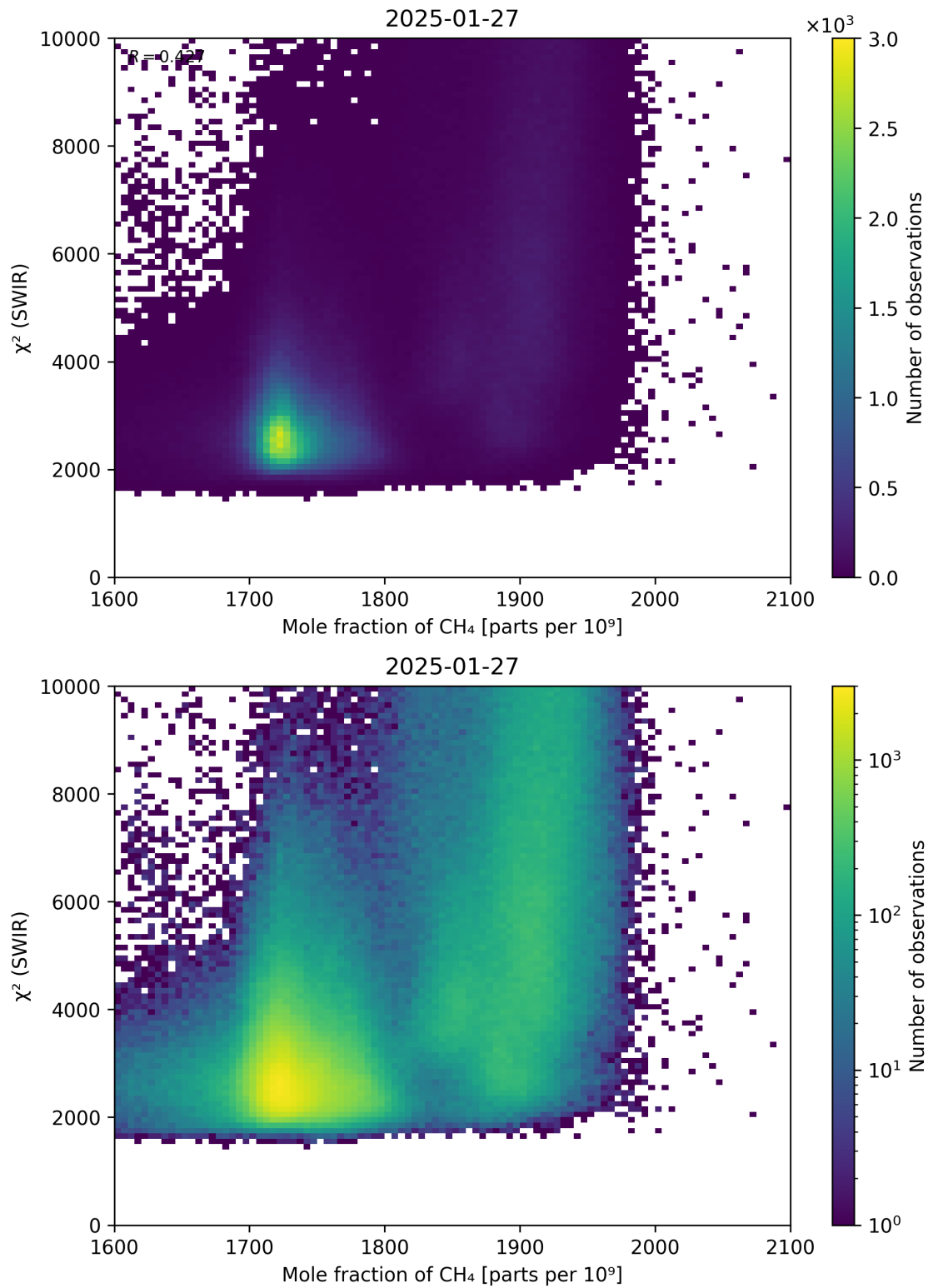
Figure 71: Scatter density plot of “Mole fraction of \text{CH}_4 ” against “ \chi^2 (SWIR)” for 2025-01-26 to 2025-01-28.
