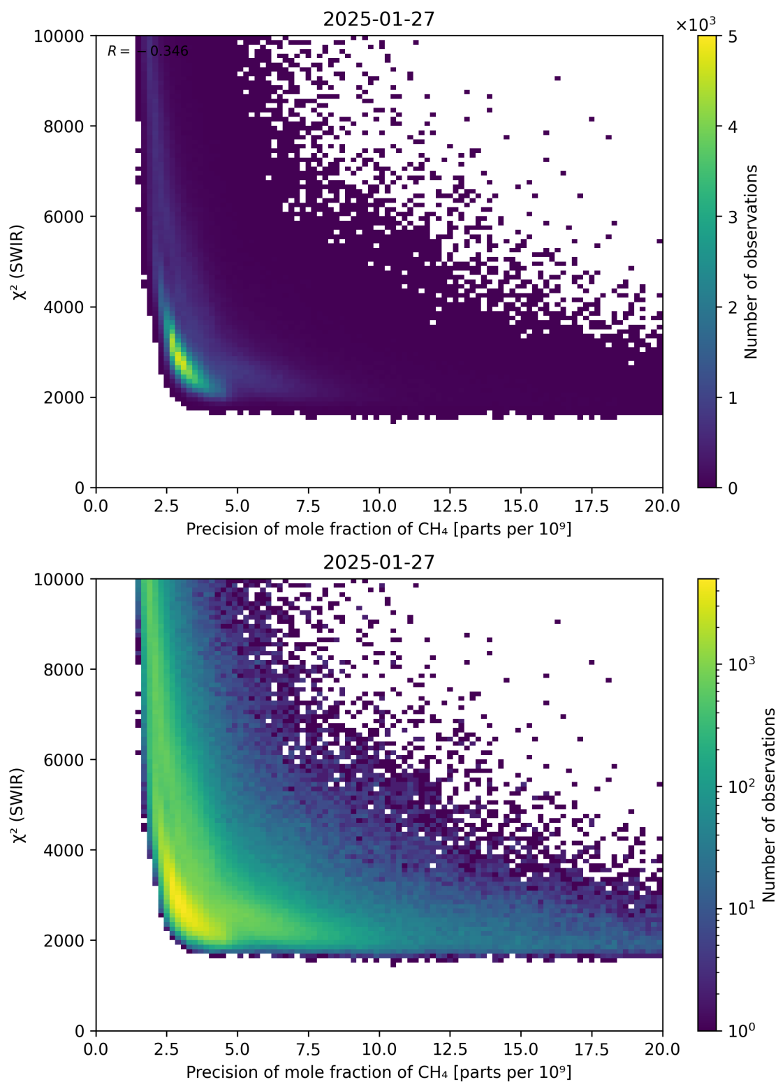
Figure 79: Scatter density plot of “Precision of mole fraction of \text{CH}_4 ” against “ \chi^2 (SWIR)” for 2025-01-26 to 2025-01-28.
