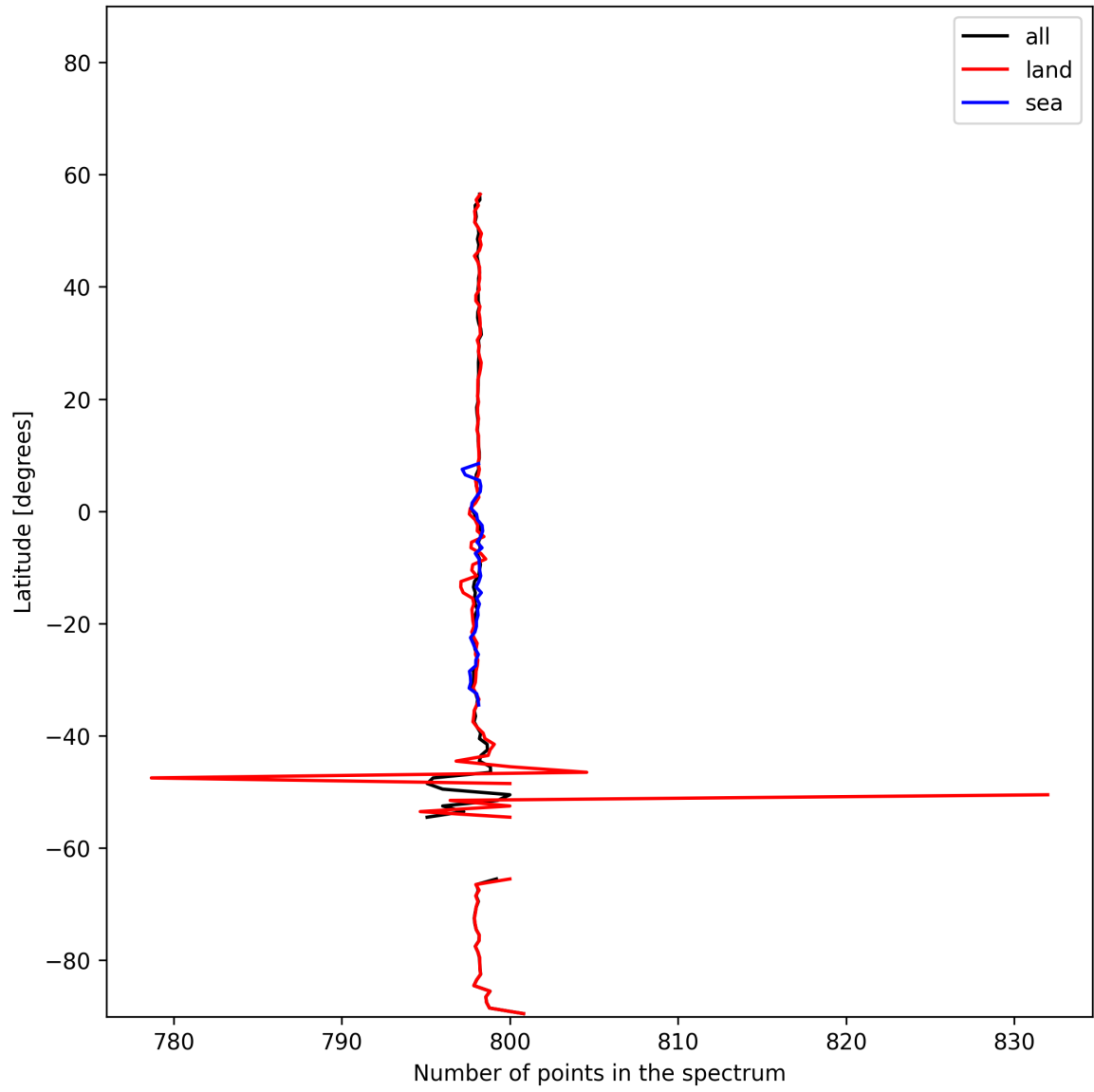
Figure 15: Zonal average of “Number of points in the spectrum” for 2025-01-26 to 2025-01-28.
