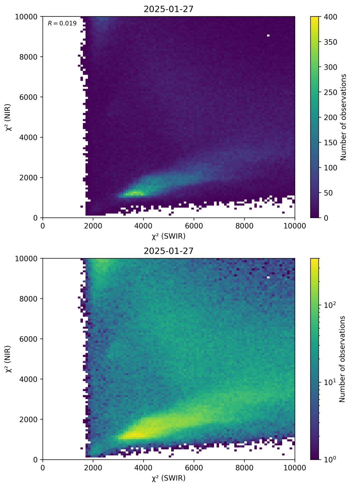
Figure 47: Scatter density plot of “ \chi^2 (SWIR)” against “ \chi^2 (NIR)” for 2025-01-26 to 2025-01-28.
