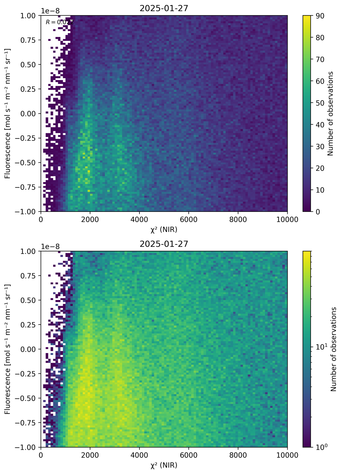
Figure 45: Scatter density plot of “ \chi^2 (NIR)” against “Fluorescence” for 2025-01-26 to 2025-01-28.
