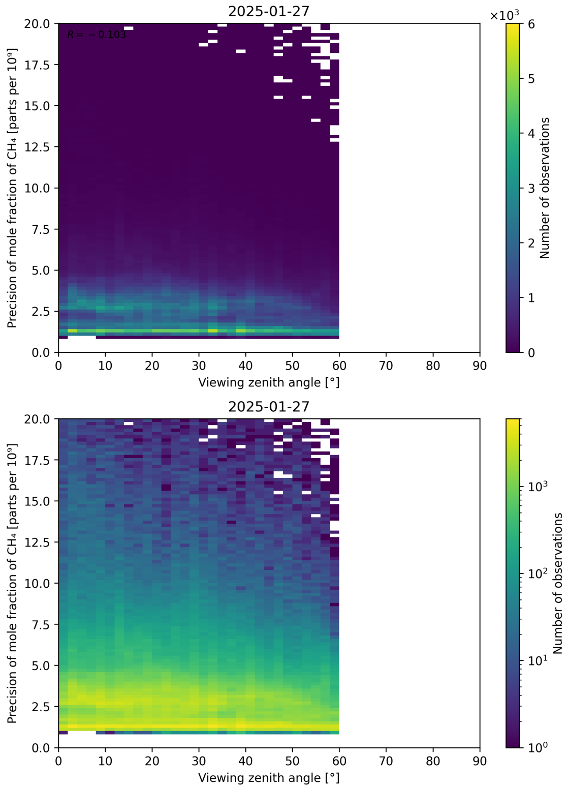
Figure 112: Scatter density plot of “Viewing zenith angle” against “Precision of mole fraction of CH 4 ” for 2025-01-26 to 2025-01-28.
