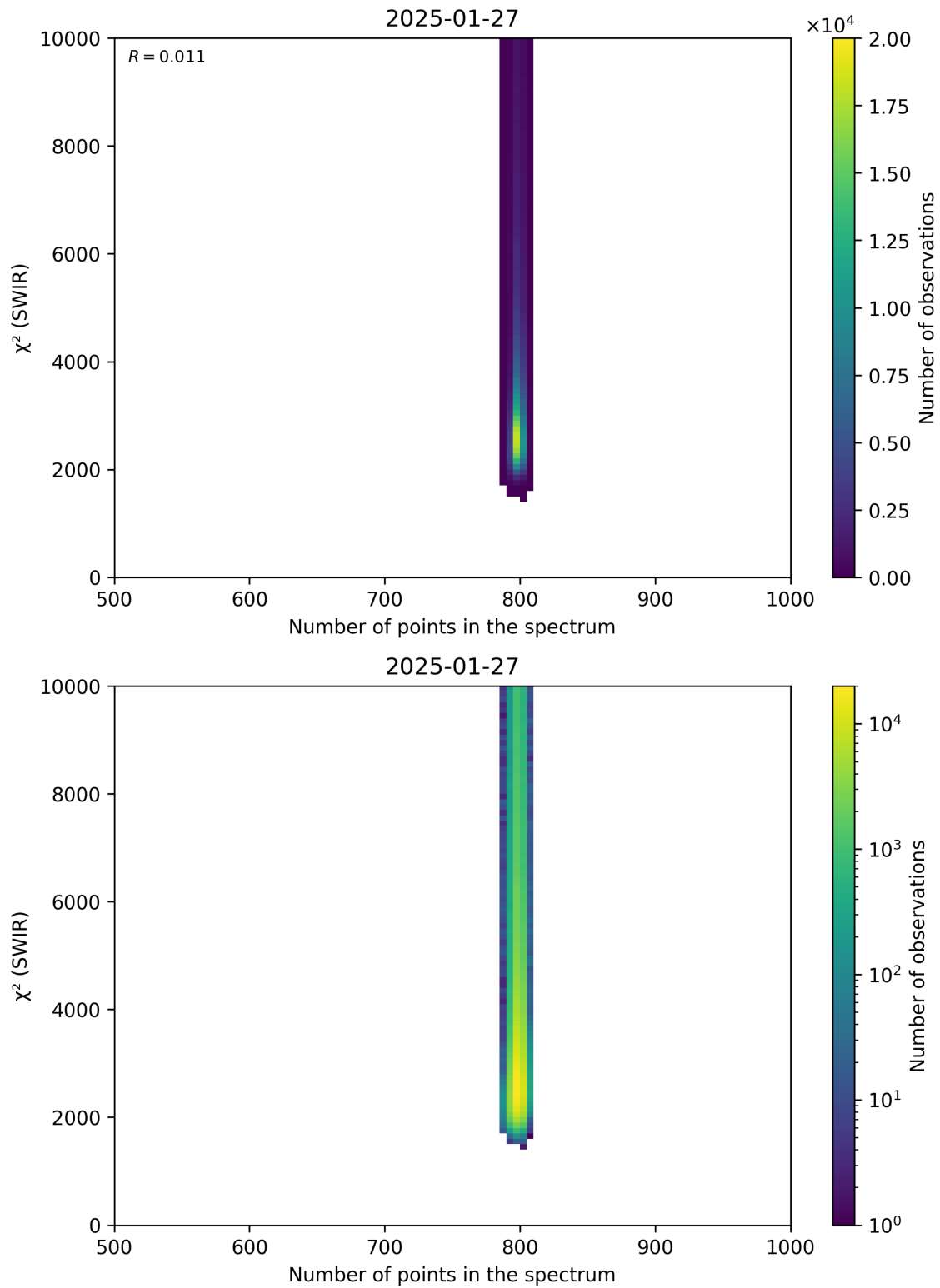
Figure 89: Scatter density plot of “Number of points in the spectrum” against “ \chi^2 (SWIR)” for 2025-01-26 to 2025-01-28.
