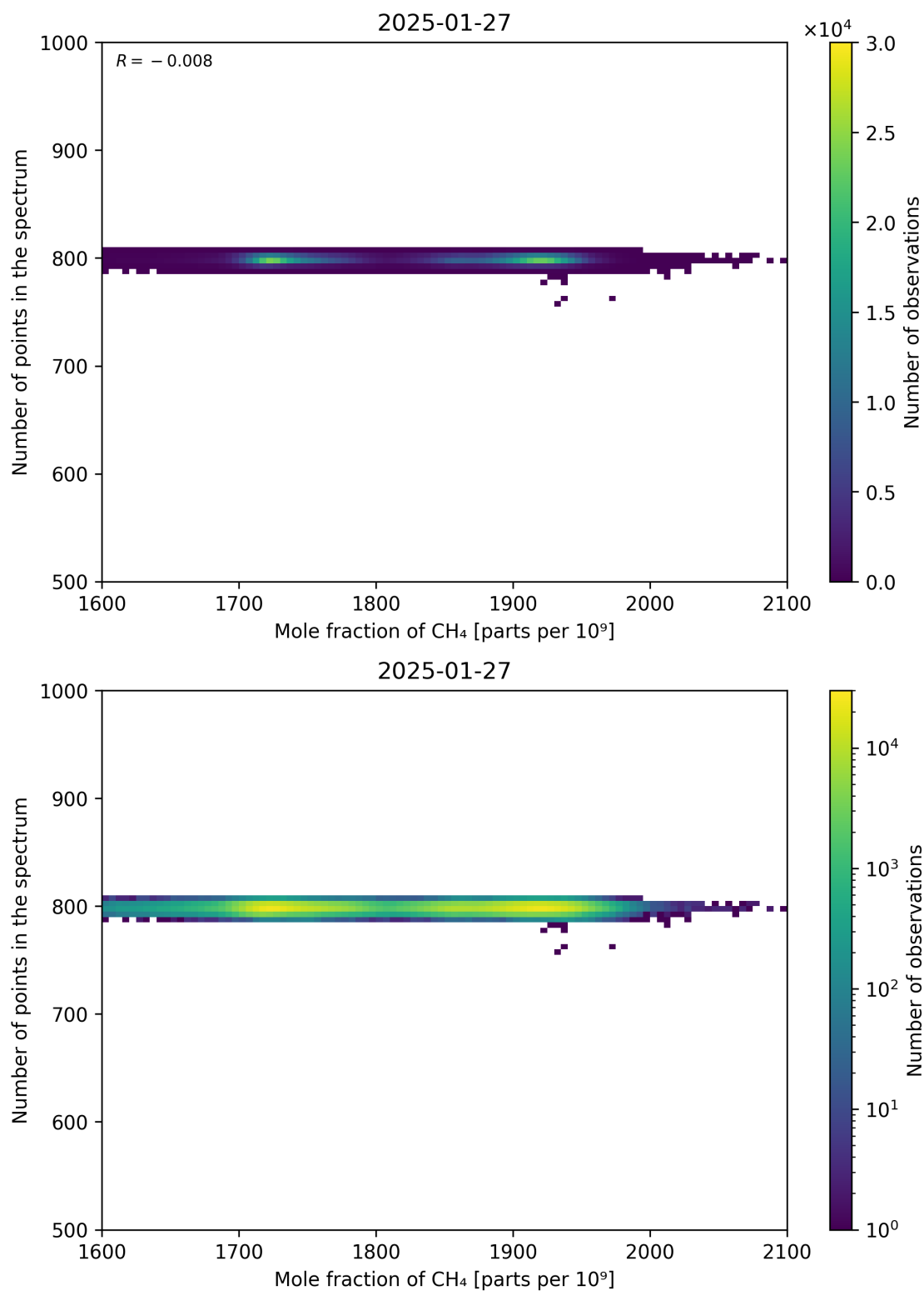
Figure 77: Scatter density plot of “Mole fraction of CH 4 ” against “Number of points in the spectrum” for 2025-01-26 to 2025-01-28.
