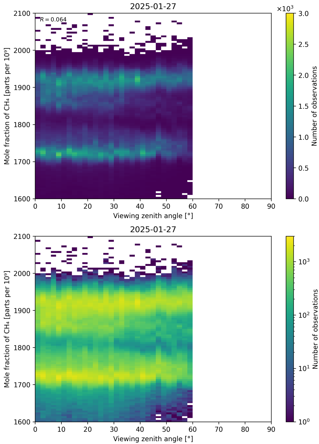
Figure 110: Scatter density plot of “Viewing zenith angle” against “Mole fraction of CH 4 ” for 2025-01-26 to 2025-01-28.
