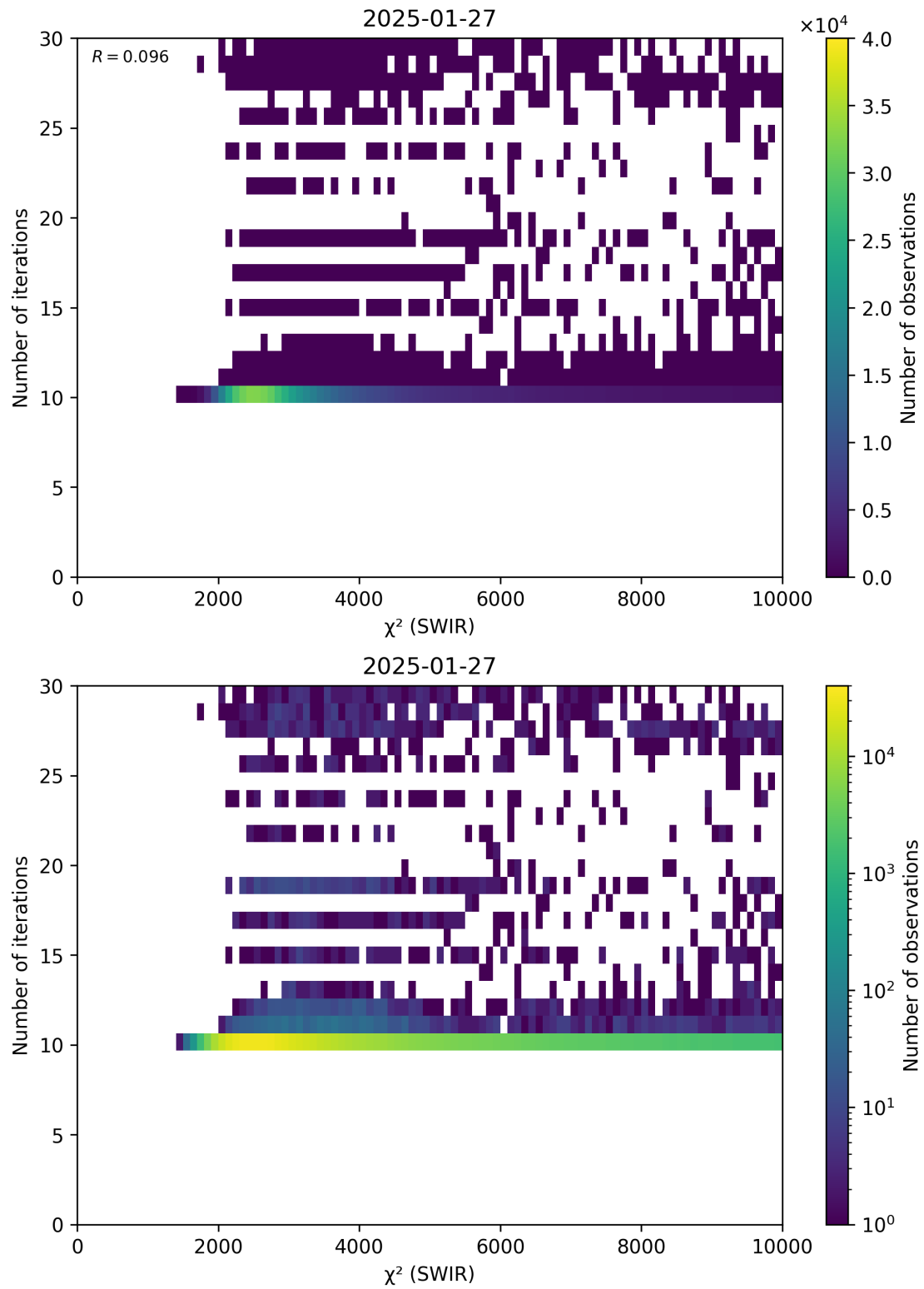
Figure 50: Scatter density plot of “ \chi^2 (SWIR)” against “Number of iterations” for 2025-01-26 to 2025-01-28.
