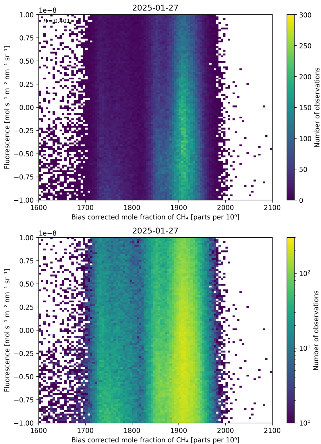
Figure 66: Scatter density plot of “Bias corrected mole fraction of \text{CH}_4 ” against “Fluorescence” for 2025-01-26 to 2025-01-28.
