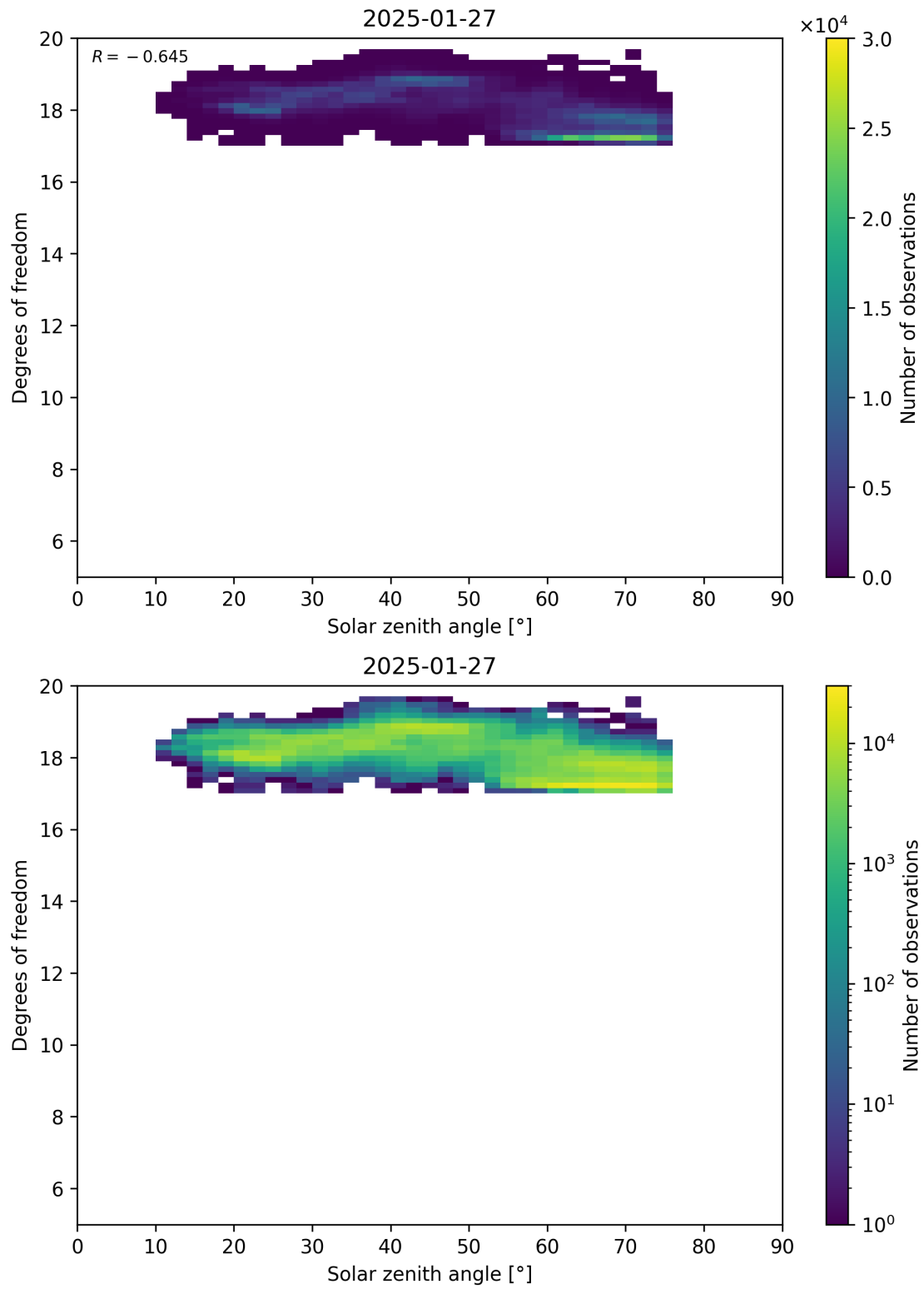
Figure 96: Scatter density plot of “Solar zenith angle” against “Degrees of freedom” for 2025-01-26 to 2025-01-28.
