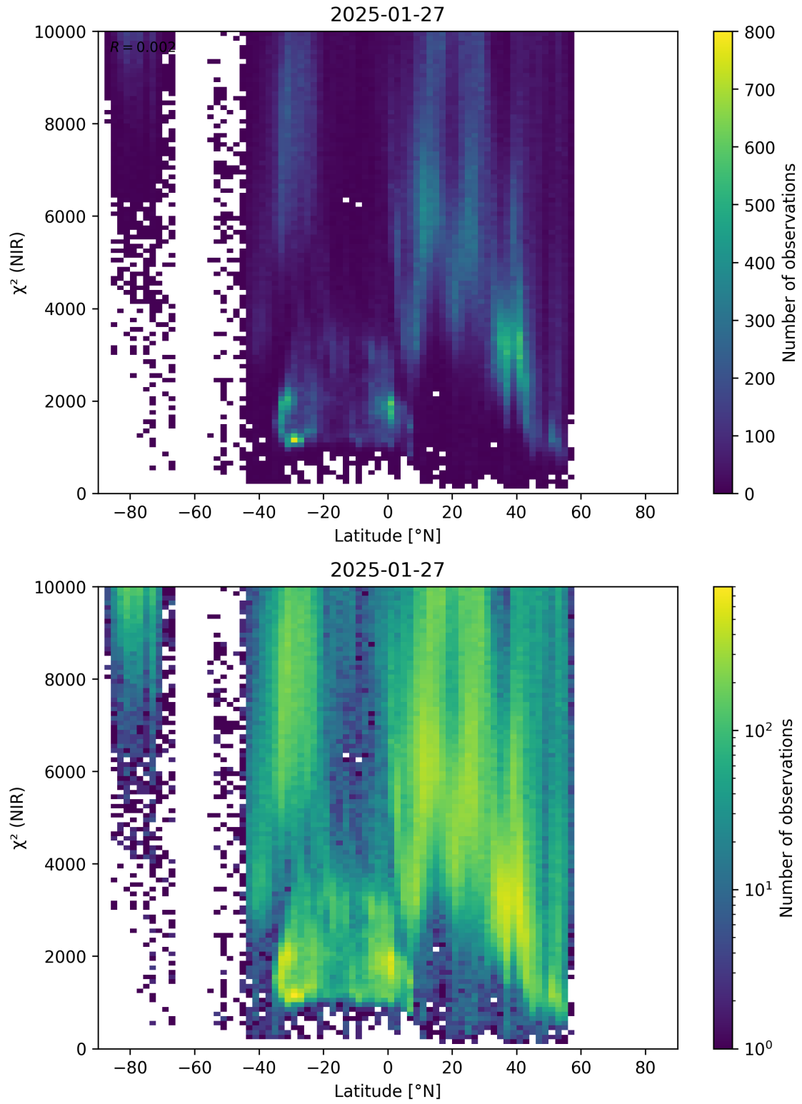
Figure 53: Scatter density plot of “Latitude” against “ \chi^2 (NIR)” for 2025-01-26 to 2025-01-28.
