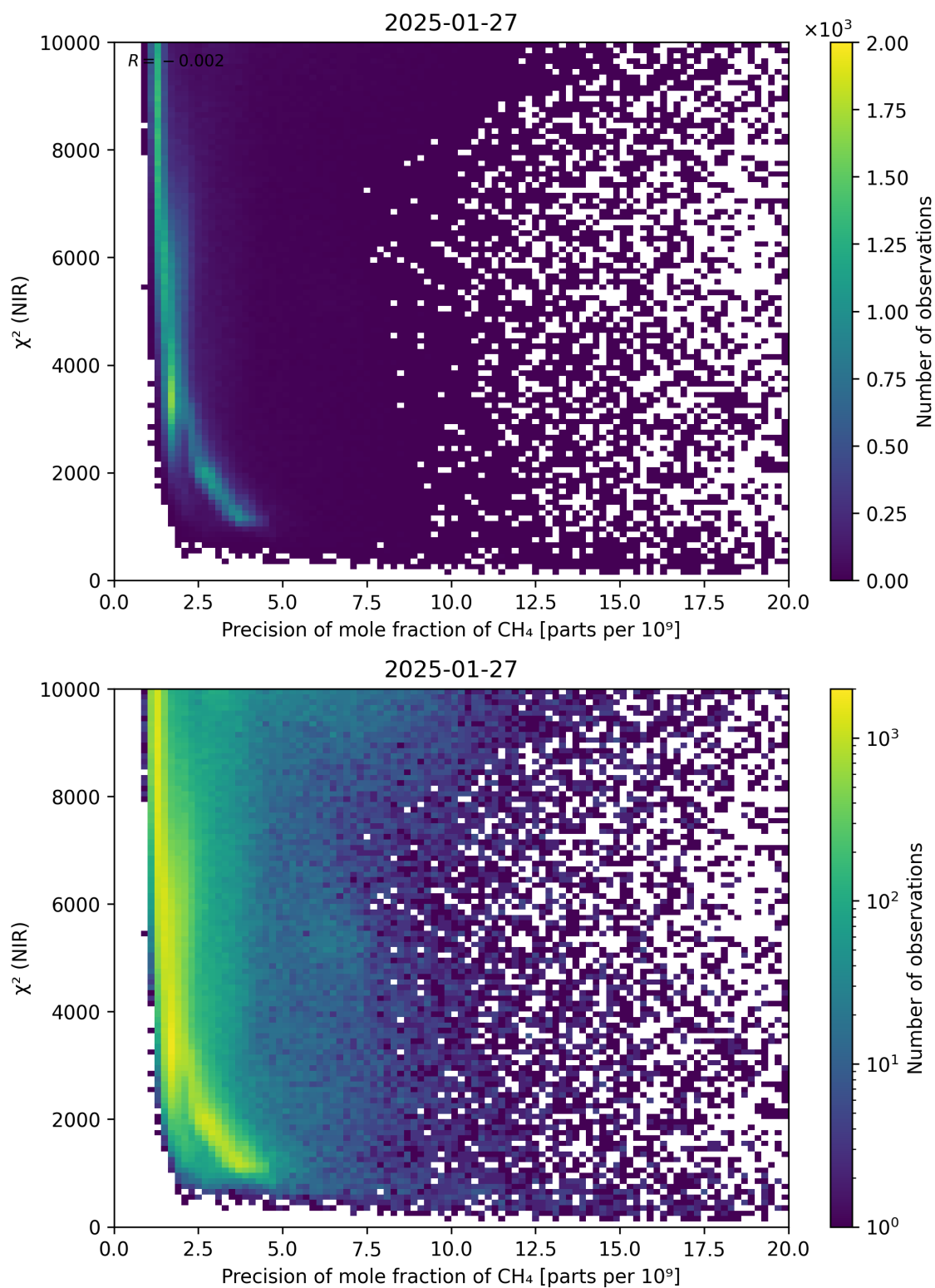
Figure 78: Scatter density plot of “Precision of mole fraction of CH 4 ” against “ \chi^2 (NIR)” for 2025-01-26 to 2025-01-28.
