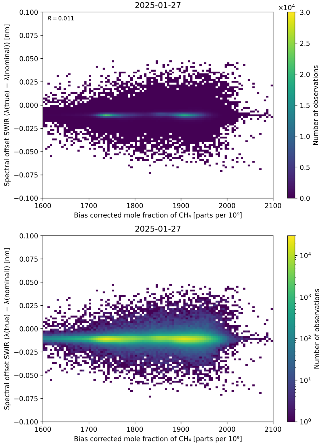
Figure 69: Scatter density plot of “Bias corrected mole fraction of \text{CH}_4 ” against “Spectral offset SWIR ( \lambda_{\text{true}} - \lambda_{\text{nominal}} )” for 2025-01-26 to 2025-01-28.
