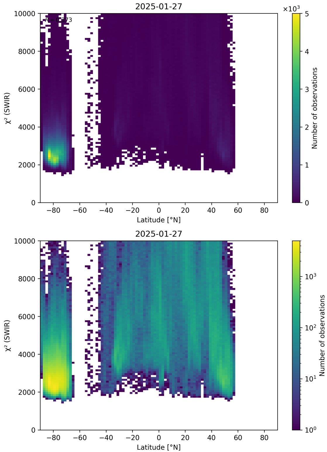
Figure 54: Scatter density plot of “Latitude” against “ \chi^2 (SWIR)” for 2025-01-26 to 2025-01-28.
