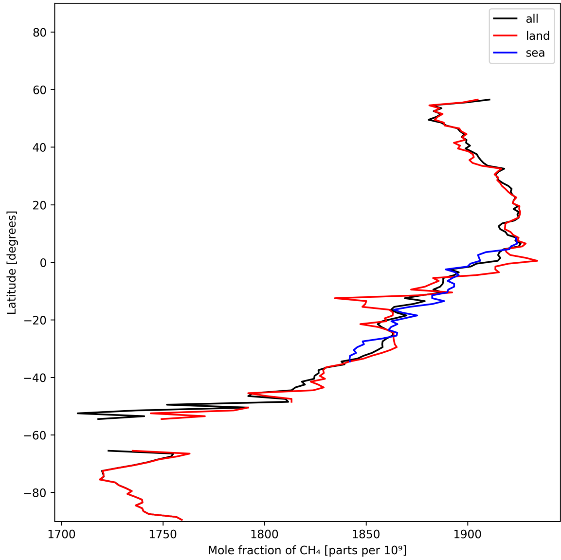
Figure 12: Zonal average of “Mole fraction of \text{CH}_4 ” for 2025-01-26 to 2025-01-28.
