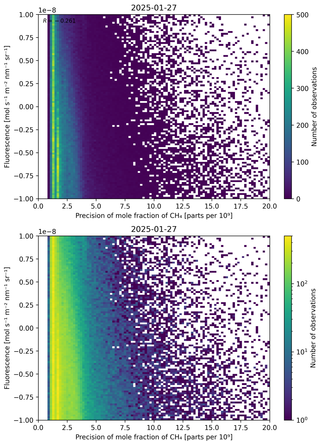
Figure 81: Scatter density plot of “Precision of mole fraction of CH 4 ” against “Fluorescence” for 2025-01-26 to 2025-01-28.
