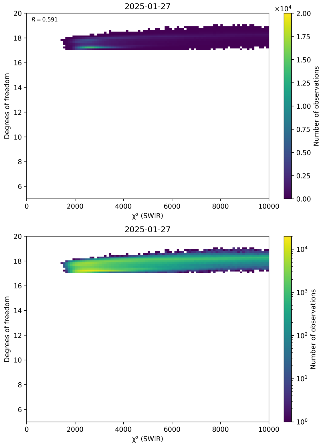
Figure 48: Scatter density plot of “ \chi^2 (SWIR)” against “Degrees of freedom” for 2025-01-26 to 2025-01-28.
