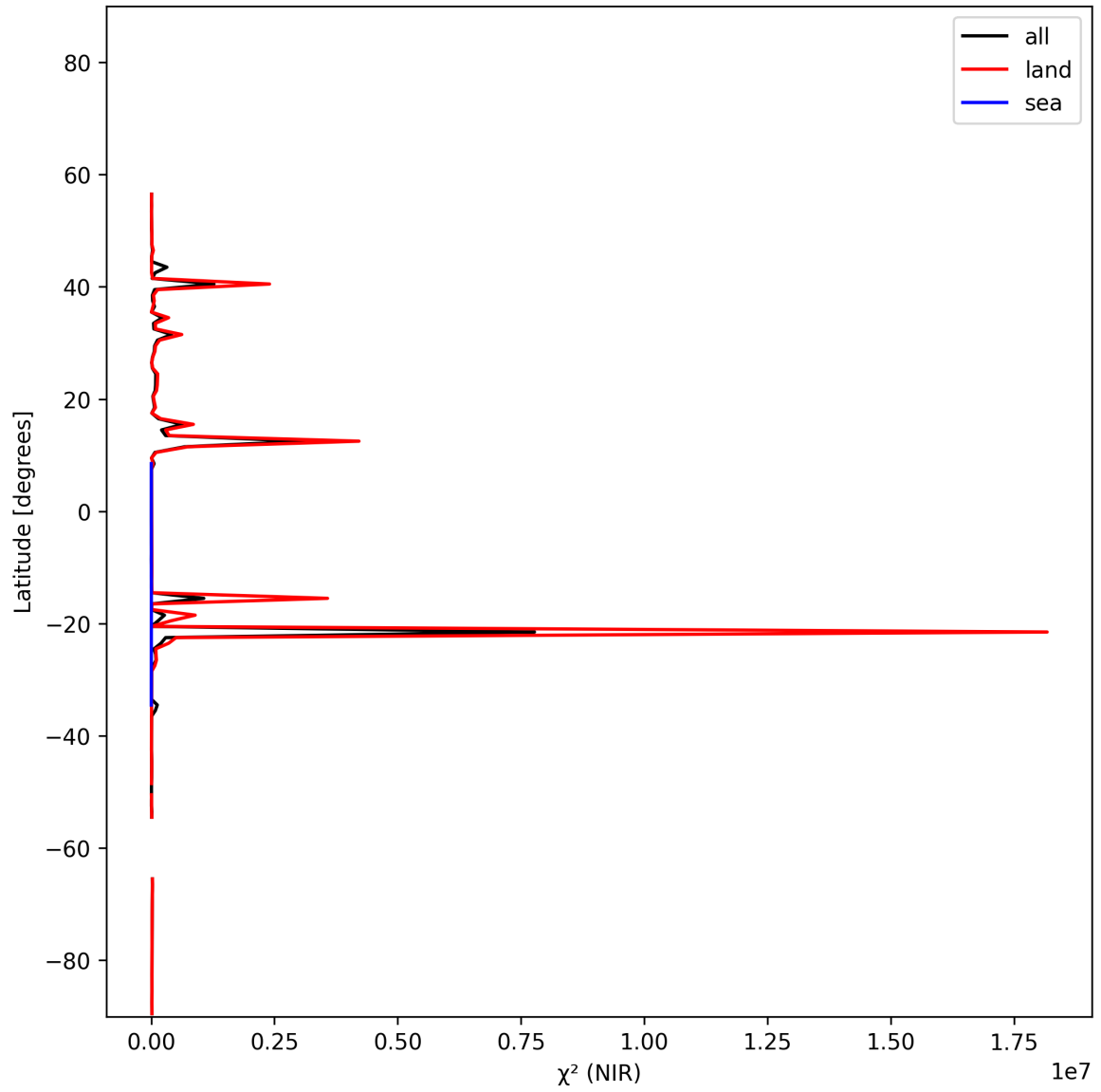
Figure 18: Zonal average of “ \chi^2 (NIR)” for 2025-01-26 to 2025-01-28.
