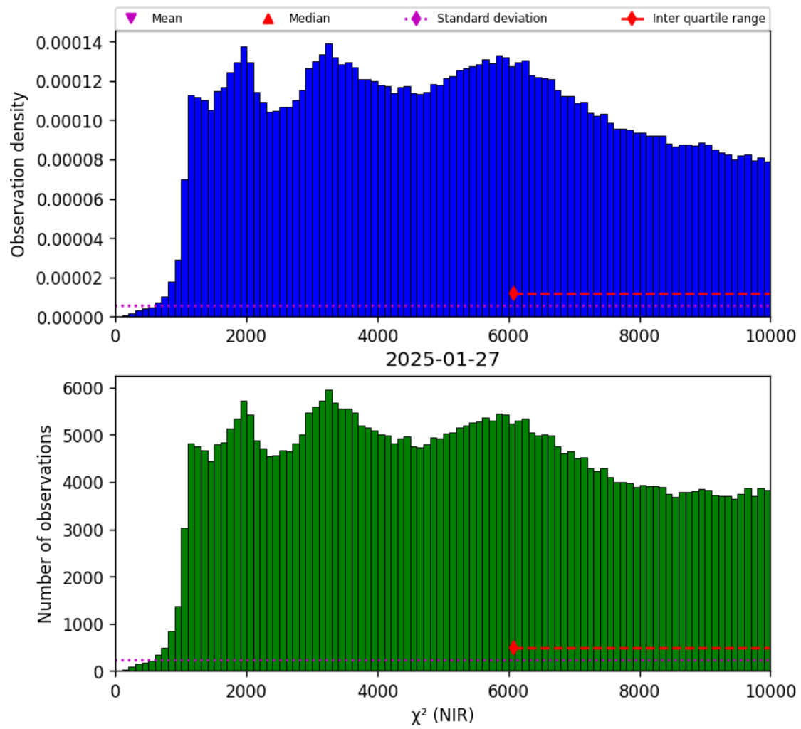
Figure 29: Histogram of “ \chi^2 (NIR)” for 2025-01-26 to 2025-01-28
