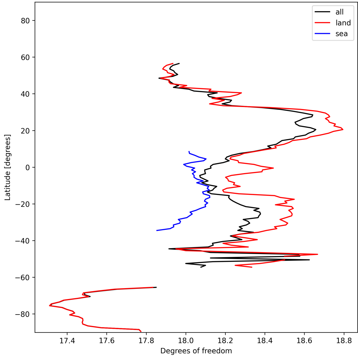
Figure 19: Zonal average of “Degrees of freedom” for 2025-01-26 to 2025-01-28.
