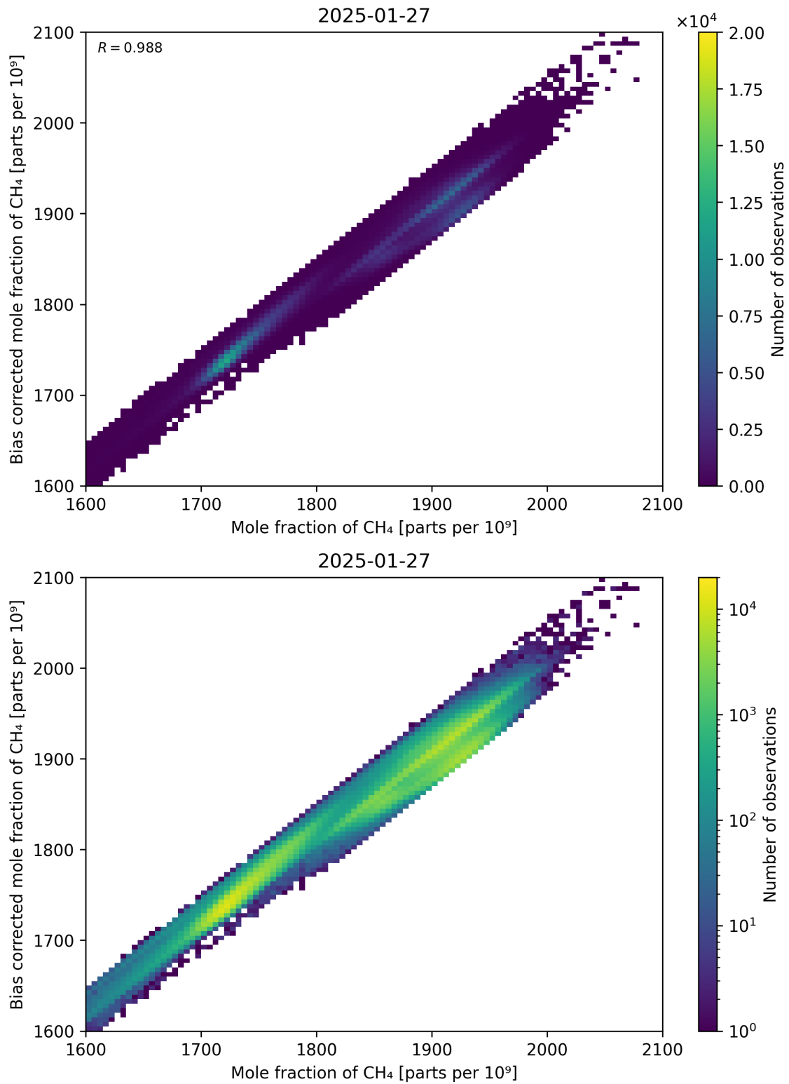
Figure 74: Scatter density plot of “Mole fraction of CH 4 ” against “Bias corrected mole fraction of CH 4 ” for 2025-01-26 to 2025-01-28.
