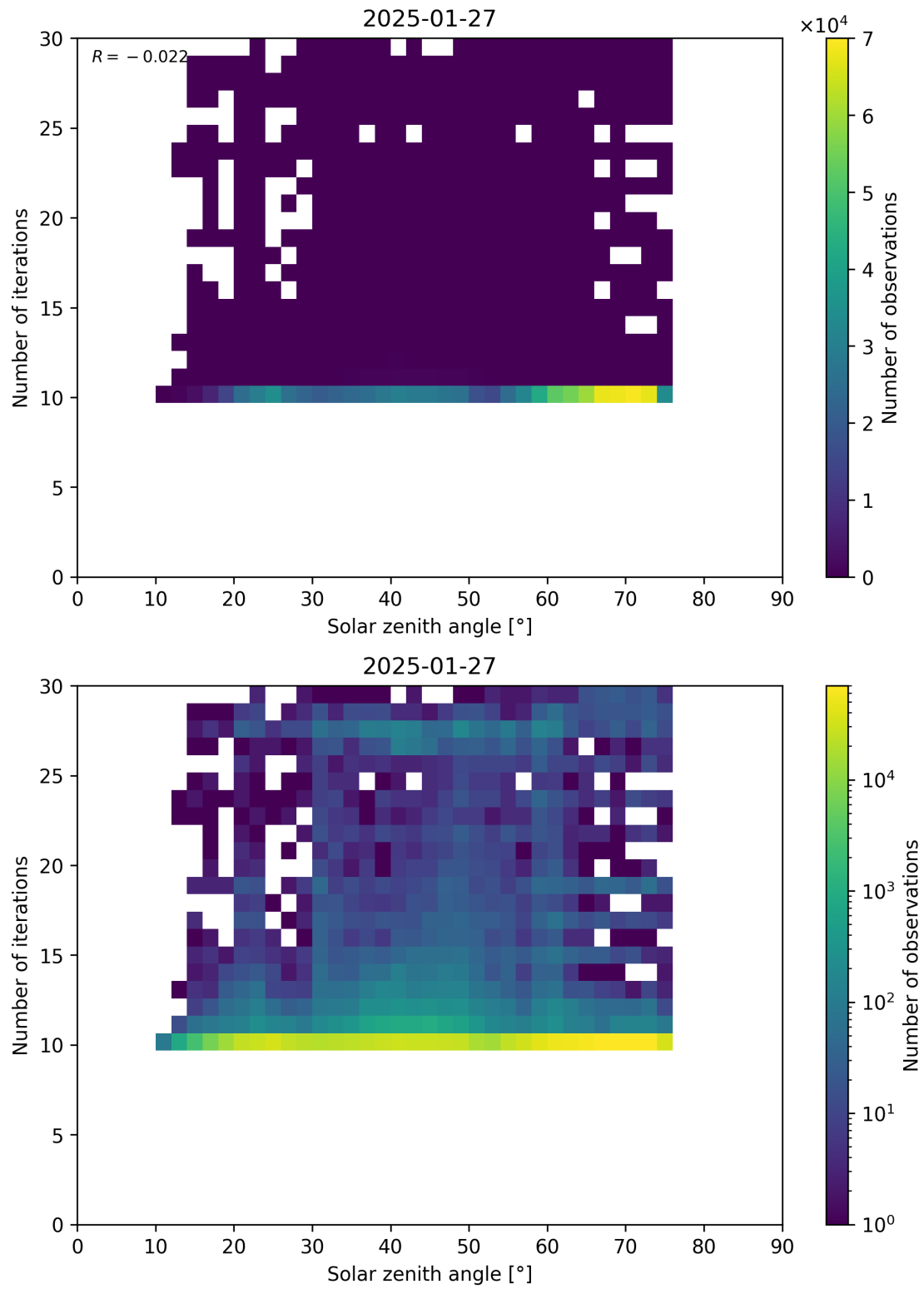
Figure 102: Scatter density plot of “Solar zenith angle” against “Number of iterations” for 2025-01-26 to 2025-01-28.
