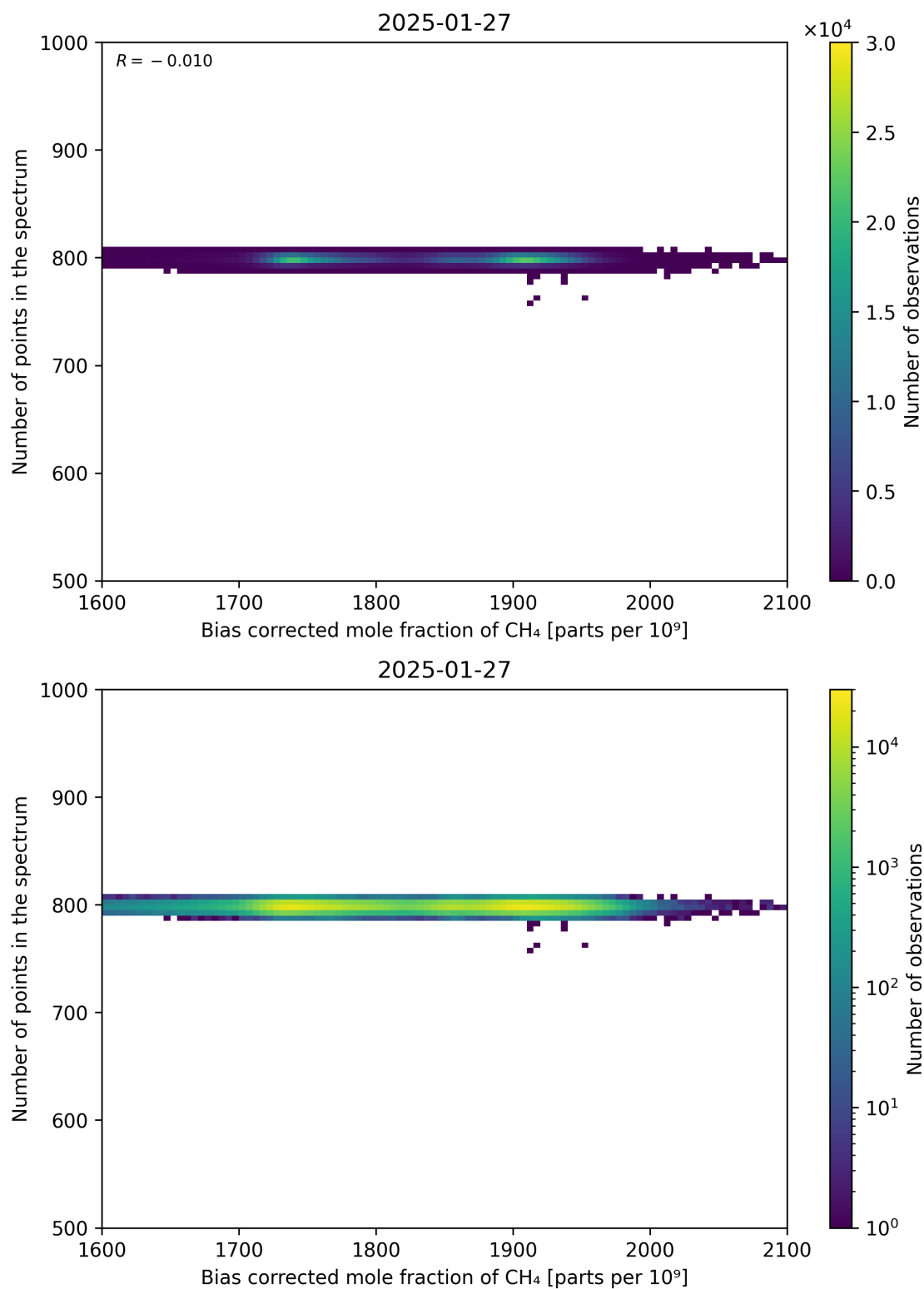
Figure 68: Scatter density plot of “Bias corrected mole fraction of CH 4 ” against “Number of points in the spectrum” for 2025-01-26 to 2025-01-28.
