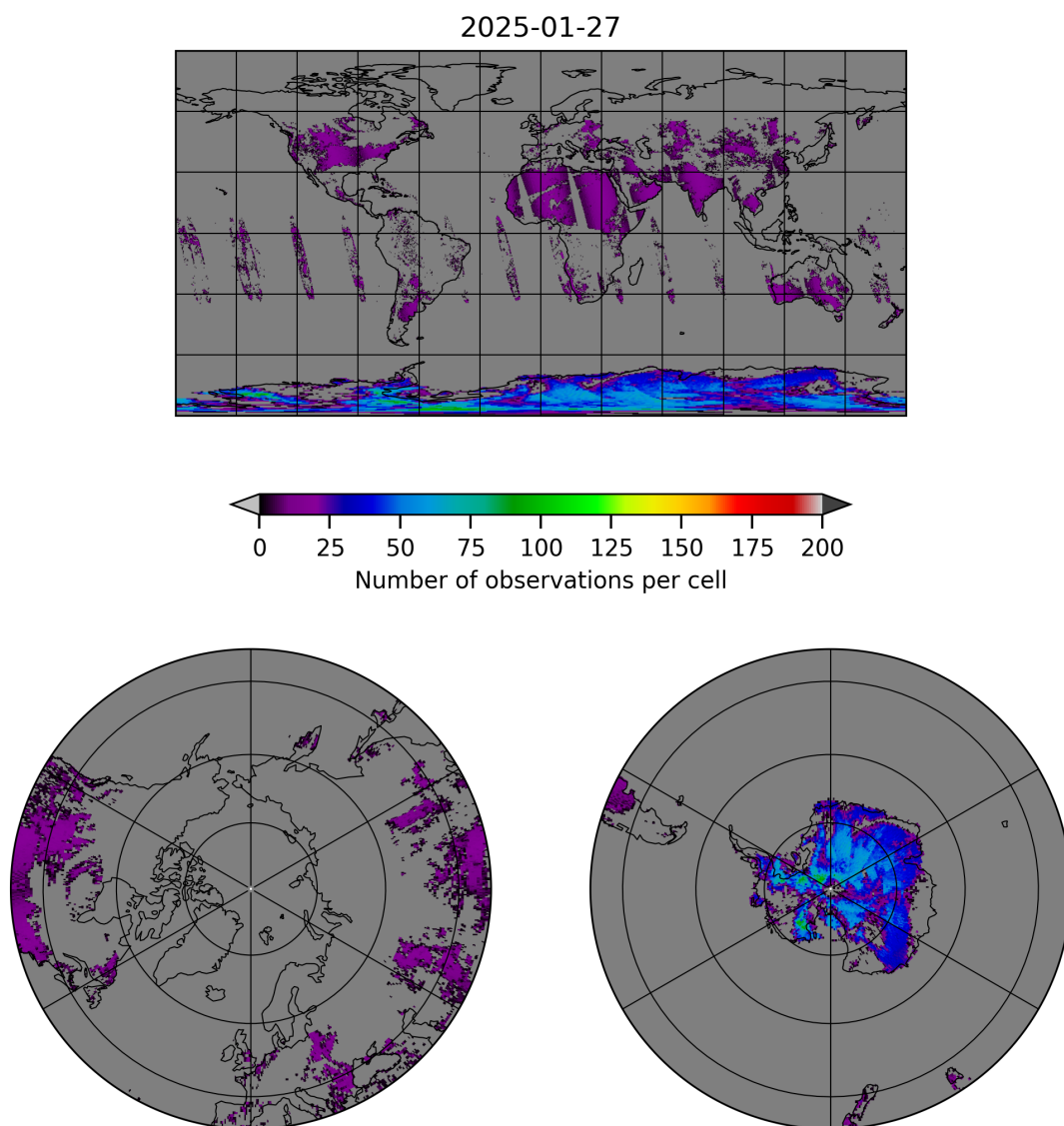
Figure 10: Map of the number of observations for 2025-01-26 to 2025-01-28
