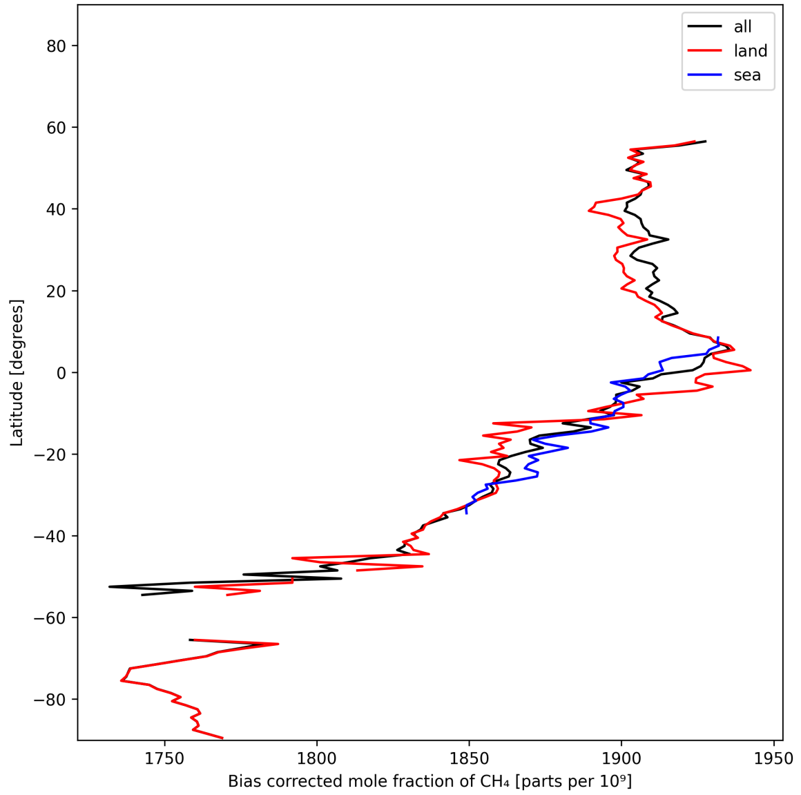
Figure 14: Zonal average of “Bias corrected mole fraction of CH 4 ” for 2025-01-26 to 2025-01-28.
