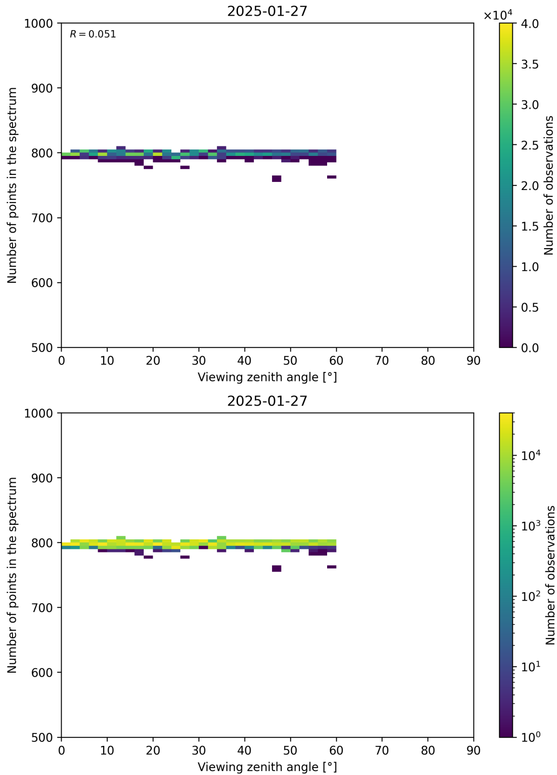
Figure 114: Scatter density plot of “Viewing zenith angle” against “Number of points in the spectrum” for 2025-01-26 to 2025-01-28.
