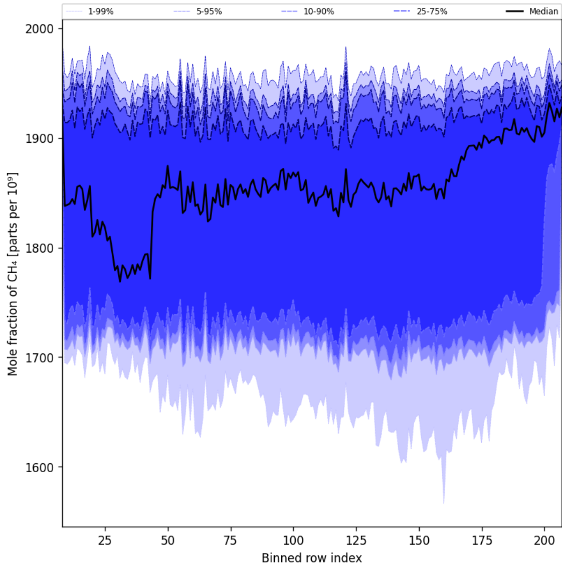
Figure 34: Along track statistics of “Mole fraction of CH 4 ” for 2025-01-26 to 2025-01-28
