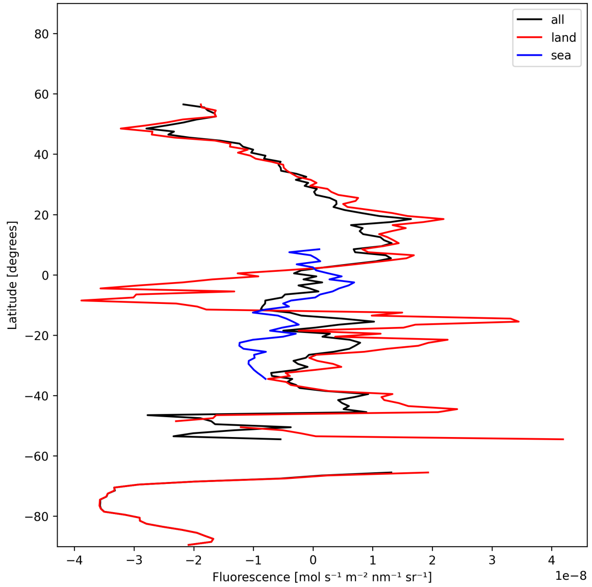
Figure 21: Zonal average of “Fluorescence” for 2025-01-26 to 2025-01-28.
