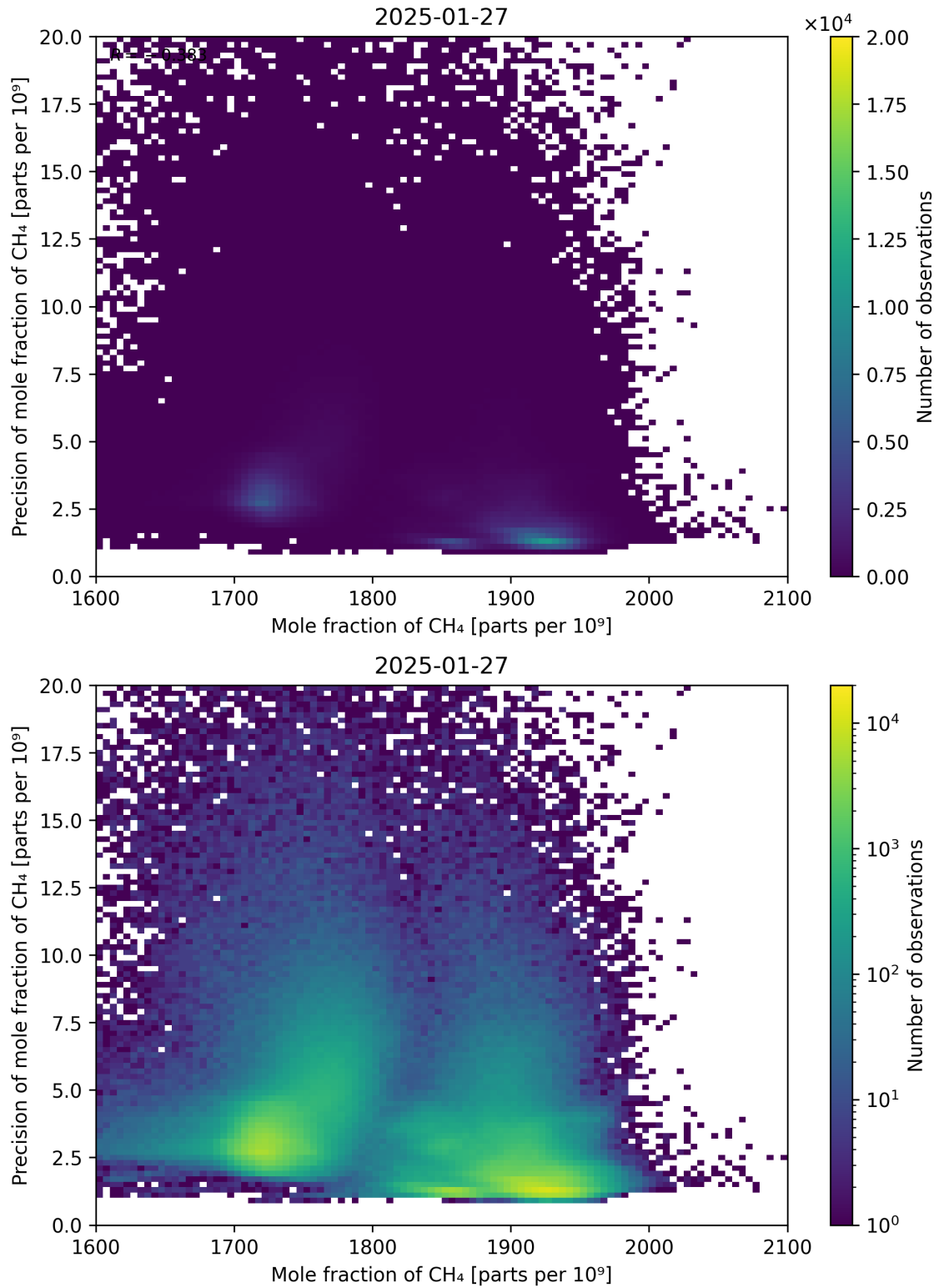
Figure 75: Scatter density plot of “Mole fraction of CH 4 ” against “Precision of mole fraction of CH 4 ” for 2025-01-26 to 2025-01-28.
