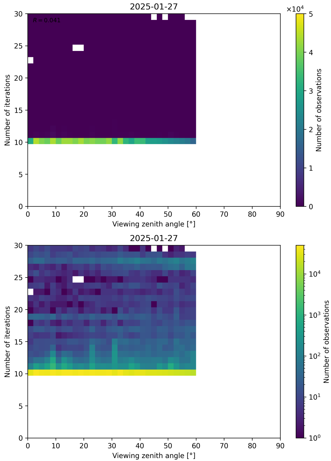
Figure 113: Scatter density plot of “Viewing zenith angle” against “Number of iterations” for 2025-01-26 to 2025-01-28.
