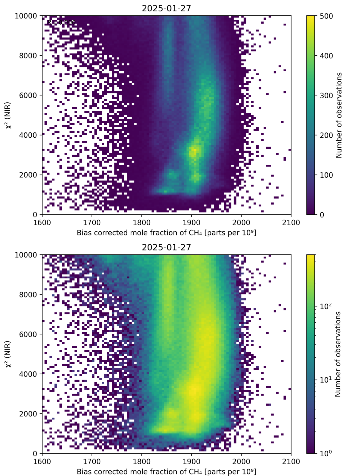
Figure 63: Scatter density plot of “Bias corrected mole fraction of \text{CH}_4 ” against “ \chi^2 (NIR)” for 2025-01-26 to 2025-01-28.
