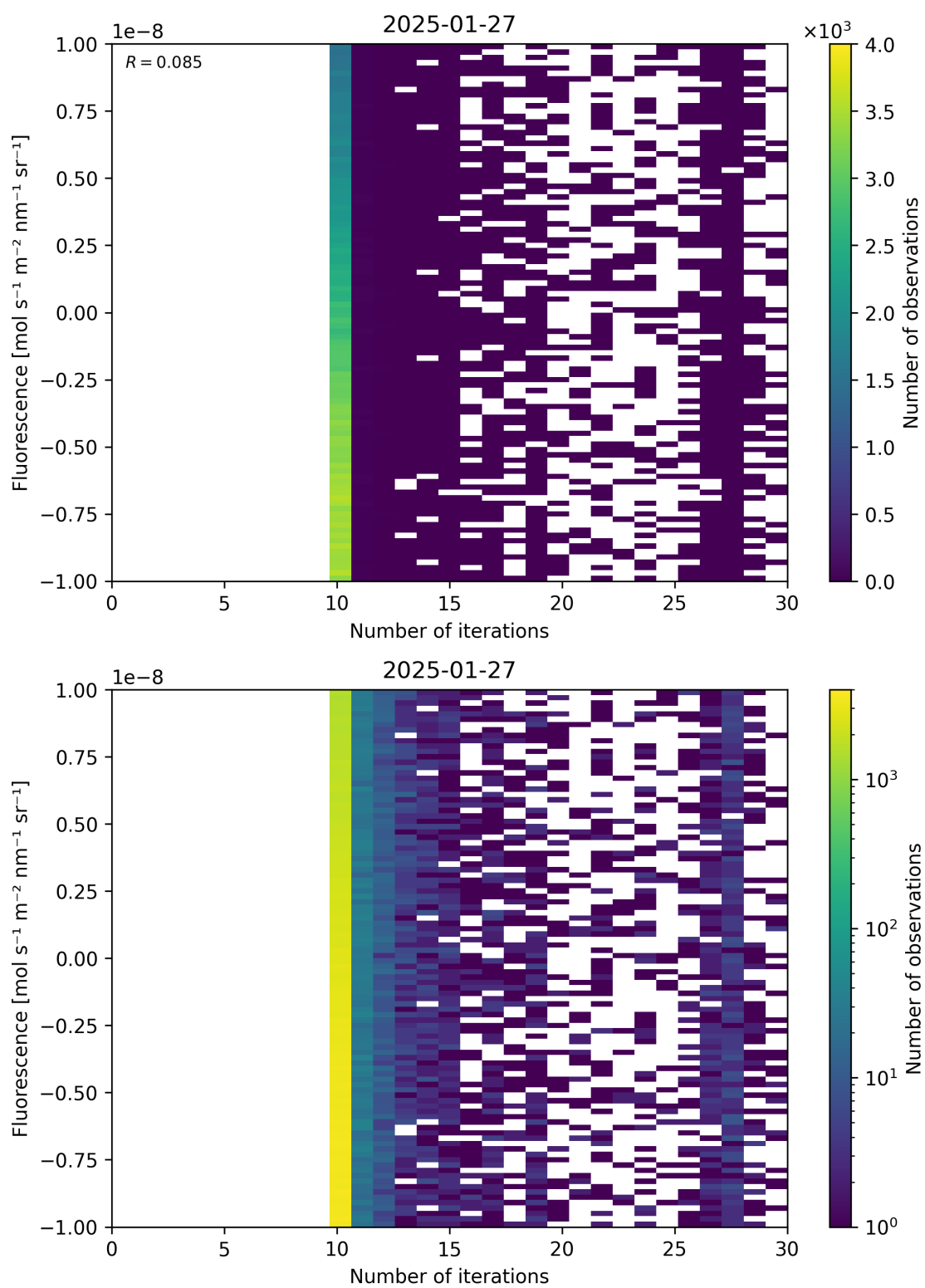
Figure 87: Scatter density plot of “Number of iterations” against “Fluorescence” for 2025-01-26 to 2025-01-28.
