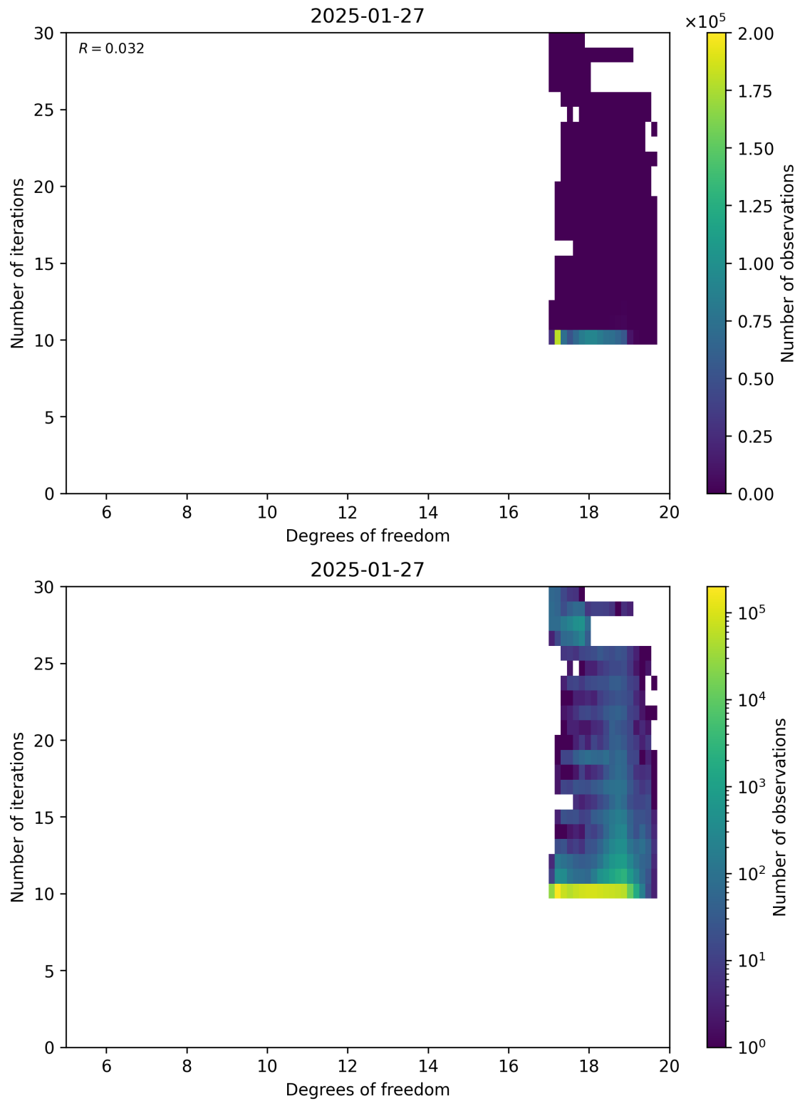
Figure 52: Scatter density plot of “Degrees of freedom” against “Number of iterations” for 2025-01-26 to 2025-01-28.
