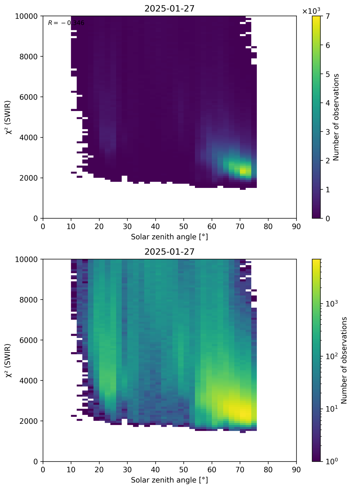
Figure 95: Scatter density plot of “Solar zenith angle” against “ \chi^2 (SWIR)” for 2025-01-26 to 2025-01-28.
