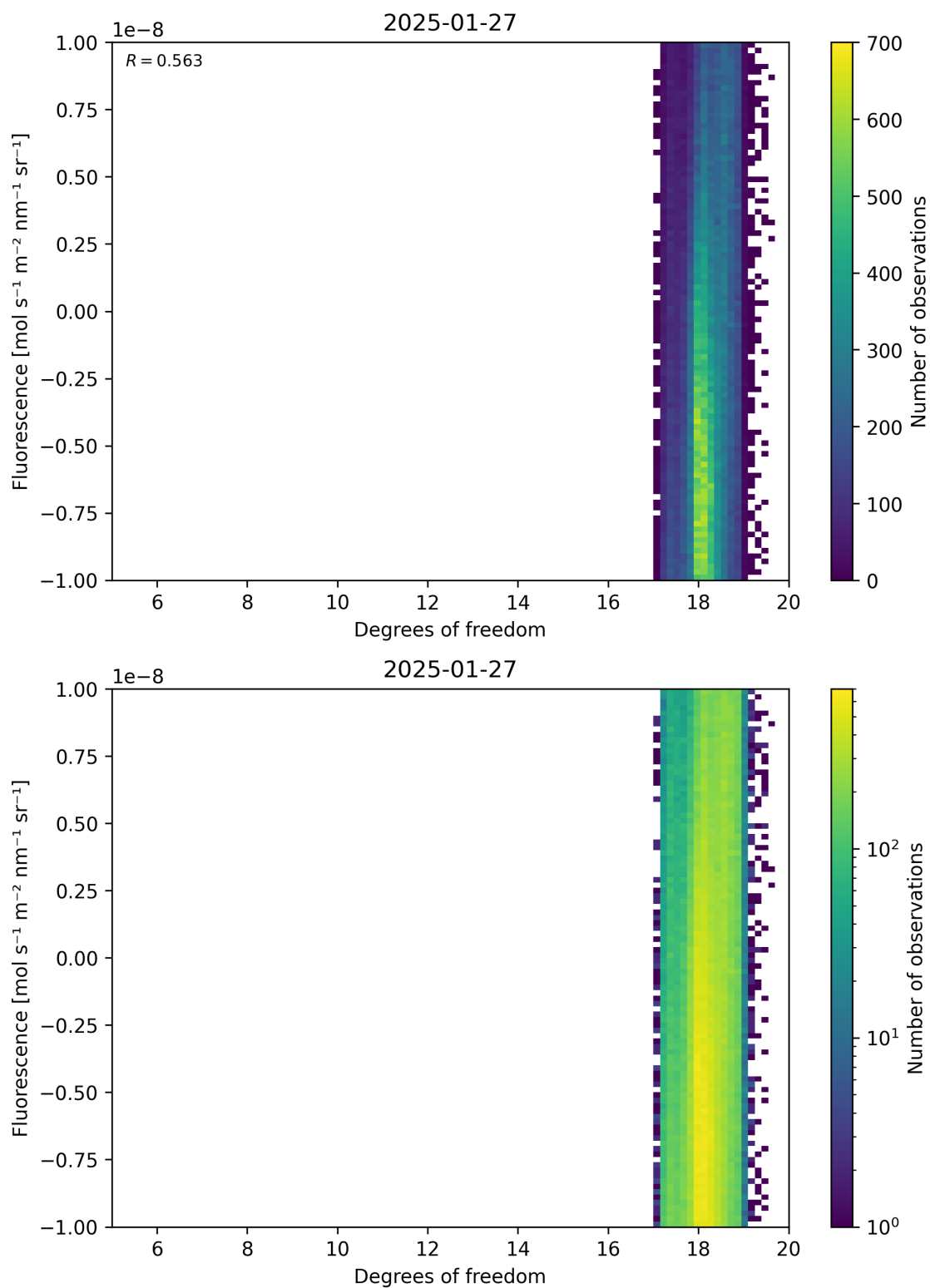
Figure 51: Scatter density plot of “Degrees of freedom” against “Fluorescence” for 2025-01-26 to 2025-01-28.
