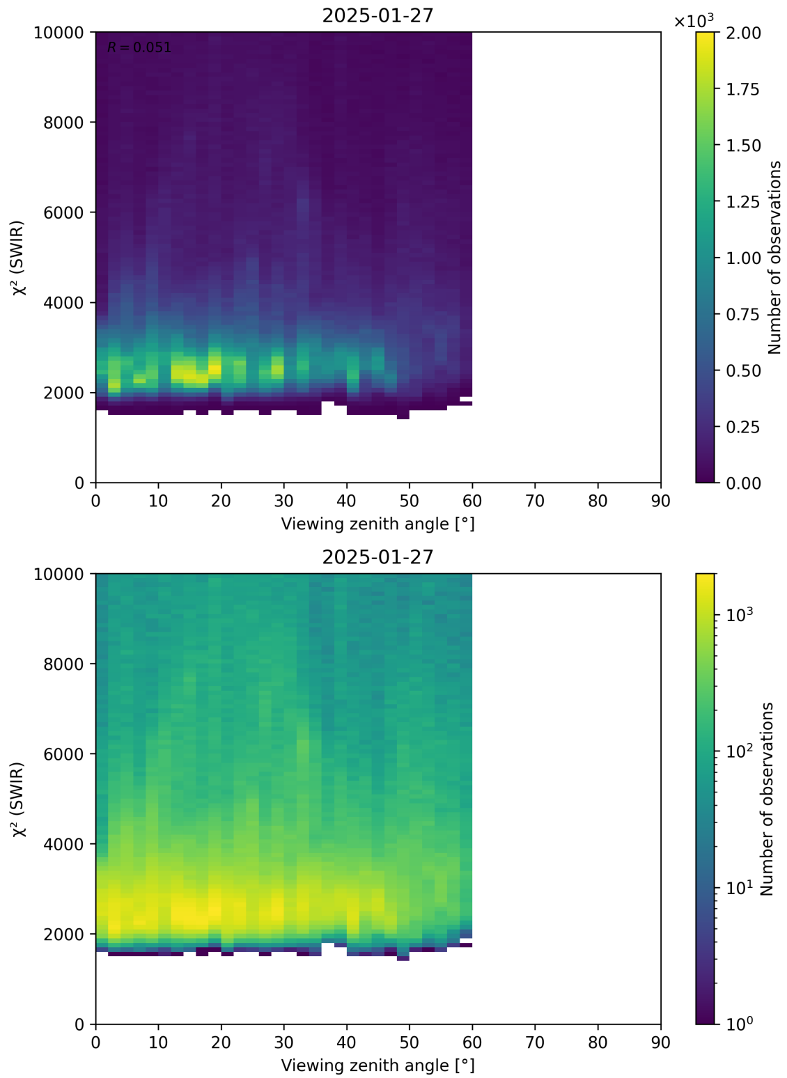
Figure 106: Scatter density plot of “Viewing zenith angle” against “ \chi^2 (SWIR)” for 2025-01-26 to 2025-01-28.
