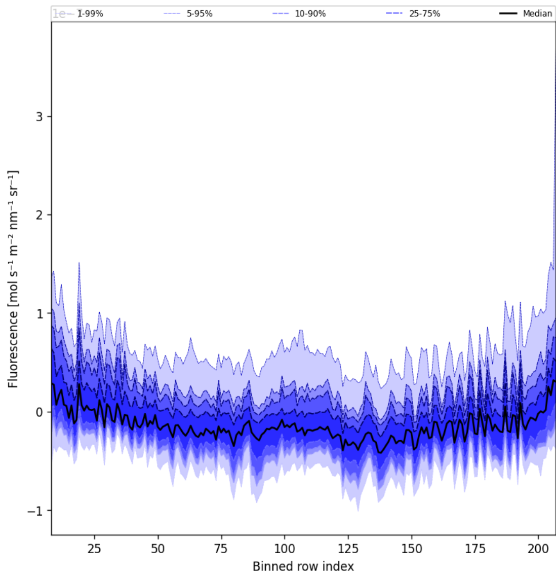
Figure 43: Along track statistics of “Fluorescence” for 2025-01-26 to 2025-01-28
