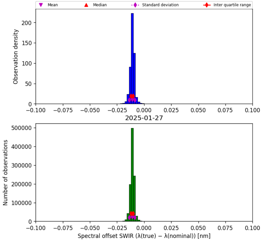
Figure 27: Histogram of “Spectral offset SWIR ( \lambda_{\text{true}} - \lambda_{\text{nominal}} )” for 2025-01-26 to 2025-01-28
