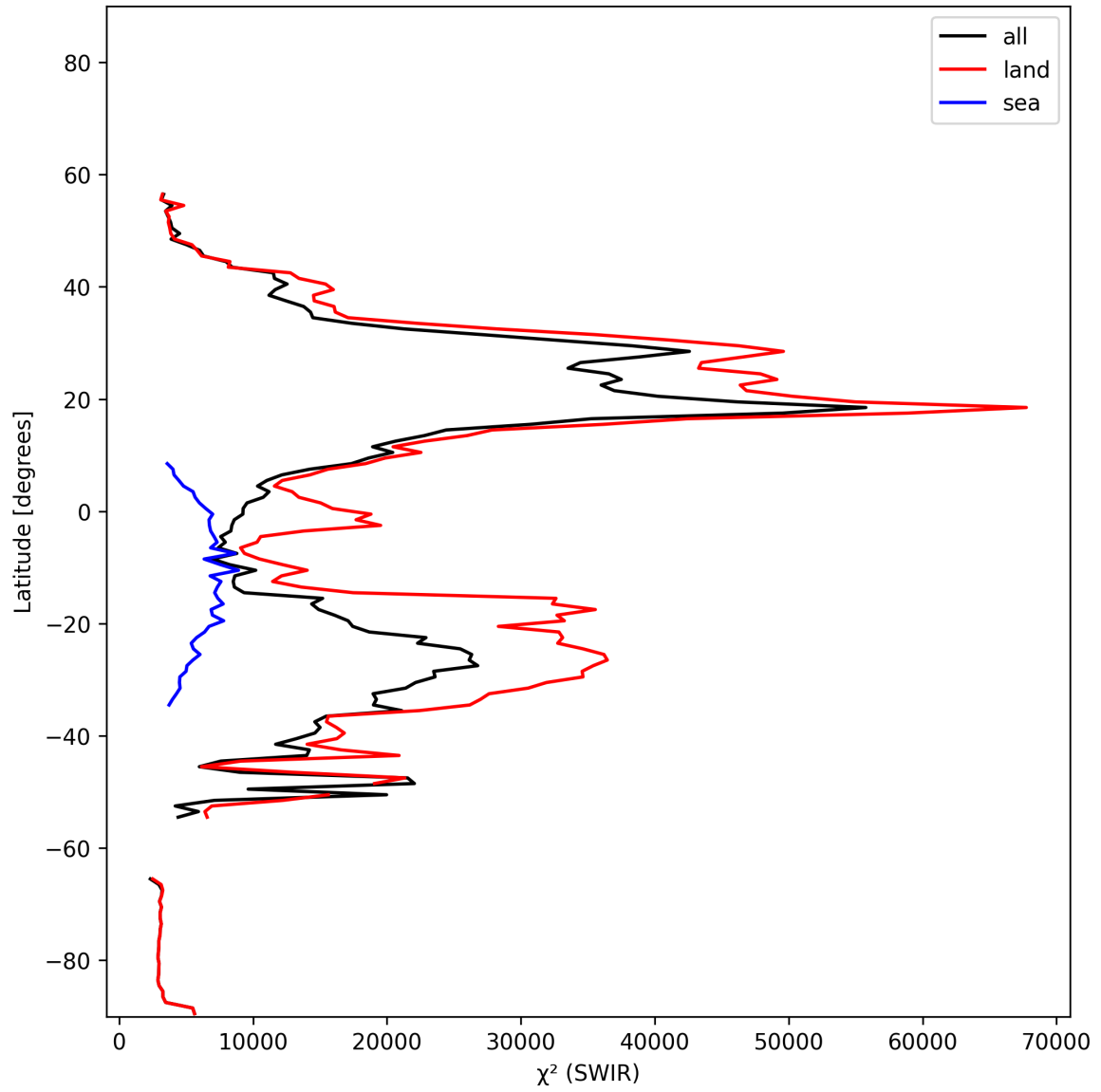
Figure 17: Zonal average of “ \chi^2 (SWIR)” for 2025-01-26 to 2025-01-28.
