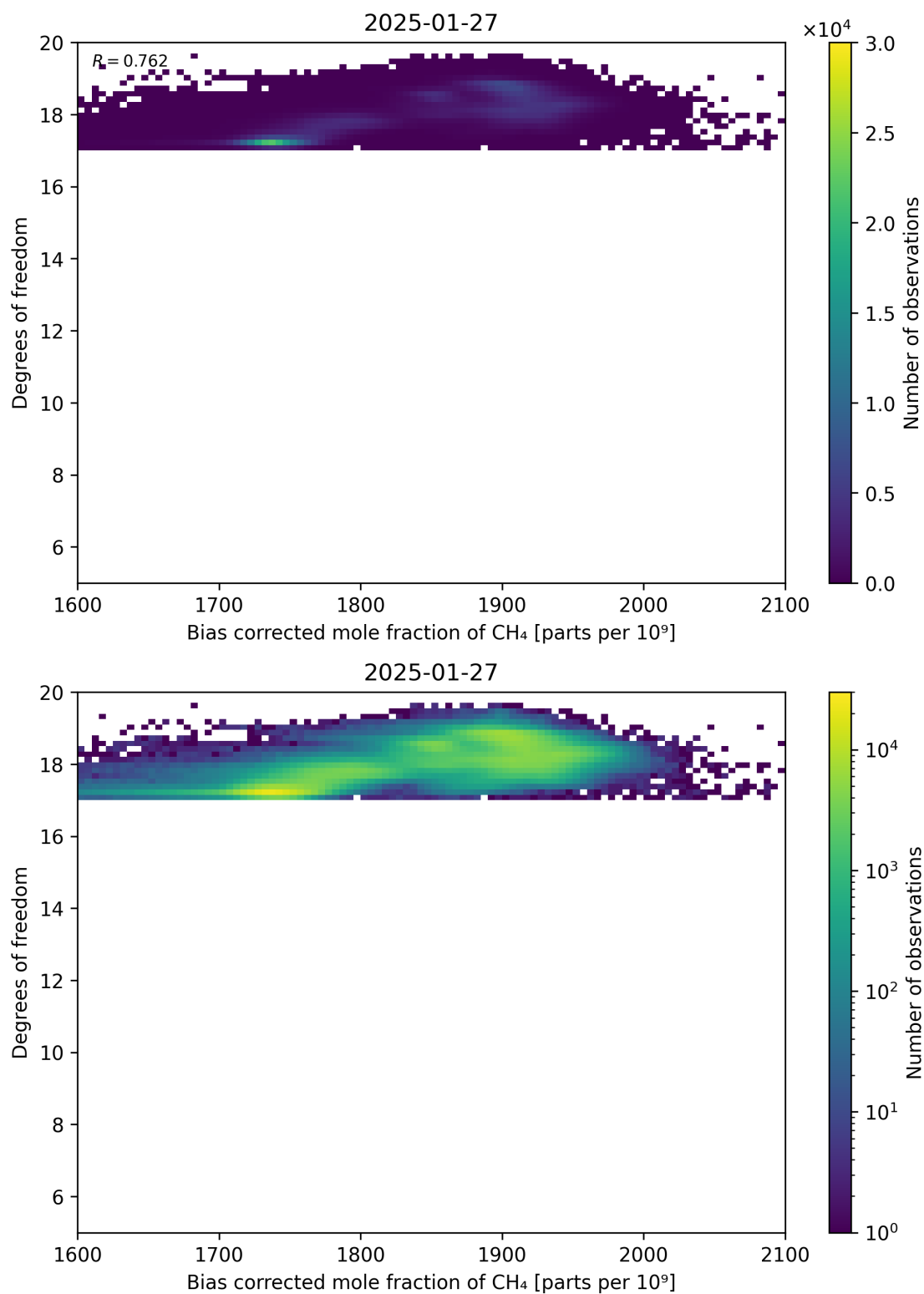
Figure 65: Scatter density plot of “Bias corrected mole fraction of CH 4 ” against “Degrees of freedom” for 2025-01-26 to 2025-01-28.
