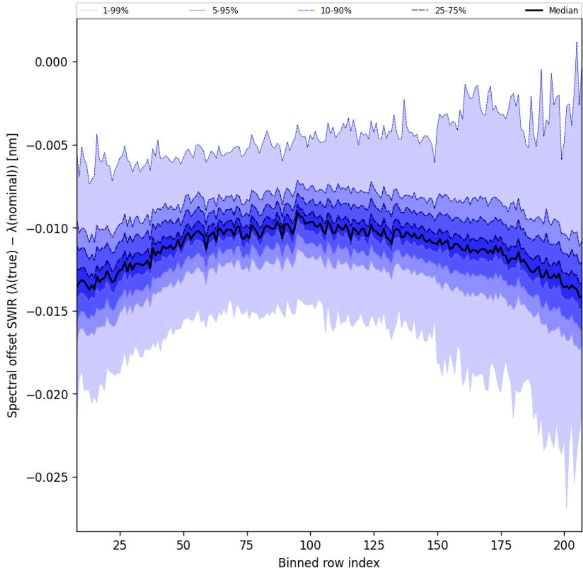
Figure 38: Along track statistics of “Spectral offset SWIR ( \lambda_{\text{true}} - \lambda_{\text{nominal}} )” for 2025-01-26 to 2025-01-28
