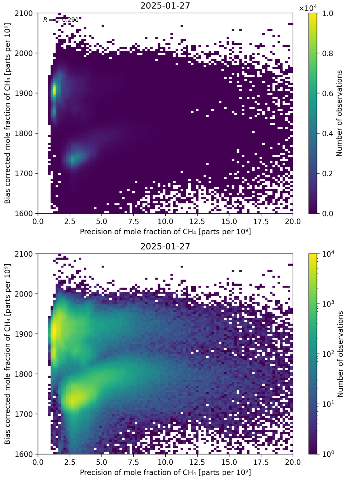
Figure 82: Scatter density plot of “Precision of mole fraction of CH 4 ” against “Bias corrected mole fraction of CH 4 ” for 2025-01-26 to 2025-01-28.
