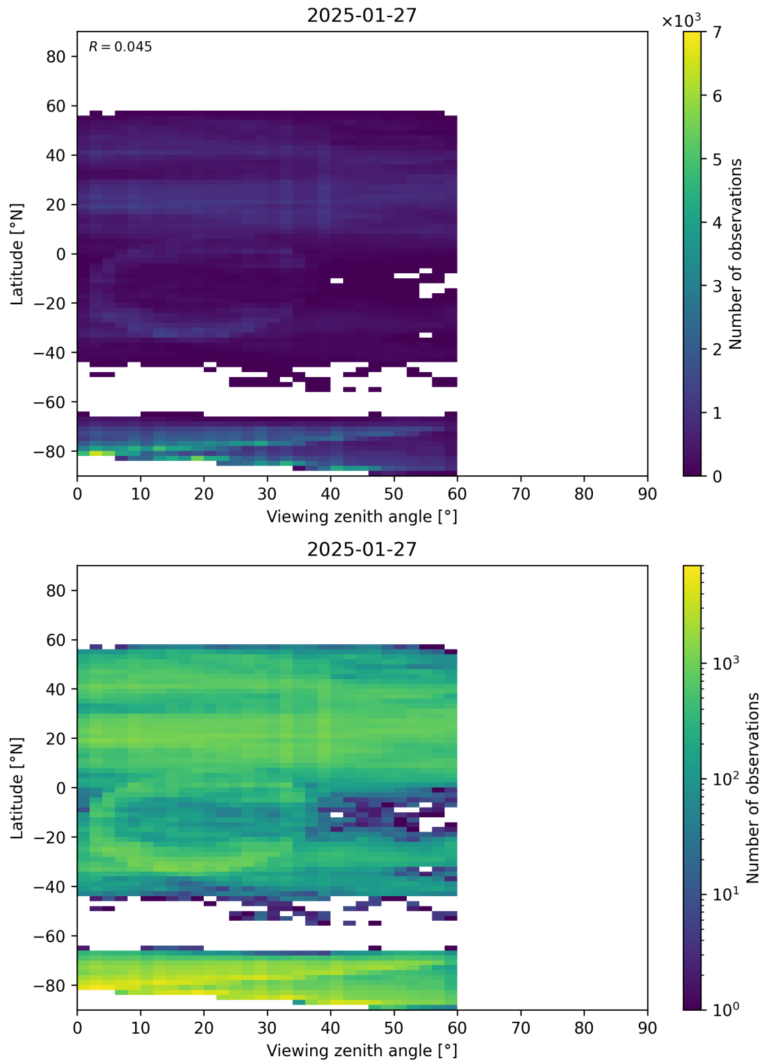
Figure 109: Scatter density plot of “Viewing zenith angle” against “Latitude” for 2025-01-26 to 2025-01-28.
