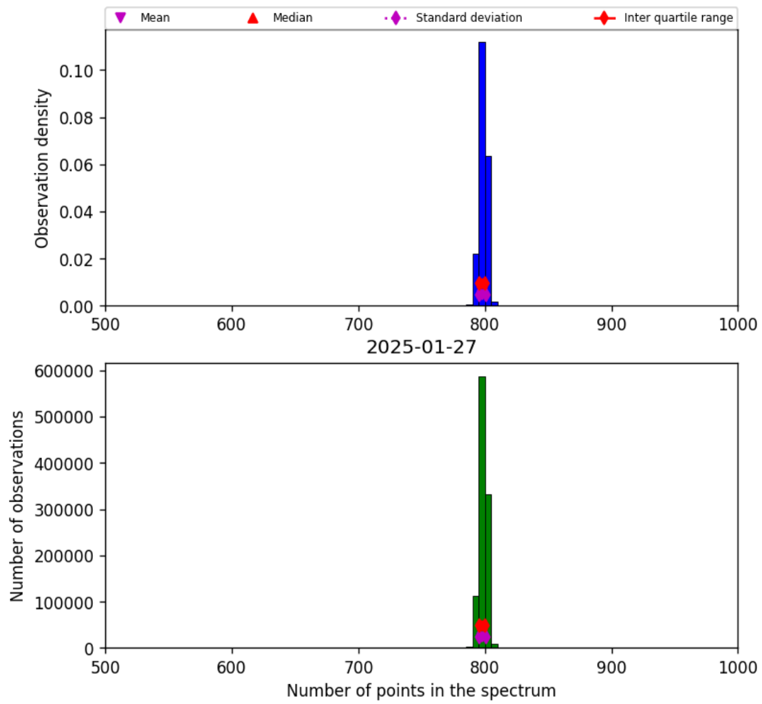
Figure 26: Histogram of “Number of points in the spectrum” for 2025-01-26 to 2025-01-28
