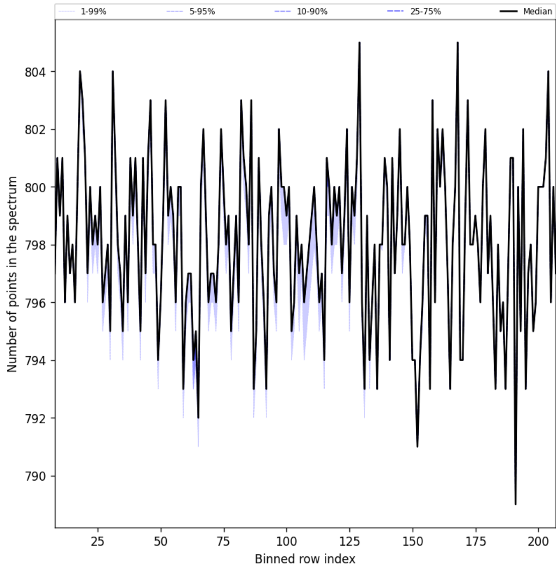
Figure 37: Along track statistics of “Number of points in the spectrum” for 2025-01-26 to 2025-01-28
