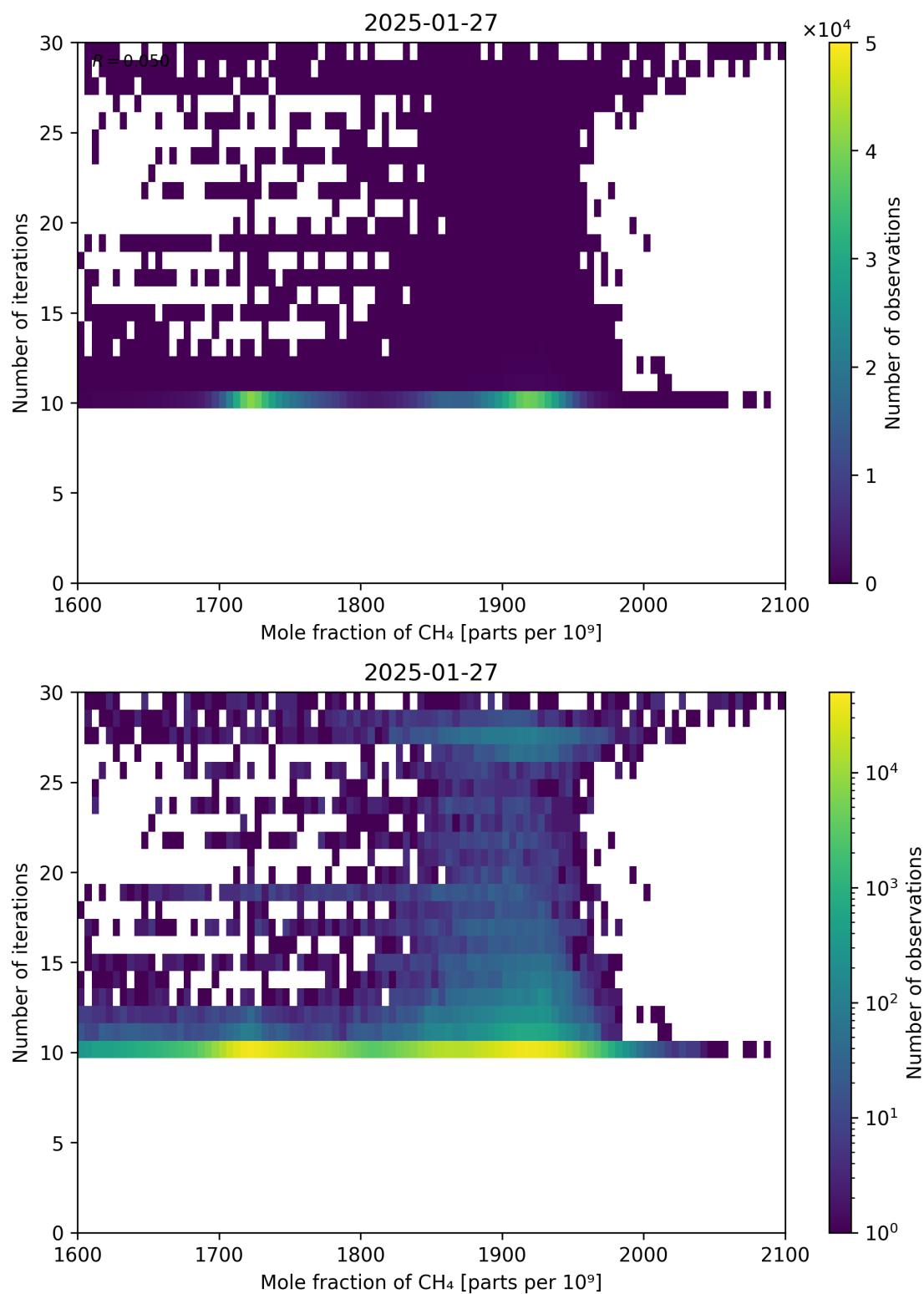
Figure 76: Scatter density plot of “Mole fraction of CH 4 ” against “Number of iterations” for 2025-01-26 to 2025-01-28.
