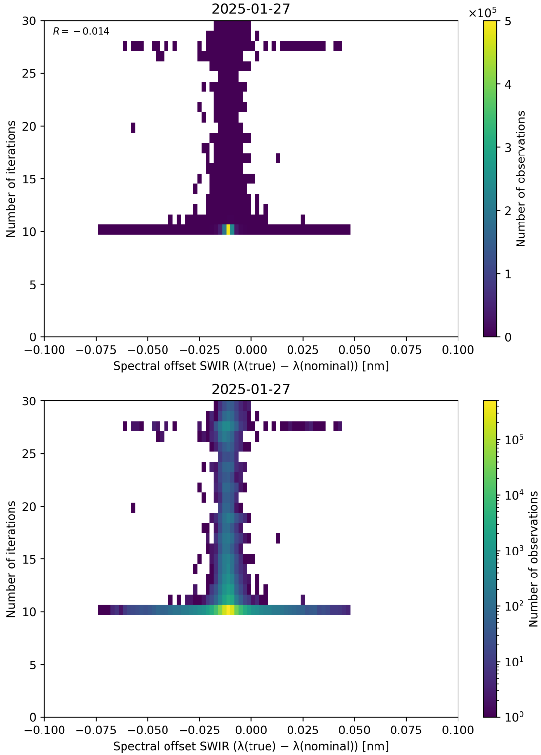
Figure 121: Scatter density plot of “Spectral offset SWIR ( \lambda_{\text{true}} - \lambda_{\text{nominal}} )” against “Number of iterations” for 2025-01-26 to 2025-01-28.
