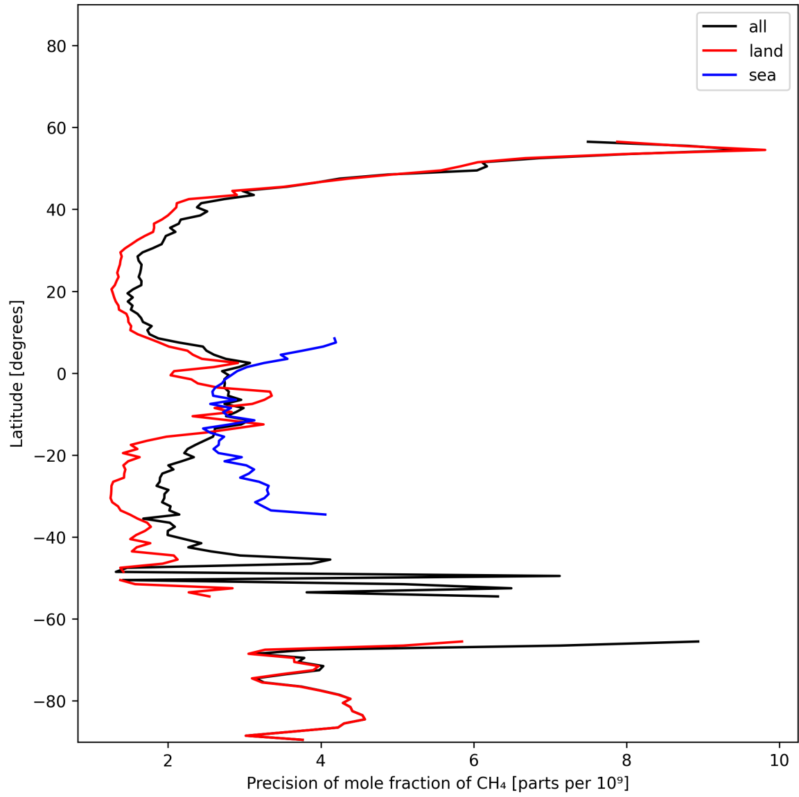
Figure 13: Zonal average of “Precision of mole fraction of CH 4 ” for 2025-01-26 to 2025-01-28.
