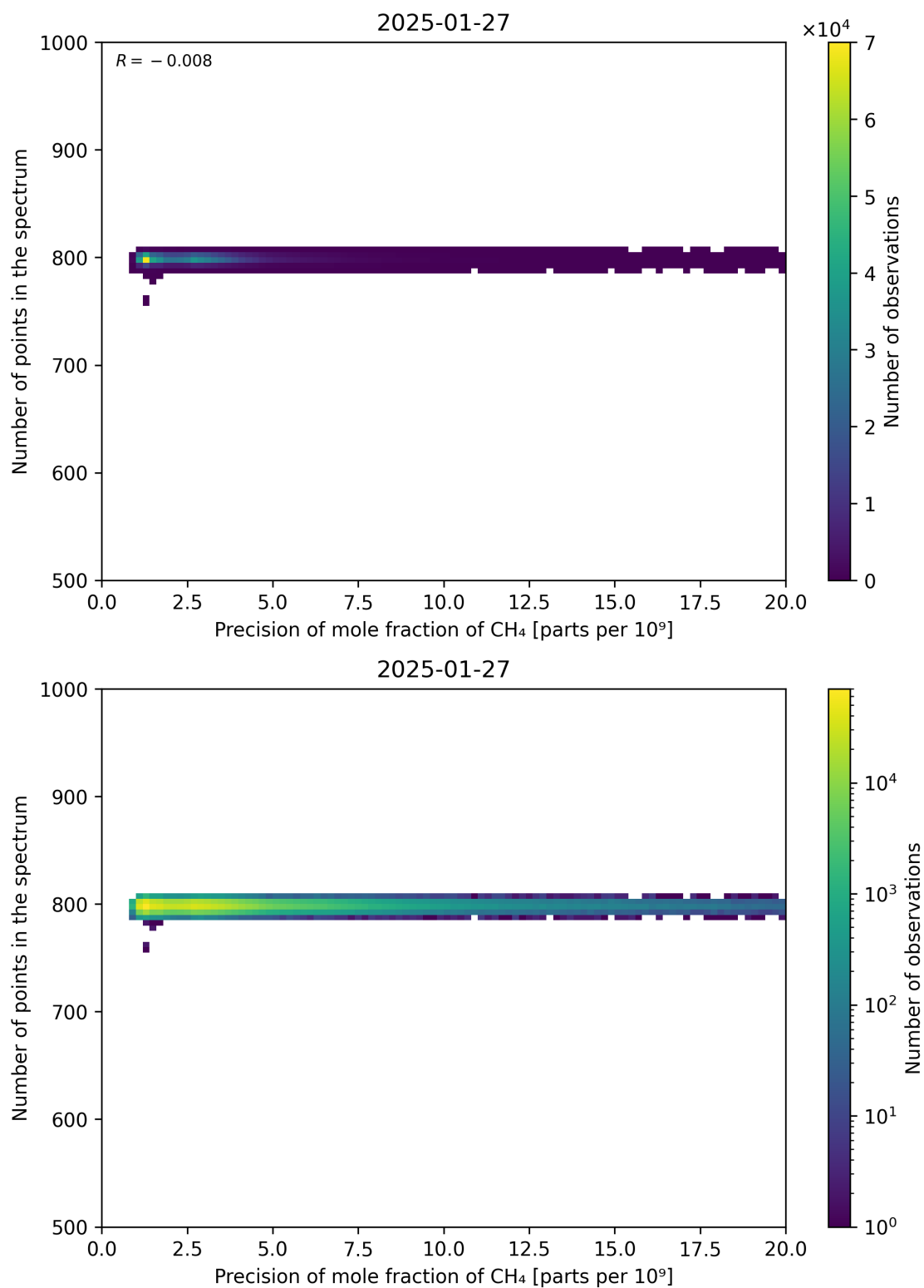
Figure 84: Scatter density plot of “Precision of mole fraction of CH 4 ” against “Number of points in the spectrum” for 2025-01-26 to 2025-01-28.
