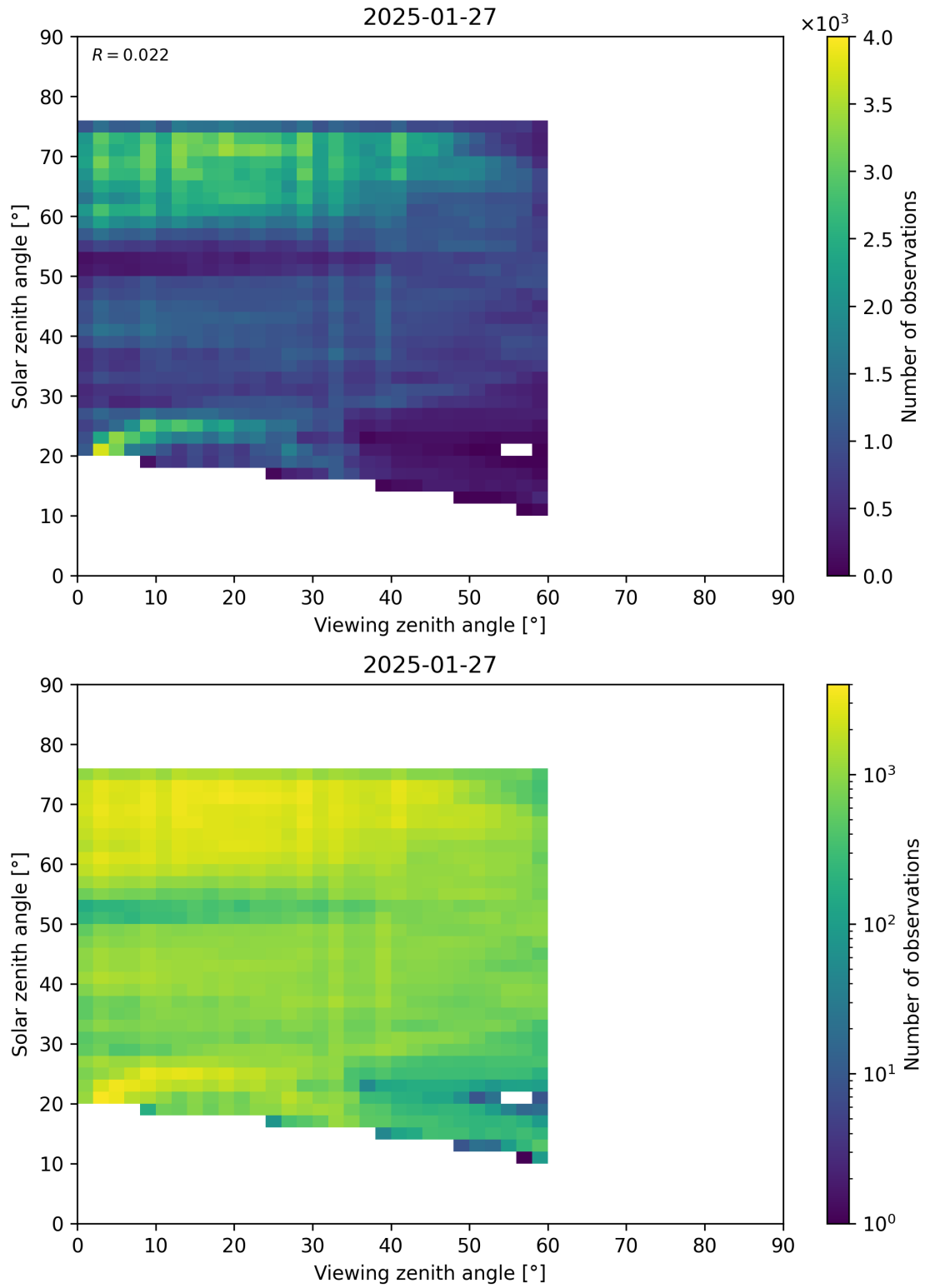
Figure 115: Scatter density plot of “Viewing zenith angle” against “Solar zenith angle” for 2025-01-26 to 2025-01-28.
