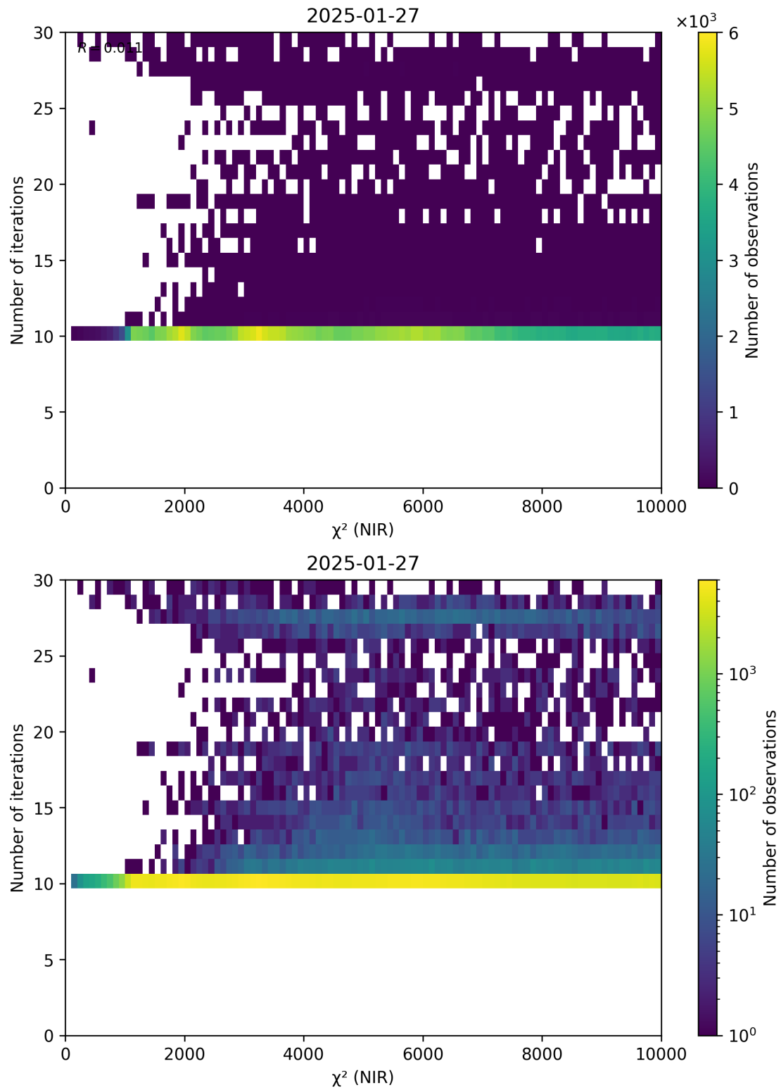
Figure 46: Scatter density plot of “ \chi^2 (NIR)” against “Number of iterations” for 2025-01-26 to 2025-01-28.
