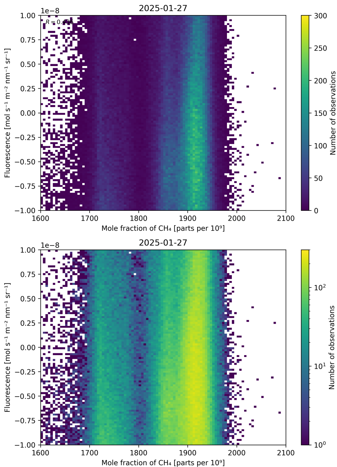
Figure 73: Scatter density plot of “Mole fraction of CH 4 ” against “Fluorescence” for 2025-01-26 to 2025-01-28.
