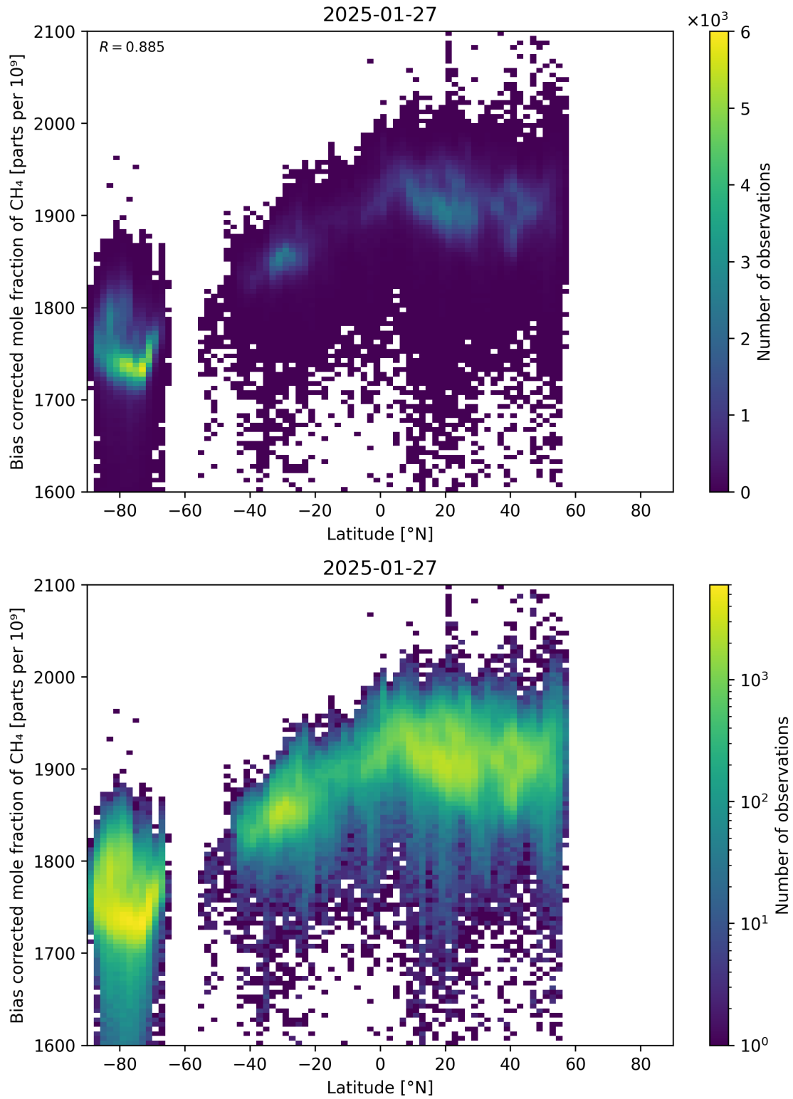
Figure 58: Scatter density plot of “Latitude” against “Bias corrected mole fraction of \text{CH}_4 ” for 2025-01-26 to 2025-01-28.
