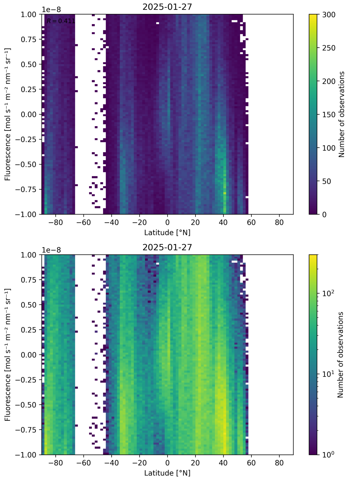
Figure 56: Scatter density plot of “Latitude” against “Fluorescence” for 2025-01-26 to 2025-01-28.
