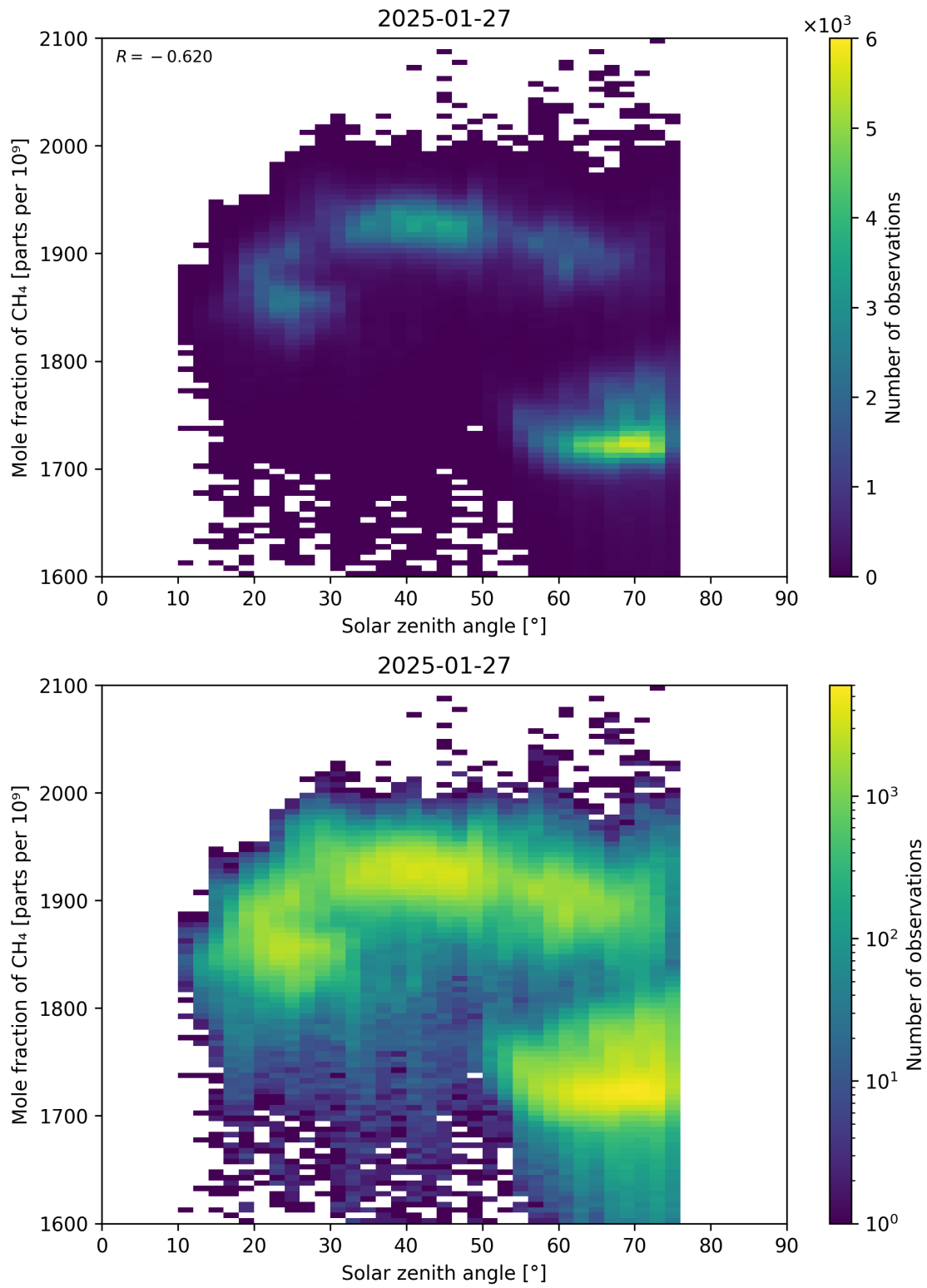
Figure 99: Scatter density plot of “Solar zenith angle” against “Mole fraction of \text{CH}_4 ” for 2025-01-26 to 2025-01-28.
