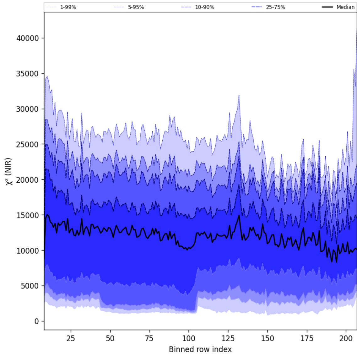
Figure 40: Along track statistics of “ \chi^2 (NIR)” for 2025-01-26 to 2025-01-28
