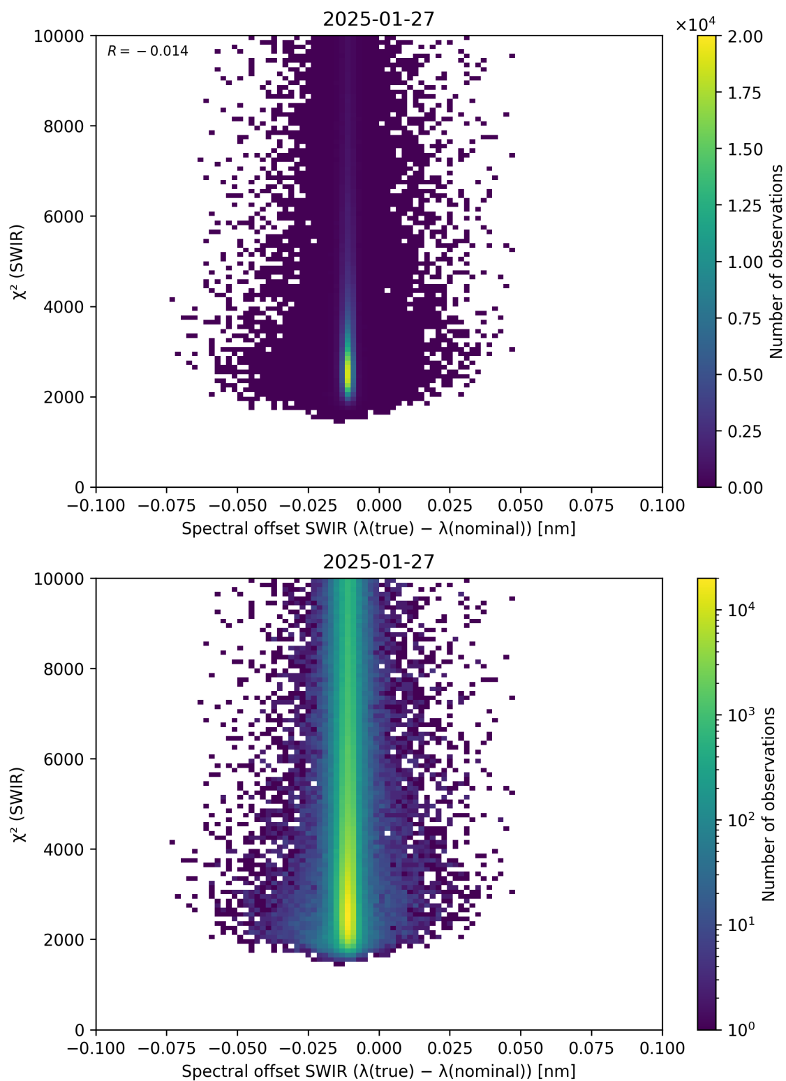
Figure 118: Scatter density plot of “Spectral offset SWIR ( \lambda_{\text{true}} - \lambda_{\text{nominal}} )” against “ \chi^2 (SWIR)” for 2025-01-26 to 2025-01-28.
