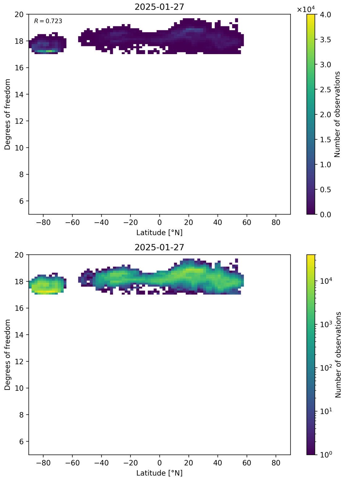
Figure 55: Scatter density plot of “Latitude” against “Degrees of freedom” for 2025-01-26 to 2025-01-28.
