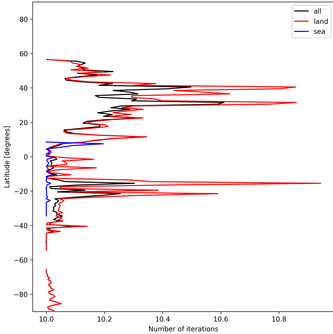
Figure 20: Zonal average of “Number of iterations” for 2025-01-26 to 2025-01-28.
