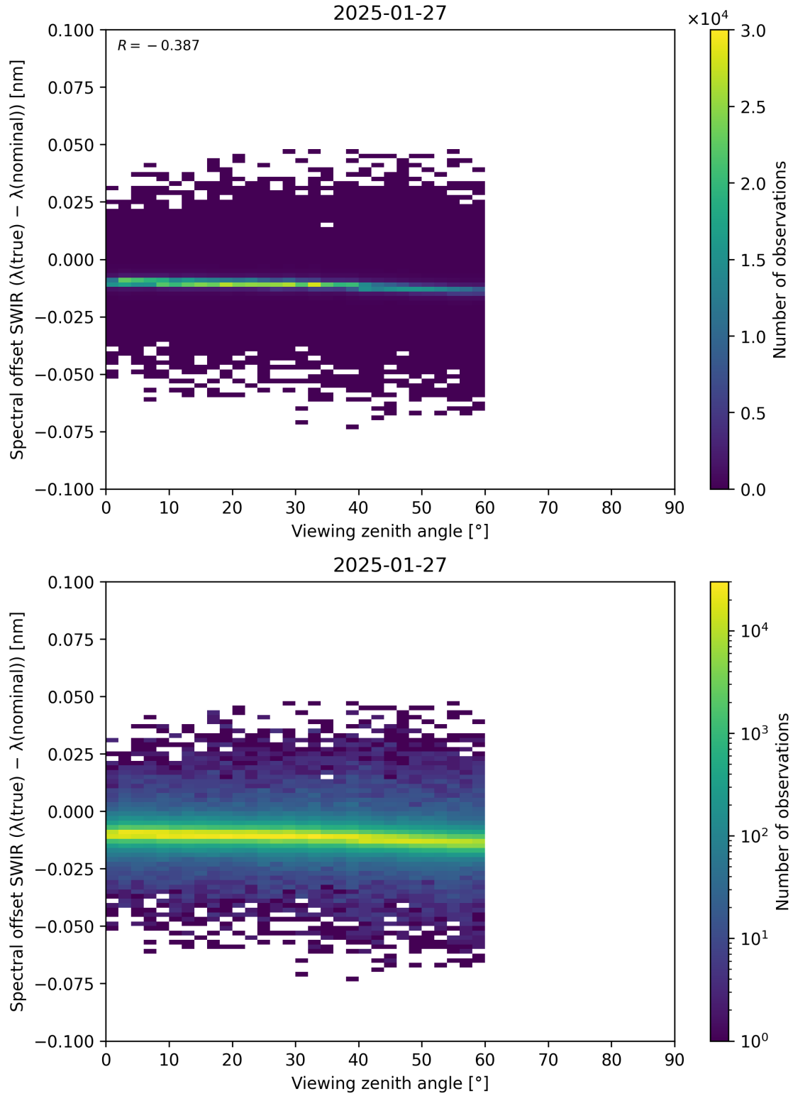
Figure 116: Scatter density plot of “Viewing zenith angle” against “Spectral offset SWIR ( \lambda_{\text{true}} - \lambda_{\text{nominal}} )” for 2025-01-26 to 2025-01-28.
