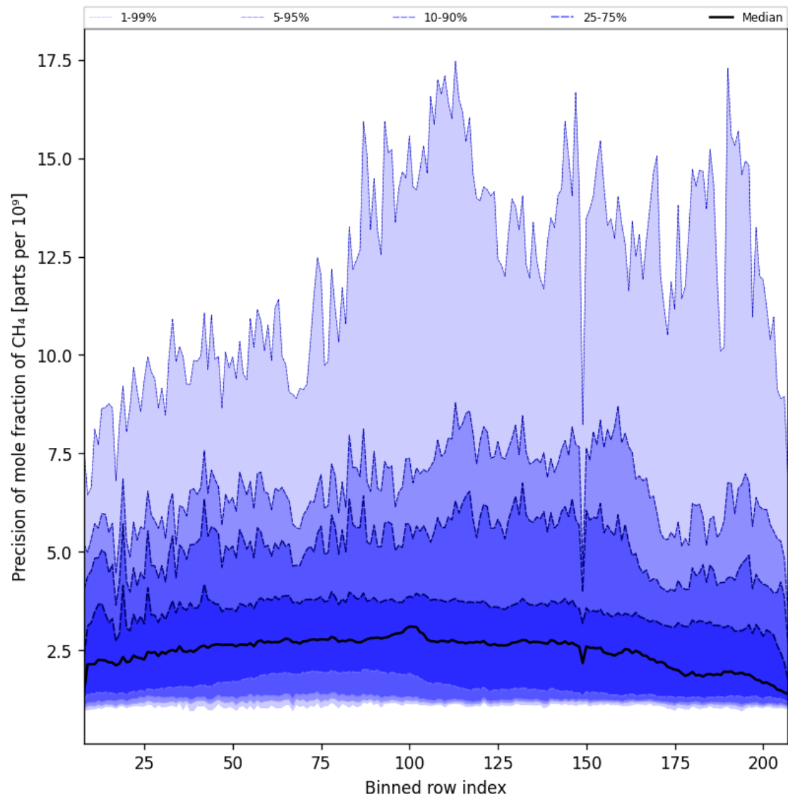
Figure 35: Along track statistics of “Precision of mole fraction of CH 4 ” for 2025-01-26 to 2025-01-28
