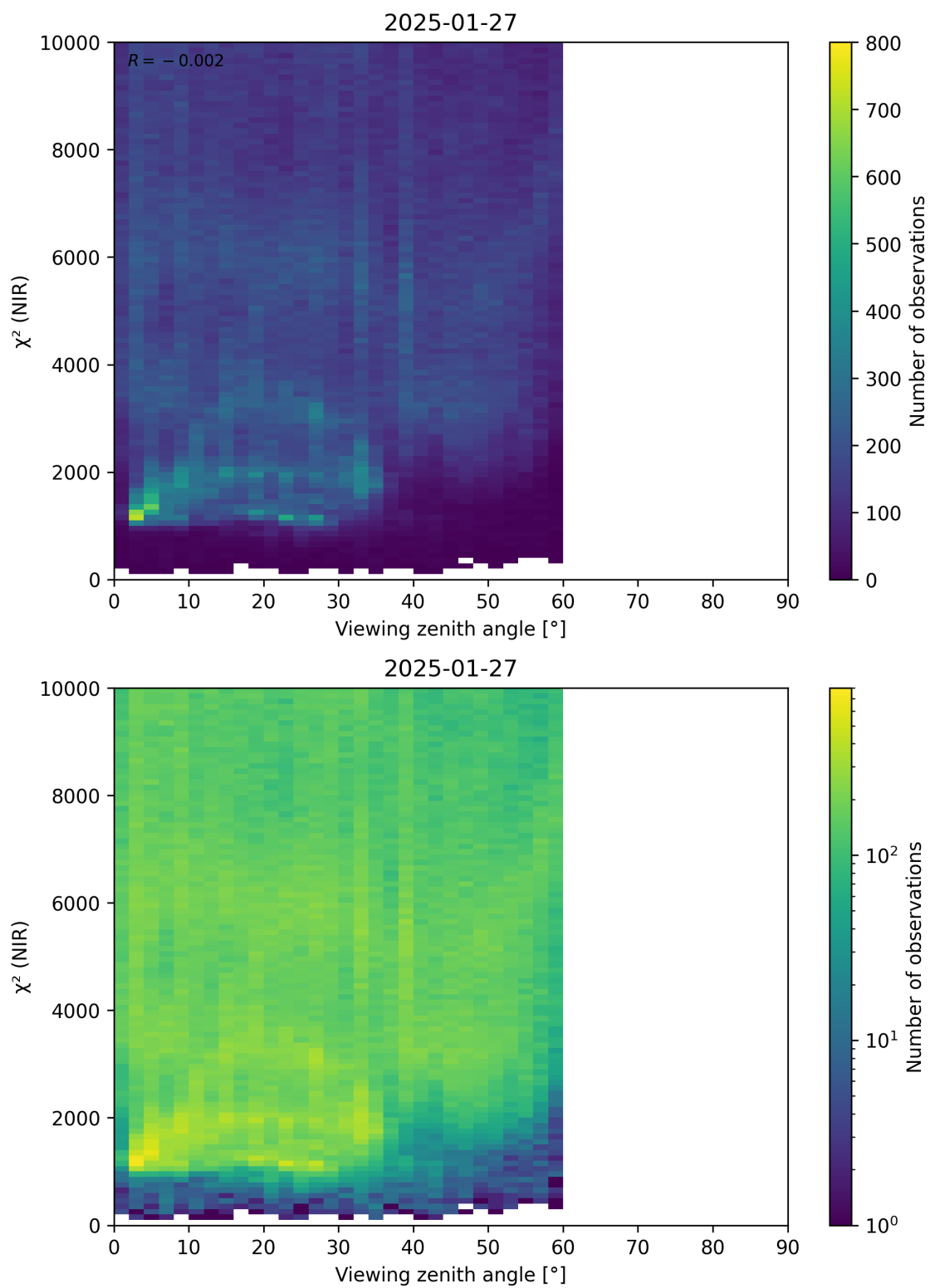
Figure 105: Scatter density plot of “Viewing zenith angle” against “ \chi^2 (NIR)” for 2025-01-26 to 2025-01-28.
