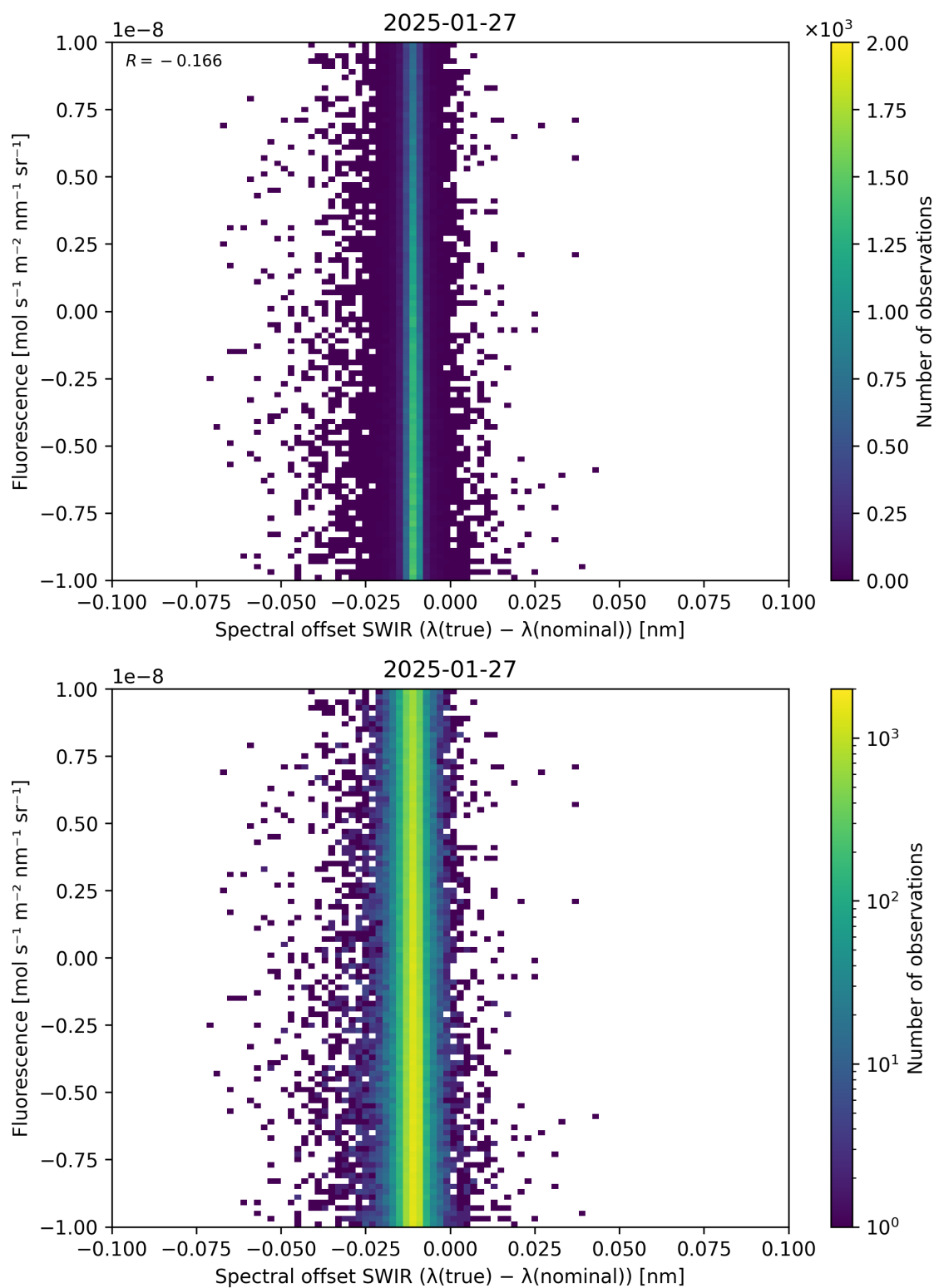
Figure 120: Scatter density plot of “Spectral offset SWIR ( \lambda_{\text{true}} - \lambda_{\text{nominal}} )” against “Fluorescence” for 2025-01-26 to 2025-01-28.
