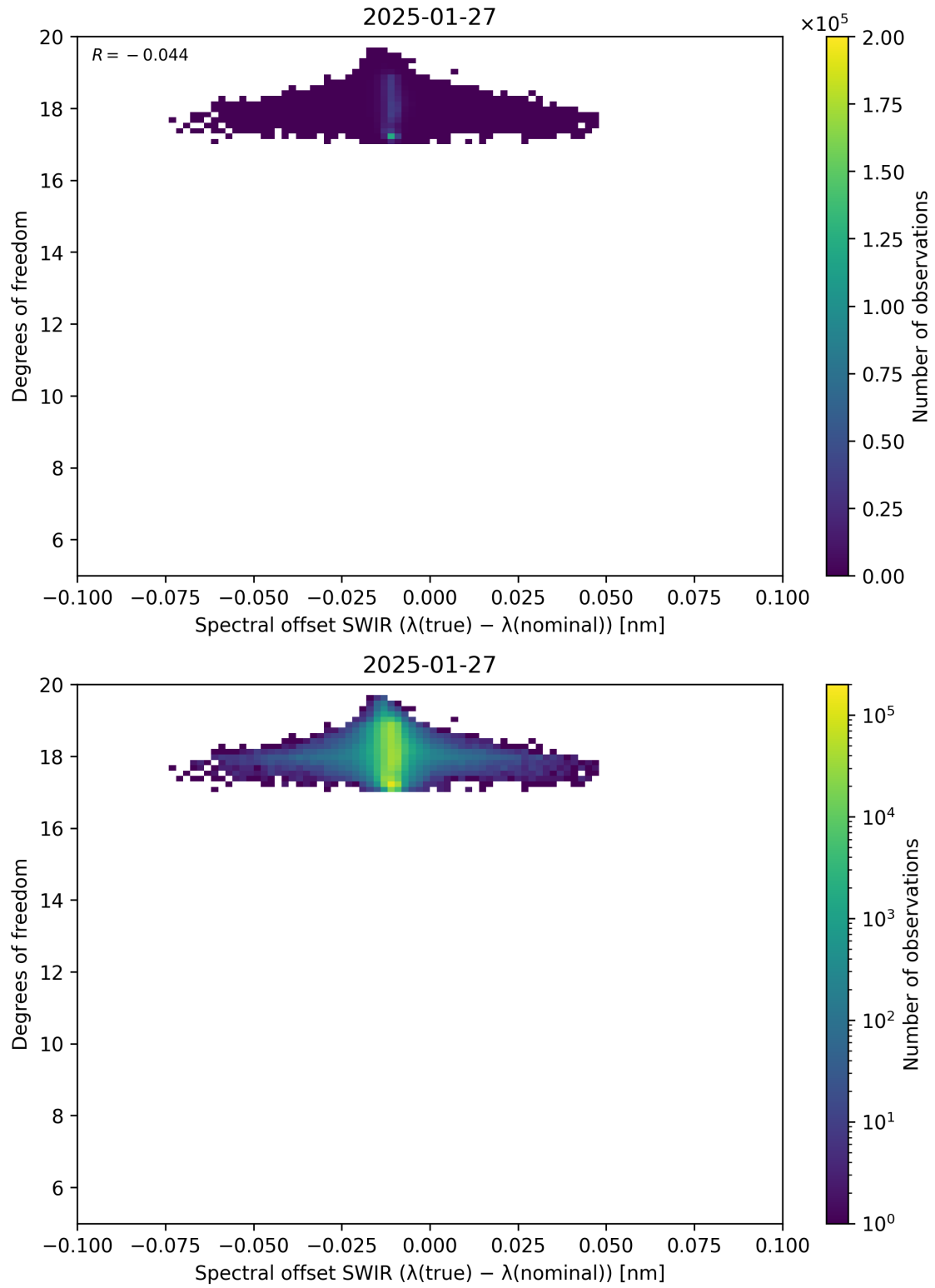
Figure 119: Scatter density plot of “Spectral offset SWIR ( \lambda_{\text{true}} - \lambda_{\text{nominal}} )” against “Degrees of freedom” for 2025-01-26 to 2025-01-28.
