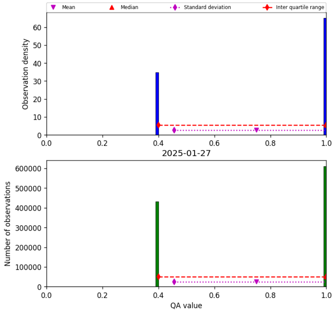
Figure 22: Histogram of “QA value” for 2025-01-26 to 2025-01-28
