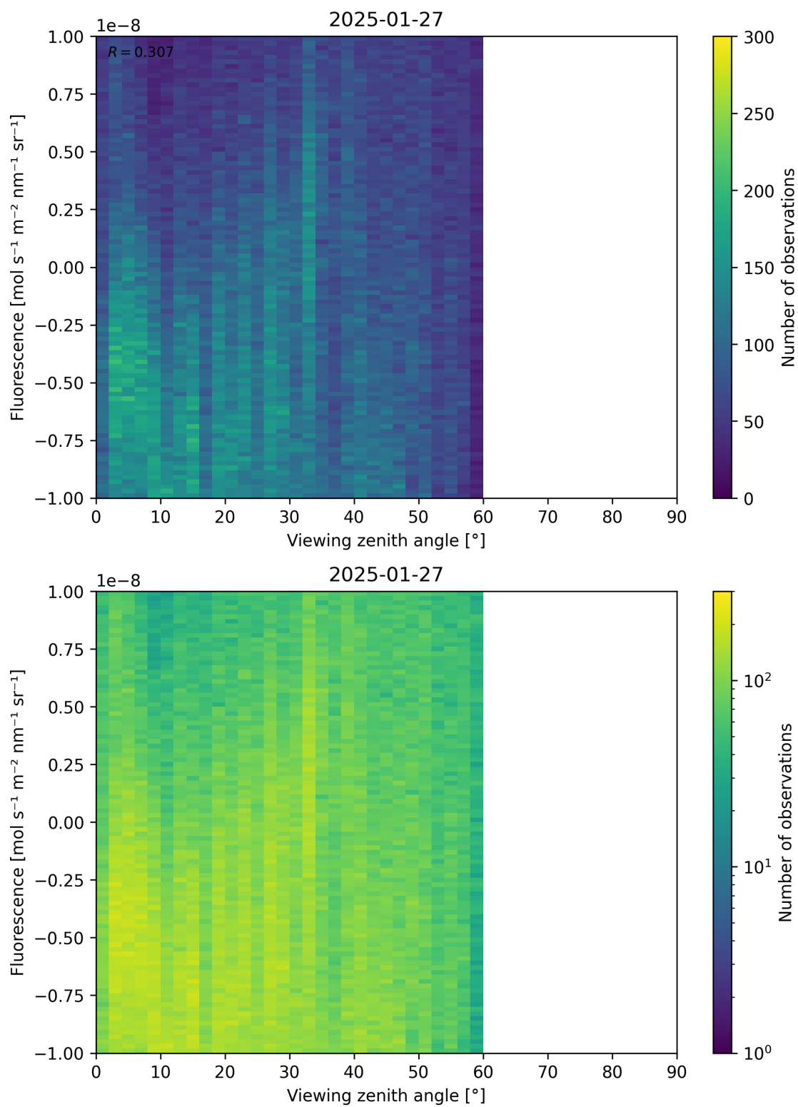
Figure 108: Scatter density plot of “Viewing zenith angle” against “Fluorescence” for 2025-01-26 to 2025-01-28.
