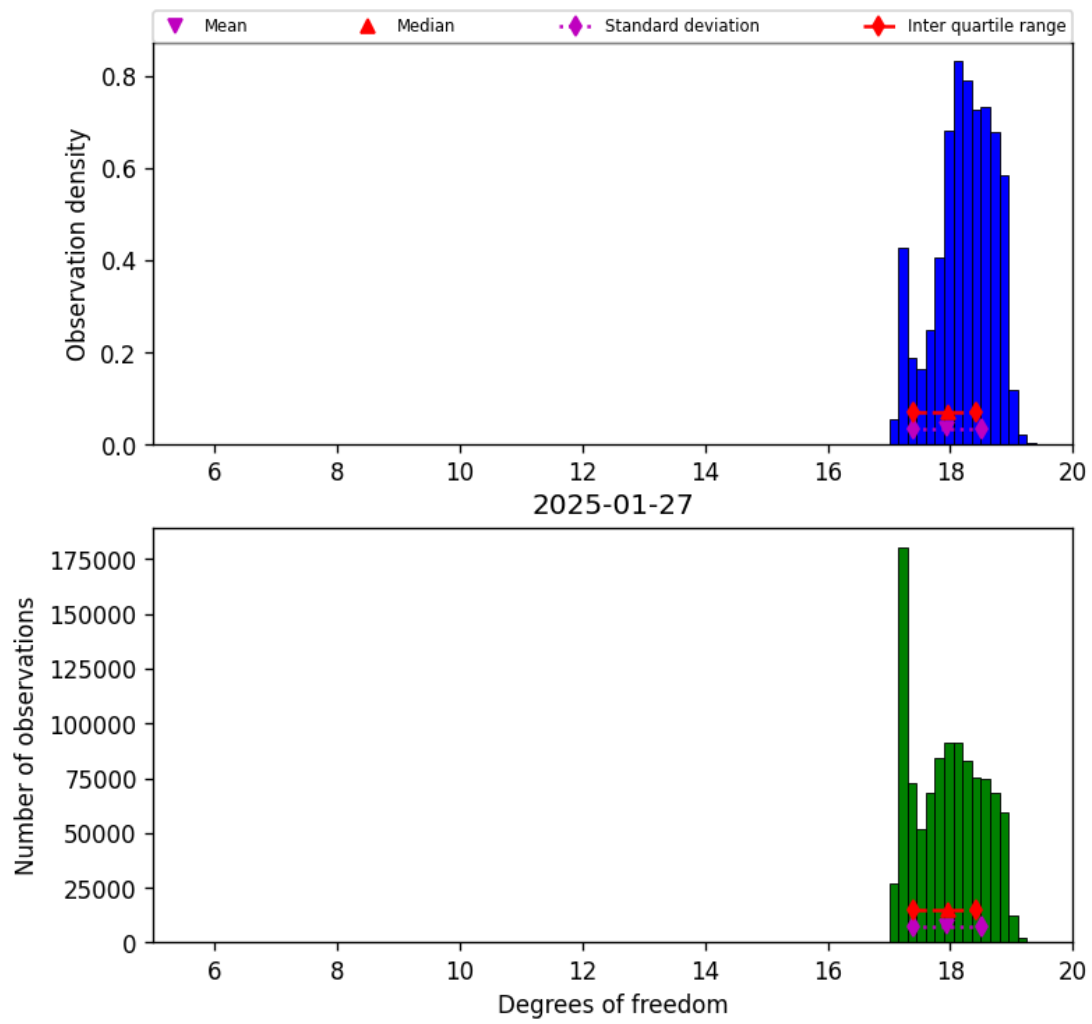
Figure 30: Histogram of “Degrees of freedom” for 2025-01-26 to 2025-01-28
