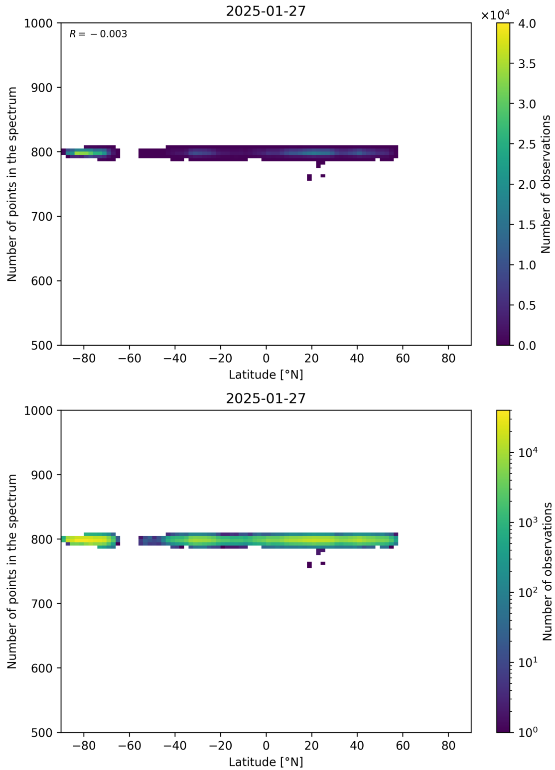
Figure 61: Scatter density plot of “Latitude” against “Number of points in the spectrum” for 2025-01-26 to 2025-01-28.
