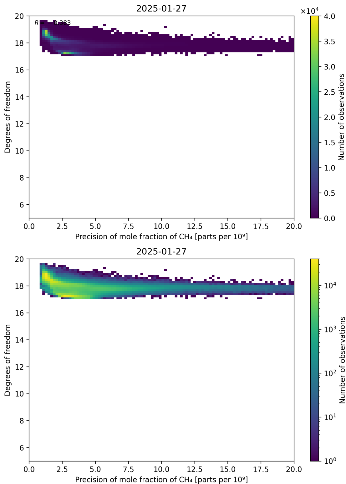
Figure 80: Scatter density plot of “Precision of mole fraction of CH 4 ” against “Degrees of freedom” for 2025-01-26 to 2025-01-28.
