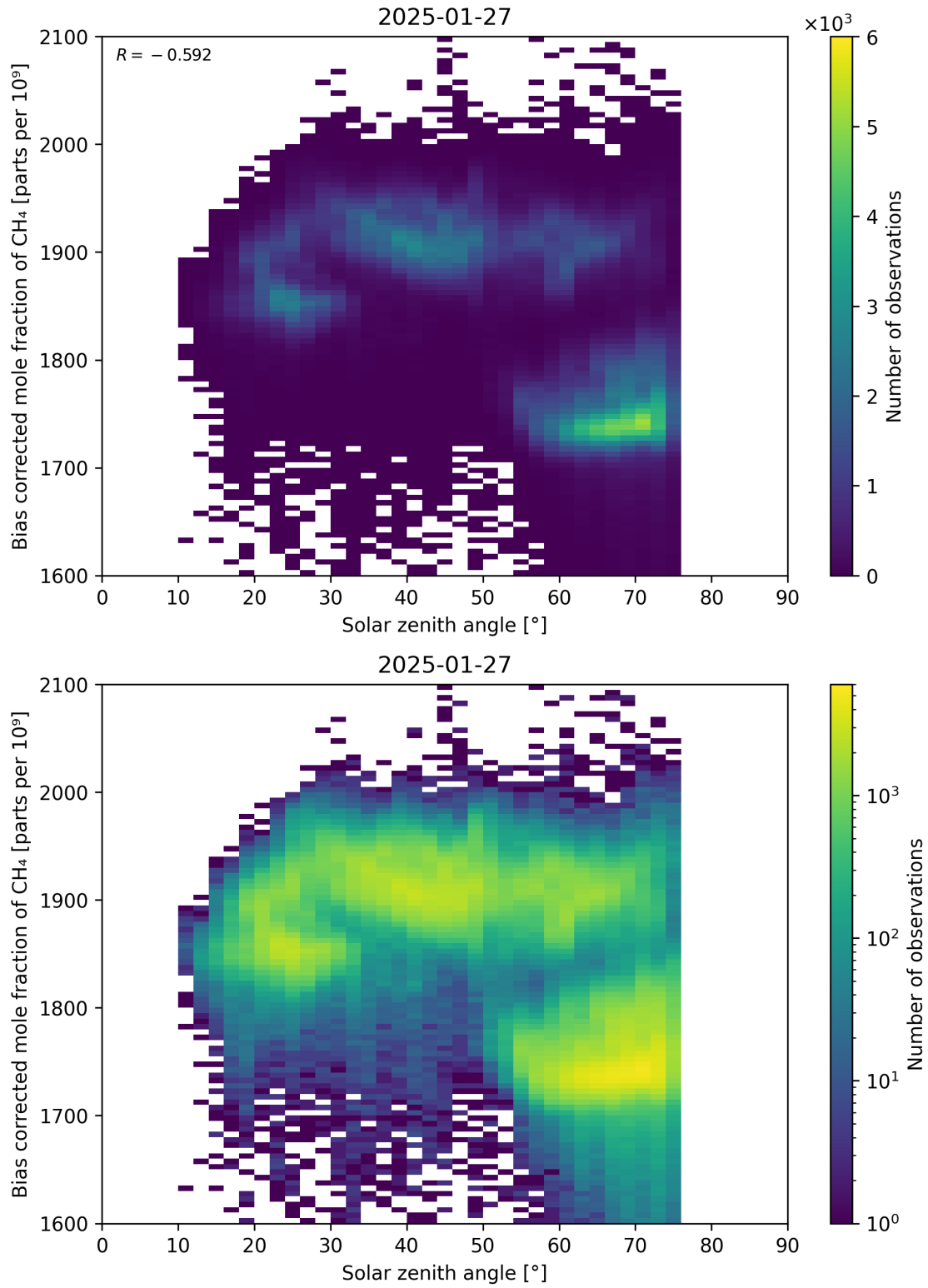
Figure 100: Scatter density plot of “Solar zenith angle” against “Bias corrected mole fraction of CH 4 ” for 2025-01-26 to 2025-01-28.
