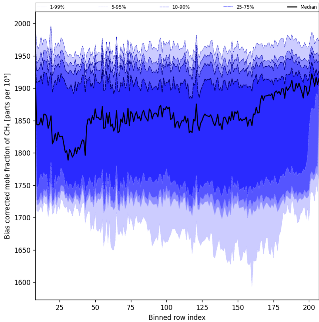
Figure 36: Along track statistics of “Bias corrected mole fraction of CH 4 ” for 2025-01-26 to 2025-01-28
