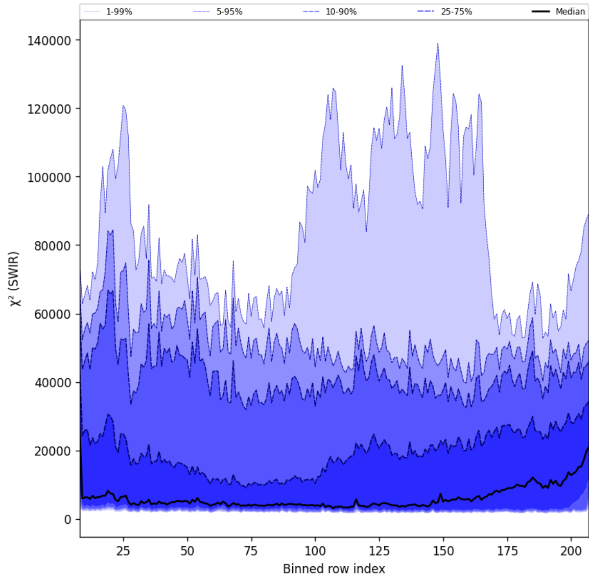
Figure 39: Along track statistics of “ \chi^2 (SWIR)” for 2025-01-26 to 2025-01-28
