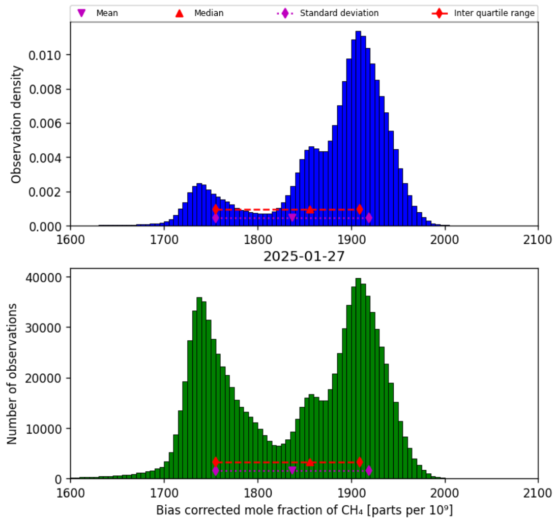
Figure 25: Histogram of “Bias corrected mole fraction of CH 4 ” for 2025-01-26 to 2025-01-28
