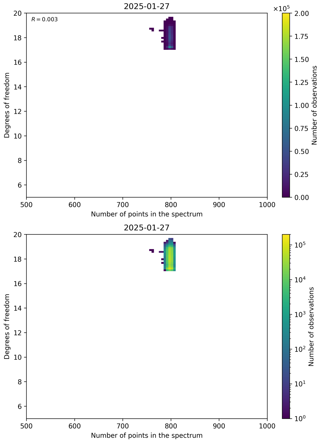
Figure 90: Scatter density plot of “Number of points in the spectrum” against “Degrees of freedom” for 2025-01-26 to 2025-01-28.
