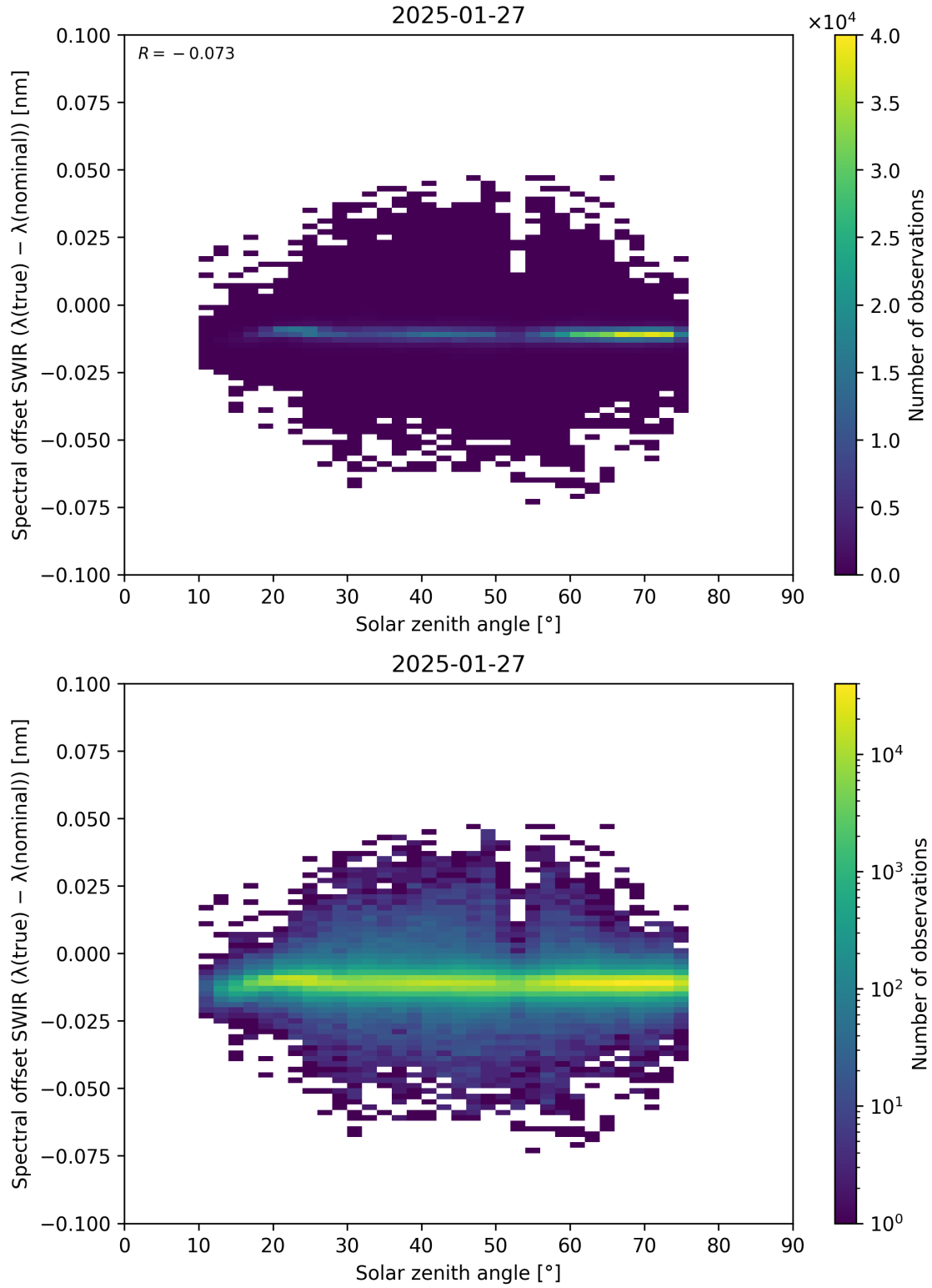
Figure 104: Scatter density plot of “Solar zenith angle” against “Spectral offset SWIR ( \lambda_{\text{true}} - \lambda_{\text{nominal}} )” for 2025-01-26 to 2025-01-28.
