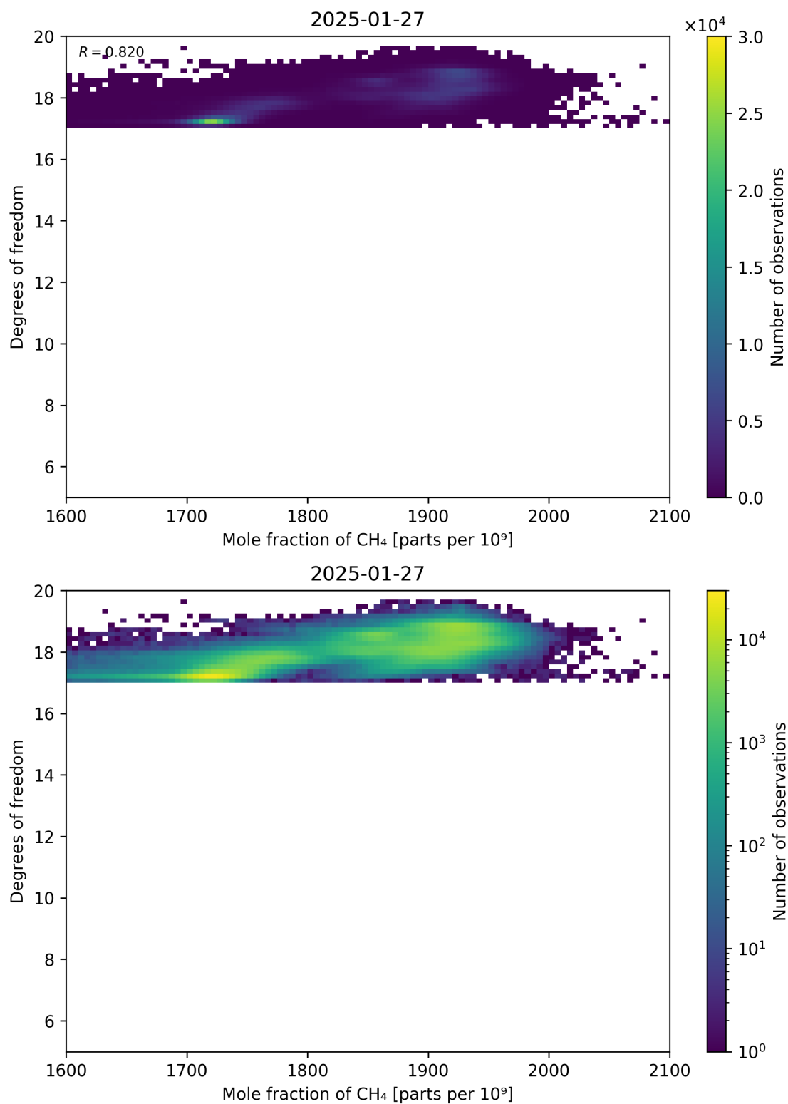
Figure 72: Scatter density plot of “Mole fraction of CH 4 ” against “Degrees of freedom” for 2025-01-26 to 2025-01-28.
