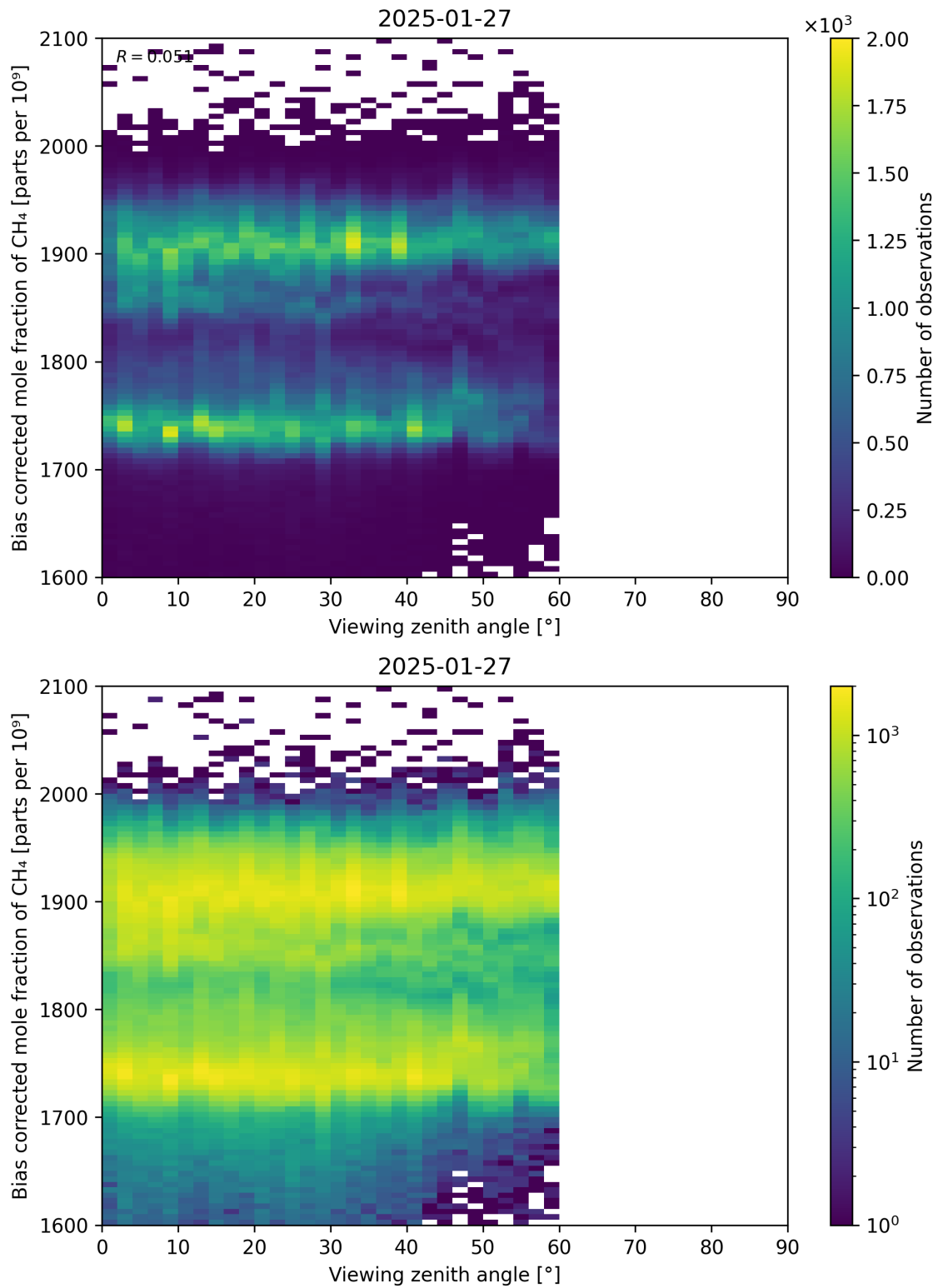
Figure 111: Scatter density plot of “Viewing zenith angle” against “Bias corrected mole fraction of CH 4 ” for 2025-01-26 to 2025-01-28.
