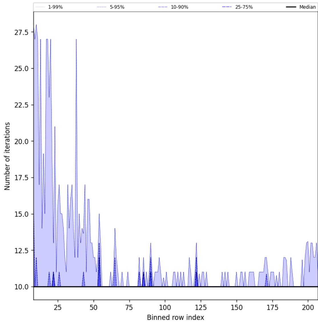
Figure 42: Along track statistics of “Number of iterations” for 2025-01-26 to 2025-01-28
