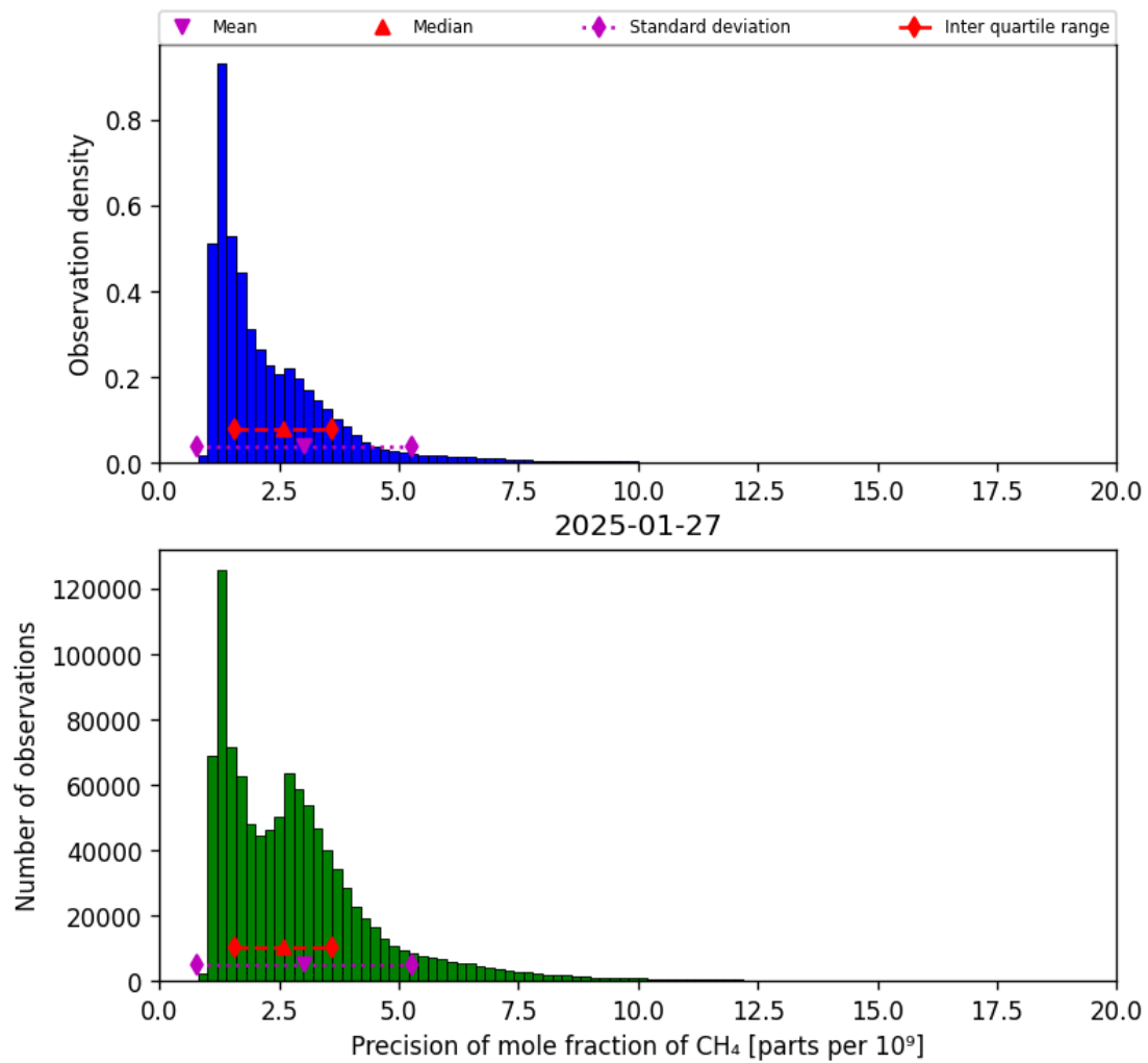
Figure 24: Histogram of “Precision of mole fraction of CH 4 ” for 2025-01-26 to 2025-01-28
