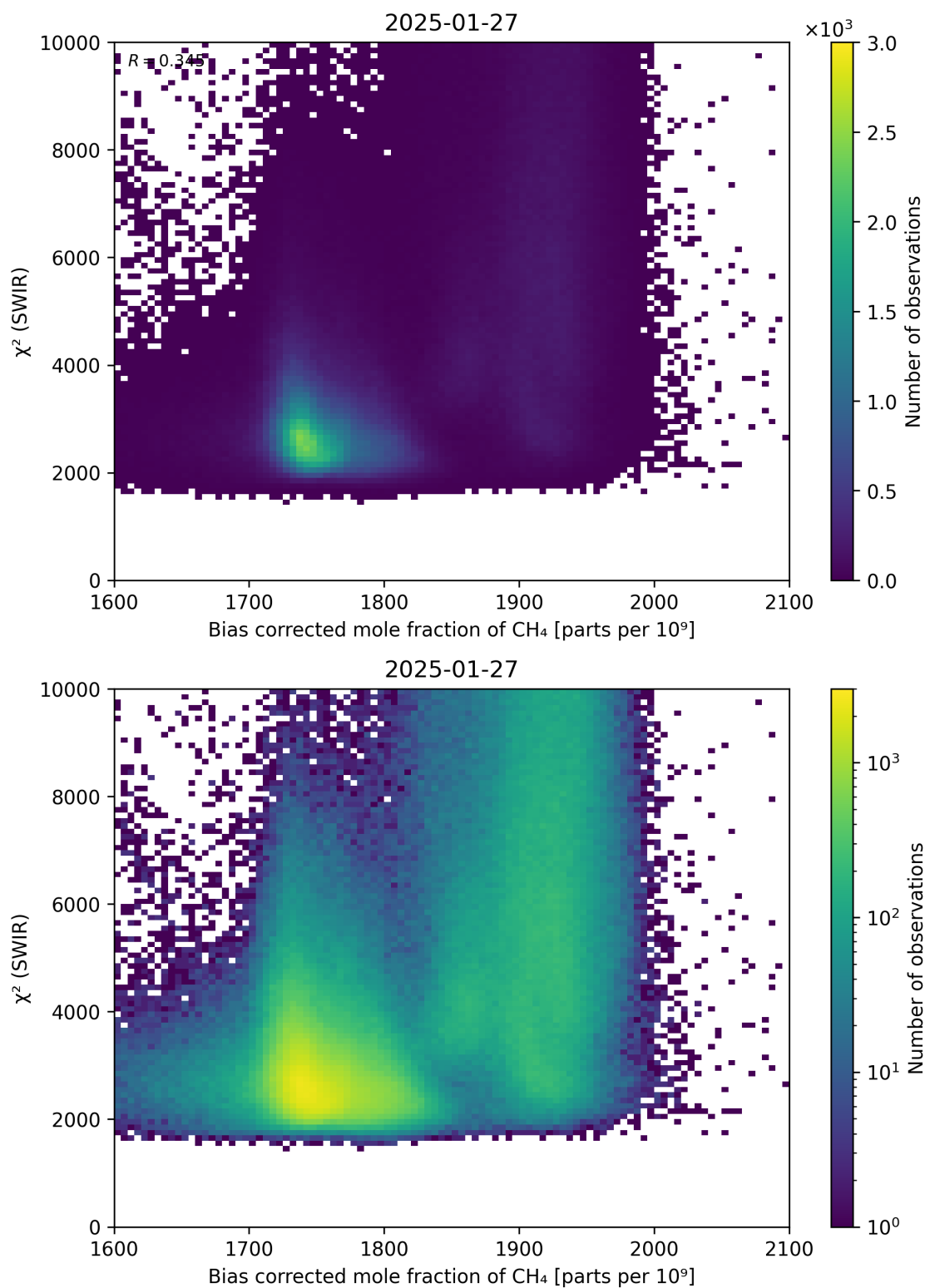
Figure 64: Scatter density plot of “Bias corrected mole fraction of \text{CH}_4 ” against “ \chi^2 (SWIR)” for 2025-01-26 to 2025-01-28.
