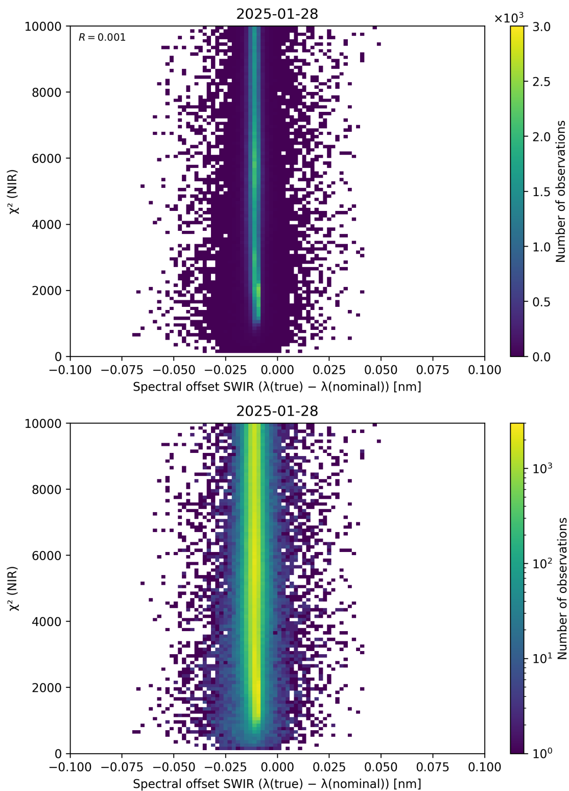
Figure 117: Scatter density plot of “Spectral offset SWIR ( \lambda_{\text{true}} - \lambda_{\text{nominal}} )” against “ \chi^2 (NIR)” for 2025-01-28 to 2025-01-29.
