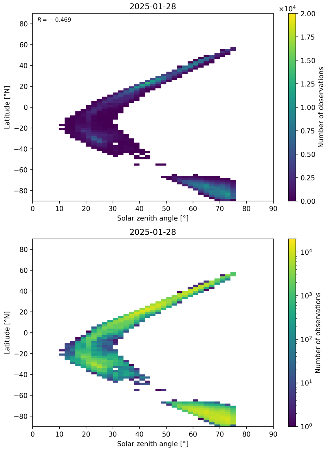
Figure 98: Scatter density plot of “Solar zenith angle” against “Latitude” for 2025-01-28 to 2025-01-29.
