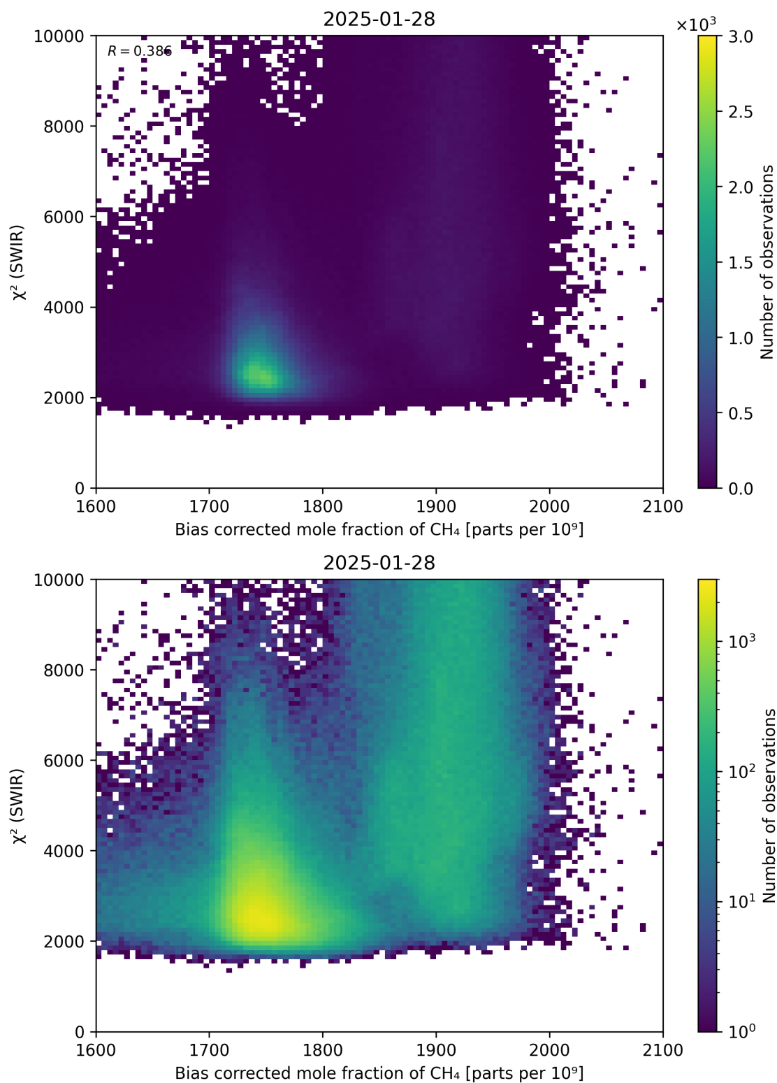
Figure 64: Scatter density plot of “Bias corrected mole fraction of CH 4 ” against “ \chi^2 (SWIR)” for 2025-01-28 to 2025-01-29.
