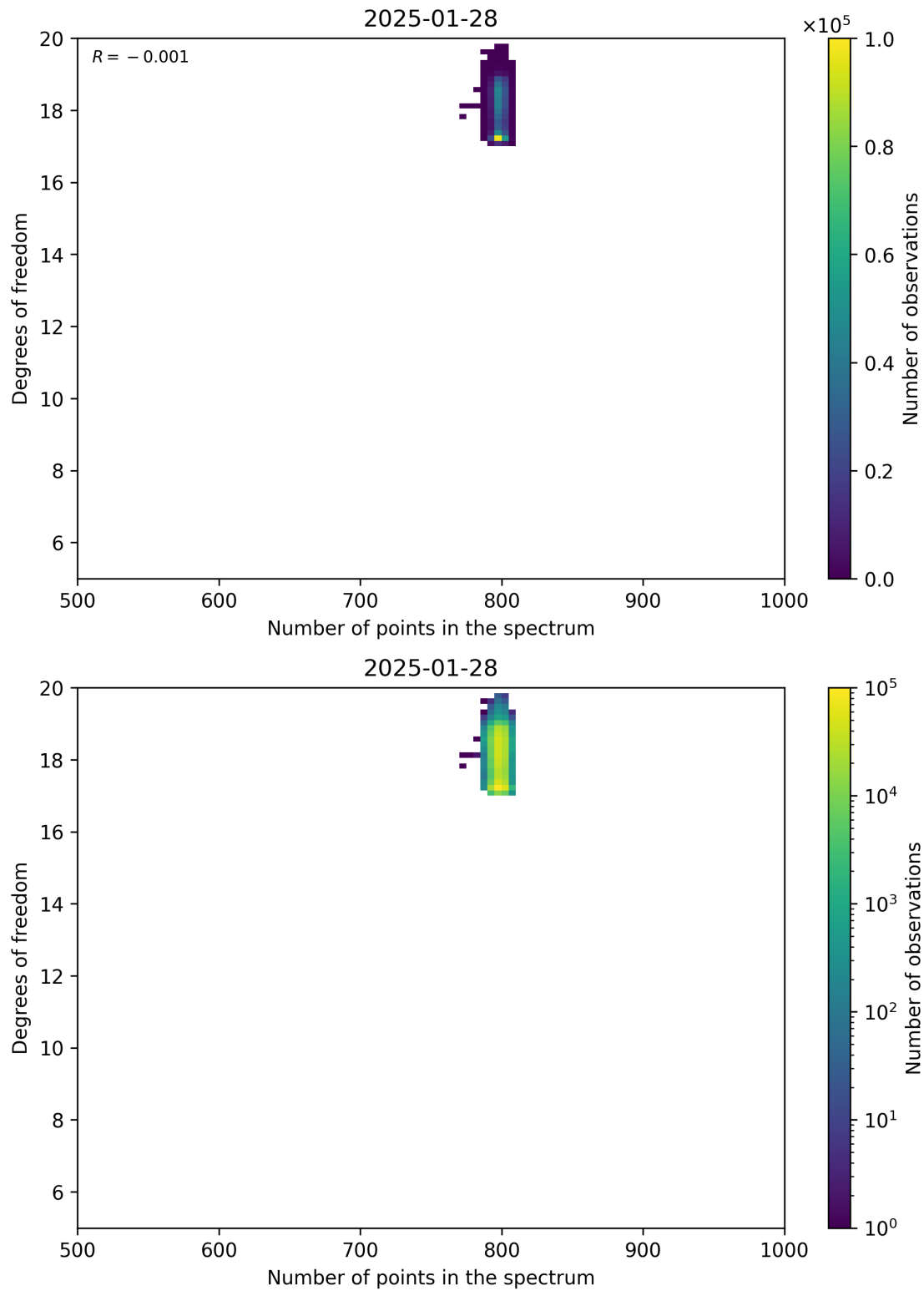
Figure 90: Scatter density plot of “Number of points in the spectrum” against “Degrees of freedom” for 2025-01-28 to 2025-01-29.
