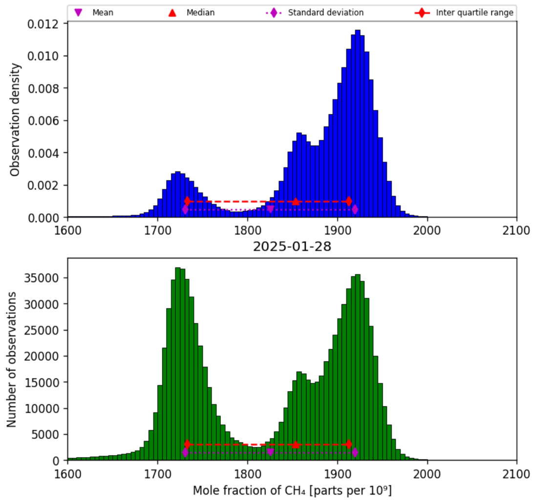
Figure 23: Histogram of “Mole fraction of CH 4 ” for 2025-01-28 to 2025-01-29
