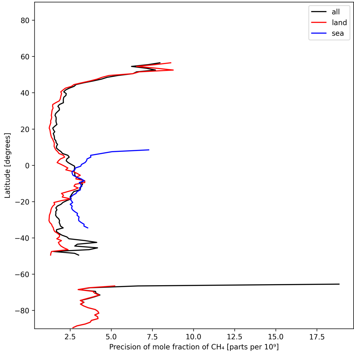
Figure 13: Zonal average of “Precision of mole fraction of CH 4 ” for 2025-01-28 to 2025-01-29.
