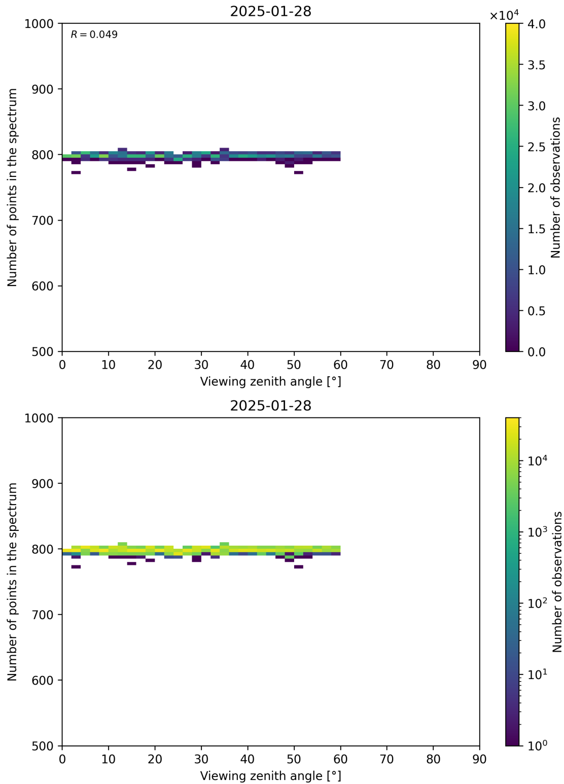
Figure 114: Scatter density plot of “Viewing zenith angle” against “Number of points in the spectrum” for 2025-01-28 to 2025-01-29.
