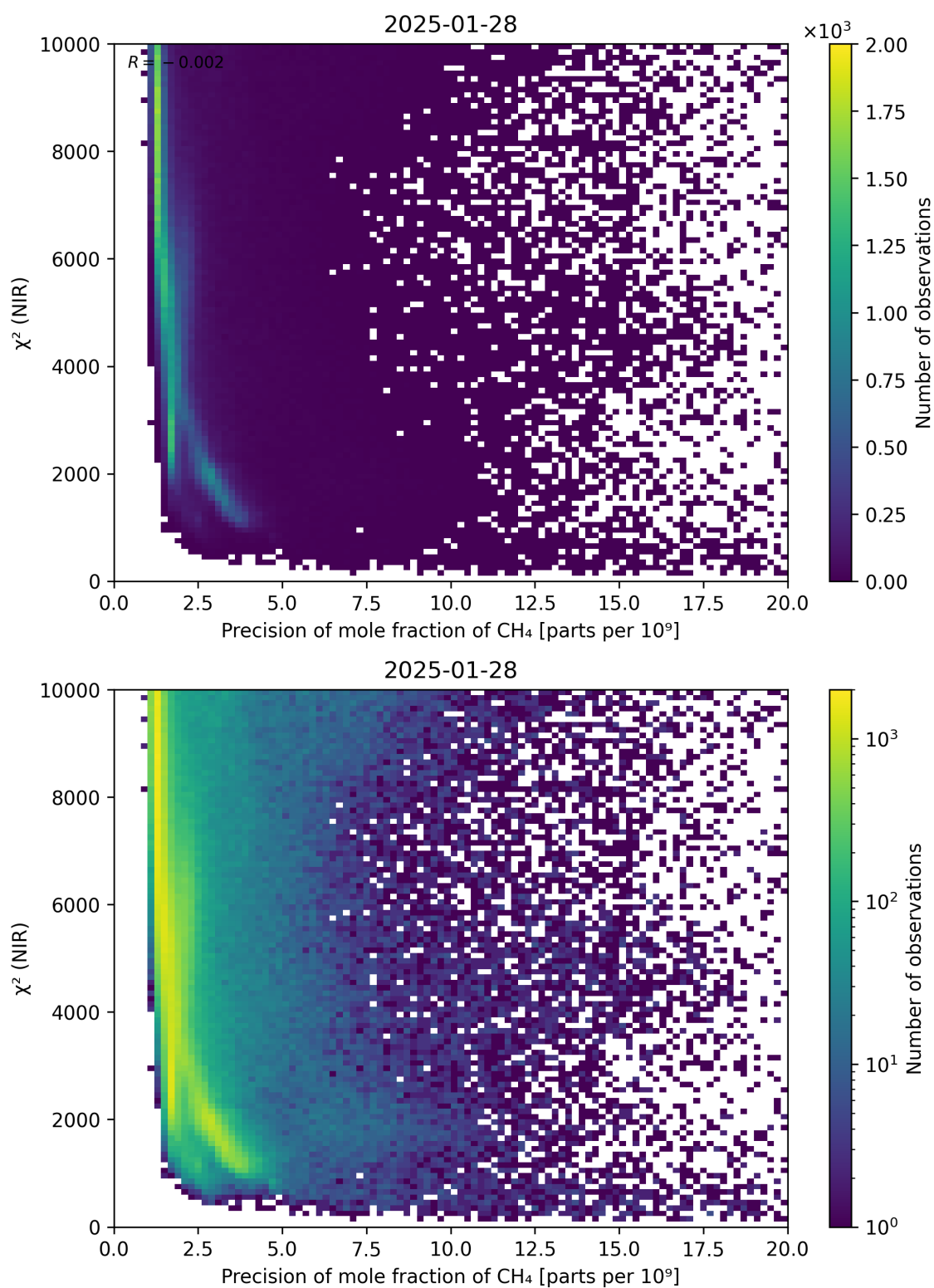
Figure 78: Scatter density plot of “Precision of mole fraction of CH 4 ” against “ \chi^2 (NIR)” for 2025-01-28 to 2025-01-29.
