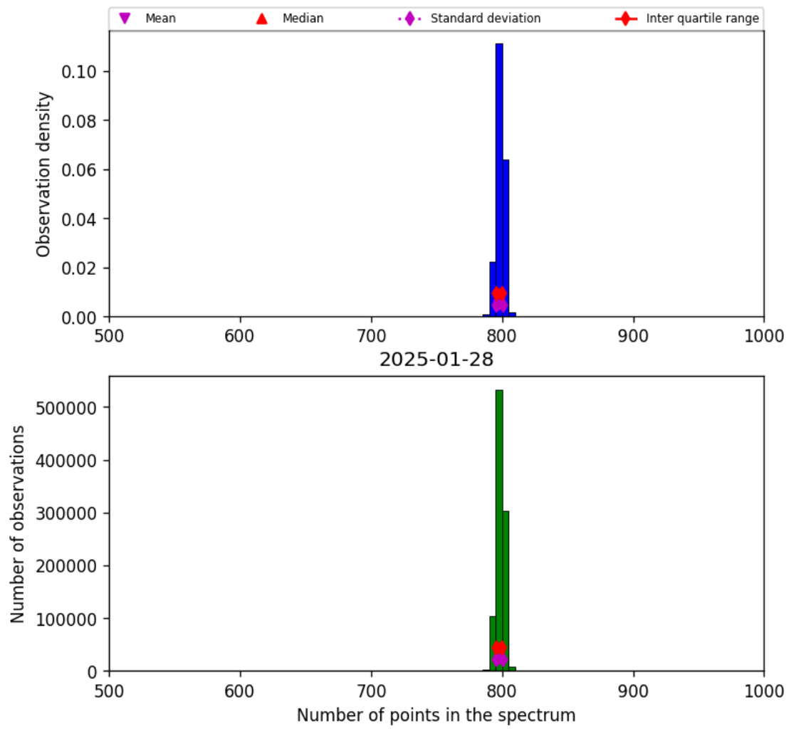
Figure 26: Histogram of “Number of points in the spectrum” for 2025-01-28 to 2025-01-29
