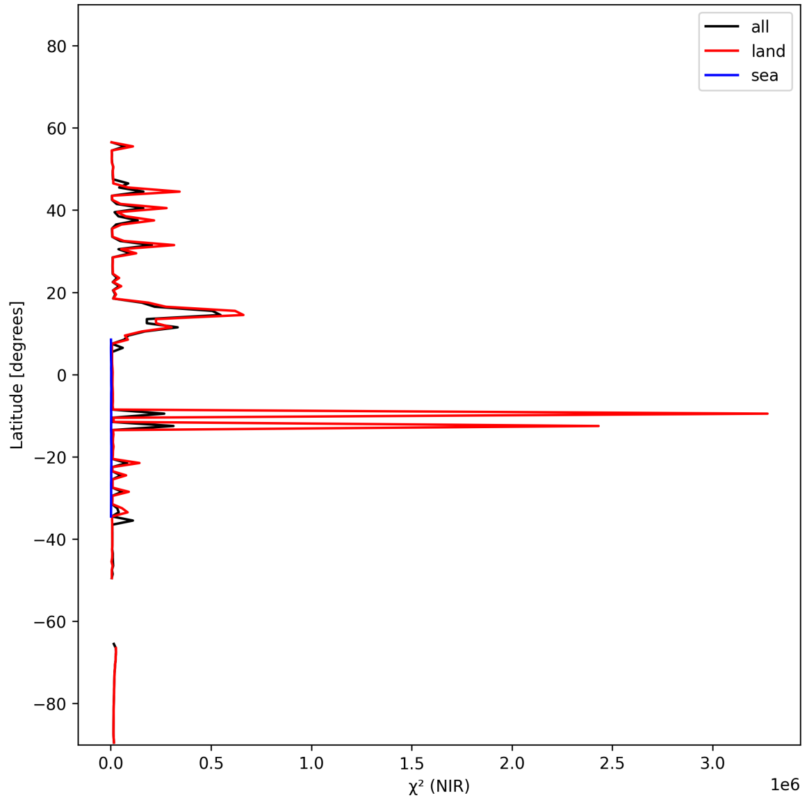
Figure 18: Zonal average of “ \chi^2 (NIR)” for 2025-01-28 to 2025-01-29.
