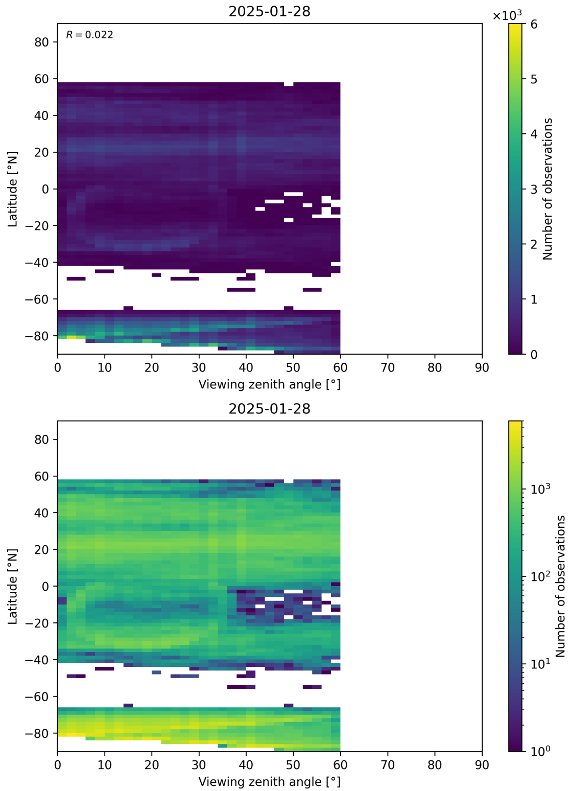
Figure 109: Scatter density plot of “Viewing zenith angle” against “Latitude” for 2025-01-28 to 2025-01-29.
