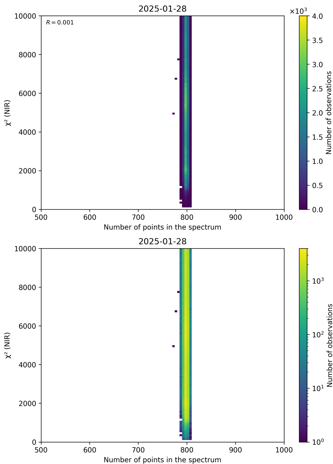
Figure 88: Scatter density plot of “Number of points in the spectrum” against “ \chi^2 (NIR)” for 2025-01-28 to 2025-01-29.
