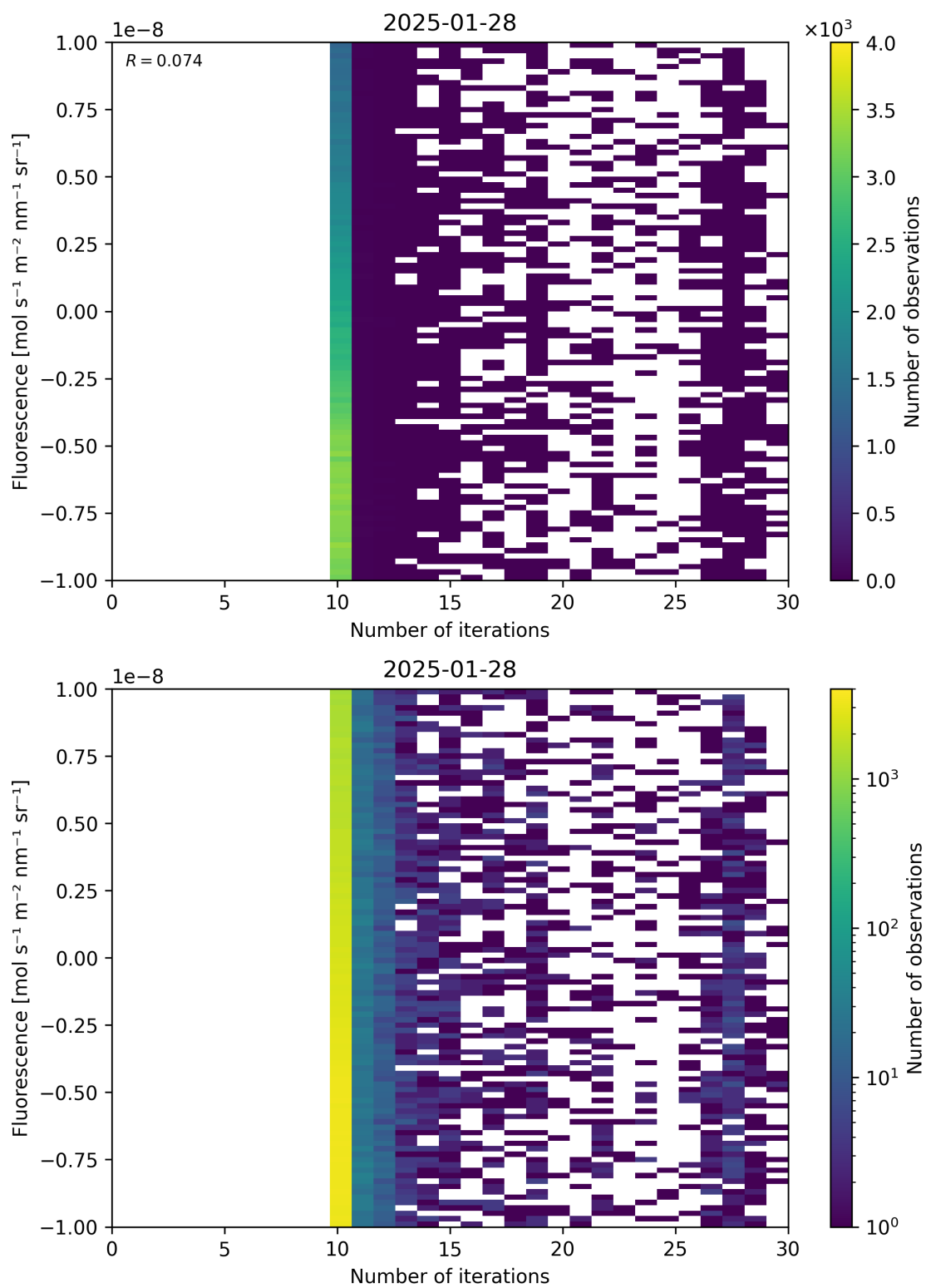
Figure 87: Scatter density plot of “Number of iterations” against “Fluorescence” for 2025-01-28 to 2025-01-29.
