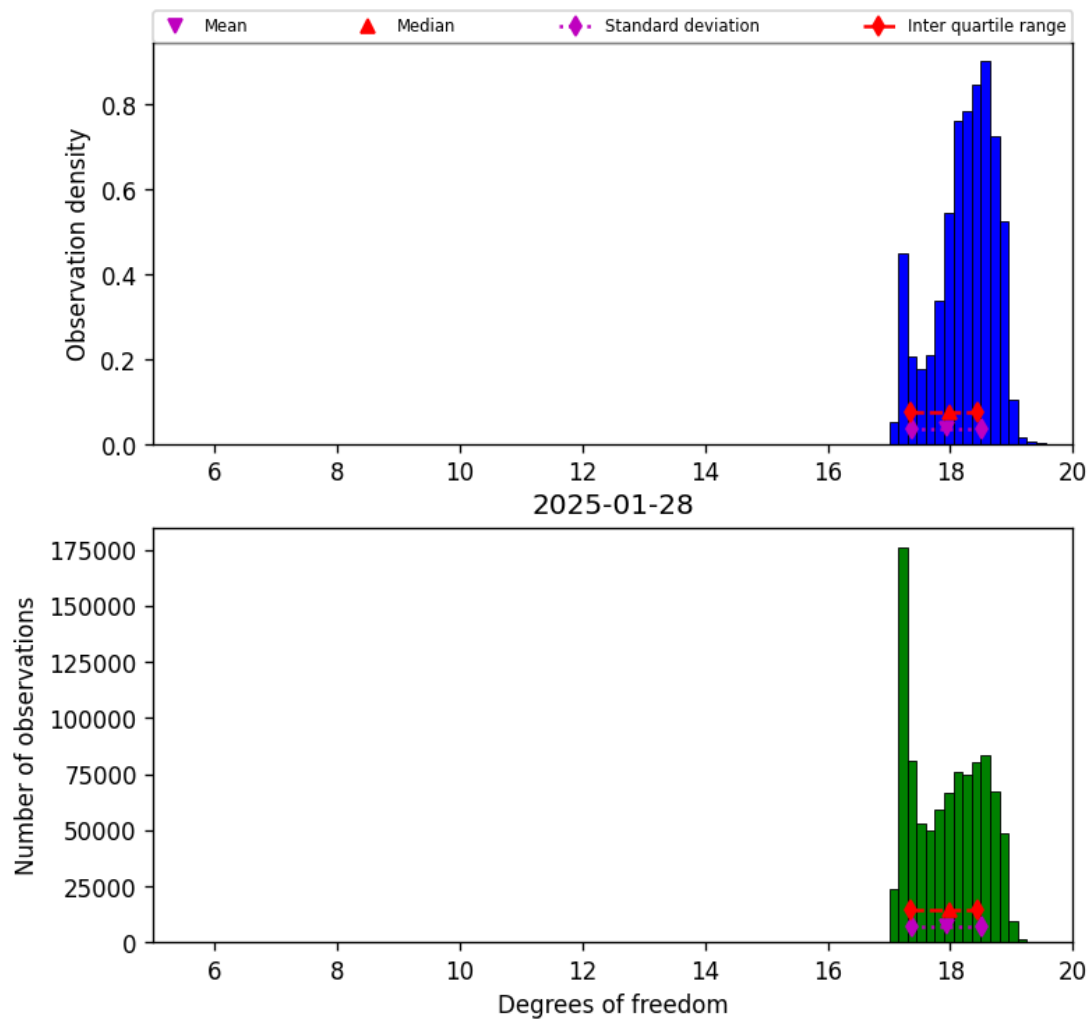
Figure 30: Histogram of “Degrees of freedom” for 2025-01-28 to 2025-01-29
