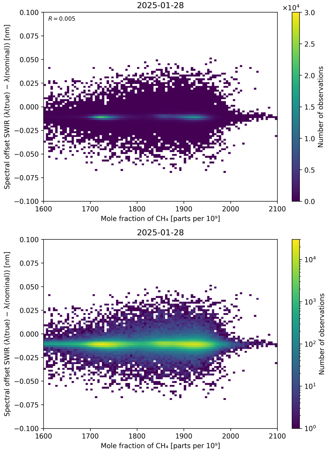
Figure 86: Scatter density plot of “Mole fraction of CH 4 ” against “Spectral offset SWIR ( \lambda_{\text{true}} - \lambda_{\text{nominal}} )” for 2025-01-28 to 2025-01-29.
