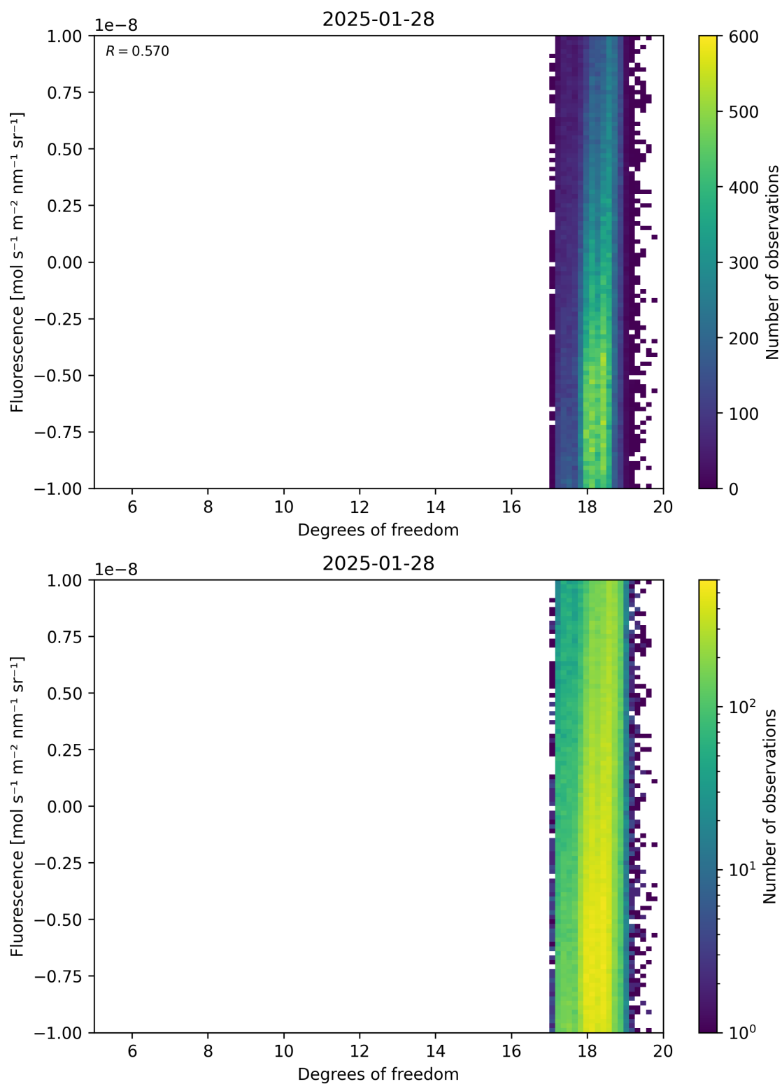
Figure 51: Scatter density plot of “Degrees of freedom” against “Fluorescence” for 2025-01-28 to 2025-01-29.
