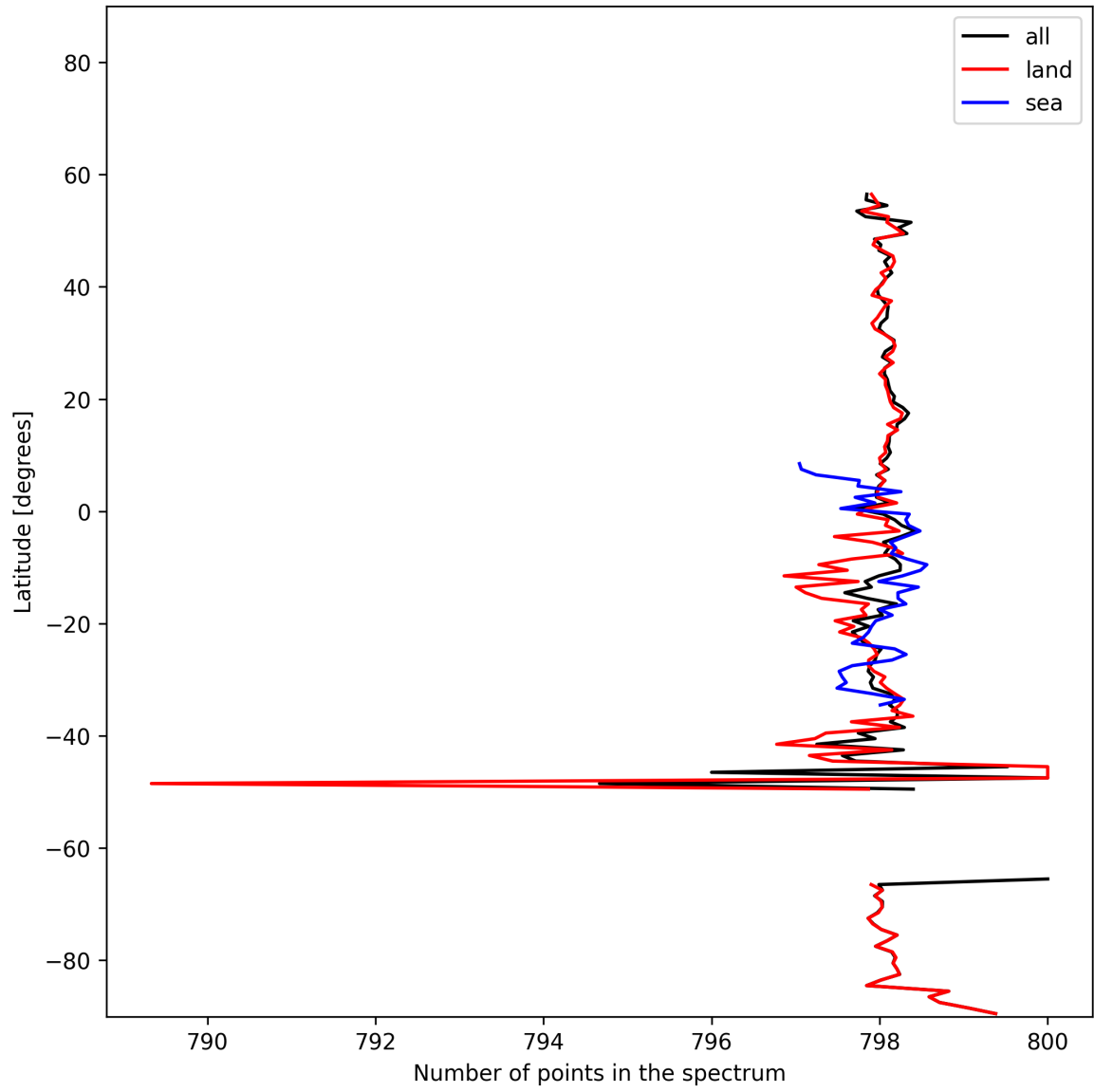
Figure 15: Zonal average of “Number of points in the spectrum” for 2025-01-28 to 2025-01-29.
