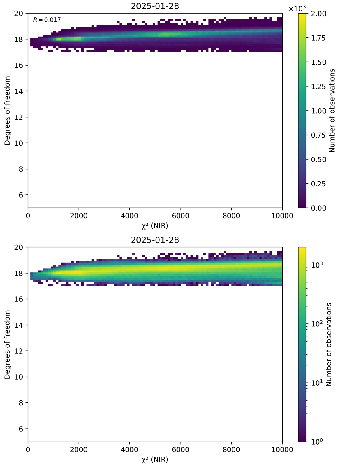
Figure 44: Scatter density plot of “ \chi^2 (NIR)” against “Degrees of freedom” for 2025-01-28 to 2025-01-29.
