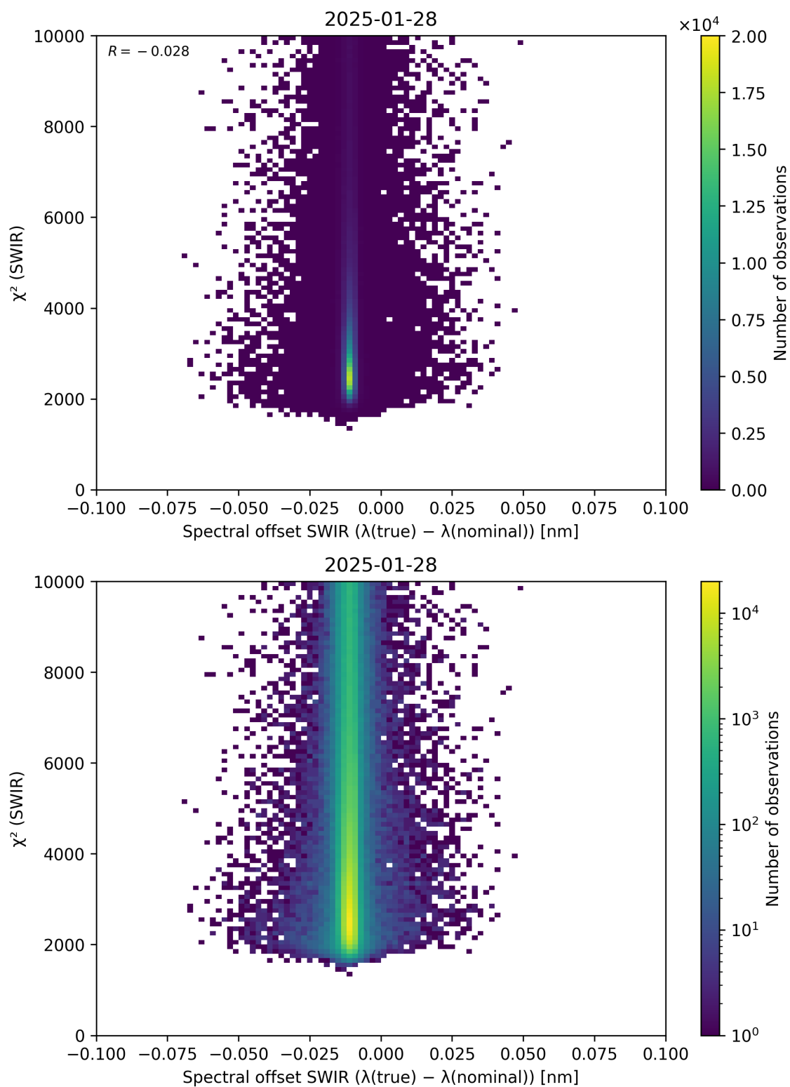
Figure 118: Scatter density plot of “Spectral offset SWIR ( \lambda_{\text{true}} - \lambda_{\text{nominal}} )” against “ \chi^2 (SWIR)” for 2025-01-28 to 2025-01-29.
