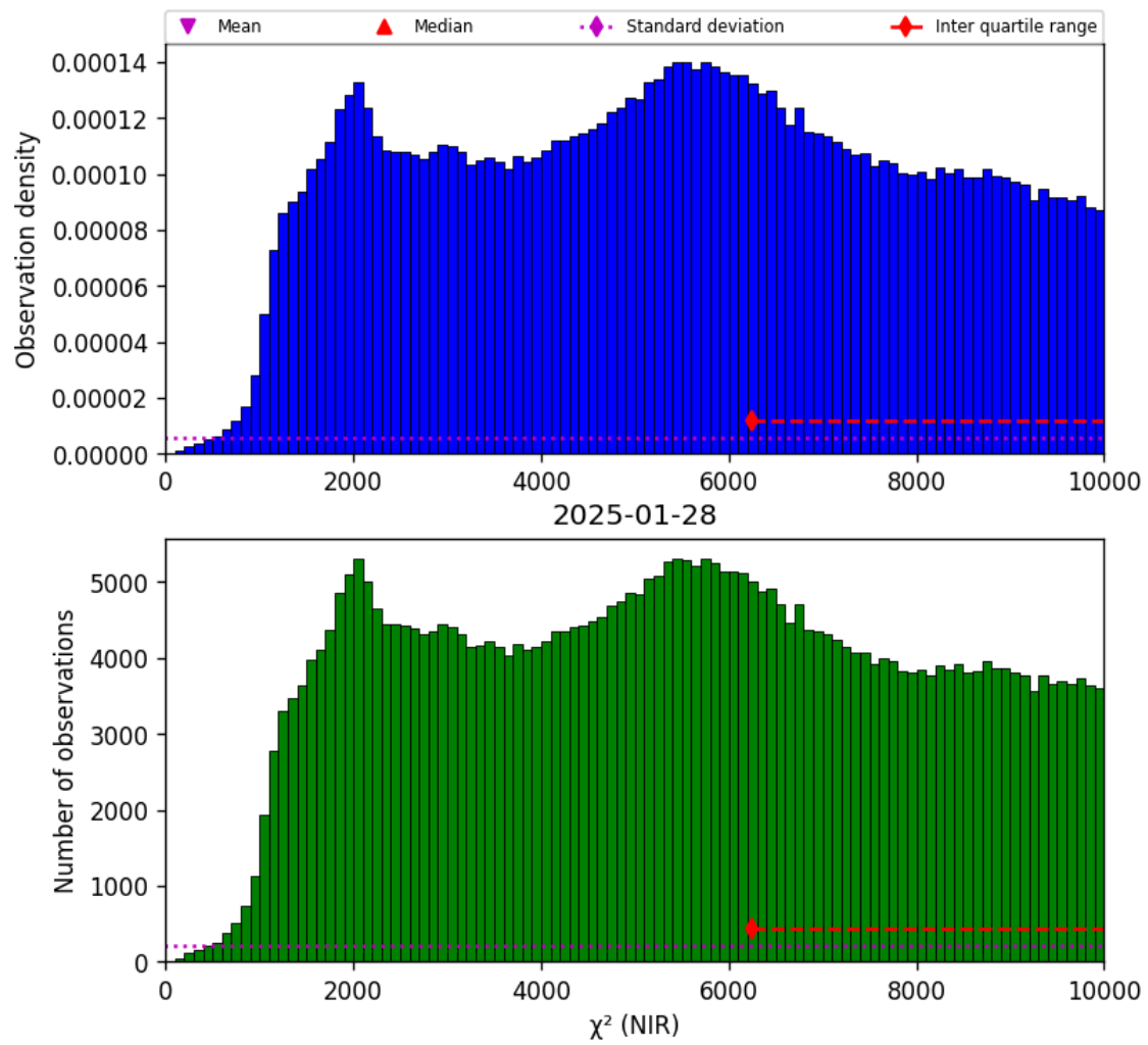
Figure 29: Histogram of “ \chi^2 (NIR)” for 2025-01-28 to 2025-01-29
