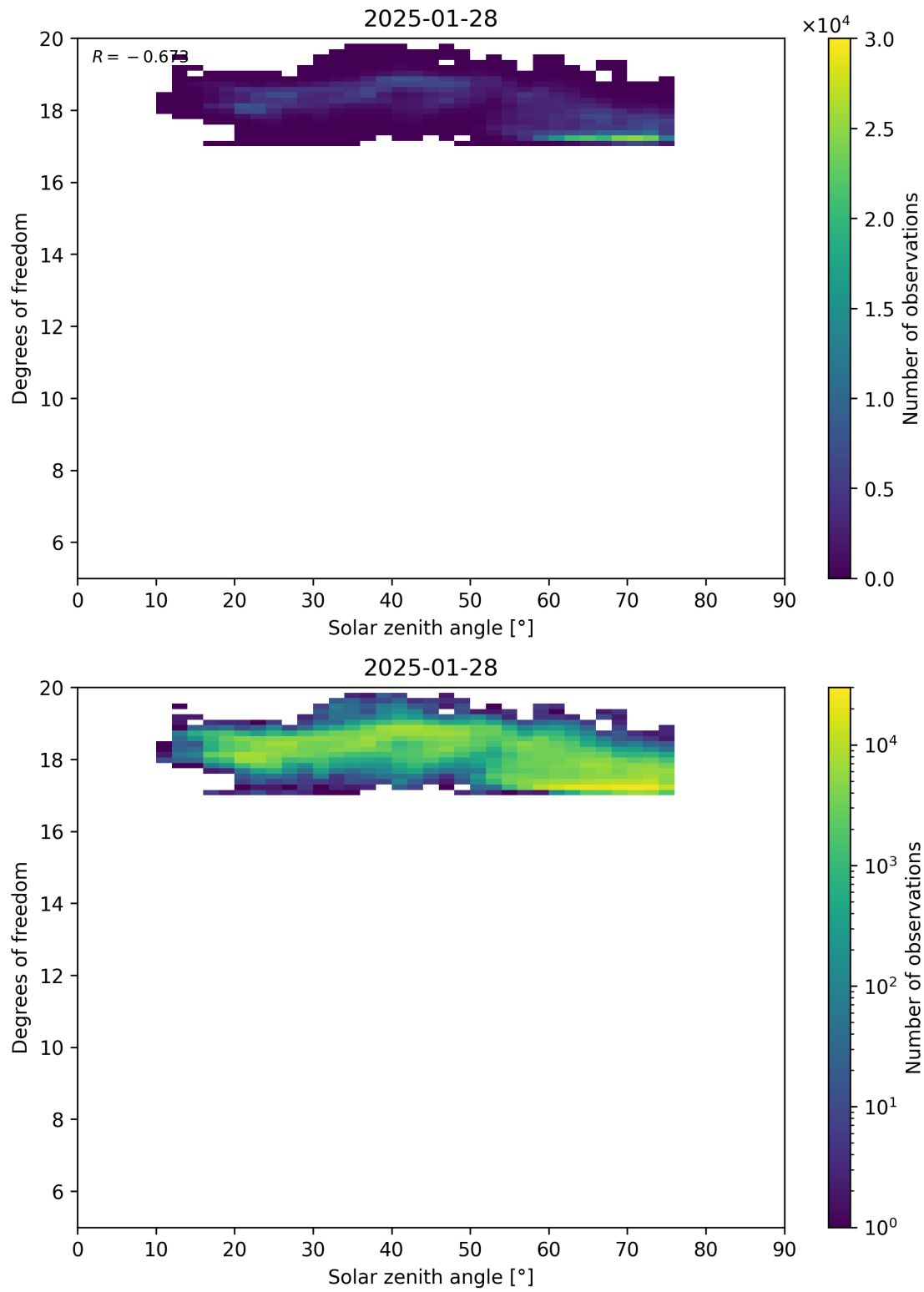
Figure 96: Scatter density plot of “Solar zenith angle” against “Degrees of freedom” for 2025-01-28 to 2025-01-29.
