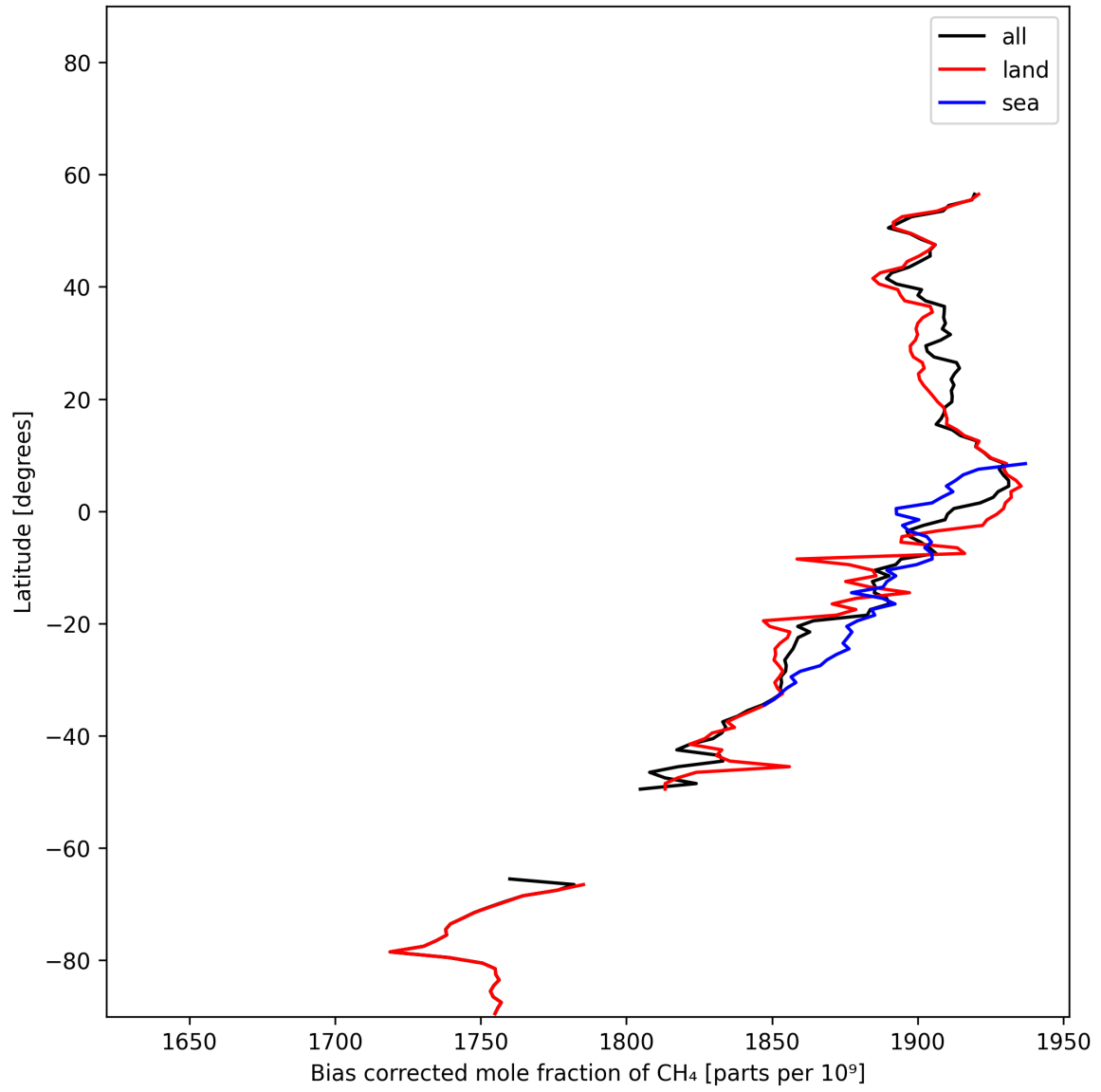
Figure 14: Zonal average of “Bias corrected mole fraction of CH 4 ” for 2025-01-28 to 2025-01-29.
