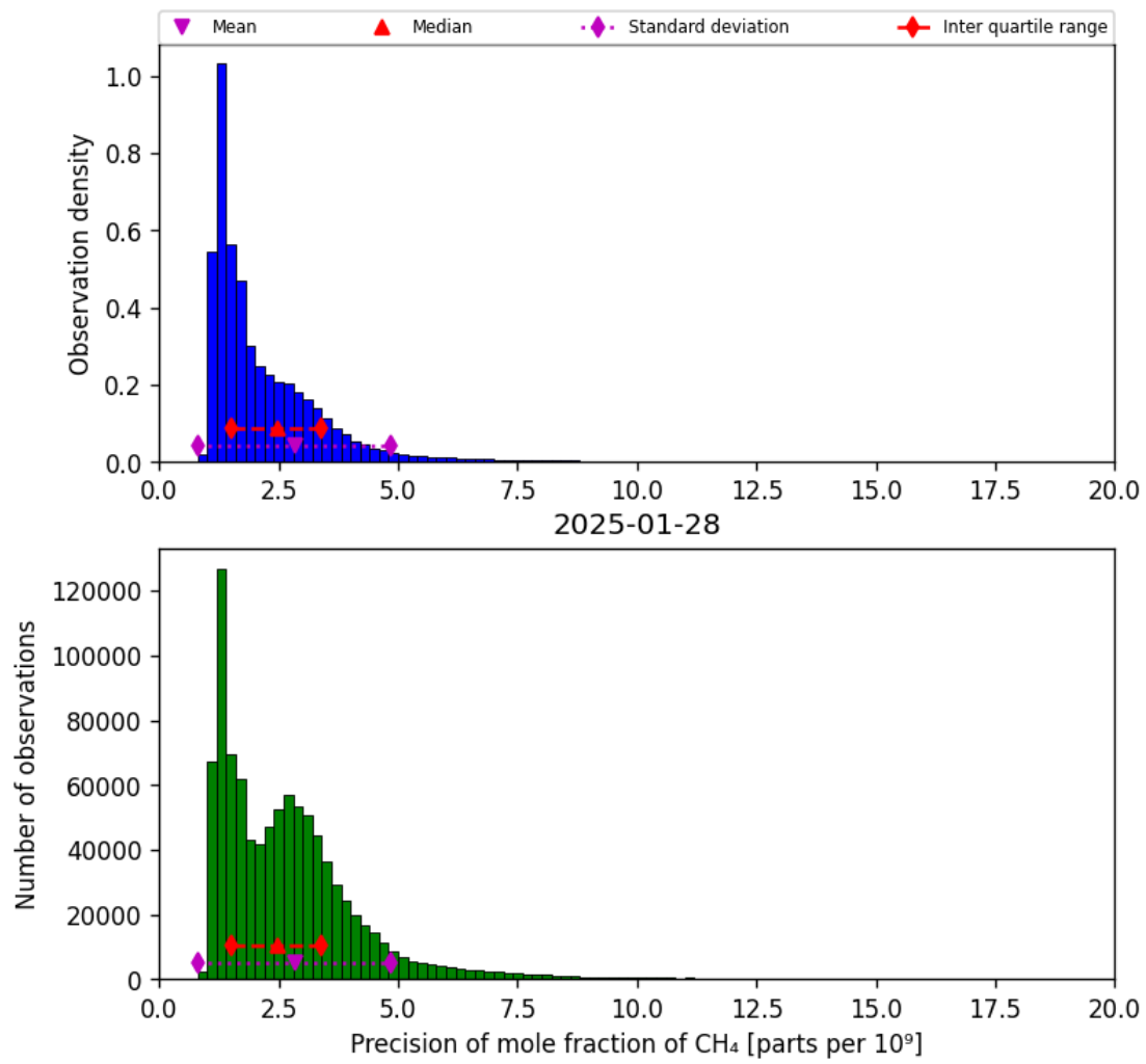
Figure 24: Histogram of “Precision of mole fraction of CH 4 ” for 2025-01-28 to 2025-01-29
