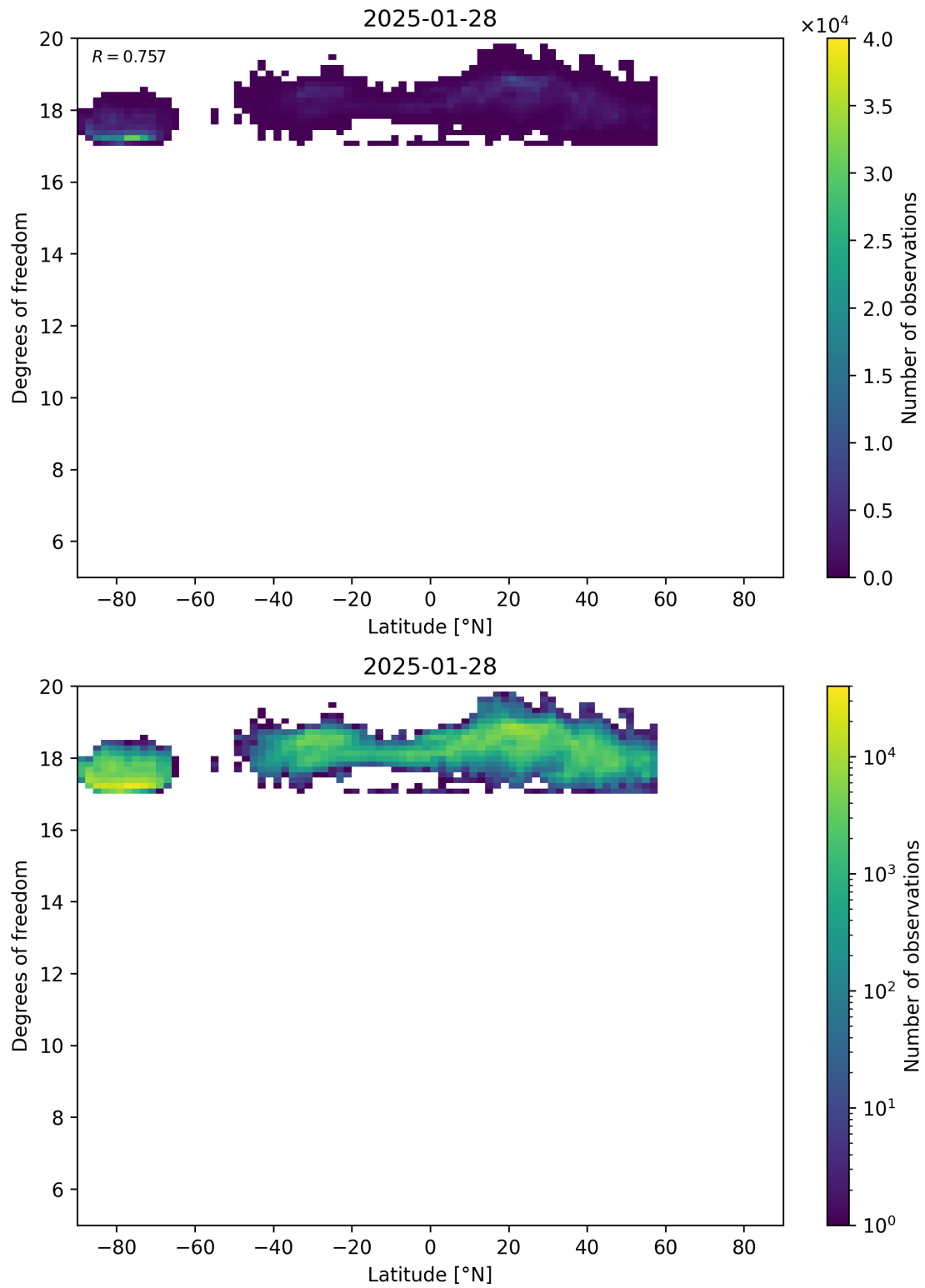
Figure 55: Scatter density plot of “Latitude” against “Degrees of freedom” for 2025-01-28 to 2025-01-29.
