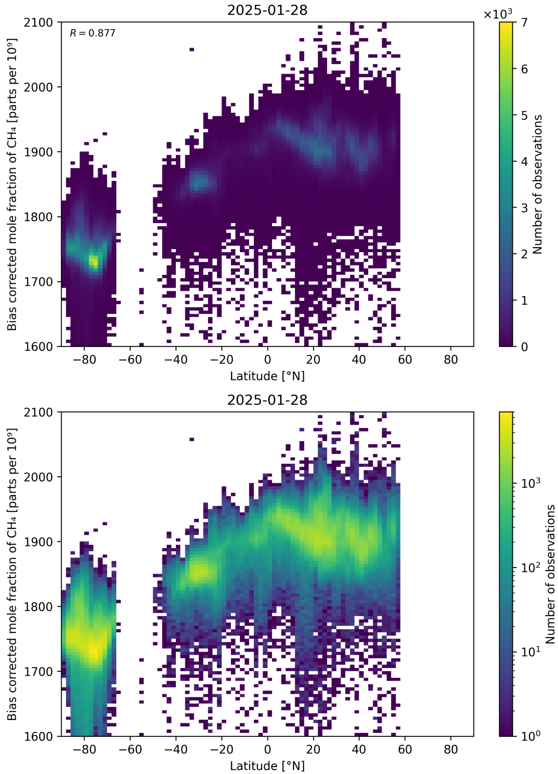
Figure 58: Scatter density plot of “Latitude” against “Bias corrected mole fraction of \text{CH}_4 ” for 2025-01-28 to 2025-01-29.
