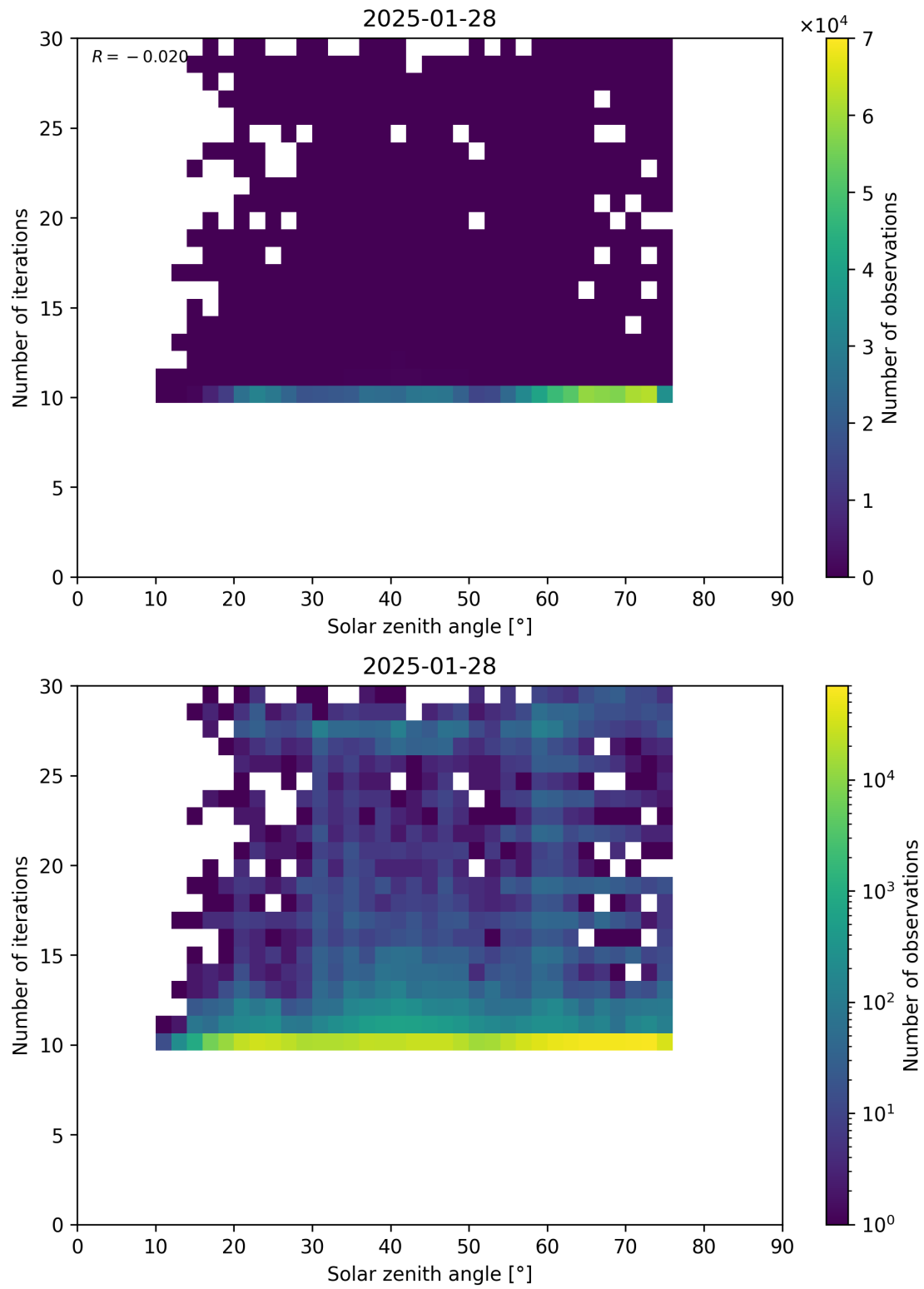
Figure 102: Scatter density plot of “Solar zenith angle” against “Number of iterations” for 2025-01-28 to 2025-01-29.
