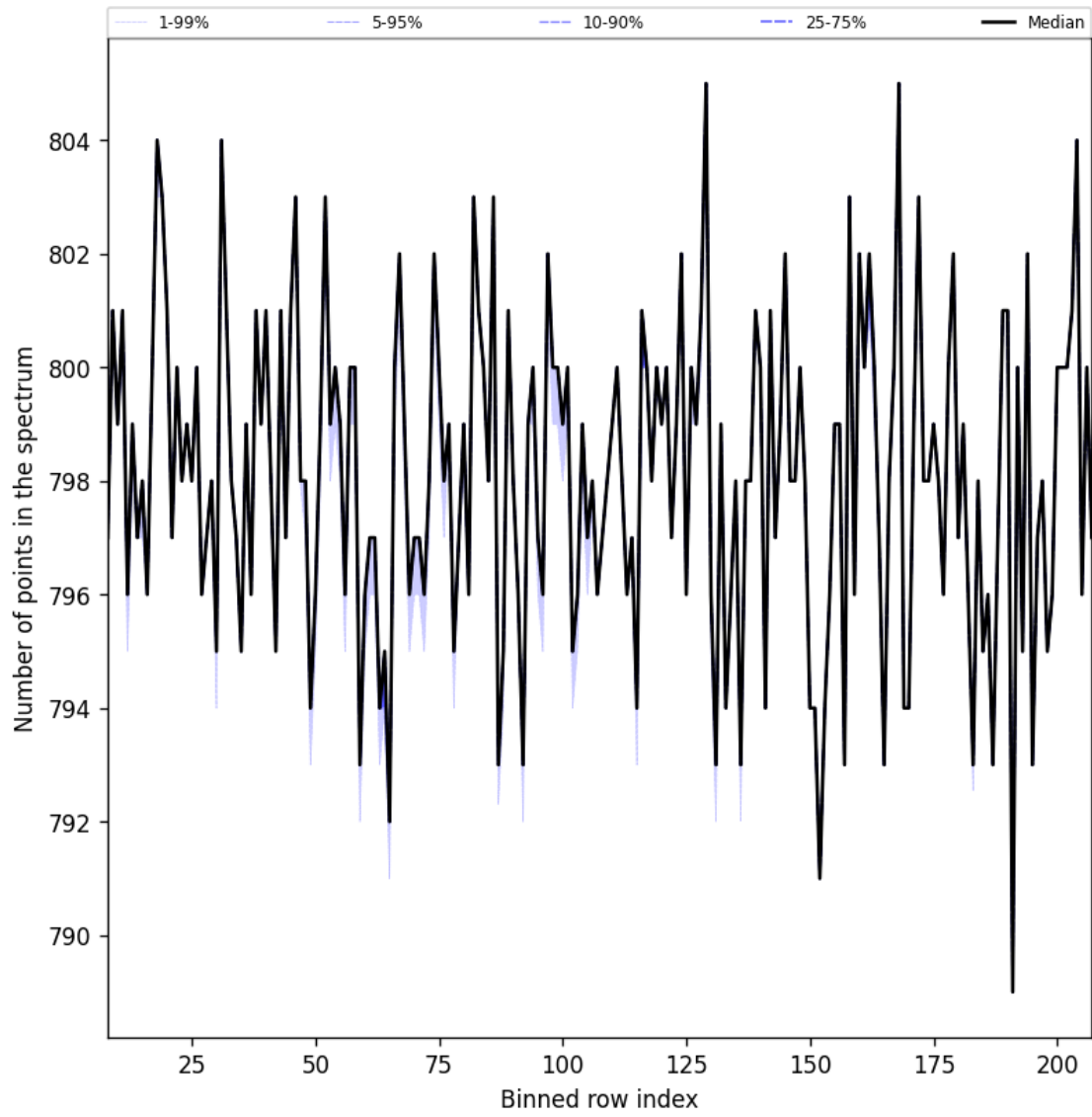
Figure 37: Along track statistics of “Number of points in the spectrum” for 2025-01-28 to 2025-01-29
