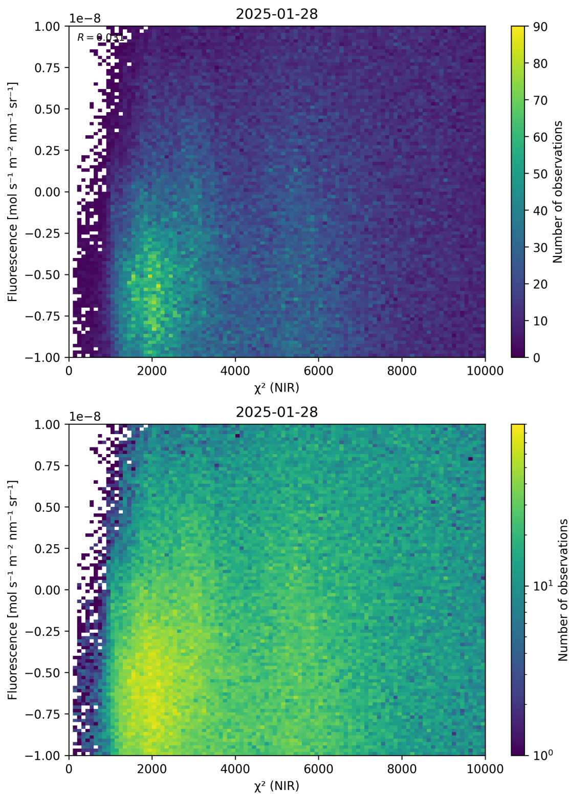
Figure 45: Scatter density plot of “ \chi^2 (NIR)” against “Fluorescence” for 2025-01-28 to 2025-01-29.
