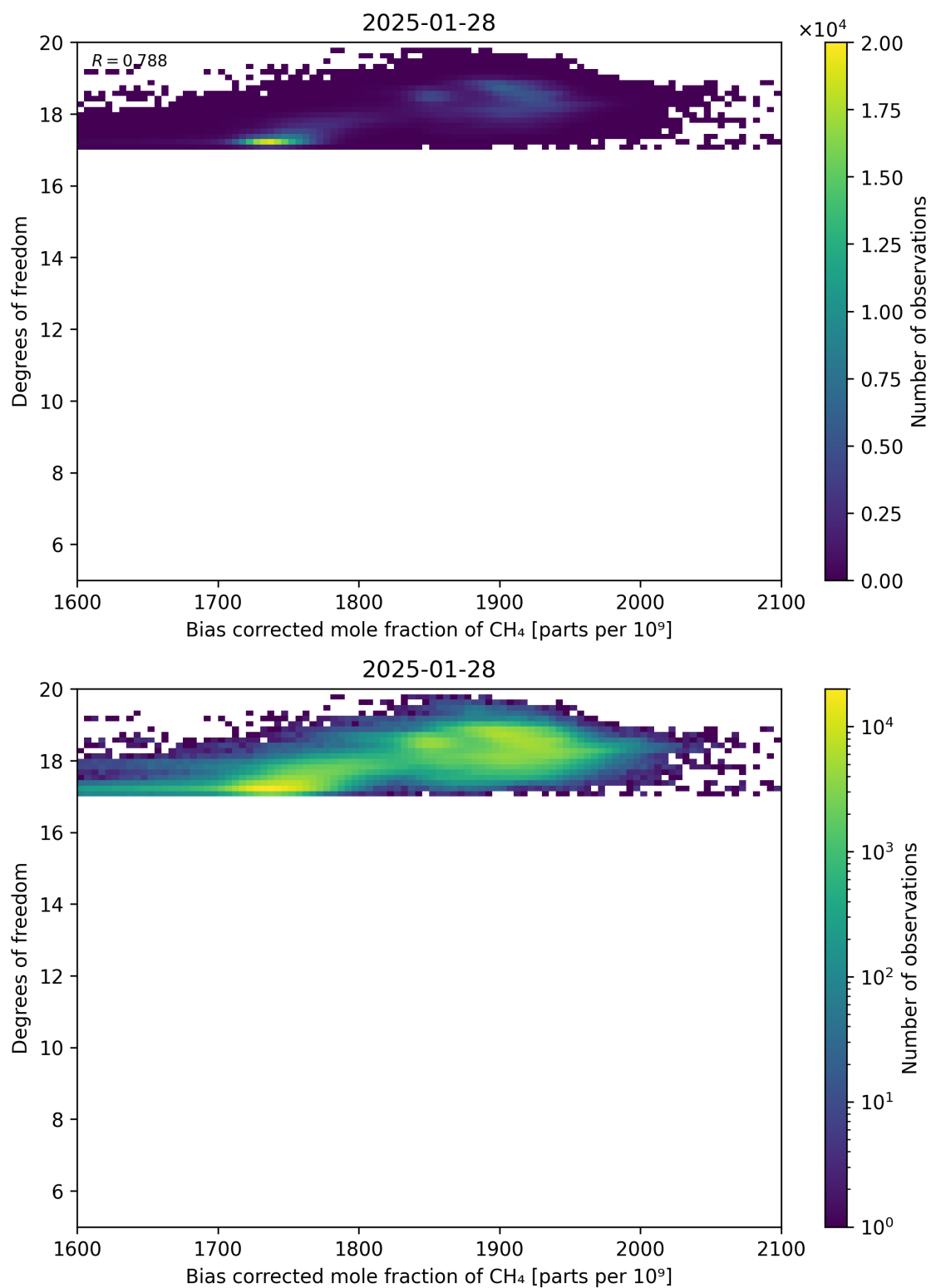
Figure 65: Scatter density plot of “Bias corrected mole fraction of CH 4 ” against “Degrees of freedom” for 2025-01-28 to 2025-01-29.
