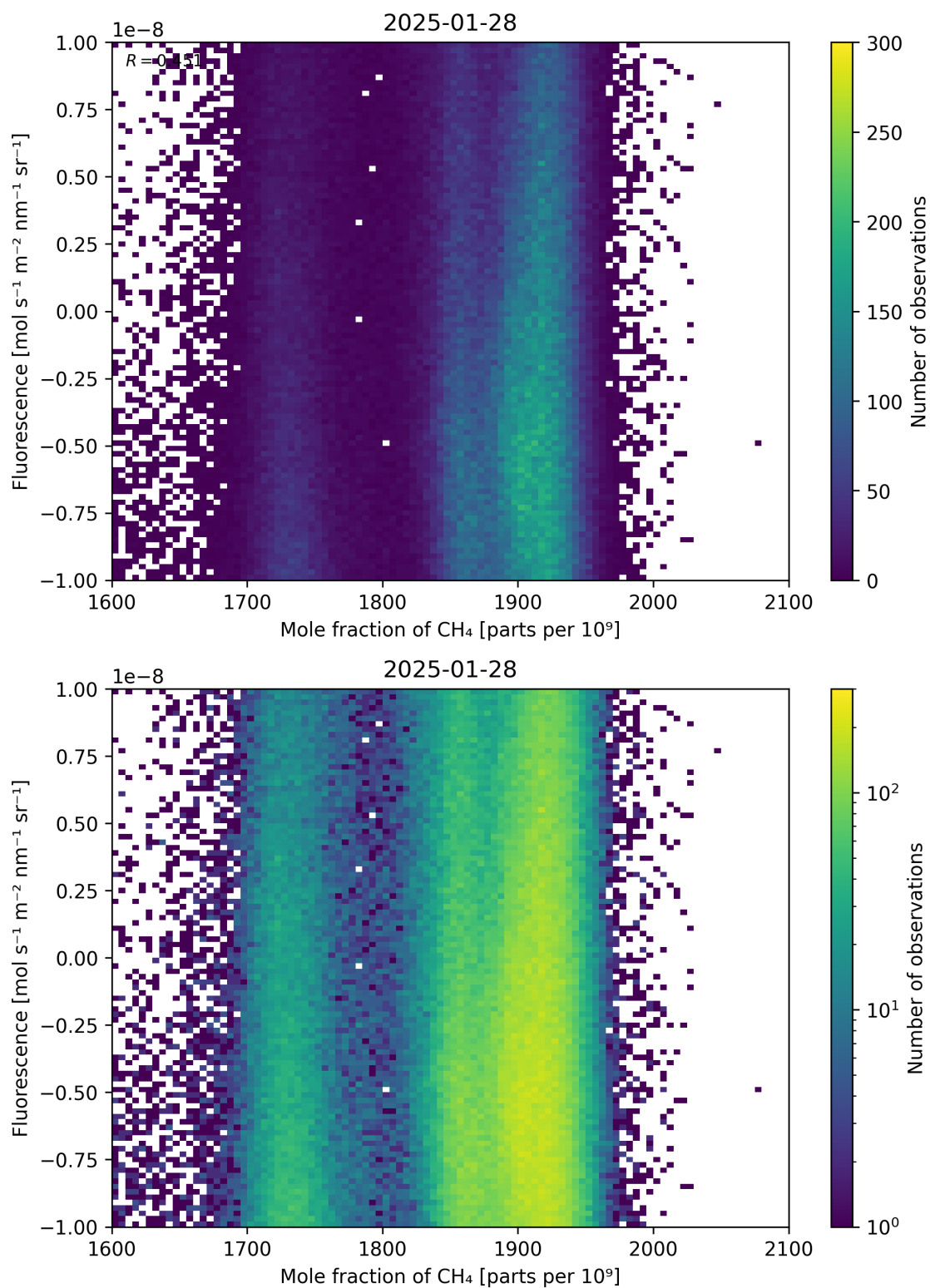
Figure 73: Scatter density plot of “Mole fraction of \text{CH}_4 ” against “Fluorescence” for 2025-01-28 to 2025-01-29.
