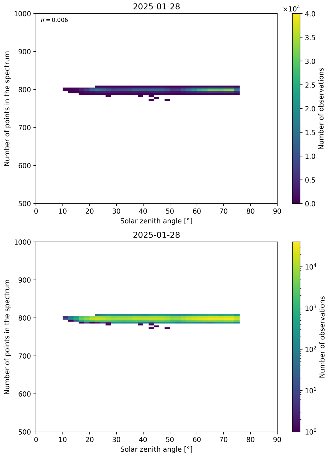
Figure 103: Scatter density plot of “Solar zenith angle” against “Number of points in the spectrum” for 2025-01-28 to 2025-01-29.
