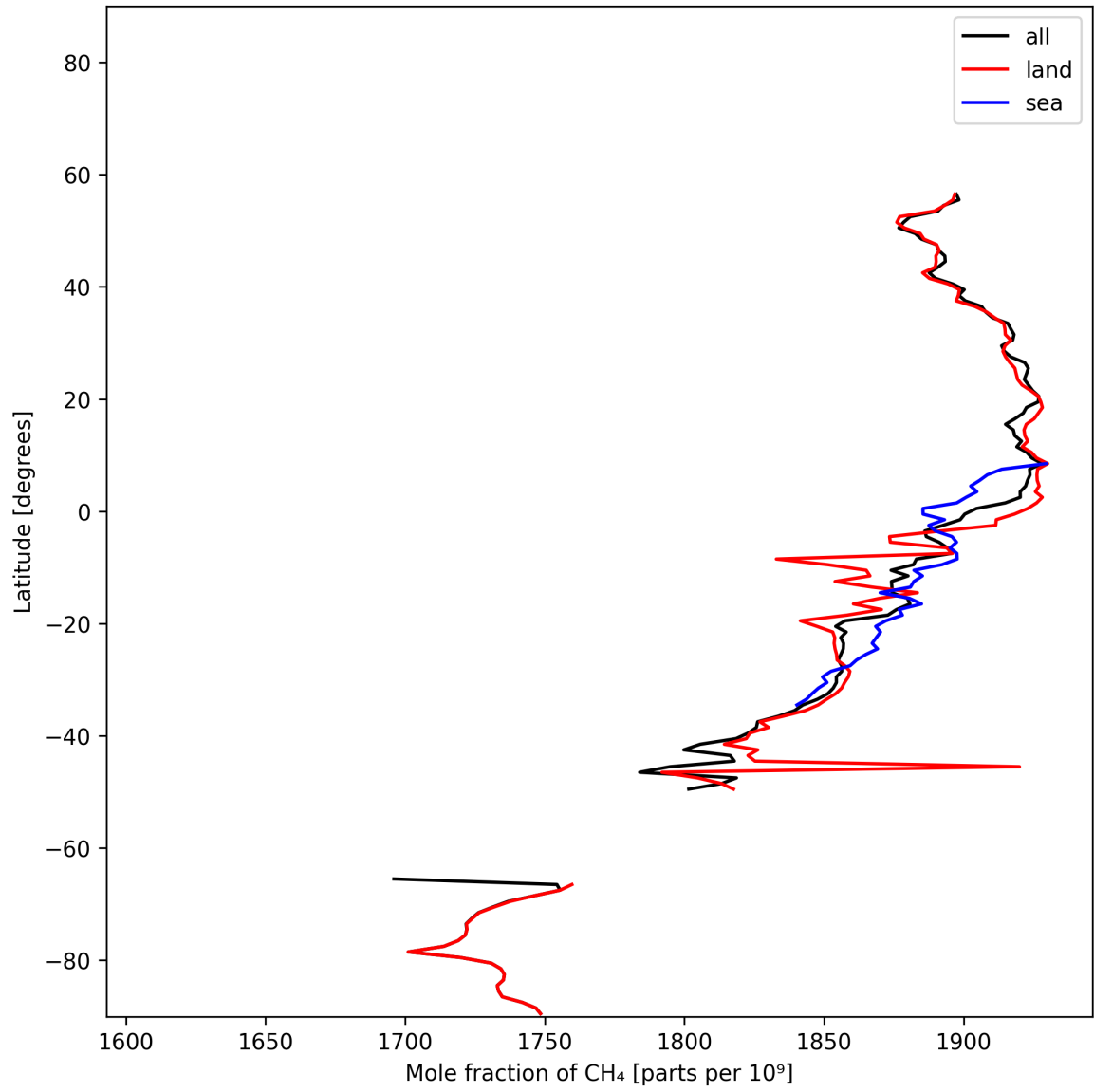
Figure 12: Zonal average of “Mole fraction of \text{CH}_4 ” for 2025-01-28 to 2025-01-29.
