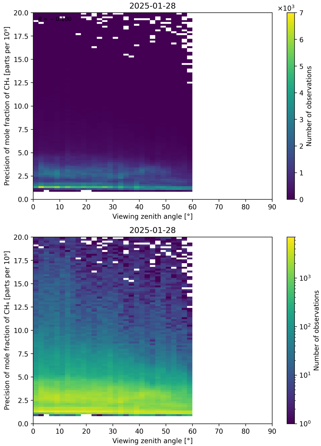
Figure 112: Scatter density plot of “Viewing zenith angle” against “Precision of mole fraction of CH 4 ” for 2025-01-28 to 2025-01-29.
