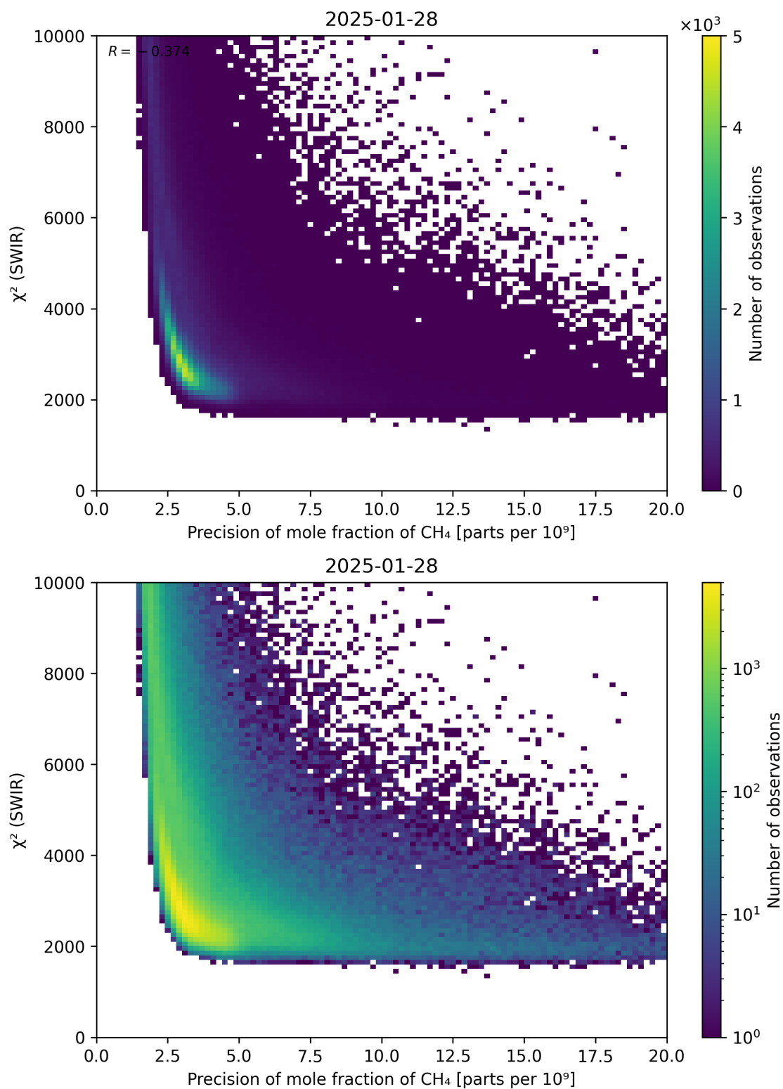
Figure 79: Scatter density plot of “Precision of mole fraction of CH 4 ” against “ \chi^2 (SWIR)” for 2025-01-28 to 2025-01-29.
