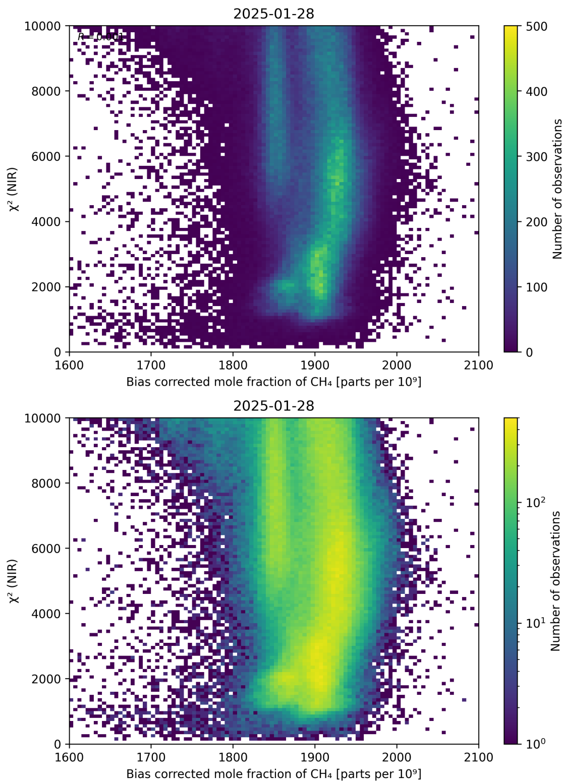
Figure 63: Scatter density plot of “Bias corrected mole fraction of \text{CH}_4 ” against “ \chi^2 (NIR)” for 2025-01-28 to 2025-01-29.
