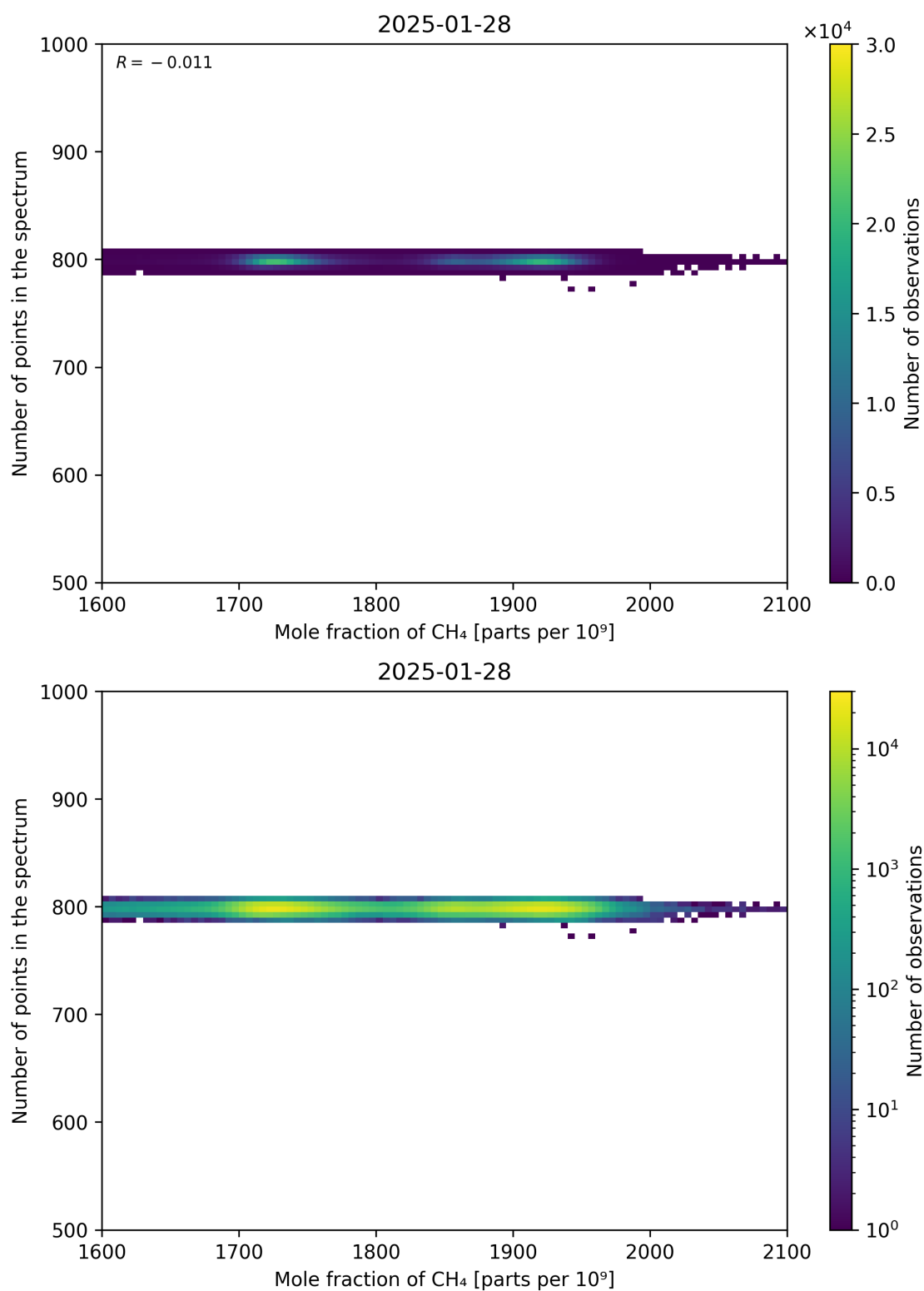
Figure 77: Scatter density plot of “Mole fraction of CH 4 ” against “Number of points in the spectrum” for 2025-01-28 to 2025-01-29.
