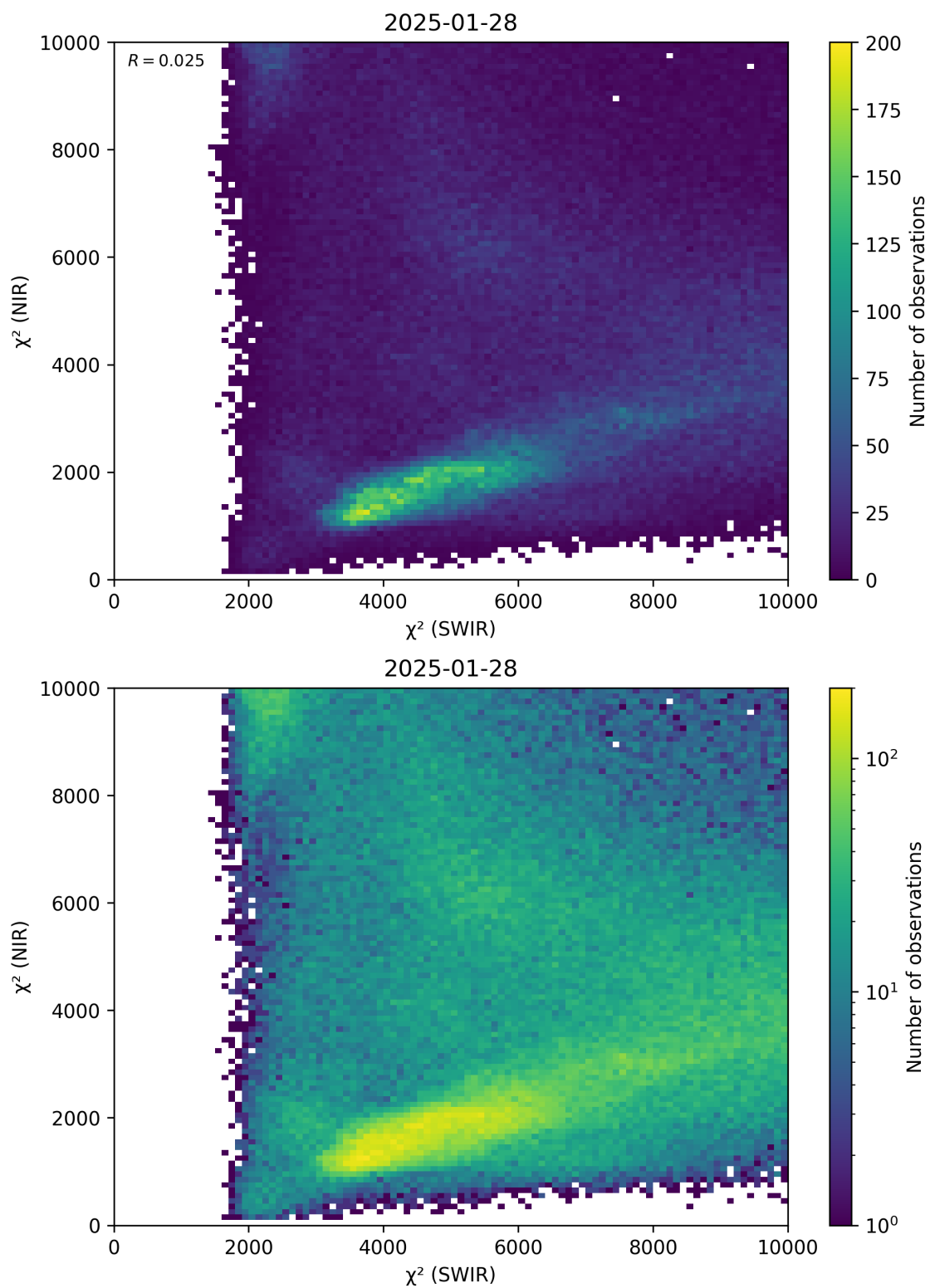
Figure 47: Scatter density plot of “ \chi^2 (SWIR)” against “ \chi^2 (NIR)” for 2025-01-28 to 2025-01-29.
