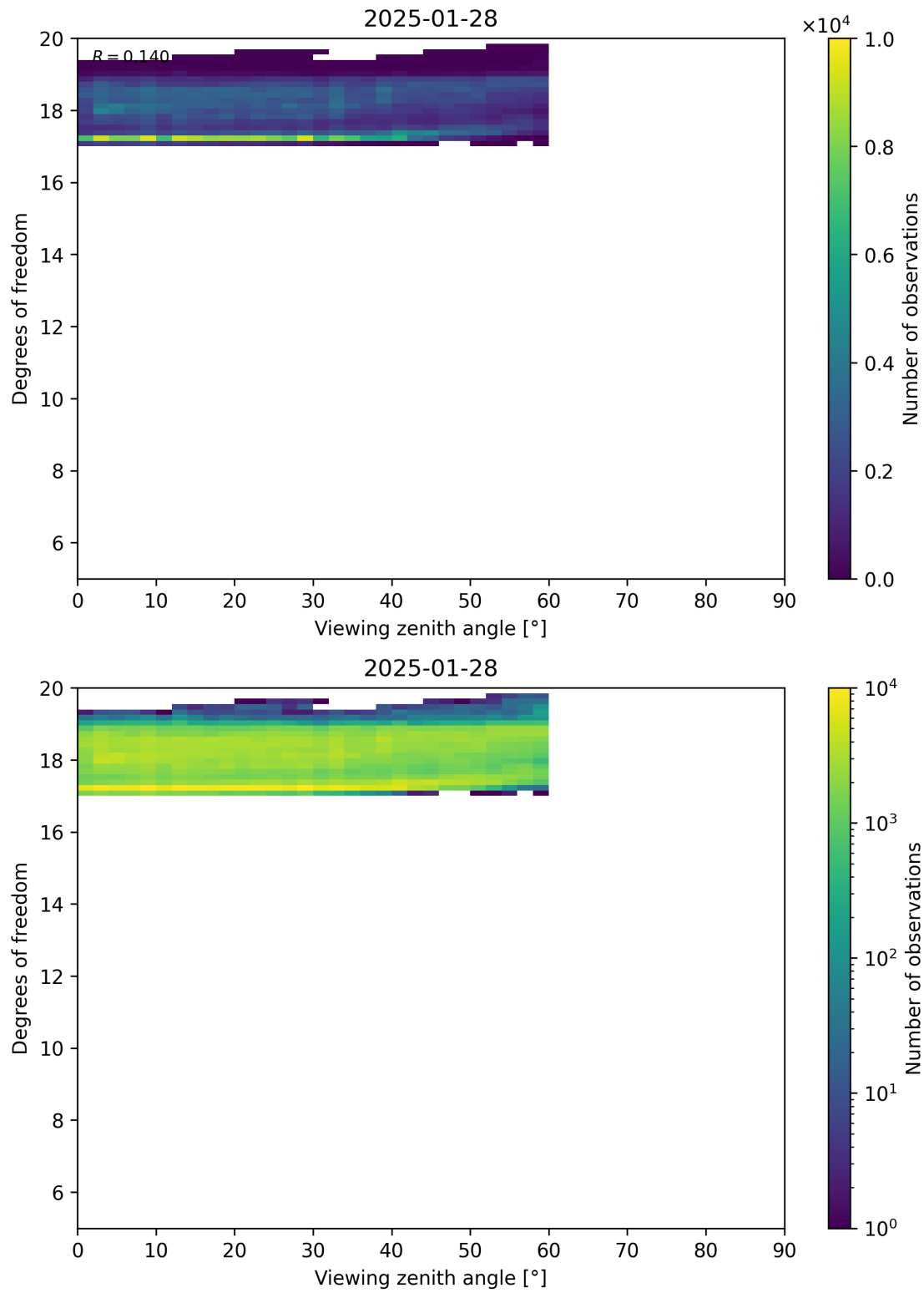
Figure 107: Scatter density plot of “Viewing zenith angle” against “Degrees of freedom” for 2025-01-28 to 2025-01-29.
