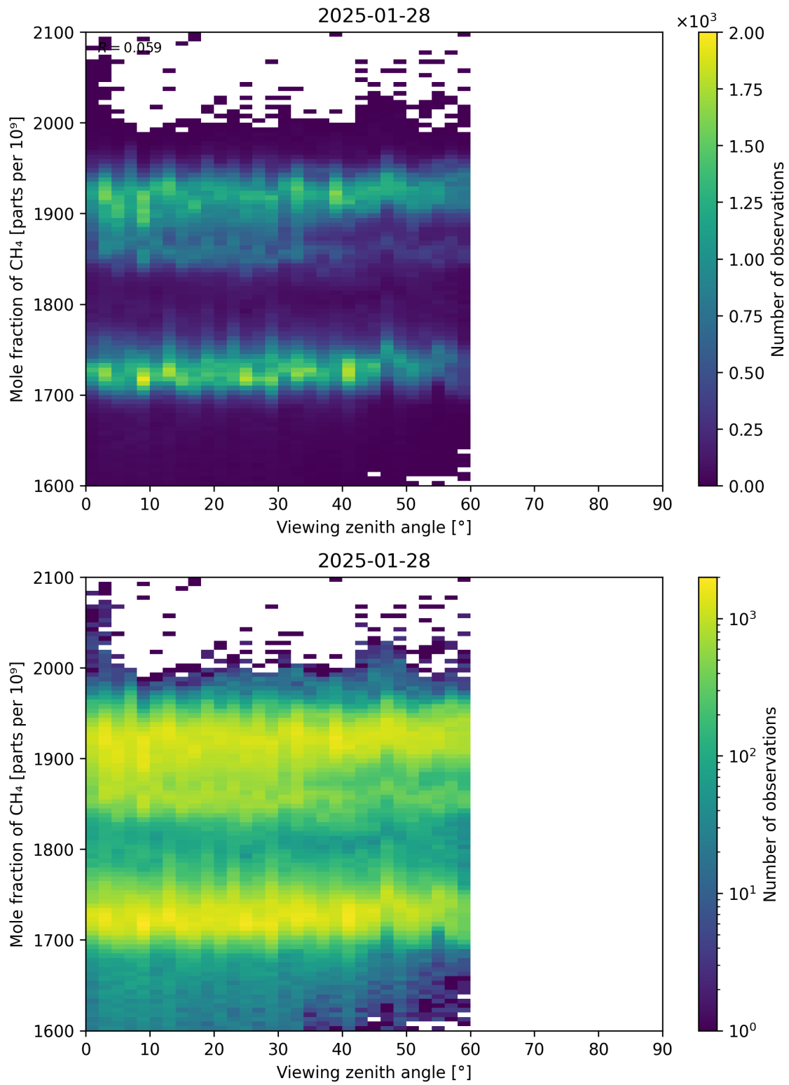
Figure 110: Scatter density plot of “Viewing zenith angle” against “Mole fraction of CH 4 ” for 2025-01-28 to 2025-01-29.
