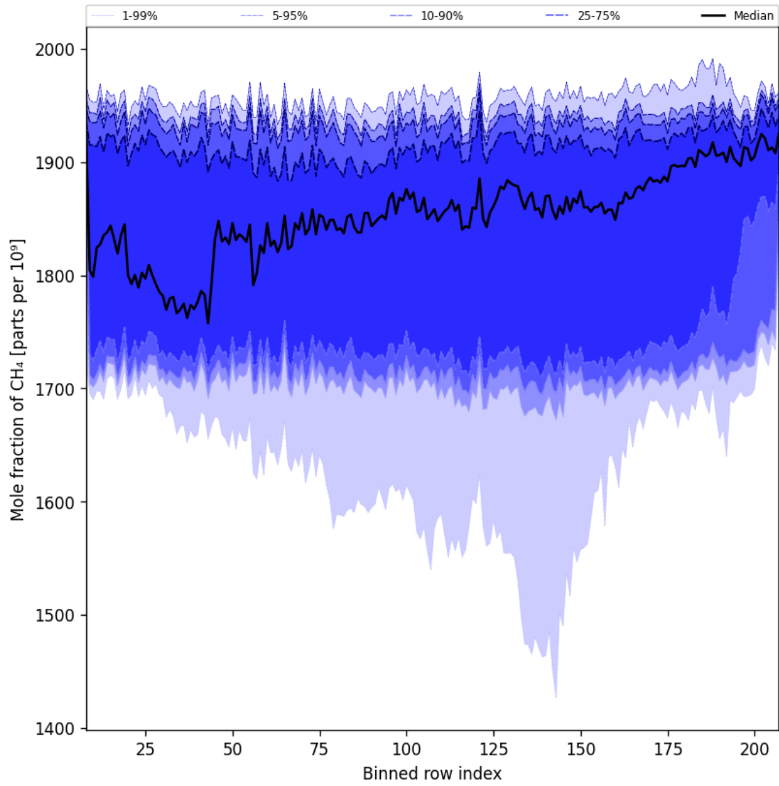
Figure 34: Along track statistics of “Mole fraction of CH 4 ” for 2025-01-28 to 2025-01-29
