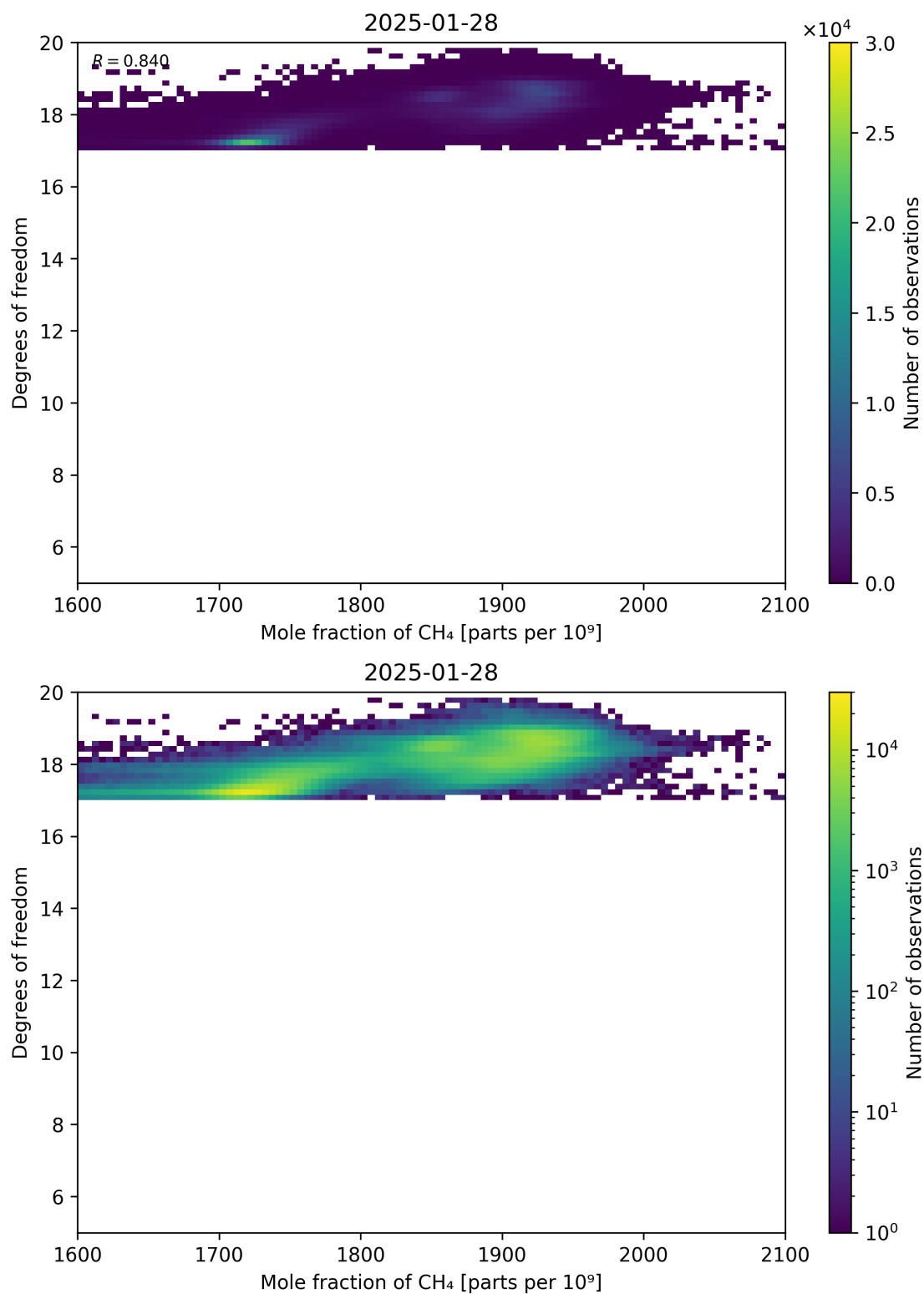
Figure 72: Scatter density plot of “Mole fraction of CH 4 ” against “Degrees of freedom” for 2025-01-28 to 2025-01-29.
