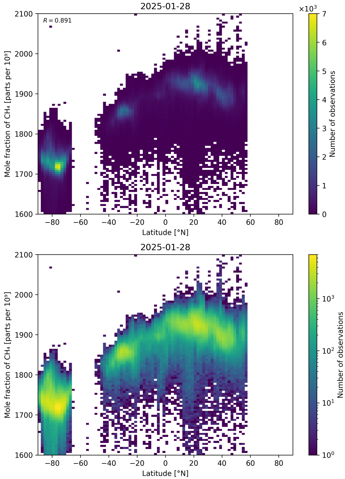
Figure 57: Scatter density plot of “Latitude” against “Mole fraction of \text{CH}_4 ” for 2025-01-28 to 2025-01-29.
