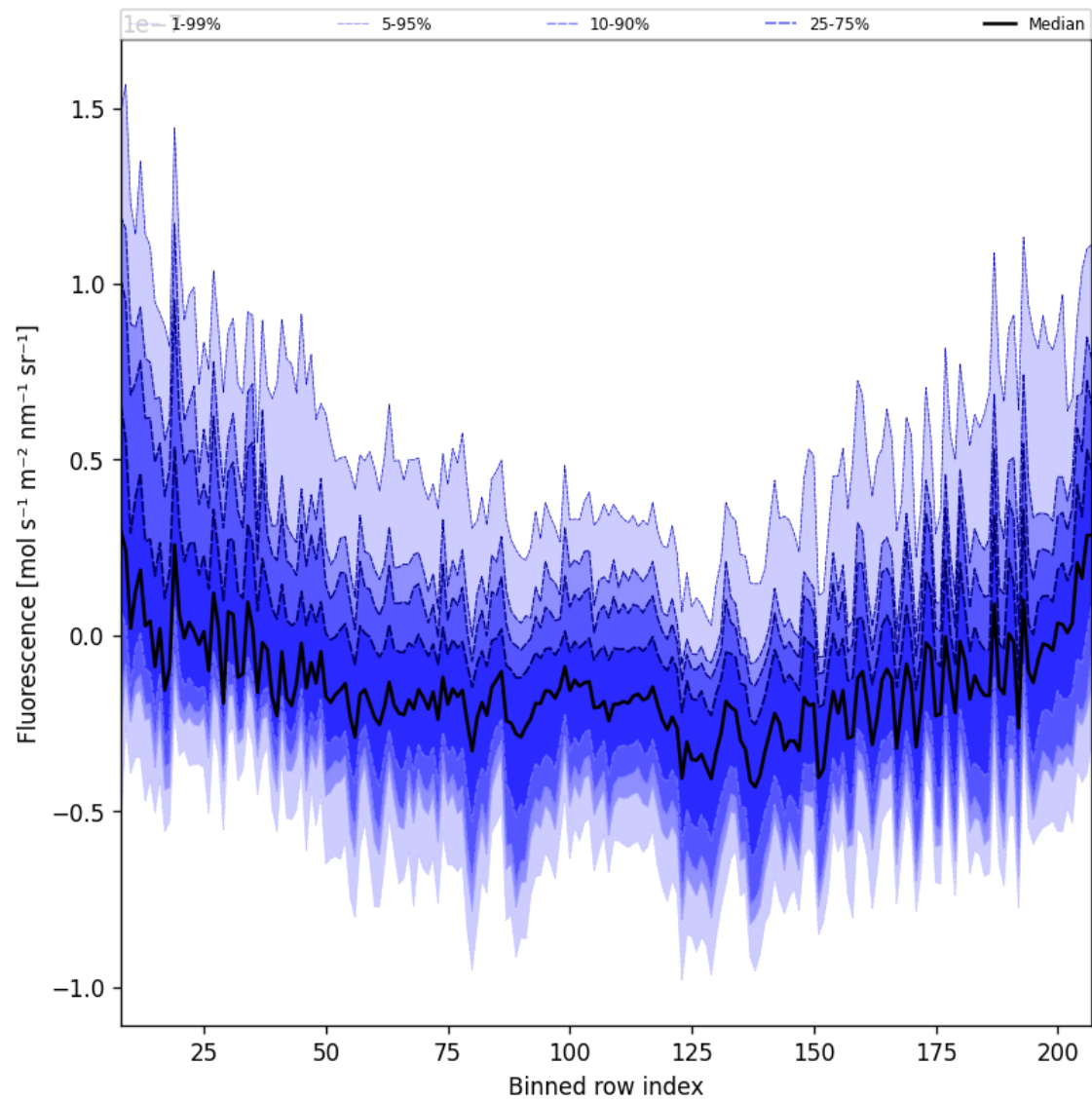
Figure 43: Along track statistics of "Fluorescence" for 2025-01-28 to 2025-01-29
