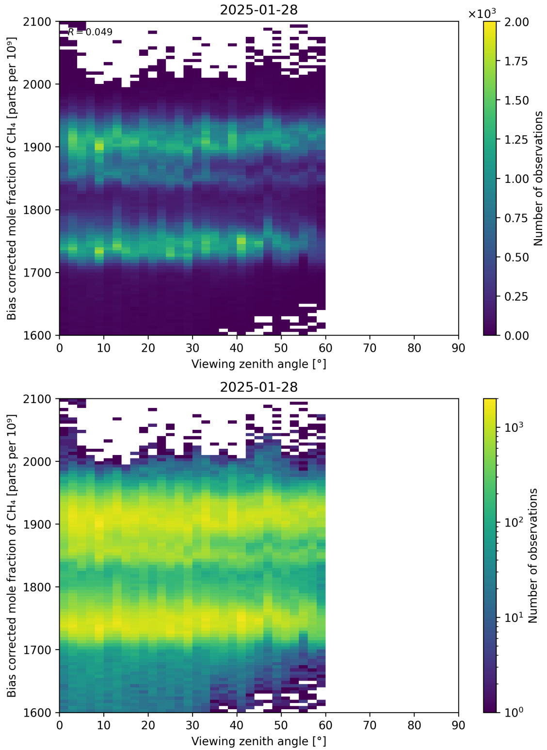
Figure 111: Scatter density plot of “Viewing zenith angle” against “Bias corrected mole fraction of CH 4 ” for 2025-01-28 to 2025-01-29.
