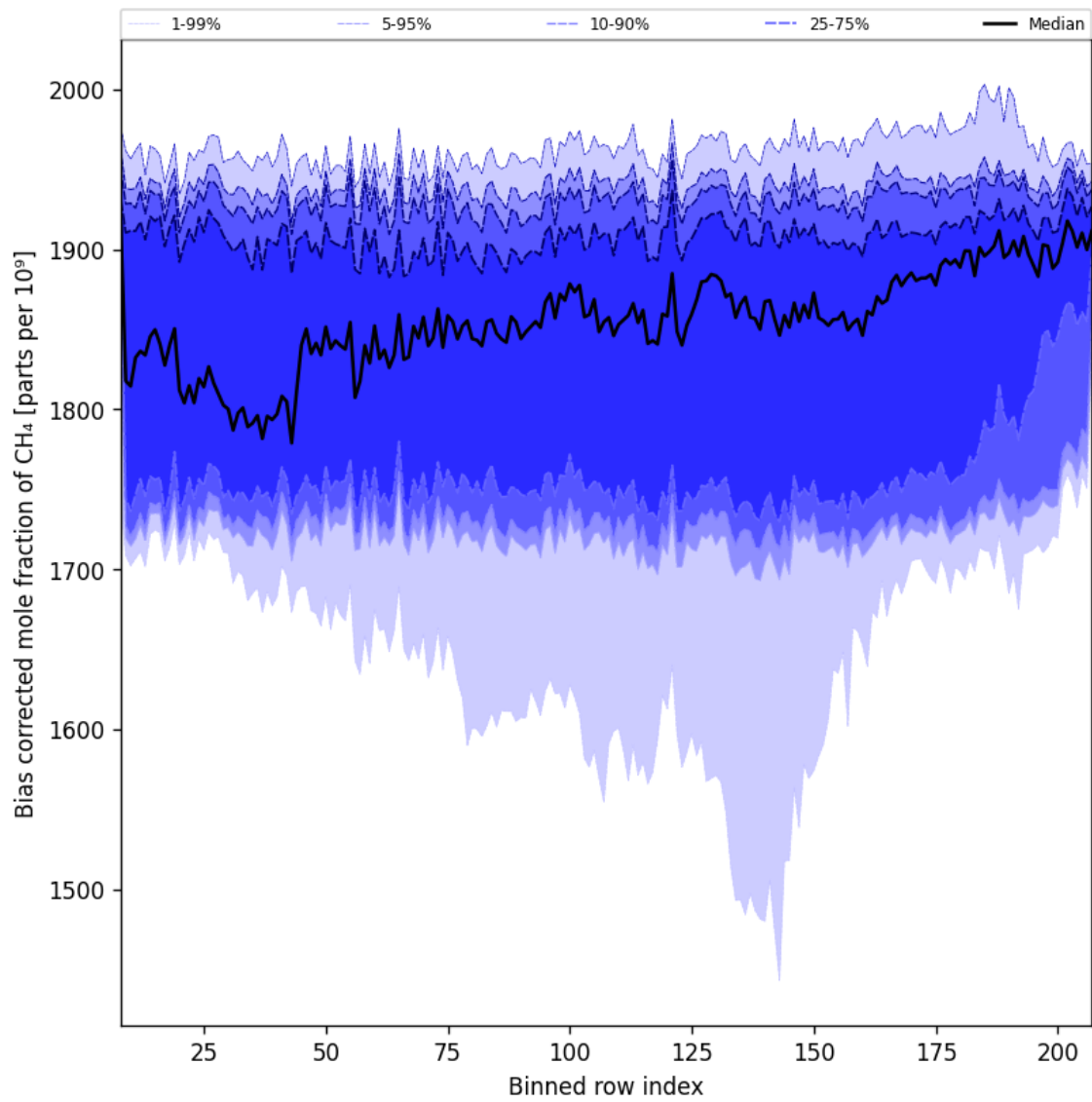
Figure 36: Along track statistics of “Bias corrected mole fraction of CH 4 ” for 2025-01-28 to 2025-01-29
