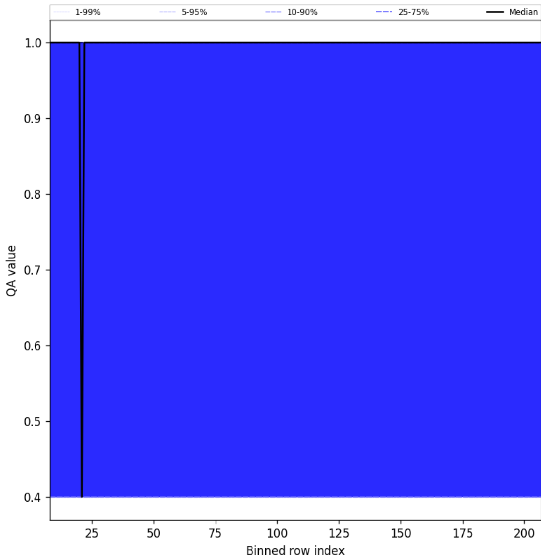
Figure 33: Along track statistics of “QA value” for 2025-01-28 to 2025-01-29
