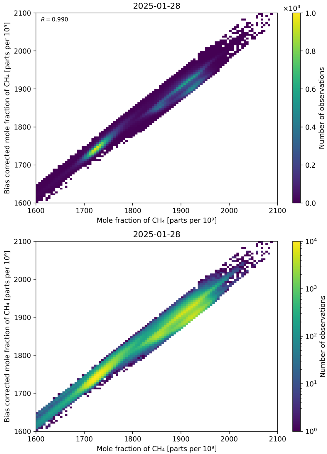
Figure 74: Scatter density plot of “Mole fraction of CH 4 ” against “Bias corrected mole fraction of CH 4 ” for 2025-01-28 to 2025-01-29.
