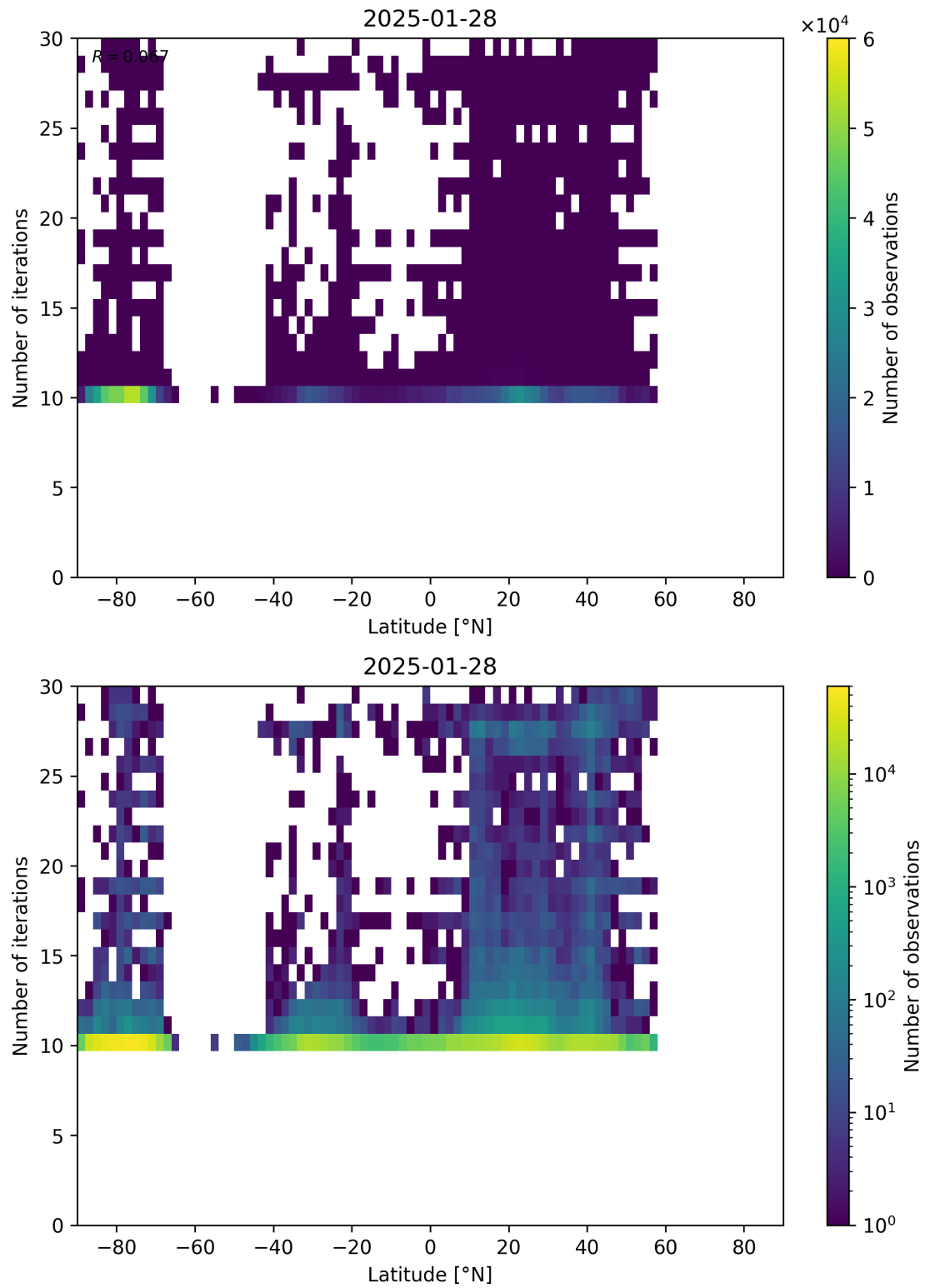
Figure 60: Scatter density plot of “Latitude” against “Number of iterations” for 2025-01-28 to 2025-01-29.
