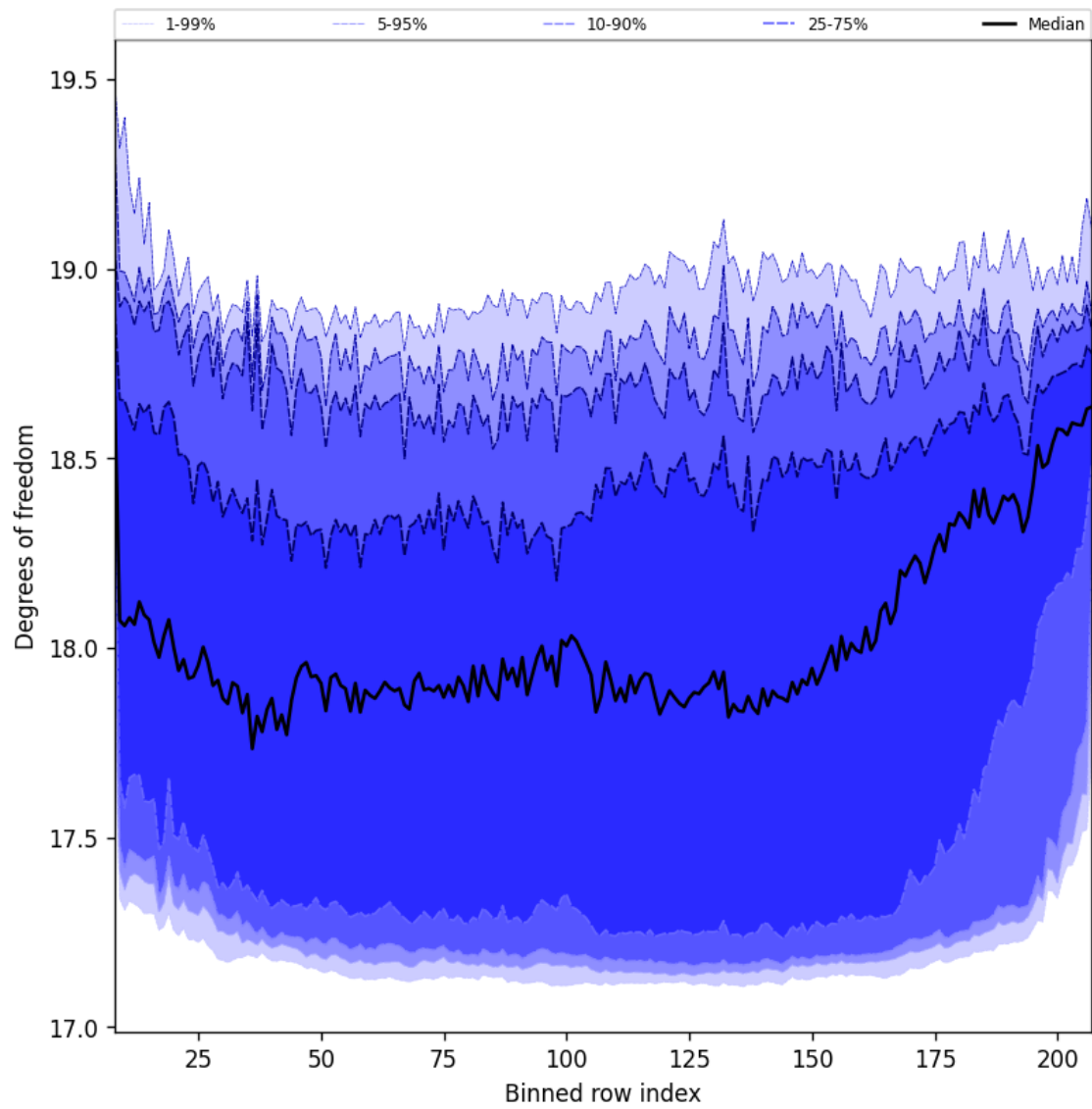
Figure 41: Along track statistics of “Degrees of freedom” for 2025-01-28 to 2025-01-29
