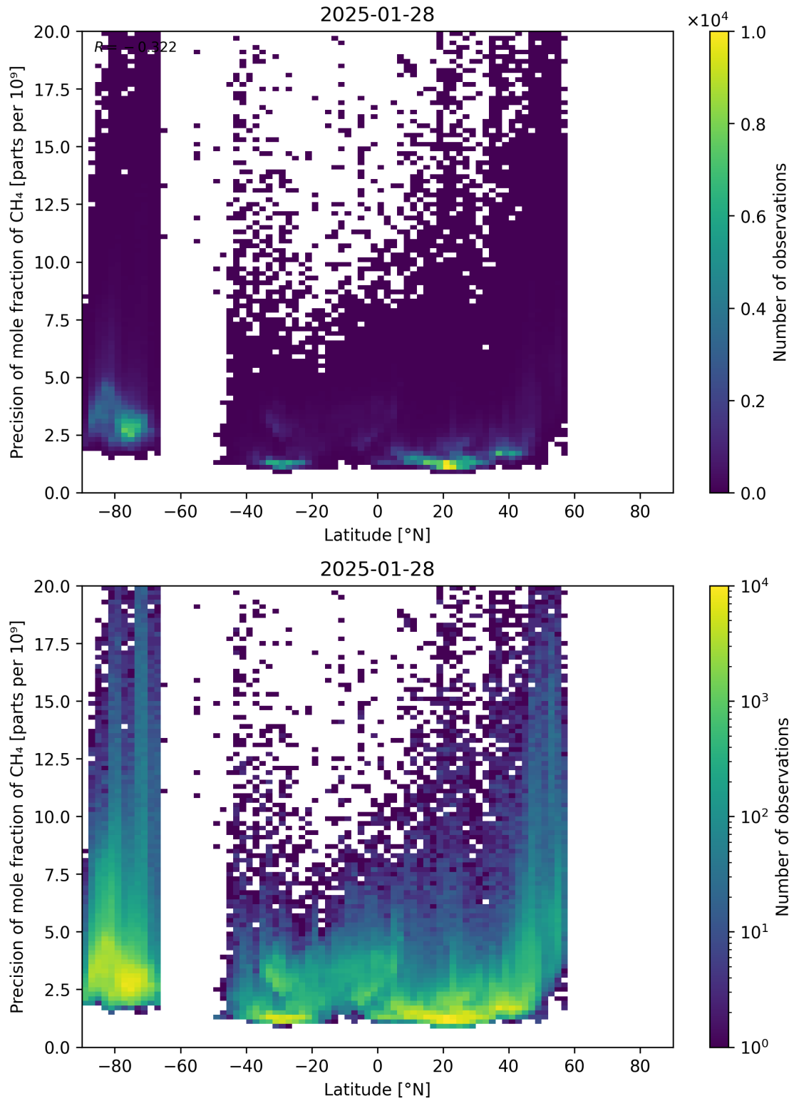
Figure 59: Scatter density plot of “Latitude” against “Precision of mole fraction of CH 4 ” for 2025-01-28 to 2025-01-29.
