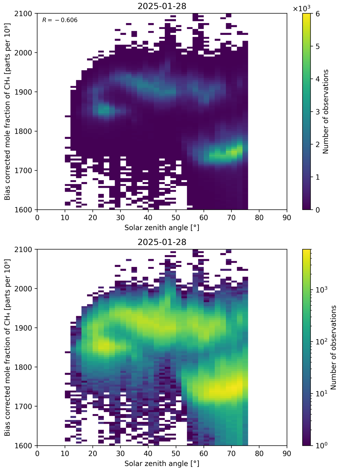
Figure 100: Scatter density plot of “Solar zenith angle” against “Bias corrected mole fraction of CH 4 ” for 2025-01-28 to 2025-01-29.
