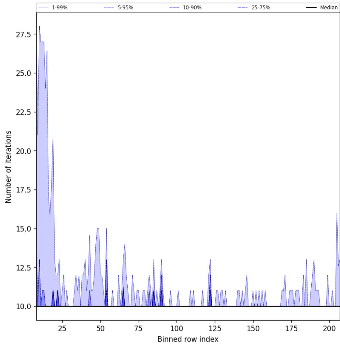
Figure 42: Along track statistics of “Number of iterations” for 2025-01-28 to 2025-01-29
