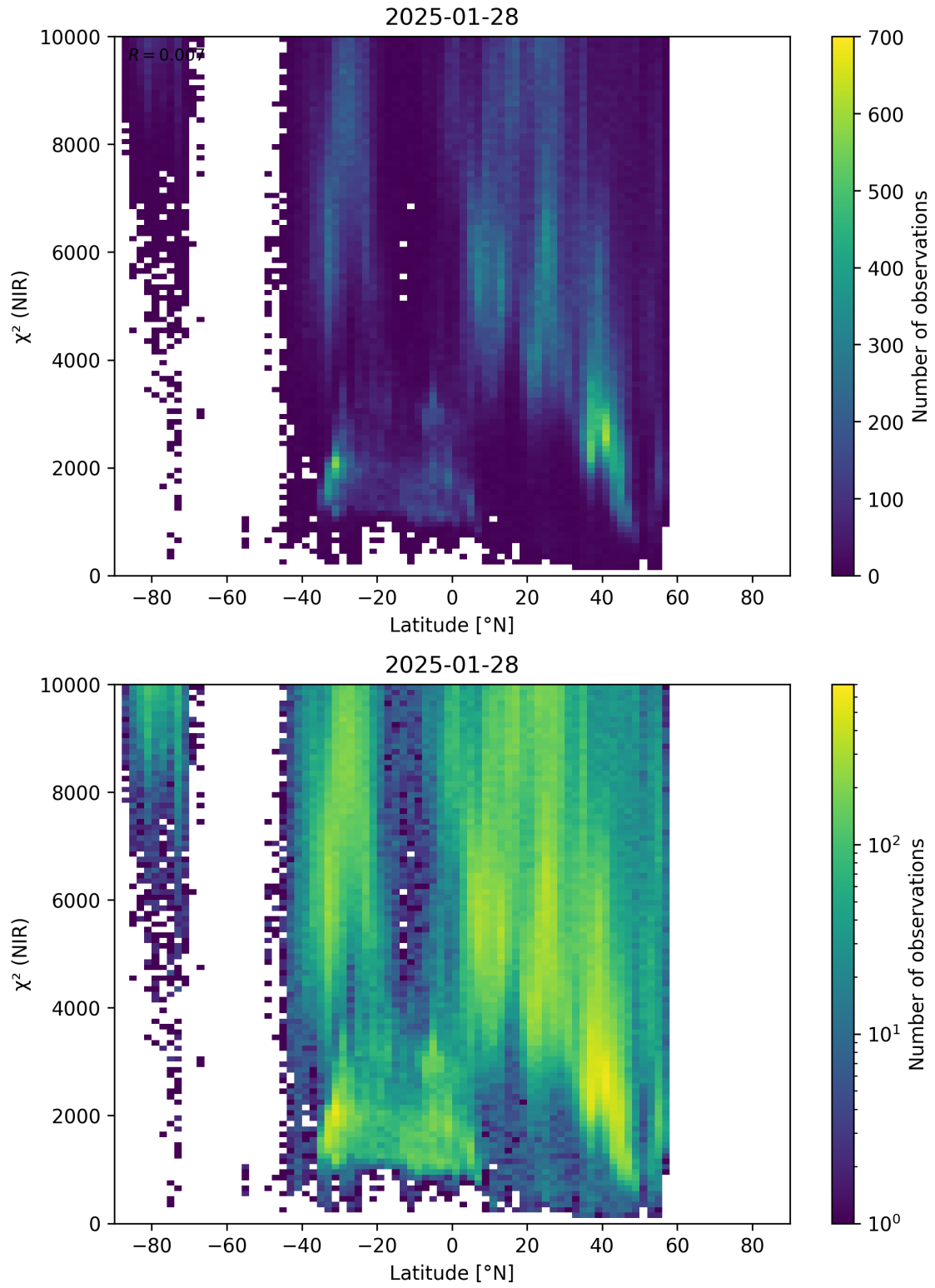
Figure 53: Scatter density plot of “Latitude” against “ \chi^2 (NIR)” for 2025-01-28 to 2025-01-29.
