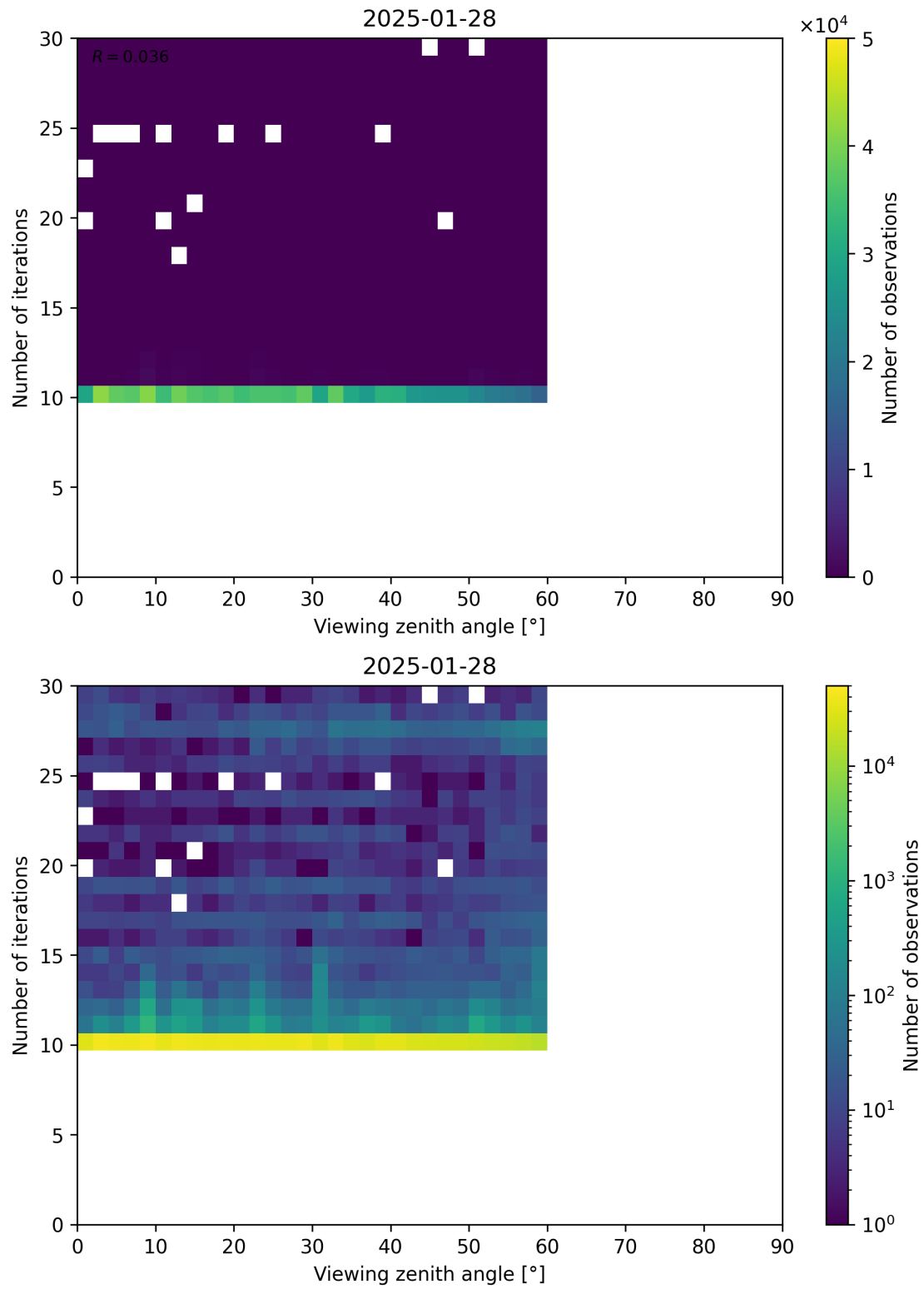
Figure 113: Scatter density plot of “Viewing zenith angle” against “Number of iterations” for 2025-01-28 to 2025-01-29.
