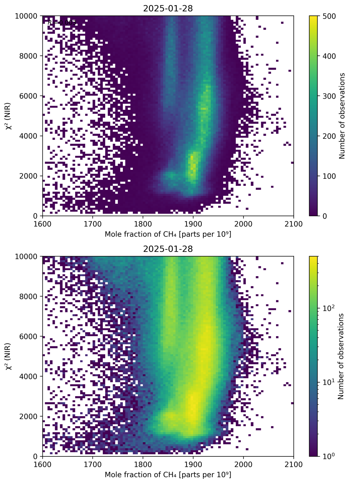
Figure 70: Scatter density plot of “Mole fraction of CH 4 ” against “ \chi^2 (NIR)” for 2025-01-28 to 2025-01-29.
