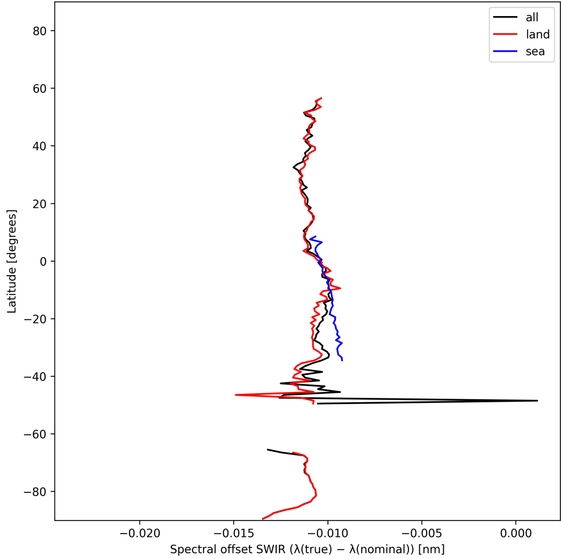
Figure 16: Zonal average of “Spectral offset SWIR ( \lambda_{\text{true}} - \lambda_{\text{nominal}} )” for 2025-01-28 to 2025-01-29.
