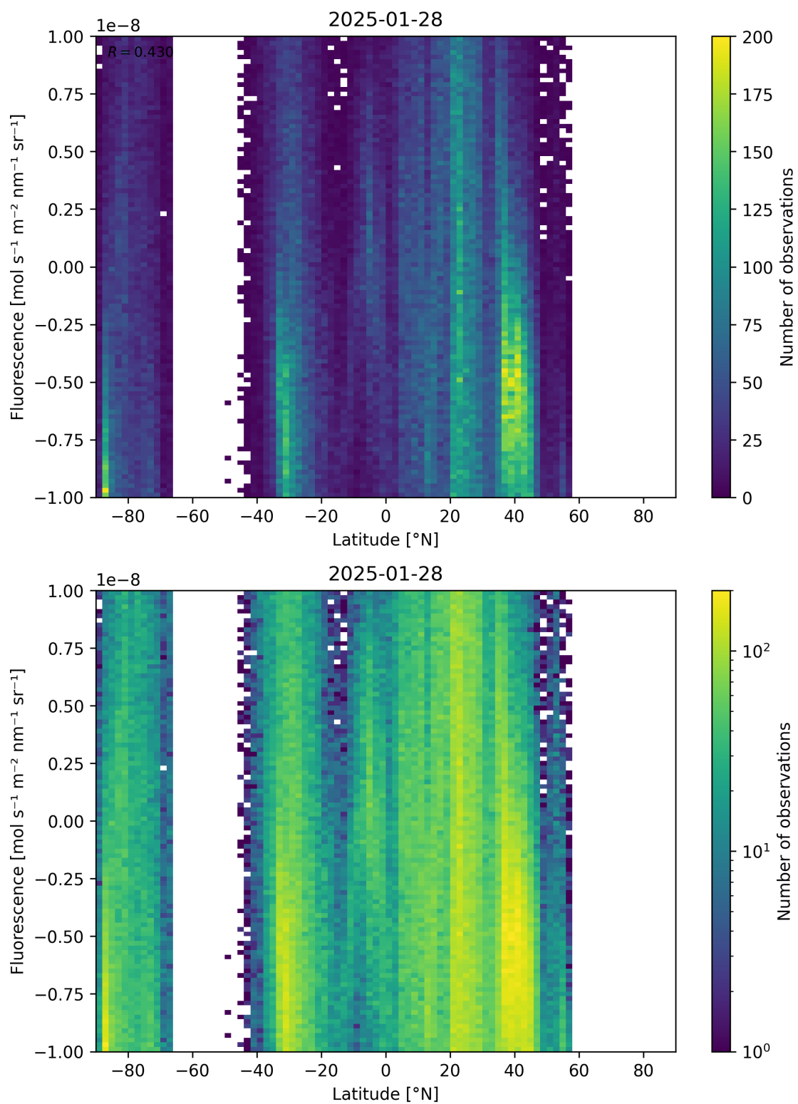
Figure 56: Scatter density plot of “Latitude” against “Fluorescence” for 2025-01-28 to 2025-01-29.
