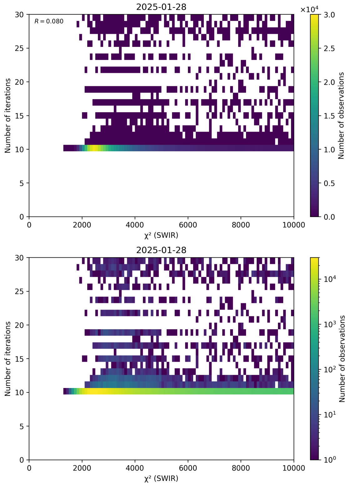
Figure 50: Scatter density plot of “ \chi^2 (SWIR)” against “Number of iterations” for 2025-01-28 to 2025-01-29.
