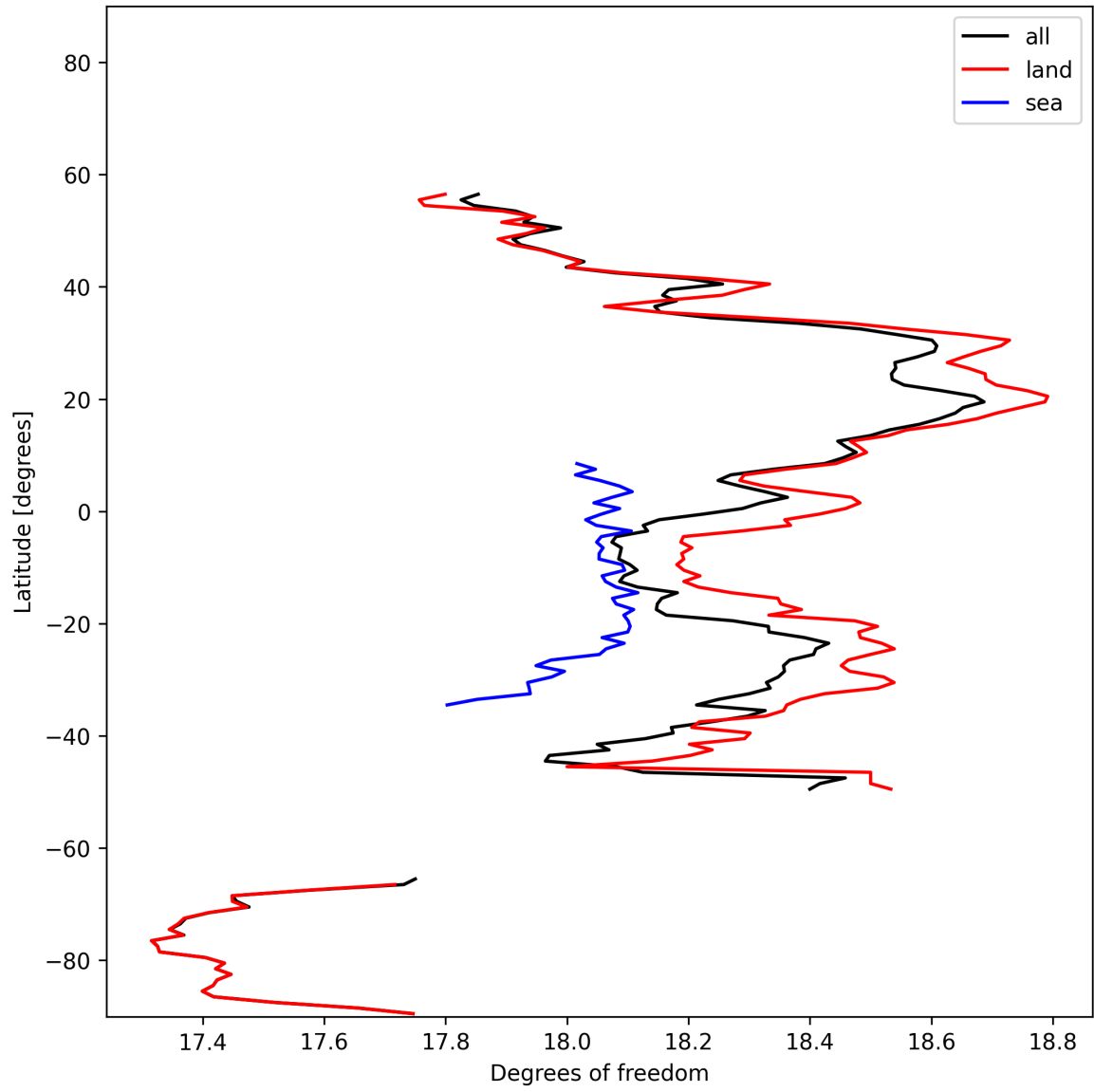
Figure 19: Zonal average of “Degrees of freedom” for 2025-01-28 to 2025-01-29.
