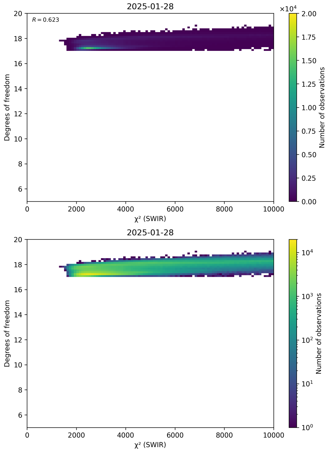
Figure 48: Scatter density plot of “ \chi^2 (SWIR)” against “Degrees of freedom” for 2025-01-28 to 2025-01-29.
