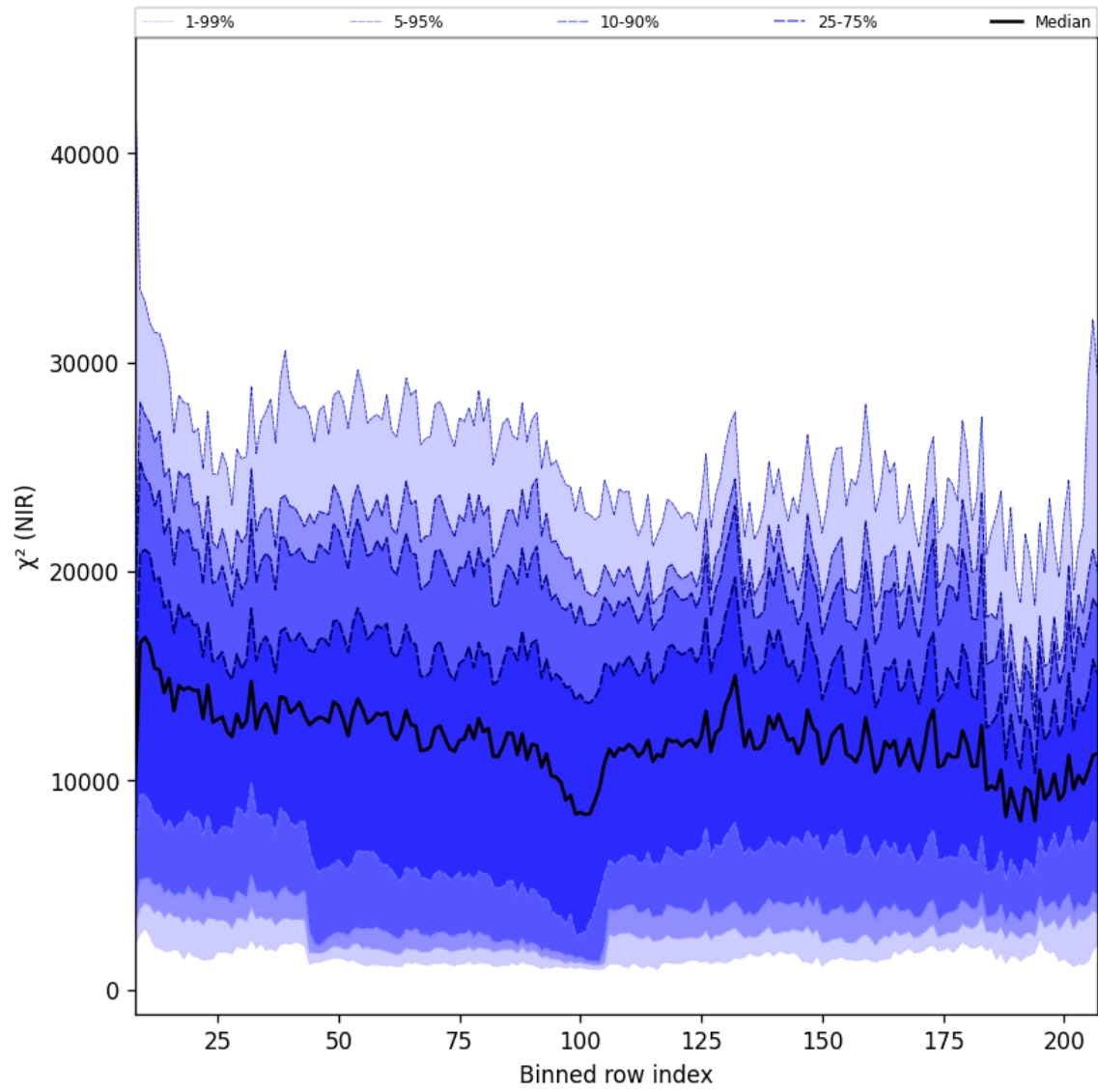
Figure 40: Along track statistics of “ \chi^2 (NIR)” for 2025-01-28 to 2025-01-29
