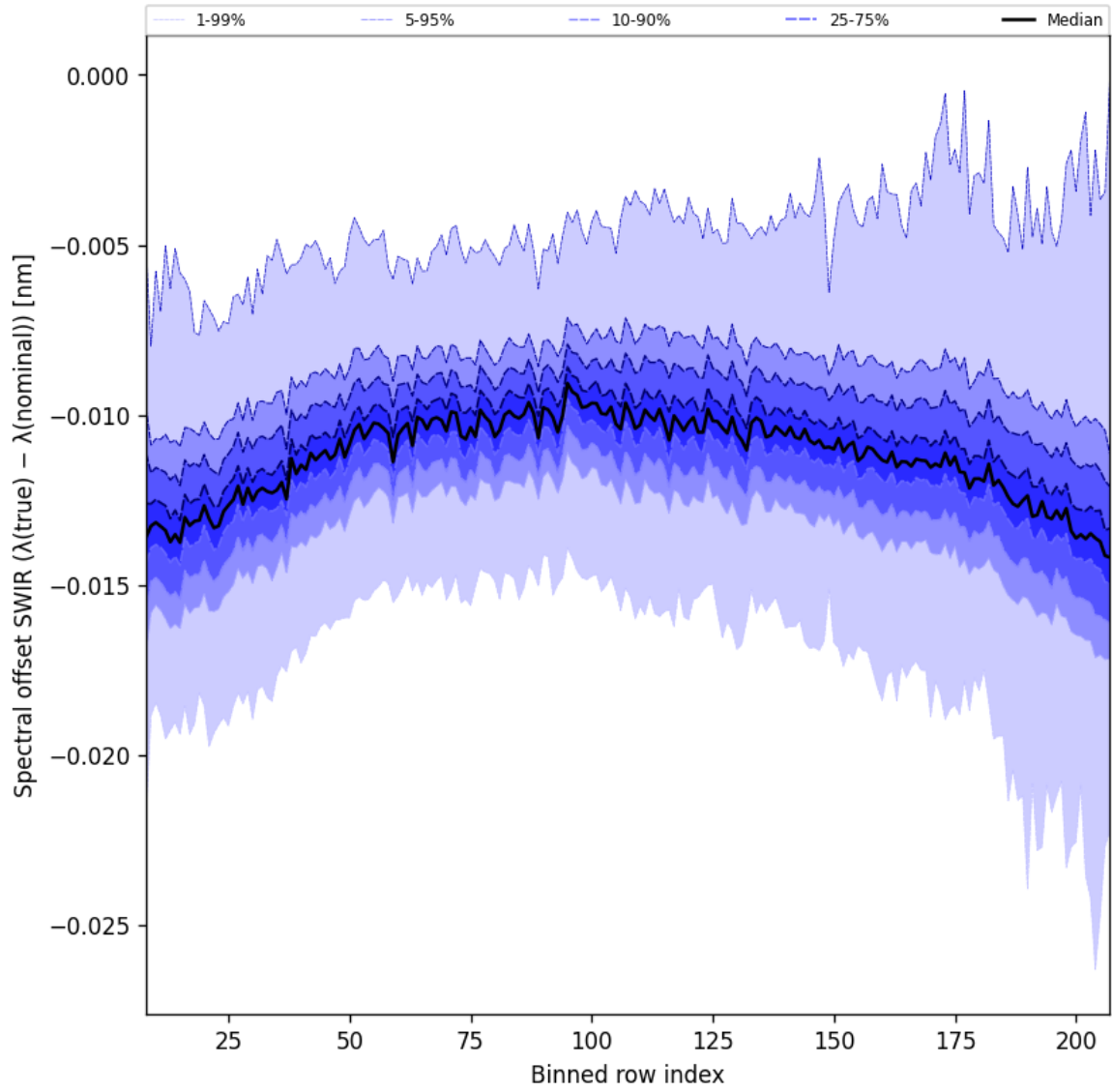
Figure 38: Along track statistics of “Spectral offset SWIR ( \lambda_{\text{true}} - \lambda_{\text{nominal}} )” for 2025-01-28 to 2025-01-29
