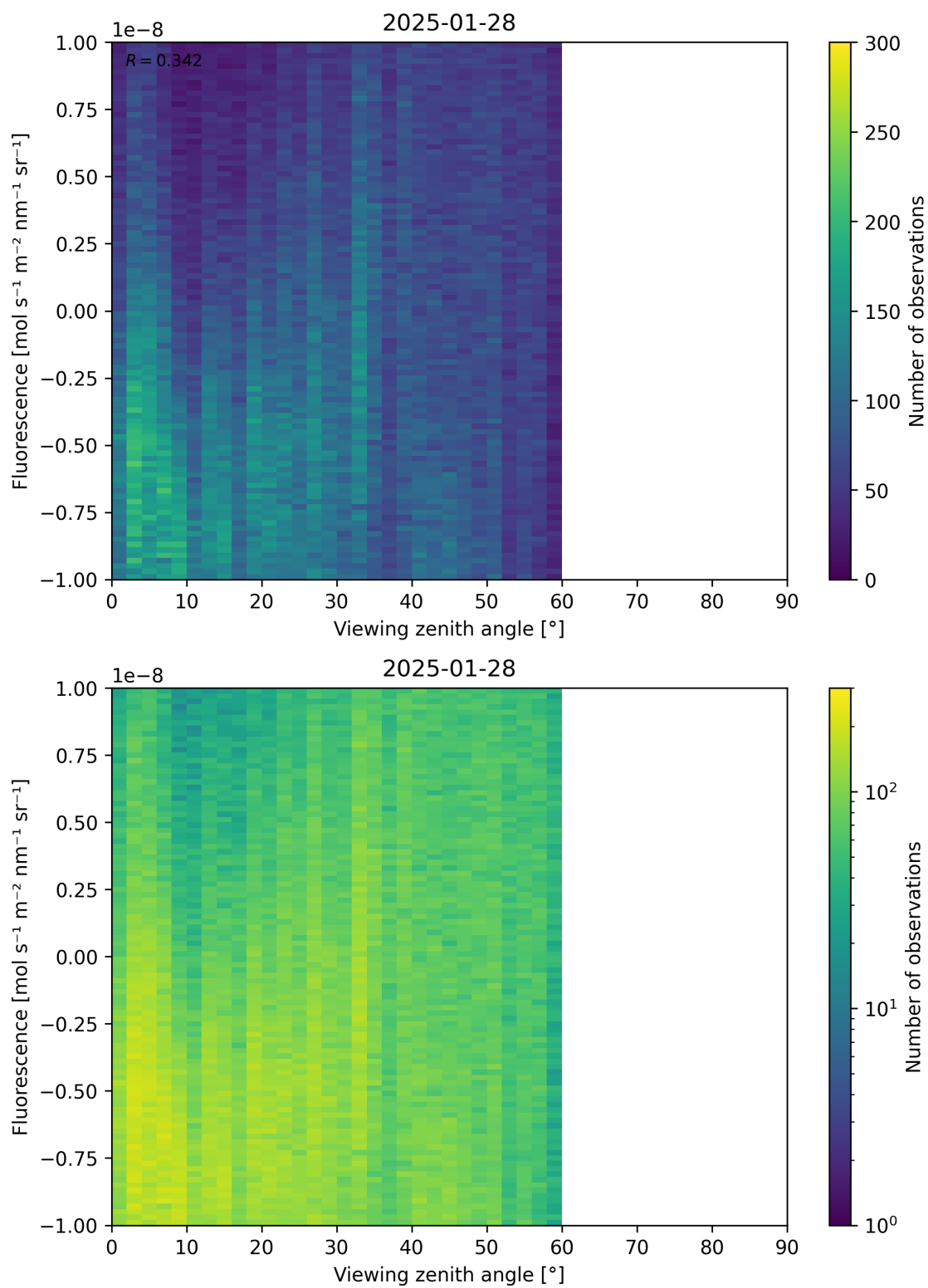
Figure 108: Scatter density plot of “Viewing zenith angle” against “Fluorescence” for 2025-01-28 to 2025-01-29.
