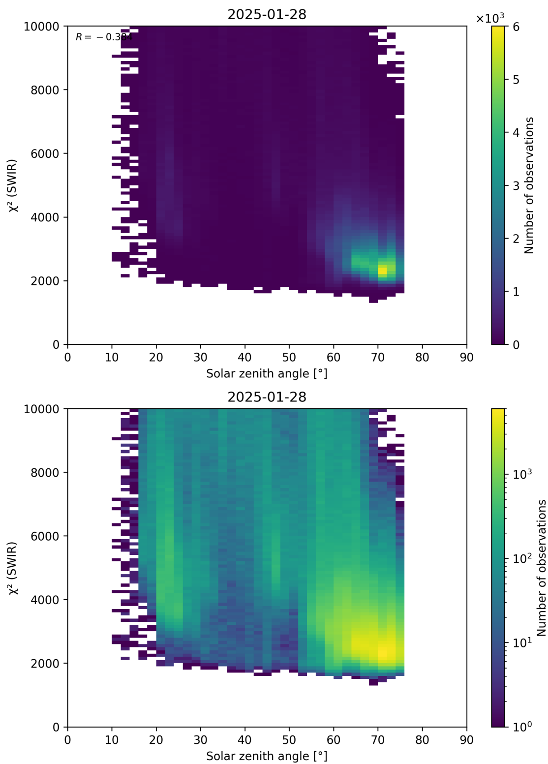
Figure 95: Scatter density plot of “Solar zenith angle” against “ \chi^2 (SWIR)” for 2025-01-28 to 2025-01-29.
