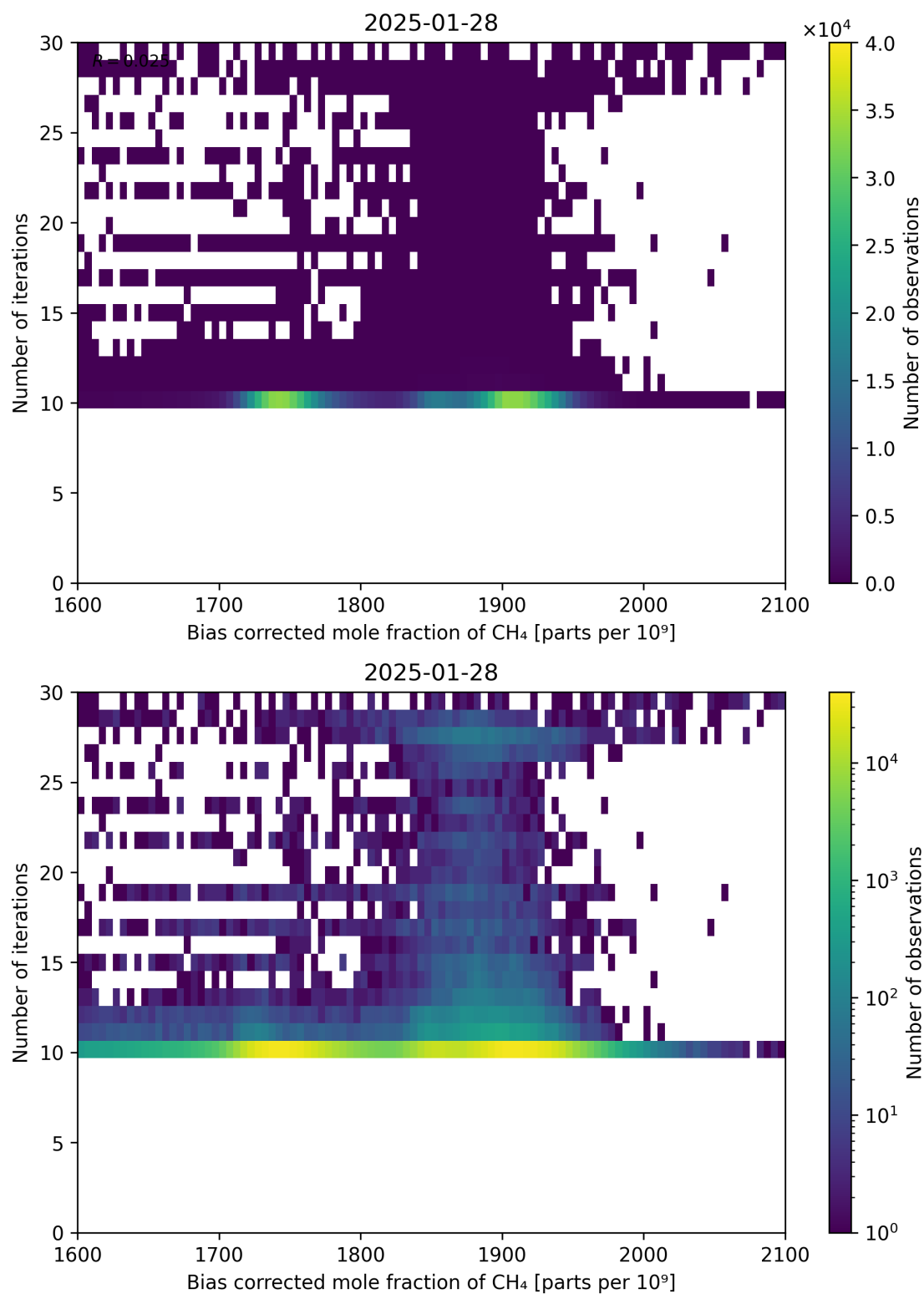
Figure 67: Scatter density plot of “Bias corrected mole fraction of \text{CH}_4 ” against “Number of iterations” for 2025-01-28 to 2025-01-29.
