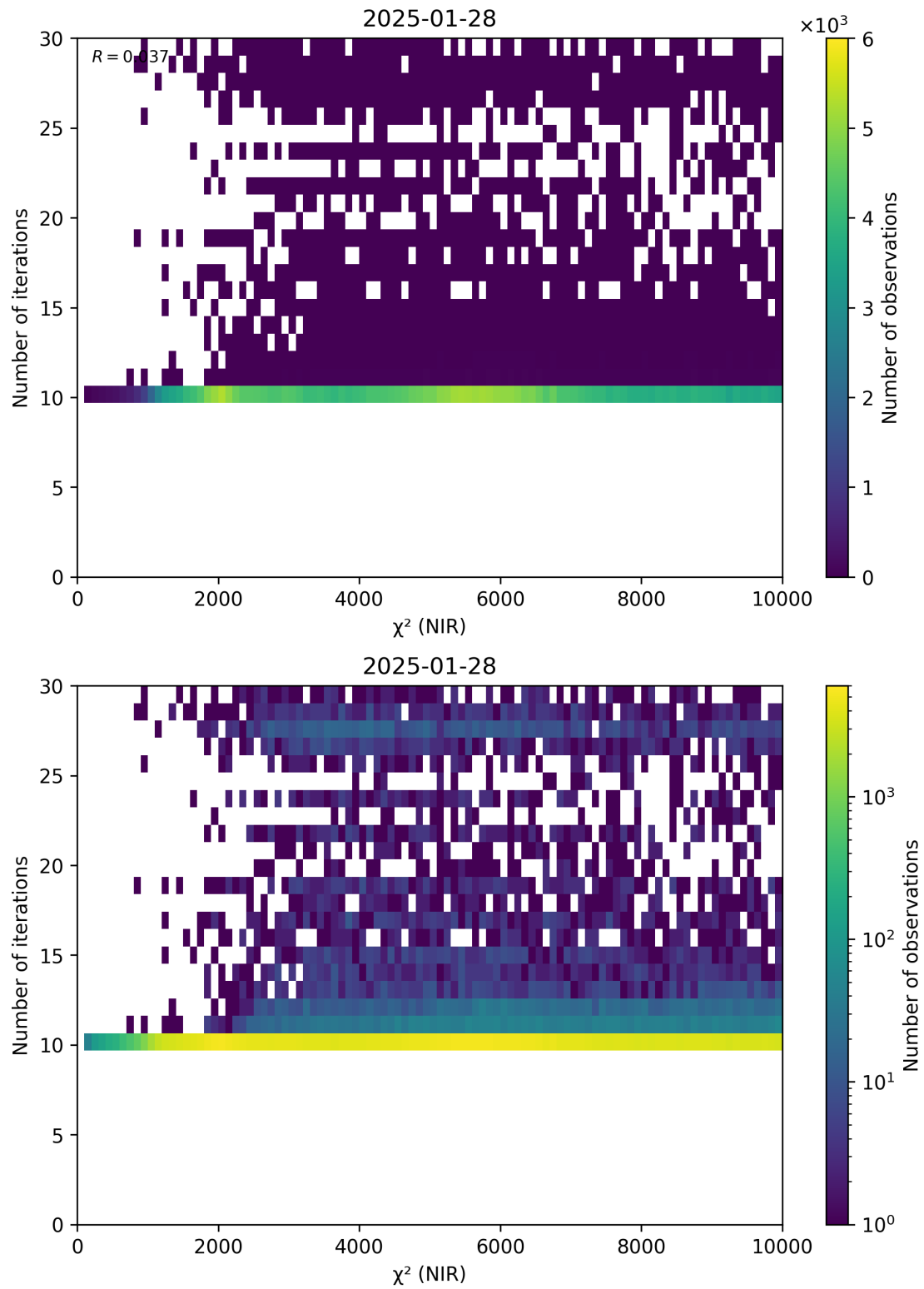
Figure 46: Scatter density plot of “ \chi^2 (NIR)” against “Number of iterations” for 2025-01-28 to 2025-01-29.
