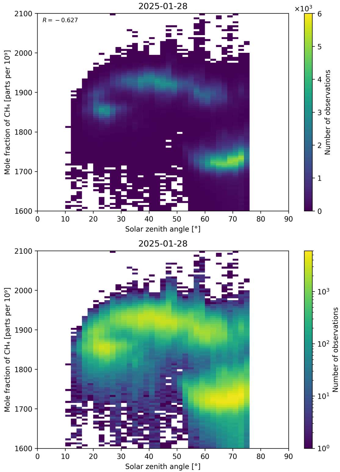
Figure 99: Scatter density plot of “Solar zenith angle” against “Mole fraction of CH 4 ” for 2025-01-28 to 2025-01-29.
