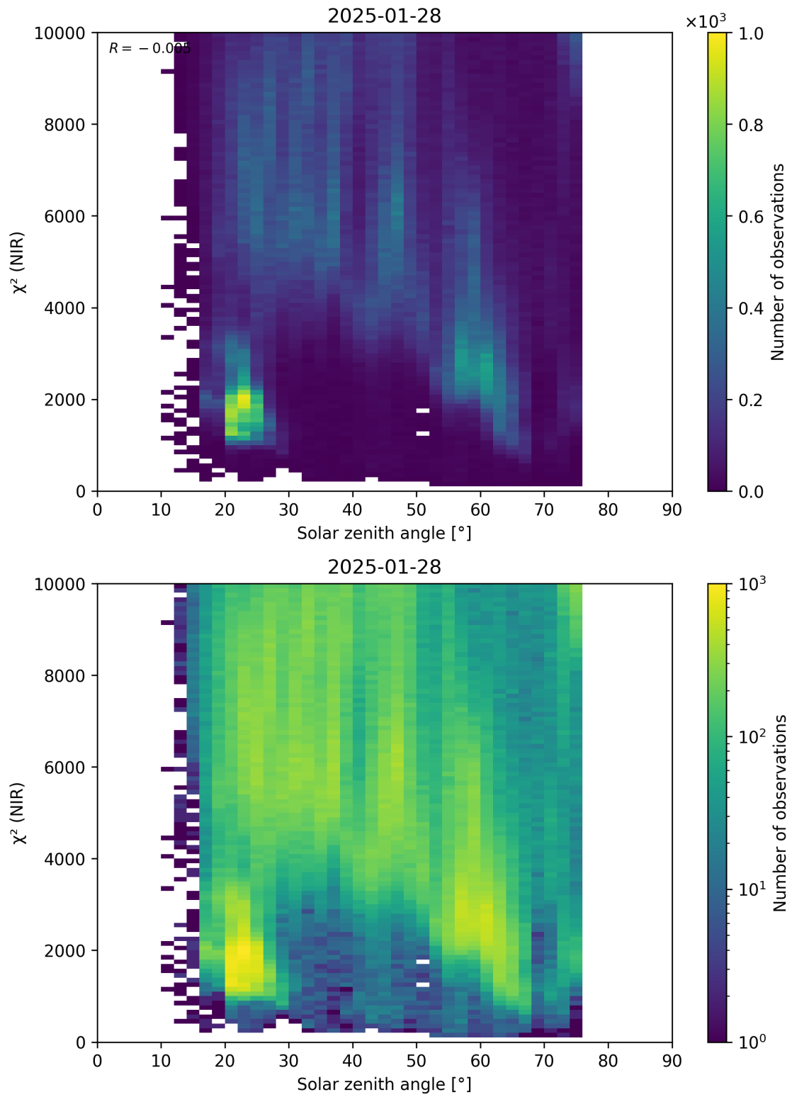
Figure 94: Scatter density plot of “Solar zenith angle” against “ \chi^2 (NIR)” for 2025-01-28 to 2025-01-29.
