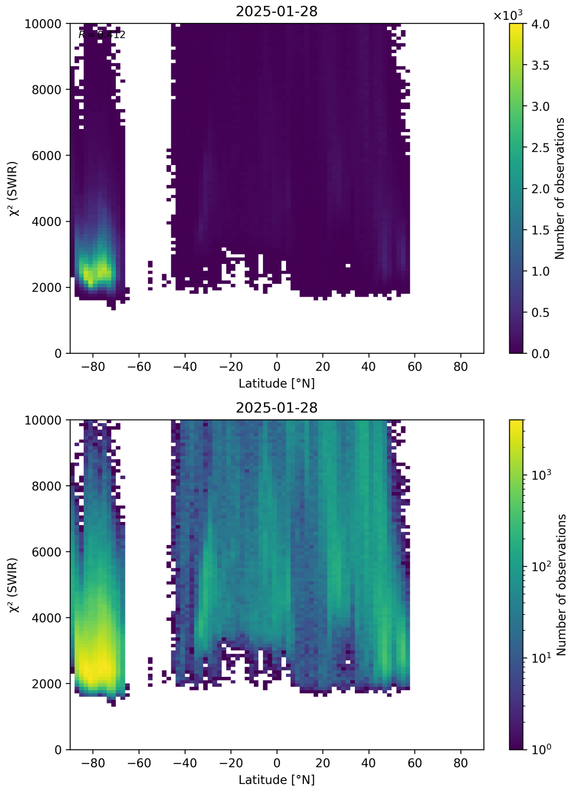
Figure 54: Scatter density plot of “Latitude” against “ \chi^2 (SWIR)” for 2025-01-28 to 2025-01-29.
