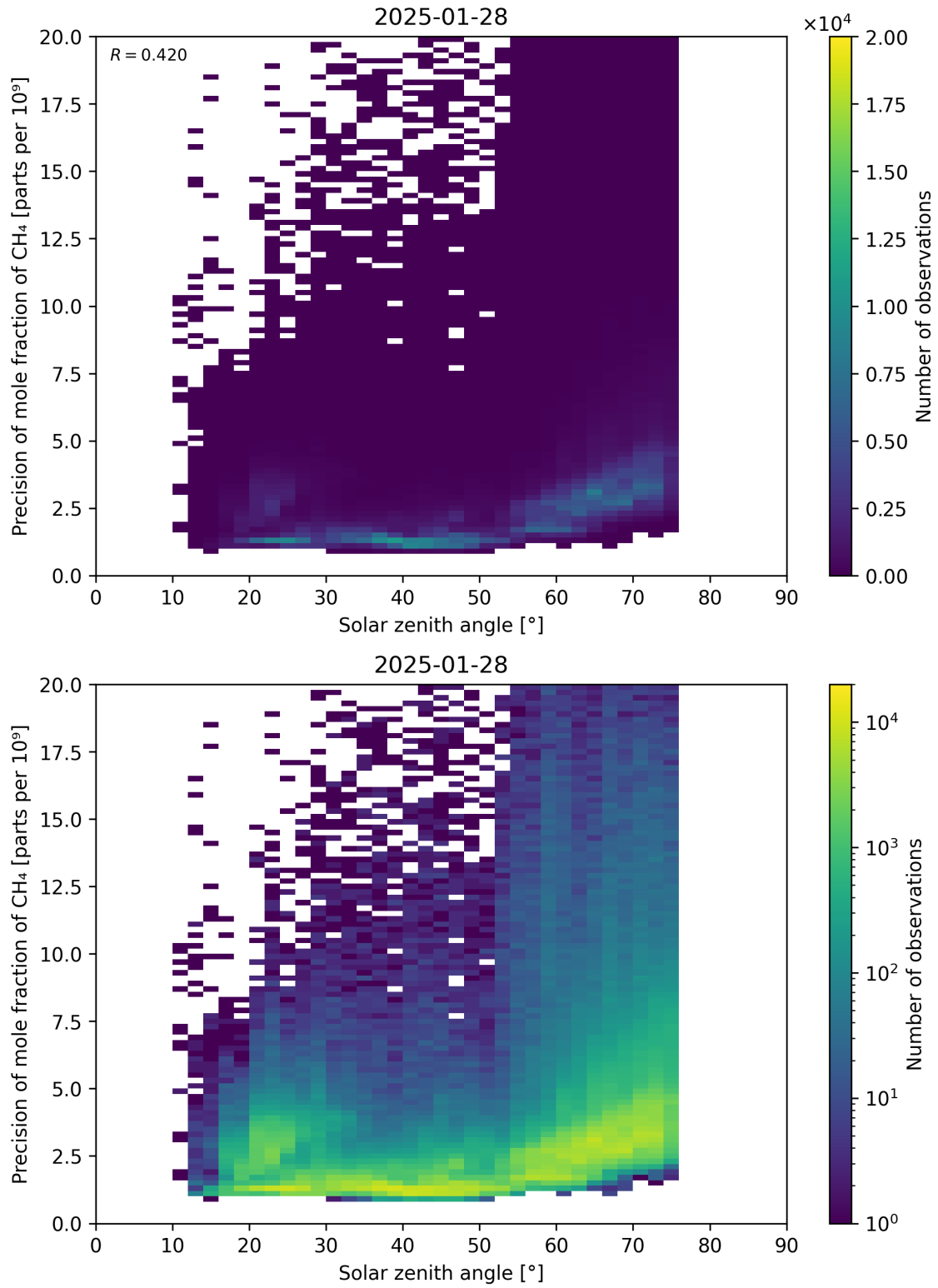
Figure 101: Scatter density plot of “Solar zenith angle” against “Precision of mole fraction of CH 4 ” for 2025-01-28 to 2025-01-29.
