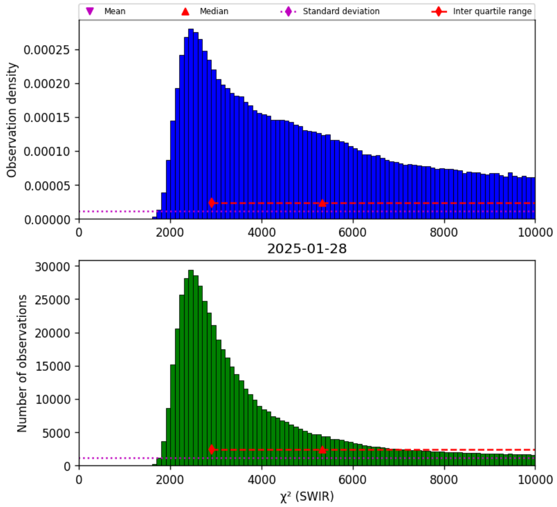
Figure 28: Histogram of “ \chi^2 (SWIR)” for 2025-01-28 to 2025-01-29
