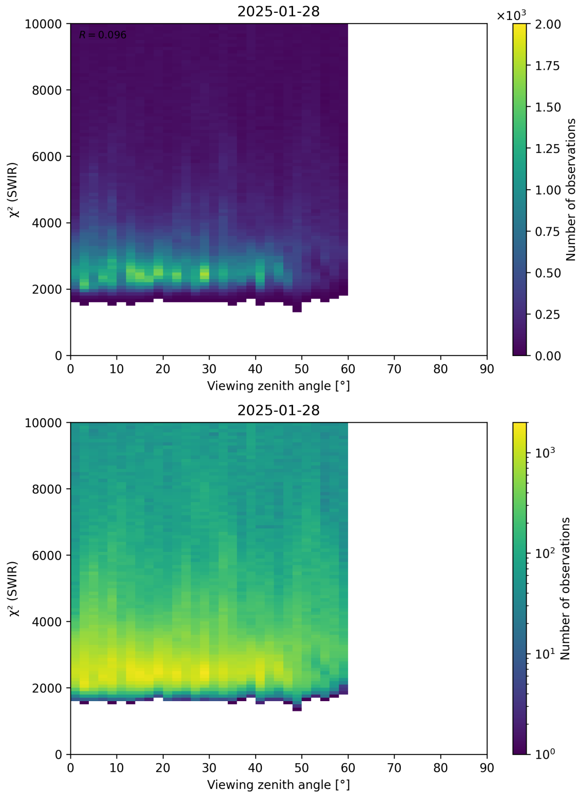
Figure 106: Scatter density plot of “Viewing zenith angle” against “ \chi^2 (SWIR)” for 2025-01-28 to 2025-01-29.
