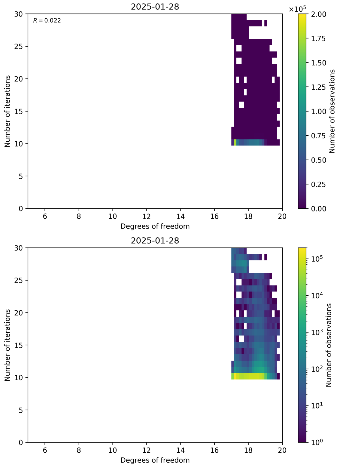
Figure 52: Scatter density plot of “Degrees of freedom” against “Number of iterations” for 2025-01-28 to 2025-01-29.
