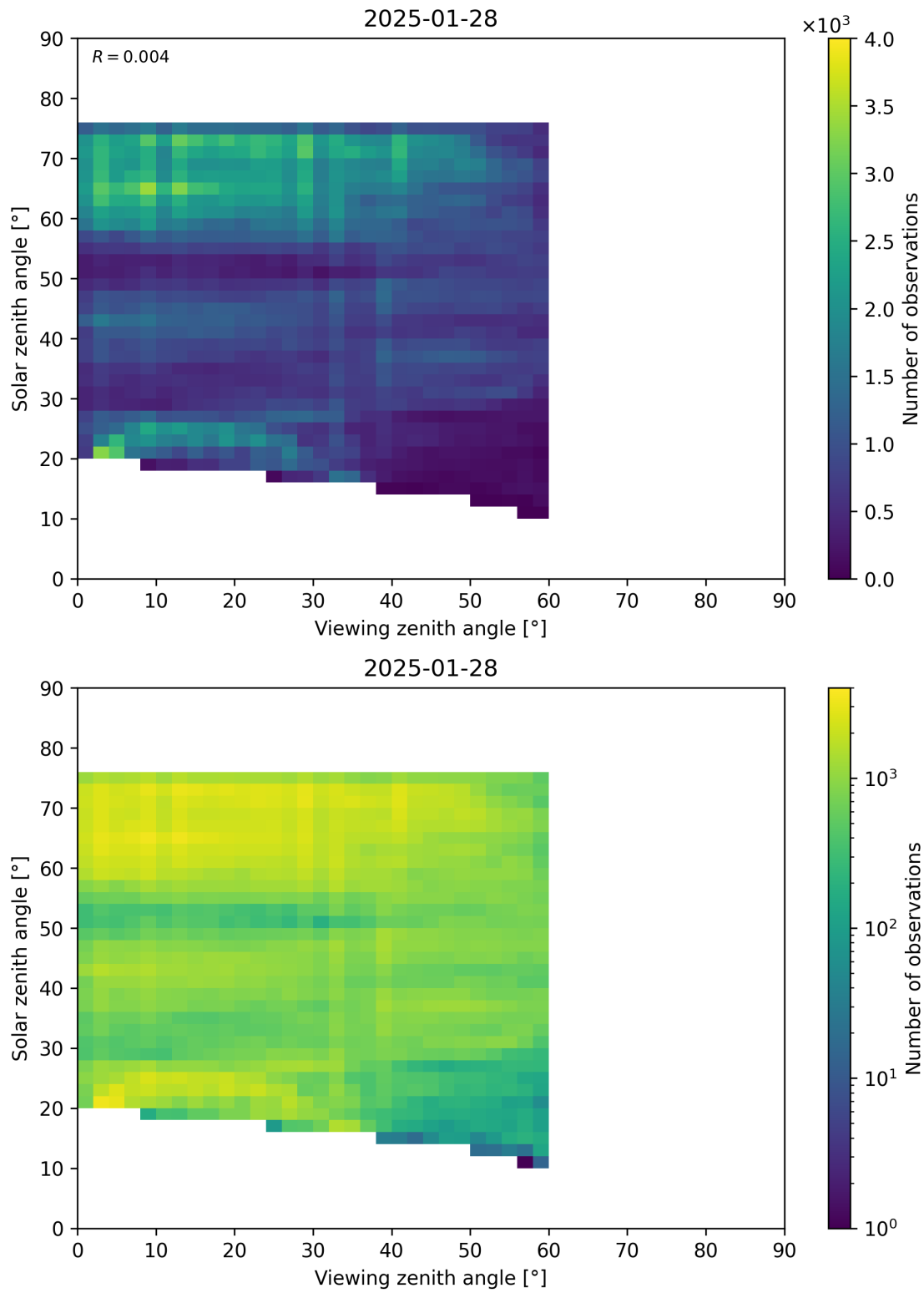
Figure 115: Scatter density plot of “Viewing zenith angle” against “Solar zenith angle” for 2025-01-28 to 2025-01-29.
