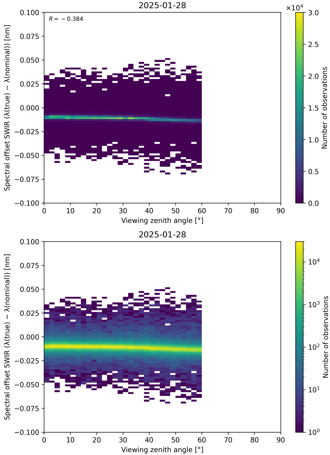
Figure 116: Scatter density plot of “Viewing zenith angle” against “Spectral offset SWIR ( \lambda_{\text{true}} - \lambda_{\text{nominal}} )” for 2025-01-28 to 2025-01-29.
