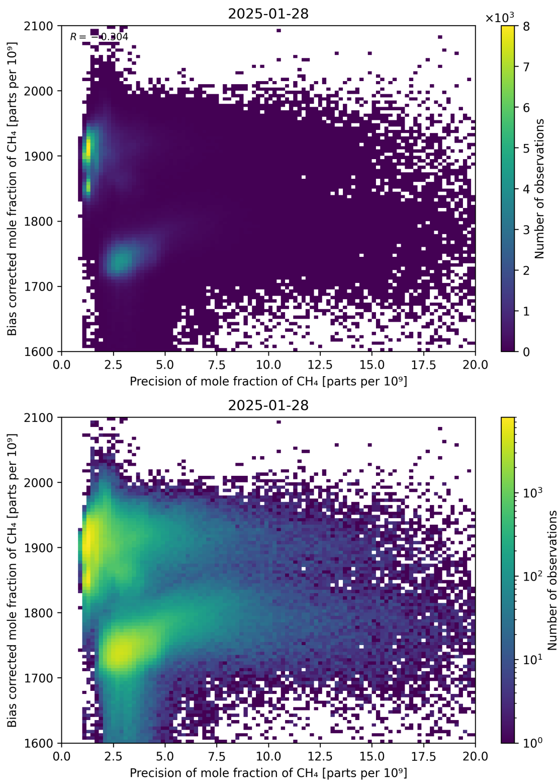
Figure 82: Scatter density plot of “Precision of mole fraction of CH 4 ” against “Bias corrected mole fraction of CH 4 ” for 2025-01-28 to 2025-01-29.
