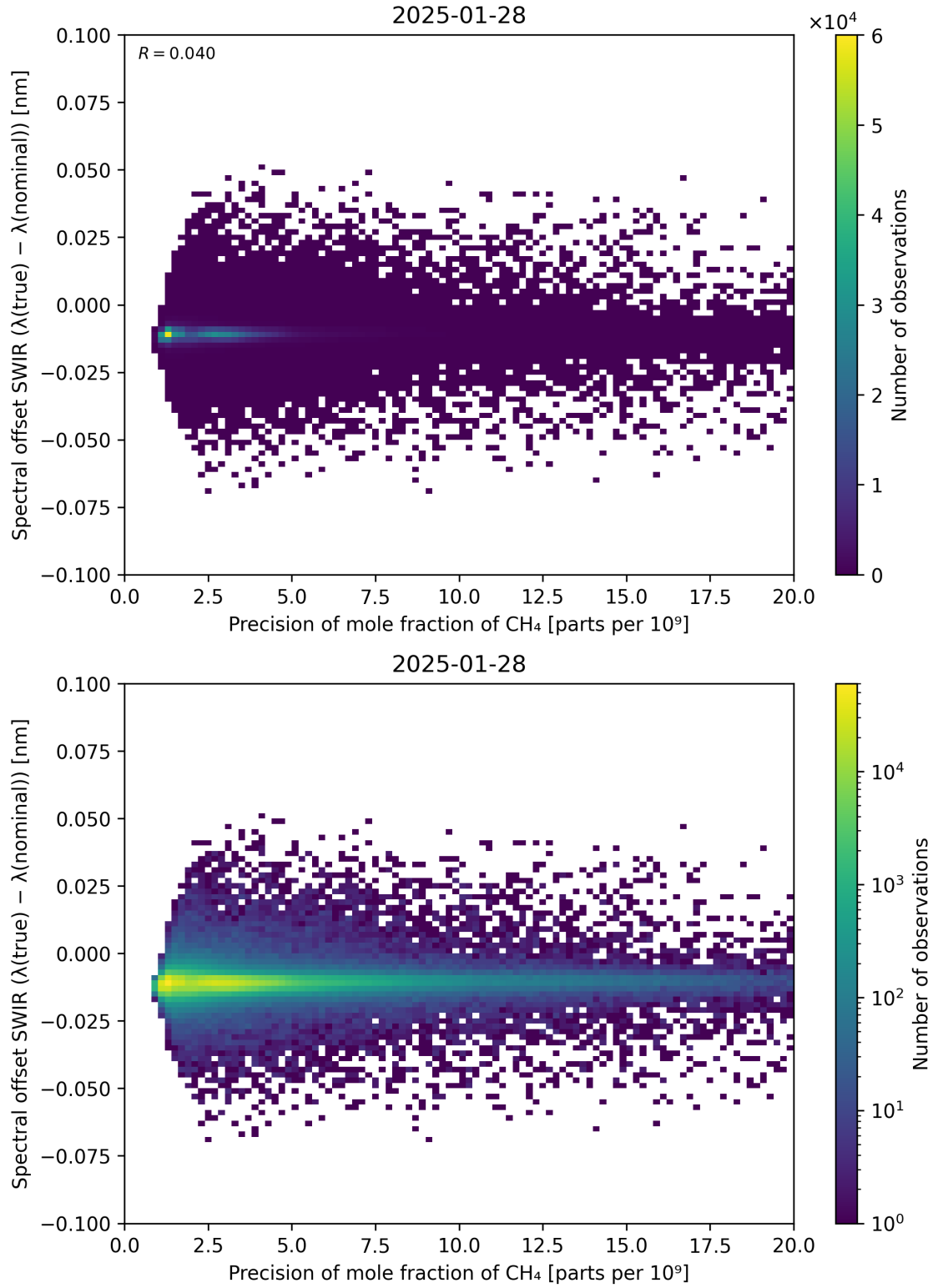
Figure 85: Scatter density plot of “Precision of mole fraction of \text{CH}_4 ” against “Spectral offset SWIR ( \lambda_{\text{true}} - \lambda_{\text{nominal}} )” for 2025-01-28 to 2025-01-29.
