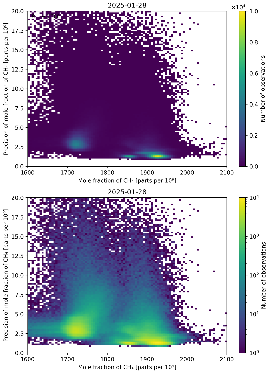
Figure 75: Scatter density plot of “Mole fraction of CH 4 ” against “Precision of mole fraction of CH 4 ” for 2025-01-28 to 2025-01-29.
