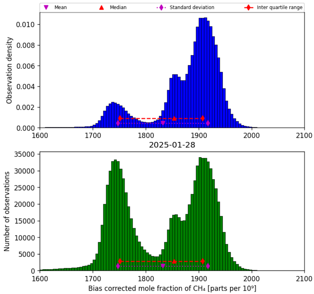
Figure 25: Histogram of “Bias corrected mole fraction of CH 4 ” for 2025-01-28 to 2025-01-29
