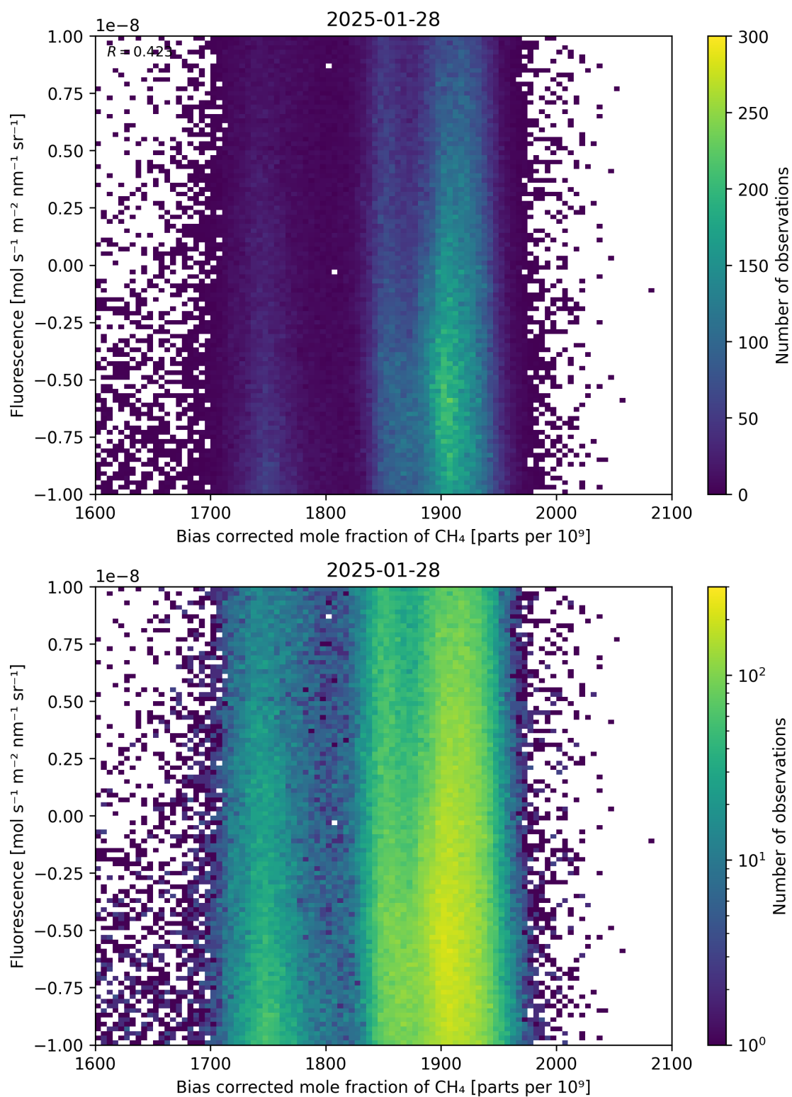
Figure 66: Scatter density plot of “Bias corrected mole fraction of \text{CH}_4 ” against “Fluorescence” for 2025-01-28 to 2025-01-29.
