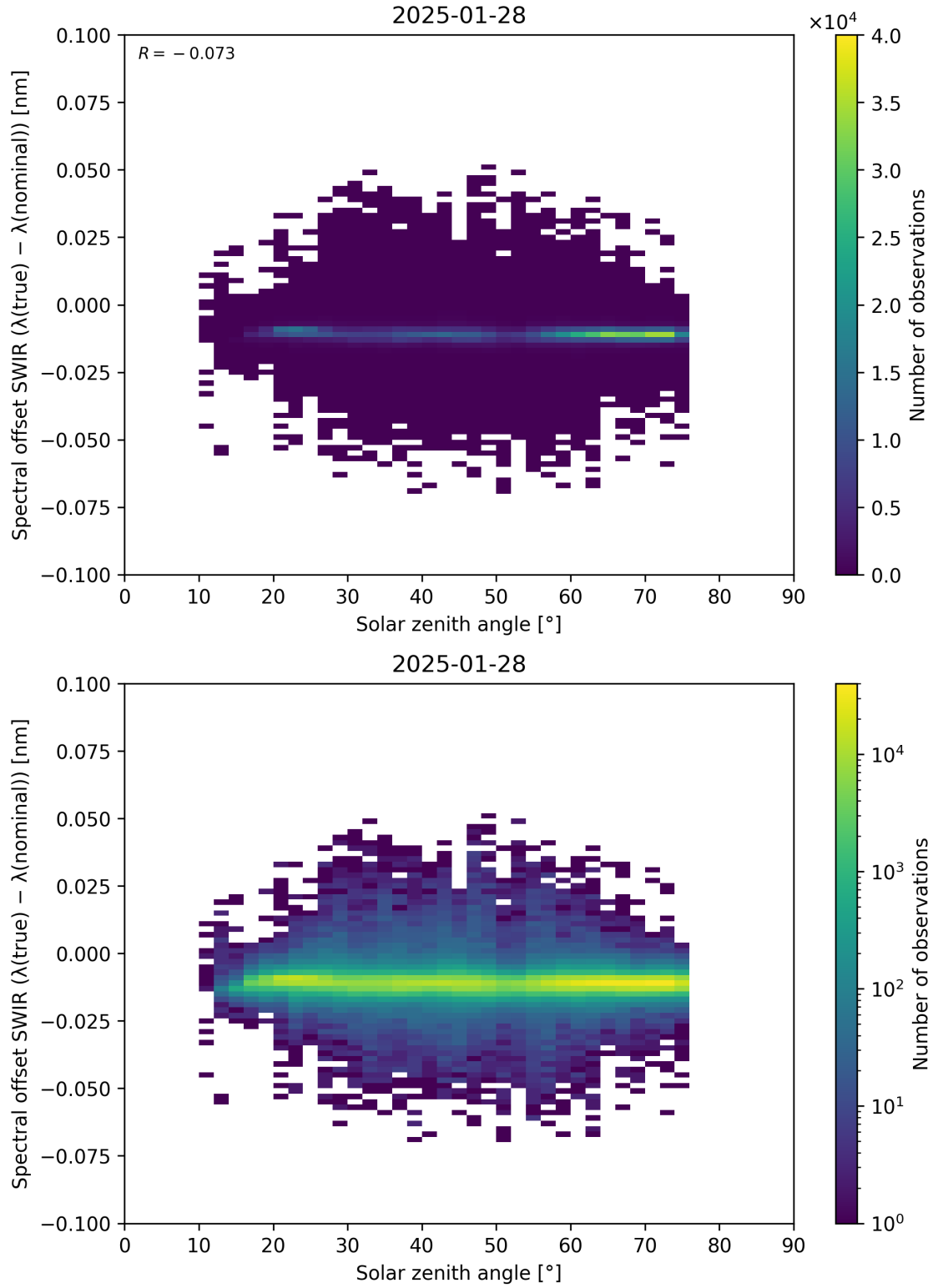
Figure 104: Scatter density plot of “Solar zenith angle” against “Spectral offset SWIR ( \lambda_{\text{true}} - \lambda_{\text{nominal}} )” for 2025-01-28 to 2025-01-29.
