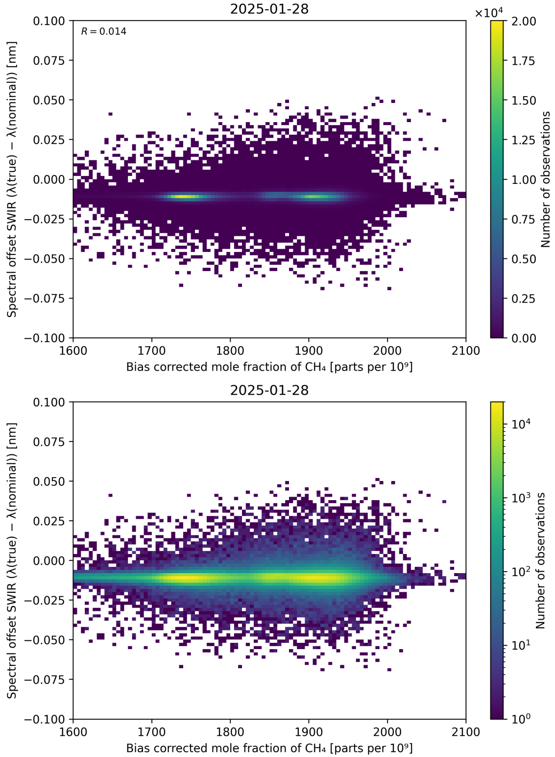
Figure 69: Scatter density plot of “Bias corrected mole fraction of \text{CH}_4 ” against “Spectral offset SWIR ( \lambda_{\text{true}} - \lambda_{\text{nominal}} )” for 2025-01-28 to 2025-01-29.
