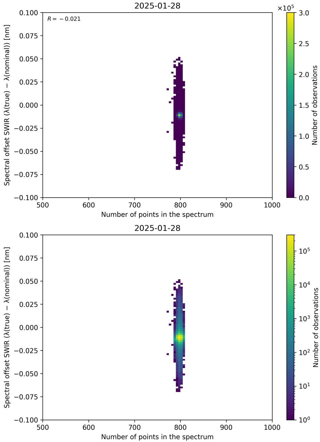
Figure 93: Scatter density plot of “Number of points in the spectrum” against “Spectral offset SWIR ( \lambda_{\text{true}} - \lambda_{\text{nominal}} )” for 2025-01-28 to 2025-01-29.
