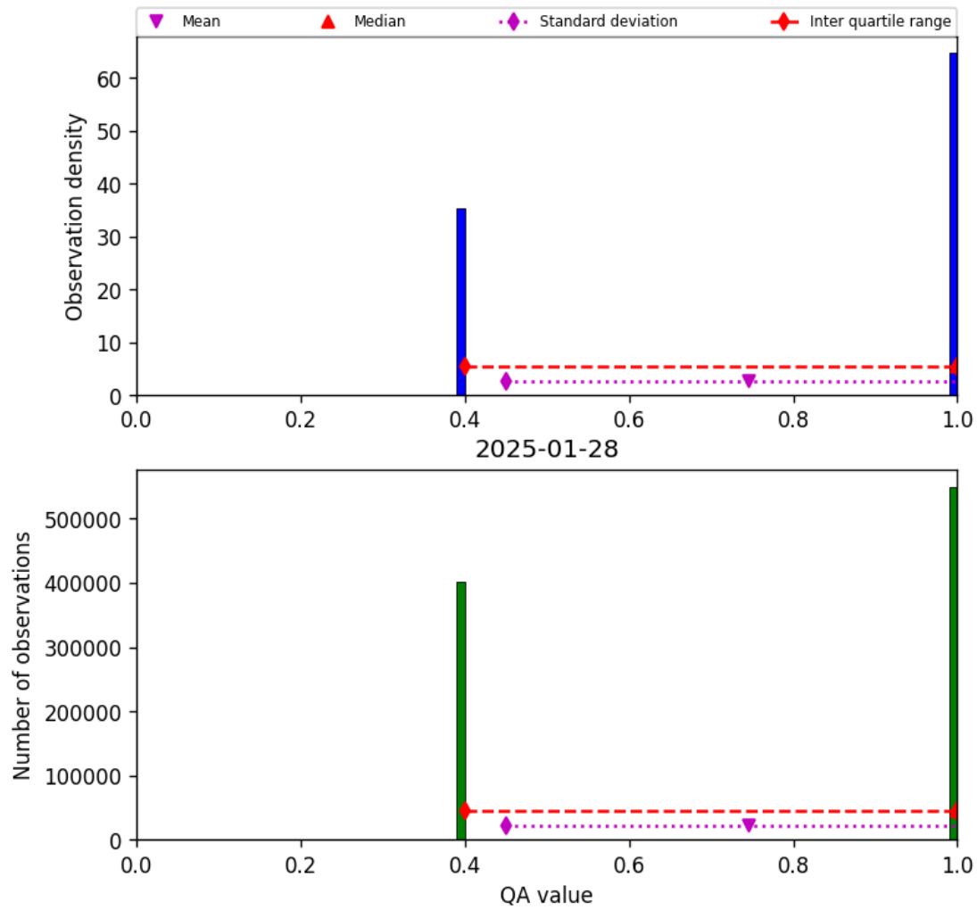
Figure 22: Histogram of “QA value” for 2025-01-28 to 2025-01-29
