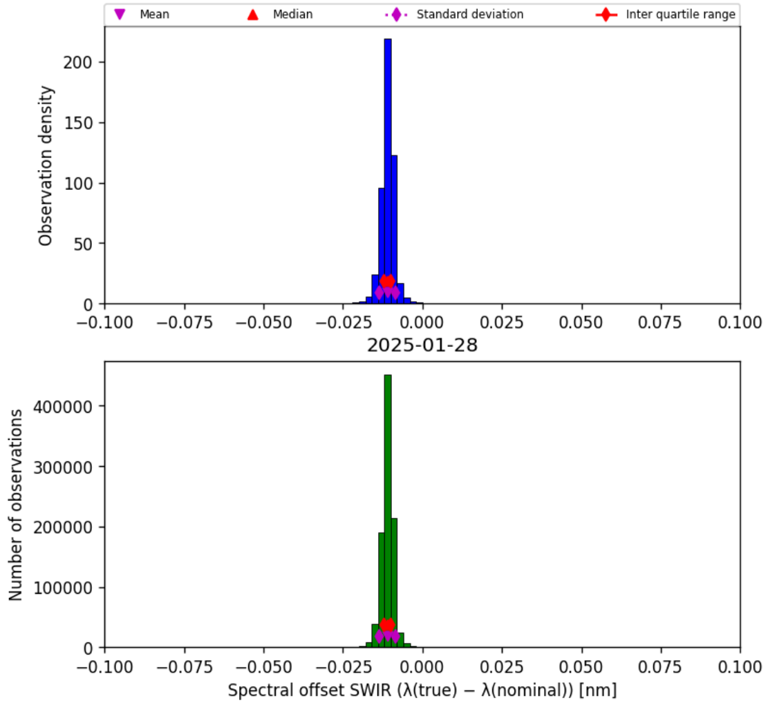
Figure 27: Histogram of “Spectral offset SWIR ( \lambda_{\text{true}} - \lambda_{\text{nominal}} )” for 2025-01-28 to 2025-01-29
