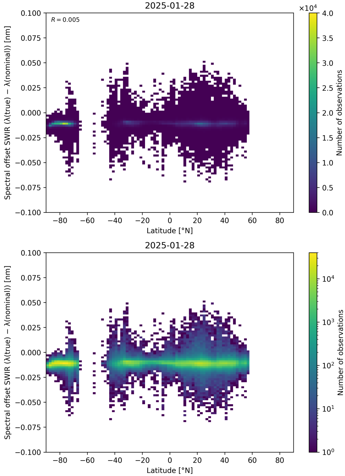
Figure 62: Scatter density plot of “Latitude” against “Spectral offset SWIR ( \lambda_{\text{true}} - \lambda_{\text{nominal}} )” for 2025-01-28 to 2025-01-29.
