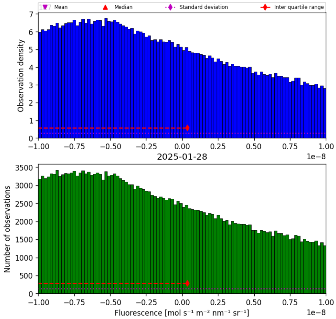
Figure 32: Histogram of “Fluorescence” for 2025-01-28 to 2025-01-29
