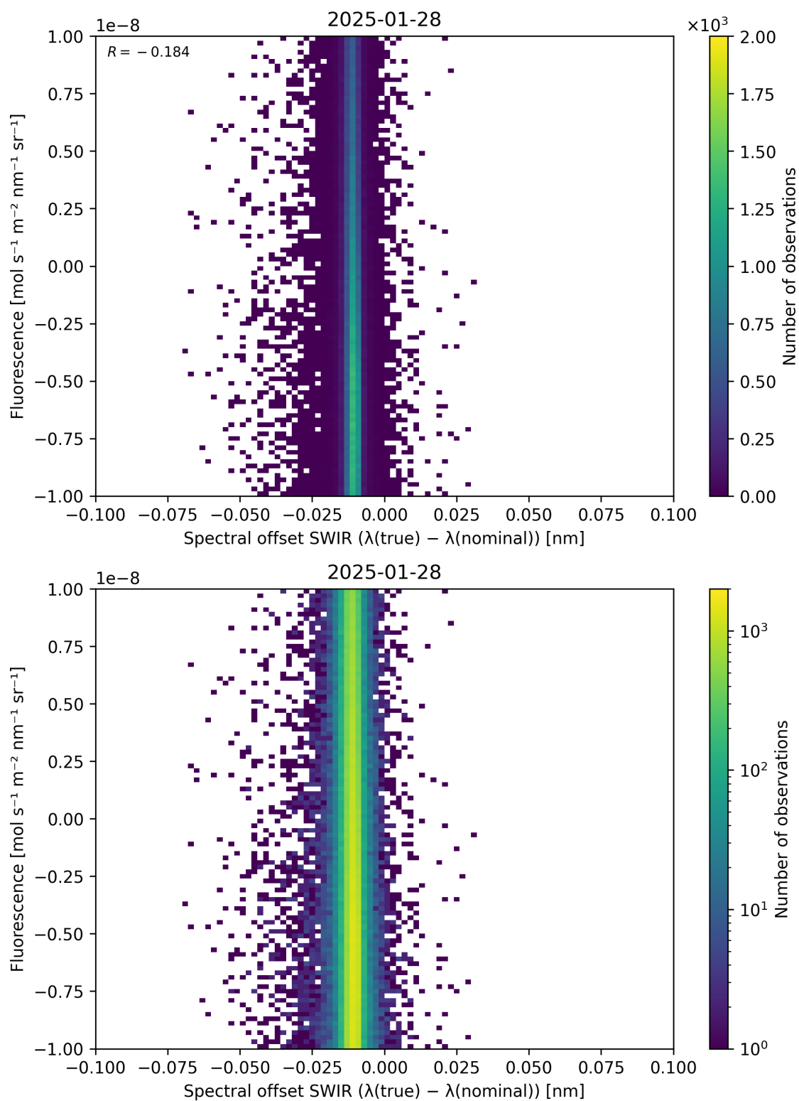
Figure 120: Scatter density plot of “Spectral offset SWIR ( \lambda_{\text{true}} - \lambda_{\text{nominal}} )” against “Fluorescence” for 2025-01-28 to 2025-01-29.
