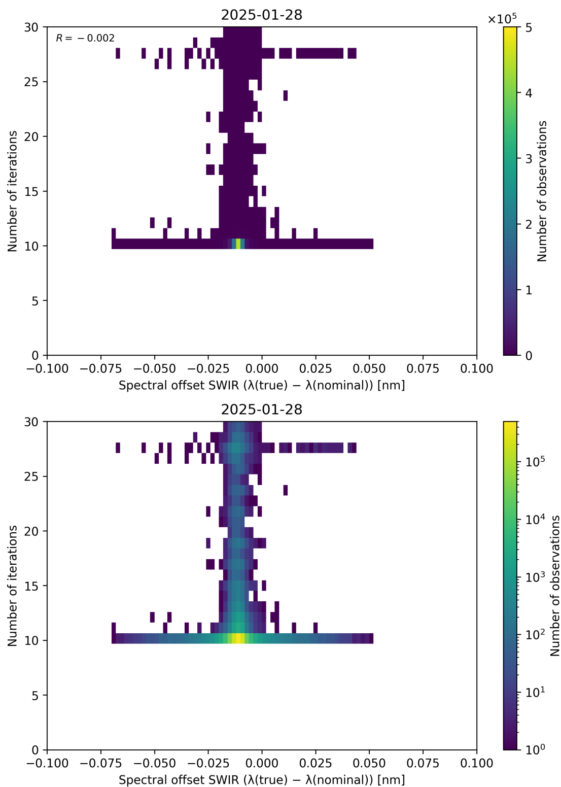
Figure 121: Scatter density plot of “Spectral offset SWIR ( \lambda_{\text{true}} - \lambda_{\text{nominal}} )” against “Number of iterations” for 2025-01-28 to 2025-01-29.
