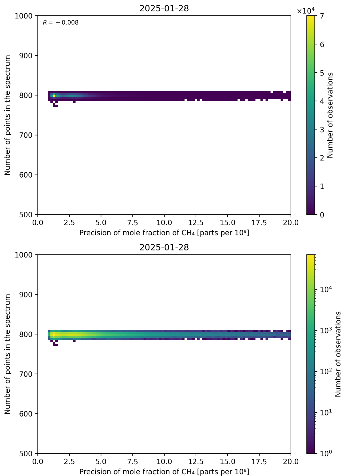
Figure 84: Scatter density plot of “Precision of mole fraction of CH 4 ” against “Number of points in the spectrum” for 2025-01-28 to 2025-01-29.
