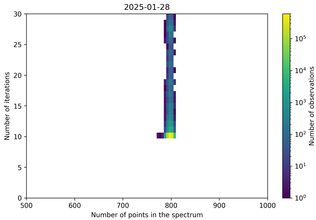
Figure 92: Scatter density plot of “Number of points in the spectrum” against “Number of iterations” for 2025-01-28 to 2025-01-29.
