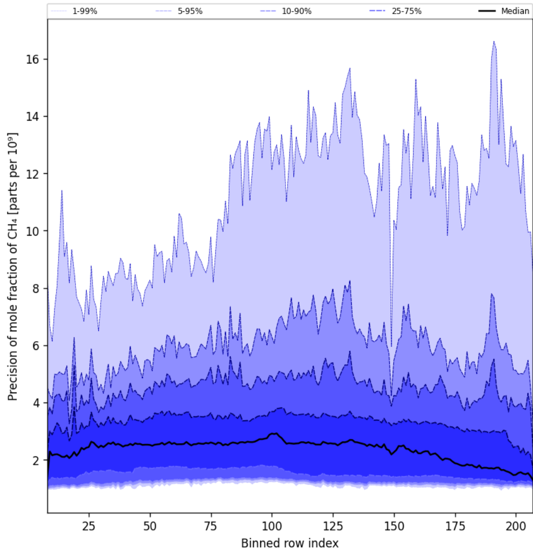
Figure 35: Along track statistics of “Precision of mole fraction of CH 4 ” for 2025-01-28 to 2025-01-29
