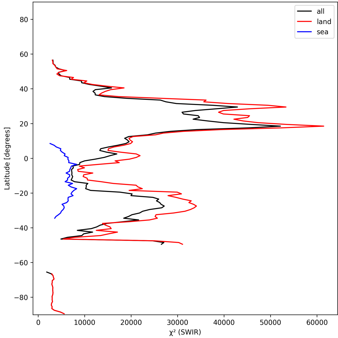
Figure 17: Zonal average of “ \chi^2 (SWIR)” for 2025-01-28 to 2025-01-29.
