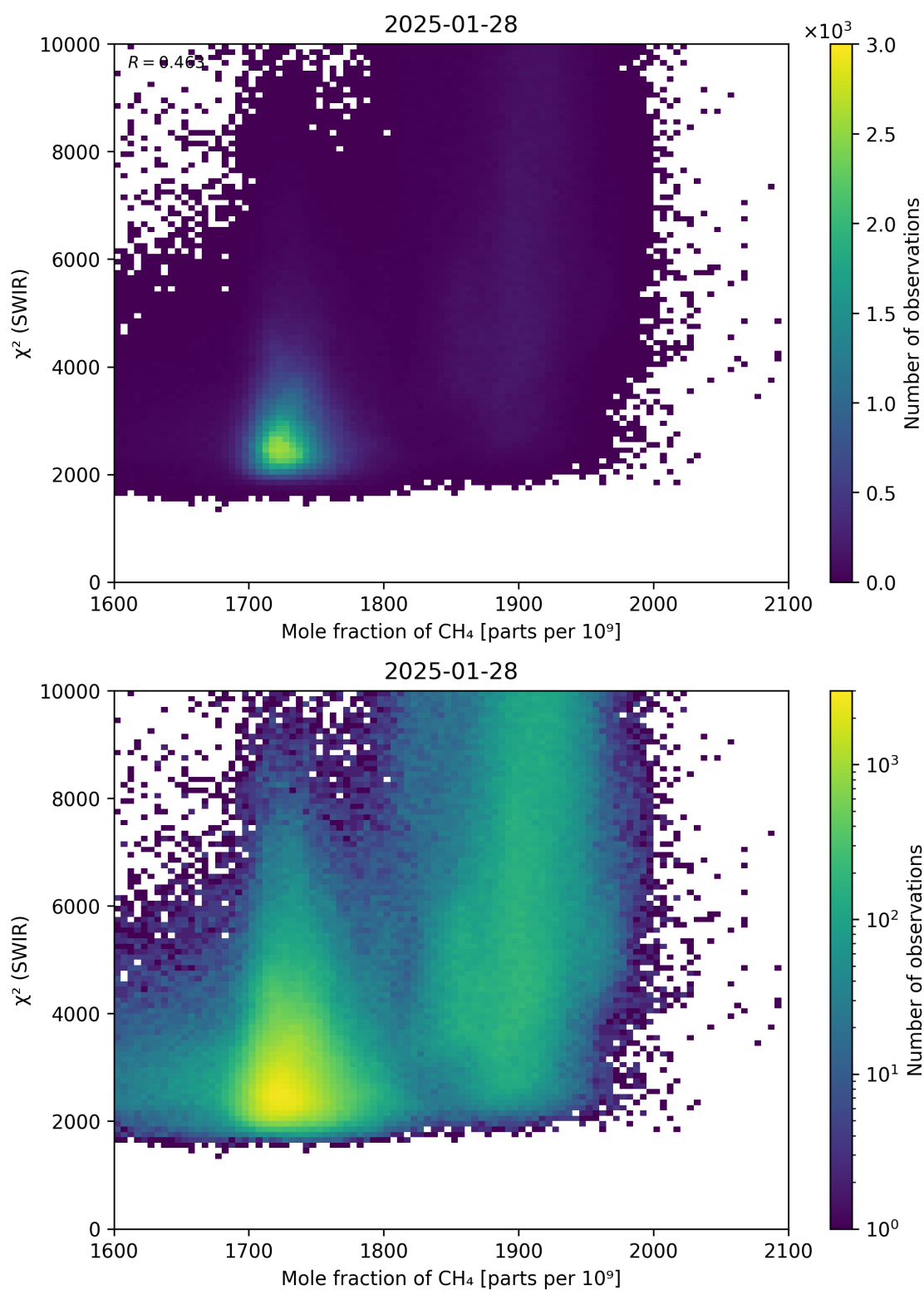
Figure 71: Scatter density plot of “Mole fraction of \text{CH}_4 ” against “ \chi^2 (SWIR)” for 2025-01-28 to 2025-01-29.
