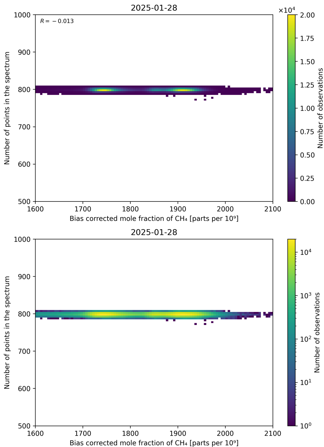
Figure 68: Scatter density plot of “Bias corrected mole fraction of CH 4 ” against “Number of points in the spectrum” for 2025-01-28 to 2025-01-29.
