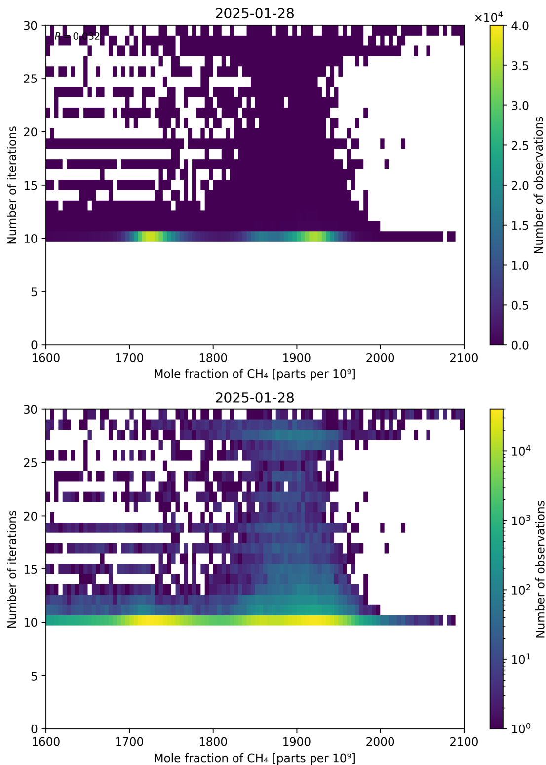
Figure 76: Scatter density plot of “Mole fraction of CH 4 ” against “Number of iterations” for 2025-01-28 to 2025-01-29.
