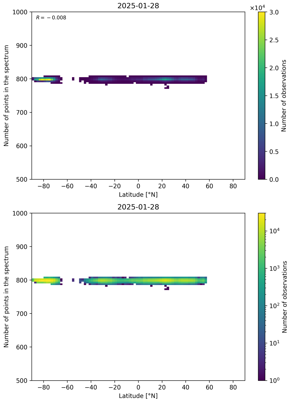
Figure 61: Scatter density plot of “Latitude” against “Number of points in the spectrum” for 2025-01-28 to 2025-01-29.
