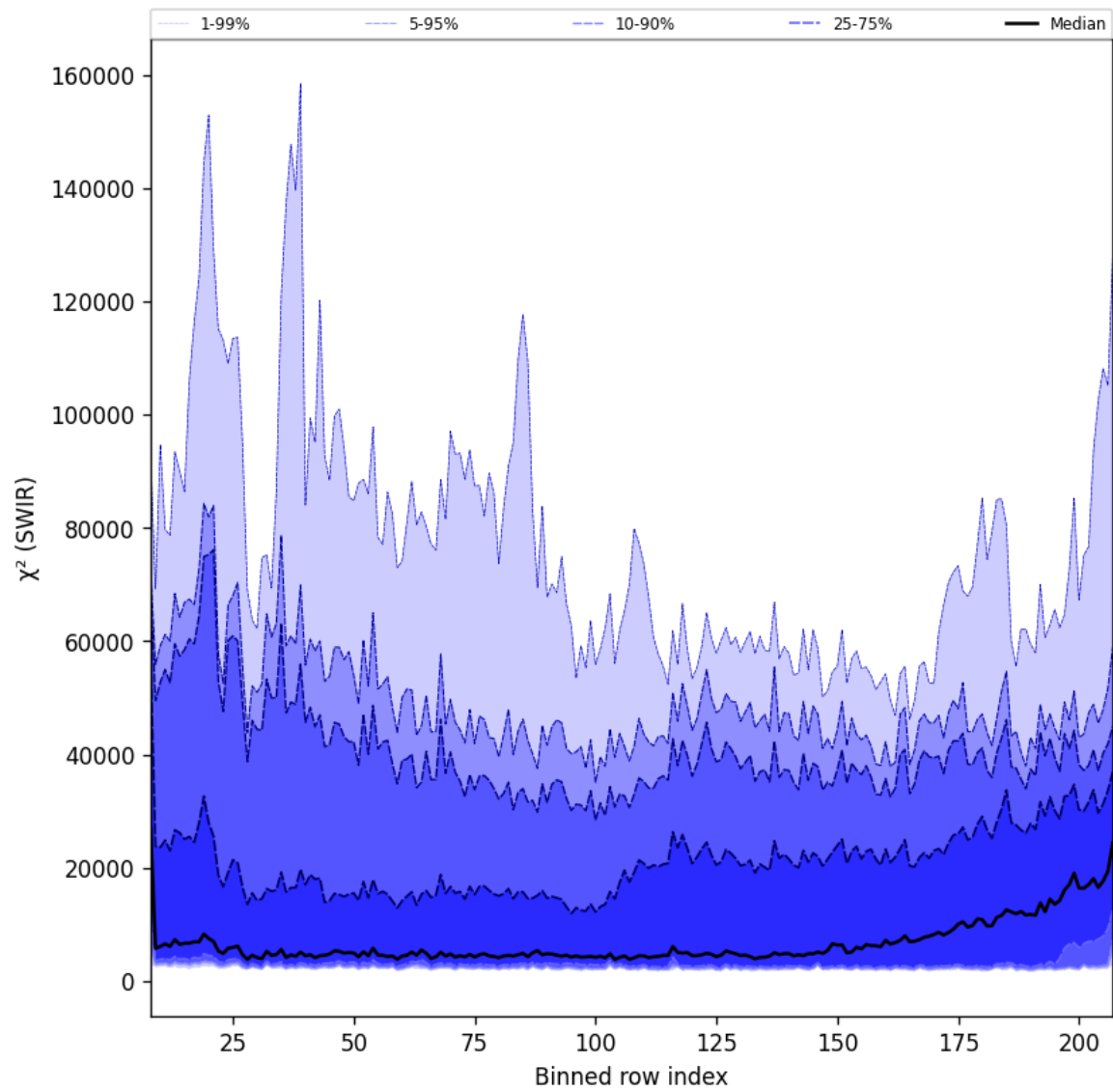
Figure 39: Along track statistics of “ \chi^2 (SWIR)” for 2025-01-28 to 2025-01-29
