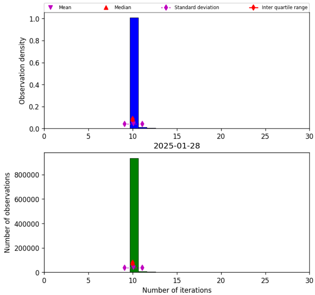
Figure 31: Histogram of “Number of iterations” for 2025-01-28 to 2025-01-29
