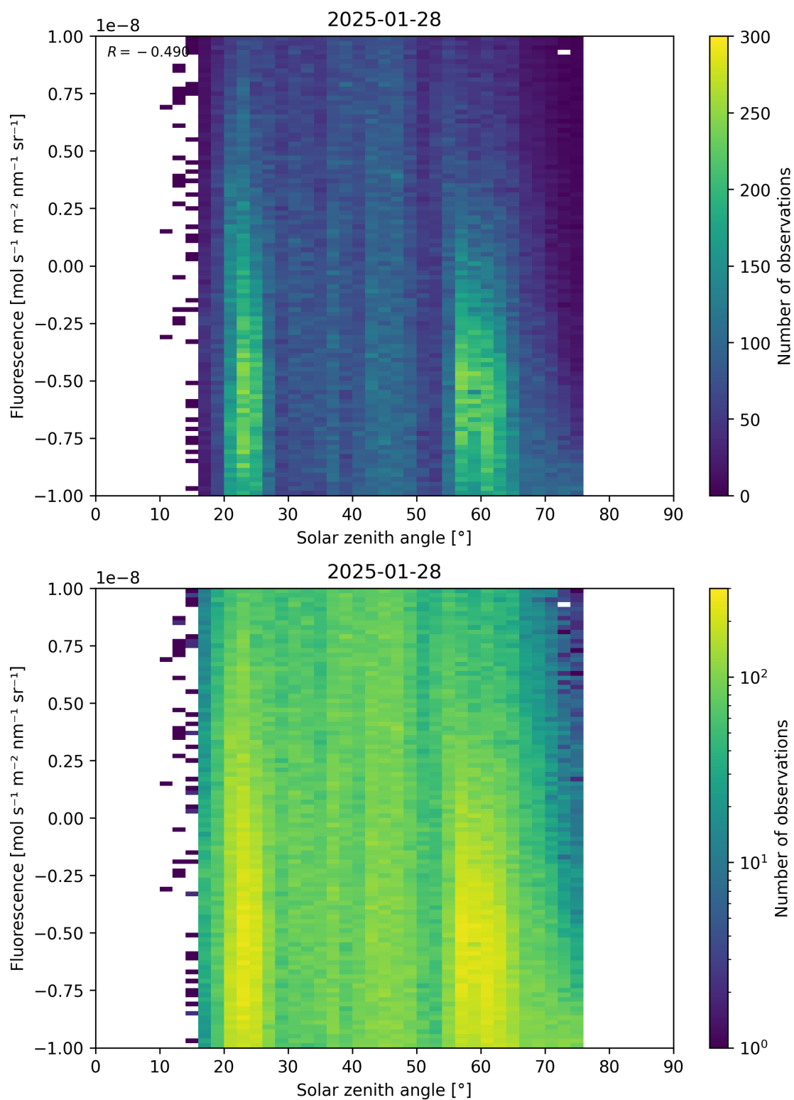
Figure 97: Scatter density plot of “Solar zenith angle” against “Fluorescence” for 2025-01-28 to 2025-01-29.
