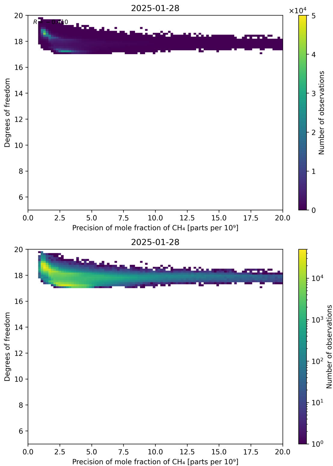
Figure 80: Scatter density plot of “Precision of mole fraction of CH 4 ” against “Degrees of freedom” for 2025-01-28 to 2025-01-29.
