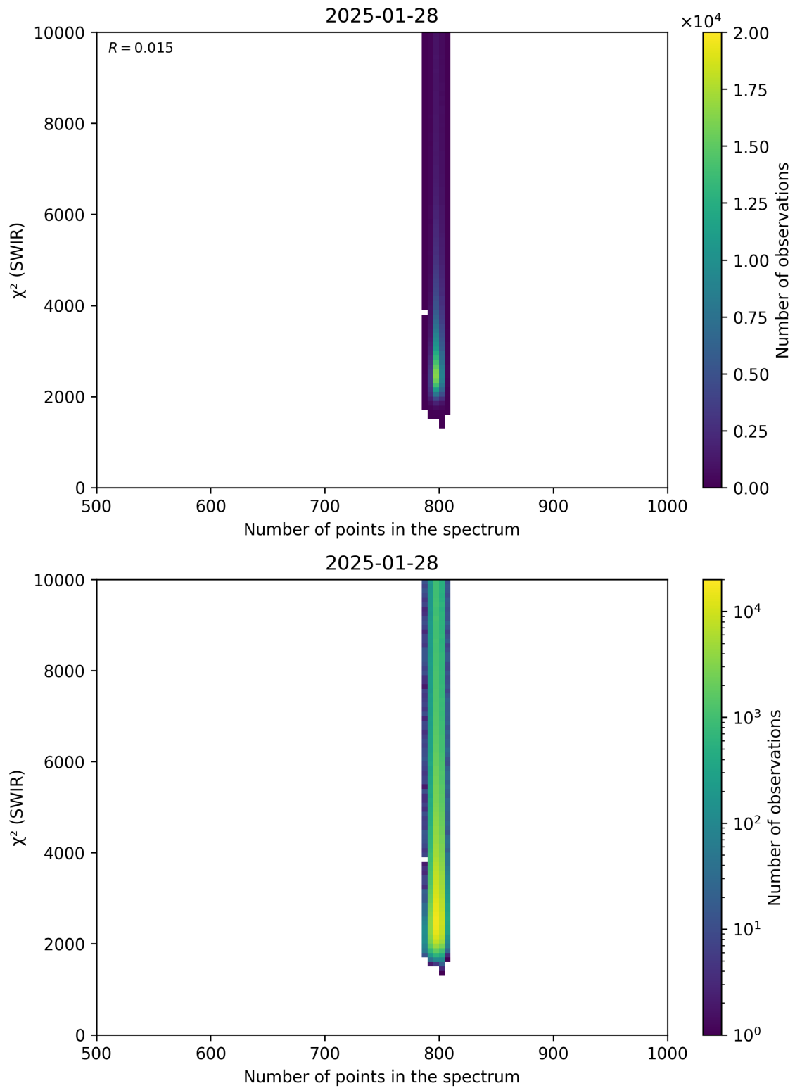
Figure 89: Scatter density plot of “Number of points in the spectrum” against “ \chi^2 (SWIR)” for 2025-01-28 to 2025-01-29.
