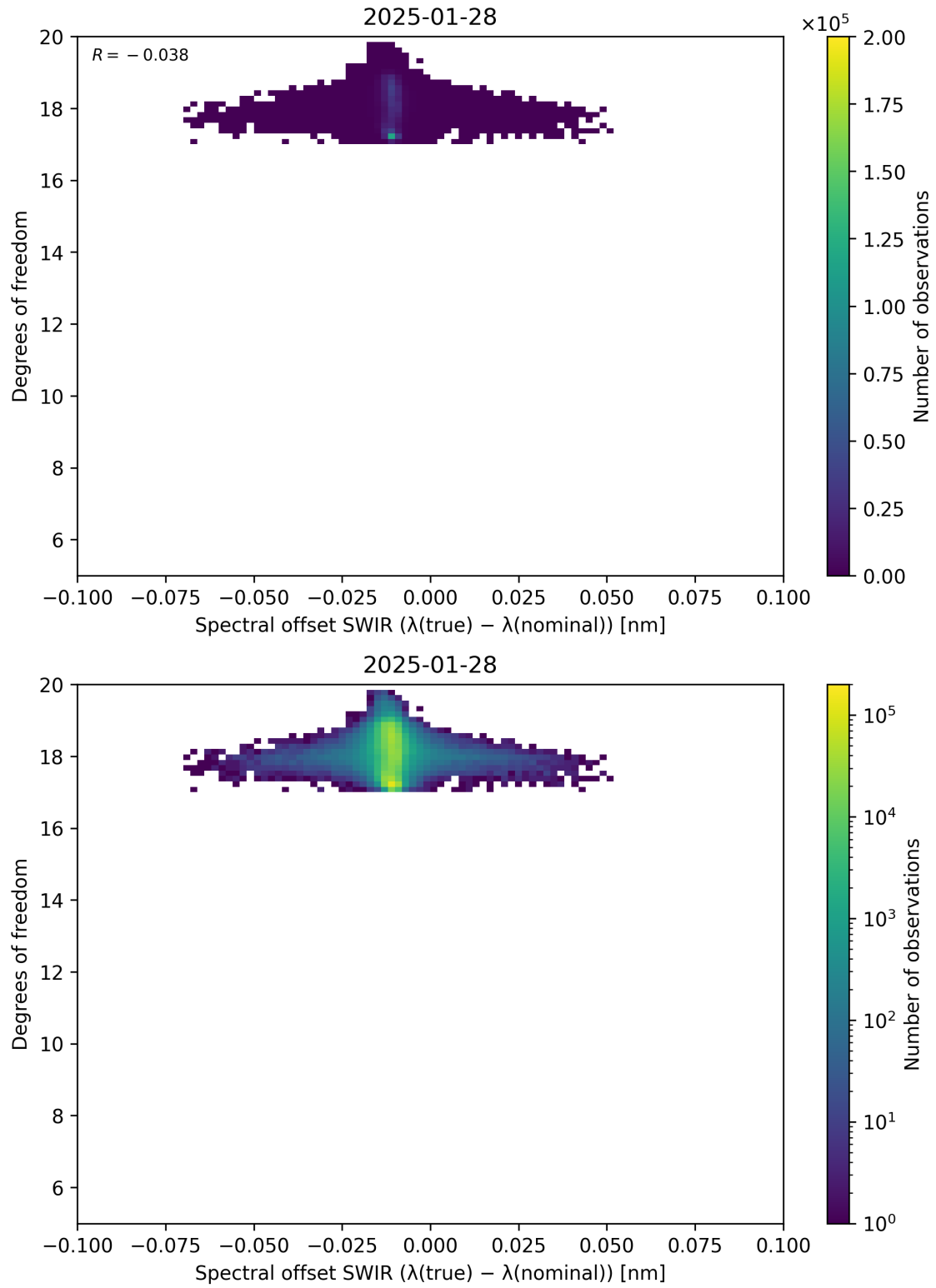
Figure 119: Scatter density plot of “Spectral offset SWIR ( \lambda_{\text{true}} - \lambda_{\text{nominal}} )” against “Degrees of freedom” for 2025-01-28 to 2025-01-29.
