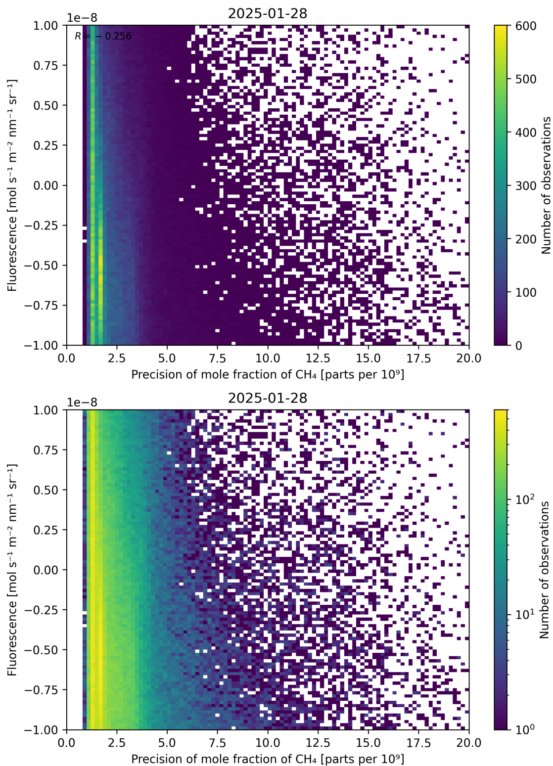
Figure 81: Scatter density plot of “Precision of mole fraction of CH 4 ” against “Fluorescence” for 2025-01-28 to 2025-01-29.
