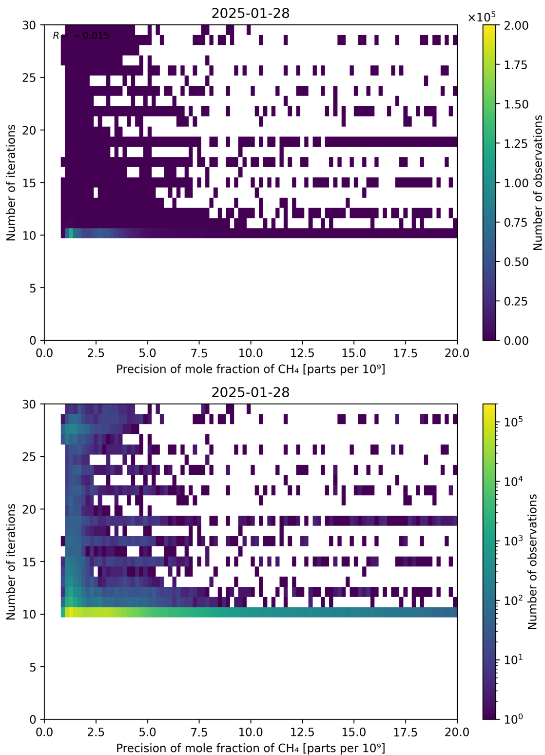
Figure 83: Scatter density plot of “Precision of mole fraction of CH 4 ” against “Number of iterations” for 2025-01-28 to 2025-01-29.
