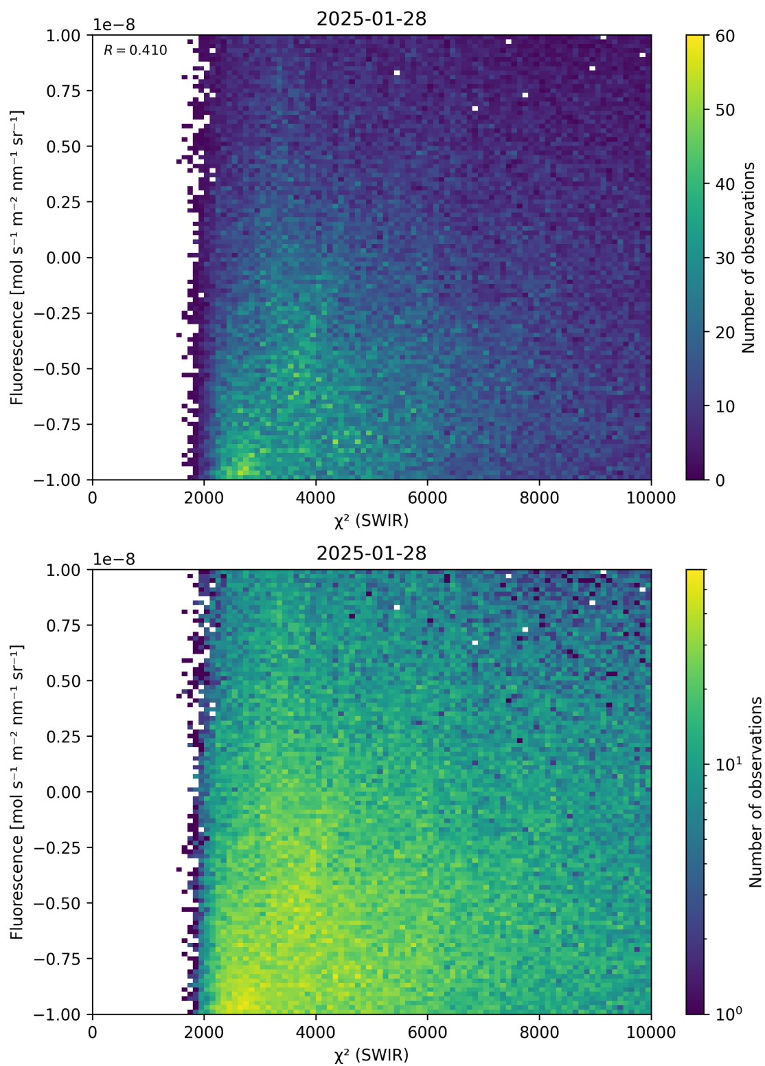
Figure 49: Scatter density plot of “ \chi^2 (SWIR)” against “Fluorescence” for 2025-01-28 to 2025-01-29.
