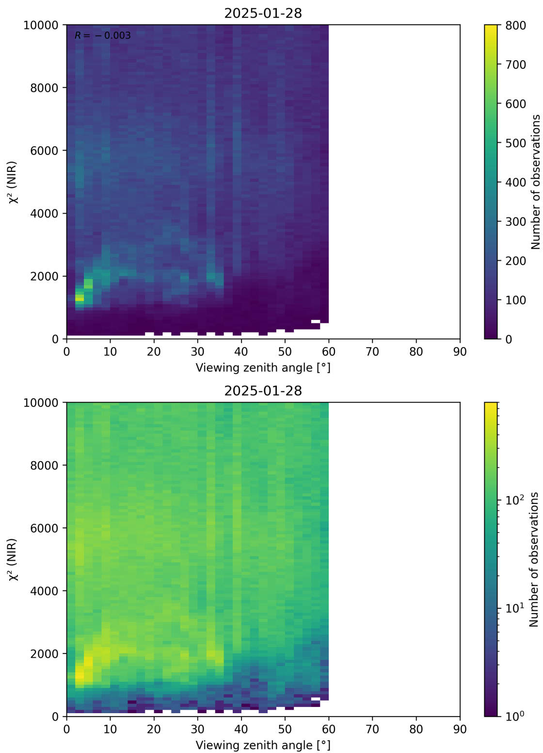
Figure 105: Scatter density plot of “Viewing zenith angle” against “ \chi^2 (NIR)” for 2025-01-28 to 2025-01-29.
