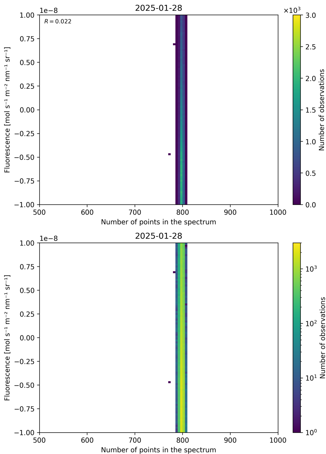
Figure 91: Scatter density plot of “Number of points in the spectrum” against “Fluorescence” for 2025-01-28 to 2025-01-29.
