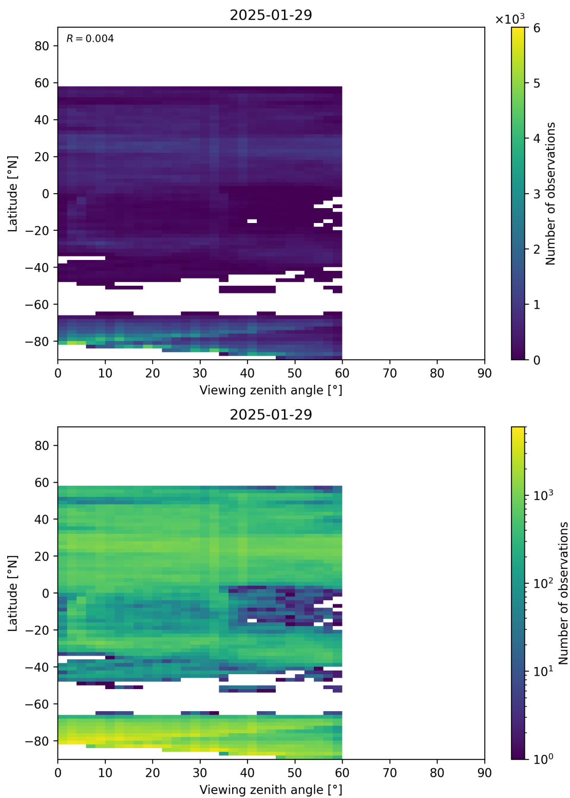
Figure 109: Scatter density plot of “Viewing zenith angle” against “Latitude” for 2025-01-28 to 2025-01-30.
