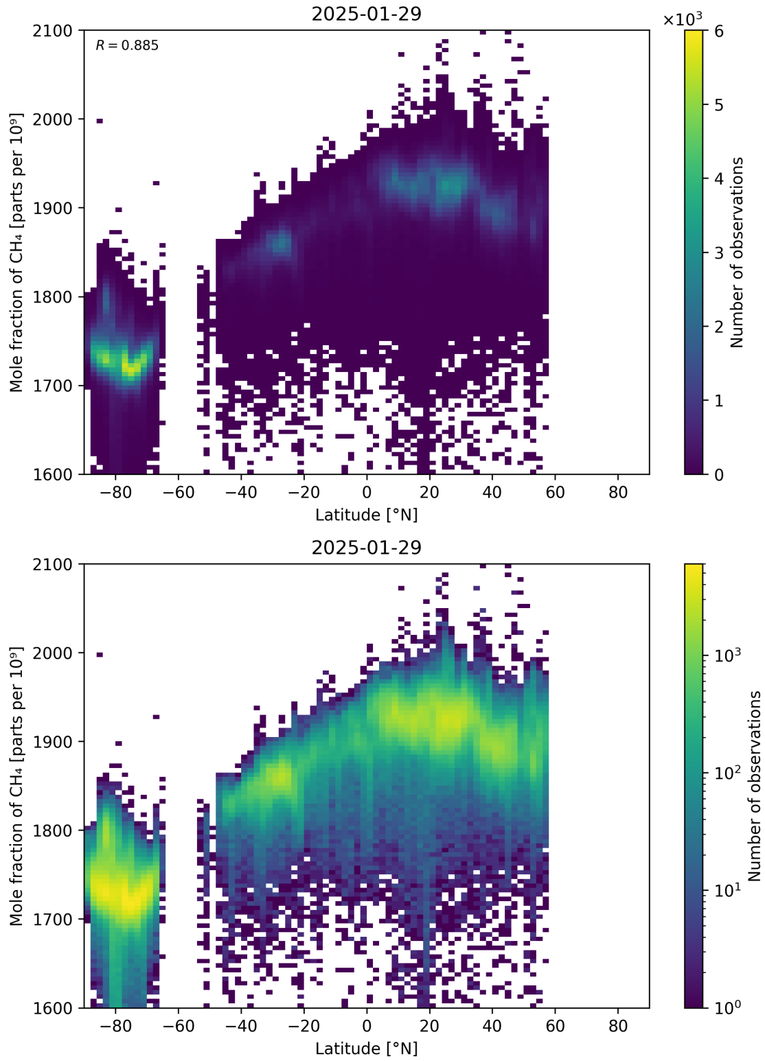
Figure 57: Scatter density plot of “Latitude” against “Mole fraction of \text{CH}_4 ” for 2025-01-28 to 2025-01-30.
