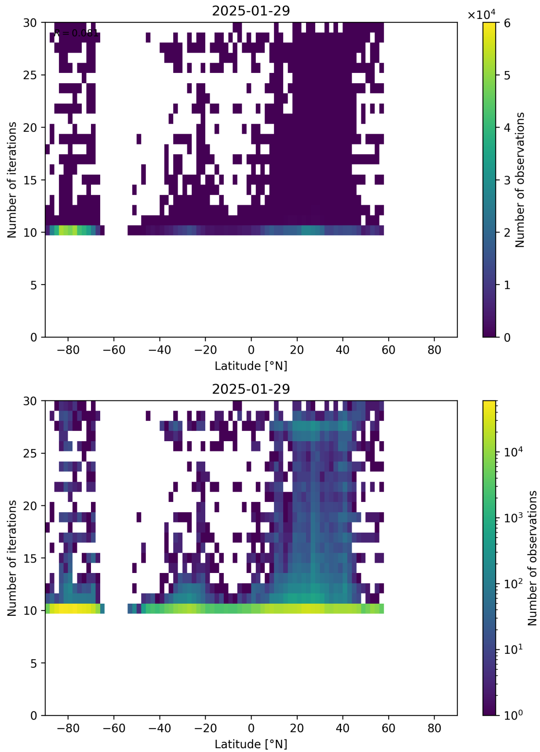
Figure 60: Scatter density plot of “Latitude” against “Number of iterations” for 2025-01-28 to 2025-01-30.
