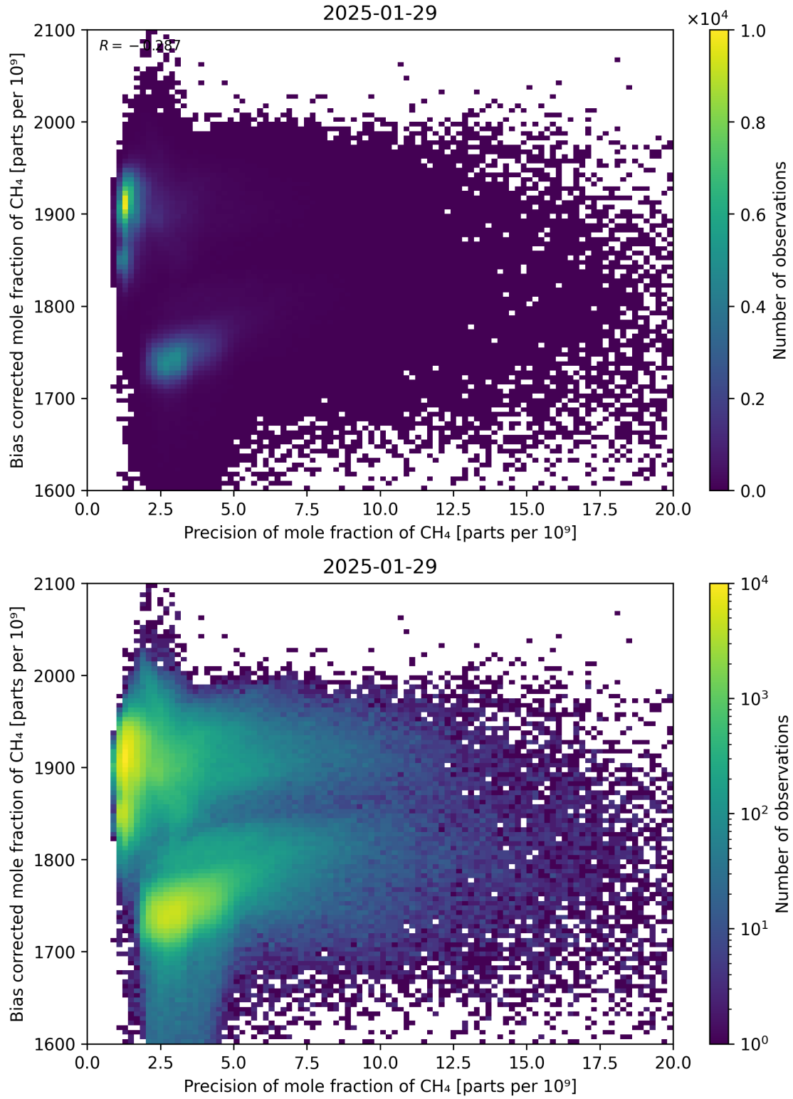
Figure 82: Scatter density plot of “Precision of mole fraction of CH 4 ” against “Bias corrected mole fraction of CH 4 ” for 2025-01-28 to 2025-01-30.
