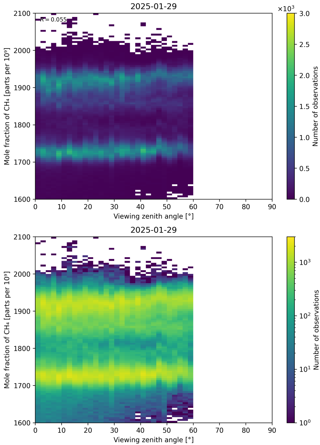
Figure 110: Scatter density plot of “Viewing zenith angle” against “Mole fraction of \text{CH}_4 ” for 2025-01-28 to 2025-01-30.
