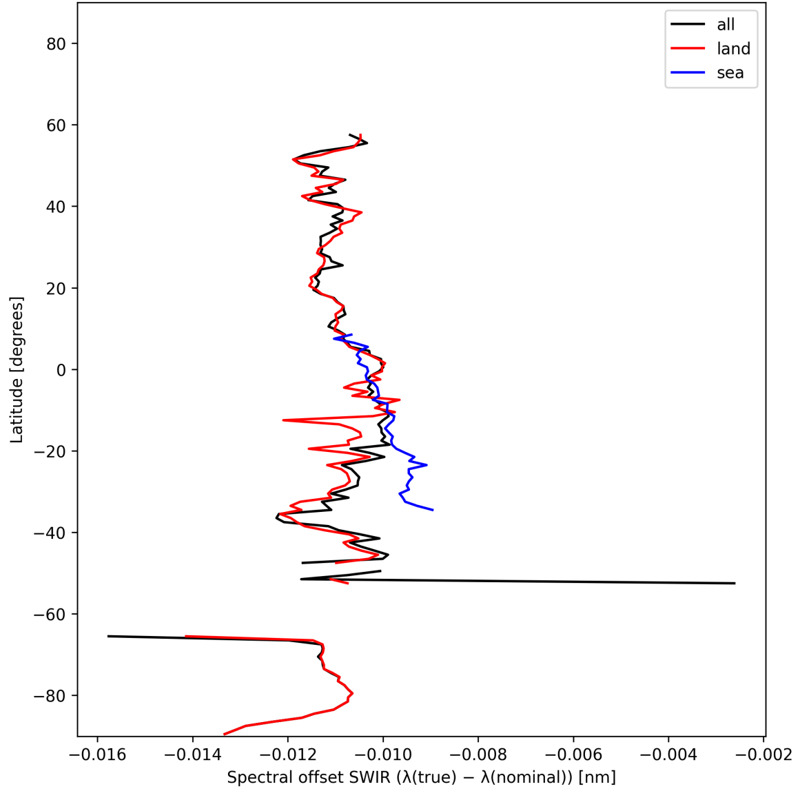
Figure 16: Zonal average of “Spectral offset SWIR ( \lambda_{\text{true}} - \lambda_{\text{nominal}} )” for 2025-01-28 to 2025-01-30.
