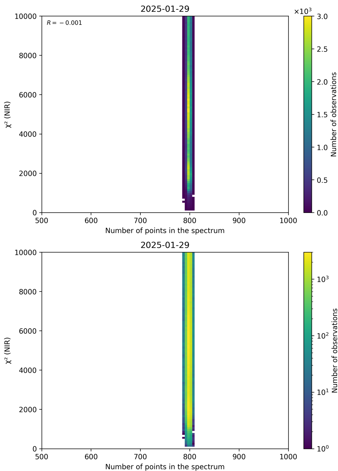
Figure 88: Scatter density plot of “Number of points in the spectrum” against “ \chi^2 (NIR)” for 2025-01-28 to 2025-01-30.
