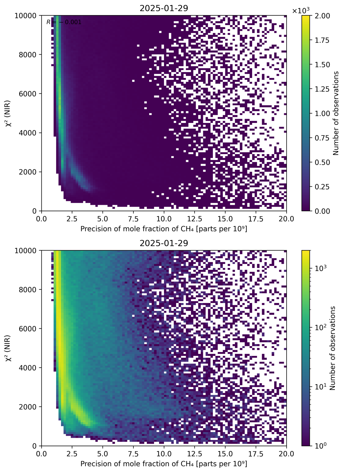
Figure 78: Scatter density plot of “Precision of mole fraction of \text{CH}_4 ” against “ \chi^2 (NIR)” for 2025-01-28 to 2025-01-30.
