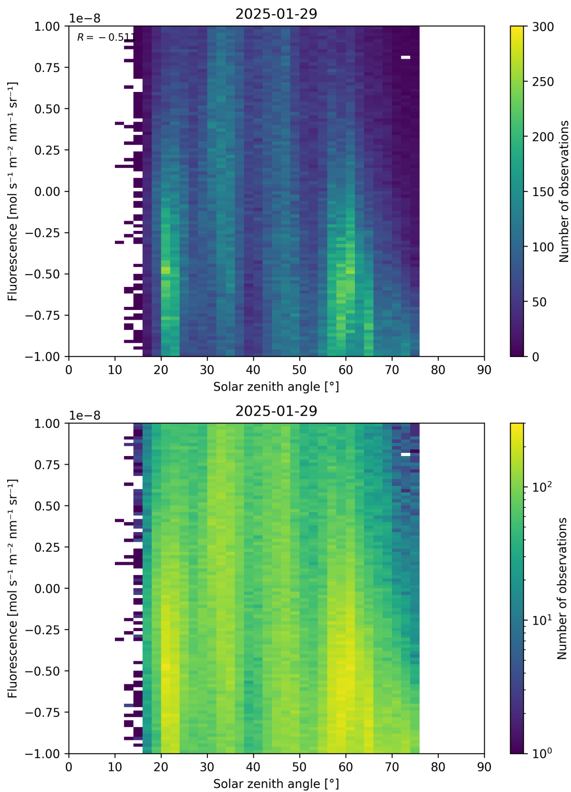
Figure 97: Scatter density plot of “Solar zenith angle” against “Fluorescence” for 2025-01-28 to 2025-01-30.
