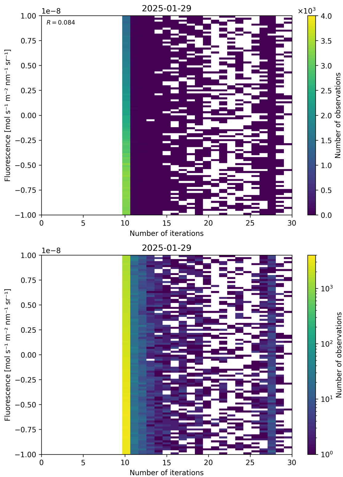
Figure 87: Scatter density plot of “Number of iterations” against “Fluorescence” for 2025-01-28 to 2025-01-30.
