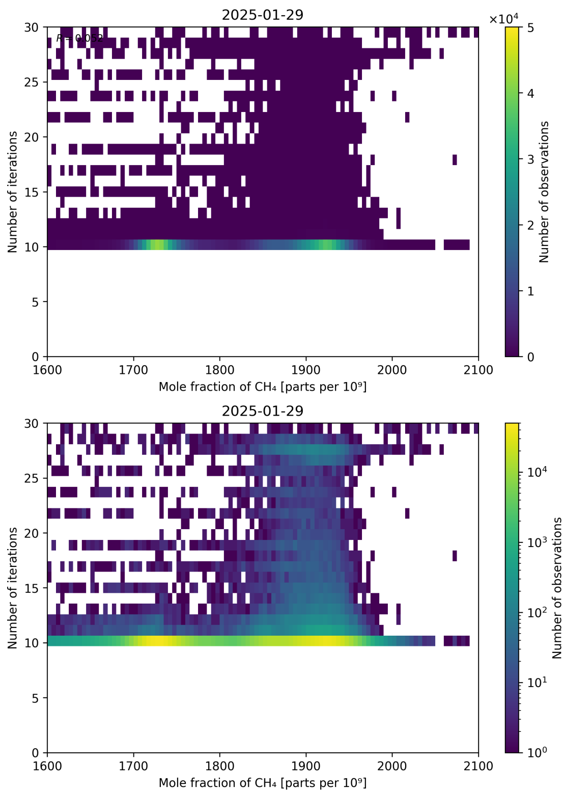
Figure 76: Scatter density plot of “Mole fraction of CH 4 ” against “Number of iterations” for 2025-01-28 to 2025-01-30.
