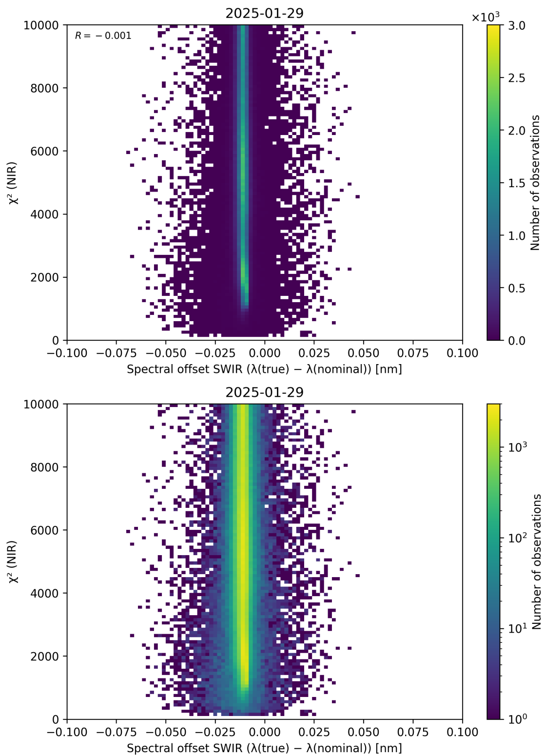
Figure 117: Scatter density plot of “Spectral offset SWIR ( \lambda_{\text{true}} - \lambda_{\text{nominal}} )” against “ \chi^2 (NIR)” for 2025-01-28 to 2025-01-30.
