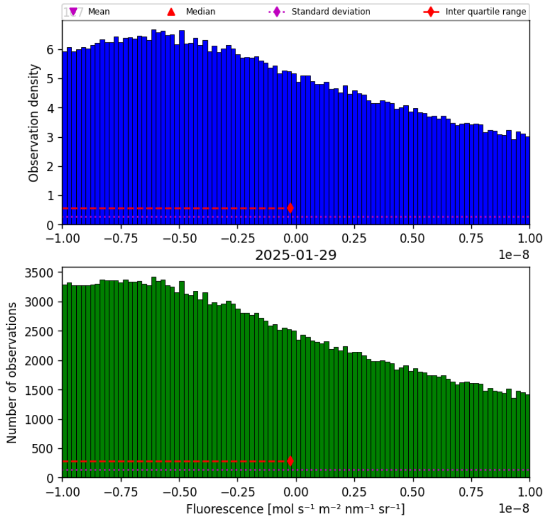
Figure 32: Histogram of “Fluorescence” for 2025-01-28 to 2025-01-30
