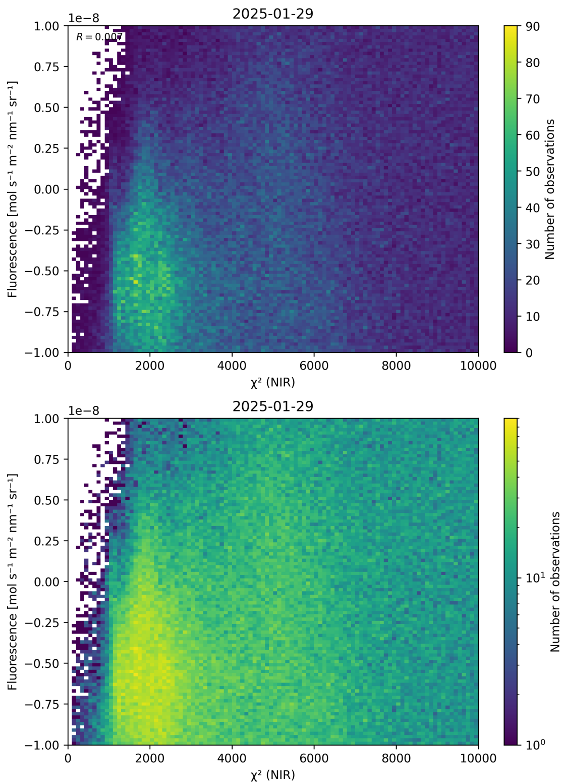
Figure 45: Scatter density plot of “ \chi^2 (NIR)” against “Fluorescence” for 2025-01-28 to 2025-01-30.
