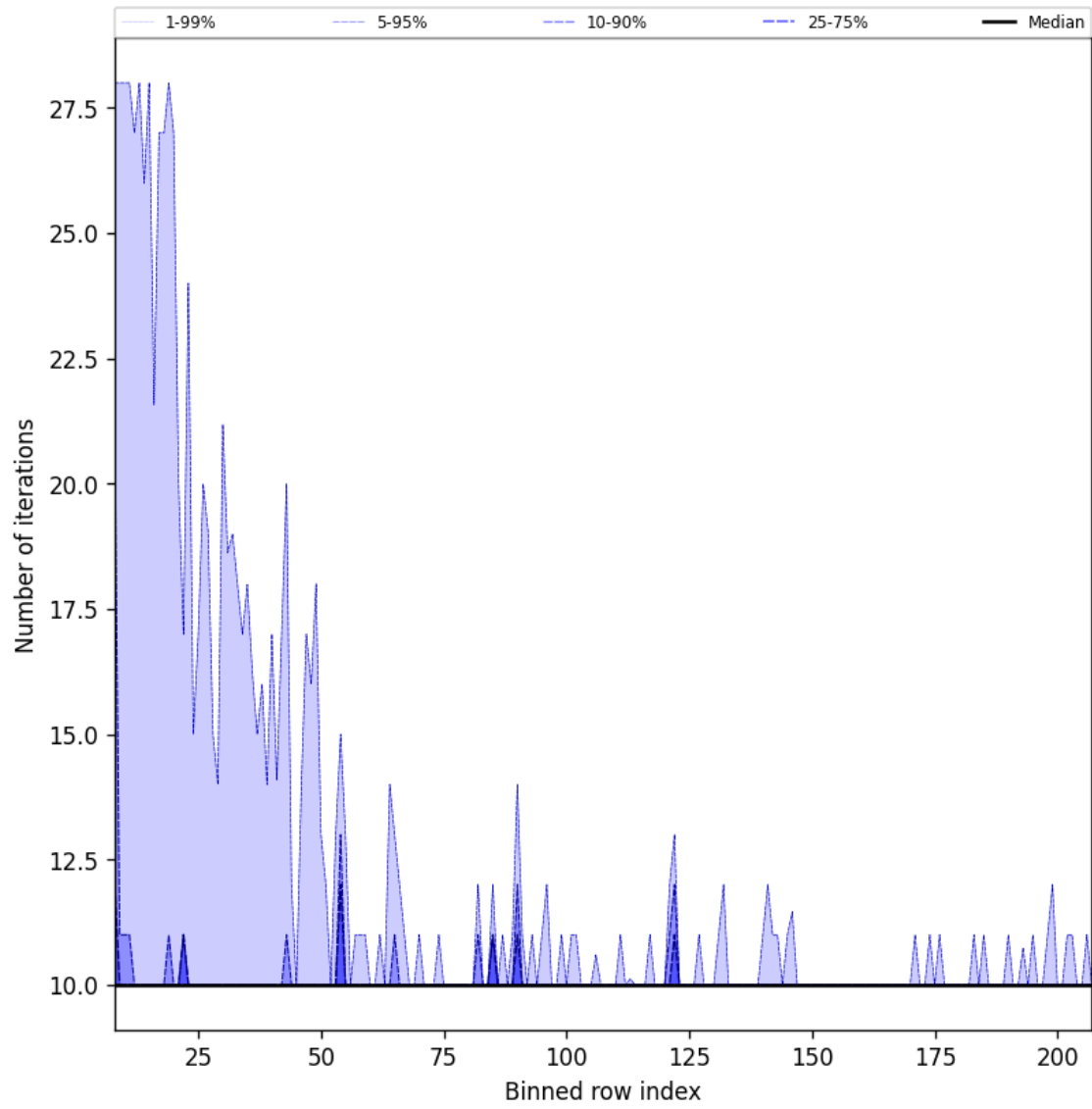
Figure 42: Along track statistics of “Number of iterations” for 2025-01-28 to 2025-01-30
