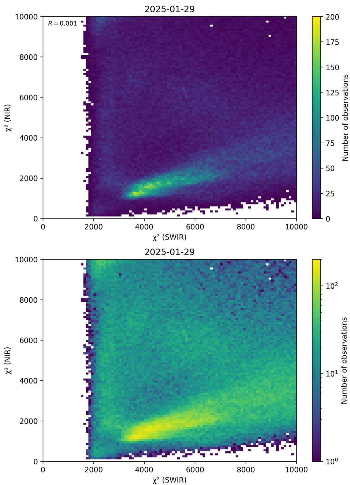
Figure 47: Scatter density plot of “ \chi^2 (SWIR)” against “ \chi^2 (NIR)” for 2025-01-28 to 2025-01-30.
