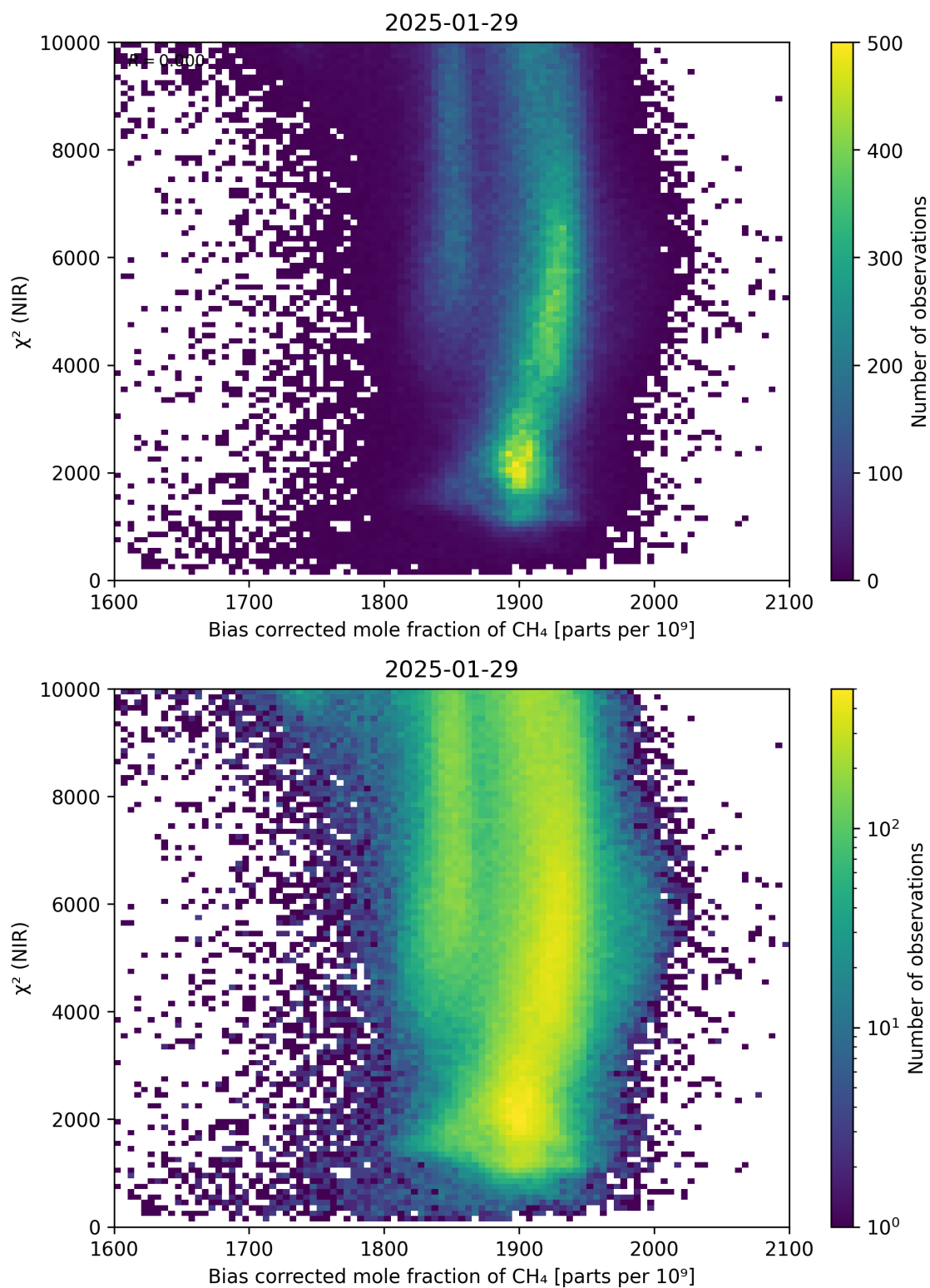
Figure 63: Scatter density plot of “Bias corrected mole fraction of \text{CH}_4 ” against “ \chi^2 (NIR)” for 2025-01-28 to 2025-01-30.
