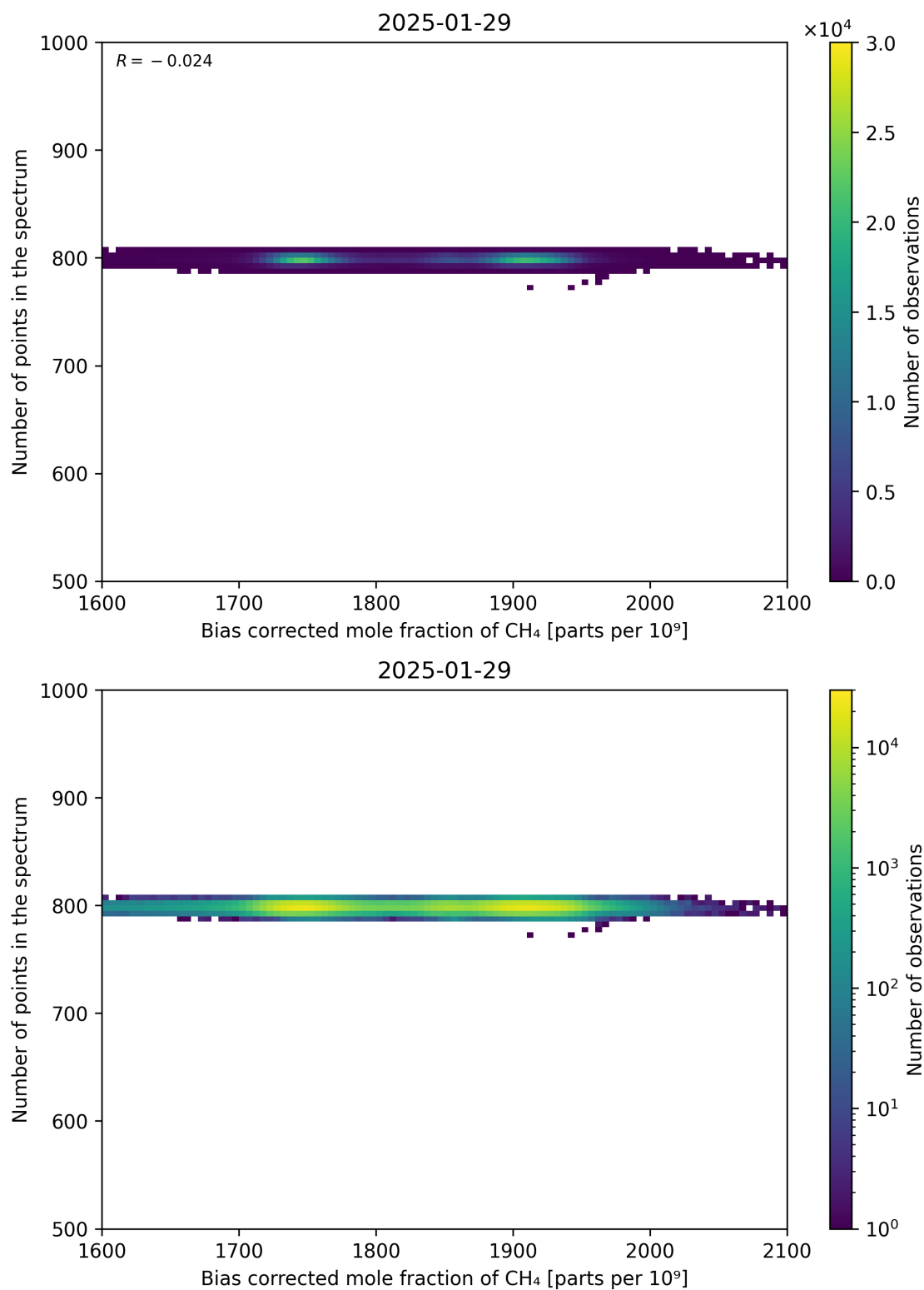
Figure 68: Scatter density plot of “Bias corrected mole fraction of CH 4 ” against “Number of points in the spectrum” for 2025-01-28 to 2025-01-30.
