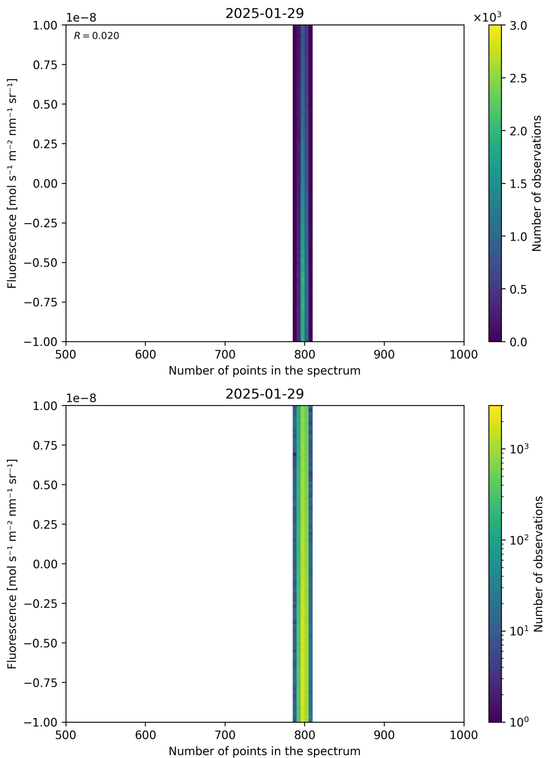
Figure 91: Scatter density plot of “Number of points in the spectrum” against “Fluorescence” for 2025-01-28 to 2025-01-30.
