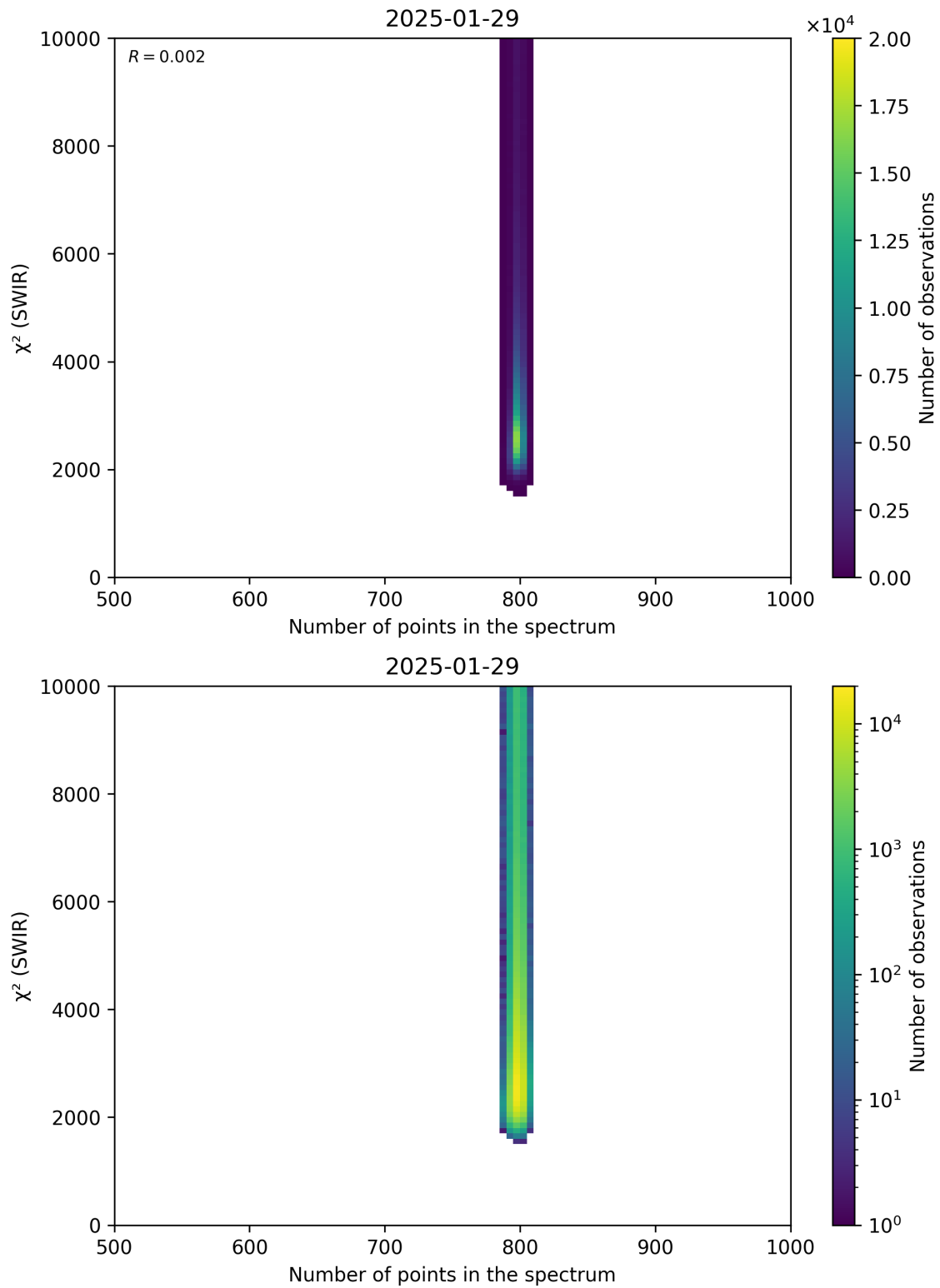
Figure 89: Scatter density plot of “Number of points in the spectrum” against “ \chi^2 (SWIR)” for 2025-01-28 to 2025-01-30.
