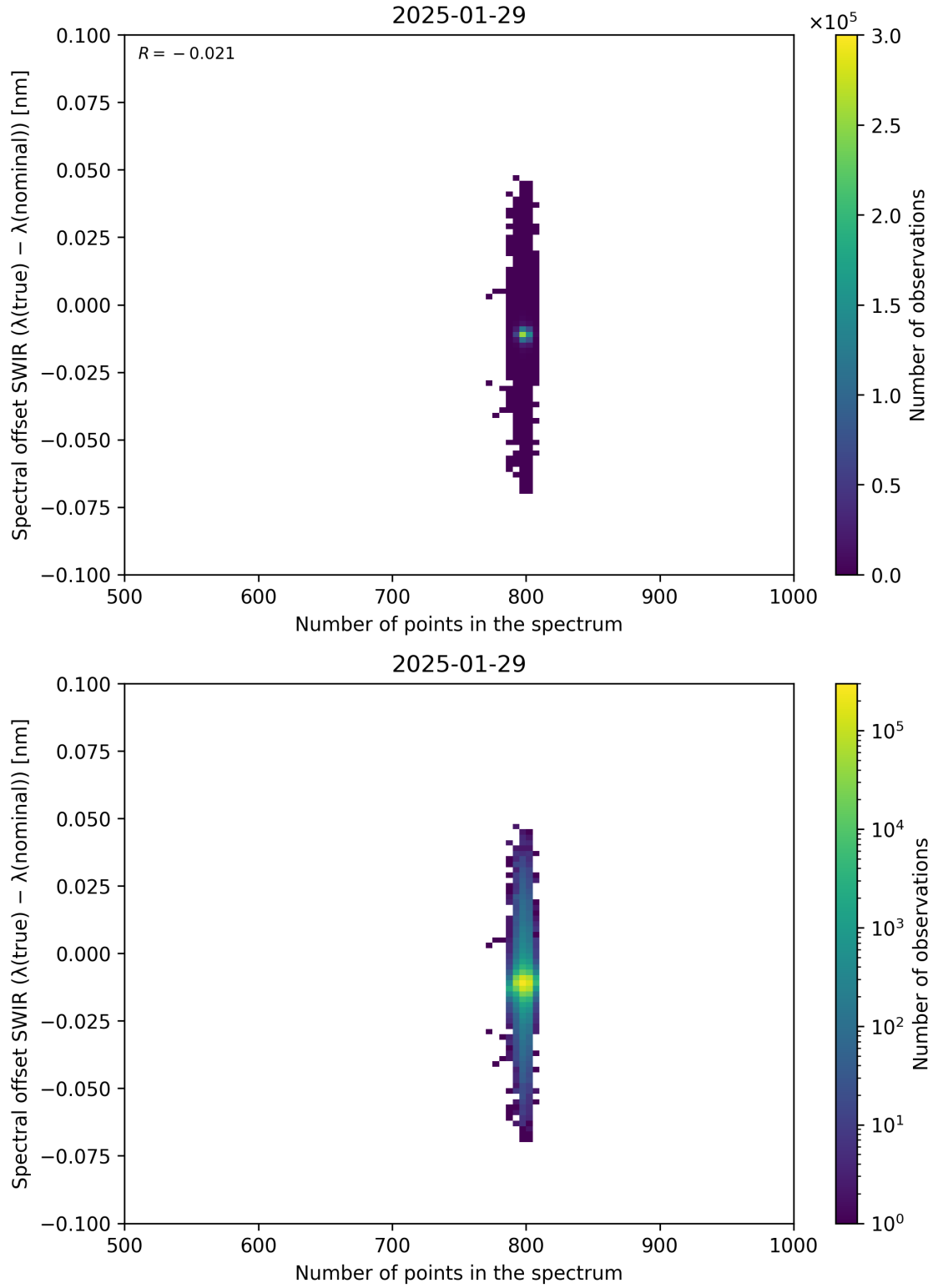
Figure 93: Scatter density plot of “Number of points in the spectrum” against “Spectral offset SWIR ( \lambda_{\text{true}} - \lambda_{\text{nominal}} )” for 2025-01-28 to 2025-01-30.
