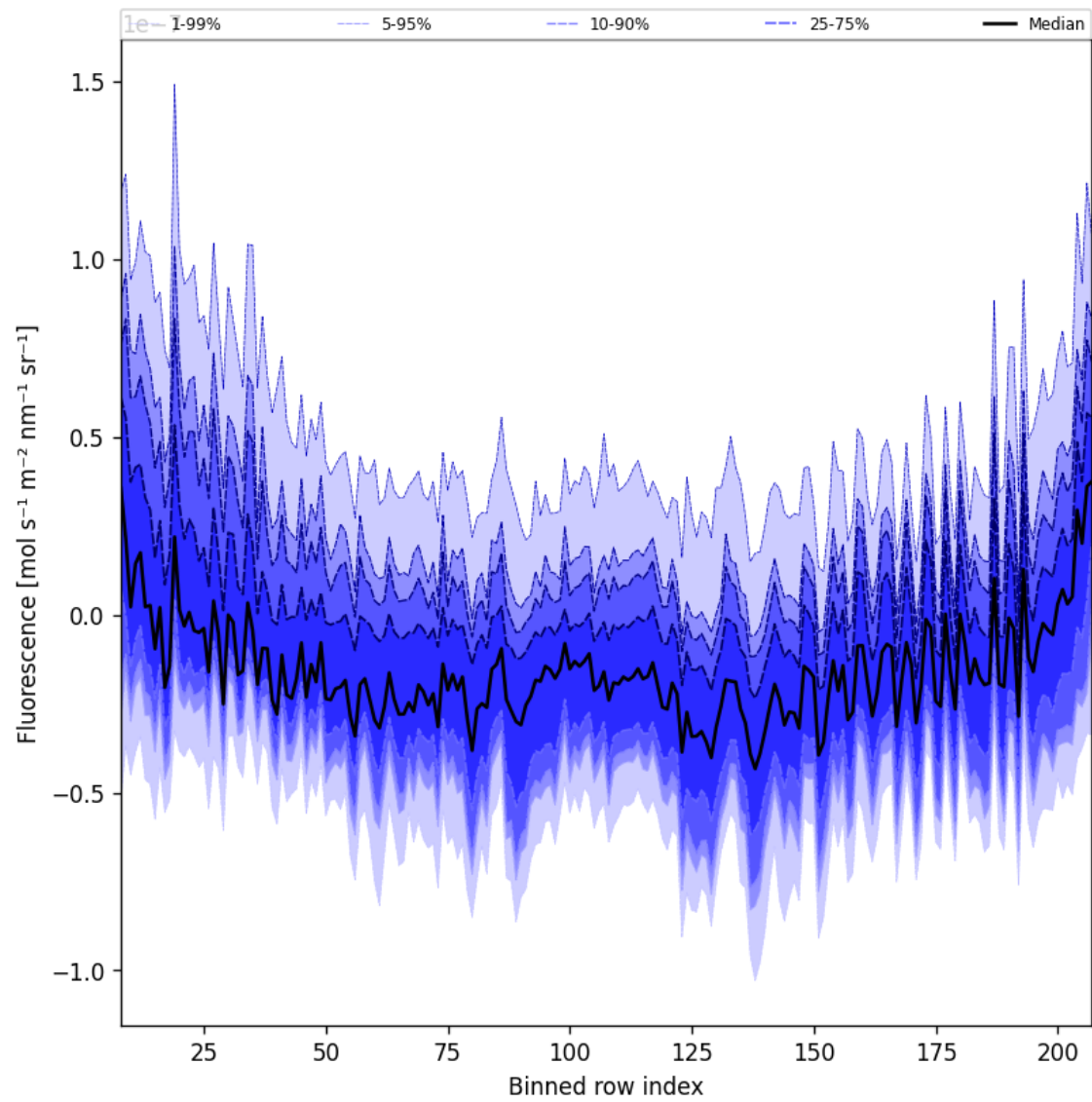
Figure 43: Along track statistics of “Fluorescence” for 2025-01-28 to 2025-01-30
