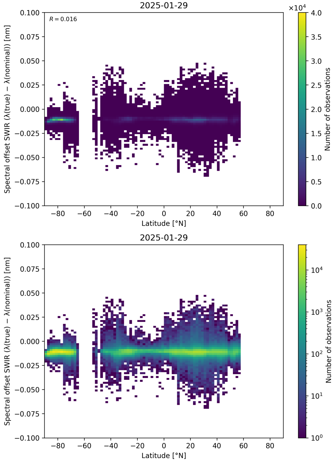
Figure 62: Scatter density plot of “Latitude” against “Spectral offset SWIR ( \lambda_{\text{true}} - \lambda_{\text{nominal}} )” for 2025-01-28 to 2025-01-30.
