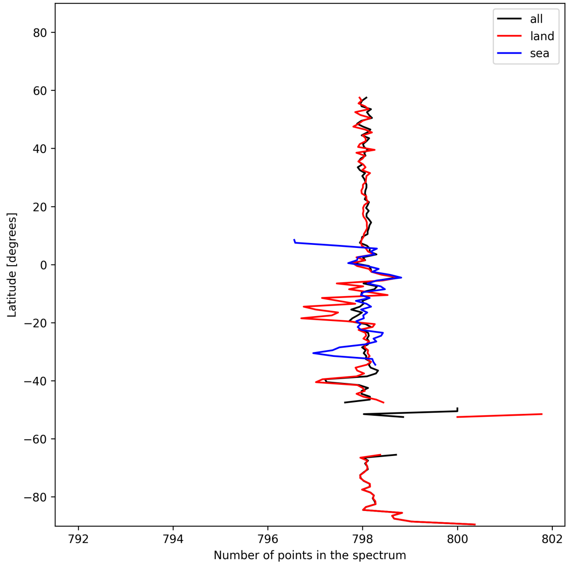
Figure 15: Zonal average of “Number of points in the spectrum” for 2025-01-28 to 2025-01-30.
