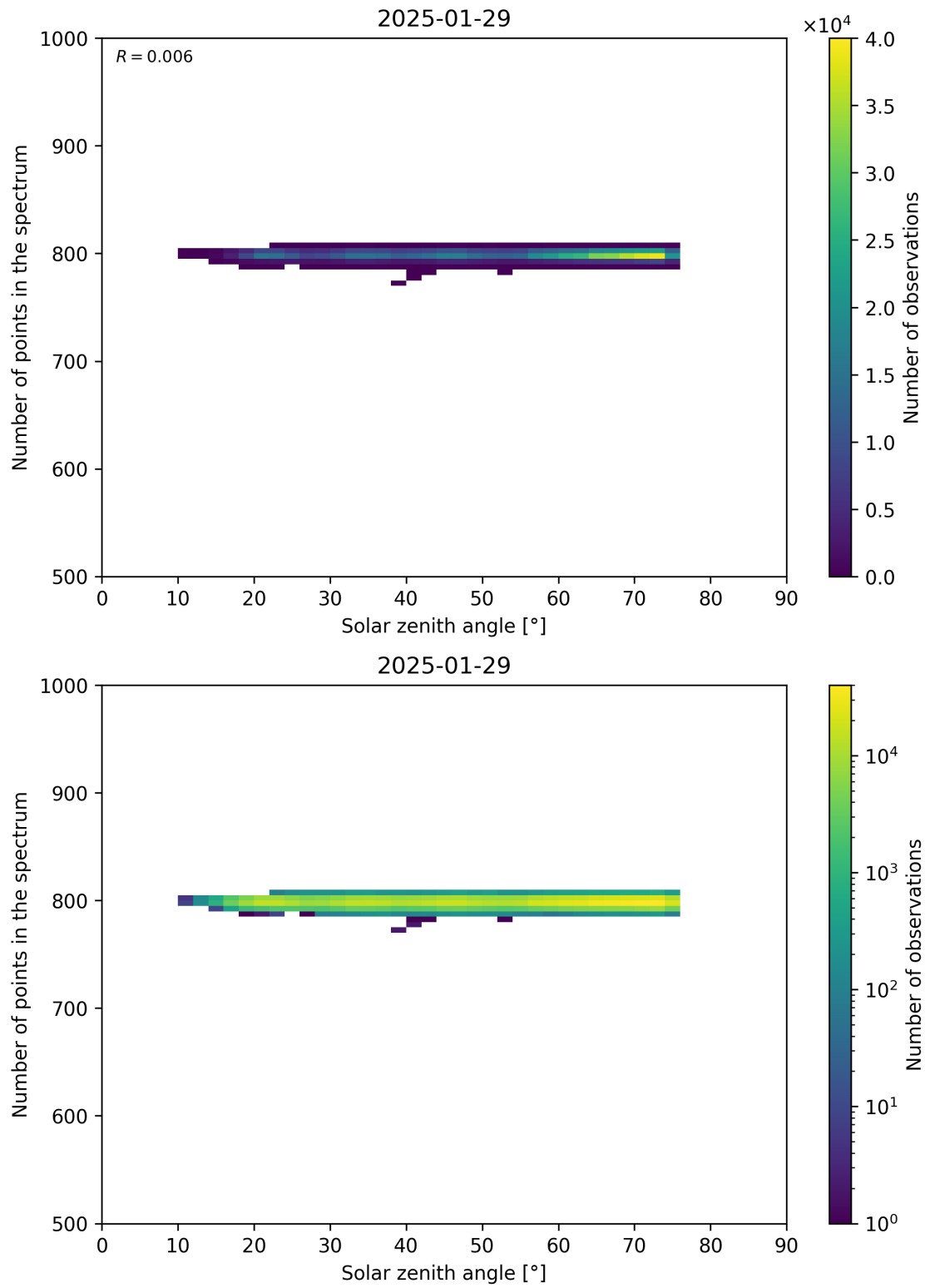
Figure 103: Scatter density plot of “Solar zenith angle” against “Number of points in the spectrum” for 2025-01-28 to 2025-01-30.
