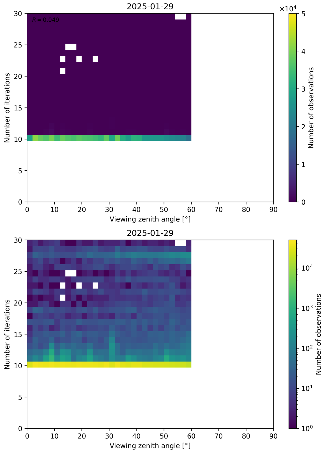
Figure 113: Scatter density plot of “Viewing zenith angle” against “Number of iterations” for 2025-01-28 to 2025-01-30.
