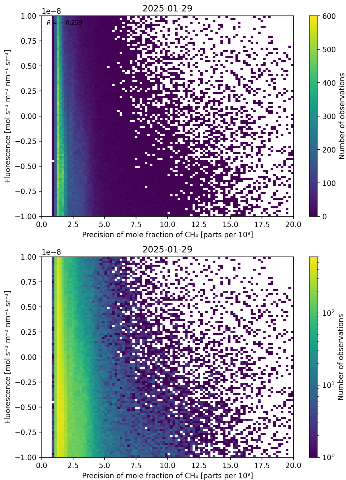
Figure 81: Scatter density plot of “Precision of mole fraction of CH 4 ” against “Fluorescence” for 2025-01-28 to 2025-01-30.
