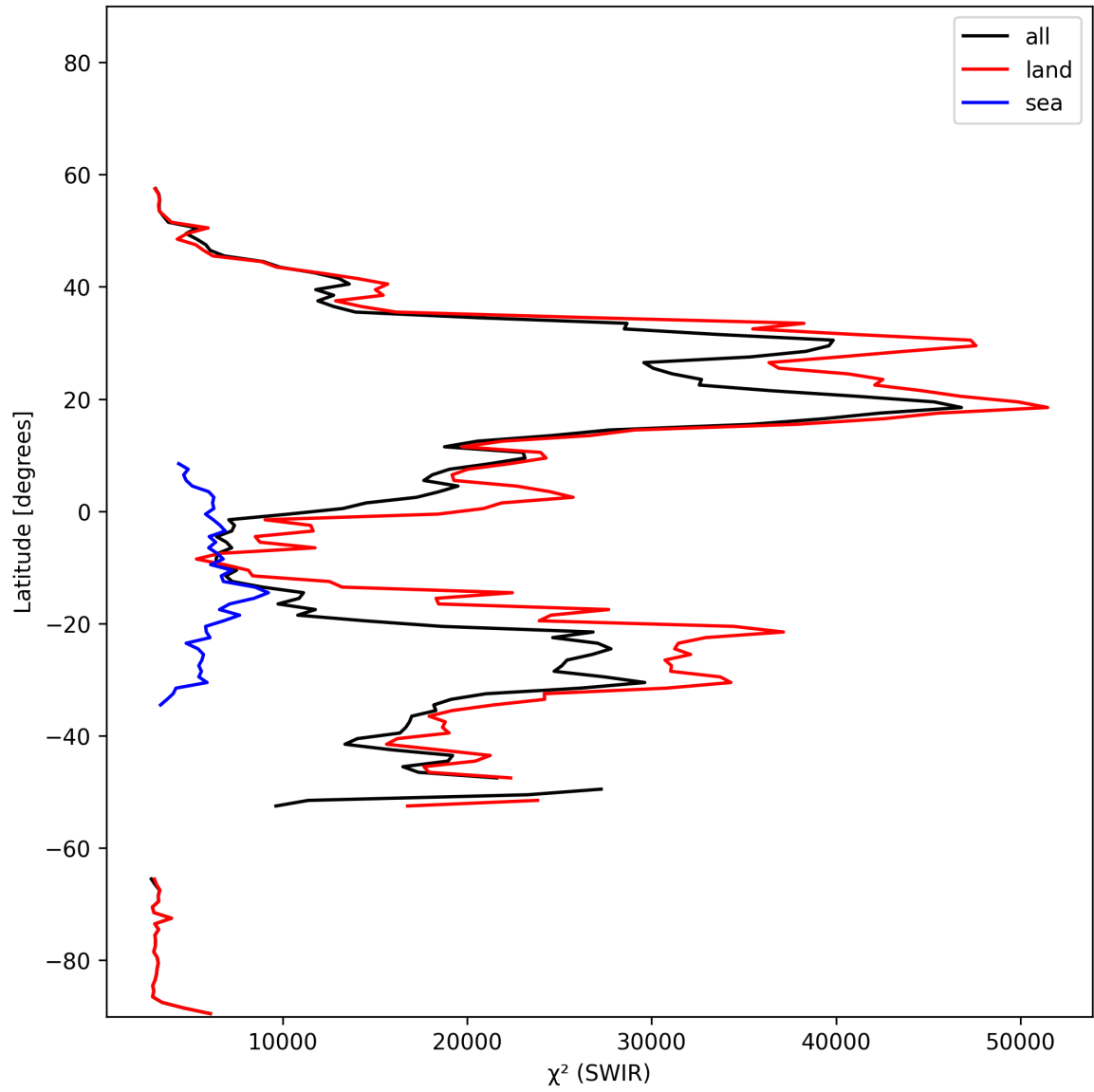
Figure 17: Zonal average of “ \chi^2 (SWIR)” for 2025-01-28 to 2025-01-30.
