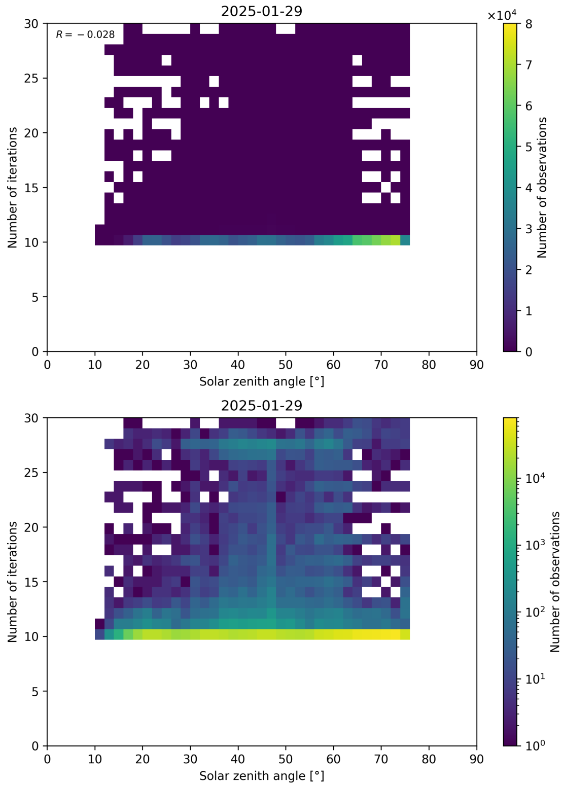
Figure 102: Scatter density plot of “Solar zenith angle” against “Number of iterations” for 2025-01-28 to 2025-01-30.
