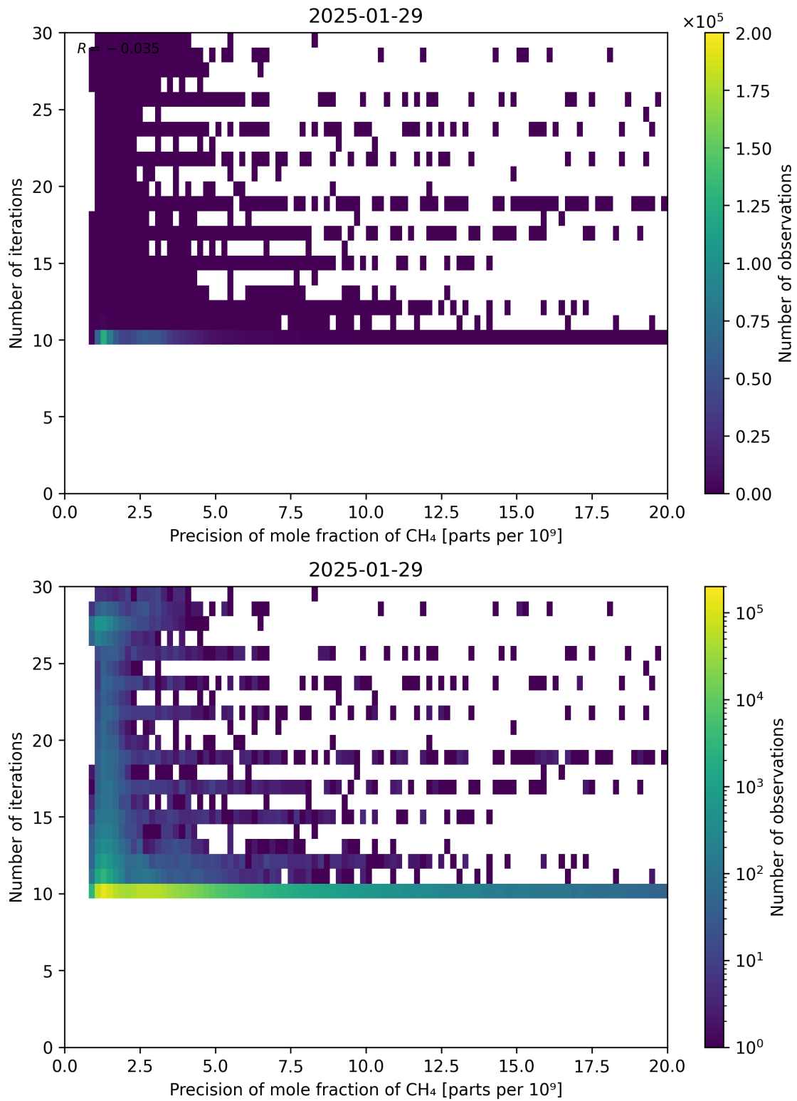
Figure 83: Scatter density plot of “Precision of mole fraction of CH 4 ” against “Number of iterations” for 2025-01-28 to 2025-01-30.
