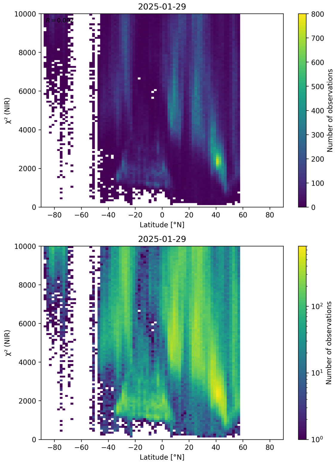
Figure 53: Scatter density plot of “Latitude” against “ \chi^2 (NIR)” for 2025-01-28 to 2025-01-30.
