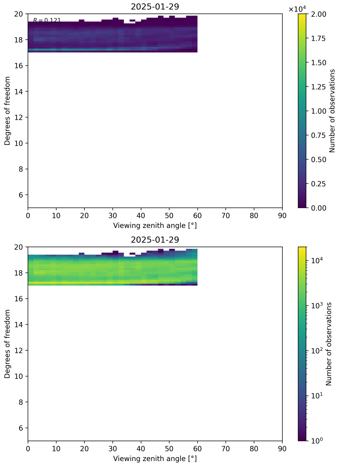
Figure 107: Scatter density plot of “Viewing zenith angle” against “Degrees of freedom” for 2025-01-28 to 2025-01-30.
