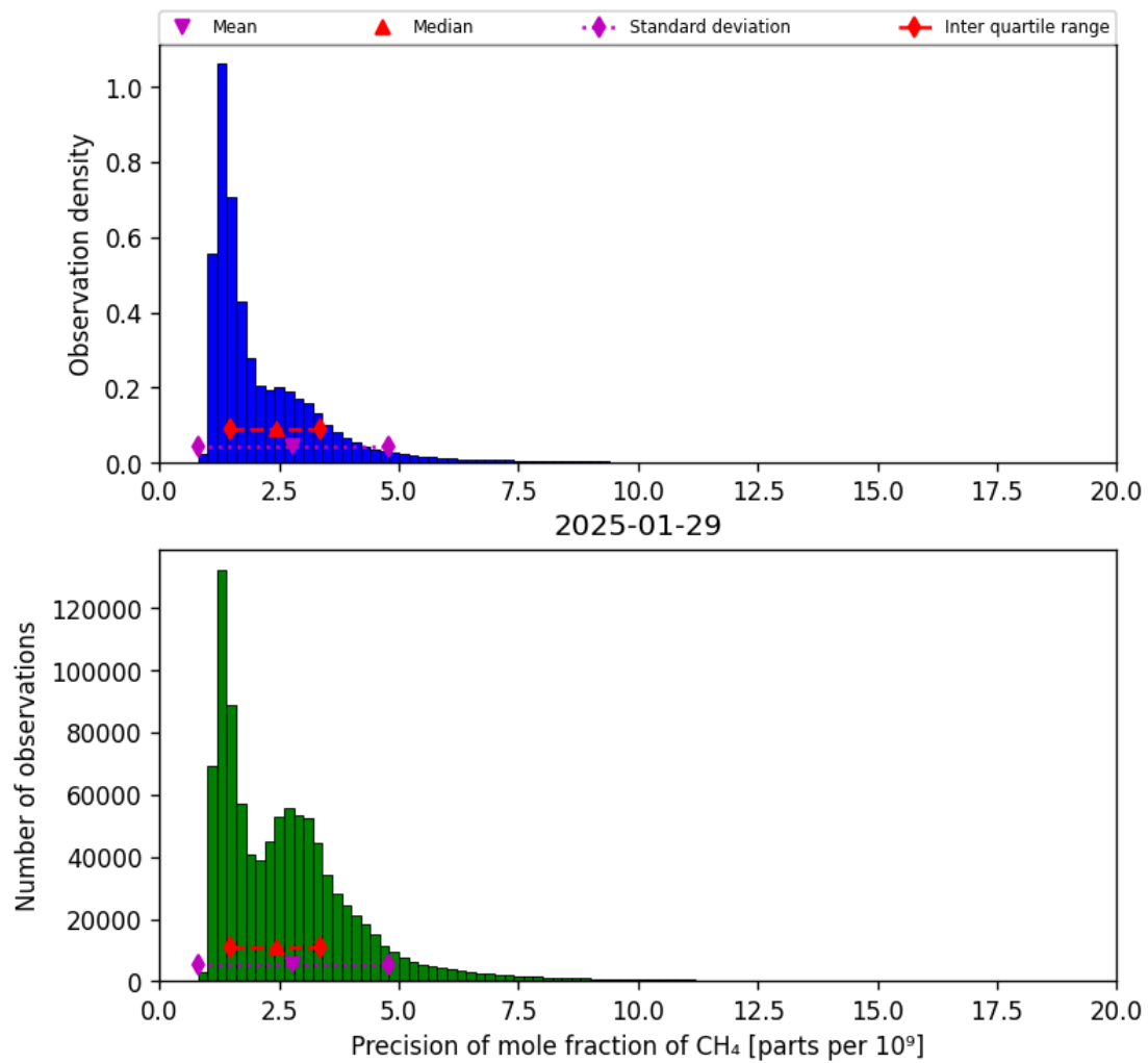
Figure 24: Histogram of “Precision of mole fraction of CH 4 ” for 2025-01-28 to 2025-01-30
