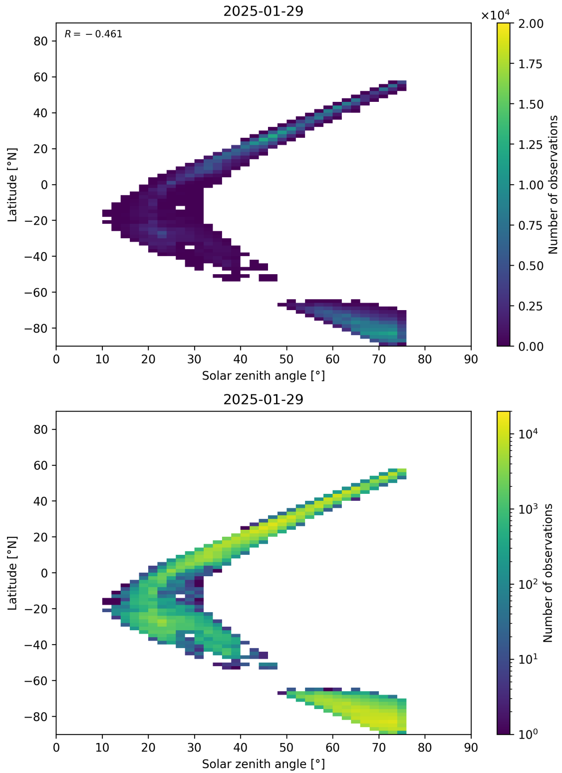
Figure 98: Scatter density plot of “Solar zenith angle” against “Latitude” for 2025-01-28 to 2025-01-30.
