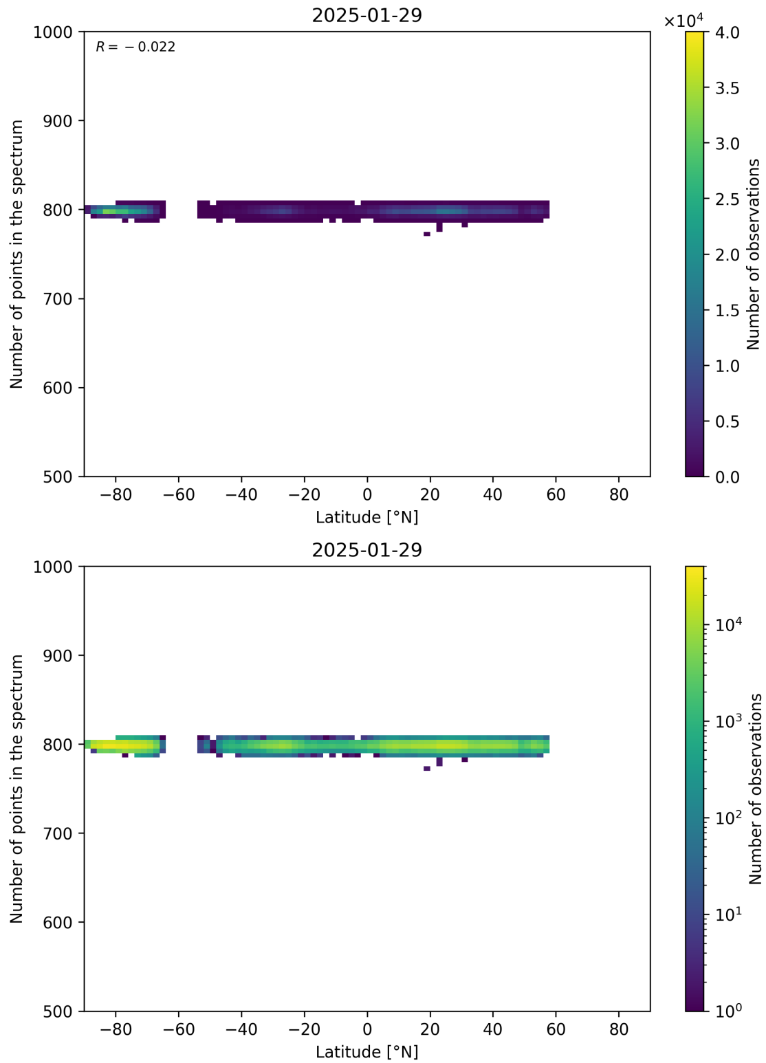
Figure 61: Scatter density plot of “Latitude” against “Number of points in the spectrum” for 2025-01-28 to 2025-01-30.
