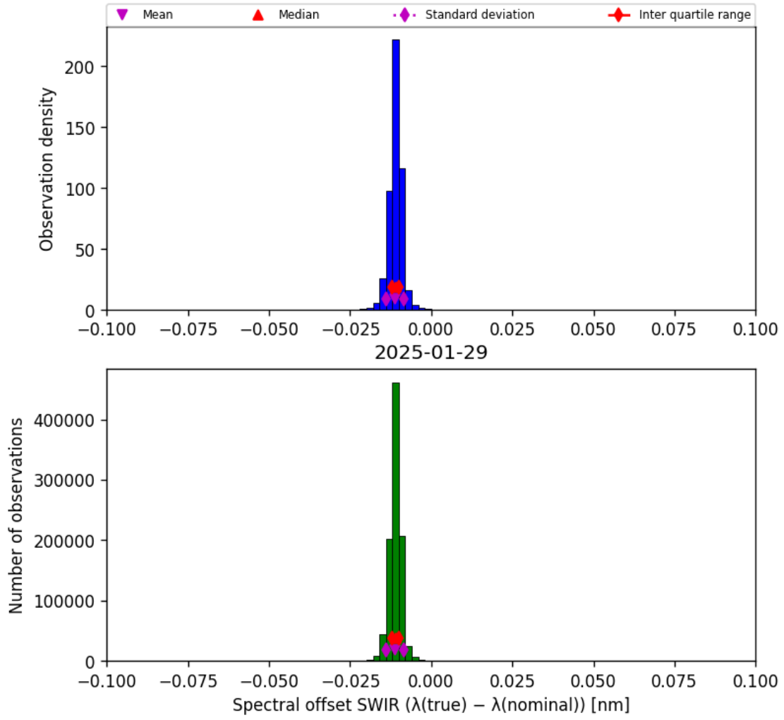
Figure 27: Histogram of “Spectral offset SWIR ( \lambda_{\text{true}} - \lambda_{\text{nominal}} )” for 2025-01-28 to 2025-01-30
