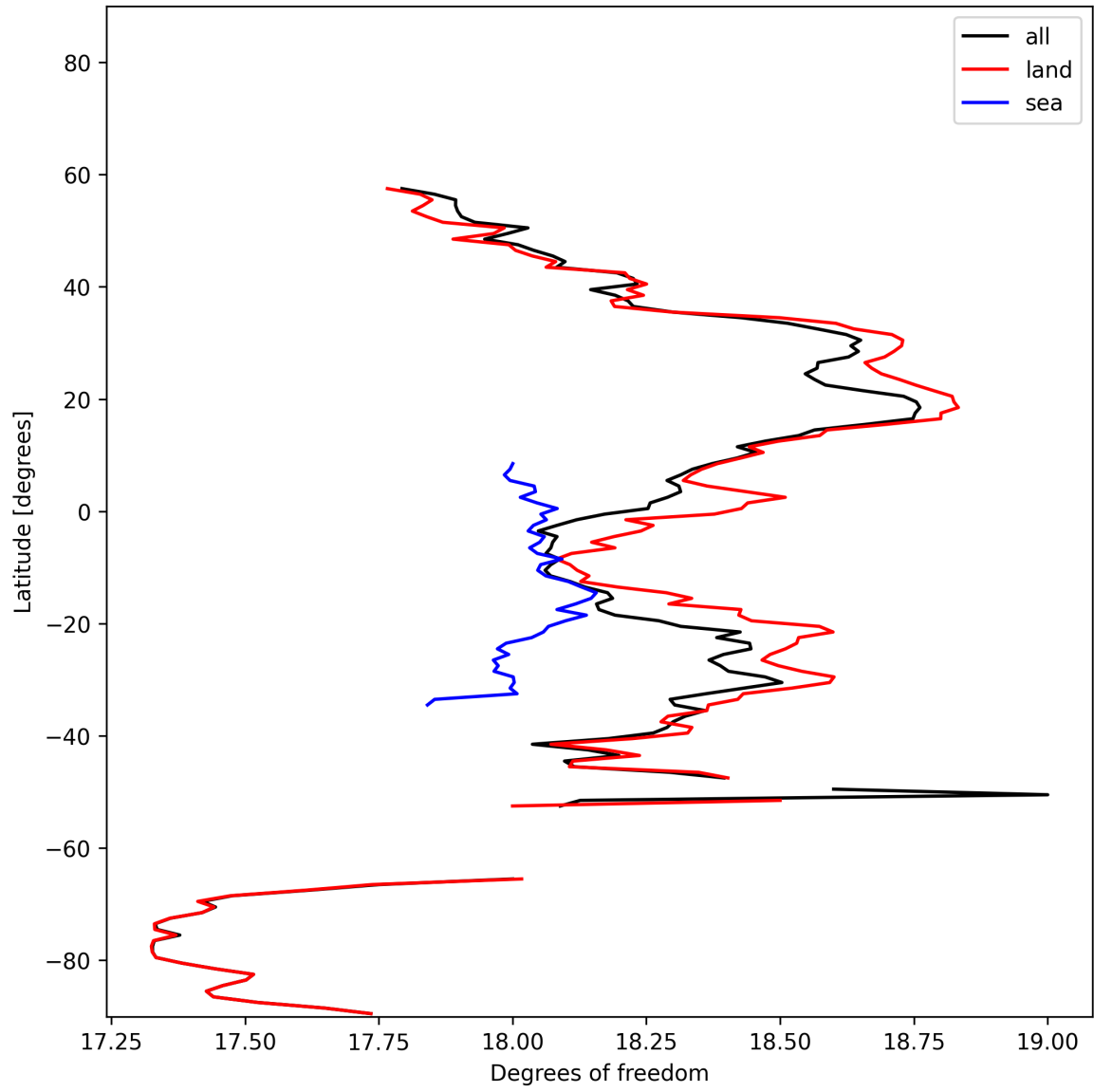
Figure 19: Zonal average of “Degrees of freedom” for 2025-01-28 to 2025-01-30.
