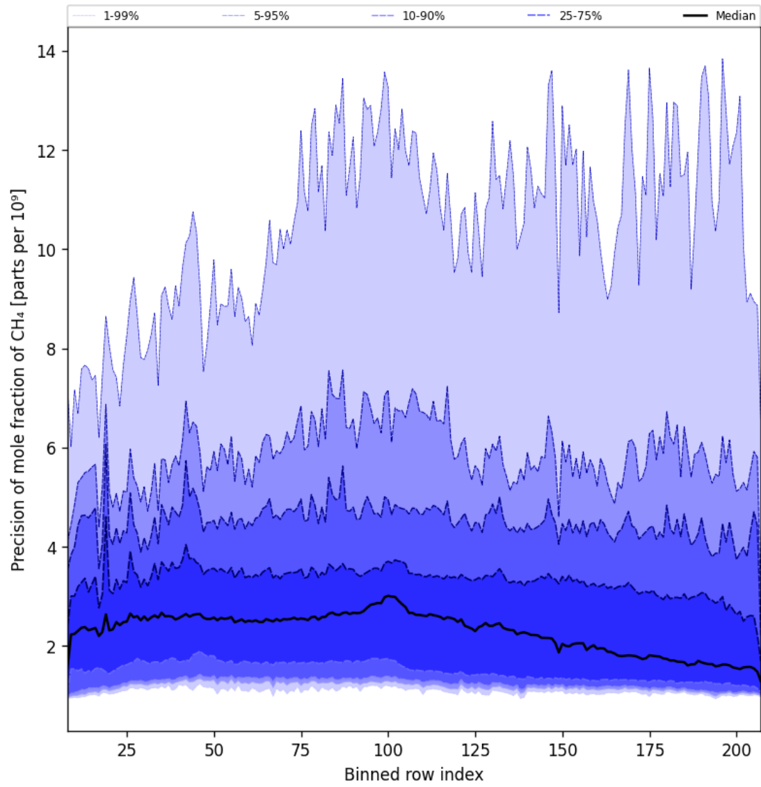
Figure 35: Along track statistics of “Precision of mole fraction of CH 4 ” for 2025-01-28 to 2025-01-30
