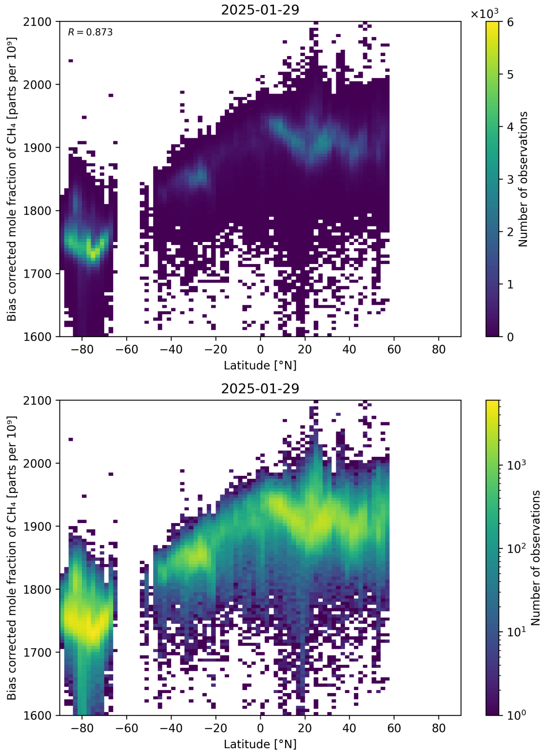
Figure 58: Scatter density plot of “Latitude” against “Bias corrected mole fraction of \text{CH}_4 ” for 2025-01-28 to 2025-01-30.
