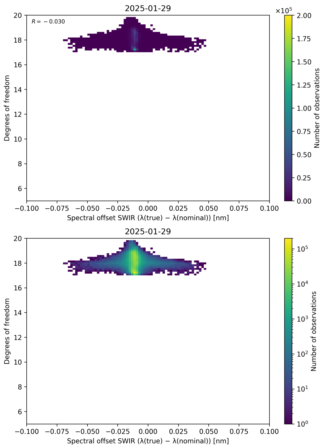
Figure 119: Scatter density plot of “Spectral offset SWIR ( \lambda_{\text{true}} - \lambda_{\text{nominal}} )” against “Degrees of freedom” for 2025-01-28 to 2025-01-30.
