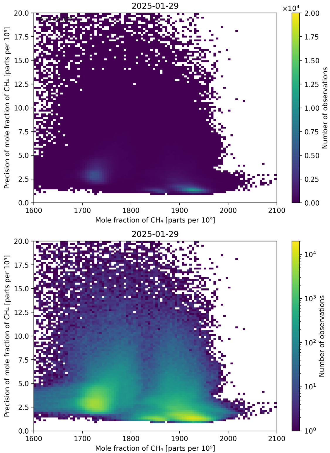
Figure 75: Scatter density plot of “Mole fraction of CH 4 ” against “Precision of mole fraction of CH 4 ” for 2025-01-28 to 2025-01-30.
