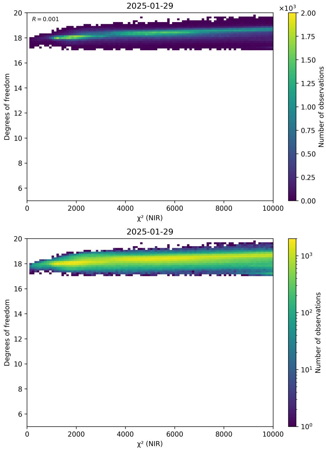
Figure 44: Scatter density plot of “ \chi^2 (NIR)” against “Degrees of freedom” for 2025-01-28 to 2025-01-30.
