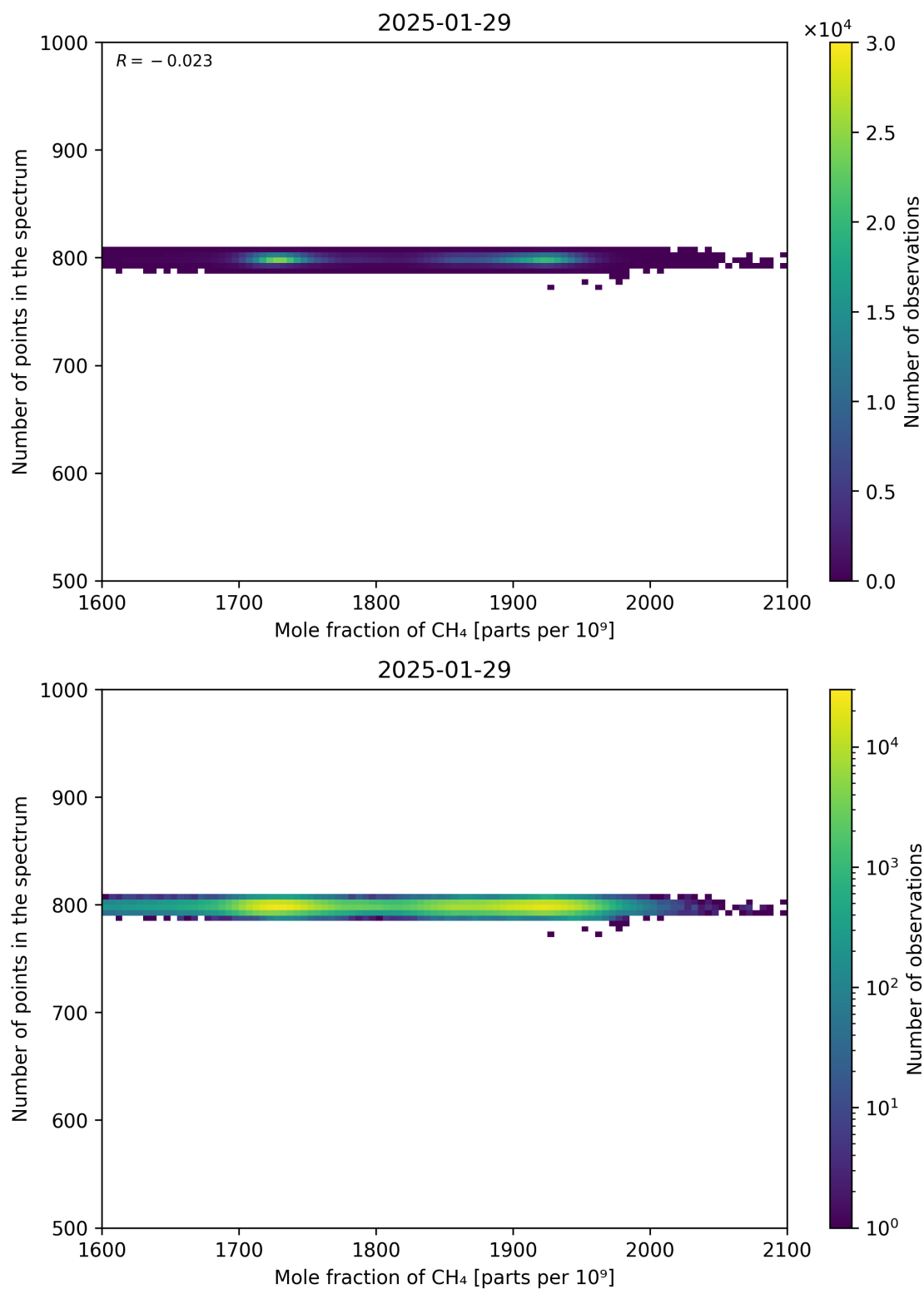
Figure 77: Scatter density plot of “Mole fraction of CH 4 ” against “Number of points in the spectrum” for 2025-01-28 to 2025-01-30.
