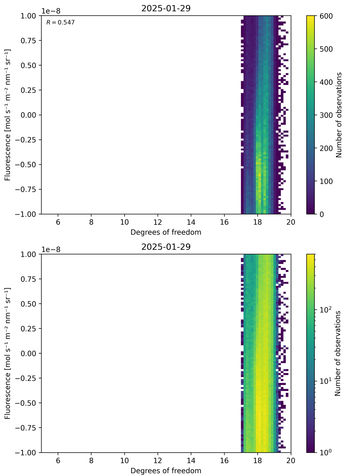
Figure 51: Scatter density plot of “Degrees of freedom” against “Fluorescence” for 2025-01-28 to 2025-01-30.
