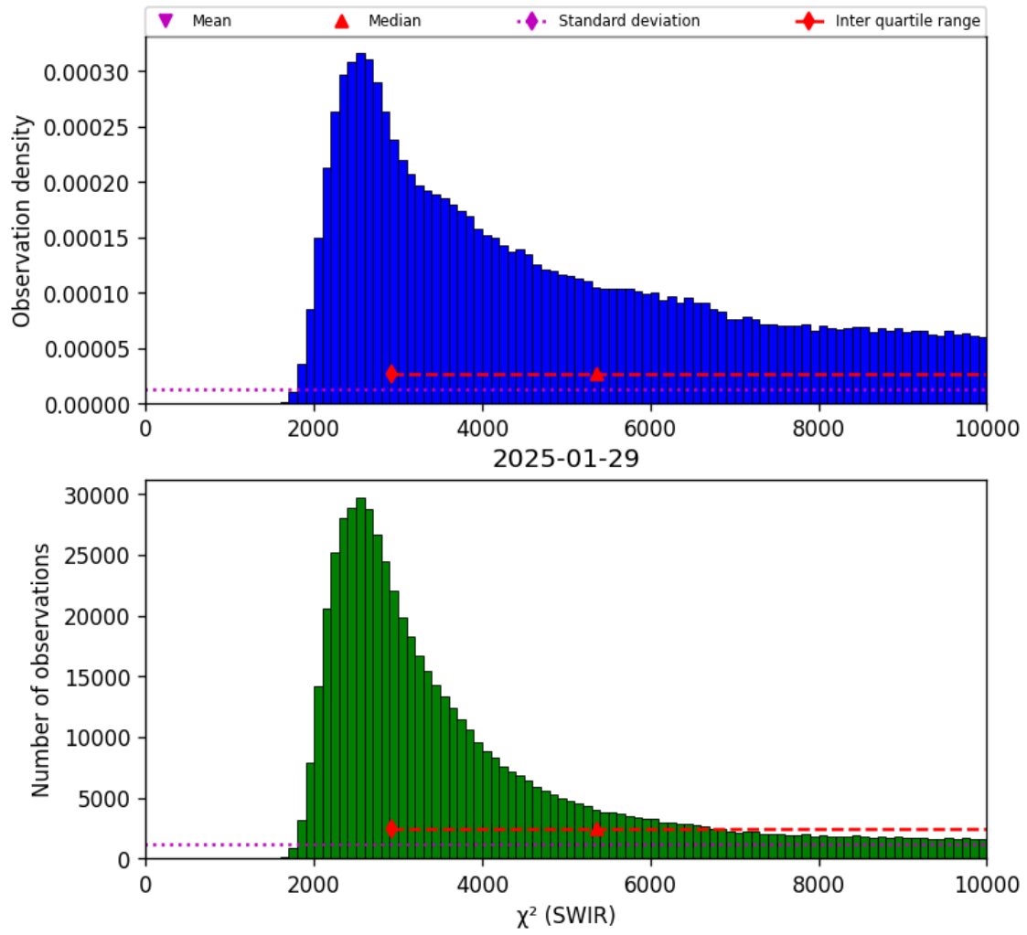
Figure 28: Histogram of “ \chi^2 (SWIR)” for 2025-01-28 to 2025-01-30
