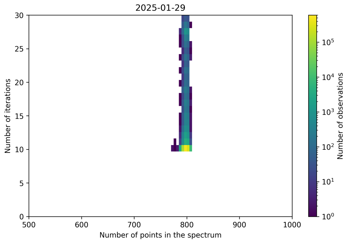
Figure 92: Scatter density plot of “Number of points in the spectrum” against “Number of iterations” for 2025-01-28 to 2025-01-30.
