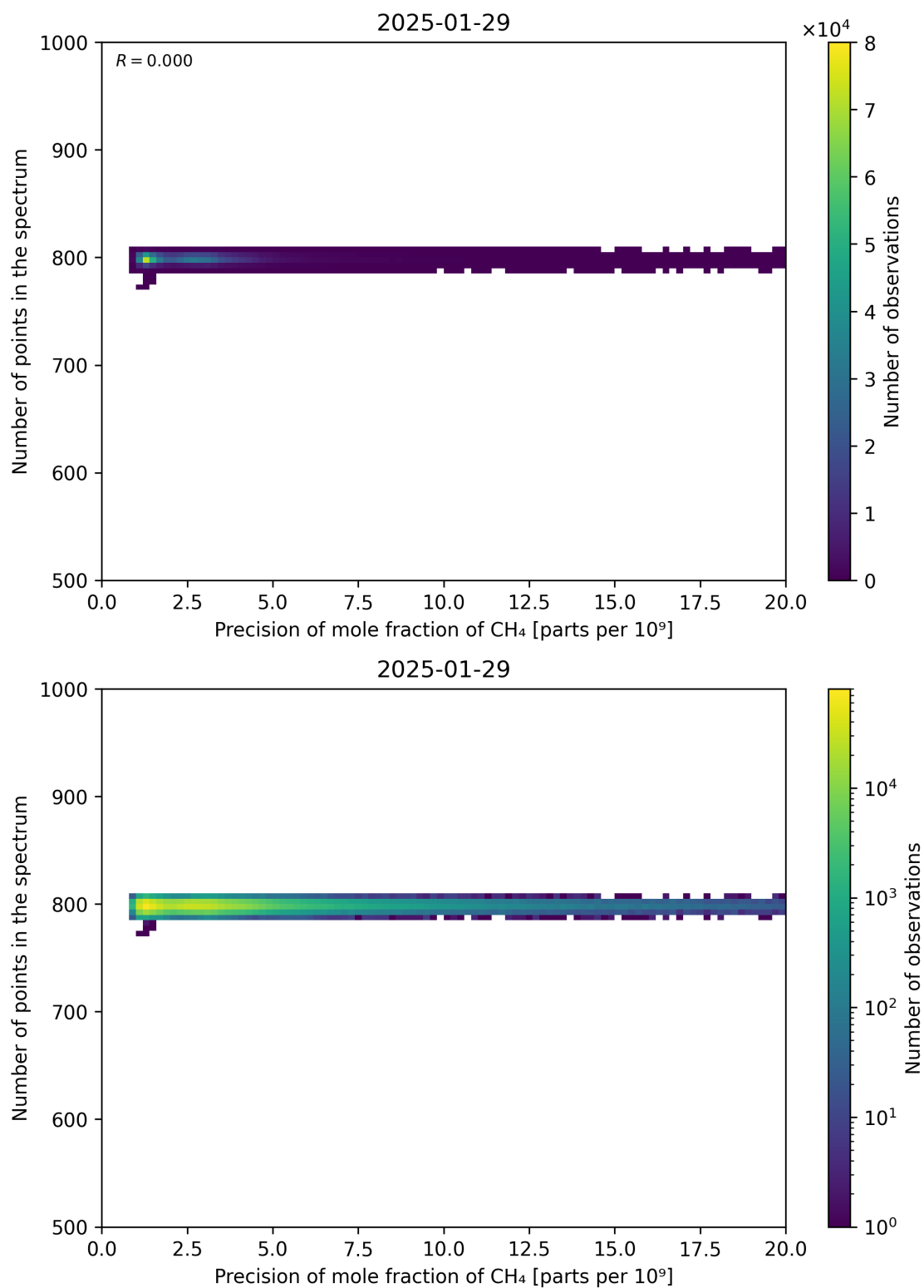
Figure 84: Scatter density plot of “Precision of mole fraction of CH 4 ” against “Number of points in the spectrum” for 2025-01-28 to 2025-01-30.
