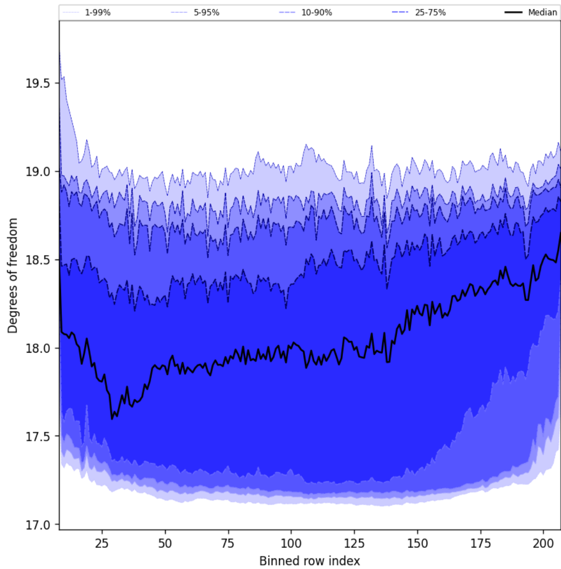
Figure 41: Along track statistics of “Degrees of freedom” for 2025-01-28 to 2025-01-30
