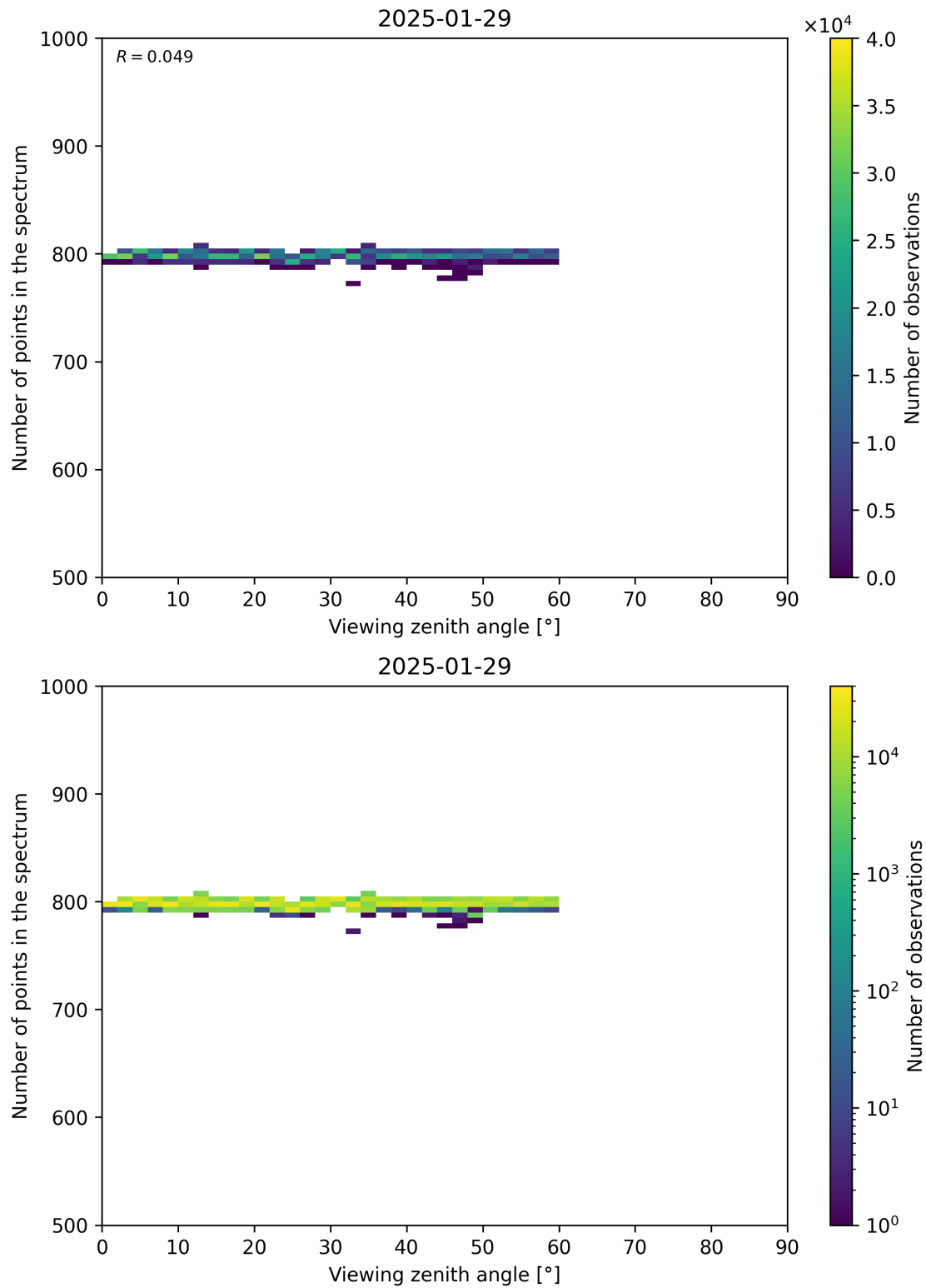
Figure 114: Scatter density plot of “Viewing zenith angle” against “Number of points in the spectrum” for 2025-01-28 to 2025-01-30.
