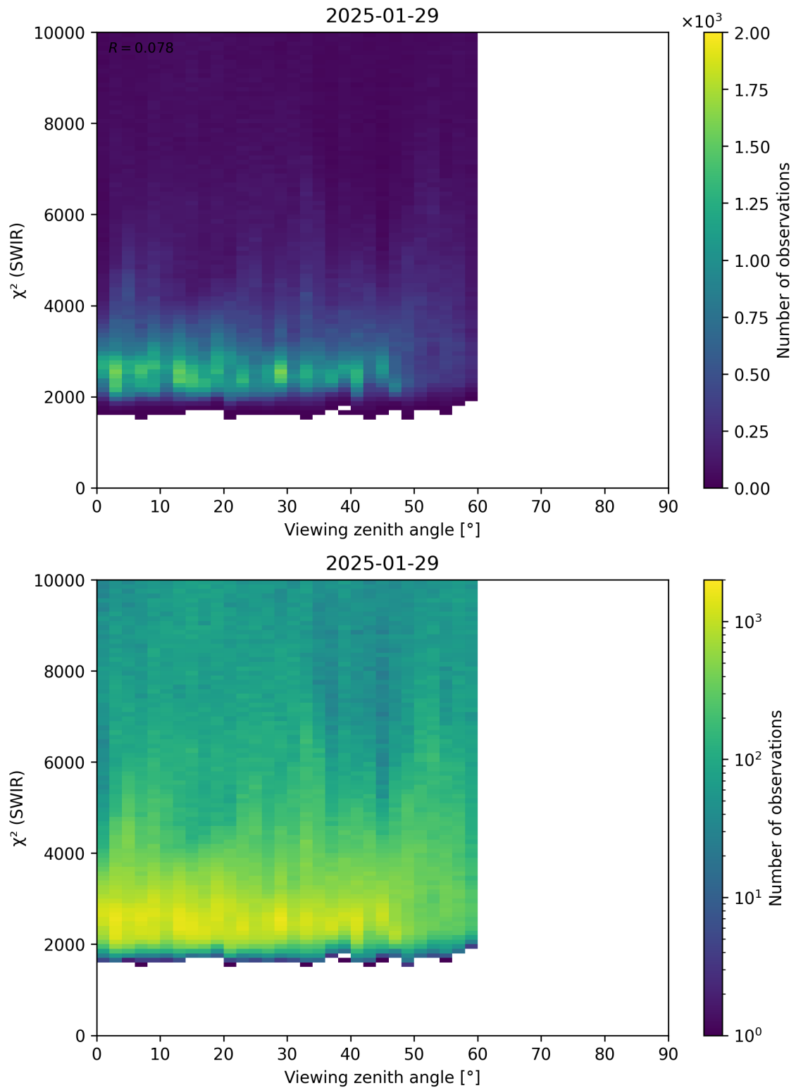
Figure 106: Scatter density plot of “Viewing zenith angle” against “ \chi^2 (SWIR)” for 2025-01-28 to 2025-01-30.
