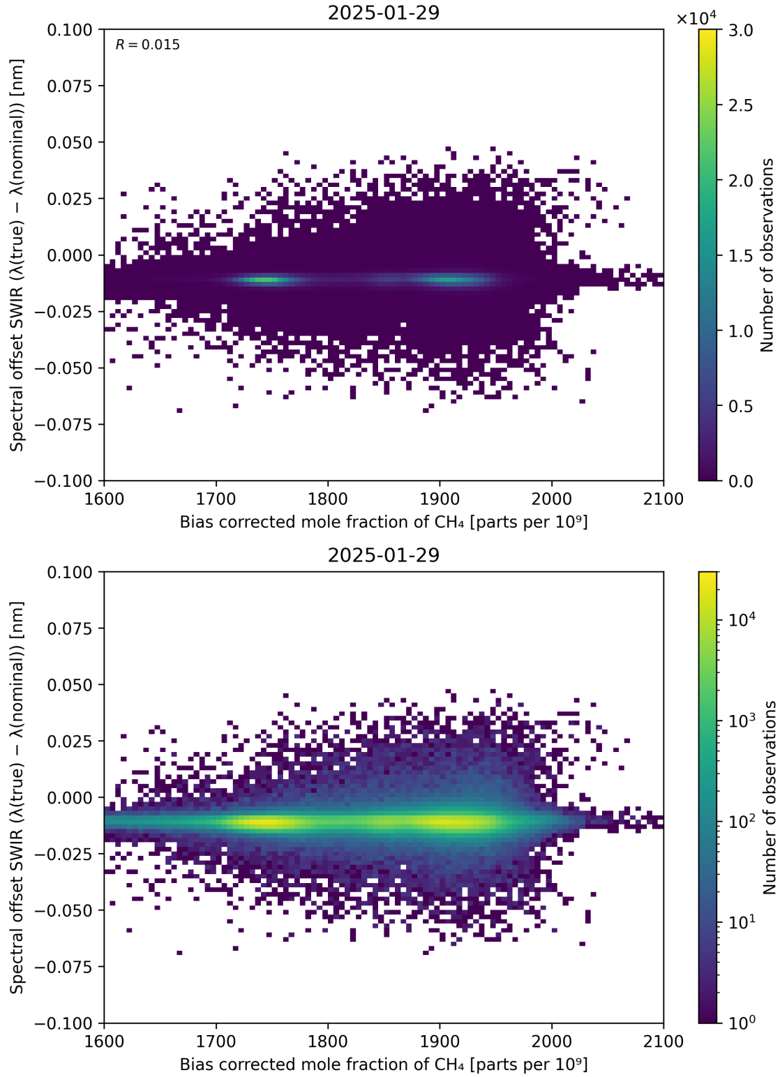
Figure 69: Scatter density plot of “Bias corrected mole fraction of \text{CH}_4 ” against “Spectral offset SWIR ( \lambda_{\text{true}} - \lambda_{\text{nominal}} )” for 2025-01-28 to 2025-01-30.
