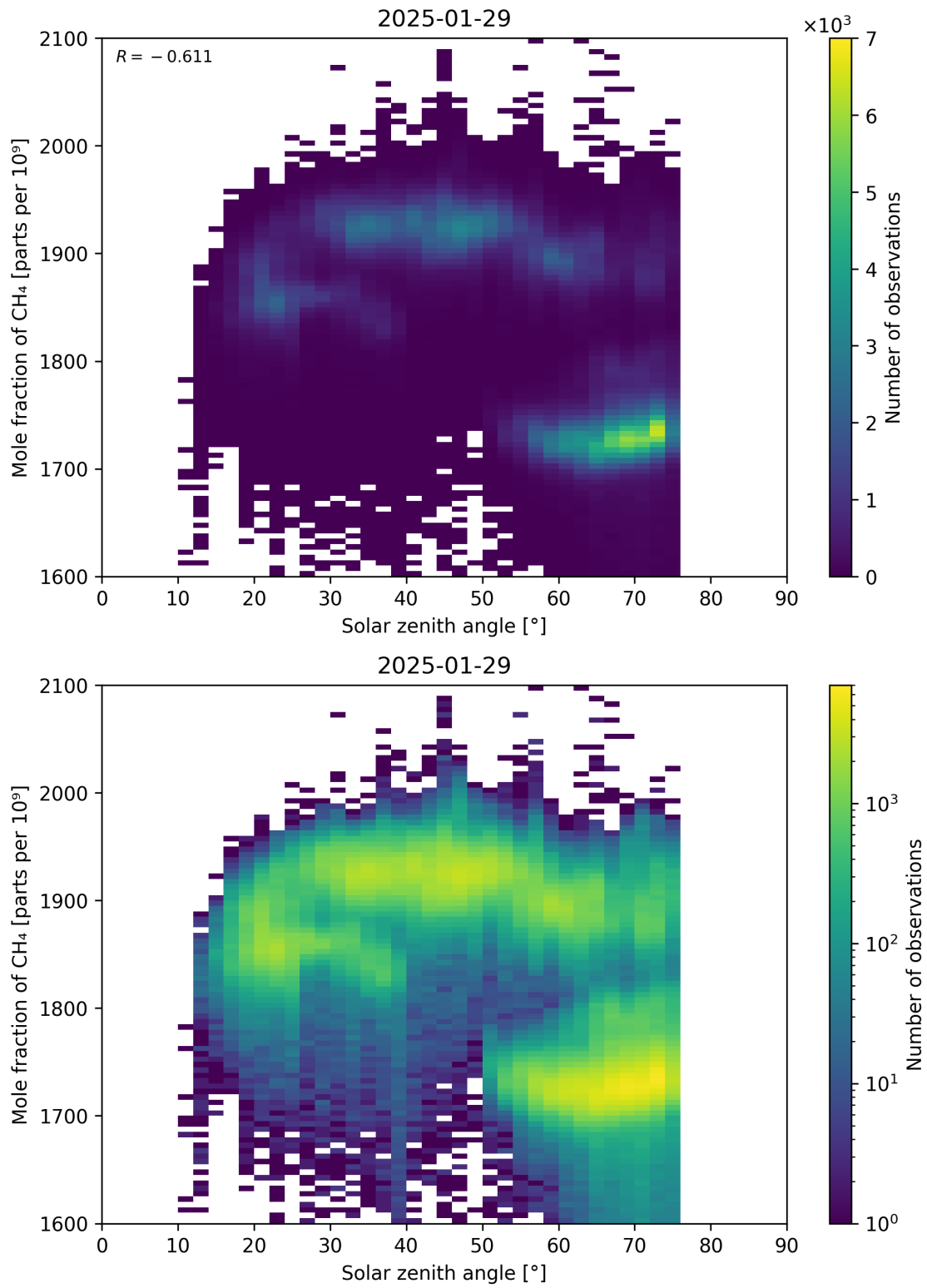
Figure 99: Scatter density plot of “Solar zenith angle” against “Mole fraction of CH 4 ” for 2025-01-28 to 2025-01-30.
