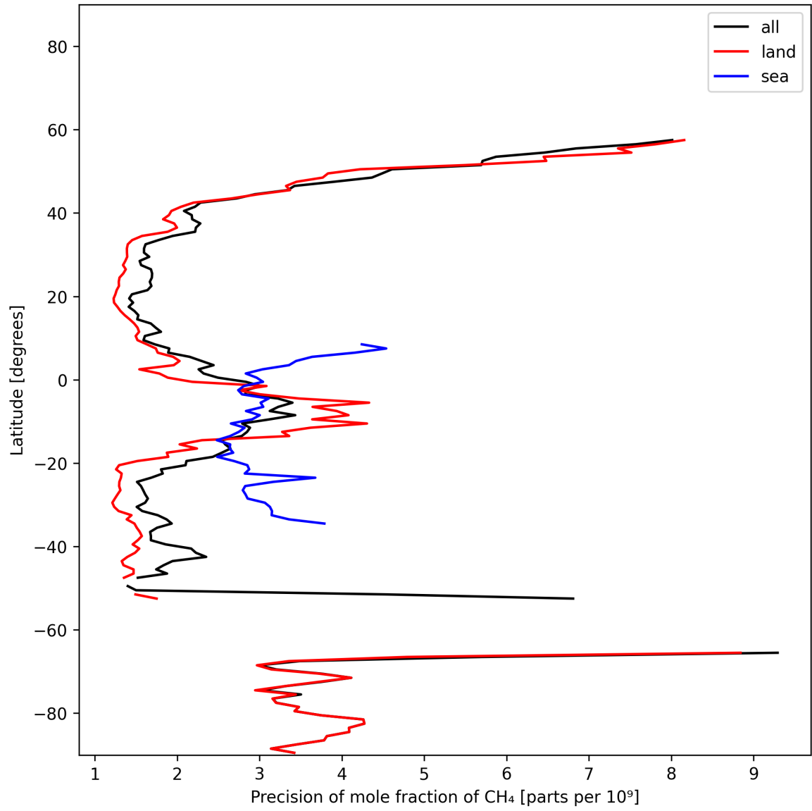
Figure 13: Zonal average of “Precision of mole fraction of CH 4 ” for 2025-01-28 to 2025-01-30.
