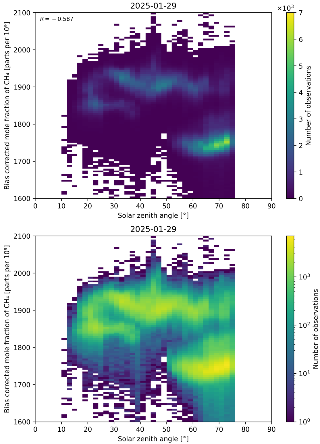
Figure 100: Scatter density plot of “Solar zenith angle” against “Bias corrected mole fraction of CH 4 ” for 2025-01-28 to 2025-01-30.
