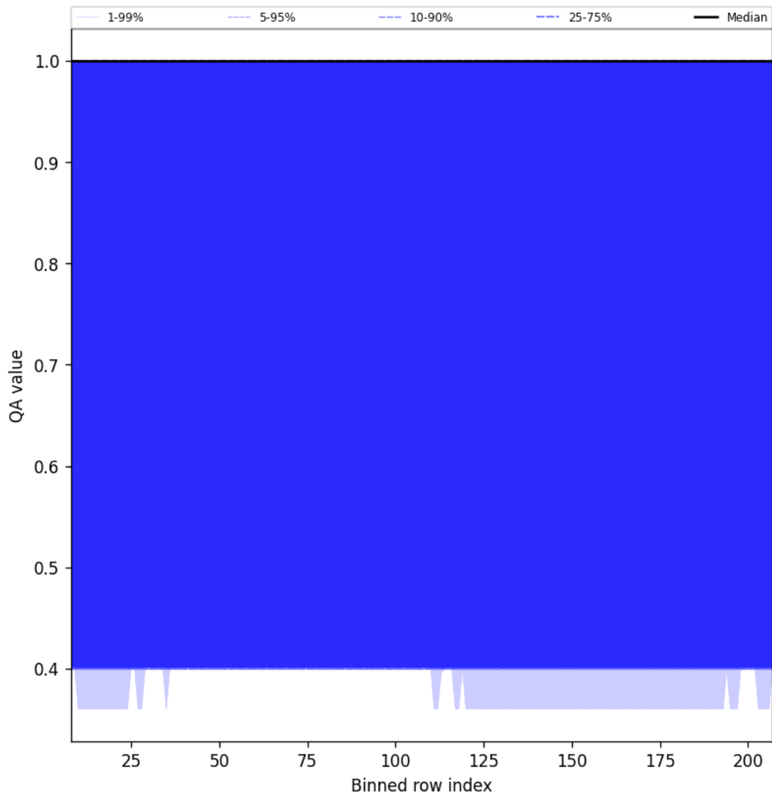
Figure 33: Along track statistics of “QA value” for 2025-01-28 to 2025-01-30
