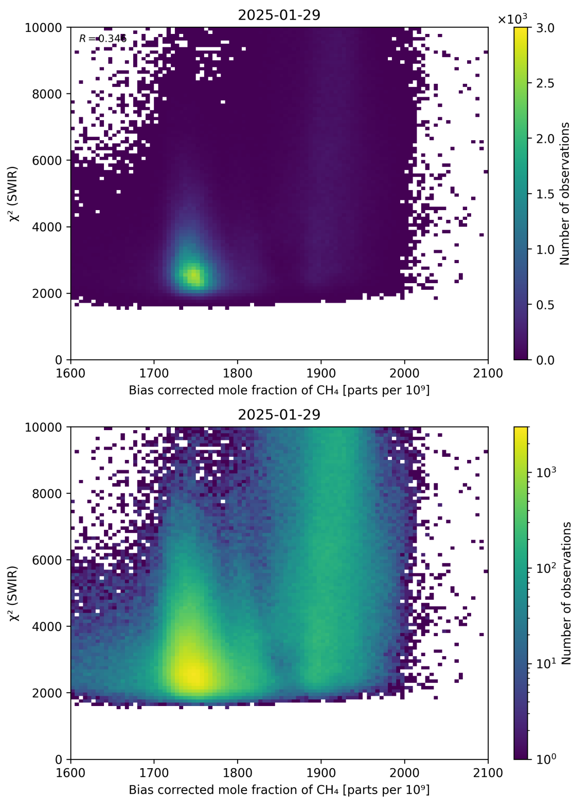
Figure 64: Scatter density plot of “Bias corrected mole fraction of \text{CH}_4 ” against “ \chi^2 (SWIR)” for 2025-01-28 to 2025-01-30.
