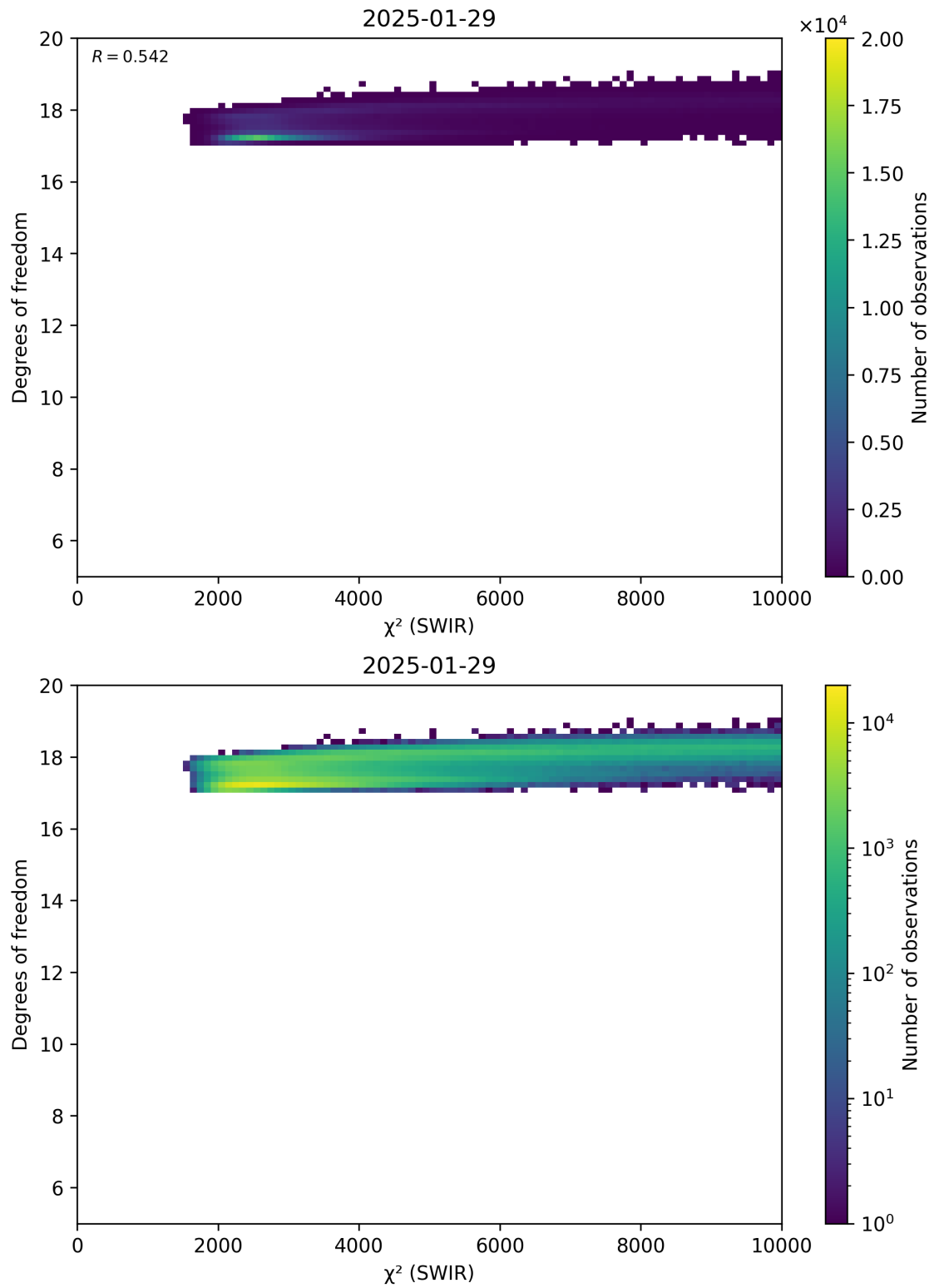
Figure 48: Scatter density plot of “ \chi^2 (SWIR)” against “Degrees of freedom” for 2025-01-28 to 2025-01-30.
