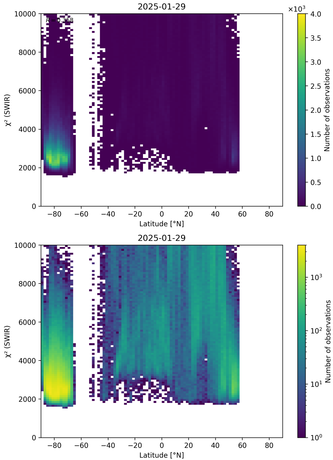
Figure 54: Scatter density plot of “Latitude” against “ \chi^2 (SWIR)” for 2025-01-28 to 2025-01-30.
