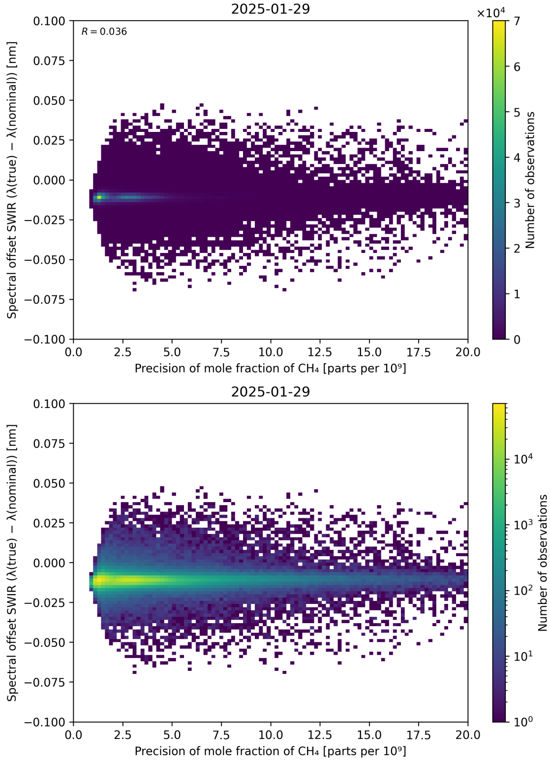
Figure 85: Scatter density plot of “Precision of mole fraction of CH 4 ” against “Spectral offset SWIR ( \lambda_{\text{true}} - \lambda_{\text{nominal}} )” for 2025-01-28 to 2025-01-30.
