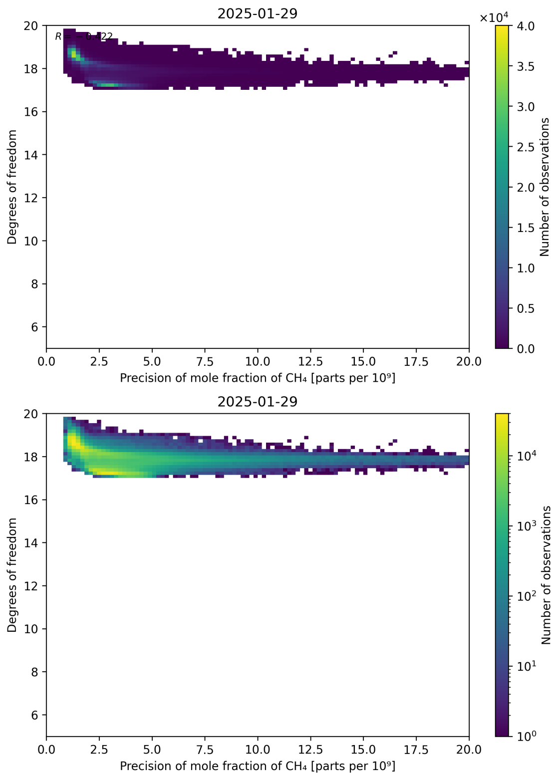
Figure 80: Scatter density plot of “Precision of mole fraction of CH 4 ” against “Degrees of freedom” for 2025-01-28 to 2025-01-30.
