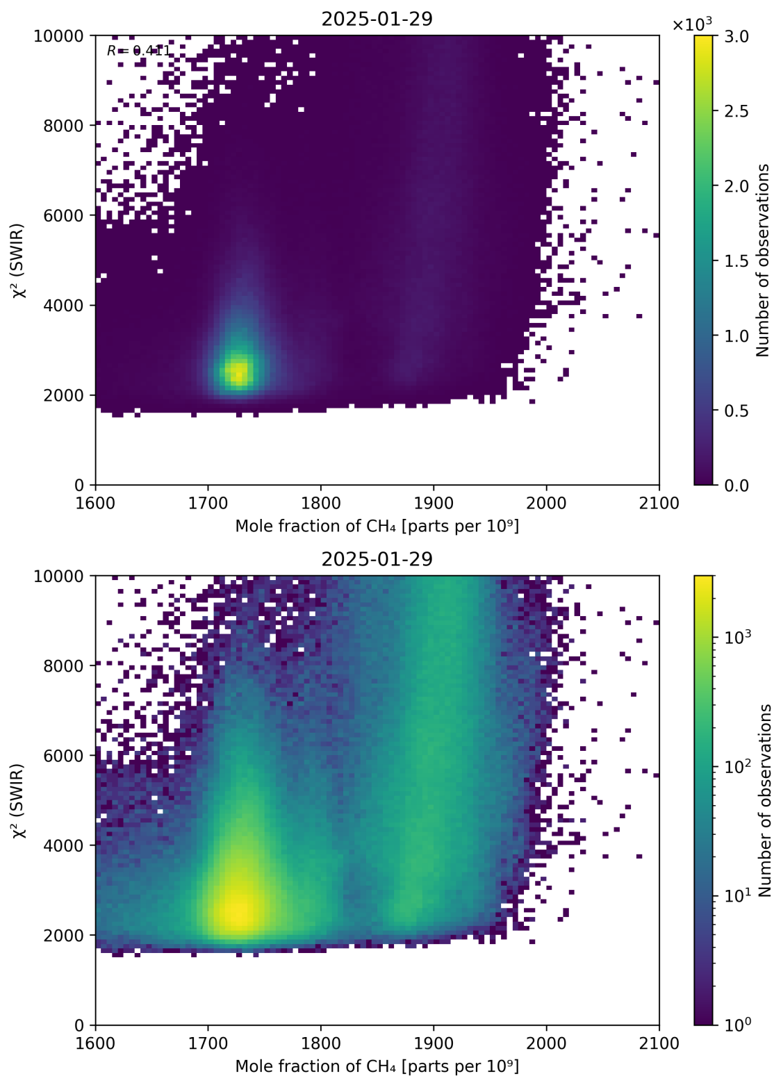
Figure 71: Scatter density plot of “Mole fraction of \text{CH}_4 ” against “ \chi^2 (SWIR)” for 2025-01-28 to 2025-01-30.
