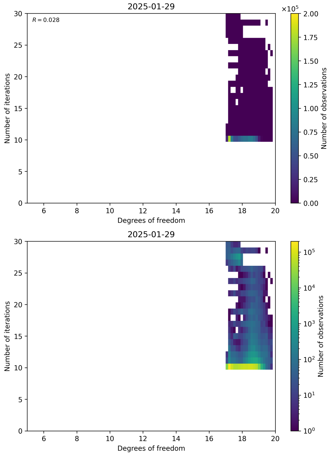
Figure 52: Scatter density plot of “Degrees of freedom” against “Number of iterations” for 2025-01-28 to 2025-01-30.
