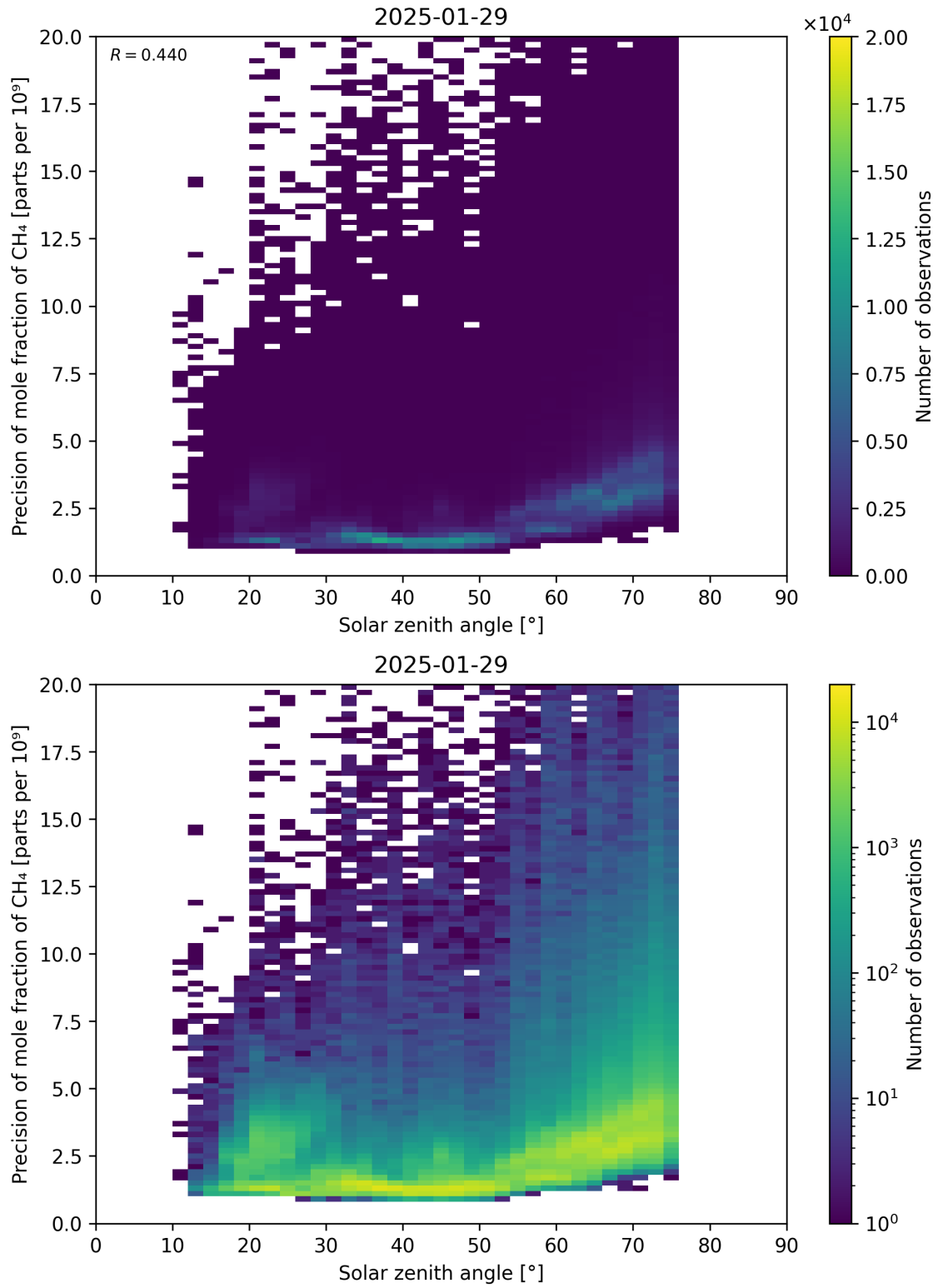
Figure 101: Scatter density plot of “Solar zenith angle” against “Precision of mole fraction of \text{CH}_4 ” for 2025-01-28 to 2025-01-30.
