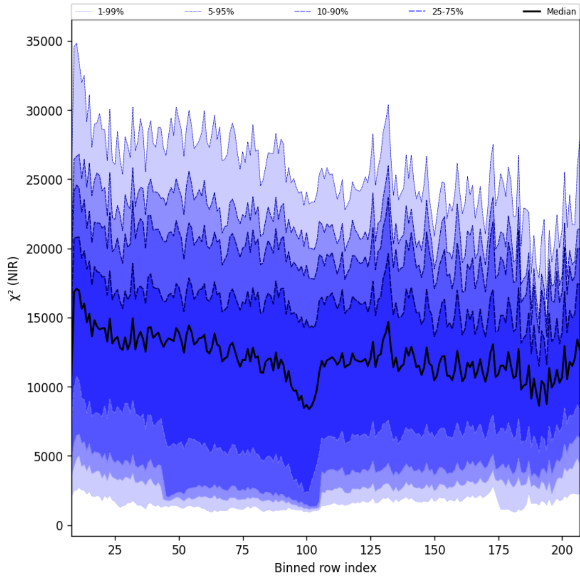
Figure 40: Along track statistics of " \chi^2 (NIR)" for 2025-01-28 to 2025-01-30
