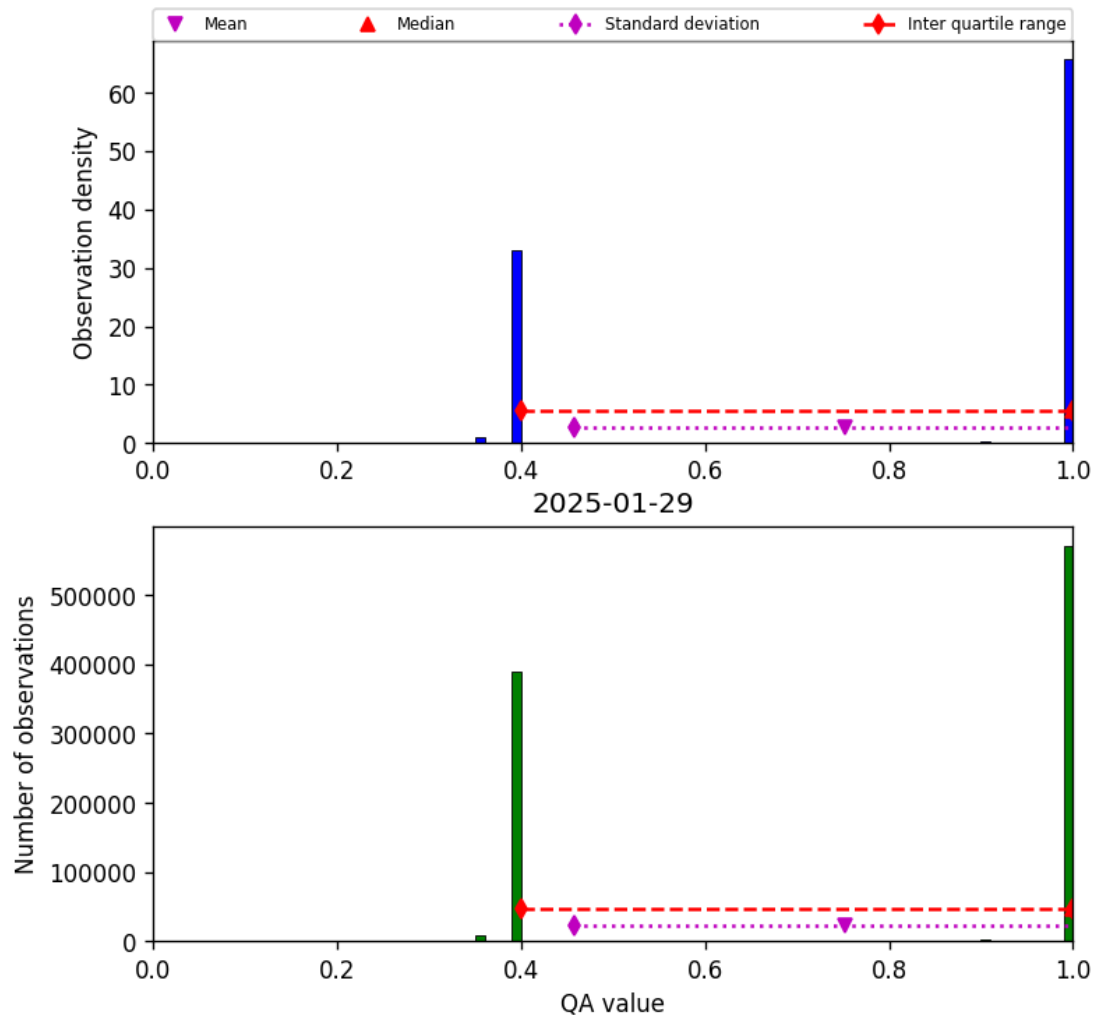
Figure 22: Histogram of “QA value” for 2025-01-28 to 2025-01-30
