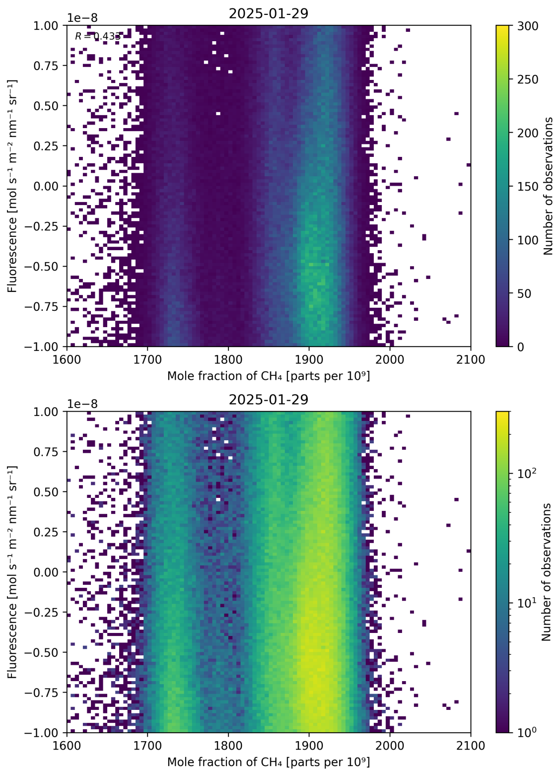
Figure 73: Scatter density plot of “Mole fraction of \text{CH}_4 ” against “Fluorescence” for 2025-01-28 to 2025-01-30.
