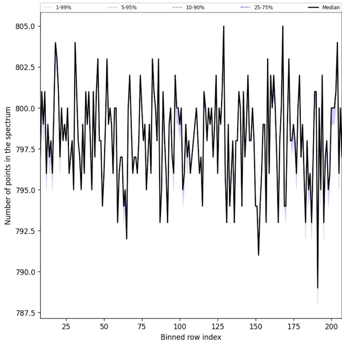
Figure 37: Along track statistics of “Number of points in the spectrum” for 2025-01-28 to 2025-01-30
