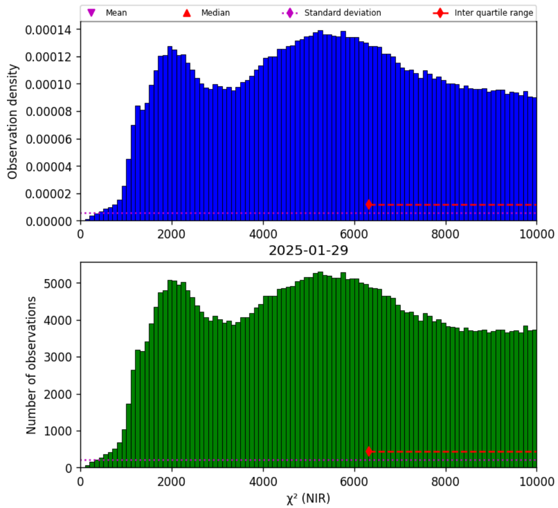
Figure 29: Histogram of “ \chi^2 (NIR)” for 2025-01-28 to 2025-01-30
