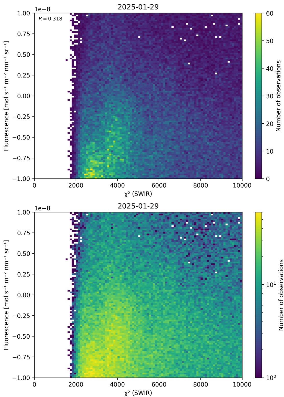
Figure 49: Scatter density plot of “ \chi^2 (SWIR)” against “Fluorescence” for 2025-01-28 to 2025-01-30.
