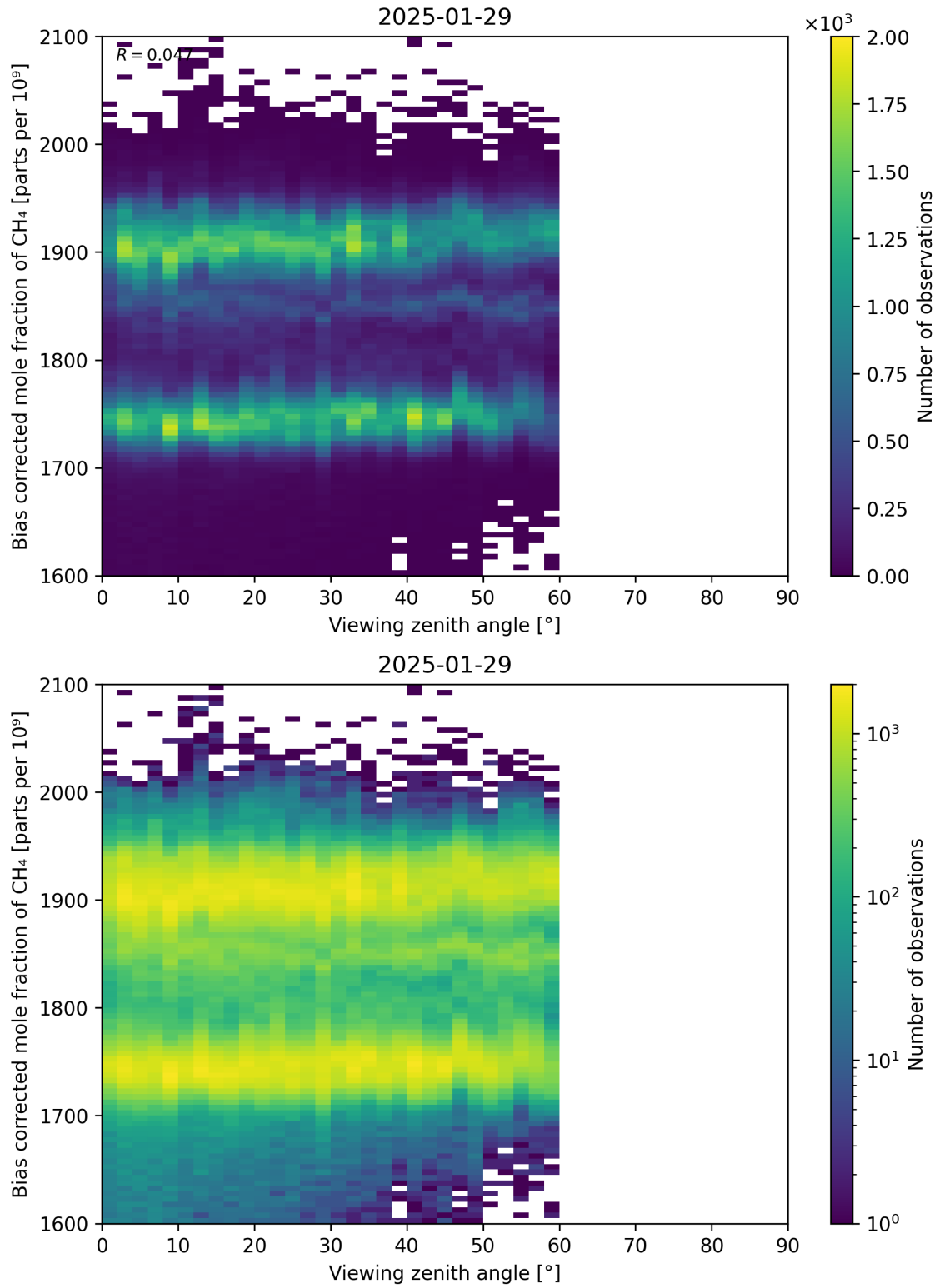
Figure 111: Scatter density plot of “Viewing zenith angle” against “Bias corrected mole fraction of CH 4 ” for 2025-01-28 to 2025-01-30.
