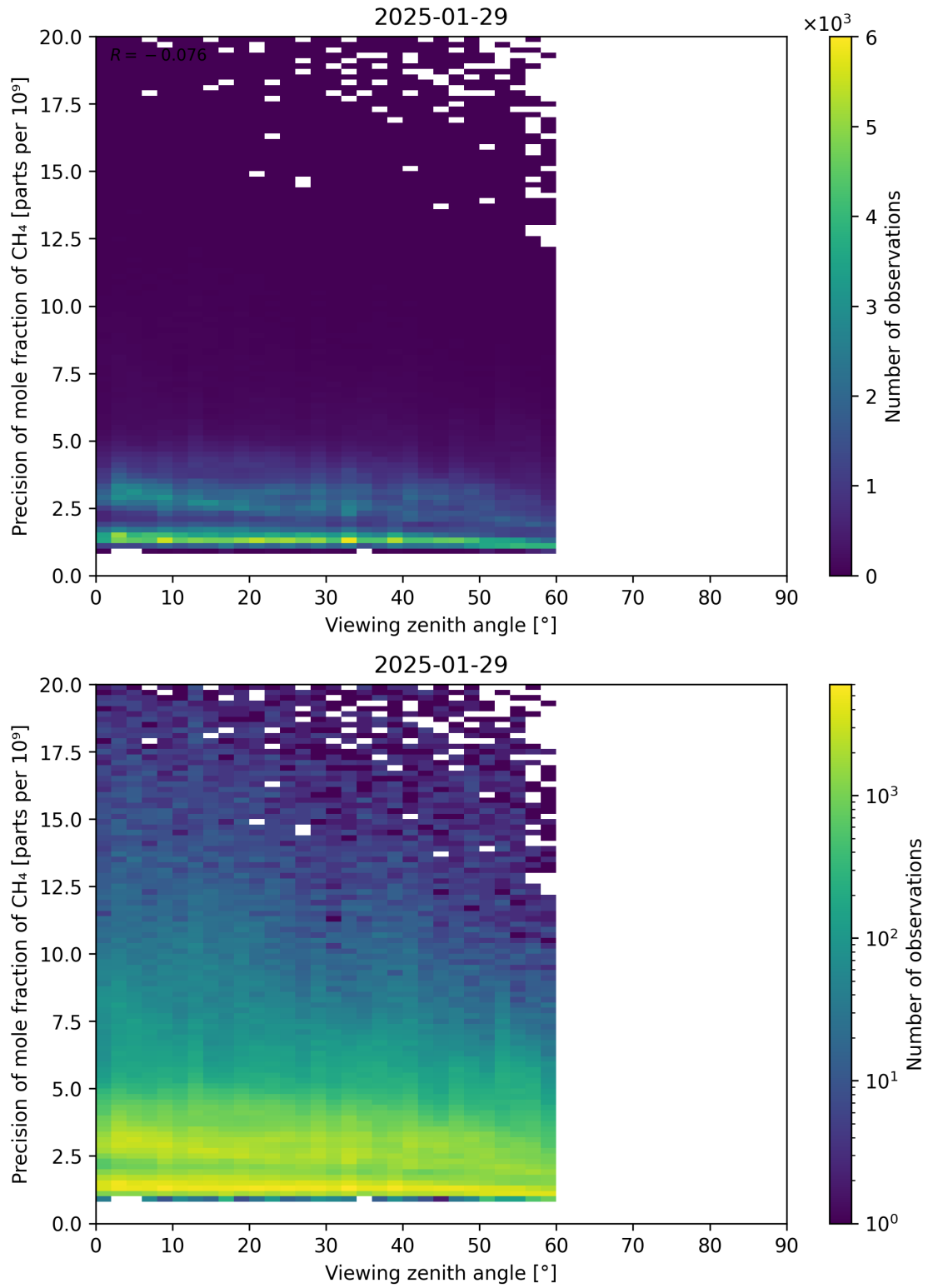
Figure 112: Scatter density plot of “Viewing zenith angle” against “Precision of mole fraction of CH 4 ” for 2025-01-28 to 2025-01-30.
