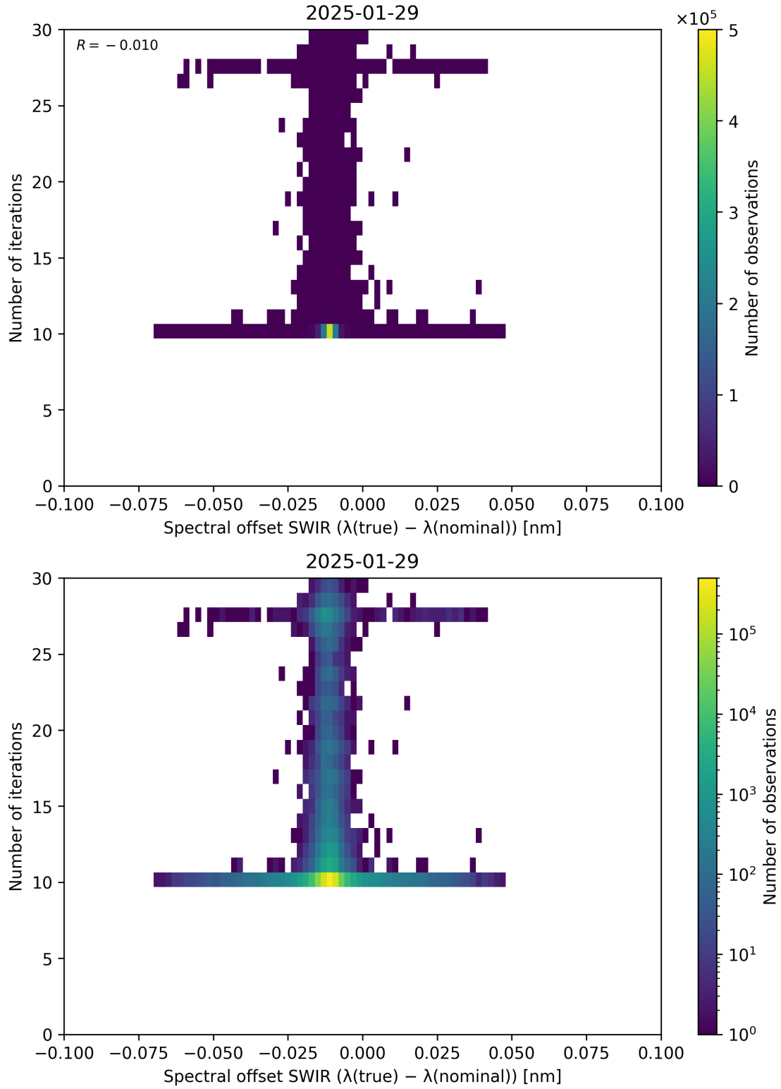
Figure 121: Scatter density plot of “Spectral offset SWIR ( \lambda_{\text{true}} - \lambda_{\text{nominal}} )” against “Number of iterations” for 2025-01-28 to 2025-01-30.
