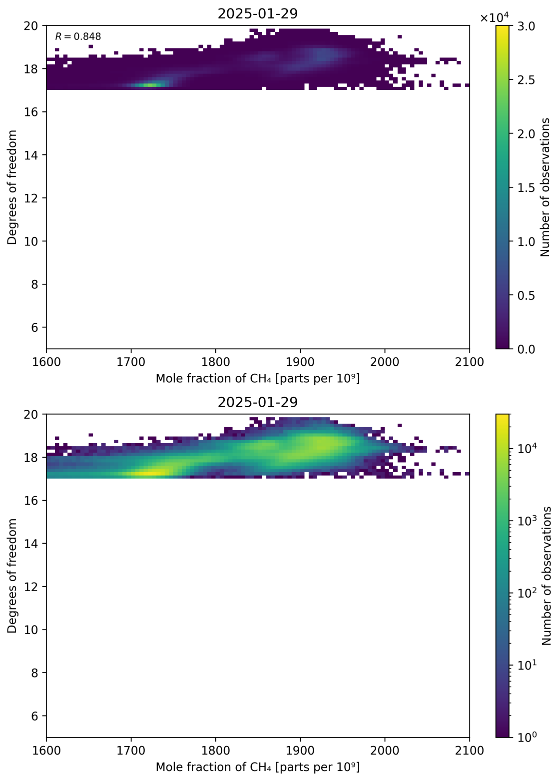
Figure 72: Scatter density plot of “Mole fraction of CH 4 ” against “Degrees of freedom” for 2025-01-28 to 2025-01-30.
