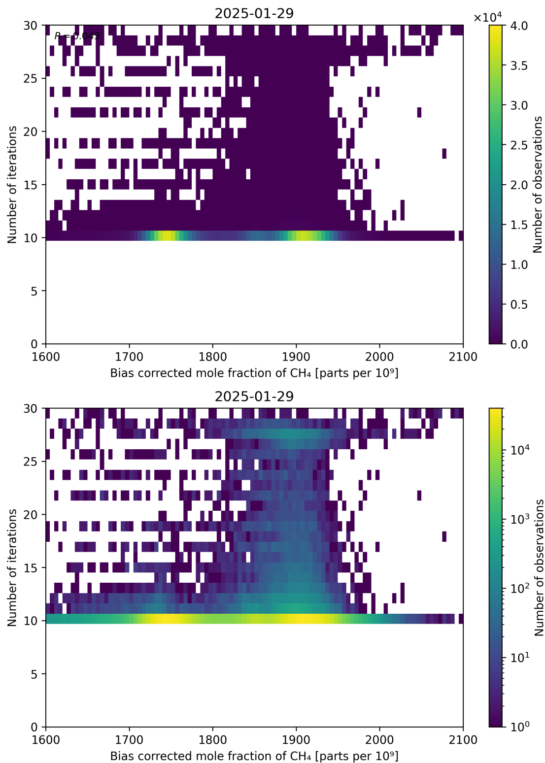
Figure 67: Scatter density plot of “Bias corrected mole fraction of CH 4 ” against “Number of iterations” for 2025-01-28 to 2025-01-30.
