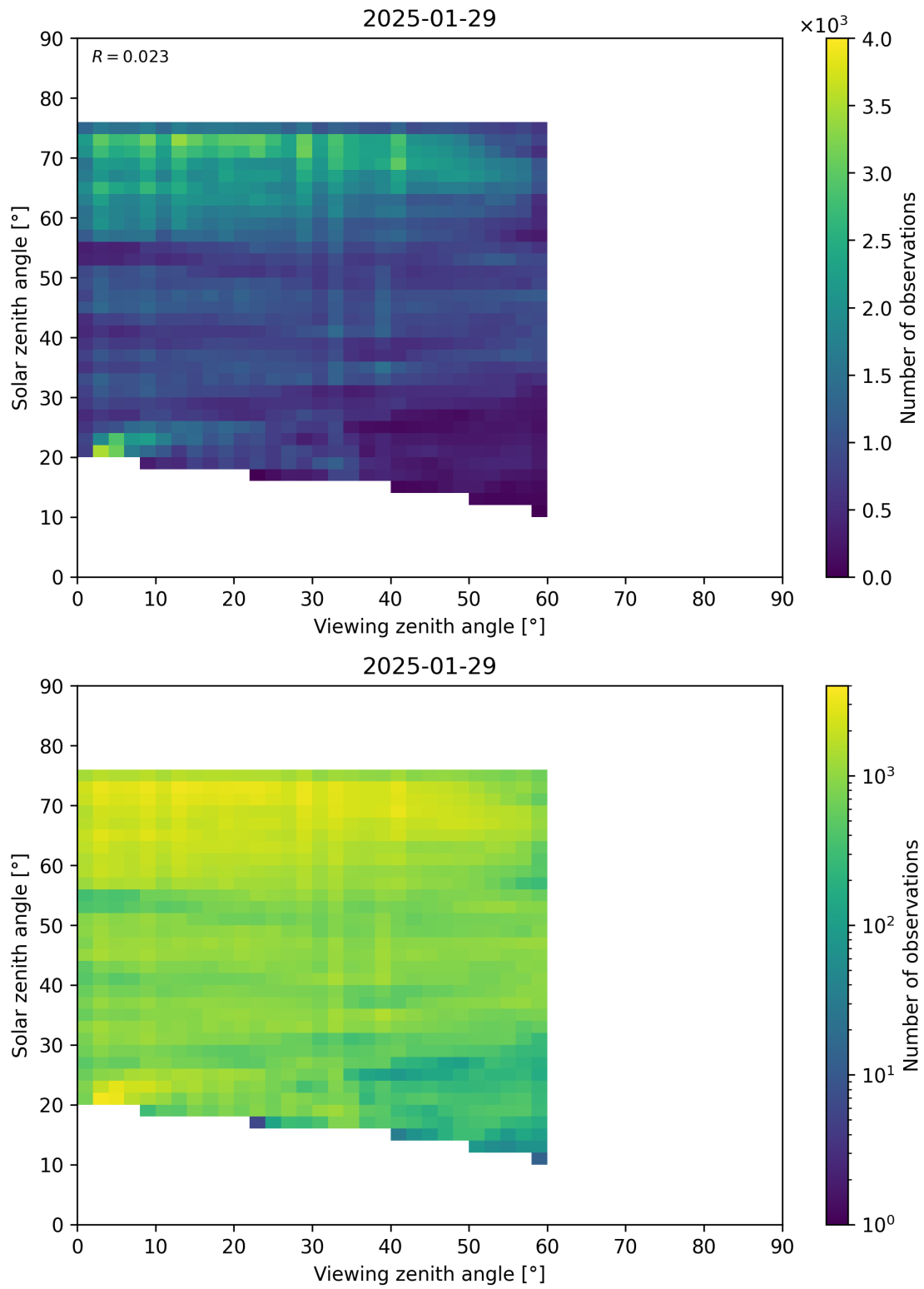
Figure 115: Scatter density plot of “Viewing zenith angle” against “Solar zenith angle” for 2025-01-28 to 2025-01-30.
