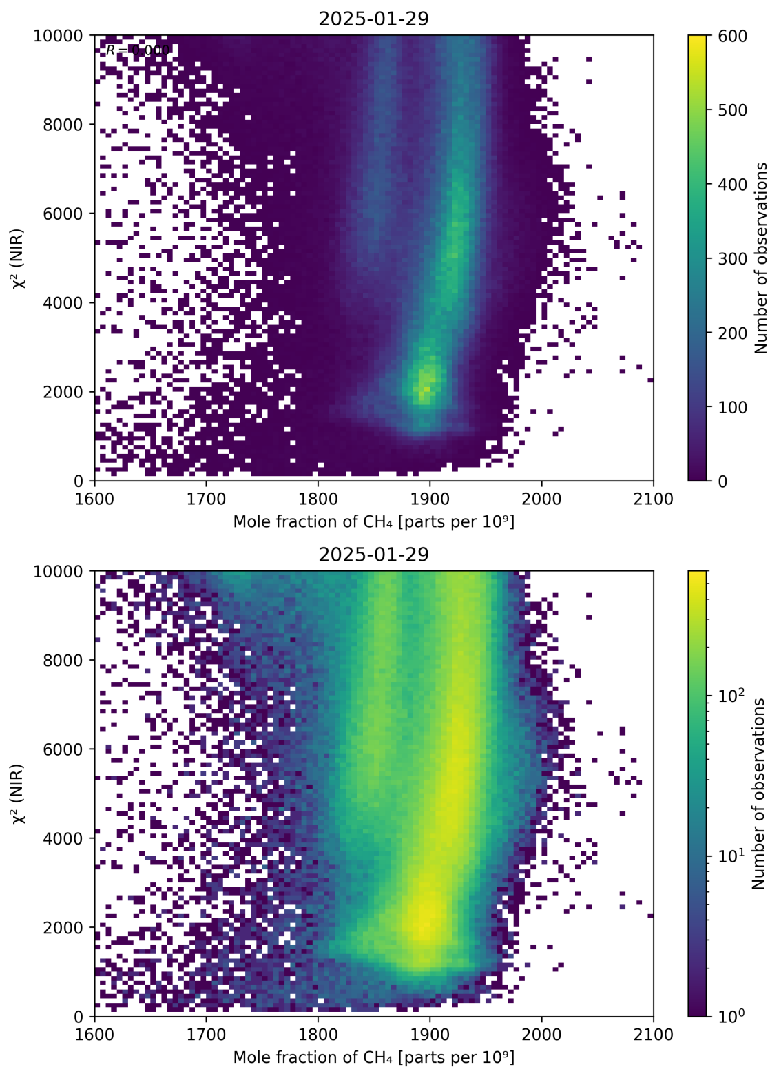
Figure 70: Scatter density plot of “Mole fraction of \text{CH}_4 ” against “ \chi^2 (NIR)” for 2025-01-28 to 2025-01-30.
