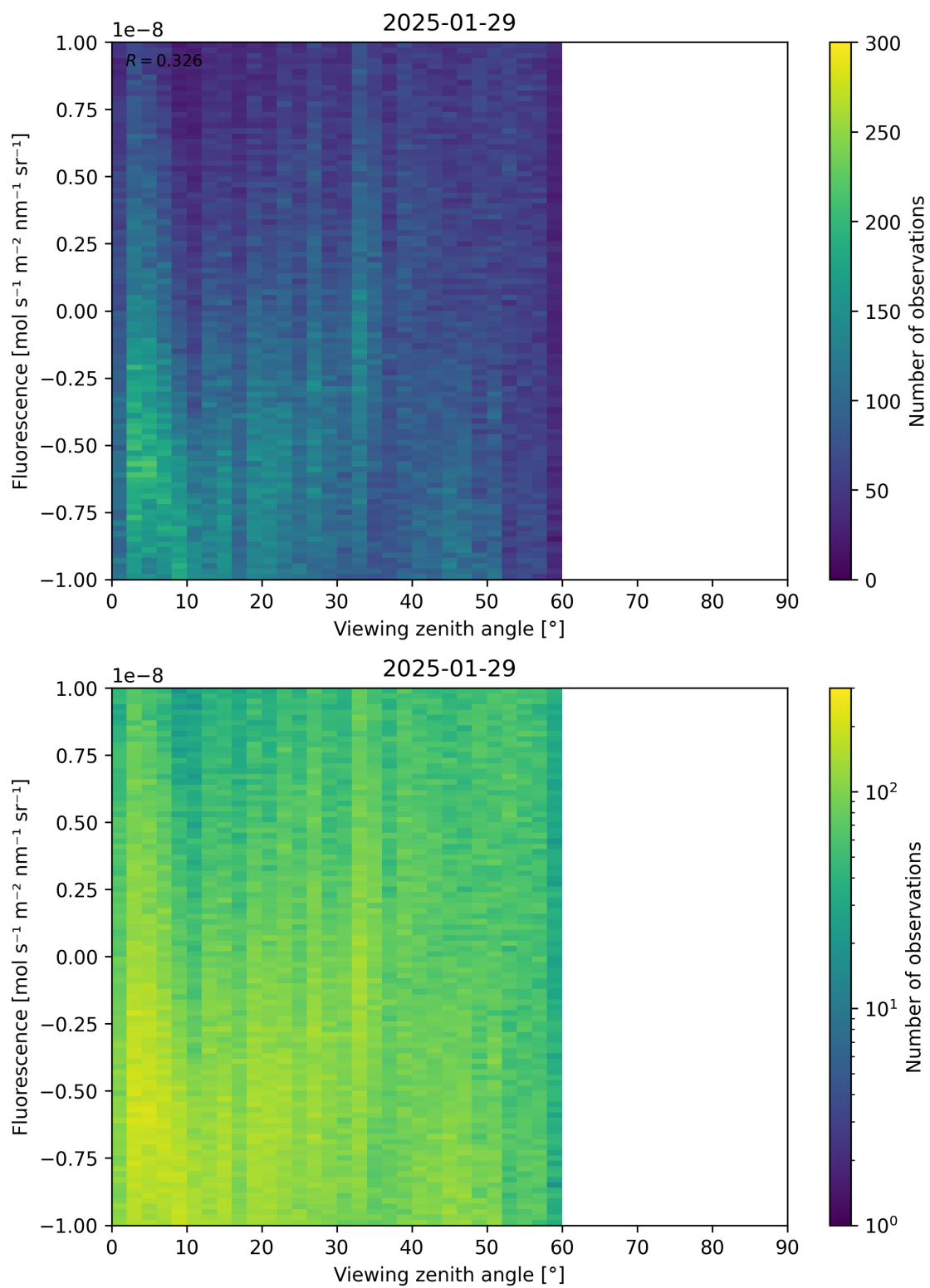
Figure 108: Scatter density plot of “Viewing zenith angle” against “Fluorescence” for 2025-01-28 to 2025-01-30.
