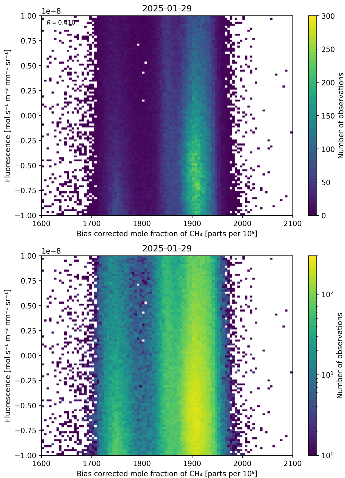
Figure 66: Scatter density plot of “Bias corrected mole fraction of \text{CH}_4 ” against “Fluorescence” for 2025-01-28 to 2025-01-30.
