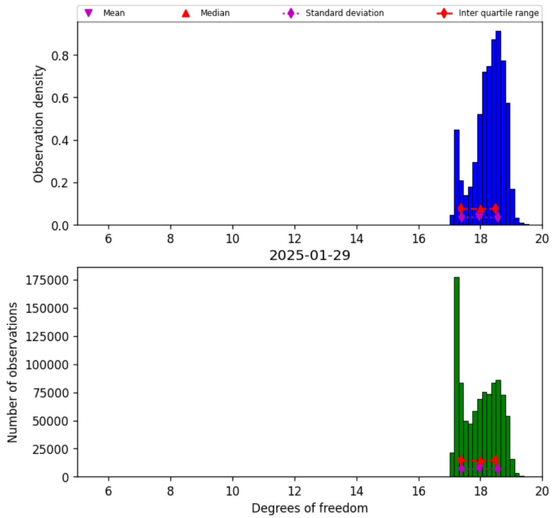
Figure 30: Histogram of “Degrees of freedom” for 2025-01-28 to 2025-01-30
