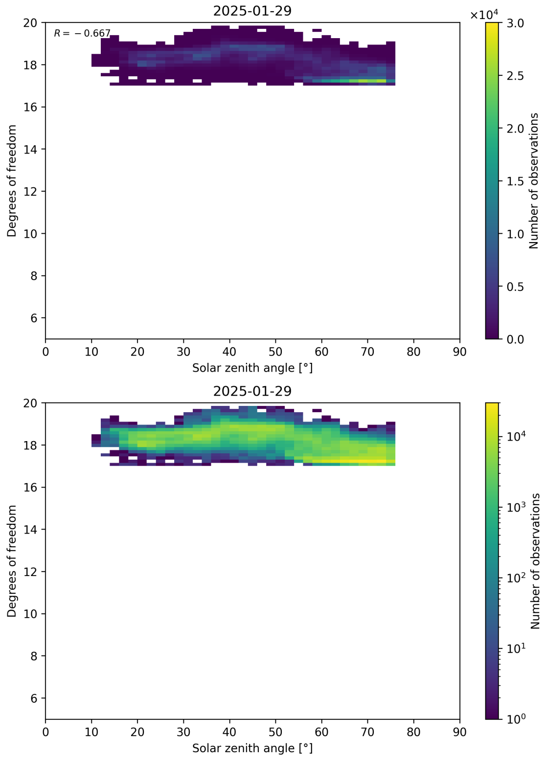
Figure 96: Scatter density plot of “Solar zenith angle” against “Degrees of freedom” for 2025-01-28 to 2025-01-30.
