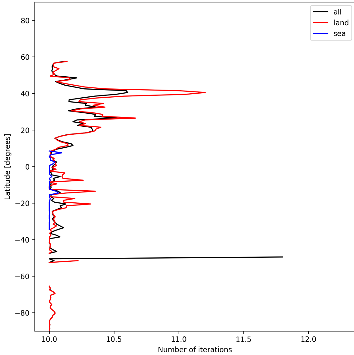
Figure 20: Zonal average of “Number of iterations” for 2025-01-28 to 2025-01-30.
