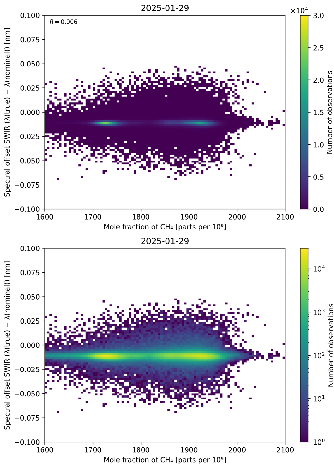
Figure 86: Scatter density plot of “Mole fraction of \text{CH}_4 ” against “Spectral offset SWIR ( \lambda_{\text{true}} - \lambda_{\text{nominal}} )” for 2025-01-28 to 2025-01-30.
