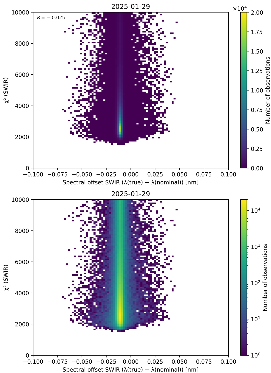
Figure 118: Scatter density plot of “Spectral offset SWIR ( \lambda_{\text{true}} - \lambda_{\text{nominal}} )” against “ \chi^2 (SWIR)” for 2025-01-28 to 2025-01-30.
