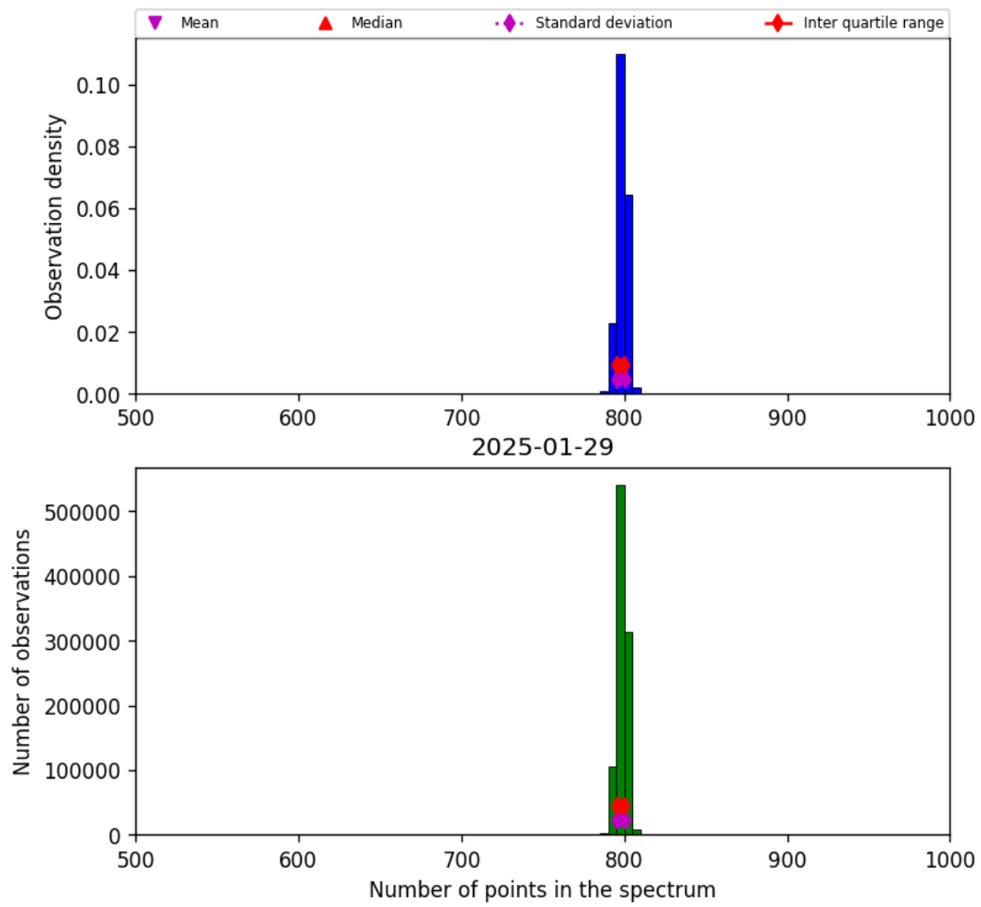
Figure 26: Histogram of “Number of points in the spectrum” for 2025-01-28 to 2025-01-30
