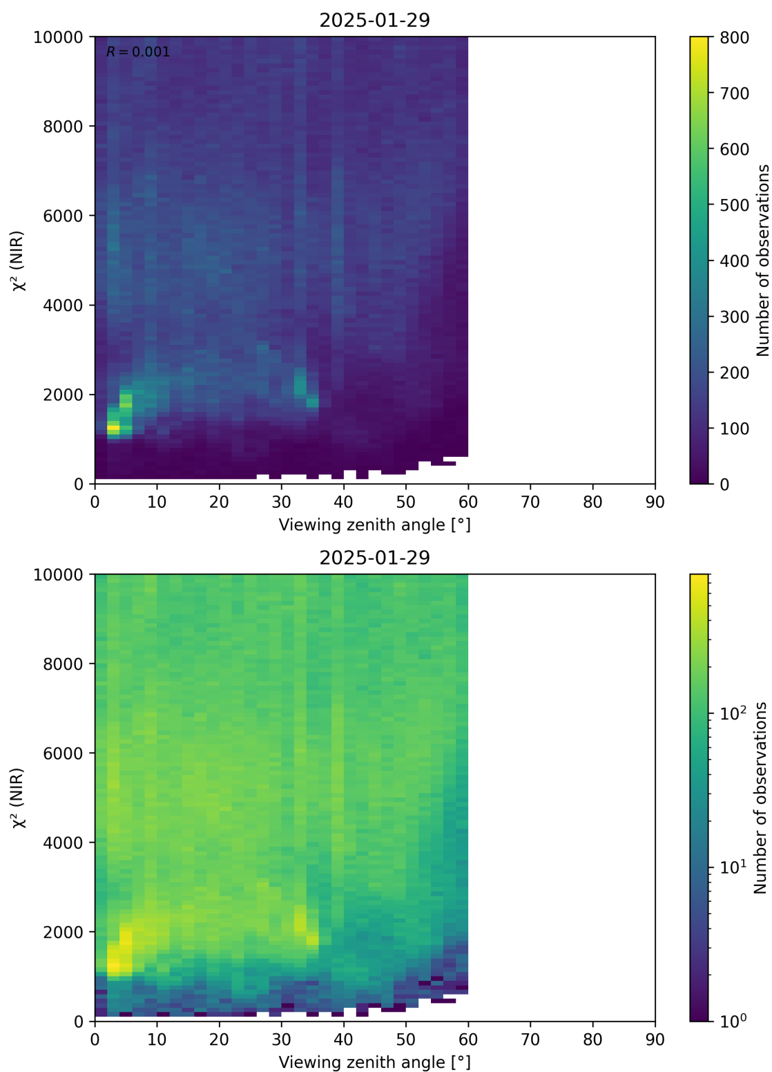
Figure 105: Scatter density plot of “Viewing zenith angle” against “ \chi^2 (NIR)” for 2025-01-28 to 2025-01-30.
