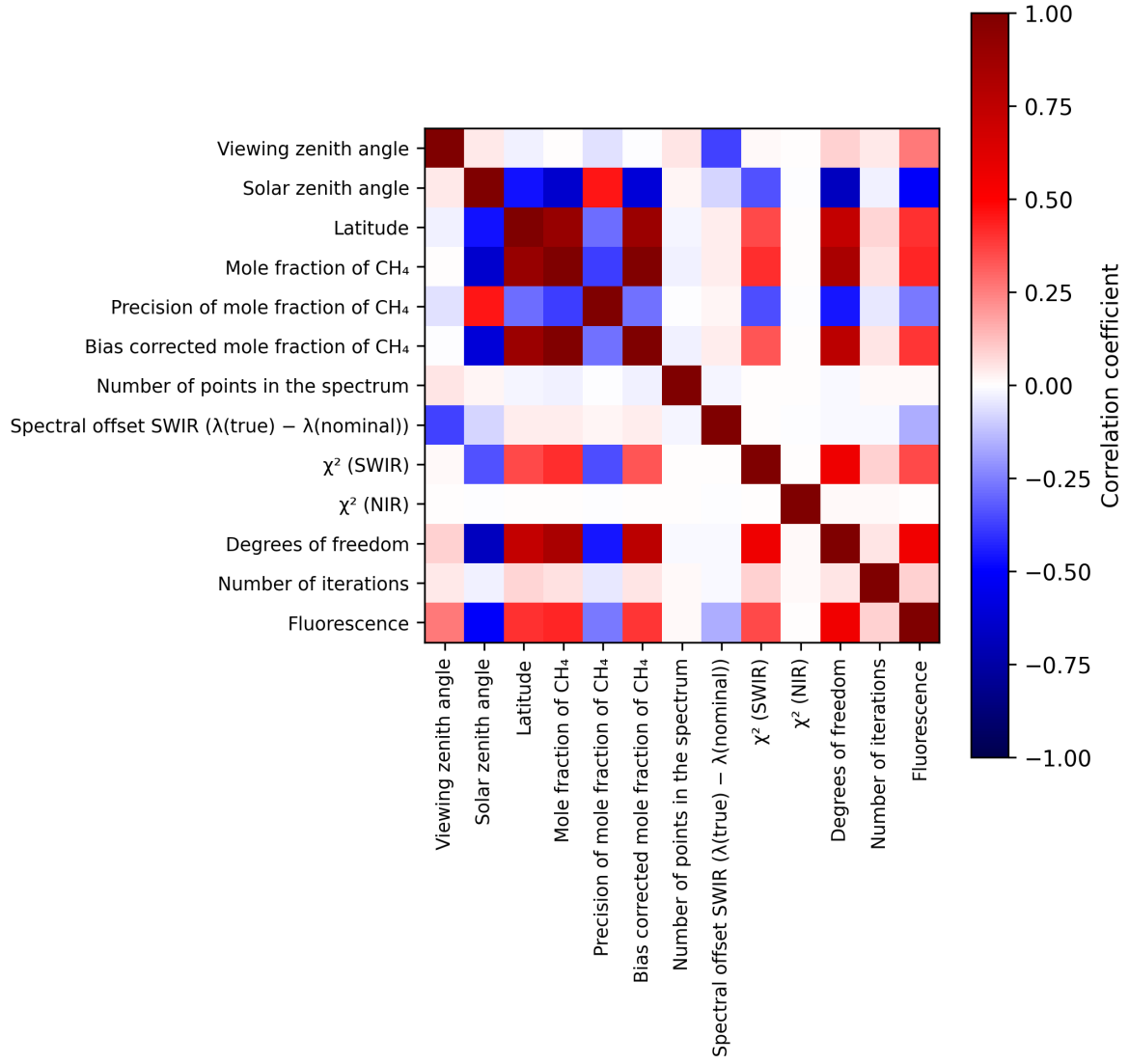
Figure 2: Map of correlation matrix for 2025-01-30 to 2025-02-01.
