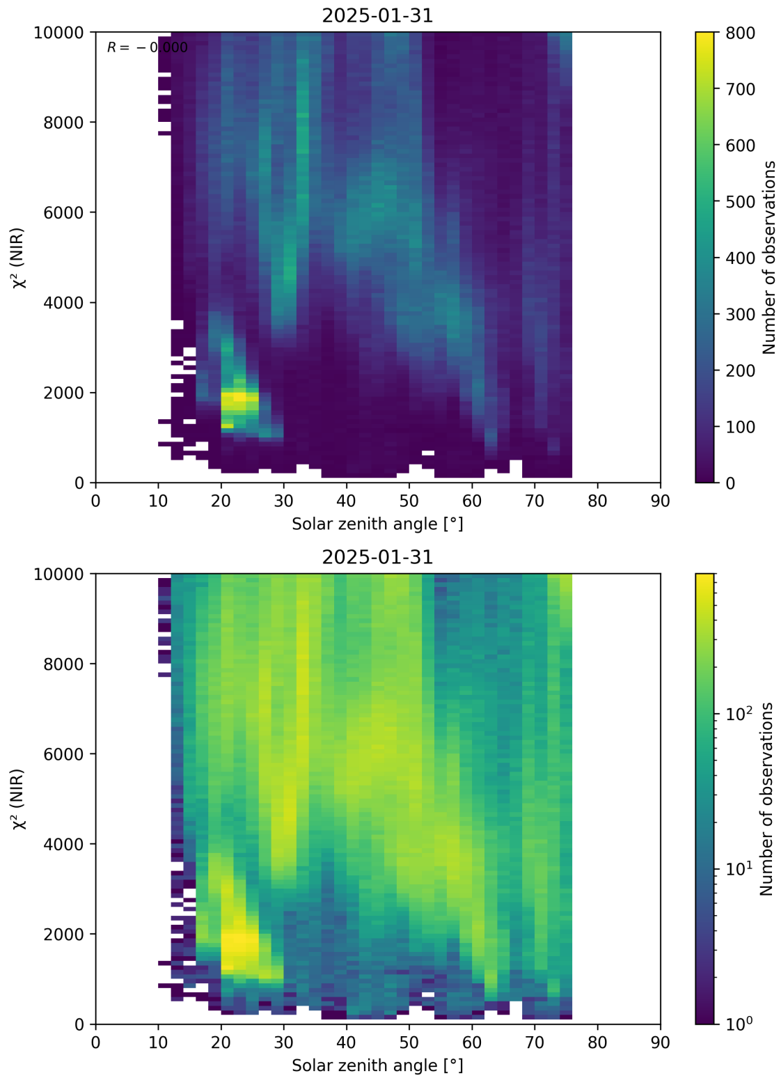
Figure 94: Scatter density plot of “Solar zenith angle” against “ \chi^2 (NIR)” for 2025-01-30 to 2025-02-01.
