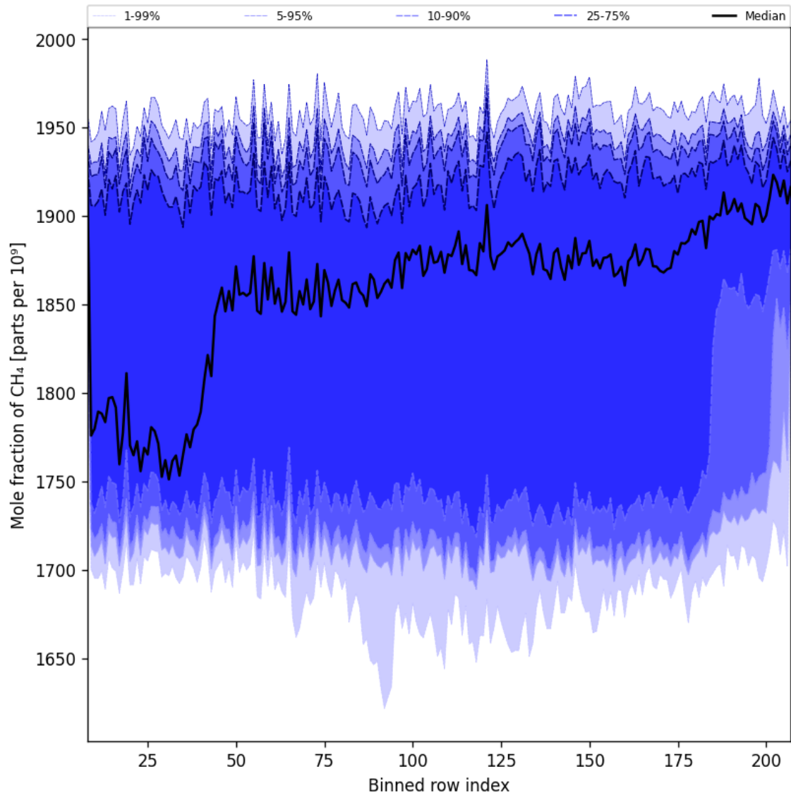
Figure 34: Along track statistics of “Mole fraction of CH 4 ” for 2025-01-30 to 2025-02-01
