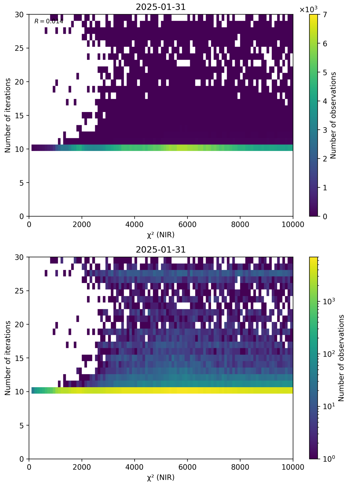
Figure 46: Scatter density plot of “ \chi^2 (NIR)” against “Number of iterations” for 2025-01-30 to 2025-02-01.
