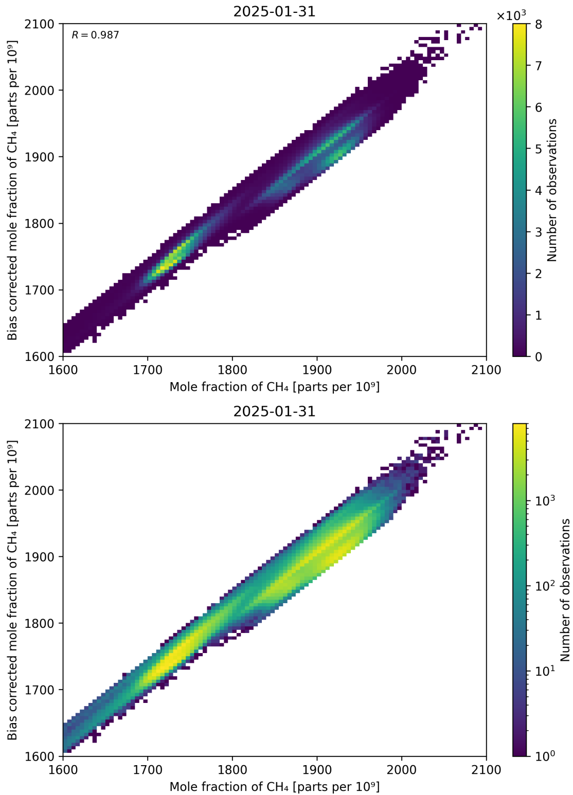
Figure 74: Scatter density plot of “Mole fraction of CH 4 ” against “Bias corrected mole fraction of CH 4 ” for 2025-01-30 to 2025-02-01.
