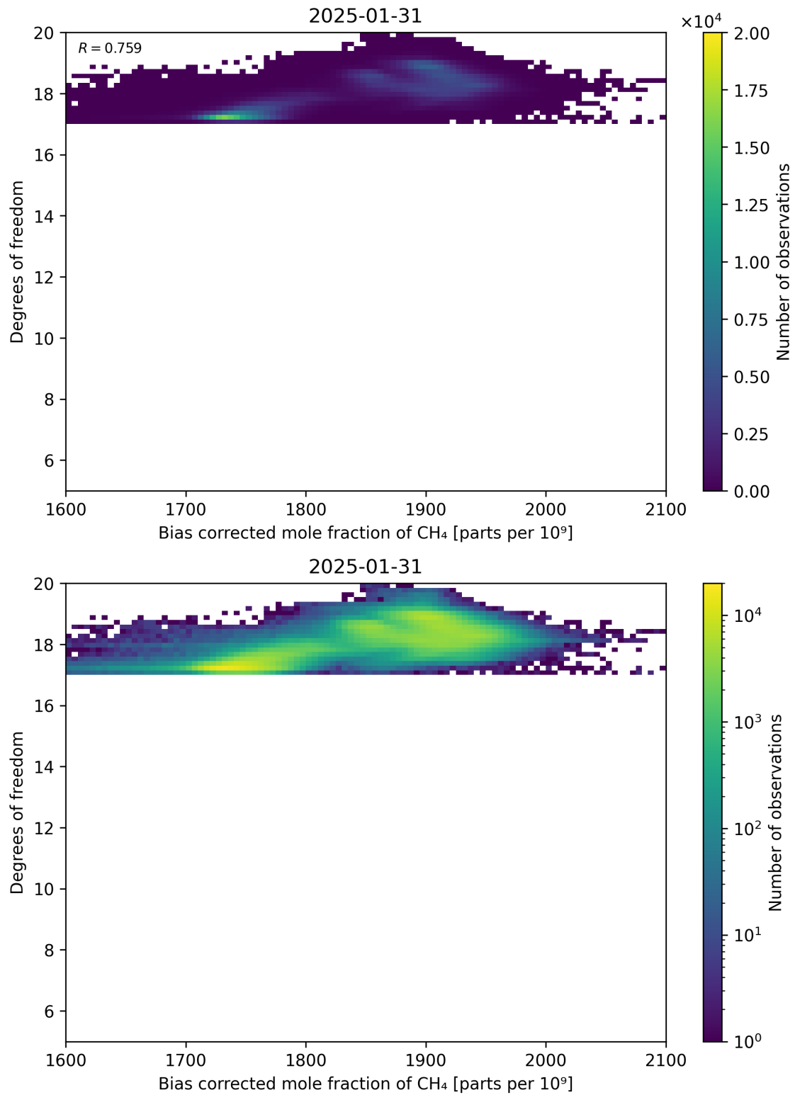
Figure 65: Scatter density plot of “Bias corrected mole fraction of CH 4 ” against “Degrees of freedom” for 2025-01-30 to 2025-02-01.
