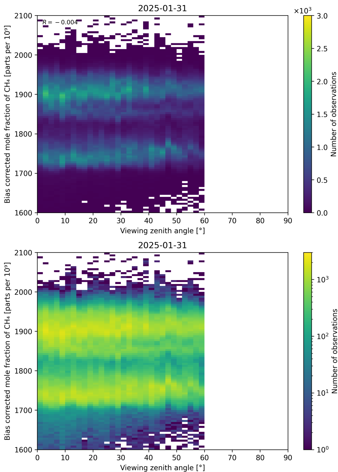
Figure 111: Scatter density plot of “Viewing zenith angle” against “Bias corrected mole fraction of CH 4 ” for 2025-01-30 to 2025-02-01.
