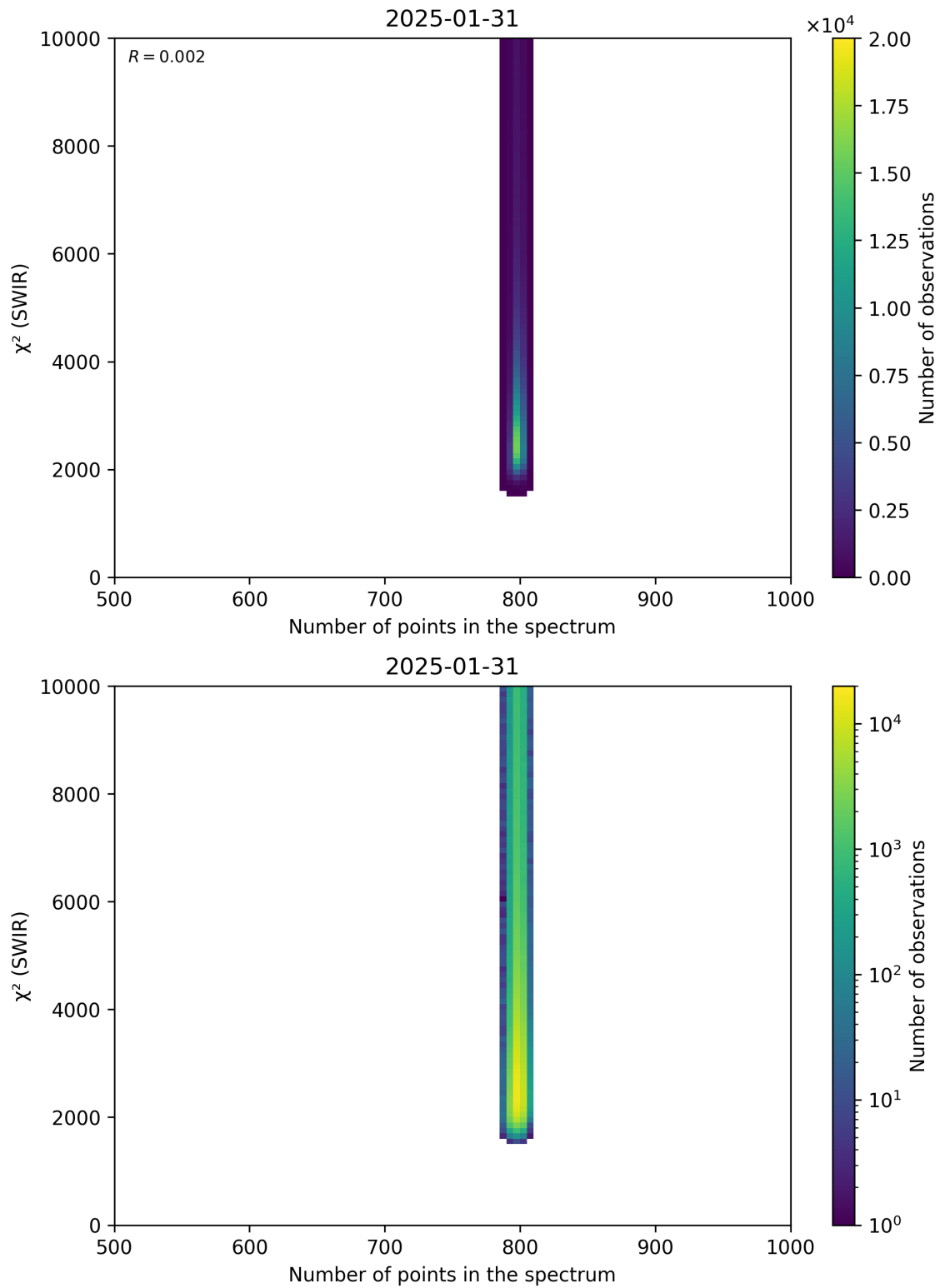
Figure 89: Scatter density plot of “Number of points in the spectrum” against “ \chi^2 (SWIR)” for 2025-01-30 to 2025-02-01.
