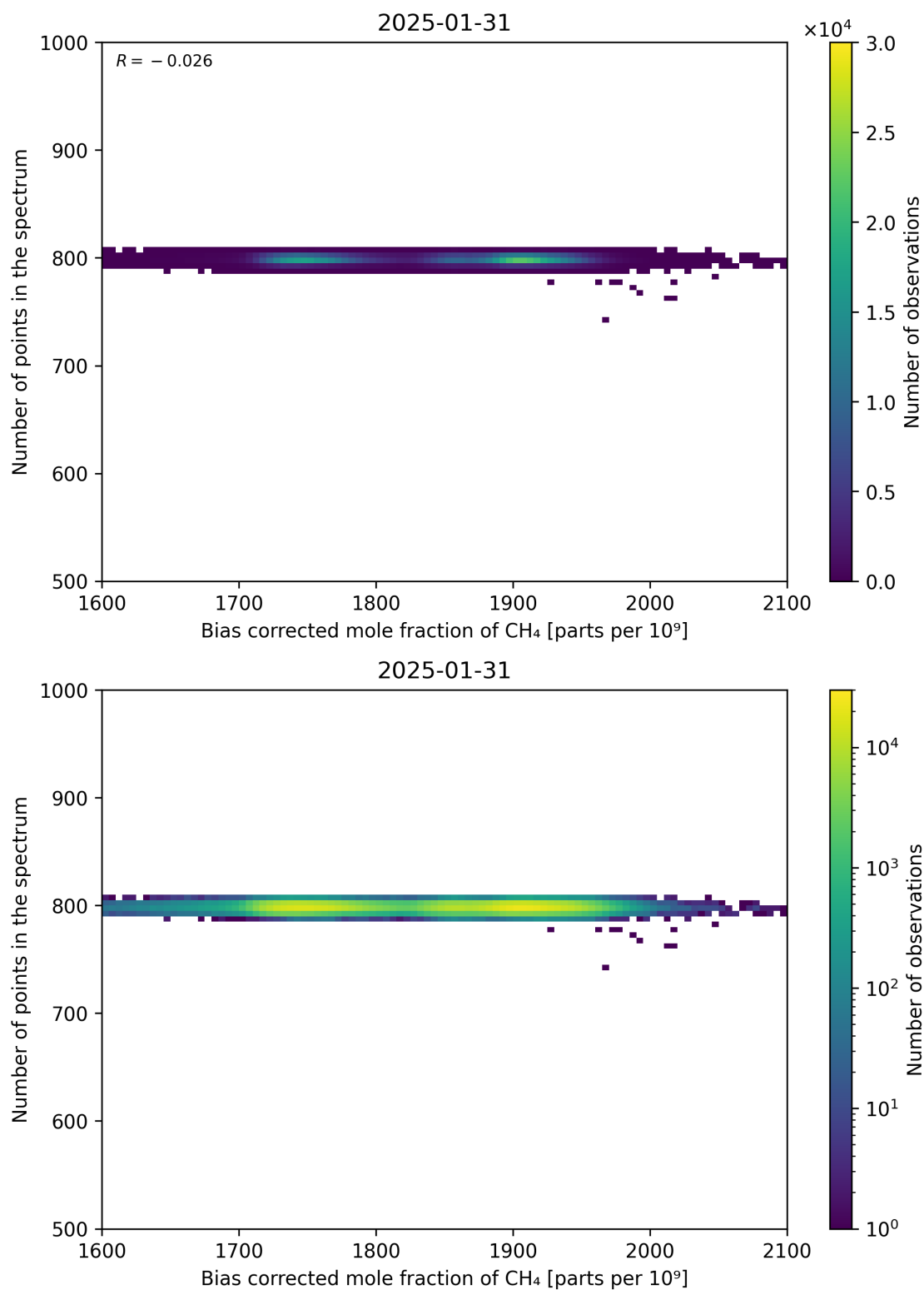
Figure 68: Scatter density plot of “Bias corrected mole fraction of CH 4 ” against “Number of points in the spectrum” for 2025-01-30 to 2025-02-01.
