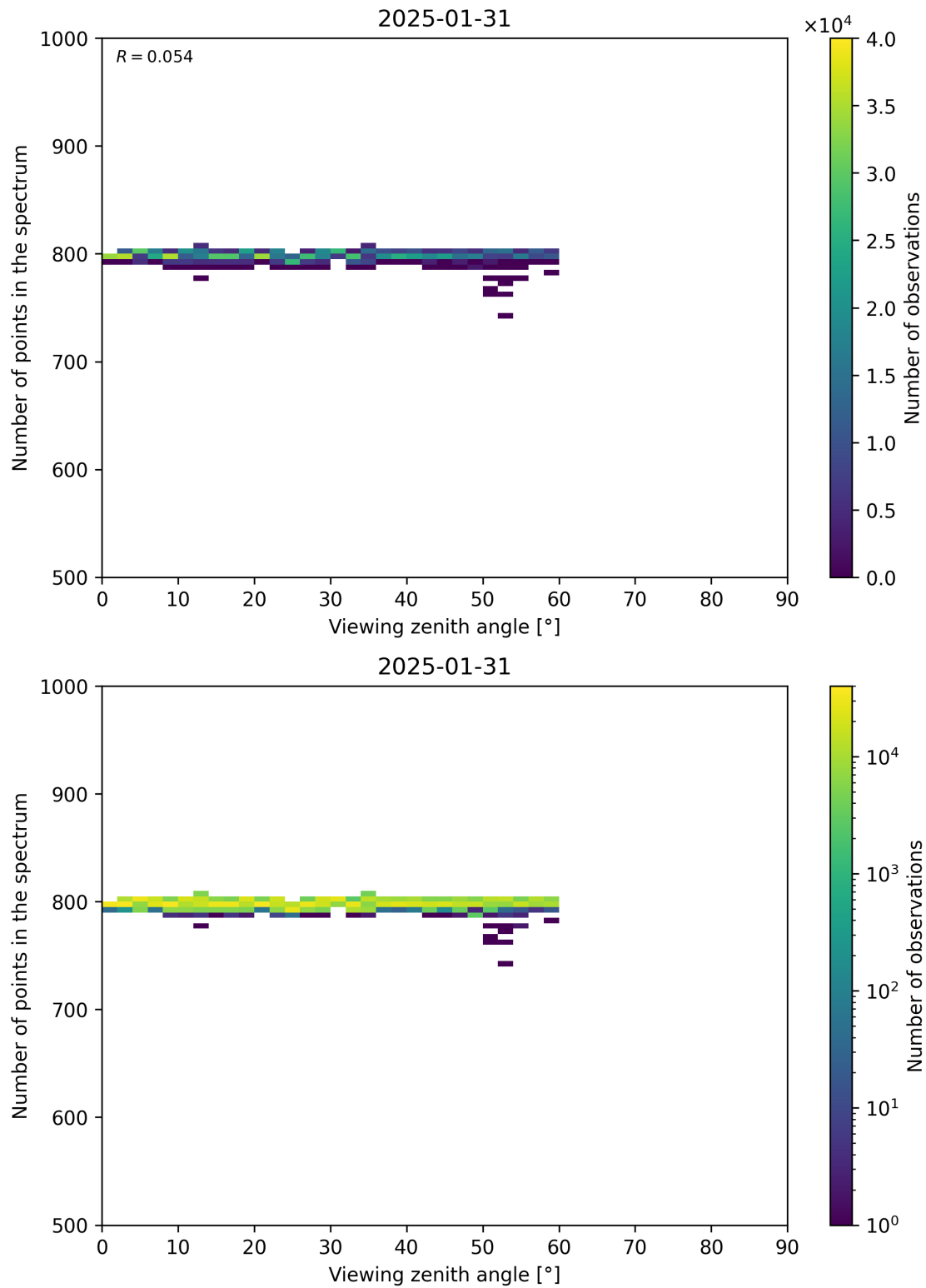
Figure 114: Scatter density plot of “Viewing zenith angle” against “Number of points in the spectrum” for 2025-01-30 to 2025-02-01.
