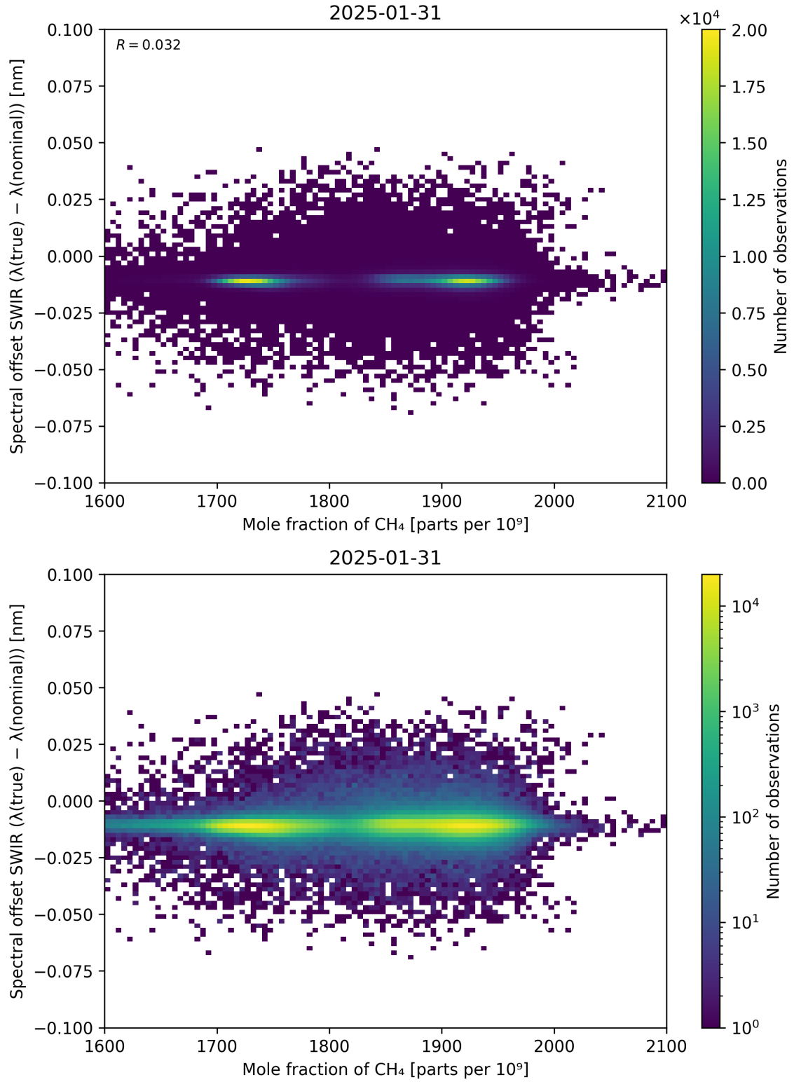
Figure 86: Scatter density plot of “Mole fraction of \text{CH}_4 ” against “Spectral offset SWIR ( \lambda_{\text{true}} - \lambda_{\text{nominal}} )” for 2025-01-30 to 2025-02-01.
