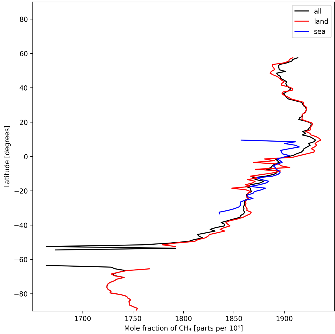
Figure 12: Zonal average of “Mole fraction of CH 4 ” for 2025-01-30 to 2025-02-01.
