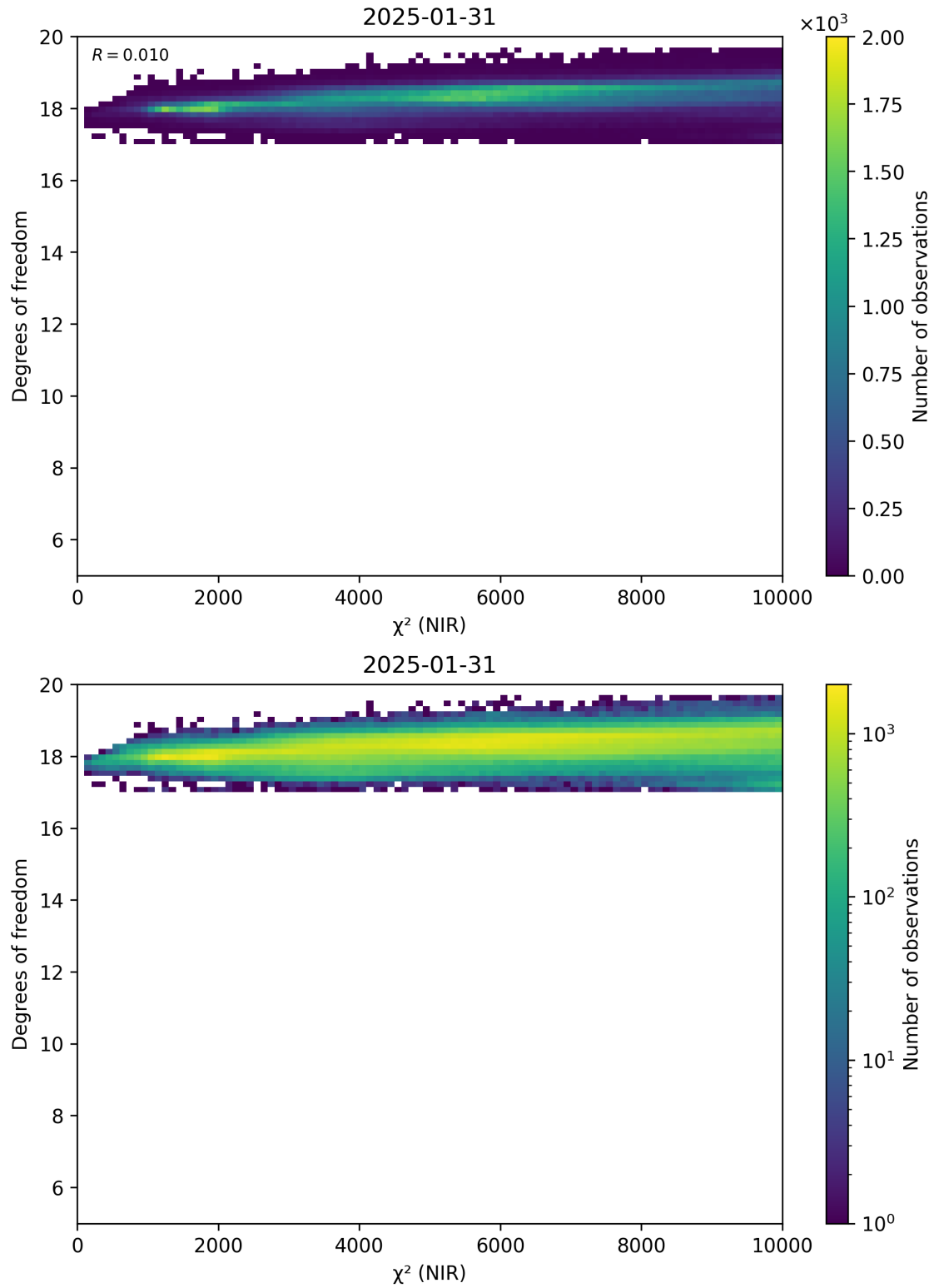
Figure 44: Scatter density plot of “ \chi^2 (NIR)” against “Degrees of freedom” for 2025-01-30 to 2025-02-01.
