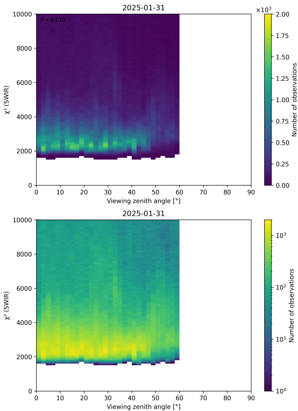
Figure 106: Scatter density plot of “Viewing zenith angle” against “ \chi^2 (SWIR)” for 2025-01-30 to 2025-02-01.
