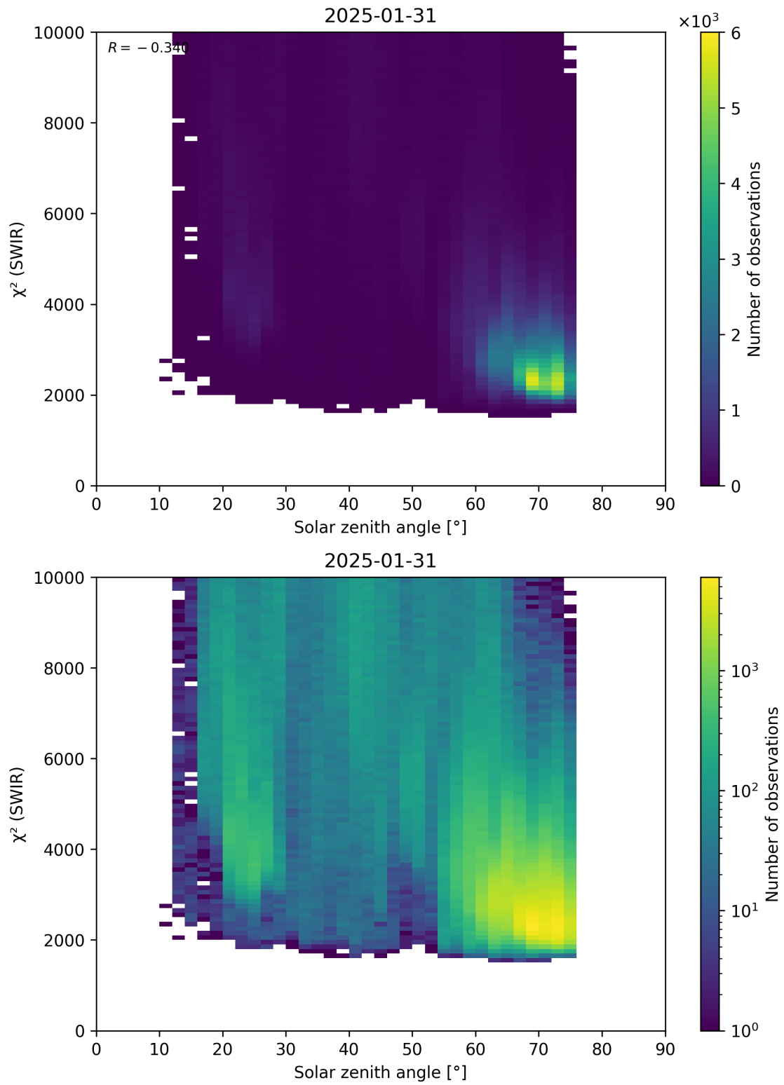
Figure 95: Scatter density plot of “Solar zenith angle” against “ \chi^2 (SWIR)” for 2025-01-30 to 2025-02-01.
