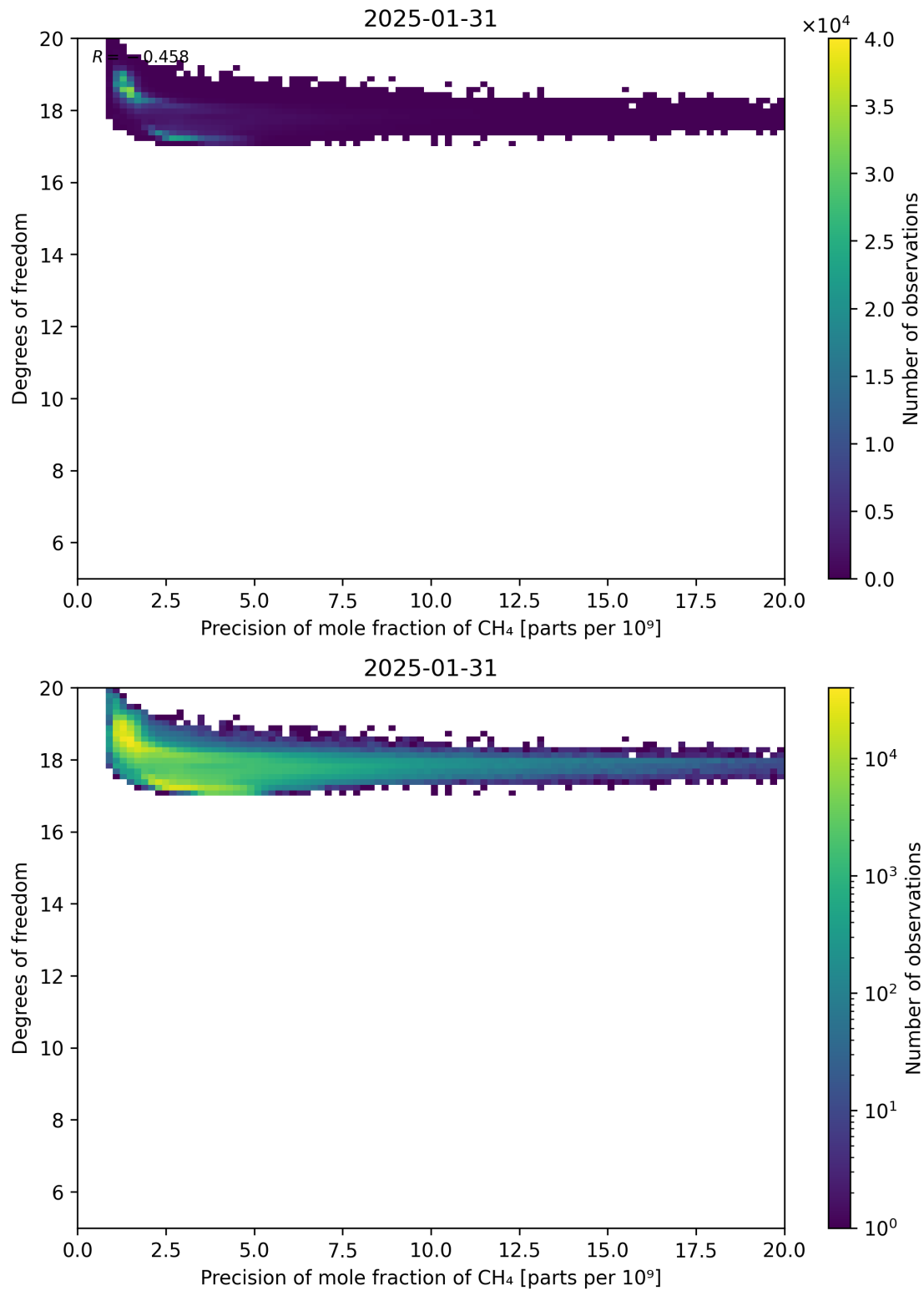
Figure 80: Scatter density plot of “Precision of mole fraction of CH 4 ” against “Degrees of freedom” for 2025-01-30 to 2025-02-01.
