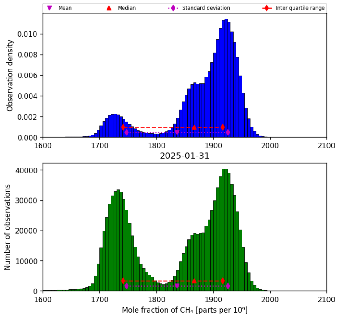
Figure 23: Histogram of “Mole fraction of CH 4 ” for 2025-01-30 to 2025-02-01
