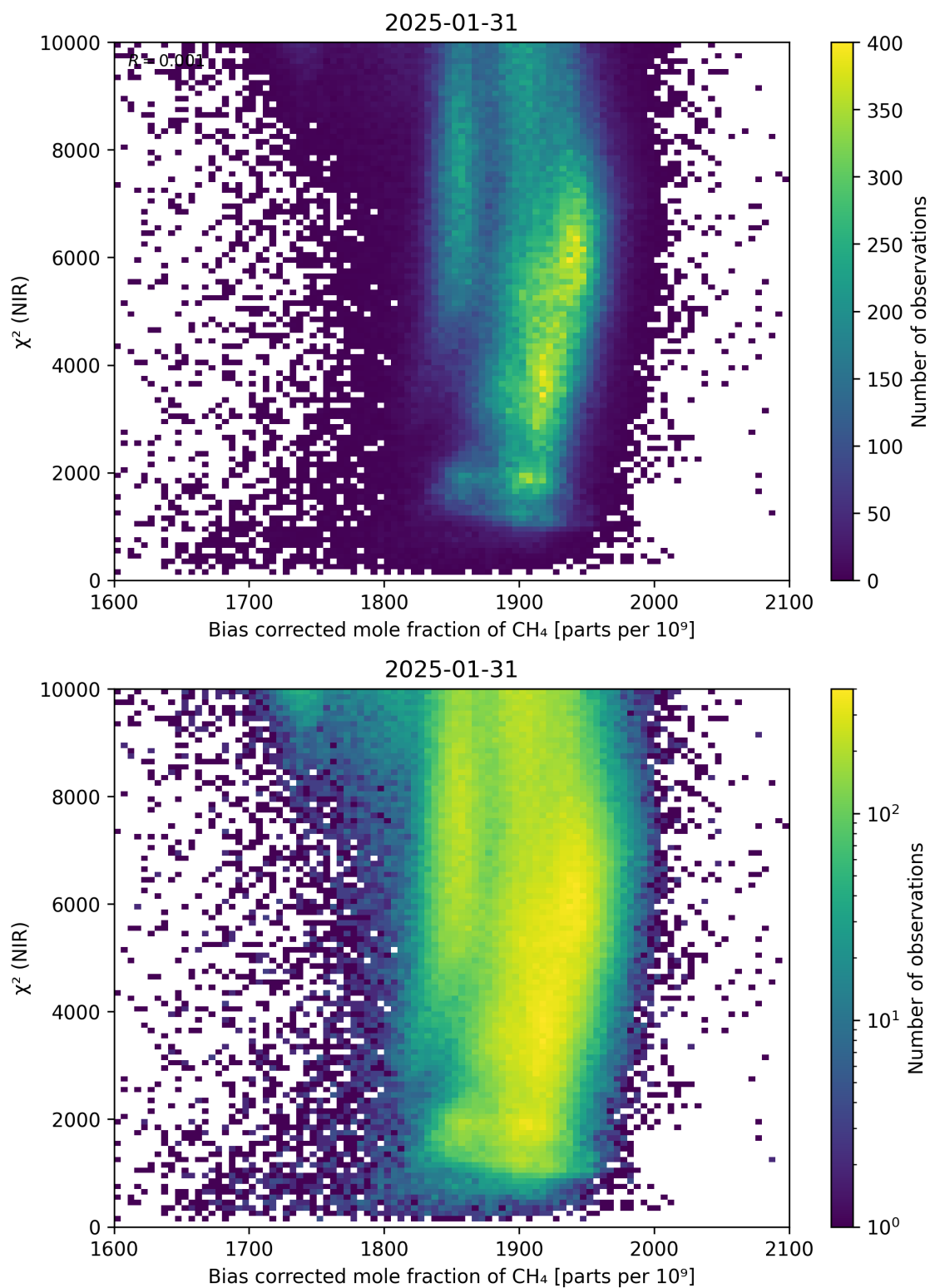
Figure 63: Scatter density plot of “Bias corrected mole fraction of \text{CH}_4 ” against “ \chi^2 (NIR)” for 2025-01-30 to 2025-02-01.
