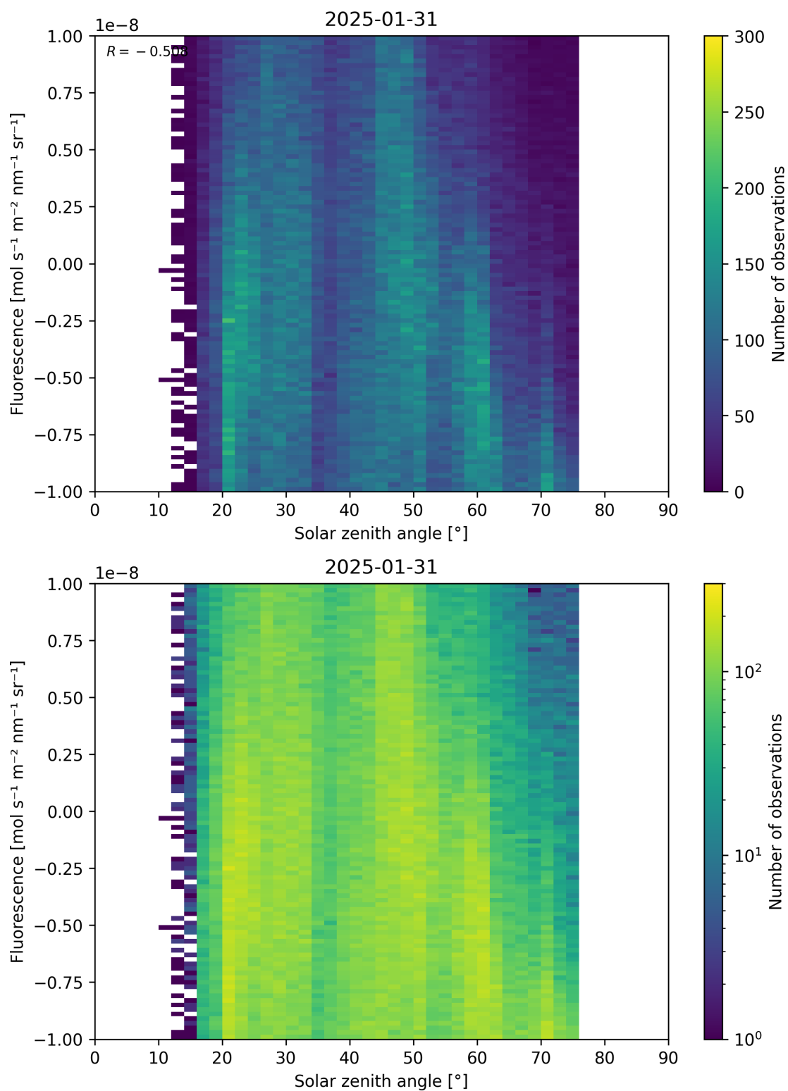
Figure 97: Scatter density plot of “Solar zenith angle” against “Fluorescence” for 2025-01-30 to 2025-02-01.
