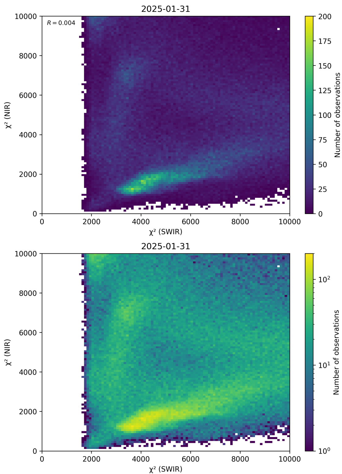
Figure 47: Scatter density plot of “ \chi^2 (SWIR)” against “ \chi^2 (NIR)” for 2025-01-30 to 2025-02-01.
