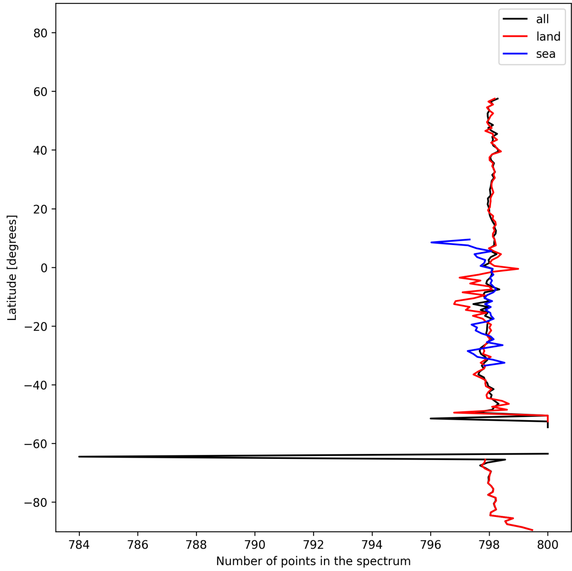
Figure 15: Zonal average of “Number of points in the spectrum” for 2025-01-30 to 2025-02-01.
