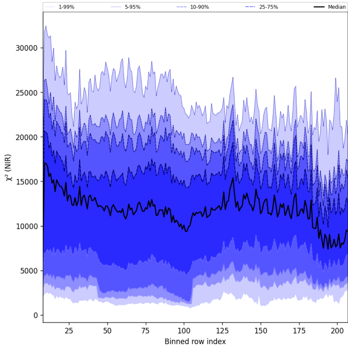
Figure 40: Along track statistics of “ \chi^2 (NIR)” for 2025-01-30 to 2025-02-01
