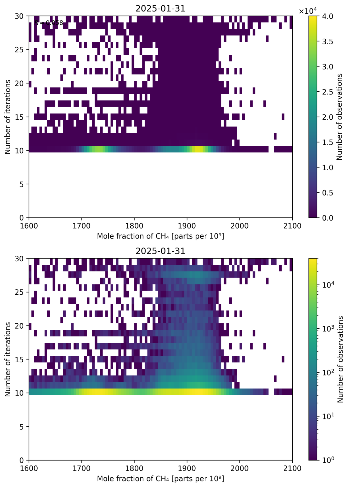
Figure 76: Scatter density plot of “Mole fraction of CH 4 ” against “Number of iterations” for 2025-01-30 to 2025-02-01.
