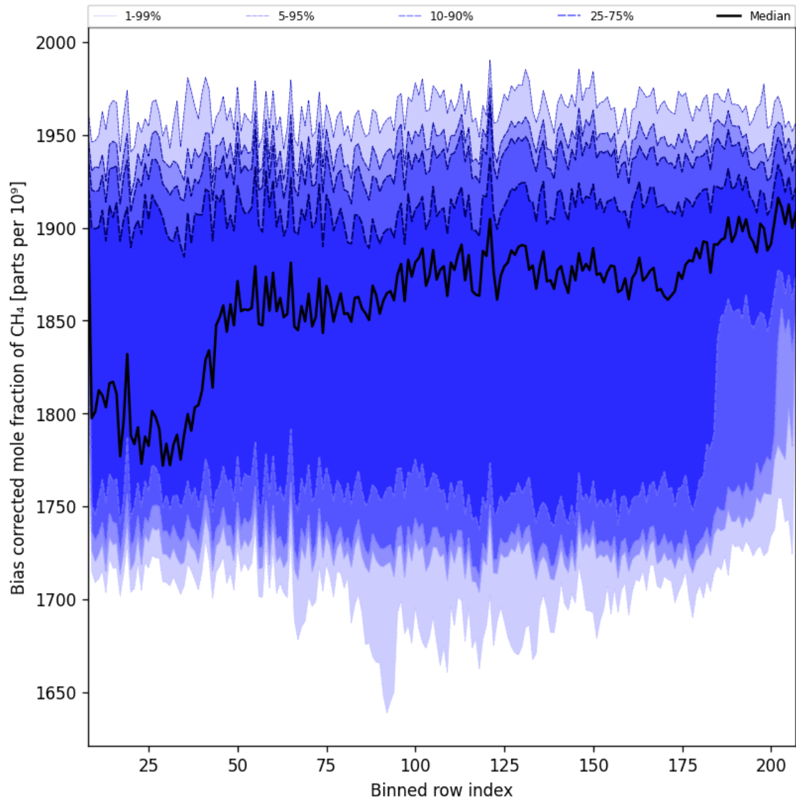
Figure 36: Along track statistics of “Bias corrected mole fraction of CH 4 ” for 2025-01-30 to 2025-02-01
