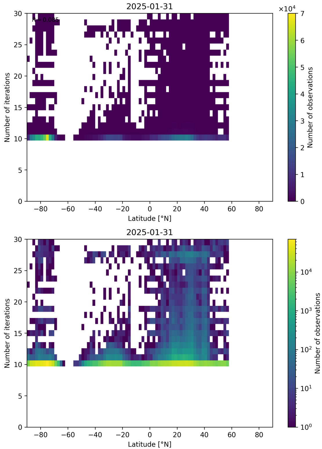
Figure 60: Scatter density plot of “Latitude” against “Number of iterations” for 2025-01-30 to 2025-02-01.
