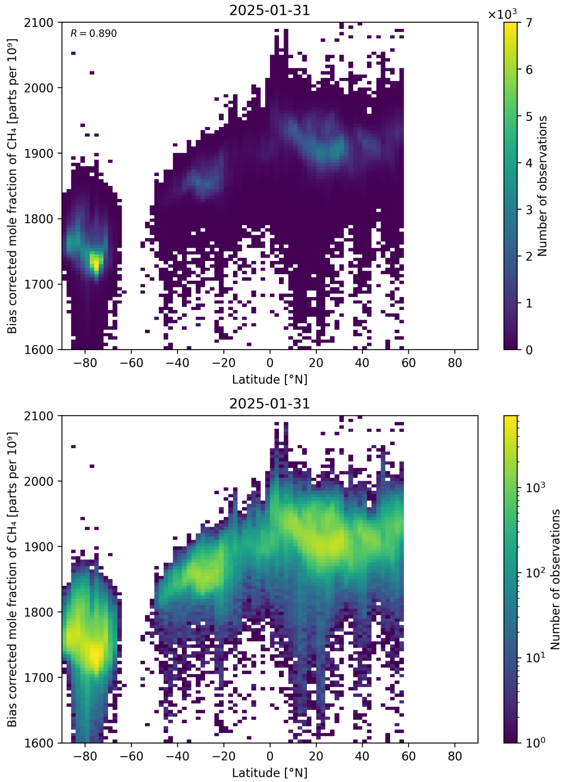
Figure 58: Scatter density plot of “Latitude” against “Bias corrected mole fraction of CH 4 ” for 2025-01-30 to 2025-02-01.
