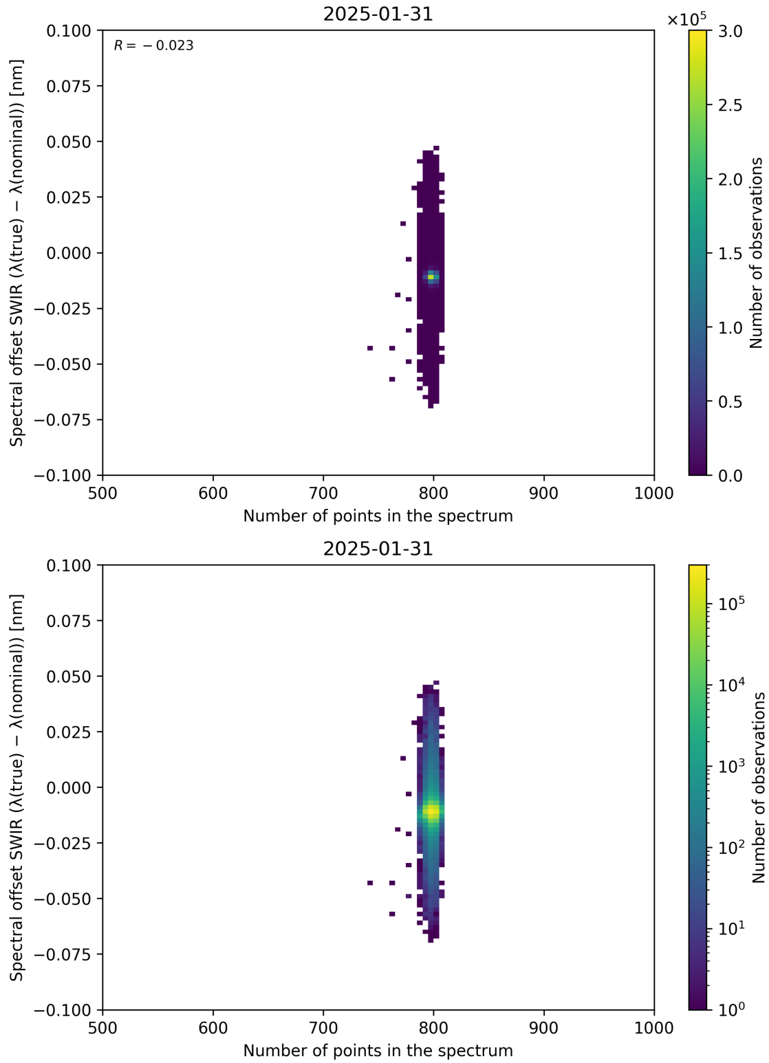
Figure 93: Scatter density plot of “Number of points in the spectrum” against “Spectral offset SWIR ( \lambda_{\text{true}} - \lambda_{\text{nominal}} )” for 2025-01-30 to 2025-02-01.
