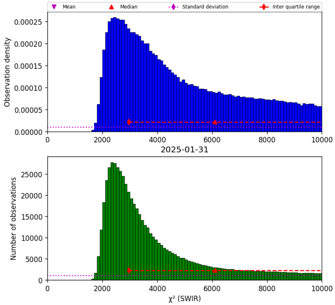
Figure 28: Histogram of “ \chi^2 (SWIR)” for 2025-01-30 to 2025-02-01
