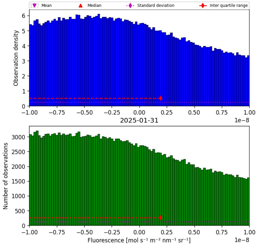
Figure 32: Histogram of “Fluorescence” for 2025-01-30 to 2025-02-01
