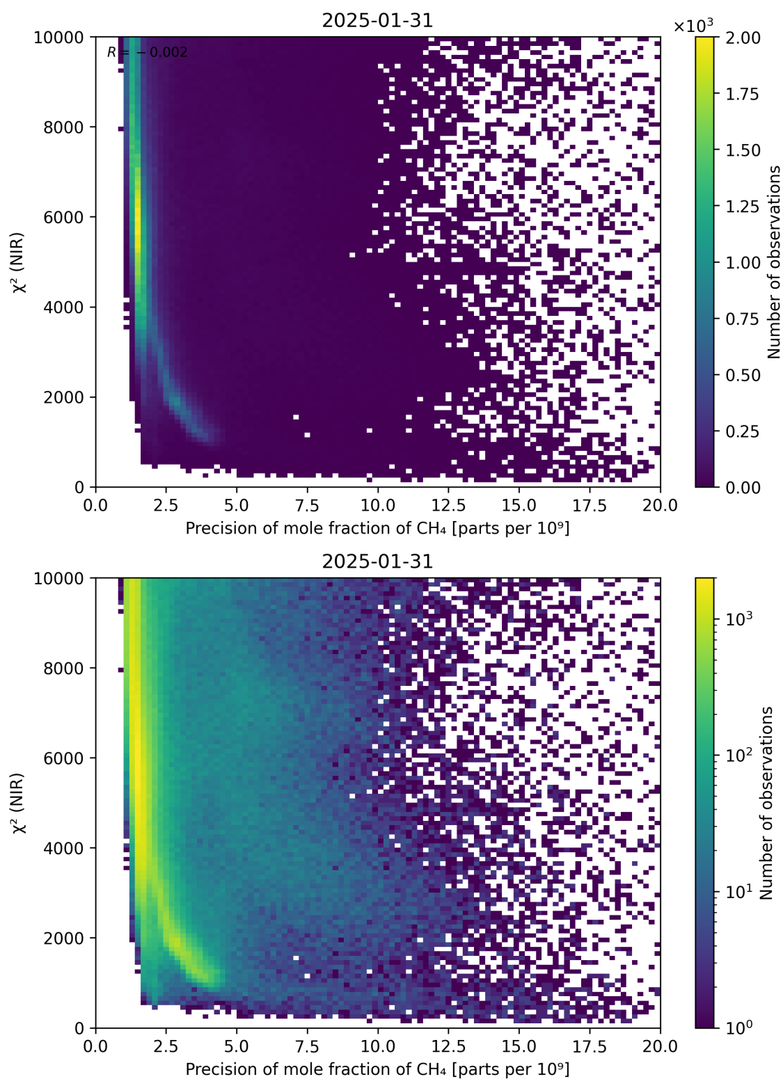
Figure 78: Scatter density plot of “Precision of mole fraction of CH 4 ” against “ \chi^2 (NIR)” for 2025-01-30 to 2025-02-01.
