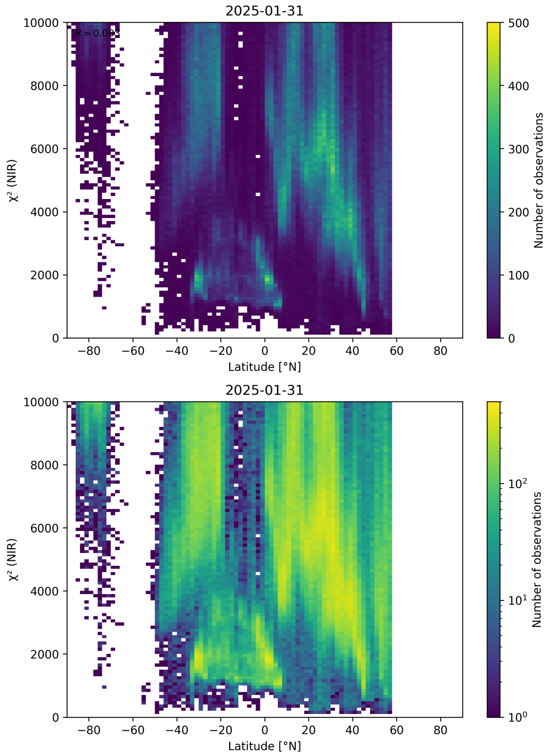
Figure 53: Scatter density plot of “Latitude” against “ \chi^2 (NIR)” for 2025-01-30 to 2025-02-01.
