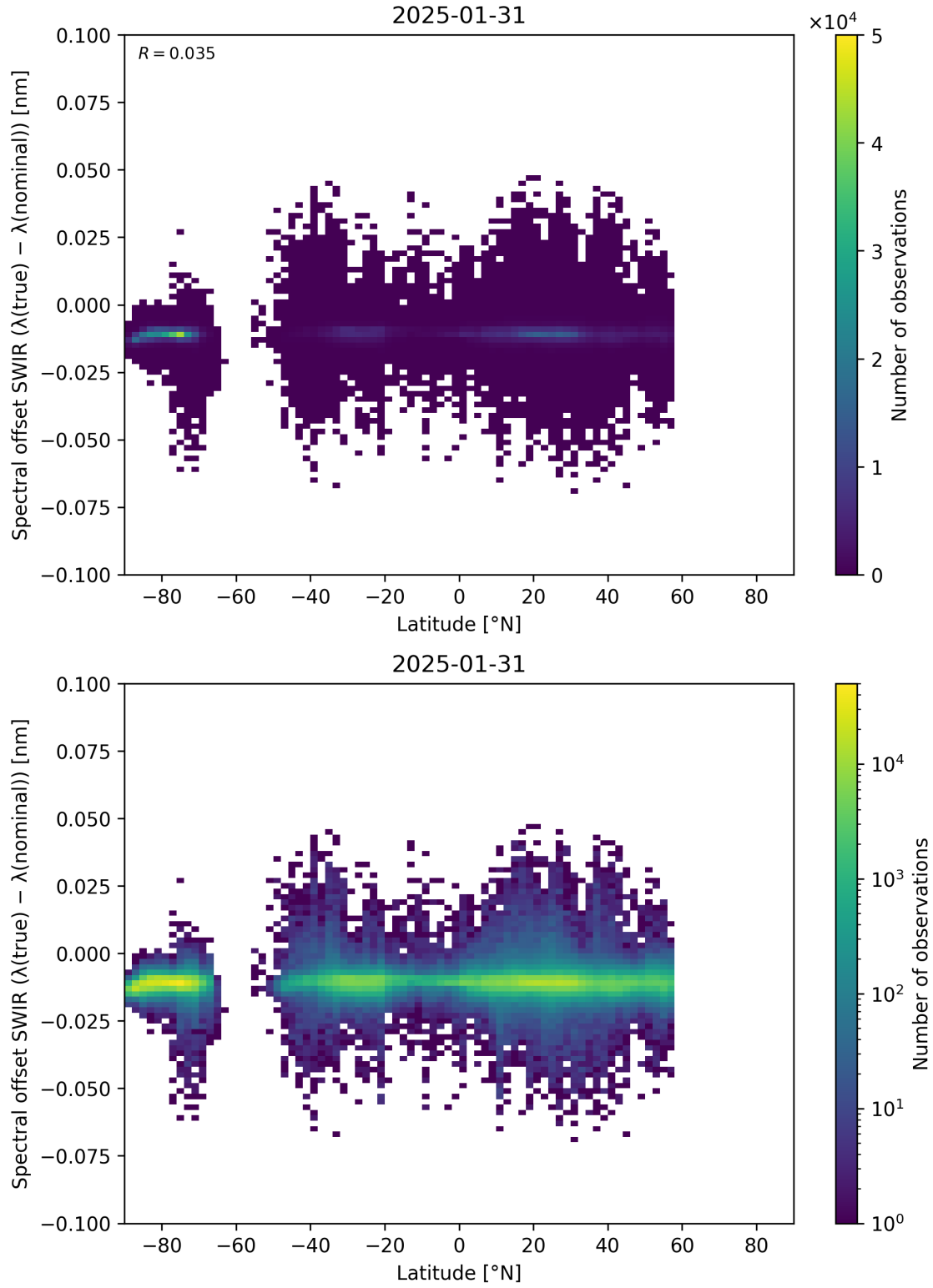
Figure 62: Scatter density plot of “Latitude” against “Spectral offset SWIR ( \lambda_{\text{true}} - \lambda_{\text{nominal}} )” for 2025-01-30 to 2025-02-01.
