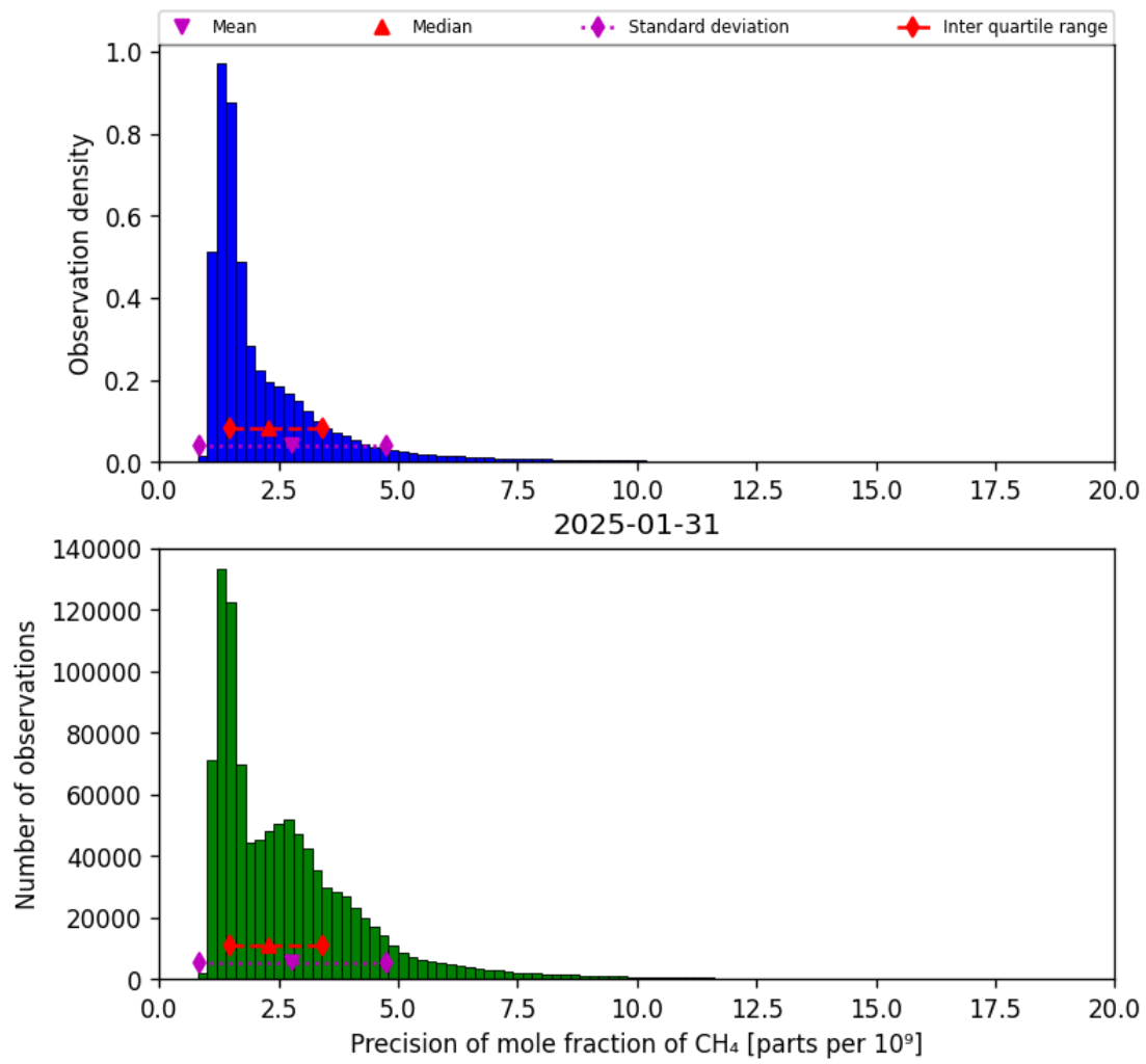
Figure 24: Histogram of “Precision of mole fraction of CH 4 ” for 2025-01-30 to 2025-02-01
