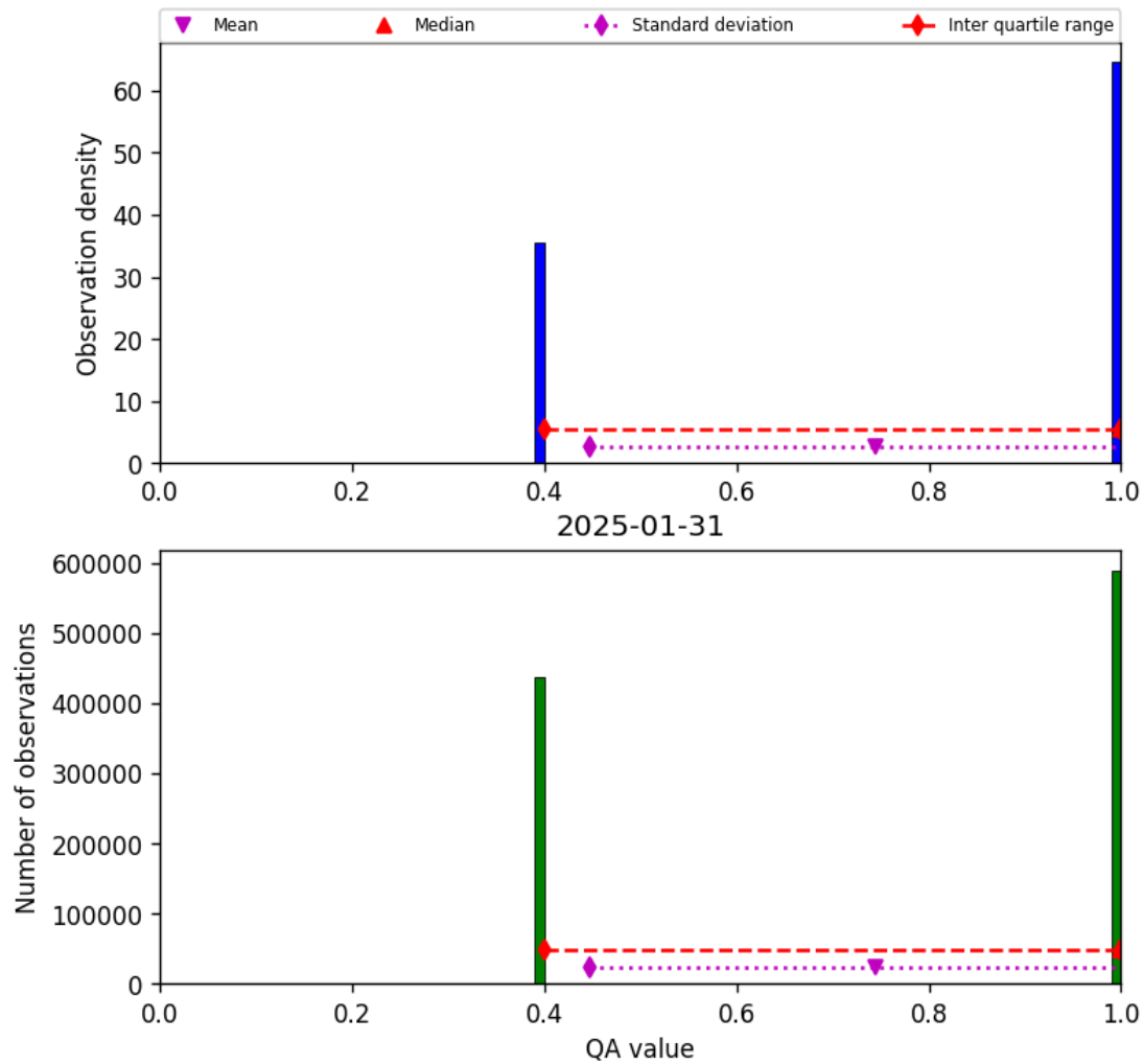
Figure 22: Histogram of “QA value” for 2025-01-30 to 2025-02-01
