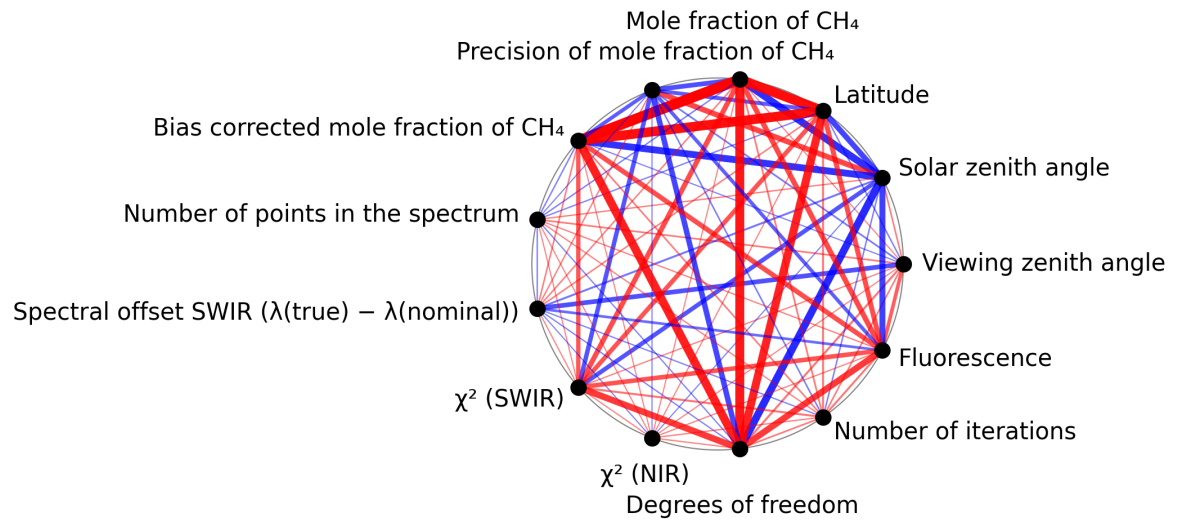
Figure 1: Map of correlation graph for 2025-01-30 to 2025-02-01.
