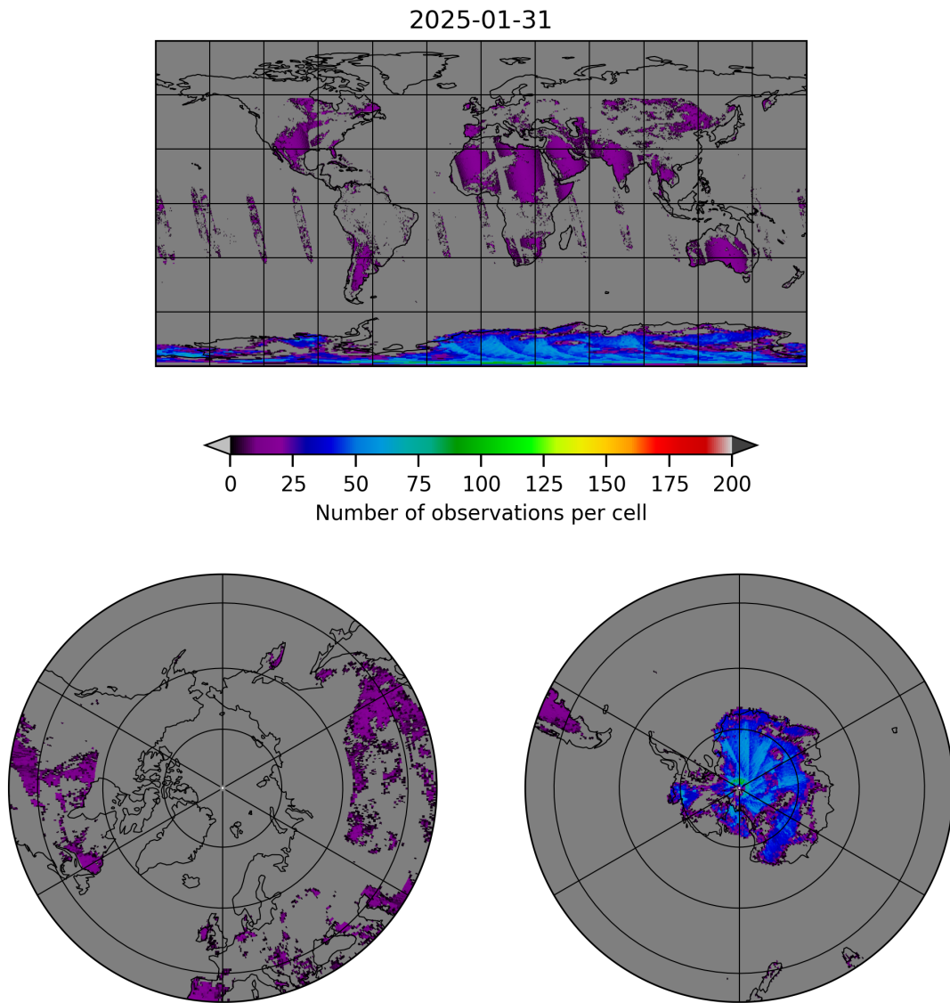
Figure 10: Map of the number of observations for 2025-01-30 to 2025-02-01
