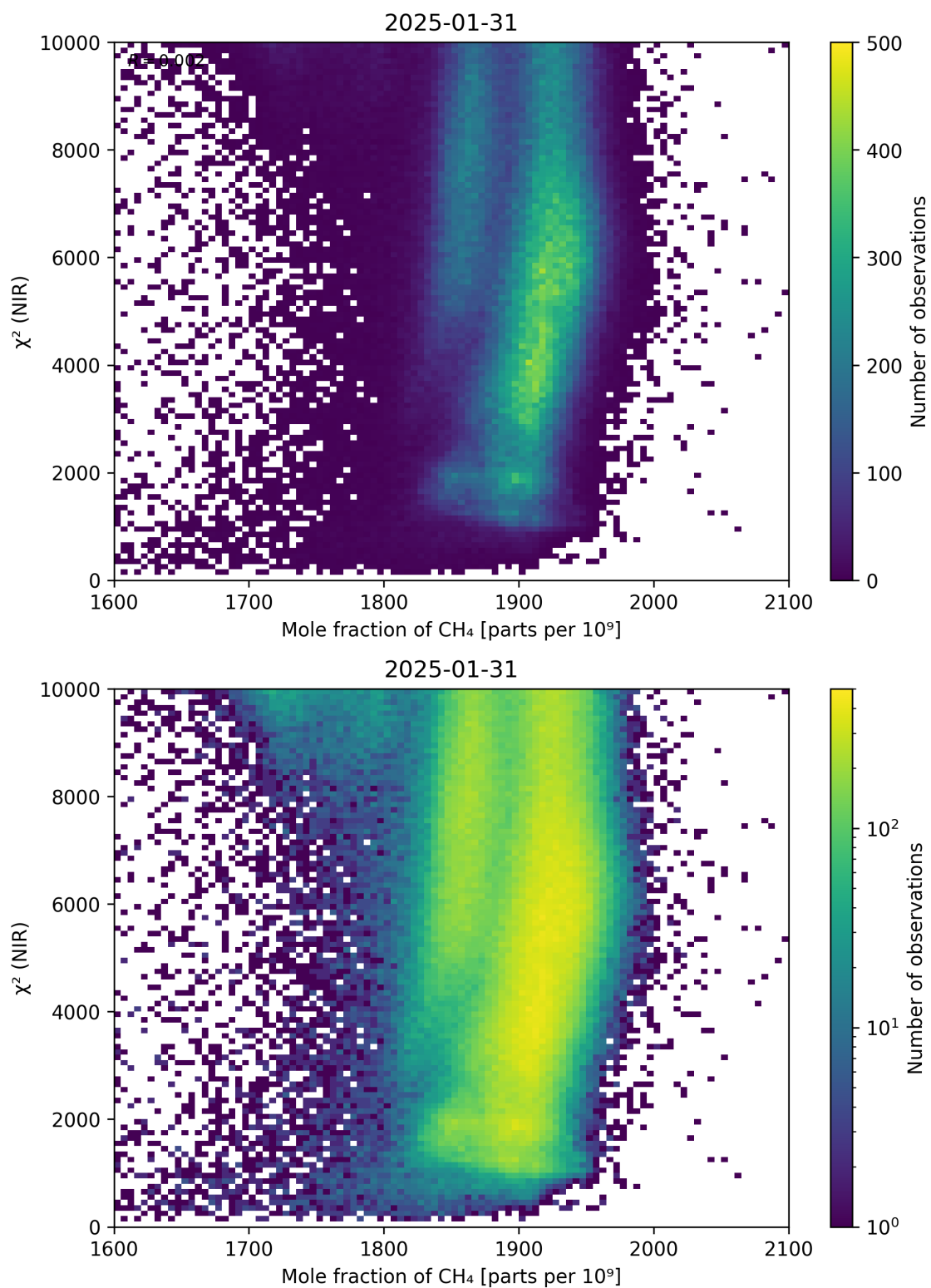
Figure 70: Scatter density plot of “Mole fraction of CH 4 ” against “ \chi^2 (NIR)” for 2025-01-30 to 2025-02-01.
