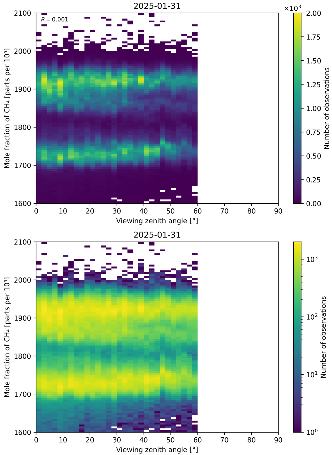
Figure 110: Scatter density plot of “Viewing zenith angle” against “Mole fraction of \text{CH}_4 ” for 2025-01-30 to 2025-02-01.
