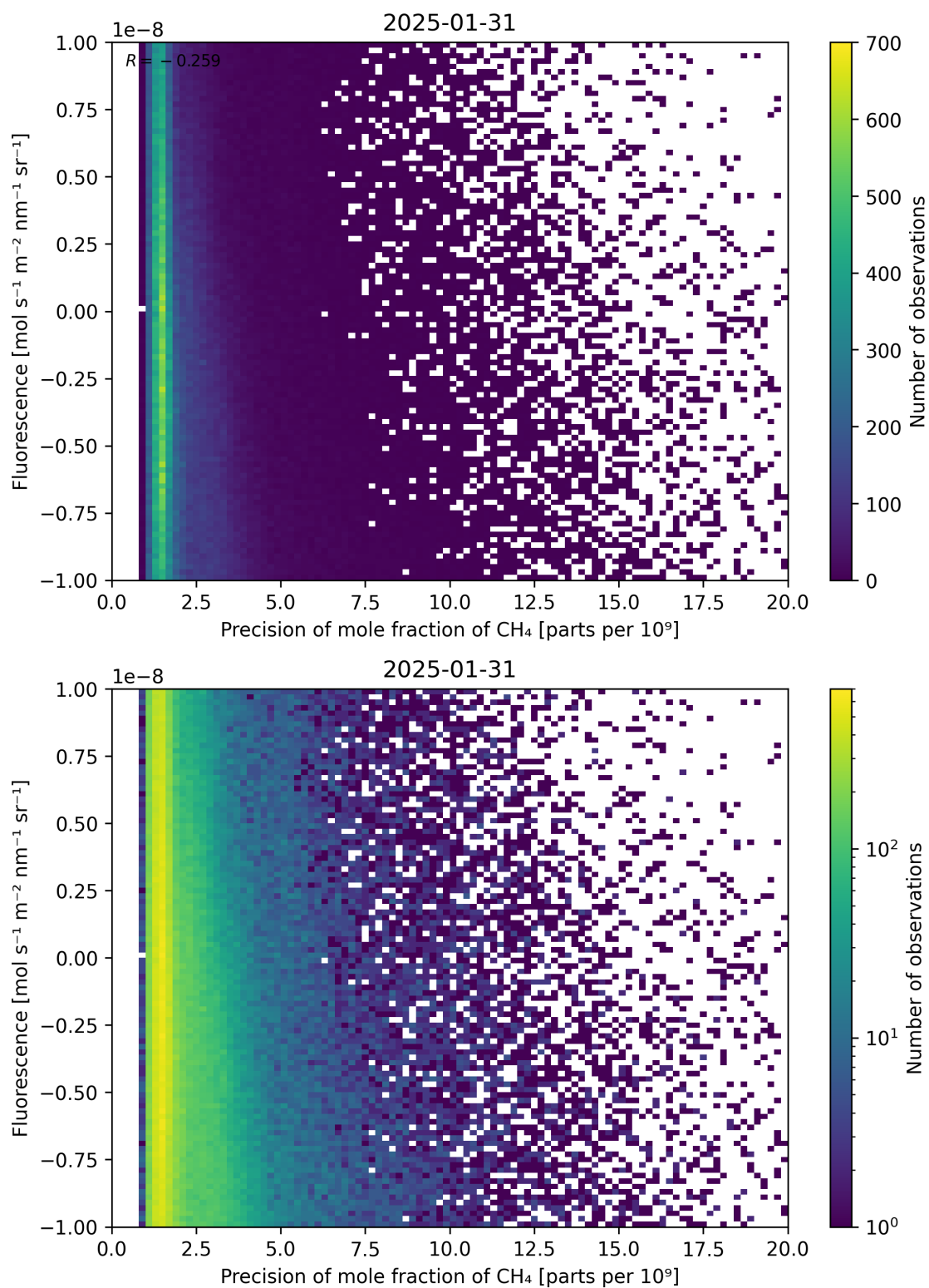
Figure 81: Scatter density plot of “Precision of mole fraction of \text{CH}_4 ” against “Fluorescence” for 2025-01-30 to 2025-02-01.
