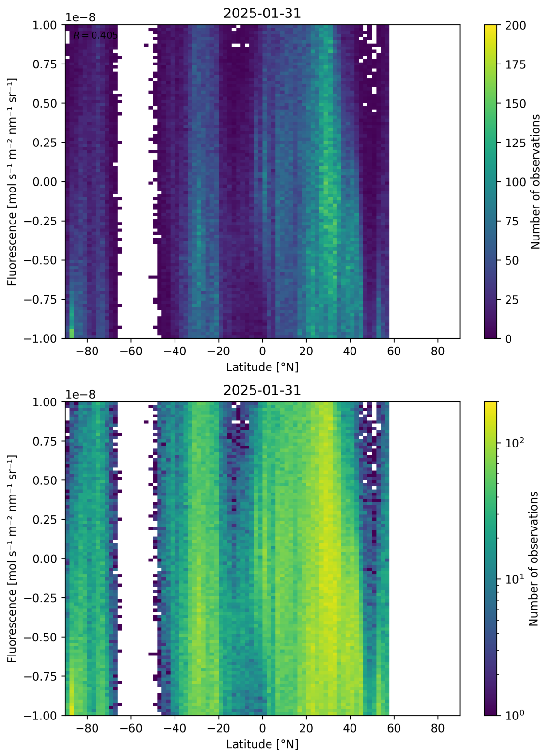
Figure 56: Scatter density plot of “Latitude” against “Fluorescence” for 2025-01-30 to 2025-02-01.
