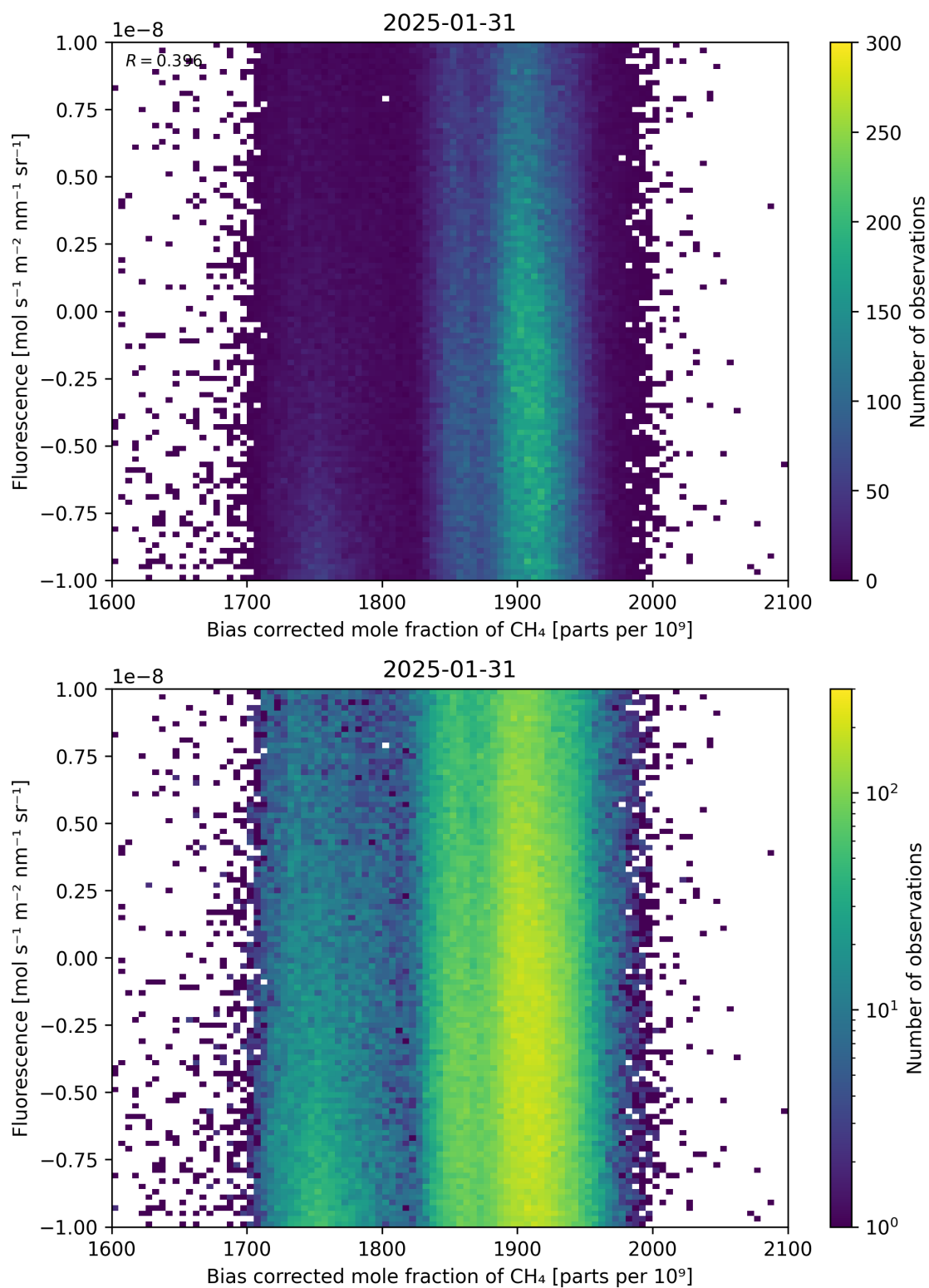
Figure 66: Scatter density plot of “Bias corrected mole fraction of \text{CH}_4 ” against “Fluorescence” for 2025-01-30 to 2025-02-01.
