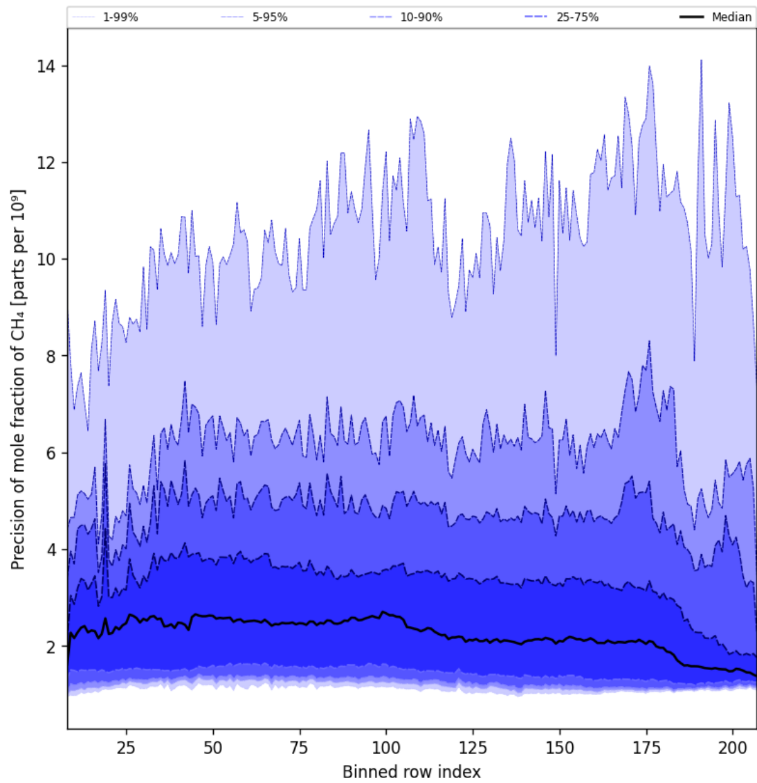
Figure 35: Along track statistics of “Precision of mole fraction of CH 4 ” for 2025-01-30 to 2025-02-01
