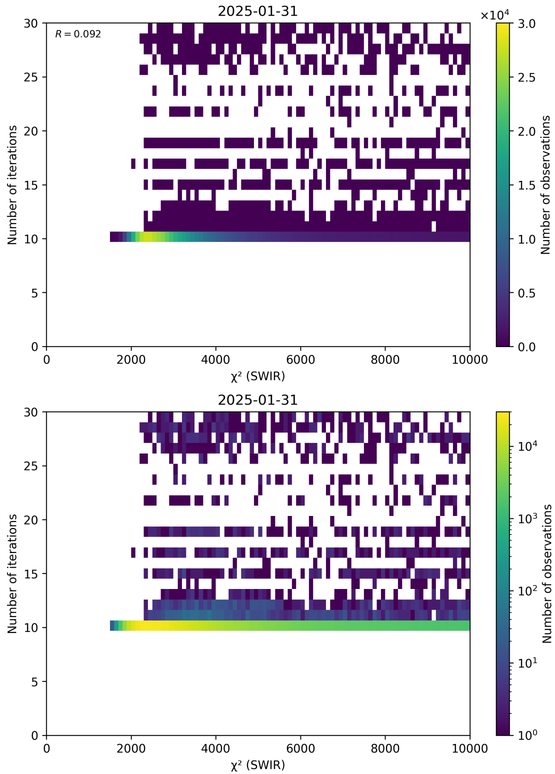
Figure 50: Scatter density plot of “ \chi^2 (SWIR)” against “Number of iterations” for 2025-01-30 to 2025-02-01.
