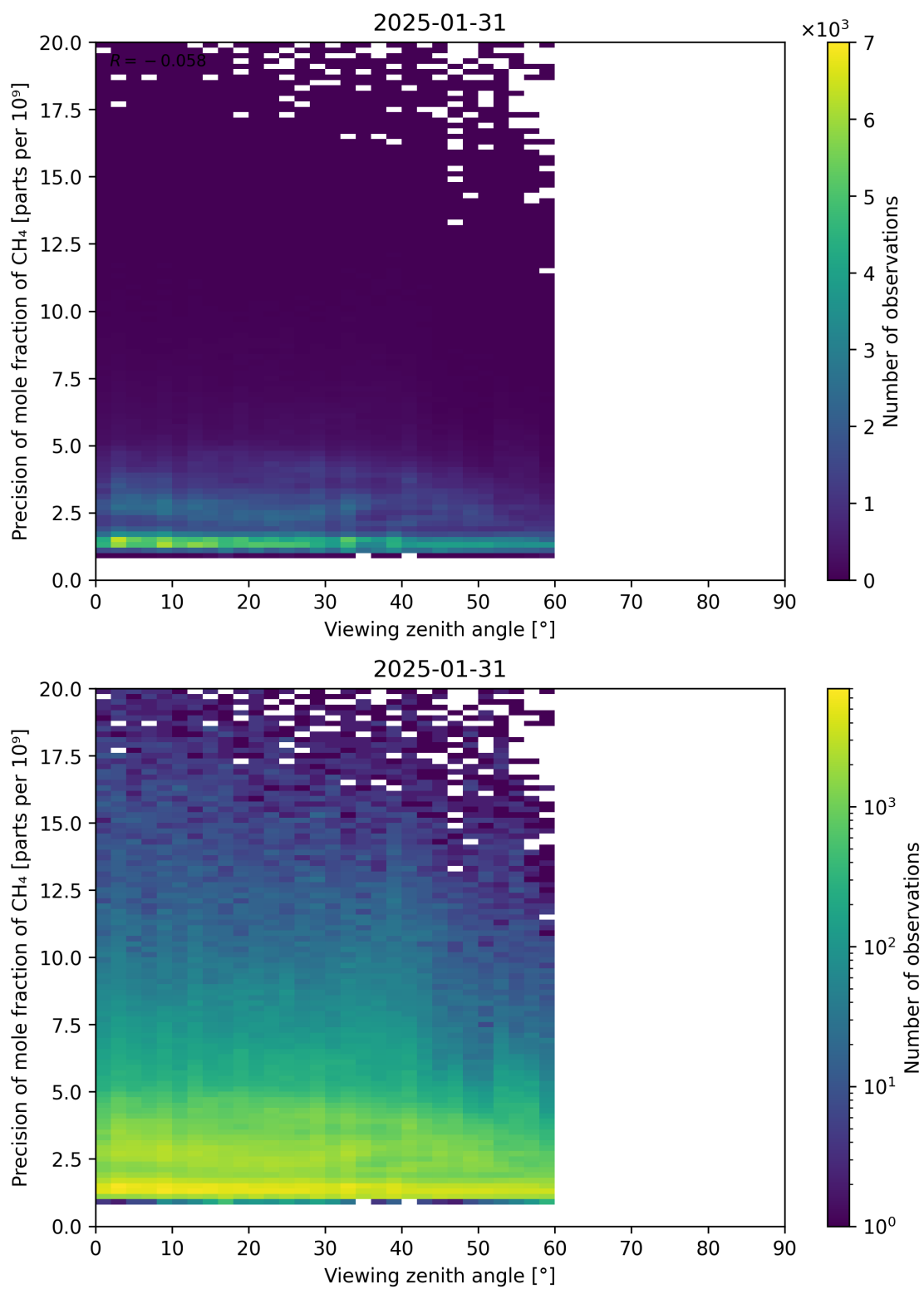
Figure 112: Scatter density plot of “Viewing zenith angle” against “Precision of mole fraction of CH 4 ” for 2025-01-30 to 2025-02-01.
