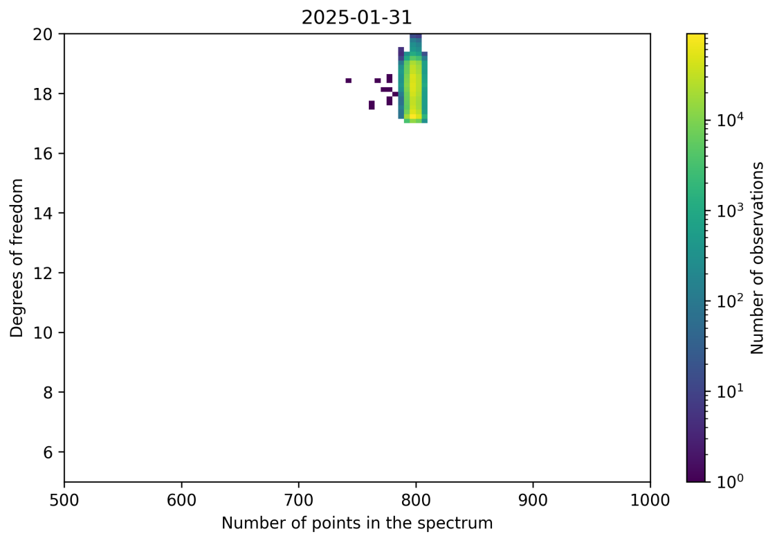
Figure 90: Scatter density plot of “Number of points in the spectrum” against “Degrees of freedom” for 2025-01-30 to 2025-02-01.
