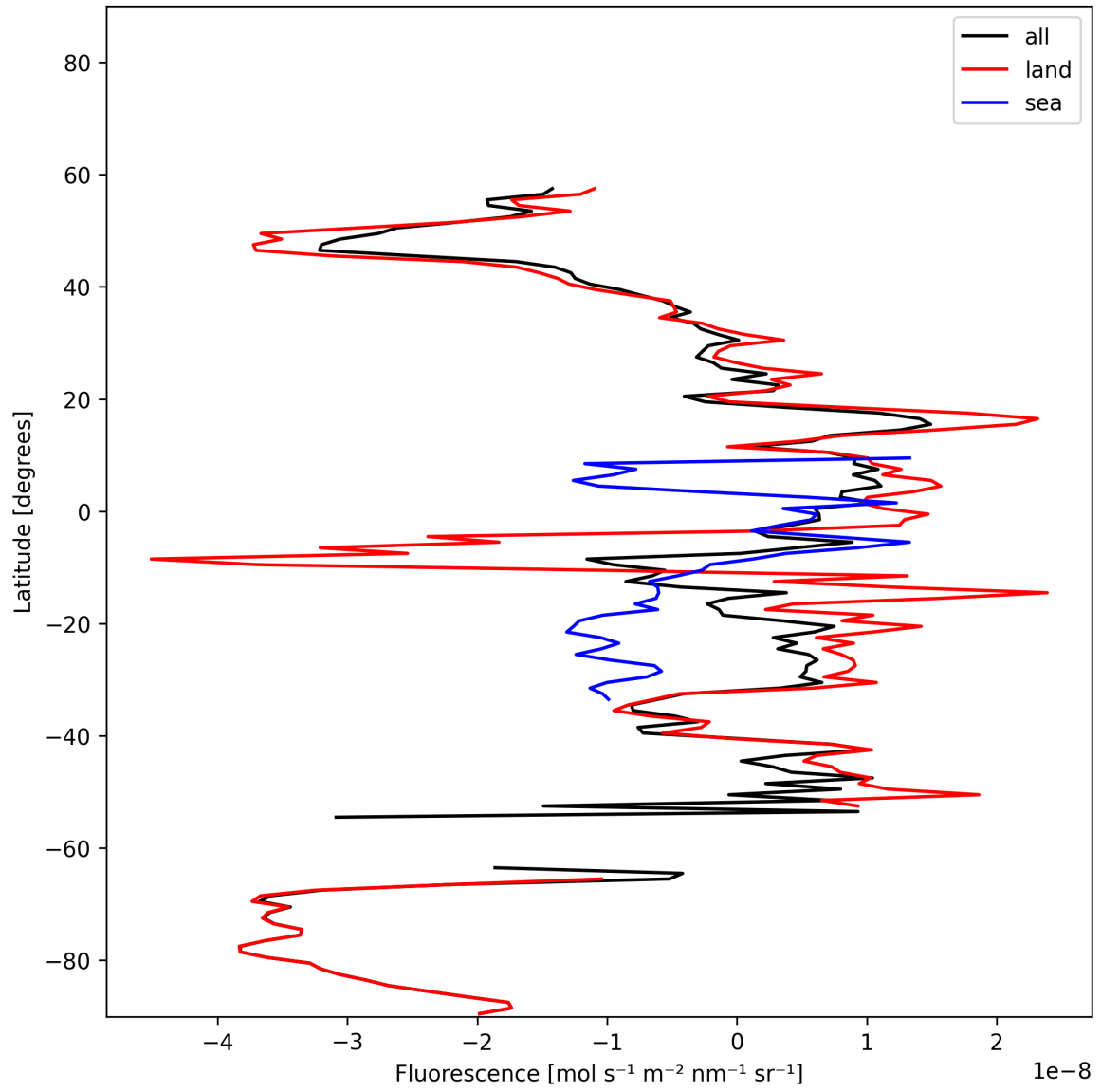
Figure 21: Zonal average of “Fluorescence” for 2025-01-30 to 2025-02-01.
