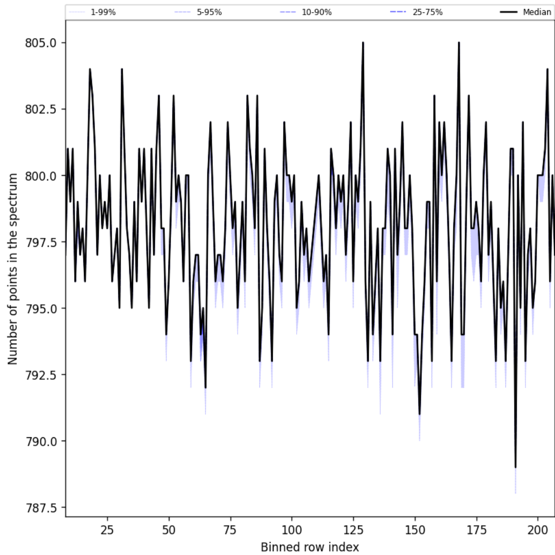
Figure 37: Along track statistics of “Number of points in the spectrum” for 2025-01-30 to 2025-02-01
