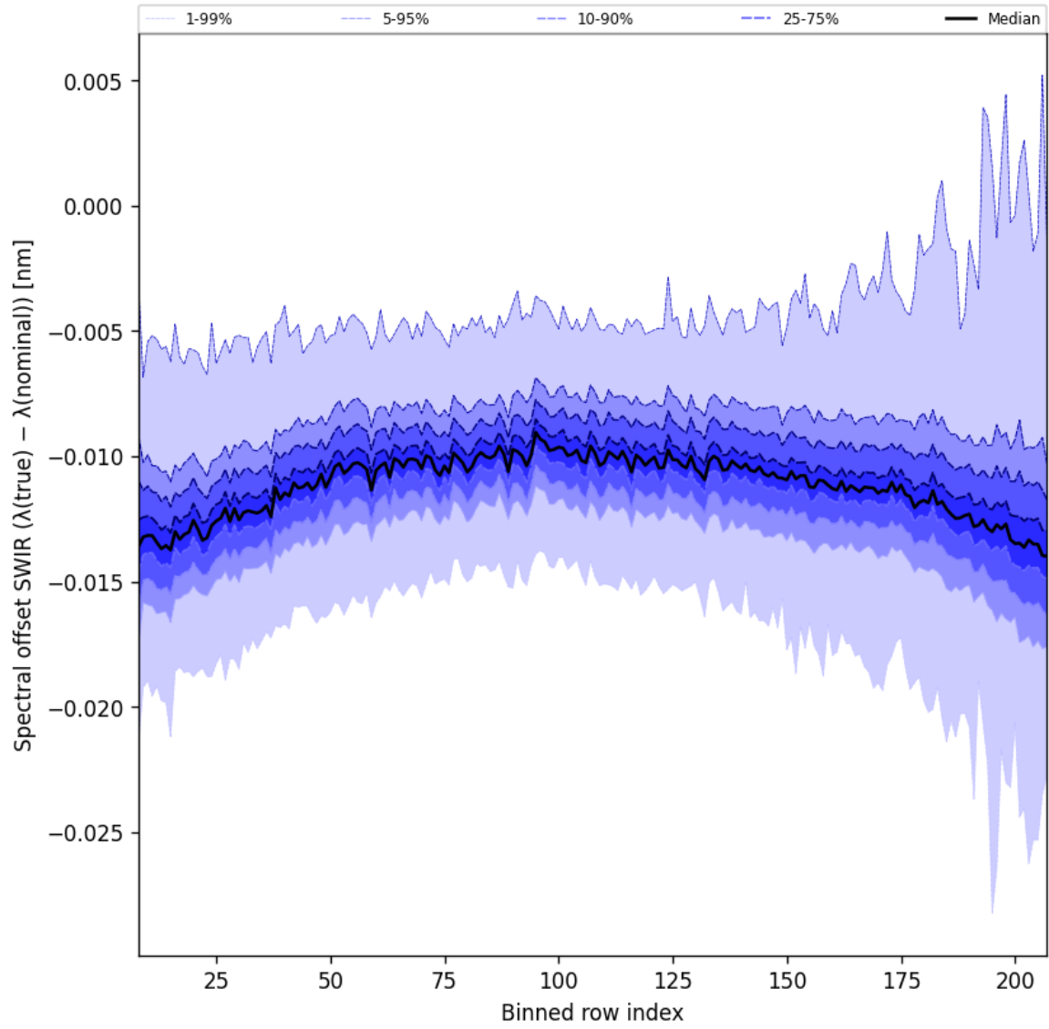
Figure 38: Along track statistics of “Spectral offset SWIR ( \lambda_{\text{true}} - \lambda_{\text{nominal}} )” for 2025-01-30 to 2025-02-01
