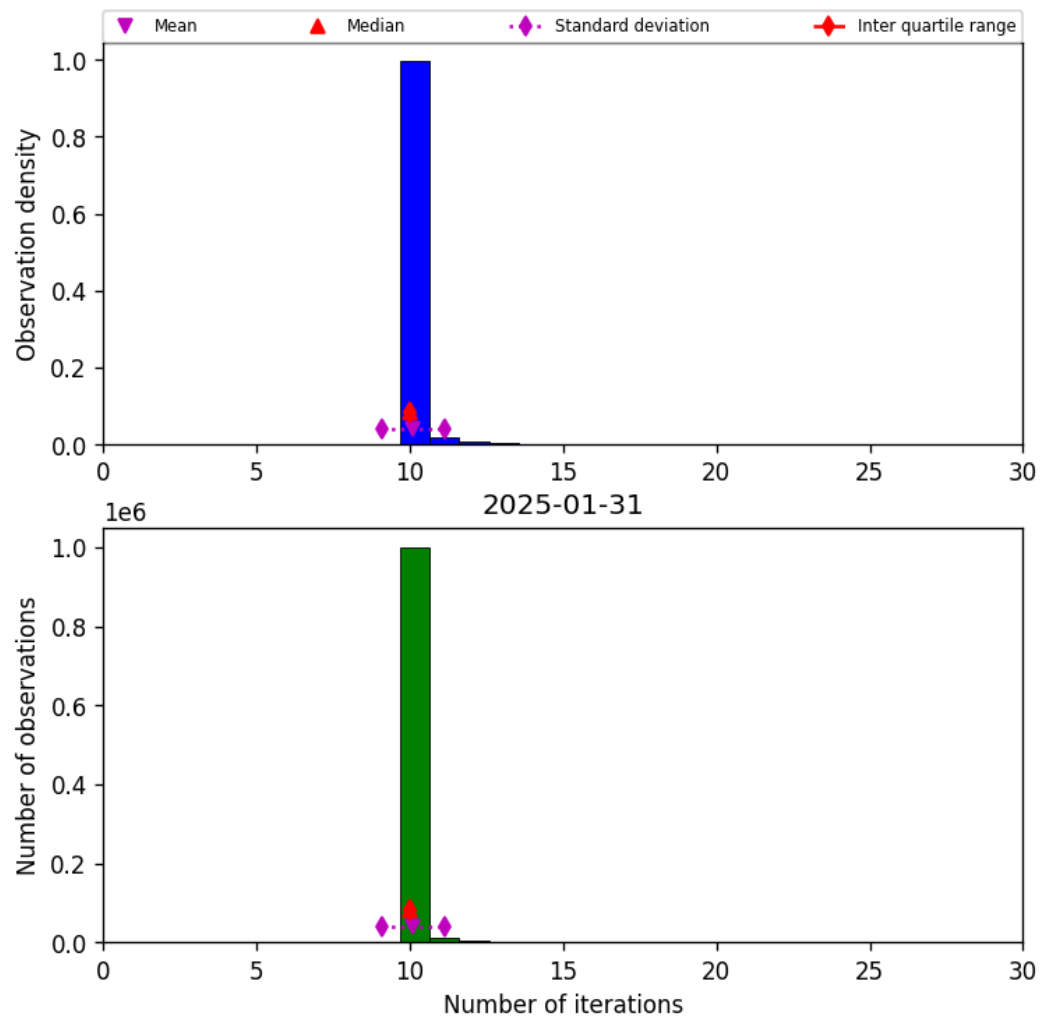
Figure 31: Histogram of “Number of iterations” for 2025-01-30 to 2025-02-01
