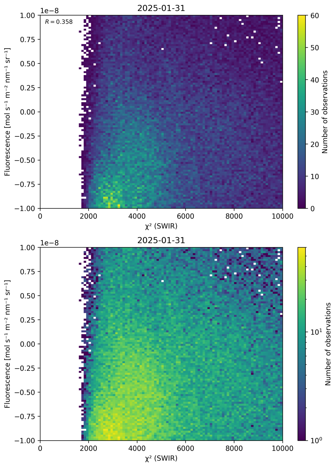
Figure 49: Scatter density plot of “ \chi^2 (SWIR)” against “Fluorescence” for 2025-01-30 to 2025-02-01.
