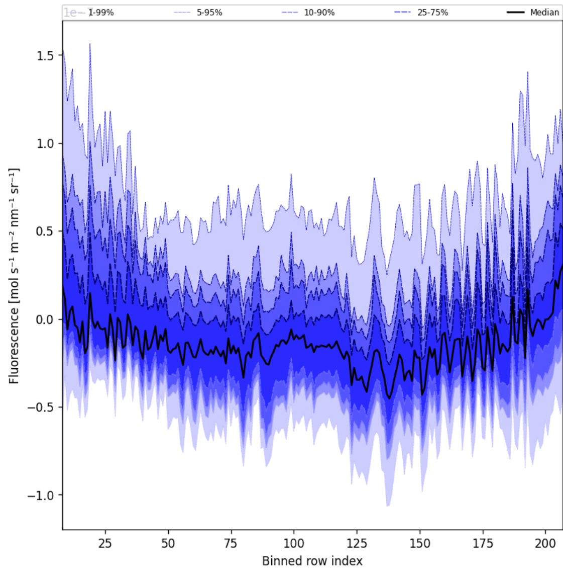
Figure 43: Along track statistics of “Fluorescence” for 2025-01-30 to 2025-02-01
