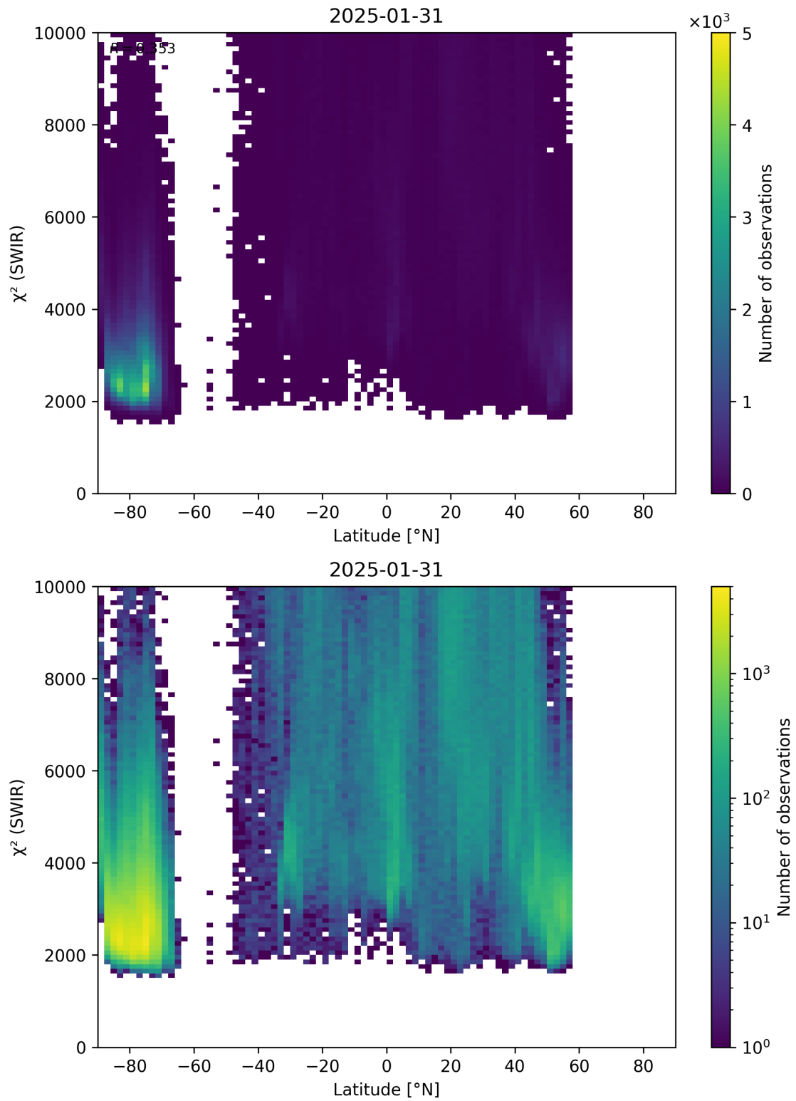
Figure 54: Scatter density plot of “Latitude” against “ \chi^2 (SWIR)” for 2025-01-30 to 2025-02-01.
