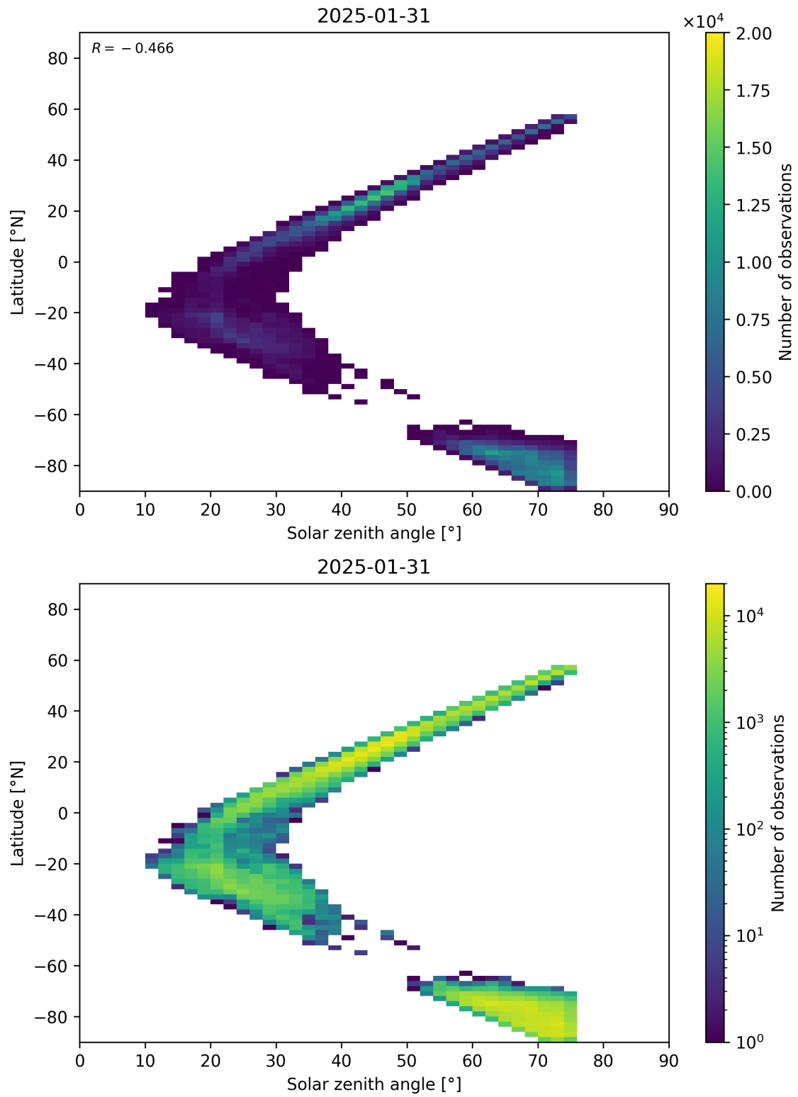
Figure 98: Scatter density plot of “Solar zenith angle” against “Latitude” for 2025-01-30 to 2025-02-01.
