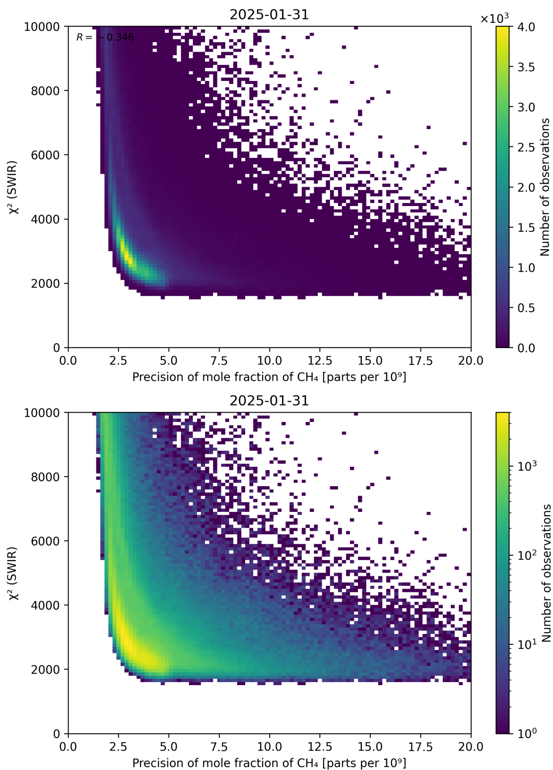
Figure 79: Scatter density plot of “Precision of mole fraction of \text{CH}_4 ” against “ \chi^2 (SWIR)” for 2025-01-30 to 2025-02-01.
