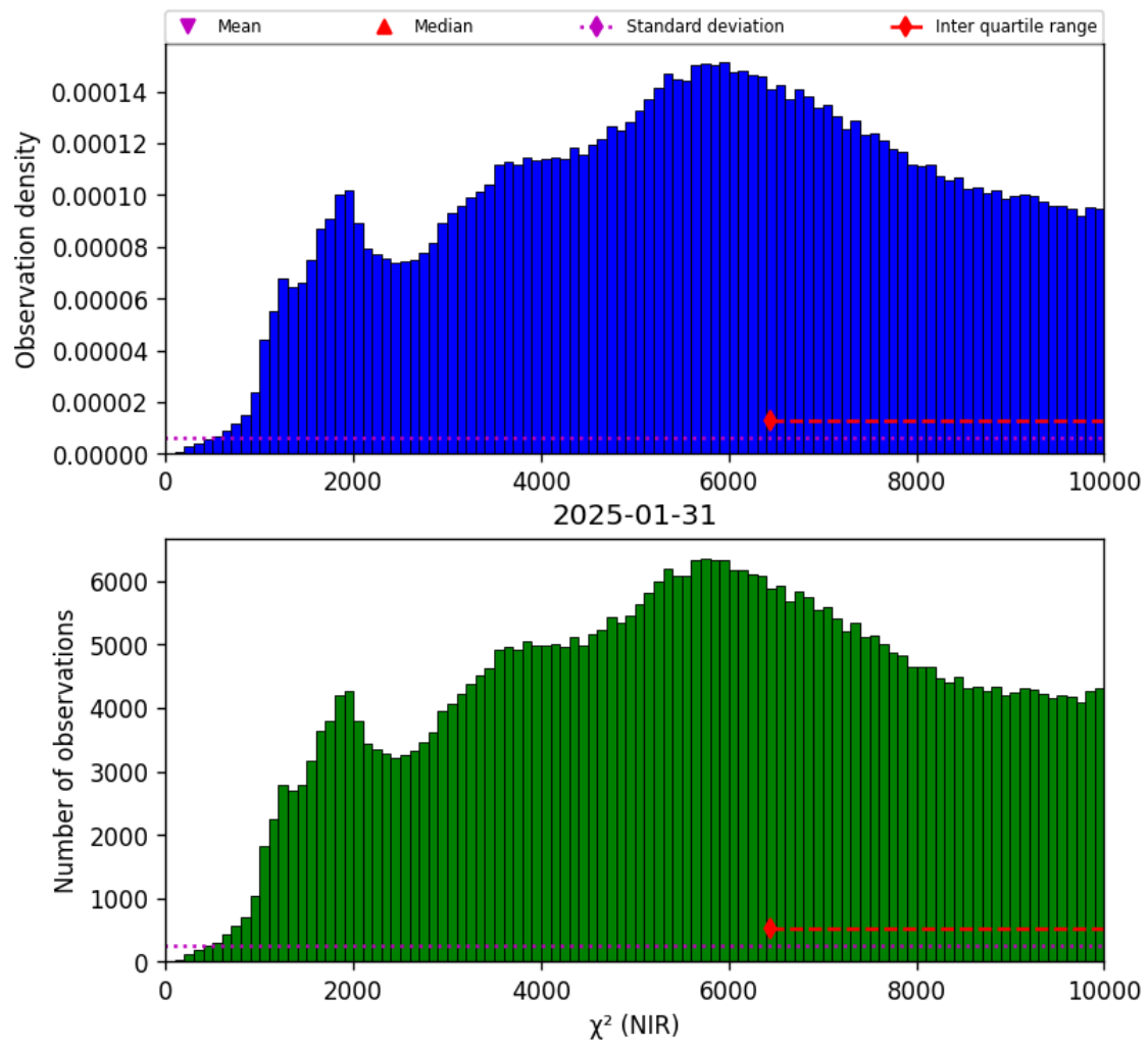
Figure 29: Histogram of “ \chi^2 (NIR)” for 2025-01-30 to 2025-02-01
