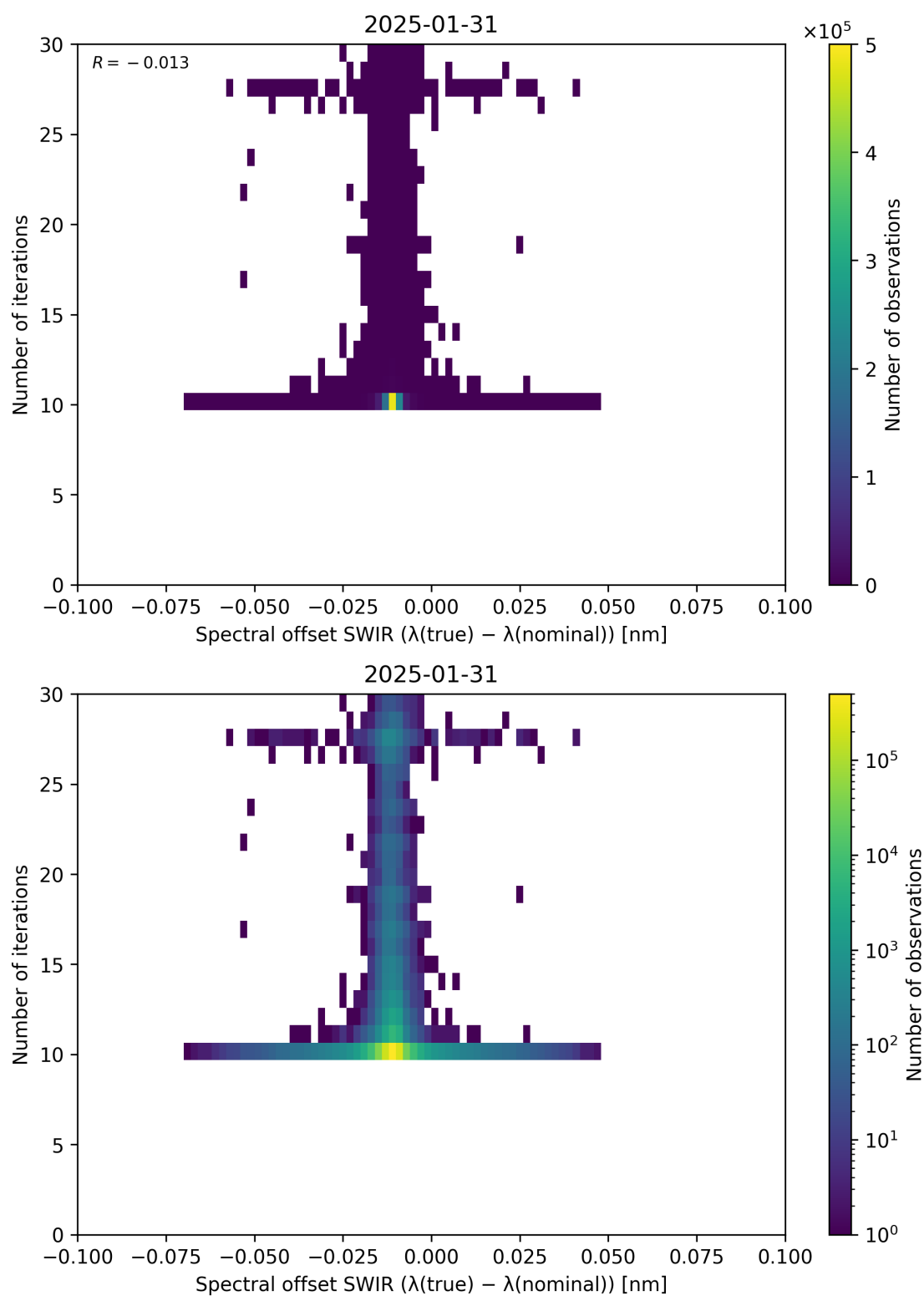
Figure 121: Scatter density plot of “Spectral offset SWIR ( \lambda_{\text{true}} - \lambda_{\text{nominal}} )” against “Number of iterations” for 2025-01-30 to 2025-02-01.
