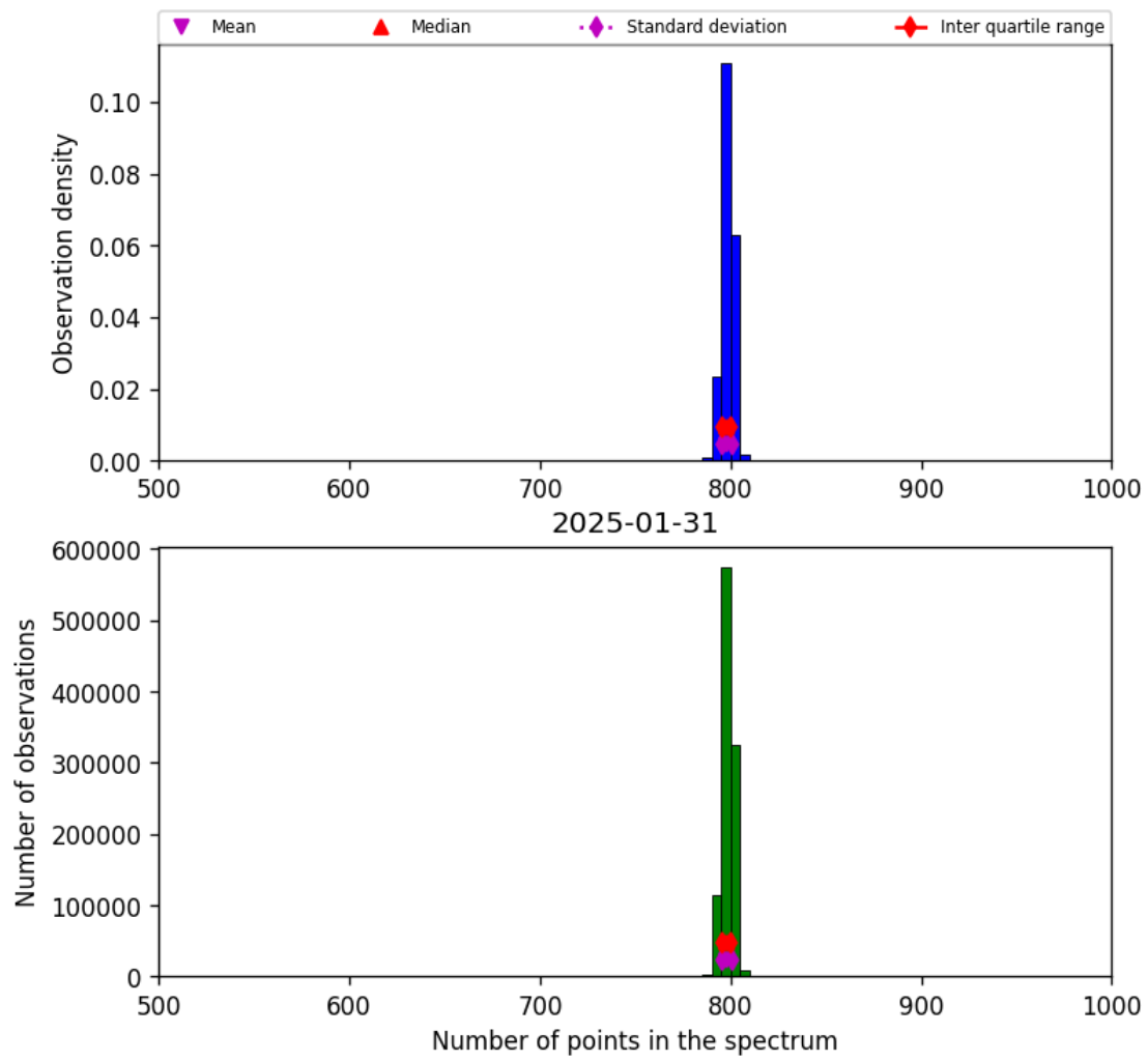
Figure 26: Histogram of “Number of points in the spectrum” for 2025-01-30 to 2025-02-01
