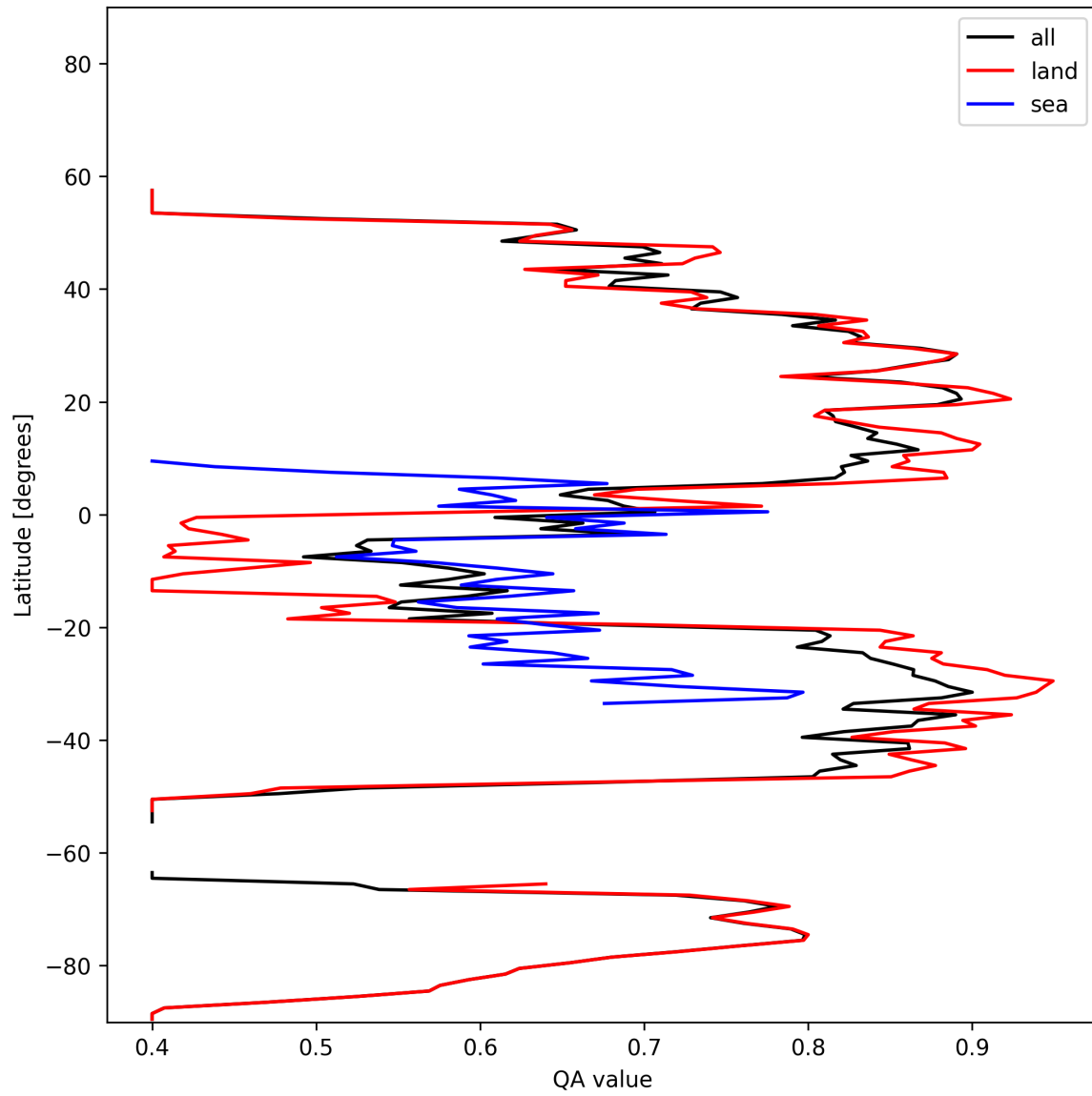
Figure 11: Zonal average of “QA value” for 2025-01-30 to 2025-02-01.
