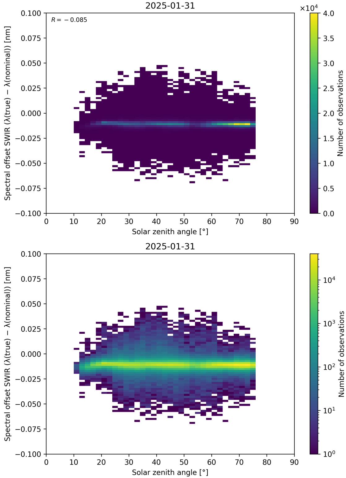
Figure 104: Scatter density plot of “Solar zenith angle” against “Spectral offset SWIR ( \lambda_{\text{true}} - \lambda_{\text{nominal}} )” for 2025-01-30 to 2025-02-01.
