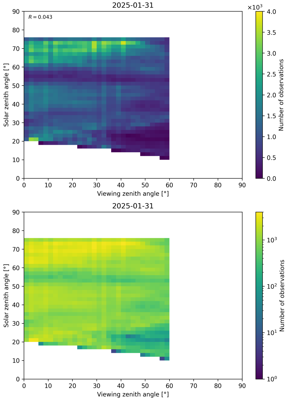
Figure 115: Scatter density plot of “Viewing zenith angle” against “Solar zenith angle” for 2025-01-30 to 2025-02-01.
