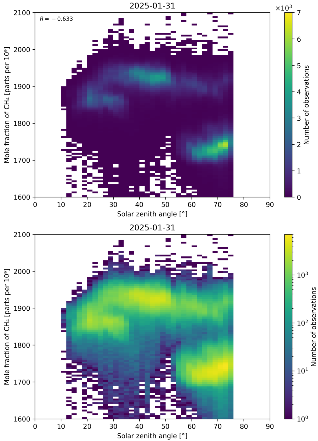
Figure 99: Scatter density plot of “Solar zenith angle” against “Mole fraction of CH 4 ” for 2025-01-30 to 2025-02-01.
