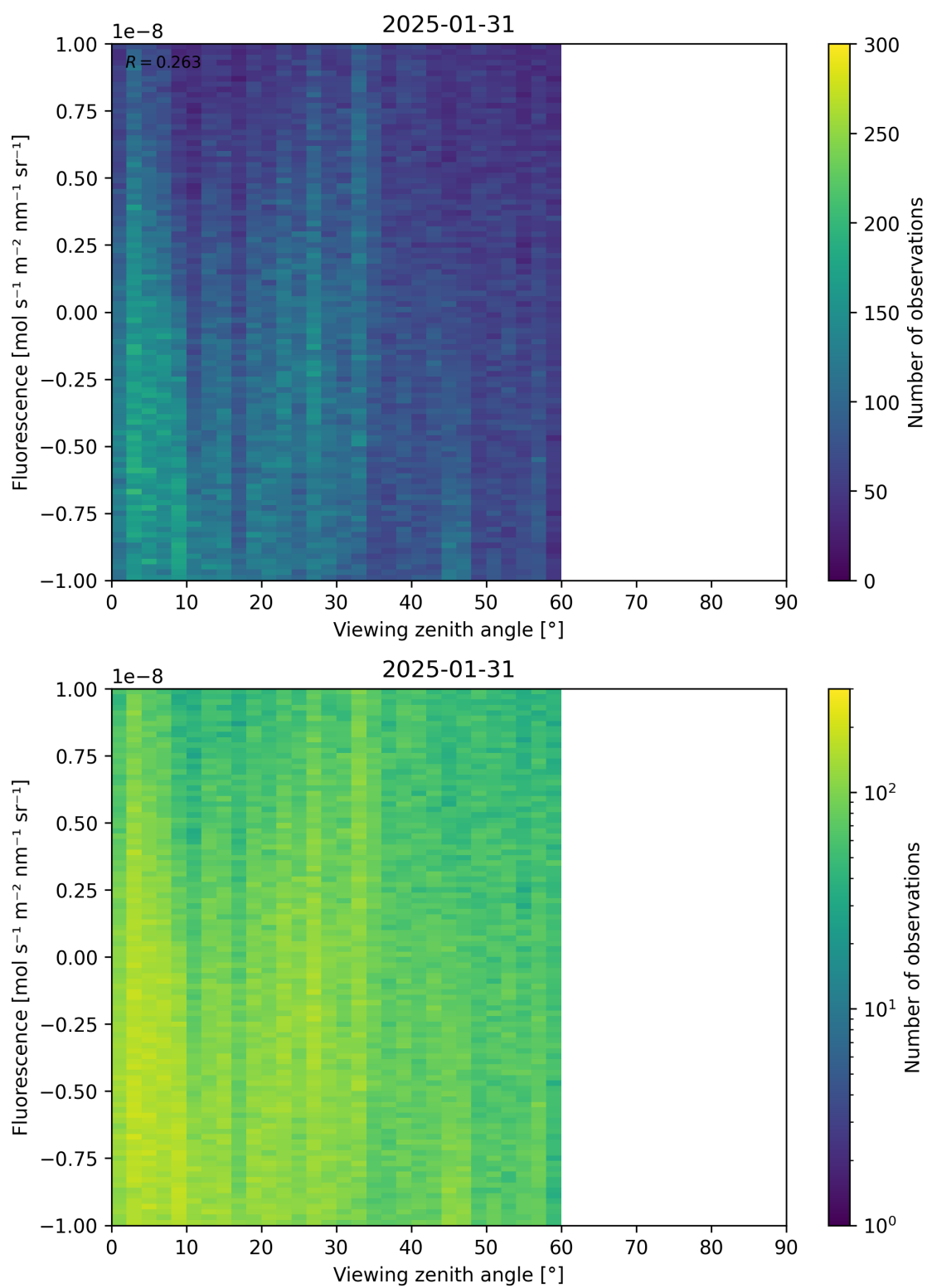
Figure 108: Scatter density plot of “Viewing zenith angle” against “Fluorescence” for 2025-01-30 to 2025-02-01.
