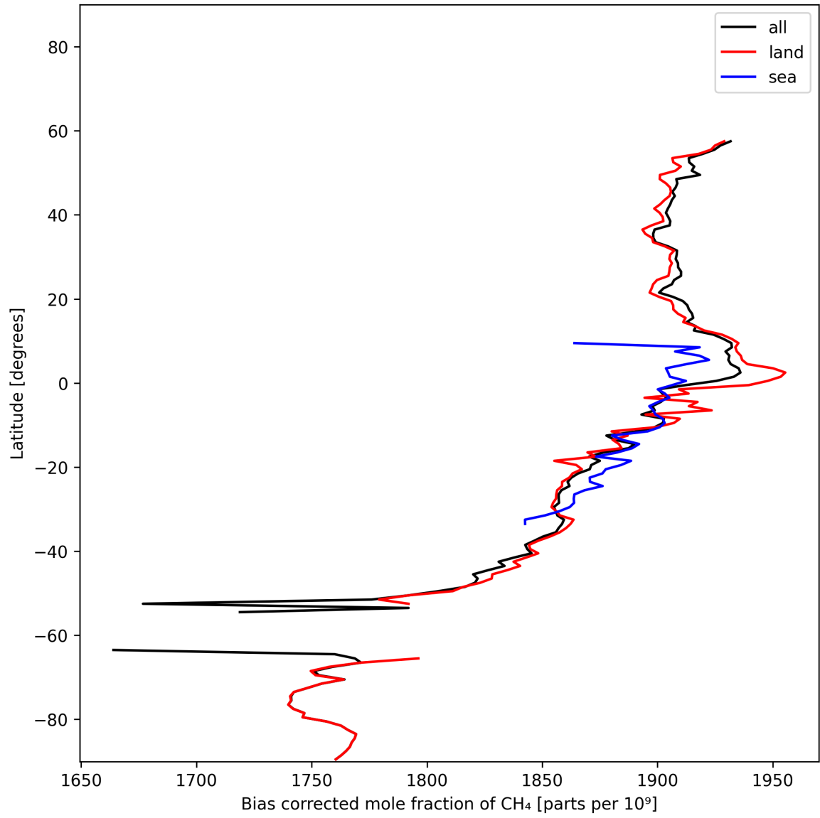
Figure 14: Zonal average of “Bias corrected mole fraction of CH 4 ” for 2025-01-30 to 2025-02-01.
