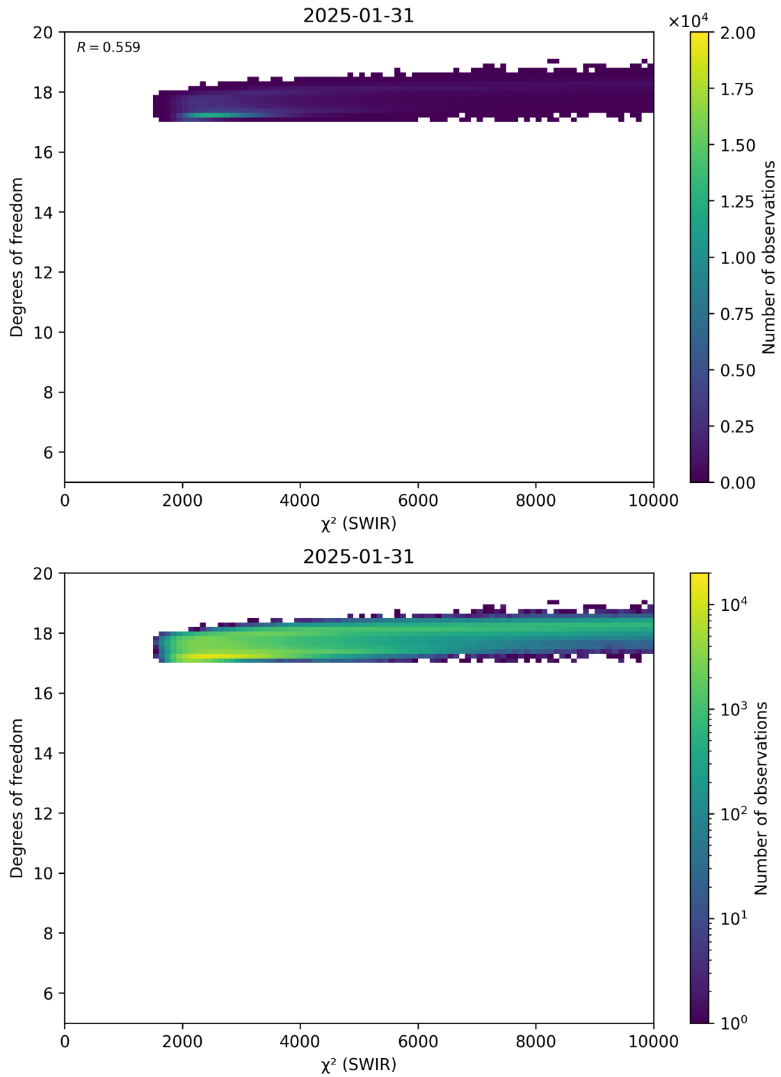
Figure 48: Scatter density plot of “ \chi^2 (SWIR)” against “Degrees of freedom” for 2025-01-30 to 2025-02-01.
