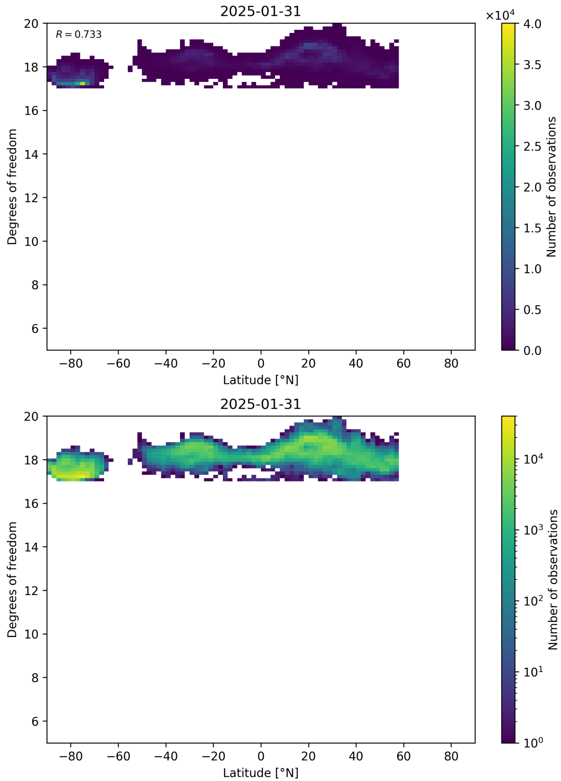
Figure 55: Scatter density plot of “Latitude” against “Degrees of freedom” for 2025-01-30 to 2025-02-01.
