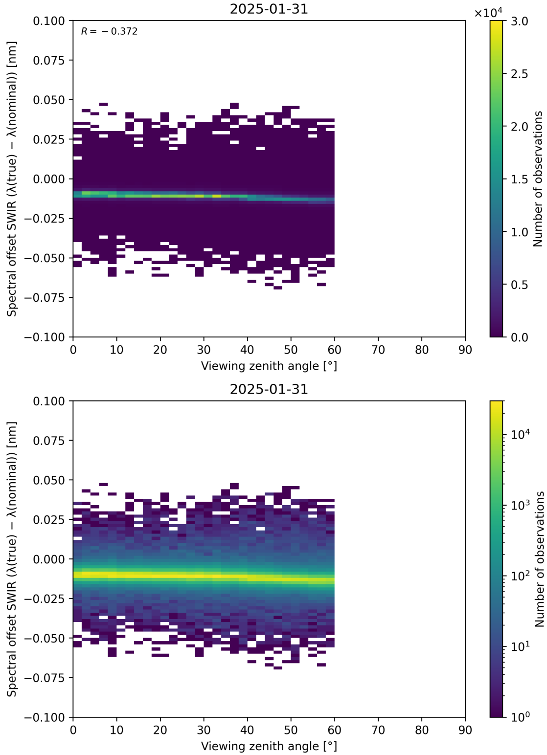
Figure 116: Scatter density plot of “Viewing zenith angle” against “Spectral offset SWIR ( \lambda_{\text{true}} - \lambda_{\text{nominal}} )” for 2025-01-30 to 2025-02-01.
