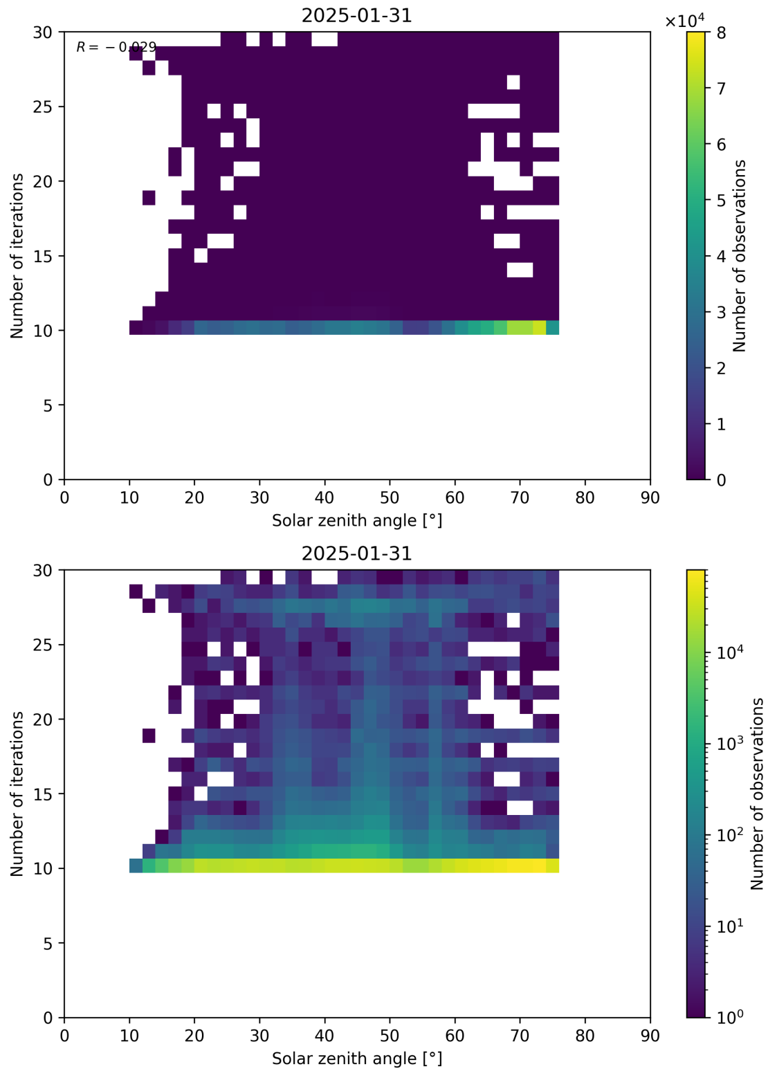
Figure 102: Scatter density plot of “Solar zenith angle” against “Number of iterations” for 2025-01-30 to 2025-02-01.
