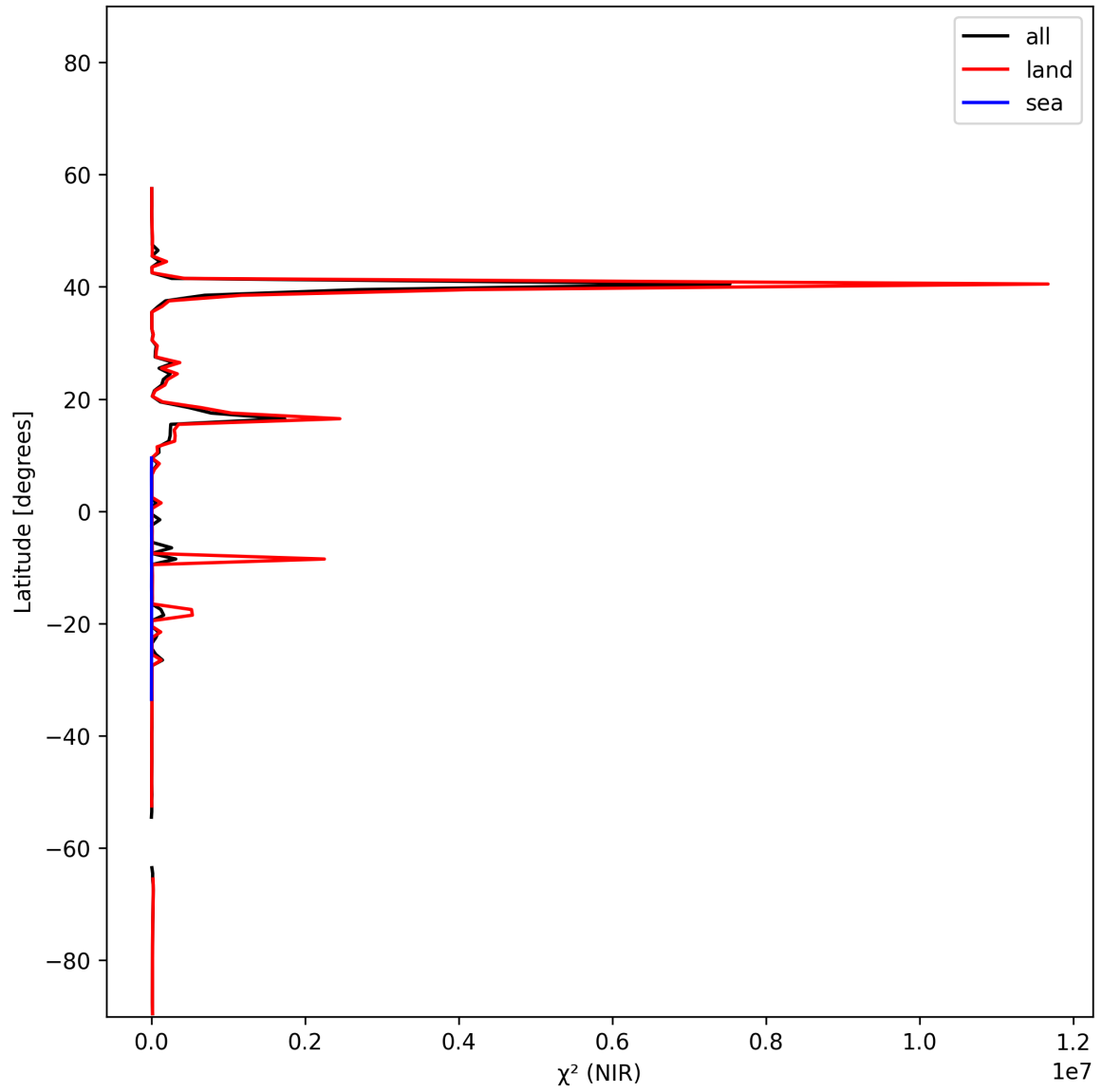
Figure 18: Zonal average of “ \chi^2 (NIR)” for 2025-01-30 to 2025-02-01.
