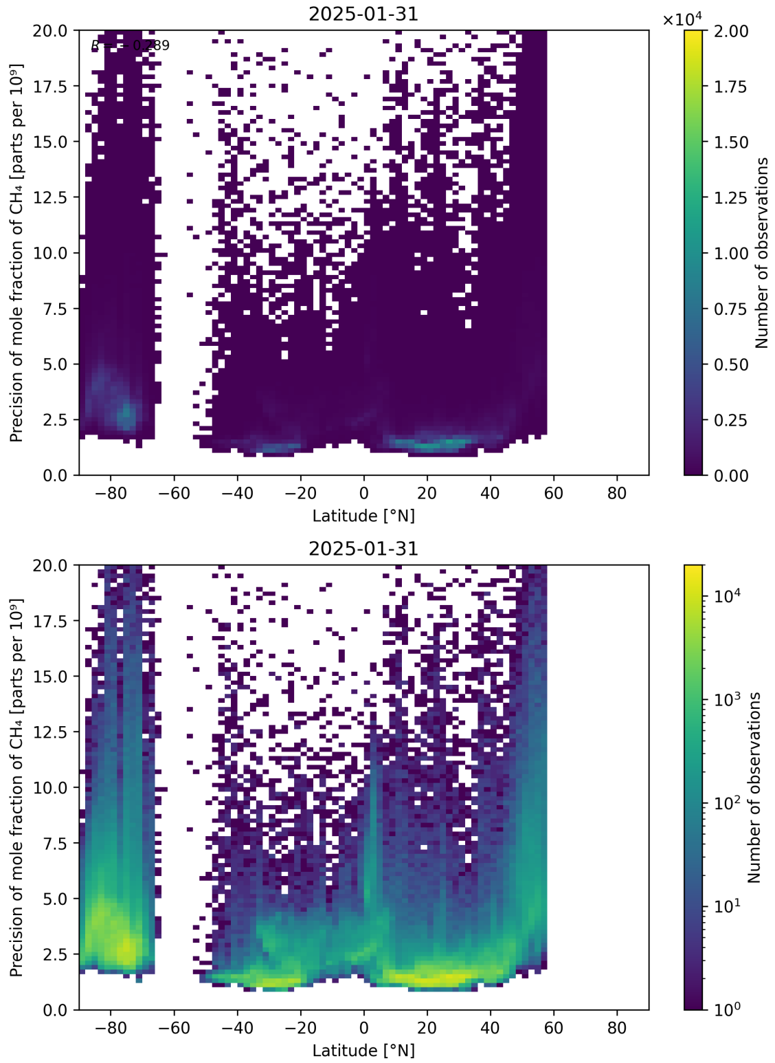
Figure 59: Scatter density plot of “Latitude” against “Precision of mole fraction of CH 4 ” for 2025-01-30 to 2025-02-01.
