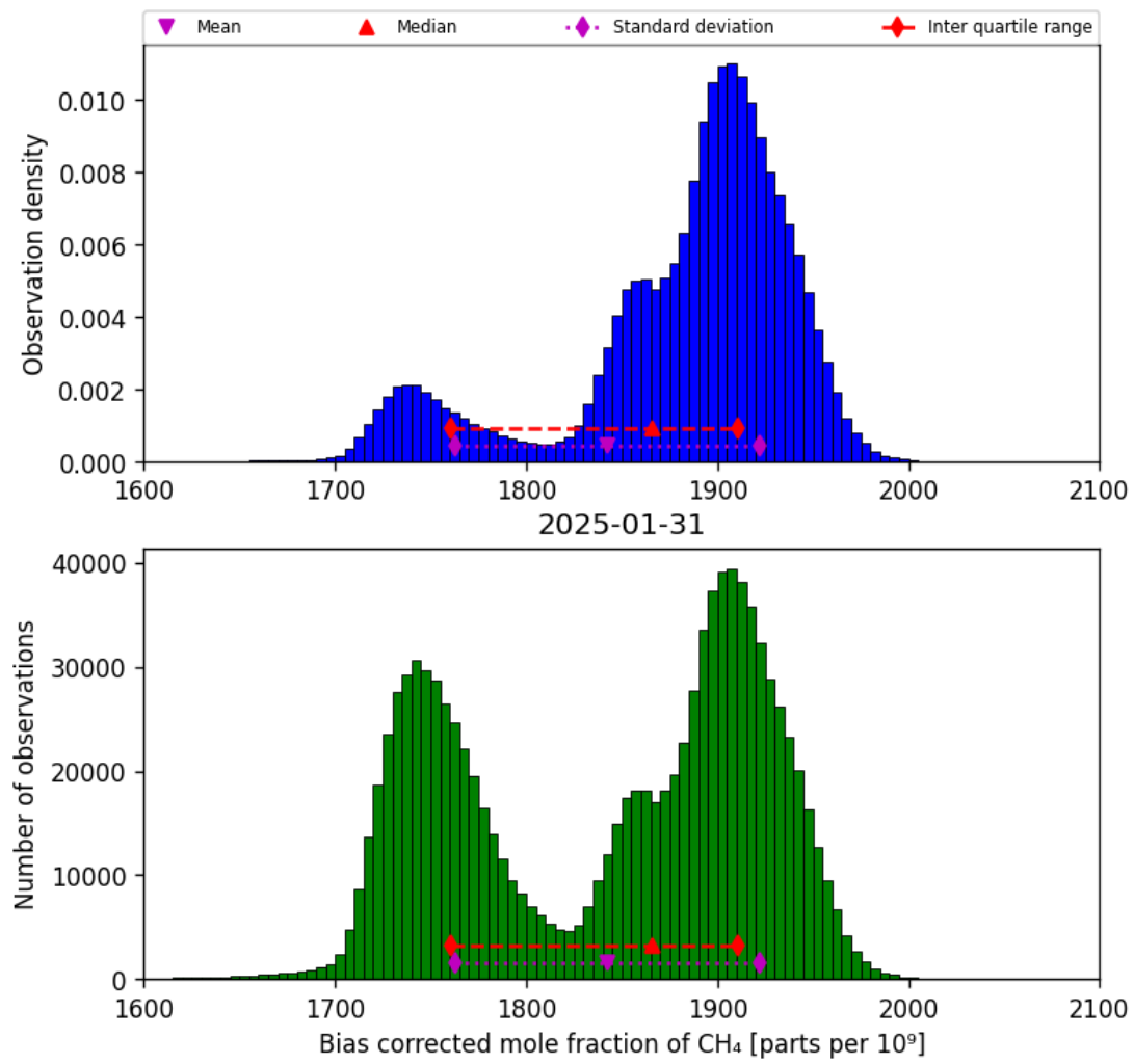
Figure 25: Histogram of “Bias corrected mole fraction of CH 4 ” for 2025-01-30 to 2025-02-01
