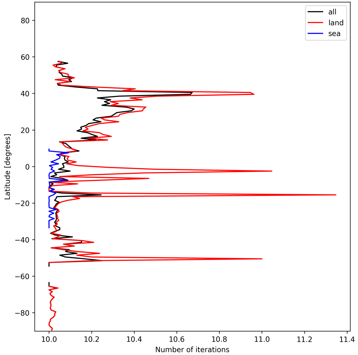
Figure 20: Zonal average of “Number of iterations” for 2025-01-30 to 2025-02-01.
