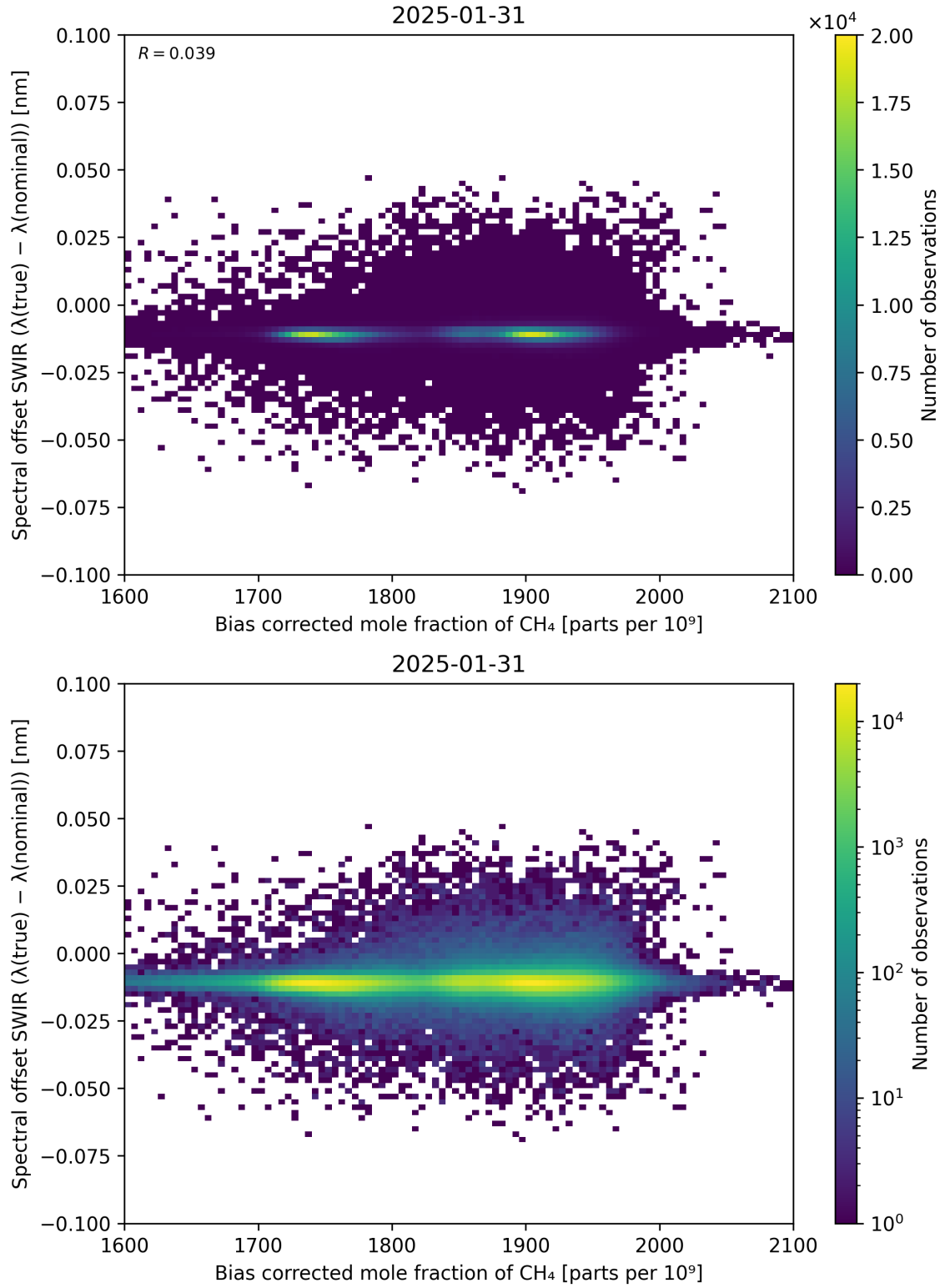
Figure 69: Scatter density plot of “Bias corrected mole fraction of CH 4 ” against “Spectral offset SWIR ( \lambda_{\text{true}} - \lambda_{\text{nominal}} )” for 2025-01-30 to 2025-02-01.
