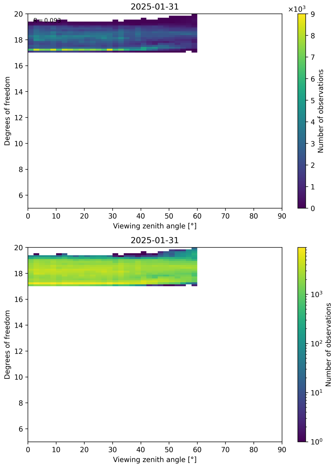
Figure 107: Scatter density plot of “Viewing zenith angle” against “Degrees of freedom” for 2025-01-30 to 2025-02-01.
