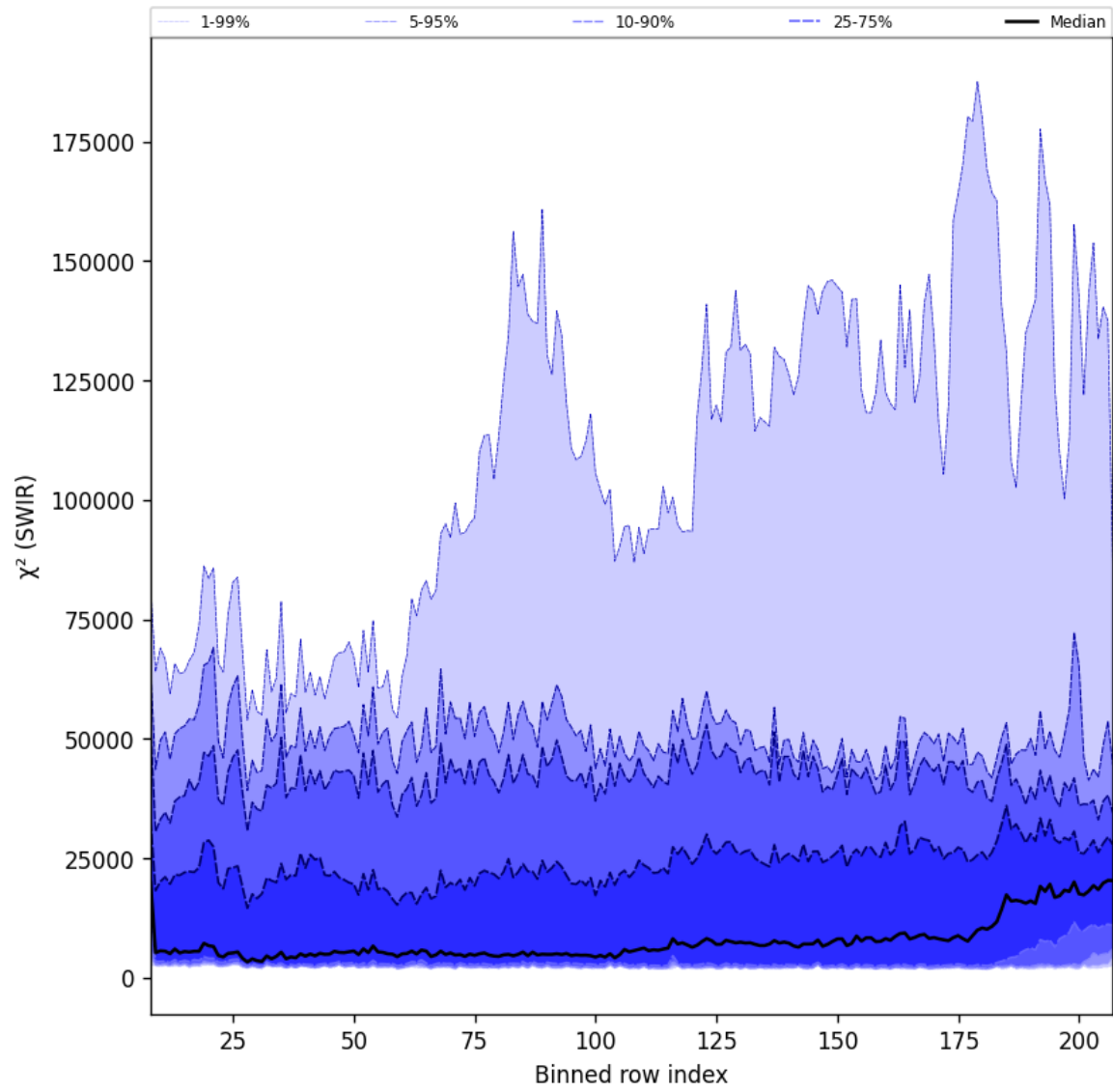
Figure 39: Along track statistics of “ \chi^2 (SWIR)” for 2025-01-30 to 2025-02-01
