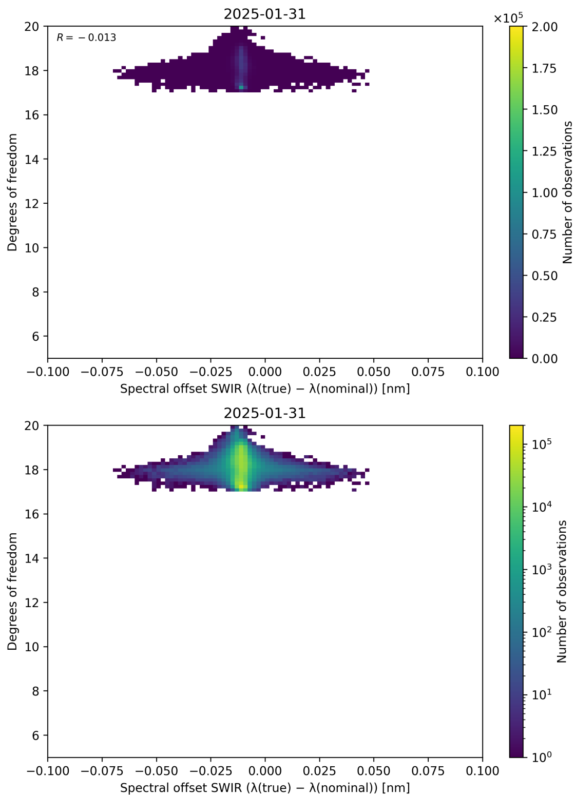
Figure 119: Scatter density plot of “Spectral offset SWIR ( \lambda_{\text{true}} - \lambda_{\text{nominal}} )” against “Degrees of freedom” for 2025-01-30 to 2025-02-01.
