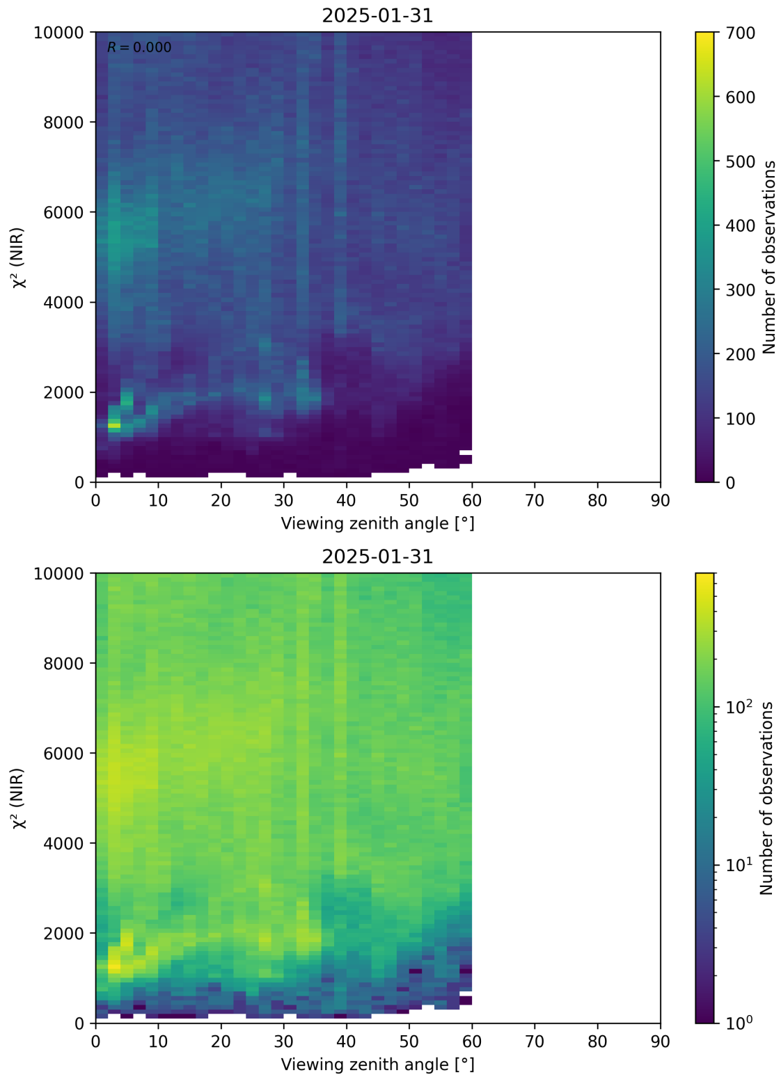
Figure 105: Scatter density plot of “Viewing zenith angle” against “ \chi^2 (NIR)” for 2025-01-30 to 2025-02-01.
