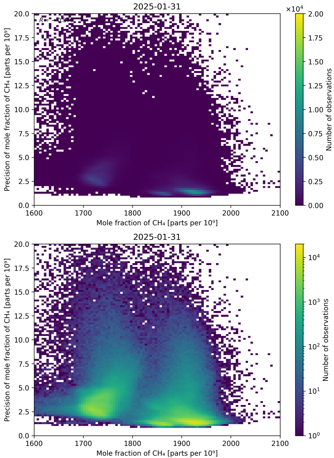
Figure 75: Scatter density plot of “Mole fraction of CH 4 ” against “Precision of mole fraction of CH 4 ” for 2025-01-30 to 2025-02-01.
