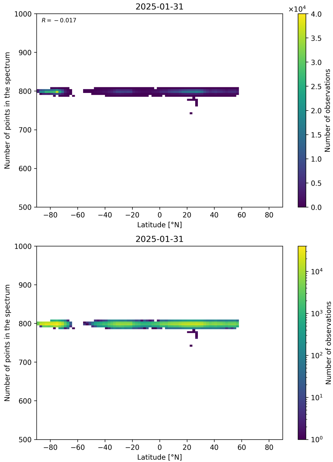
Figure 61: Scatter density plot of “Latitude” against “Number of points in the spectrum” for 2025-01-30 to 2025-02-01.
