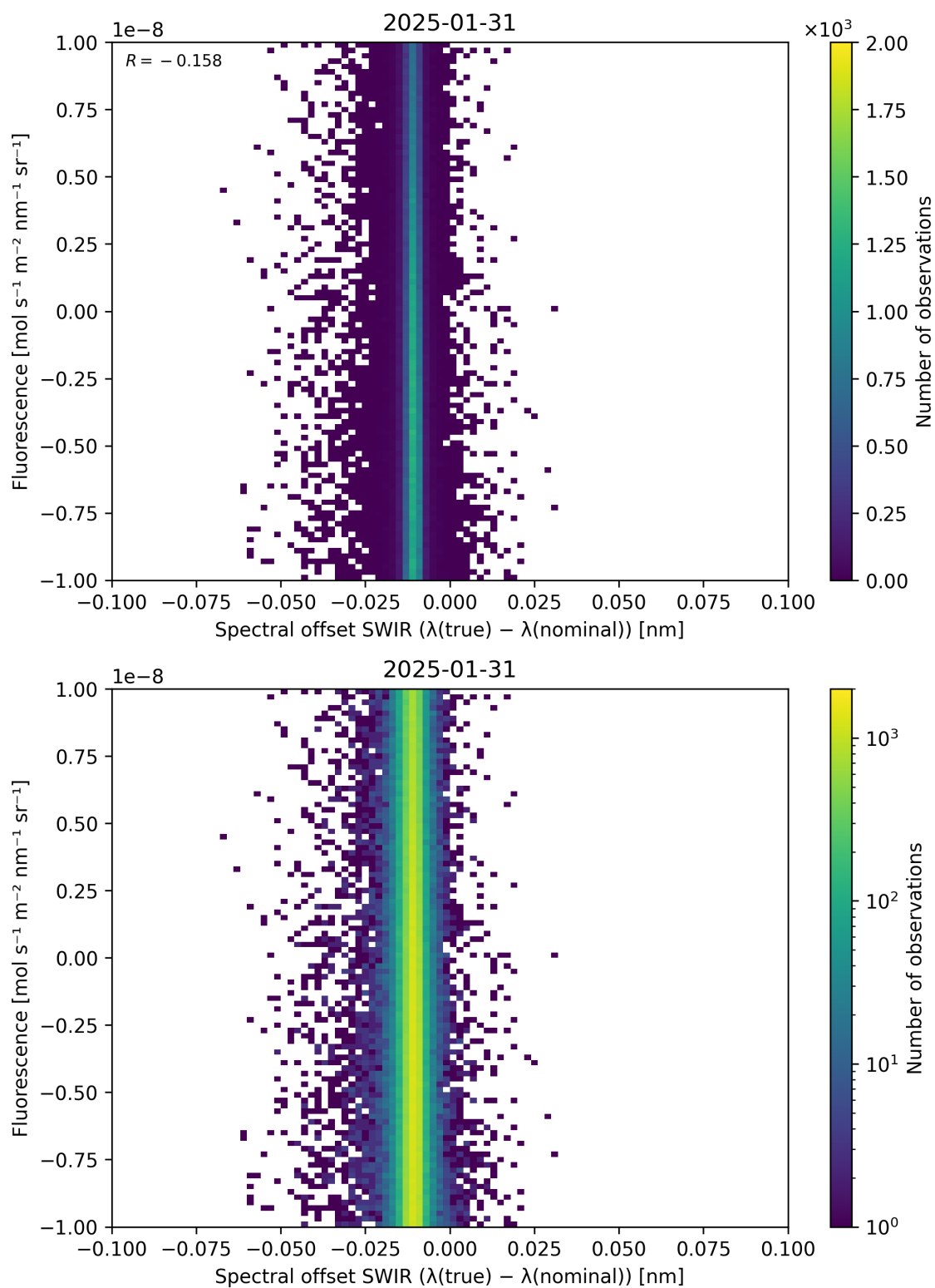
Figure 120: Scatter density plot of “Spectral offset SWIR ( \lambda_{\text{true}} - \lambda_{\text{nominal}} )” against “Fluorescence” for 2025-01-30 to 2025-02-01.
