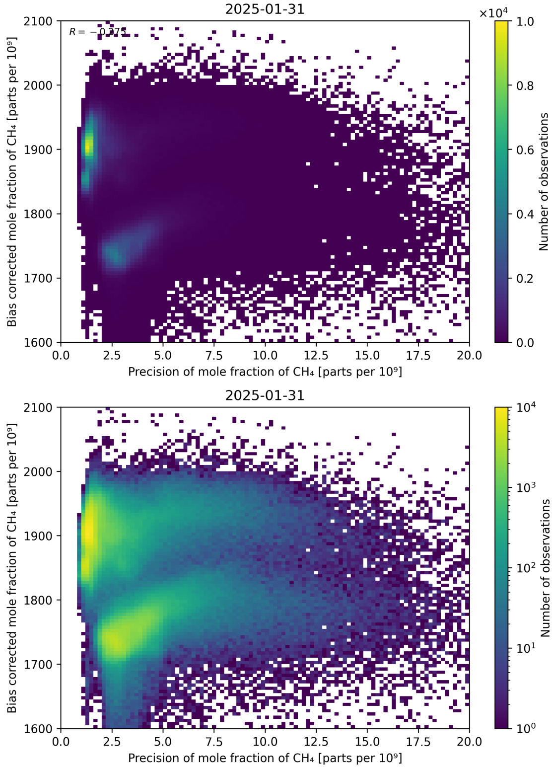
Figure 82: Scatter density plot of “Precision of mole fraction of CH 4 ” against “Bias corrected mole fraction of CH 4 ” for 2025-01-30 to 2025-02-01.
