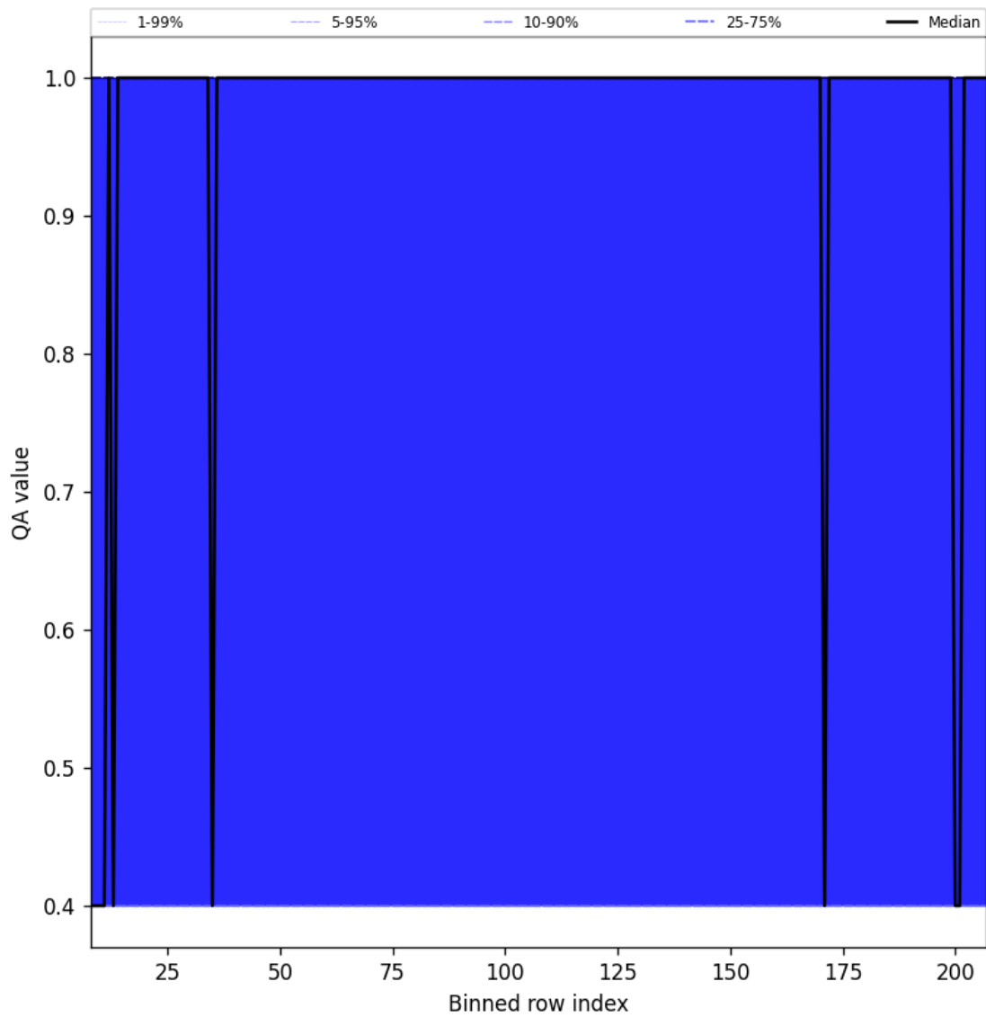
Figure 33: Along track statistics of “QA value” for 2025-01-30 to 2025-02-01
