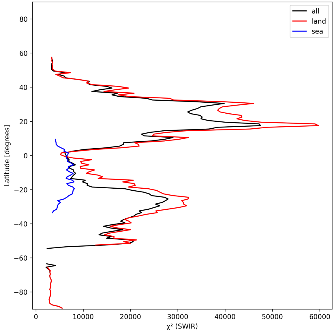
Figure 17: Zonal average of “ \chi^2 (SWIR)” for 2025-01-30 to 2025-02-01.
