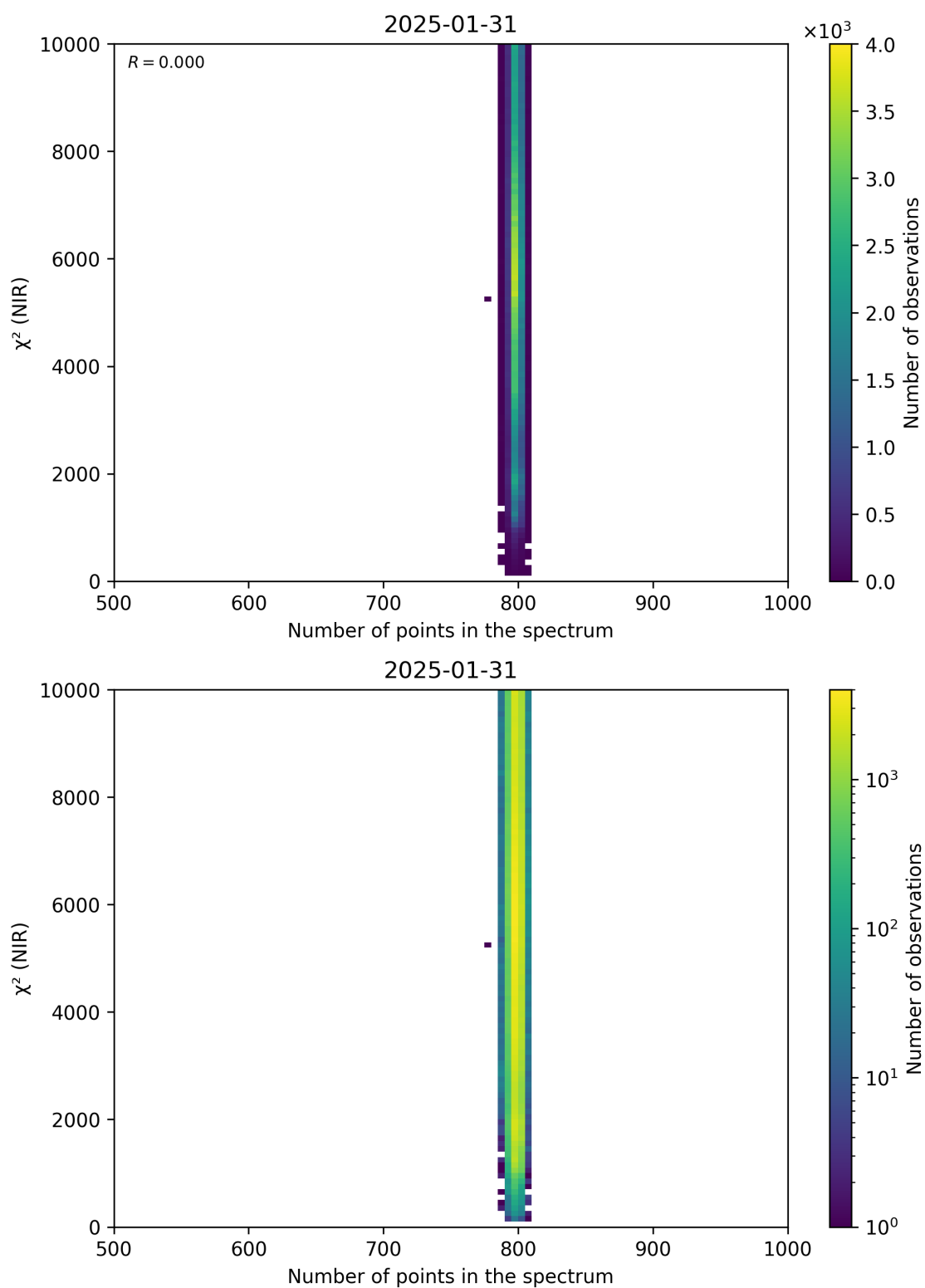
Figure 88: Scatter density plot of “Number of points in the spectrum” against “ \chi^2 (NIR)” for 2025-01-30 to 2025-02-01.
