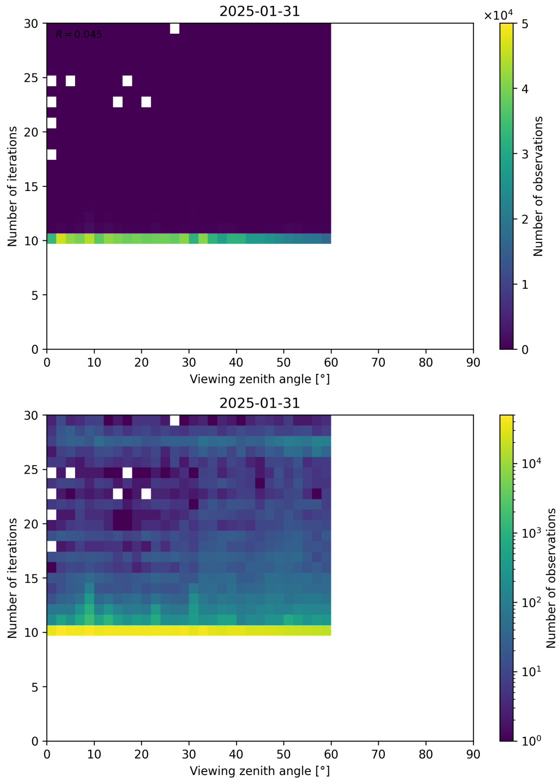
Figure 113: Scatter density plot of “Viewing zenith angle” against “Number of iterations” for 2025-01-30 to 2025-02-01.
