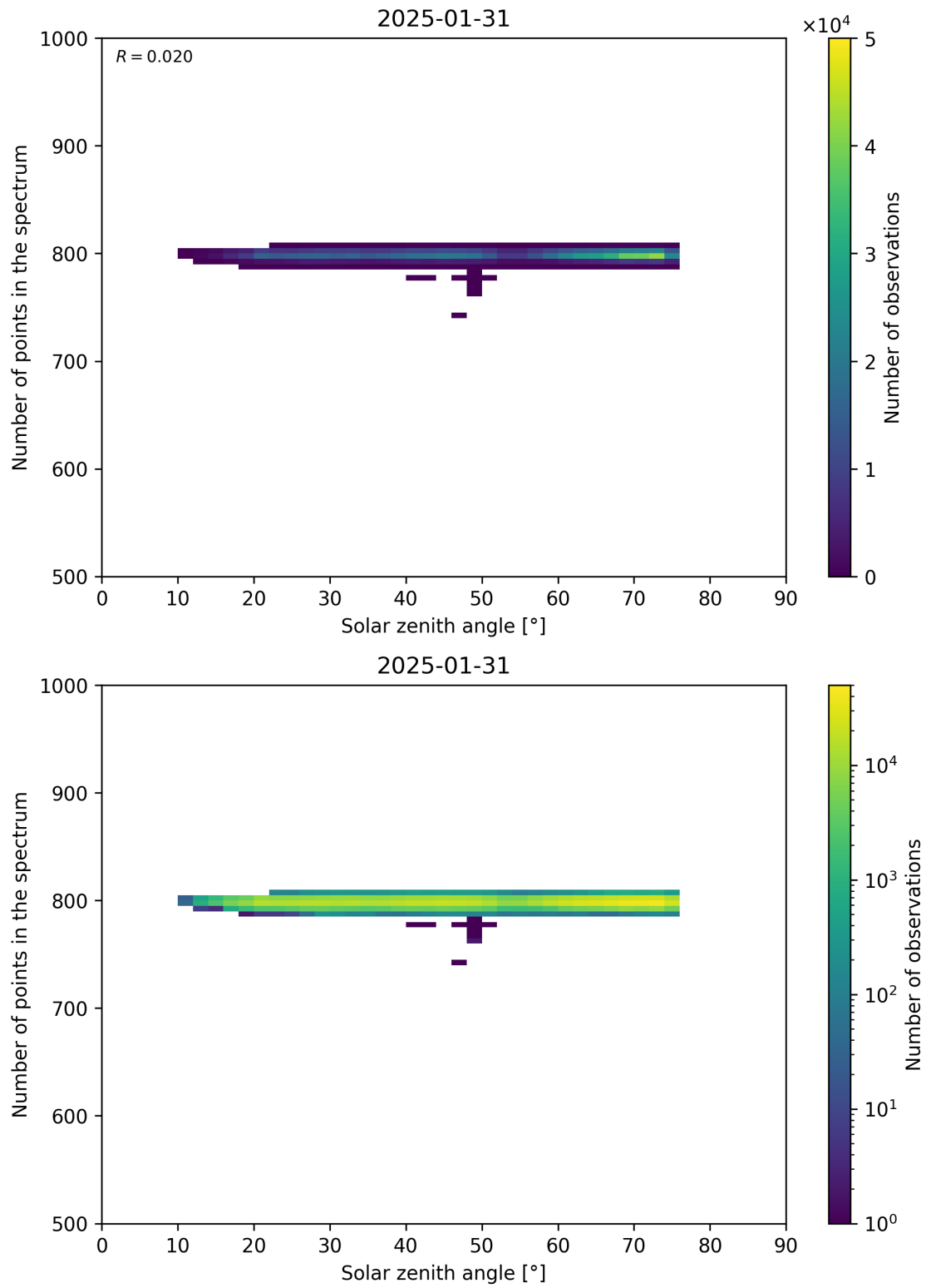
Figure 103: Scatter density plot of “Solar zenith angle” against “Number of points in the spectrum” for 2025-01-30 to 2025-02-01.
