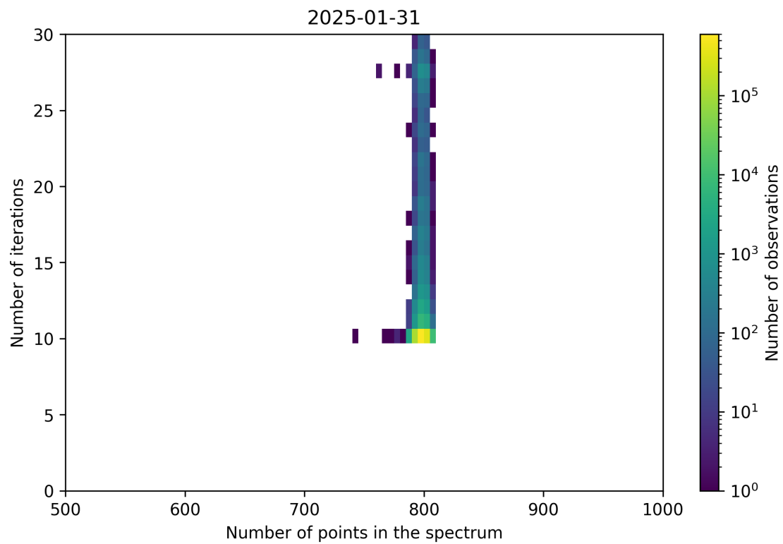
Figure 92: Scatter density plot of “Number of points in the spectrum” against “Number of iterations” for 2025-01-30 to 2025-02-01.
