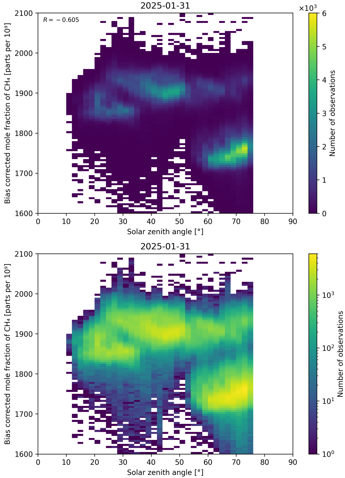
Figure 100: Scatter density plot of “Solar zenith angle” against “Bias corrected mole fraction of CH 4 ” for 2025-01-30 to 2025-02-01.
