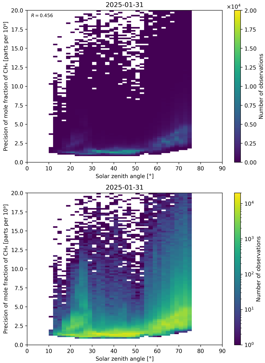
Figure 101: Scatter density plot of “Solar zenith angle” against “Precision of mole fraction of \text{CH}_4 ” for 2025-01-30 to 2025-02-01.
