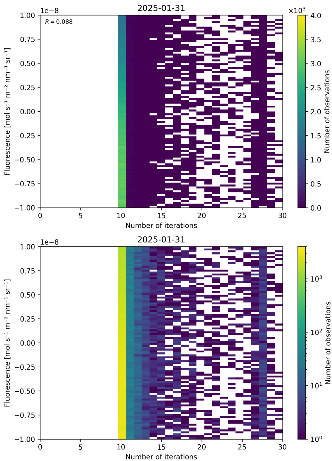
Figure 87: Scatter density plot of “Number of iterations” against “Fluorescence” for 2025-01-30 to 2025-02-01.
