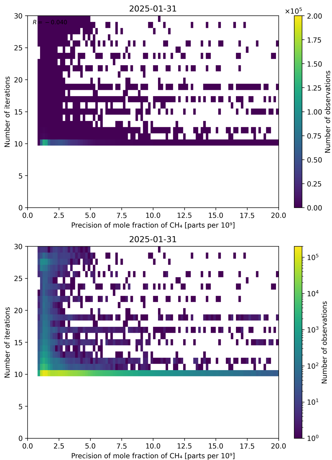
Figure 83: Scatter density plot of “Precision of mole fraction of CH 4 ” against “Number of iterations” for 2025-01-30 to 2025-02-01.
