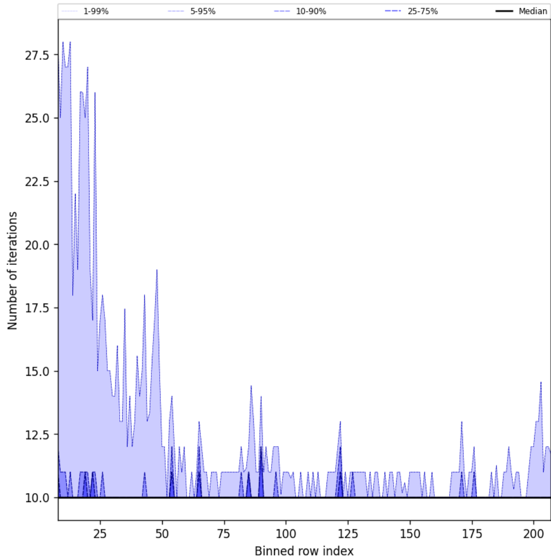
Figure 42: Along track statistics of “Number of iterations” for 2025-01-30 to 2025-02-01
