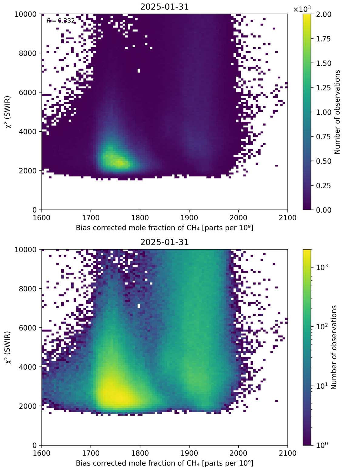
Figure 64: Scatter density plot of “Bias corrected mole fraction of \text{CH}_4 ” against “ \chi^2 (SWIR)” for 2025-01-30 to 2025-02-01.
