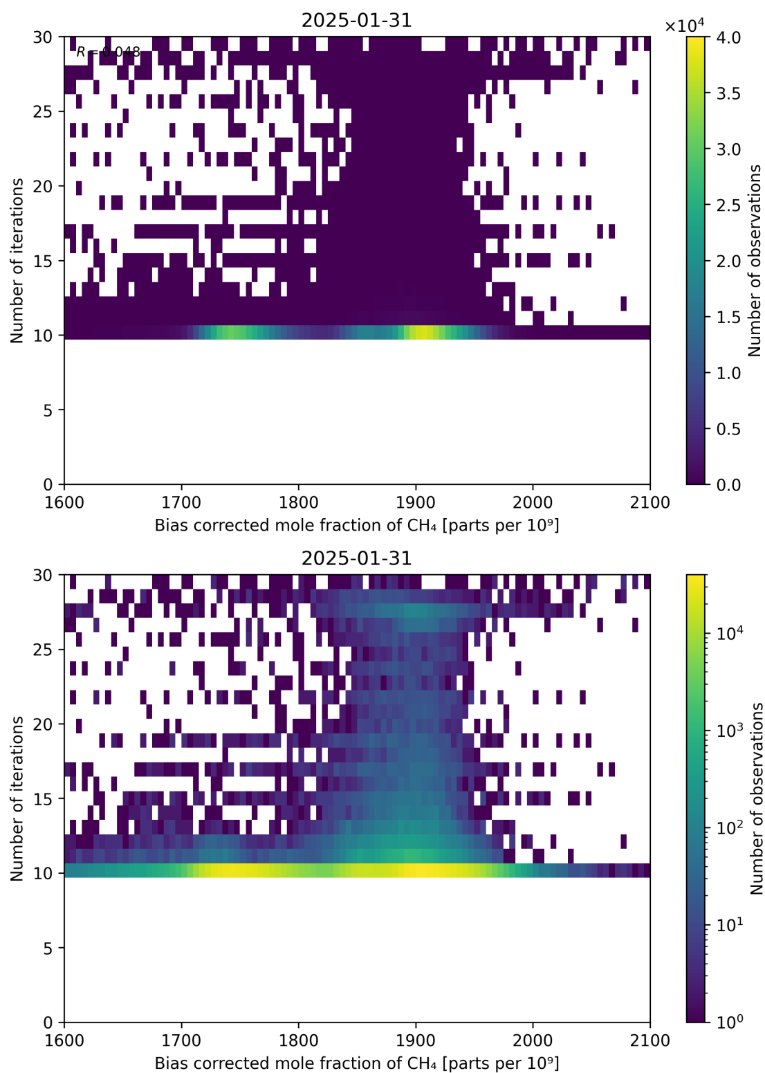
Figure 67: Scatter density plot of “Bias corrected mole fraction of CH 4 ” against “Number of iterations” for 2025-01-30 to 2025-02-01.
