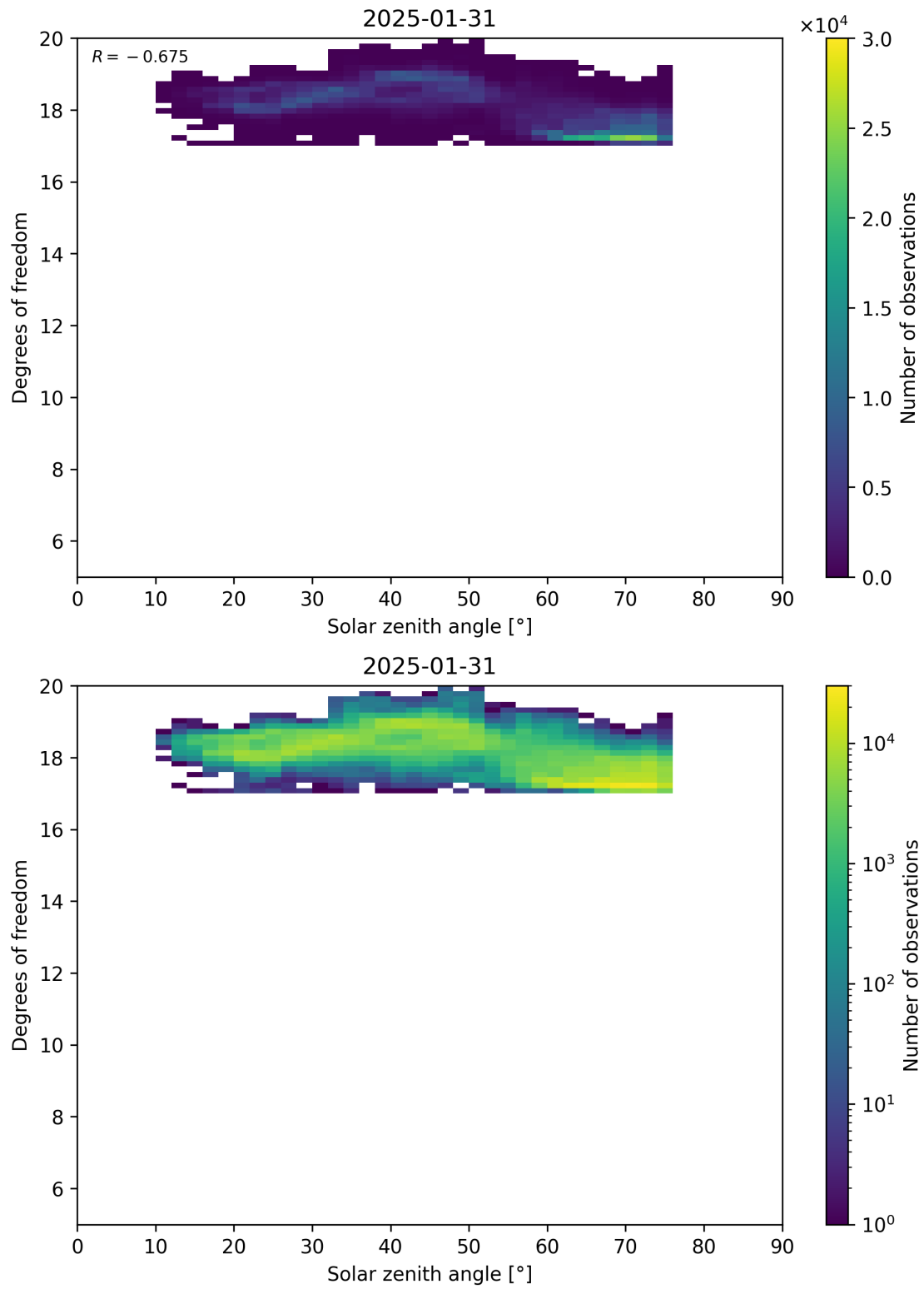
Figure 96: Scatter density plot of “Solar zenith angle” against “Degrees of freedom” for 2025-01-30 to 2025-02-01.
