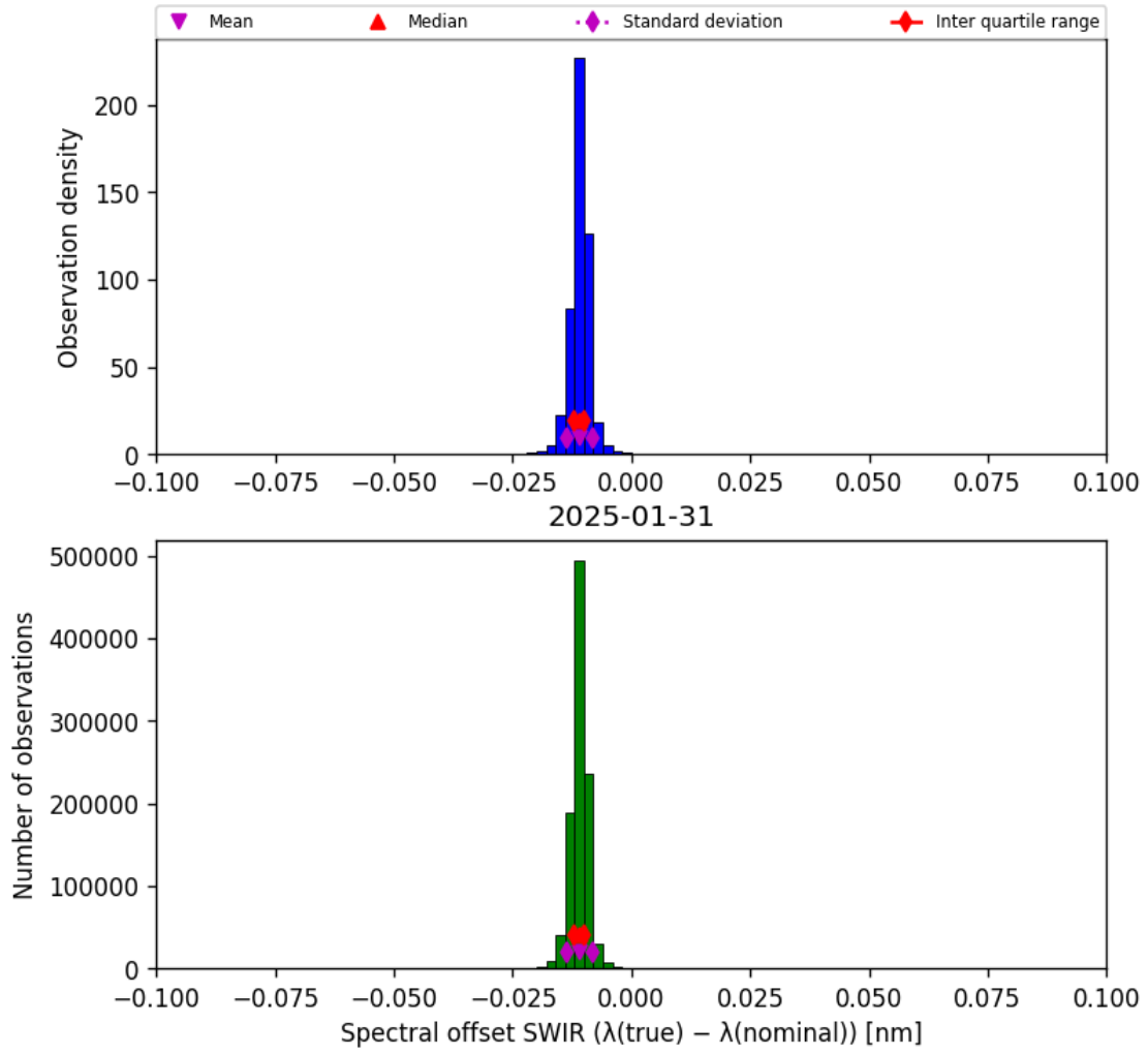
Figure 27: Histogram of “Spectral offset SWIR ( \lambda_{\text{true}} - \lambda_{\text{nominal}} )” for 2025-01-30 to 2025-02-01
