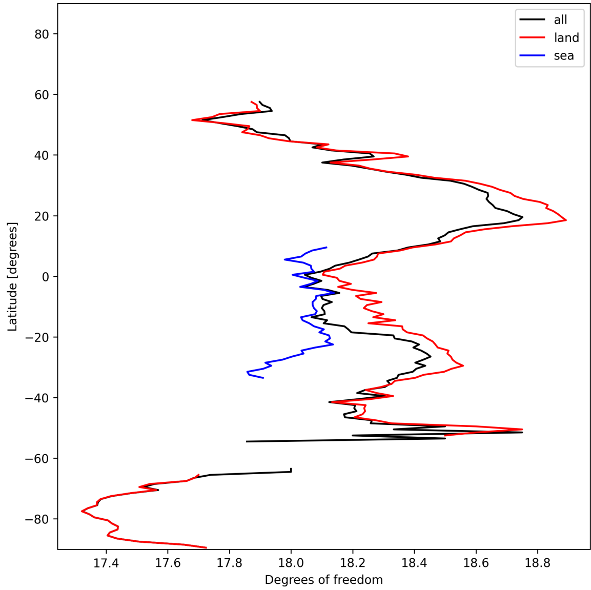
Figure 19: Zonal average of “Degrees of freedom” for 2025-01-30 to 2025-02-01.
