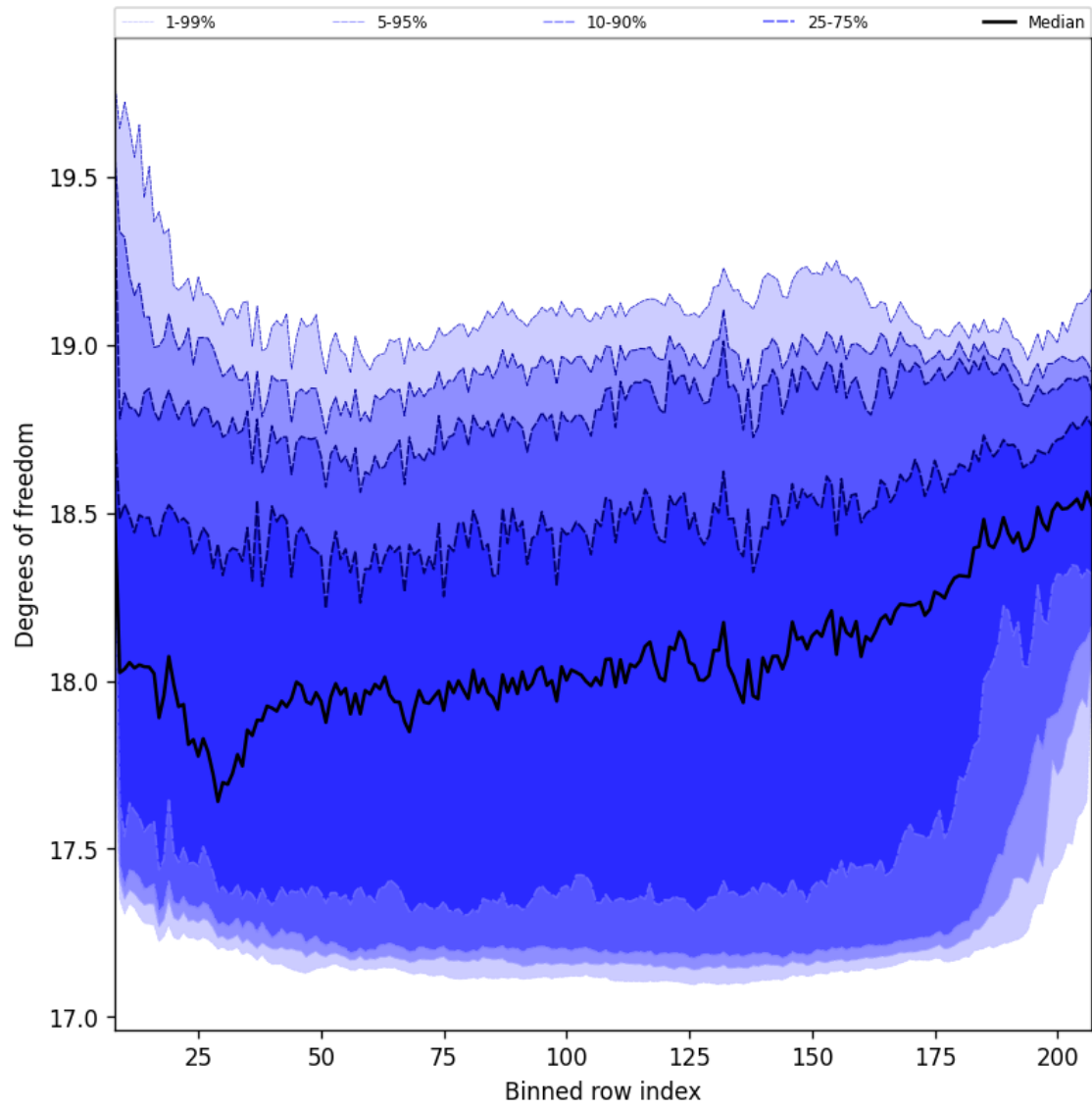
Figure 41: Along track statistics of “Degrees of freedom” for 2025-01-30 to 2025-02-01
