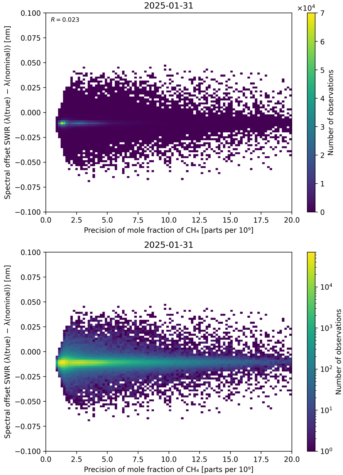
Figure 85: Scatter density plot of “Precision of mole fraction of \text{CH}_4 ” against “Spectral offset SWIR ( \lambda_{\text{true}} - \lambda_{\text{nominal}} )” for 2025-01-30 to 2025-02-01.
