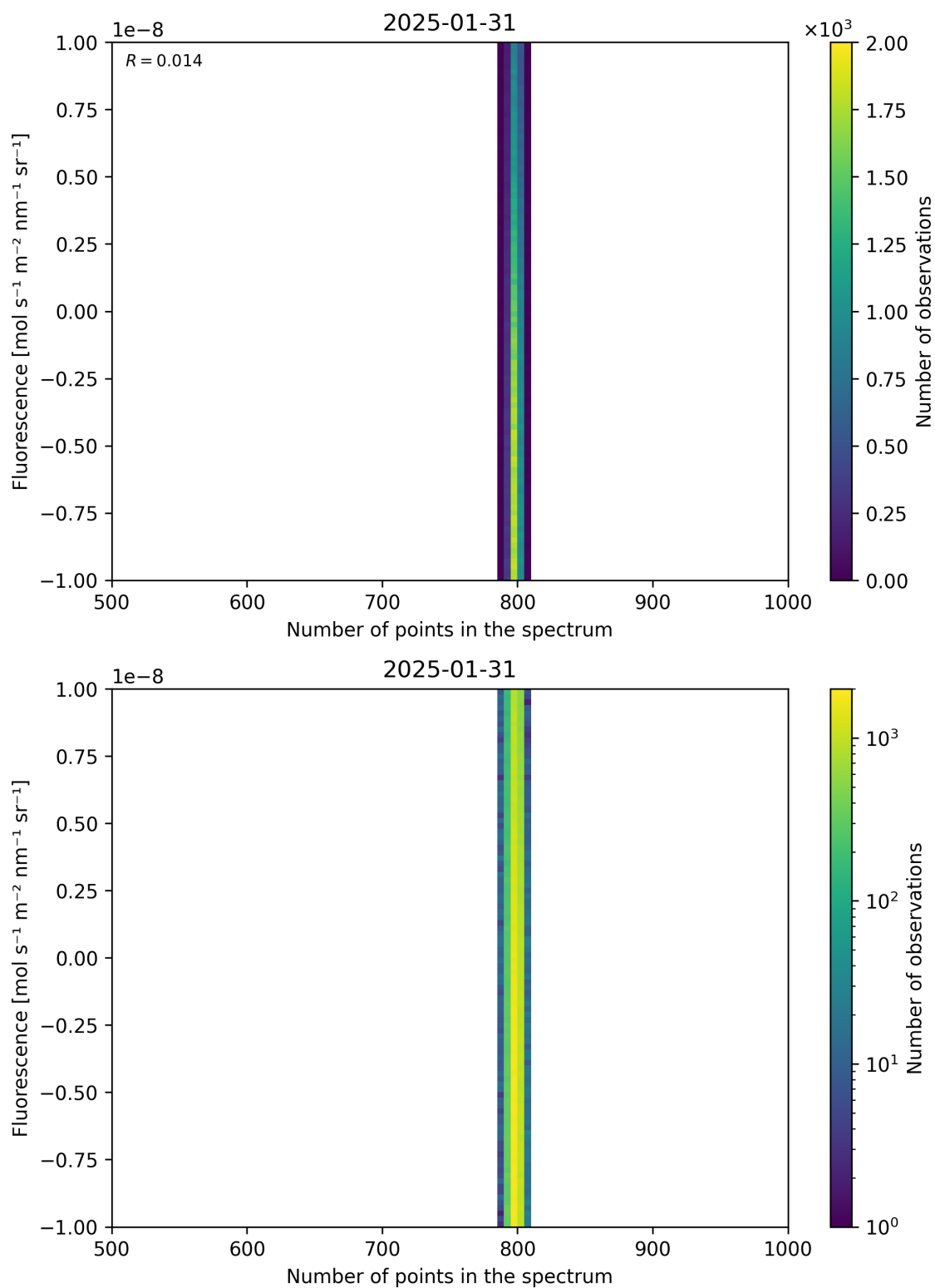
Figure 91: Scatter density plot of “Number of points in the spectrum” against “Fluorescence” for 2025-01-30 to 2025-02-01.
