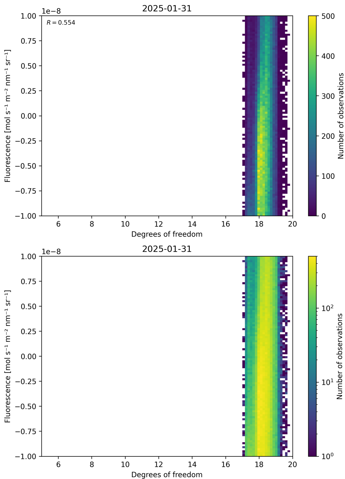
Figure 51: Scatter density plot of “Degrees of freedom” against “Fluorescence” for 2025-01-30 to 2025-02-01.
