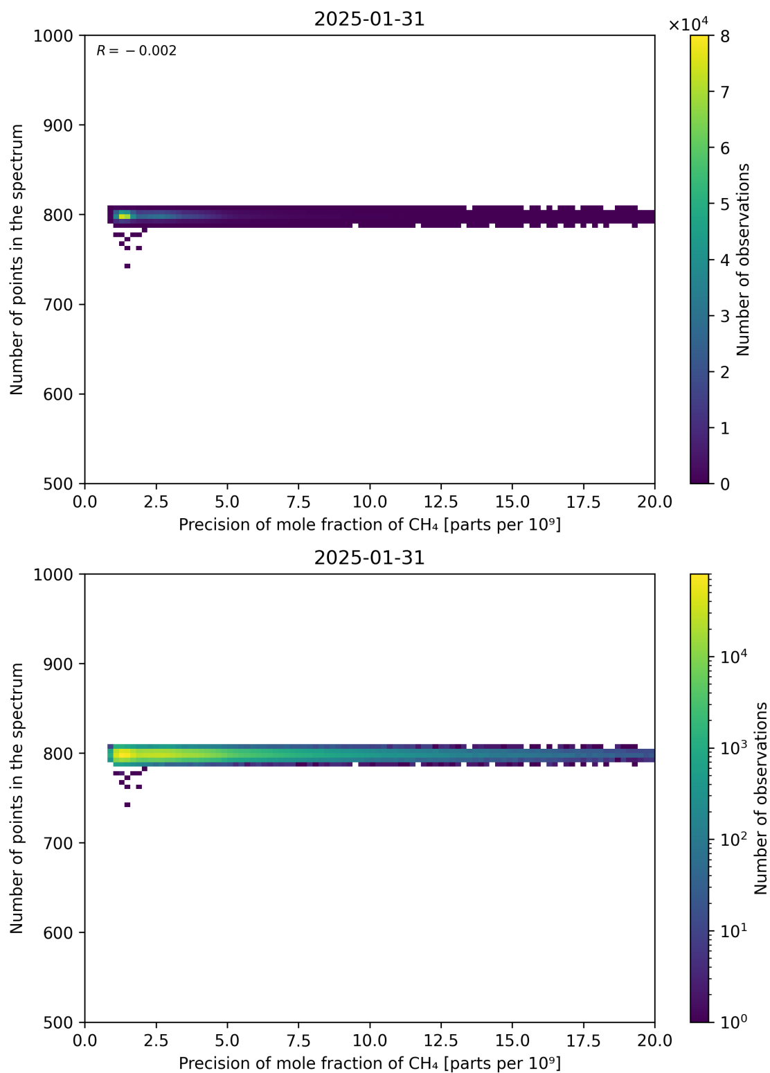
Figure 84: Scatter density plot of “Precision of mole fraction of CH 4 ” against “Number of points in the spectrum” for 2025-01-30 to 2025-02-01.
