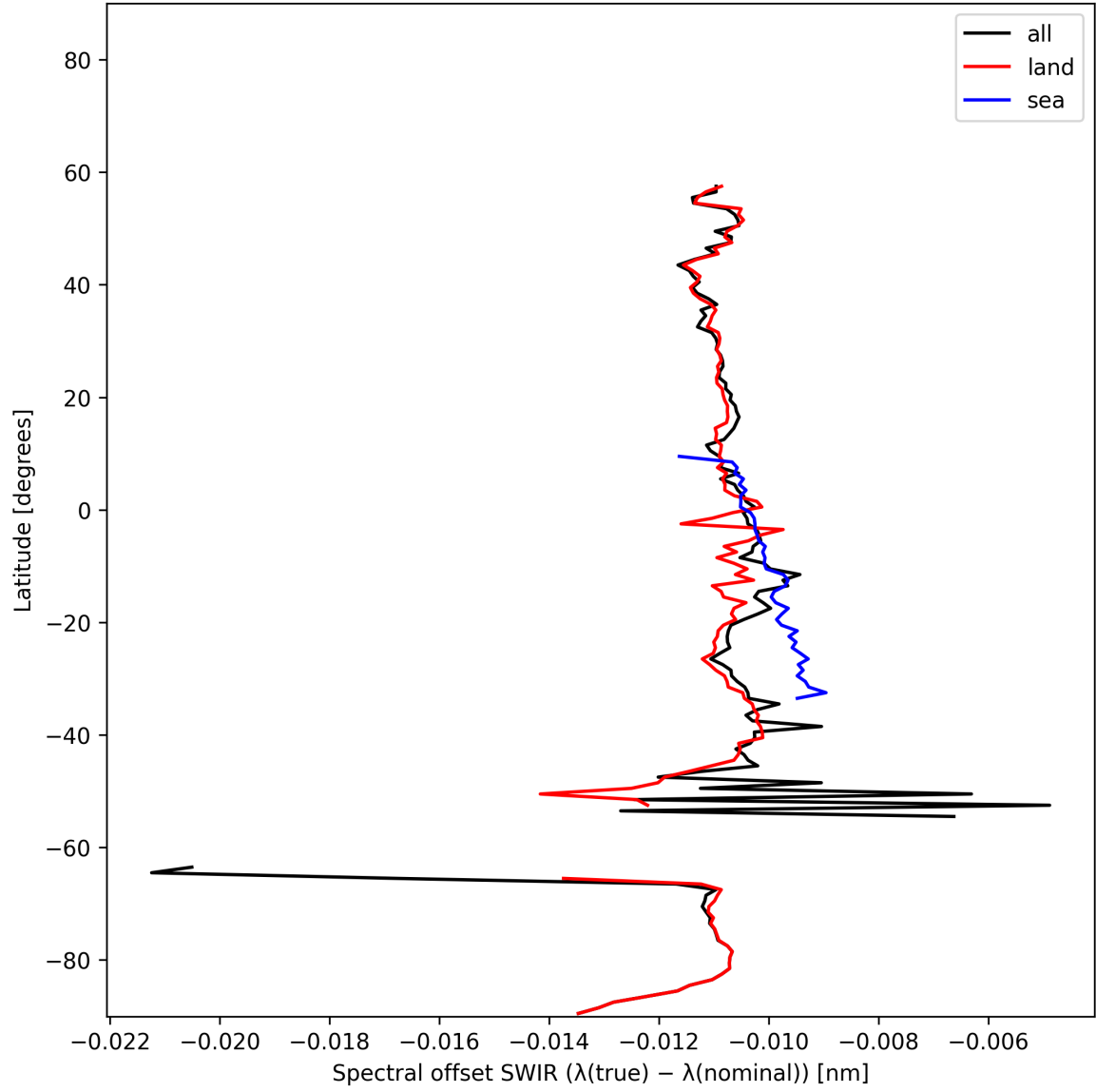
Figure 16: Zonal average of “Spectral offset SWIR ( \lambda_{\text{true}} - \lambda_{\text{nominal}} )” for 2025-01-30 to 2025-02-01.
