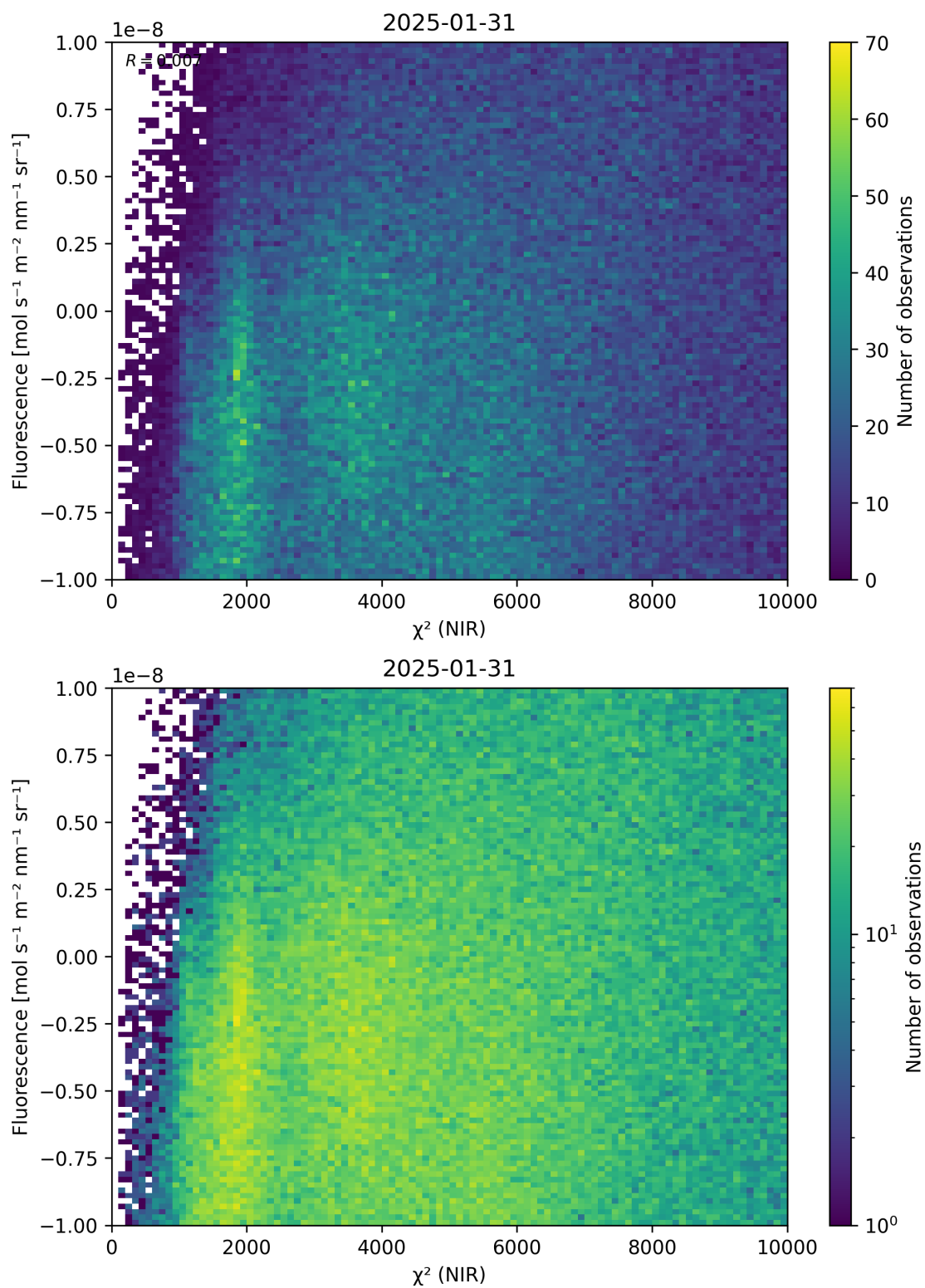
Figure 45: Scatter density plot of “ \chi^2 (NIR)” against “Fluorescence” for 2025-01-30 to 2025-02-01.
