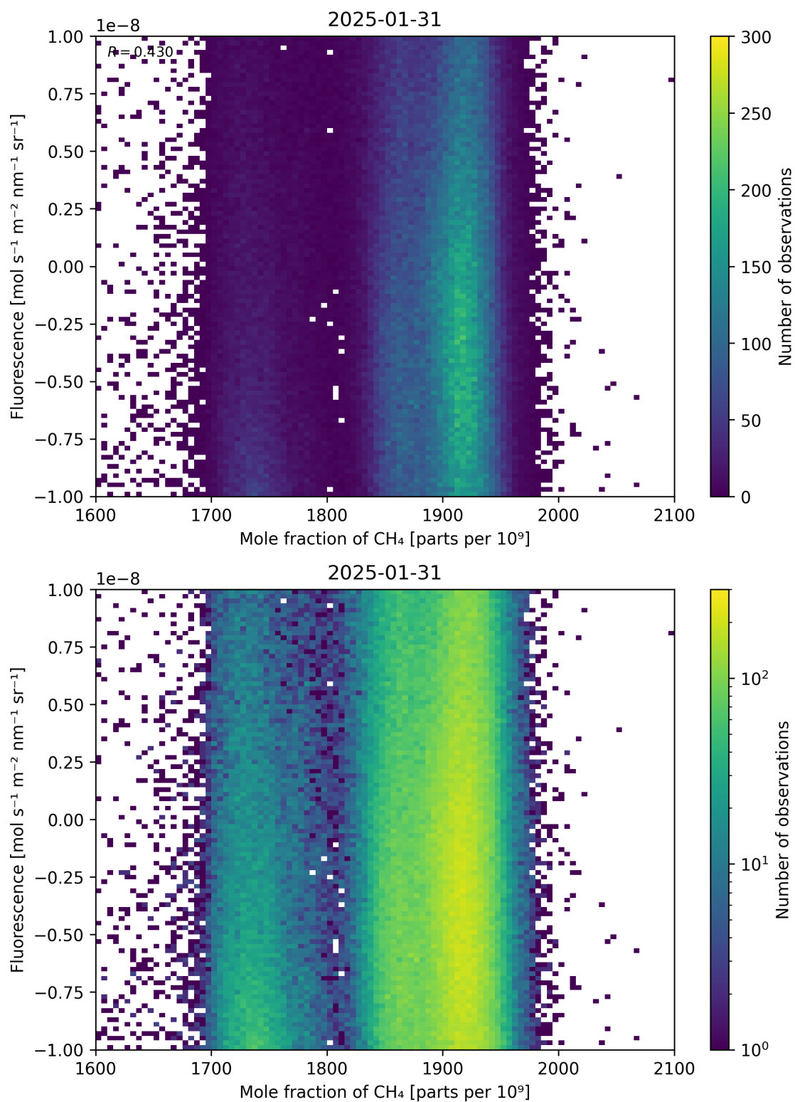
Figure 73: Scatter density plot of “Mole fraction of \text{CH}_4 ” against “Fluorescence” for 2025-01-30 to 2025-02-01.
