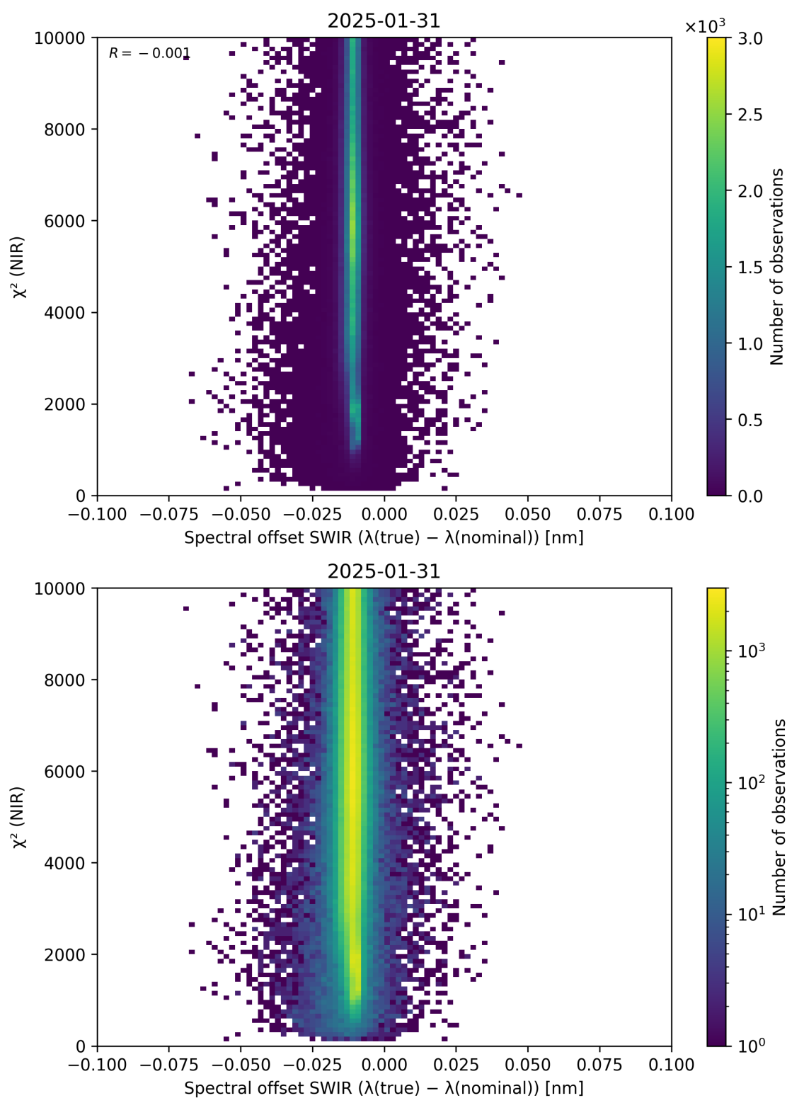
Figure 117: Scatter density plot of “Spectral offset SWIR ( \lambda_{\text{true}} - \lambda_{\text{nominal}} )” against “ \chi^2 (NIR)” for 2025-01-30 to 2025-02-01.
