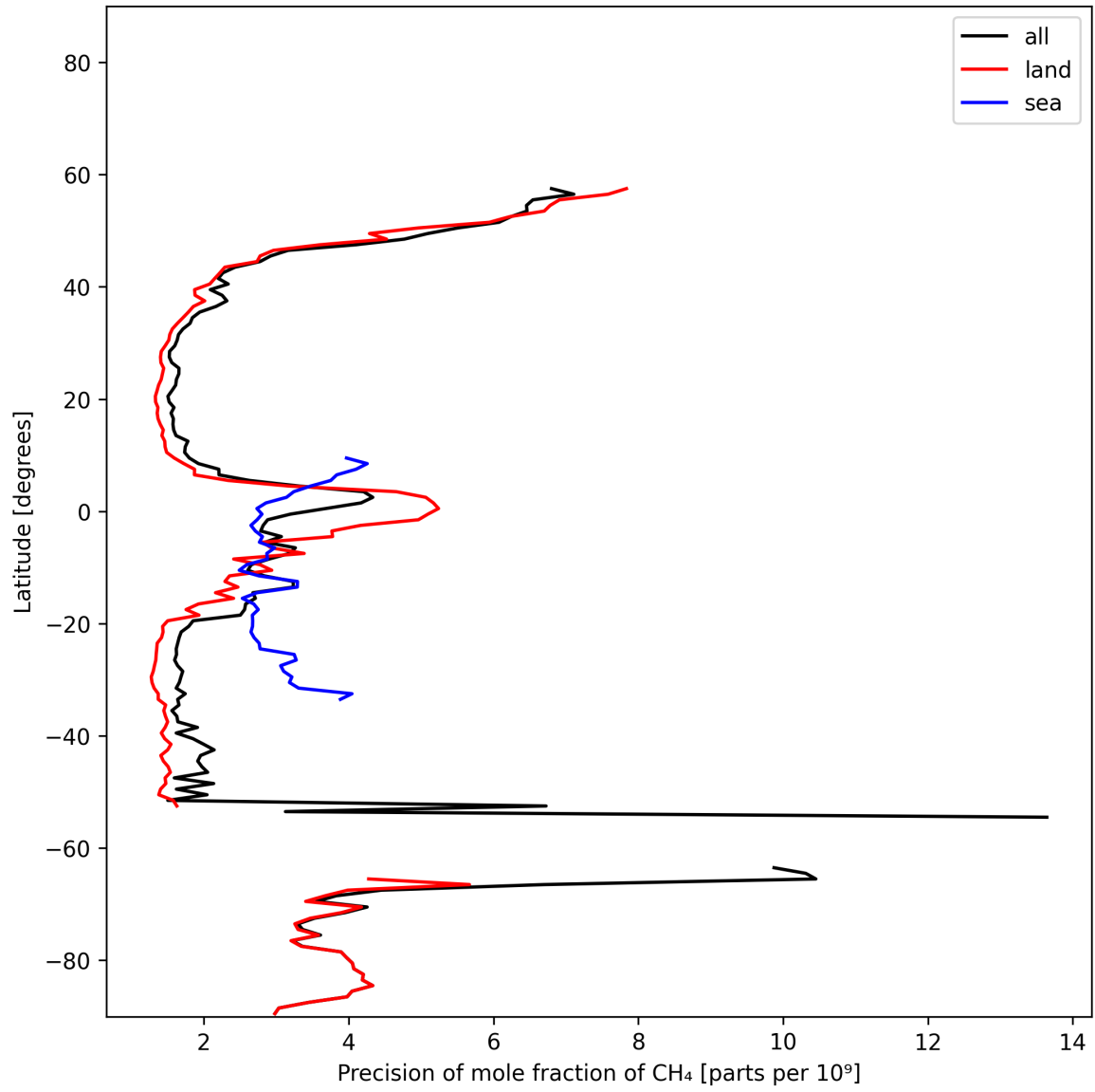
Figure 13: Zonal average of “Precision of mole fraction of CH 4 ” for 2025-01-30 to 2025-02-01.
