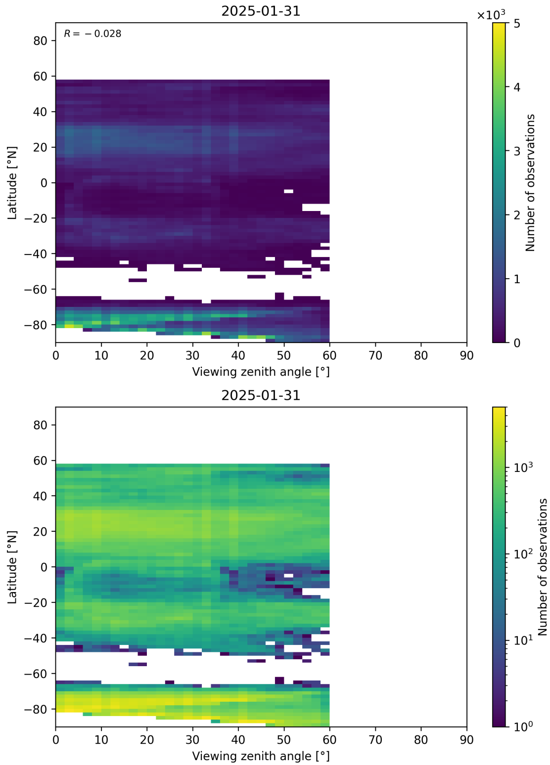
Figure 109: Scatter density plot of “Viewing zenith angle” against “Latitude” for 2025-01-30 to 2025-02-01.
