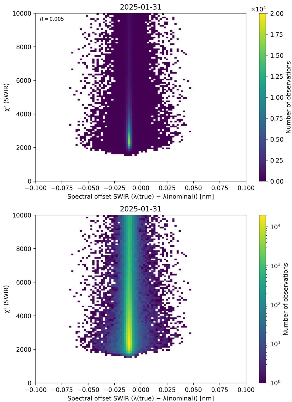
Figure 118: Scatter density plot of “Spectral offset SWIR ( \lambda_{\text{true}} - \lambda_{\text{nominal}} )” against “ \chi^2 (SWIR)” for 2025-01-30 to 2025-02-01.
