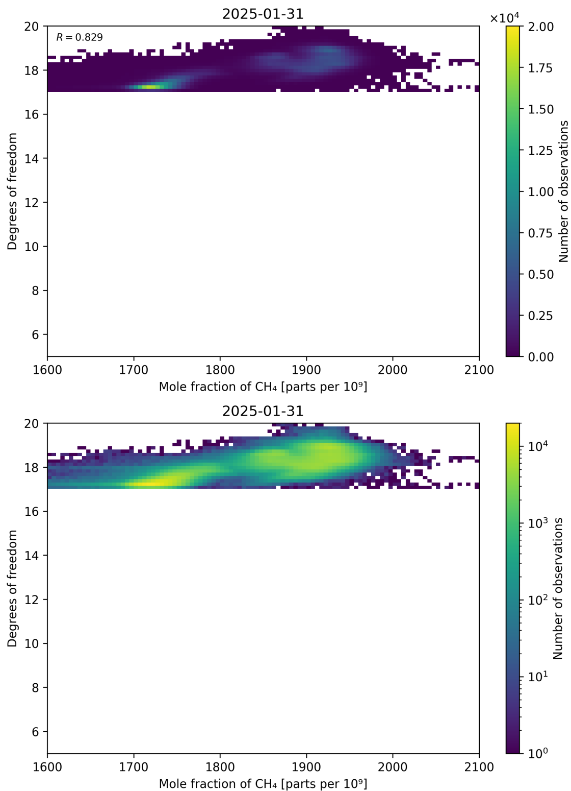
Figure 72: Scatter density plot of “Mole fraction of CH 4 ” against “Degrees of freedom” for 2025-01-30 to 2025-02-01.
