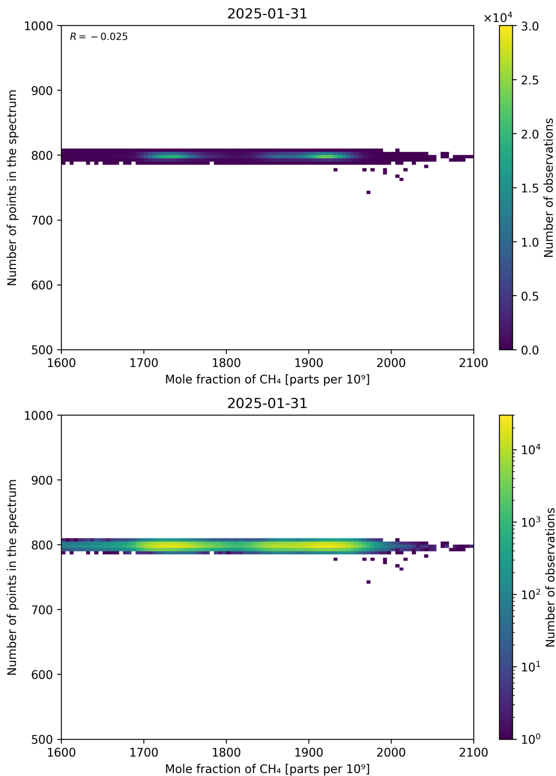
Figure 77: Scatter density plot of “Mole fraction of CH 4 ” against “Number of points in the spectrum” for 2025-01-30 to 2025-02-01.
