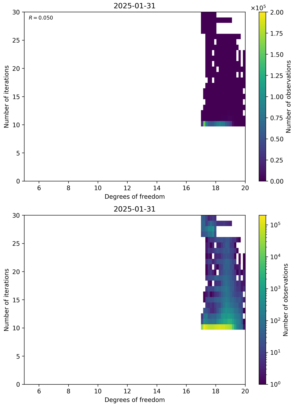
Figure 52: Scatter density plot of “Degrees of freedom” against “Number of iterations” for 2025-01-30 to 2025-02-01.
