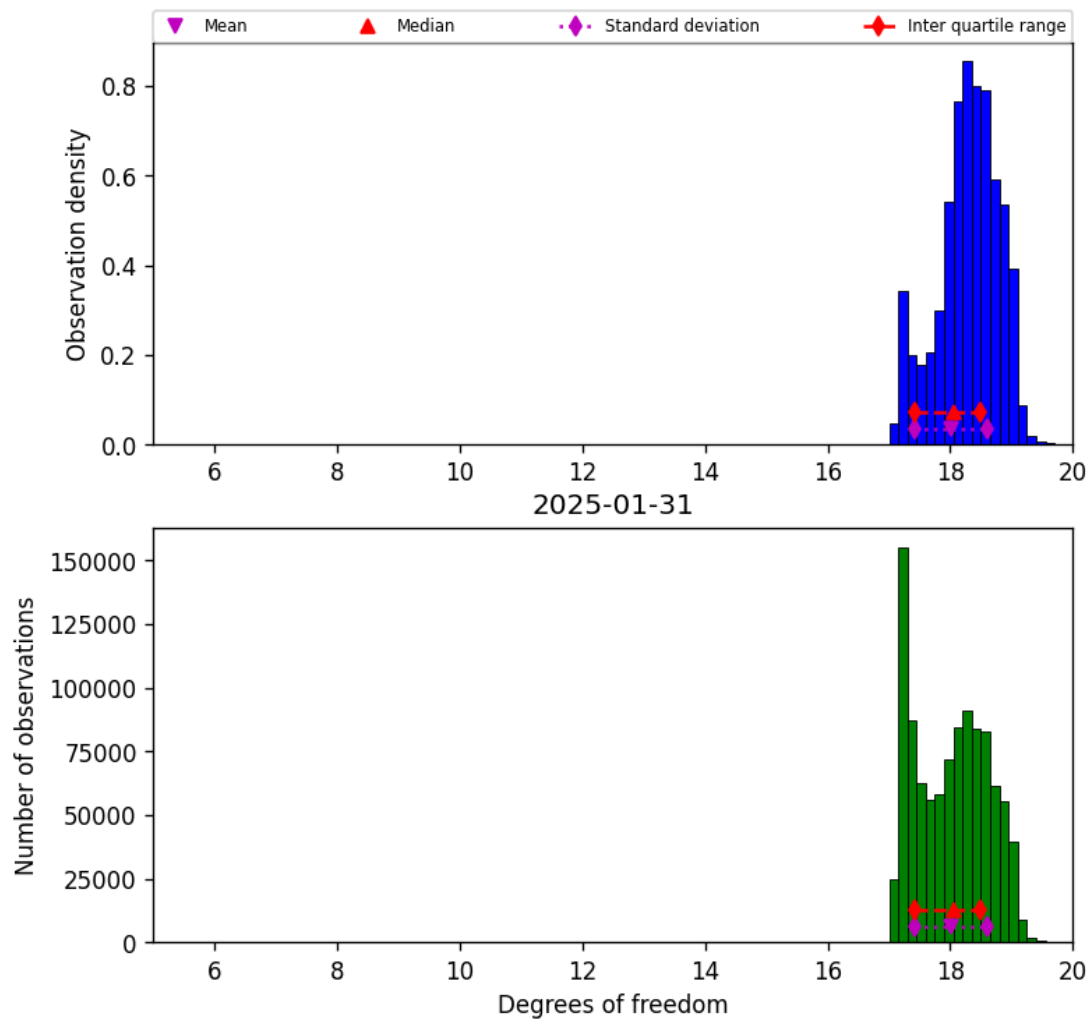
Figure 30: Histogram of “Degrees of freedom” for 2025-01-30 to 2025-02-01
