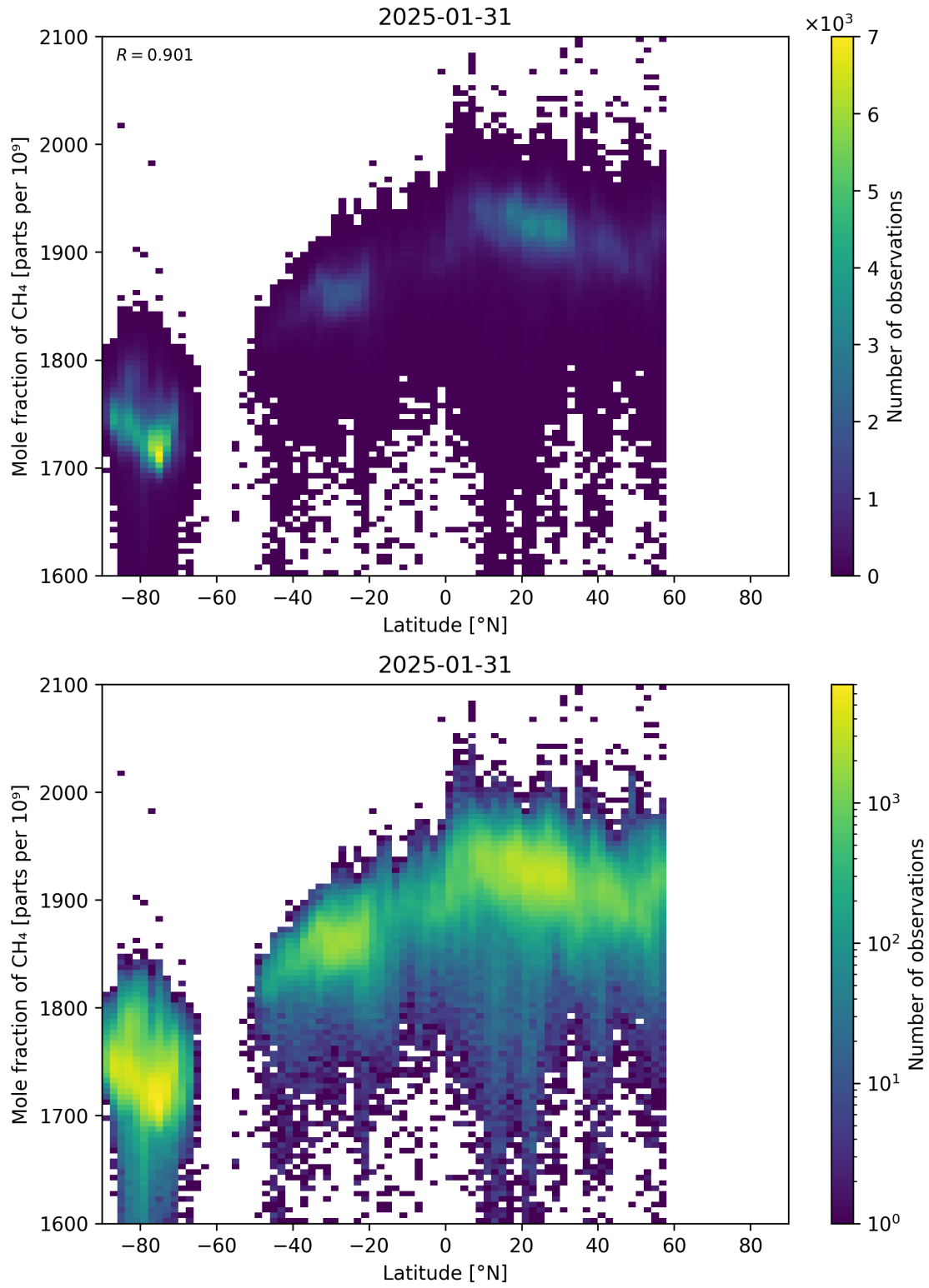
Figure 57: Scatter density plot of “Latitude” against “Mole fraction of CH 4 ” for 2025-01-30 to 2025-02-01.
