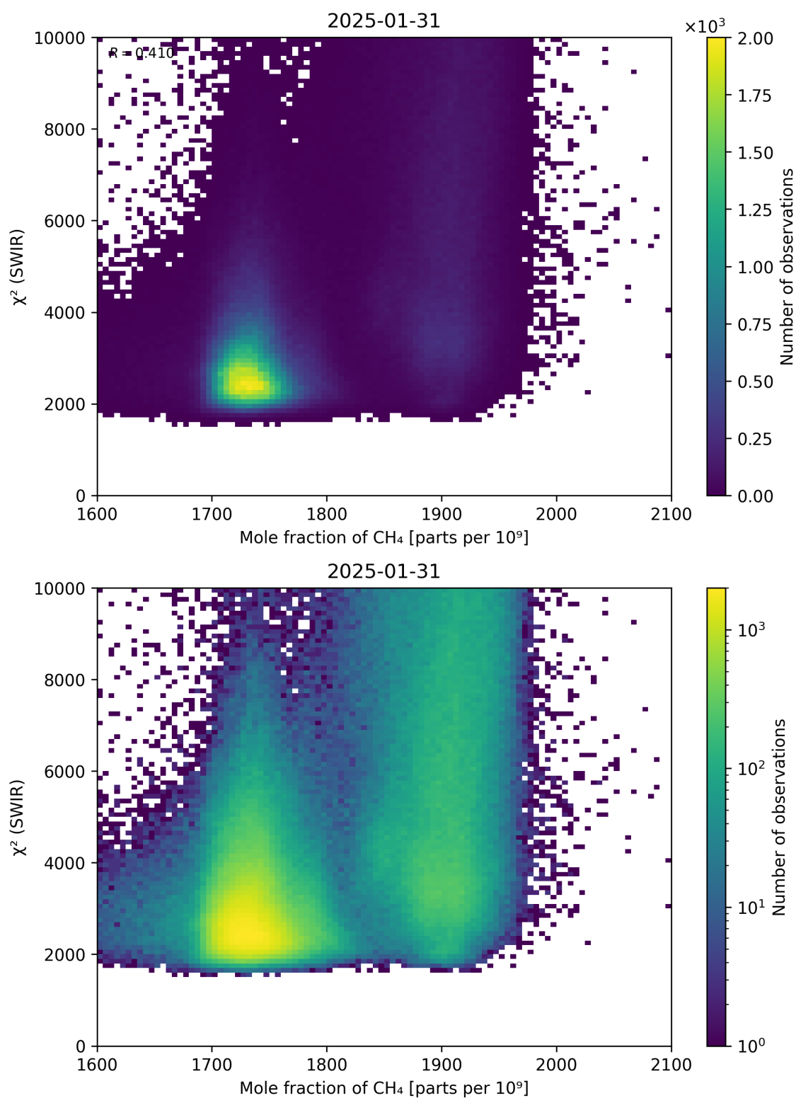
Figure 71: Scatter density plot of “Mole fraction of \text{CH}_4 ” against “ \chi^2 (SWIR)” for 2025-01-30 to 2025-02-01.
