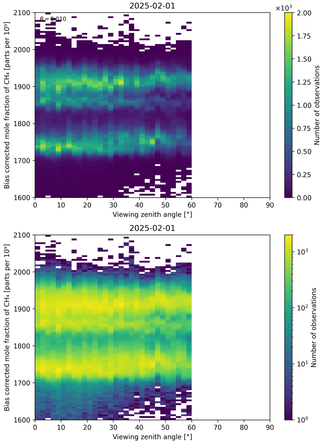
Figure 111: Scatter density plot of “Viewing zenith angle” against “Bias corrected mole fraction of CH 4 ” for 2025-01-31 to 2025-02-02.
