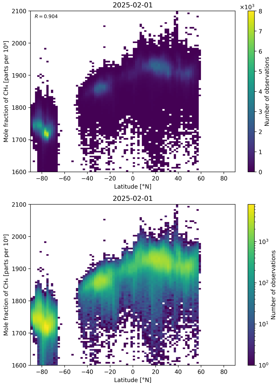
Figure 57: Scatter density plot of “Latitude” against “Mole fraction of CH 4 ” for 2025-01-31 to 2025-02-02.
