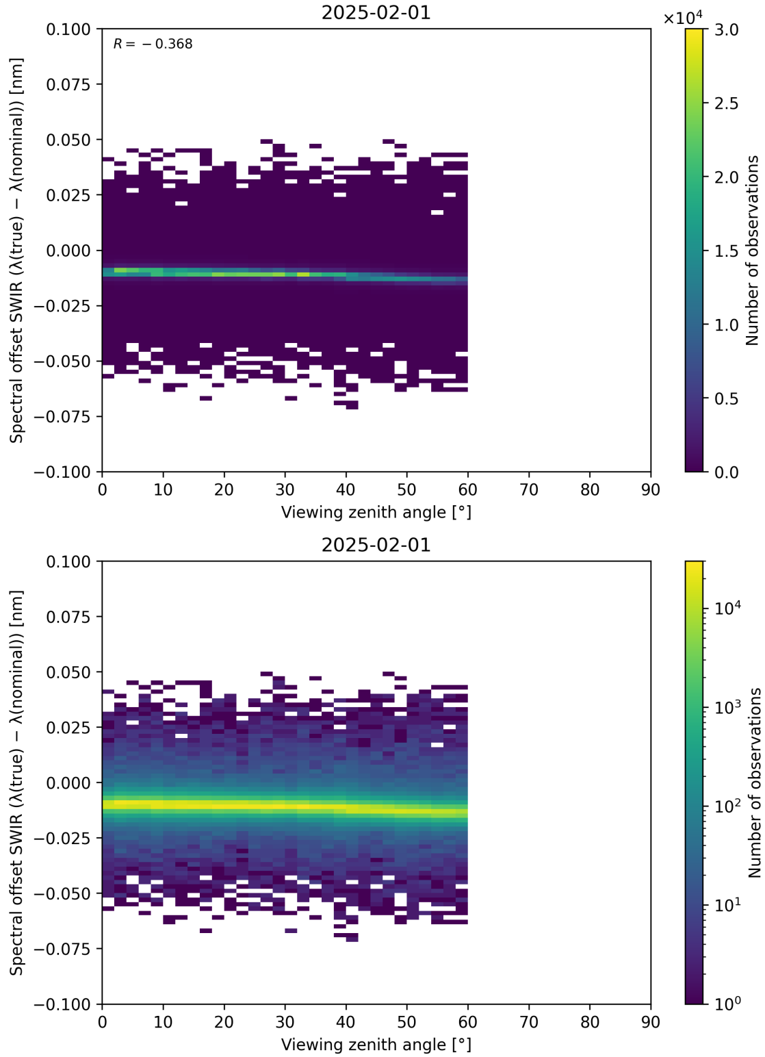
Figure 116: Scatter density plot of “Viewing zenith angle” against “Spectral offset SWIR ( \lambda_{\text{true}} - \lambda_{\text{nominal}} )” for 2025-01-31 to 2025-02-02.
