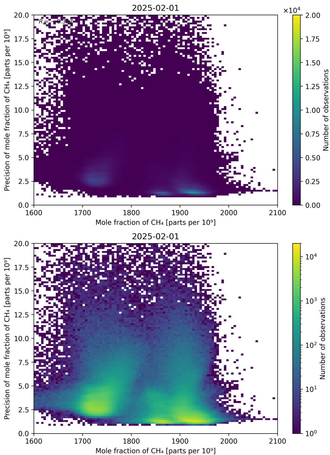
Figure 75: Scatter density plot of “Mole fraction of CH 4 ” against “Precision of mole fraction of CH 4 ” for 2025-01-31 to 2025-02-02.
