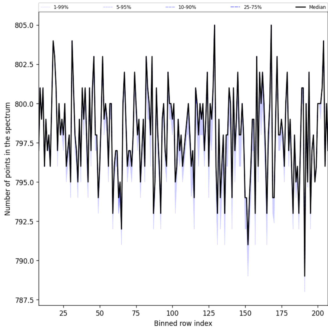
Figure 37: Along track statistics of “Number of points in the spectrum” for 2025-01-31 to 2025-02-02
