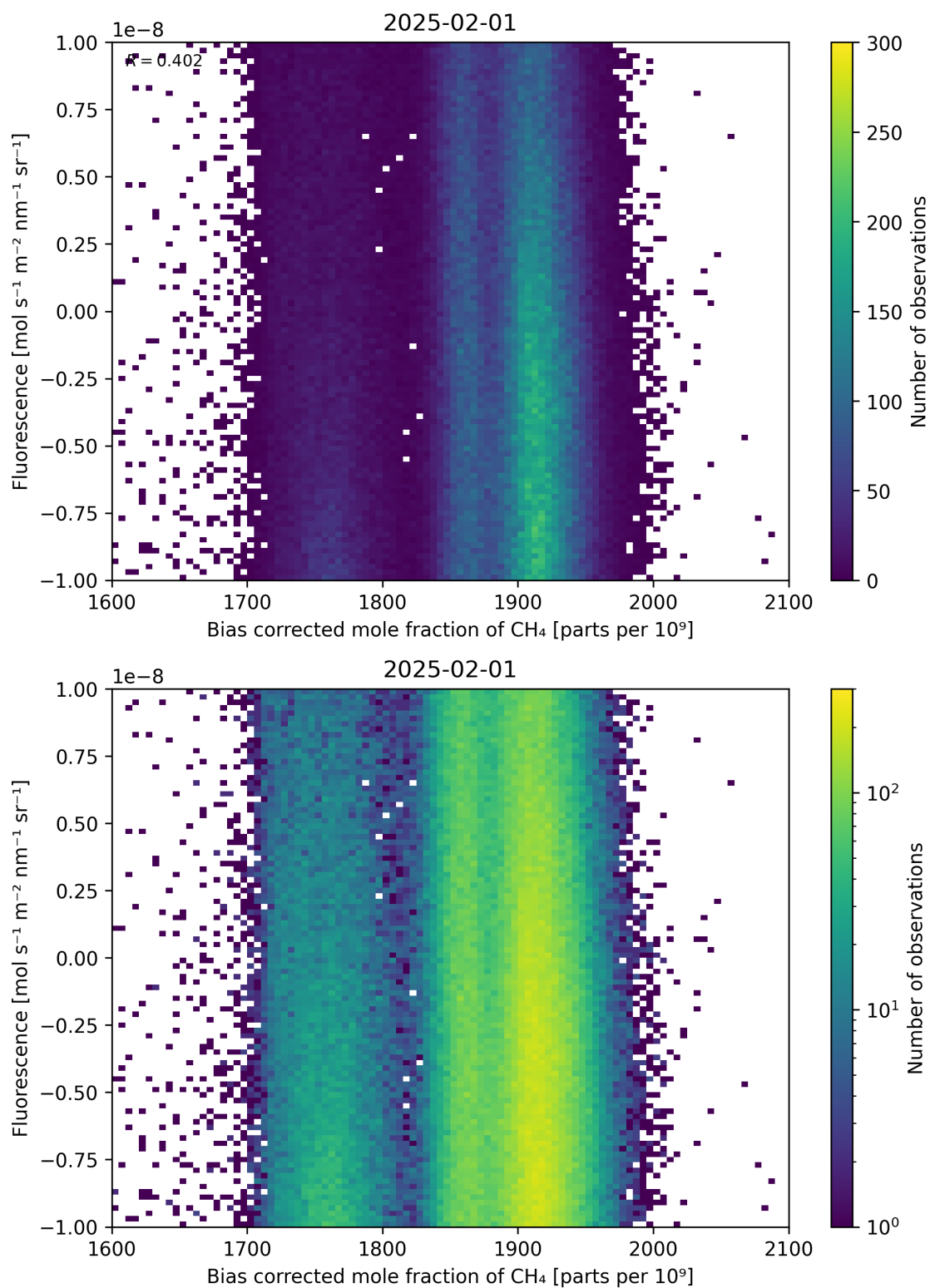
Figure 66: Scatter density plot of “Bias corrected mole fraction of \text{CH}_4 ” against “Fluorescence” for 2025-01-31 to 2025-02-02.
