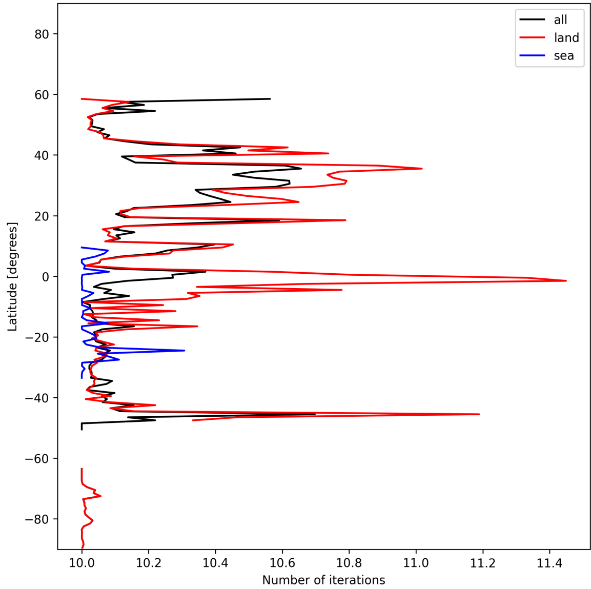
Figure 20: Zonal average of “Number of iterations” for 2025-01-31 to 2025-02-02.
