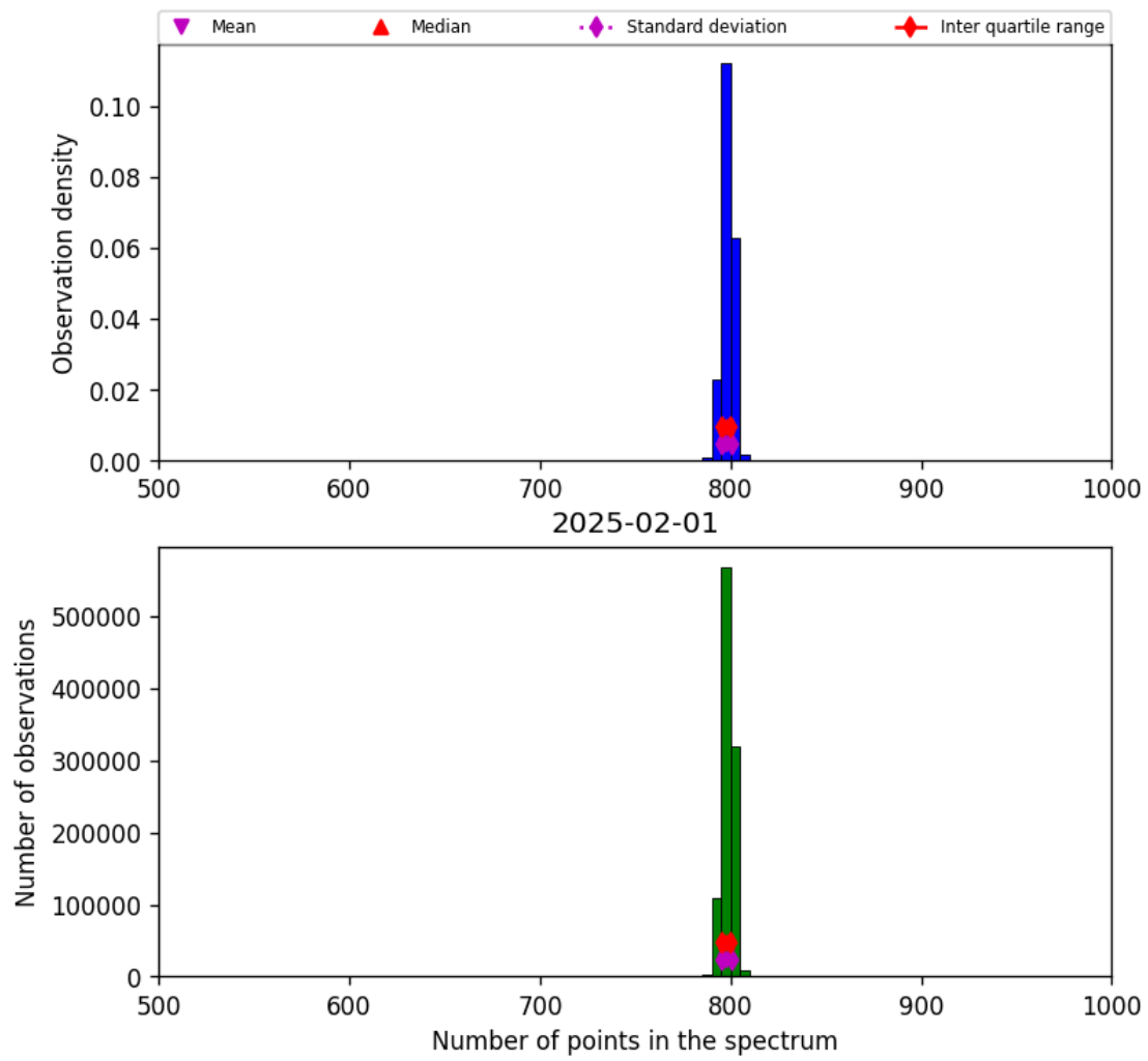
Figure 26: Histogram of “Number of points in the spectrum” for 2025-01-31 to 2025-02-02
