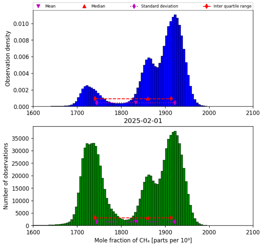
Figure 23: Histogram of “Mole fraction of CH 4 ” for 2025-01-31 to 2025-02-02
