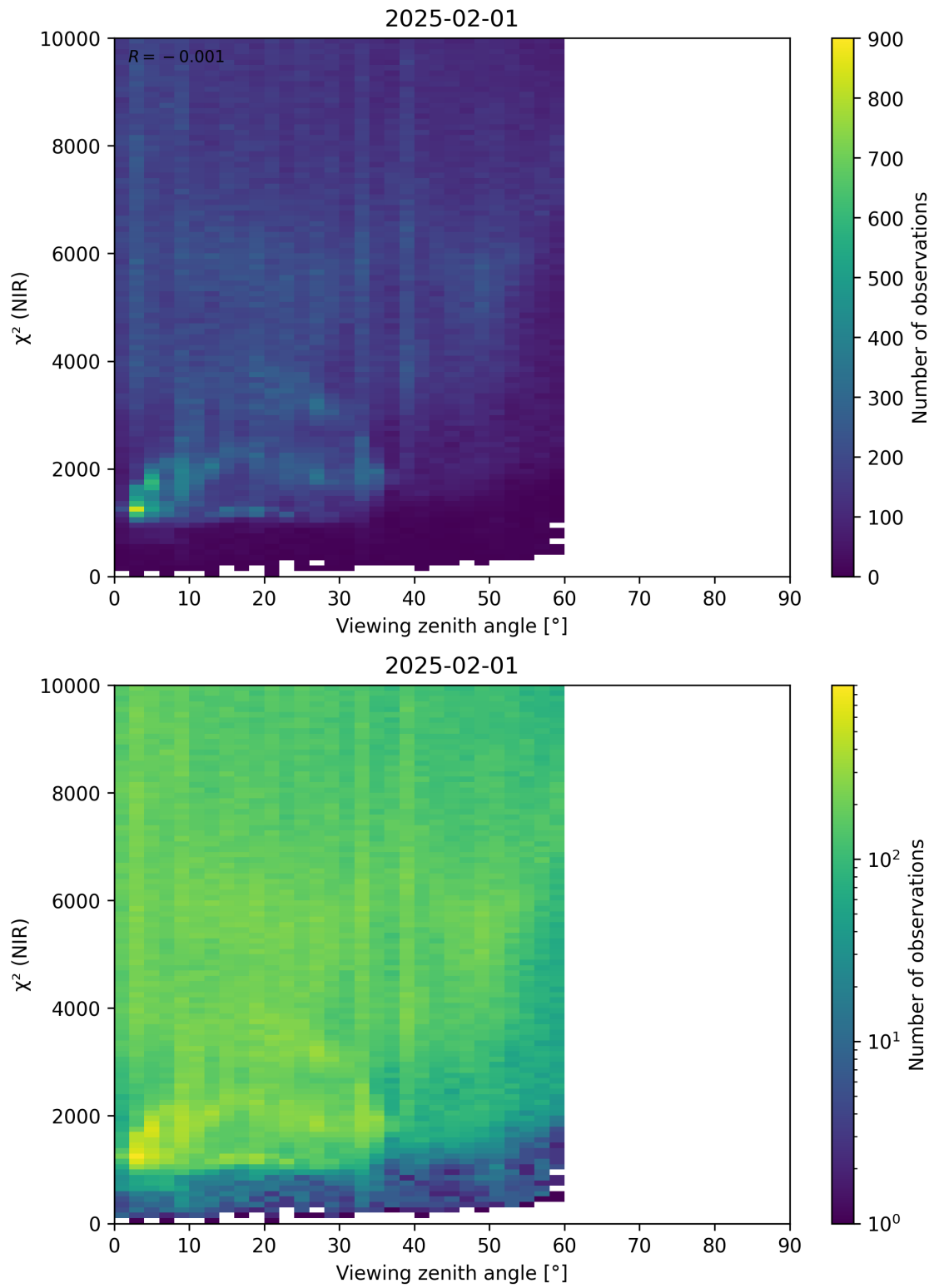
Figure 105: Scatter density plot of “Viewing zenith angle” against “ \chi^2 (NIR)” for 2025-01-31 to 2025-02-02.
