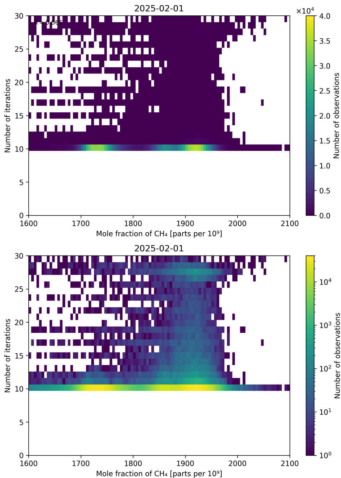
Figure 76: Scatter density plot of “Mole fraction of CH 4 ” against “Number of iterations” for 2025-01-31 to 2025-02-02.
