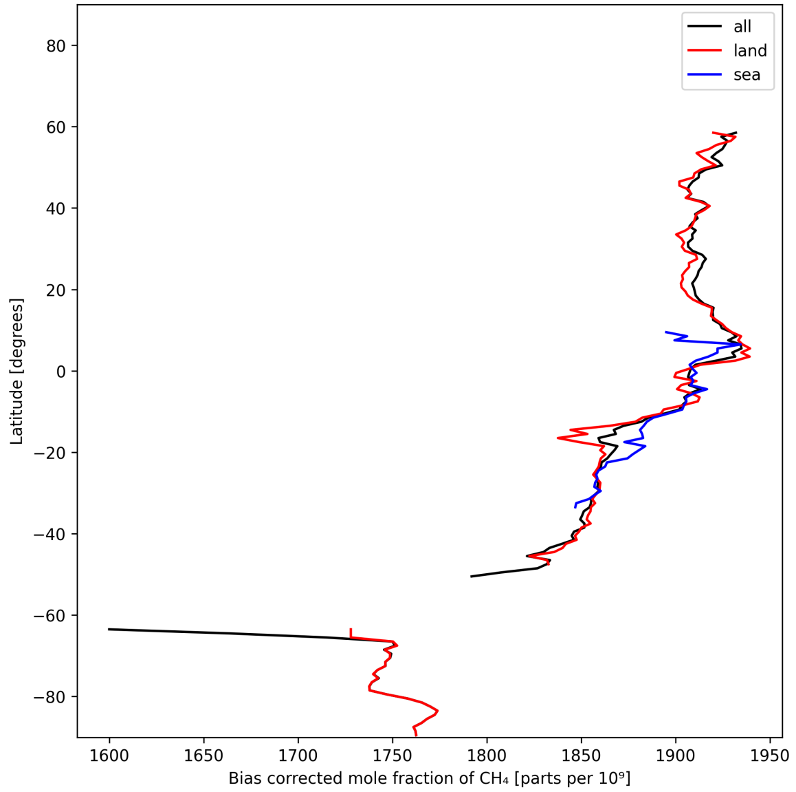
Figure 14: Zonal average of “Bias corrected mole fraction of CH 4 ” for 2025-01-31 to 2025-02-02.
