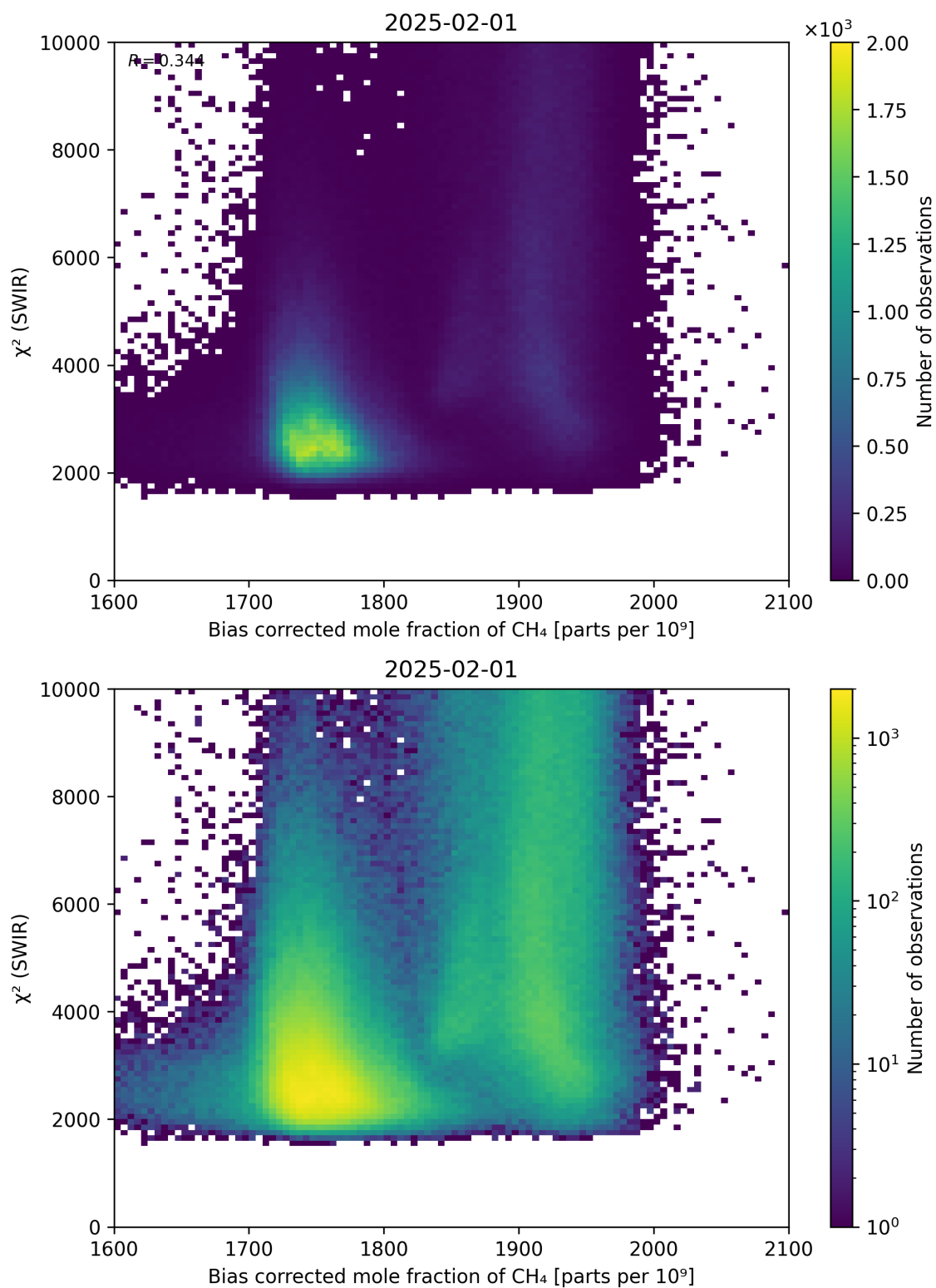
Figure 64: Scatter density plot of “Bias corrected mole fraction of \text{CH}_4 ” against “ \chi^2 (SWIR)” for 2025-01-31 to 2025-02-02.
