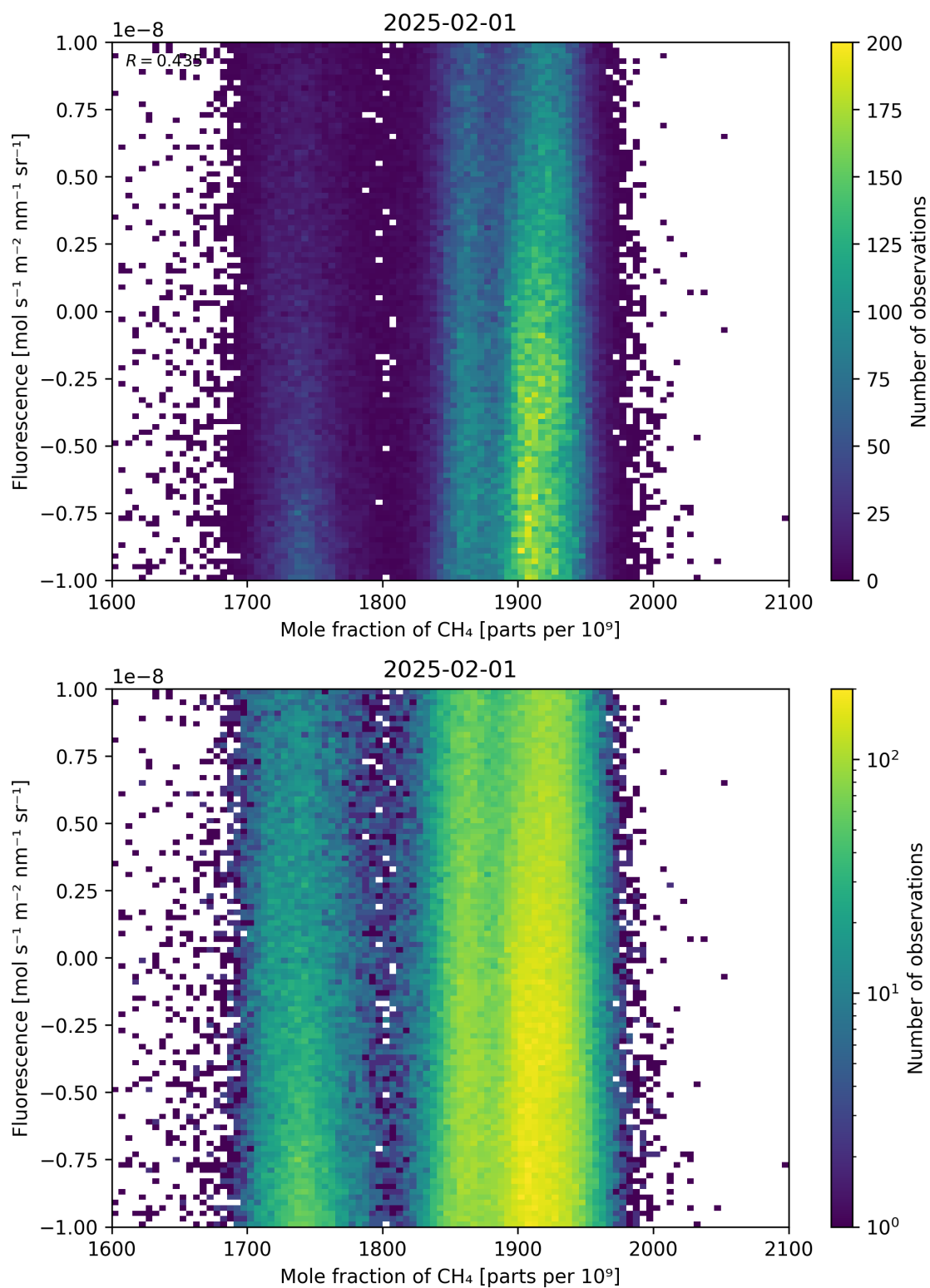
Figure 73: Scatter density plot of “Mole fraction of \text{CH}_4 ” against “Fluorescence” for 2025-01-31 to 2025-02-02.
