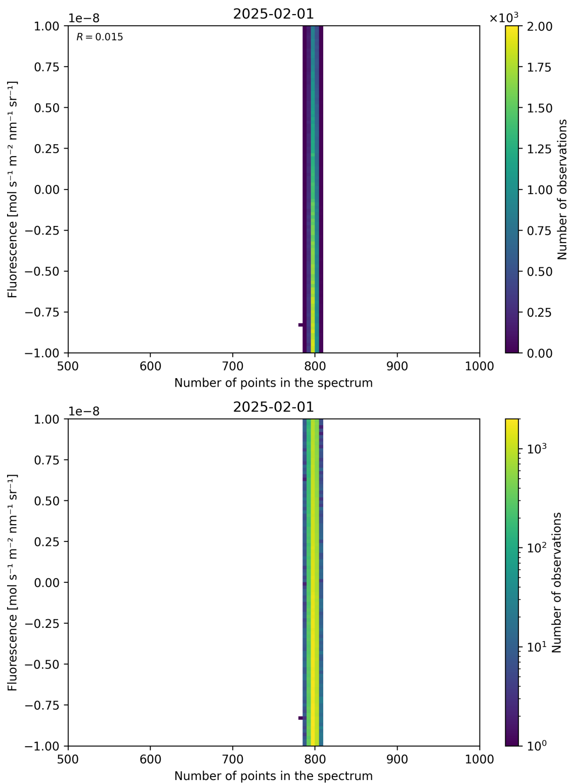
Figure 91: Scatter density plot of “Number of points in the spectrum” against “Fluorescence” for 2025-01-31 to 2025-02-02.
