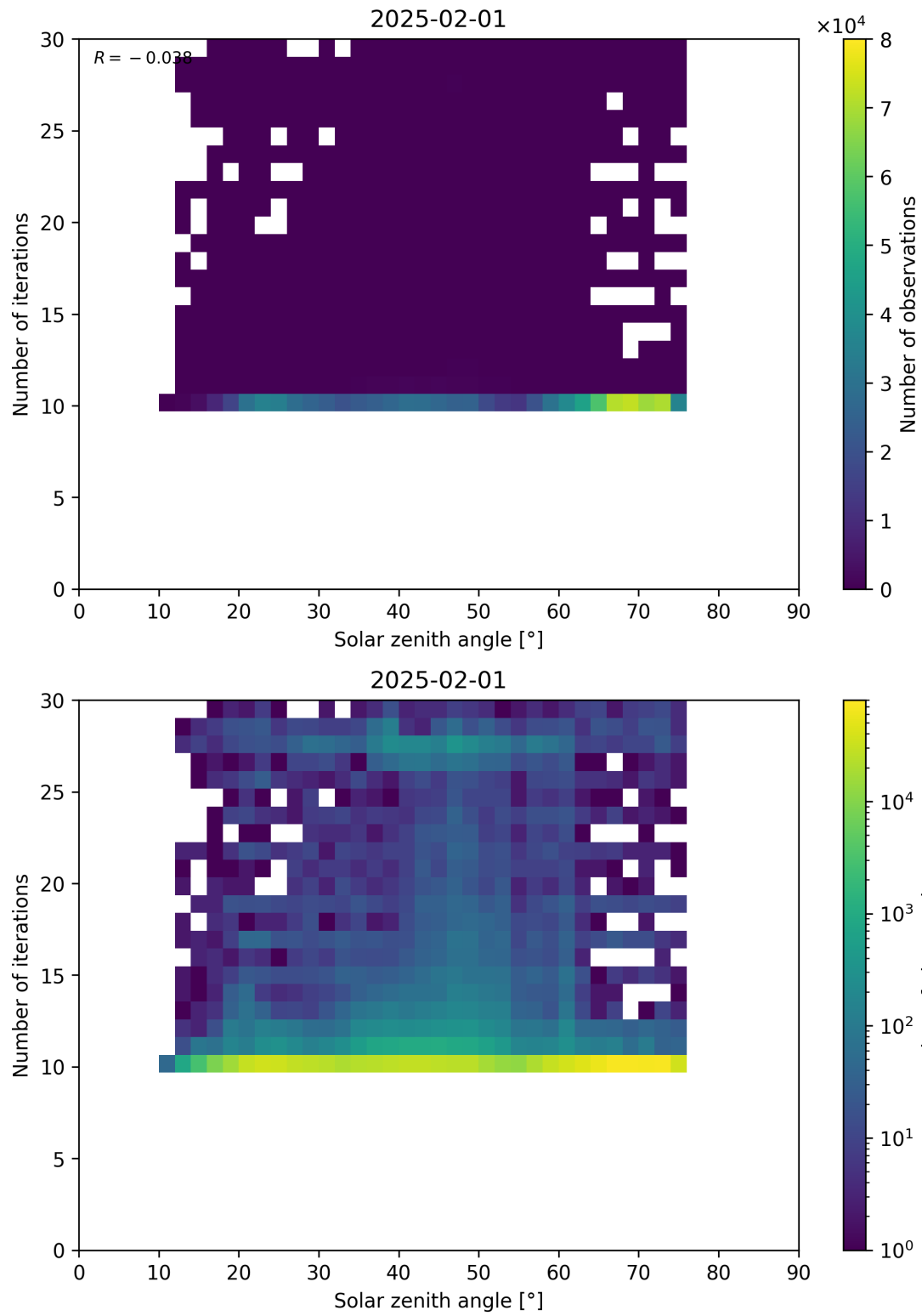
Figure 102: Scatter density plot of “Solar zenith angle” against “Number of iterations” for 2025-01-31 to 2025-02-02.
