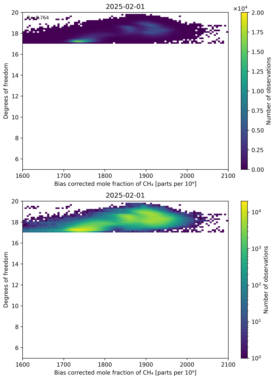
Figure 65: Scatter density plot of “Bias corrected mole fraction of CH 4 ” against “Degrees of freedom” for 2025-01-31 to 2025-02-02.
