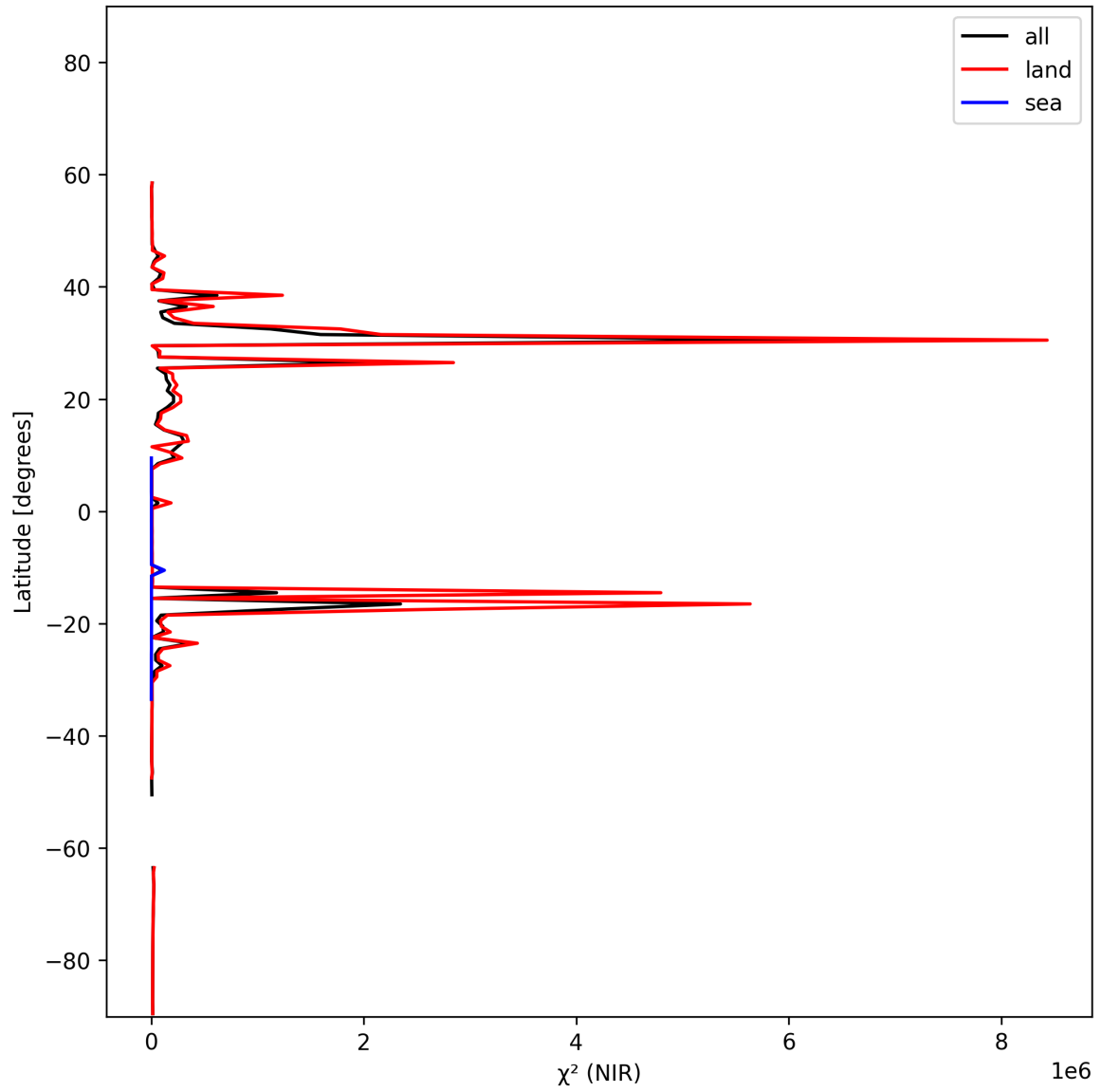
Figure 18: Zonal average of “ \chi^2 (NIR)” for 2025-01-31 to 2025-02-02.
