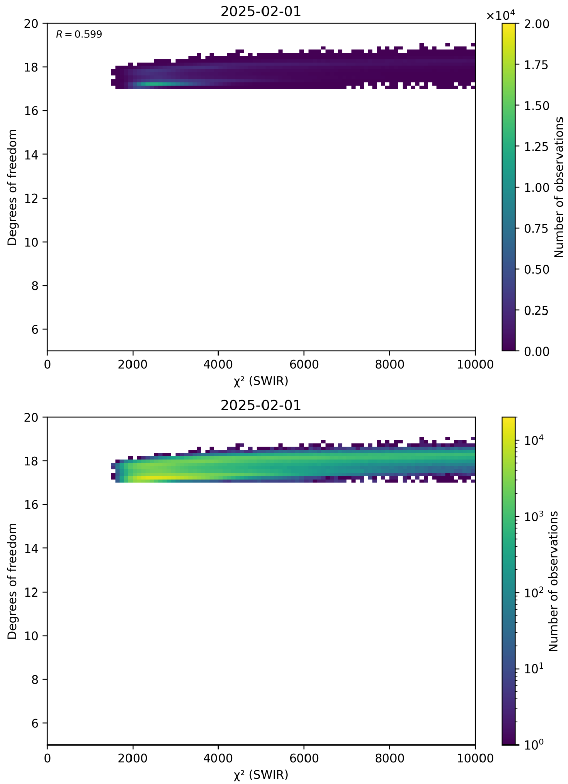
Figure 48: Scatter density plot of “ \chi^2 (SWIR)” against “Degrees of freedom” for 2025-01-31 to 2025-02-02.
