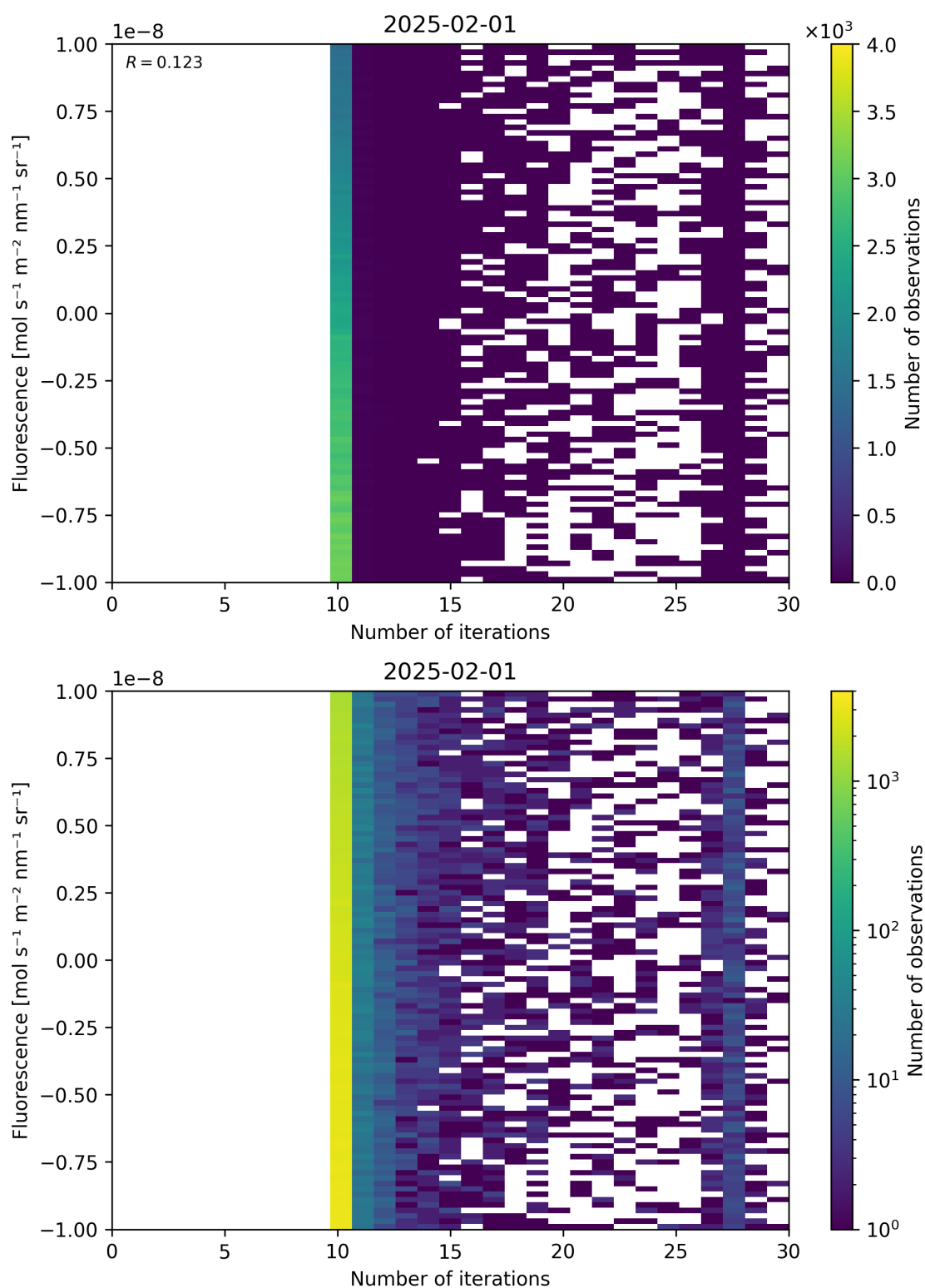
Figure 87: Scatter density plot of "Number of iterations" against "Fluorescence" for 2025-01-31 to 2025-02-02.
