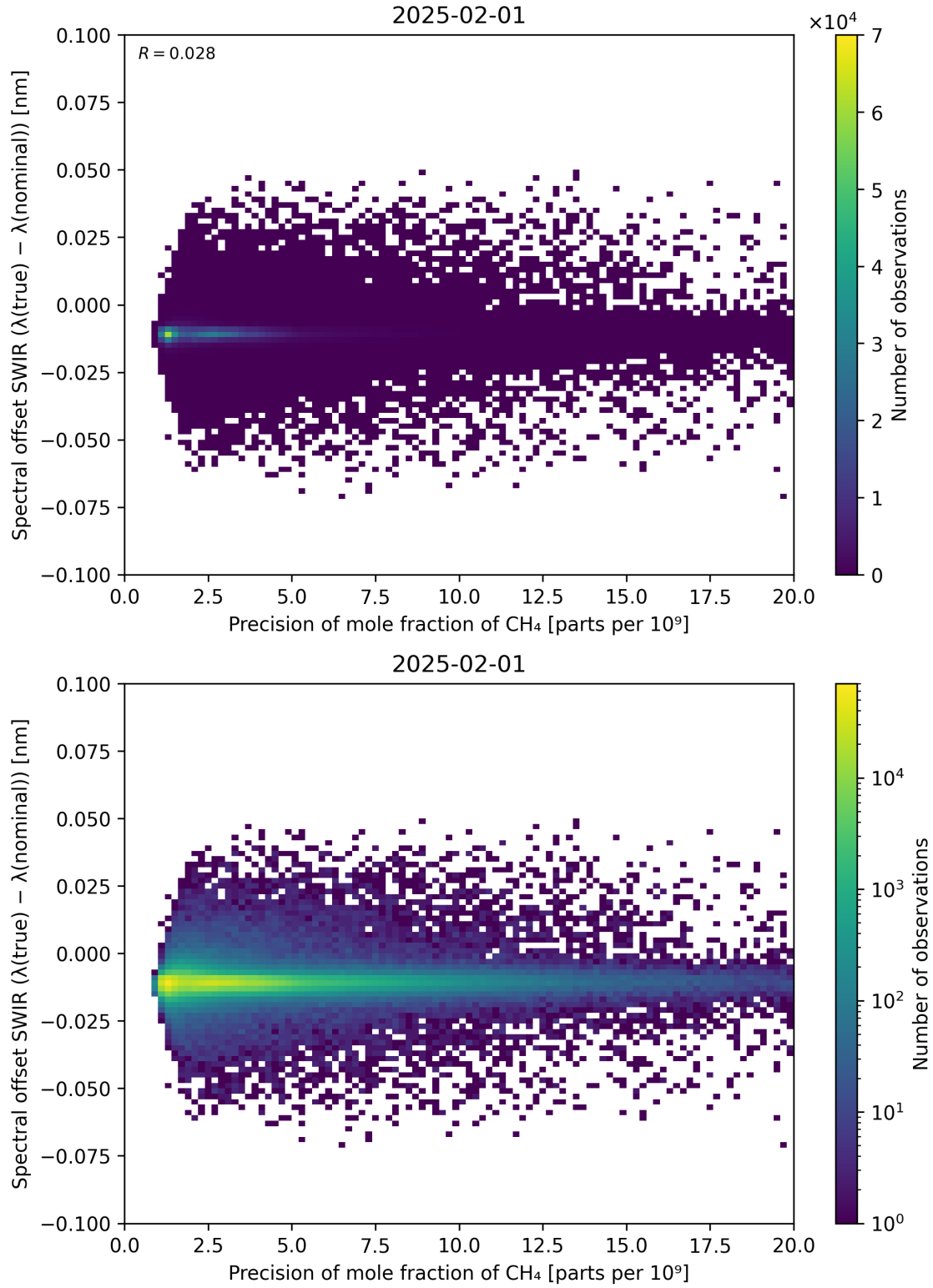
Figure 85: Scatter density plot of “Precision of mole fraction of \text{CH}_4 ” against “Spectral offset SWIR ( \lambda_{\text{true}} - \lambda_{\text{nominal}} )” for 2025-01-31 to 2025-02-02.
