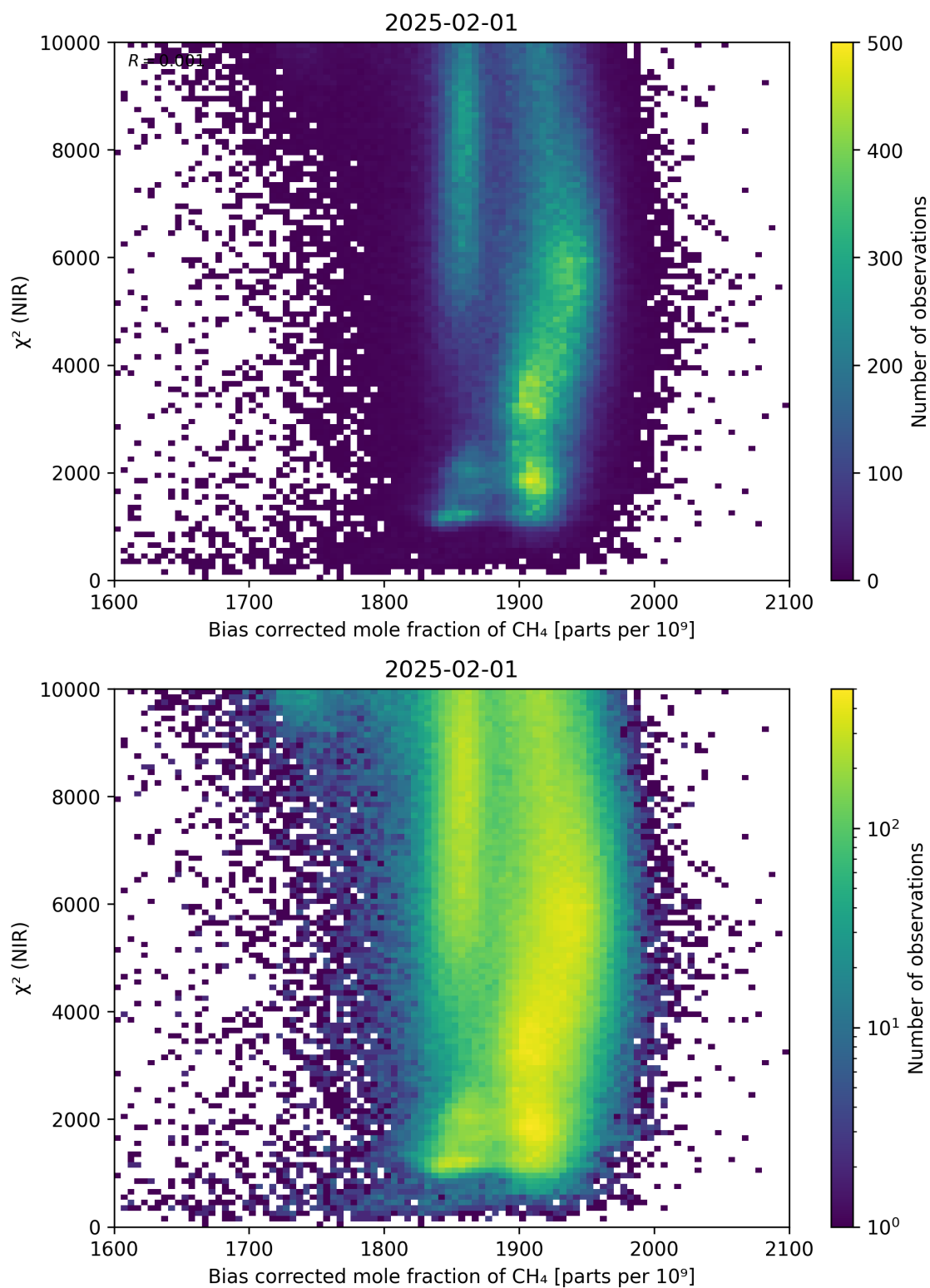
Figure 63: Scatter density plot of “Bias corrected mole fraction of \text{CH}_4 ” against “ \chi^2 (NIR)” for 2025-01-31 to 2025-02-02.
