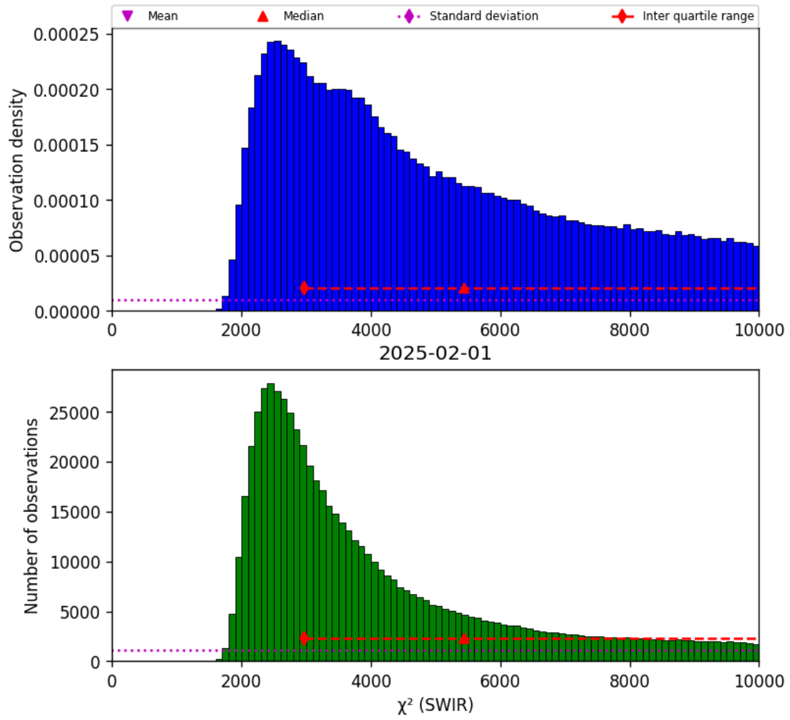
Figure 28: Histogram of “ \chi^2 (SWIR)” for 2025-01-31 to 2025-02-02
