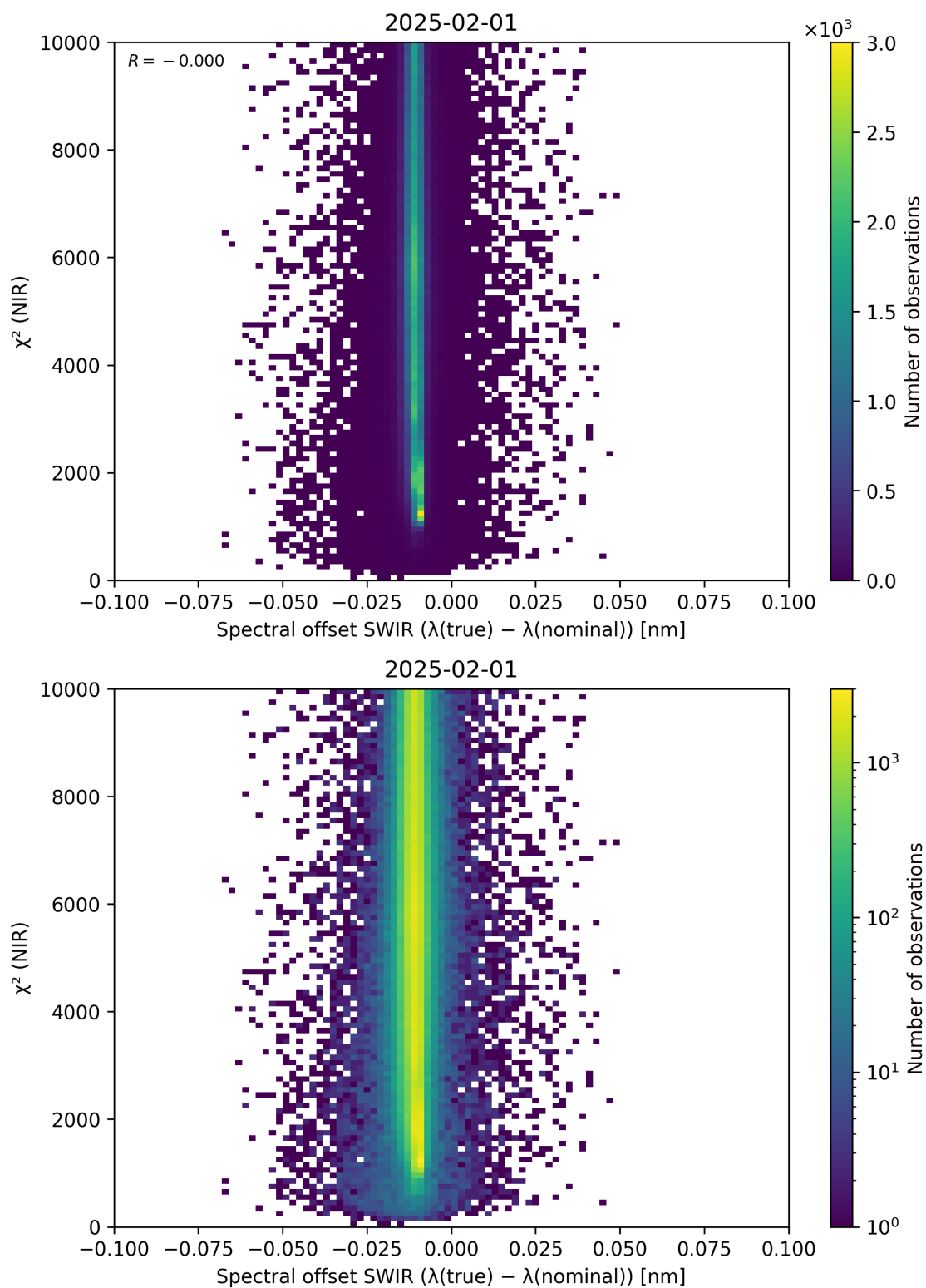
Figure 117: Scatter density plot of “Spectral offset SWIR ( \lambda_{\text{true}} - \lambda_{\text{nominal}} )” against “ \chi^2 (NIR)” for 2025-01-31 to 2025-02-02.
