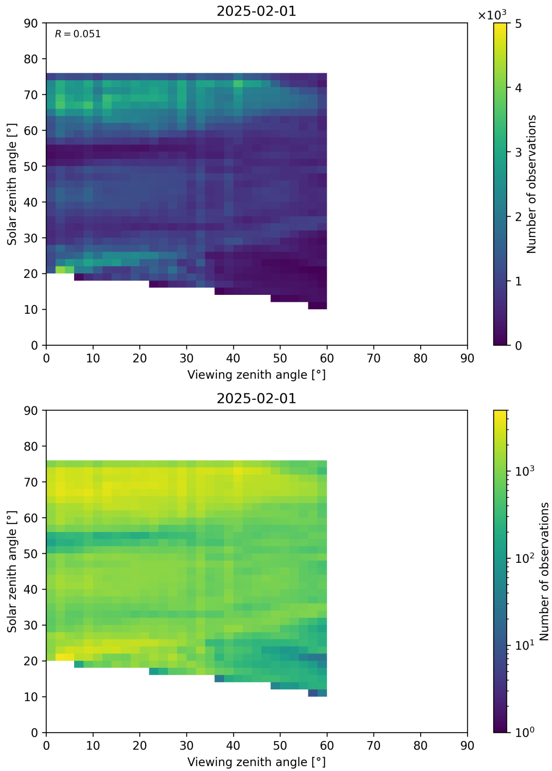
Figure 115: Scatter density plot of “Viewing zenith angle” against “Solar zenith angle” for 2025-01-31 to 2025-02-02.
