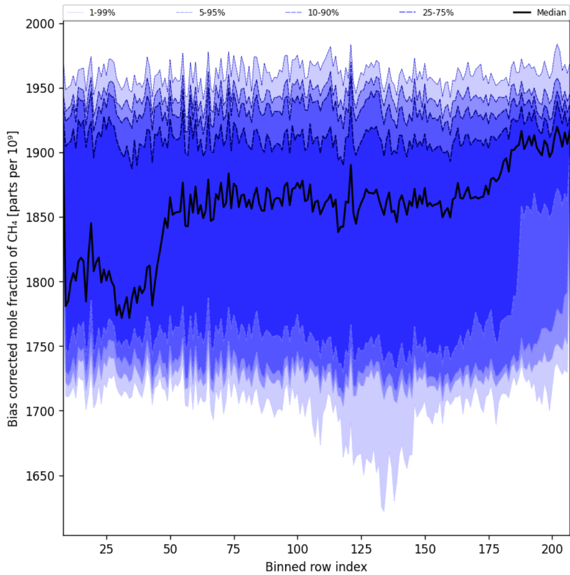
Figure 36: Along track statistics of “Bias corrected mole fraction of CH 4 ” for 2025-01-31 to 2025-02-02
