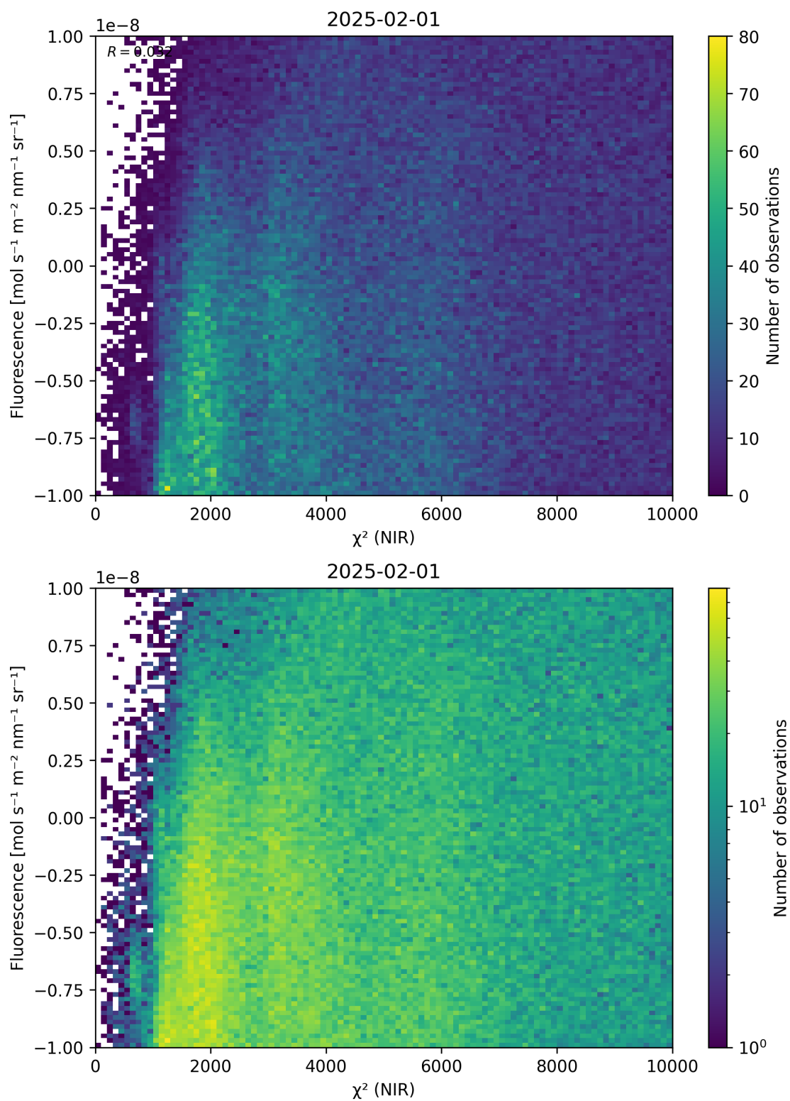
Figure 45: Scatter density plot of “ \chi^2 (NIR)” against “Fluorescence” for 2025-01-31 to 2025-02-02.
