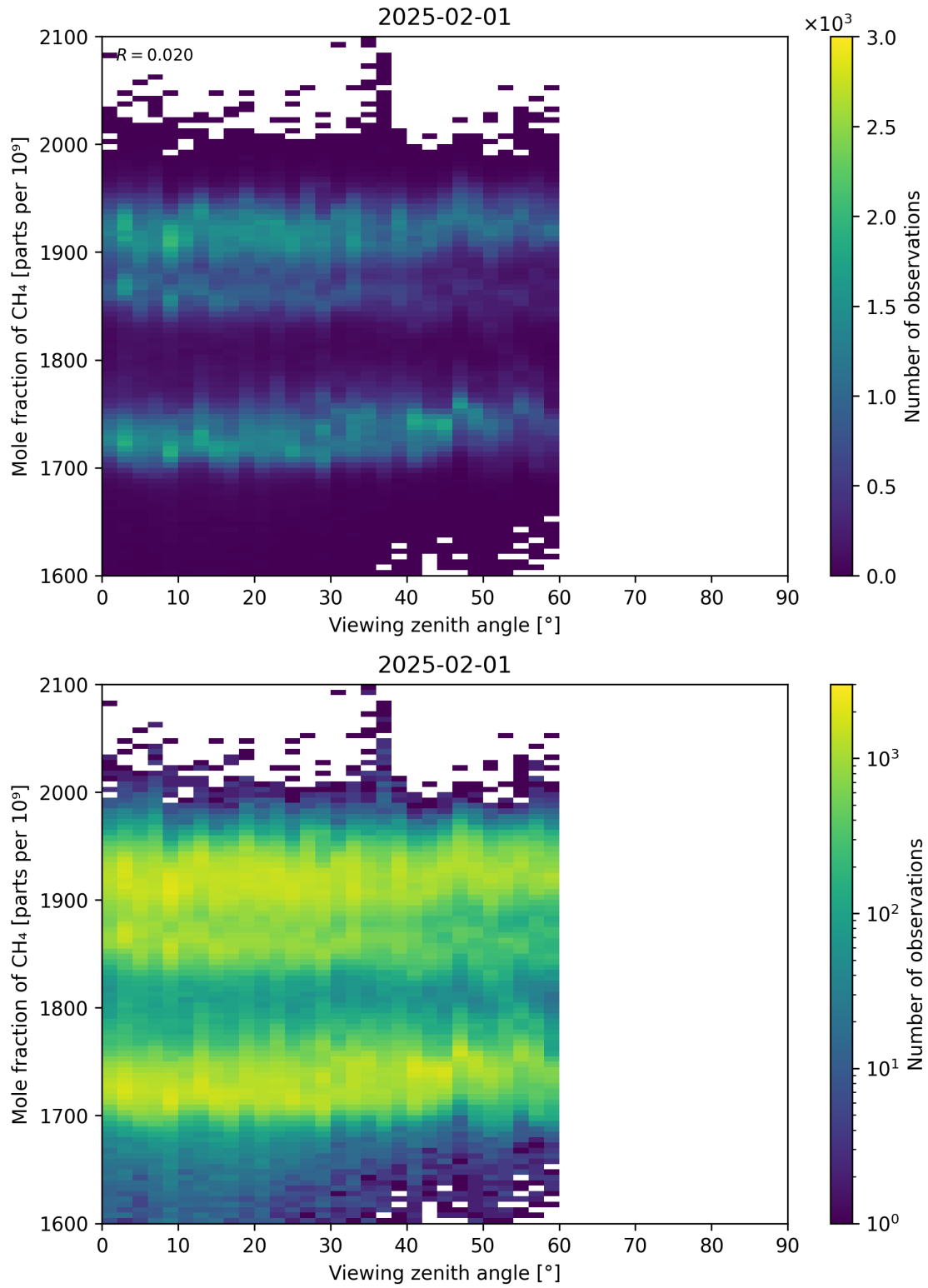
Figure 110: Scatter density plot of “Viewing zenith angle” against “Mole fraction of CH 4 ” for 2025-01-31 to 2025-02-02.
