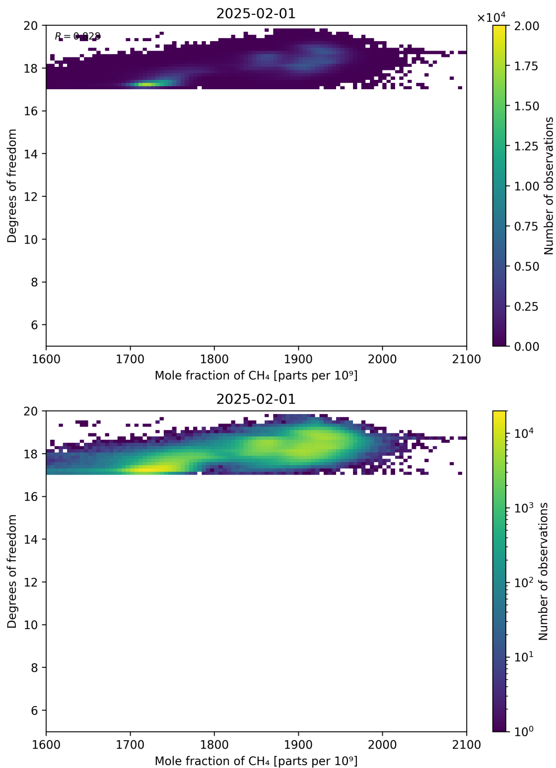
Figure 72: Scatter density plot of “Mole fraction of CH 4 ” against “Degrees of freedom” for 2025-01-31 to 2025-02-02.
