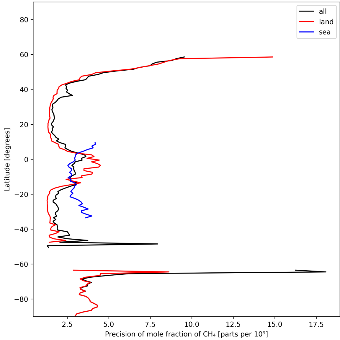
Figure 13: Zonal average of “Precision of mole fraction of CH 4 ” for 2025-01-31 to 2025-02-02.
