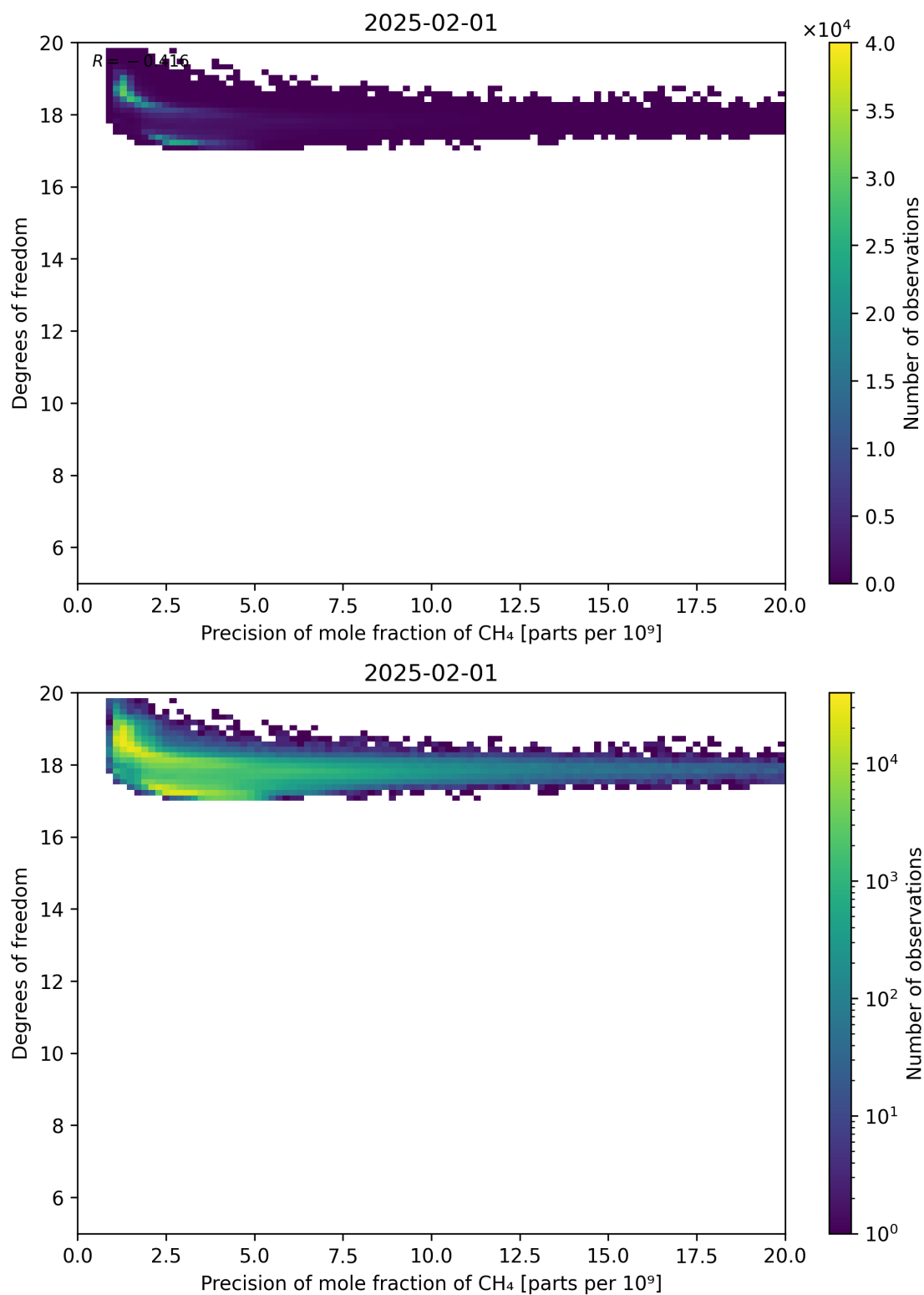
Figure 80: Scatter density plot of “Precision of mole fraction of CH 4 ” against “Degrees of freedom” for 2025-01-31 to 2025-02-02.
