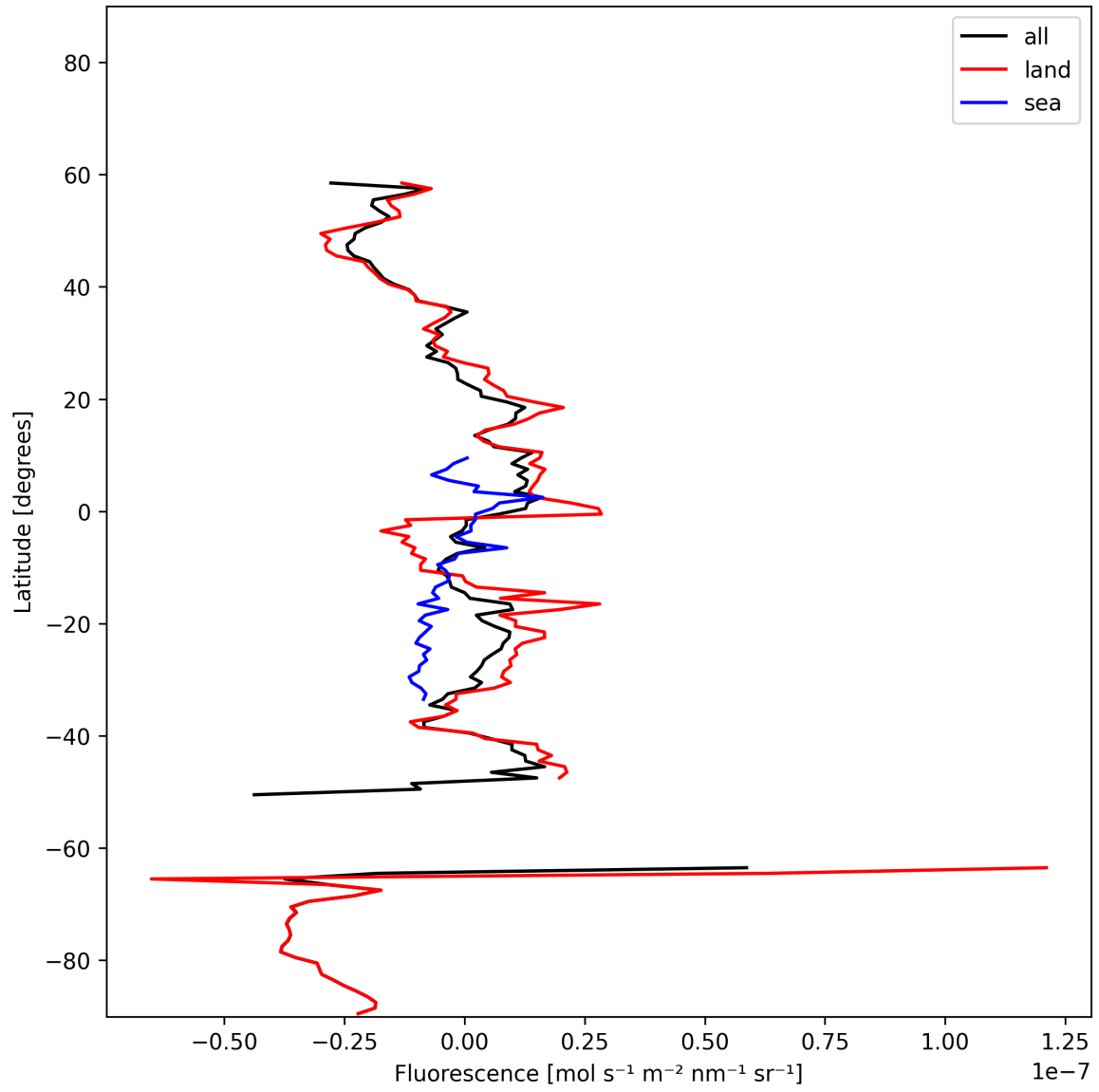
Figure 21: Zonal average of “Fluorescence” for 2025-01-31 to 2025-02-02.
