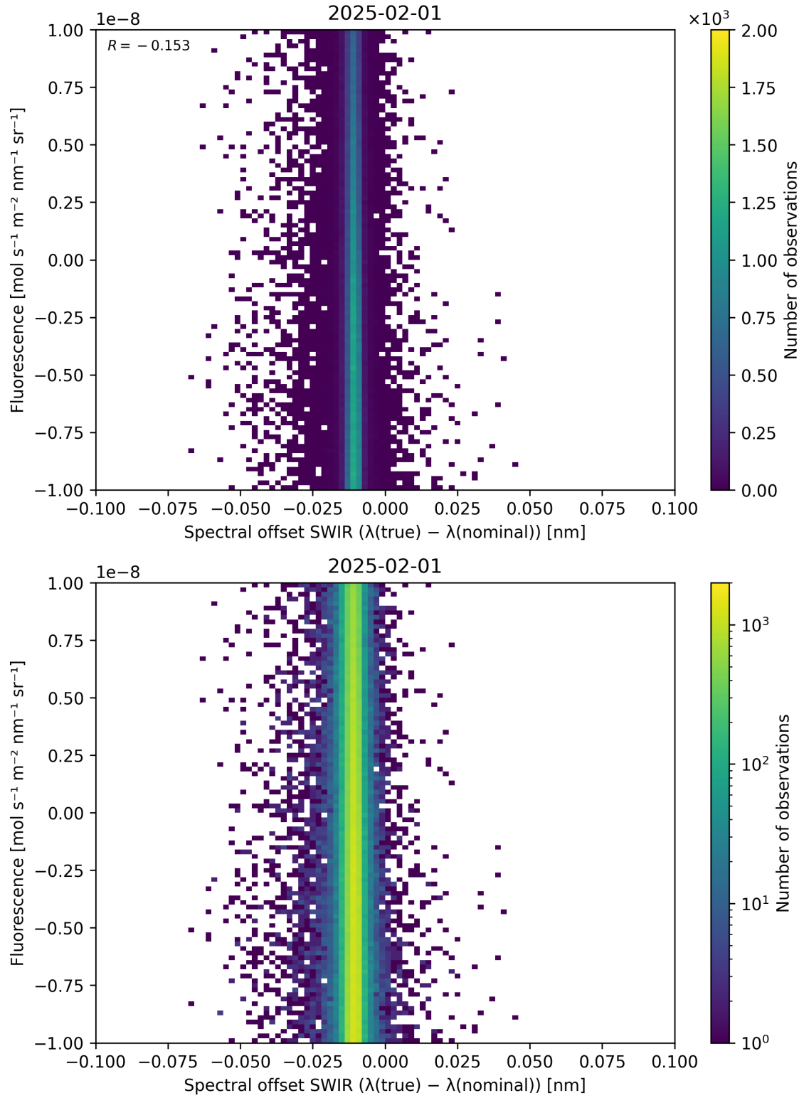
Figure 120: Scatter density plot of “Spectral offset SWIR ( \lambda_{\text{true}} - \lambda_{\text{nominal}} )” against “Fluorescence” for 2025-01-31 to 2025-02-02.
