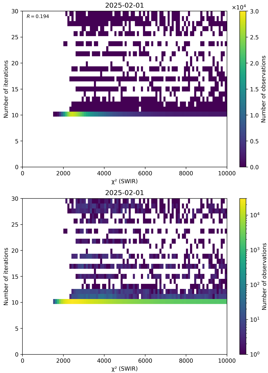
Figure 50: Scatter density plot of “ \chi^2 (SWIR)” against “Number of iterations” for 2025-01-31 to 2025-02-02.
