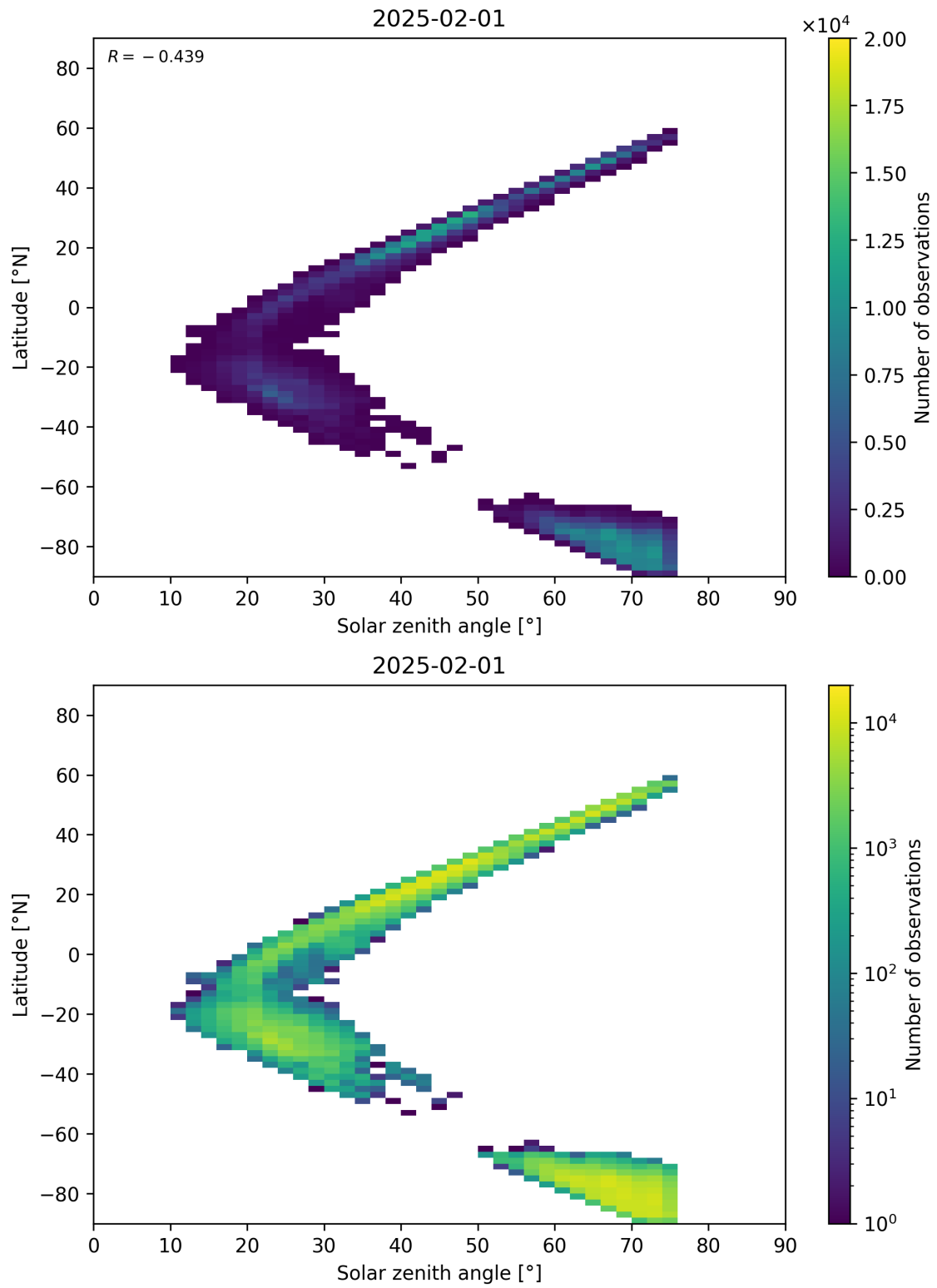
Figure 98: Scatter density plot of “Solar zenith angle” against “Latitude” for 2025-01-31 to 2025-02-02.
