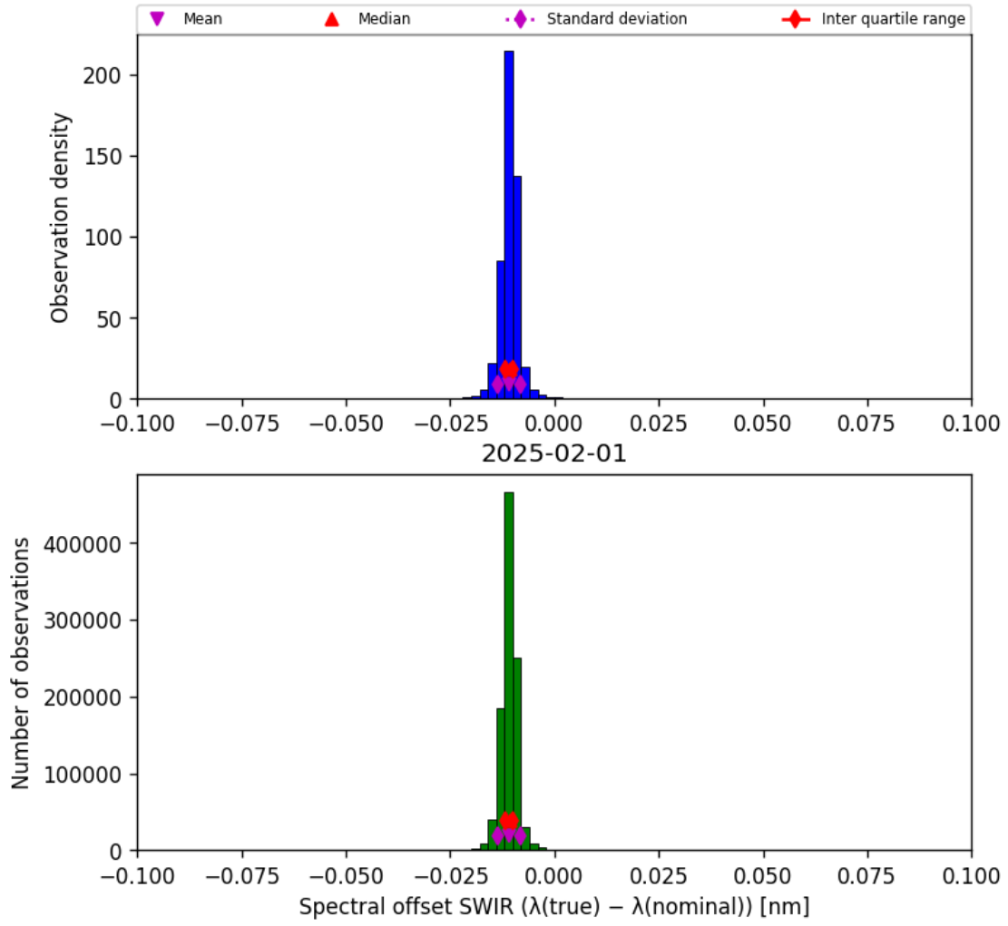
Figure 27: Histogram of “Spectral offset SWIR ( \lambda_{\text{true}} - \lambda_{\text{nominal}} )” for 2025-01-31 to 2025-02-02
