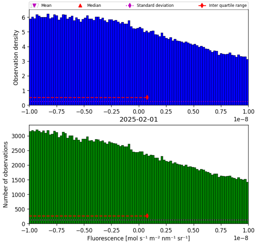
Figure 32: Histogram of “Fluorescence” for 2025-01-31 to 2025-02-02
