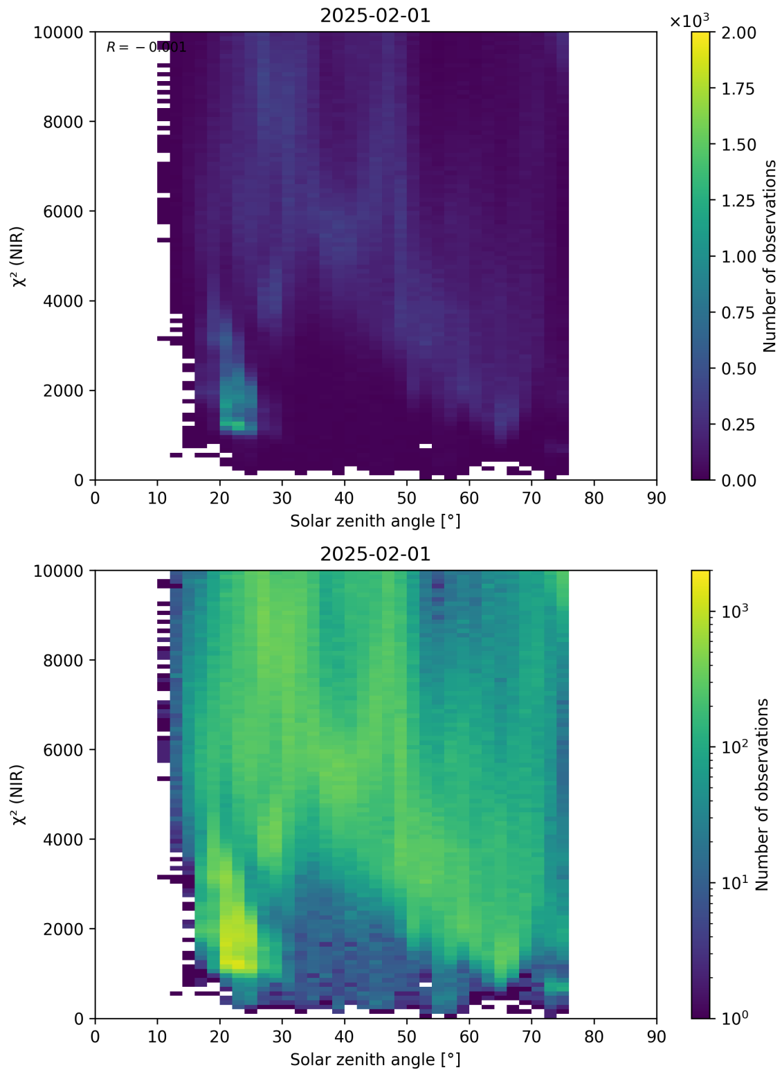
Figure 94: Scatter density plot of “Solar zenith angle” against “ \chi^2 (NIR)” for 2025-01-31 to 2025-02-02.
