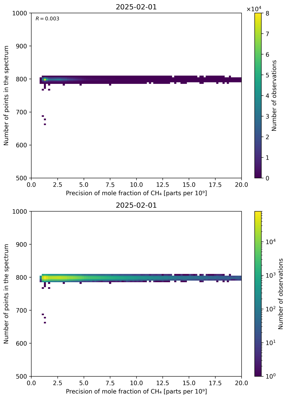
Figure 84: Scatter density plot of “Precision of mole fraction of CH 4 ” against “Number of points in the spectrum” for 2025-01-31 to 2025-02-02.
