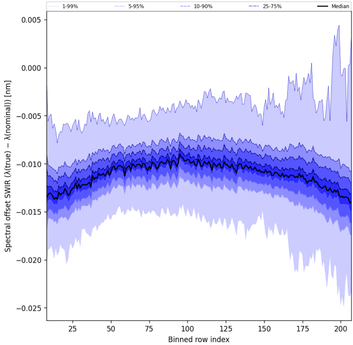
Figure 38: Along track statistics of “Spectral offset SWIR ( \lambda_{\text{true}} - \lambda_{\text{nominal}} )” for 2025-01-31 to 2025-02-02
