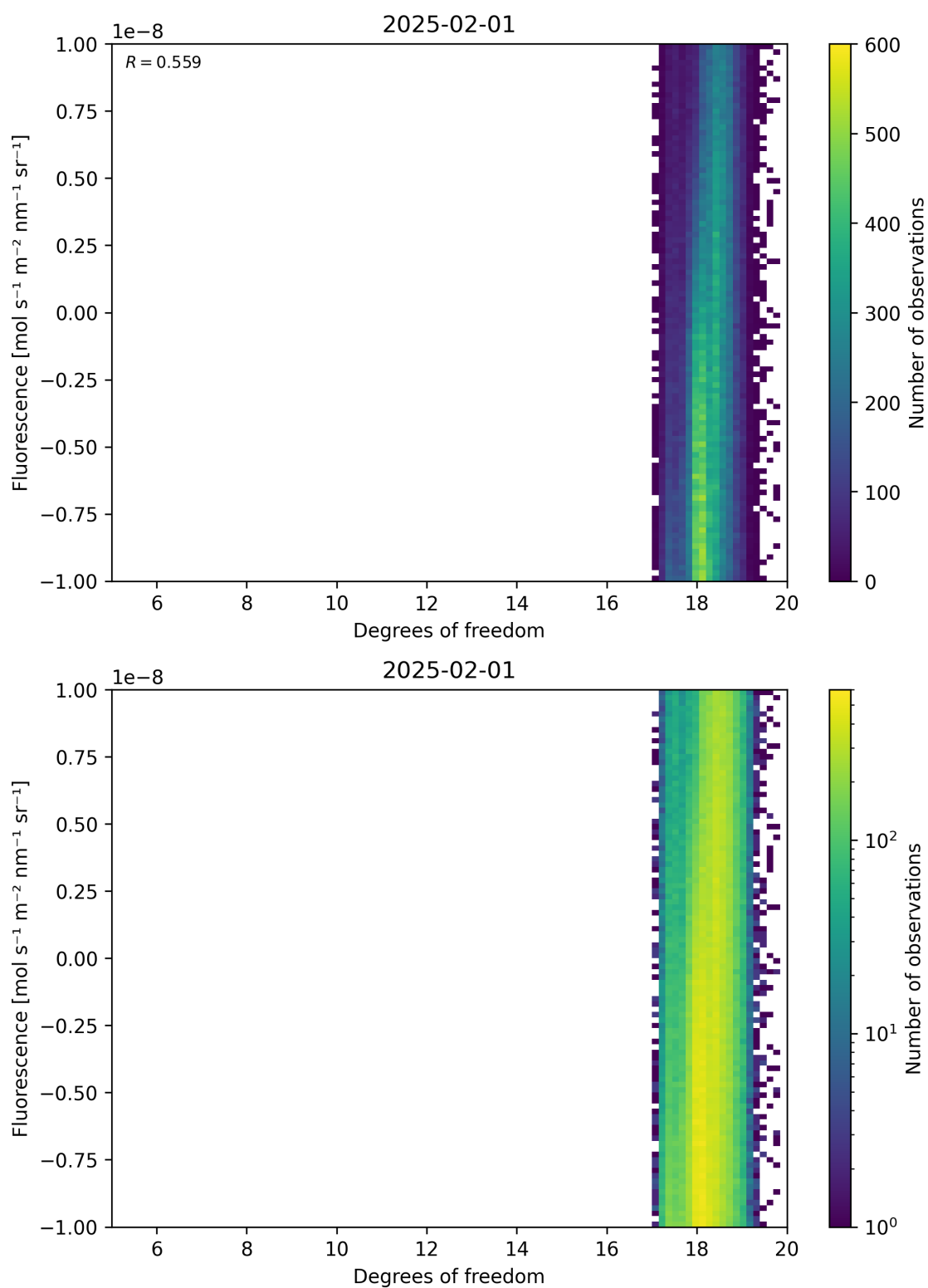
Figure 51: Scatter density plot of “Degrees of freedom” against “Fluorescence” for 2025-01-31 to 2025-02-02.
