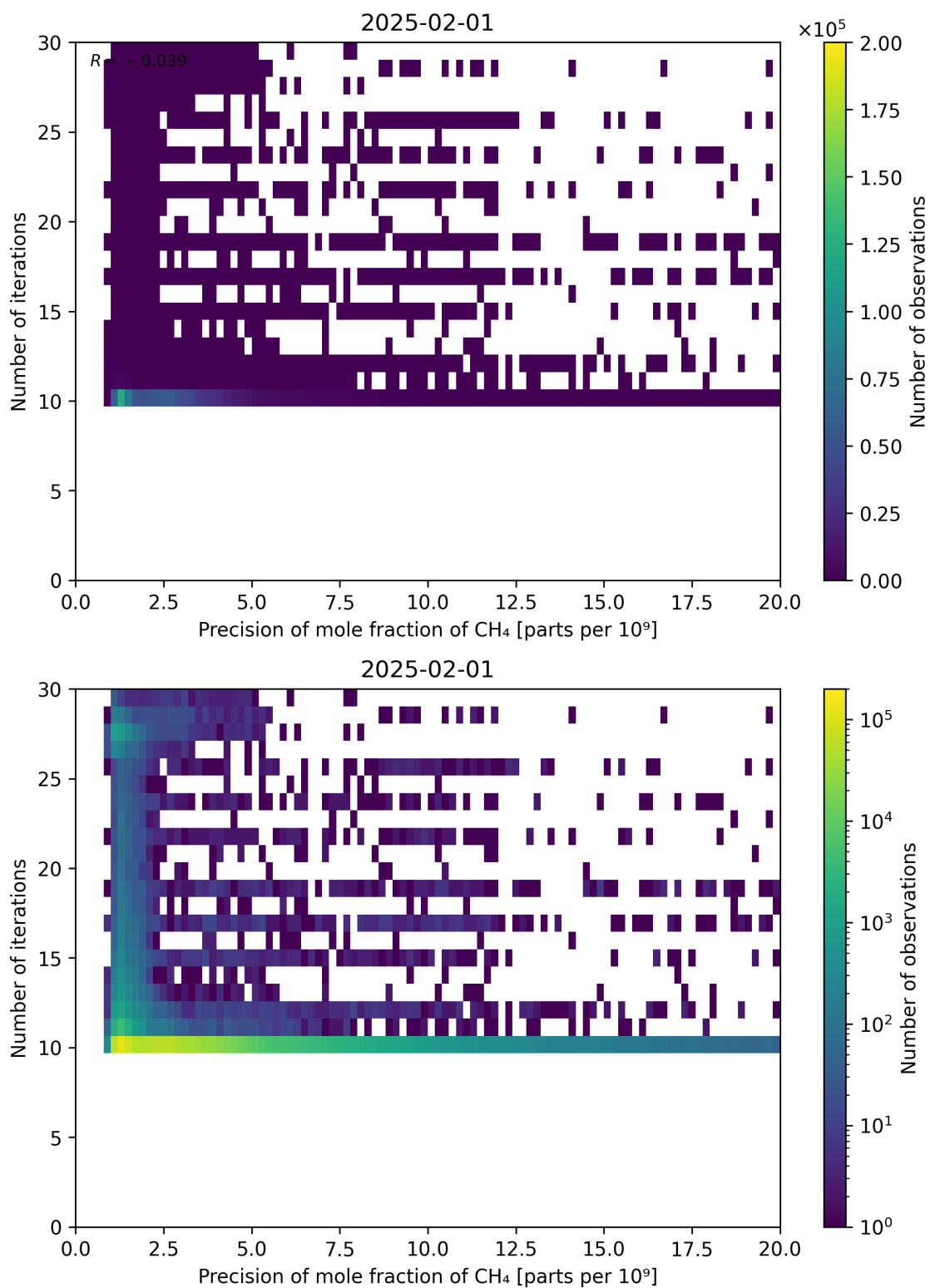
Figure 83: Scatter density plot of “Precision of mole fraction of CH 4 ” against “Number of iterations” for 2025-01-31 to 2025-02-02.
