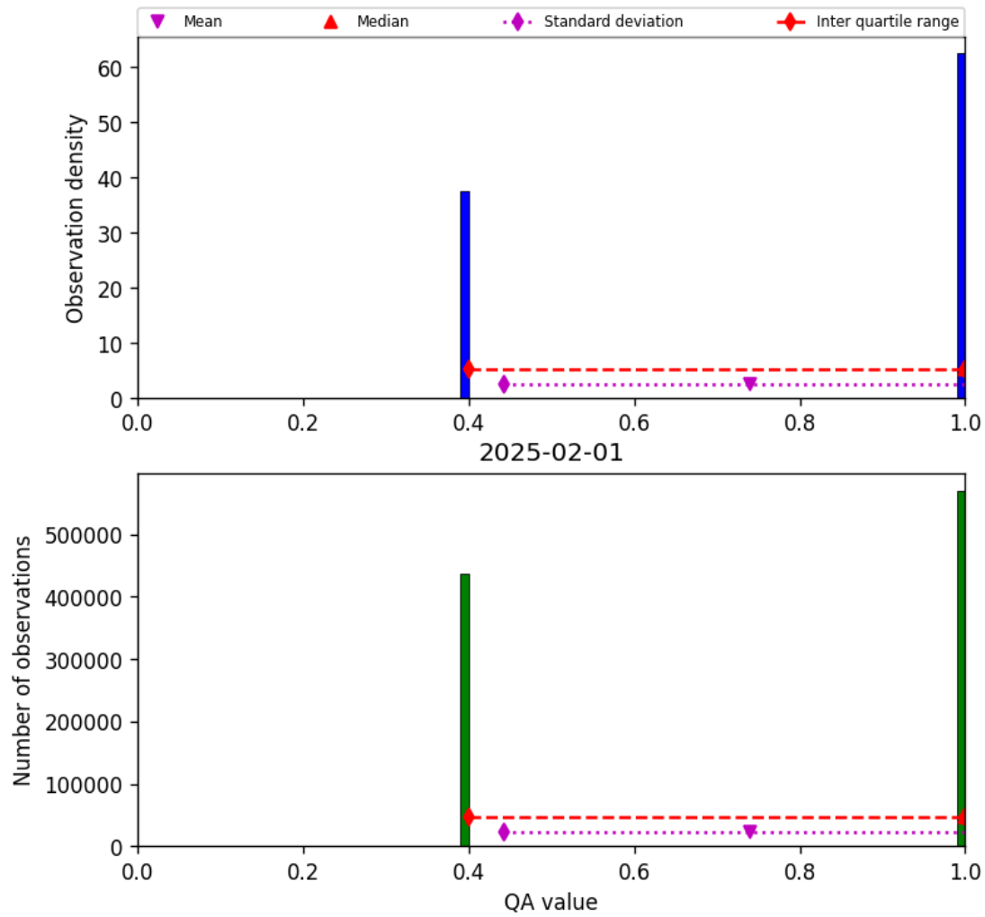
Figure 22: Histogram of “QA value” for 2025-01-31 to 2025-02-02
