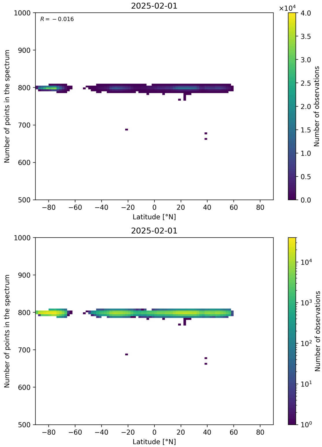
Figure 61: Scatter density plot of “Latitude” against “Number of points in the spectrum” for 2025-01-31 to 2025-02-02.
