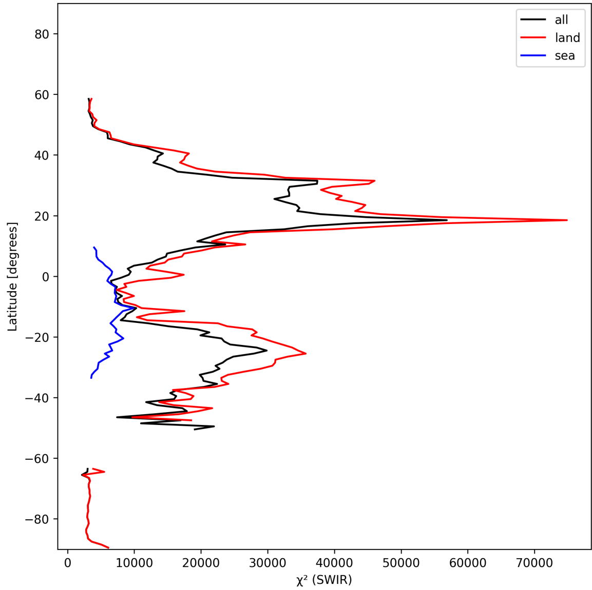
Figure 17: Zonal average of “ \chi^2 (SWIR)” for 2025-01-31 to 2025-02-02.
