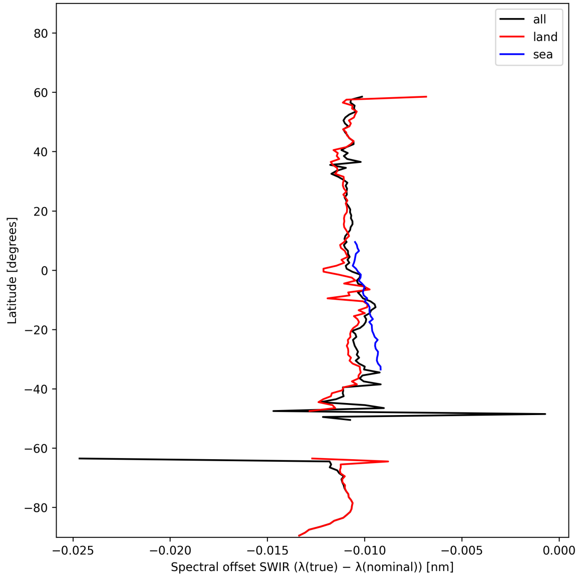
Figure 16: Zonal average of “Spectral offset SWIR ( \lambda_{\text{true}} - \lambda_{\text{nominal}} )” for 2025-01-31 to 2025-02-02.
