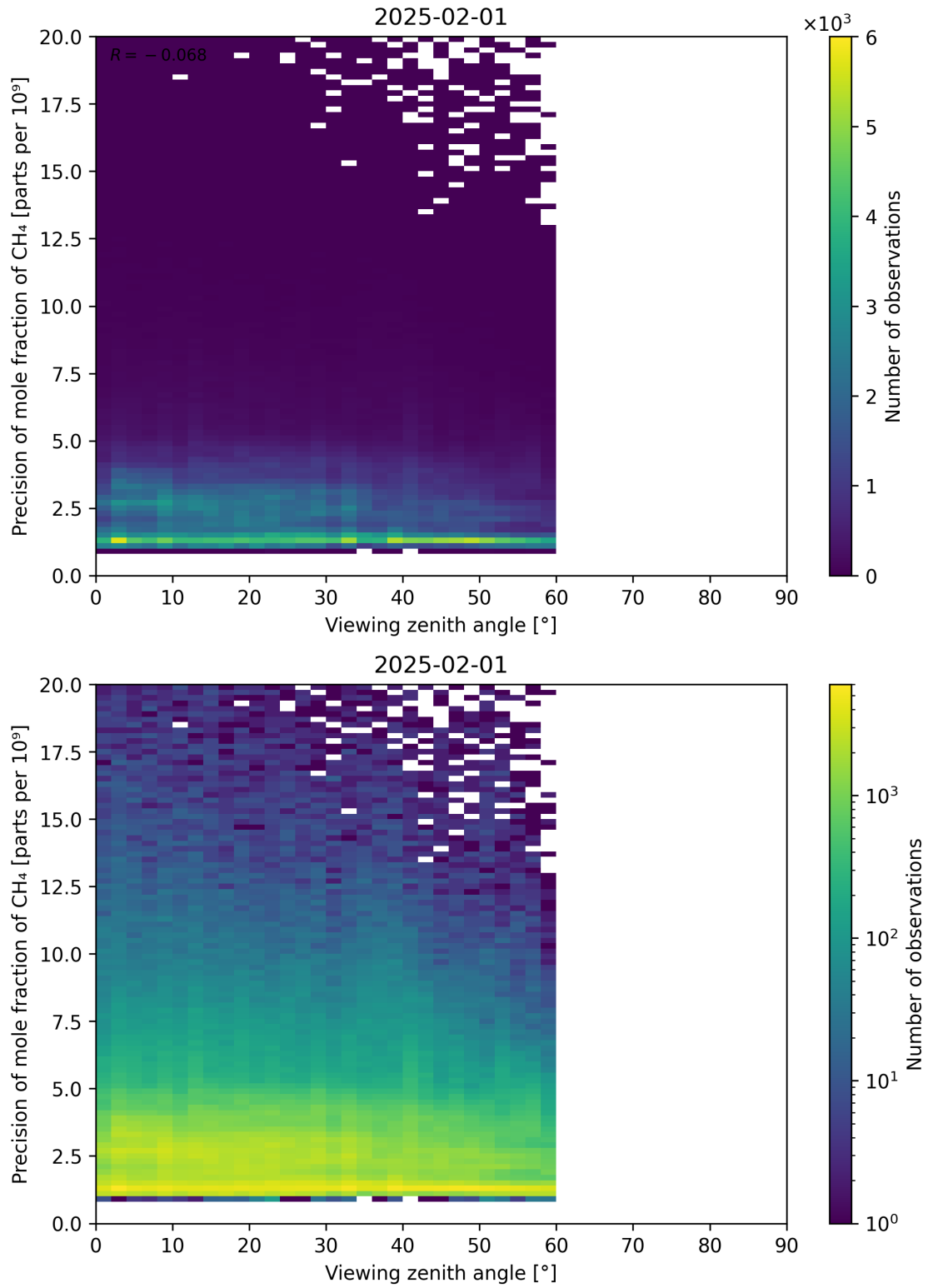
Figure 112: Scatter density plot of “Viewing zenith angle” against “Precision of mole fraction of CH 4 ” for 2025-01-31 to 2025-02-02.
