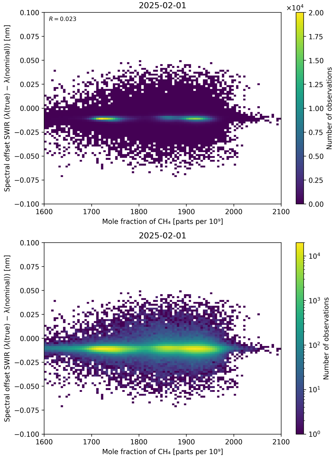
Figure 86: Scatter density plot of “Mole fraction of \text{CH}_4 ” against “Spectral offset SWIR ( \lambda_{\text{true}} - \lambda_{\text{nominal}} )” for 2025-01-31 to 2025-02-02.
