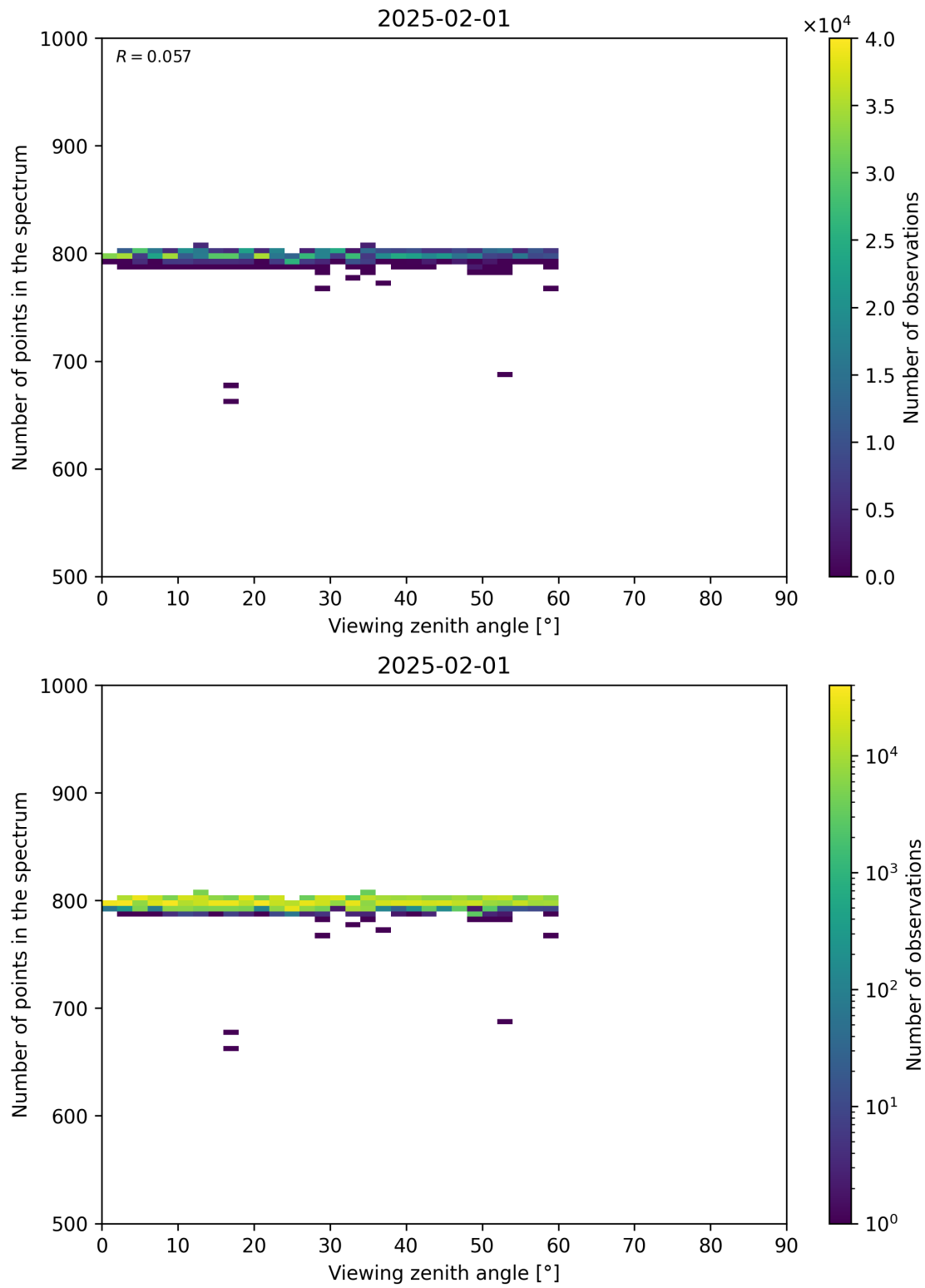
Figure 114: Scatter density plot of “Viewing zenith angle” against “Number of points in the spectrum” for 2025-01-31 to 2025-02-02.
