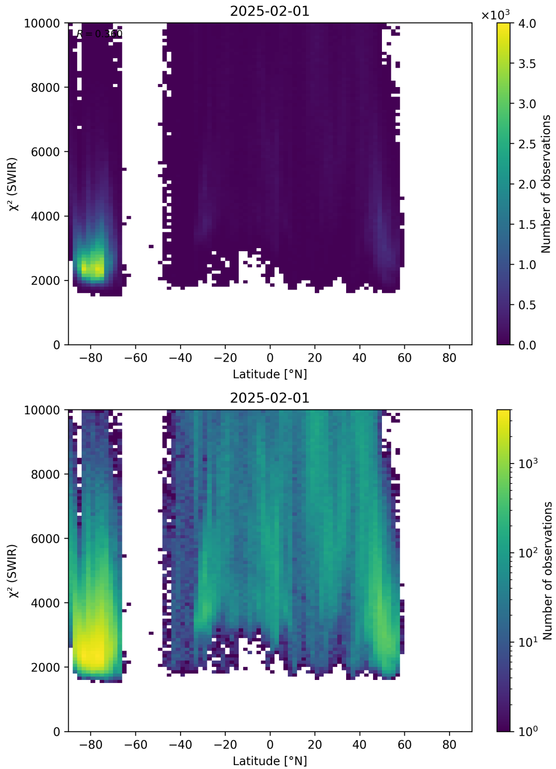
Figure 54: Scatter density plot of “Latitude” against “ \chi^2 (SWIR)” for 2025-01-31 to 2025-02-02.
