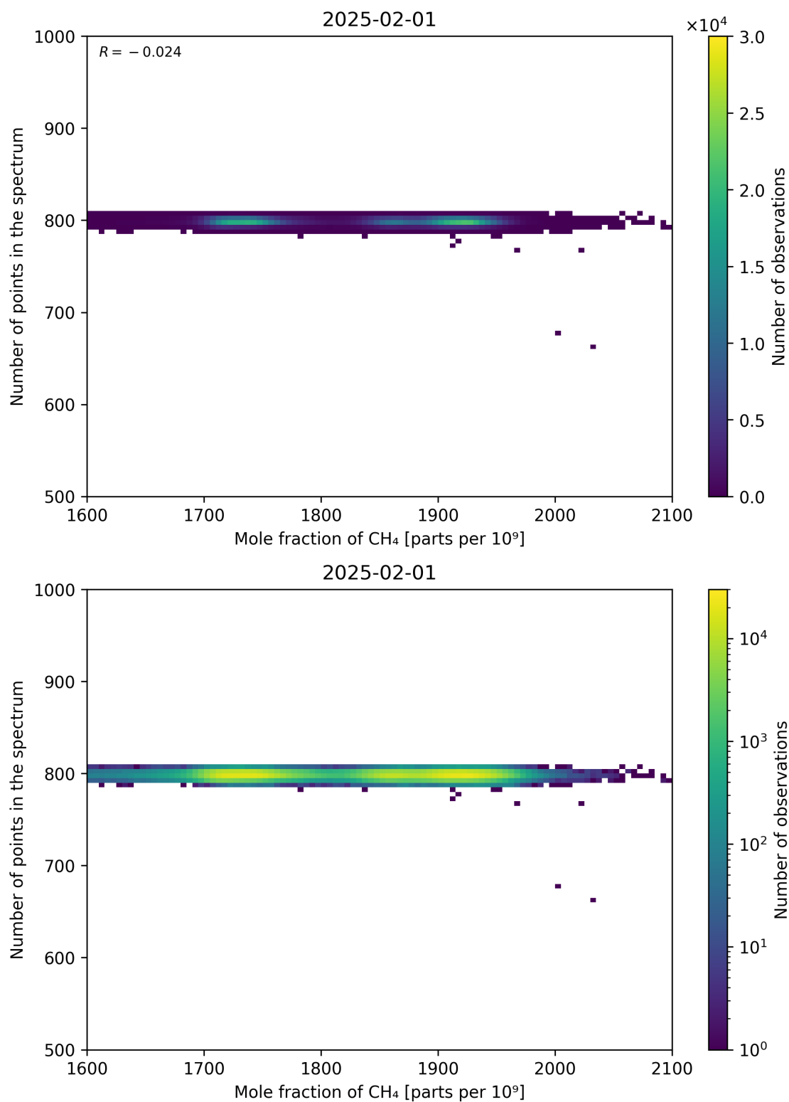
Figure 77: Scatter density plot of “Mole fraction of CH 4 ” against “Number of points in the spectrum” for 2025-01-31 to 2025-02-02.
