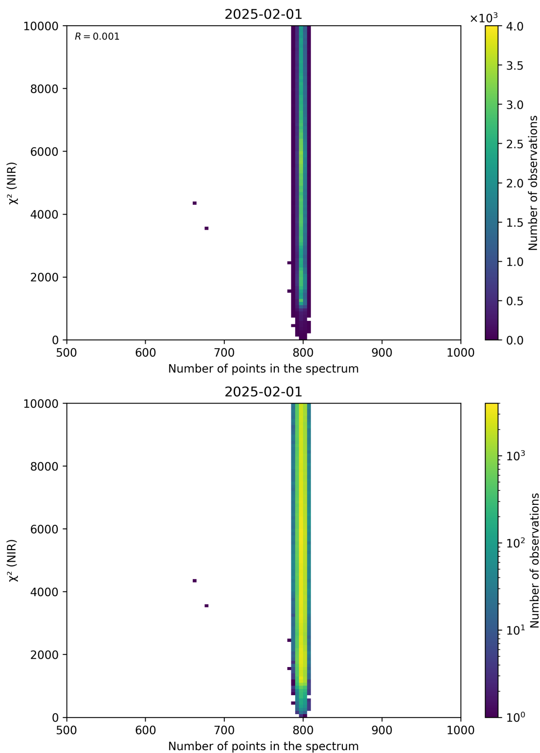
Figure 88: Scatter density plot of “Number of points in the spectrum” against “ \chi^2 (NIR)” for 2025-01-31 to 2025-02-02.
