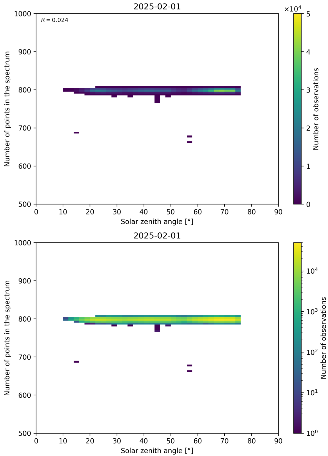
Figure 103: Scatter density plot of “Solar zenith angle” against “Number of points in the spectrum” for 2025-01-31 to 2025-02-02.
