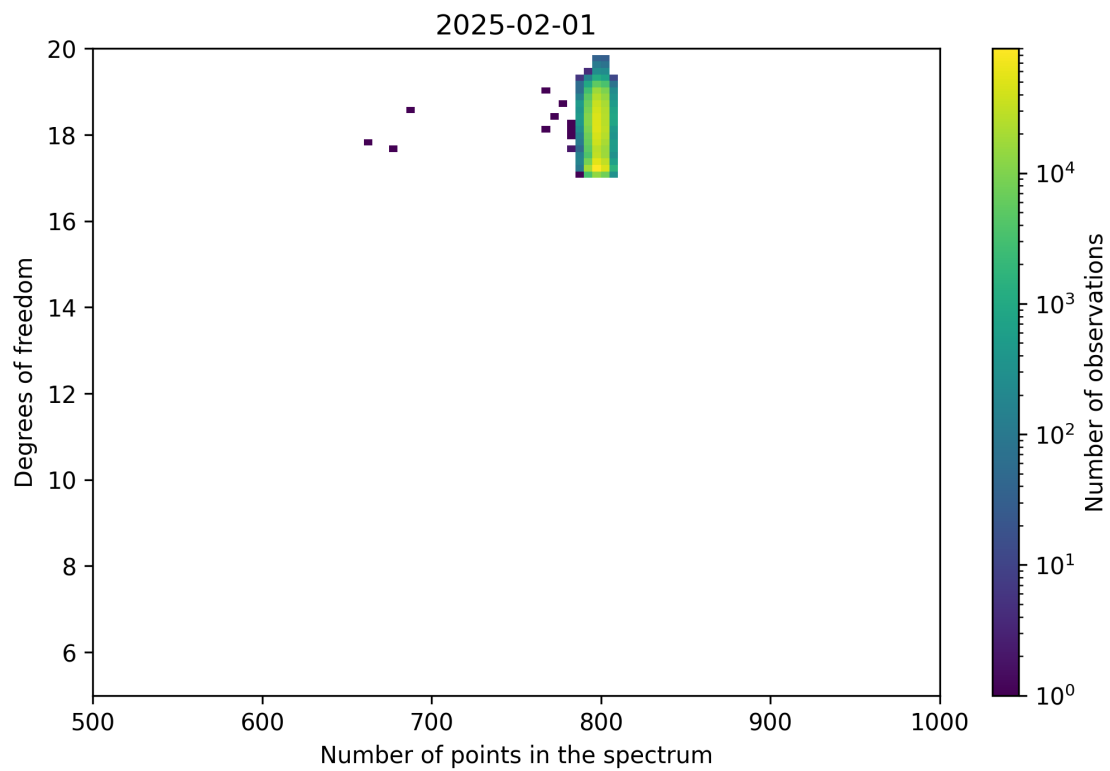
Figure 90: Scatter density plot of “Number of points in the spectrum” against “Degrees of freedom” for 2025-01-31 to 2025-02-02.
