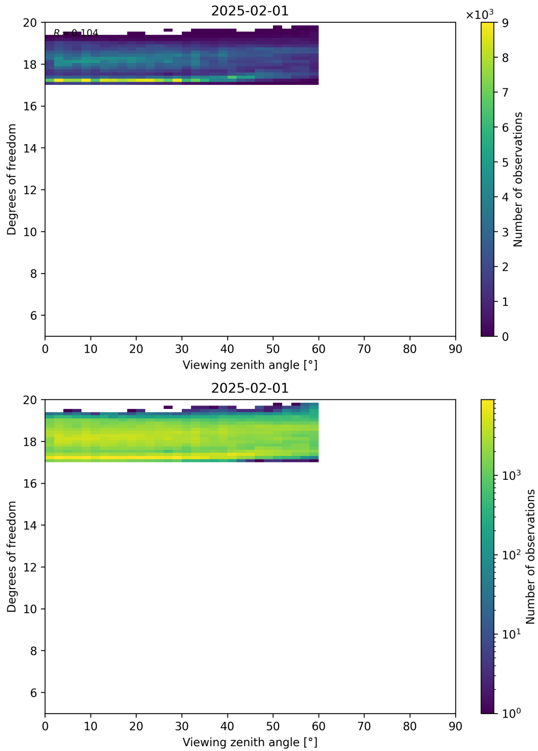
Figure 107: Scatter density plot of “Viewing zenith angle” against “Degrees of freedom” for 2025-01-31 to 2025-02-02.
