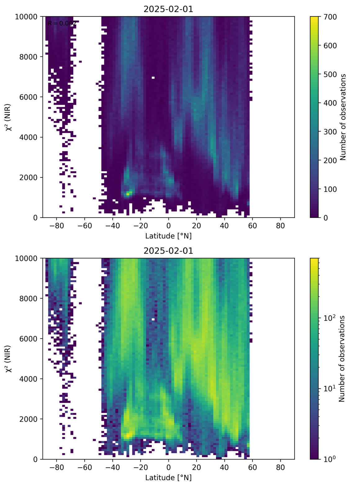
Figure 53: Scatter density plot of “Latitude” against “ \chi^2 (NIR)” for 2025-01-31 to 2025-02-02.
