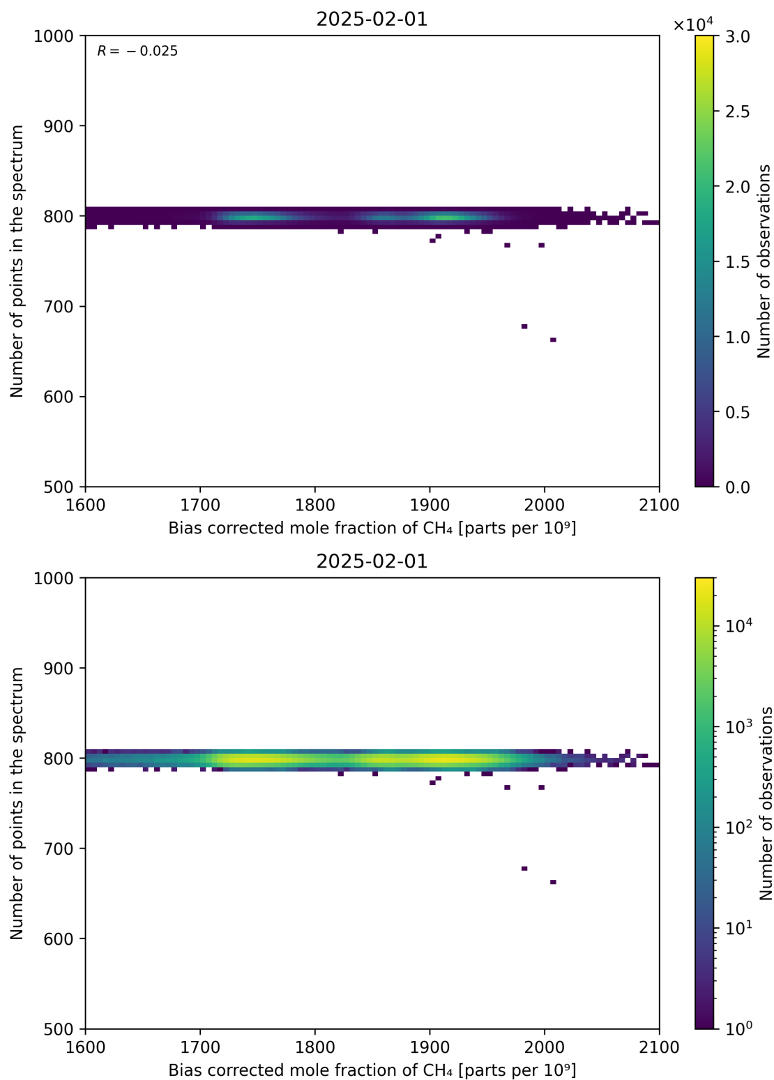
Figure 68: Scatter density plot of “Bias corrected mole fraction of CH 4 ” against “Number of points in the spectrum” for 2025-01-31 to 2025-02-02.
