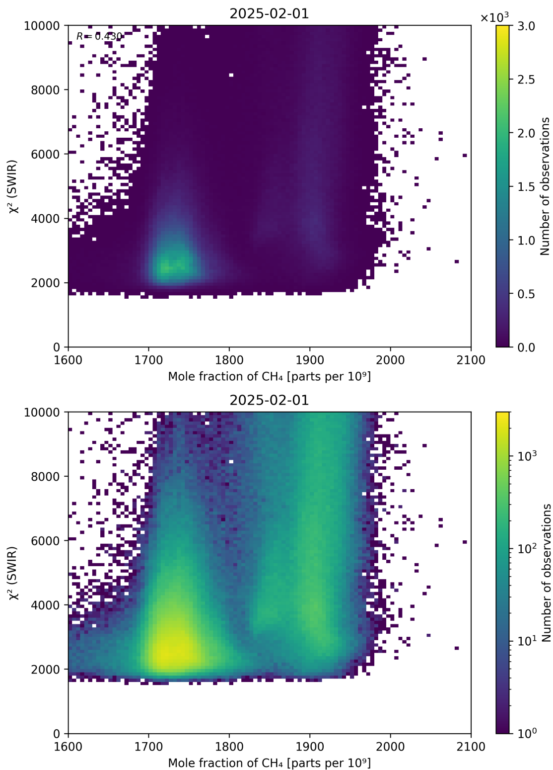
Figure 71: Scatter density plot of “Mole fraction of \text{CH}_4 ” against “ \chi^2 (SWIR)” for 2025-01-31 to 2025-02-02.
