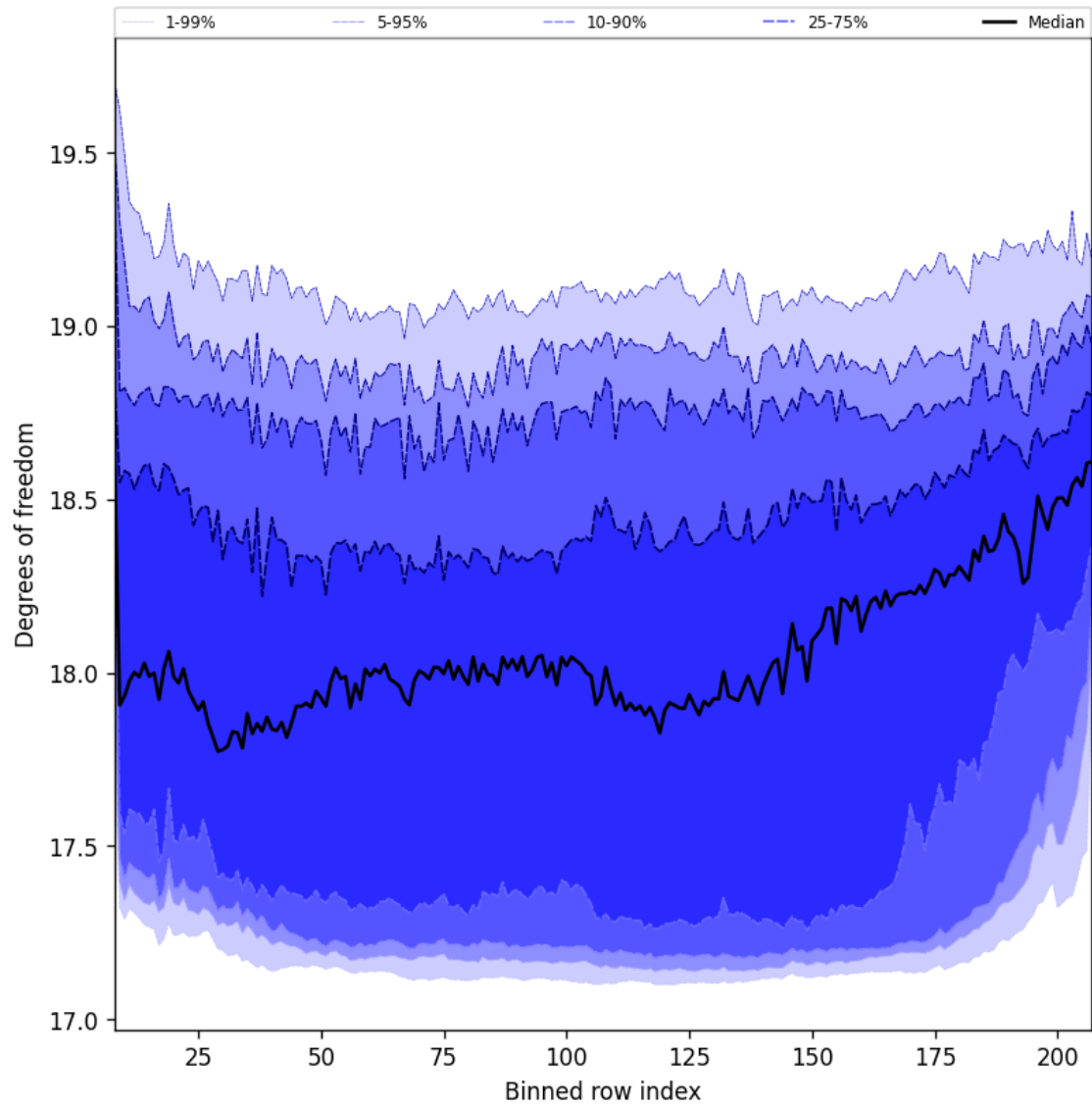
Figure 41: Along track statistics of “Degrees of freedom” for 2025-01-31 to 2025-02-02
