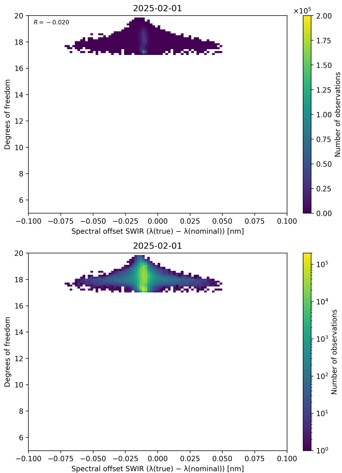
Figure 119: Scatter density plot of “Spectral offset SWIR ( \lambda_{\text{true}} - \lambda_{\text{nominal}} )” against “Degrees of freedom” for 2025-01-31 to 2025-02-02.
