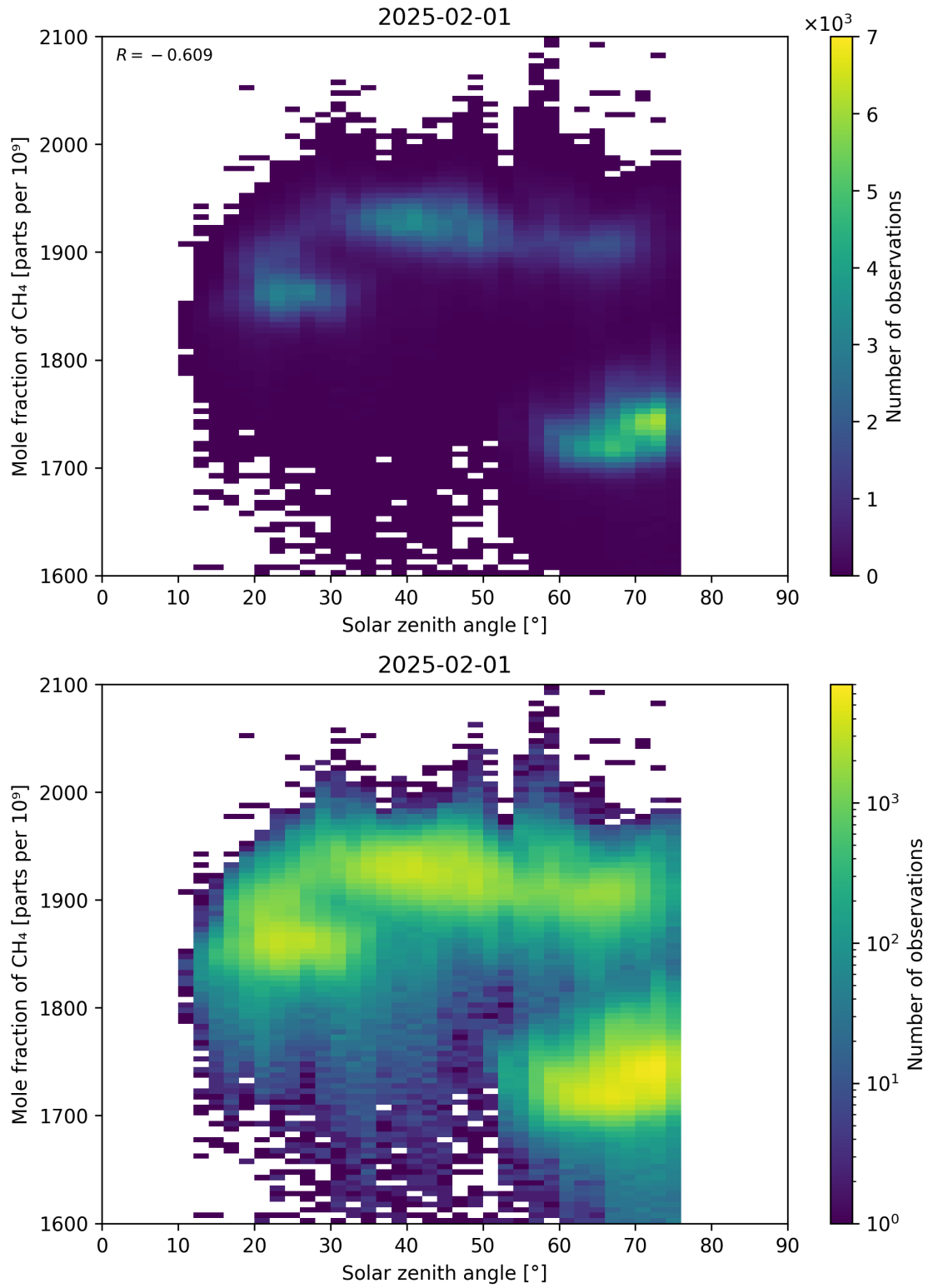
Figure 99: Scatter density plot of “Solar zenith angle” against “Mole fraction of CH 4 ” for 2025-01-31 to 2025-02-02.
