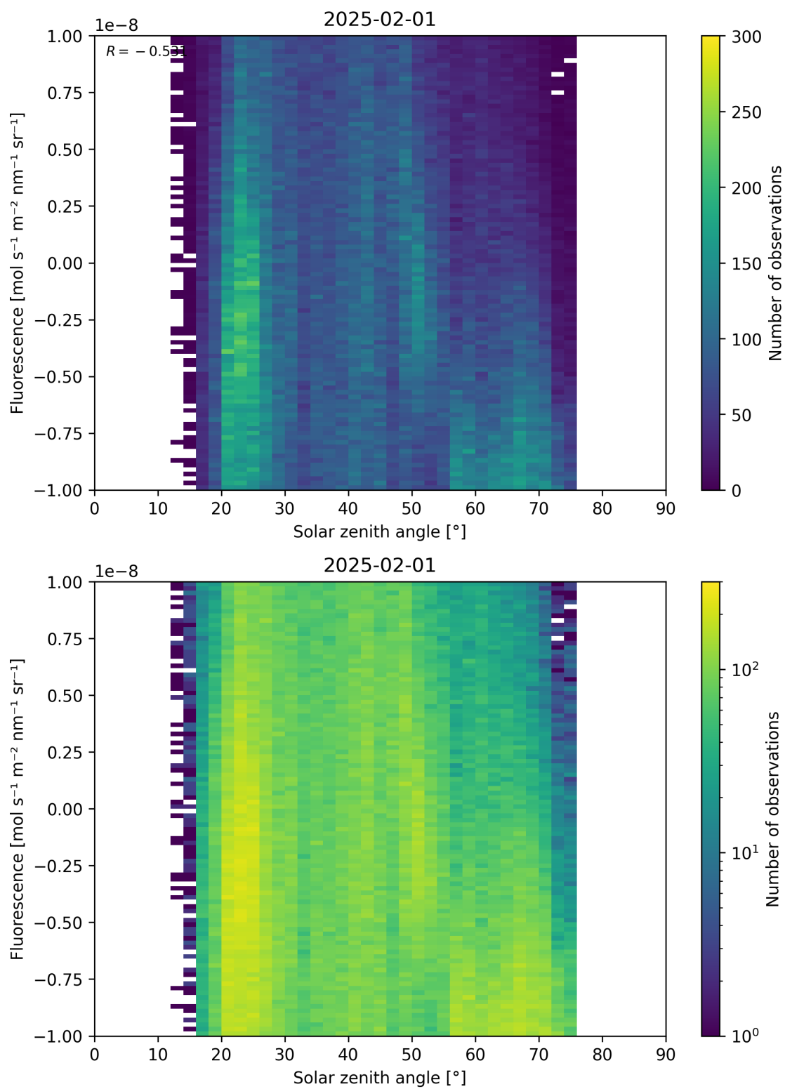
Figure 97: Scatter density plot of “Solar zenith angle” against “Fluorescence” for 2025-01-31 to 2025-02-02.
