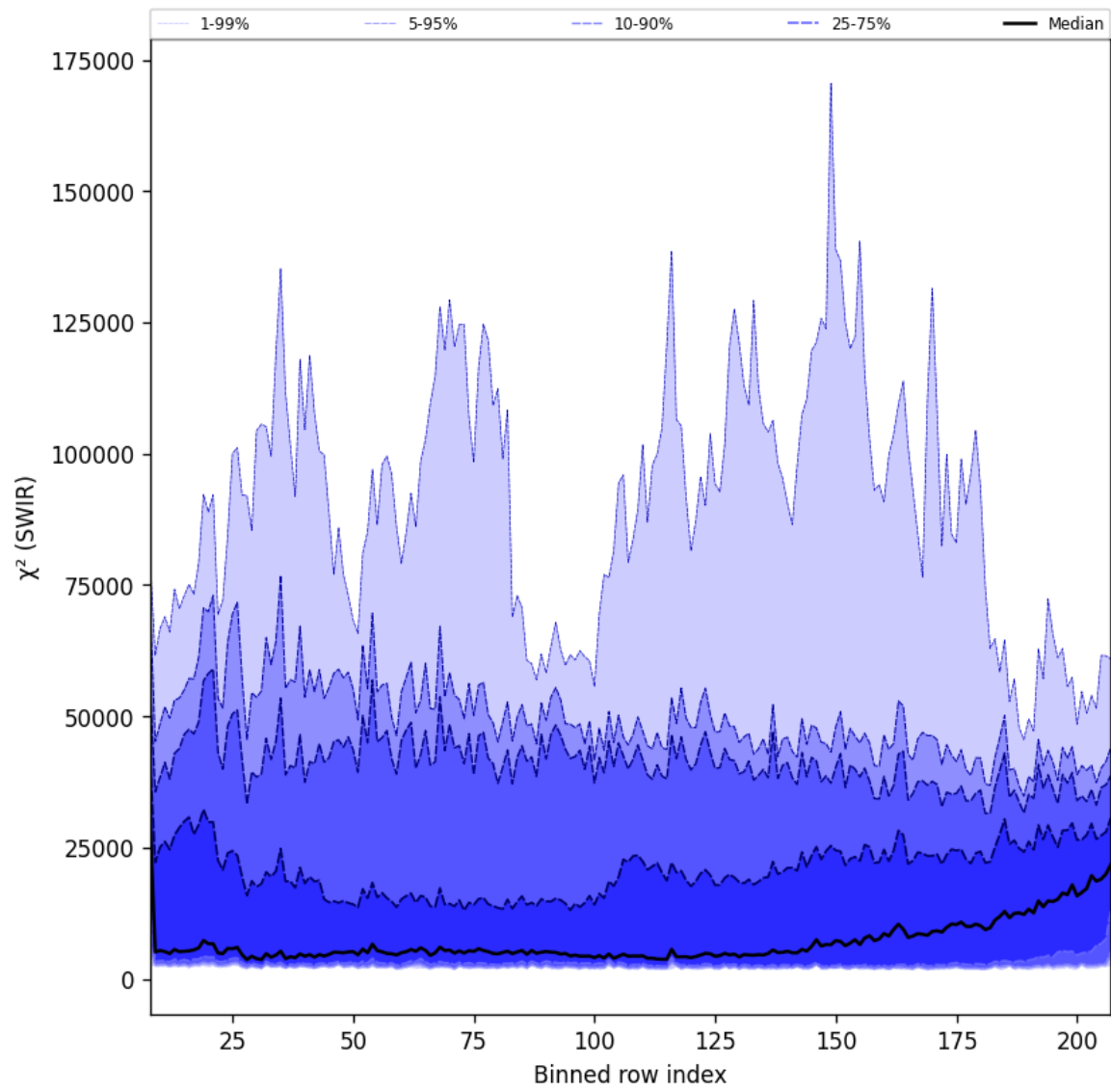
Figure 39: Along track statistics of “ \chi^2 (SWIR)” for 2025-01-31 to 2025-02-02
