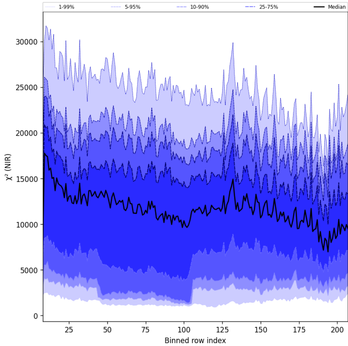
Figure 40: Along track statistics of “ \chi^2 (NIR)” for 2025-01-31 to 2025-02-02
