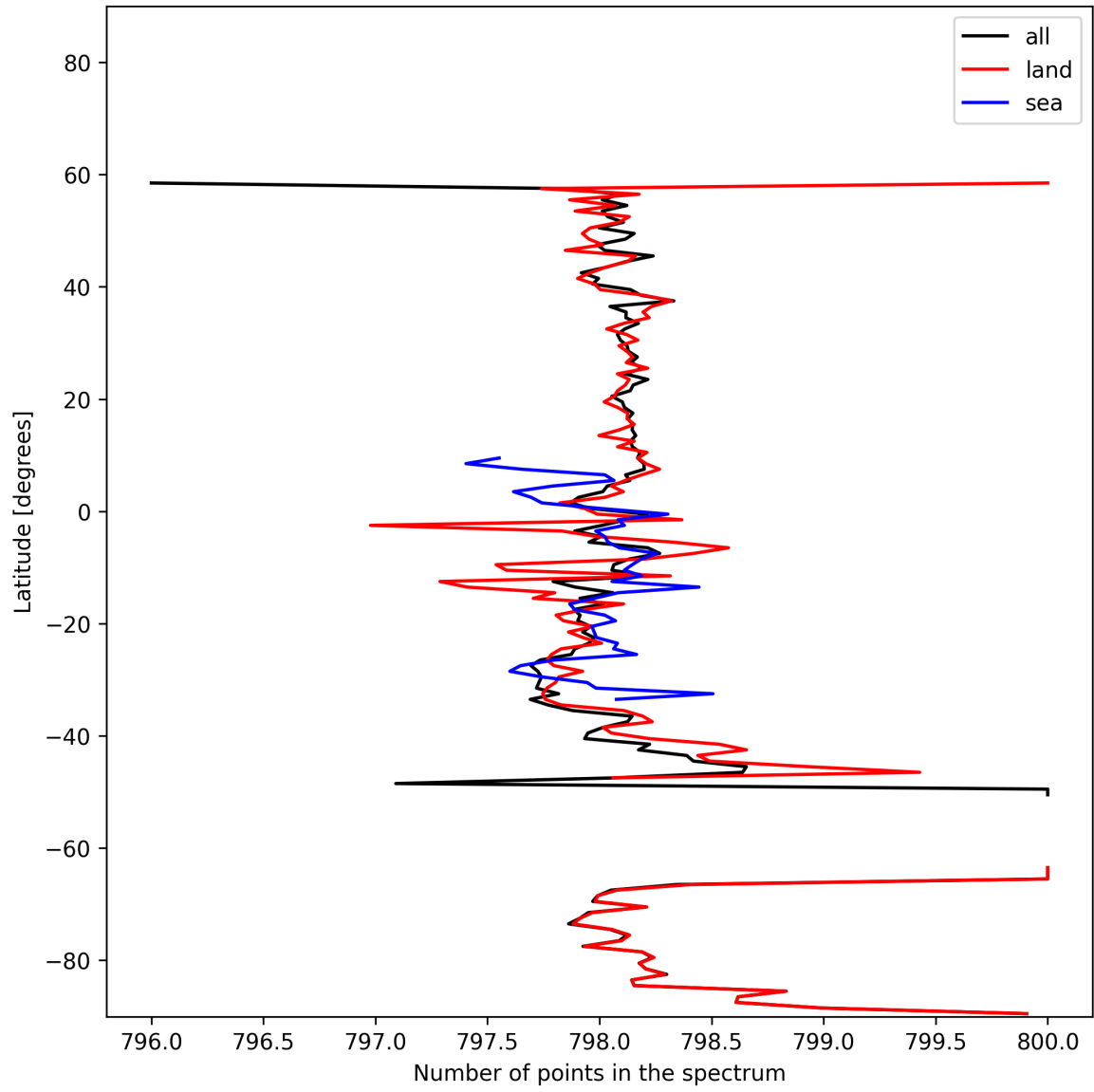
Figure 15: Zonal average of “Number of points in the spectrum” for 2025-01-31 to 2025-02-02.
