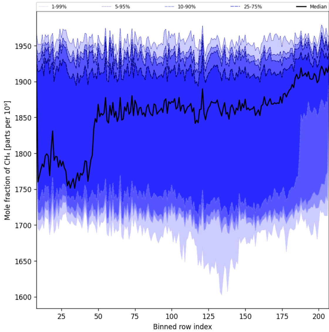
Figure 34: Along track statistics of “Mole fraction of CH 4 ” for 2025-01-31 to 2025-02-02
