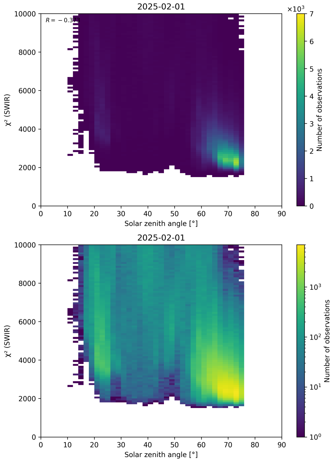
Figure 95: Scatter density plot of “Solar zenith angle” against “ \chi^2 (SWIR)” for 2025-01-31 to 2025-02-02.
