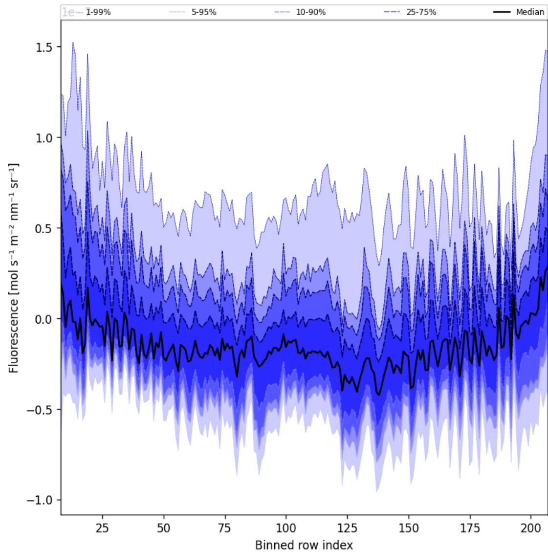
Figure 43: Along track statistics of “Fluorescence” for 2025-01-31 to 2025-02-02
