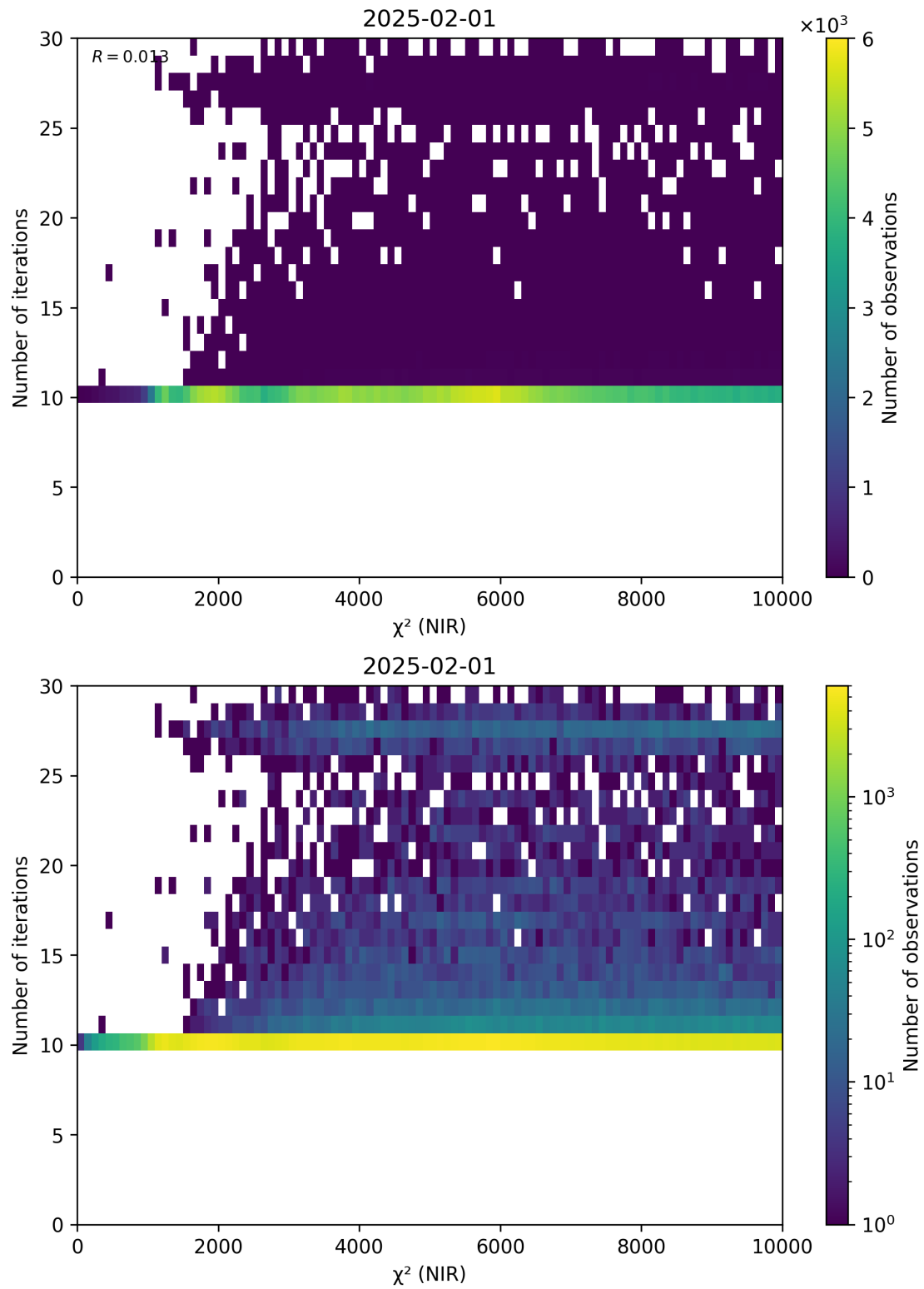
Figure 46: Scatter density plot of “ \chi^2 (NIR)” against “Number of iterations” for 2025-01-31 to 2025-02-02.
