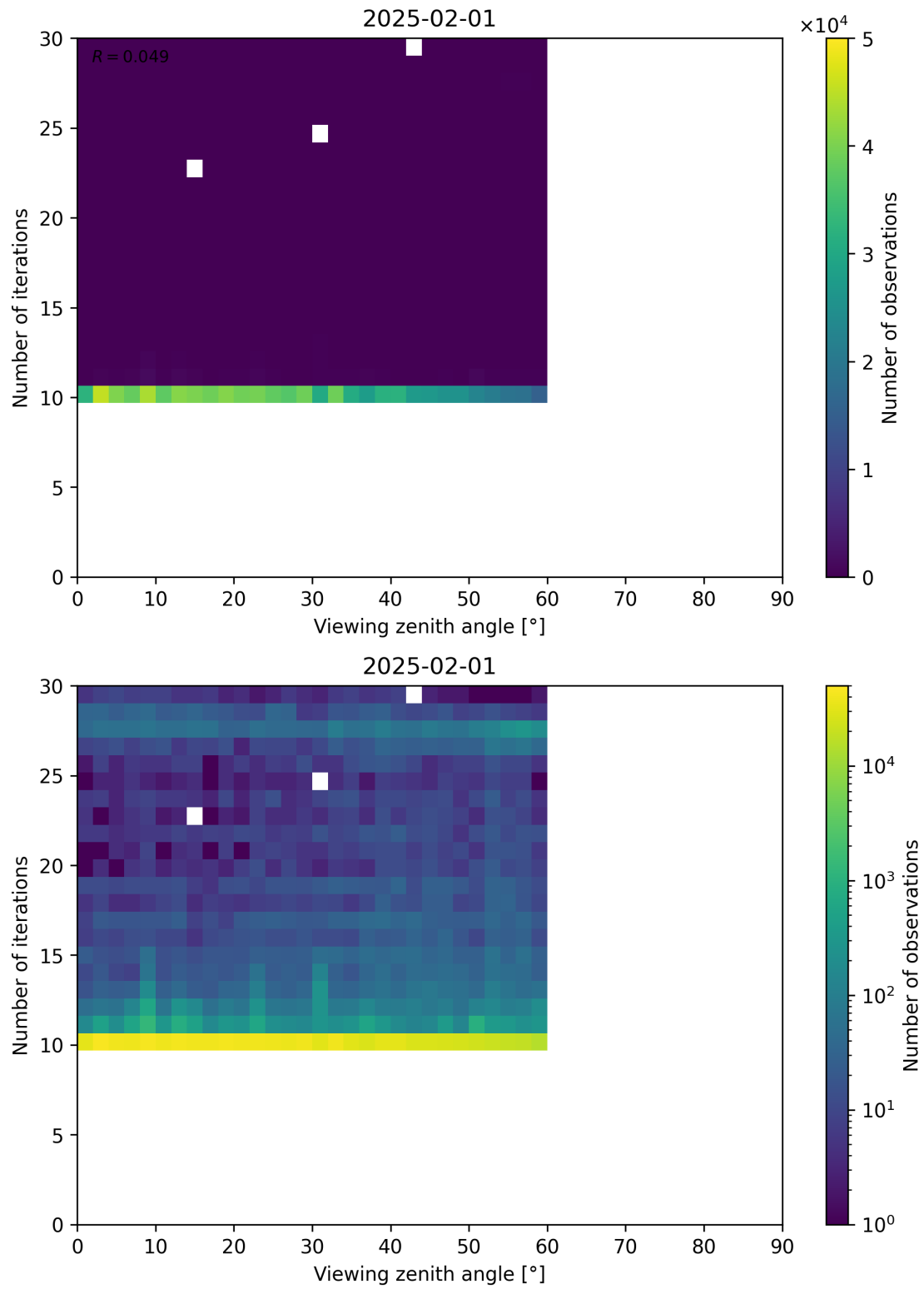
Figure 113: Scatter density plot of “Viewing zenith angle” against “Number of iterations” for 2025-01-31 to 2025-02-02.
