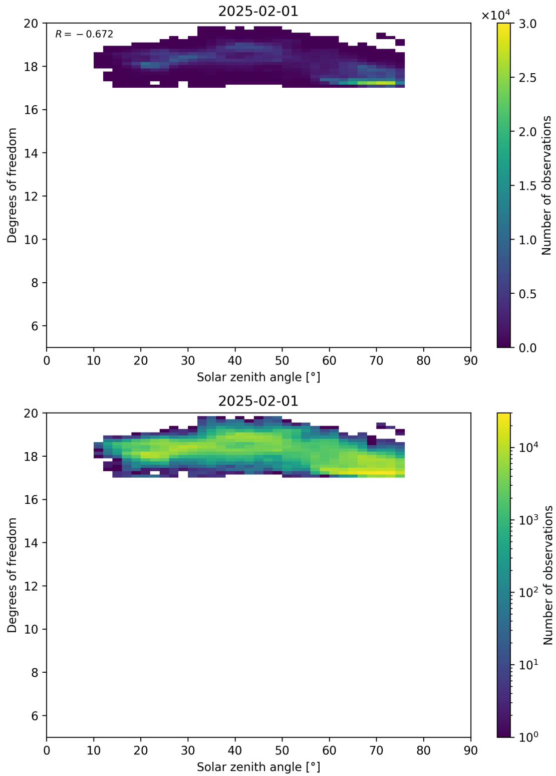
Figure 96: Scatter density plot of “Solar zenith angle” against “Degrees of freedom” for 2025-01-31 to 2025-02-02.
