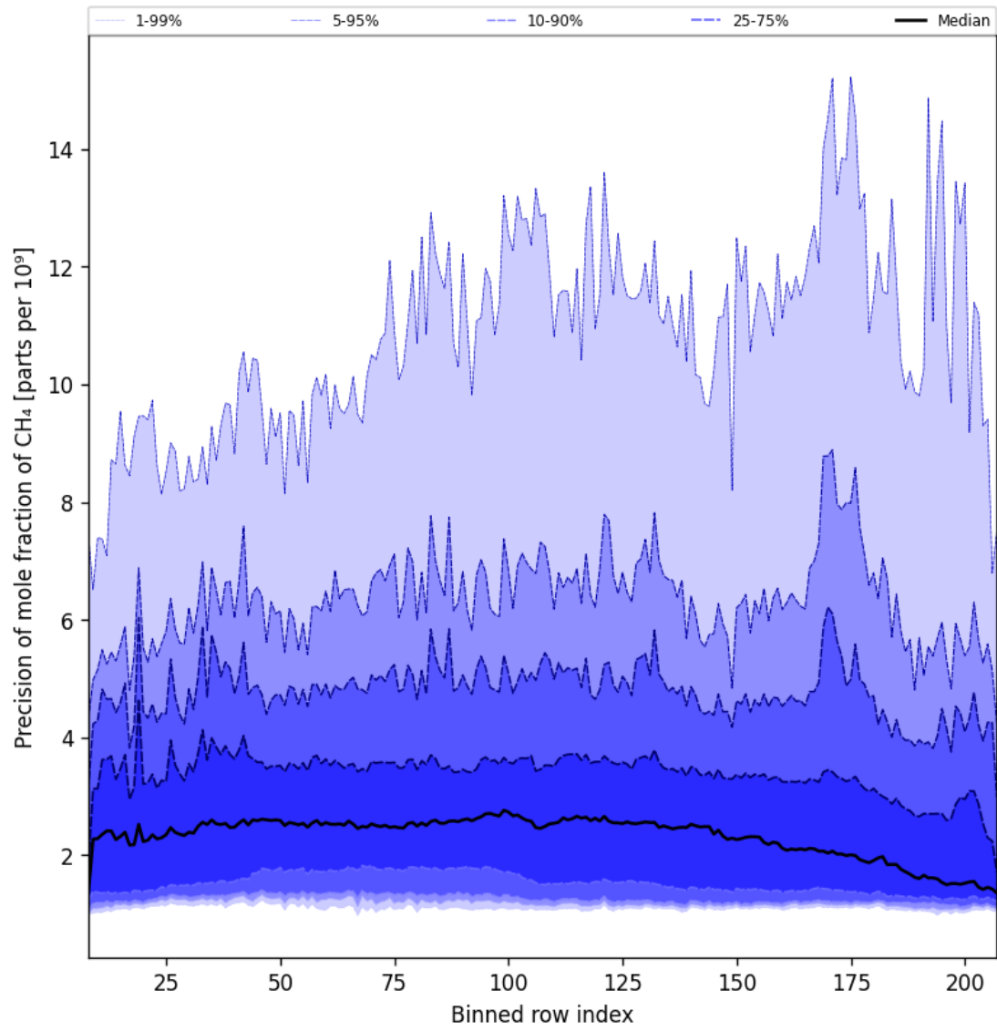
Figure 35: Along track statistics of “Precision of mole fraction of CH 4 ” for 2025-01-31 to 2025-02-02
