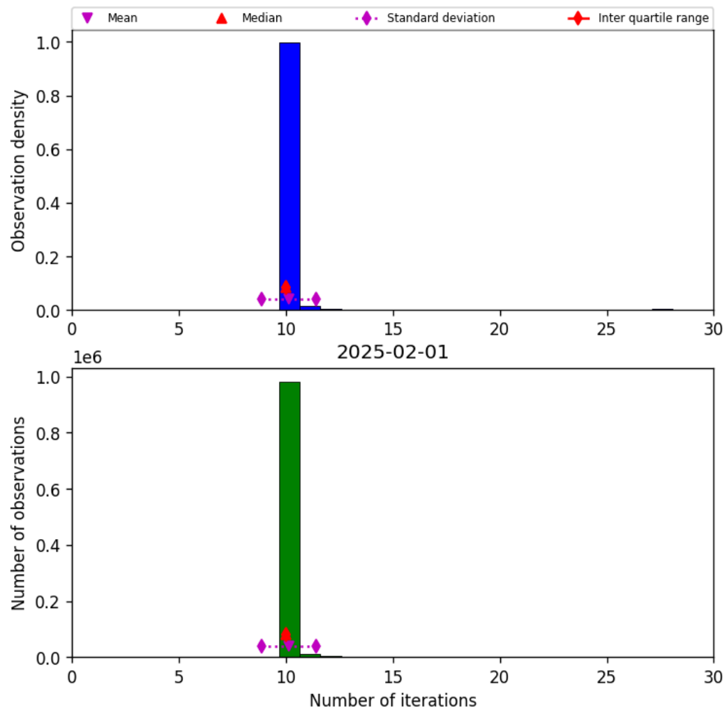
Figure 31: Histogram of “Number of iterations” for 2025-01-31 to 2025-02-02
