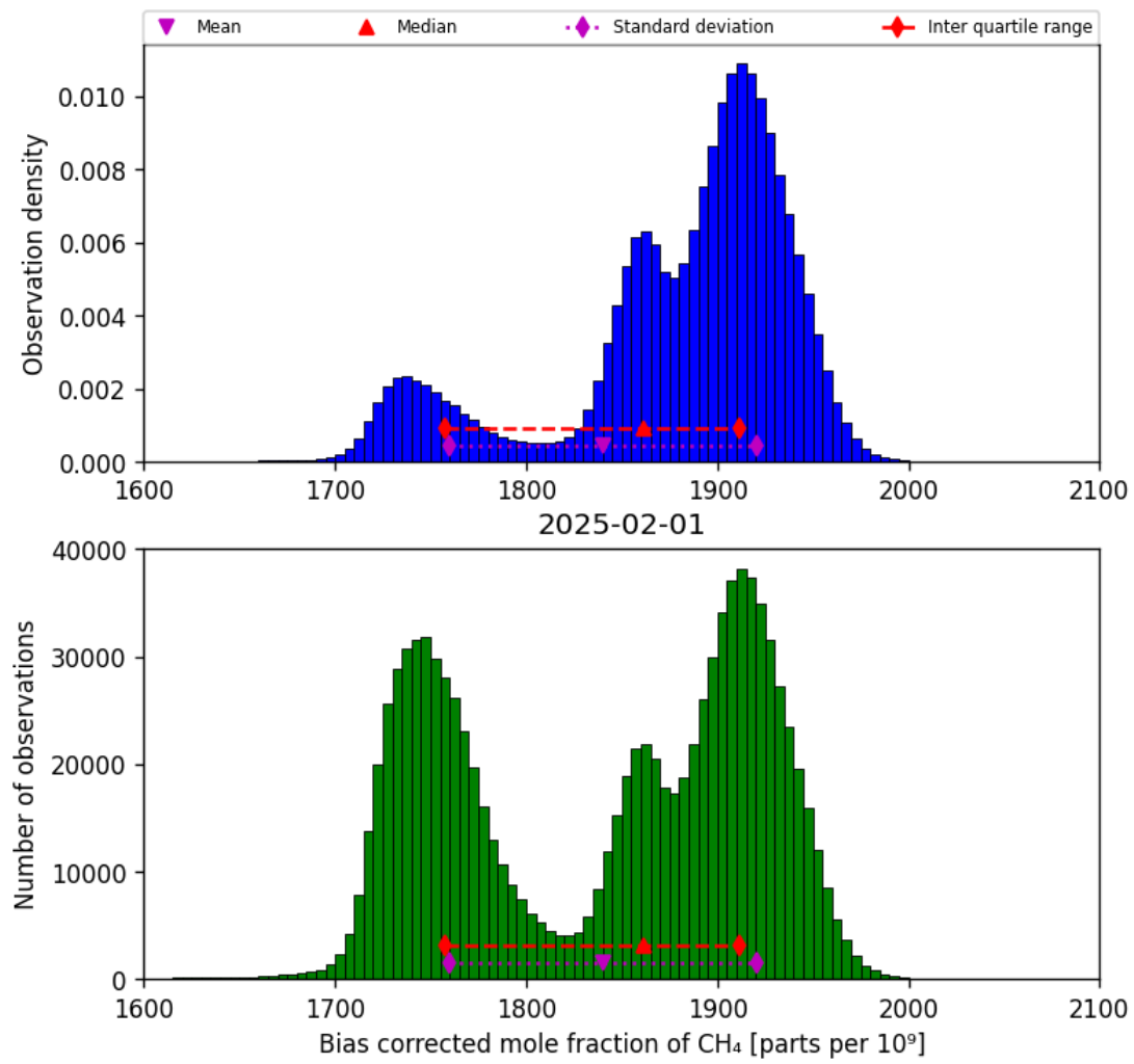
Figure 25: Histogram of “Bias corrected mole fraction of CH 4 ” for 2025-01-31 to 2025-02-02
