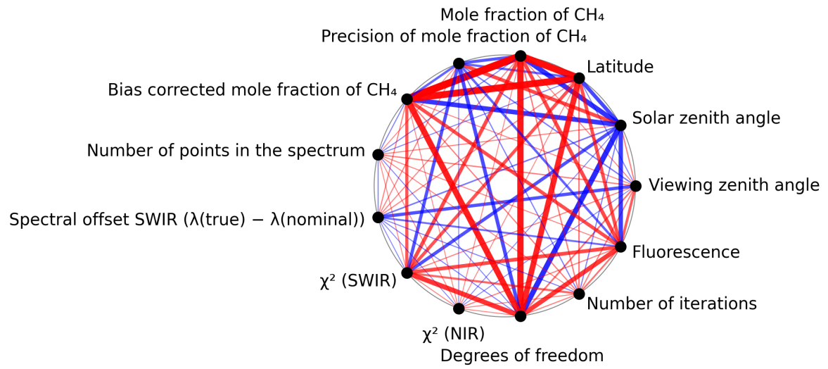
Figure 1: Map of correlation graph for 2025-01-31 to 2025-02-02.
