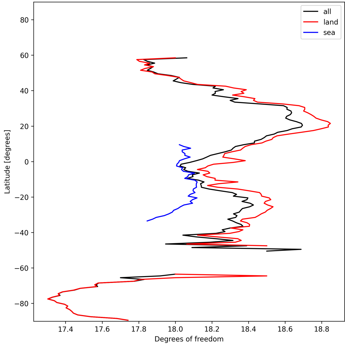
Figure 19: Zonal average of “Degrees of freedom” for 2025-01-31 to 2025-02-02.
