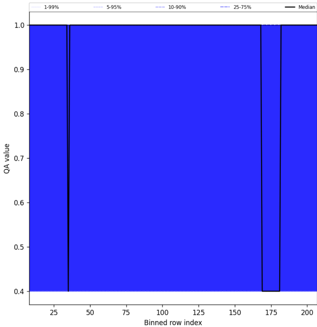
Figure 33: Along track statistics of “QA value” for 2025-01-31 to 2025-02-02
