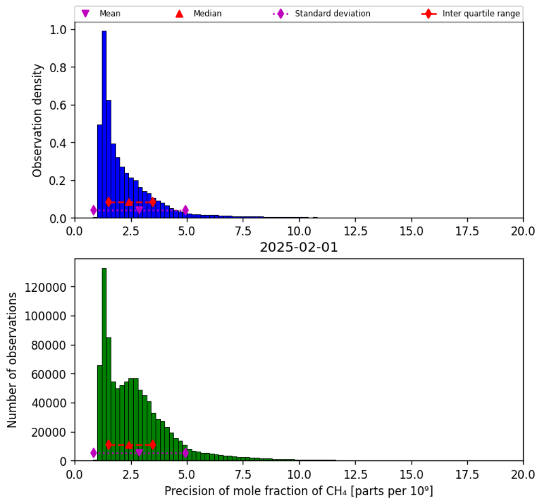
Figure 24: Histogram of “Precision of mole fraction of CH 4 ” for 2025-01-31 to 2025-02-02
