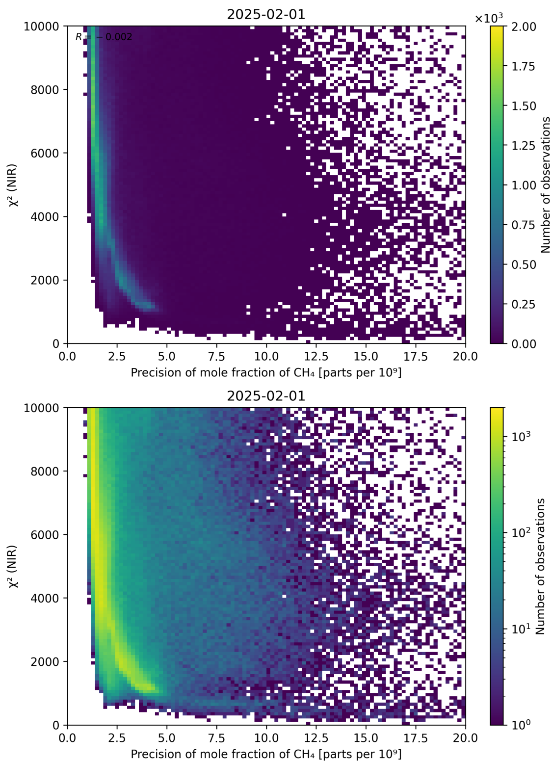
Figure 78: Scatter density plot of “Precision of mole fraction of CH 4 ” against “ \chi^2 (NIR)” for 2025-01-31 to 2025-02-02.
