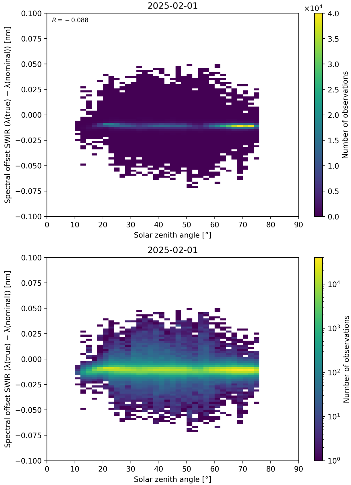
Figure 104: Scatter density plot of “Solar zenith angle” against “Spectral offset SWIR ( \lambda_{\text{true}} - \lambda_{\text{nominal}} )” for 2025-01-31 to 2025-02-02.
