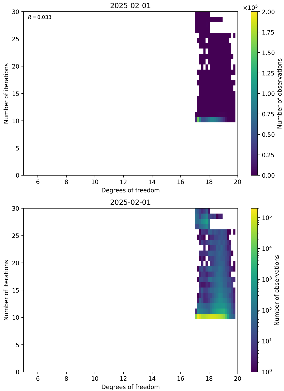
Figure 52: Scatter density plot of “Degrees of freedom” against “Number of iterations” for 2025-01-31 to 2025-02-02.
