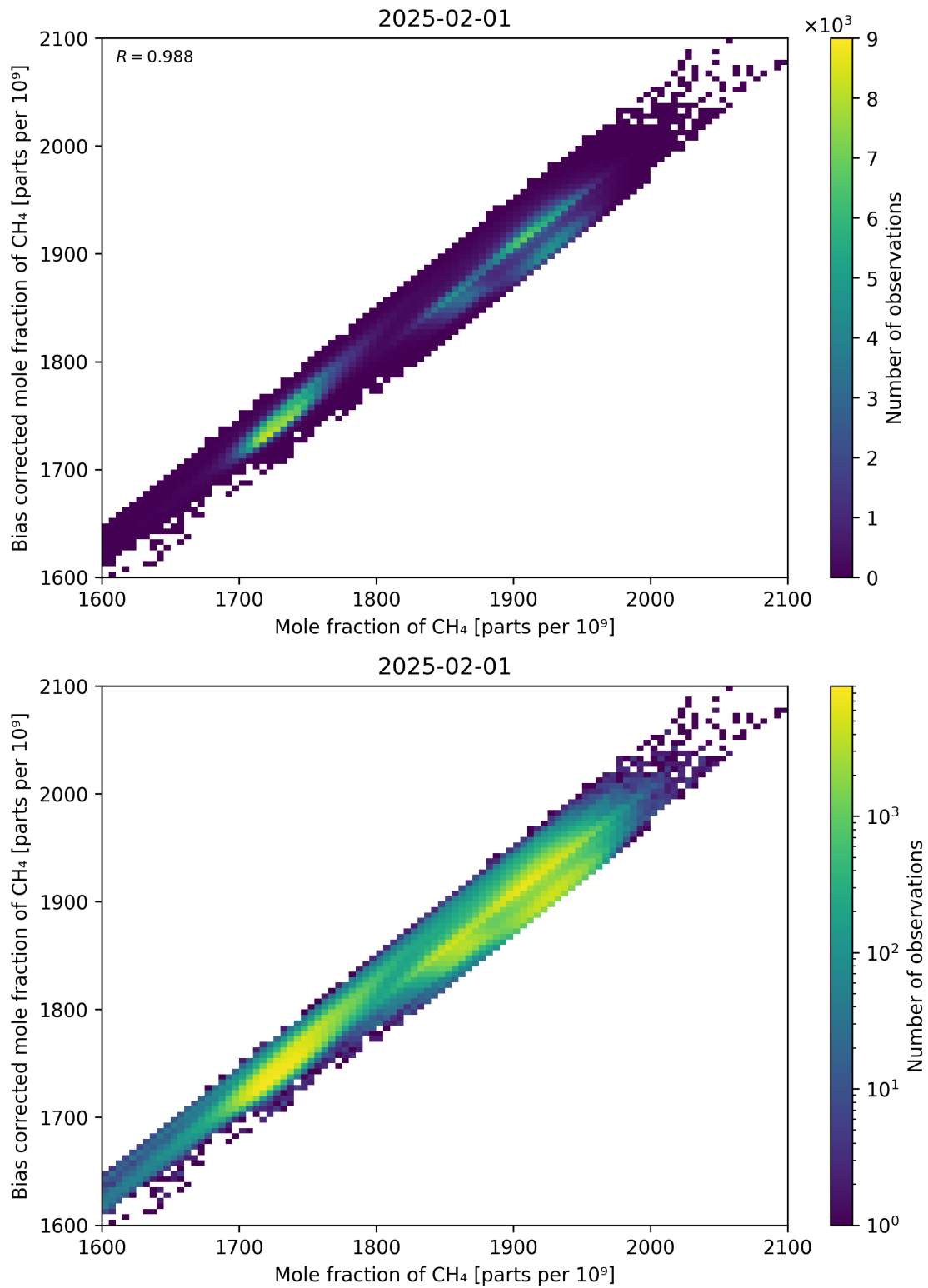
Figure 74: Scatter density plot of “Mole fraction of CH 4 ” against “Bias corrected mole fraction of CH 4 ” for 2025-01-31 to 2025-02-02.
