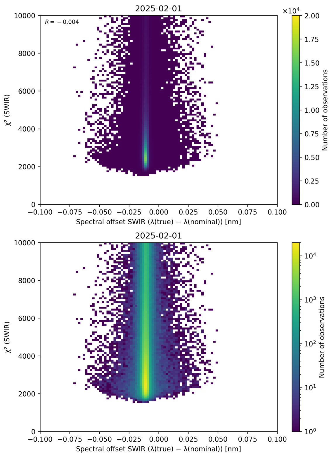
Figure 118: Scatter density plot of “Spectral offset SWIR ( \lambda_{\text{true}} - \lambda_{\text{nominal}} )” against “ \chi^2 (SWIR)” for 2025-01-31 to 2025-02-02.
