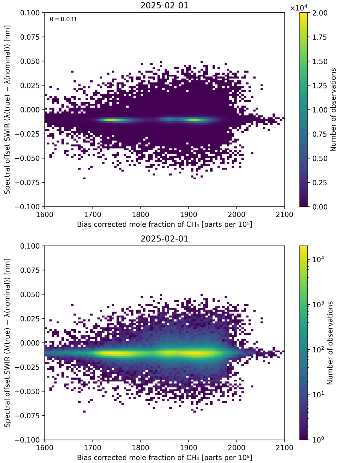
Figure 69: Scatter density plot of “Bias corrected mole fraction of \text{CH}_4 ” against “Spectral offset SWIR ( \lambda_{\text{true}} - \lambda_{\text{nominal}} )” for 2025-01-31 to 2025-02-02.
