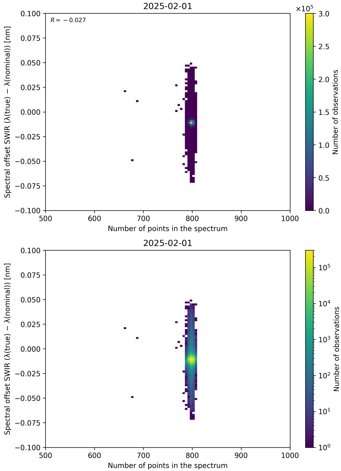
Figure 93: Scatter density plot of “Number of points in the spectrum” against “Spectral offset SWIR ( \lambda_{\text{true}} - \lambda_{\text{nominal}} )” for 2025-01-31 to 2025-02-02.
