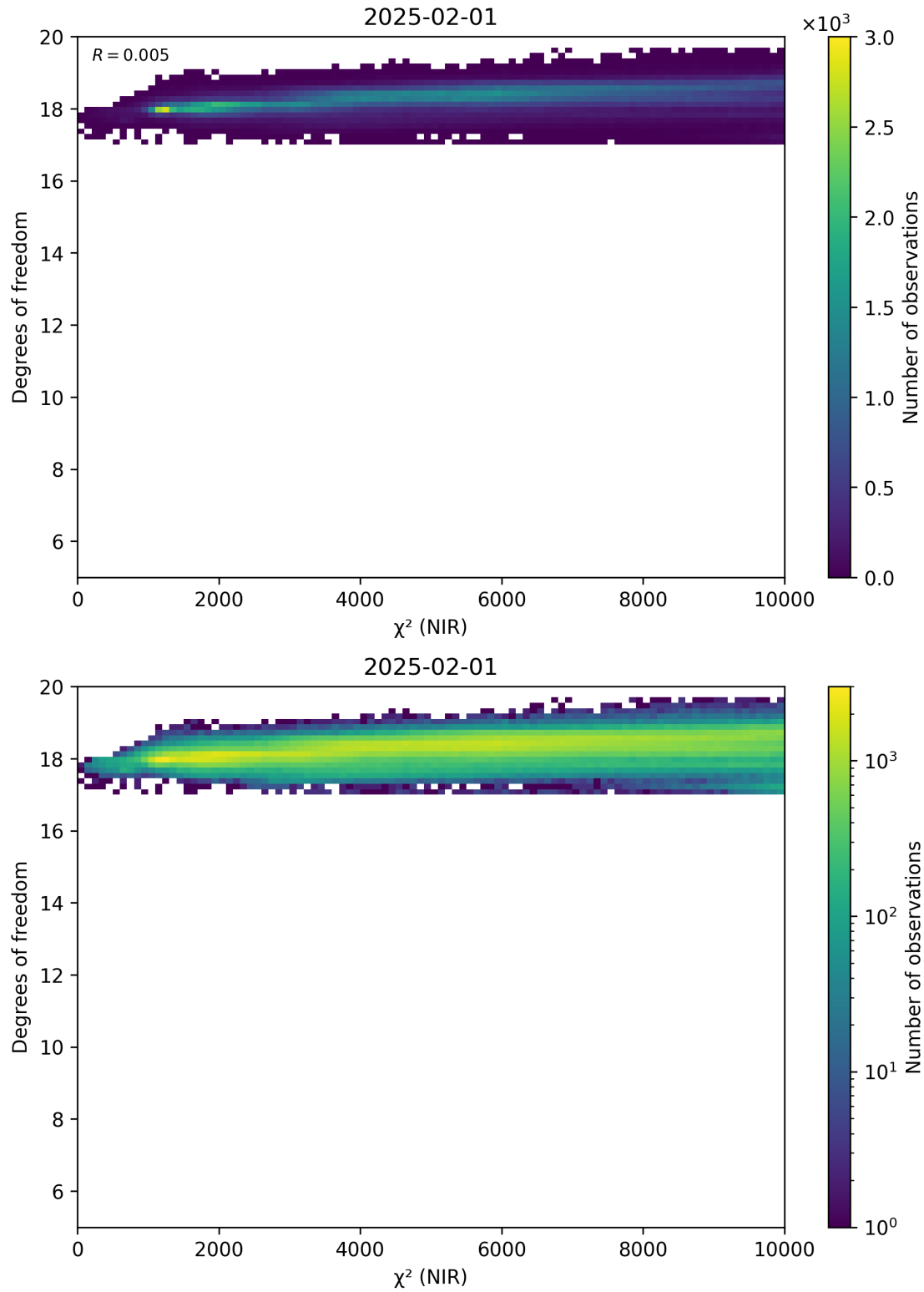
Figure 44: Scatter density plot of “ \chi^2 (NIR)” against “Degrees of freedom” for 2025-01-31 to 2025-02-02.
