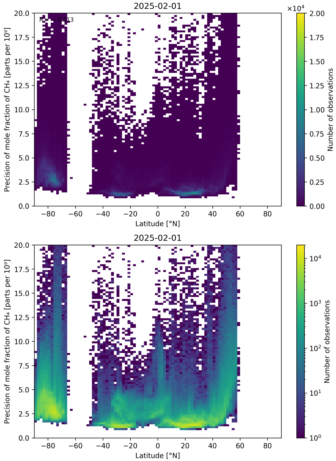
Figure 59: Scatter density plot of “Latitude” against “Precision of mole fraction of CH 4 ” for 2025-01-31 to 2025-02-02.
