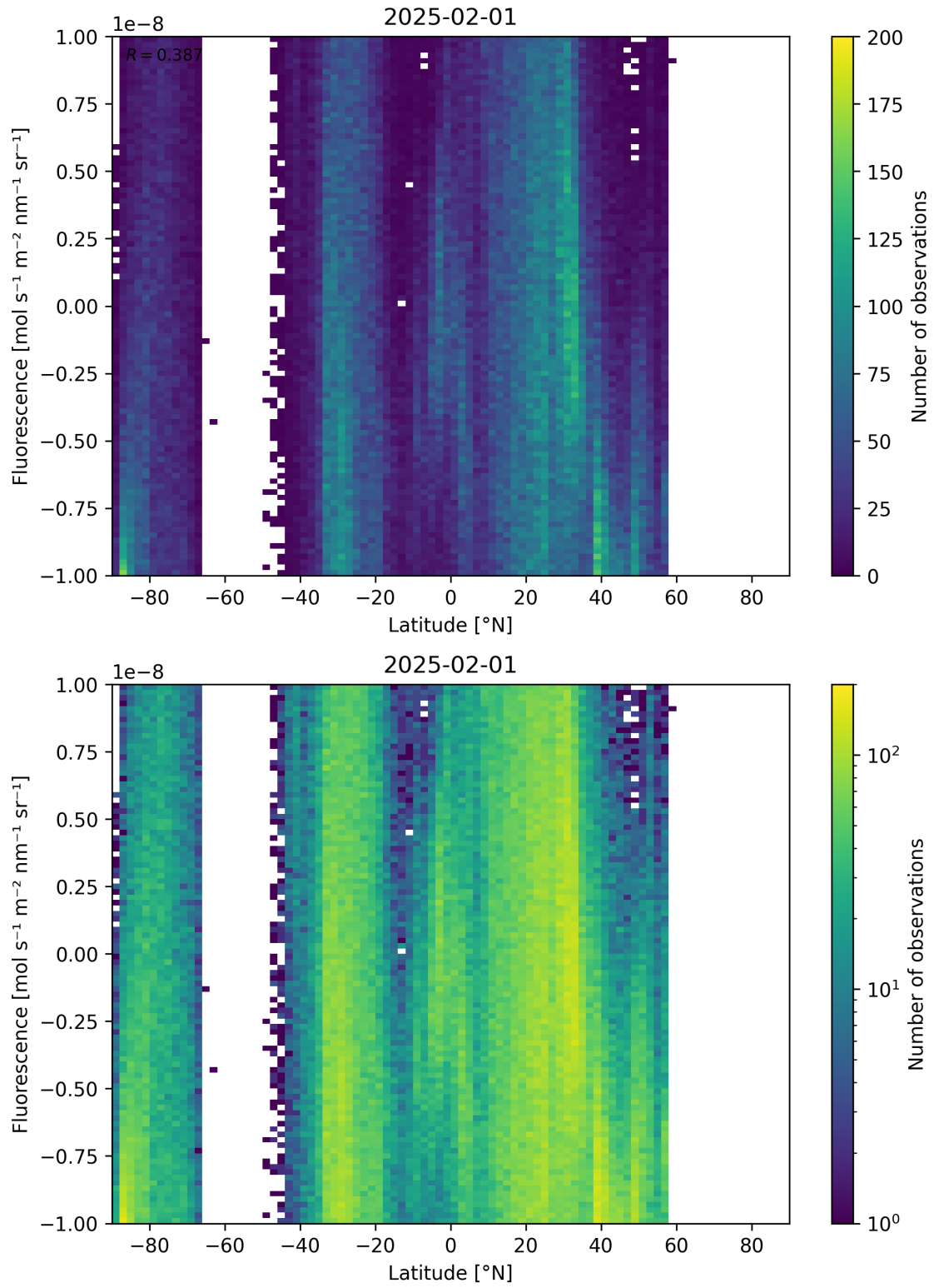
Figure 56: Scatter density plot of “Latitude” against “Fluorescence” for 2025-01-31 to 2025-02-02.
