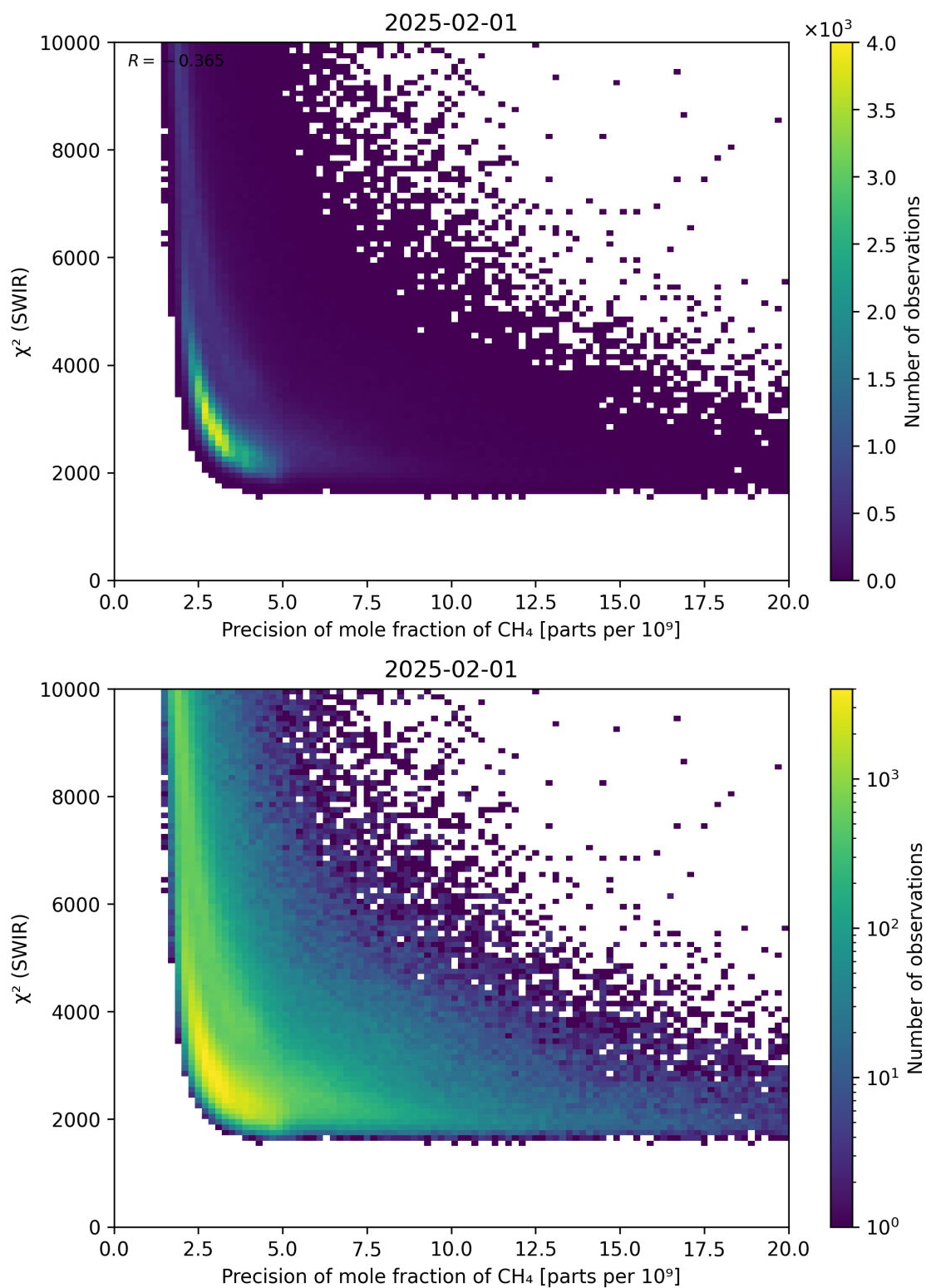
Figure 79: Scatter density plot of “Precision of mole fraction of \text{CH}_4 ” against “ \chi^2 (SWIR)” for 2025-01-31 to 2025-02-02.
