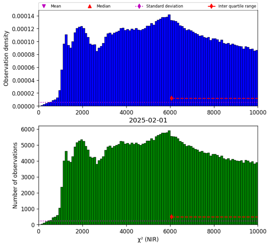
Figure 29: Histogram of “ \chi^2 (NIR)” for 2025-01-31 to 2025-02-02
