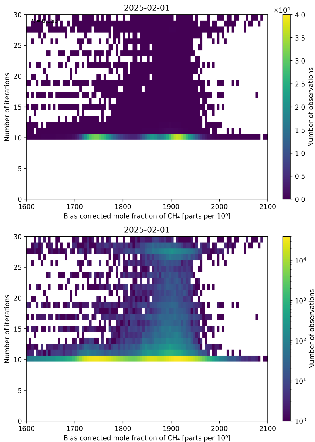
Figure 67: Scatter density plot of “Bias corrected mole fraction of CH 4 ” against “Number of iterations” for 2025-01-31 to 2025-02-02.
