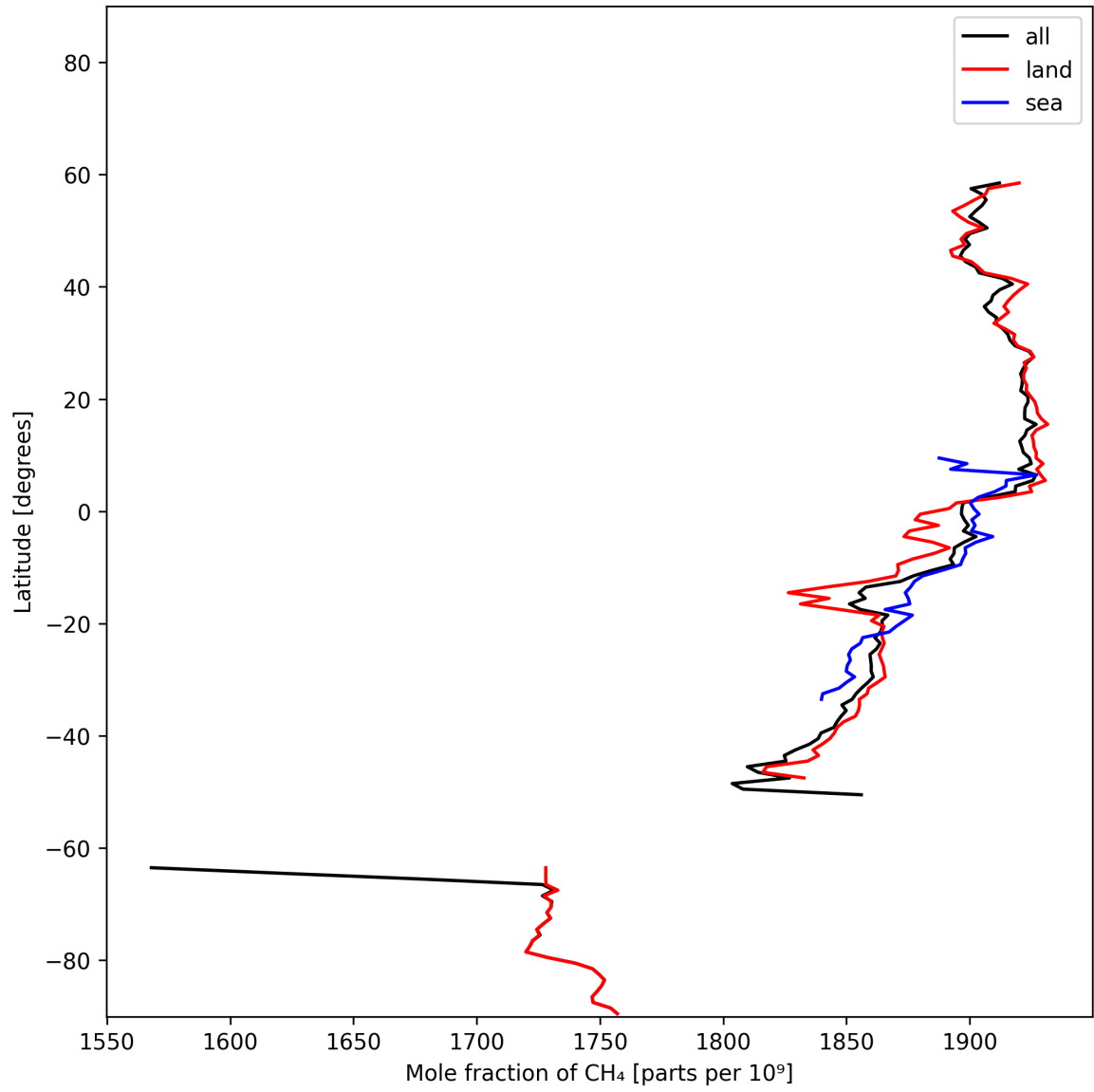
Figure 12: Zonal average of “Mole fraction of CH 4 ” for 2025-01-31 to 2025-02-02.
