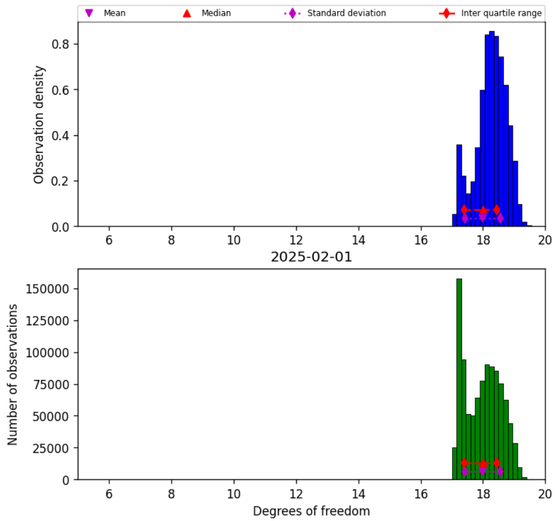
Figure 30: Histogram of “Degrees of freedom” for 2025-01-31 to 2025-02-02
