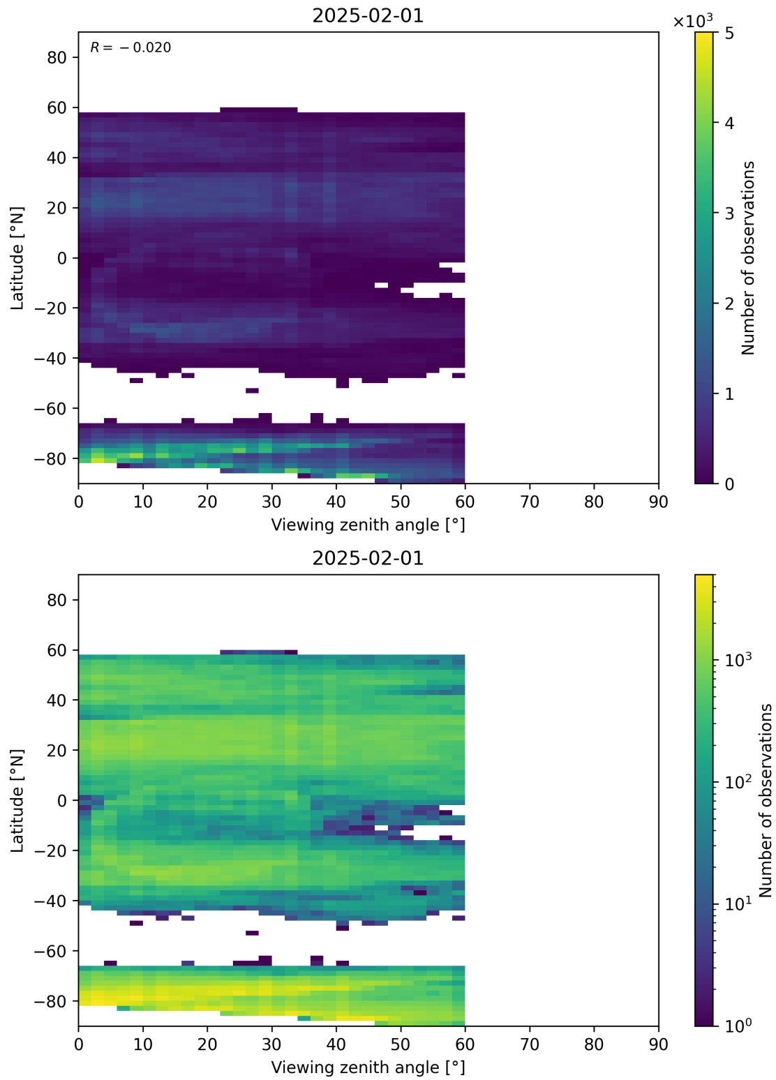
Figure 109: Scatter density plot of “Viewing zenith angle” against “Latitude” for 2025-01-31 to 2025-02-02.
