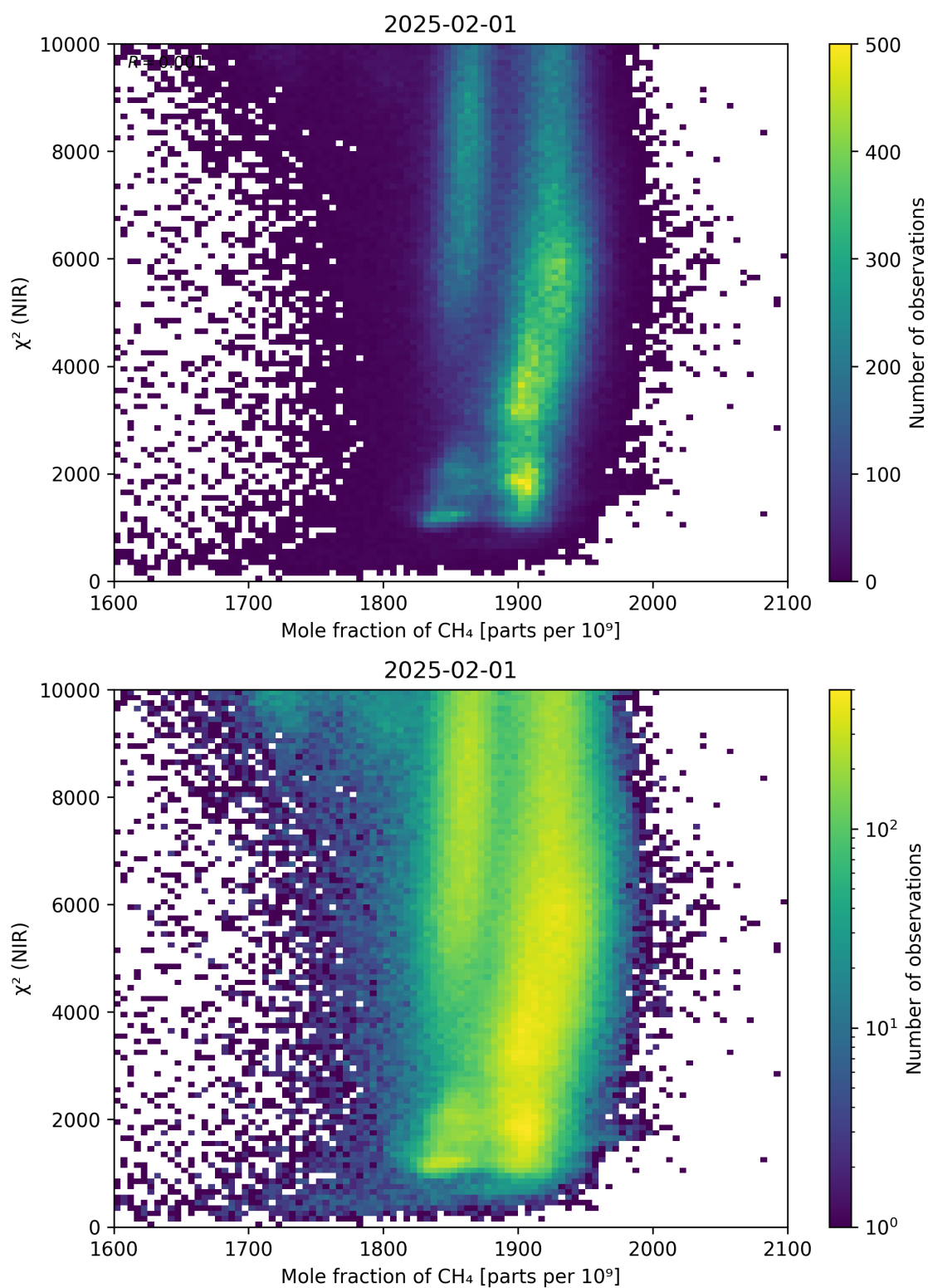
Figure 70: Scatter density plot of “Mole fraction of CH 4 ” against “ \chi^2 (NIR)” for 2025-01-31 to 2025-02-02.
