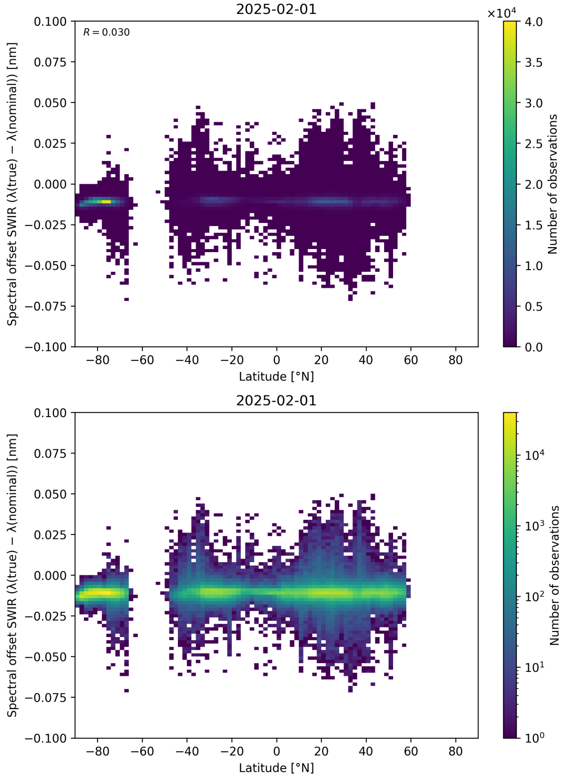
Figure 62: Scatter density plot of “Latitude” against “Spectral offset SWIR ( \lambda_{\text{true}} - \lambda_{\text{nominal}} )” for 2025-01-31 to 2025-02-02.
