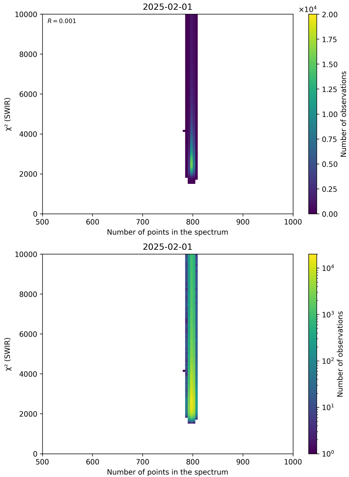
Figure 89: Scatter density plot of “Number of points in the spectrum” against “ \chi^2 (SWIR)” for 2025-01-31 to 2025-02-02.
