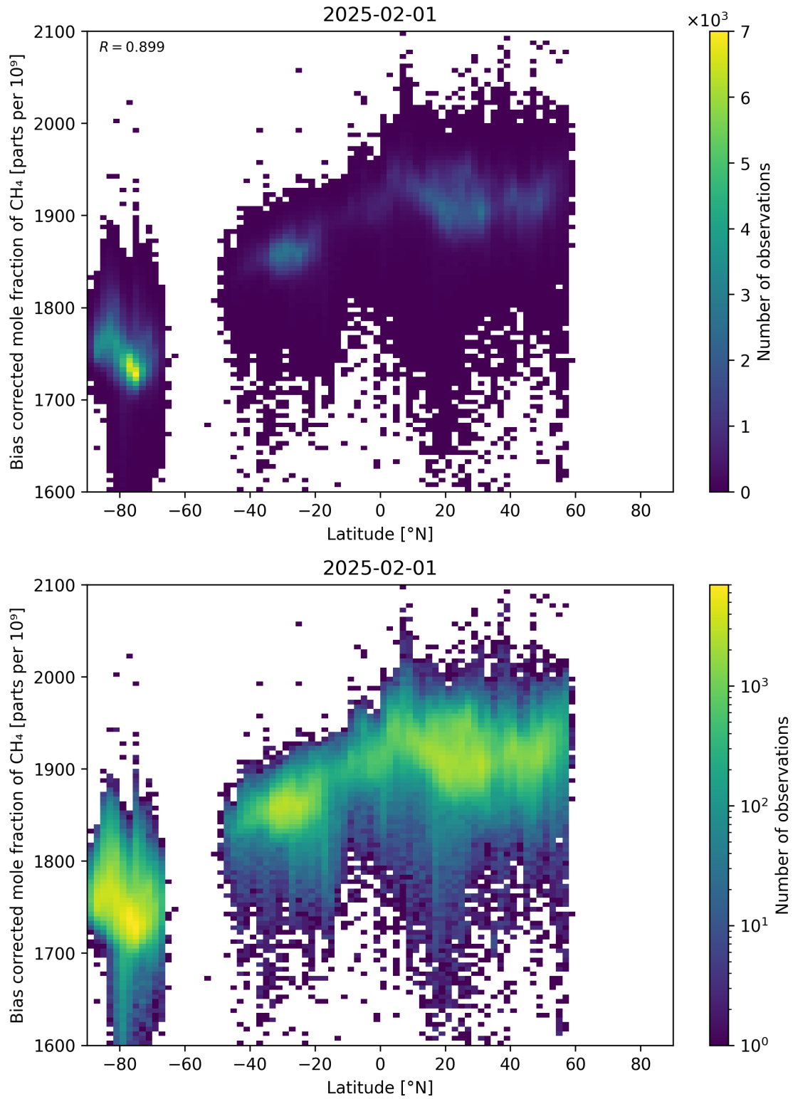
Figure 58: Scatter density plot of “Latitude” against “Bias corrected mole fraction of CH 4 ” for 2025-01-31 to 2025-02-02.
