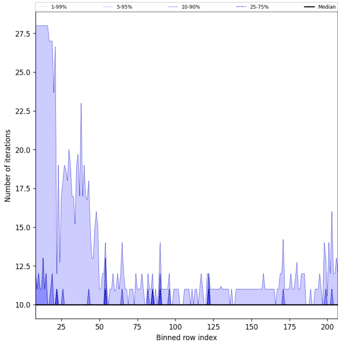
Figure 42: Along track statistics of “Number of iterations” for 2025-01-31 to 2025-02-02
