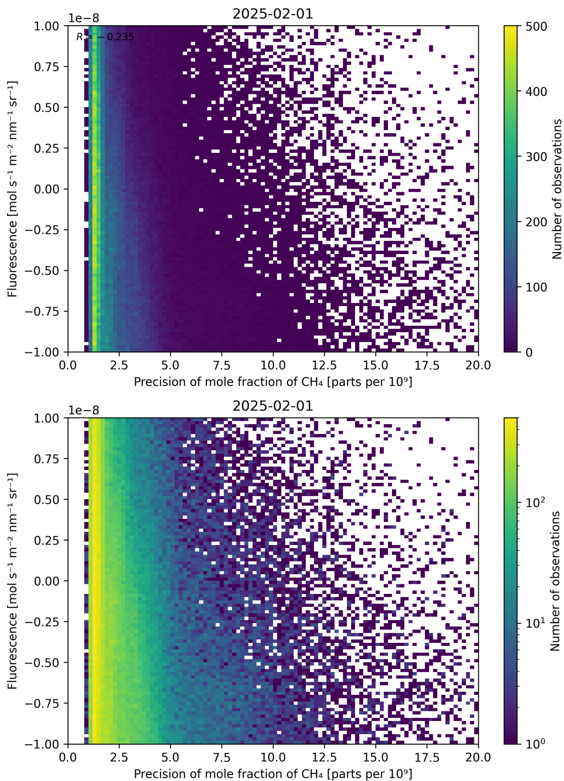
Figure 81: Scatter density plot of “Precision of mole fraction of \text{CH}_4 ” against “Fluorescence” for 2025-01-31 to 2025-02-02.
