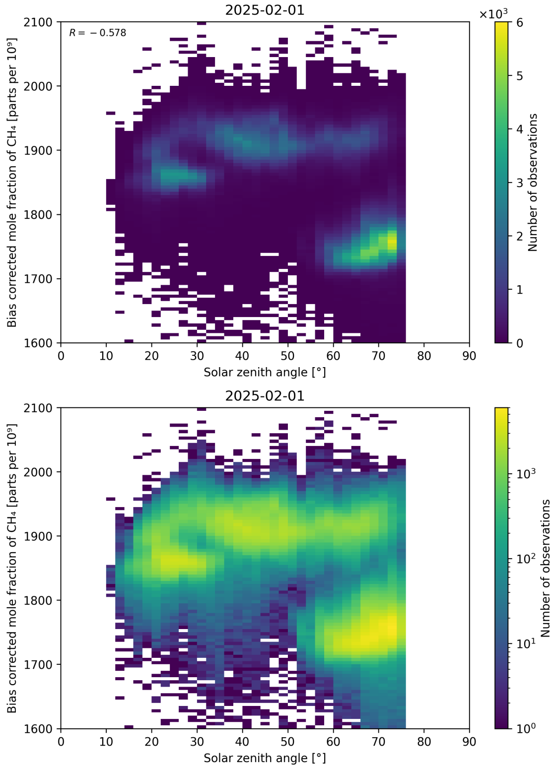
Figure 100: Scatter density plot of “Solar zenith angle” against “Bias corrected mole fraction of CH 4 ” for 2025-01-31 to 2025-02-02.
