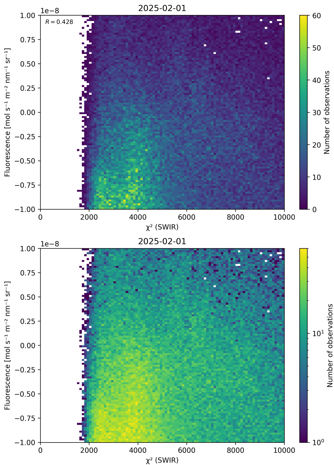
Figure 49: Scatter density plot of “ \chi^2 (SWIR)” against “Fluorescence” for 2025-01-31 to 2025-02-02.
