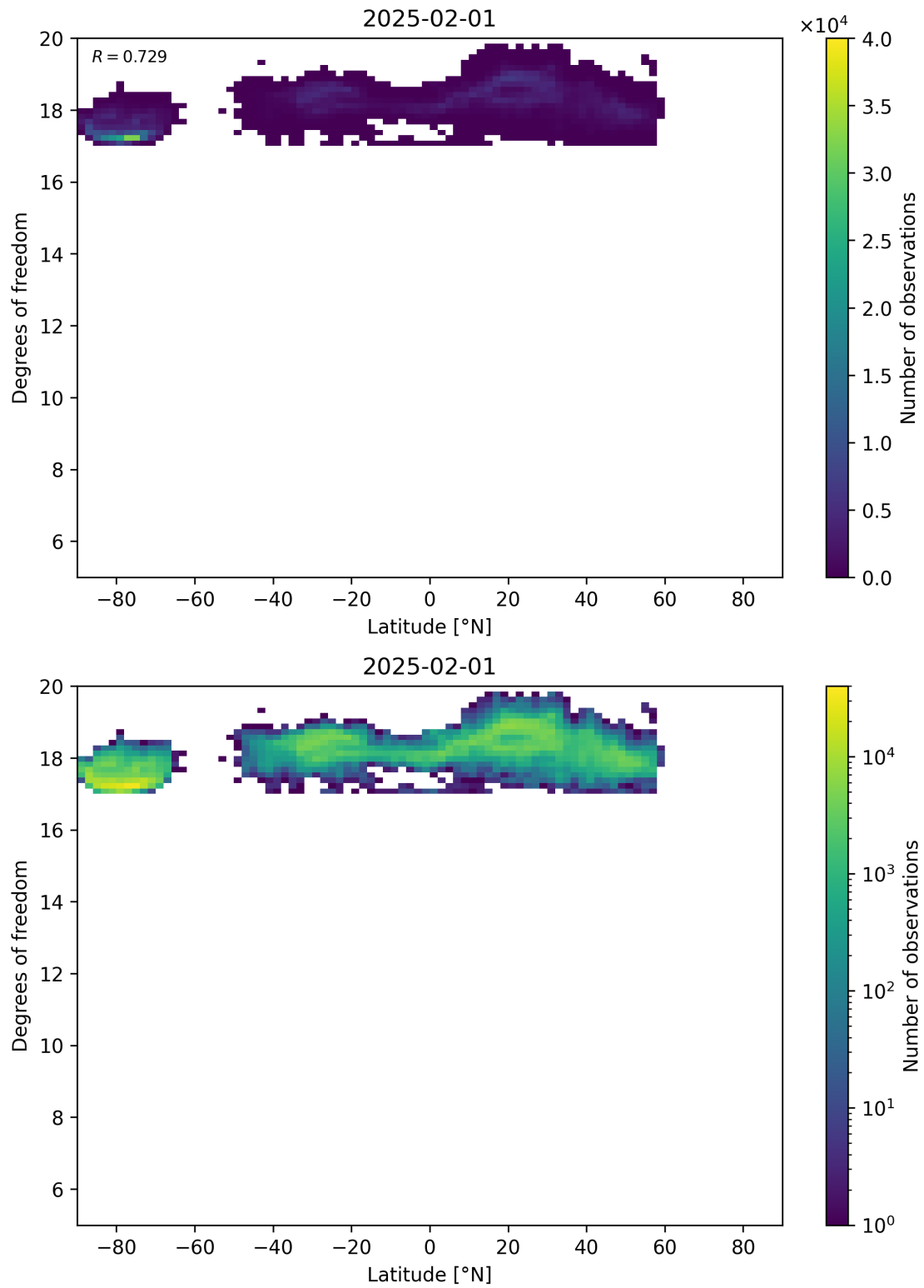
Figure 55: Scatter density plot of “Latitude” against “Degrees of freedom” for 2025-01-31 to 2025-02-02.
