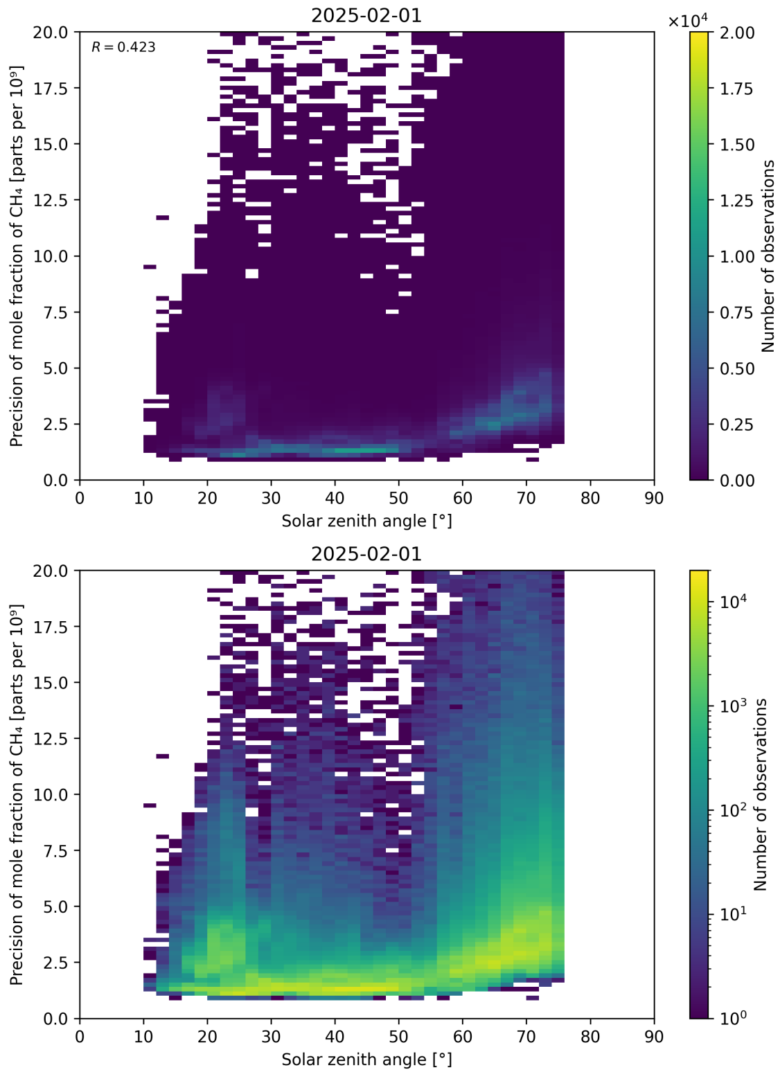
Figure 101: Scatter density plot of “Solar zenith angle” against “Precision of mole fraction of CH 4 ” for 2025-01-31 to 2025-02-02.
