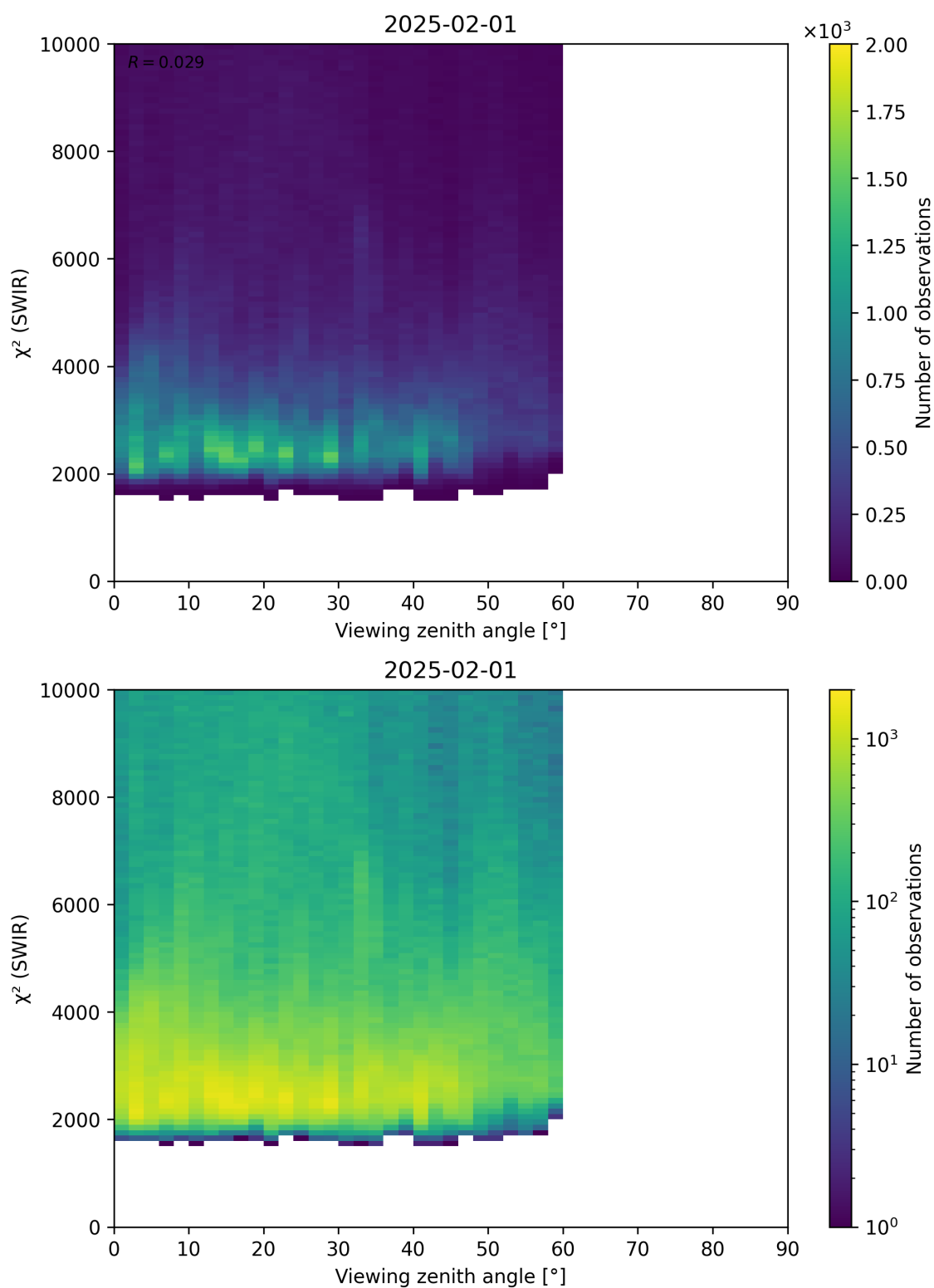
Figure 106: Scatter density plot of “Viewing zenith angle” against “ \chi^2 (SWIR)” for 2025-01-31 to 2025-02-02.
