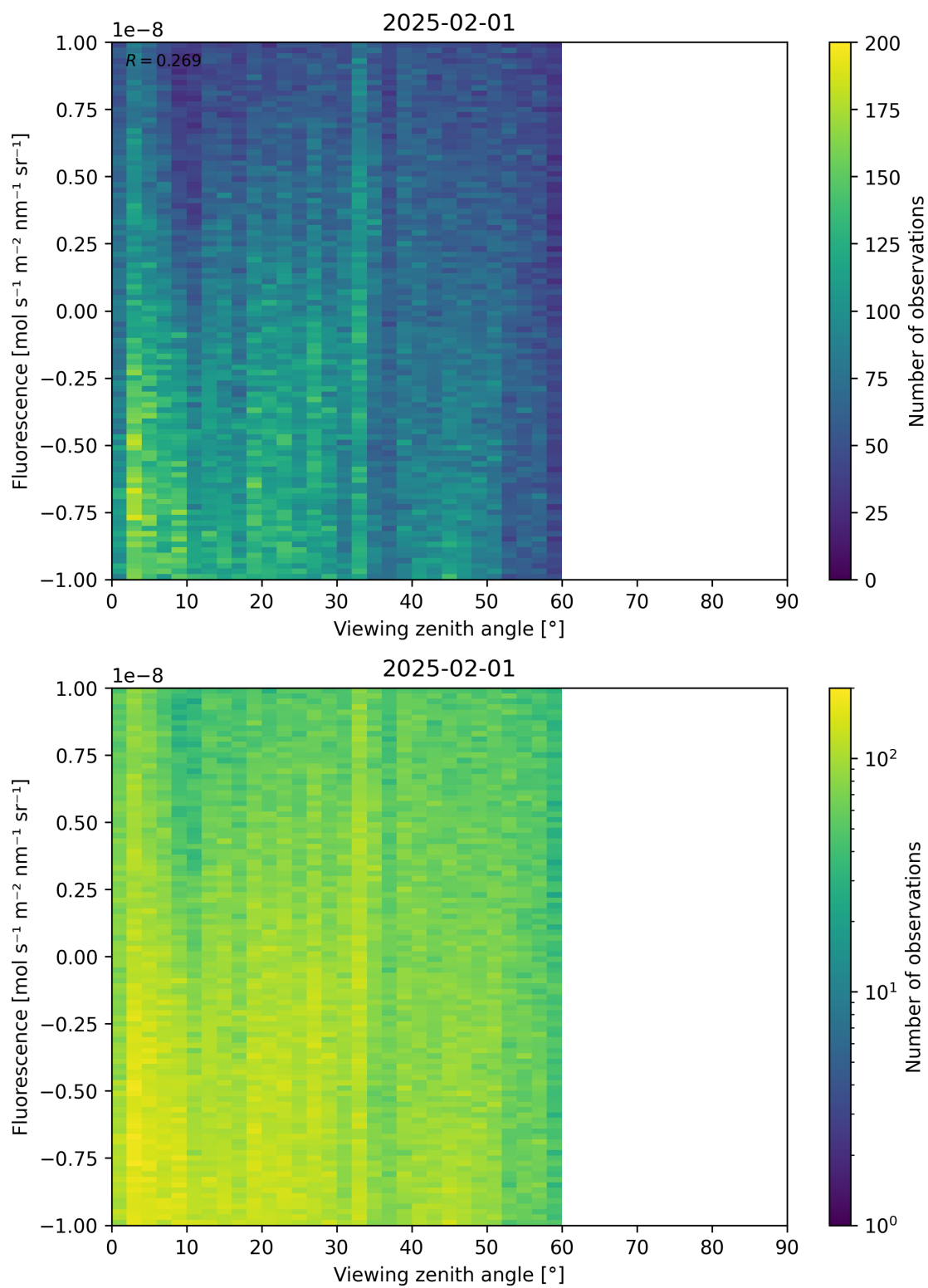
Figure 108: Scatter density plot of “Viewing zenith angle” against “Fluorescence” for 2025-01-31 to 2025-02-02.
