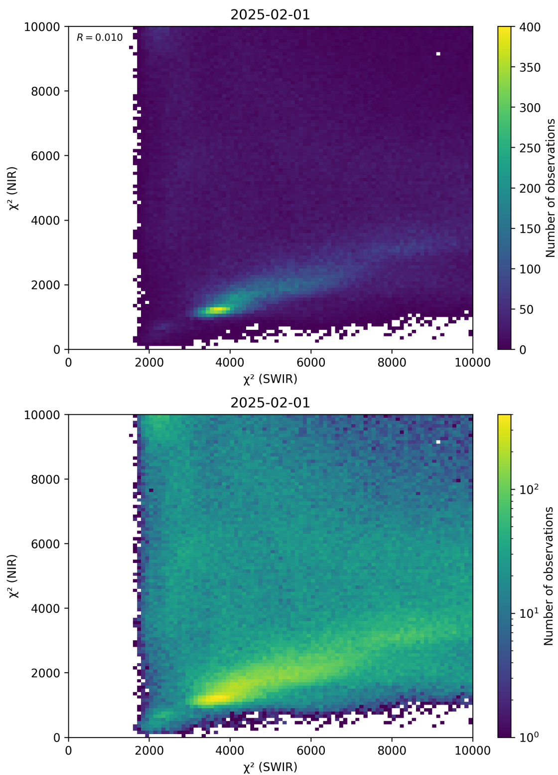
Figure 47: Scatter density plot of “ \chi^2 (SWIR)” against “ \chi^2 (NIR)” for 2025-01-31 to 2025-02-02.
