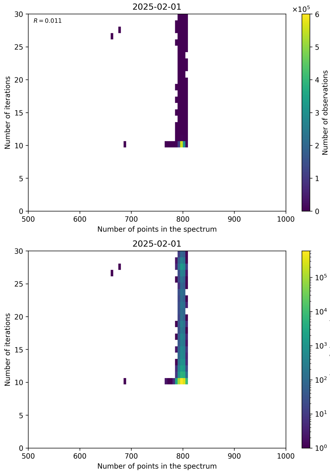
Figure 92: Scatter density plot of “Number of points in the spectrum” against “Number of iterations” for 2025-01-31 to 2025-02-02.
