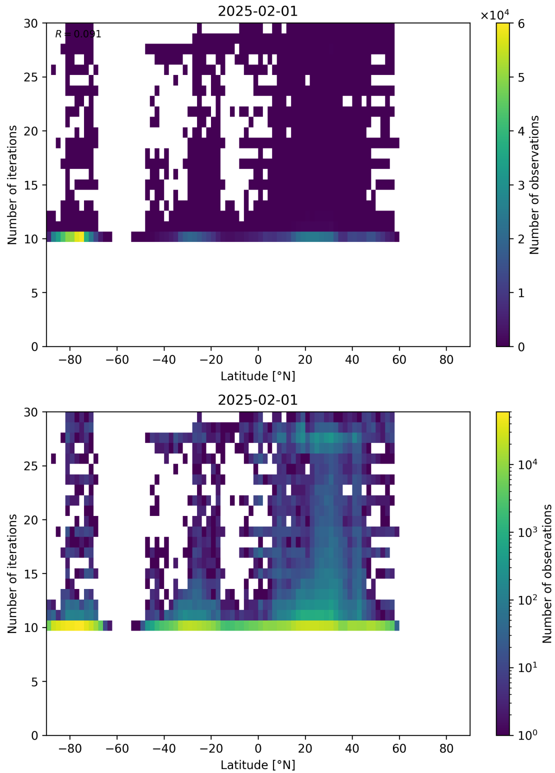
Figure 60: Scatter density plot of “Latitude” against “Number of iterations” for 2025-01-31 to 2025-02-02.
