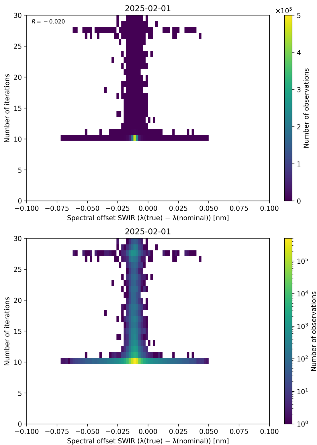
Figure 121: Scatter density plot of “Spectral offset SWIR ( \lambda_{\text{true}} - \lambda_{\text{nominal}} )” against “Number of iterations” for 2025-01-31 to 2025-02-02.
