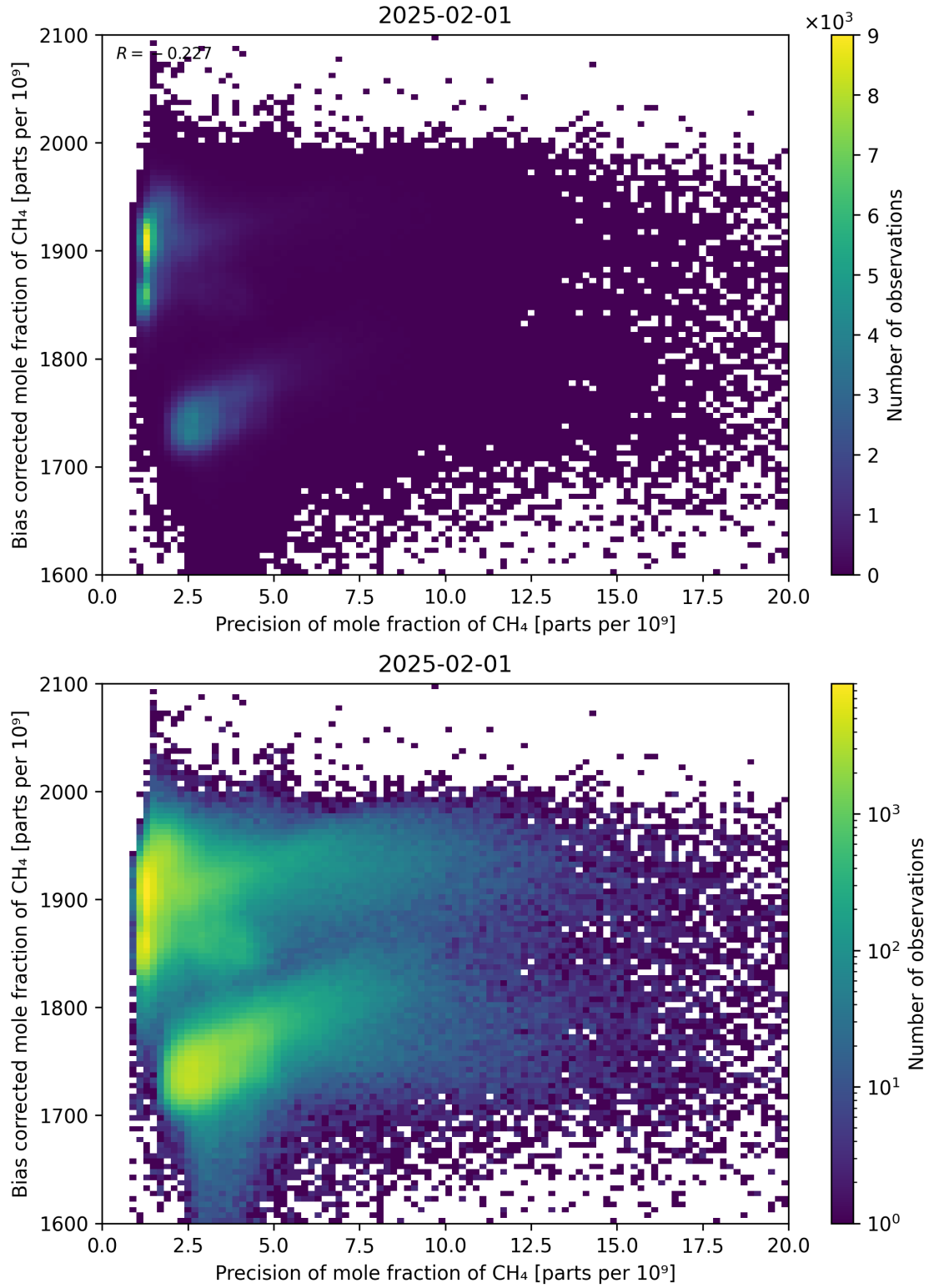
Figure 82: Scatter density plot of “Precision of mole fraction of CH 4 ” against “Bias corrected mole fraction of CH 4 ” for 2025-01-31 to 2025-02-02.
