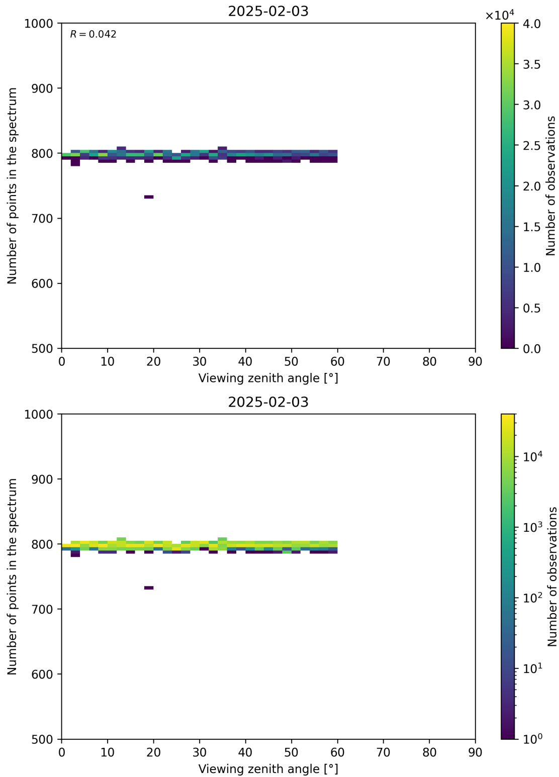
Figure 114: Scatter density plot of “Viewing zenith angle” against “Number of points in the spectrum” for 2025-02-03 to 2025-02-04.
