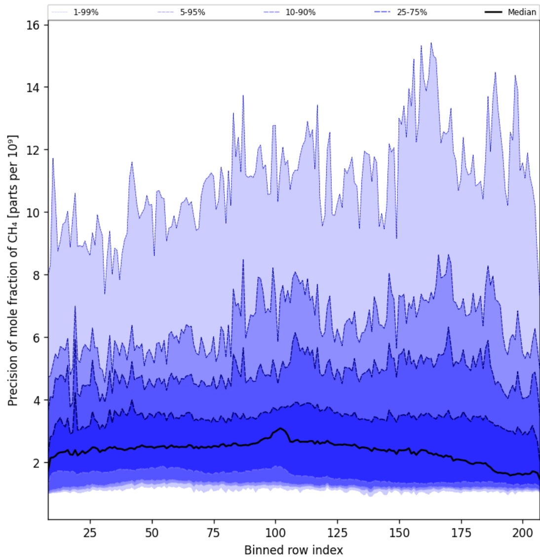
Figure 35: Along track statistics of “Precision of mole fraction of CH 4 ” for 2025-02-03 to 2025-02-04
