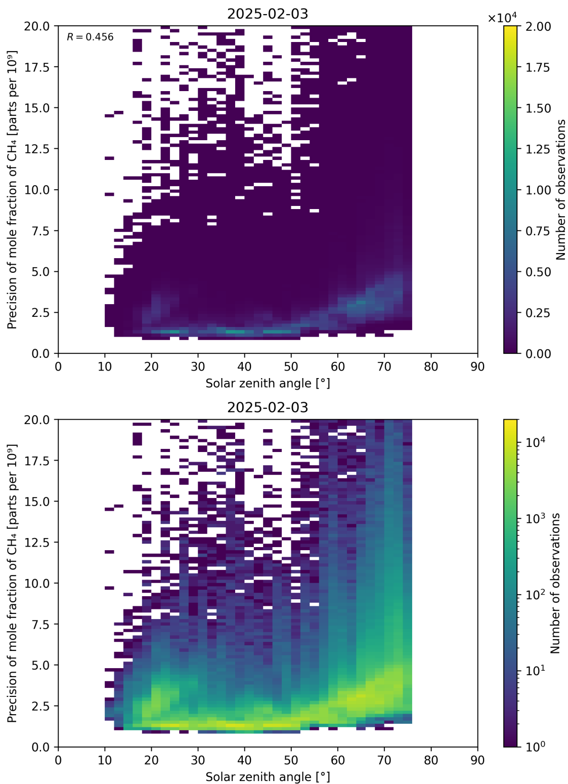
Figure 101: Scatter density plot of “Solar zenith angle” against “Precision of mole fraction of CH 4 ” for 2025-02-03 to 2025-02-04.
