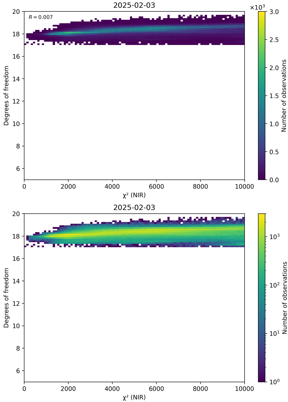
Figure 44: Scatter density plot of “ \chi^2 (NIR)” against “Degrees of freedom” for 2025-02-03 to 2025-02-04.
