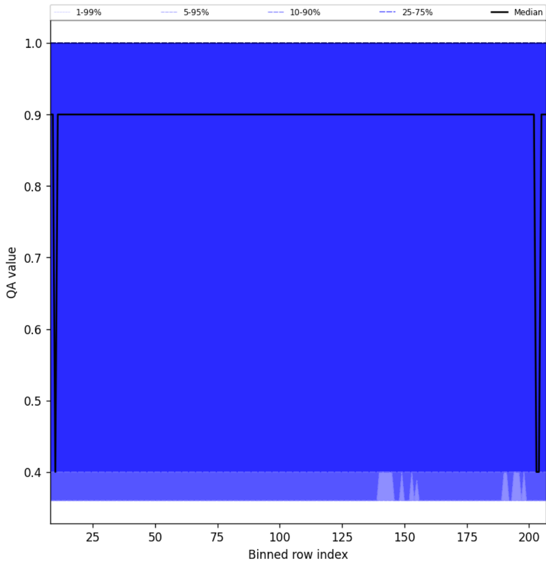
Figure 33: Along track statistics of “QA value” for 2025-02-03 to 2025-02-04
