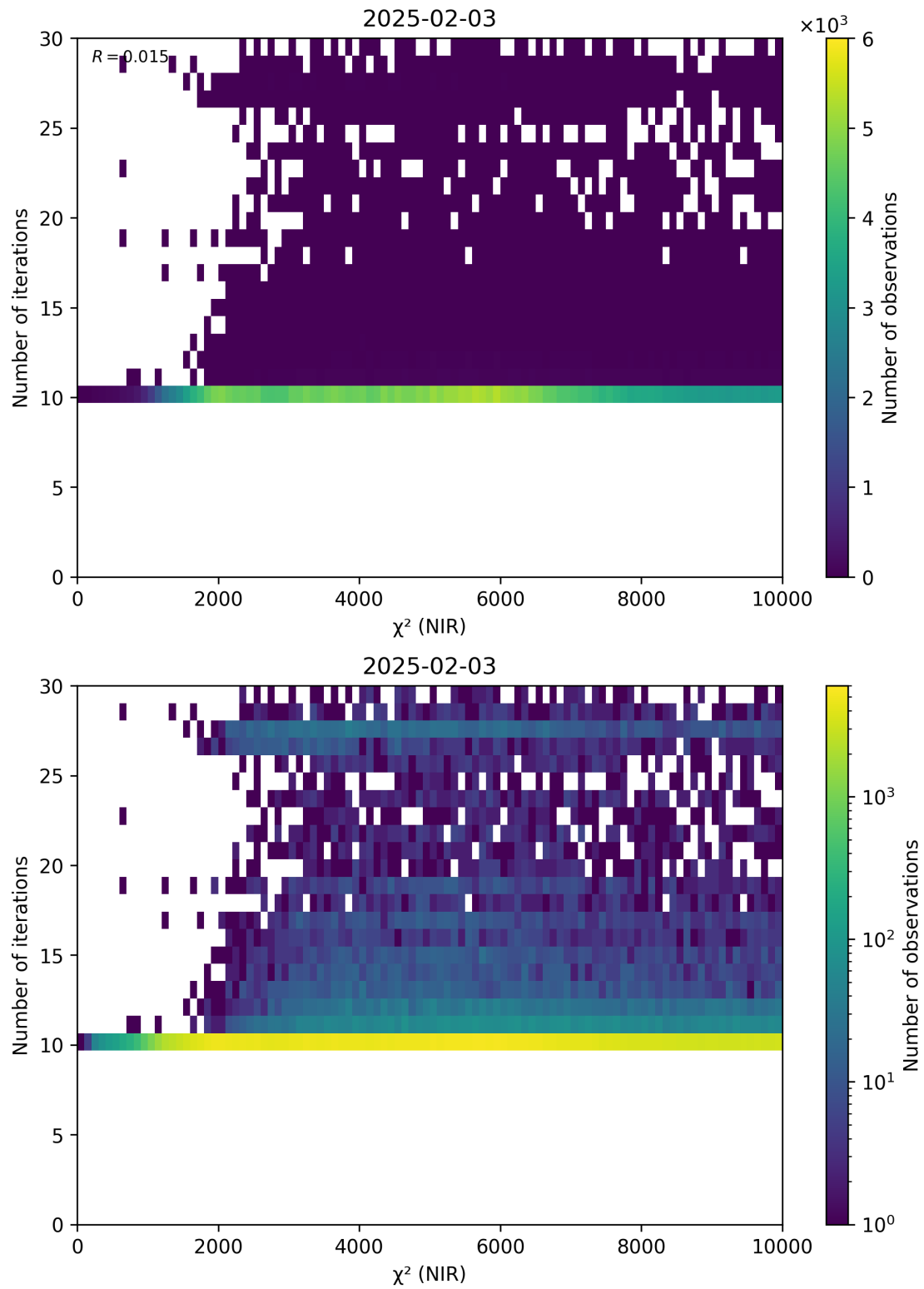
Figure 46: Scatter density plot of “ \chi^2 (NIR)” against “Number of iterations” for 2025-02-03 to 2025-02-04.
