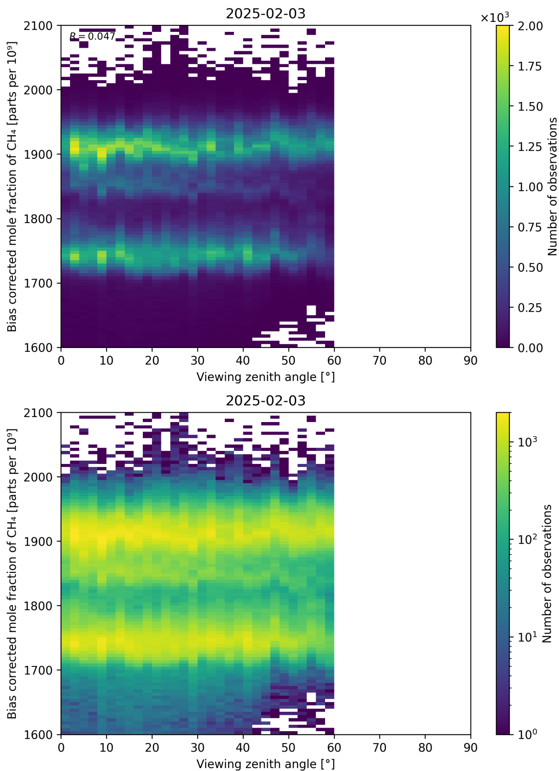
Figure 111: Scatter density plot of “Viewing zenith angle” against “Bias corrected mole fraction of CH 4 ” for 2025-02-03 to 2025-02-04.
