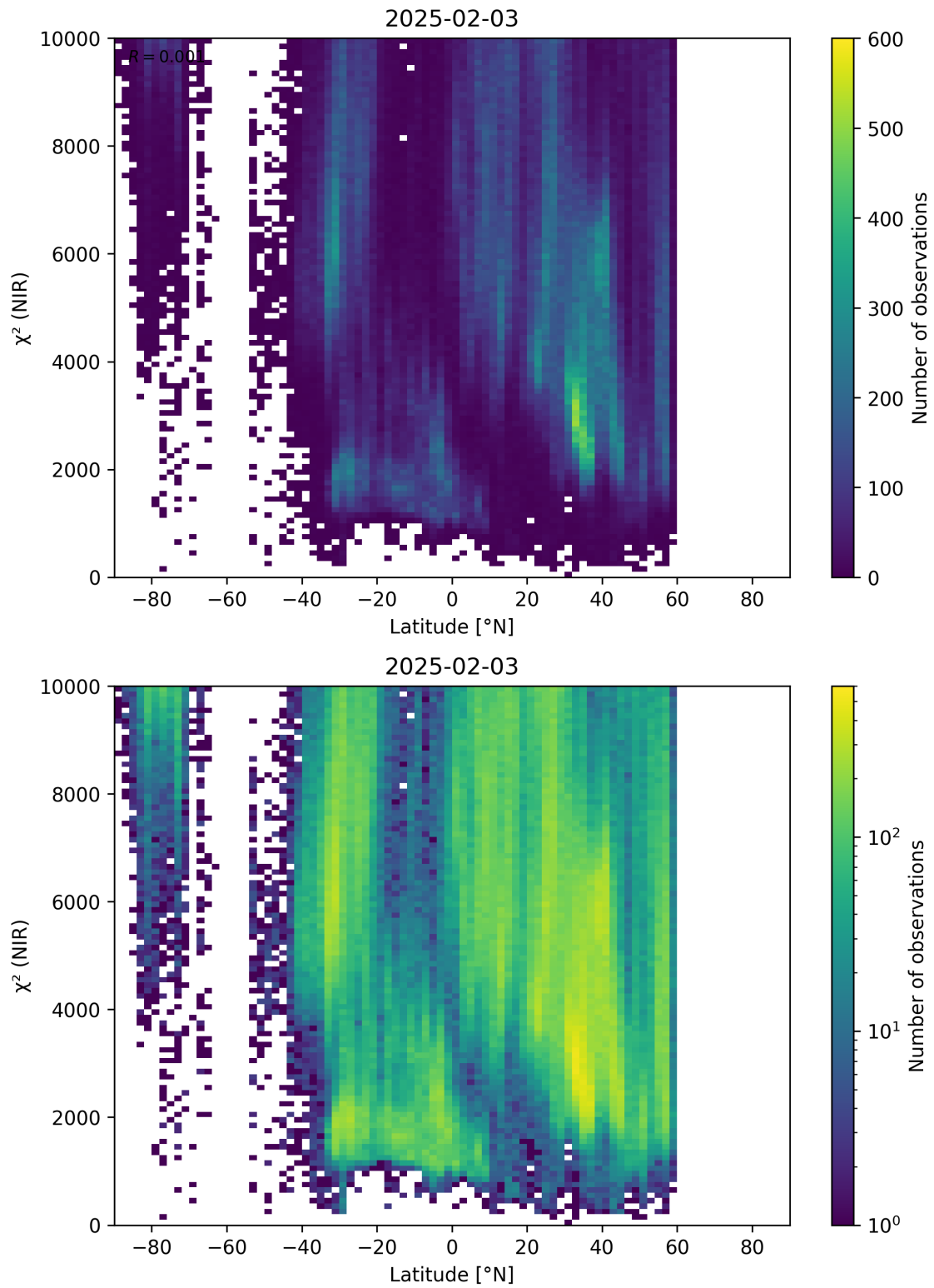
Figure 53: Scatter density plot of “Latitude” against “ \chi^2 (NIR)” for 2025-02-03 to 2025-02-04.
