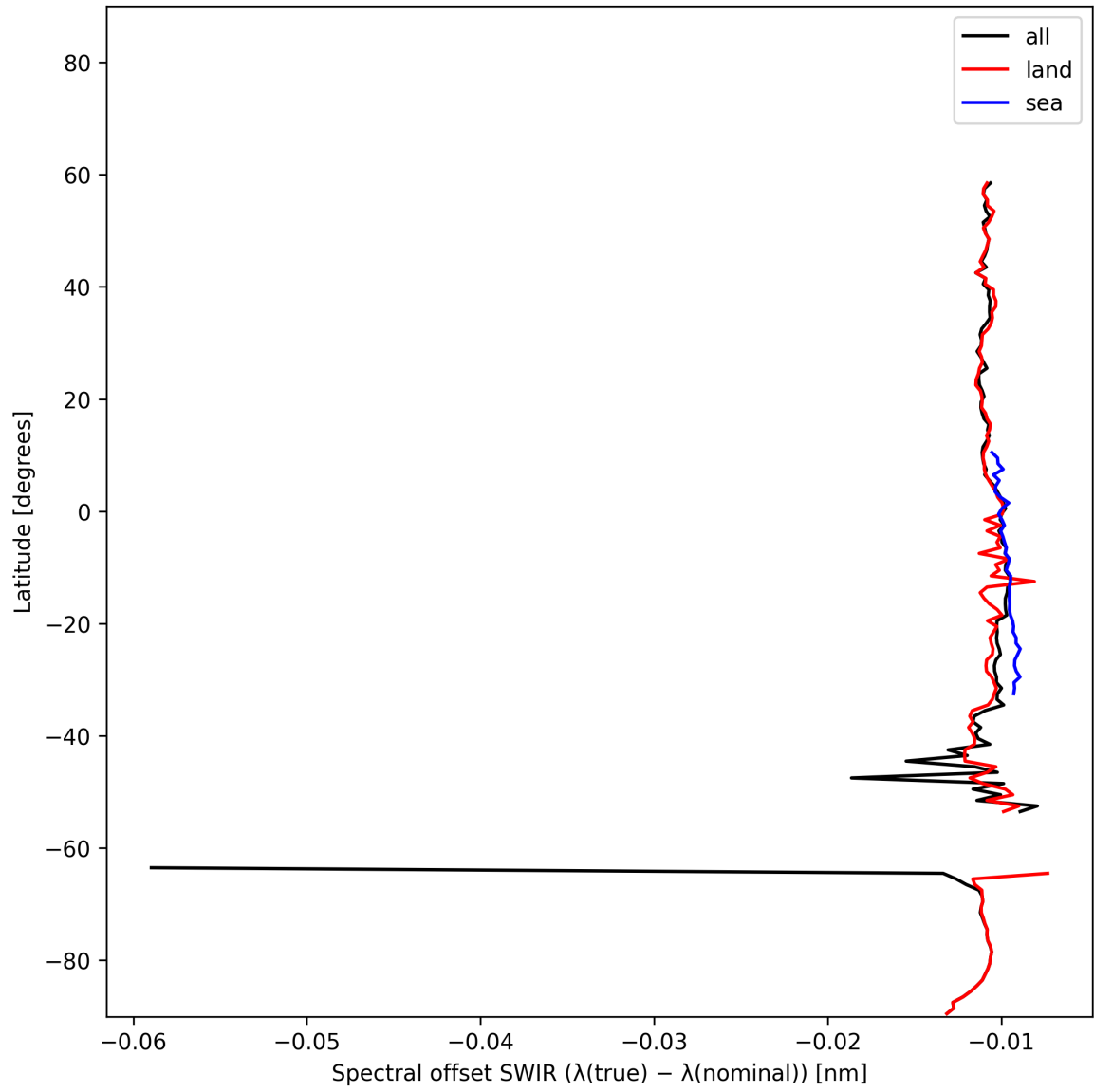
Figure 16: Zonal average of “Spectral offset SWIR ( \lambda_{\text{true}} - \lambda_{\text{nominal}} )” for 2025-02-03 to 2025-02-04.
