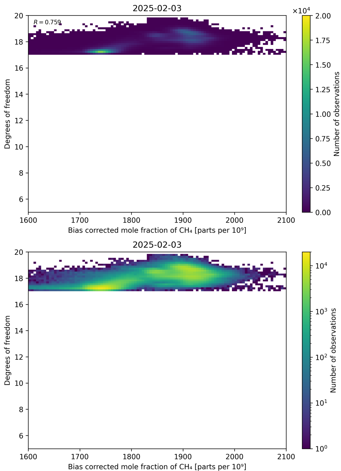
Figure 65: Scatter density plot of “Bias corrected mole fraction of CH 4 ” against “Degrees of freedom” for 2025-02-03 to 2025-02-04.
