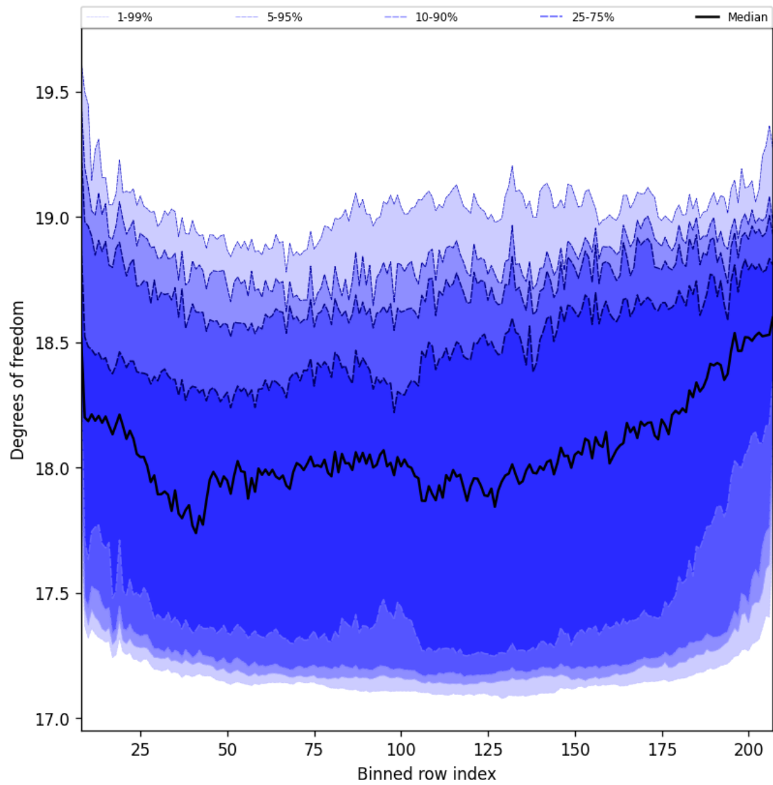
Figure 41: Along track statistics of “Degrees of freedom” for 2025-02-03 to 2025-02-04
