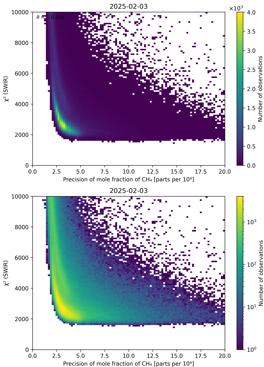
Figure 79: Scatter density plot of “Precision of mole fraction of \text{CH}_4 ” against “ \chi^2 (SWIR)” for 2025-02-03 to 2025-02-04.
