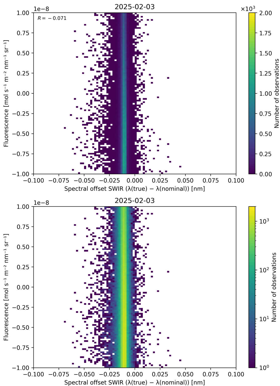
Figure 120: Scatter density plot of “Spectral offset SWIR ( \lambda_{\text{true}} - \lambda_{\text{nominal}} )” against “Fluorescence” for 2025-02-03 to 2025-02-04.
