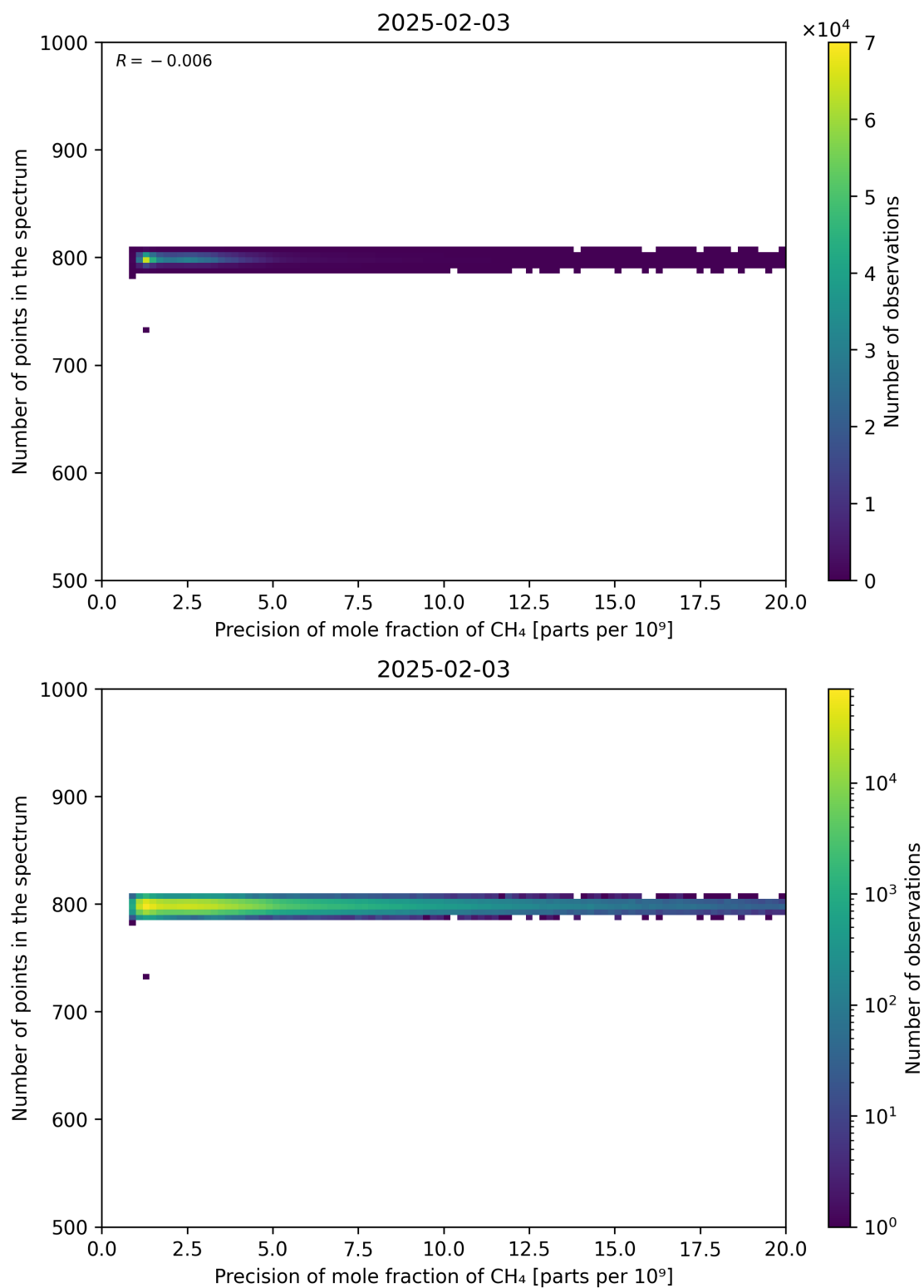
Figure 84: Scatter density plot of “Precision of mole fraction of CH 4 ” against “Number of points in the spectrum” for 2025-02-03 to 2025-02-04.
