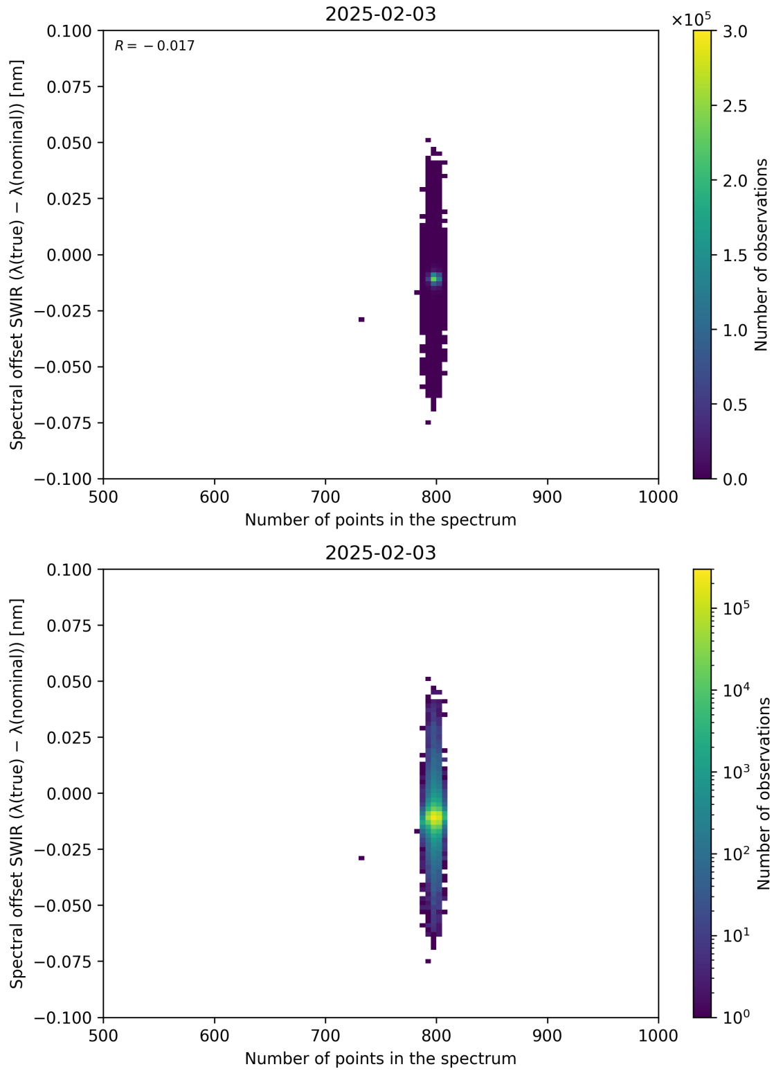
Figure 93: Scatter density plot of “Number of points in the spectrum” against “Spectral offset SWIR ( \lambda_{\text{true}} - \lambda_{\text{nominal}} )” for 2025-02-03 to 2025-02-04.
