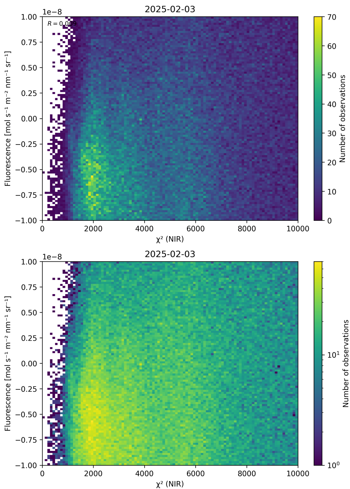
Figure 45: Scatter density plot of “ \chi^2 (NIR)” against “Fluorescence” for 2025-02-03 to 2025-02-04.
