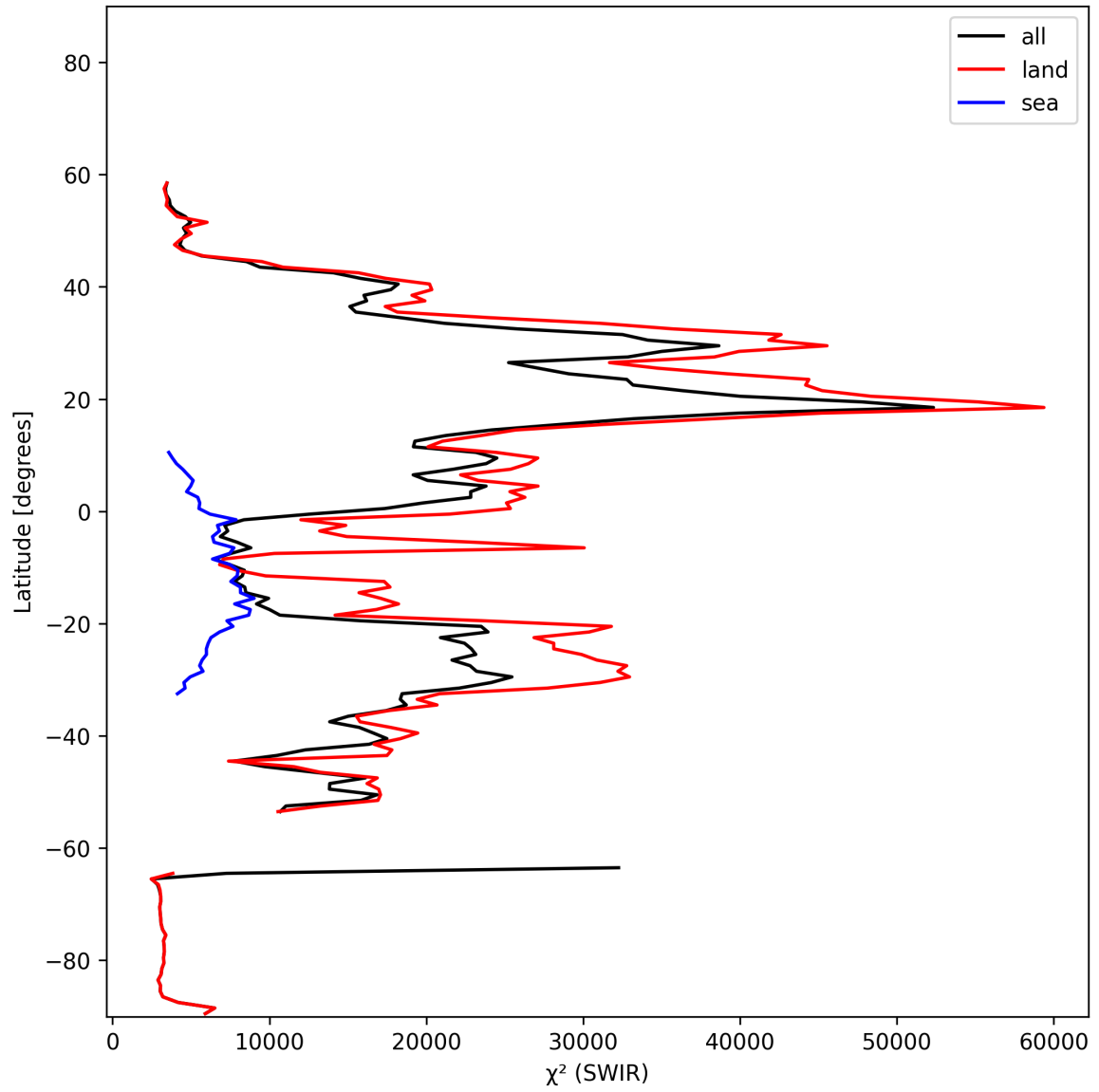
Figure 17: Zonal average of “ \chi^2 (SWIR)” for 2025-02-03 to 2025-02-04.
