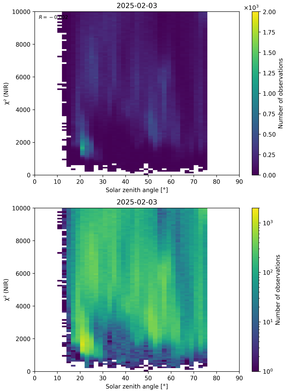
Figure 94: Scatter density plot of “Solar zenith angle” against “ \chi^2 (NIR)” for 2025-02-03 to 2025-02-04.
