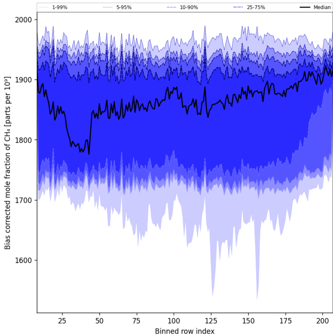
Figure 36: Along track statistics of “Bias corrected mole fraction of CH 4 ” for 2025-02-03 to 2025-02-04
