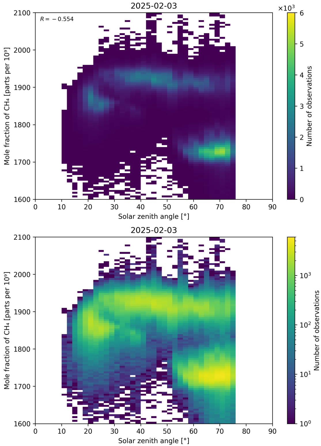
Figure 99: Scatter density plot of “Solar zenith angle” against “Mole fraction of CH 4 ” for 2025-02-03 to 2025-02-04.
