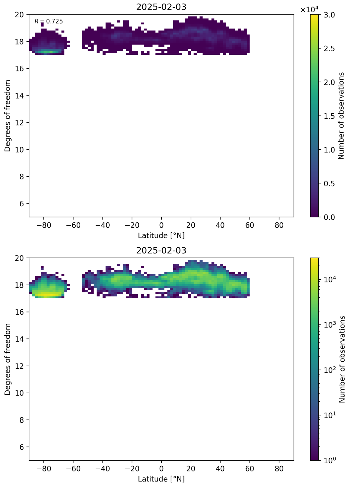
Figure 55: Scatter density plot of “Latitude” against “Degrees of freedom” for 2025-02-03 to 2025-02-04.
