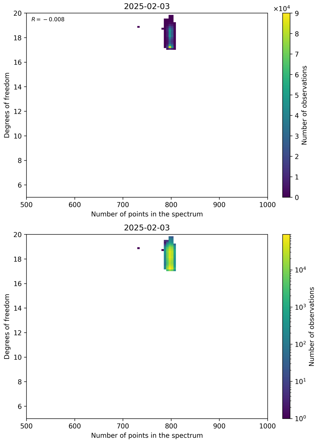
Figure 90: Scatter density plot of “Number of points in the spectrum” against “Degrees of freedom” for 2025-02-03 to 2025-02-04.
