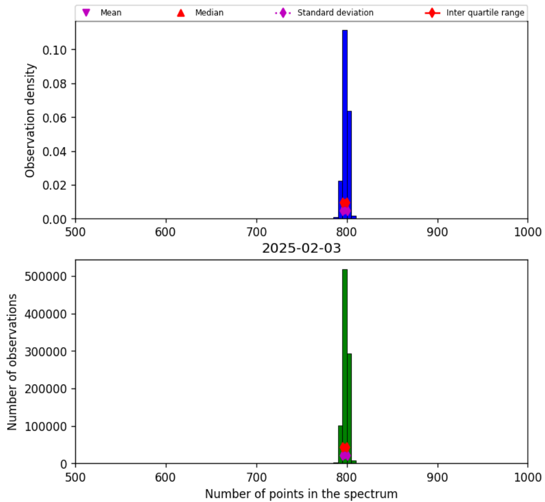
Figure 26: Histogram of “Number of points in the spectrum” for 2025-02-03 to 2025-02-04
