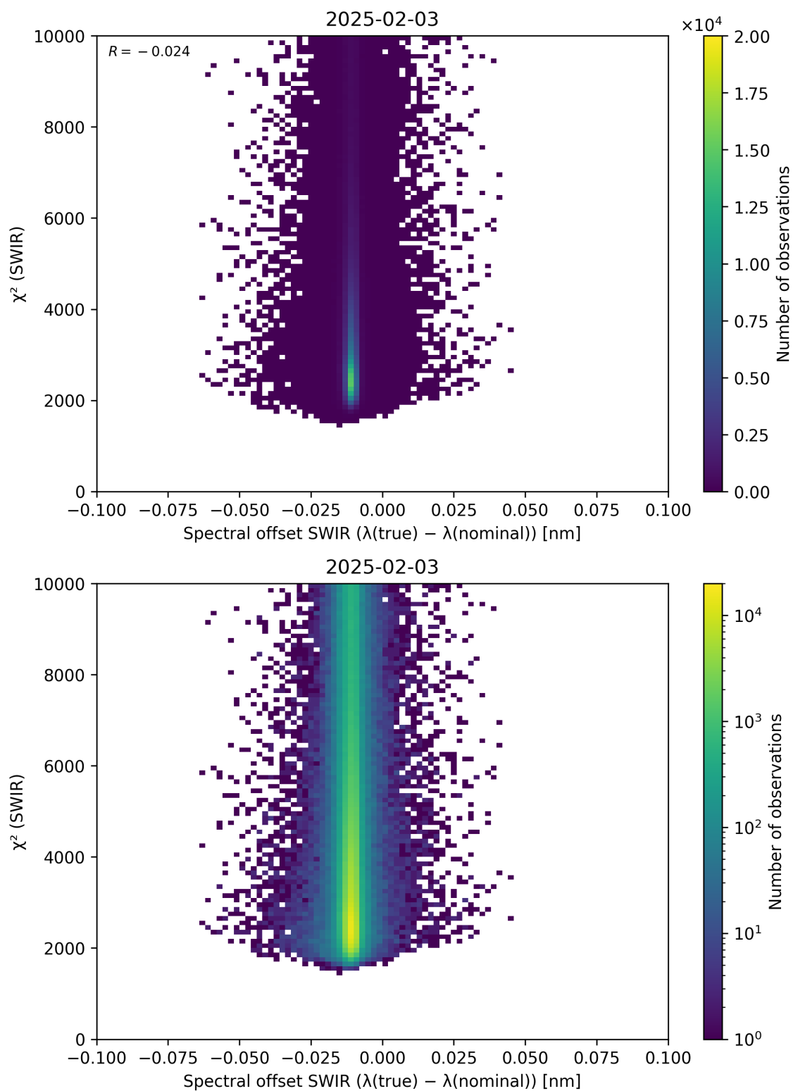
Figure 118: Scatter density plot of “Spectral offset SWIR ( \lambda_{\text{true}} - \lambda_{\text{nominal}} )” against “ \chi^2 (SWIR)” for 2025-02-03 to 2025-02-04.
