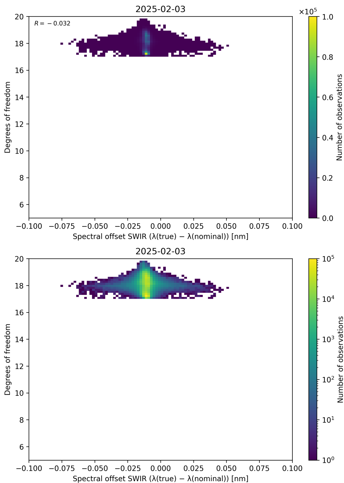
Figure 119: Scatter density plot of “Spectral offset SWIR ( \lambda_{\text{true}} - \lambda_{\text{nominal}} )” against “Degrees of freedom” for 2025-02-03 to 2025-02-04.
