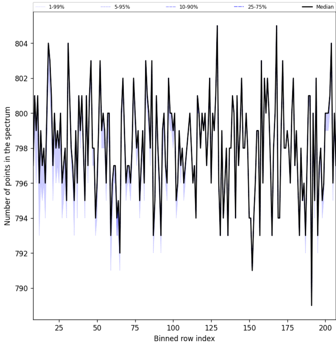
Figure 37: Along track statistics of “Number of points in the spectrum” for 2025-02-03 to 2025-02-04
