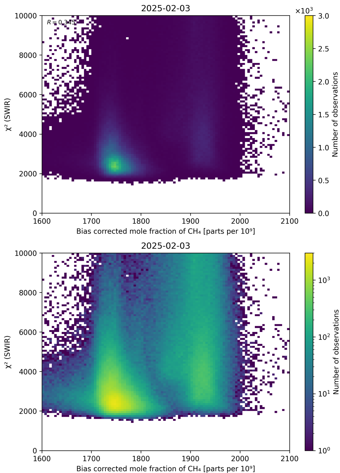
Figure 64: Scatter density plot of “Bias corrected mole fraction of \text{CH}_4 ” against “ \chi^2 (SWIR)” for 2025-02-03 to 2025-02-04.
