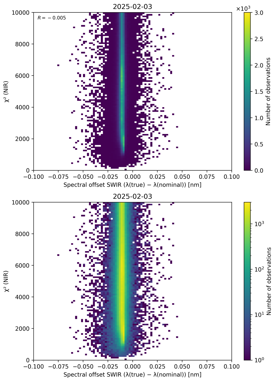
Figure 117: Scatter density plot of “Spectral offset SWIR ( \lambda_{\text{true}} - \lambda_{\text{nominal}} )” against “ \chi^2 (NIR)” for 2025-02-03 to 2025-02-04.
