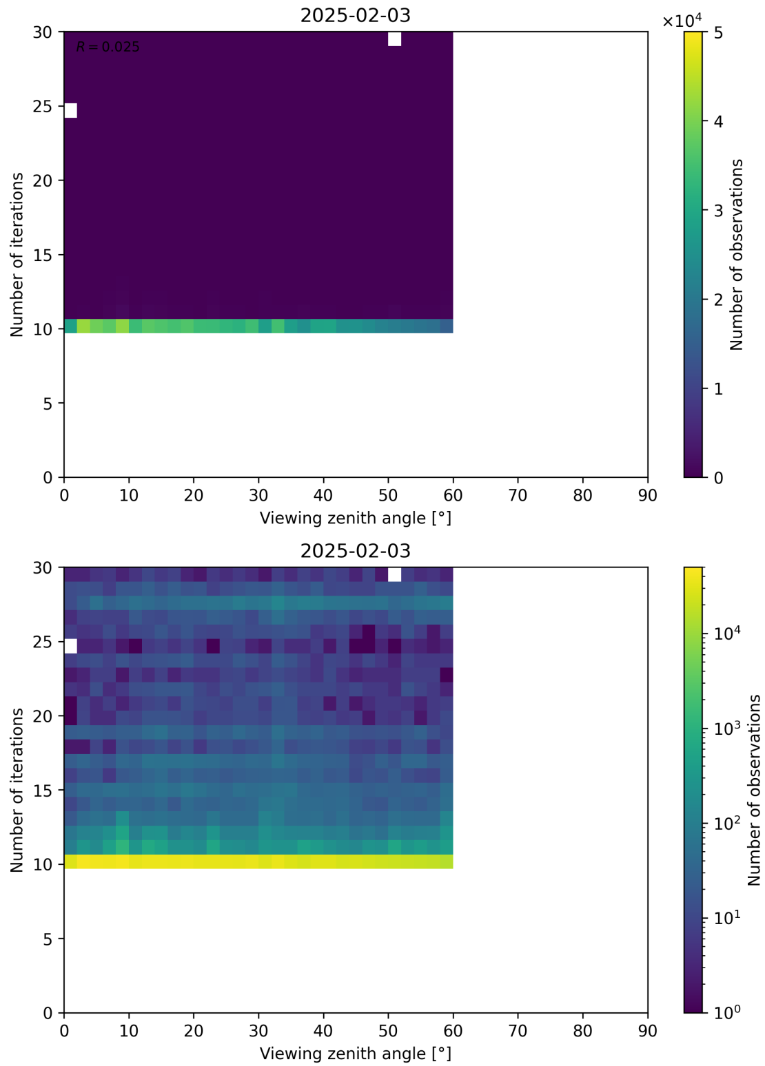
Figure 113: Scatter density plot of “Viewing zenith angle” against “Number of iterations” for 2025-02-03 to 2025-02-04.
