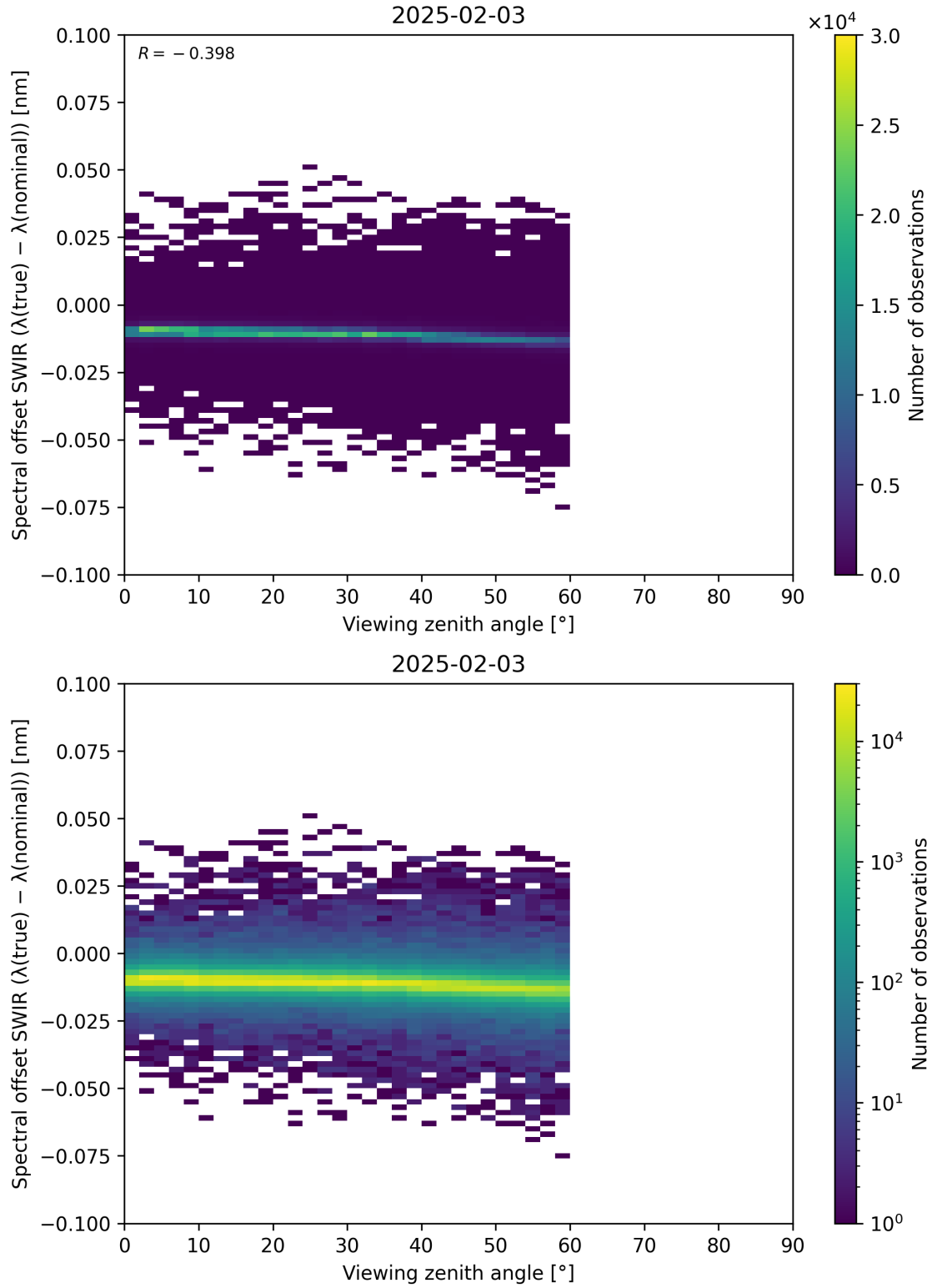
Figure 116: Scatter density plot of “Viewing zenith angle” against “Spectral offset SWIR ( \lambda_{\text{true}} - \lambda_{\text{nominal}} )” for 2025-02-03 to 2025-02-04.
