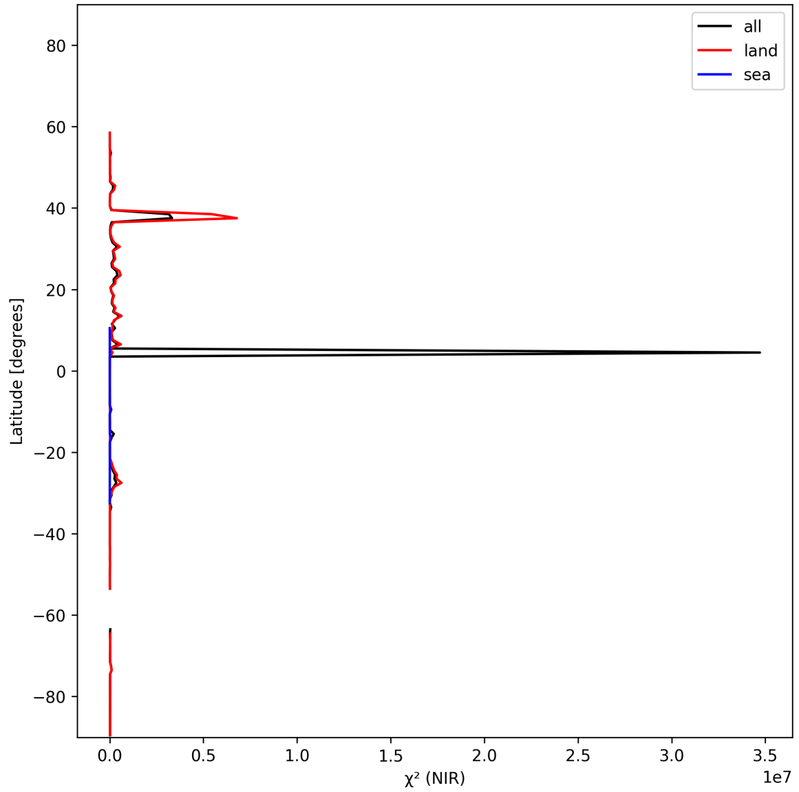
Figure 18: Zonal average of “ \chi^2 (NIR)” for 2025-02-03 to 2025-02-04.
