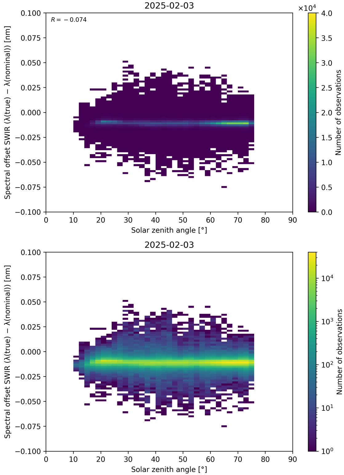
Figure 104: Scatter density plot of “Solar zenith angle” against “Spectral offset SWIR ( \lambda_{\text{true}} - \lambda_{\text{nominal}} )” for 2025-02-03 to 2025-02-04.
