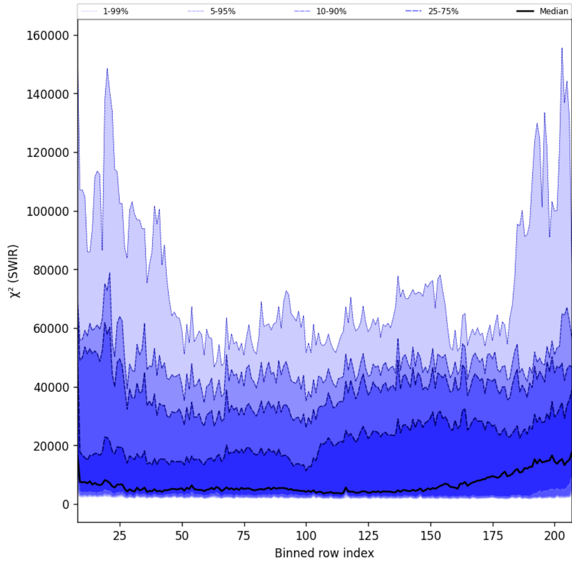
Figure 39: Along track statistics of “ \chi^2 (SWIR)” for 2025-02-03 to 2025-02-04
