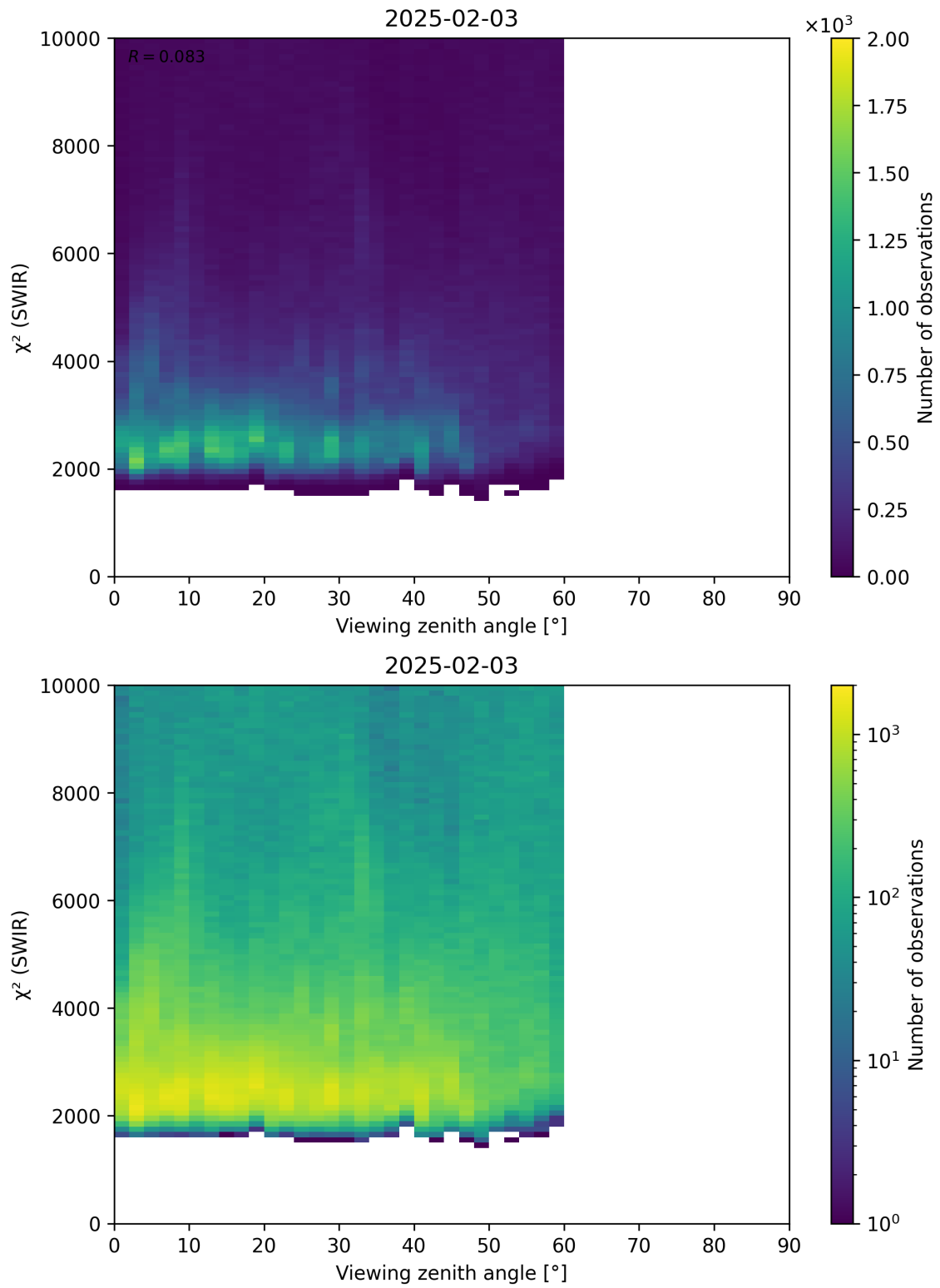
Figure 106: Scatter density plot of “Viewing zenith angle” against “ \chi^2 (SWIR)” for 2025-02-03 to 2025-02-04.
