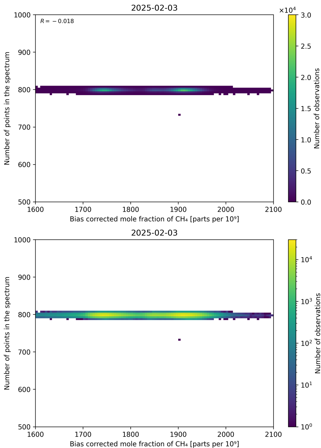
Figure 68: Scatter density plot of “Bias corrected mole fraction of CH 4 ” against “Number of points in the spectrum” for 2025-02-03 to 2025-02-04.
