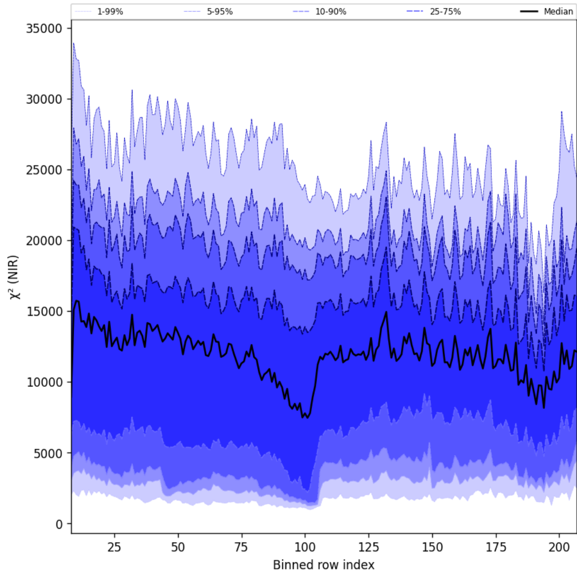
Figure 40: Along track statistics of “ \chi^2 (NIR)” for 2025-02-03 to 2025-02-04
