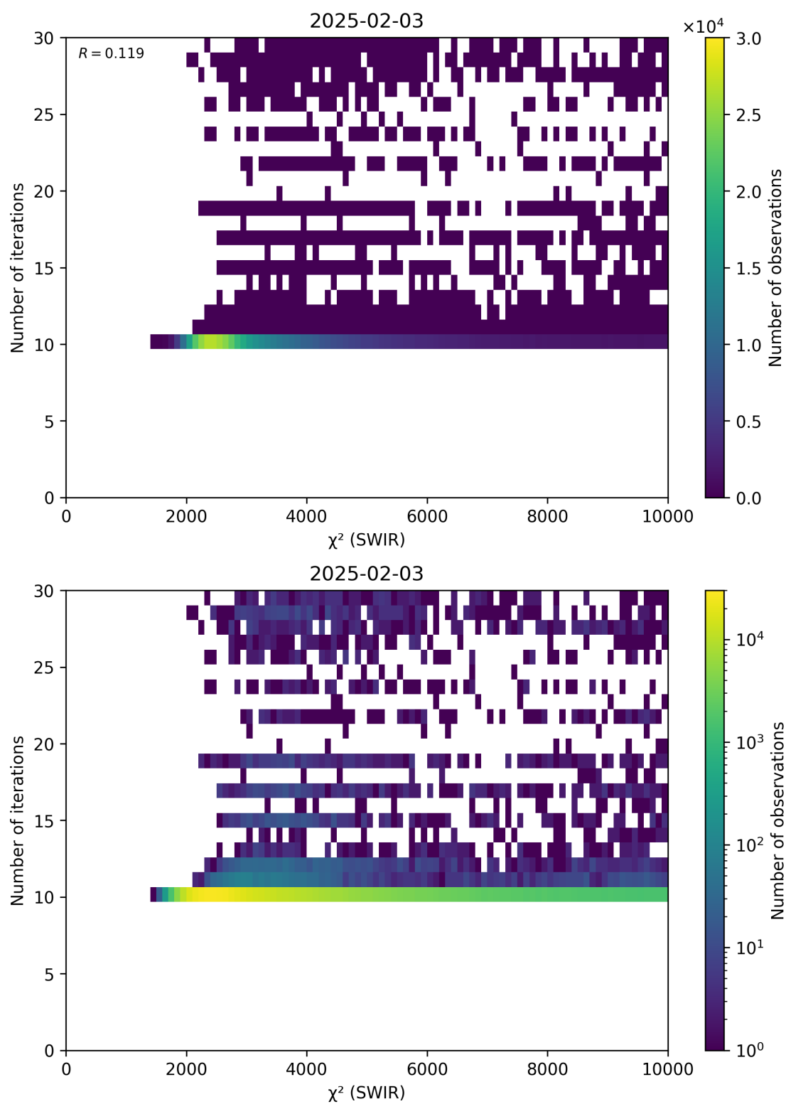
Figure 50: Scatter density plot of “ \chi^2 (SWIR)” against “Number of iterations” for 2025-02-03 to 2025-02-04.
