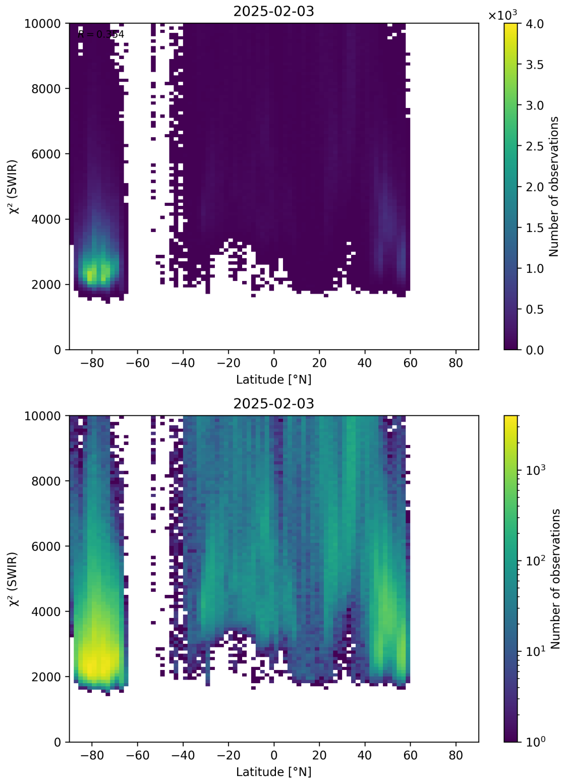
Figure 54: Scatter density plot of “Latitude” against “ \chi^2 (SWIR)” for 2025-02-03 to 2025-02-04.
