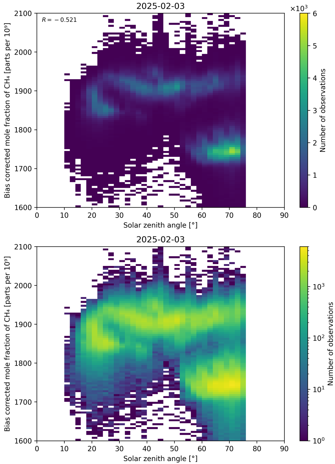
Figure 100: Scatter density plot of “Solar zenith angle” against “Bias corrected mole fraction of CH 4 ” for 2025-02-03 to 2025-02-04.
