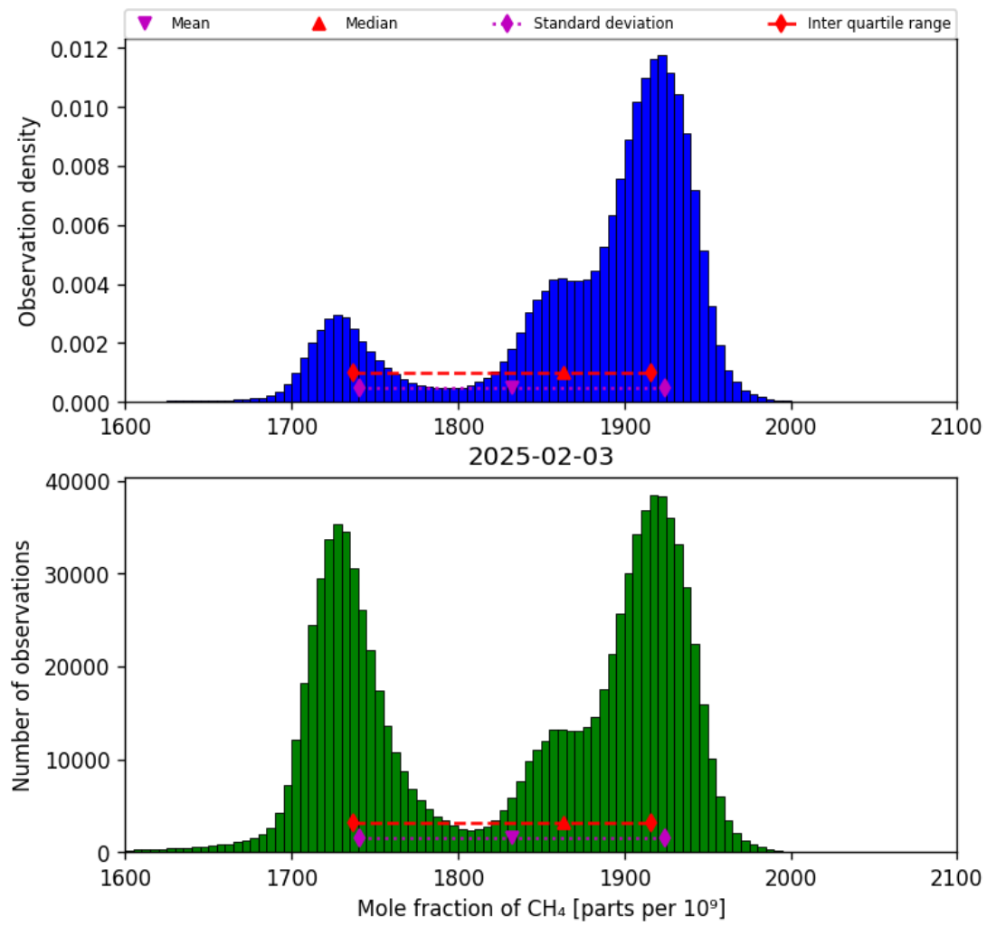
Figure 23: Histogram of “Mole fraction of CH 4 ” for 2025-02-03 to 2025-02-04
