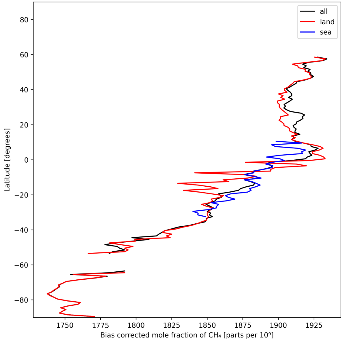
Figure 14: Zonal average of “Bias corrected mole fraction of CH 4 ” for 2025-02-03 to 2025-02-04.
