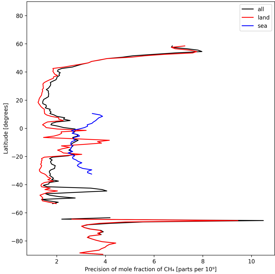
Figure 13: Zonal average of “Precision of mole fraction of CH 4 ” for 2025-02-03 to 2025-02-04.
