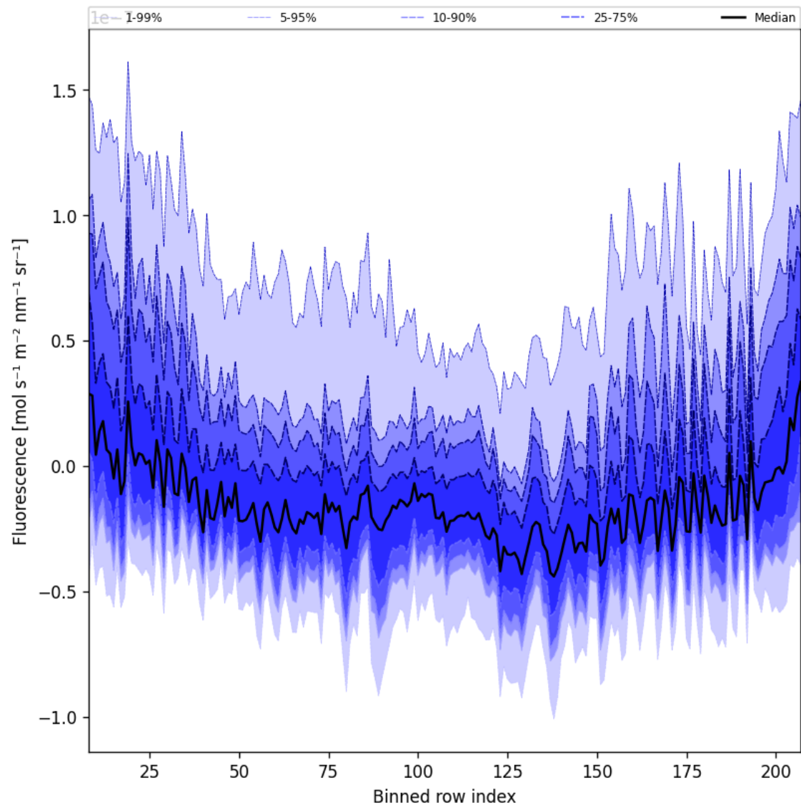
Figure 43: Along track statistics of “Fluorescence” for 2025-02-03 to 2025-02-04
