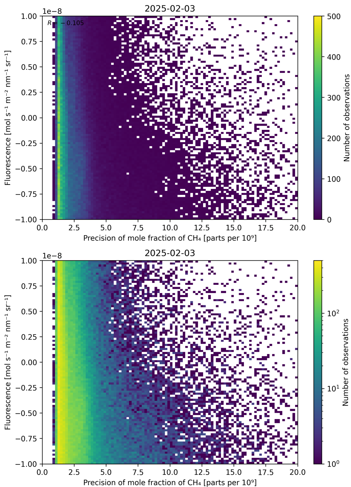
Figure 81: Scatter density plot of “Precision of mole fraction of CH 4 ” against “Fluorescence” for 2025-02-03 to 2025-02-04.
