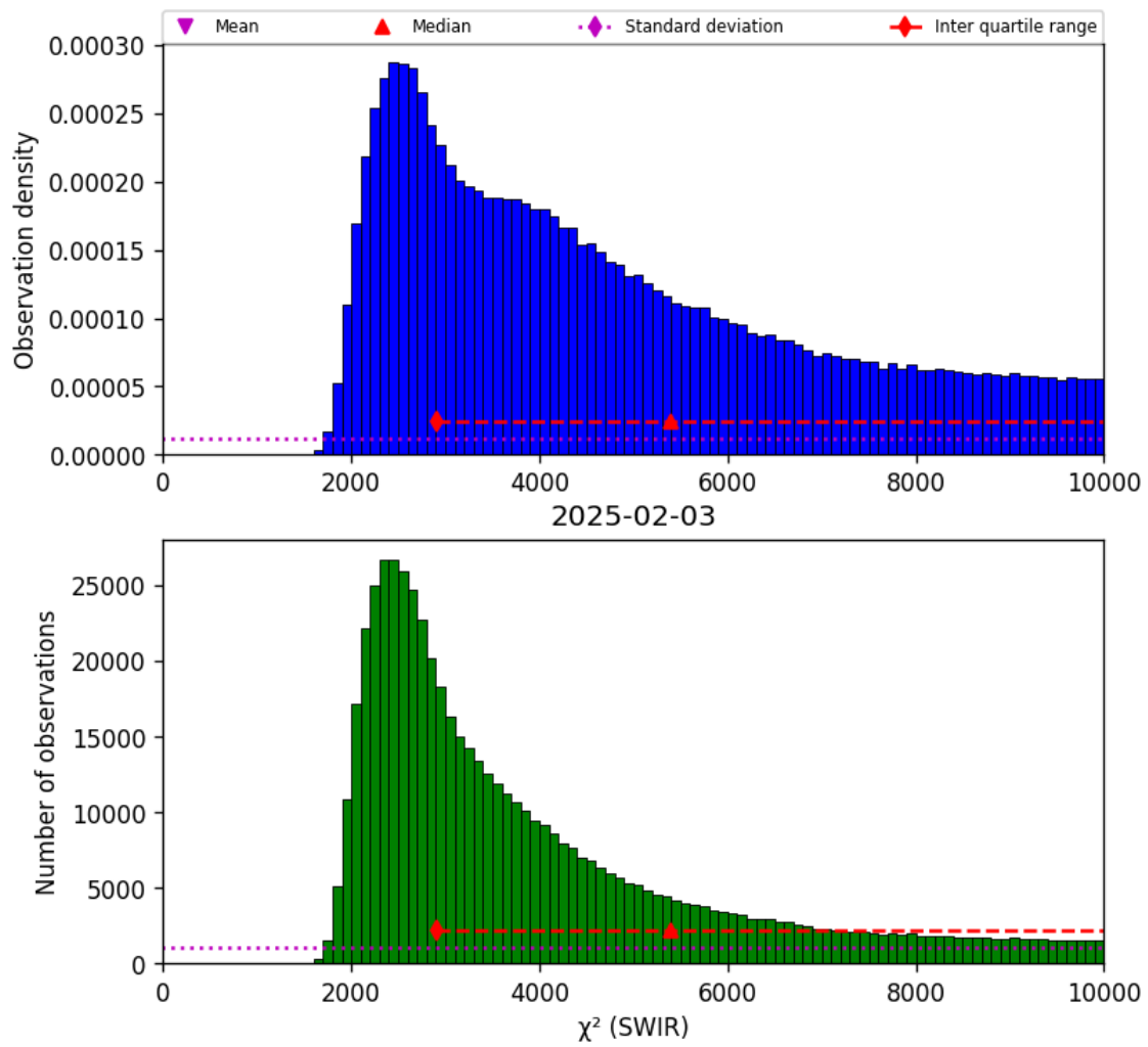
Figure 28: Histogram of “ \chi^2 (SWIR)” for 2025-02-03 to 2025-02-04
