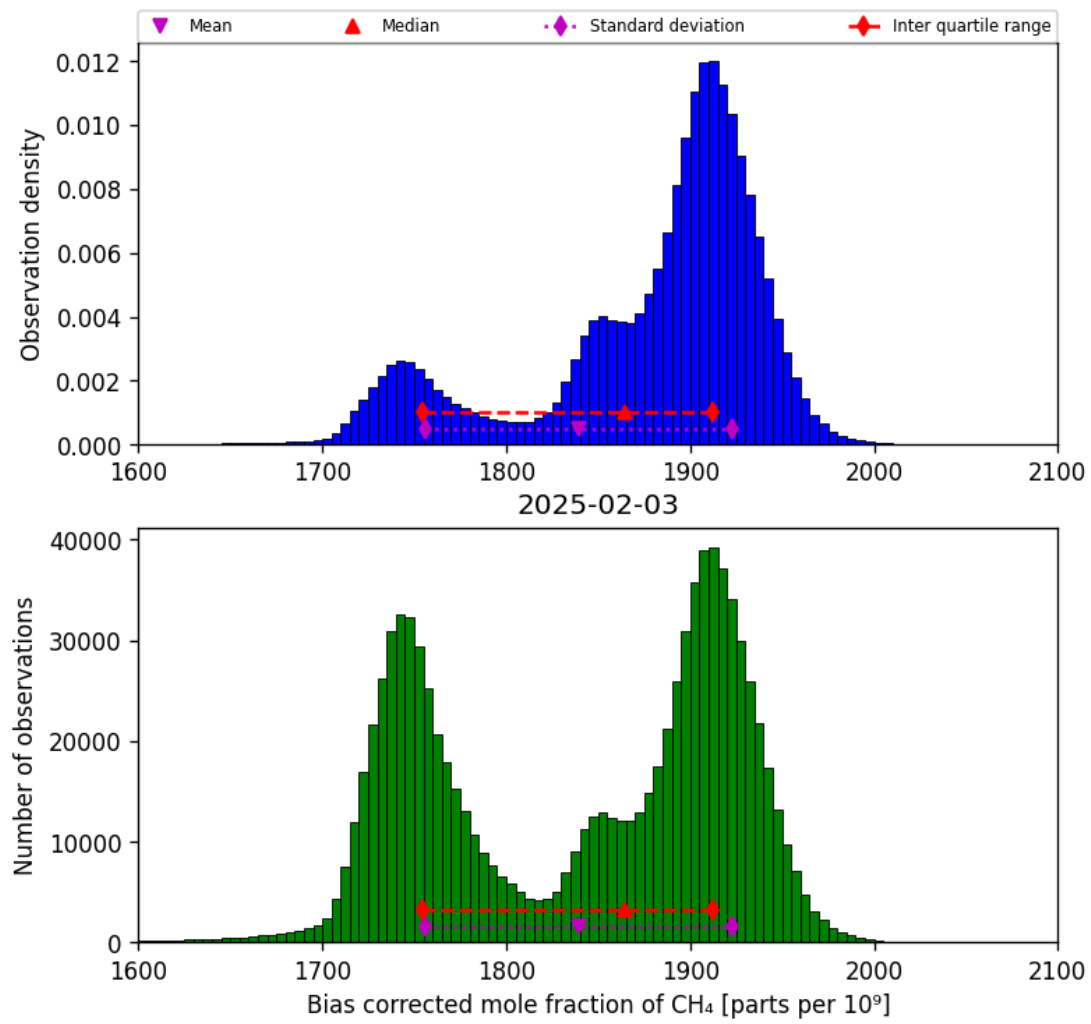
Figure 25: Histogram of “Bias corrected mole fraction of CH 4 ” for 2025-02-03 to 2025-02-04
