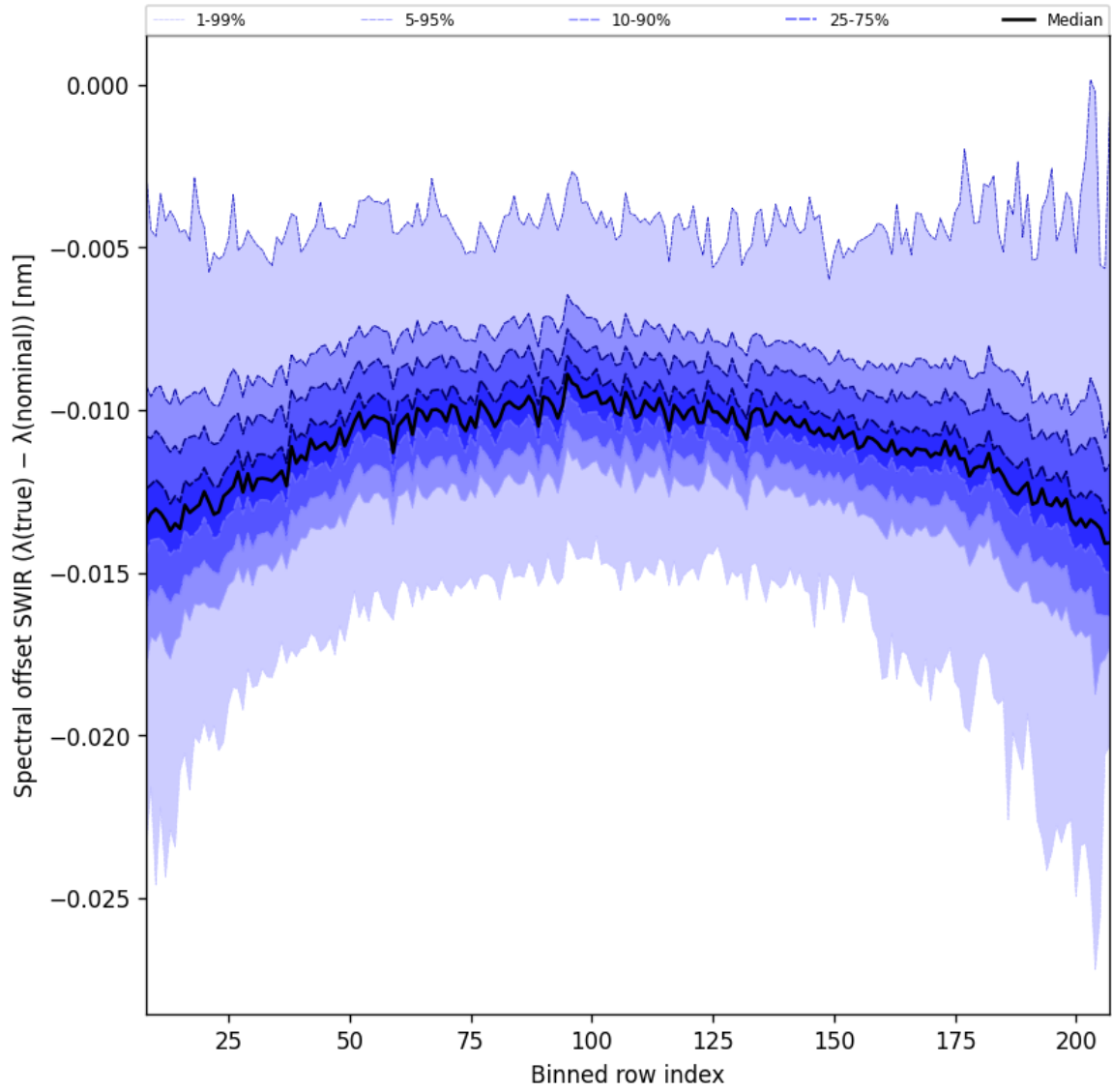
Figure 38: Along track statistics of “Spectral offset SWIR ( \lambda_{\text{true}} - \lambda_{\text{nominal}} )” for 2025-02-03 to 2025-02-04
