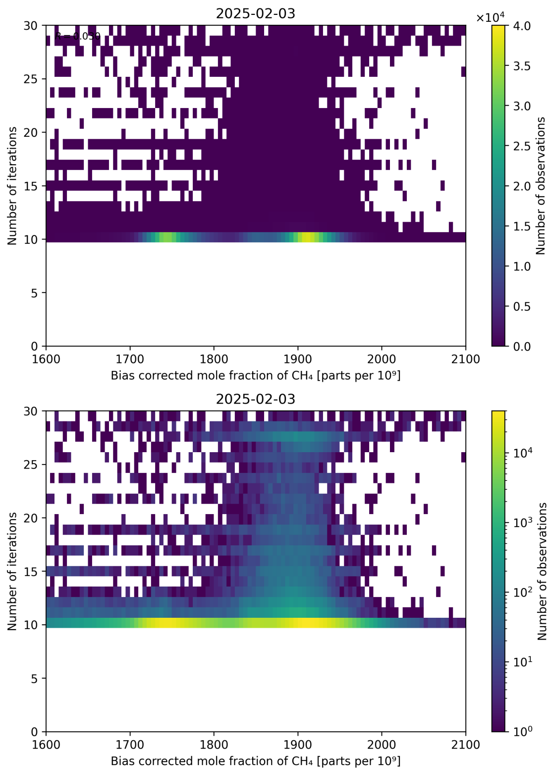
Figure 67: Scatter density plot of “Bias corrected mole fraction of CH 4 ” against “Number of iterations” for 2025-02-03 to 2025-02-04.
