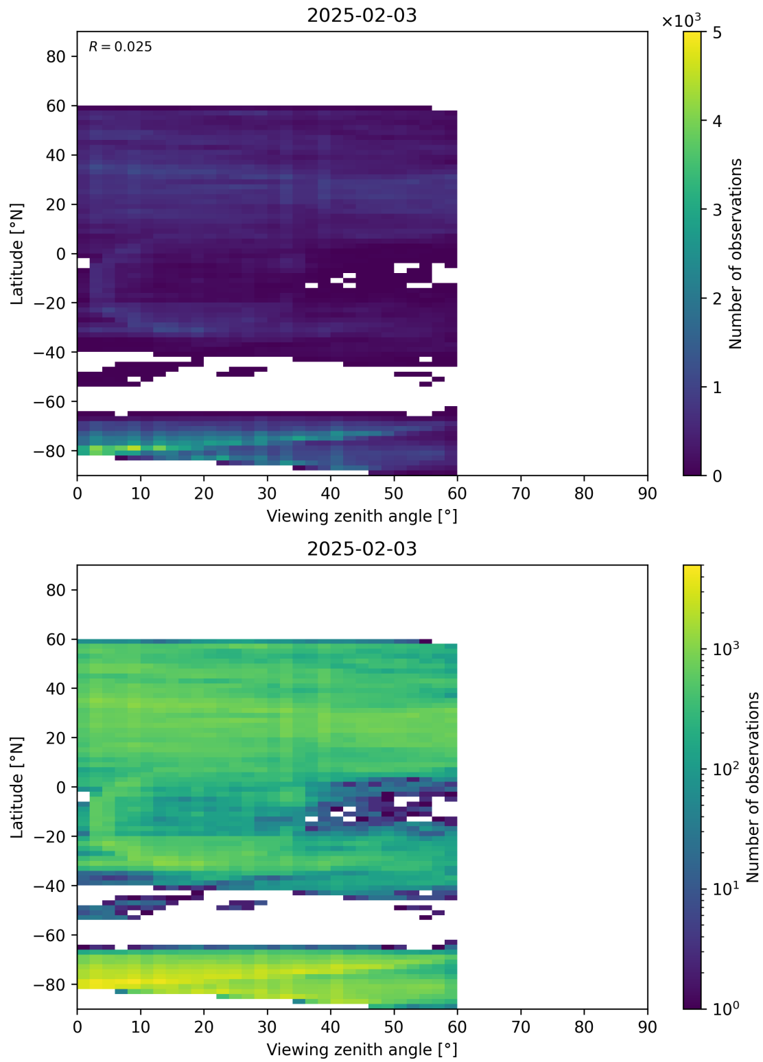
Figure 109: Scatter density plot of “Viewing zenith angle” against “Latitude” for 2025-02-03 to 2025-02-04.
