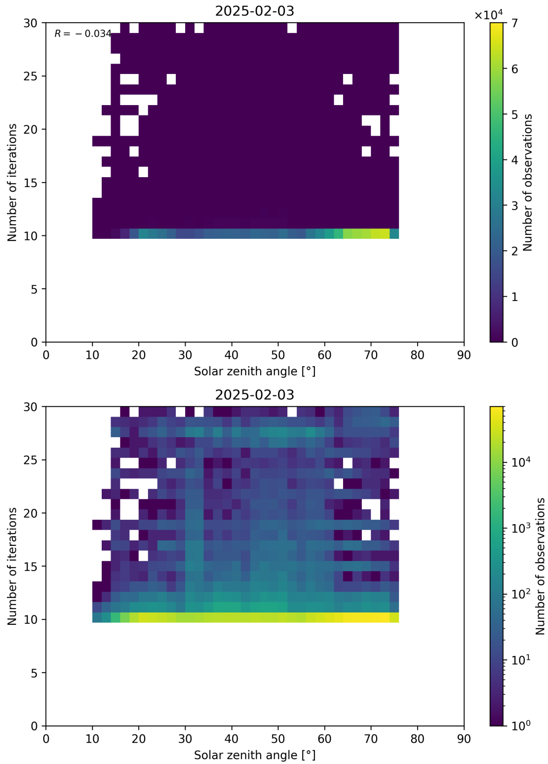
Figure 102: Scatter density plot of “Solar zenith angle” against “Number of iterations” for 2025-02-03 to 2025-02-04.
