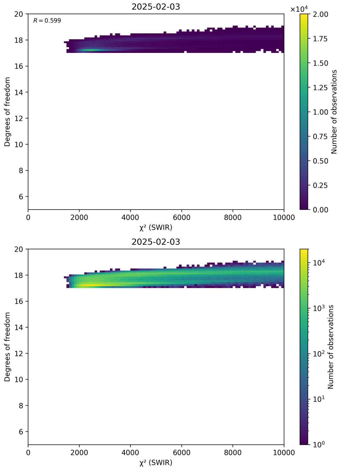
Figure 48: Scatter density plot of “ \chi^2 (SWIR)” against “Degrees of freedom” for 2025-02-03 to 2025-02-04.
