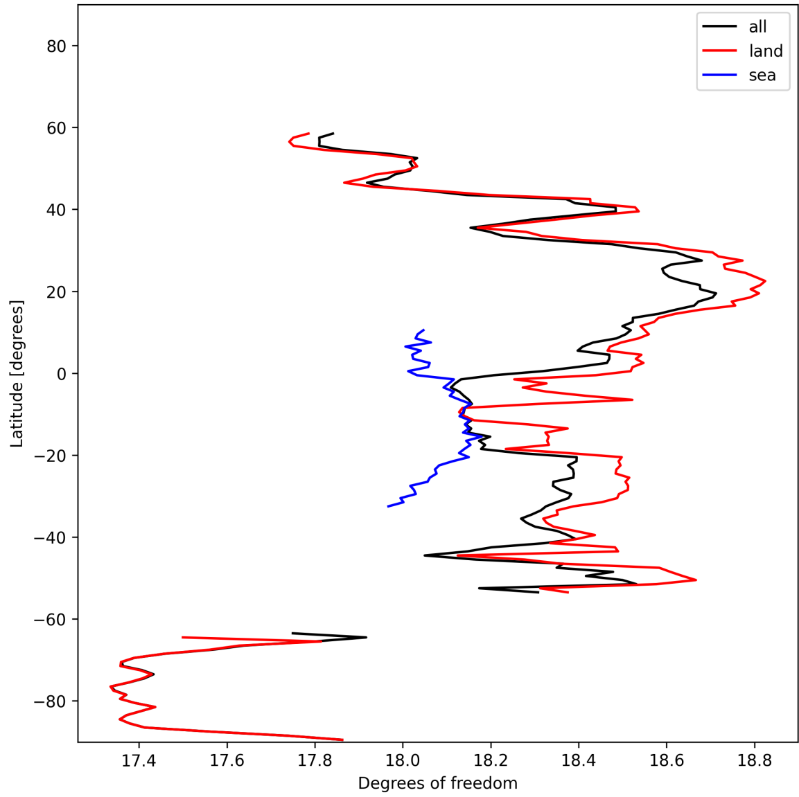
Figure 19: Zonal average of “Degrees of freedom” for 2025-02-03 to 2025-02-04.
