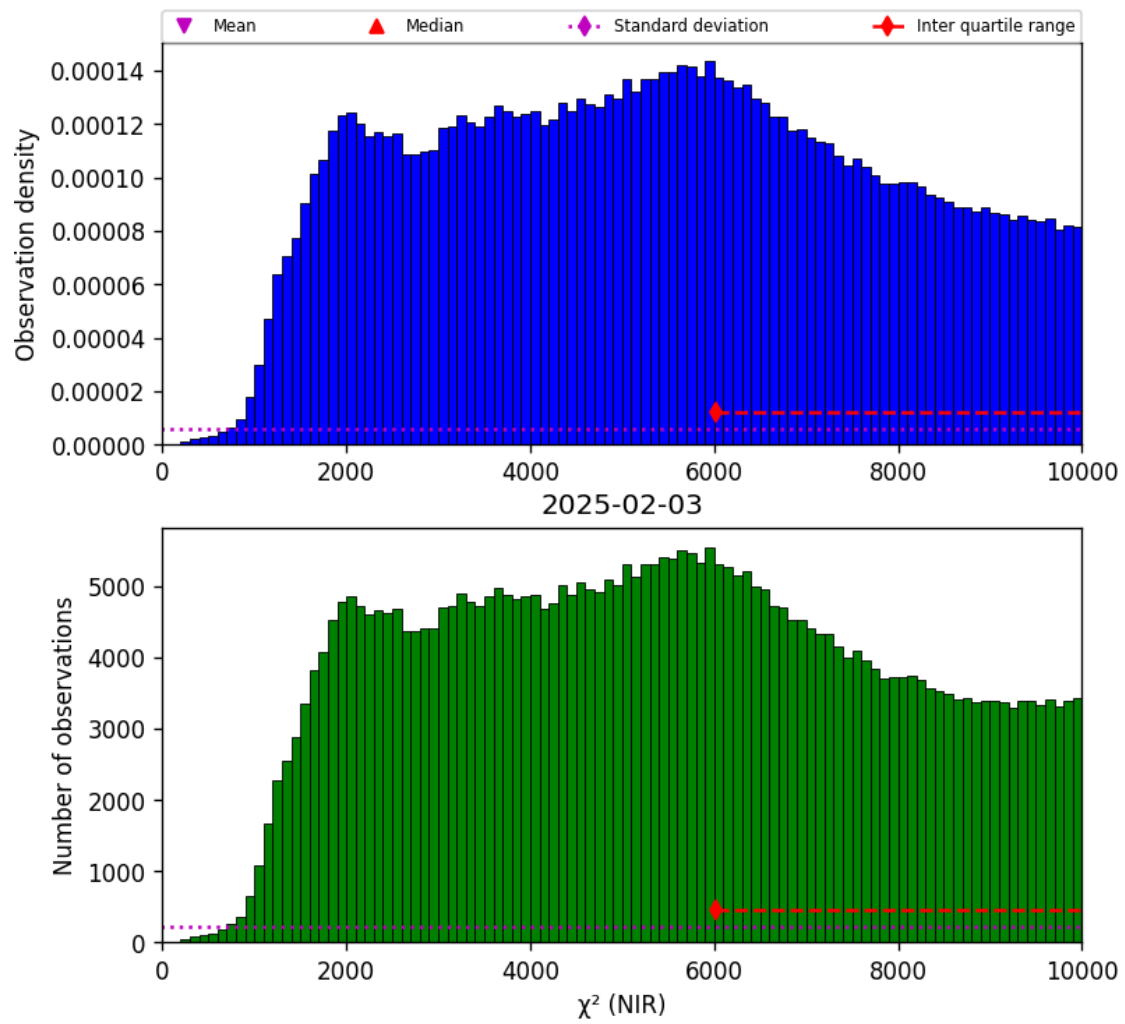
Figure 29: Histogram of " \chi^2 (NIR)" for 2025-02-03 to 2025-02-04
