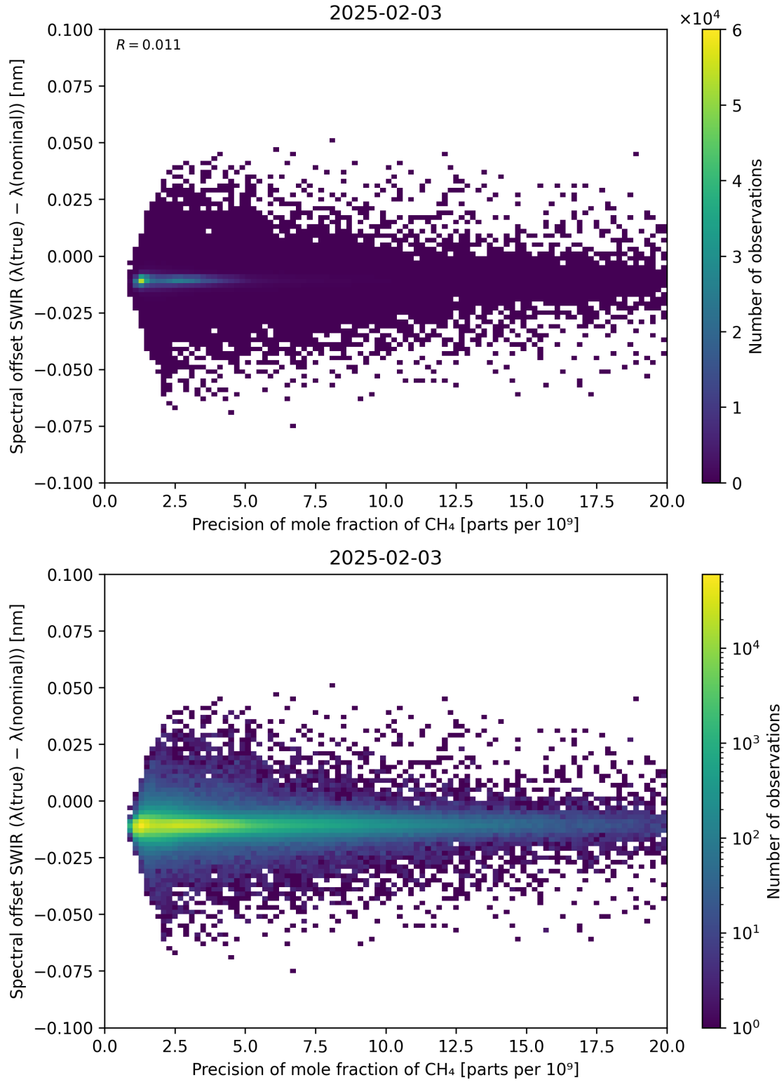
Figure 85: Scatter density plot of “Precision of mole fraction of \text{CH}_4 ” against “Spectral offset SWIR ( \lambda_{\text{true}} - \lambda_{\text{nominal}} )” for 2025-02-03 to 2025-02-04.
