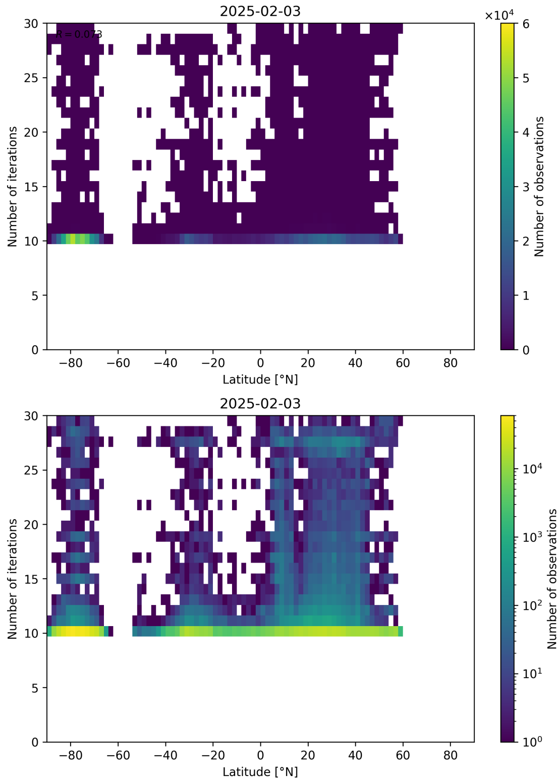
Figure 60: Scatter density plot of “Latitude” against “Number of iterations” for 2025-02-03 to 2025-02-04.
