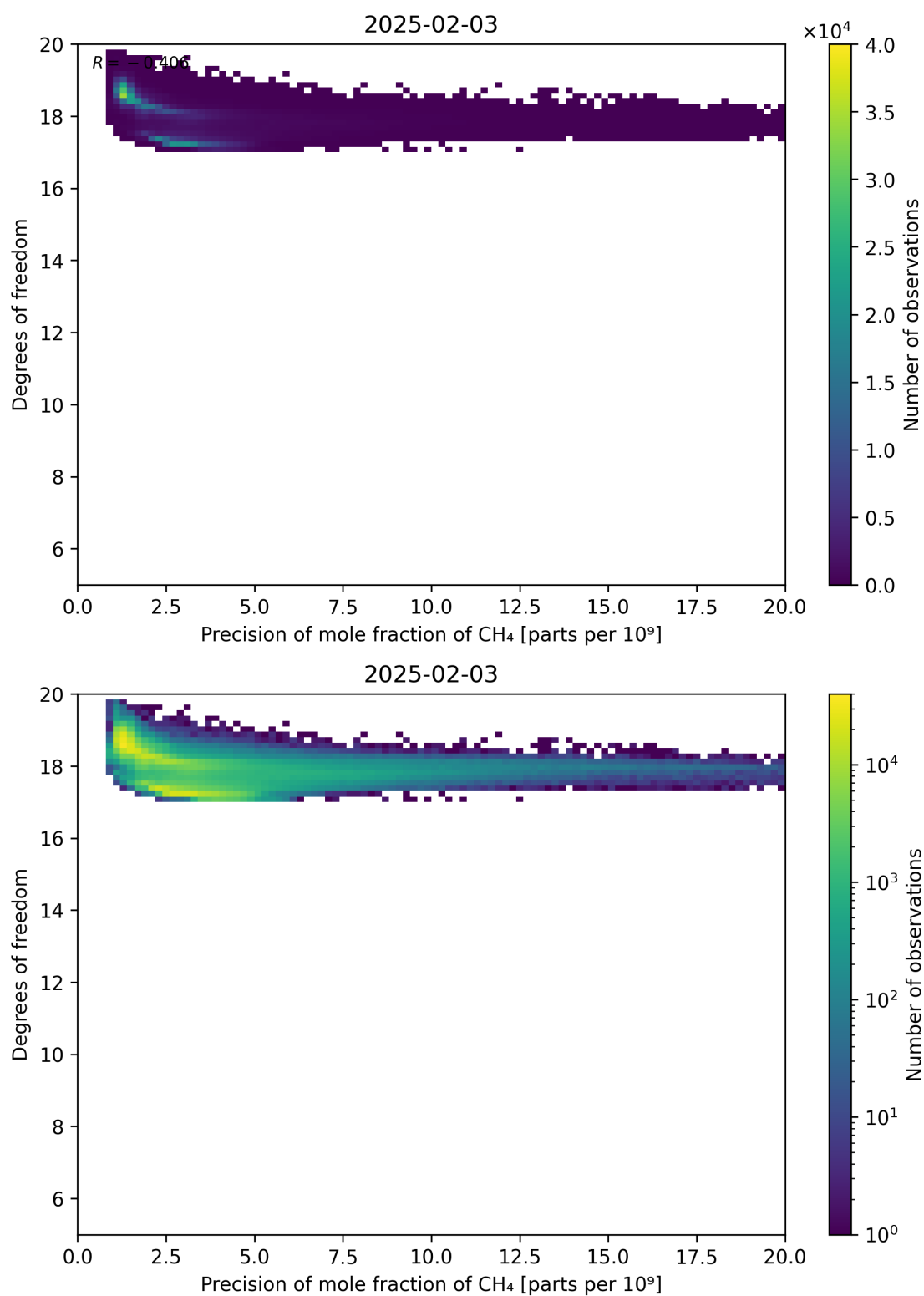
Figure 80: Scatter density plot of “Precision of mole fraction of CH 4 ” against “Degrees of freedom” for 2025-02-03 to 2025-02-04.
