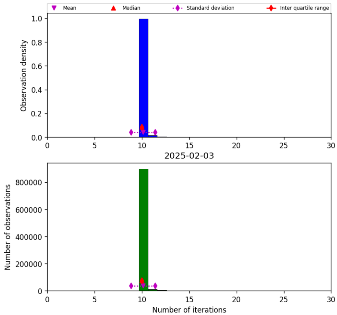
Figure 31: Histogram of “Number of iterations” for 2025-02-03 to 2025-02-04
