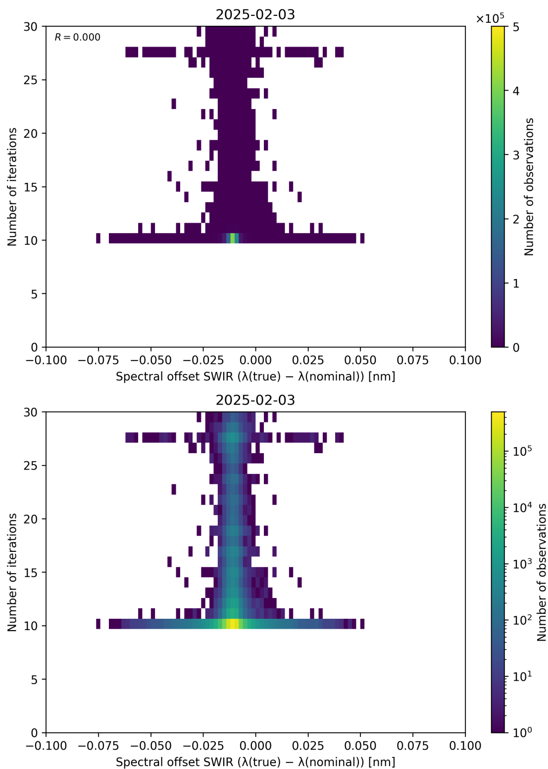
Figure 121: Scatter density plot of “Spectral offset SWIR ( \lambda_{\text{true}} - \lambda_{\text{nominal}} )” against “Number of iterations” for 2025-02-03 to 2025-02-04.
