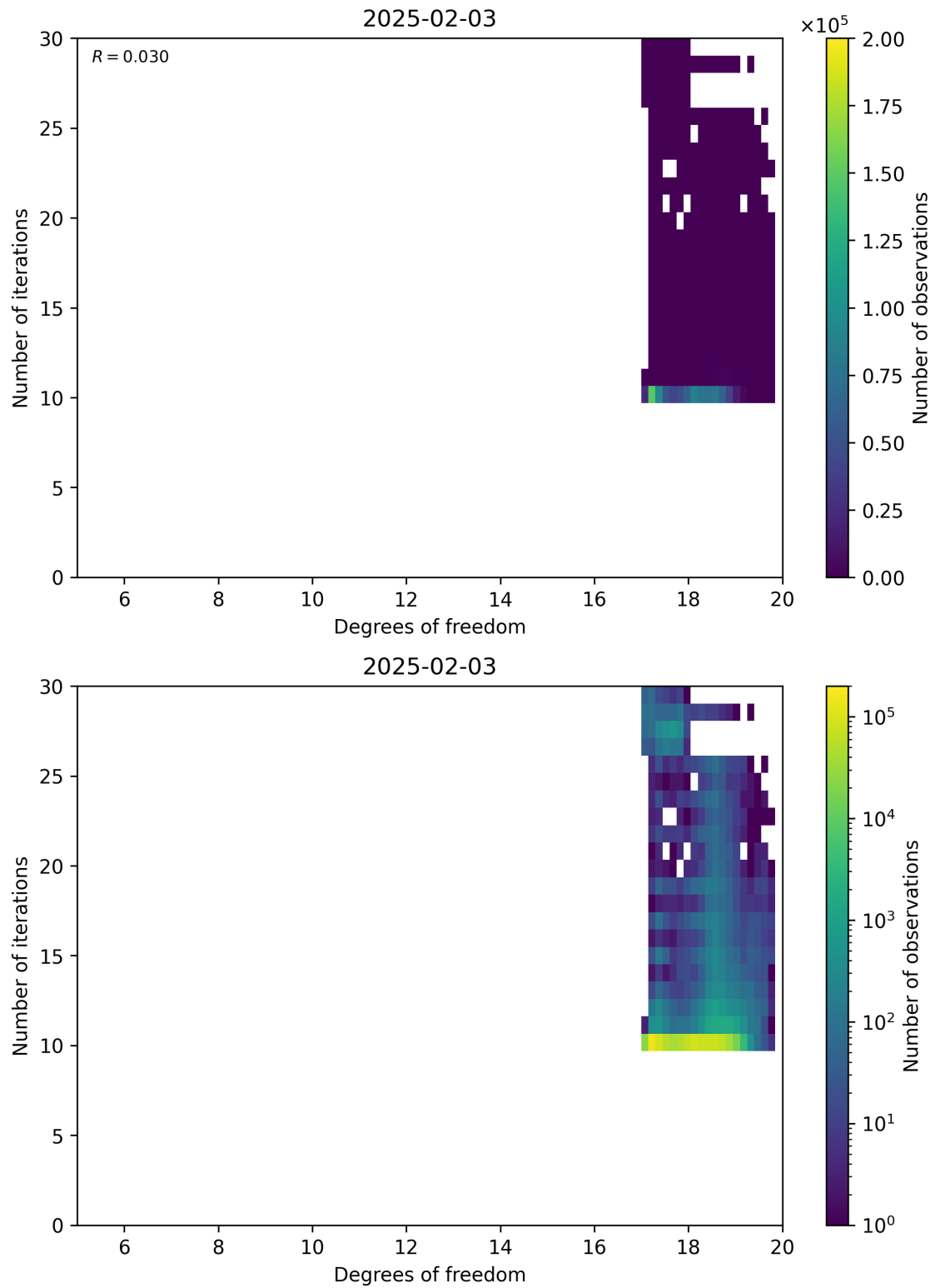
Figure 52: Scatter density plot of “Degrees of freedom” against “Number of iterations” for 2025-02-03 to 2025-02-04.
