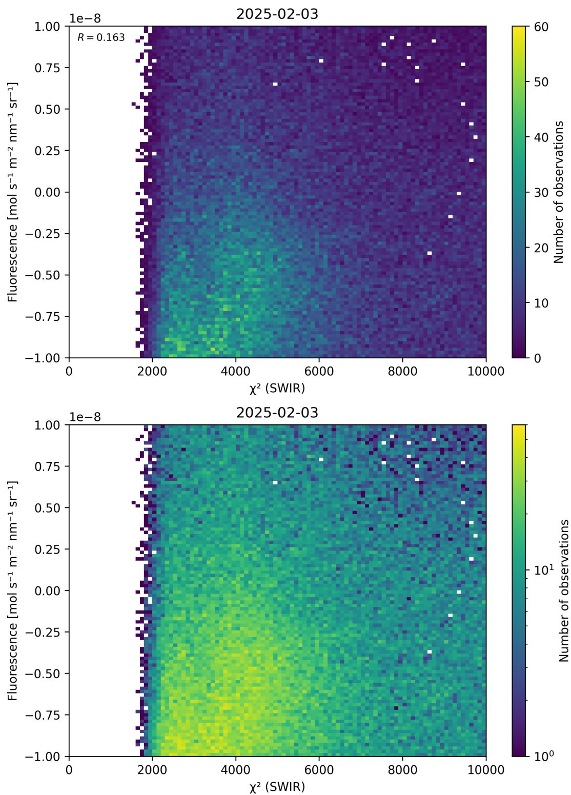
Figure 49: Scatter density plot of “ \chi^2 (SWIR)” against “Fluorescence” for 2025-02-03 to 2025-02-04.
