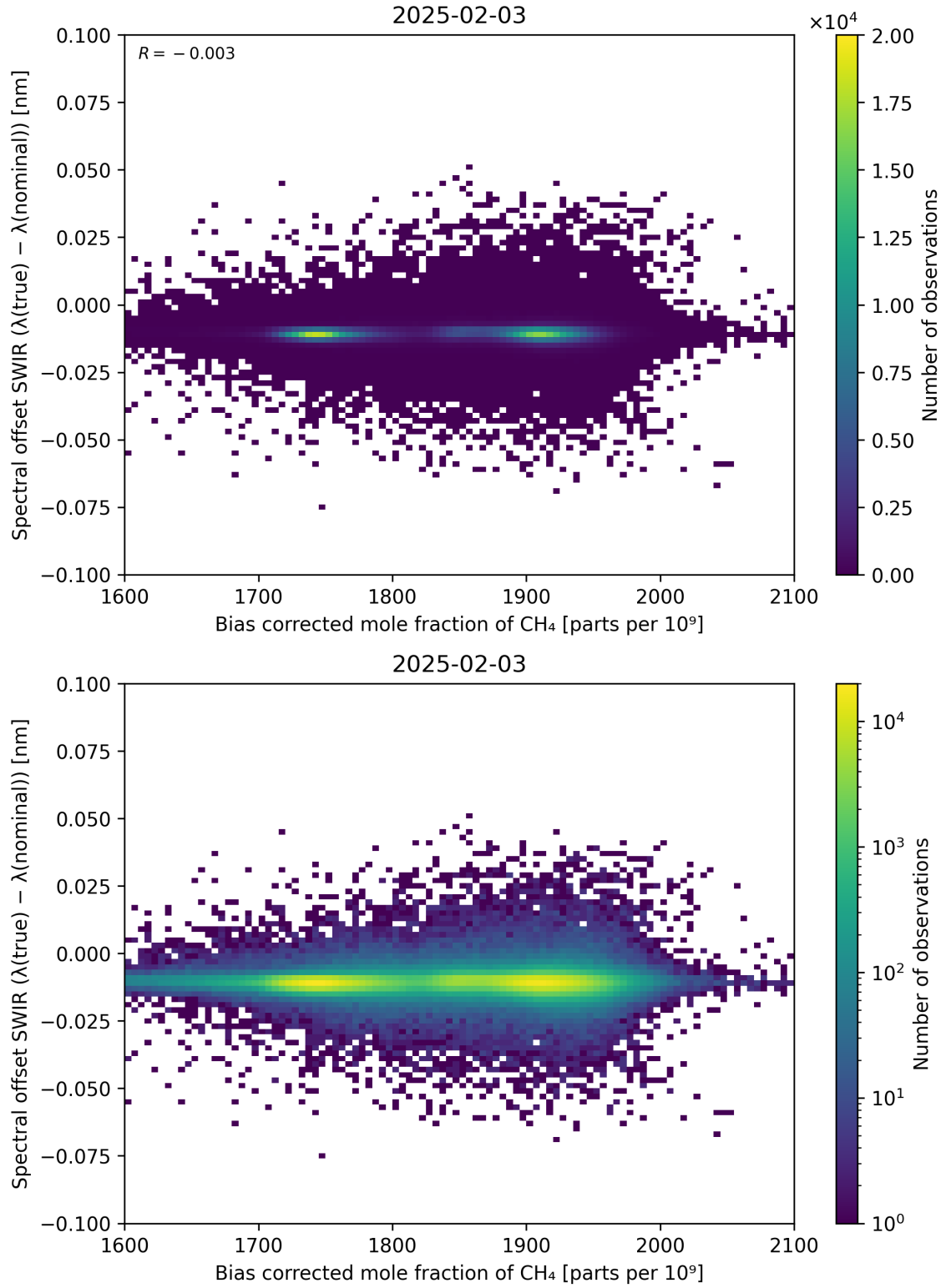
Figure 69: Scatter density plot of “Bias corrected mole fraction of CH 4 ” against “Spectral offset SWIR ( \lambda_{\text{true}} - \lambda_{\text{nominal}} )” for 2025-02-03 to 2025-02-04.
