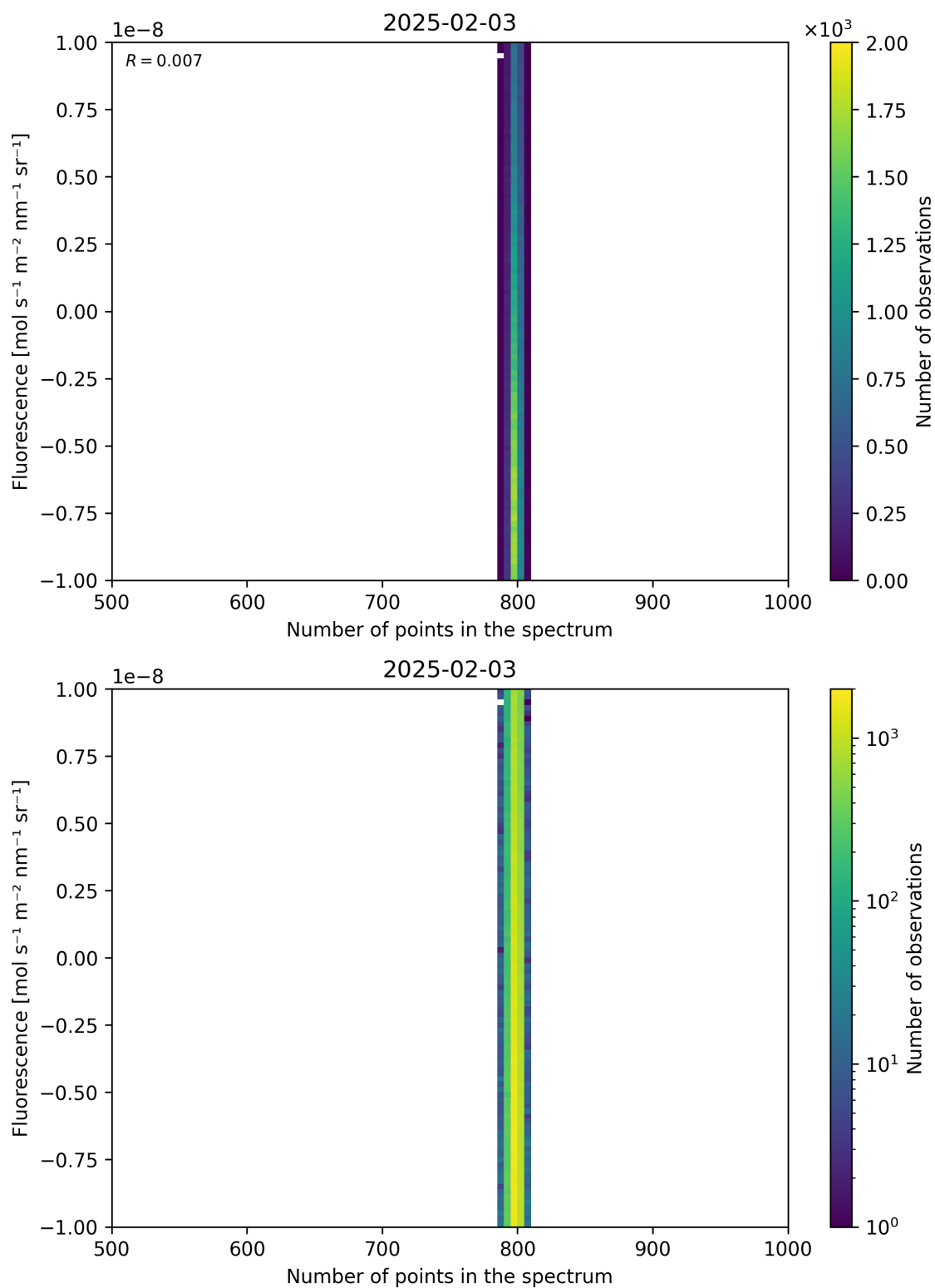
Figure 91: Scatter density plot of “Number of points in the spectrum” against “Fluorescence” for 2025-02-03 to 2025-02-04.
