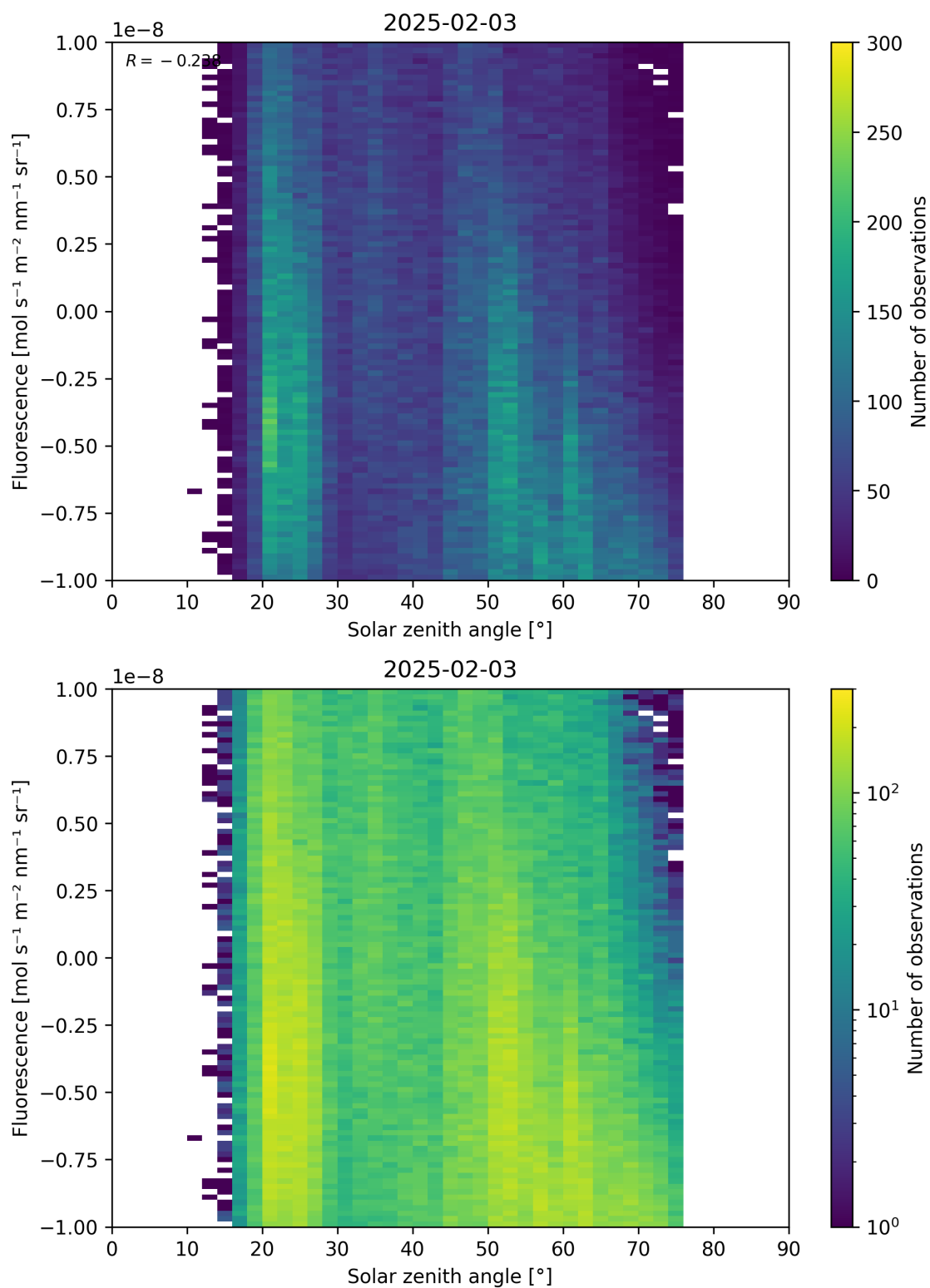
Figure 97: Scatter density plot of “Solar zenith angle” against “Fluorescence” for 2025-02-03 to 2025-02-04.
