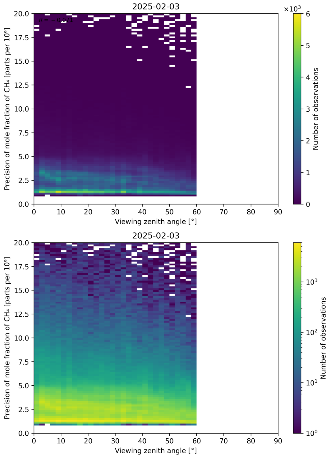
Figure 112: Scatter density plot of “Viewing zenith angle” against “Precision of mole fraction of CH 4 ” for 2025-02-03 to 2025-02-04.
