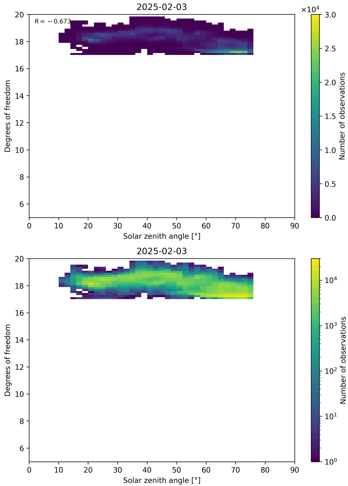
Figure 96: Scatter density plot of “Solar zenith angle” against “Degrees of freedom” for 2025-02-03 to 2025-02-04.
