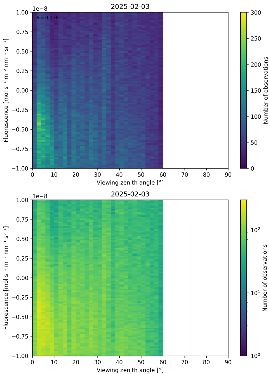
Figure 108: Scatter density plot of “Viewing zenith angle” against “Fluorescence” for 2025-02-03 to 2025-02-04.
