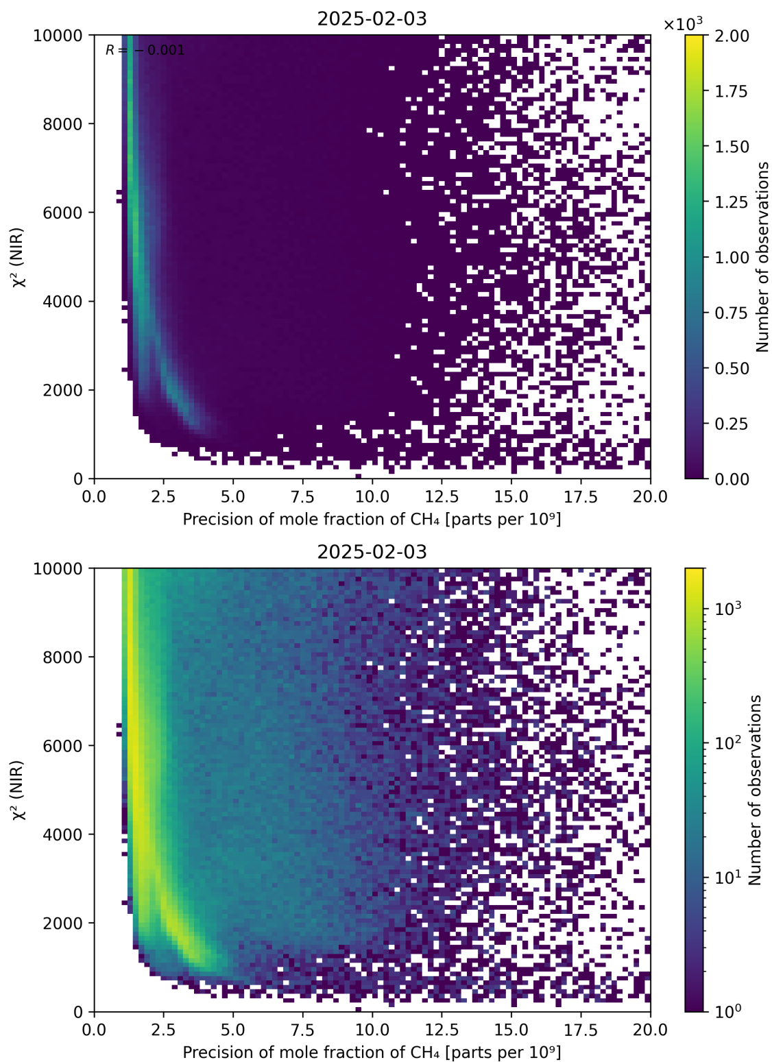
Figure 78: Scatter density plot of “Precision of mole fraction of CH 4 ” against “ \chi^2 (NIR)” for 2025-02-03 to 2025-02-04.
