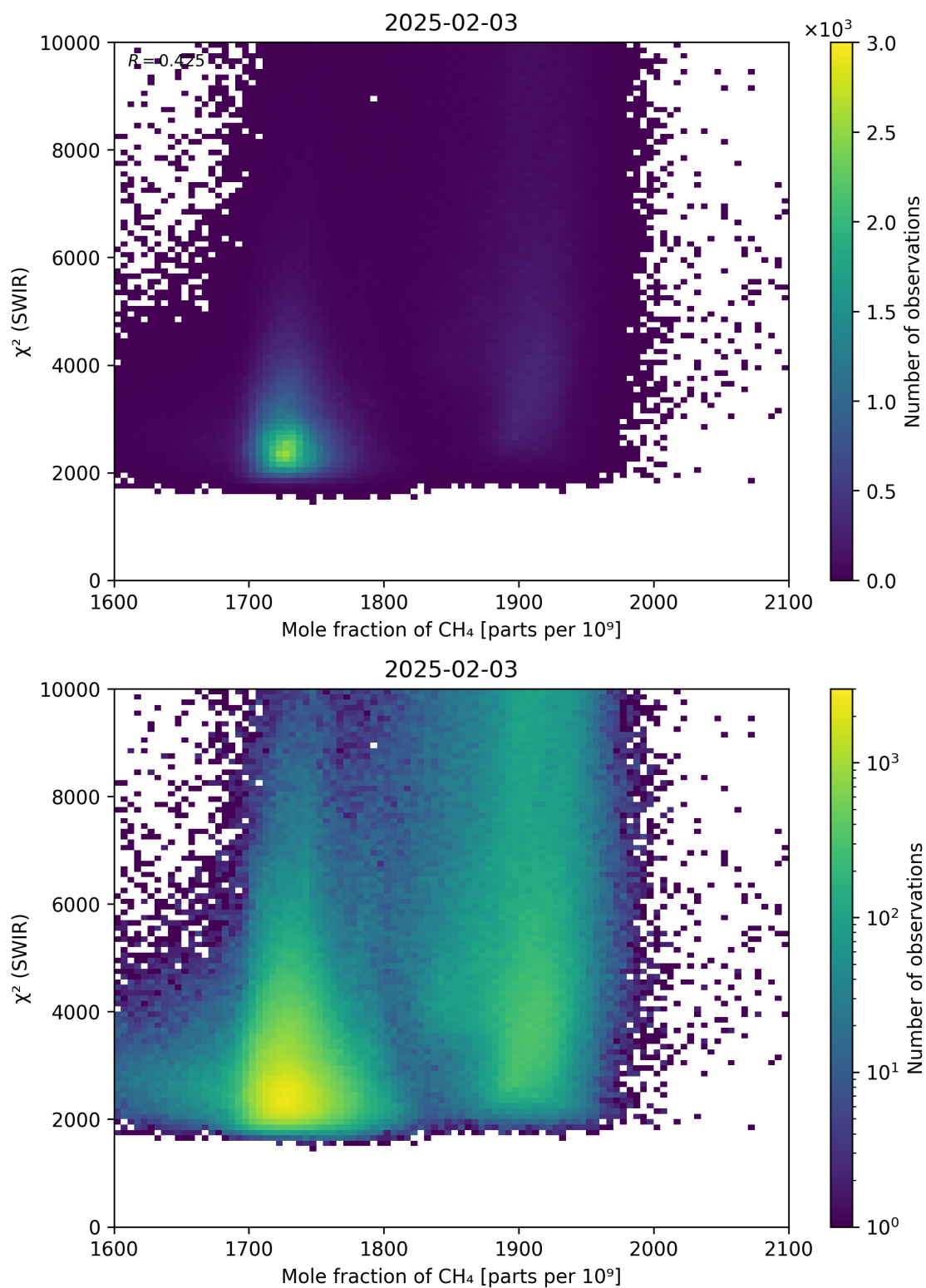
Figure 71: Scatter density plot of “Mole fraction of \text{CH}_4 ” against “ \chi^2 (SWIR)” for 2025-02-03 to 2025-02-04.
