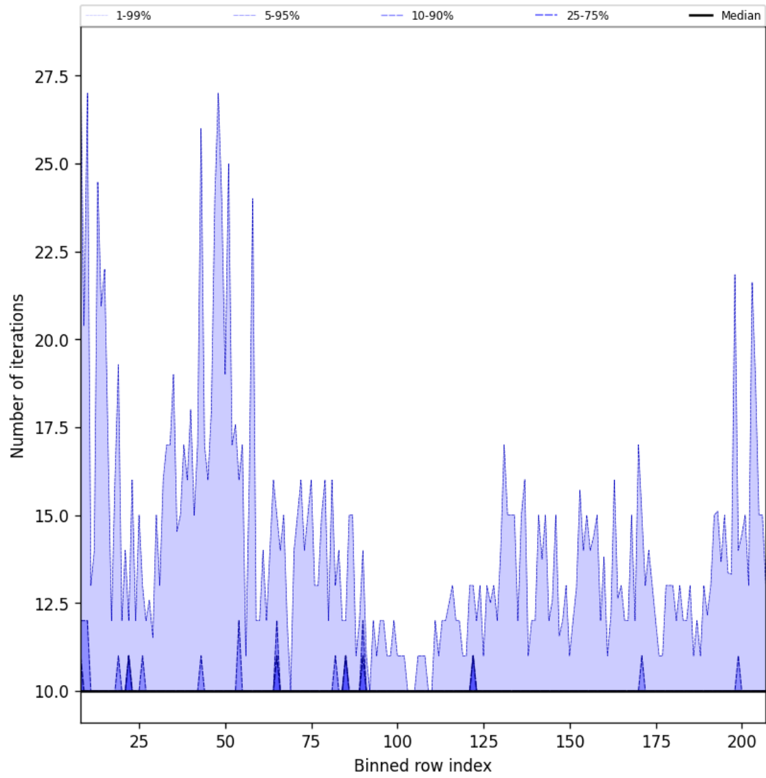
Figure 42: Along track statistics of “Number of iterations” for 2025-02-03 to 2025-02-04
