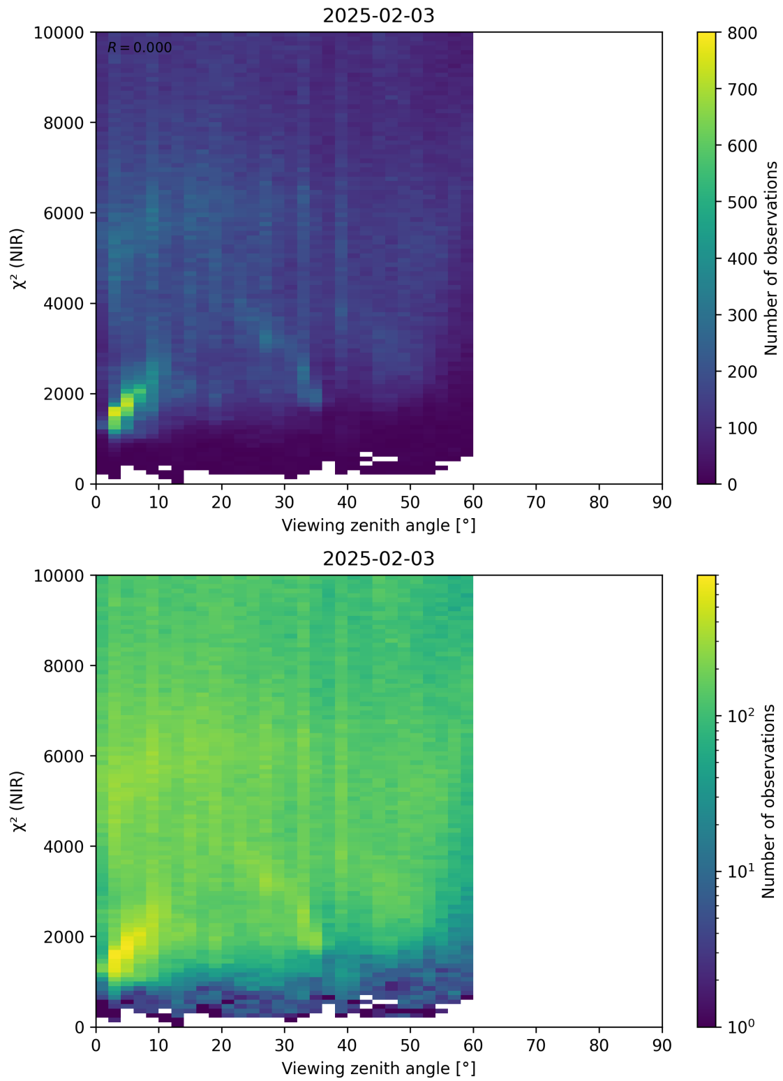
Figure 105: Scatter density plot of “Viewing zenith angle” against “ \chi^2 (NIR)” for 2025-02-03 to 2025-02-04.
