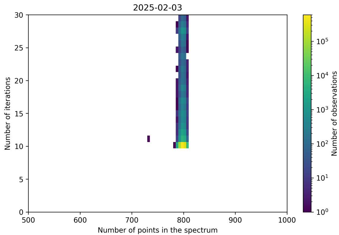
Figure 92: Scatter density plot of “Number of points in the spectrum” against “Number of iterations” for 2025-02-03 to 2025-02-04.
