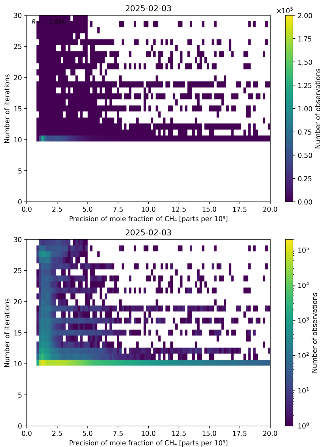
Figure 83: Scatter density plot of “Precision of mole fraction of CH 4 ” against “Number of iterations” for 2025-02-03 to 2025-02-04.
