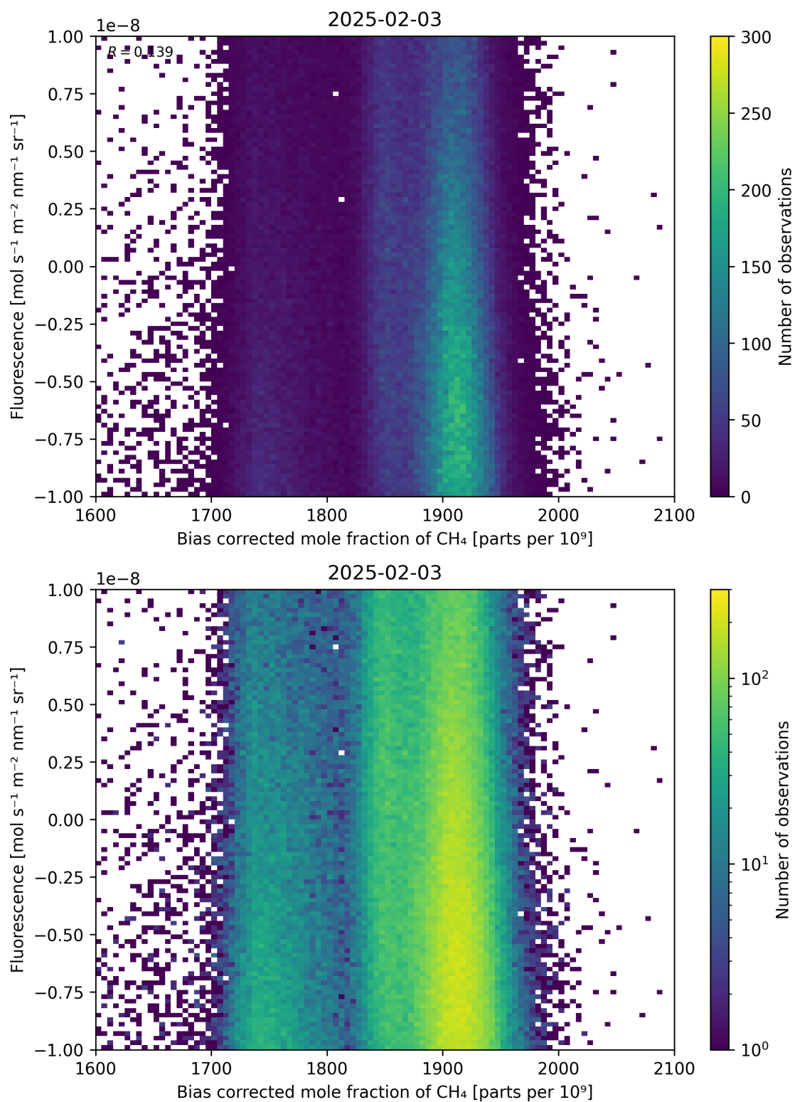
Figure 66: Scatter density plot of “Bias corrected mole fraction of CH 4 ” against “Fluorescence” for 2025-02-03 to 2025-02-04.
