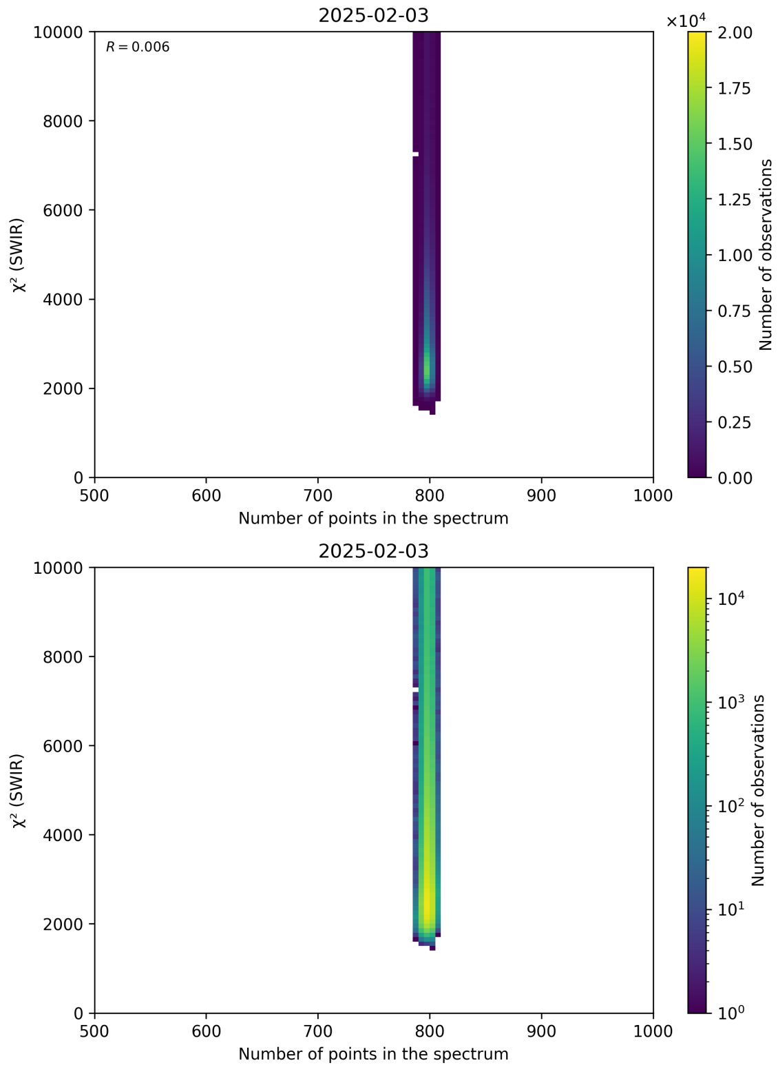
Figure 89: Scatter density plot of “Number of points in the spectrum” against “ \chi^2 (SWIR)” for 2025-02-03 to 2025-02-04.
