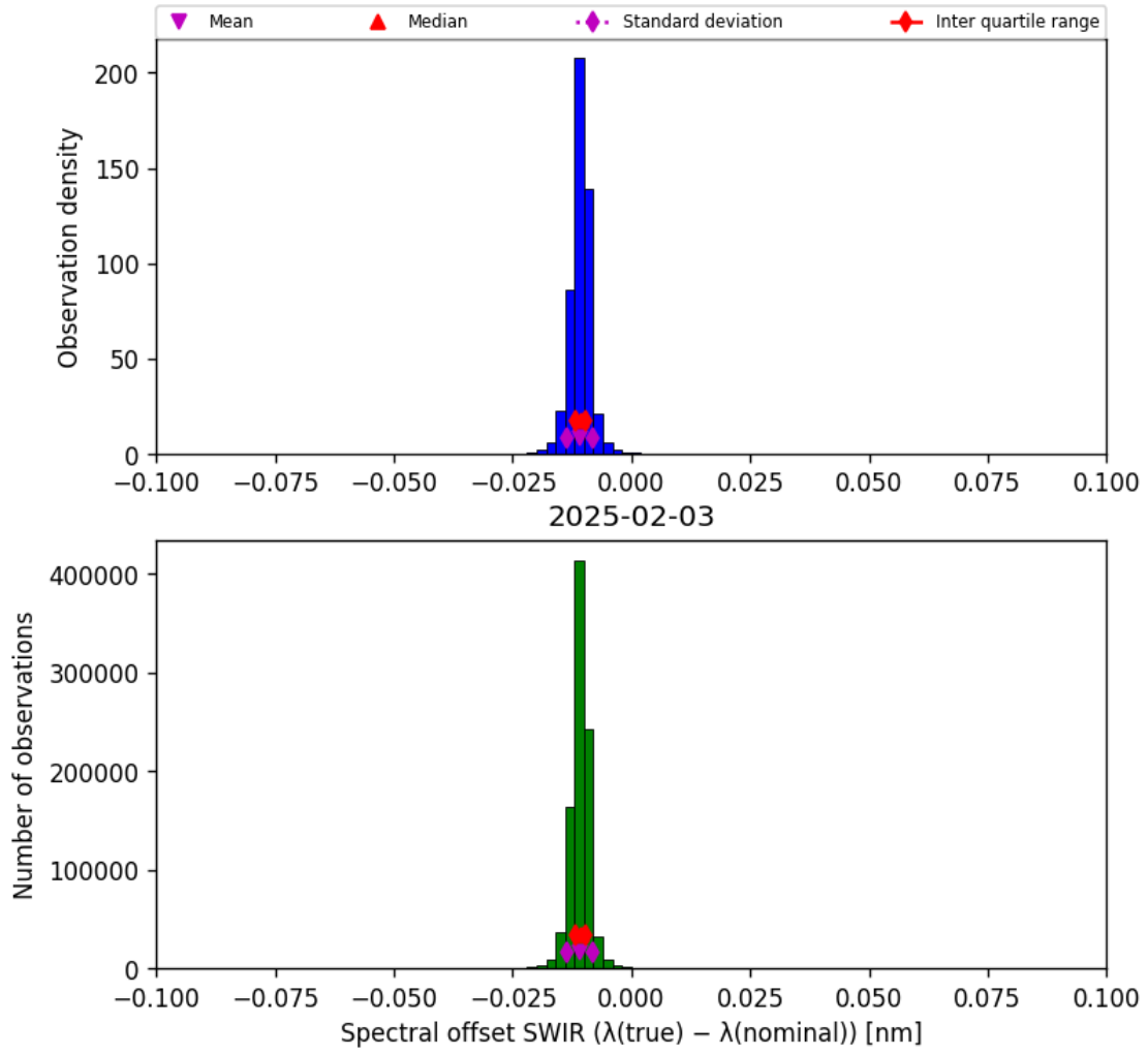
Figure 27: Histogram of “Spectral offset SWIR ( \lambda_{\text{true}} - \lambda_{\text{nominal}} )” for 2025-02-03 to 2025-02-04
