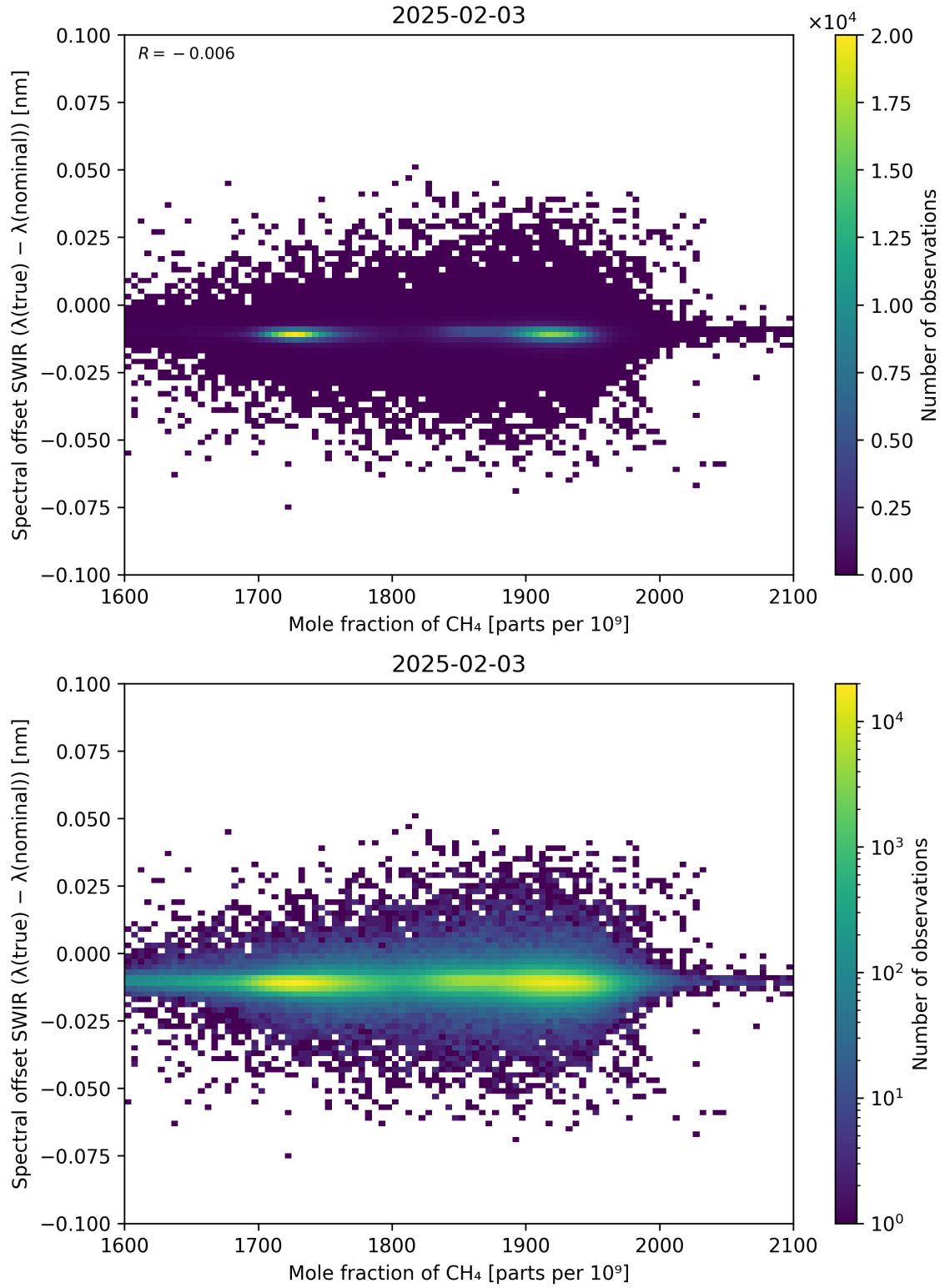
Figure 86: Scatter density plot of “Mole fraction of \text{CH}_4 ” against “Spectral offset SWIR ( \lambda_{\text{true}} - \lambda_{\text{nominal}} )” for 2025-02-03 to 2025-02-04.
