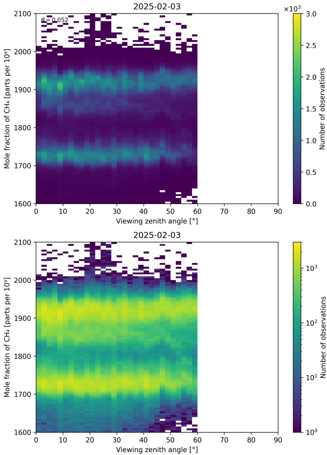
Figure 110: Scatter density plot of “Viewing zenith angle” against “Mole fraction of CH 4 ” for 2025-02-03 to 2025-02-04.
