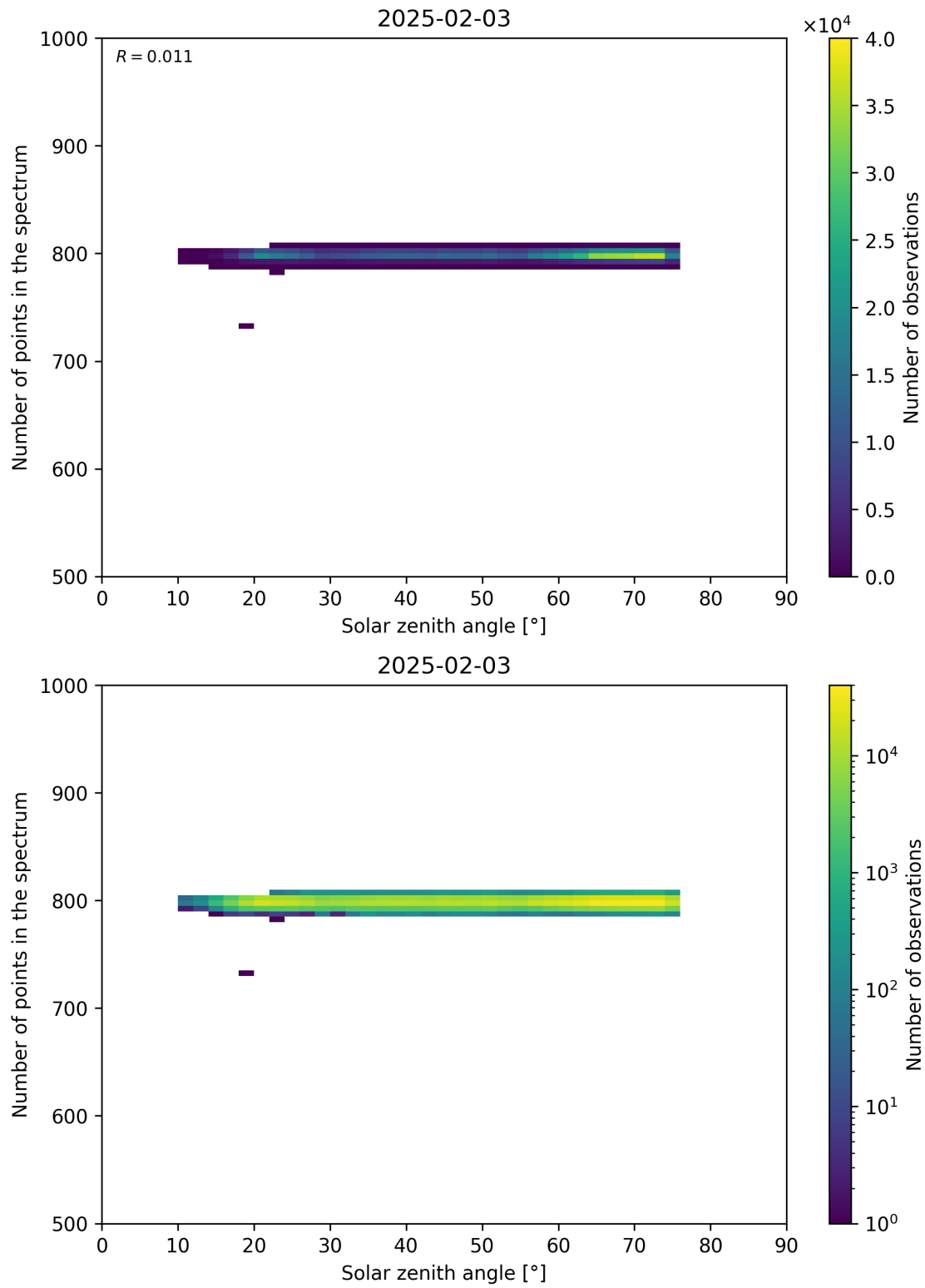
Figure 103: Scatter density plot of “Solar zenith angle” against “Number of points in the spectrum” for 2025-02-03 to 2025-02-04.
