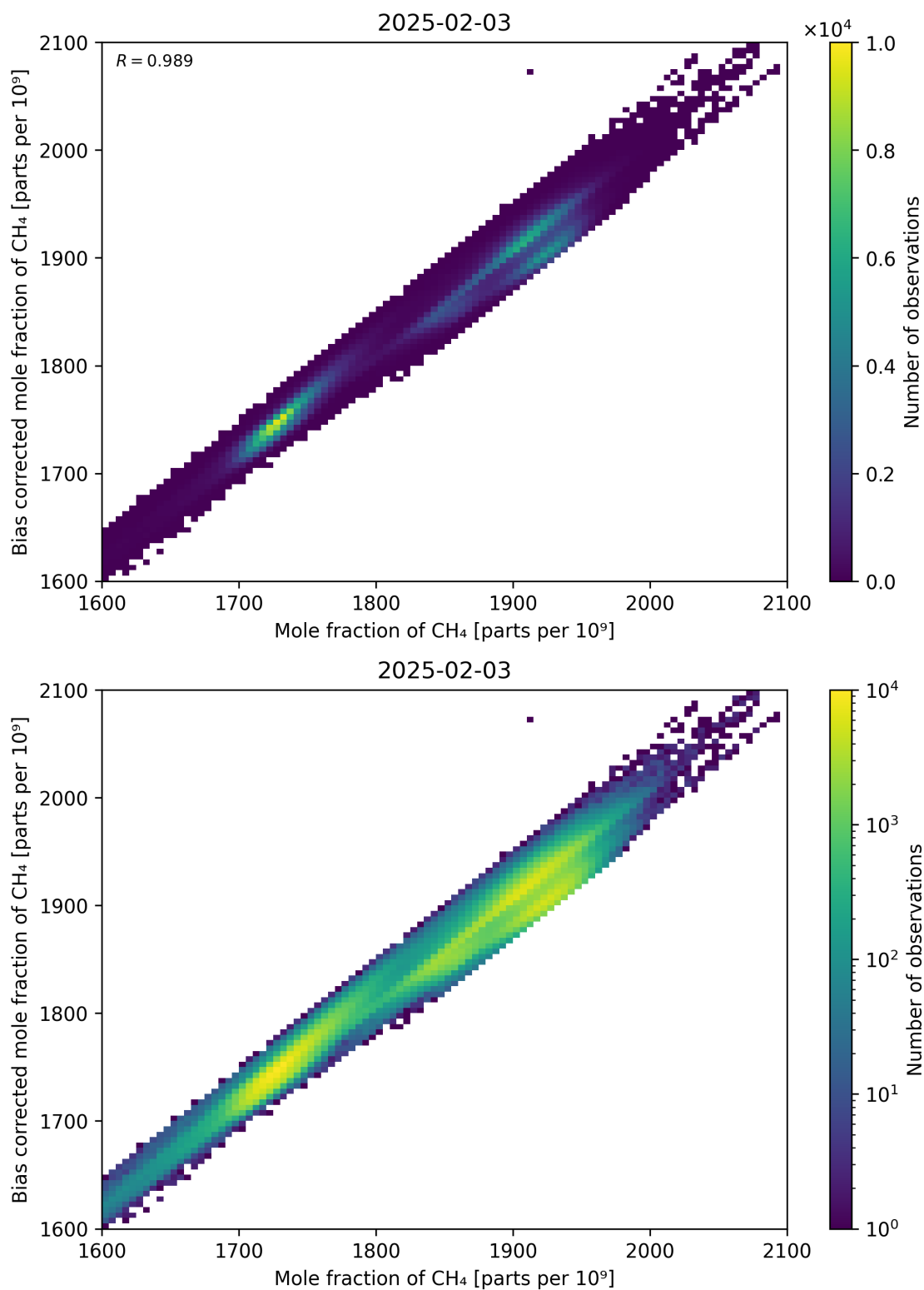
Figure 74: Scatter density plot of “Mole fraction of CH 4 ” against “Bias corrected mole fraction of CH 4 ” for 2025-02-03 to 2025-02-04.
