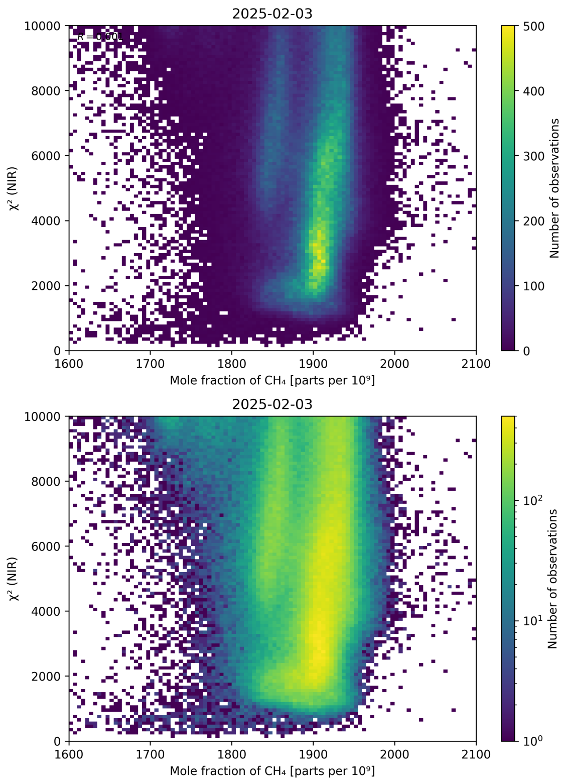
Figure 70: Scatter density plot of “Mole fraction of CH 4 ” against “ \chi^2 (NIR)” for 2025-02-03 to 2025-02-04.
