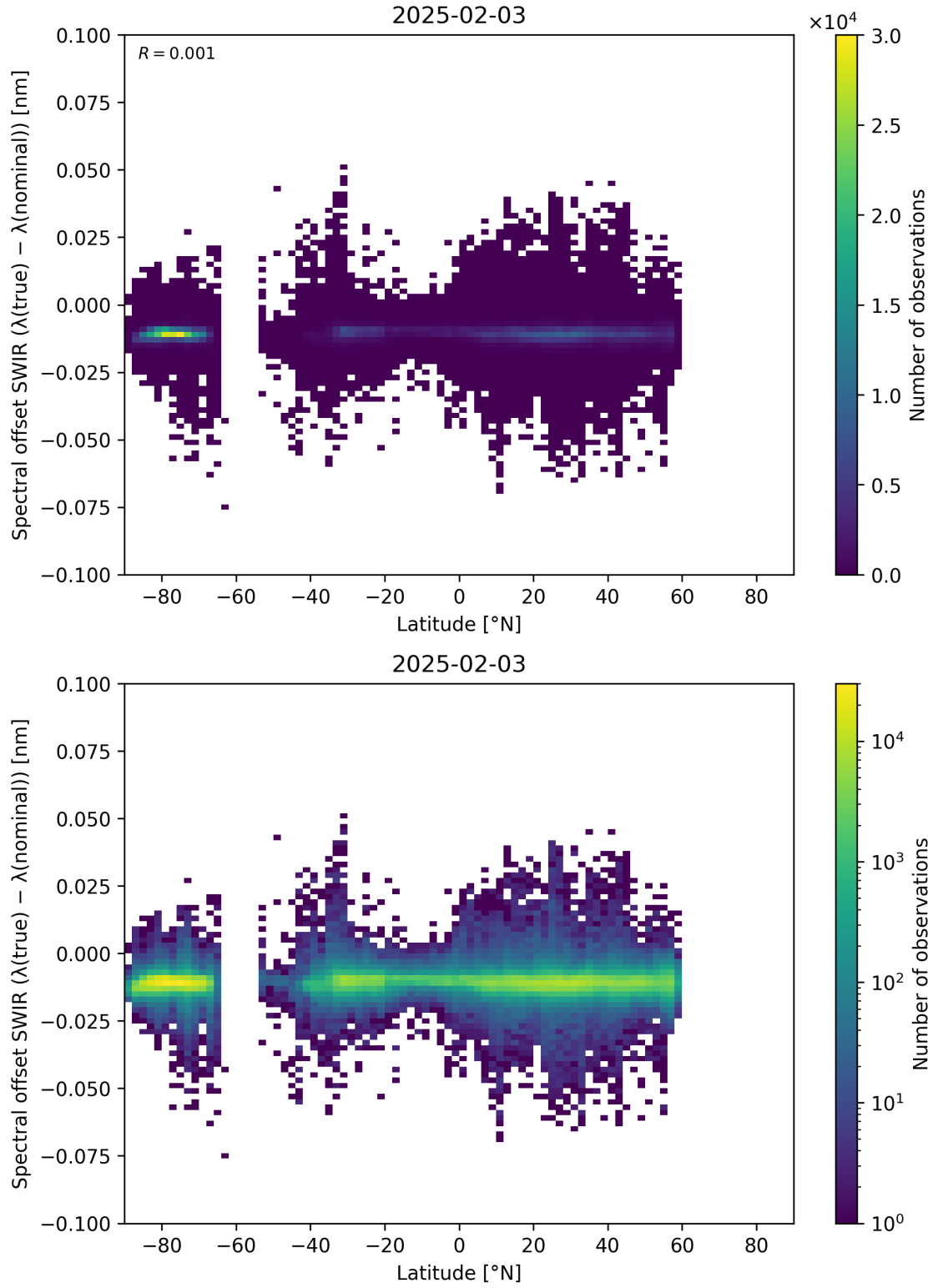
Figure 62: Scatter density plot of “Latitude” against “Spectral offset SWIR ( \lambda_{\text{true}} - \lambda_{\text{nominal}} )” for 2025-02-03 to 2025-02-04.
