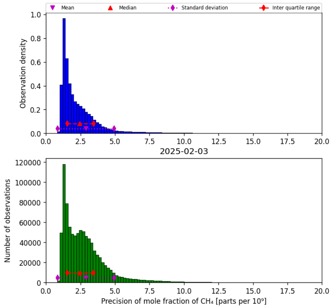
Figure 24: Histogram of “Precision of mole fraction of CH 4 ” for 2025-02-03 to 2025-02-04
