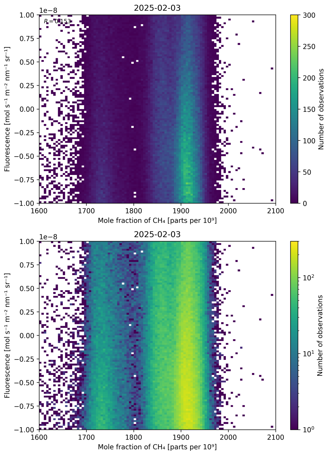
Figure 73: Scatter density plot of “Mole fraction of \text{CH}_4 ” against “Fluorescence” for 2025-02-03 to 2025-02-04.
