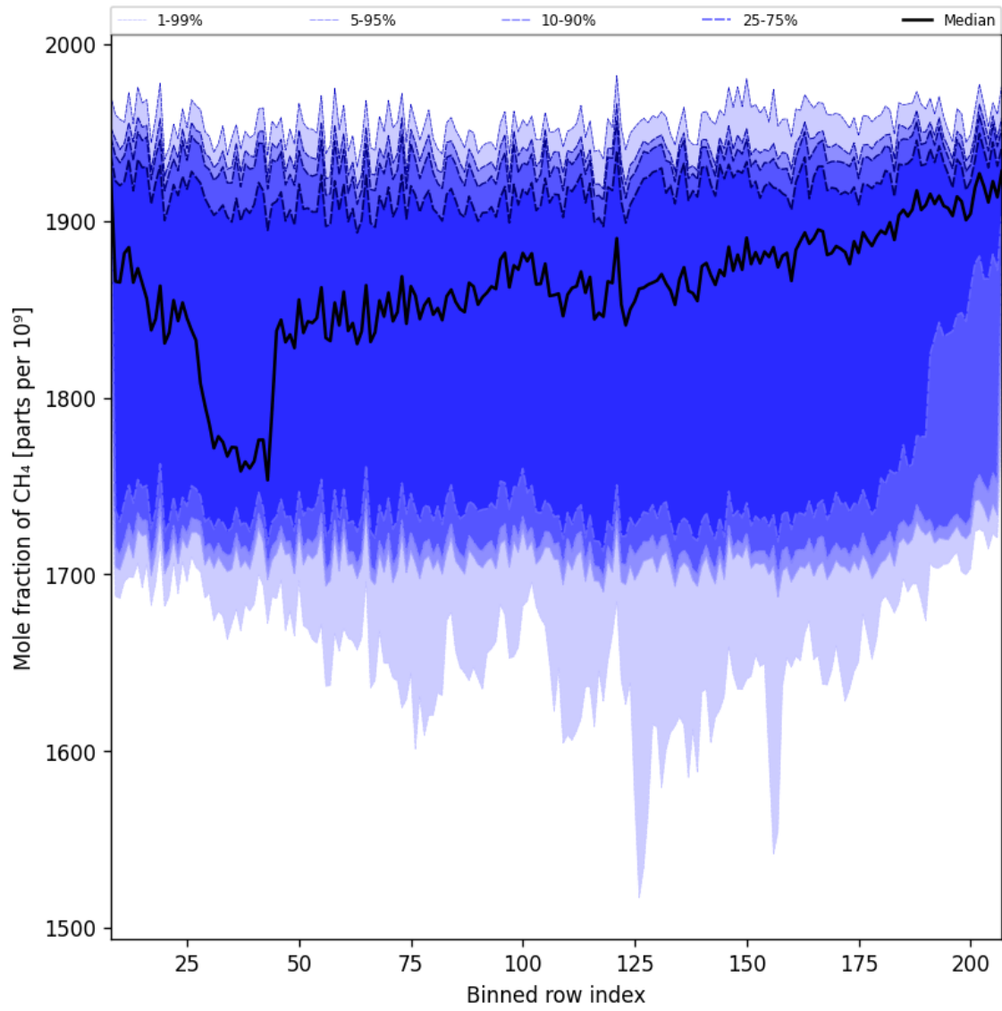
Figure 34: Along track statistics of “Mole fraction of CH 4 ” for 2025-02-03 to 2025-02-04
