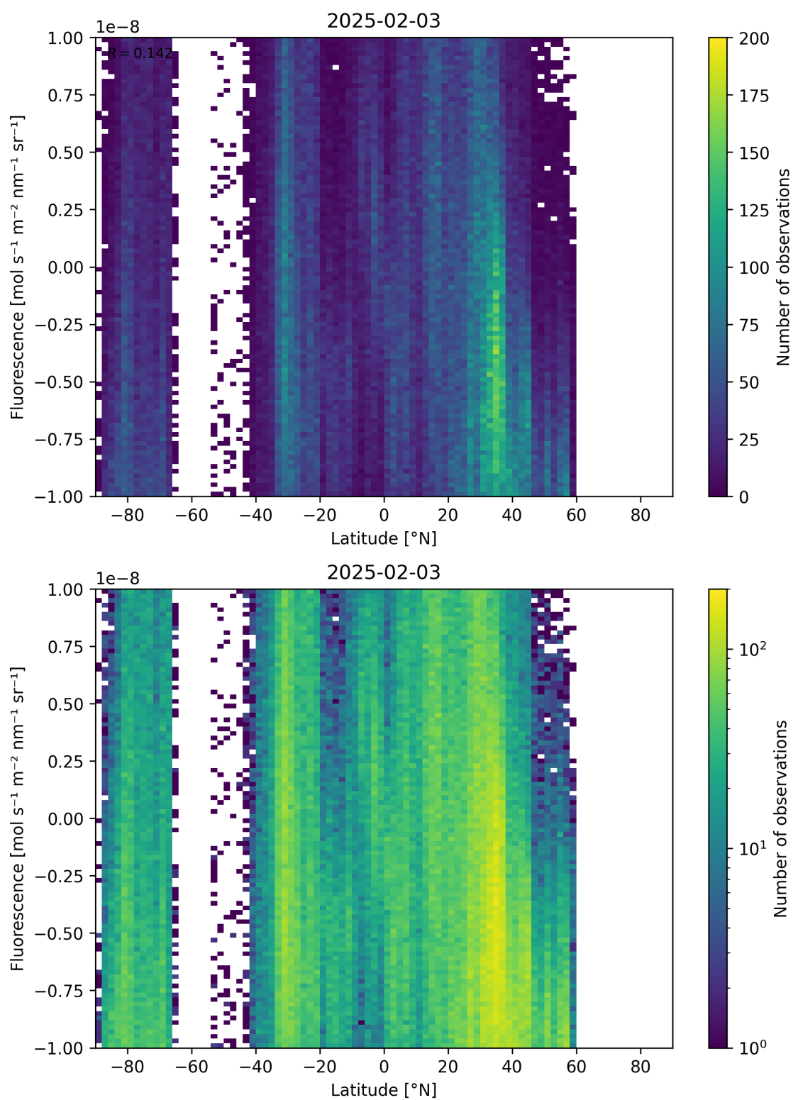
Figure 56: Scatter density plot of “Latitude” against “Fluorescence” for 2025-02-03 to 2025-02-04.
