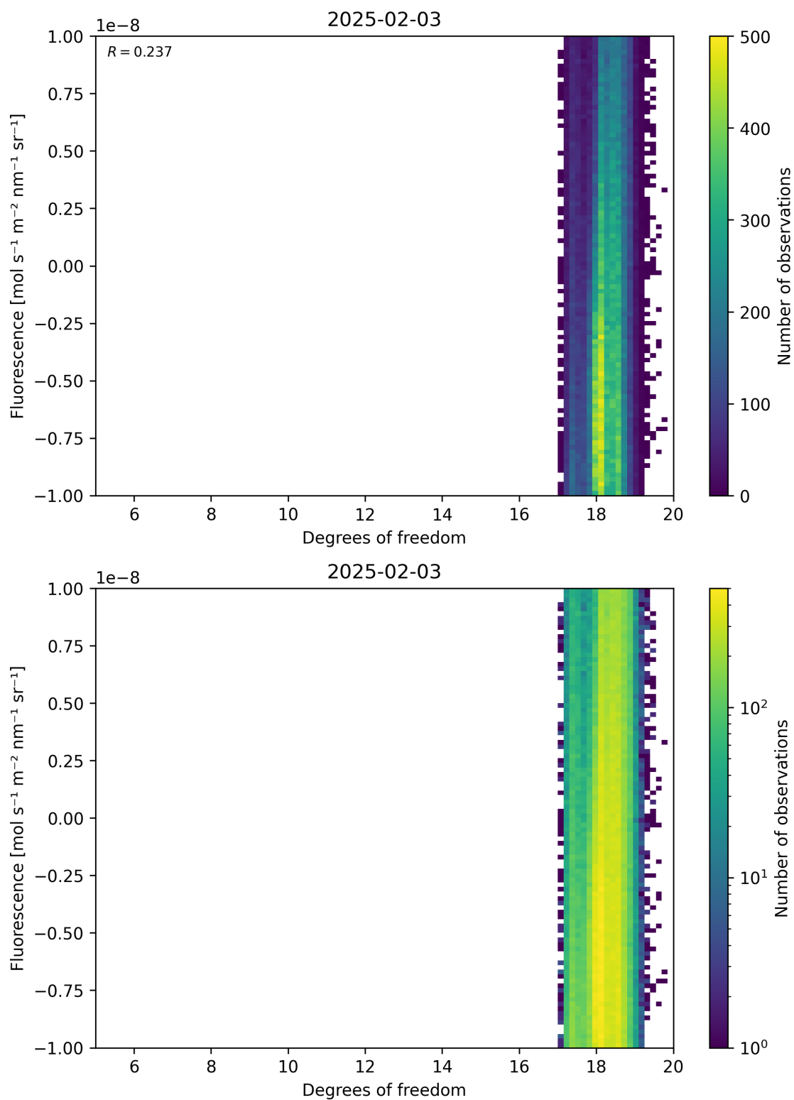
Figure 51: Scatter density plot of “Degrees of freedom” against “Fluorescence” for 2025-02-03 to 2025-02-04.
