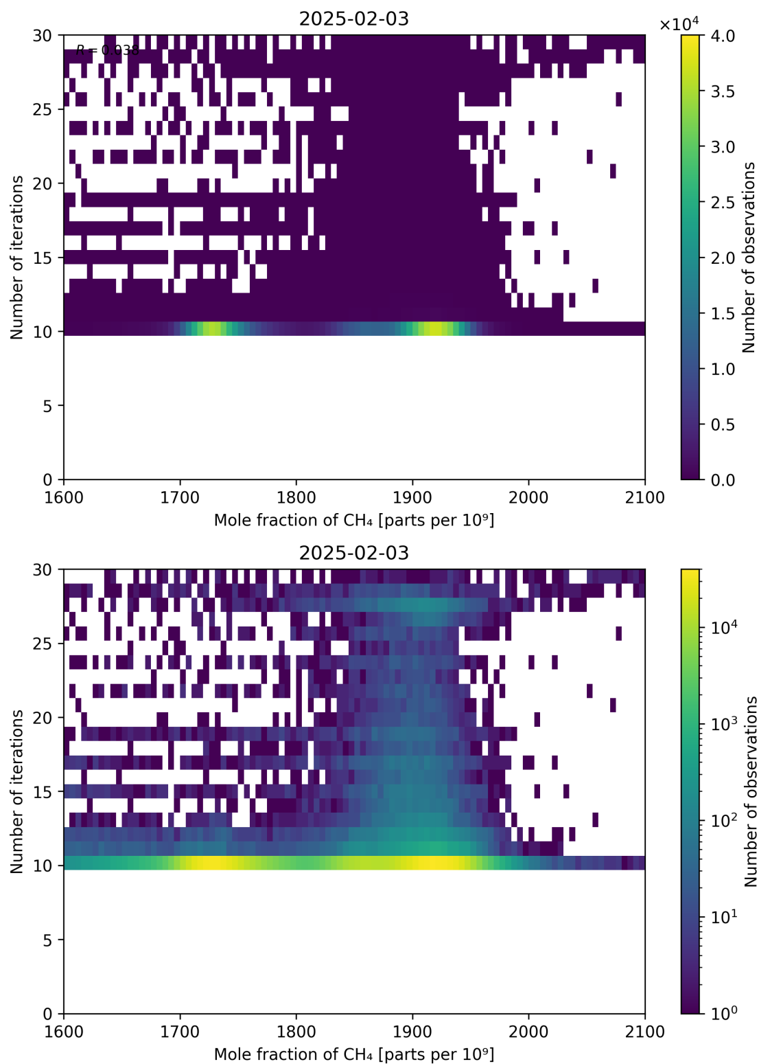
Figure 76: Scatter density plot of “Mole fraction of CH 4 ” against “Number of iterations” for 2025-02-03 to 2025-02-04.
