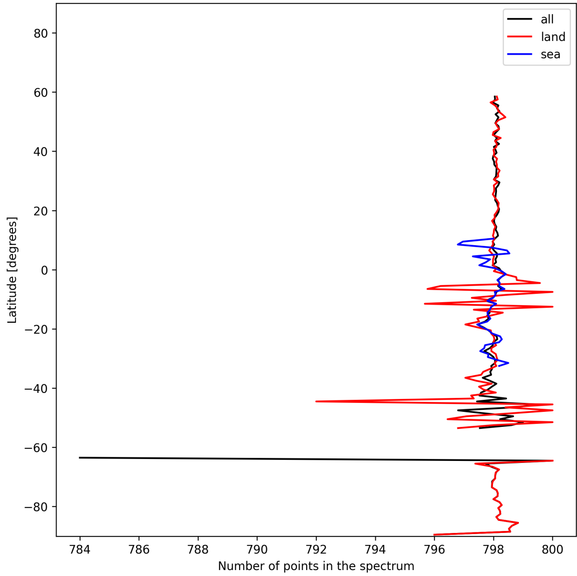
Figure 15: Zonal average of “Number of points in the spectrum” for 2025-02-03 to 2025-02-04.
