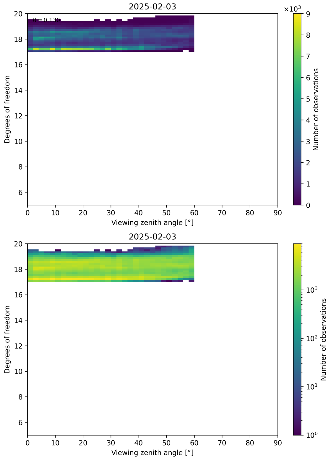
Figure 107: Scatter density plot of “Viewing zenith angle” against “Degrees of freedom” for 2025-02-03 to 2025-02-04.
