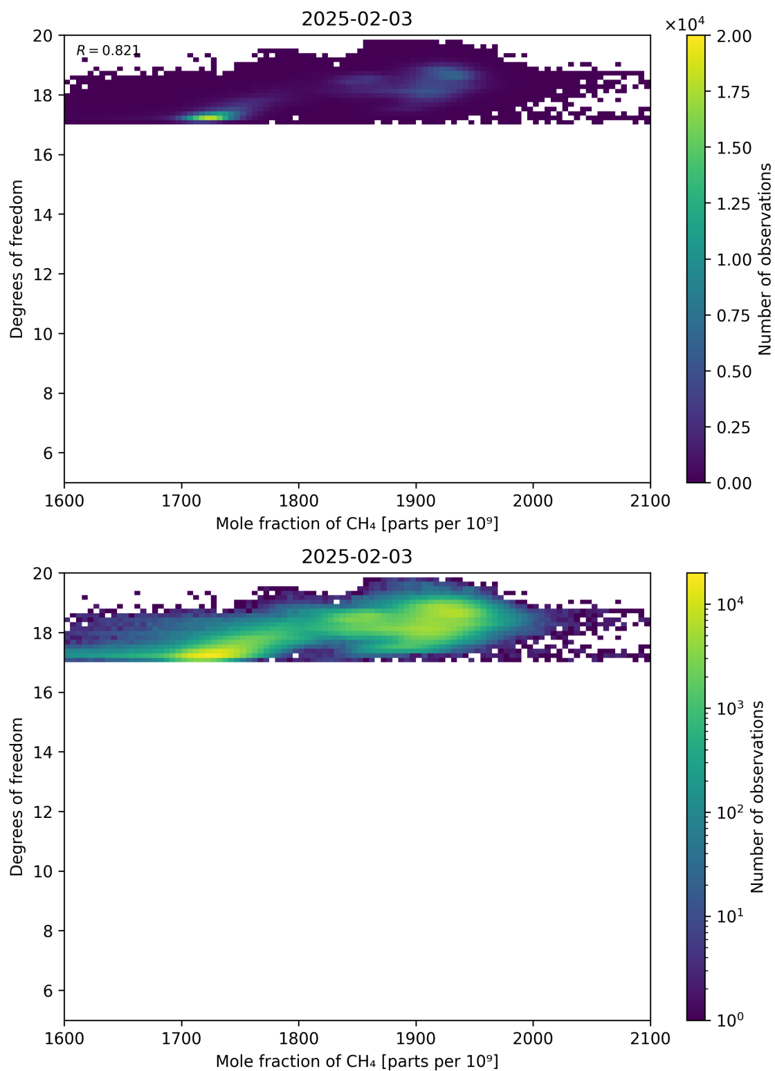
Figure 72: Scatter density plot of “Mole fraction of CH 4 ” against “Degrees of freedom” for 2025-02-03 to 2025-02-04.
