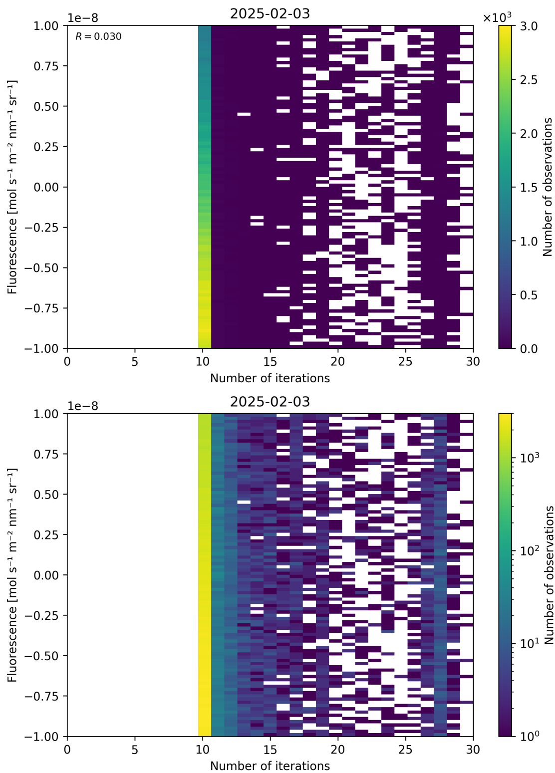
Figure 87: Scatter density plot of "Number of iterations" against "Fluorescence" for 2025-02-03 to 2025-02-04.
