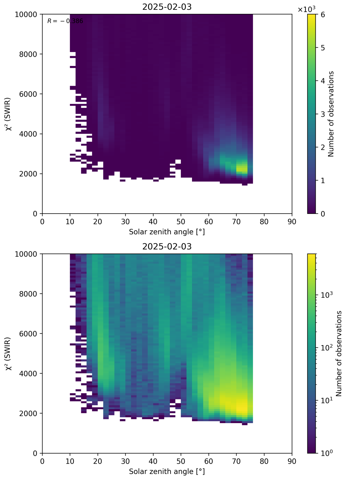
Figure 95: Scatter density plot of “Solar zenith angle” against “ \chi^2 (SWIR)” for 2025-02-03 to 2025-02-04.
