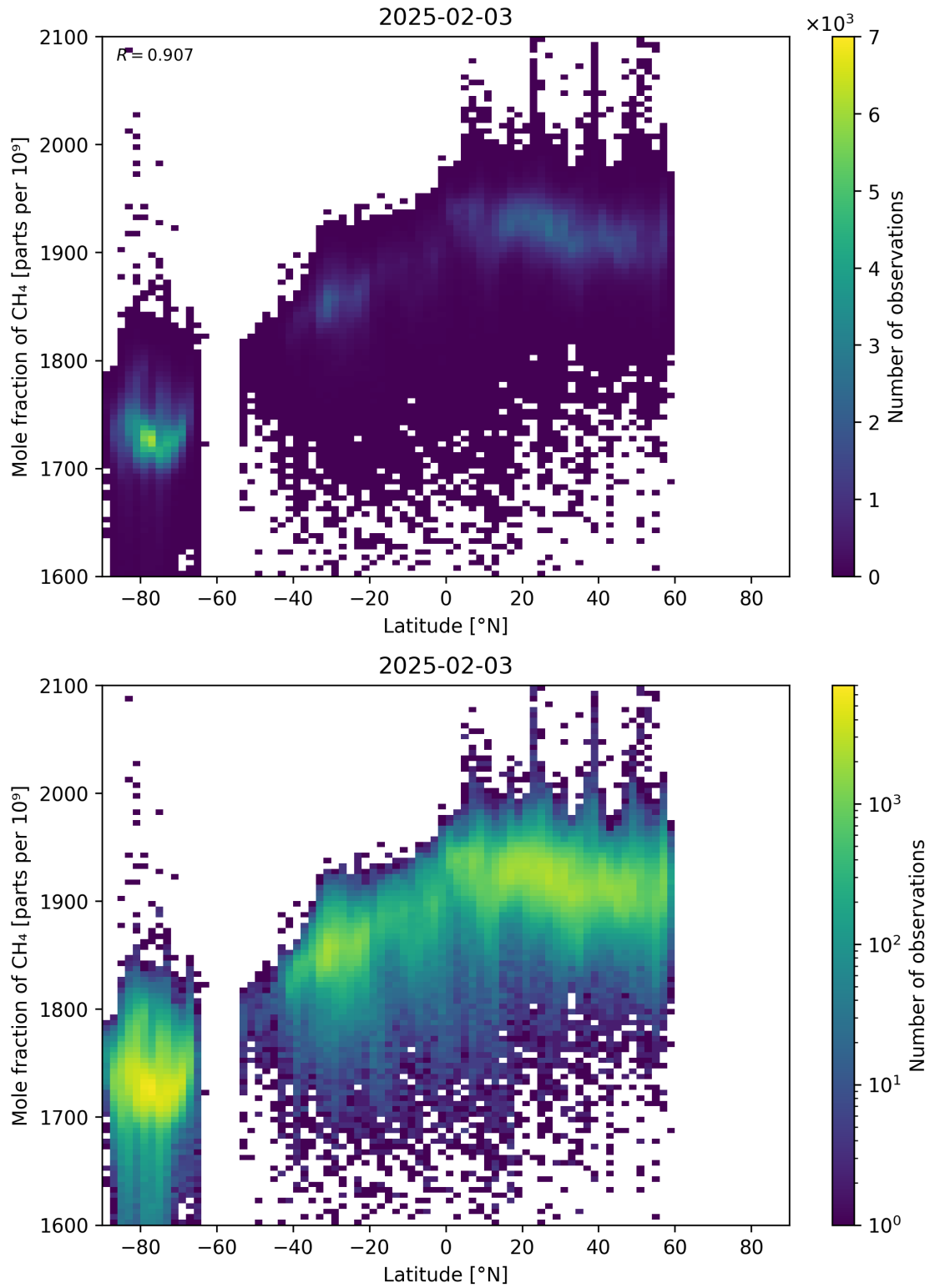
Figure 57: Scatter density plot of “Latitude” against “Mole fraction of \text{CH}_4 ” for 2025-02-03 to 2025-02-04.
