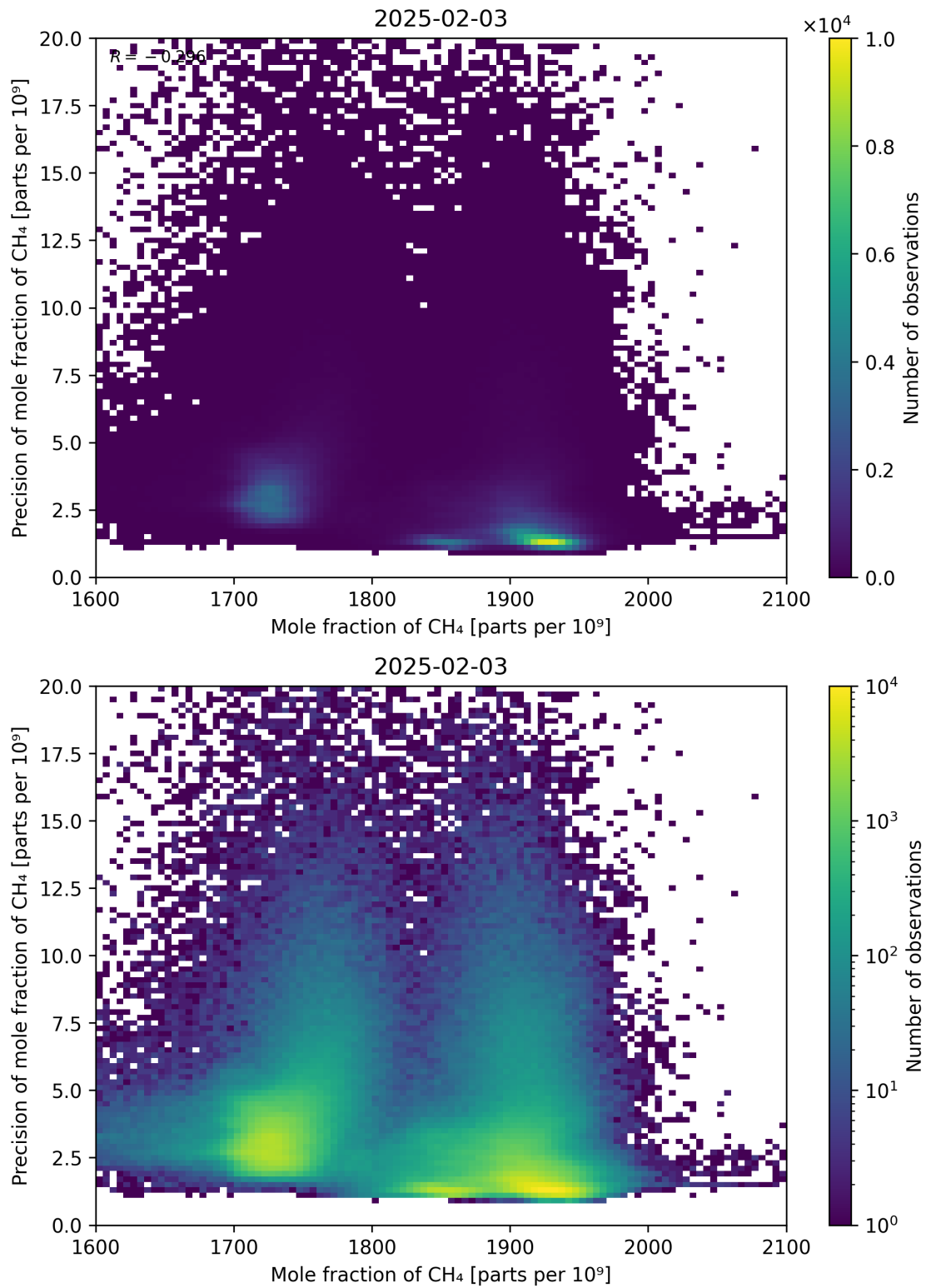
Figure 75: Scatter density plot of “Mole fraction of CH 4 ” against “Precision of mole fraction of CH 4 ” for 2025-02-03 to 2025-02-04.
