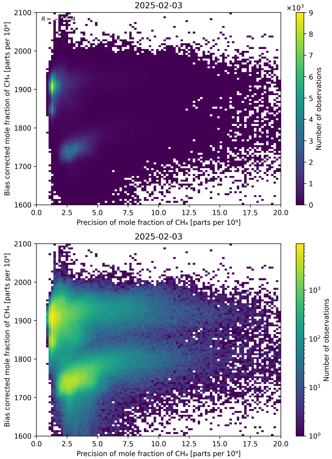
Figure 82: Scatter density plot of “Precision of mole fraction of CH 4 ” against “Bias corrected mole fraction of CH 4 ” for 2025-02-03 to 2025-02-04.
