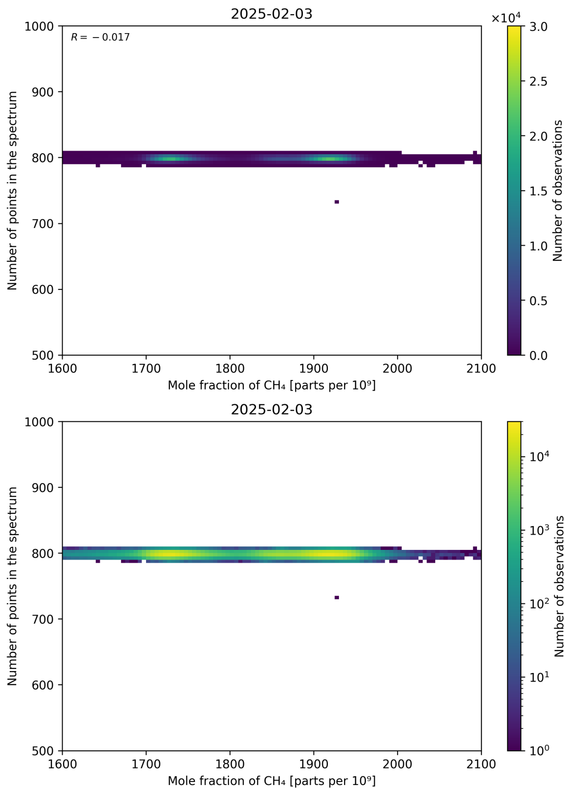
Figure 77: Scatter density plot of “Mole fraction of CH 4 ” against “Number of points in the spectrum” for 2025-02-03 to 2025-02-04.
