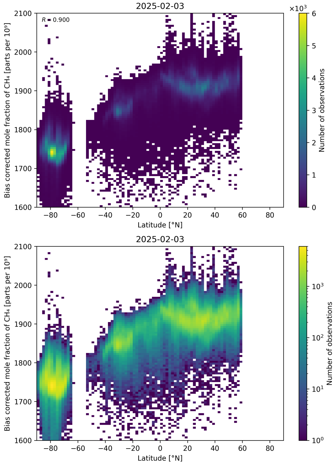
Figure 58: Scatter density plot of “Latitude” against “Bias corrected mole fraction of CH 4 ” for 2025-02-03 to 2025-02-04.
