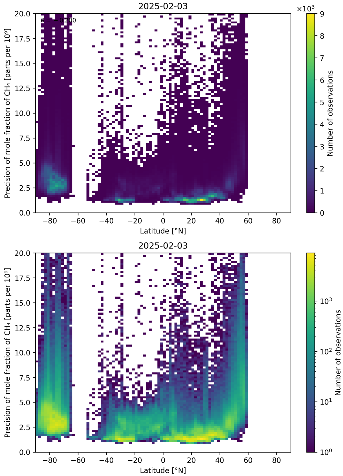
Figure 59: Scatter density plot of “Latitude” against “Precision of mole fraction of CH 4 ” for 2025-02-03 to 2025-02-04.
