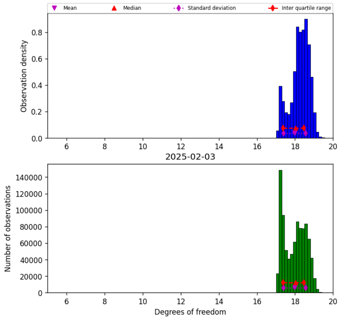
Figure 30: Histogram of “Degrees of freedom” for 2025-02-03 to 2025-02-04
