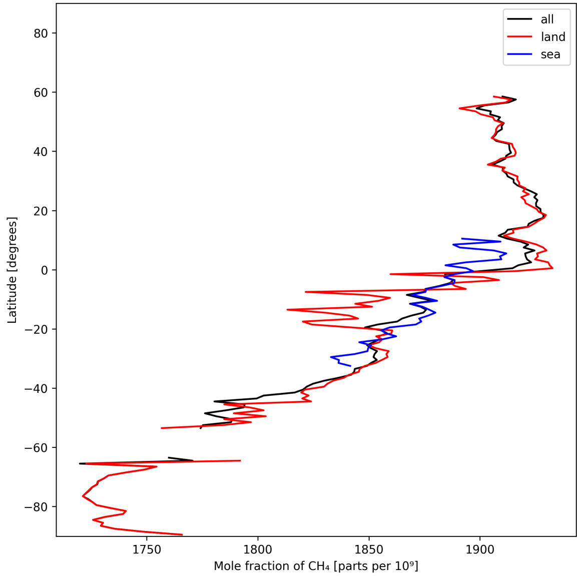
Figure 12: Zonal average of “Mole fraction of CH 4 ” for 2025-02-03 to 2025-02-04.
