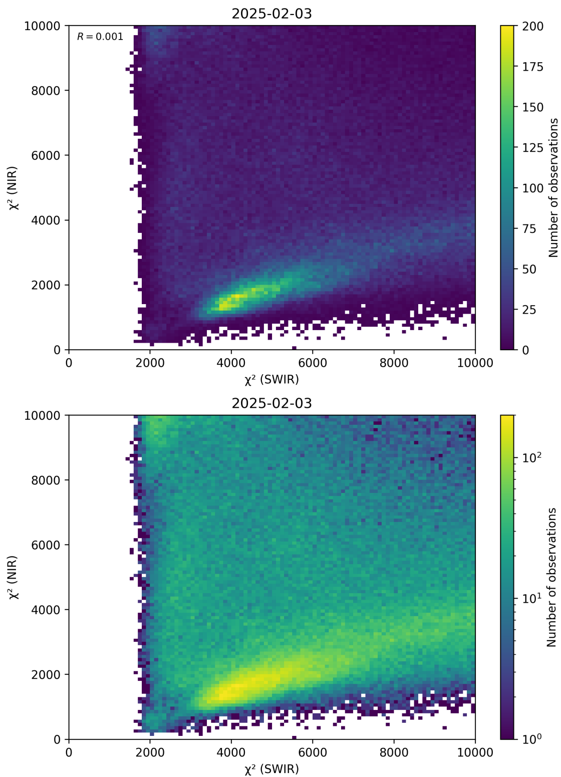
Figure 47: Scatter density plot of “ \chi^2 (SWIR)” against “ \chi^2 (NIR)” for 2025-02-03 to 2025-02-04.
