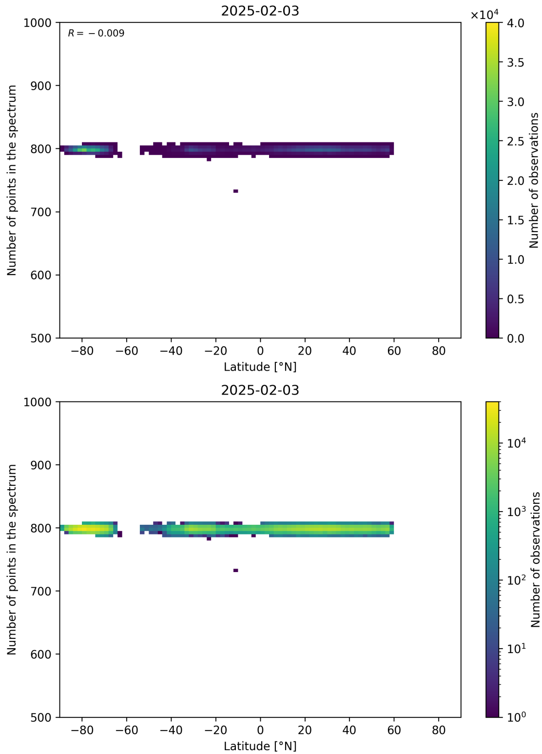
Figure 61: Scatter density plot of “Latitude” against “Number of points in the spectrum” for 2025-02-03 to 2025-02-04.
