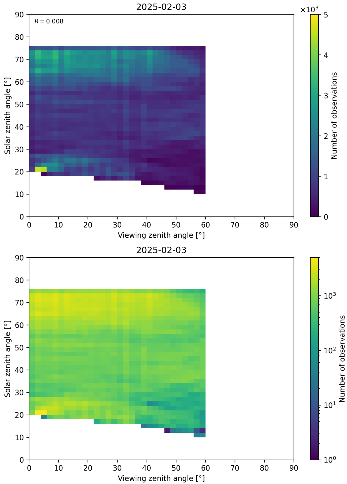
Figure 115: Scatter density plot of “Viewing zenith angle” against “Solar zenith angle” for 2025-02-03 to 2025-02-04.
