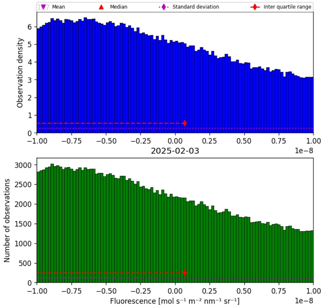
Figure 32: Histogram of “Fluorescence” for 2025-02-03 to 2025-02-04
