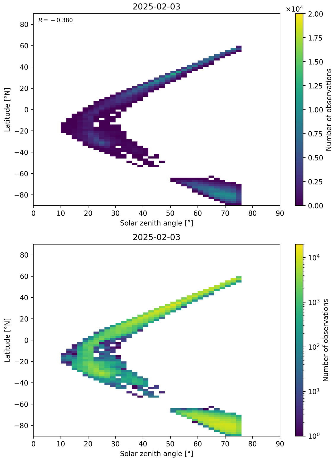
Figure 98: Scatter density plot of “Solar zenith angle” against “Latitude” for 2025-02-03 to 2025-02-04.
