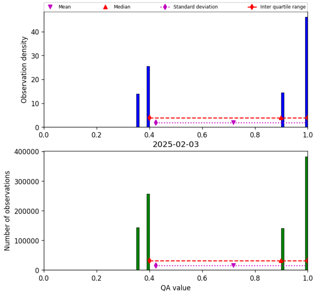
Figure 22: Histogram of “QA value” for 2025-02-03 to 2025-02-04
