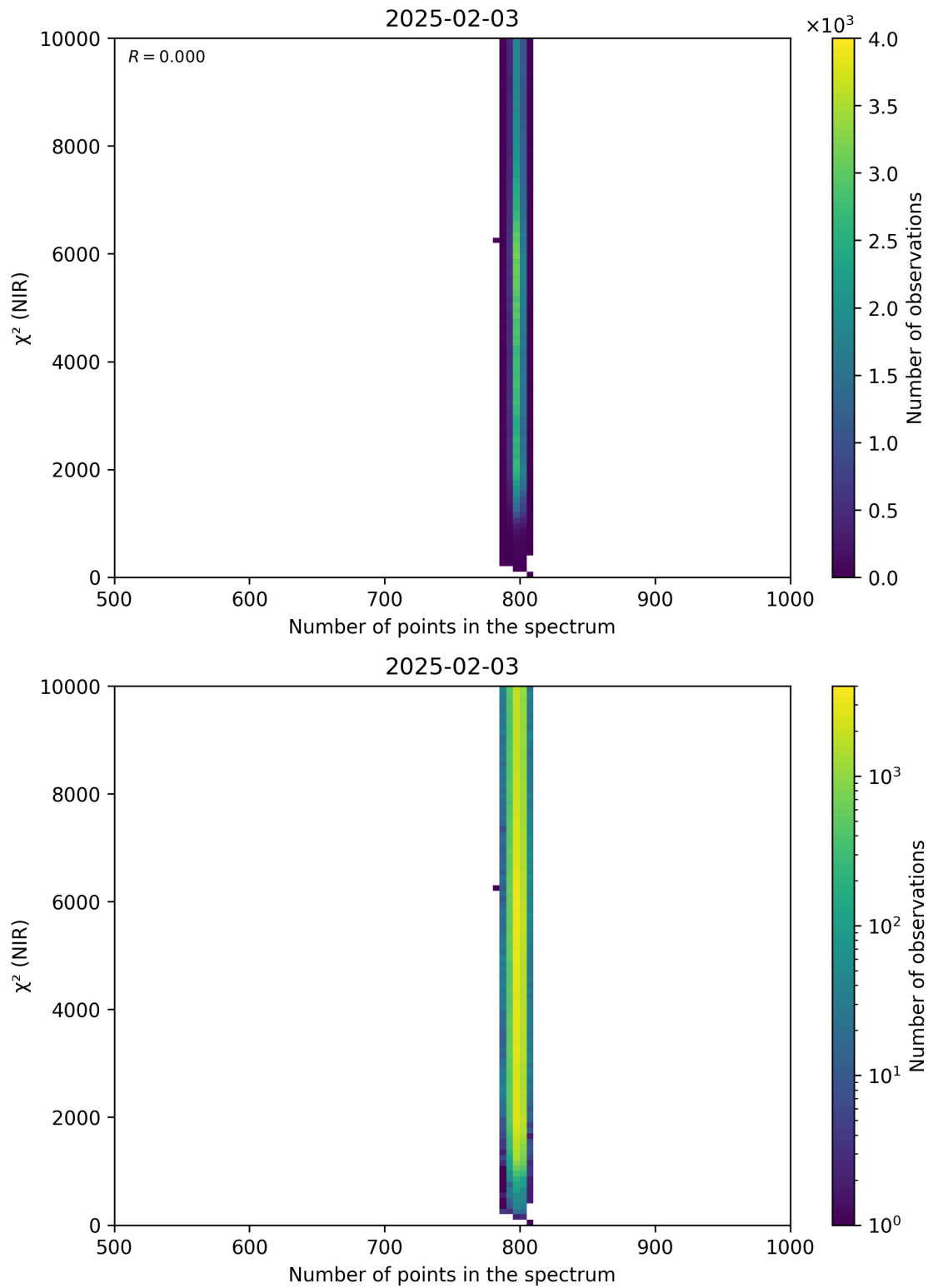
Figure 88: Scatter density plot of “Number of points in the spectrum” against “ \chi^2 (NIR)” for 2025-02-03 to 2025-02-04.
