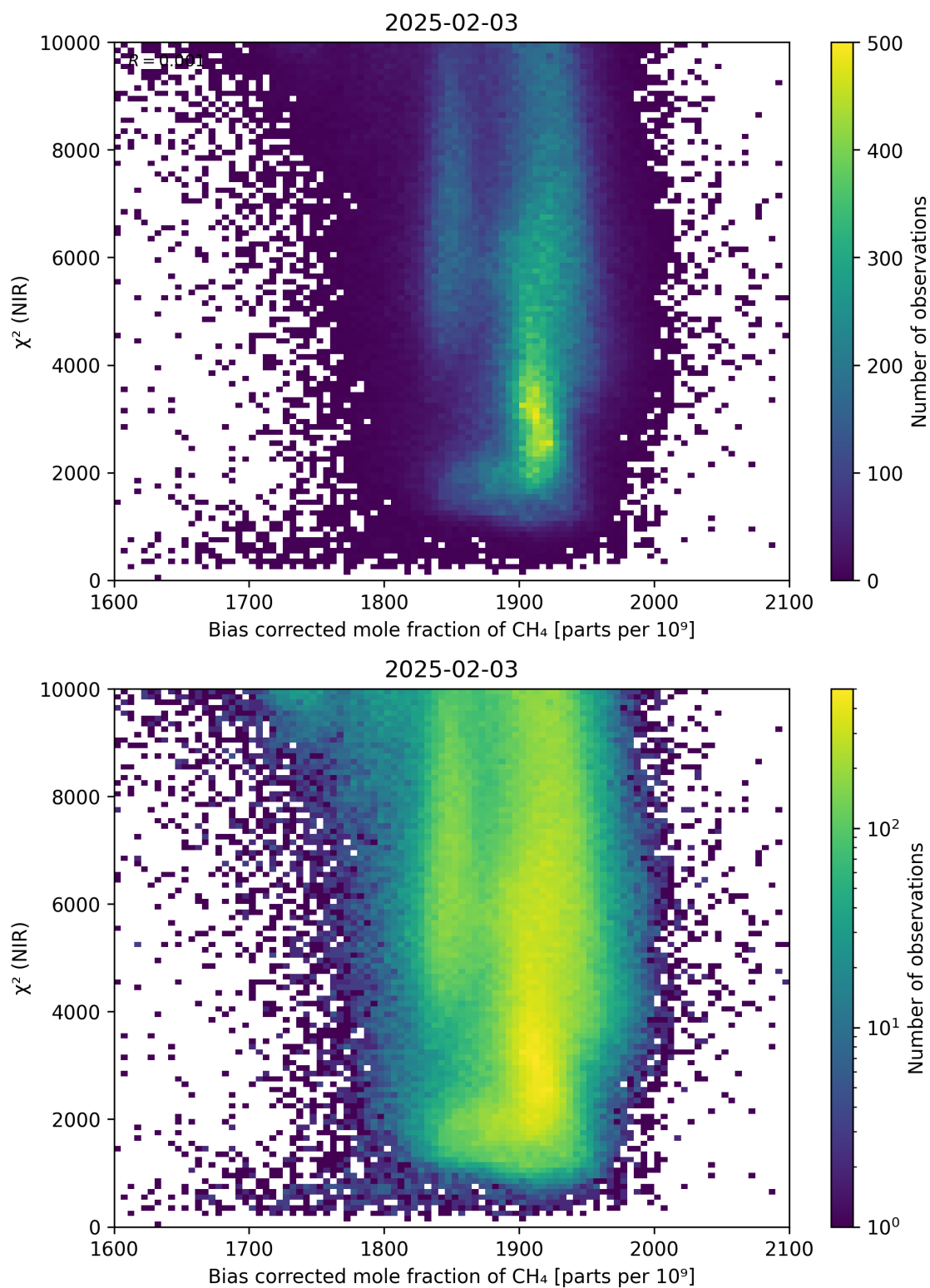
Figure 63: Scatter density plot of “Bias corrected mole fraction of \text{CH}_4 ” against “ \chi^2 (NIR)” for 2025-02-03 to 2025-02-04.
