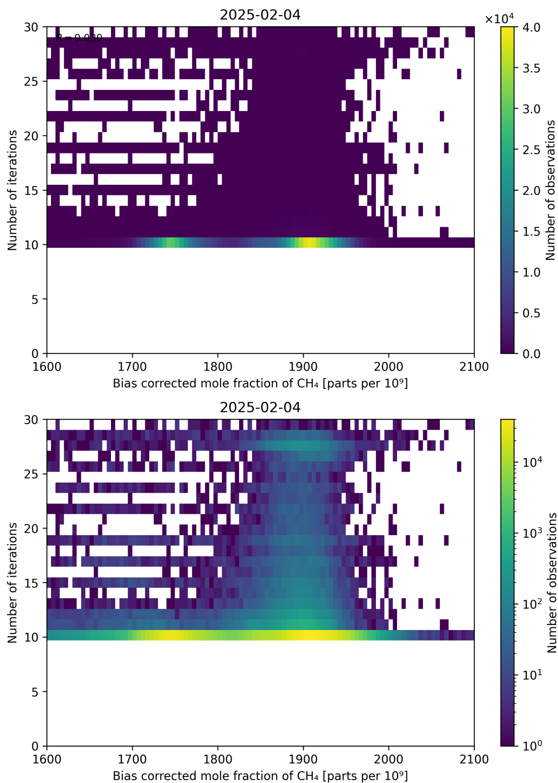
Figure 67: Scatter density plot of “Bias corrected mole fraction of \text{CH}_4 ” against “Number of iterations” for 2025-02-03 to 2025-02-05.
