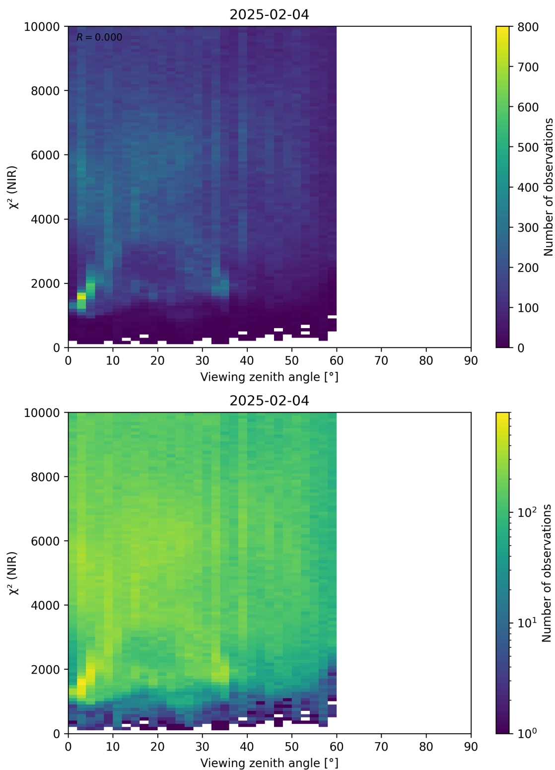
Figure 105: Scatter density plot of “Viewing zenith angle” against “ \chi^2 (NIR)” for 2025-02-03 to 2025-02-05.
