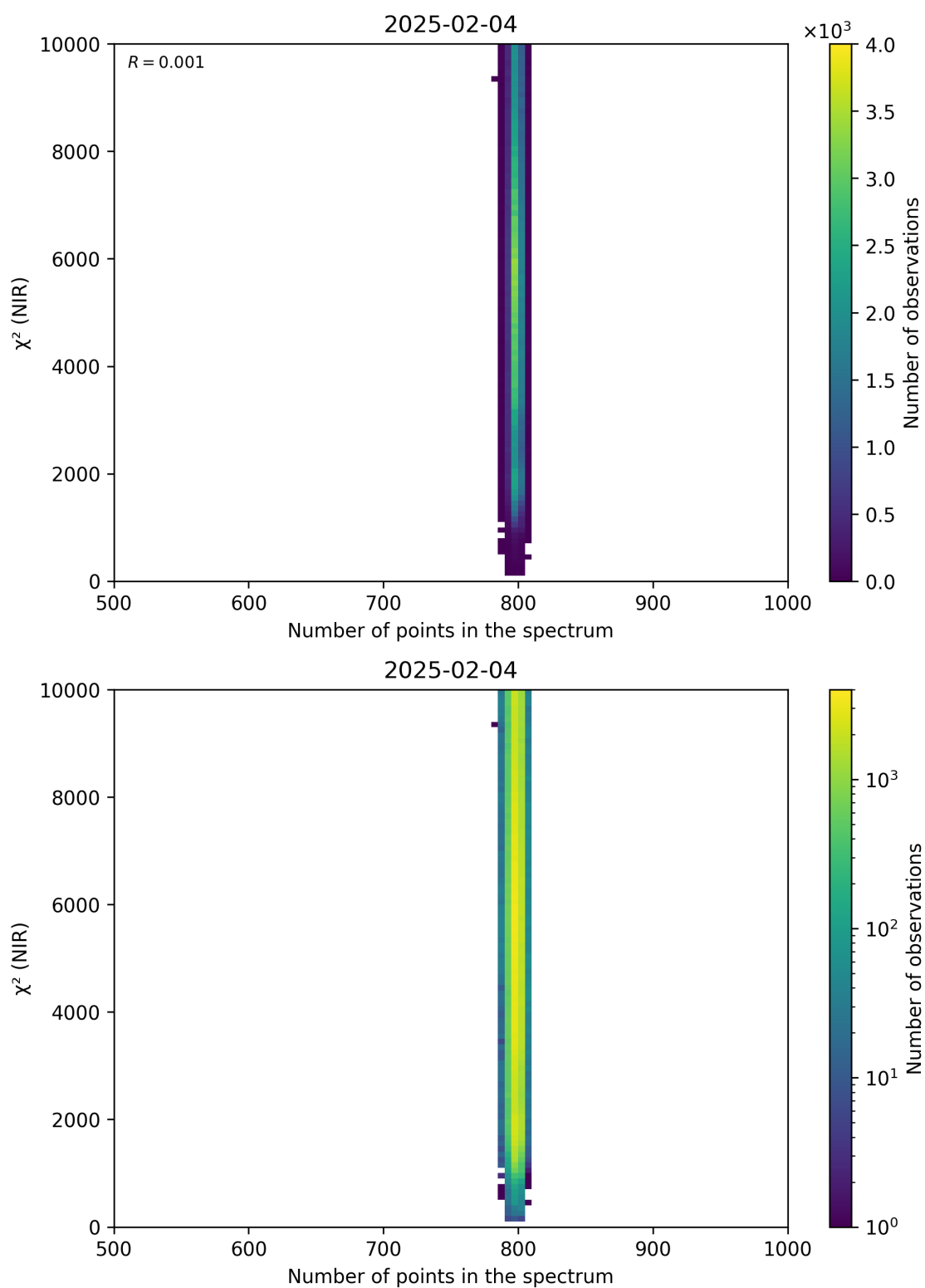
Figure 88: Scatter density plot of “Number of points in the spectrum” against “ \chi^2 (NIR)” for 2025-02-03 to 2025-02-05.
