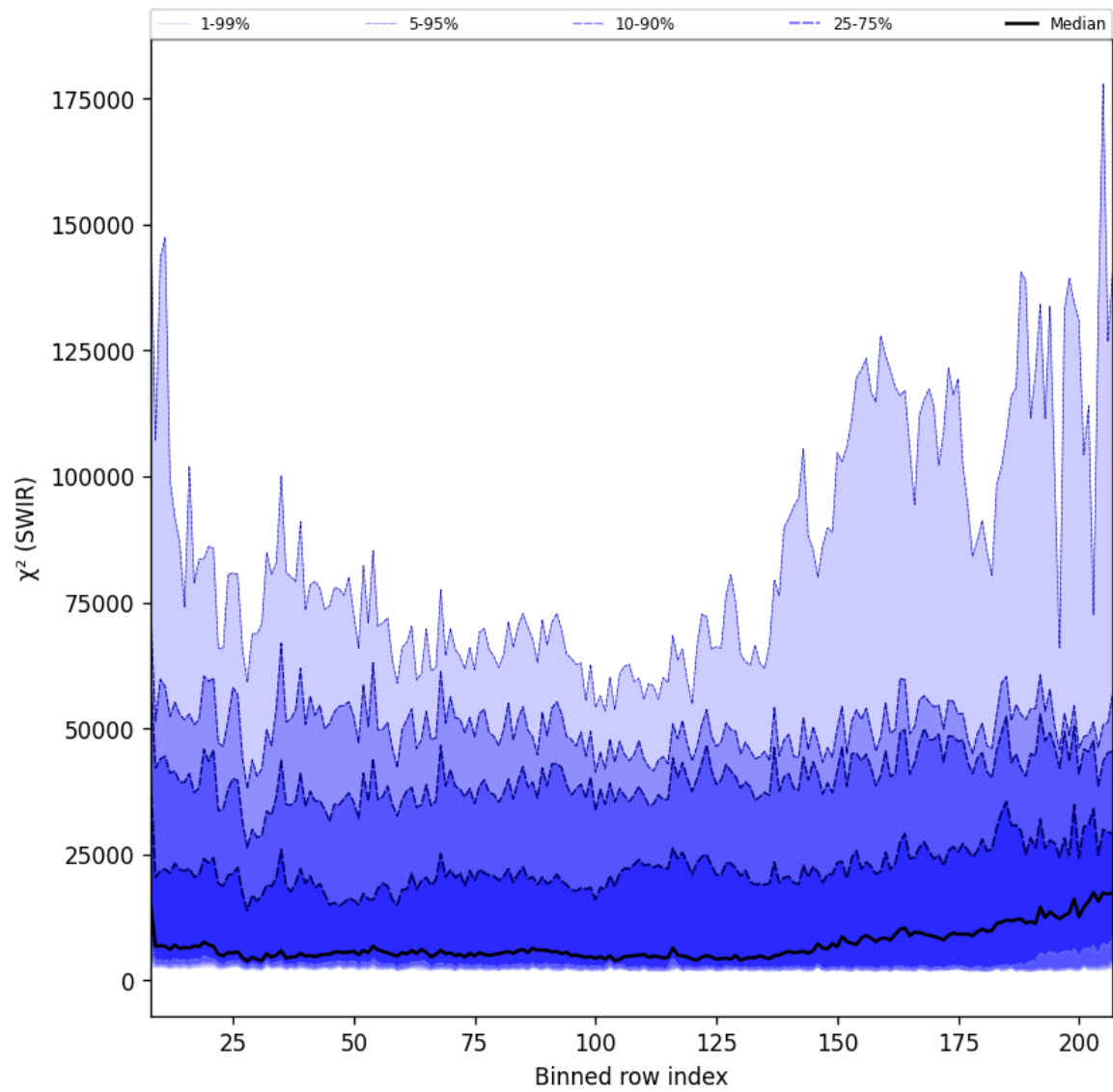
Figure 39: Along track statistics of “ \chi^2 (SWIR)” for 2025-02-03 to 2025-02-05
