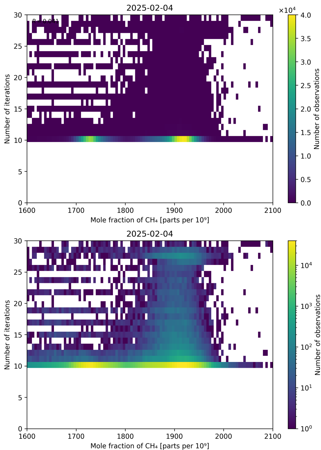
Figure 76: Scatter density plot of “Mole fraction of CH 4 ” against “Number of iterations” for 2025-02-03 to 2025-02-05.
