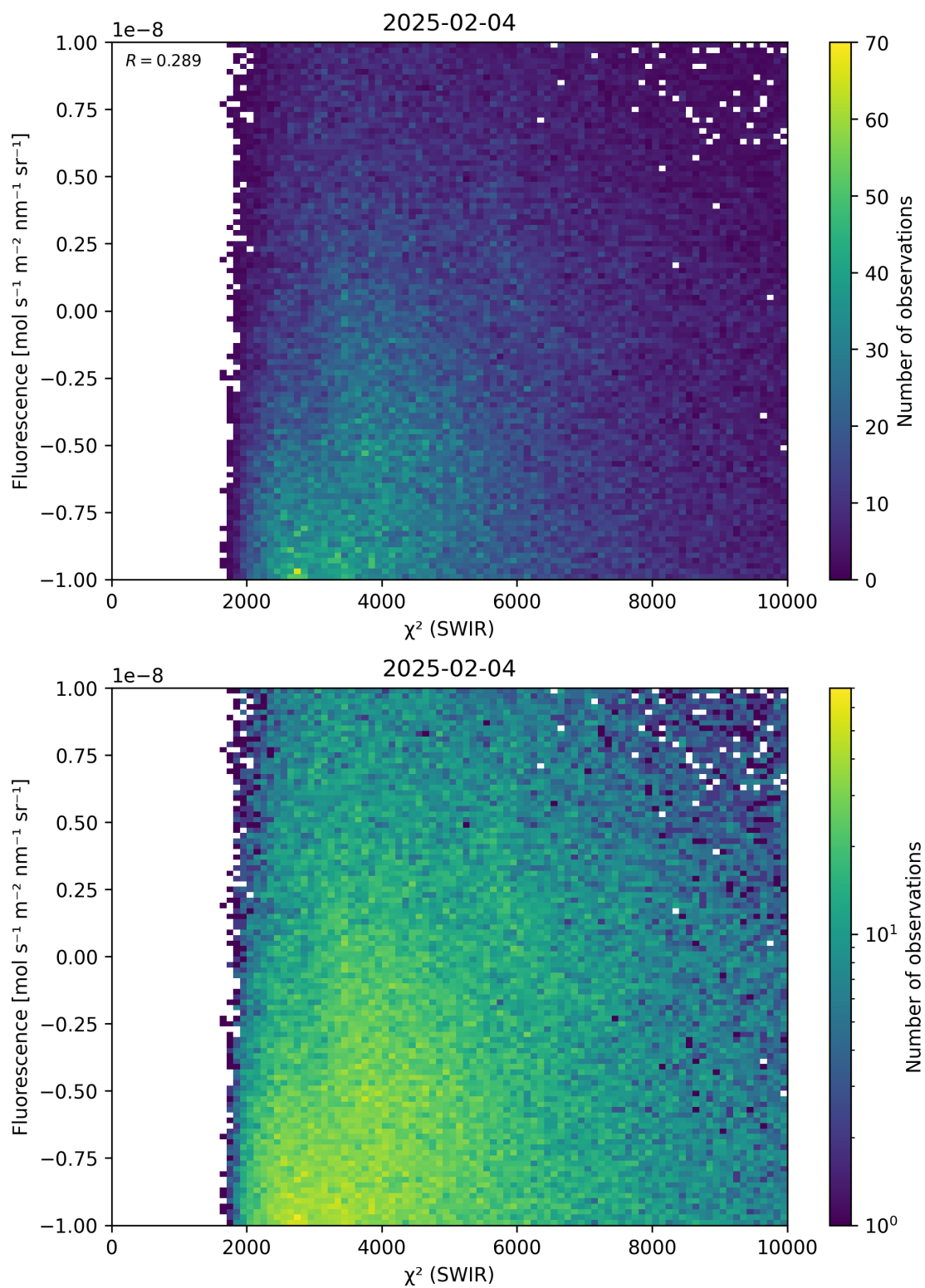
Figure 49: Scatter density plot of “ \chi^2 (SWIR)” against “Fluorescence” for 2025-02-03 to 2025-02-05.
