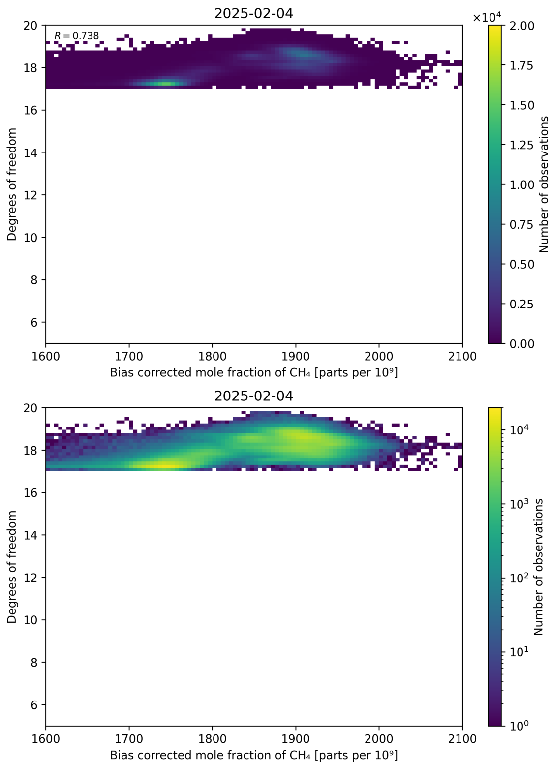
Figure 65: Scatter density plot of “Bias corrected mole fraction of CH 4 ” against “Degrees of freedom” for 2025-02-03 to 2025-02-05.
