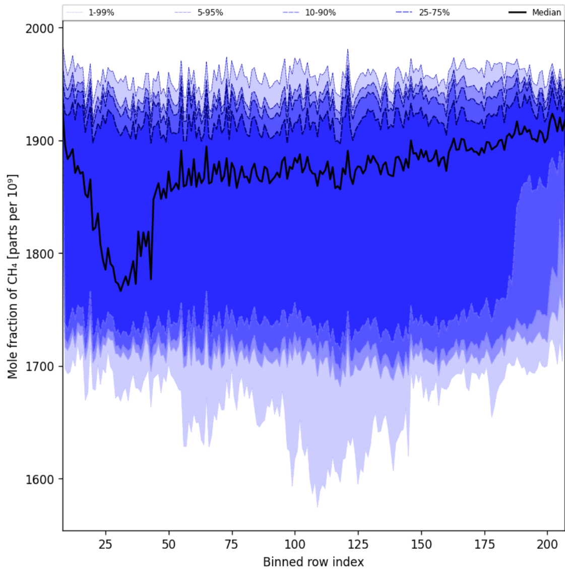
Figure 34: Along track statistics of “Mole fraction of CH 4 ” for 2025-02-03 to 2025-02-05
