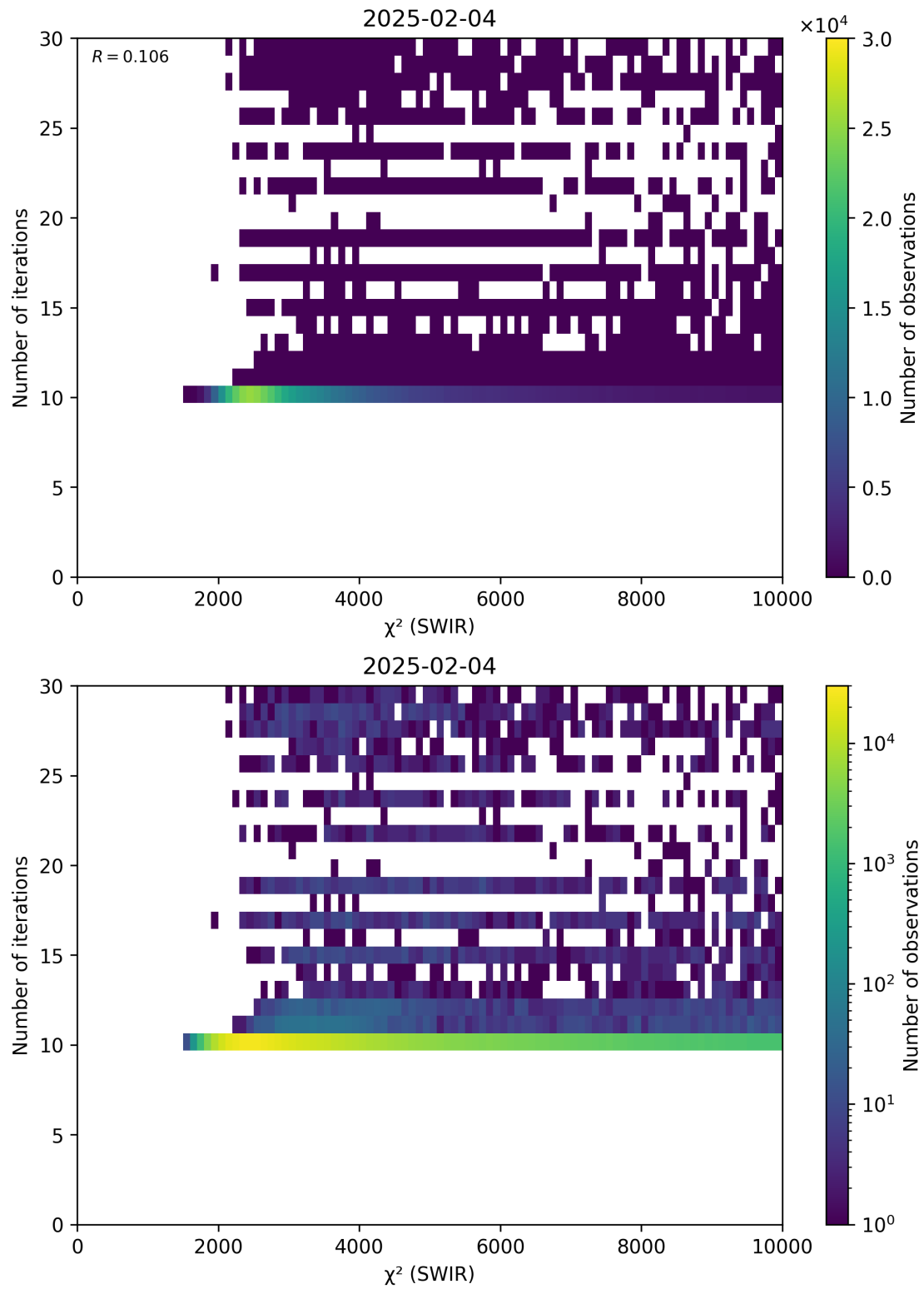
Figure 50: Scatter density plot of “ \chi^2 (SWIR)” against “Number of iterations” for 2025-02-03 to 2025-02-05.
