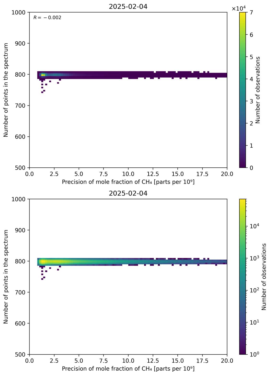
Figure 84: Scatter density plot of “Precision of mole fraction of CH 4 ” against “Number of points in the spectrum” for 2025-02-03 to 2025-02-05.
