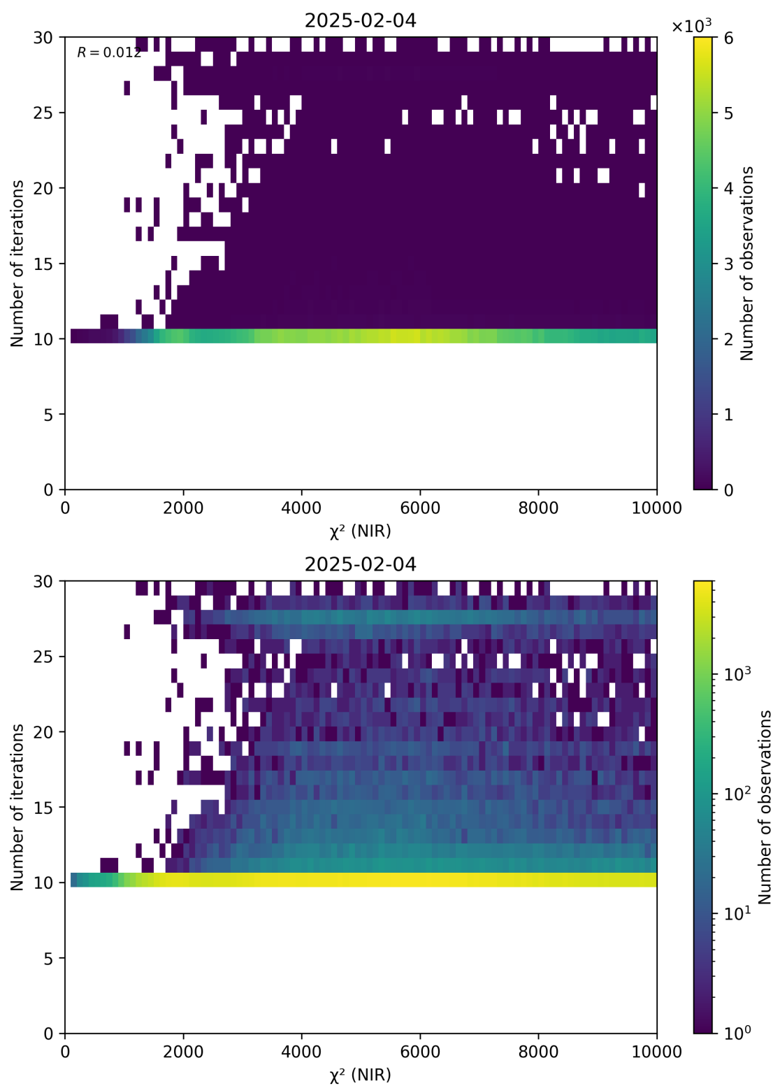
Figure 46: Scatter density plot of “ \chi^2 (NIR)” against “Number of iterations” for 2025-02-03 to 2025-02-05.
