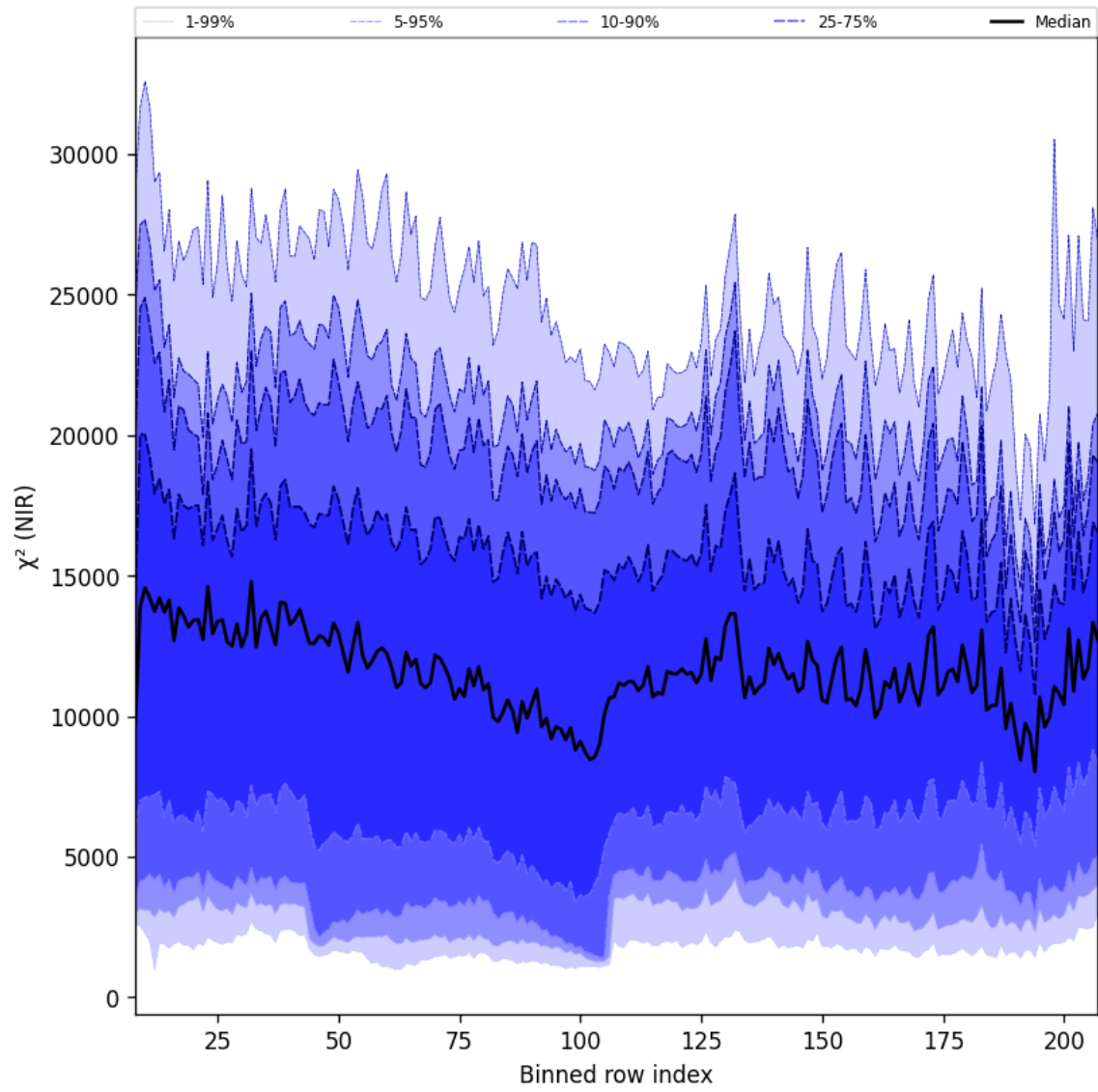
Figure 40: Along track statistics of “ \chi^2 (NIR)” for 2025-02-03 to 2025-02-05
