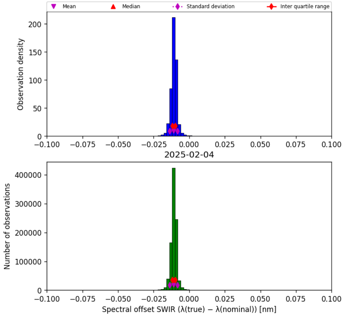
Figure 27: Histogram of “Spectral offset SWIR ( \lambda_{\text{true}} - \lambda_{\text{nominal}} )” for 2025-02-03 to 2025-02-05
