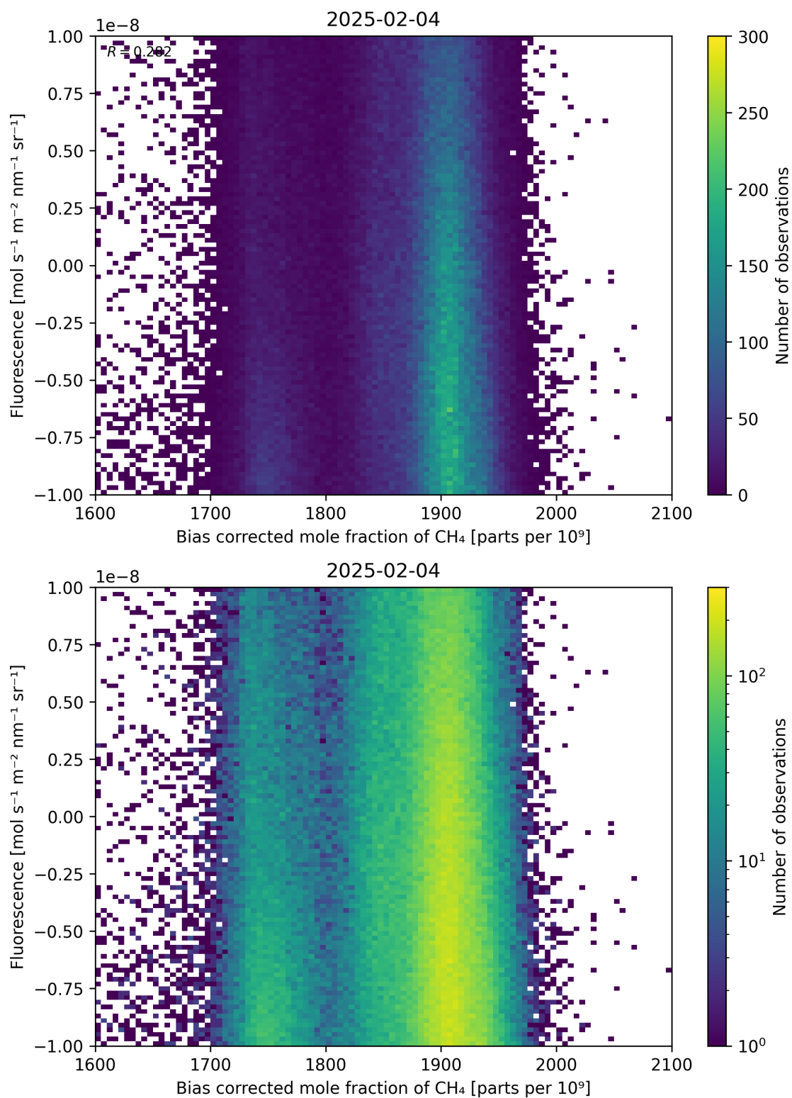
Figure 66: Scatter density plot of “Bias corrected mole fraction of \text{CH}_4 ” against “Fluorescence” for 2025-02-03 to 2025-02-05.
