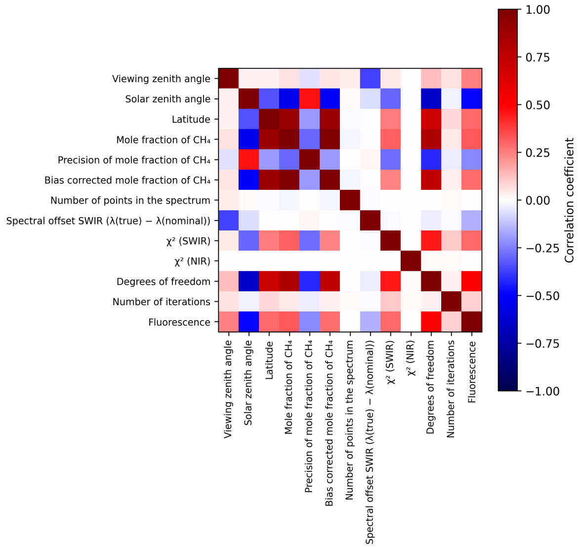
Figure 2: Map of correlation matrix for 2025-02-03 to 2025-02-05.
