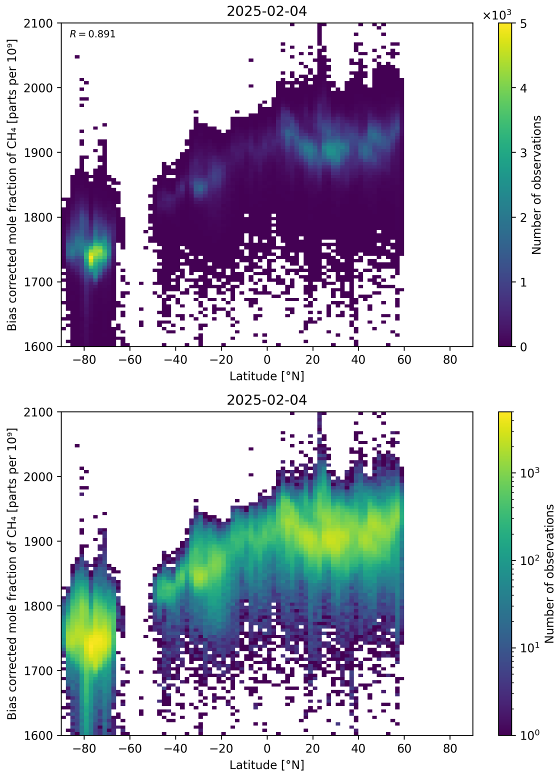
Figure 58: Scatter density plot of “Latitude” against “Bias corrected mole fraction of \text{CH}_4 ” for 2025-02-03 to 2025-02-05.
