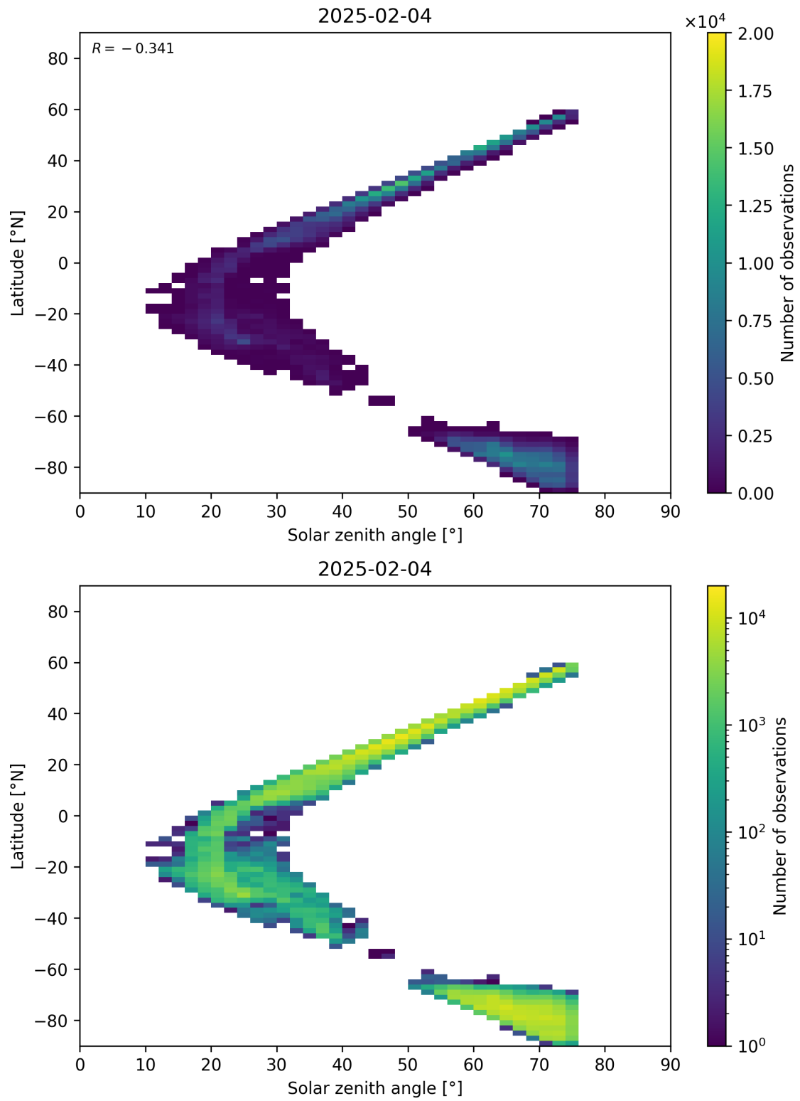
Figure 98: Scatter density plot of “Solar zenith angle” against “Latitude” for 2025-02-03 to 2025-02-05.
