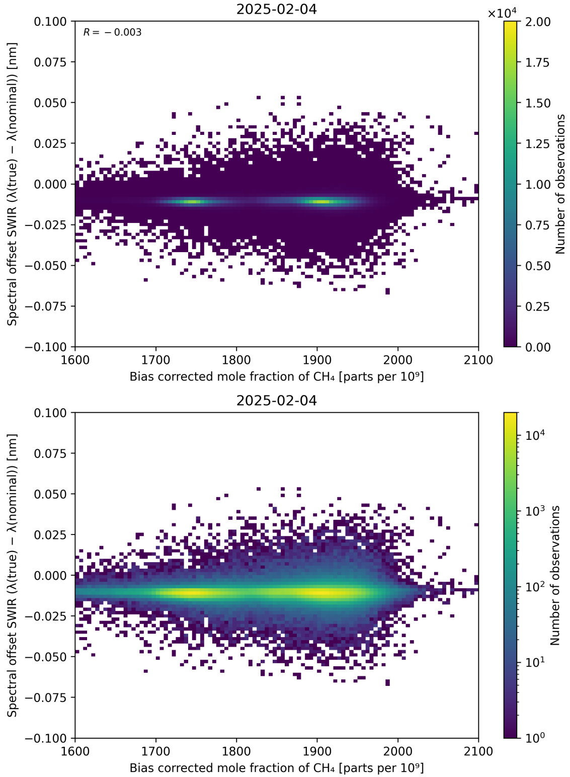
Figure 69: Scatter density plot of “Bias corrected mole fraction of \text{CH}_4 ” against “Spectral offset SWIR ( \lambda_{\text{true}} - \lambda_{\text{nominal}} )” for 2025-02-03 to 2025-02-05.
