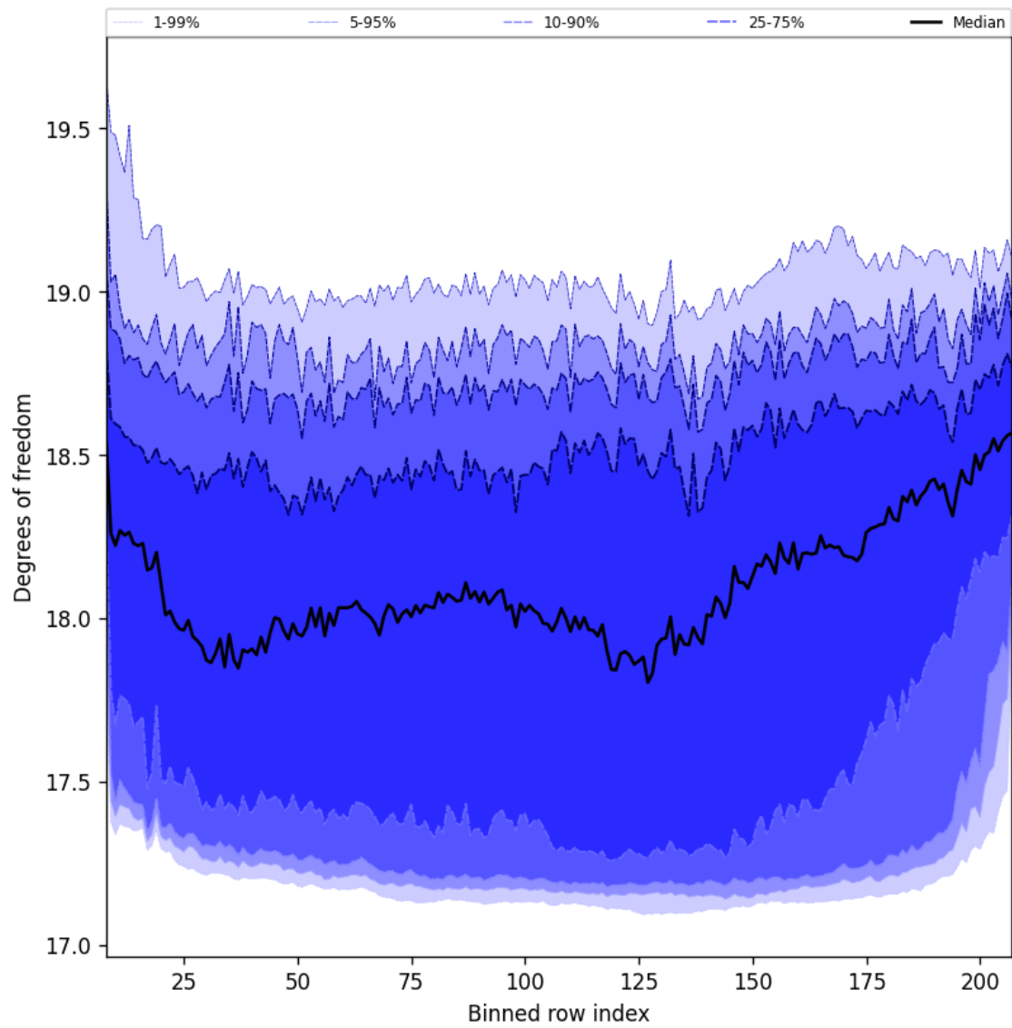
Figure 41: Along track statistics of “Degrees of freedom” for 2025-02-03 to 2025-02-05
