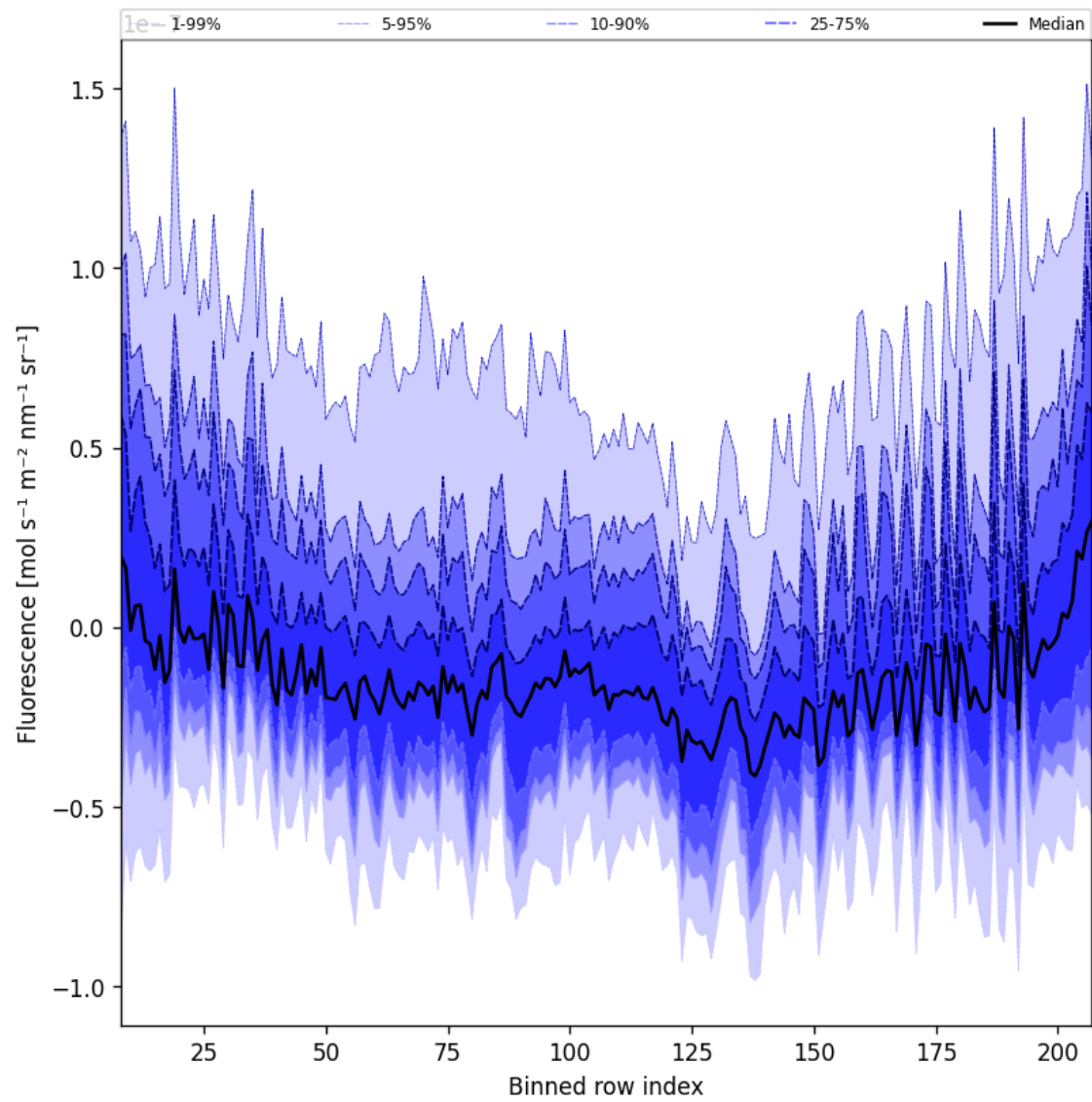
Figure 43: Along track statistics of “Fluorescence” for 2025-02-03 to 2025-02-05
