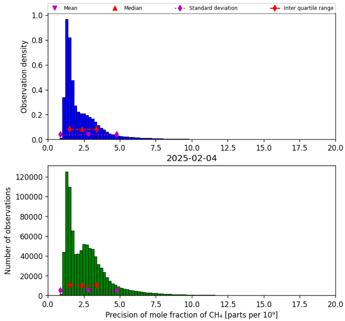
Figure 24: Histogram of “Precision of mole fraction of CH 4 ” for 2025-02-03 to 2025-02-05
