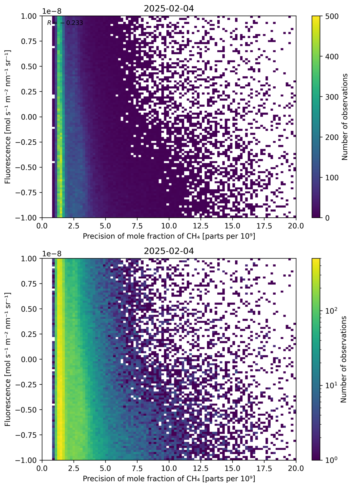
Figure 81: Scatter density plot of “Precision of mole fraction of \text{CH}_4 ” against “Fluorescence” for 2025-02-03 to 2025-02-05.
