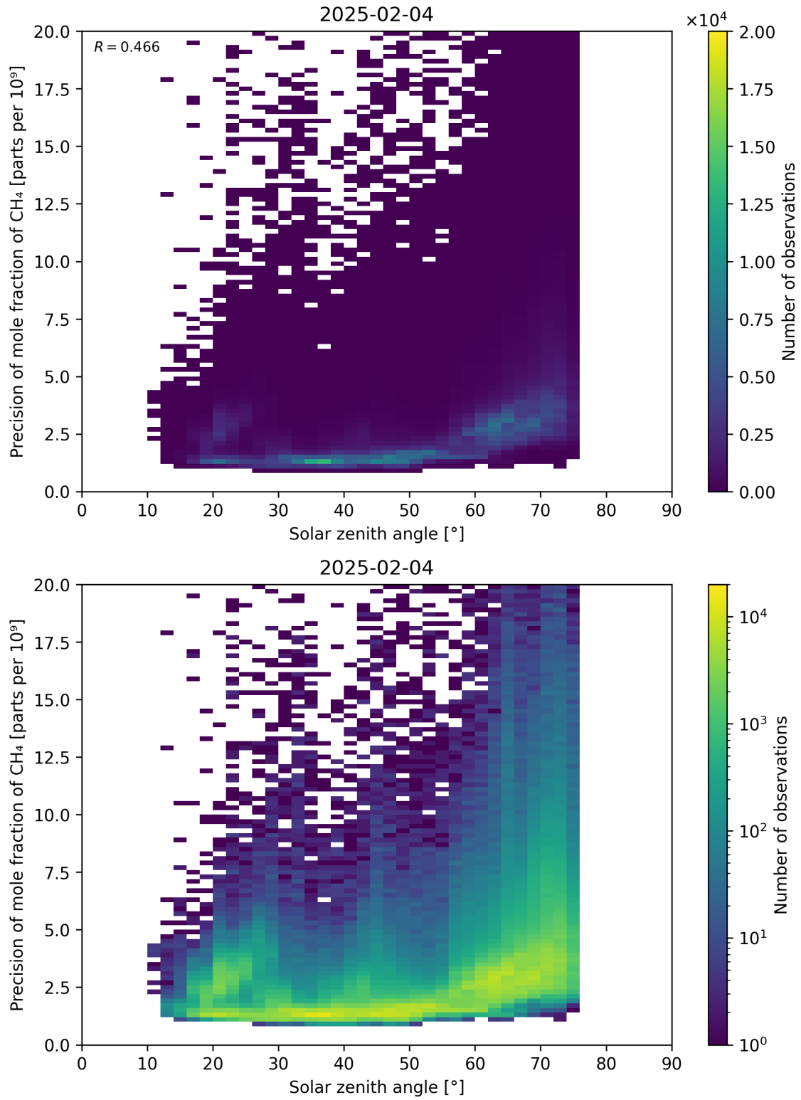
Figure 101: Scatter density plot of “Solar zenith angle” against “Precision of mole fraction of CH 4 ” for 2025-02-03 to 2025-02-05.
