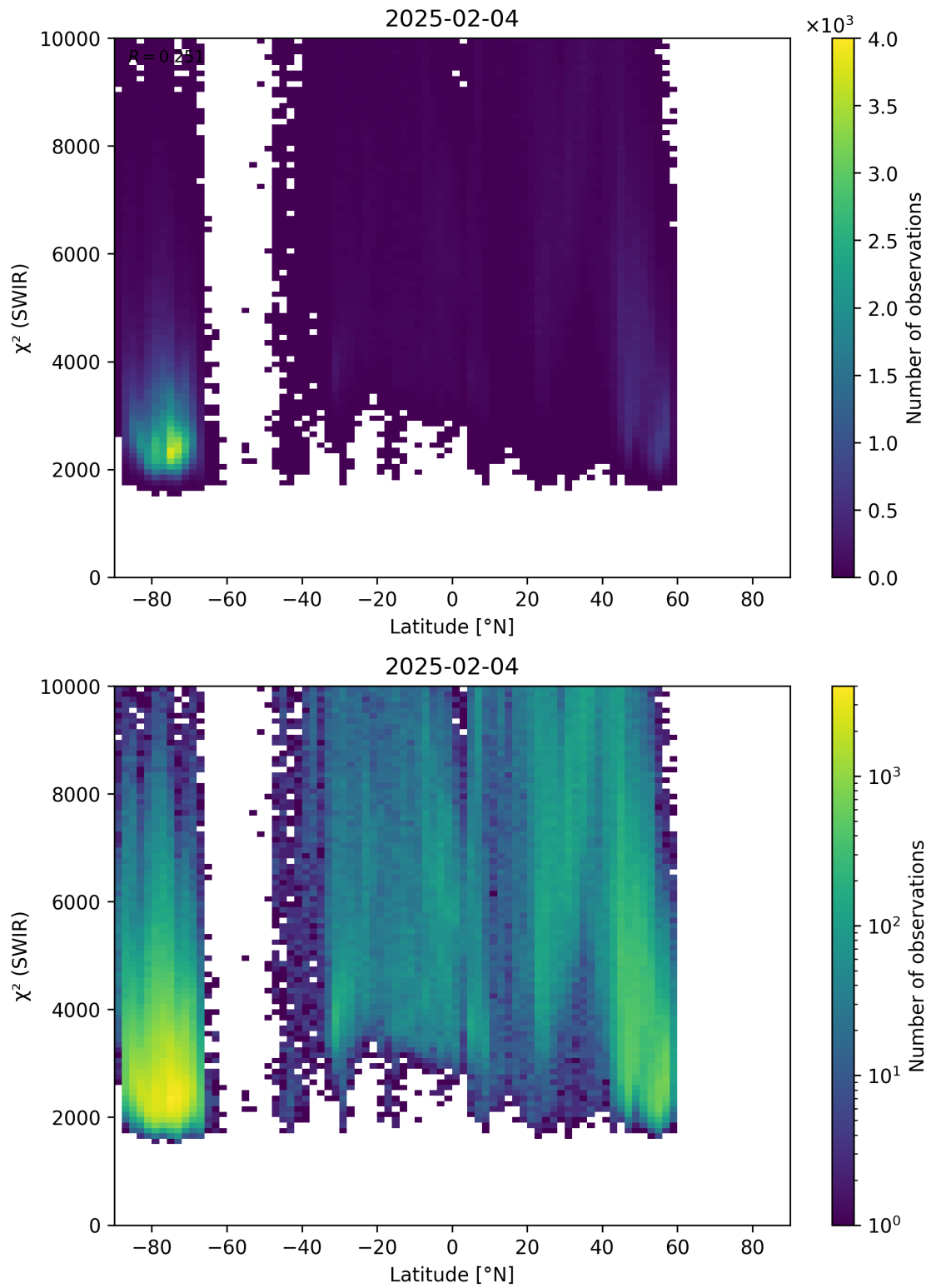
Figure 54: Scatter density plot of “Latitude” against “ \chi^2 (SWIR)” for 2025-02-03 to 2025-02-05.
