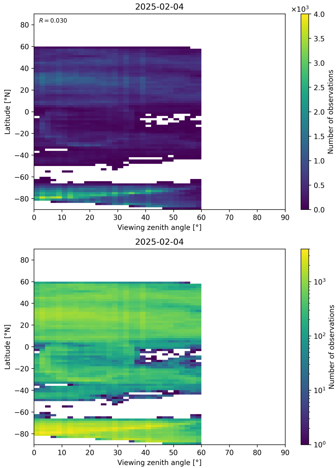
Figure 109: Scatter density plot of “Viewing zenith angle” against “Latitude” for 2025-02-03 to 2025-02-05.
