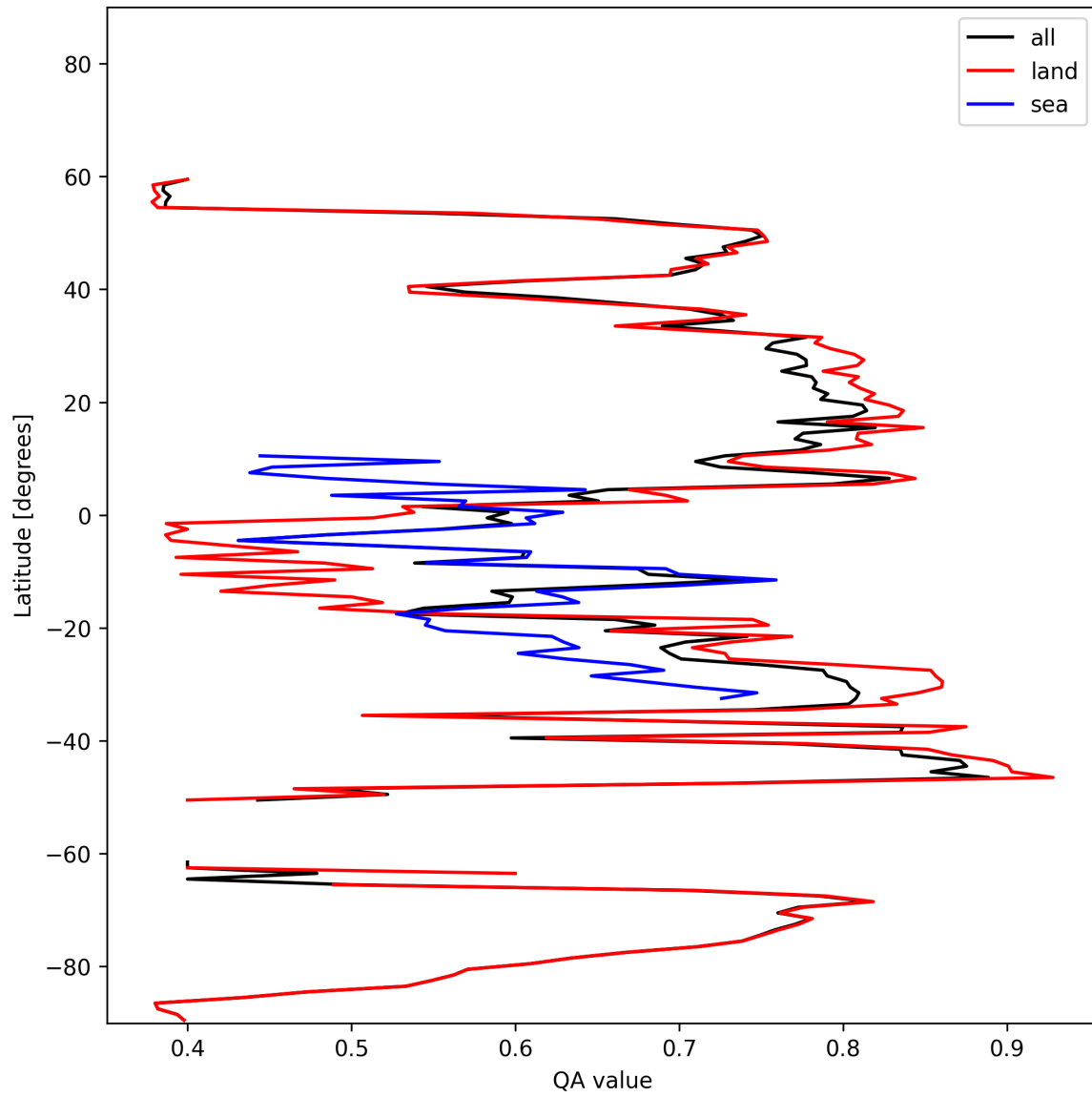
Figure 11: Zonal average of “QA value” for 2025-02-03 to 2025-02-05.
