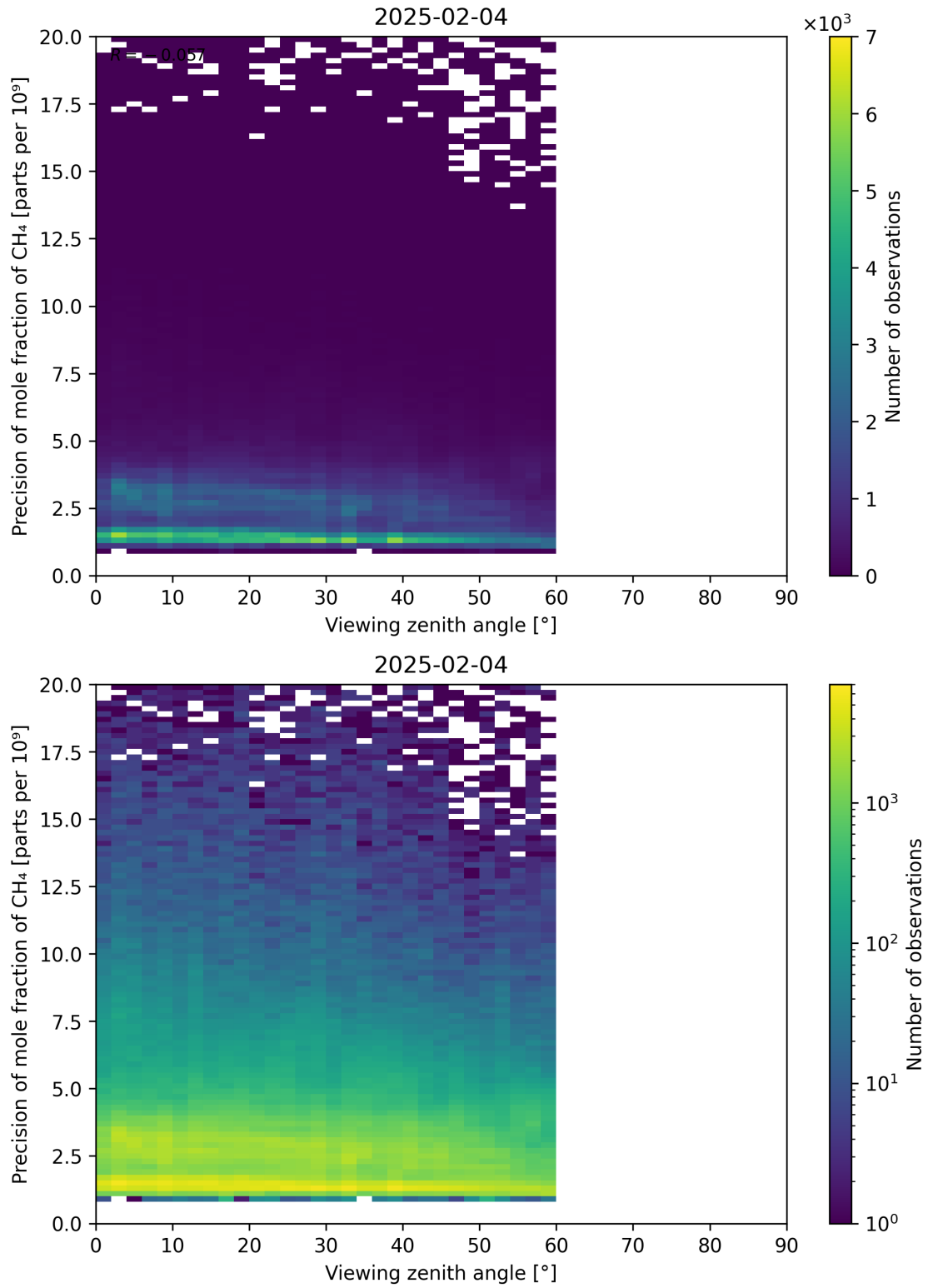
Figure 112: Scatter density plot of “Viewing zenith angle” against “Precision of mole fraction of CH 4 ” for 2025-02-03 to 2025-02-05.
