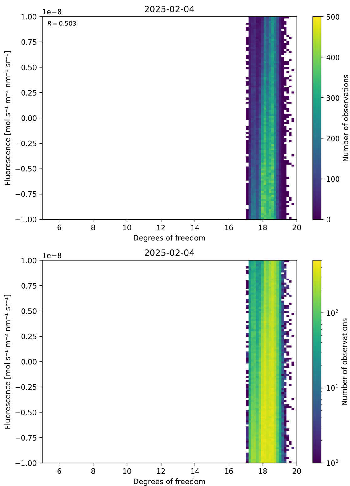
Figure 51: Scatter density plot of “Degrees of freedom” against “Fluorescence” for 2025-02-03 to 2025-02-05.
