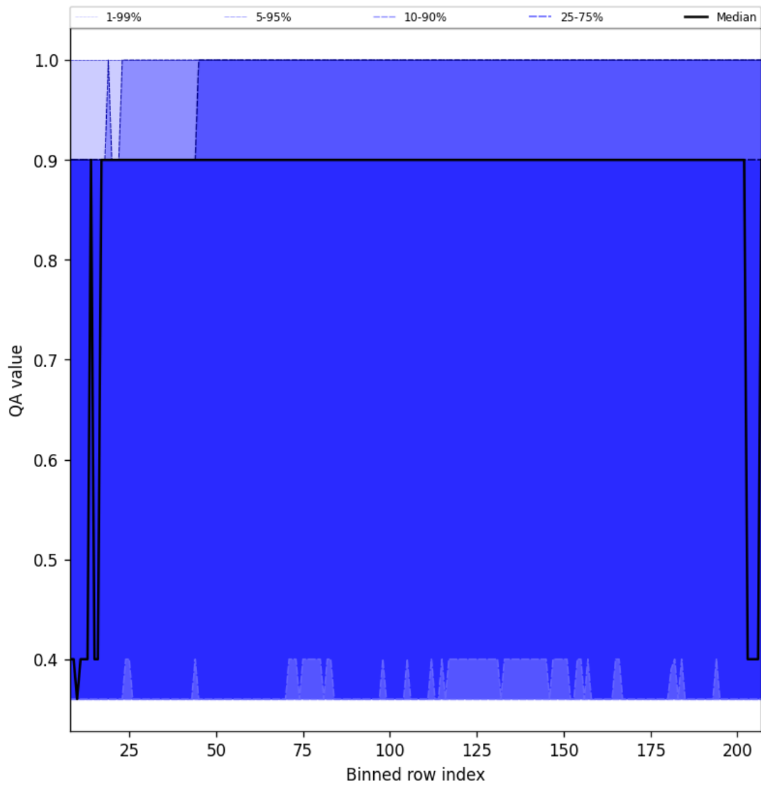
Figure 33: Along track statistics of “QA value” for 2025-02-03 to 2025-02-05
