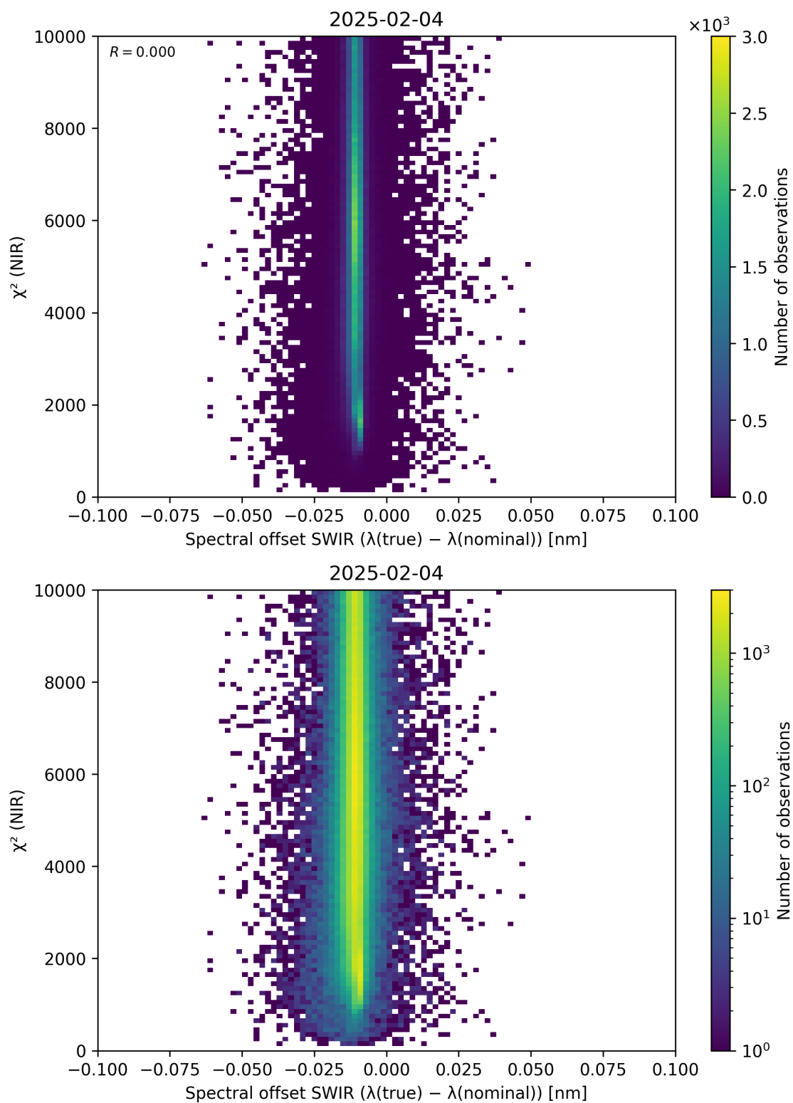
Figure 117: Scatter density plot of “Spectral offset SWIR ( \lambda_{\text{true}} - \lambda_{\text{nominal}} )” against “ \chi^2 (NIR)” for 2025-02-03 to 2025-02-05.
