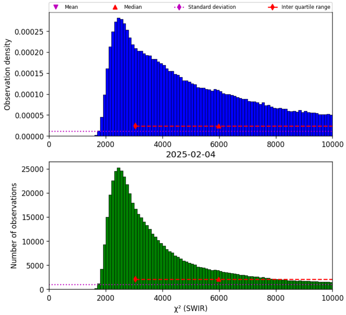
Figure 28: Histogram of “ \chi^2 (SWIR)” for 2025-02-03 to 2025-02-05
