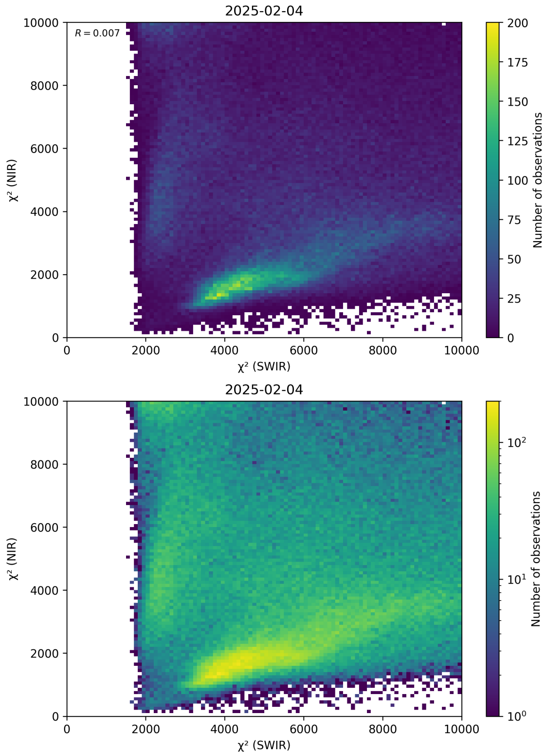
Figure 47: Scatter density plot of “ \chi^2 (SWIR)” against “ \chi^2 (NIR)” for 2025-02-03 to 2025-02-05.
