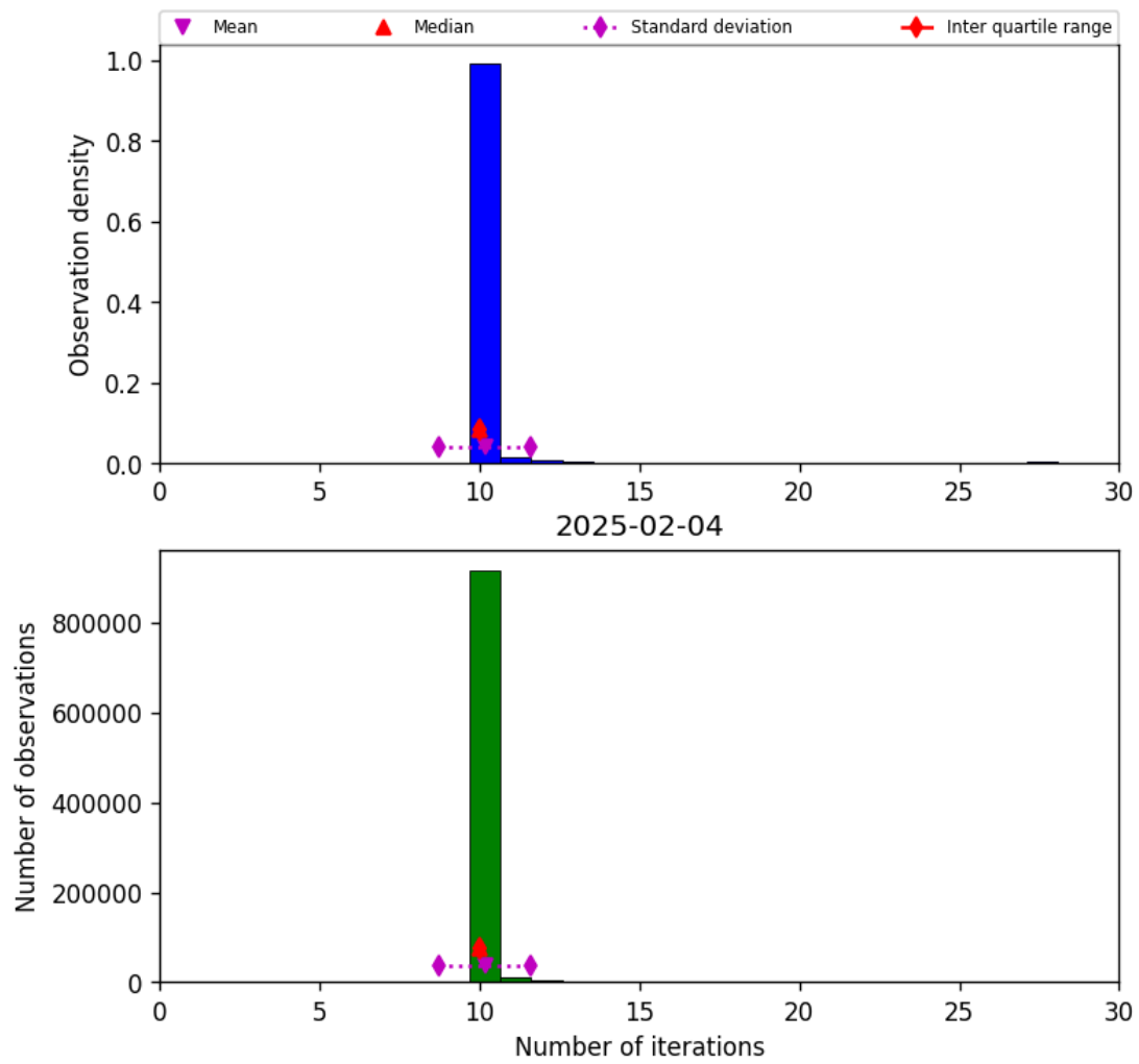
Figure 31: Histogram of “Number of iterations” for 2025-02-03 to 2025-02-05
