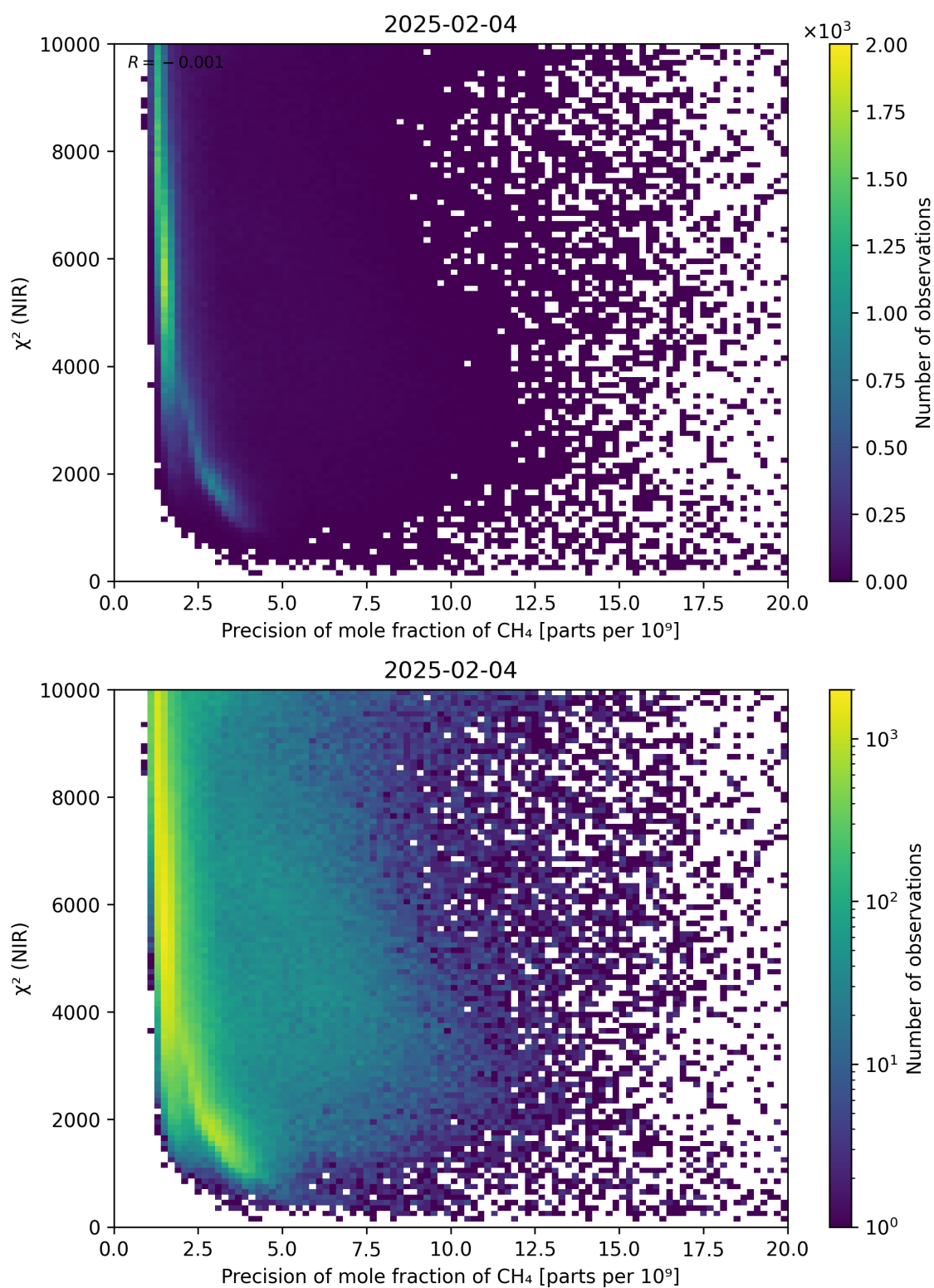
Figure 78: Scatter density plot of “Precision of mole fraction of \text{CH}_4 ” against “ \chi^2 (NIR)” for 2025-02-03 to 2025-02-05.
