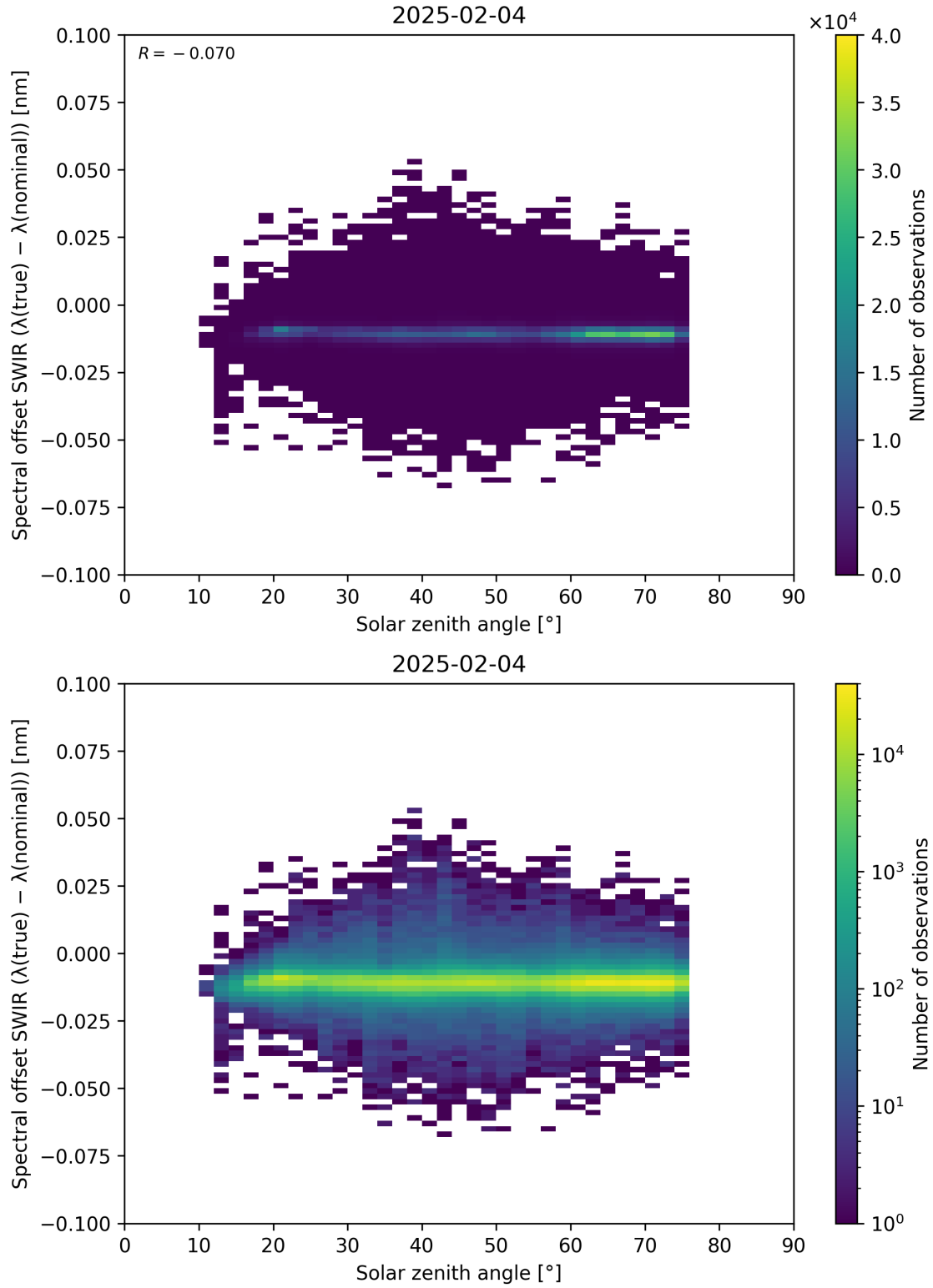
Figure 104: Scatter density plot of “Solar zenith angle” against “Spectral offset SWIR ( \lambda_{\text{true}} - \lambda_{\text{nominal}} )” for 2025-02-03 to 2025-02-05.
