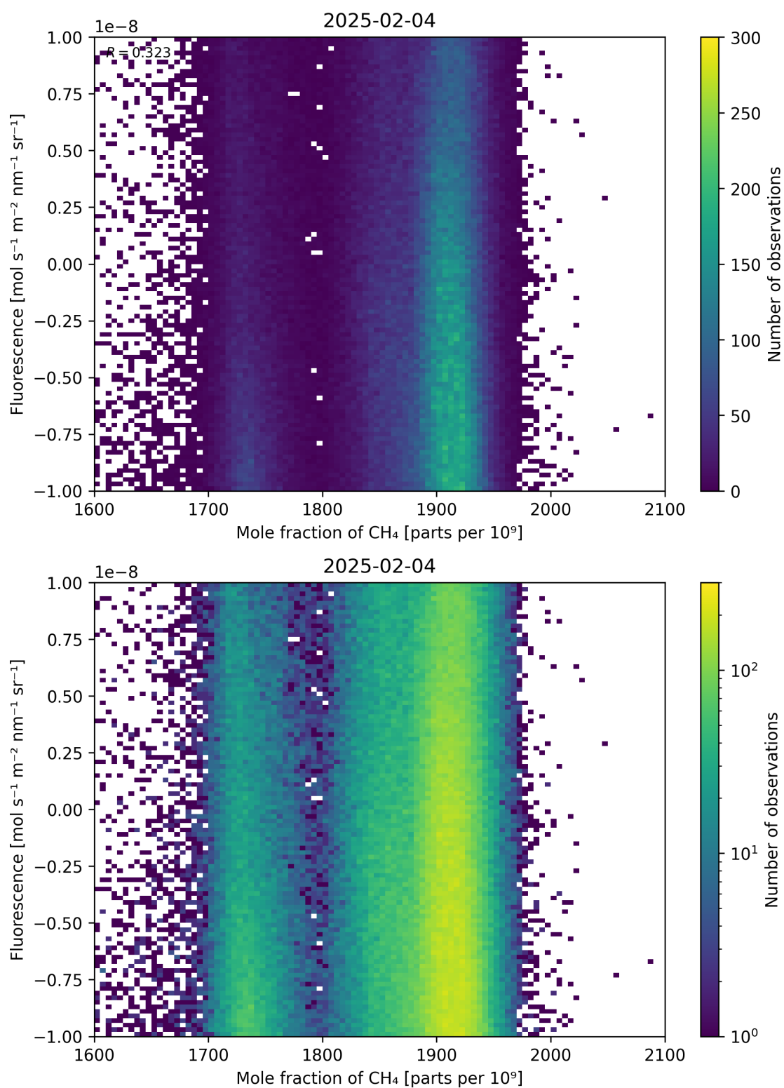
Figure 73: Scatter density plot of “Mole fraction of \text{CH}_4 ” against “Fluorescence” for 2025-02-03 to 2025-02-05.
