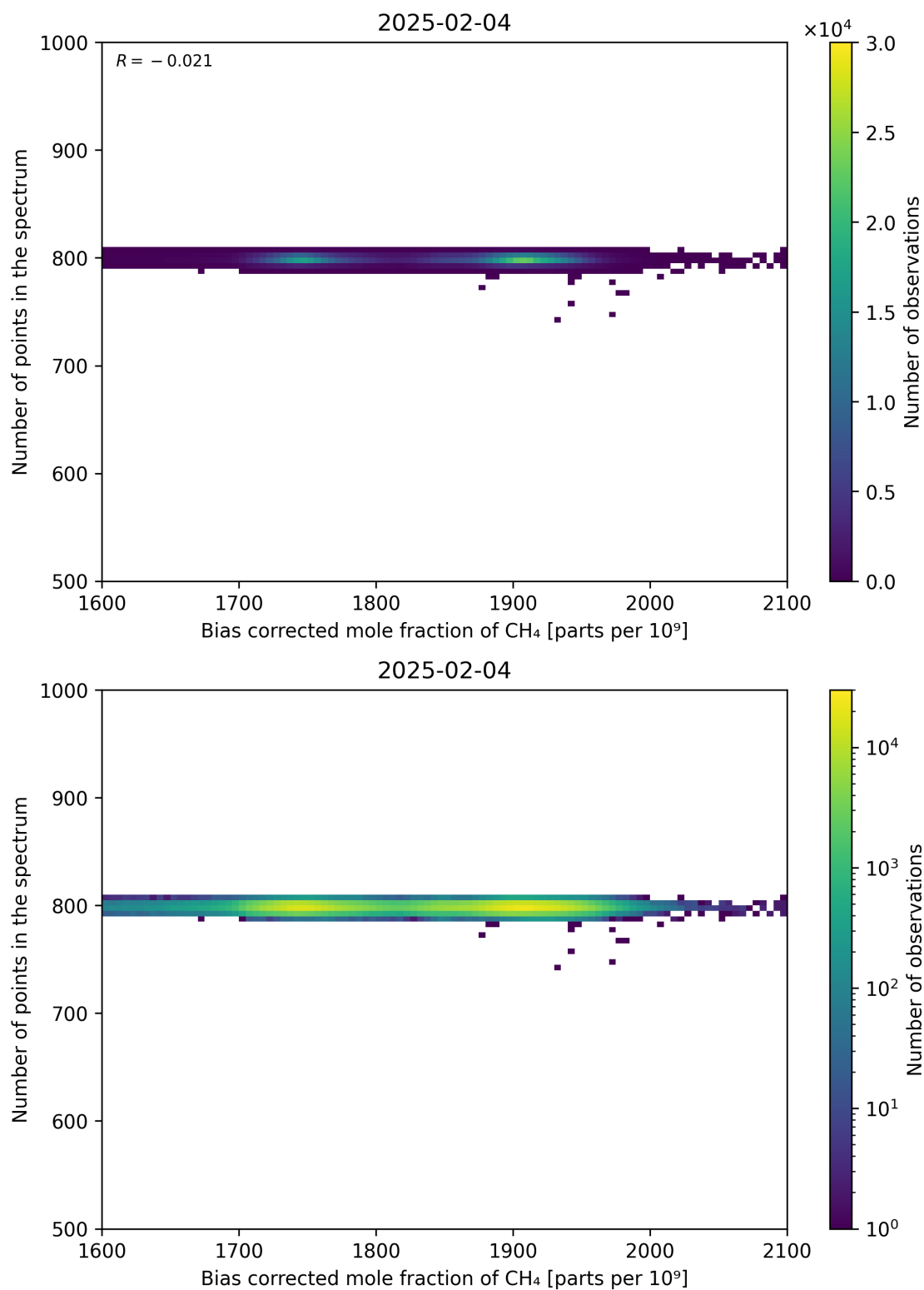
Figure 68: Scatter density plot of “Bias corrected mole fraction of CH 4 ” against “Number of points in the spectrum” for 2025-02-03 to 2025-02-05.
