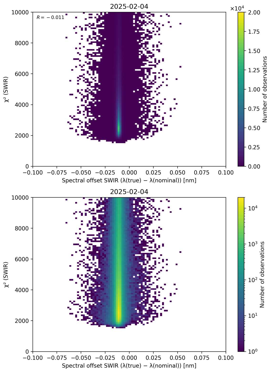
Figure 118: Scatter density plot of “Spectral offset SWIR ( \lambda_{\text{true}} - \lambda_{\text{nominal}} )” against “ \chi^2 (SWIR)” for 2025-02-03 to 2025-02-05.
