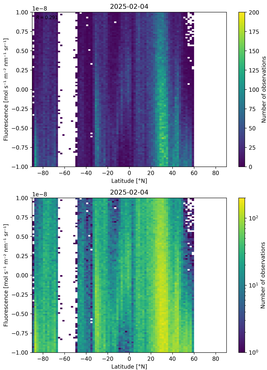
Figure 56: Scatter density plot of “Latitude” against “Fluorescence” for 2025-02-03 to 2025-02-05.
