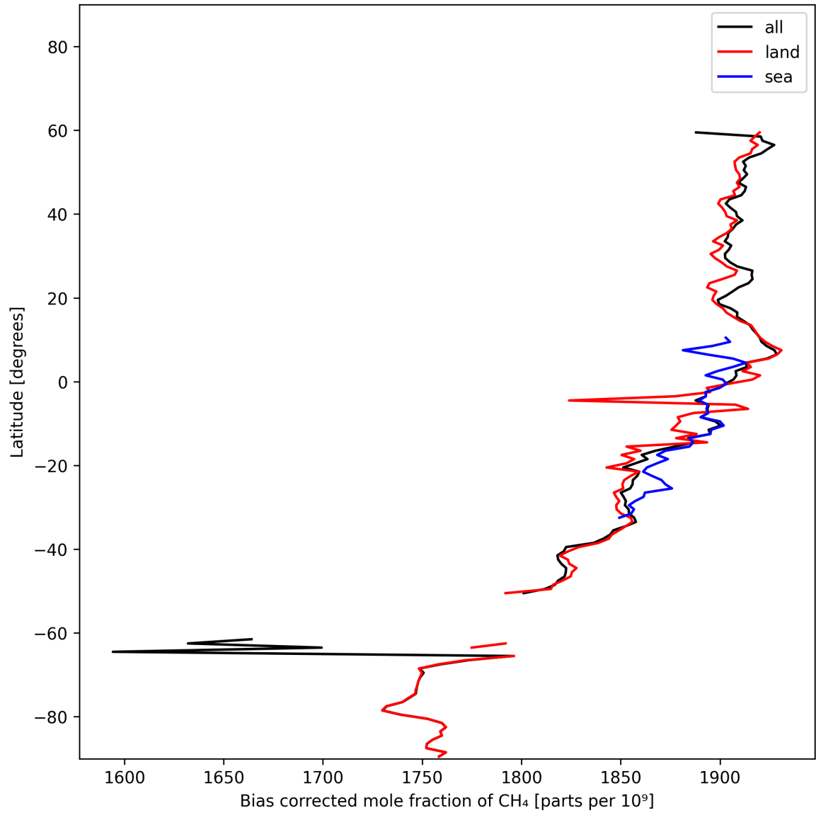
Figure 14: Zonal average of “Bias corrected mole fraction of CH 4 ” for 2025-02-03 to 2025-02-05.
