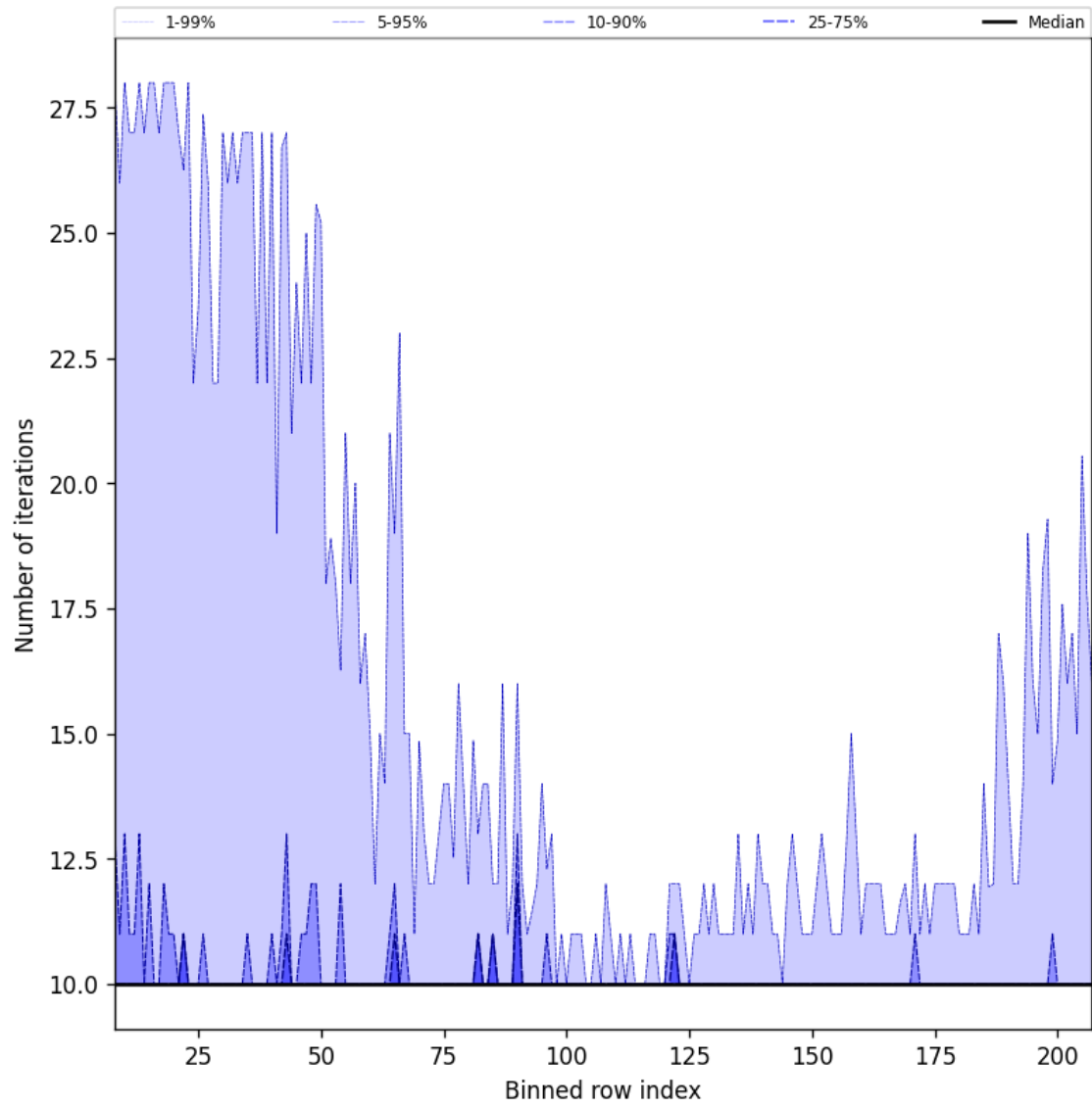
Figure 42: Along track statistics of “Number of iterations” for 2025-02-03 to 2025-02-05
