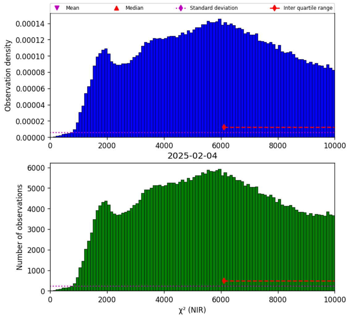
Figure 29: Histogram of " \chi^2 (NIR)" for 2025-02-03 to 2025-02-05
