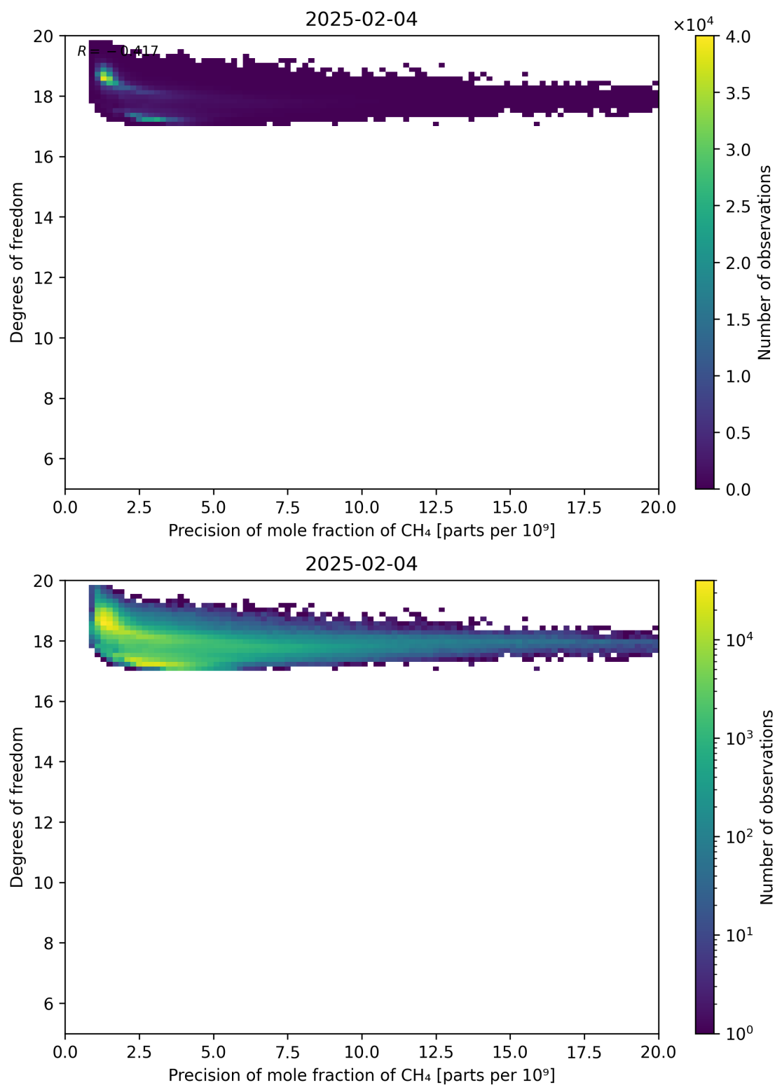
Figure 80: Scatter density plot of “Precision of mole fraction of CH 4 ” against “Degrees of freedom” for 2025-02-03 to 2025-02-05.
