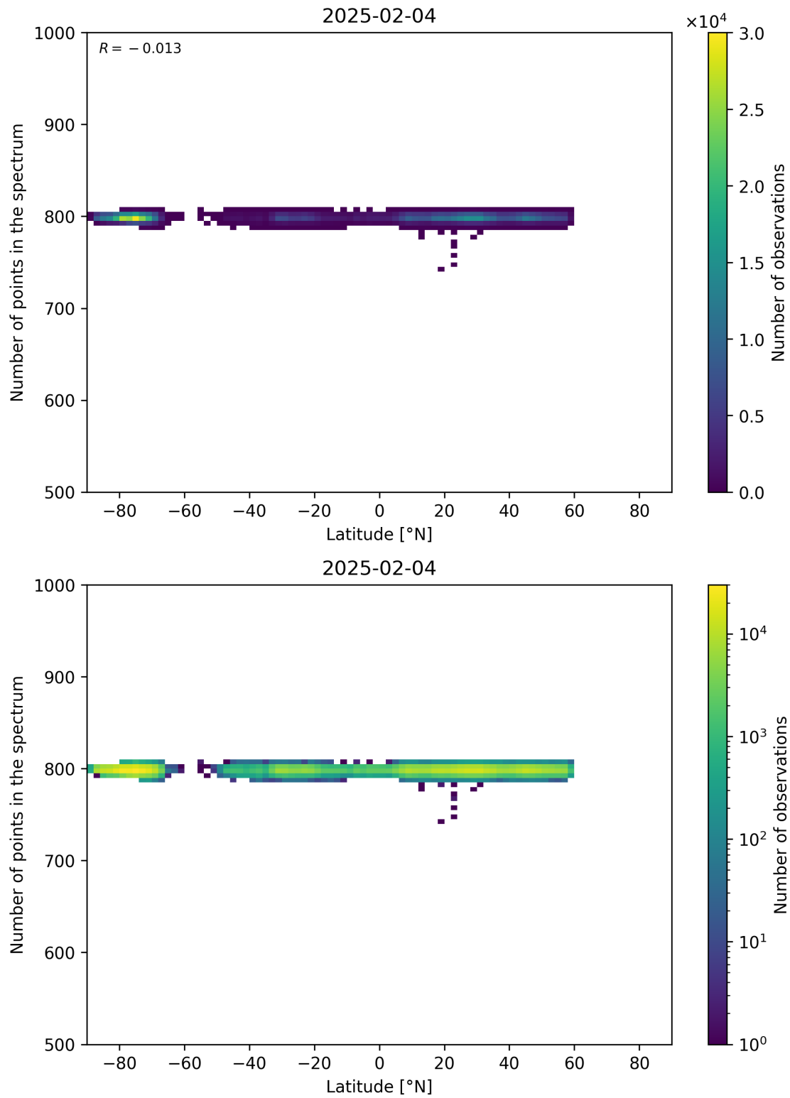
Figure 61: Scatter density plot of “Latitude” against “Number of points in the spectrum” for 2025-02-03 to 2025-02-05.
