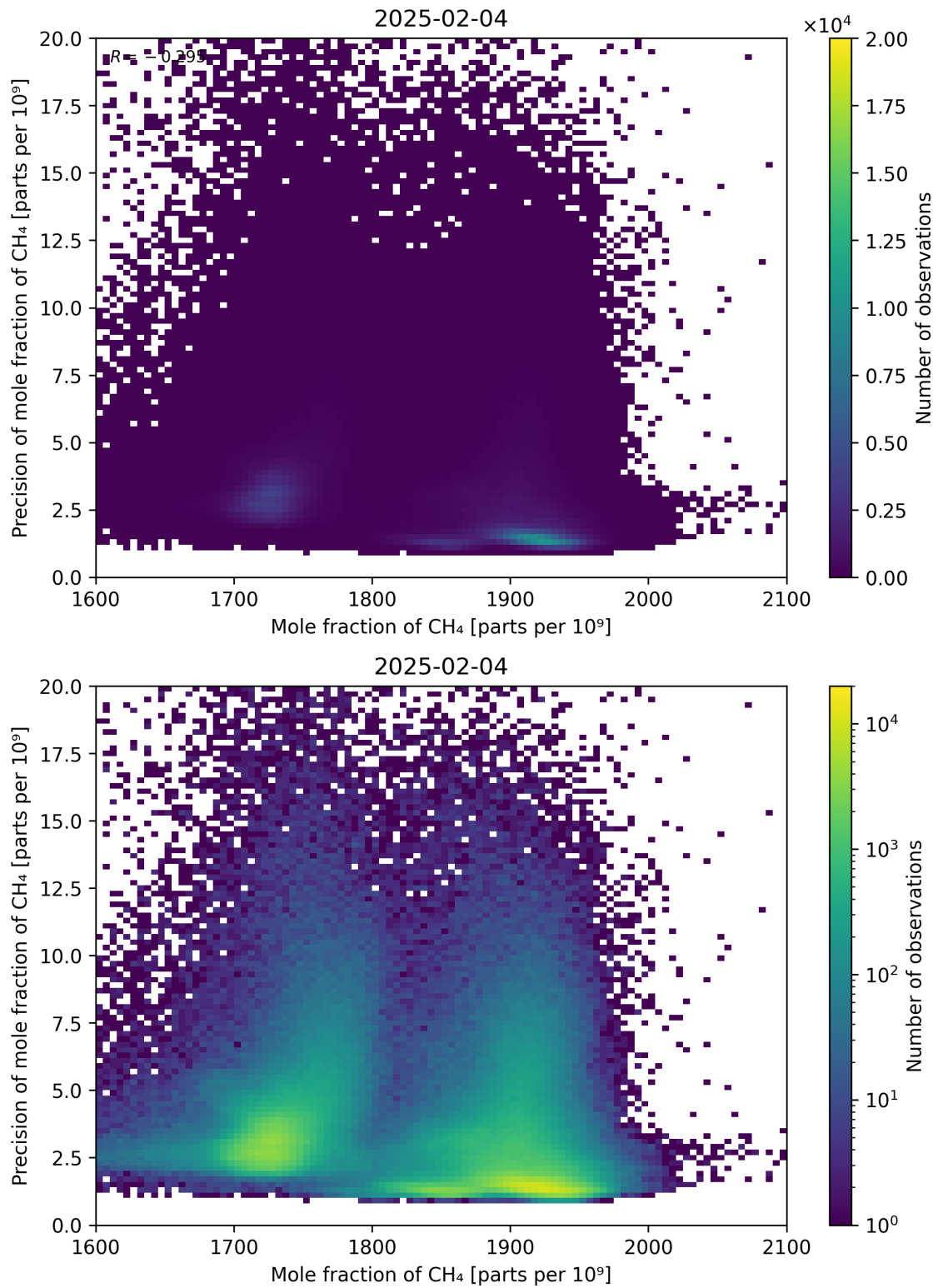
Figure 75: Scatter density plot of “Mole fraction of CH 4 ” against “Precision of mole fraction of CH 4 ” for 2025-02-03 to 2025-02-05.
