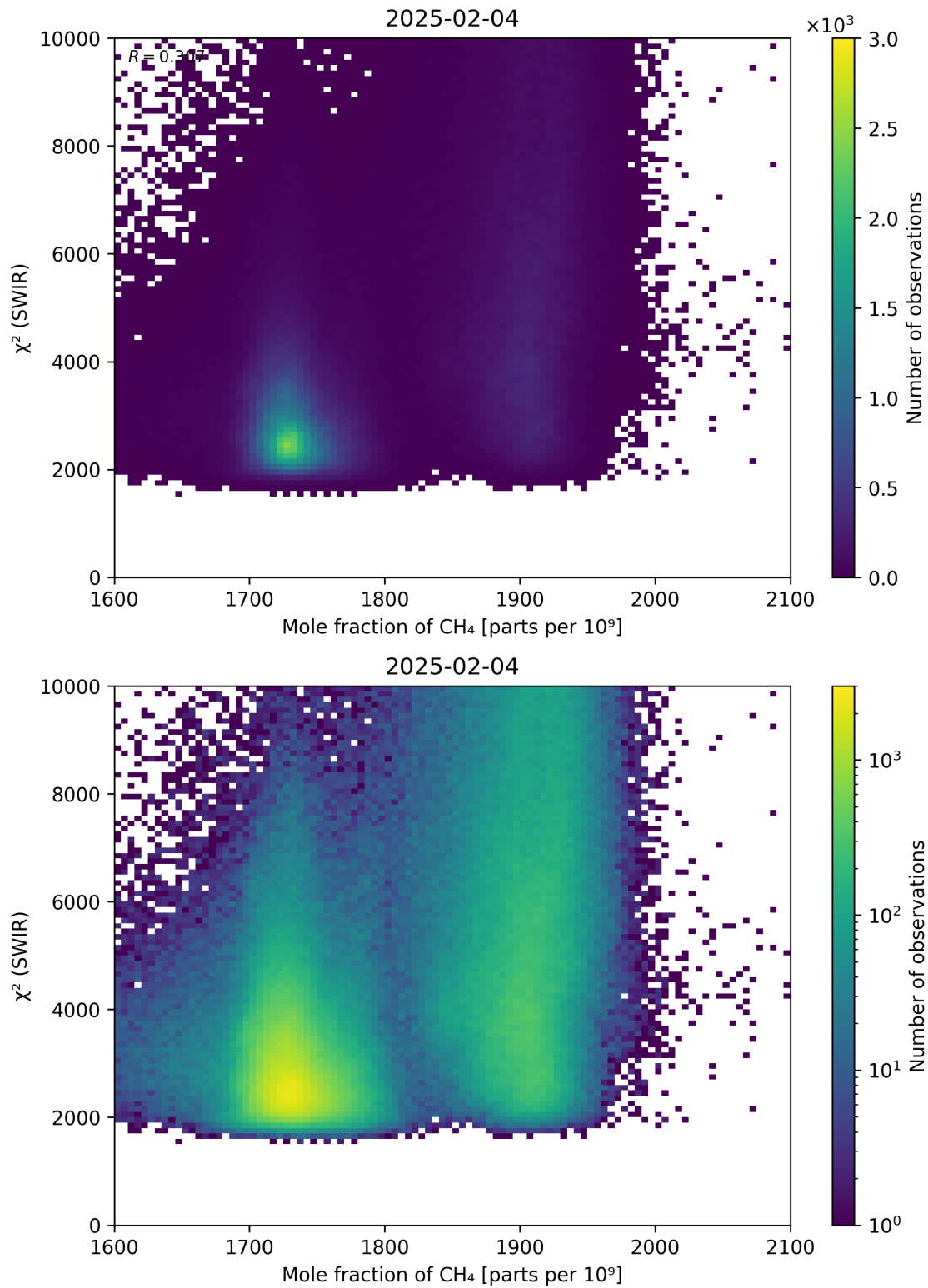
Figure 71: Scatter density plot of “Mole fraction of \text{CH}_4 ” against “ \chi^2 (SWIR)” for 2025-02-03 to 2025-02-05.
