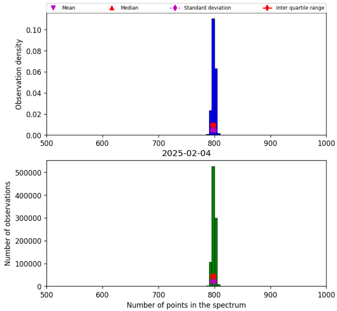
Figure 26: Histogram of “Number of points in the spectrum” for 2025-02-03 to 2025-02-05
