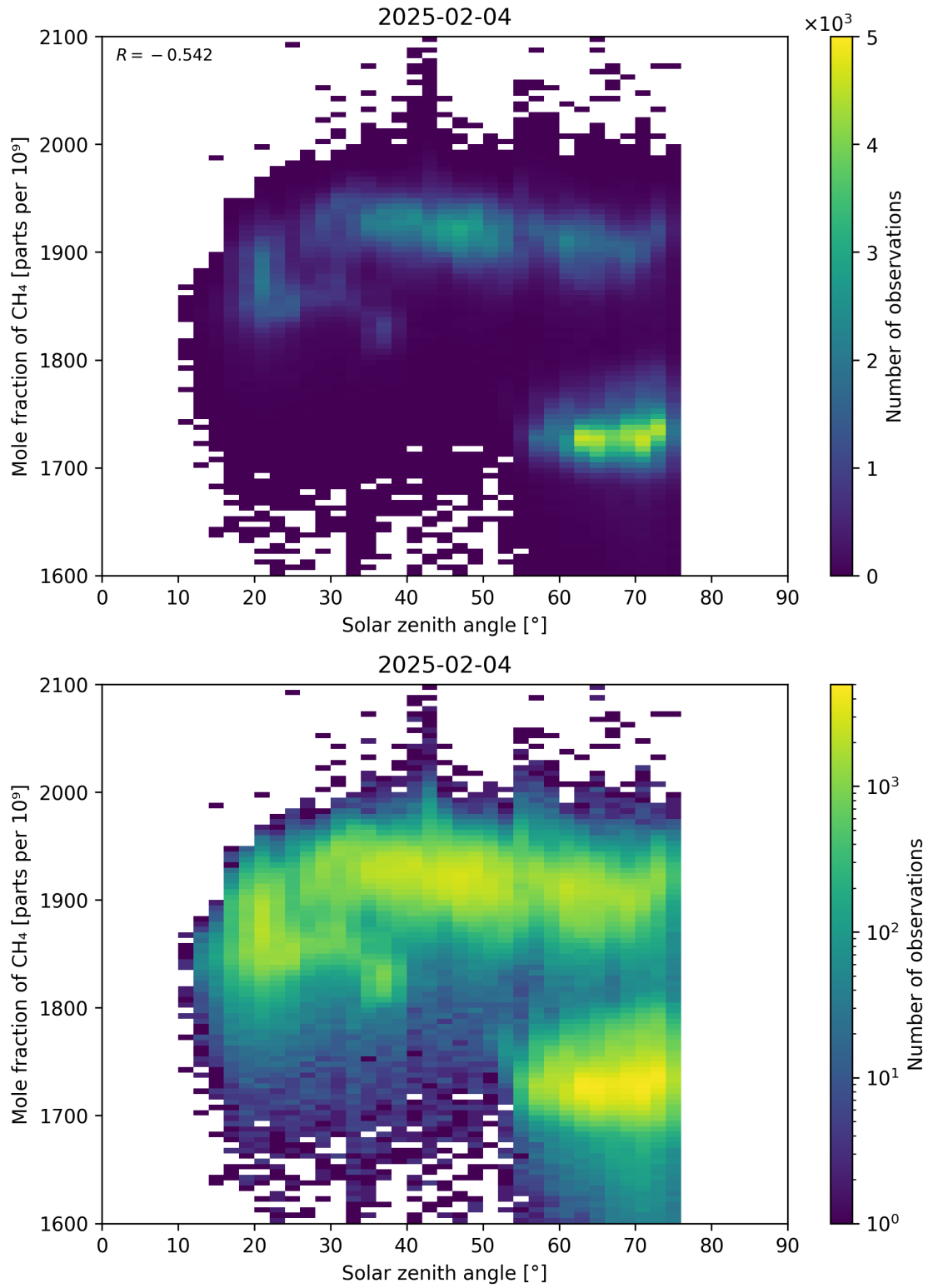
Figure 99: Scatter density plot of “Solar zenith angle” against “Mole fraction of CH 4 ” for 2025-02-03 to 2025-02-05.
