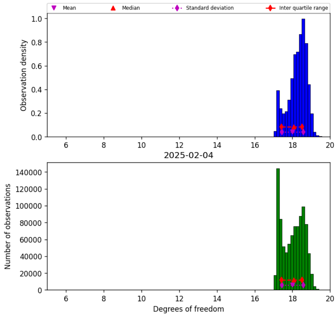
Figure 30: Histogram of “Degrees of freedom” for 2025-02-03 to 2025-02-05
