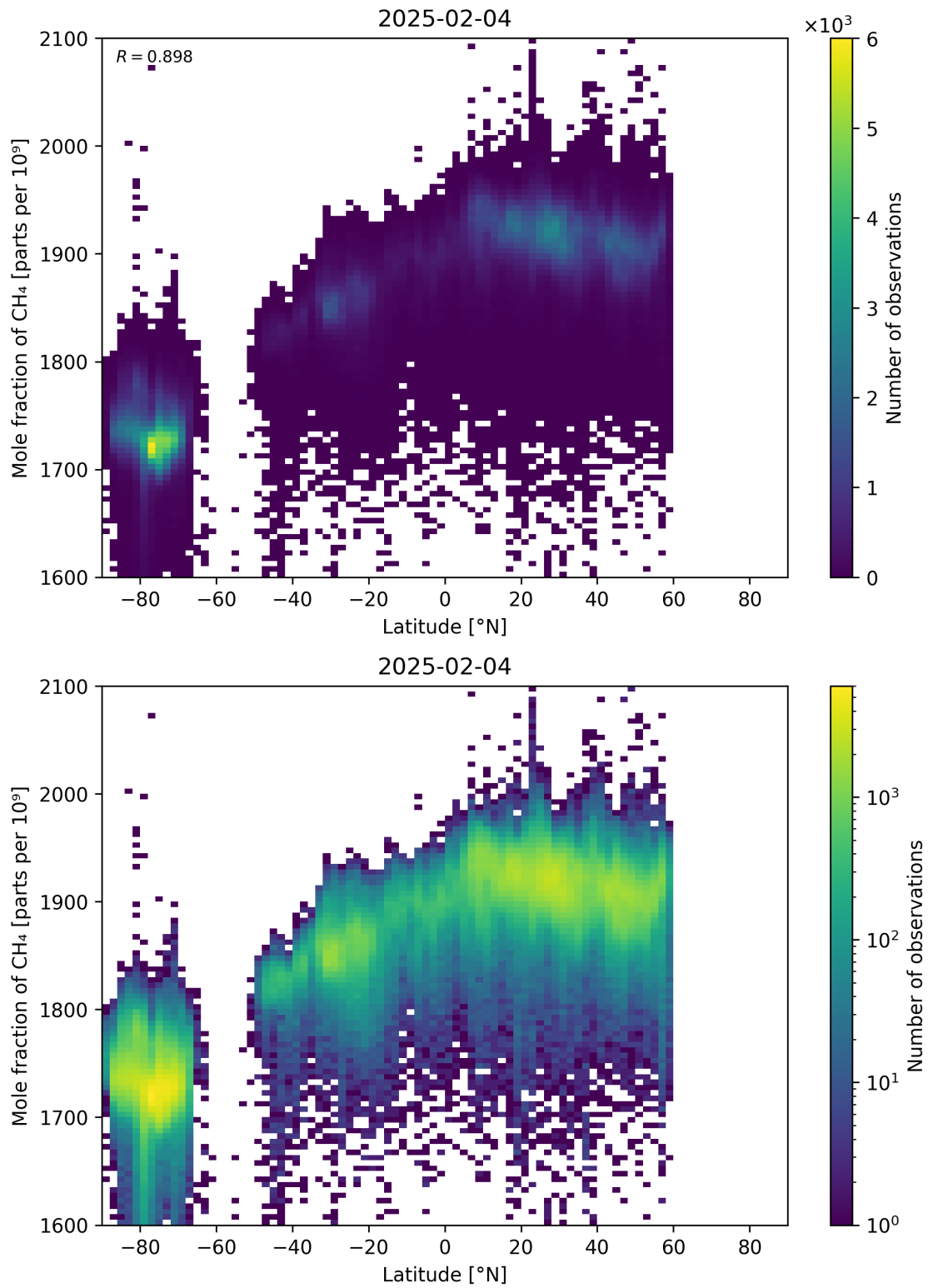
Figure 57: Scatter density plot of “Latitude” against “Mole fraction of CH 4 ” for 2025-02-03 to 2025-02-05.
