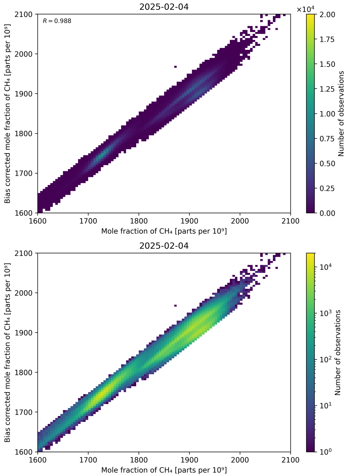
Figure 74: Scatter density plot of “Mole fraction of CH 4 ” against “Bias corrected mole fraction of CH 4 ” for 2025-02-03 to 2025-02-05.
