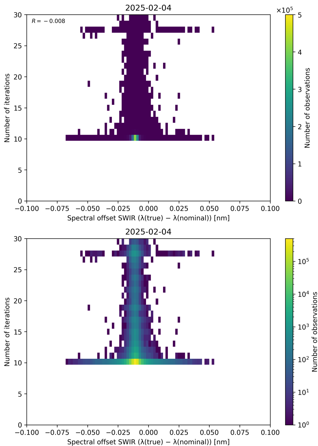
Figure 121: Scatter density plot of “Spectral offset SWIR ( \lambda_{\text{true}} - \lambda_{\text{nominal}} )” against “Number of iterations” for 2025-02-03 to 2025-02-05.
