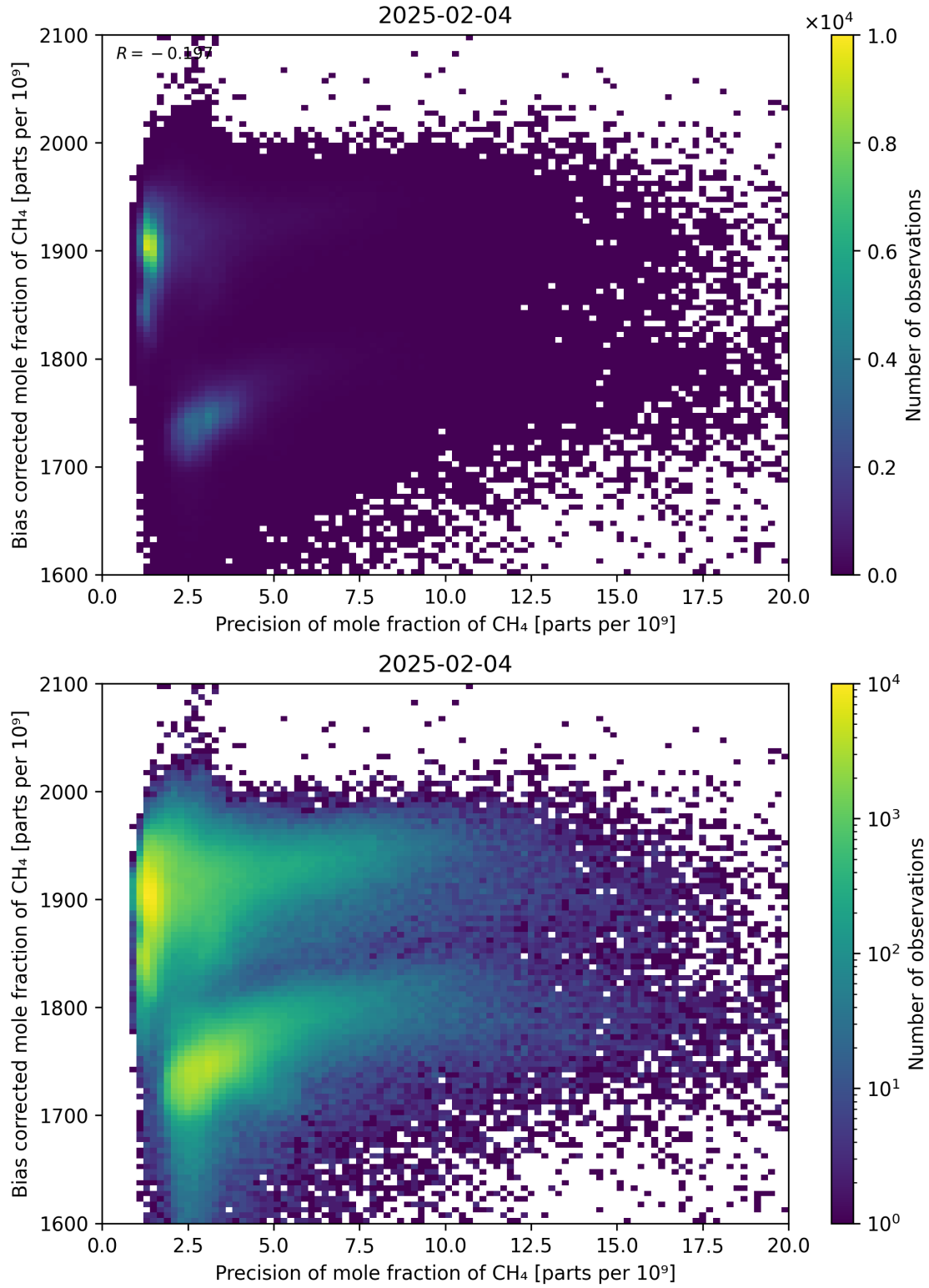
Figure 82: Scatter density plot of “Precision of mole fraction of CH 4 ” against “Bias corrected mole fraction of CH 4 ” for 2025-02-03 to 2025-02-05.
