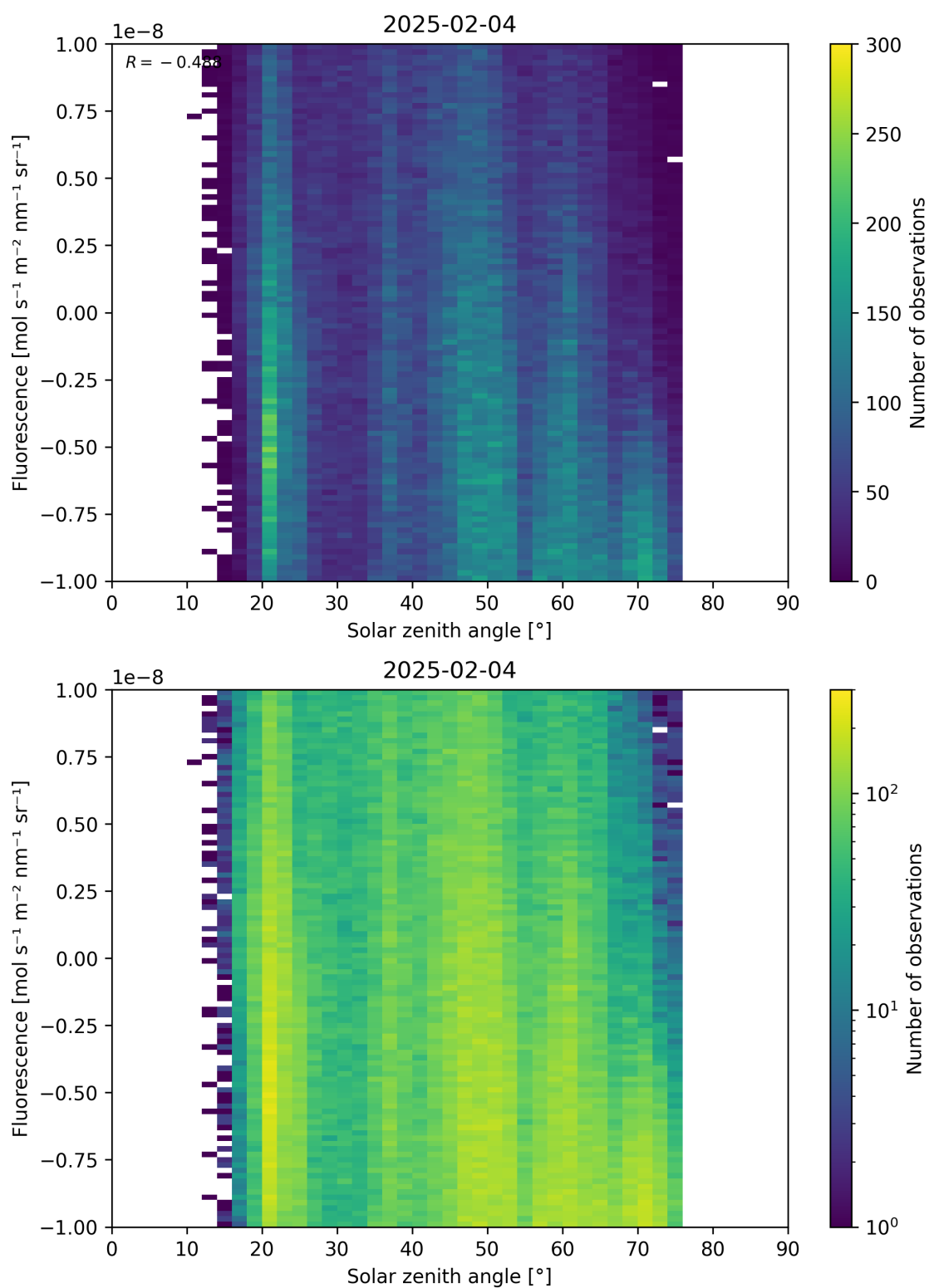
Figure 97: Scatter density plot of “Solar zenith angle” against “Fluorescence” for 2025-02-03 to 2025-02-05.
