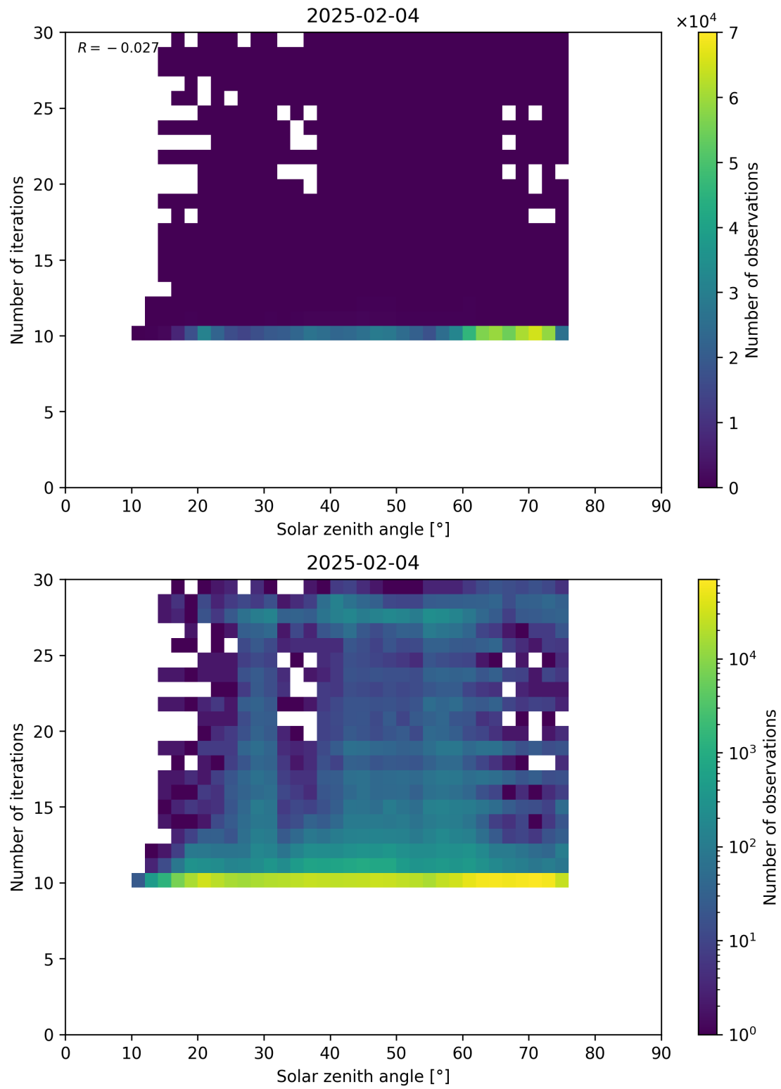
Figure 102: Scatter density plot of “Solar zenith angle” against “Number of iterations” for 2025-02-03 to 2025-02-05.
