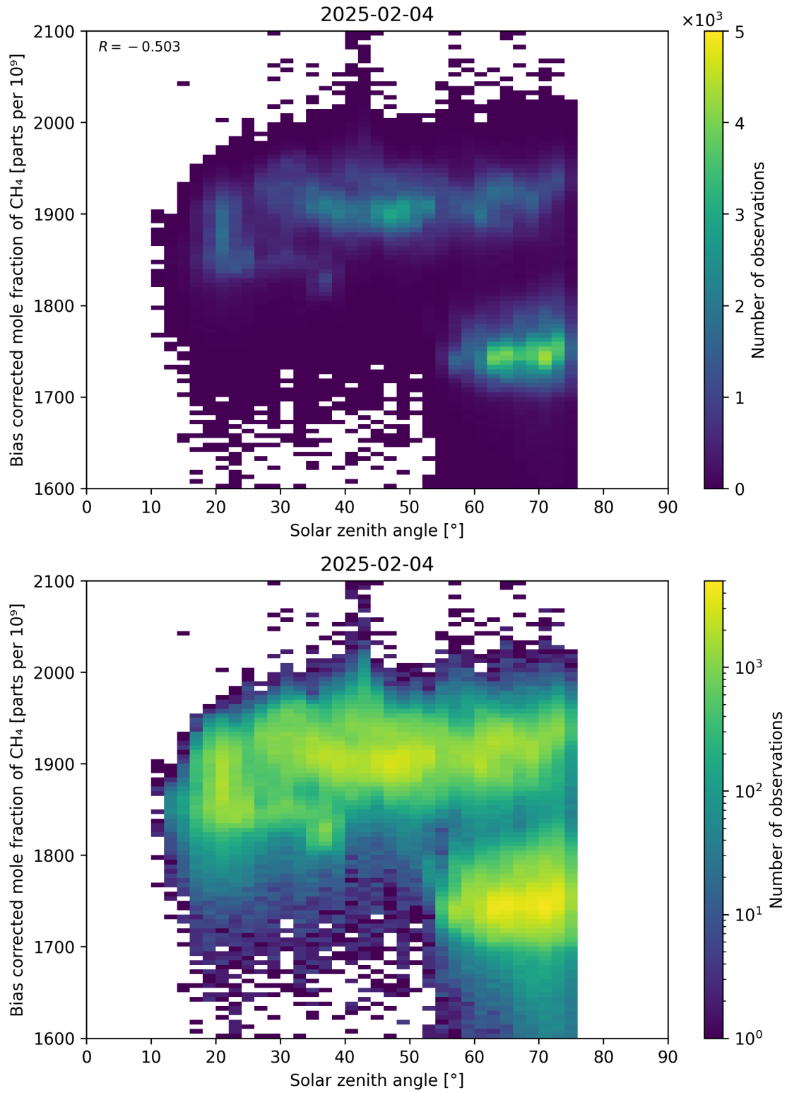
Figure 100: Scatter density plot of “Solar zenith angle” against “Bias corrected mole fraction of CH 4 ” for 2025-02-03 to 2025-02-05.
