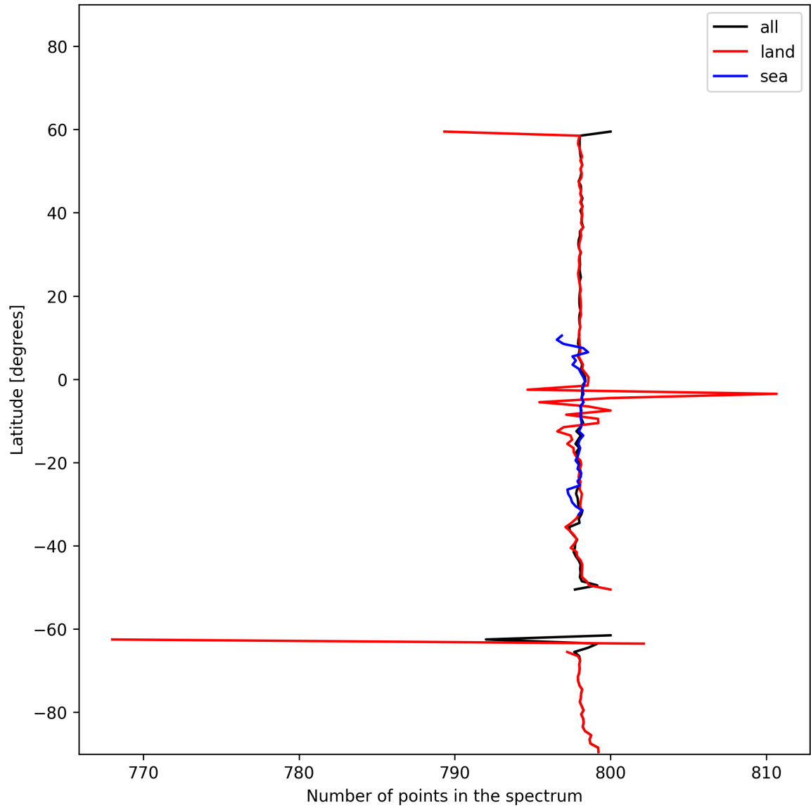
Figure 15: Zonal average of “Number of points in the spectrum” for 2025-02-03 to 2025-02-05.
