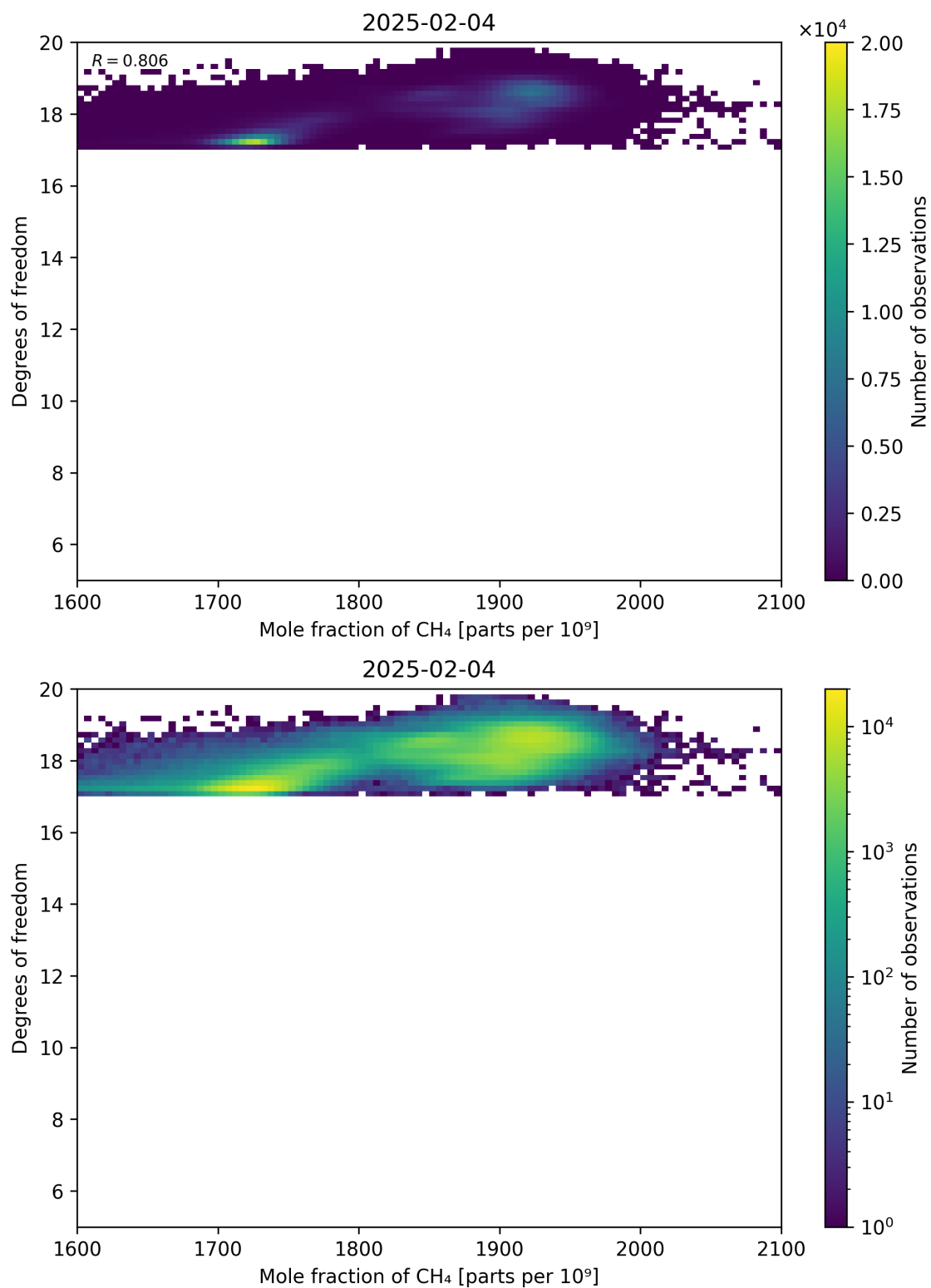
Figure 72: Scatter density plot of “Mole fraction of CH 4 ” against “Degrees of freedom” for 2025-02-03 to 2025-02-05.
