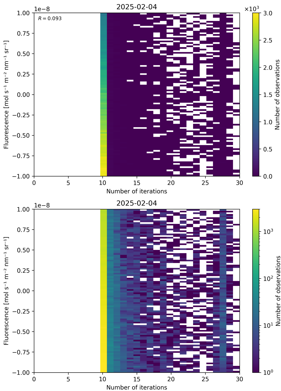
Figure 87: Scatter density plot of “Number of iterations” against “Fluorescence” for 2025-02-03 to 2025-02-05.
