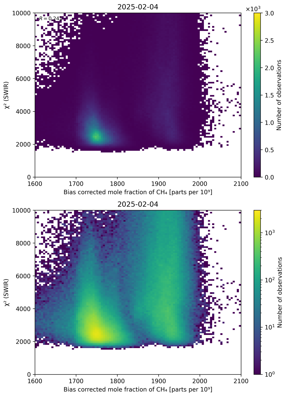
Figure 64: Scatter density plot of “Bias corrected mole fraction of \text{CH}_4 ” against “ \chi^2 (SWIR)” for 2025-02-03 to 2025-02-05.
