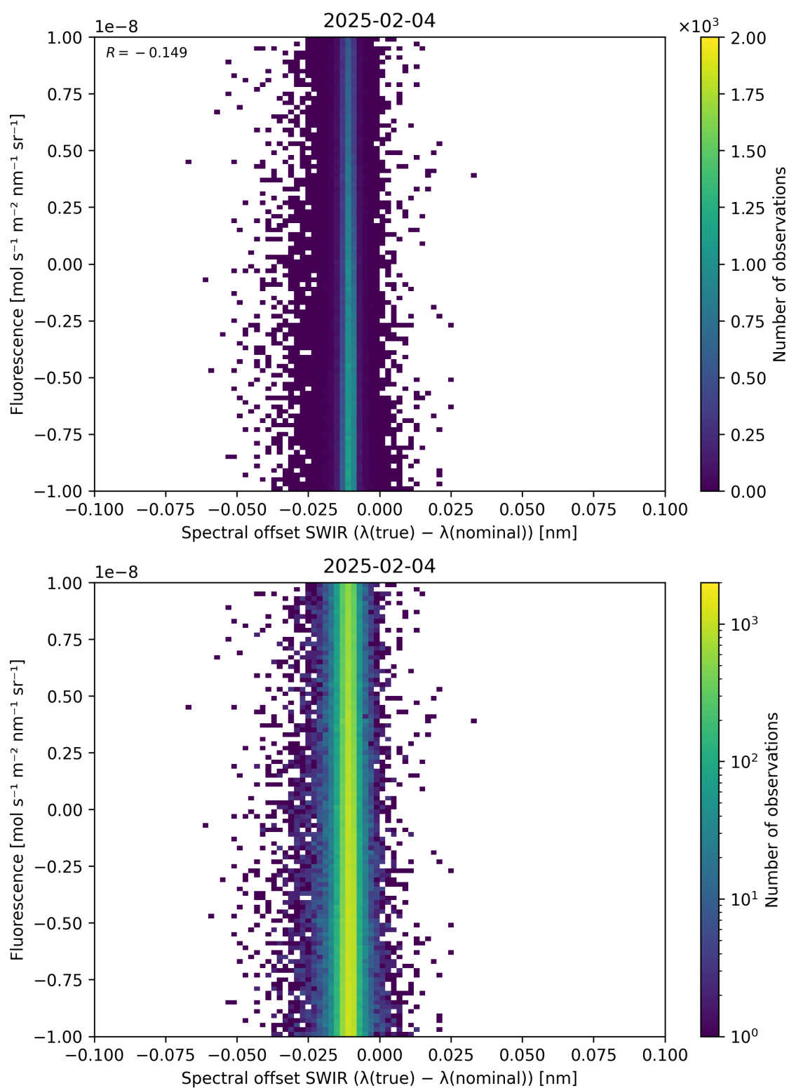
Figure 120: Scatter density plot of “Spectral offset SWIR ( \lambda_{\text{true}} - \lambda_{\text{nominal}} )” against “Fluorescence” for 2025-02-03 to 2025-02-05.
