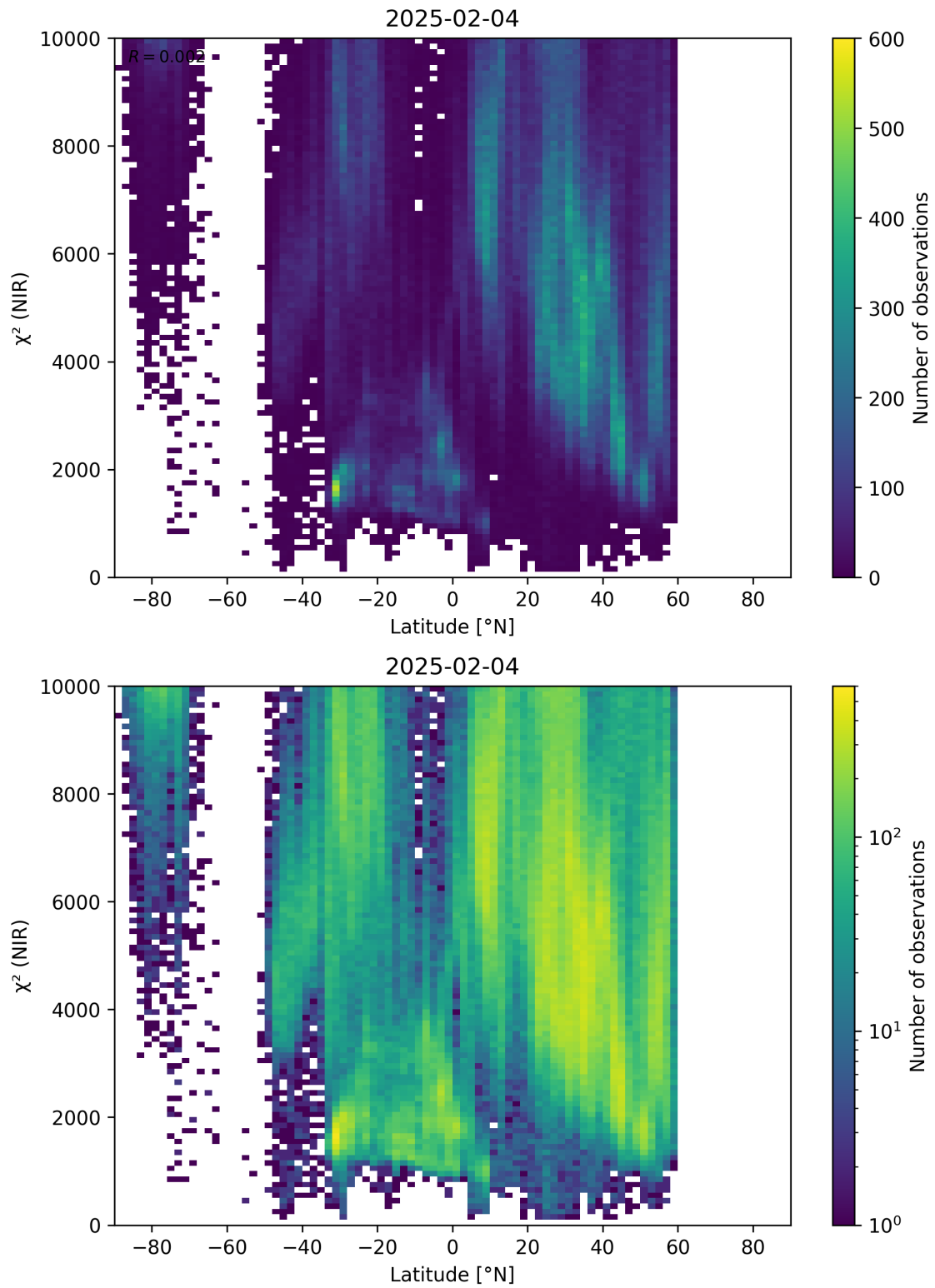
Figure 53: Scatter density plot of “Latitude” against “ \chi^2 (NIR)” for 2025-02-03 to 2025-02-05.
