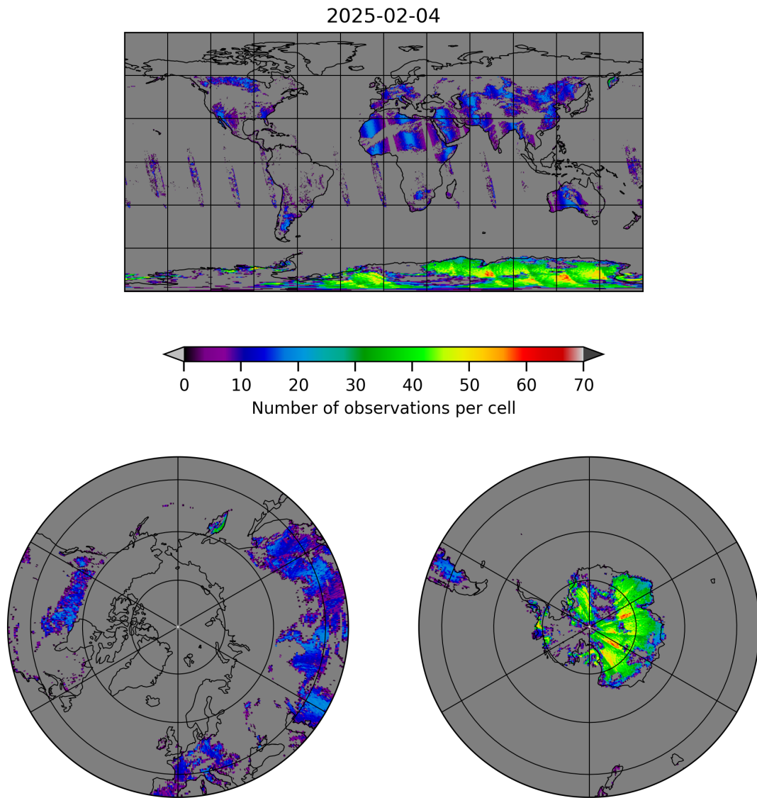
Figure 10: Map of the number of observations for 2025-02-03 to 2025-02-05
