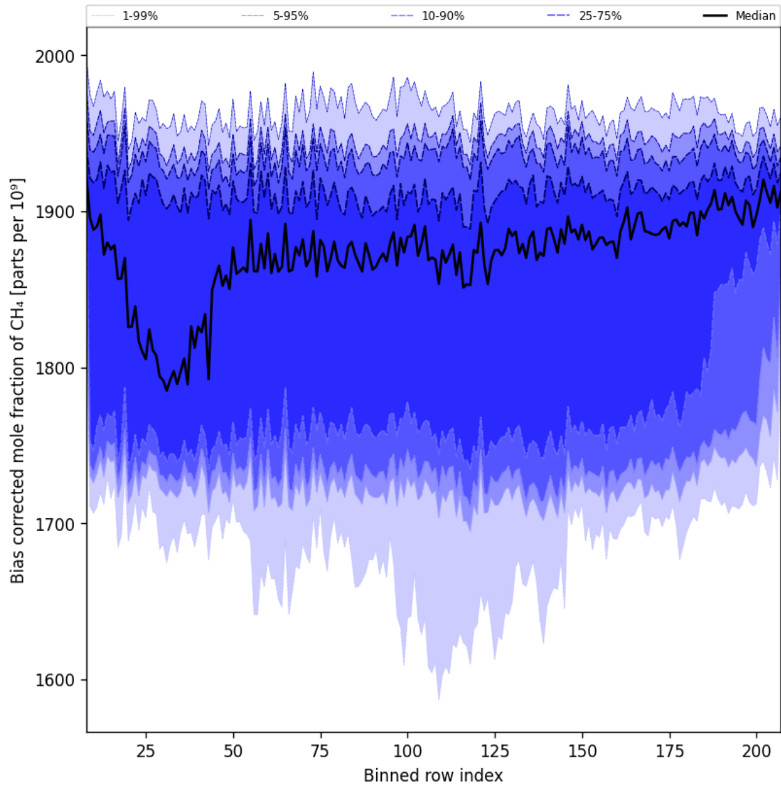
Figure 36: Along track statistics of “Bias corrected mole fraction of CH 4 ” for 2025-02-03 to 2025-02-05
