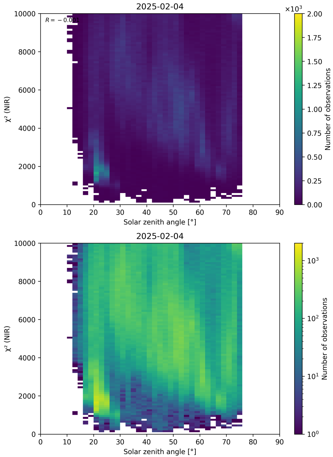
Figure 94: Scatter density plot of “Solar zenith angle” against “ \chi^2 (NIR)” for 2025-02-03 to 2025-02-05.
