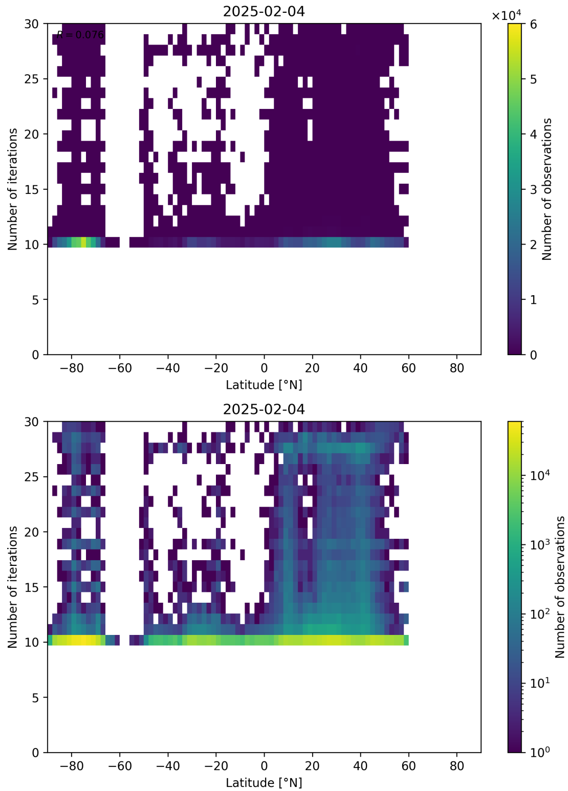
Figure 60: Scatter density plot of “Latitude” against “Number of iterations” for 2025-02-03 to 2025-02-05.
