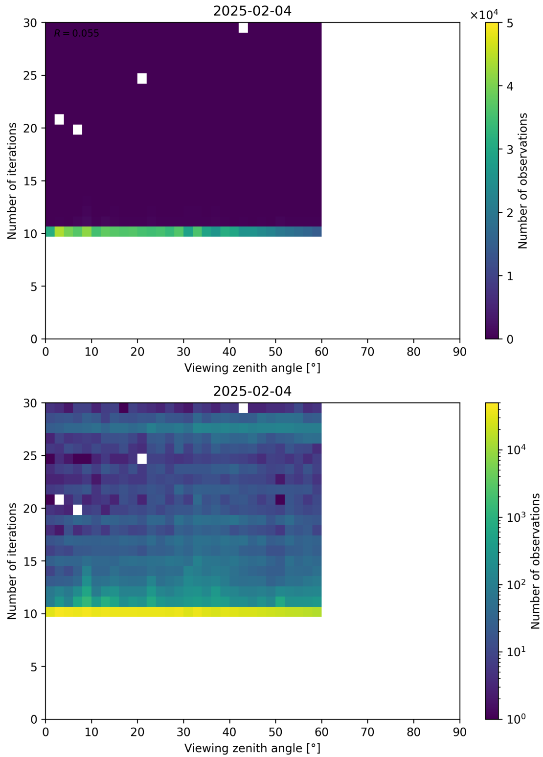
Figure 113: Scatter density plot of “Viewing zenith angle” against “Number of iterations” for 2025-02-03 to 2025-02-05.
