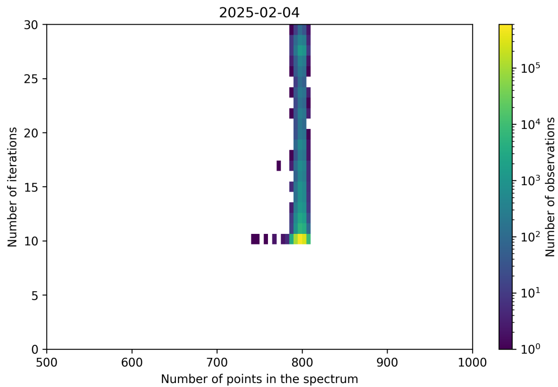
Figure 92: Scatter density plot of “Number of points in the spectrum” against “Number of iterations” for 2025-02-03 to 2025-02-05.
