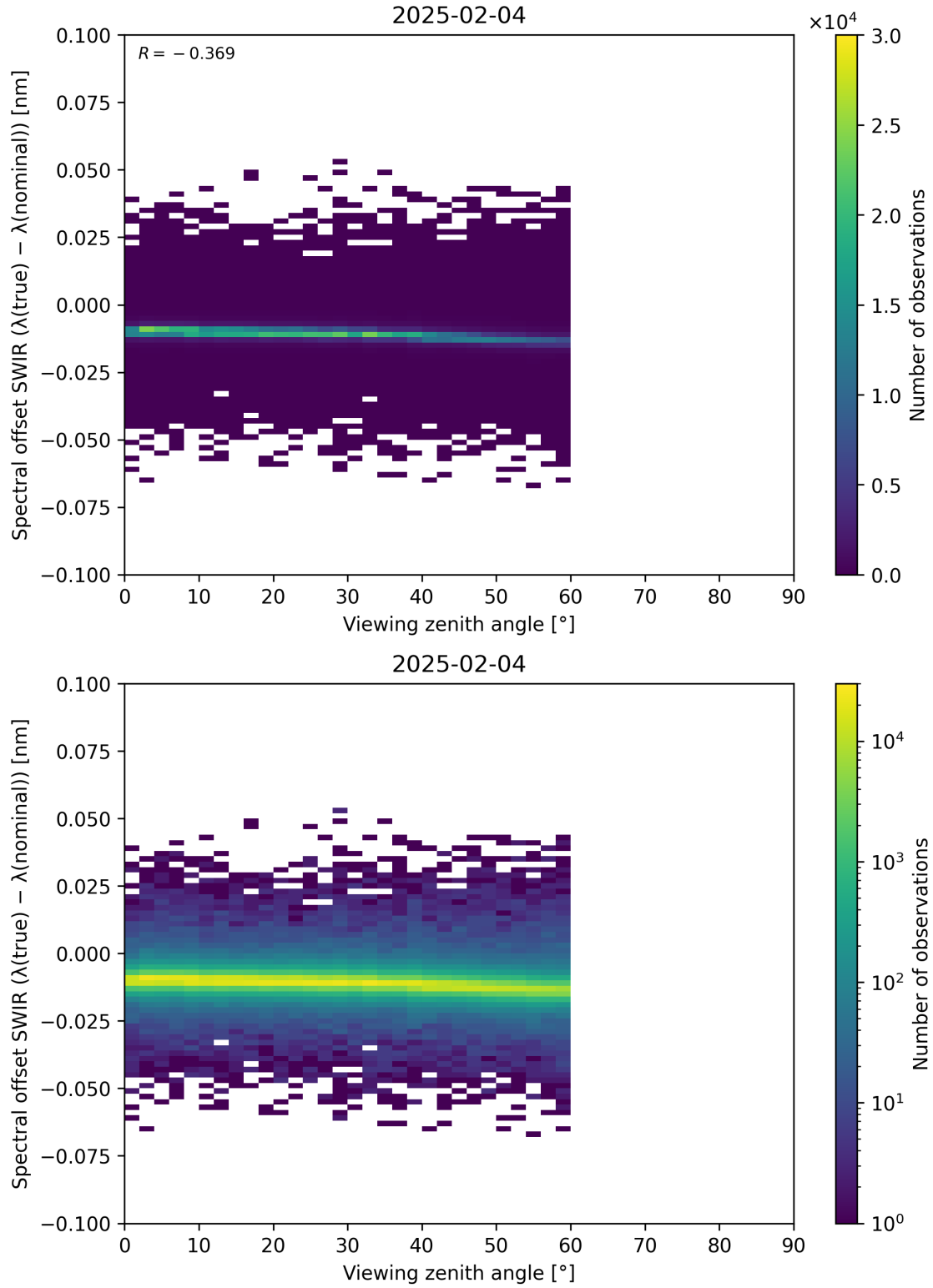
Figure 116: Scatter density plot of “Viewing zenith angle” against “Spectral offset SWIR ( \lambda_{\text{true}} - \lambda_{\text{nominal}} )” for 2025-02-03 to 2025-02-05.
