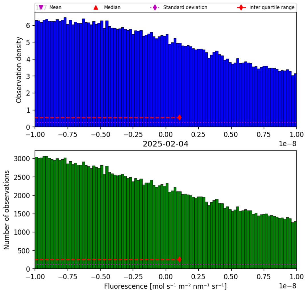
Figure 32: Histogram of “Fluorescence” for 2025-02-03 to 2025-02-05
