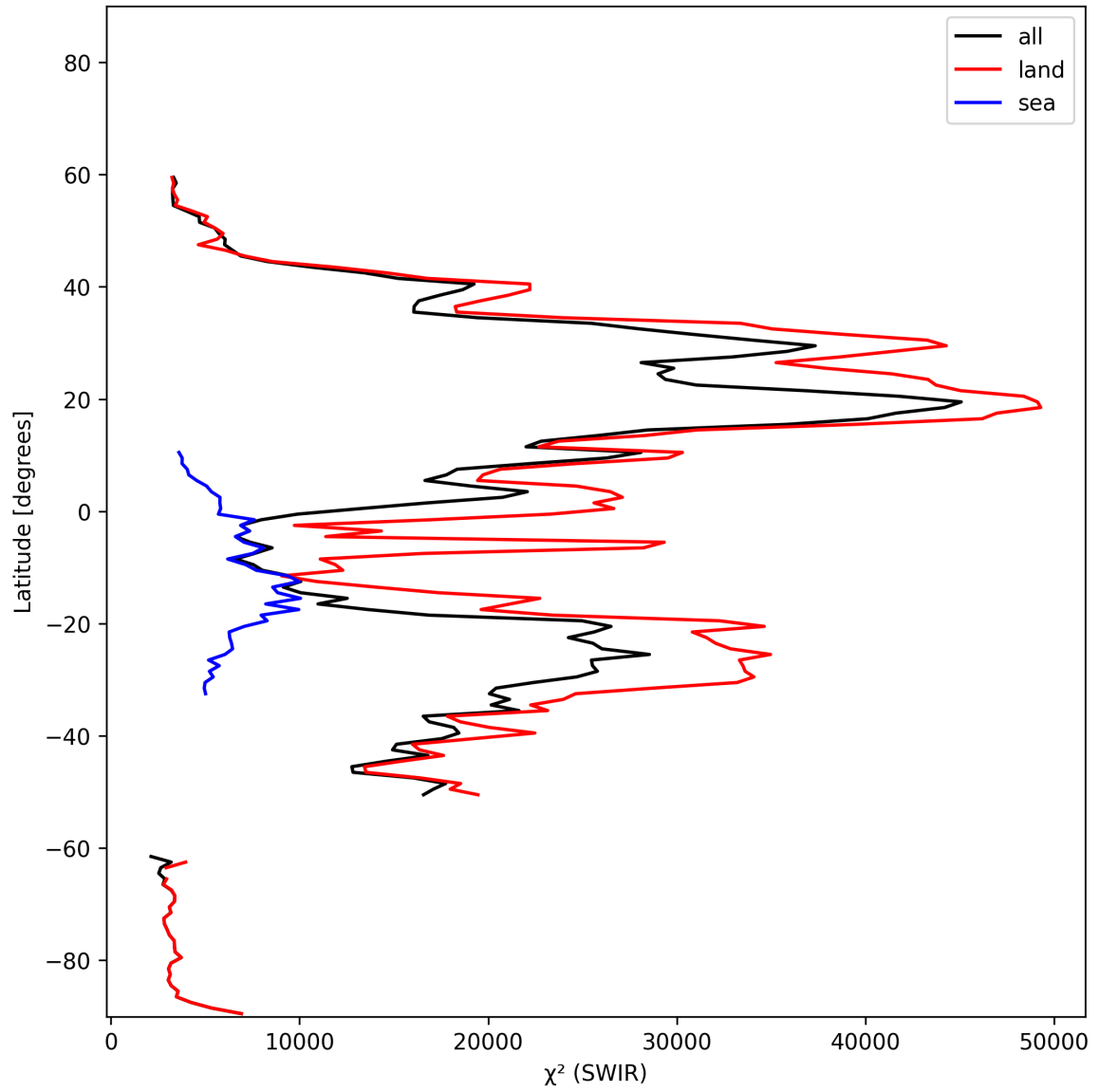
Figure 17: Zonal average of “ \chi^2 (SWIR)” for 2025-02-03 to 2025-02-05.
