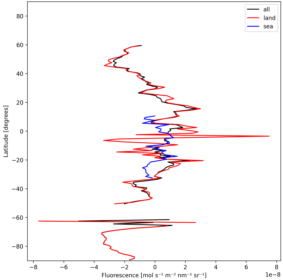
Figure 21: Zonal average of “Fluorescence” for 2025-02-03 to 2025-02-05.
