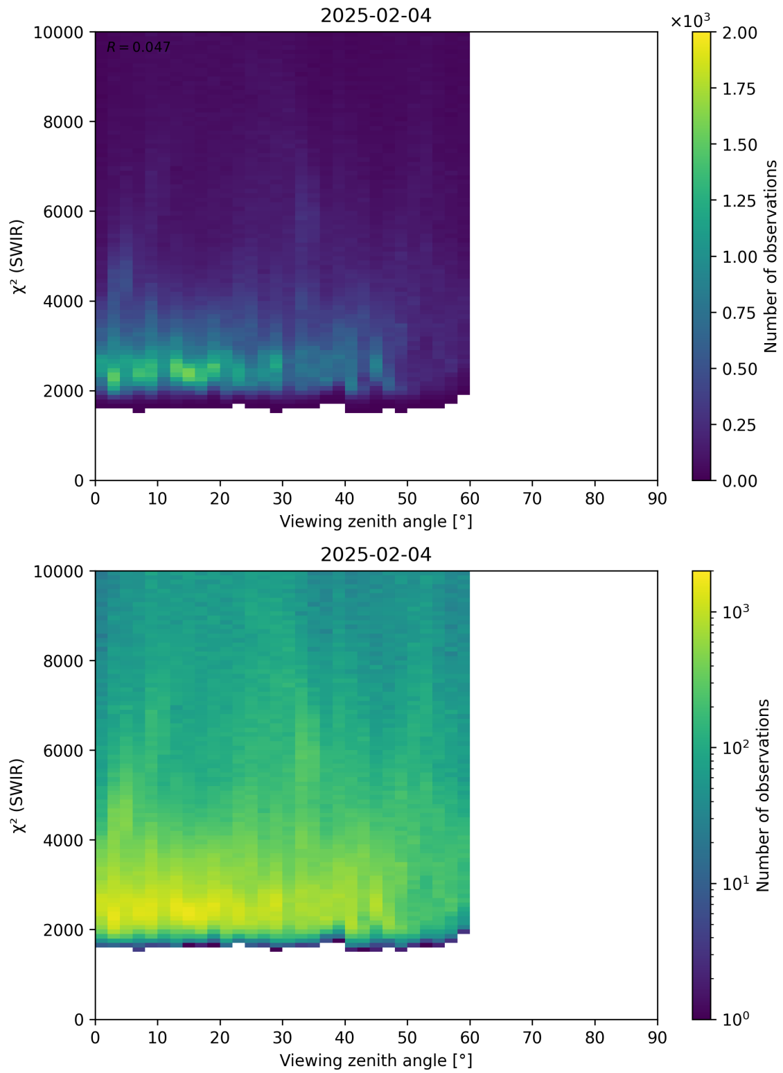
Figure 106: Scatter density plot of “Viewing zenith angle” against “ \chi^2 (SWIR)” for 2025-02-03 to 2025-02-05.
