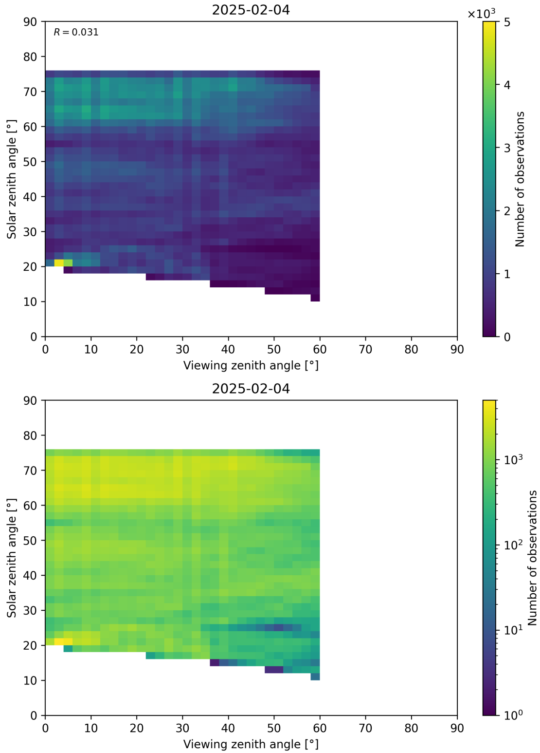
Figure 115: Scatter density plot of “Viewing zenith angle” against “Solar zenith angle” for 2025-02-03 to 2025-02-05.
