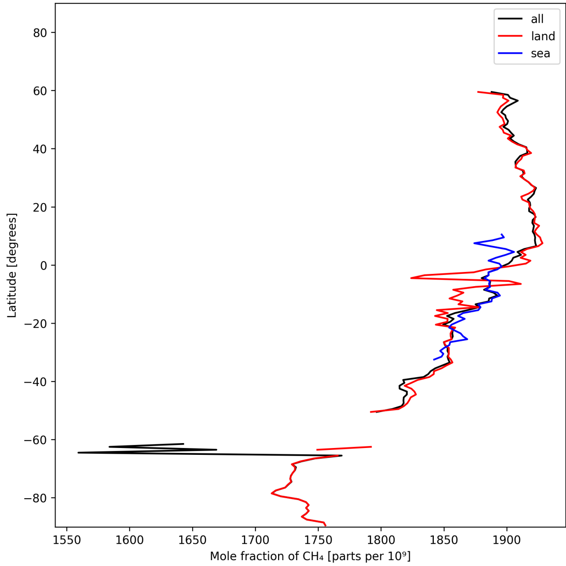
Figure 12: Zonal average of “Mole fraction of CH 4 ” for 2025-02-03 to 2025-02-05.
