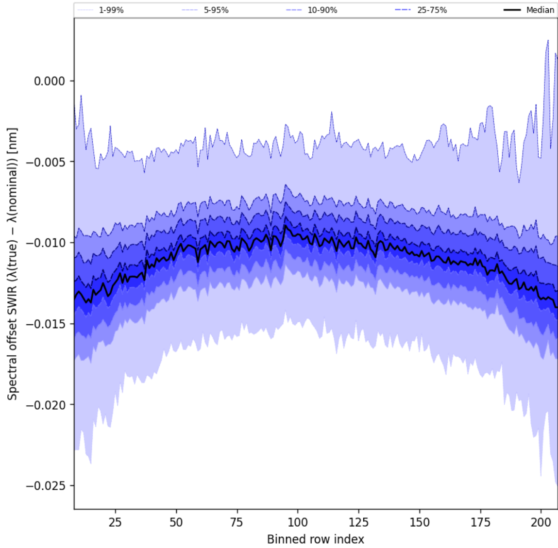
Figure 38: Along track statistics of “Spectral offset SWIR ( \lambda_{\text{true}} - \lambda_{\text{nominal}} )” for 2025-02-03 to 2025-02-05
