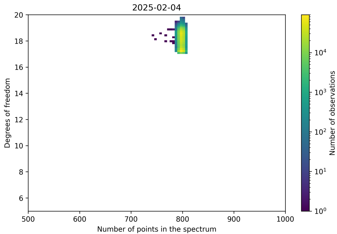
Figure 90: Scatter density plot of “Number of points in the spectrum” against “Degrees of freedom” for 2025-02-03 to 2025-02-05.
