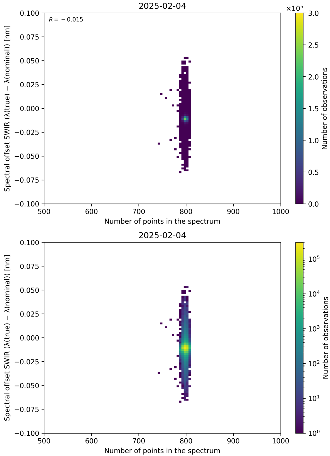
Figure 93: Scatter density plot of “Number of points in the spectrum” against “Spectral offset SWIR ( \lambda_{\text{true}} - \lambda_{\text{nominal}} )” for 2025-02-03 to 2025-02-05.
