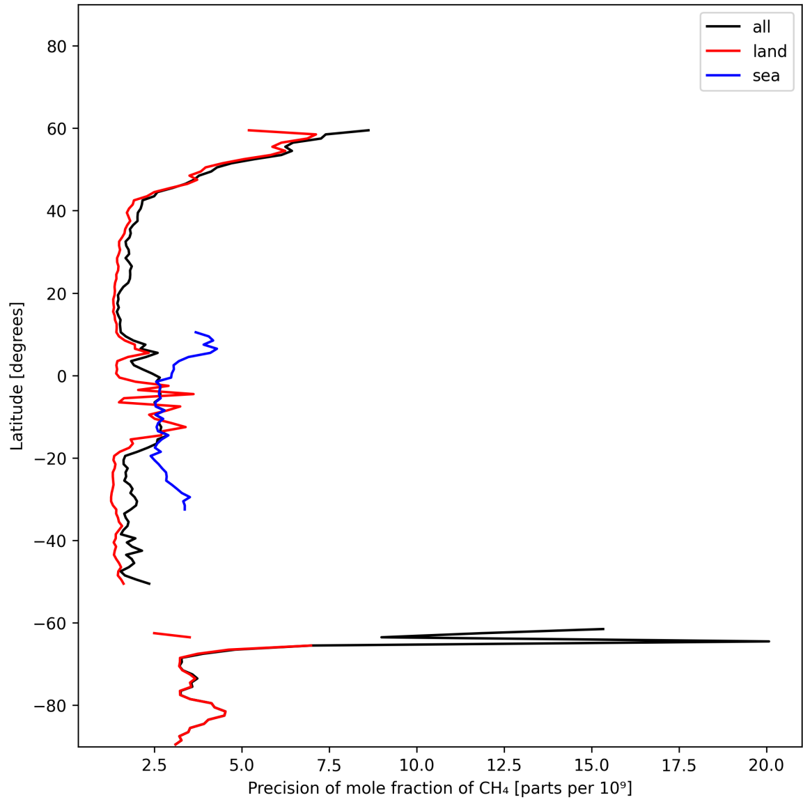
Figure 13: Zonal average of “Precision of mole fraction of CH 4 ” for 2025-02-03 to 2025-02-05.
