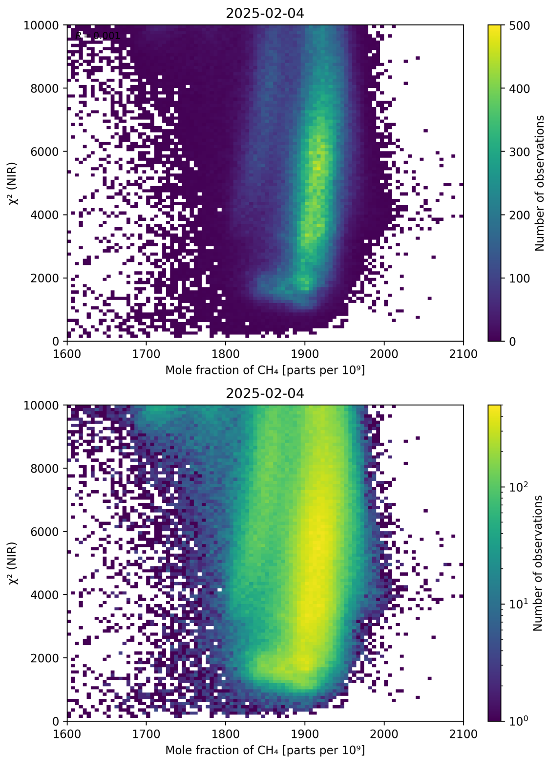
Figure 70: Scatter density plot of “Mole fraction of \text{CH}_4 ” against “ \chi^2 (NIR)” for 2025-02-03 to 2025-02-05.
