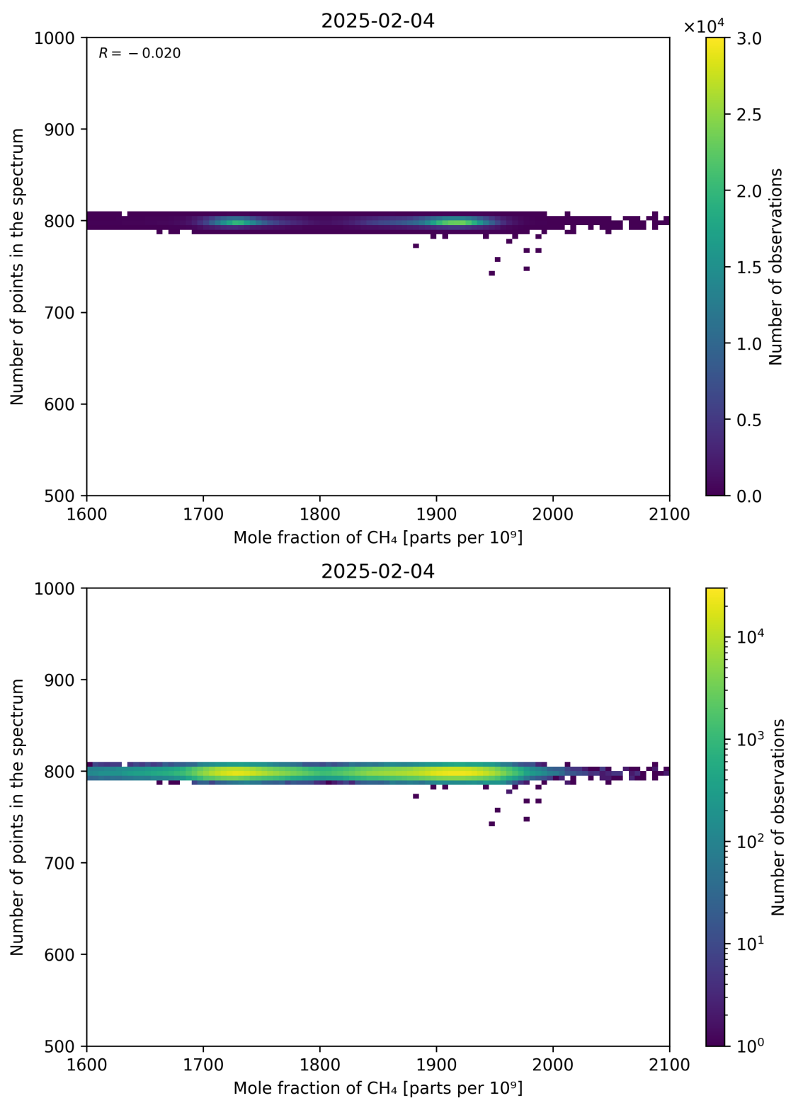
Figure 77: Scatter density plot of “Mole fraction of CH 4 ” against “Number of points in the spectrum” for 2025-02-03 to 2025-02-05.
