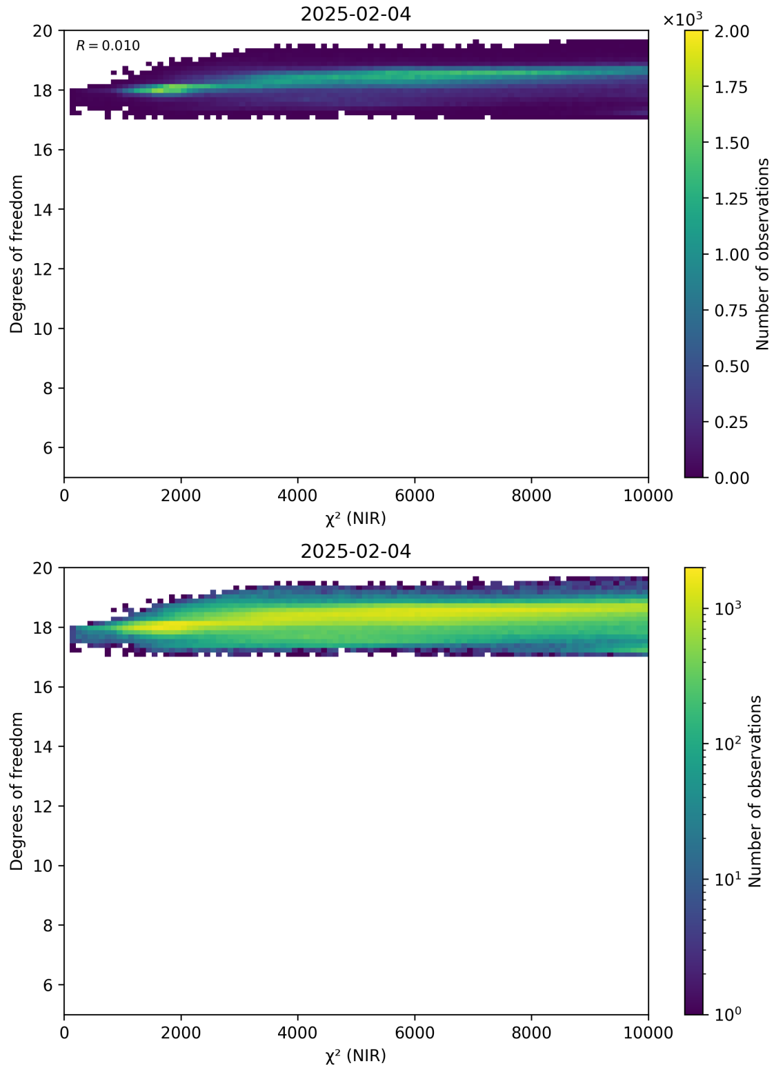
Figure 44: Scatter density plot of “ \chi^2 (NIR)” against “Degrees of freedom” for 2025-02-03 to 2025-02-05.
