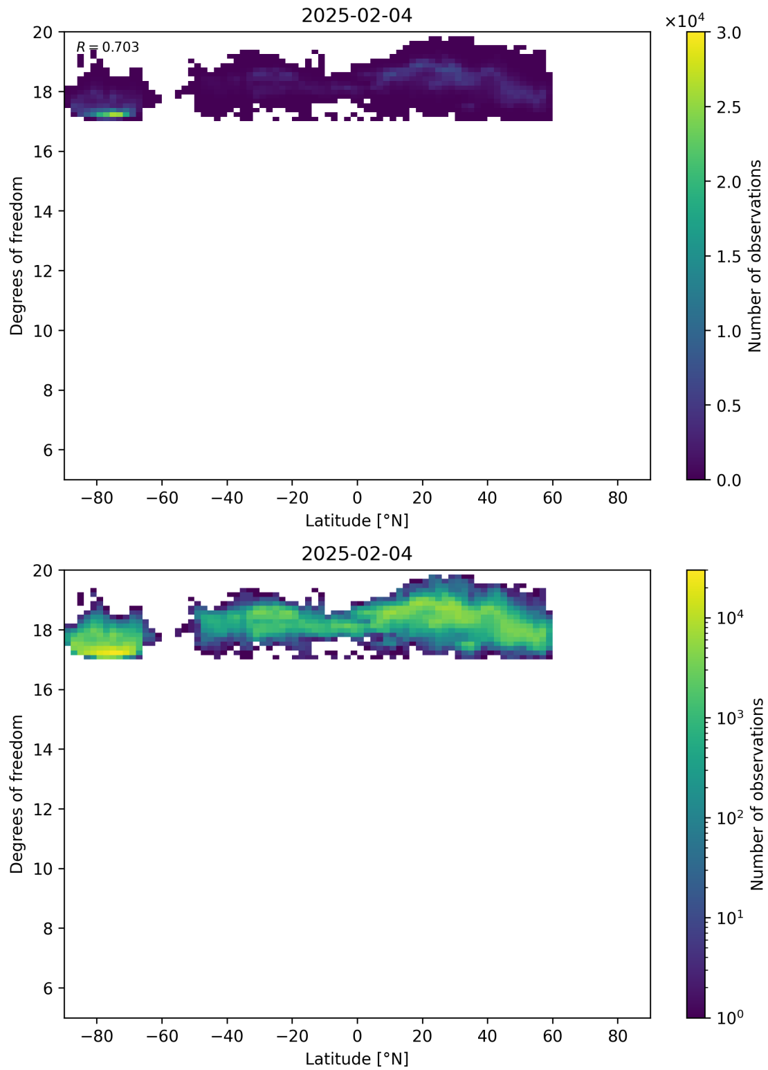
Figure 55: Scatter density plot of “Latitude” against “Degrees of freedom” for 2025-02-03 to 2025-02-05.
