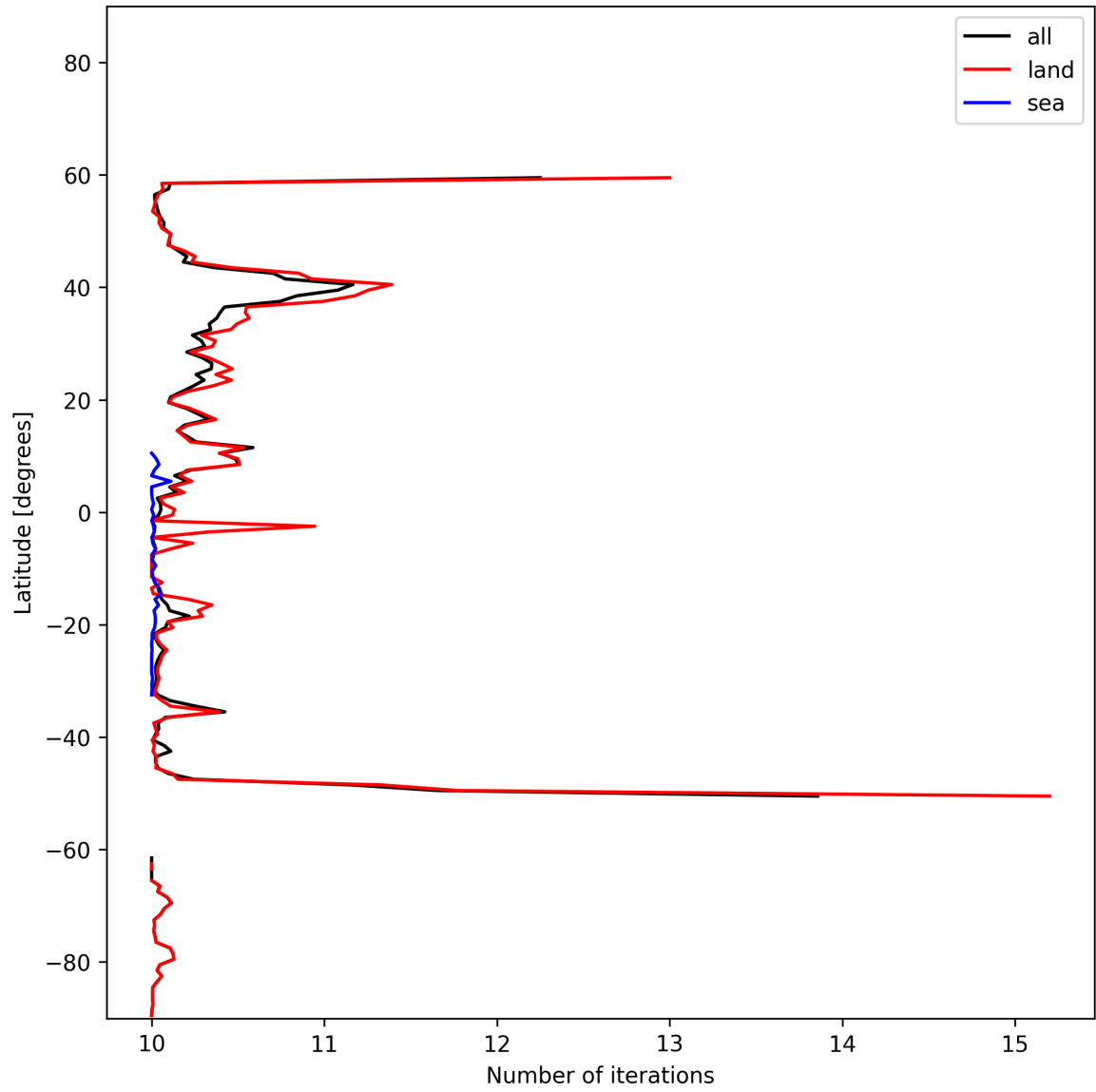
Figure 20: Zonal average of “Number of iterations” for 2025-02-03 to 2025-02-05.
