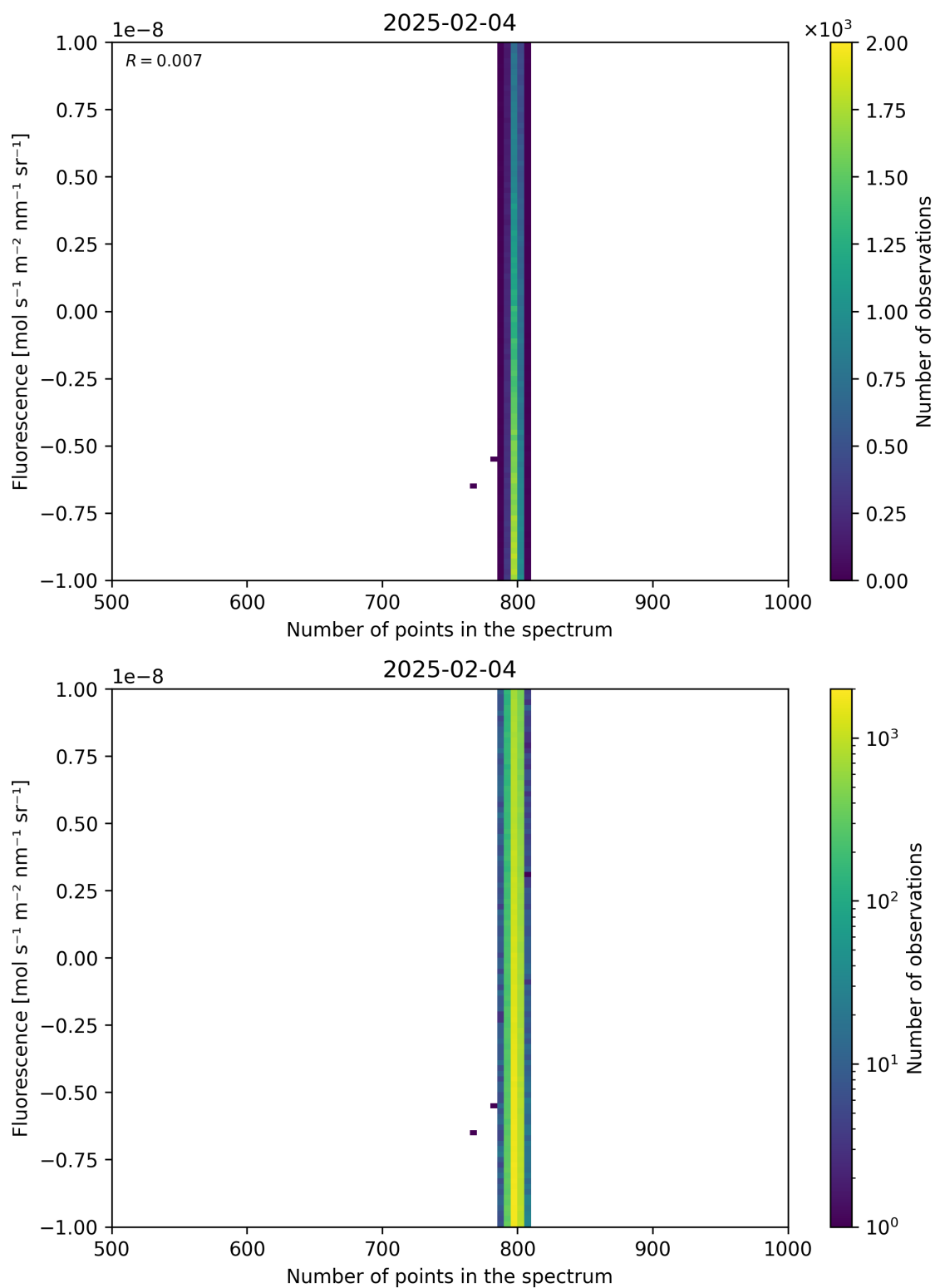
Figure 91: Scatter density plot of “Number of points in the spectrum” against “Fluorescence” for 2025-02-03 to 2025-02-05.
