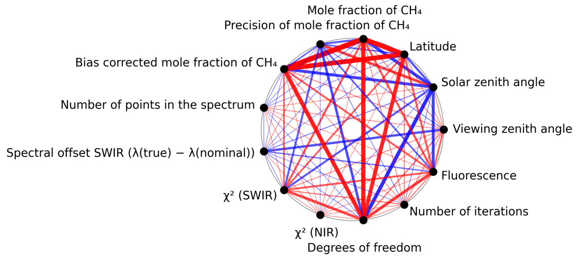
Figure 1: Map of correlation graph for 2025-02-03 to 2025-02-05.
