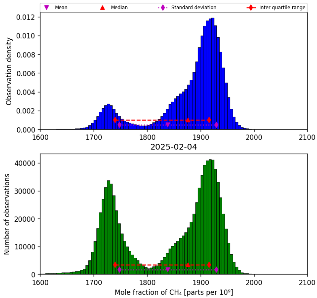
Figure 23: Histogram of “Mole fraction of CH 4 ” for 2025-02-03 to 2025-02-05
