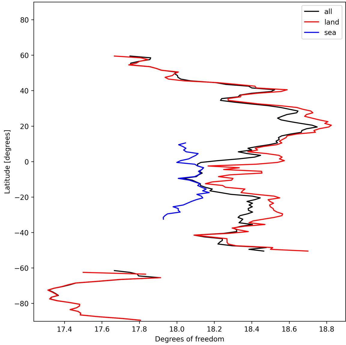
Figure 19: Zonal average of “Degrees of freedom” for 2025-02-03 to 2025-02-05.
