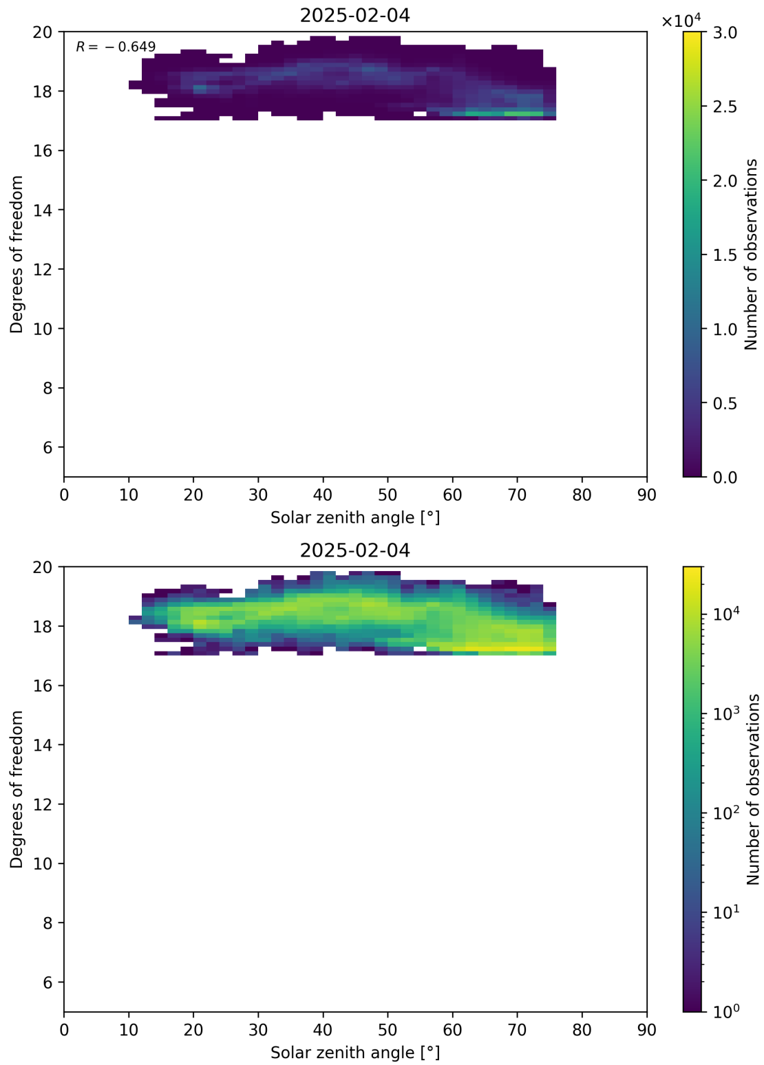
Figure 96: Scatter density plot of “Solar zenith angle” against “Degrees of freedom” for 2025-02-03 to 2025-02-05.
