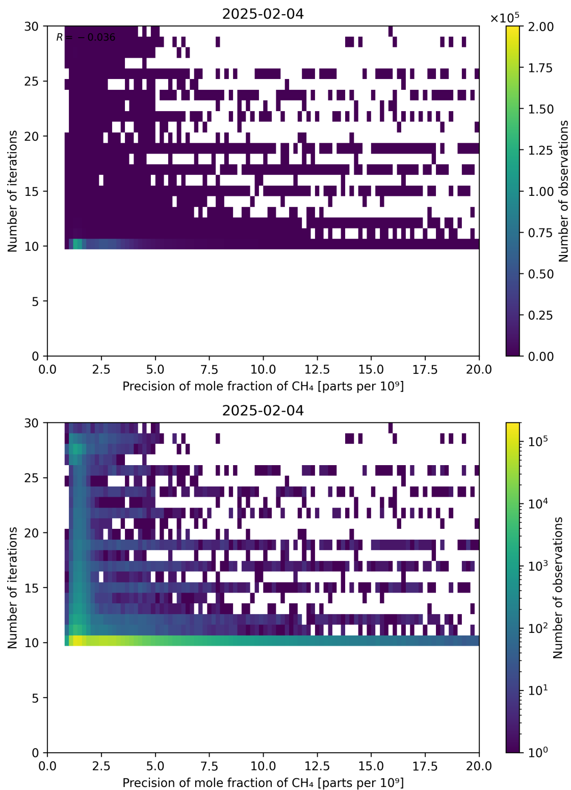
Figure 83: Scatter density plot of “Precision of mole fraction of CH 4 ” against “Number of iterations” for 2025-02-03 to 2025-02-05.
