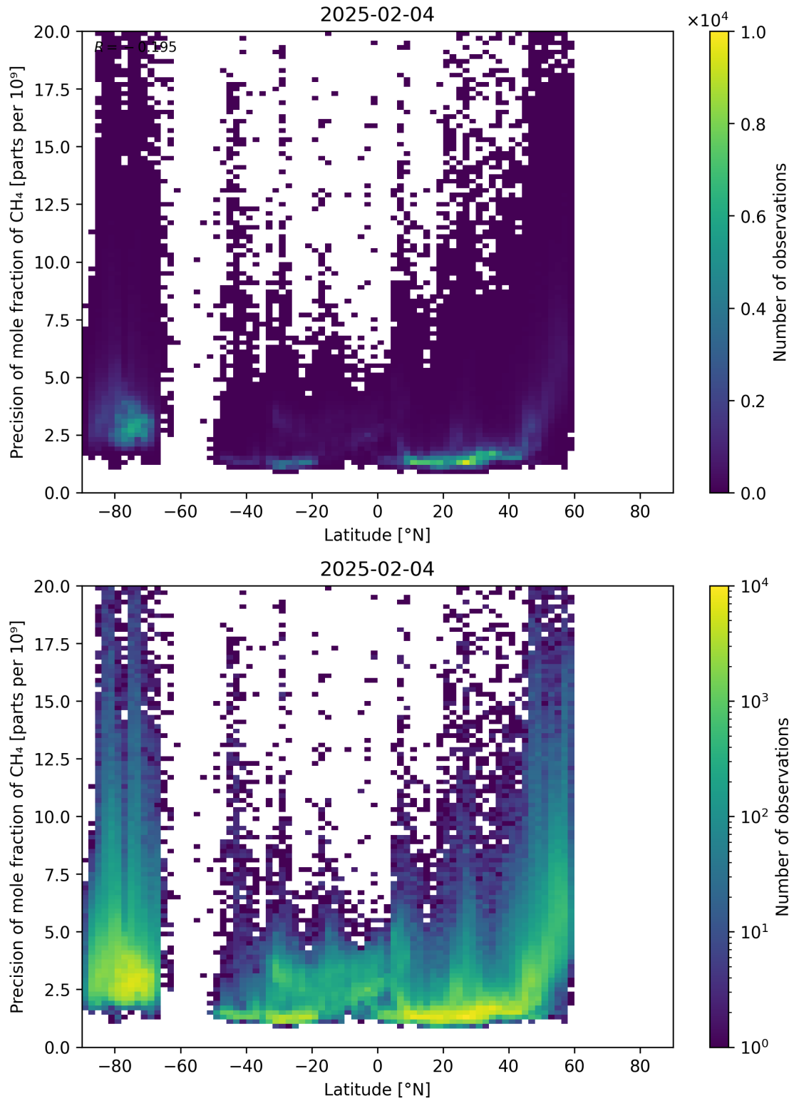
Figure 59: Scatter density plot of “Latitude” against “Precision of mole fraction of CH 4 ” for 2025-02-03 to 2025-02-05.
