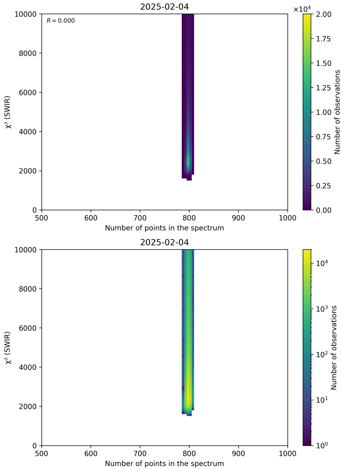
Figure 89: Scatter density plot of “Number of points in the spectrum” against “ \chi^2 (SWIR)” for 2025-02-03 to 2025-02-05.
