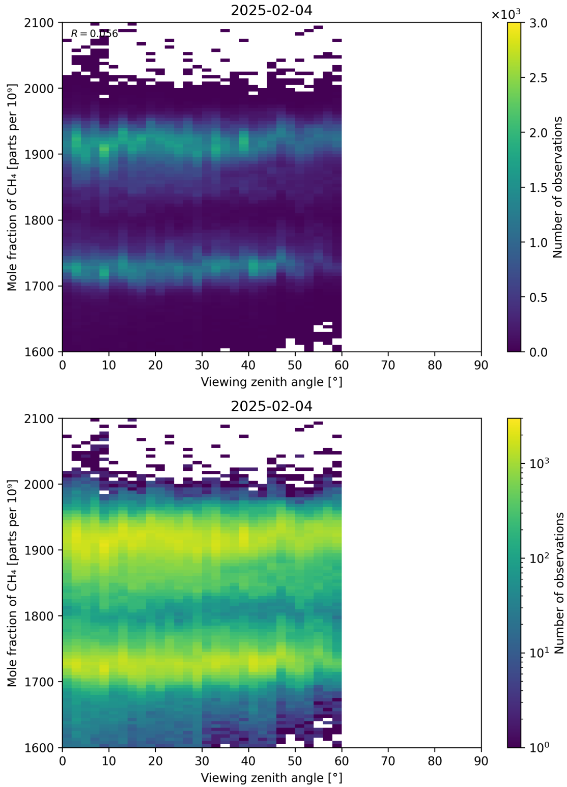
Figure 110: Scatter density plot of “Viewing zenith angle” against “Mole fraction of CH 4 ” for 2025-02-03 to 2025-02-05.
