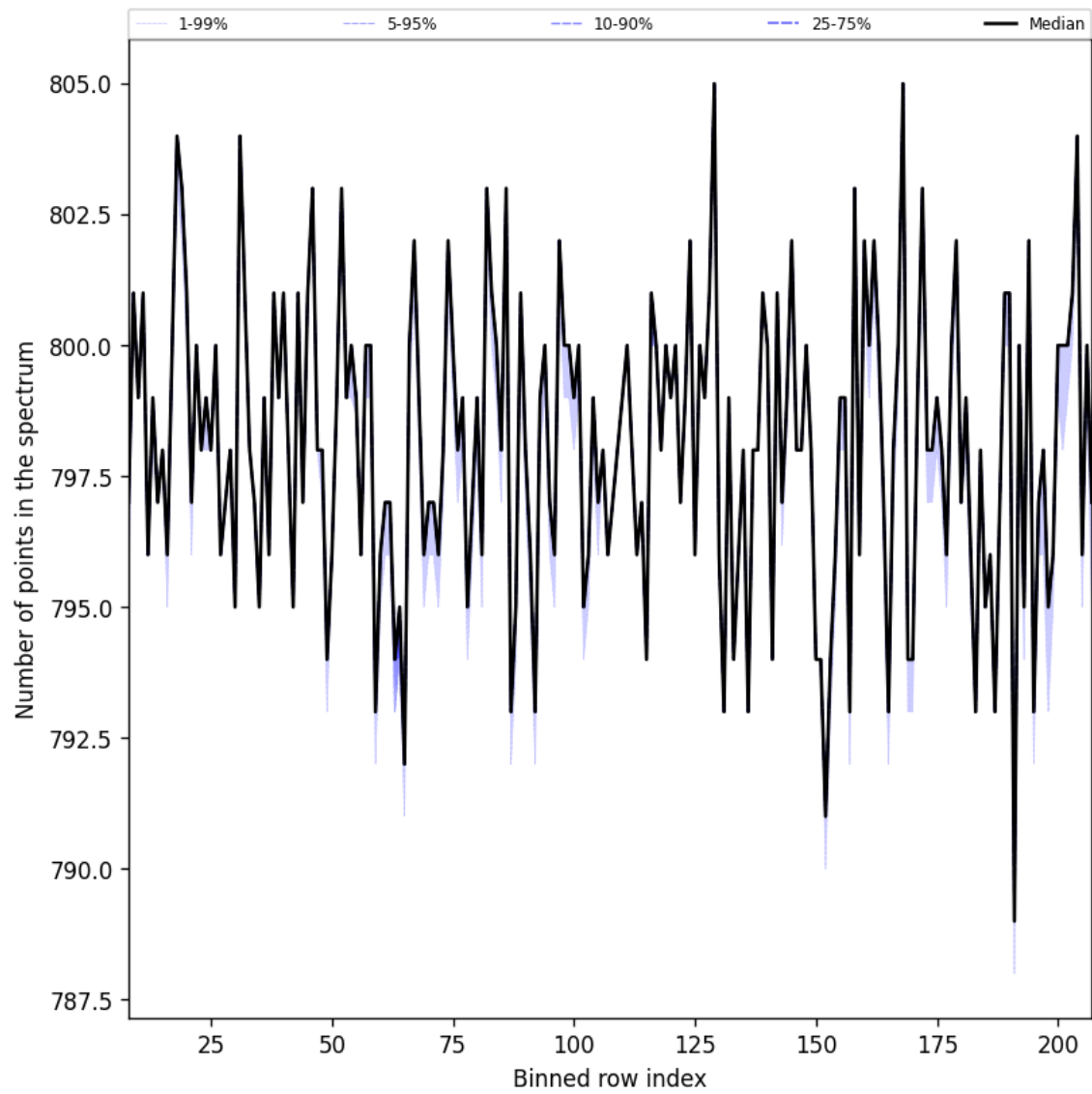
Figure 37: Along track statistics of “Number of points in the spectrum” for 2025-02-03 to 2025-02-05
