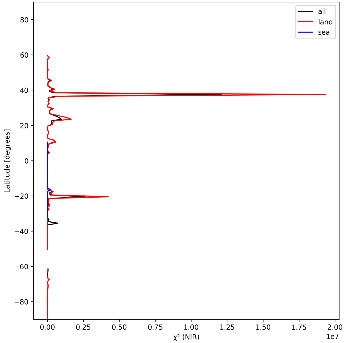
Figure 18: Zonal average of “ \chi^2 (NIR)” for 2025-02-03 to 2025-02-05.
