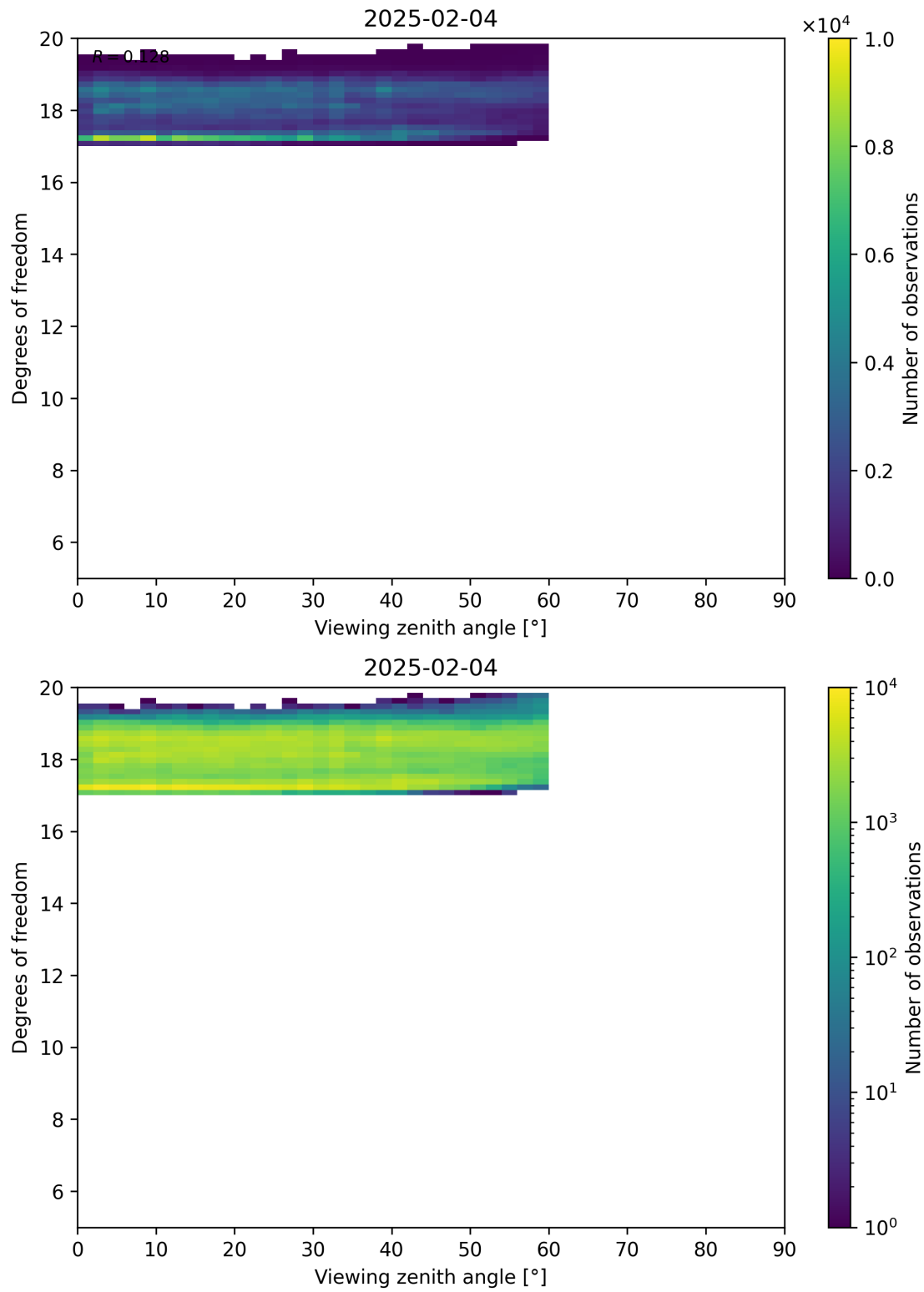
Figure 107: Scatter density plot of “Viewing zenith angle” against “Degrees of freedom” for 2025-02-03 to 2025-02-05.
