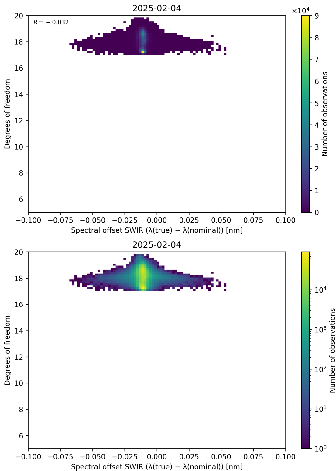
Figure 119: Scatter density plot of “Spectral offset SWIR ( \lambda_{\text{true}} - \lambda_{\text{nominal}} )” against “Degrees of freedom” for 2025-02-03 to 2025-02-05.
