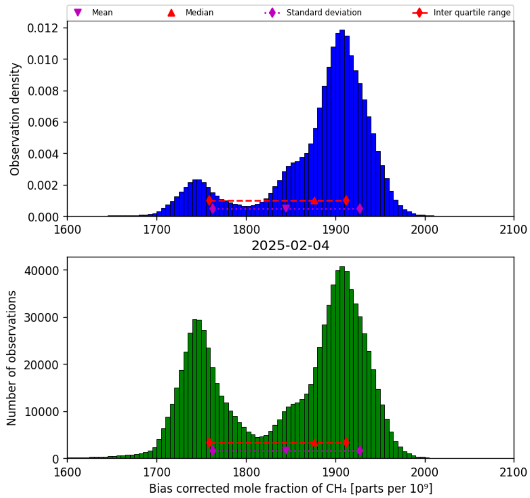
Figure 25: Histogram of “Bias corrected mole fraction of CH 4 ” for 2025-02-03 to 2025-02-05
