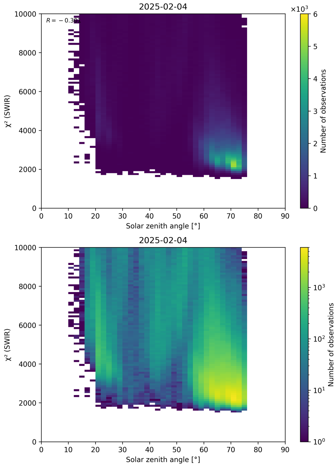
Figure 95: Scatter density plot of “Solar zenith angle” against “ \chi^2 (SWIR)” for 2025-02-03 to 2025-02-05.
