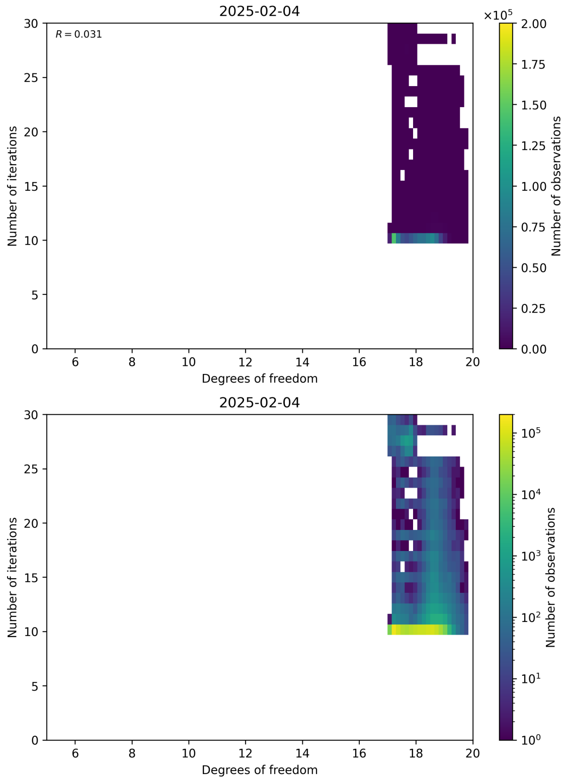
Figure 52: Scatter density plot of “Degrees of freedom” against “Number of iterations” for 2025-02-03 to 2025-02-05.
