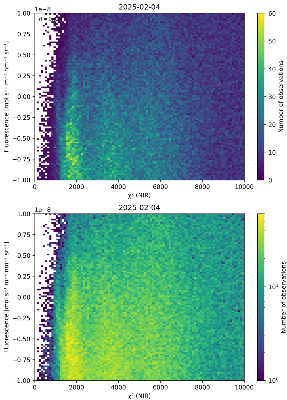
Figure 45: Scatter density plot of “ \chi^2 (NIR)” against “Fluorescence” for 2025-02-03 to 2025-02-05.
