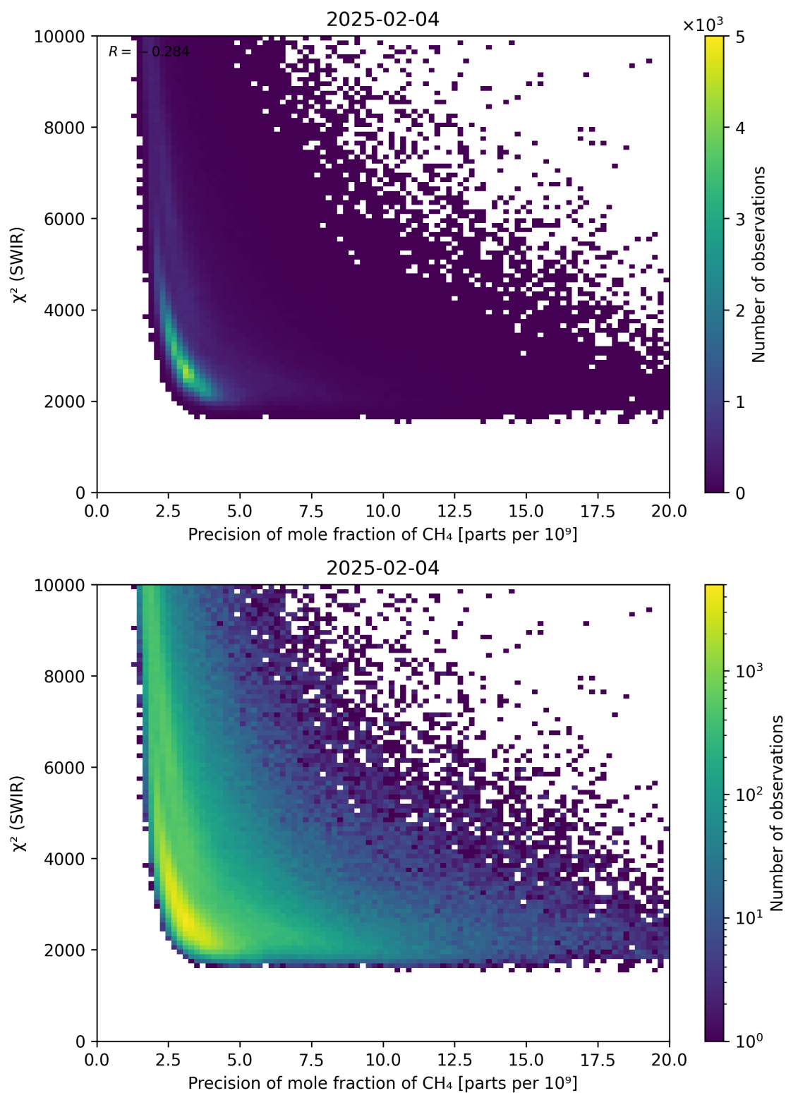
Figure 79: Scatter density plot of “Precision of mole fraction of \text{CH}_4 ” against “ \chi^2 (SWIR)” for 2025-02-03 to 2025-02-05.
