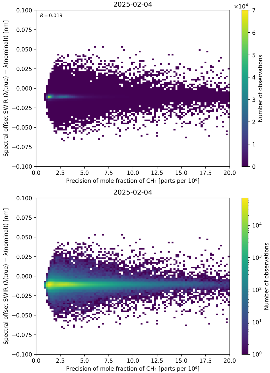
Figure 85: Scatter density plot of “Precision of mole fraction of \text{CH}_4 ” against “Spectral offset SWIR ( \lambda_{\text{true}} - \lambda_{\text{nominal}} )” for 2025-02-03 to 2025-02-05.
