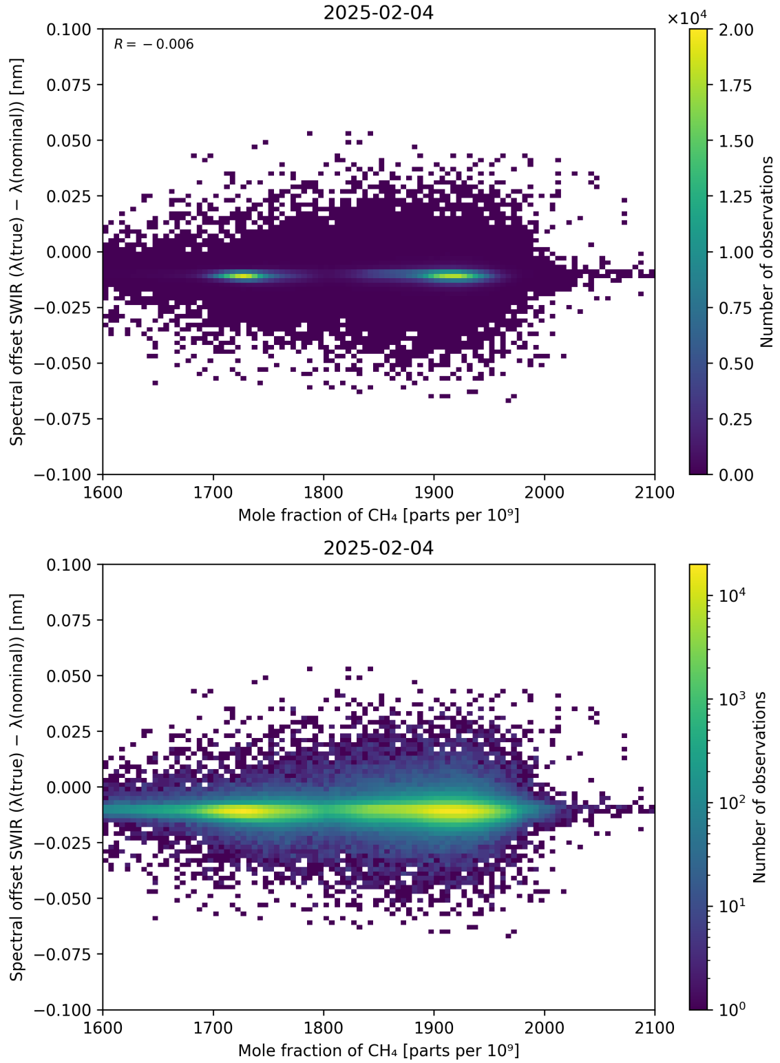
Figure 86: Scatter density plot of “Mole fraction of \text{CH}_4 ” against “Spectral offset SWIR ( \lambda_{\text{true}} - \lambda_{\text{nominal}} )” for 2025-02-03 to 2025-02-05.
