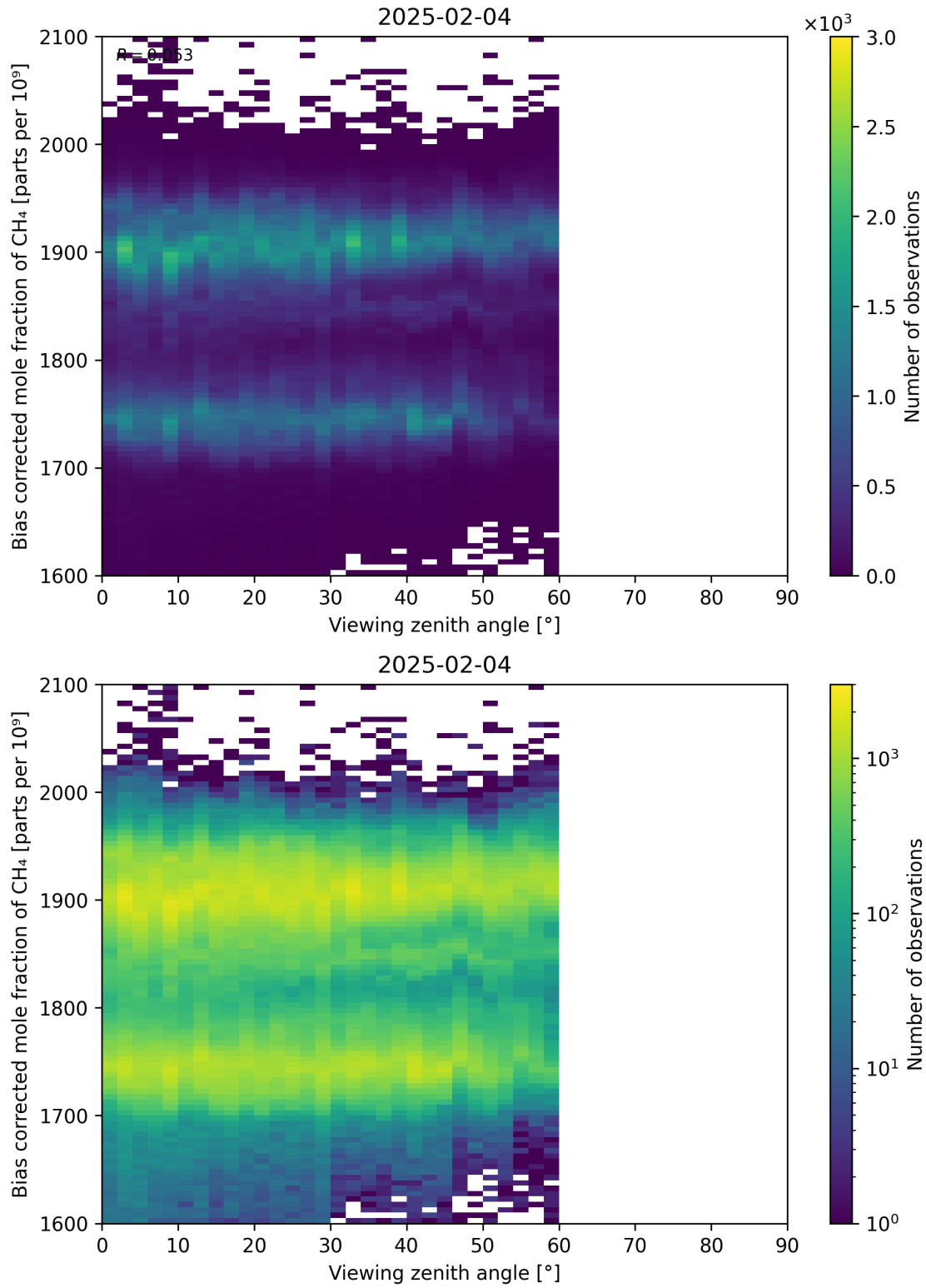
Figure 111: Scatter density plot of “Viewing zenith angle” against “Bias corrected mole fraction of CH 4 ” for 2025-02-03 to 2025-02-05.
