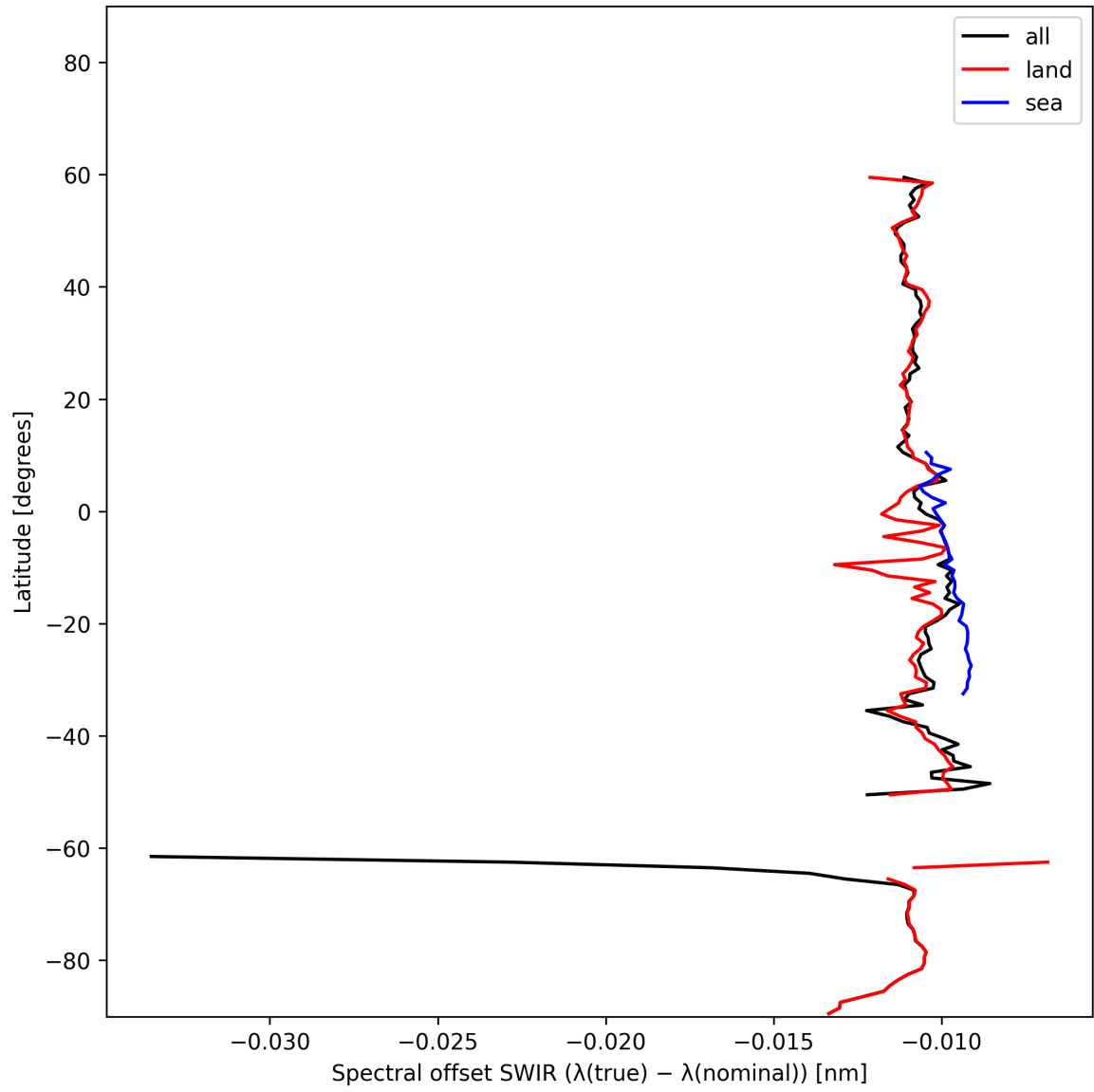
Figure 16: Zonal average of “Spectral offset SWIR ( \lambda_{\text{true}} - \lambda_{\text{nominal}} )” for 2025-02-03 to 2025-02-05.
