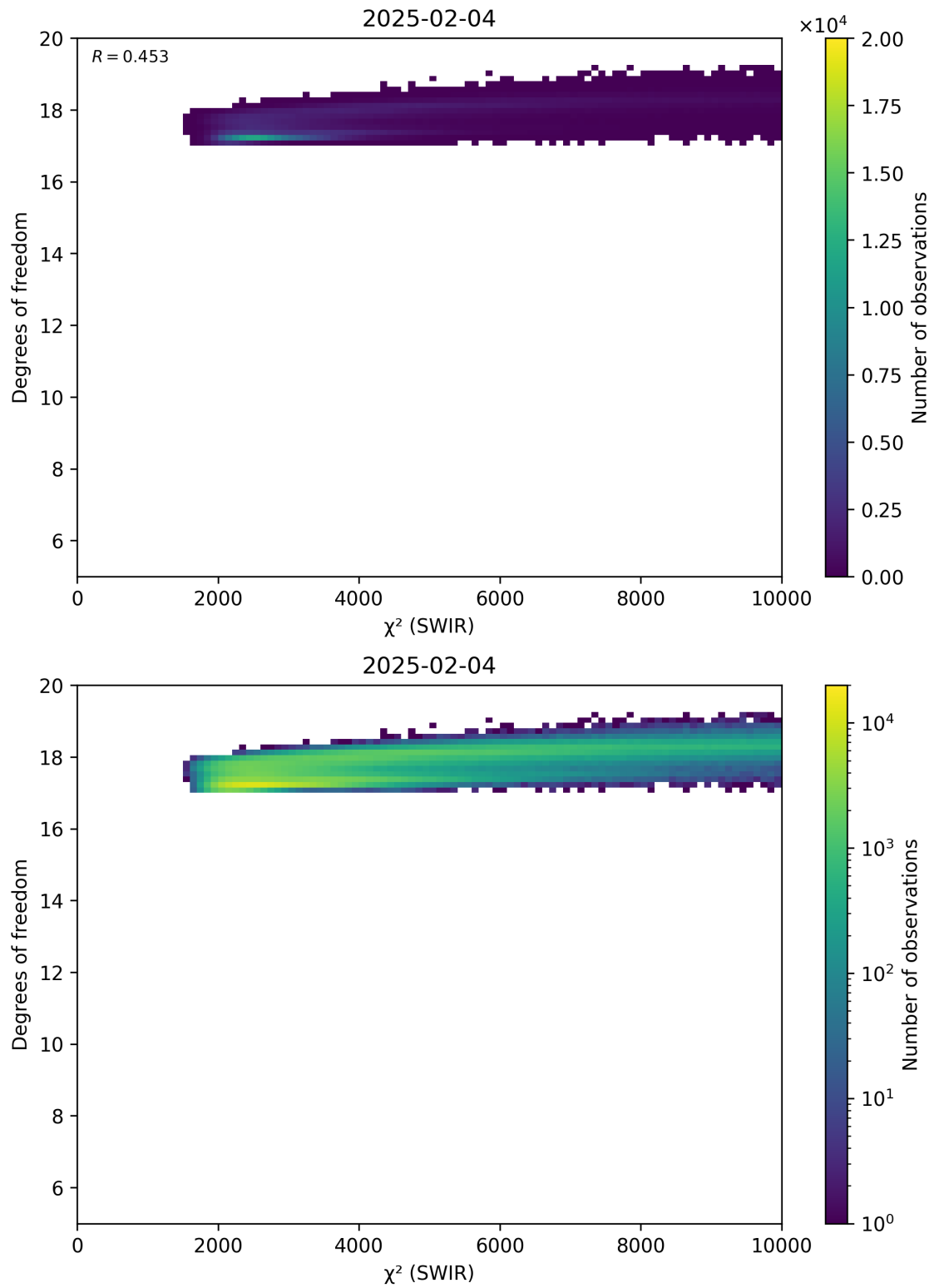
Figure 48: Scatter density plot of “ \chi^2 (SWIR)” against “Degrees of freedom” for 2025-02-03 to 2025-02-05.
