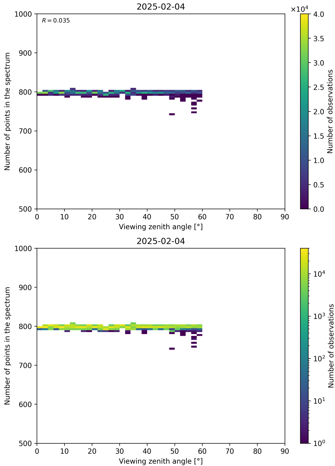
Figure 114: Scatter density plot of “Viewing zenith angle” against “Number of points in the spectrum” for 2025-02-03 to 2025-02-05.
