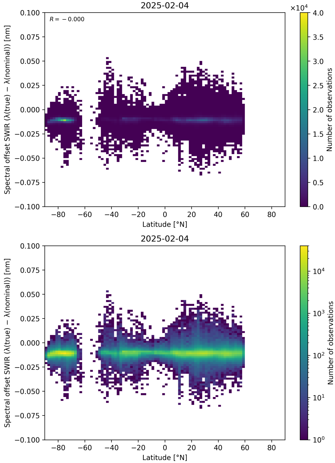
Figure 62: Scatter density plot of “Latitude” against “Spectral offset SWIR ( \lambda_{\text{true}} - \lambda_{\text{nominal}} )” for 2025-02-03 to 2025-02-05.
