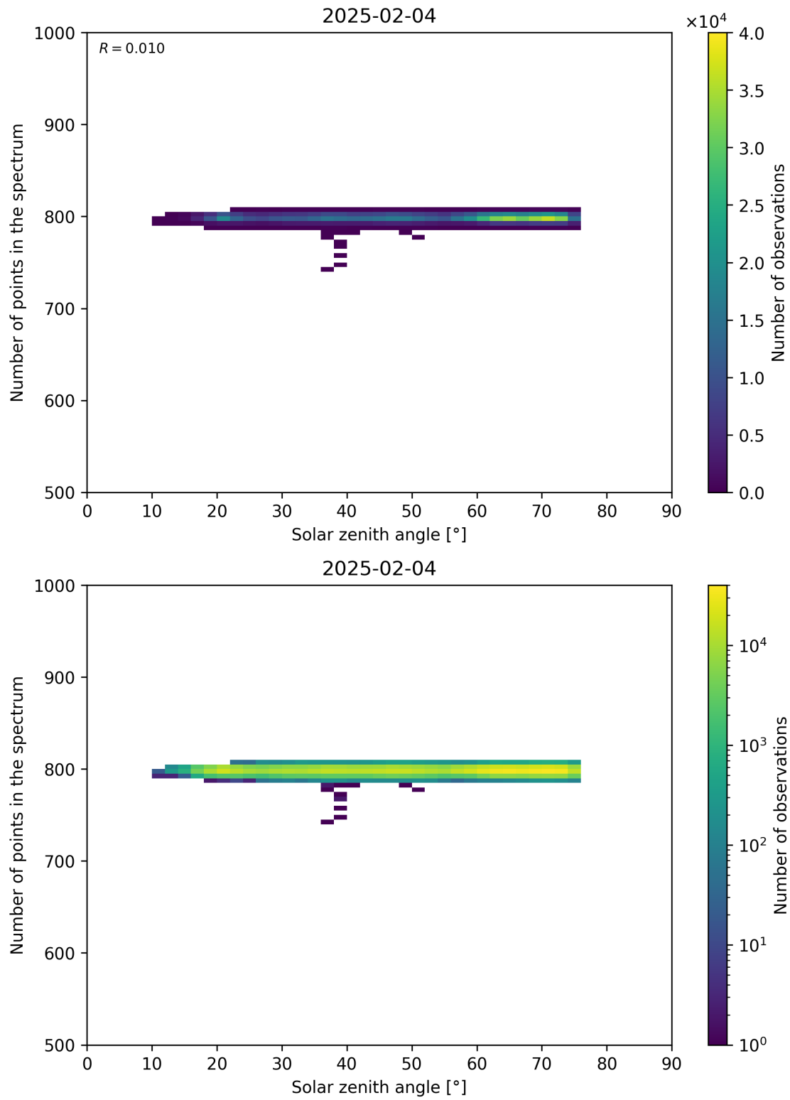
Figure 103: Scatter density plot of “Solar zenith angle” against “Number of points in the spectrum” for 2025-02-03 to 2025-02-05.
