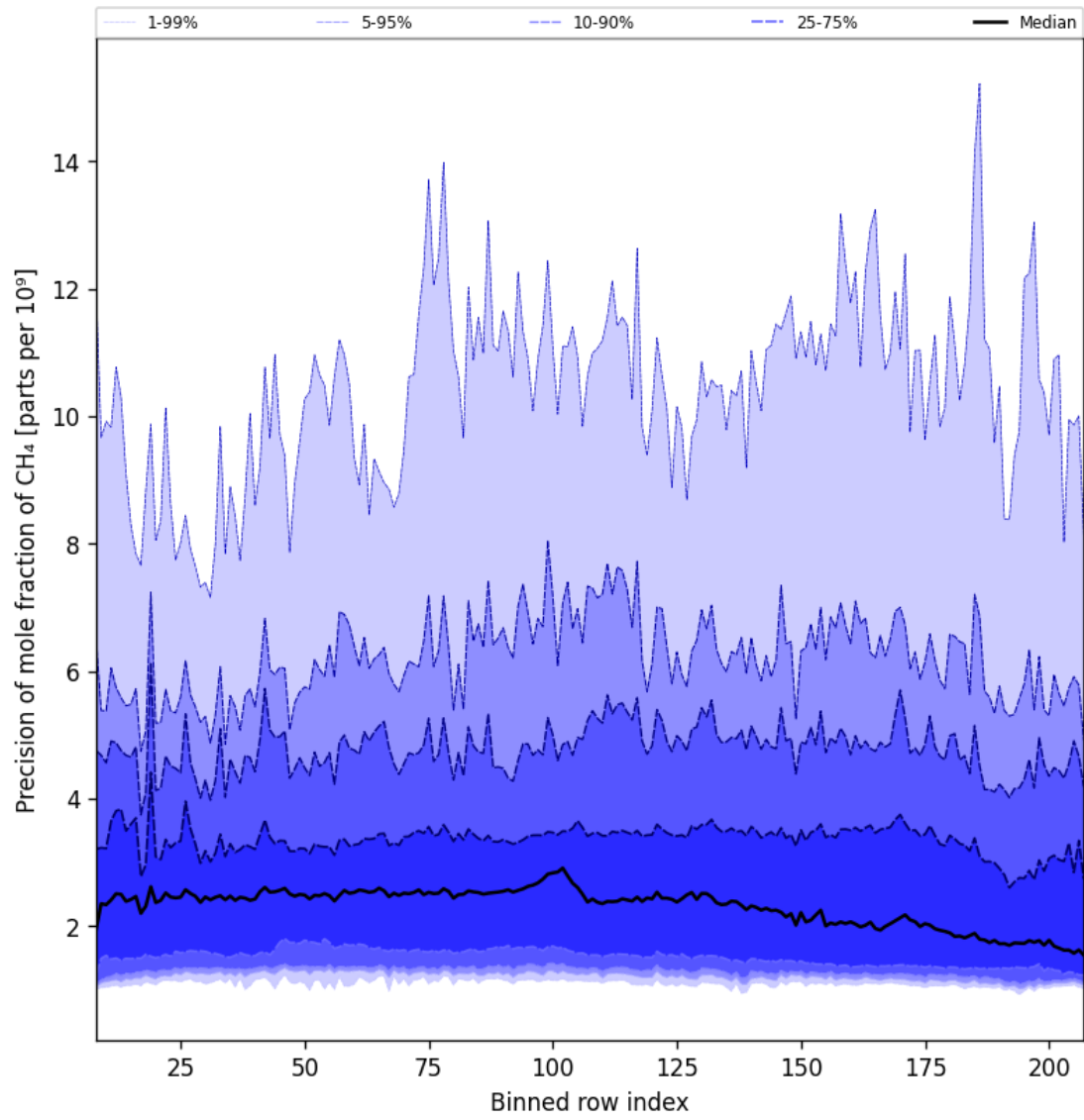
Figure 35: Along track statistics of “Precision of mole fraction of CH 4 ” for 2025-02-03 to 2025-02-05
