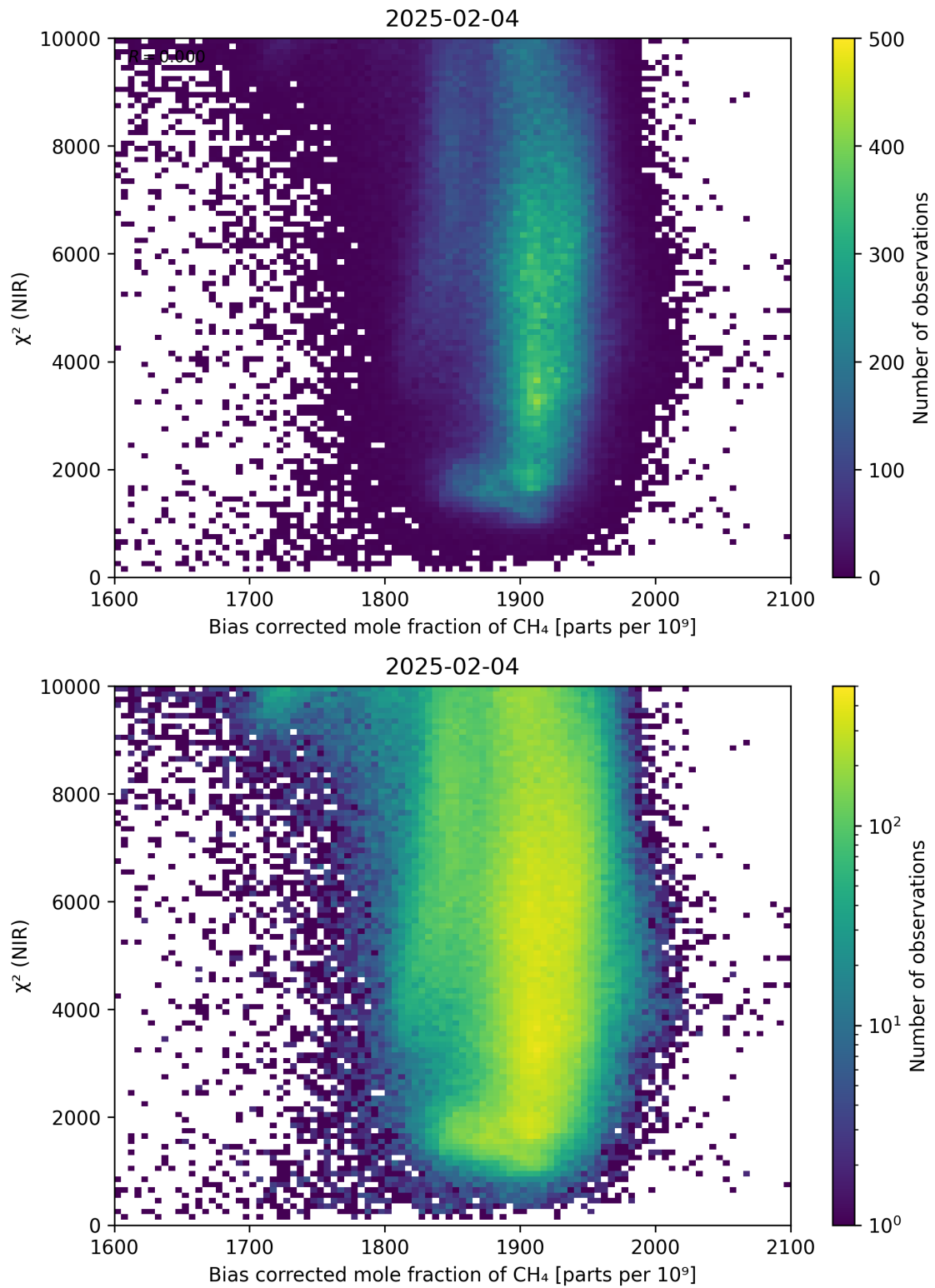
Figure 63: Scatter density plot of “Bias corrected mole fraction of \text{CH}_4 ” against “ \chi^2 (NIR)” for 2025-02-03 to 2025-02-05.
