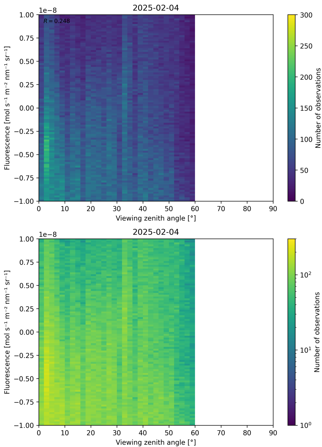
Figure 108: Scatter density plot of “Viewing zenith angle” against “Fluorescence” for 2025-02-03 to 2025-02-05.
