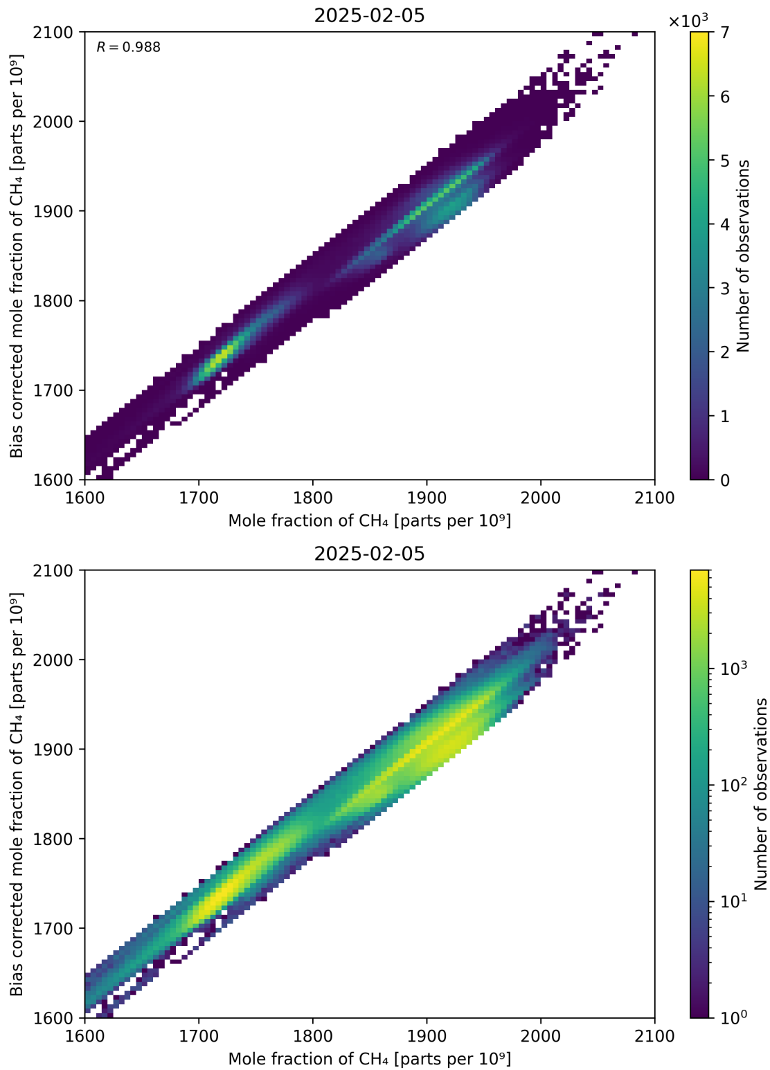
Figure 74: Scatter density plot of “Mole fraction of CH 4 ” against “Bias corrected mole fraction of CH 4 ” for 2025-02-04 to 2025-02-06.
