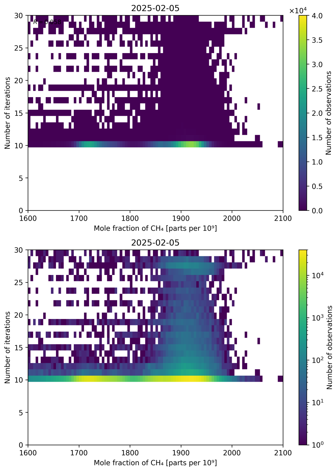
Figure 76: Scatter density plot of “Mole fraction of CH 4 ” against “Number of iterations” for 2025-02-04 to 2025-02-06.
