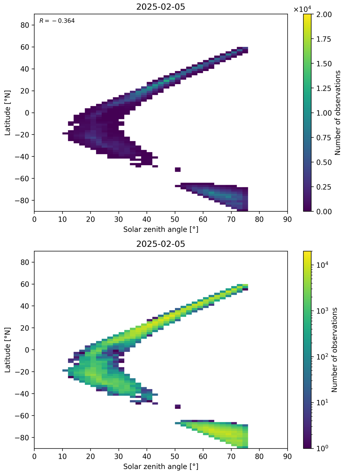
Figure 98: Scatter density plot of “Solar zenith angle” against “Latitude” for 2025-02-04 to 2025-02-06.
