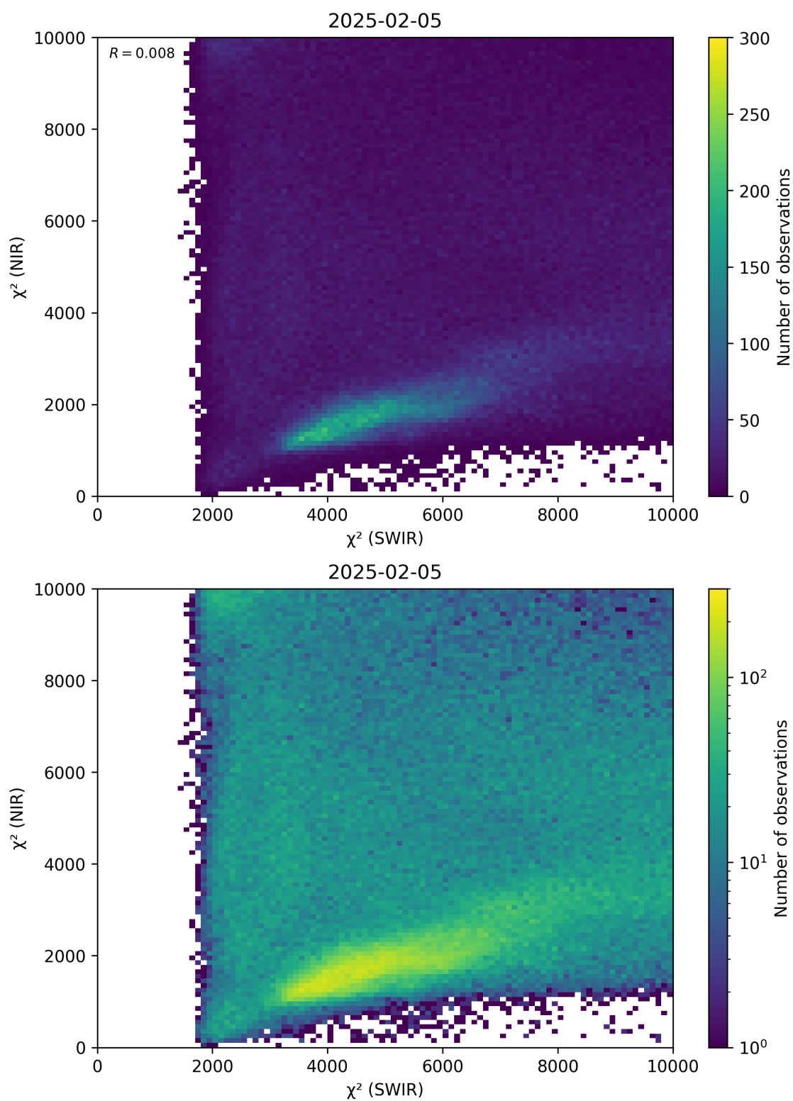
Figure 47: Scatter density plot of “ \chi^2 (SWIR)” against “ \chi^2 (NIR)” for 2025-02-04 to 2025-02-06.
