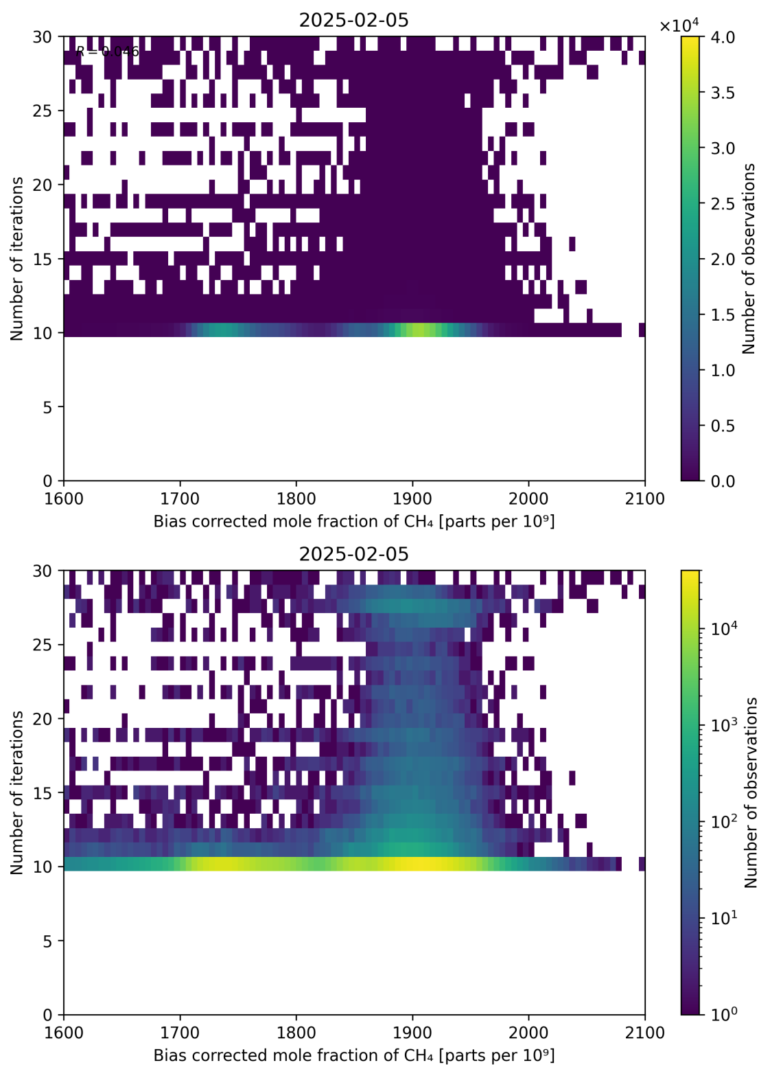
Figure 67: Scatter density plot of “Bias corrected mole fraction of CH 4 ” against “Number of iterations” for 2025-02-04 to 2025-02-06.
