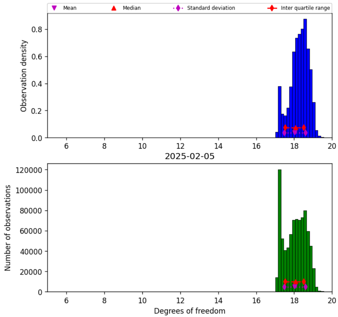
Figure 30: Histogram of “Degrees of freedom” for 2025-02-04 to 2025-02-06
