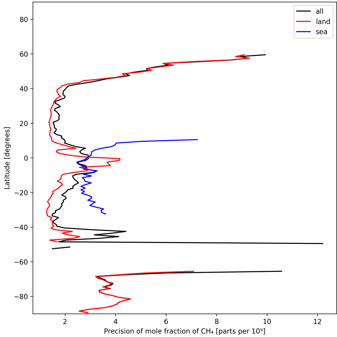
Figure 13: Zonal average of “Precision of mole fraction of CH 4 ” for 2025-02-04 to 2025-02-06.
