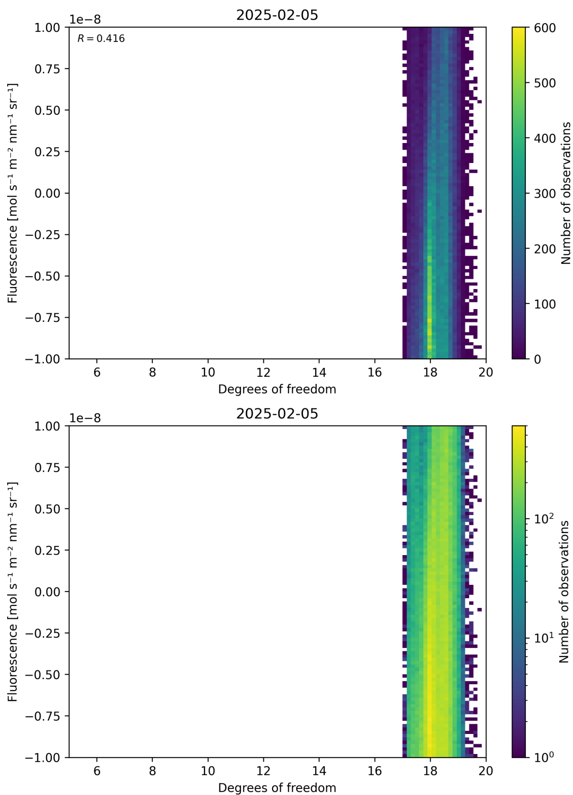
Figure 51: Scatter density plot of “Degrees of freedom” against “Fluorescence” for 2025-02-04 to 2025-02-06.
