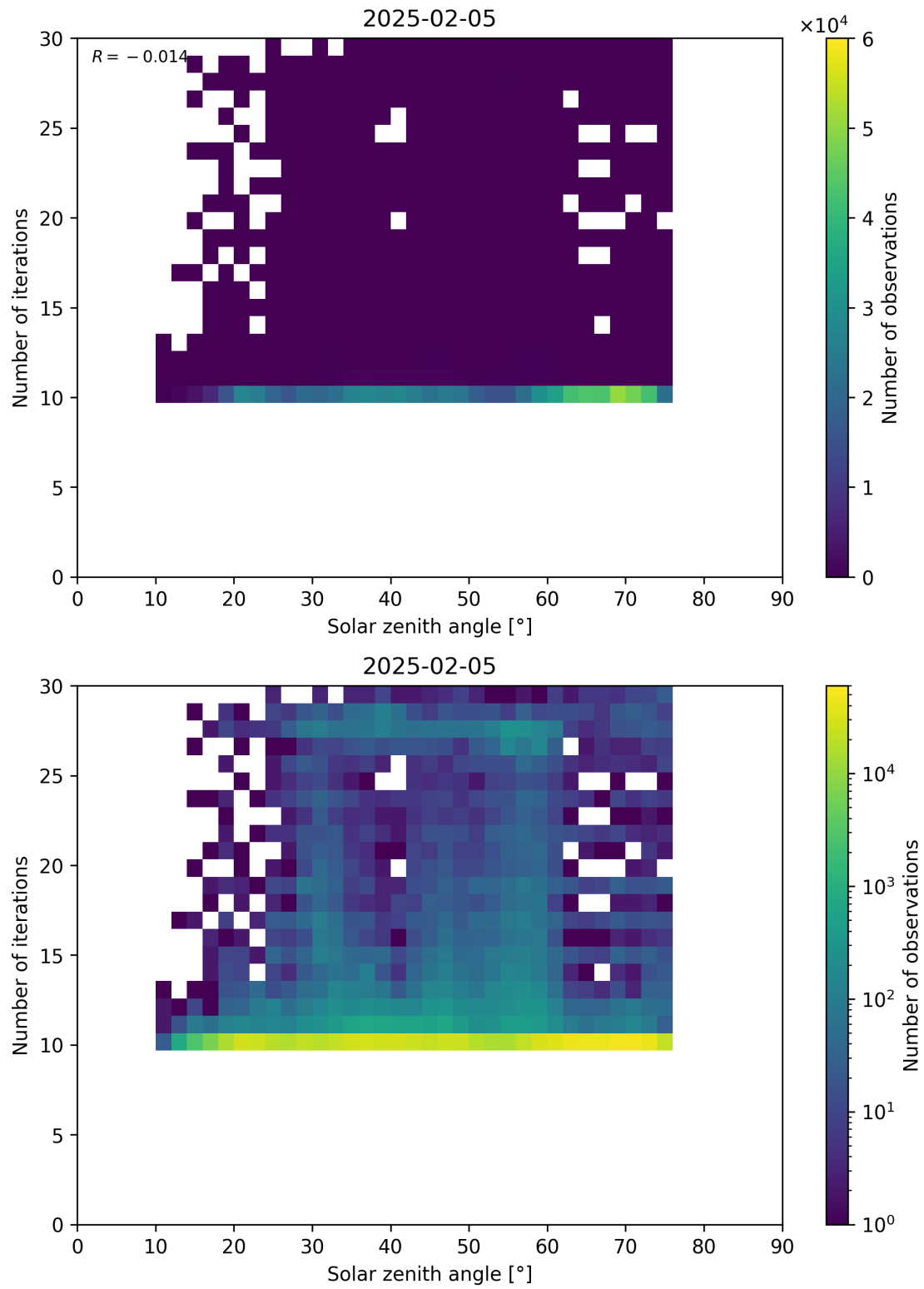
Figure 102: Scatter density plot of “Solar zenith angle” against “Number of iterations” for 2025-02-04 to 2025-02-06.
