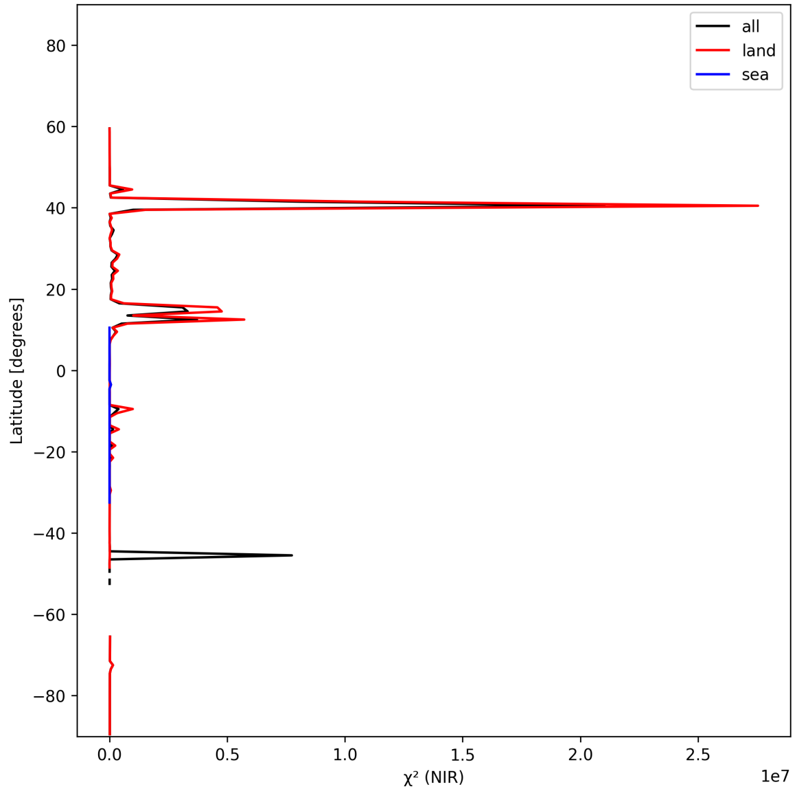
Figure 18: Zonal average of “ \chi^2 (NIR)” for 2025-02-04 to 2025-02-06.
