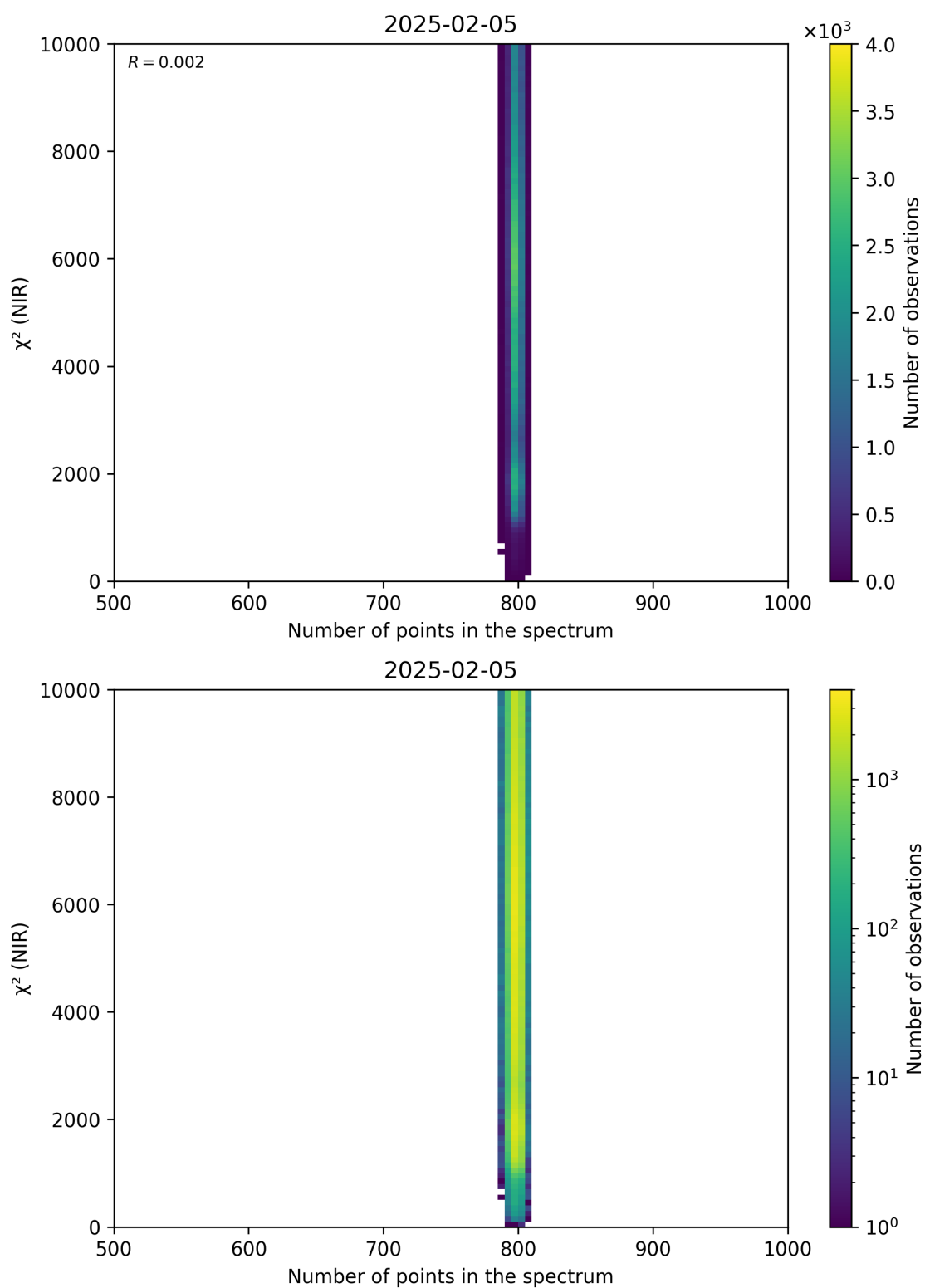
Figure 88: Scatter density plot of “Number of points in the spectrum” against “ \chi^2 (NIR)” for 2025-02-04 to 2025-02-06.
