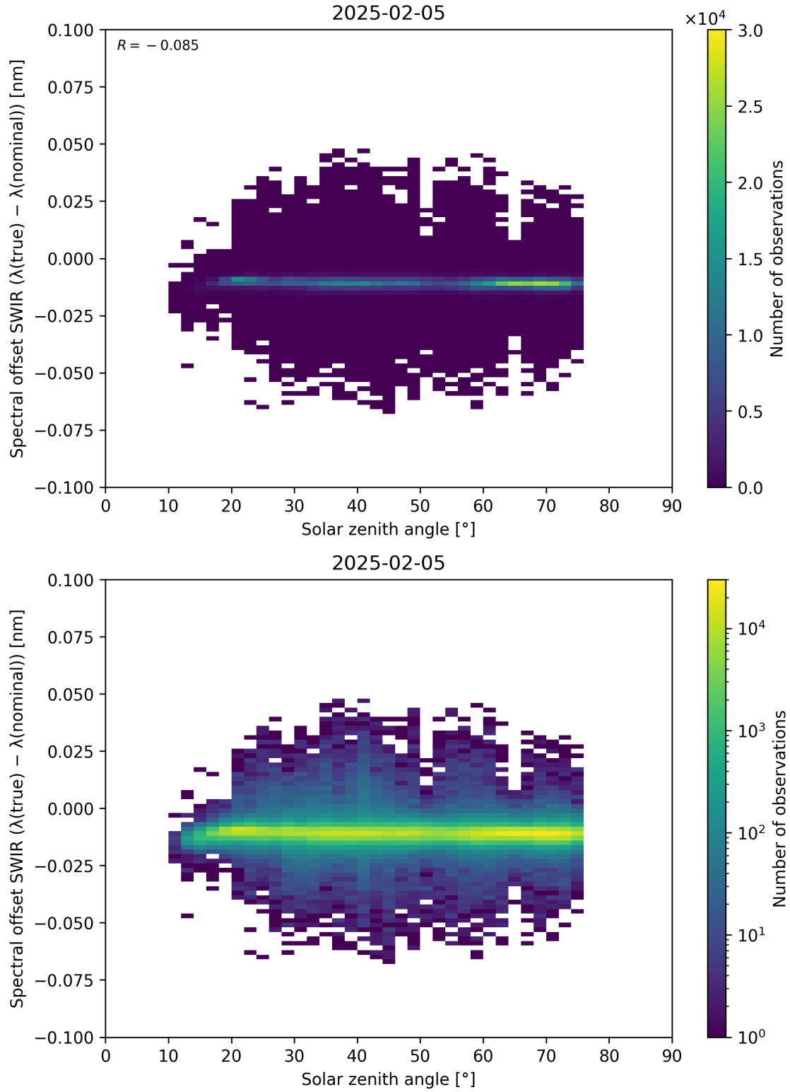
Figure 104: Scatter density plot of “Solar zenith angle” against “Spectral offset SWIR ( \lambda_{\text{true}} - \lambda_{\text{nominal}} )” for 2025-02-04 to 2025-02-06.
