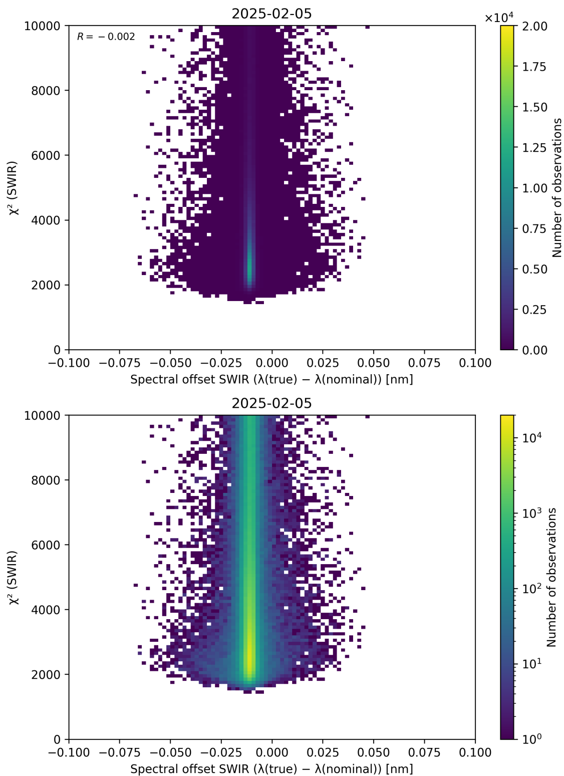
Figure 118: Scatter density plot of “Spectral offset SWIR ( \lambda_{\text{true}} - \lambda_{\text{nominal}} )” against “ \chi^2 (SWIR)” for 2025-02-04 to 2025-02-06.
