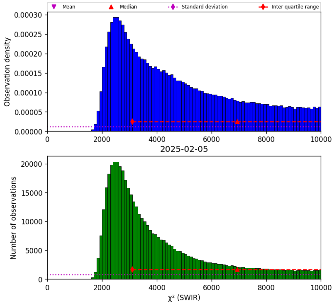
Figure 28: Histogram of “ \chi^2 (SWIR)” for 2025-02-04 to 2025-02-06
