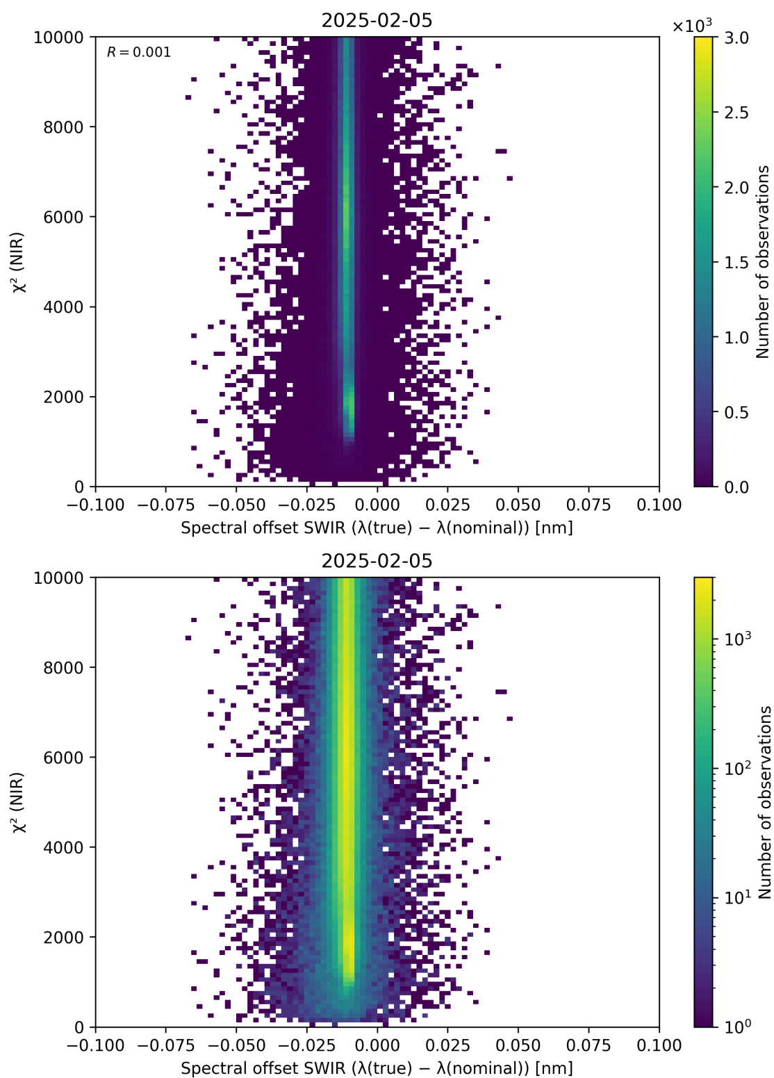
Figure 117: Scatter density plot of “Spectral offset SWIR ( \lambda_{\text{true}} - \lambda_{\text{nominal}} )” against “ \chi^2 (NIR)” for 2025-02-04 to 2025-02-06.
