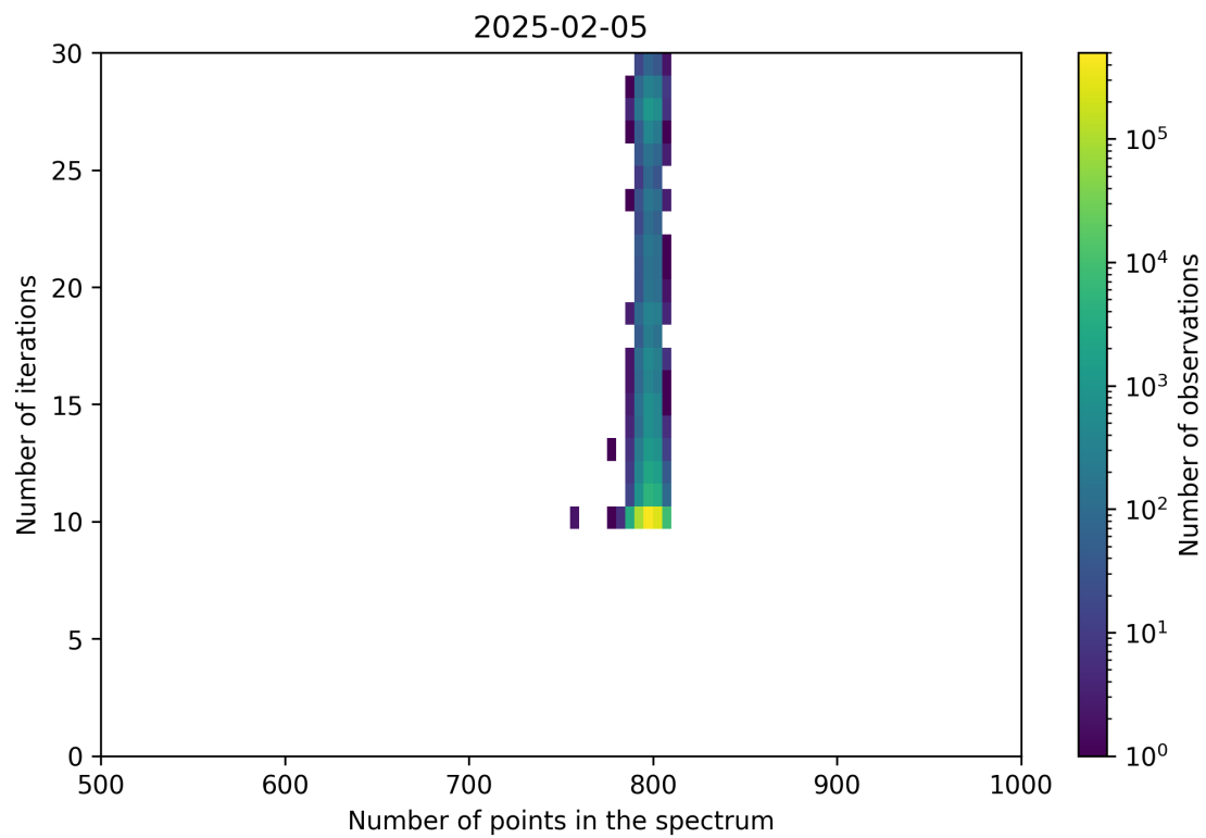
Figure 92: Scatter density plot of “Number of points in the spectrum” against “Number of iterations” for 2025-02-04 to 2025-02-06.
