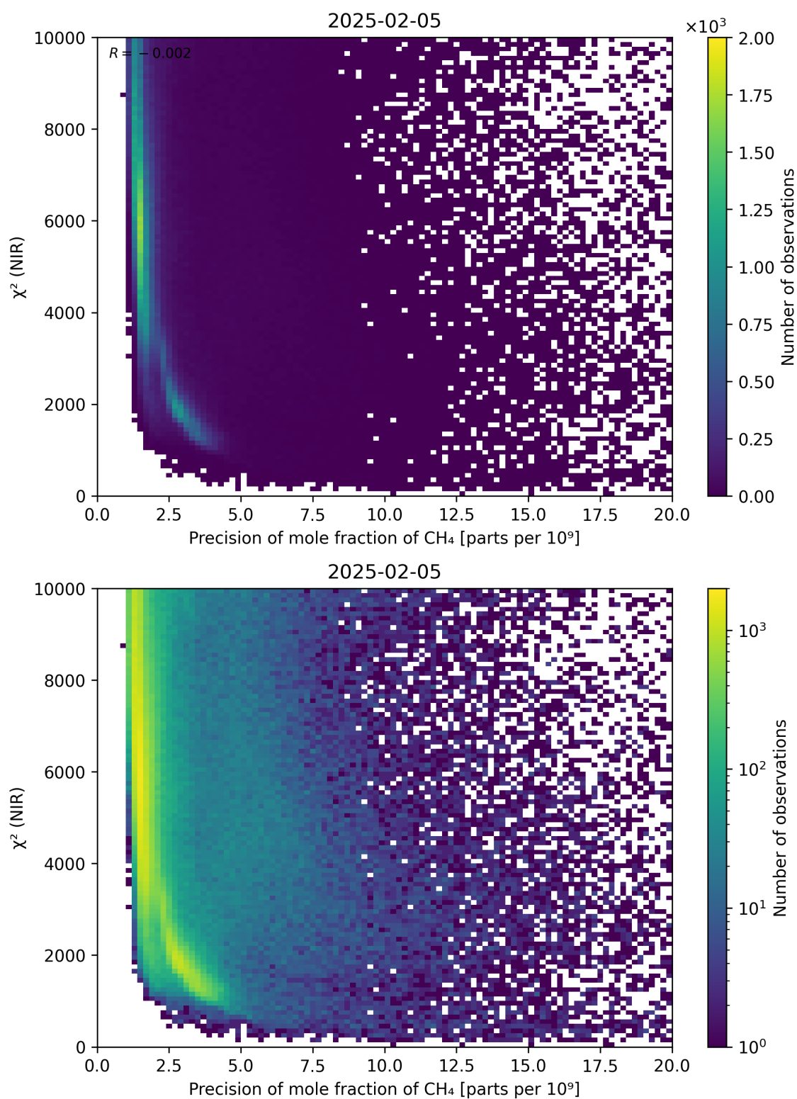
Figure 78: Scatter density plot of “Precision of mole fraction of CH 4 ” against “ \chi^2 (NIR)” for 2025-02-04 to 2025-02-06.
