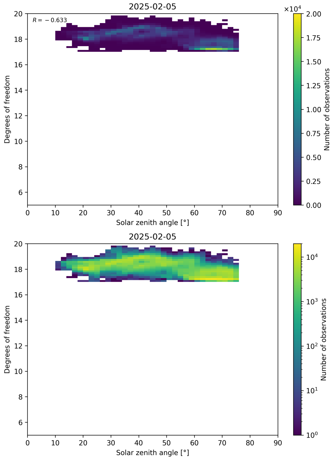
Figure 96: Scatter density plot of “Solar zenith angle” against “Degrees of freedom” for 2025-02-04 to 2025-02-06.
