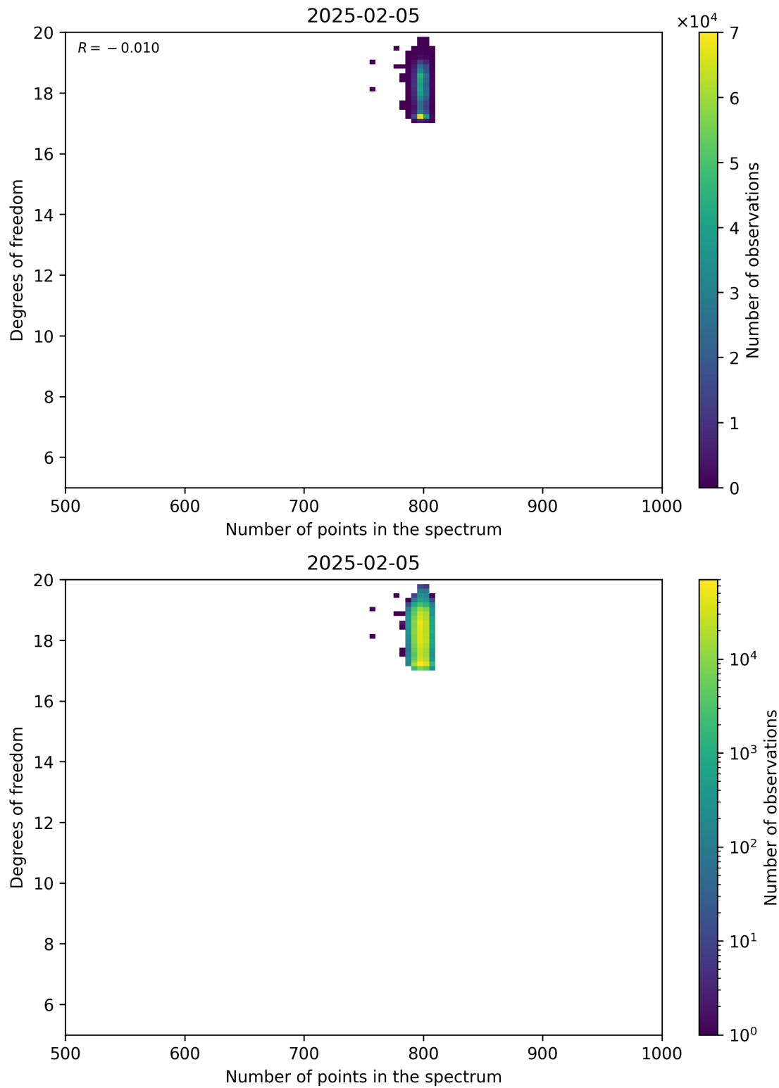
Figure 90: Scatter density plot of “Number of points in the spectrum” against “Degrees of freedom” for 2025-02-04 to 2025-02-06.
