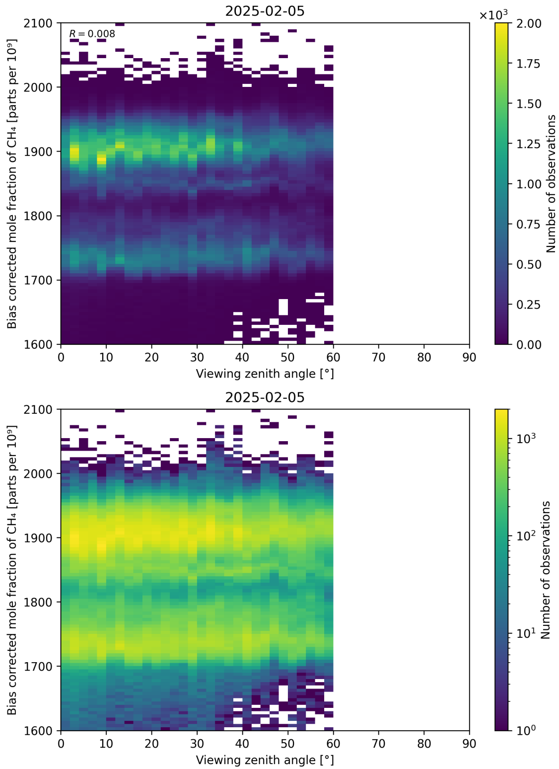
Figure 111: Scatter density plot of “Viewing zenith angle” against “Bias corrected mole fraction of CH 4 ” for 2025-02-04 to 2025-02-06.
