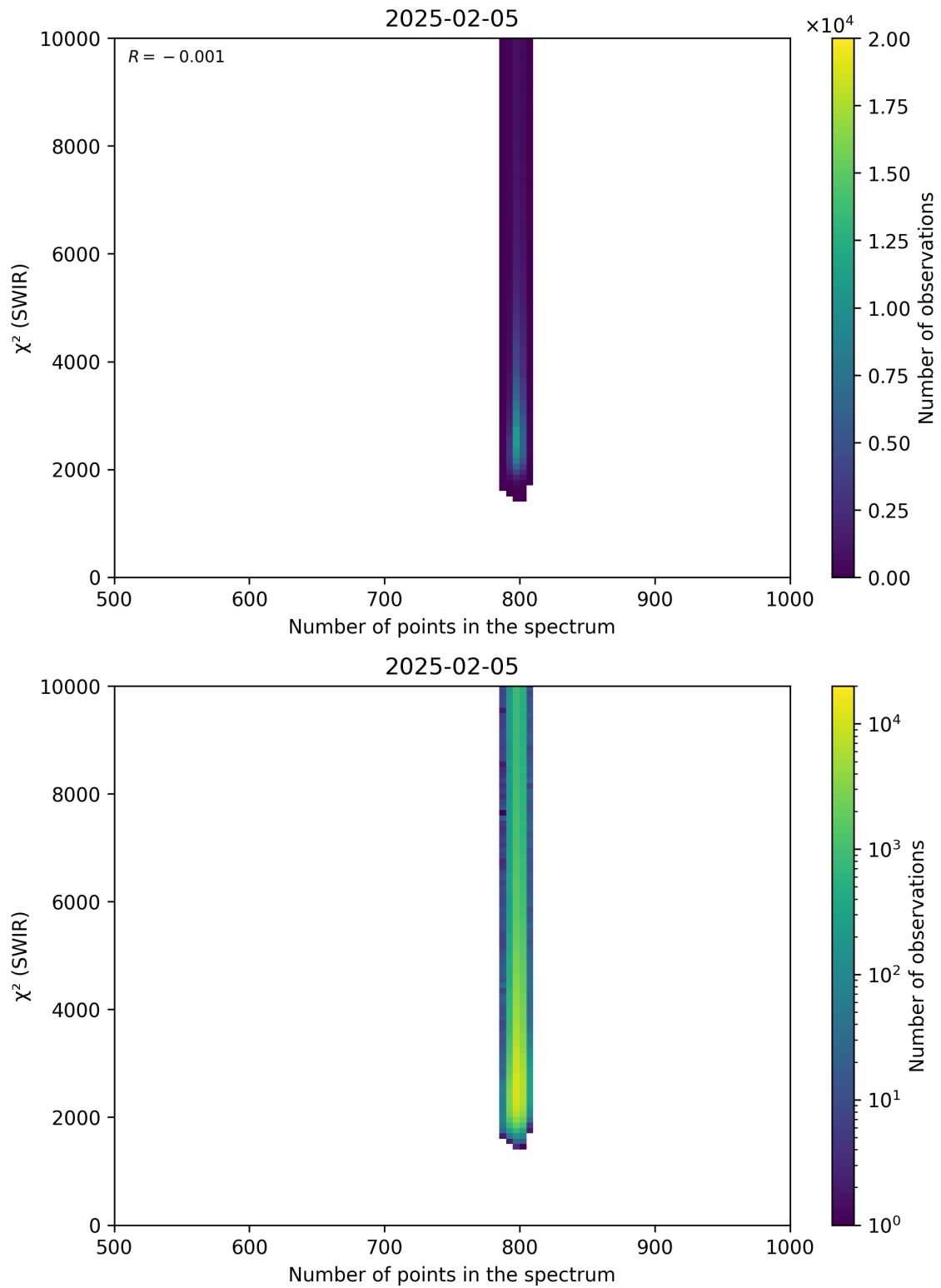
Figure 89: Scatter density plot of “Number of points in the spectrum” against “ \chi^2 (SWIR)” for 2025-02-04 to 2025-02-06.
