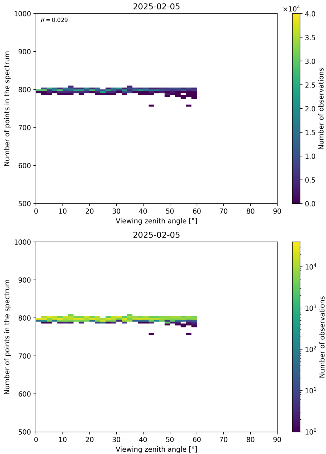
Figure 114: Scatter density plot of “Viewing zenith angle” against “Number of points in the spectrum” for 2025-02-04 to 2025-02-06.
