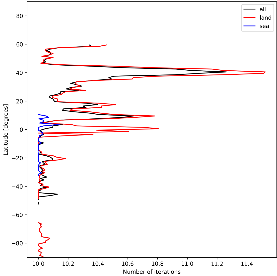
Figure 20: Zonal average of “Number of iterations” for 2025-02-04 to 2025-02-06.
