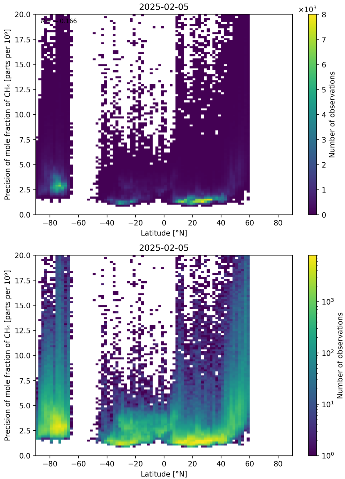
Figure 59: Scatter density plot of “Latitude” against “Precision of mole fraction of CH 4 ” for 2025-02-04 to 2025-02-06.
