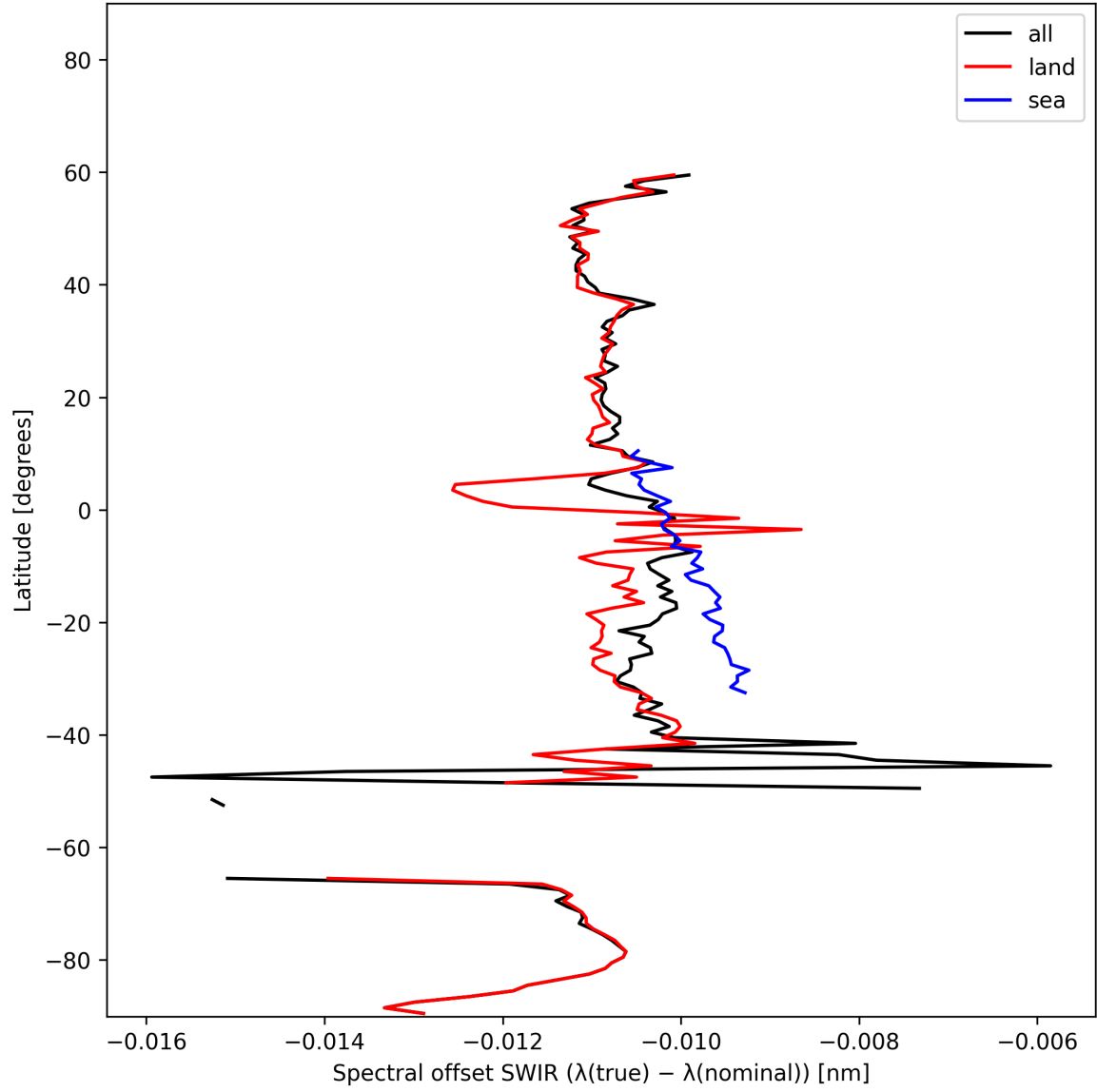
Figure 16: Zonal average of “Spectral offset SWIR ( \lambda_{\text{true}} - \lambda_{\text{nominal}} )” for 2025-02-04 to 2025-02-06.
