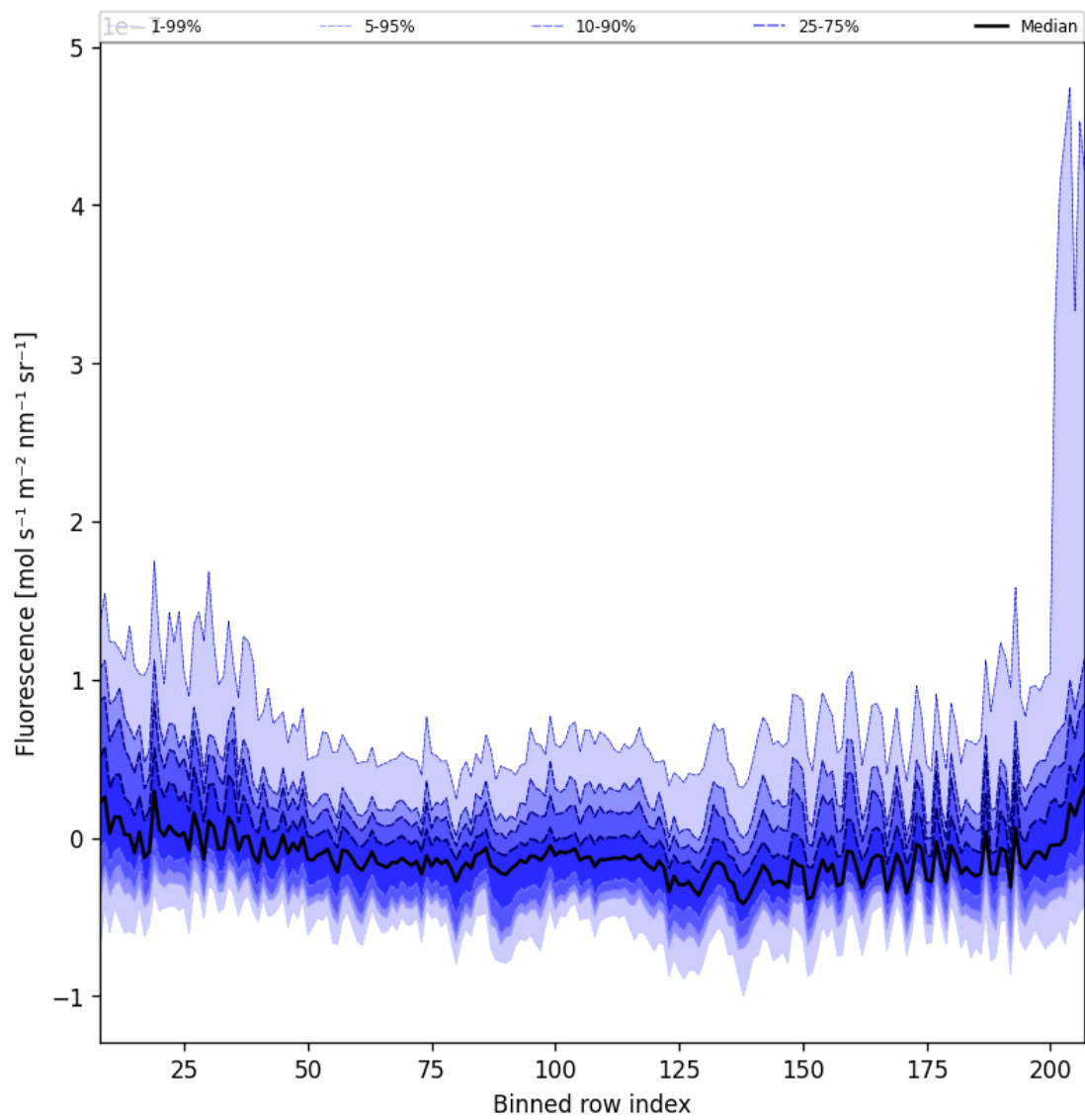
Figure 43: Along track statistics of “Fluorescence” for 2025-02-04 to 2025-02-06
