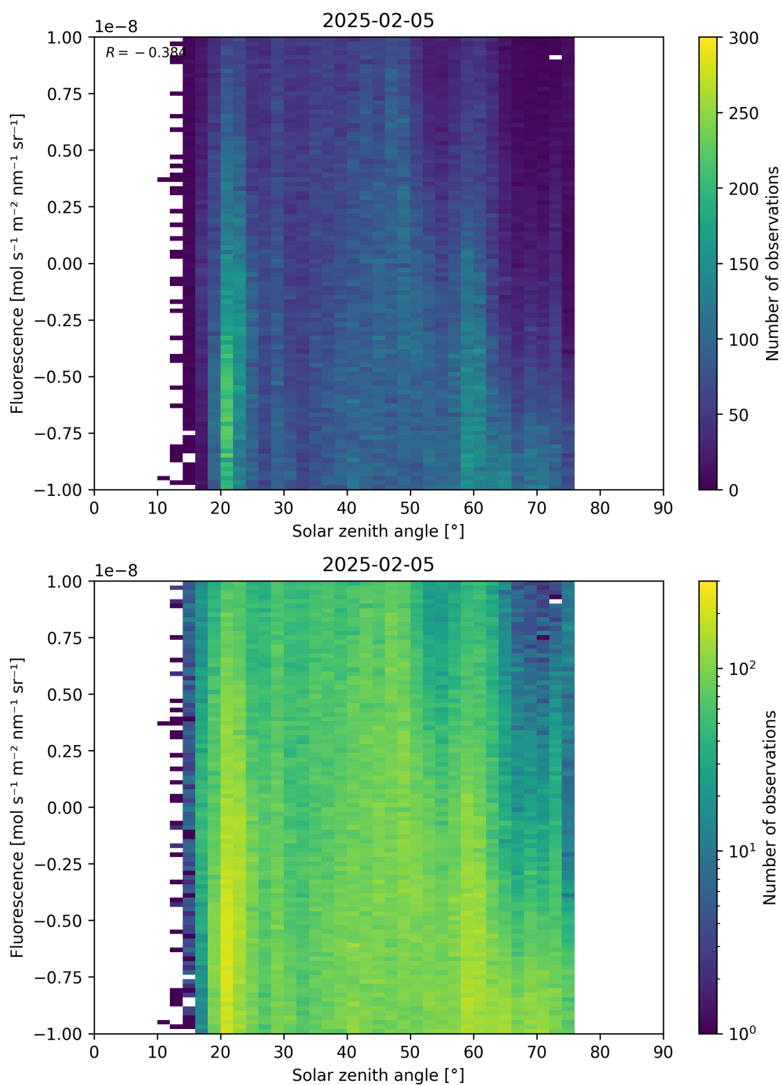
Figure 97: Scatter density plot of “Solar zenith angle” against “Fluorescence” for 2025-02-04 to 2025-02-06.
