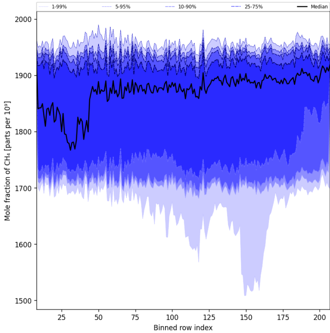
Figure 34: Along track statistics of “Mole fraction of CH 4 ” for 2025-02-04 to 2025-02-06
