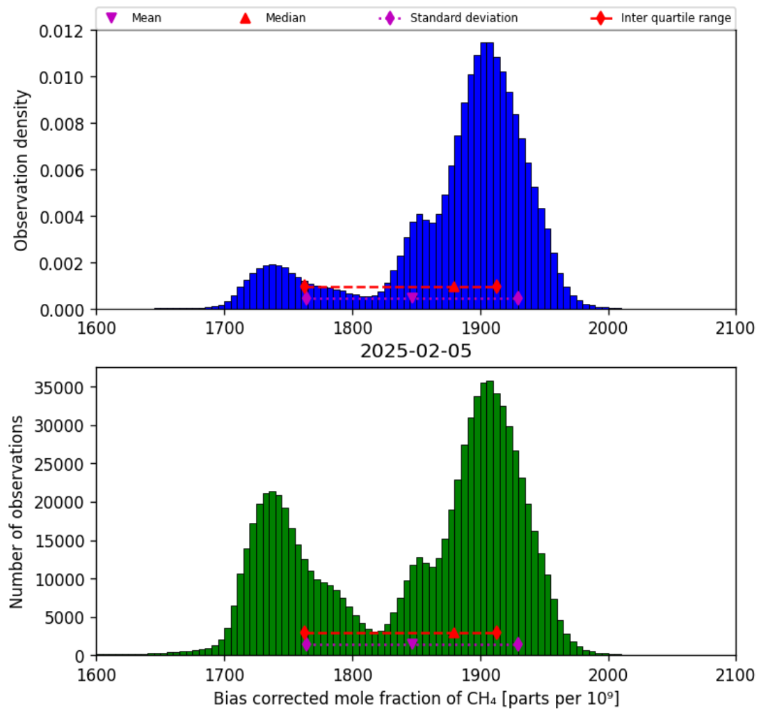
Figure 25: Histogram of “Bias corrected mole fraction of CH 4 ” for 2025-02-04 to 2025-02-06
