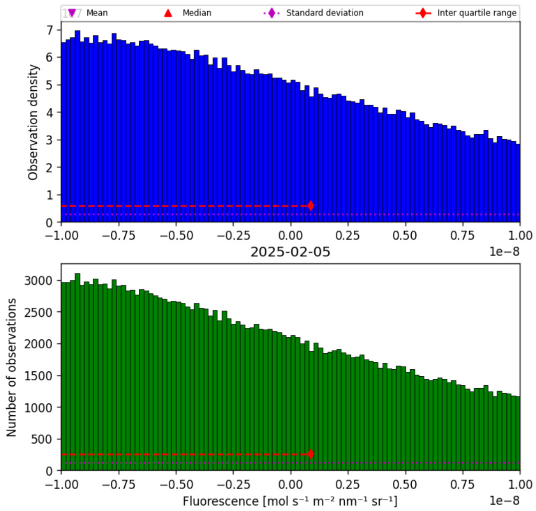
Figure 32: Histogram of “Fluorescence” for 2025-02-04 to 2025-02-06
