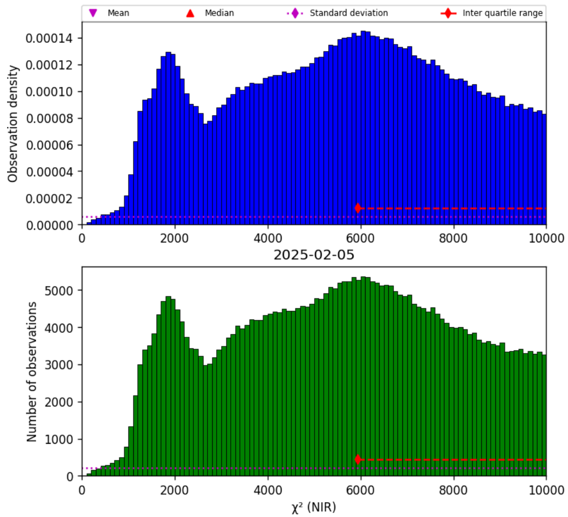
Figure 29: Histogram of " \chi^2 (NIR)" for 2025-02-04 to 2025-02-06
