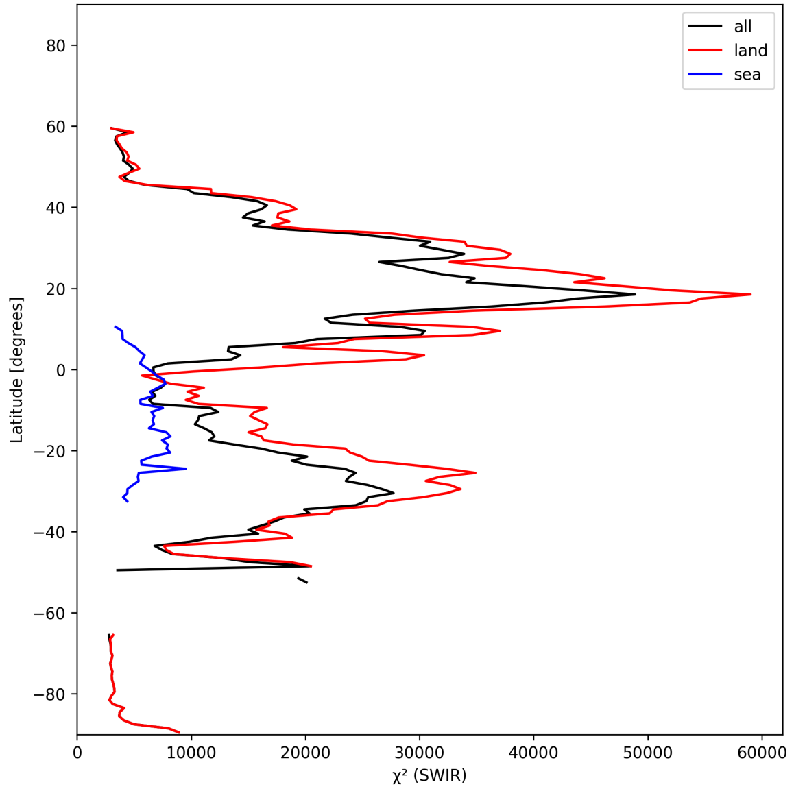
Figure 17: Zonal average of “ \chi^2 (SWIR)” for 2025-02-04 to 2025-02-06.
