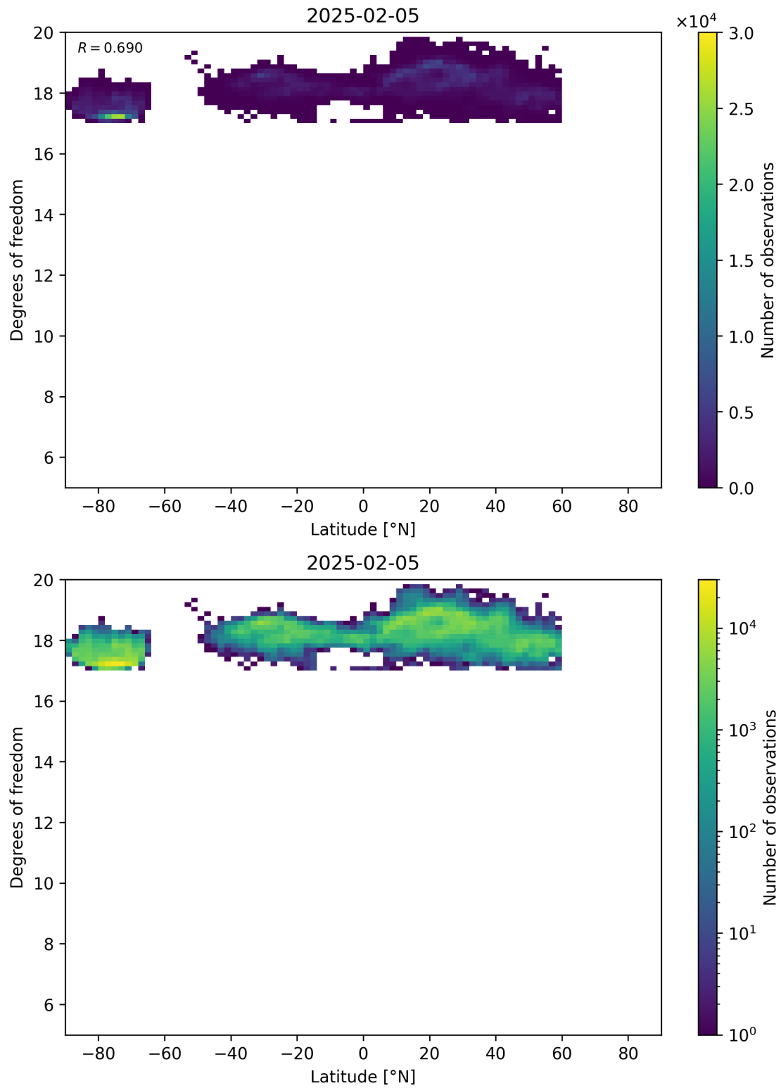
Figure 55: Scatter density plot of “Latitude” against “Degrees of freedom” for 2025-02-04 to 2025-02-06.
