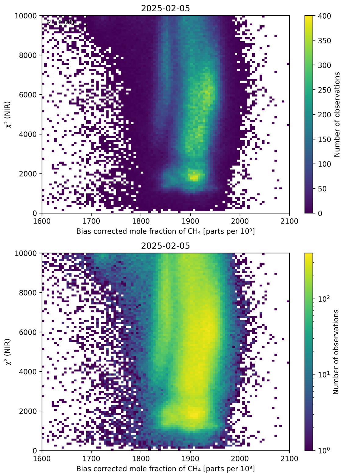
Figure 63: Scatter density plot of “Bias corrected mole fraction of \text{CH}_4 ” against “ \chi^2 (NIR)” for 2025-02-04 to 2025-02-06.
