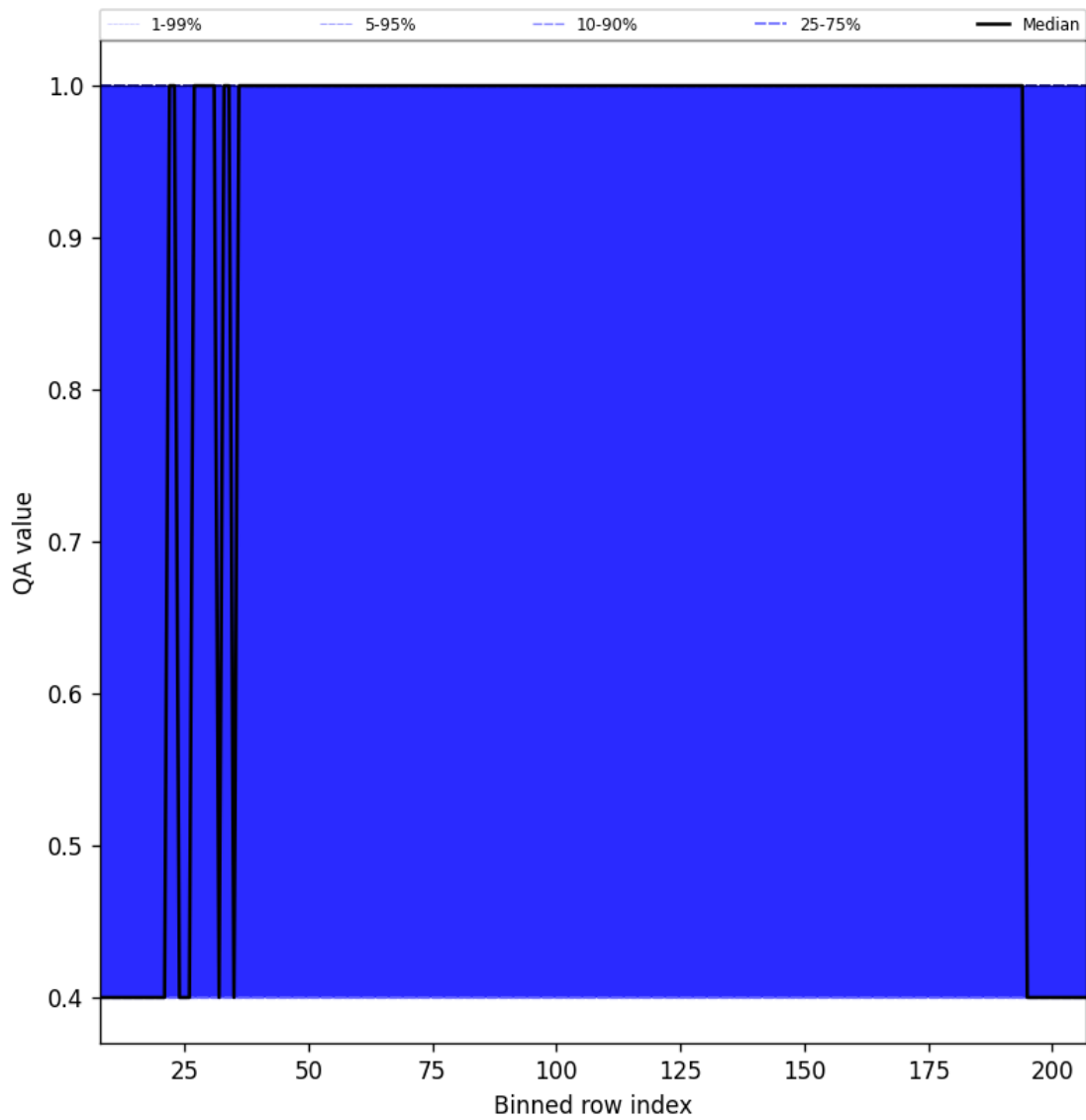
Figure 33: Along track statistics of “QA value” for 2025-02-04 to 2025-02-06
