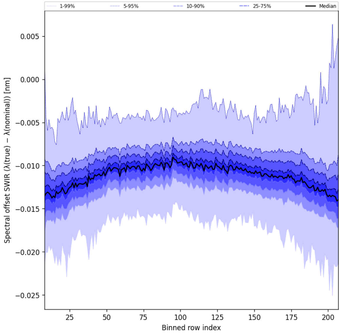
Figure 38: Along track statistics of “Spectral offset SWIR ( \lambda_{\text{true}} - \lambda_{\text{nominal}} )” for 2025-02-04 to 2025-02-06
