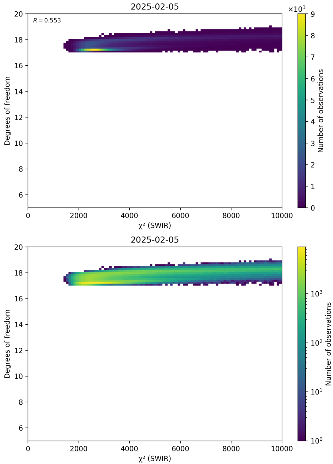
Figure 48: Scatter density plot of “ \chi^2 (SWIR)” against “Degrees of freedom” for 2025-02-04 to 2025-02-06.
