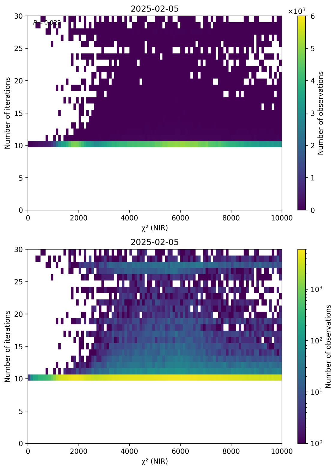
Figure 46: Scatter density plot of “ \chi^2 (NIR)” against “Number of iterations” for 2025-02-04 to 2025-02-06.
