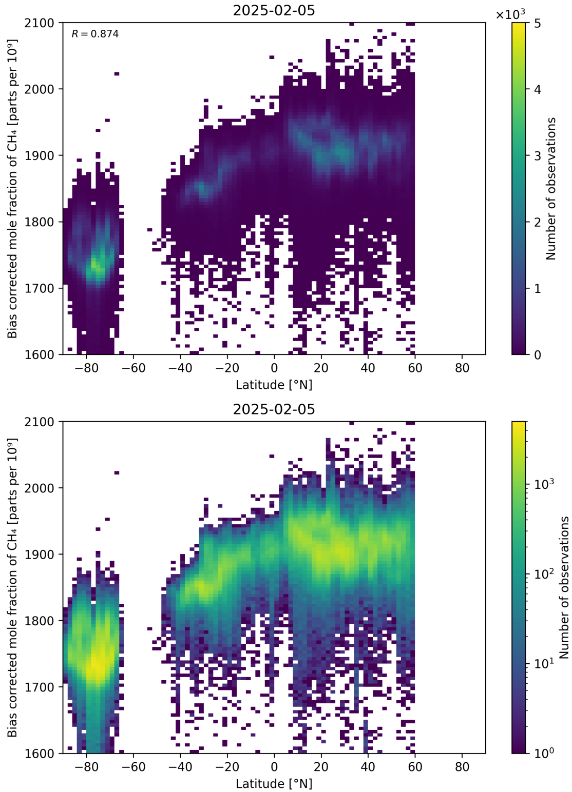
Figure 58: Scatter density plot of “Latitude” against “Bias corrected mole fraction of \text{CH}_4 ” for 2025-02-04 to 2025-02-06.
