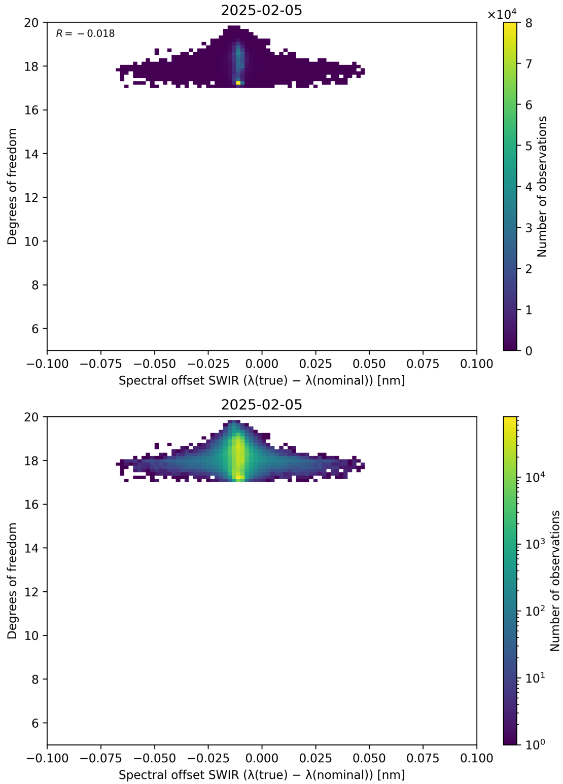
Figure 119: Scatter density plot of “Spectral offset SWIR ( \lambda_{\text{true}} - \lambda_{\text{nominal}} )” against “Degrees of freedom” for 2025-02-04 to 2025-02-06.
