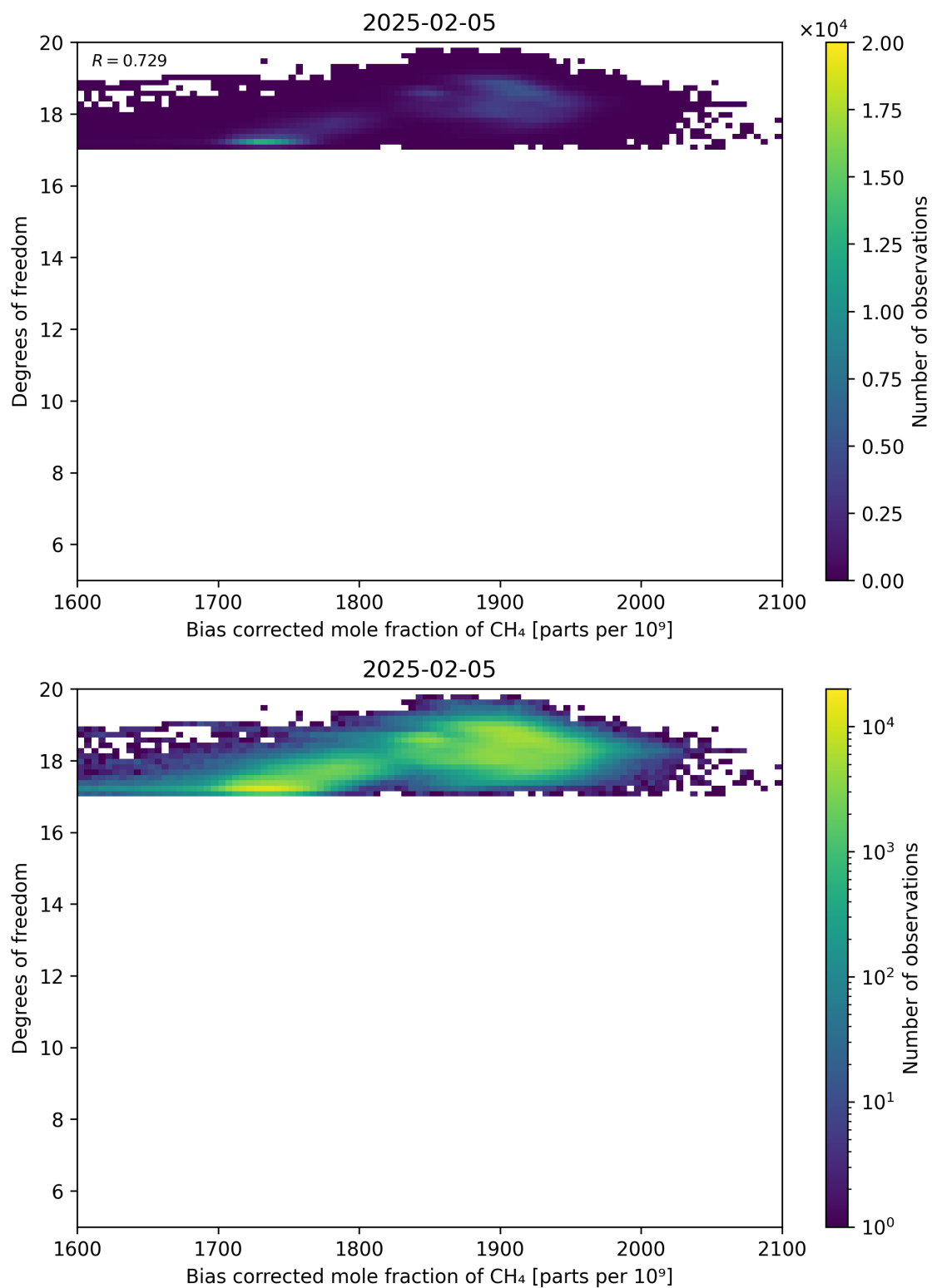
Figure 65: Scatter density plot of “Bias corrected mole fraction of CH 4 ” against “Degrees of freedom” for 2025-02-04 to 2025-02-06.
