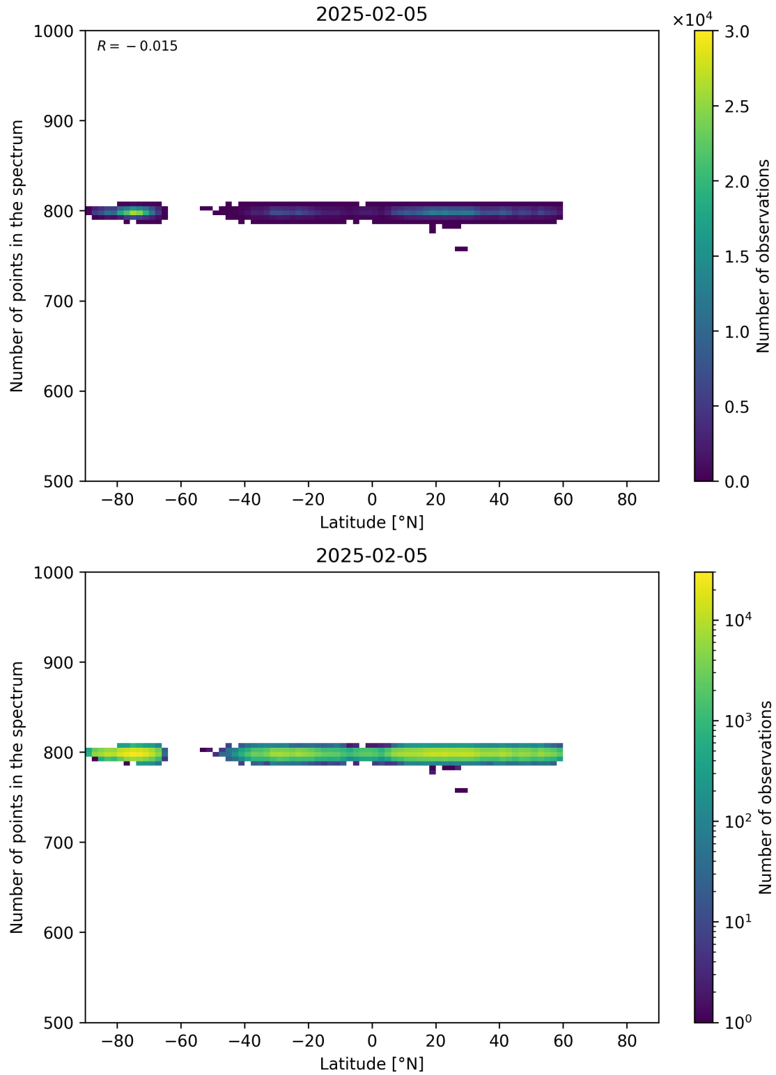
Figure 61: Scatter density plot of “Latitude” against “Number of points in the spectrum” for 2025-02-04 to 2025-02-06.
