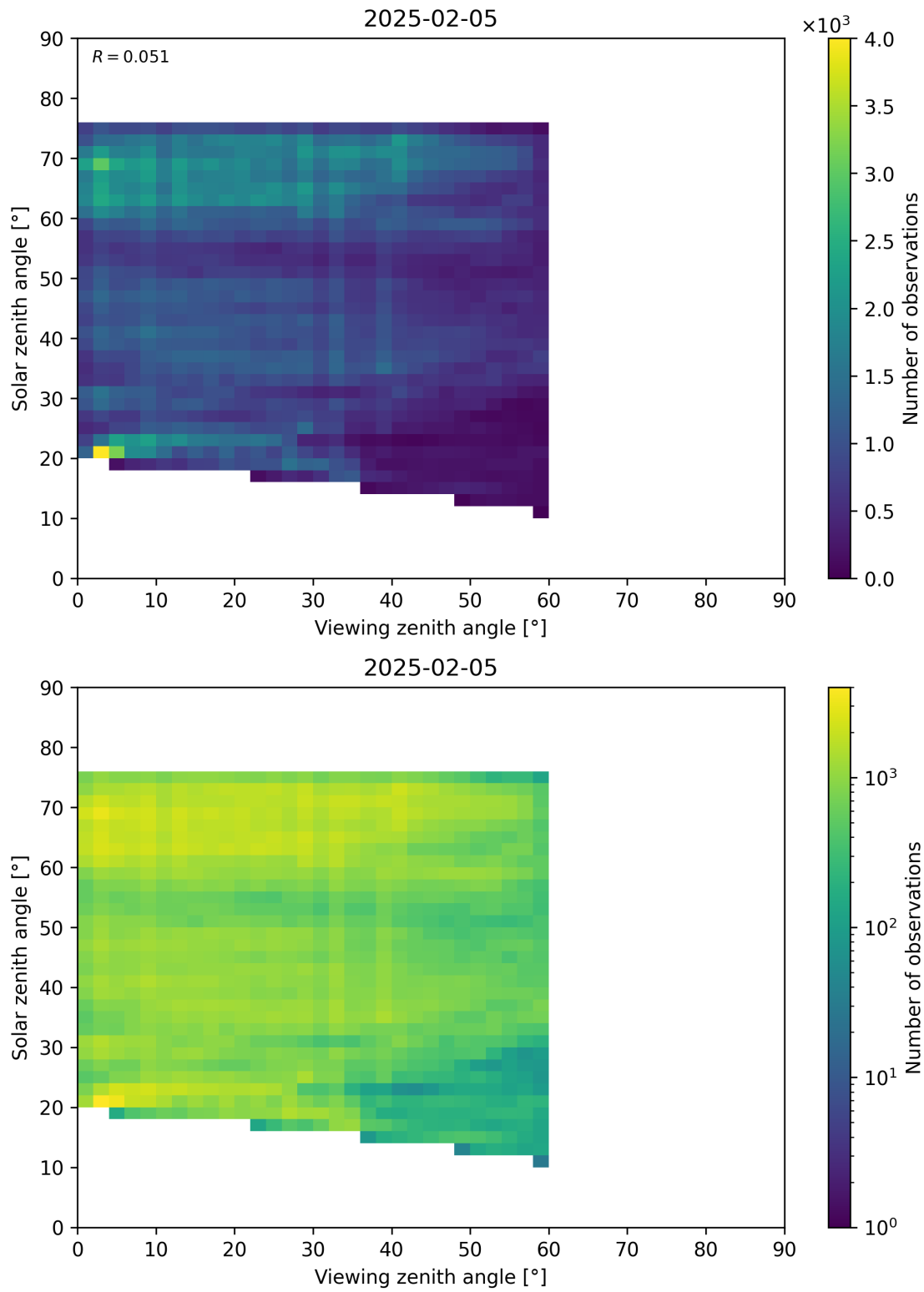
Figure 115: Scatter density plot of “Viewing zenith angle” against “Solar zenith angle” for 2025-02-04 to 2025-02-06.
