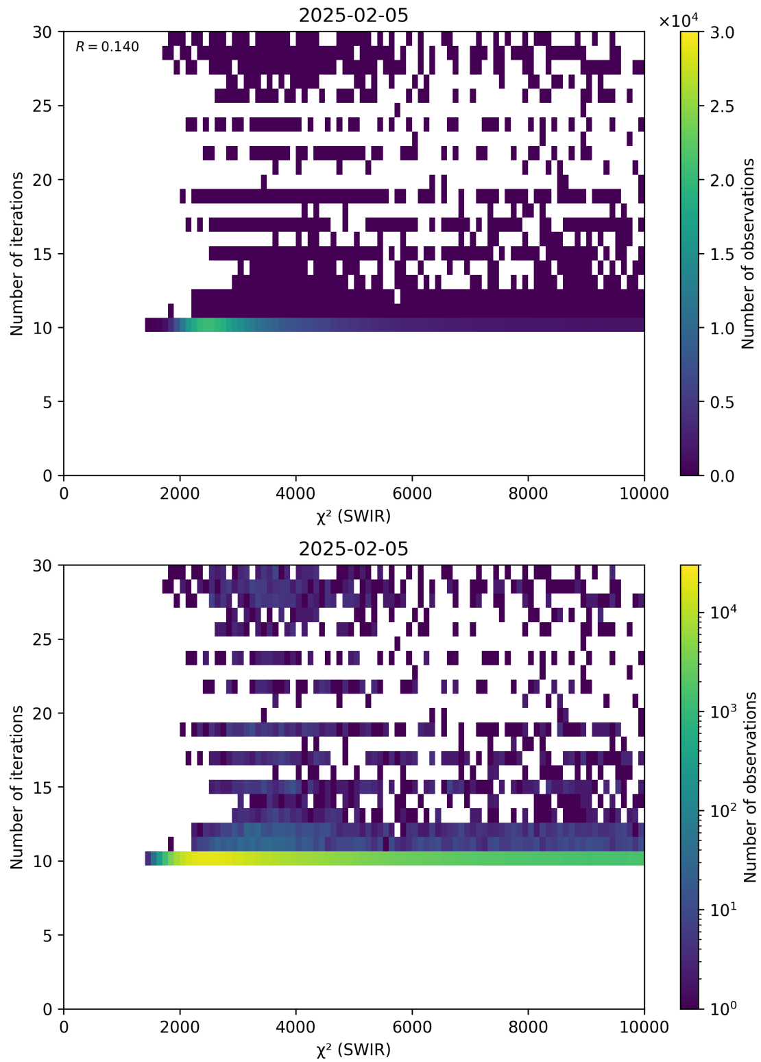
Figure 50: Scatter density plot of “ \chi^2 (SWIR)” against “Number of iterations” for 2025-02-04 to 2025-02-06.
