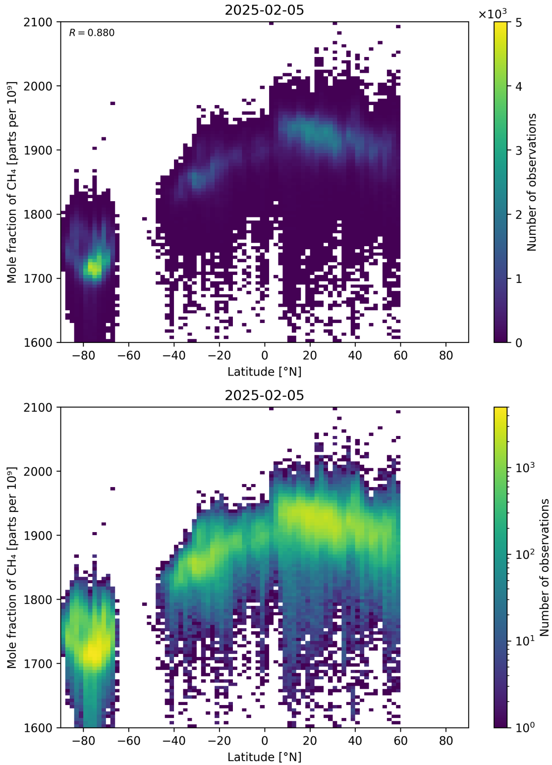
Figure 57: Scatter density plot of “Latitude” against “Mole fraction of CH 4 ” for 2025-02-04 to 2025-02-06.
