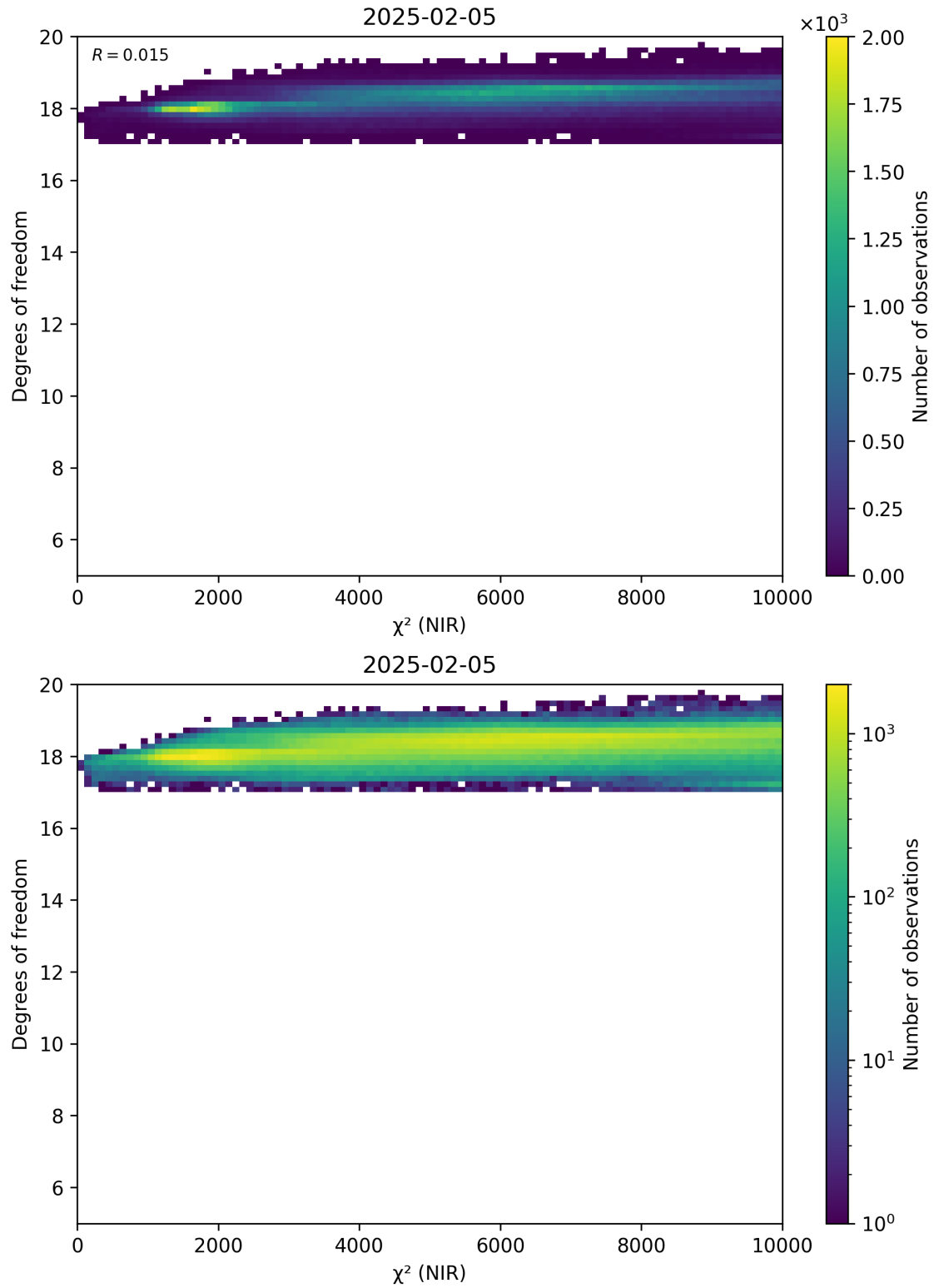
Figure 44: Scatter density plot of “ \chi^2 (NIR)” against “Degrees of freedom” for 2025-02-04 to 2025-02-06.
