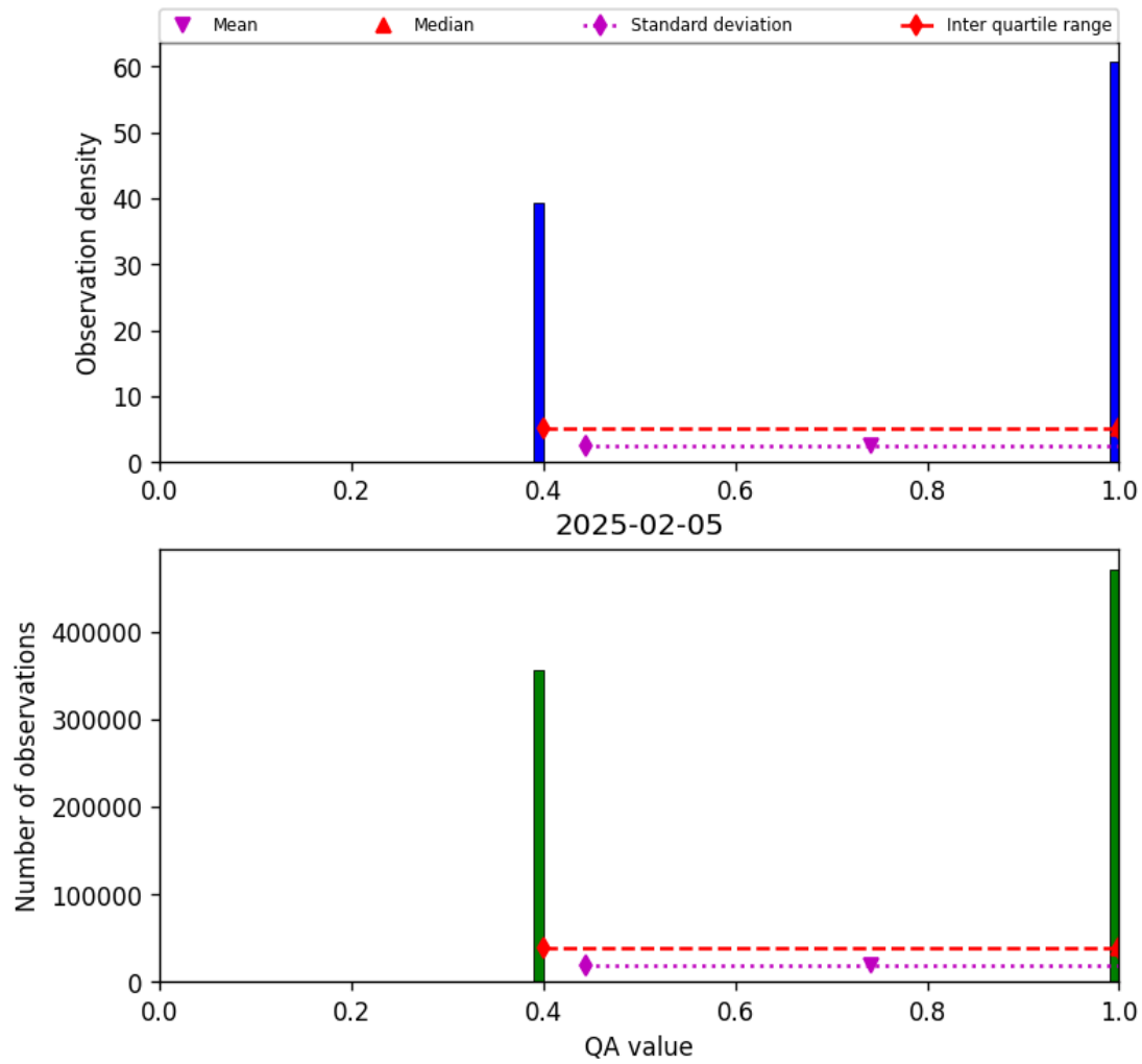
Figure 22: Histogram of “QA value” for 2025-02-04 to 2025-02-06
