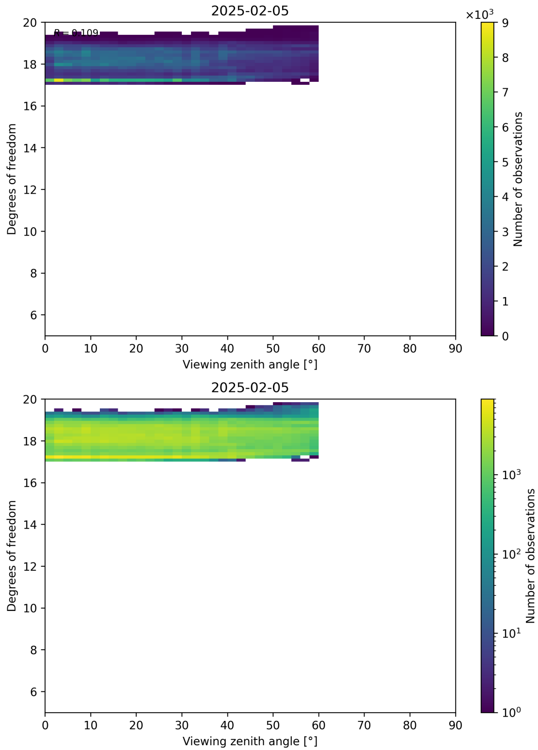
Figure 107: Scatter density plot of “Viewing zenith angle” against “Degrees of freedom” for 2025-02-04 to 2025-02-06.
