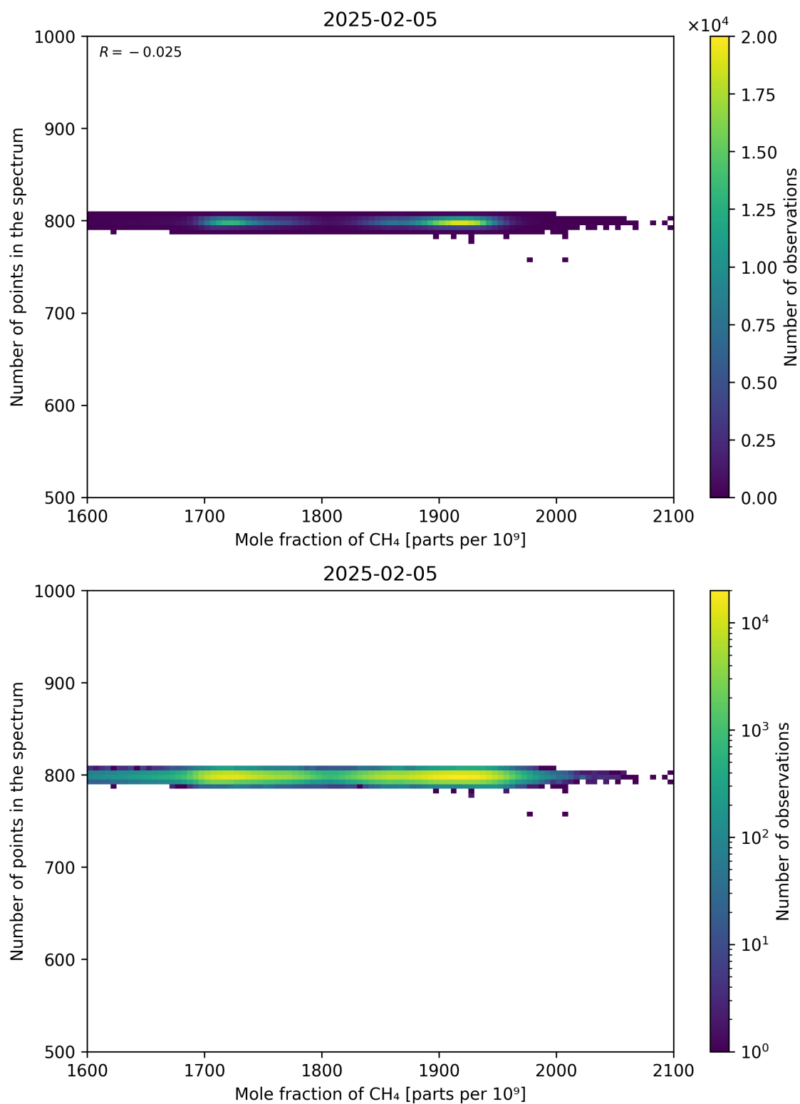
Figure 77: Scatter density plot of “Mole fraction of CH 4 ” against “Number of points in the spectrum” for 2025-02-04 to 2025-02-06.
