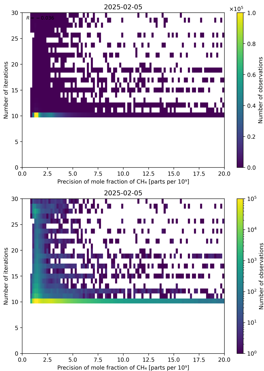
Figure 83: Scatter density plot of “Precision of mole fraction of CH 4 ” against “Number of iterations” for 2025-02-04 to 2025-02-06.
