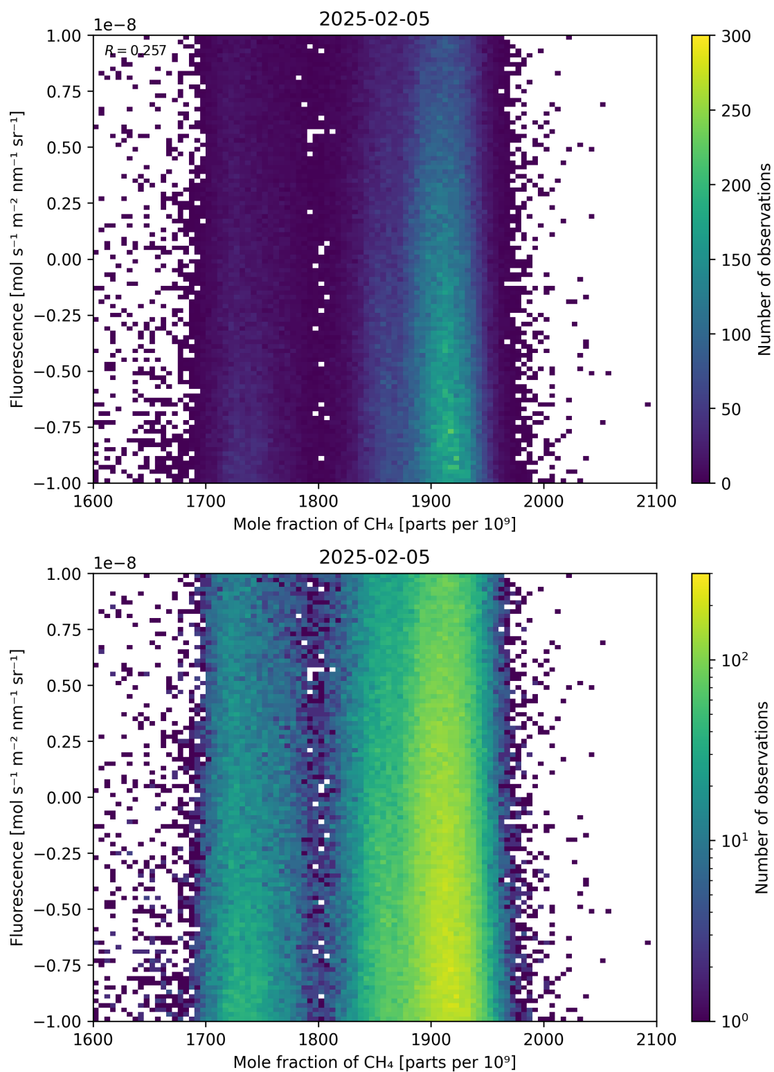
Figure 73: Scatter density plot of “Mole fraction of \text{CH}_4 ” against “Fluorescence” for 2025-02-04 to 2025-02-06.
