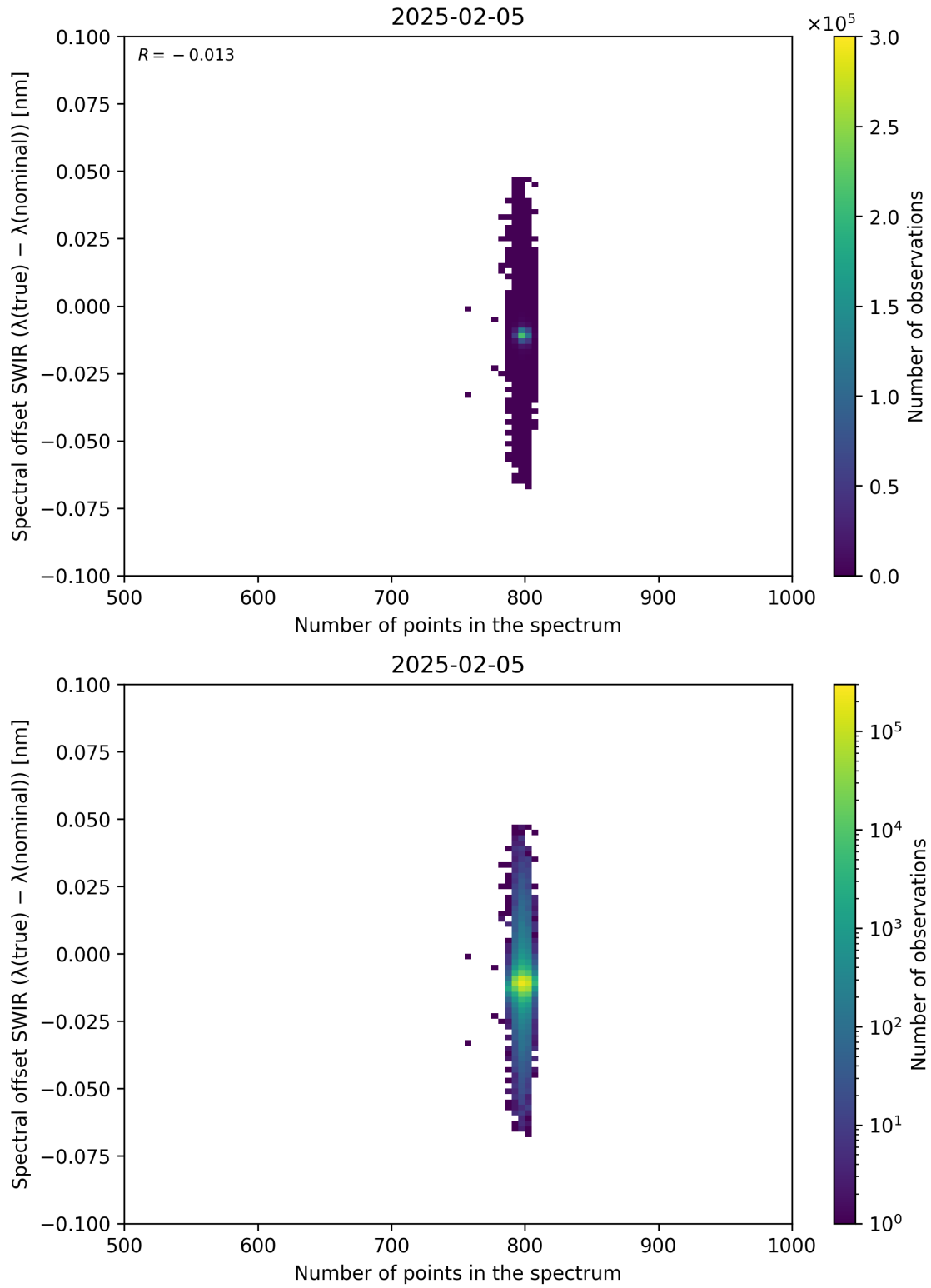
Figure 93: Scatter density plot of “Number of points in the spectrum” against “Spectral offset SWIR ( \lambda_{\text{true}} - \lambda_{\text{nominal}} )” for 2025-02-04 to 2025-02-06.
