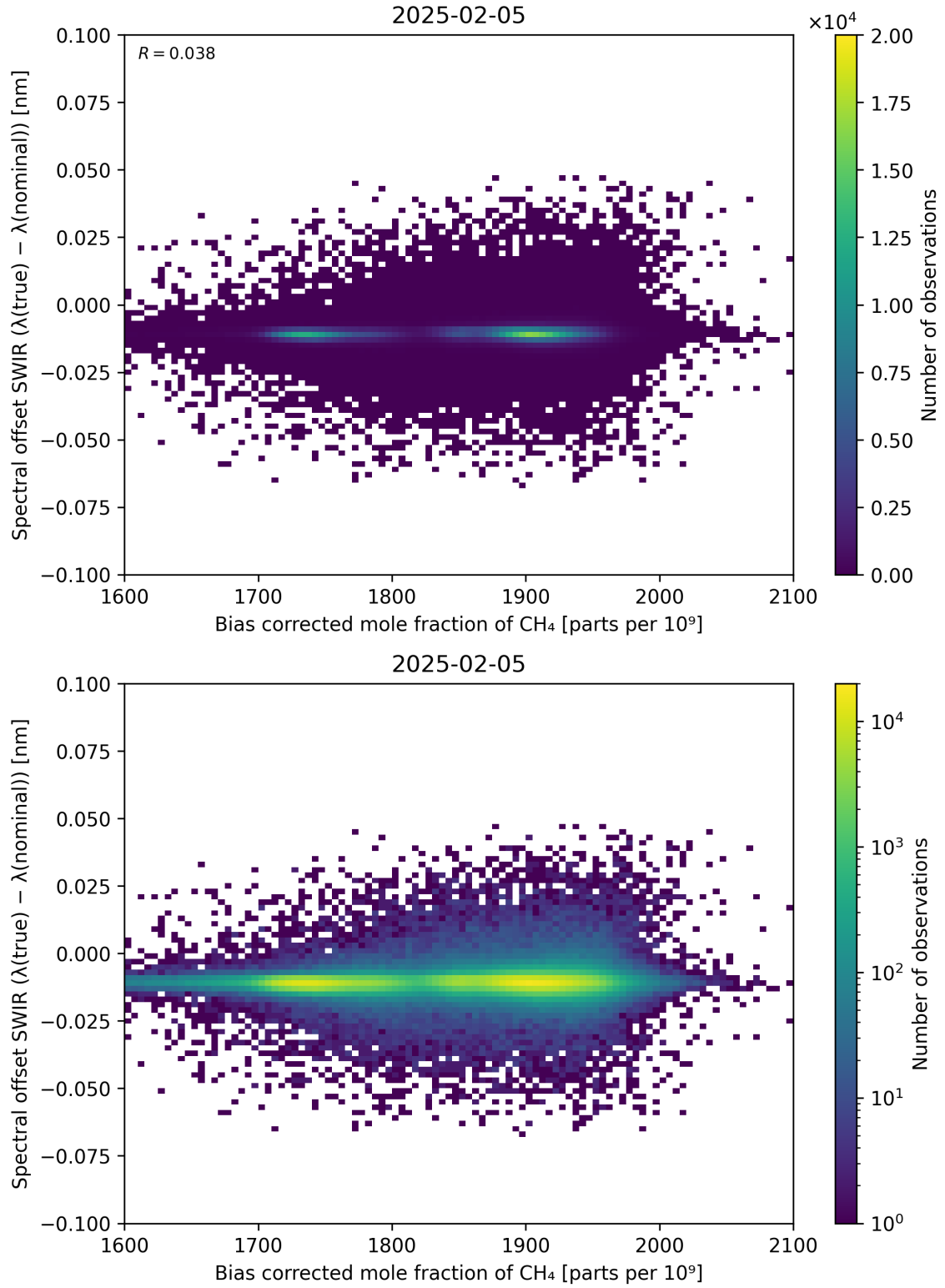
Figure 69: Scatter density plot of “Bias corrected mole fraction of \text{CH}_4 ” against “Spectral offset SWIR ( \lambda_{\text{true}} - \lambda_{\text{nominal}} )” for 2025-02-04 to 2025-02-06.
