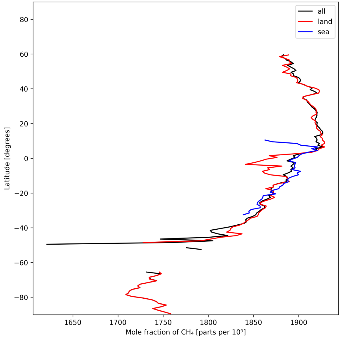
Figure 12: Zonal average of “Mole fraction of \text{CH}_4 ” for 2025-02-04 to 2025-02-06.
