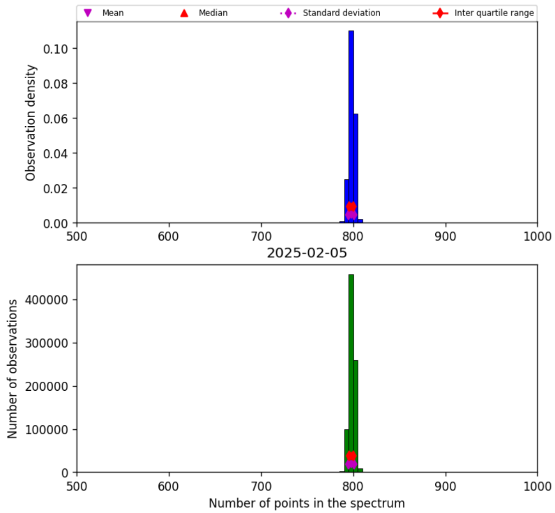
Figure 26: Histogram of “Number of points in the spectrum” for 2025-02-04 to 2025-02-06
