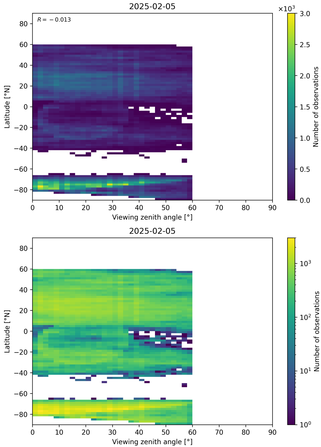
Figure 109: Scatter density plot of “Viewing zenith angle” against “Latitude” for 2025-02-04 to 2025-02-06.
