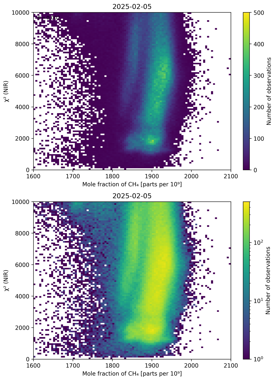
Figure 70: Scatter density plot of “Mole fraction of CH 4 ” against “ \chi^2 (NIR)” for 2025-02-04 to 2025-02-06.
