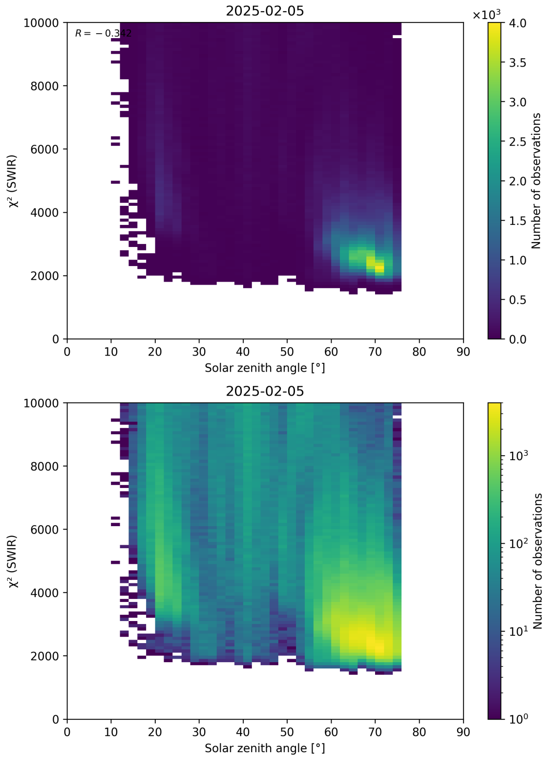
Figure 95: Scatter density plot of “Solar zenith angle” against “ \chi^2 (SWIR)” for 2025-02-04 to 2025-02-06.
