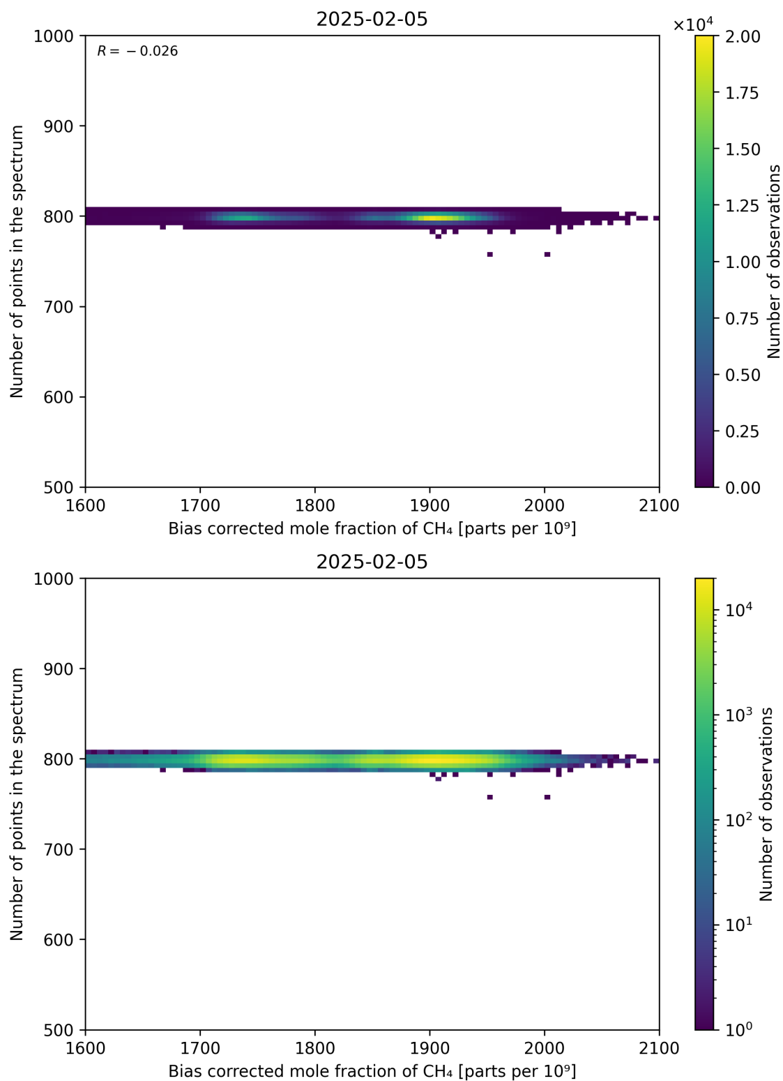
Figure 68: Scatter density plot of “Bias corrected mole fraction of CH 4 ” against “Number of points in the spectrum” for 2025-02-04 to 2025-02-06.
