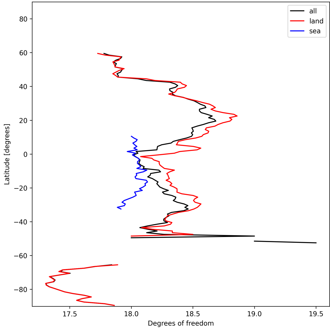
Figure 19: Zonal average of “Degrees of freedom” for 2025-02-04 to 2025-02-06.
