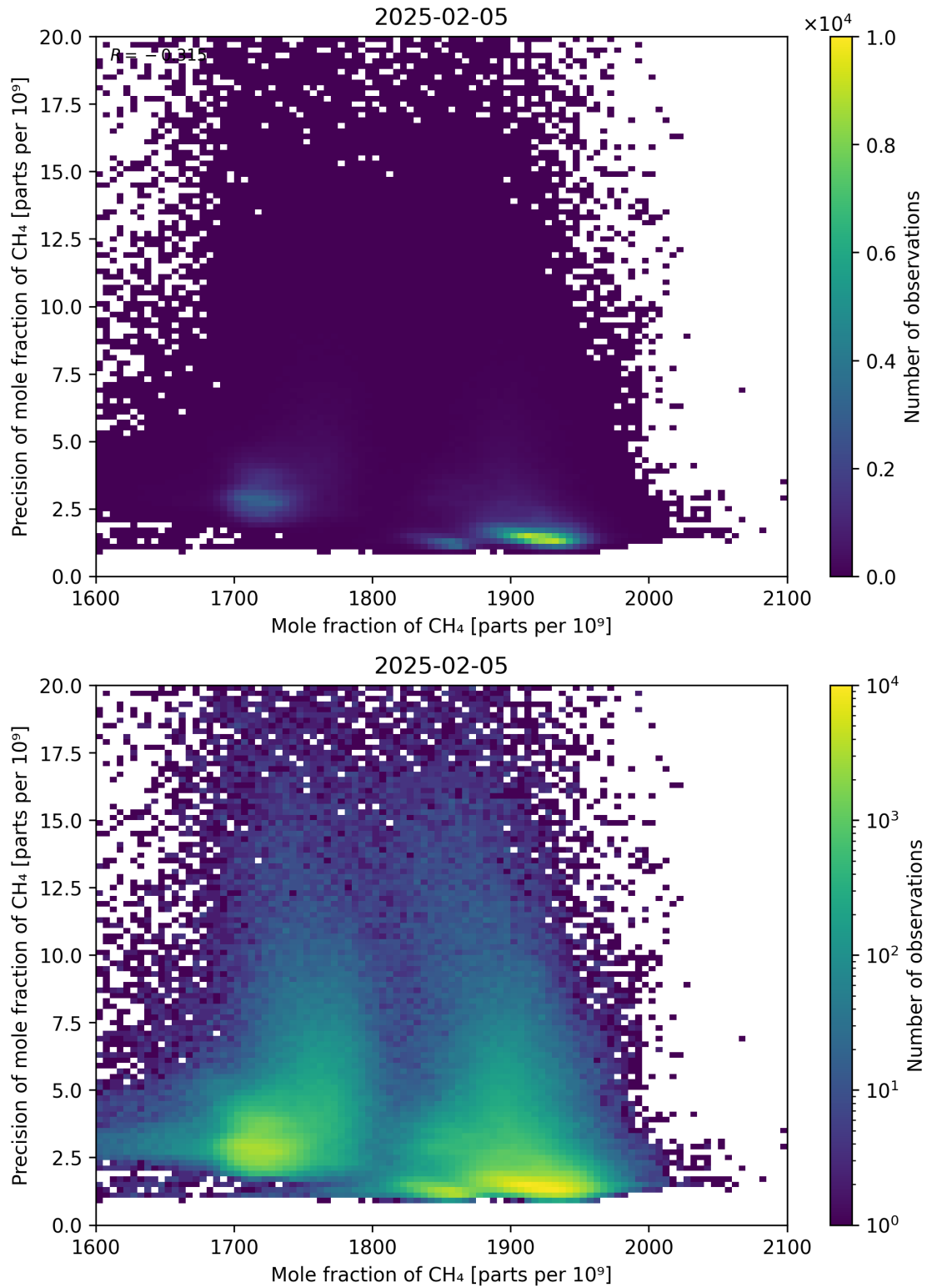
Figure 75: Scatter density plot of “Mole fraction of CH 4 ” against “Precision of mole fraction of CH 4 ” for 2025-02-04 to 2025-02-06.
