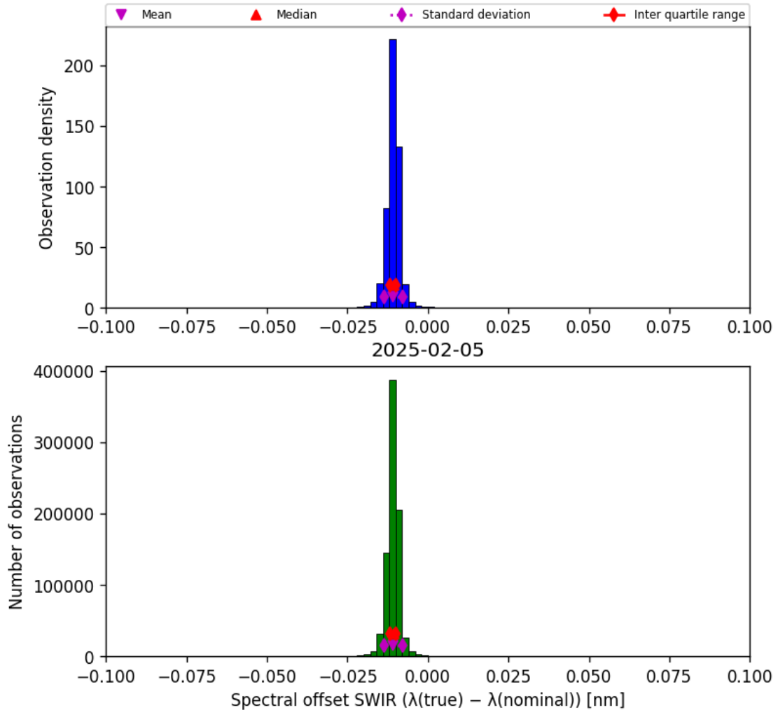
Figure 27: Histogram of “Spectral offset SWIR ( \lambda_{\text{true}} - \lambda_{\text{nominal}} )” for 2025-02-04 to 2025-02-06
