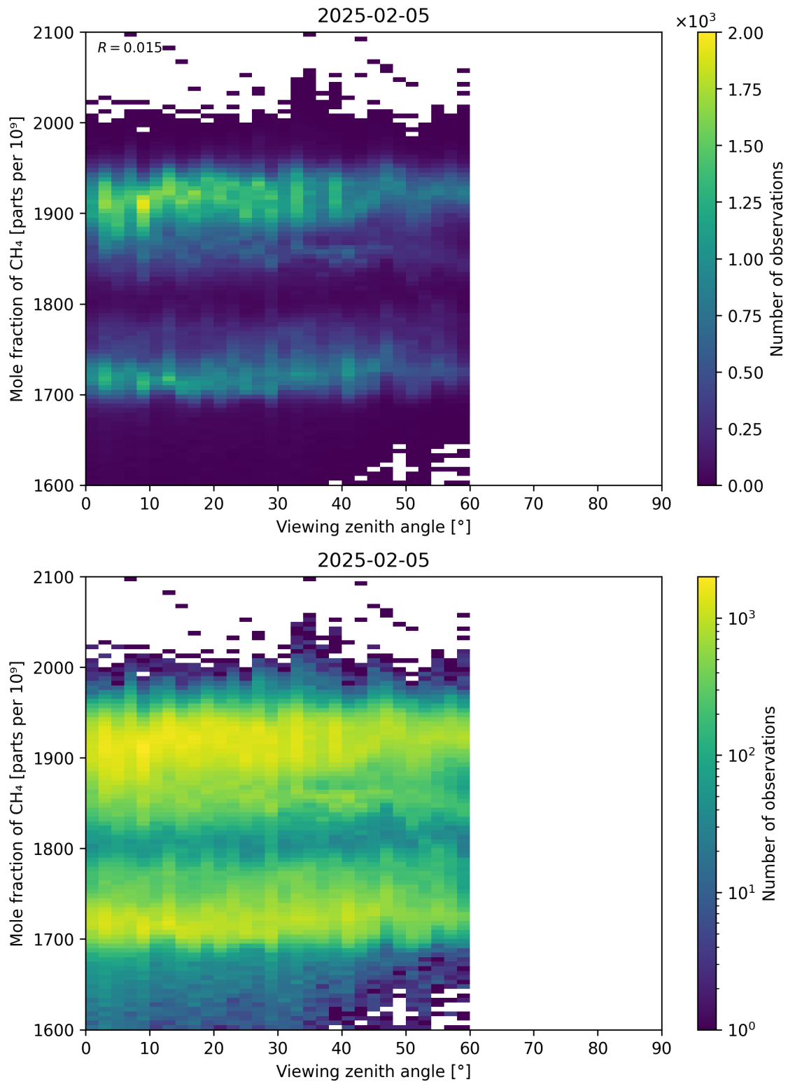
Figure 110: Scatter density plot of “Viewing zenith angle” against “Mole fraction of CH 4 ” for 2025-02-04 to 2025-02-06.
