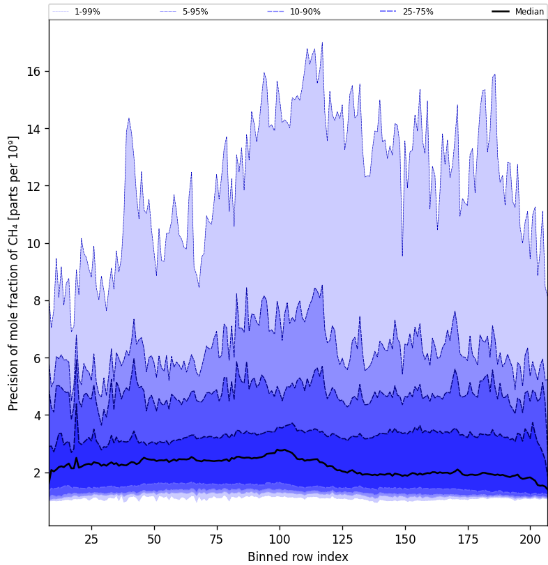
Figure 35: Along track statistics of “Precision of mole fraction of CH 4 ” for 2025-02-04 to 2025-02-06
