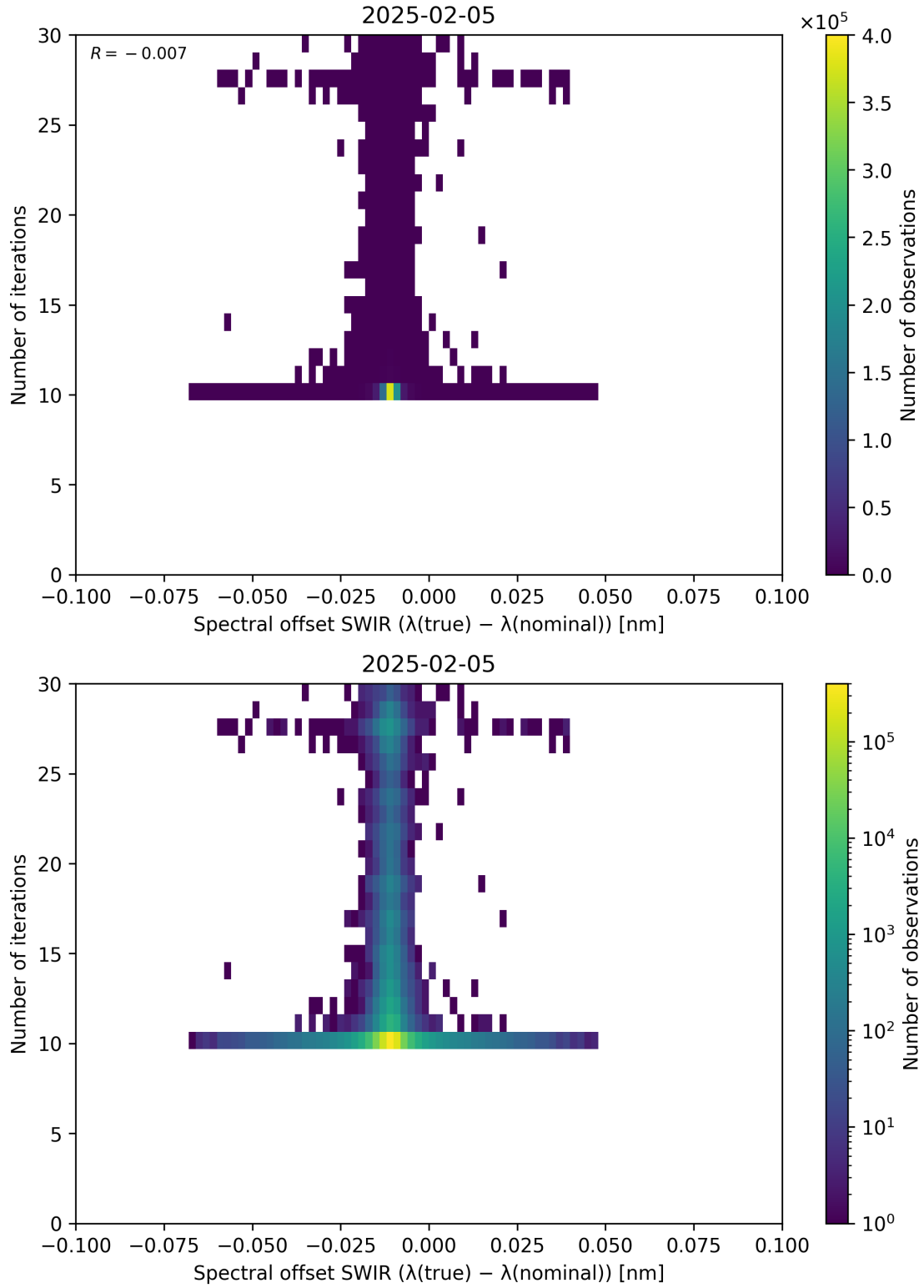
Figure 121: Scatter density plot of “Spectral offset SWIR ( \lambda_{\text{true}} - \lambda_{\text{nominal}} )” against “Number of iterations” for 2025-02-04 to 2025-02-06.
