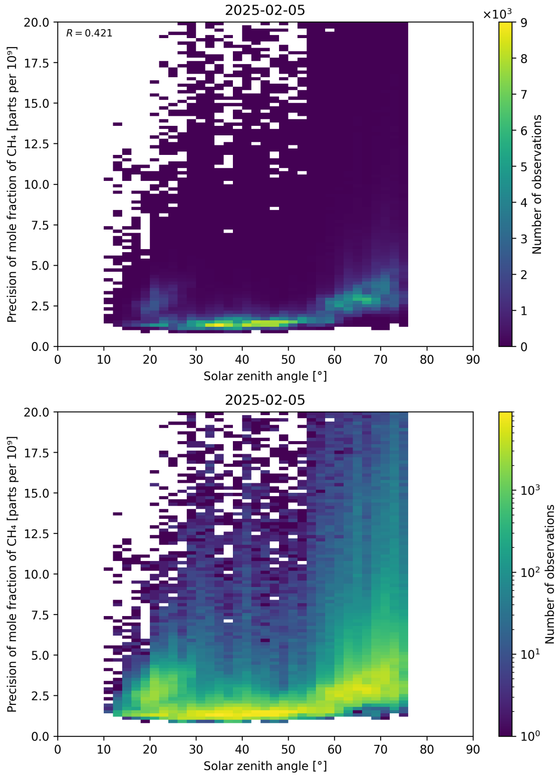
Figure 101: Scatter density plot of “Solar zenith angle” against “Precision of mole fraction of CH 4 ” for 2025-02-04 to 2025-02-06.
