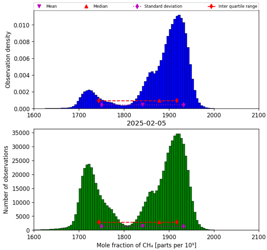
Figure 23: Histogram of “Mole fraction of CH 4 ” for 2025-02-04 to 2025-02-06
