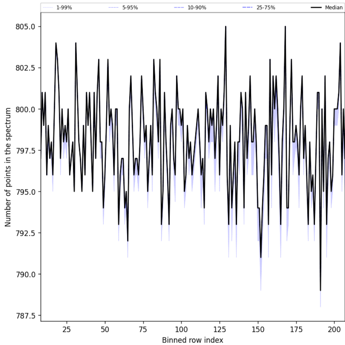
Figure 37: Along track statistics of “Number of points in the spectrum” for 2025-02-04 to 2025-02-06
