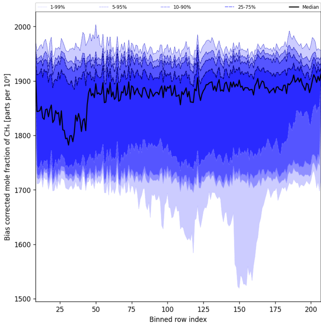
Figure 36: Along track statistics of “Bias corrected mole fraction of CH 4 ” for 2025-02-04 to 2025-02-06
