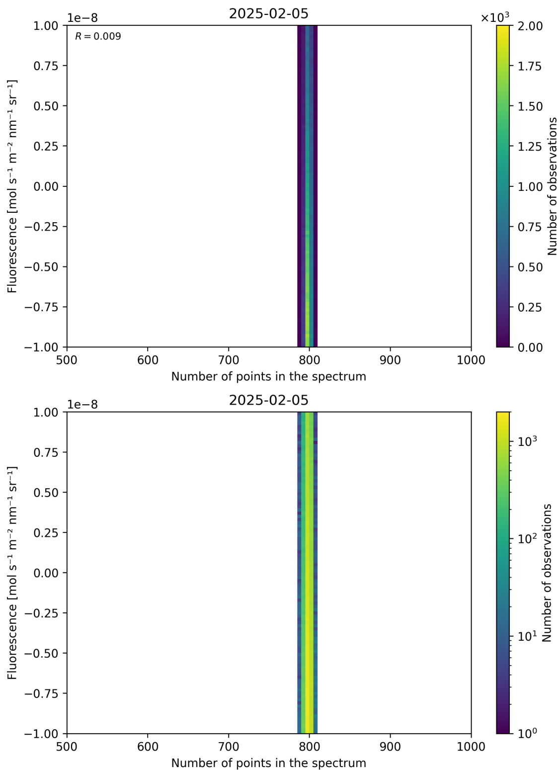
Figure 91: Scatter density plot of “Number of points in the spectrum” against “Fluorescence” for 2025-02-04 to 2025-02-06.
