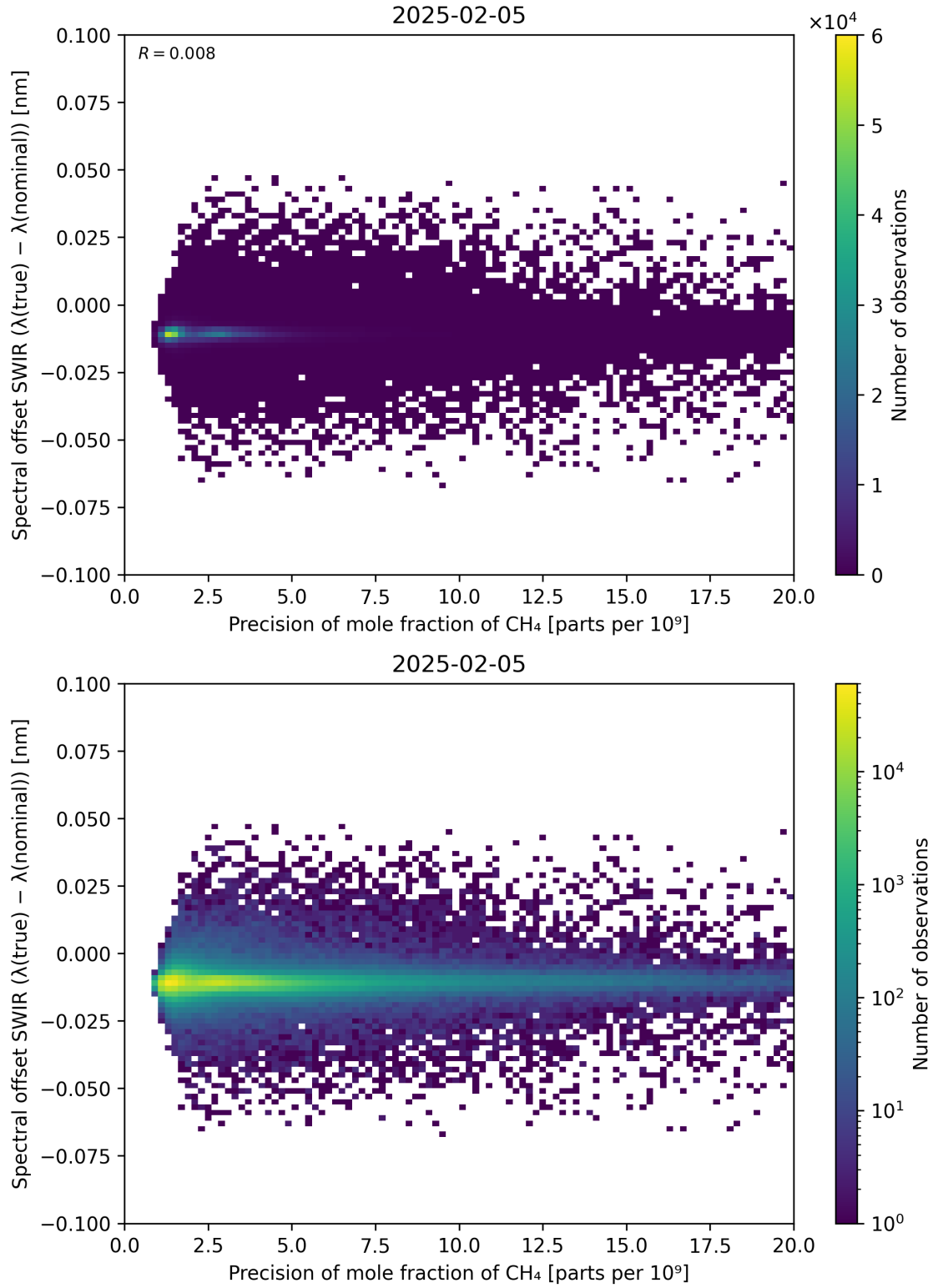
Figure 85: Scatter density plot of “Precision of mole fraction of \text{CH}_4 ” against “Spectral offset SWIR ( \lambda_{\text{true}} - \lambda_{\text{nominal}} )” for 2025-02-04 to 2025-02-06.
