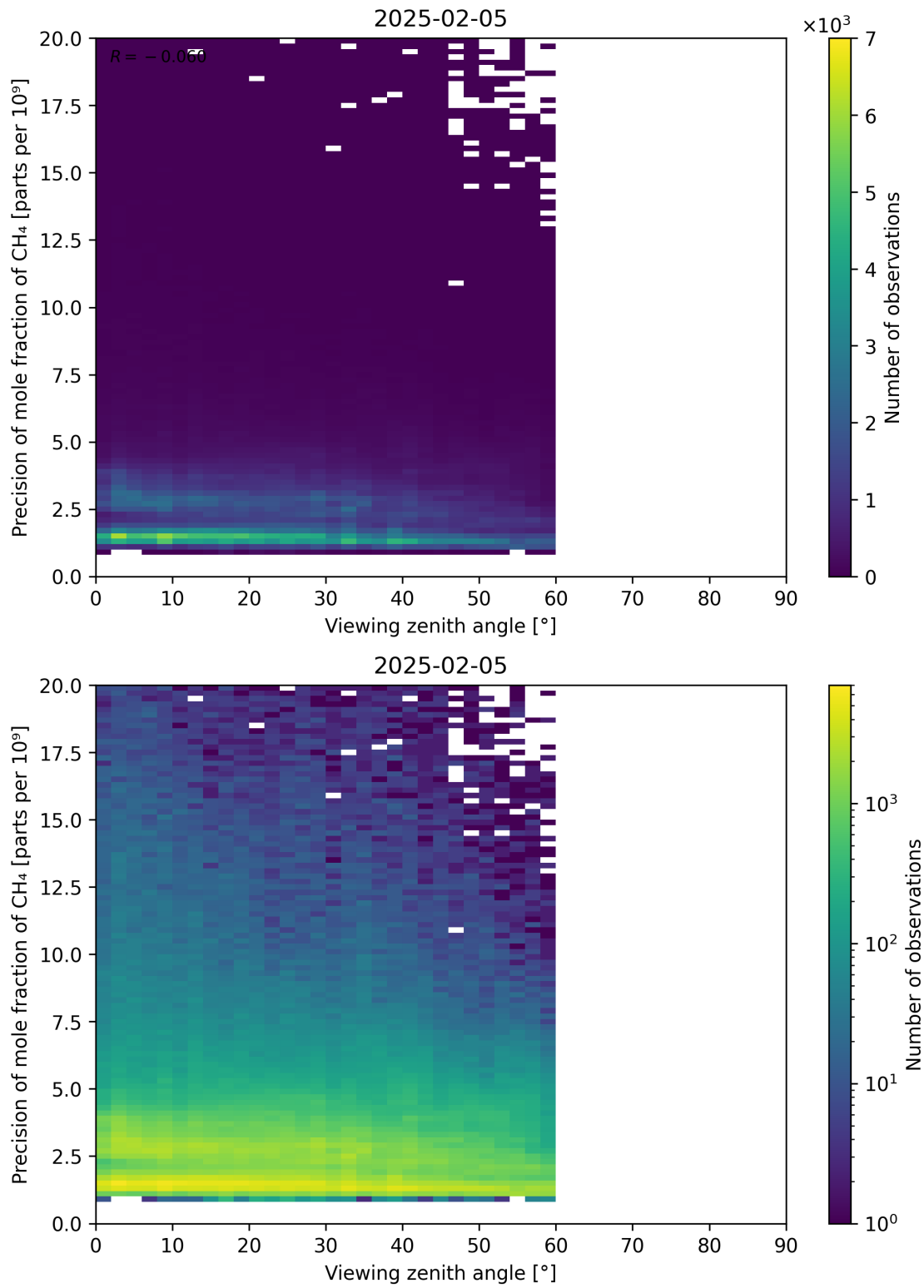
Figure 112: Scatter density plot of “Viewing zenith angle” against “Precision of mole fraction of CH 4 ” for 2025-02-04 to 2025-02-06.
