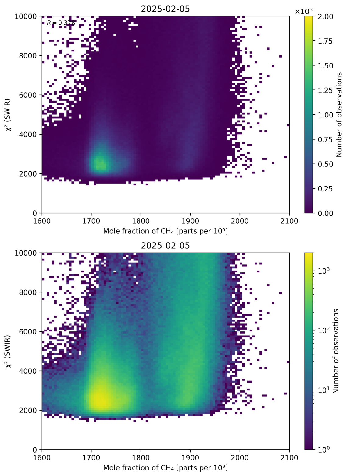
Figure 71: Scatter density plot of “Mole fraction of \text{CH}_4 ” against “ \chi^2 (SWIR)” for 2025-02-04 to 2025-02-06.
