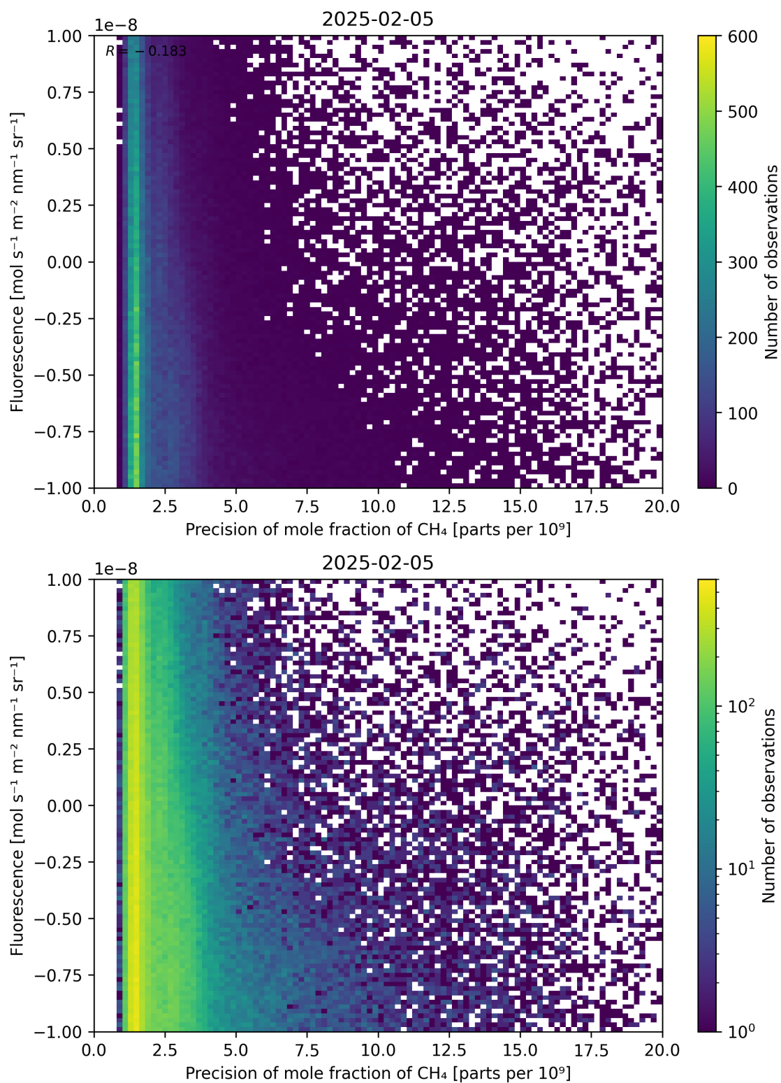
Figure 81: Scatter density plot of “Precision of mole fraction of \text{CH}_4 ” against “Fluorescence” for 2025-02-04 to 2025-02-06.
