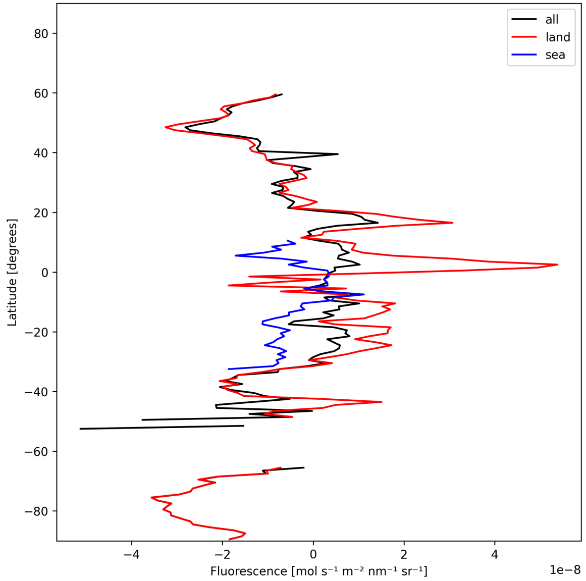
Figure 21: Zonal average of “Fluorescence” for 2025-02-04 to 2025-02-06.
