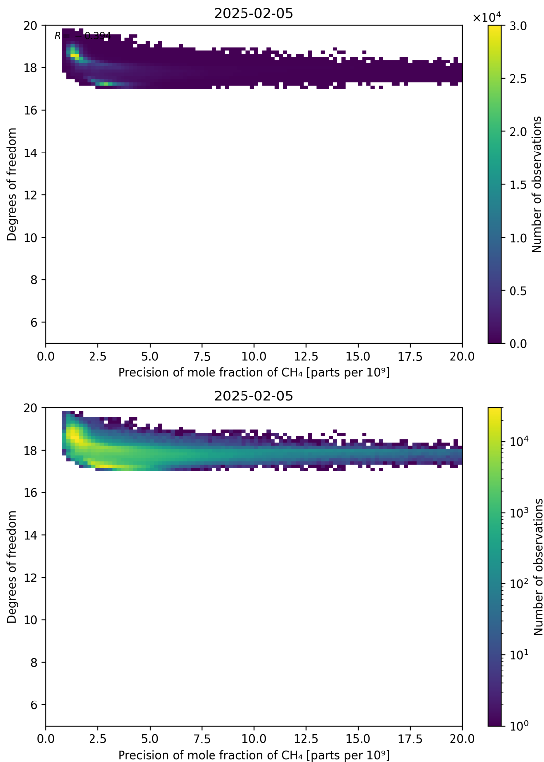
Figure 80: Scatter density plot of “Precision of mole fraction of CH 4 ” against “Degrees of freedom” for 2025-02-04 to 2025-02-06.
