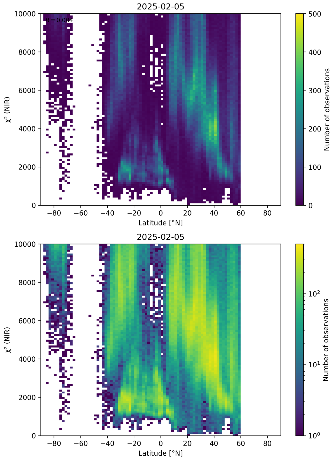
Figure 53: Scatter density plot of “Latitude” against “ \chi^2 (NIR)” for 2025-02-04 to 2025-02-06.
