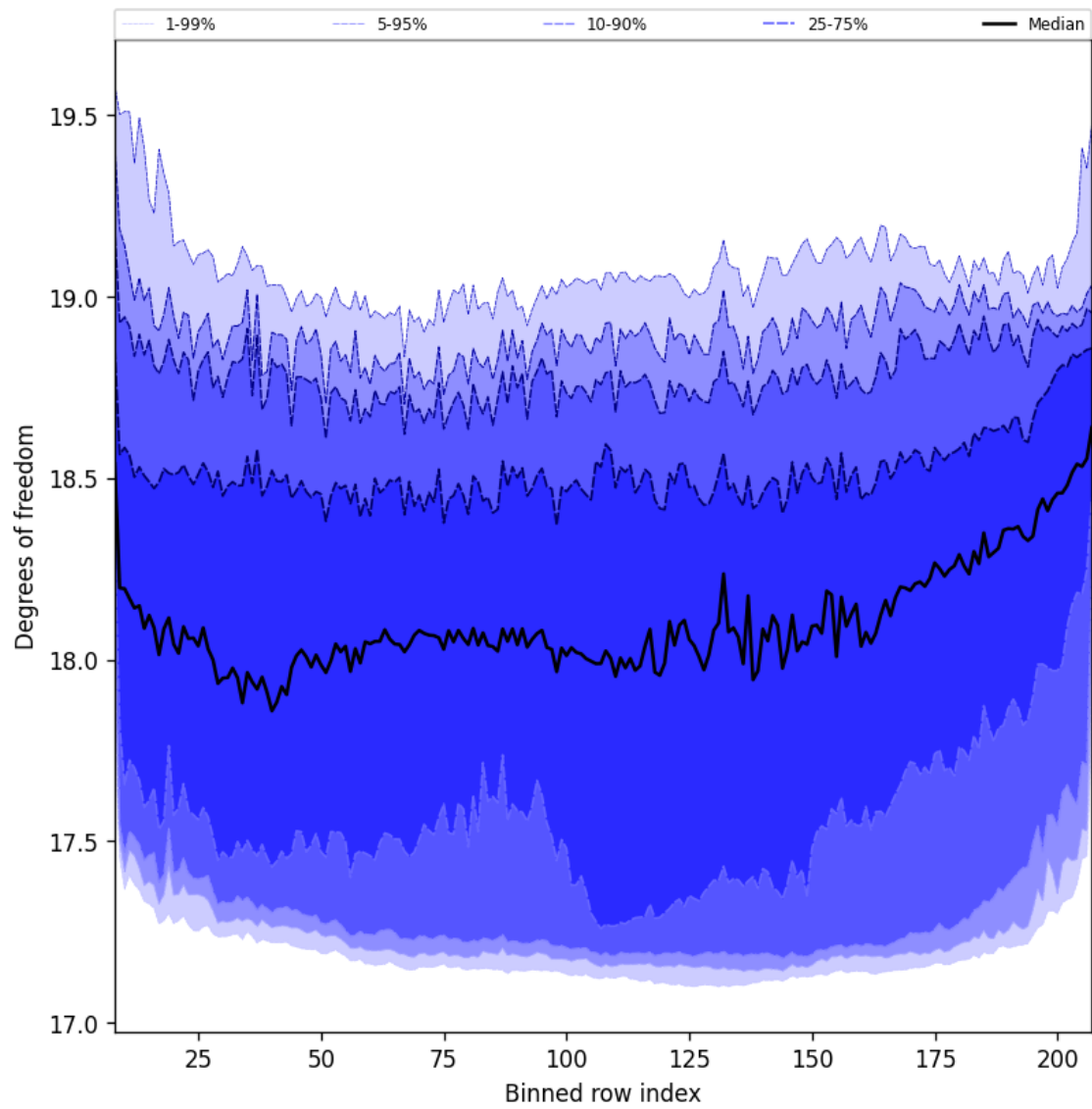
Figure 41: Along track statistics of “Degrees of freedom” for 2025-02-04 to 2025-02-06
