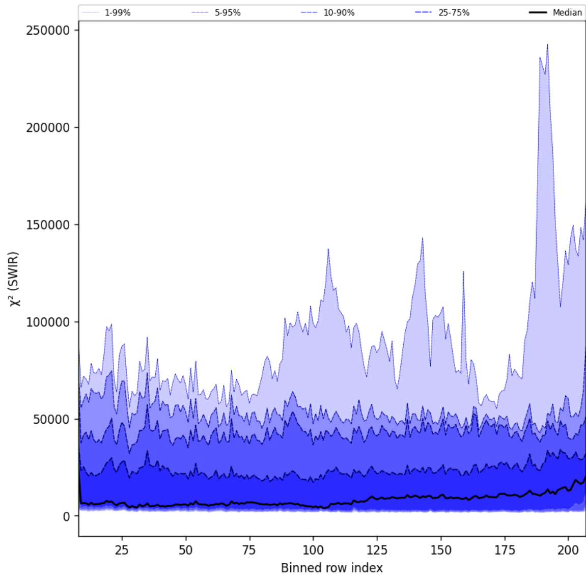
Figure 39: Along track statistics of “ \chi^2 (SWIR)” for 2025-02-04 to 2025-02-06
