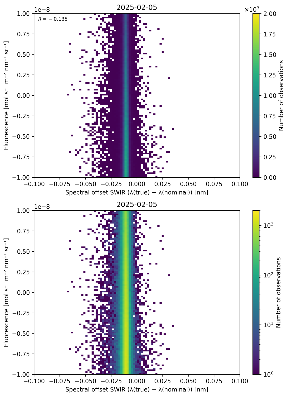
Figure 120: Scatter density plot of “Spectral offset SWIR ( \lambda_{\text{true}} - \lambda_{\text{nominal}} )” against “Fluorescence” for 2025-02-04 to 2025-02-06.
