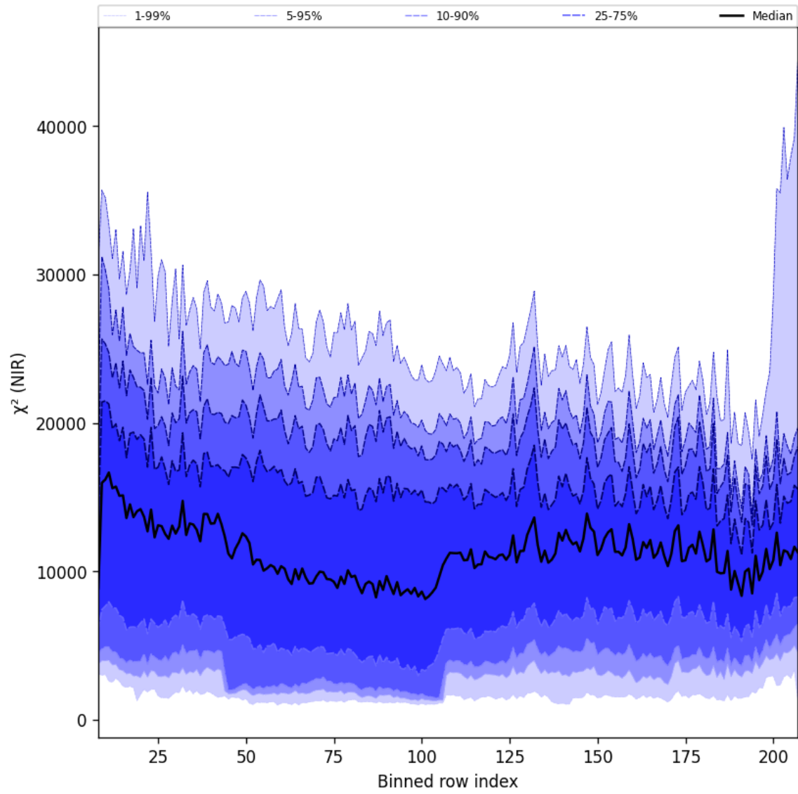
Figure 40: Along track statistics of “ \chi^2 (NIR)” for 2025-02-04 to 2025-02-06
