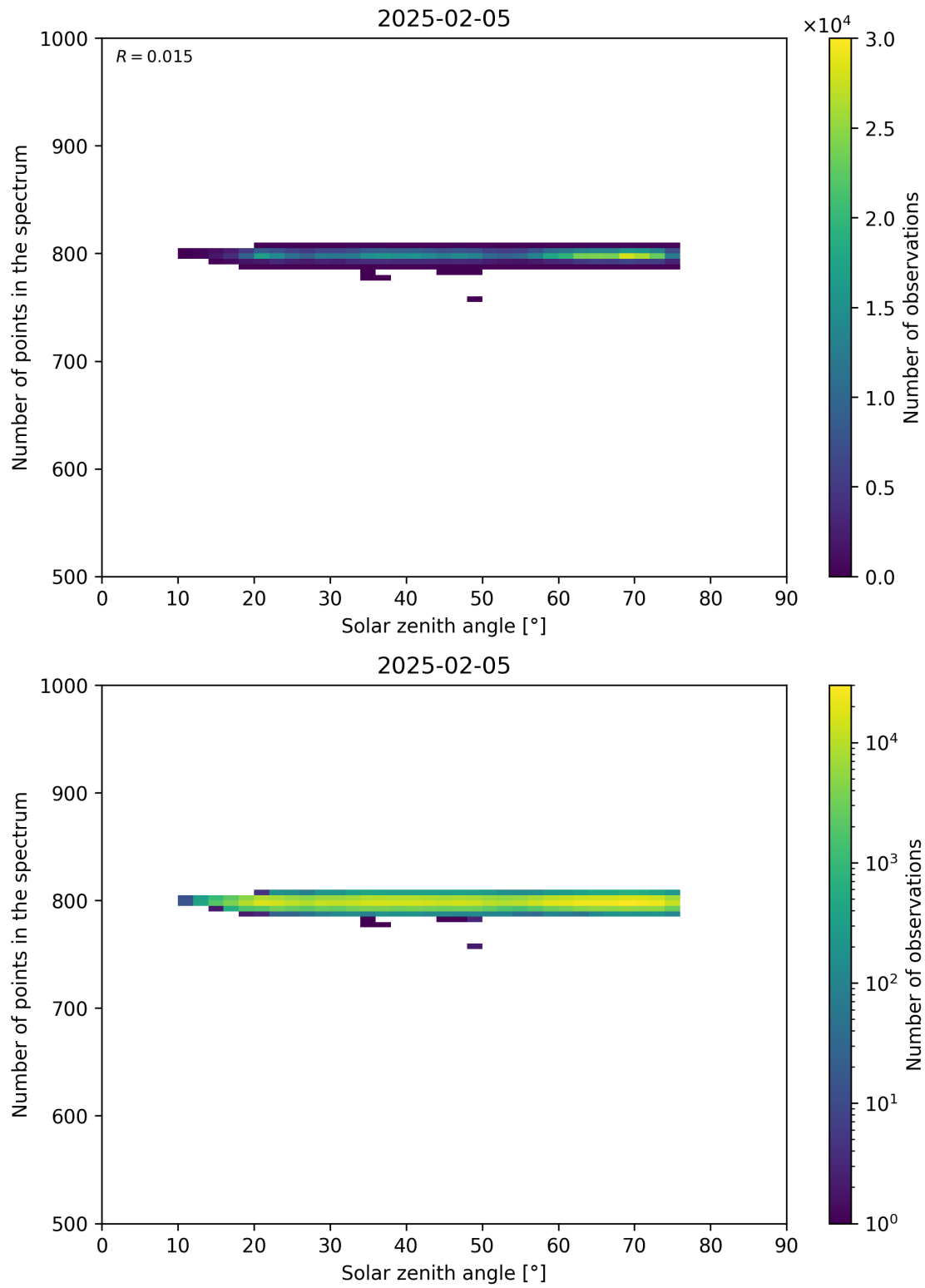
Figure 103: Scatter density plot of “Solar zenith angle” against “Number of points in the spectrum” for 2025-02-04 to 2025-02-06.
