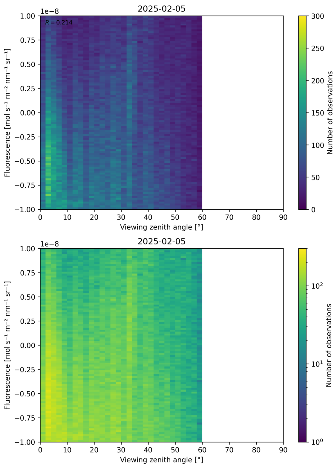
Figure 108: Scatter density plot of “Viewing zenith angle” against “Fluorescence” for 2025-02-04 to 2025-02-06.
