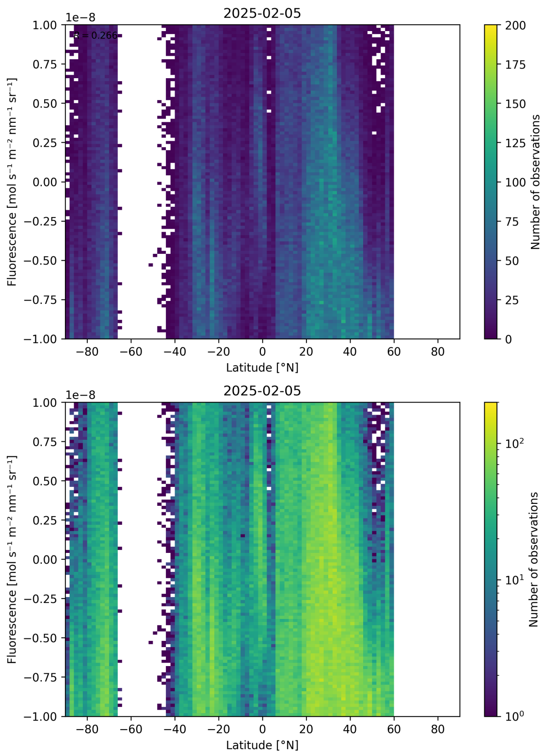
Figure 56: Scatter density plot of “Latitude” against “Fluorescence” for 2025-02-04 to 2025-02-06.
