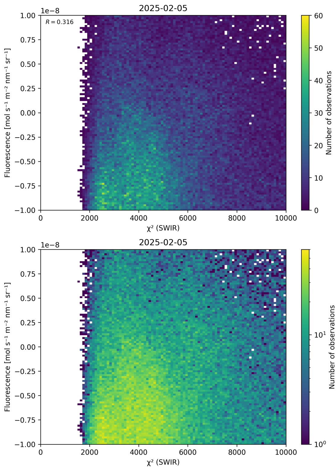
Figure 49: Scatter density plot of “ \chi^2 (SWIR)” against “Fluorescence” for 2025-02-04 to 2025-02-06.
