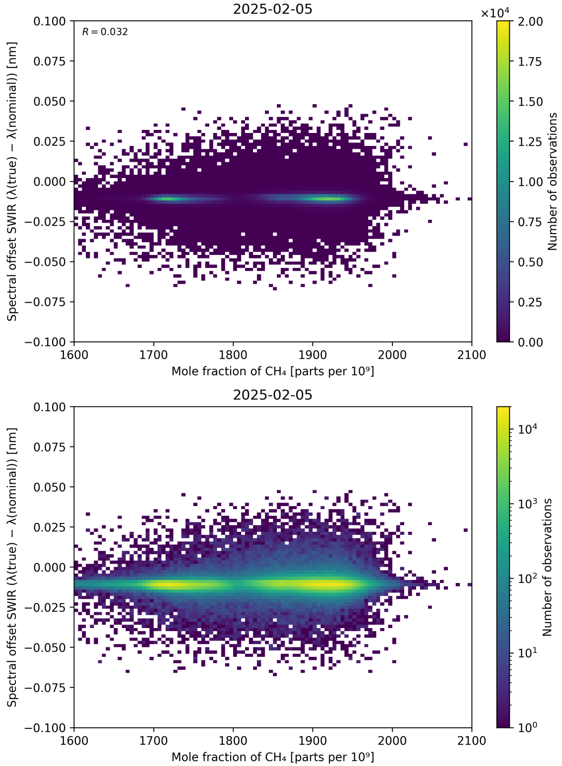
Figure 86: Scatter density plot of “Mole fraction of CH 4 ” against “Spectral offset SWIR ( \lambda_{\text{true}} - \lambda_{\text{nominal}} )” for 2025-02-04 to 2025-02-06.
