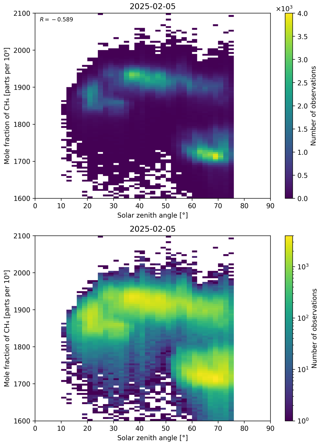
Figure 99: Scatter density plot of “Solar zenith angle” against “Mole fraction of CH 4 ” for 2025-02-04 to 2025-02-06.
