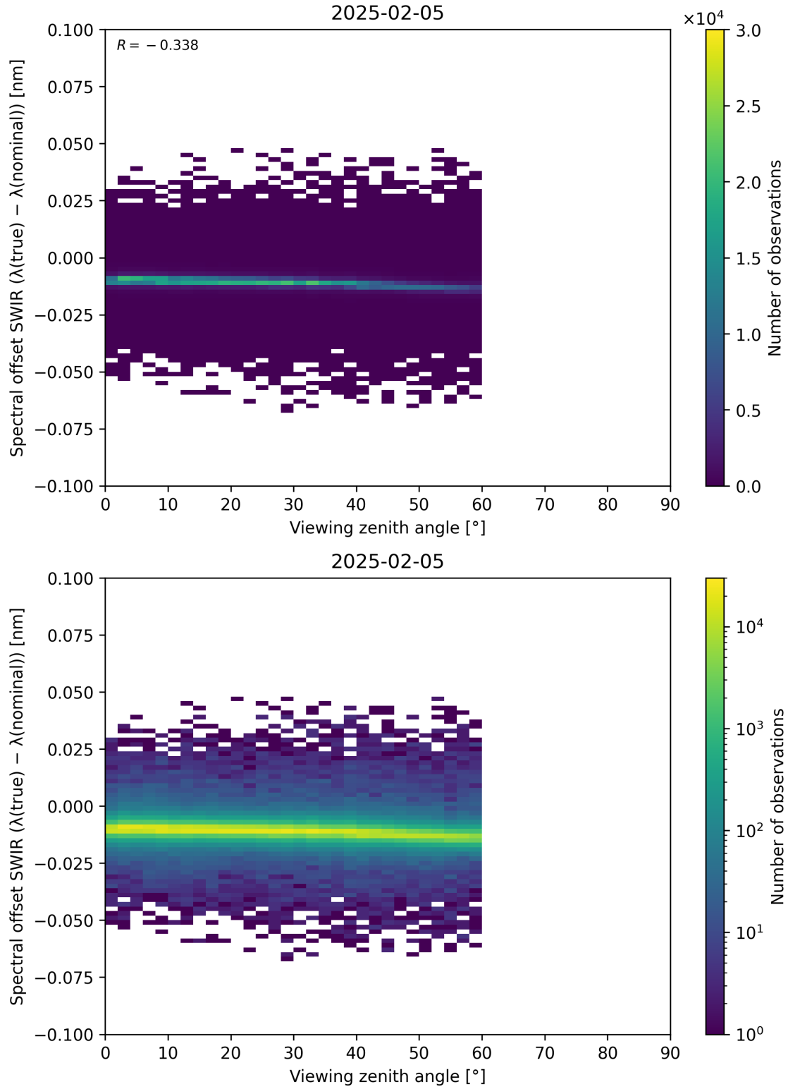
Figure 116: Scatter density plot of “Viewing zenith angle” against “Spectral offset SWIR ( \lambda_{\text{true}} - \lambda_{\text{nominal}} )” for 2025-02-04 to 2025-02-06.
