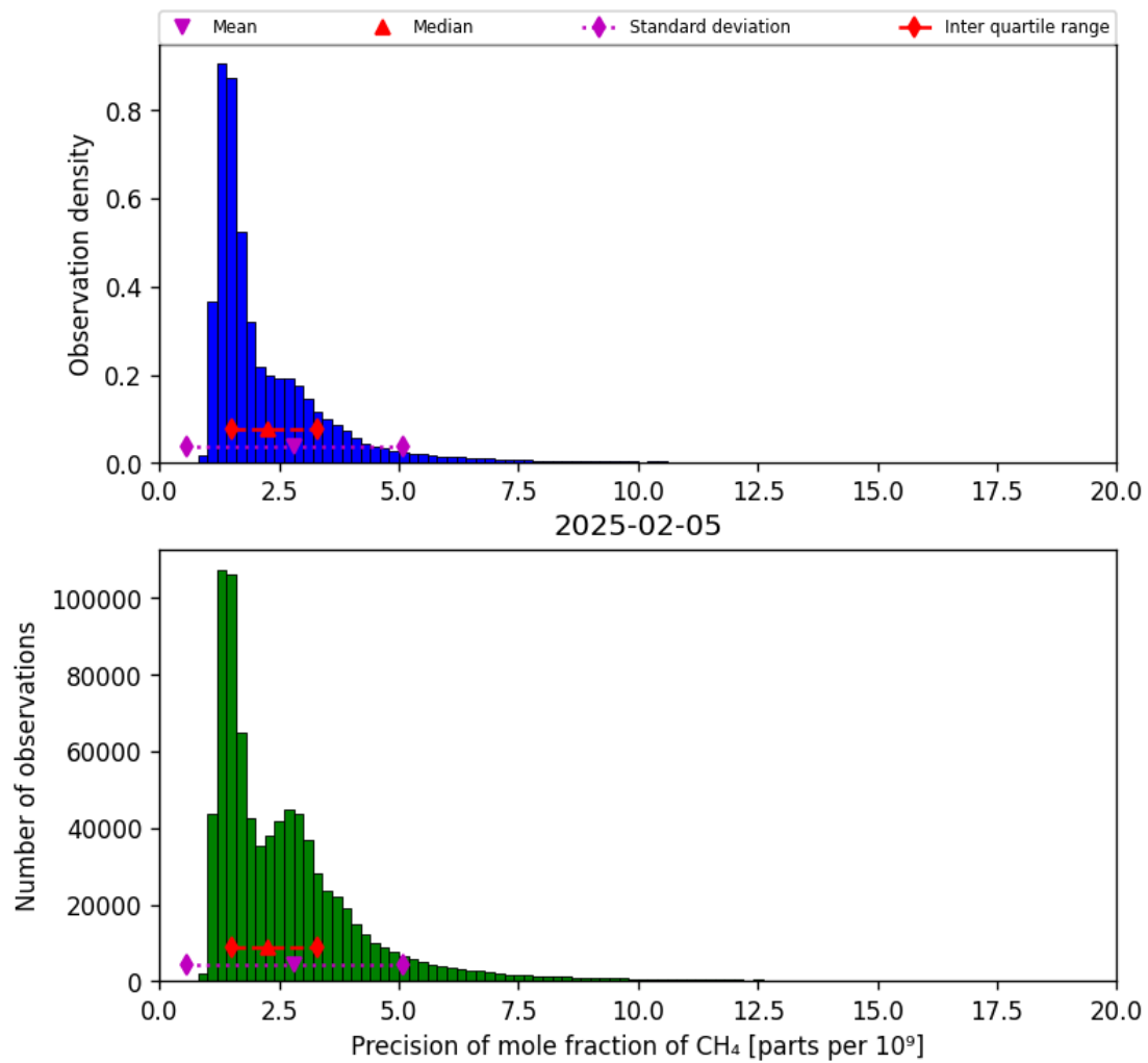
Figure 24: Histogram of “Precision of mole fraction of CH 4 ” for 2025-02-04 to 2025-02-06
