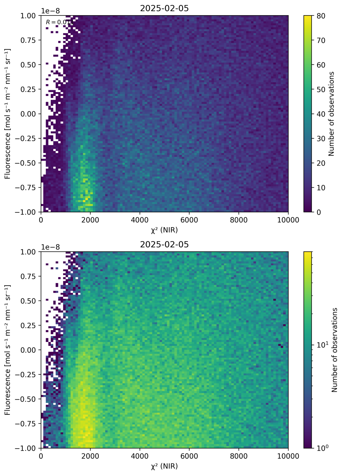
Figure 45: Scatter density plot of “ \chi^2 (NIR)” against “Fluorescence” for 2025-02-04 to 2025-02-06.
