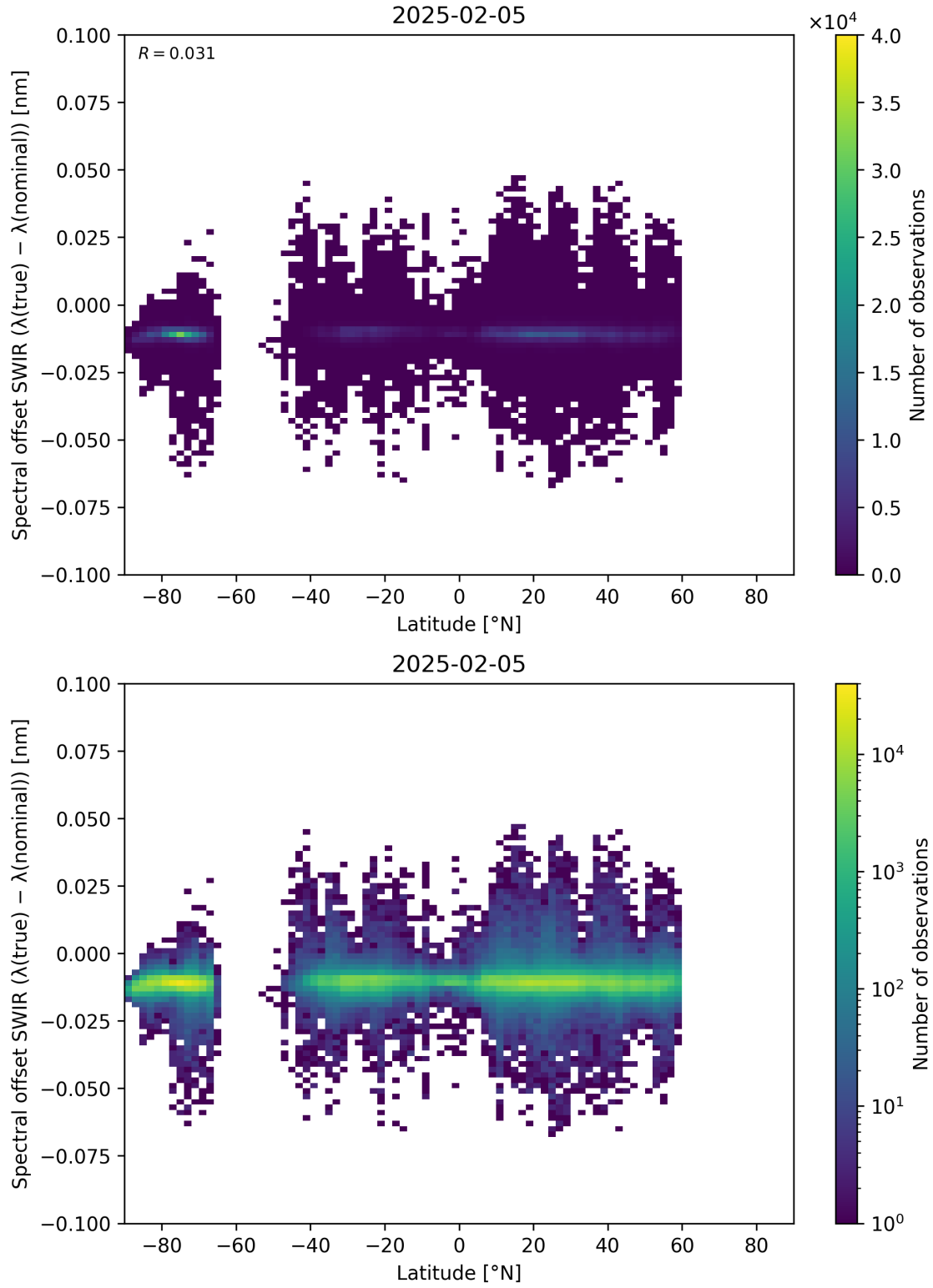
Figure 62: Scatter density plot of “Latitude” against “Spectral offset SWIR ( \lambda_{\text{true}} - \lambda_{\text{nominal}} )” for 2025-02-04 to 2025-02-06.
