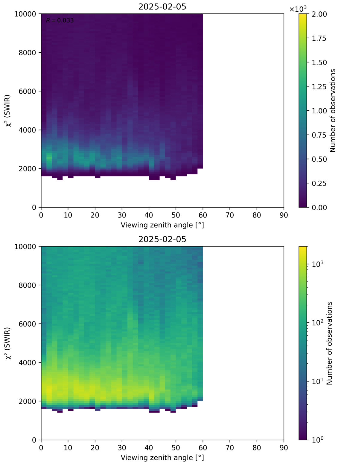
Figure 106: Scatter density plot of “Viewing zenith angle” against “ \chi^2 (SWIR)” for 2025-02-04 to 2025-02-06.
