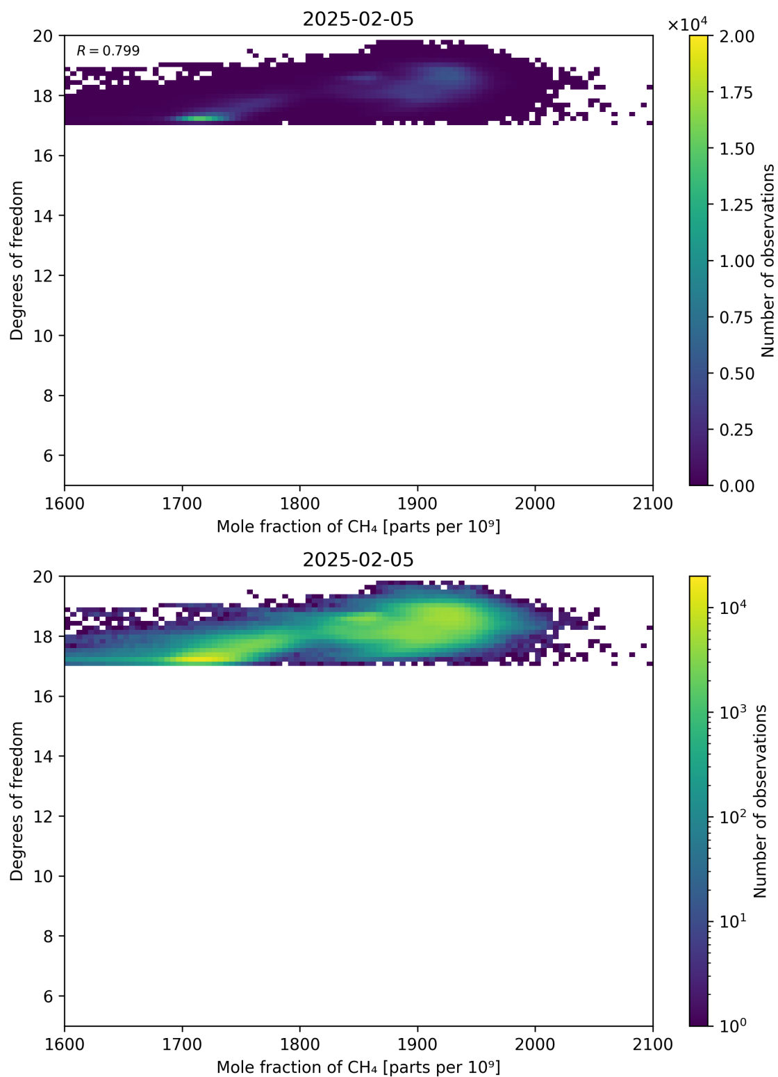
Figure 72: Scatter density plot of “Mole fraction of CH 4 ” against “Degrees of freedom” for 2025-02-04 to 2025-02-06.
