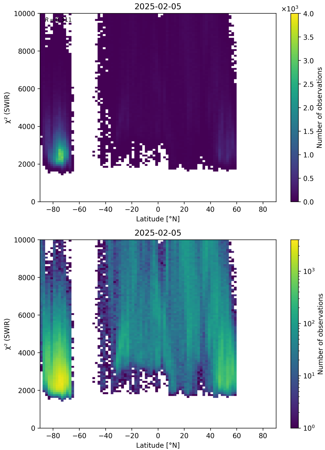
Figure 54: Scatter density plot of “Latitude” against “ \chi^2 (SWIR)” for 2025-02-04 to 2025-02-06.
