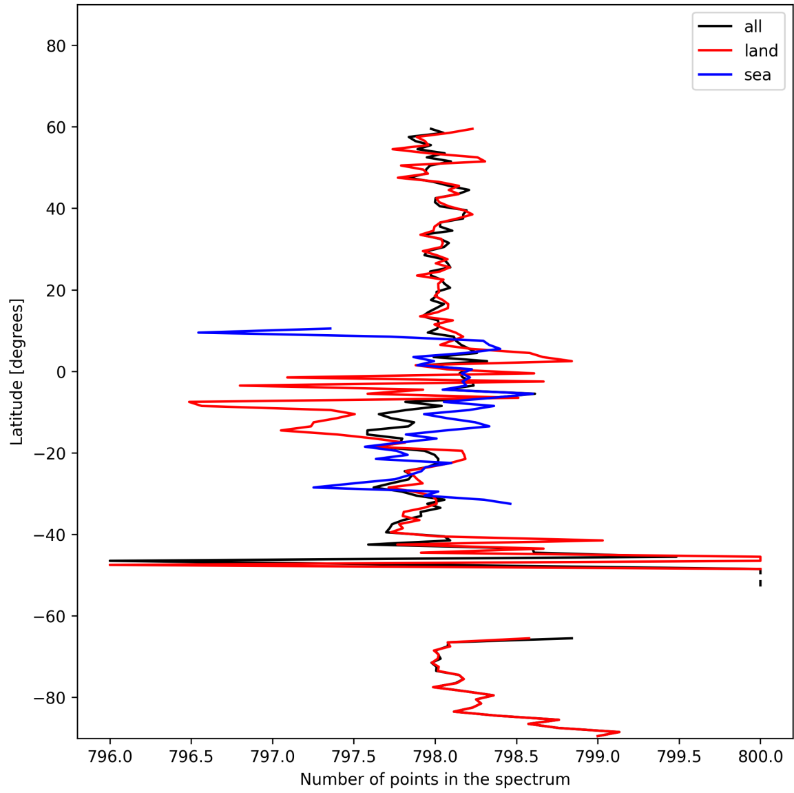
Figure 15: Zonal average of “Number of points in the spectrum” for 2025-02-04 to 2025-02-06.
