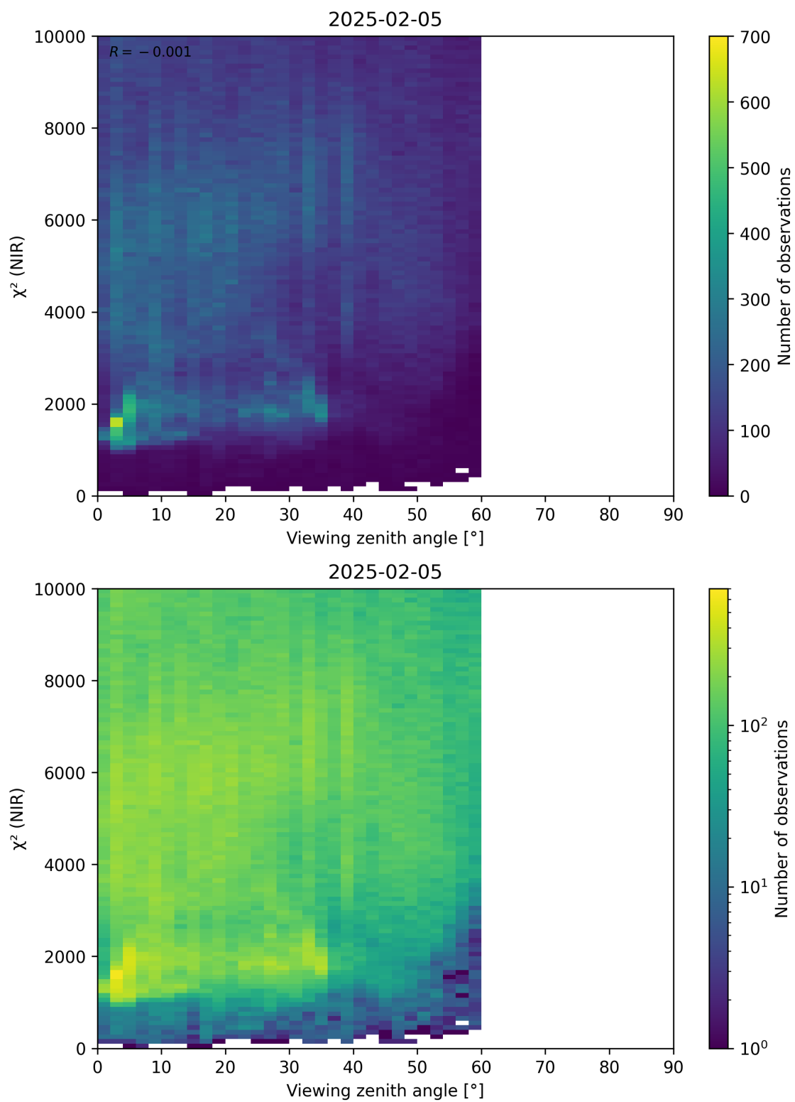
Figure 105: Scatter density plot of “Viewing zenith angle” against “ \chi^2 (NIR)” for 2025-02-04 to 2025-02-06.
