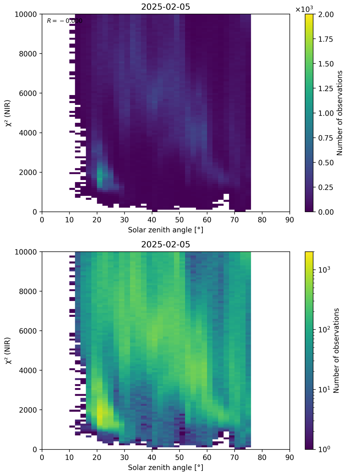
Figure 94: Scatter density plot of “Solar zenith angle” against “ \chi^2 (NIR)” for 2025-02-04 to 2025-02-06.
