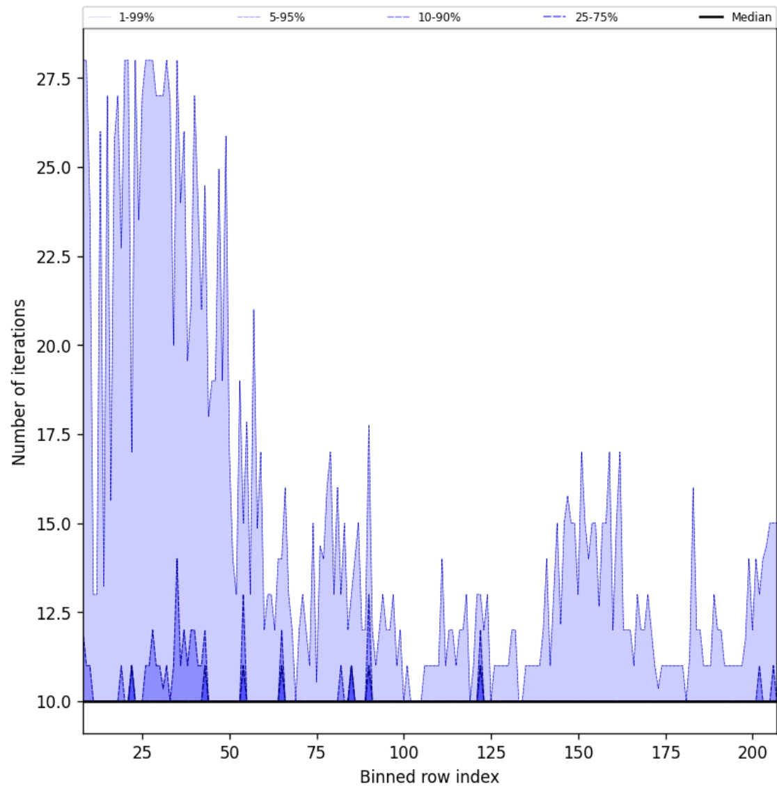
Figure 42: Along track statistics of “Number of iterations” for 2025-02-04 to 2025-02-06
