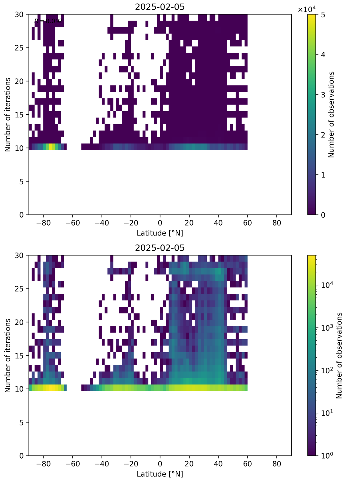
Figure 60: Scatter density plot of “Latitude” against “Number of iterations” for 2025-02-04 to 2025-02-06.
