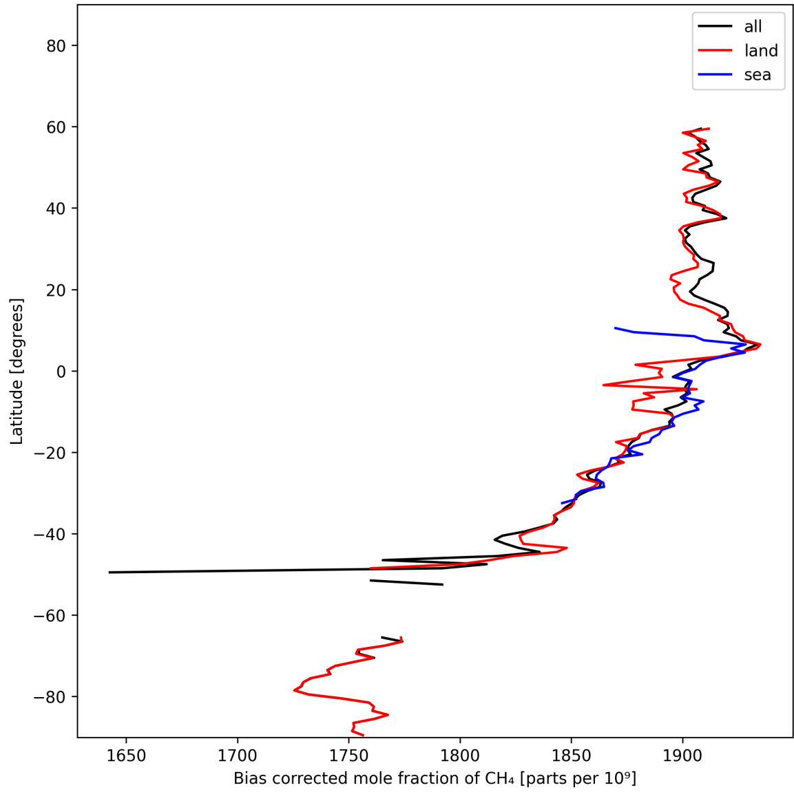
Figure 14: Zonal average of “Bias corrected mole fraction of CH 4 ” for 2025-02-04 to 2025-02-06.
