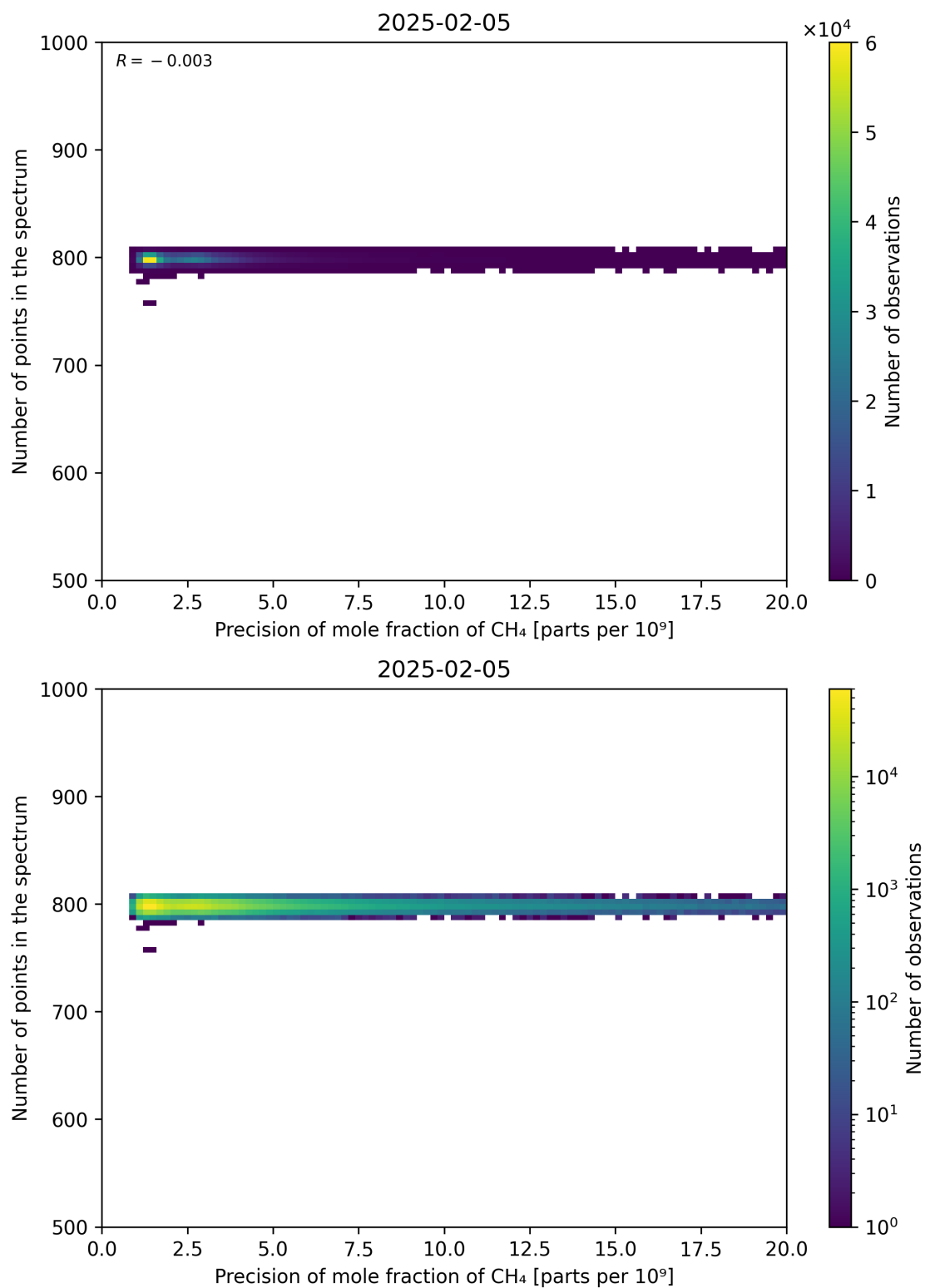
Figure 84: Scatter density plot of “Precision of mole fraction of CH 4 ” against “Number of points in the spectrum” for 2025-02-04 to 2025-02-06.
