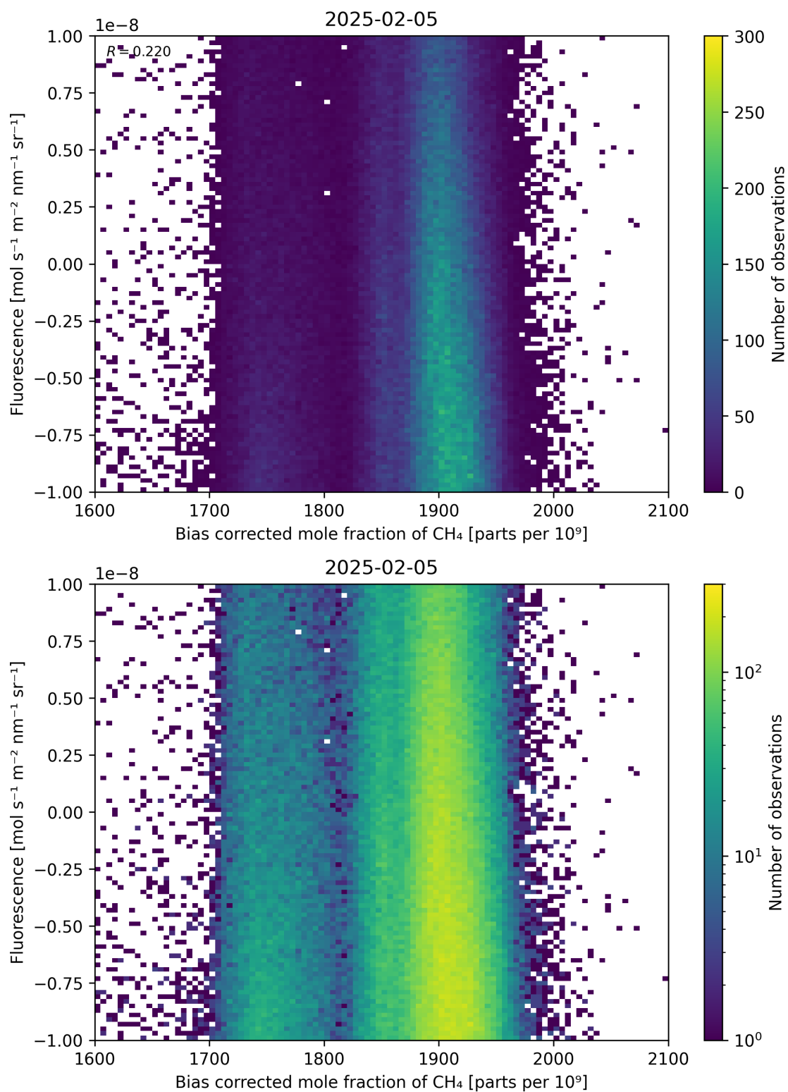
Figure 66: Scatter density plot of “Bias corrected mole fraction of \text{CH}_4 ” against “Fluorescence” for 2025-02-04 to 2025-02-06.
