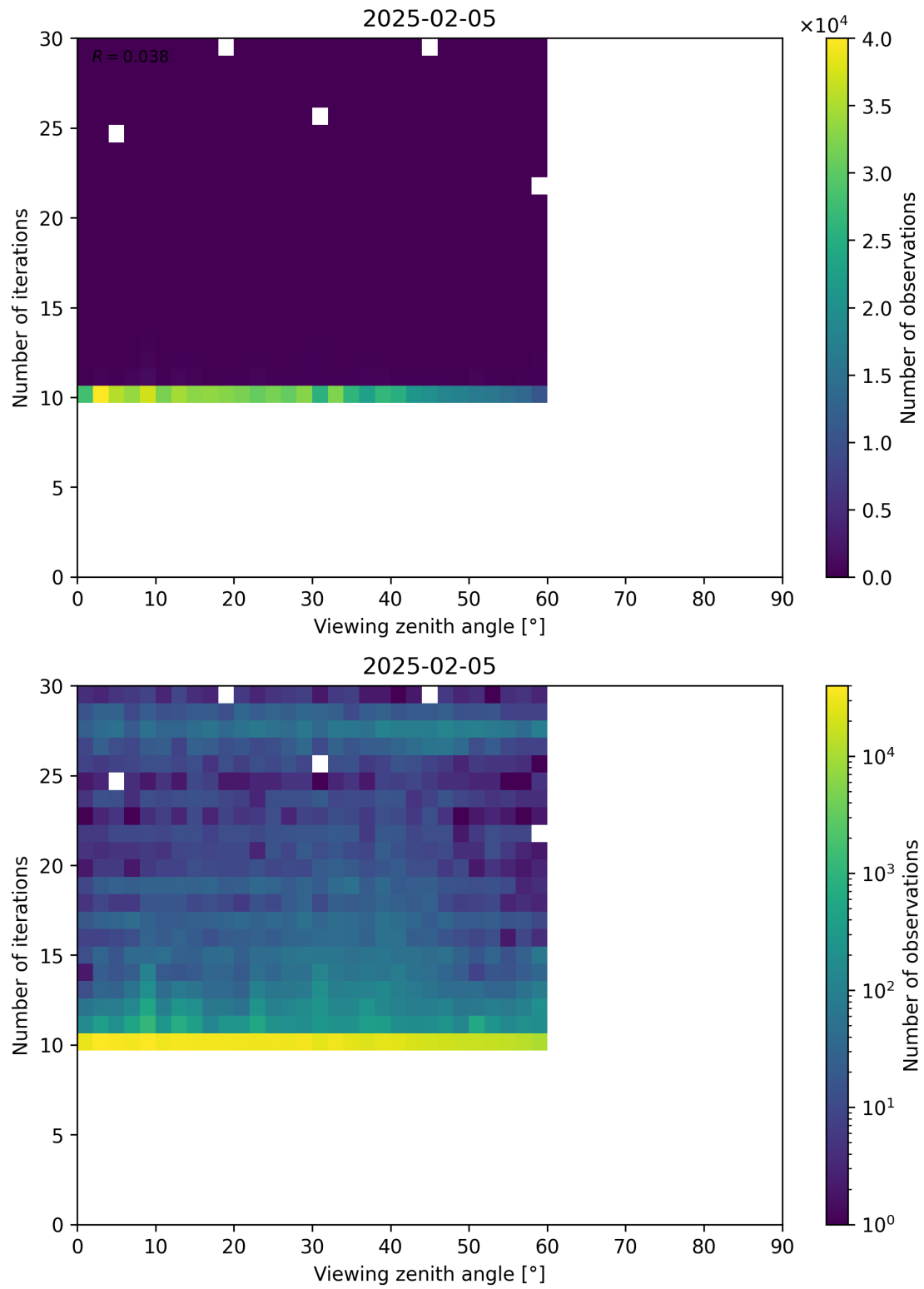
Figure 113: Scatter density plot of “Viewing zenith angle” against “Number of iterations” for 2025-02-04 to 2025-02-06.
