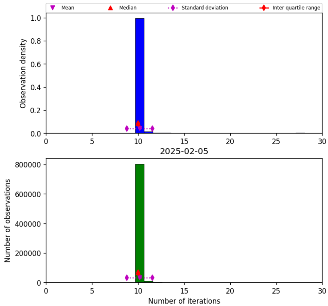
Figure 31: Histogram of “Number of iterations” for 2025-02-04 to 2025-02-06
