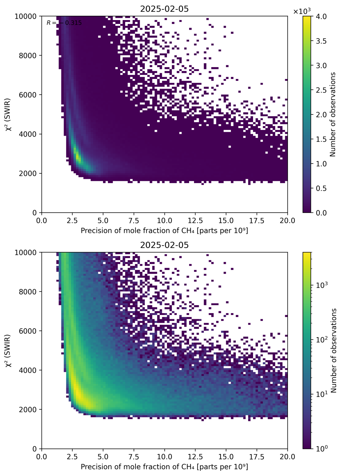
Figure 79: Scatter density plot of “Precision of mole fraction of CH 4 ” against “ \chi^2 (SWIR)” for 2025-02-04 to 2025-02-06.
