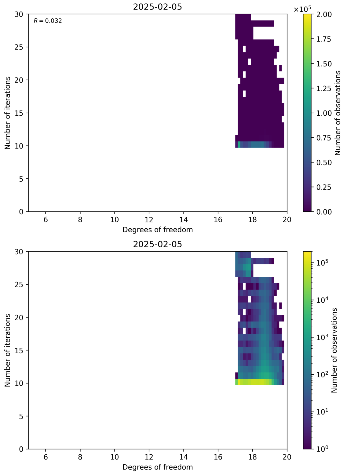
Figure 52: Scatter density plot of “Degrees of freedom” against “Number of iterations” for 2025-02-04 to 2025-02-06.
