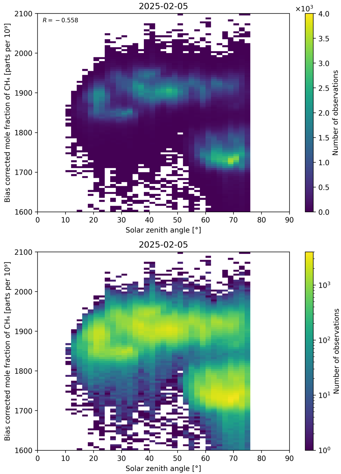
Figure 100: Scatter density plot of “Solar zenith angle” against “Bias corrected mole fraction of CH 4 ” for 2025-02-04 to 2025-02-06.
