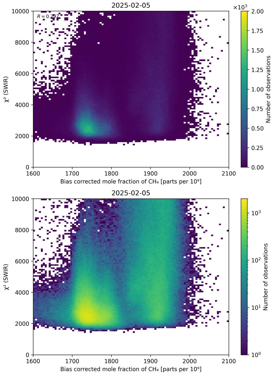
Figure 64: Scatter density plot of “Bias corrected mole fraction of \text{CH}_4 ” against “ \chi^2 (SWIR)” for 2025-02-04 to 2025-02-06.
