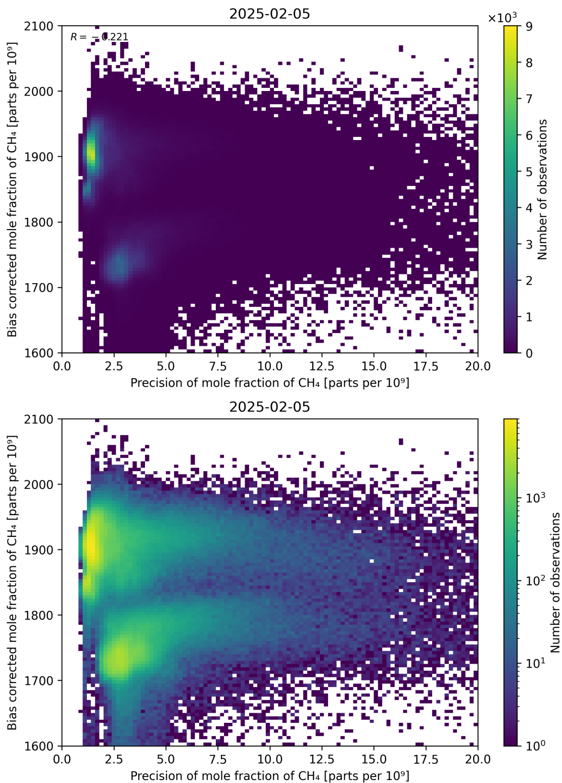
Figure 82: Scatter density plot of “Precision of mole fraction of CH 4 ” against “Bias corrected mole fraction of CH 4 ” for 2025-02-04 to 2025-02-06.
