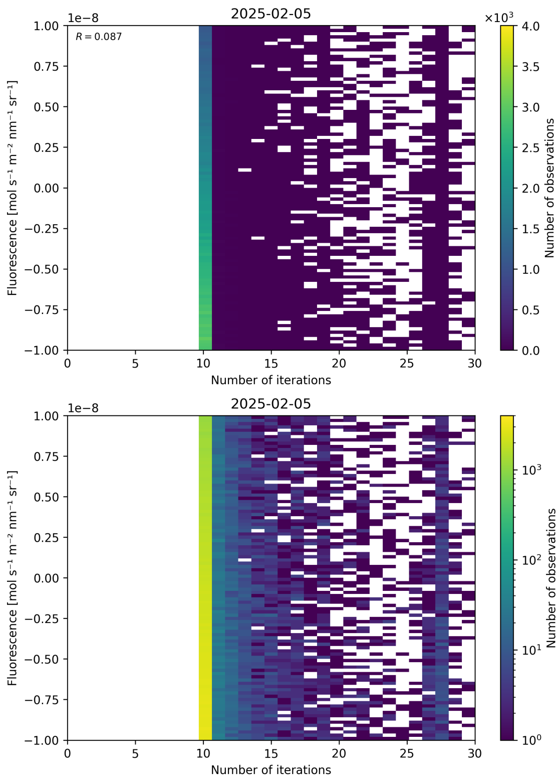
Figure 87: Scatter density plot of “Number of iterations” against “Fluorescence” for 2025-02-04 to 2025-02-06.
