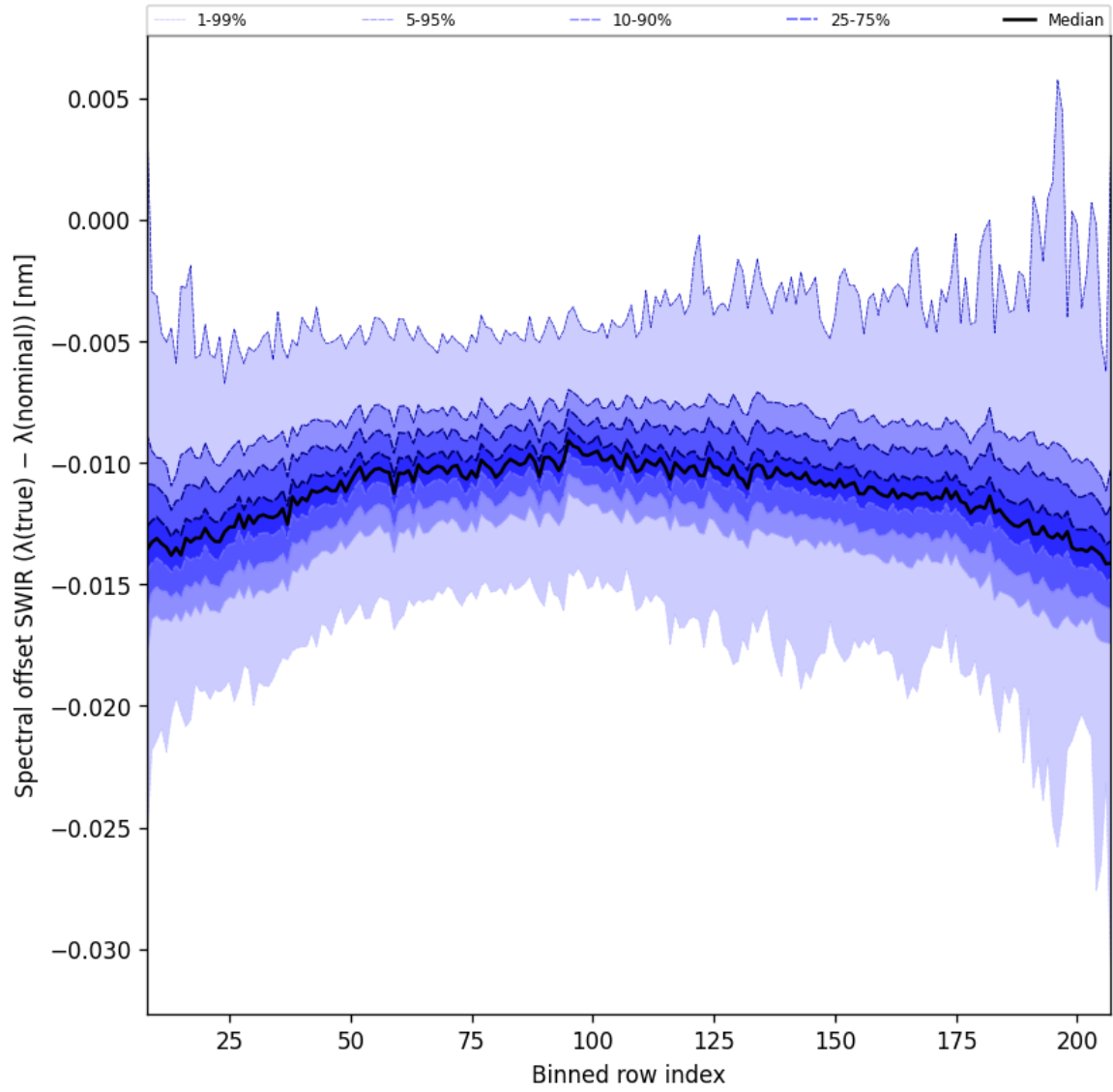
Figure 38: Along track statistics of “Spectral offset SWIR ( \lambda_{\text{true}} - \lambda_{\text{nominal}} )” for 2025-02-06 to 2025-02-08
