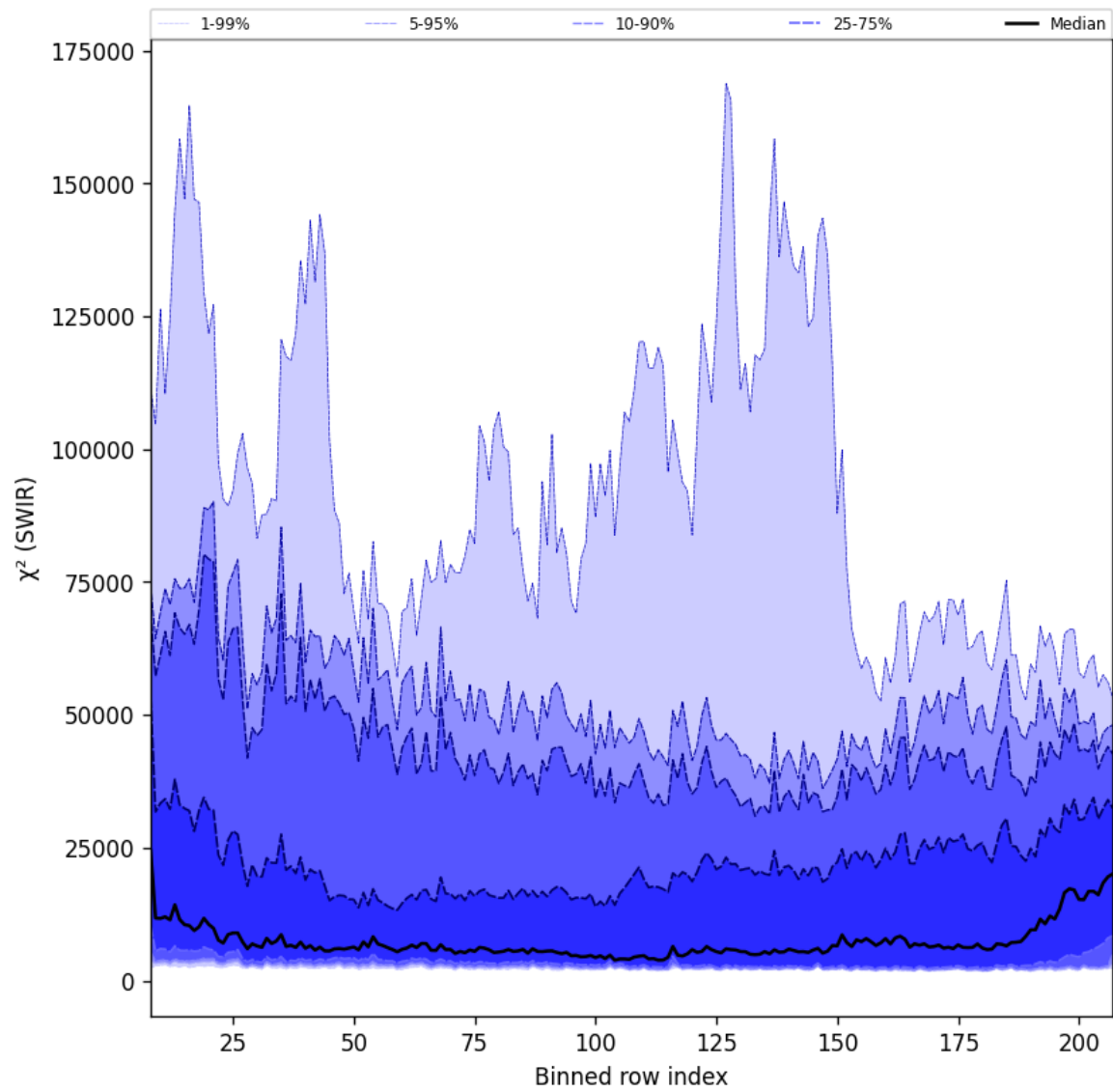
Figure 39: Along track statistics of “ \chi^2 (SWIR)” for 2025-02-06 to 2025-02-08
