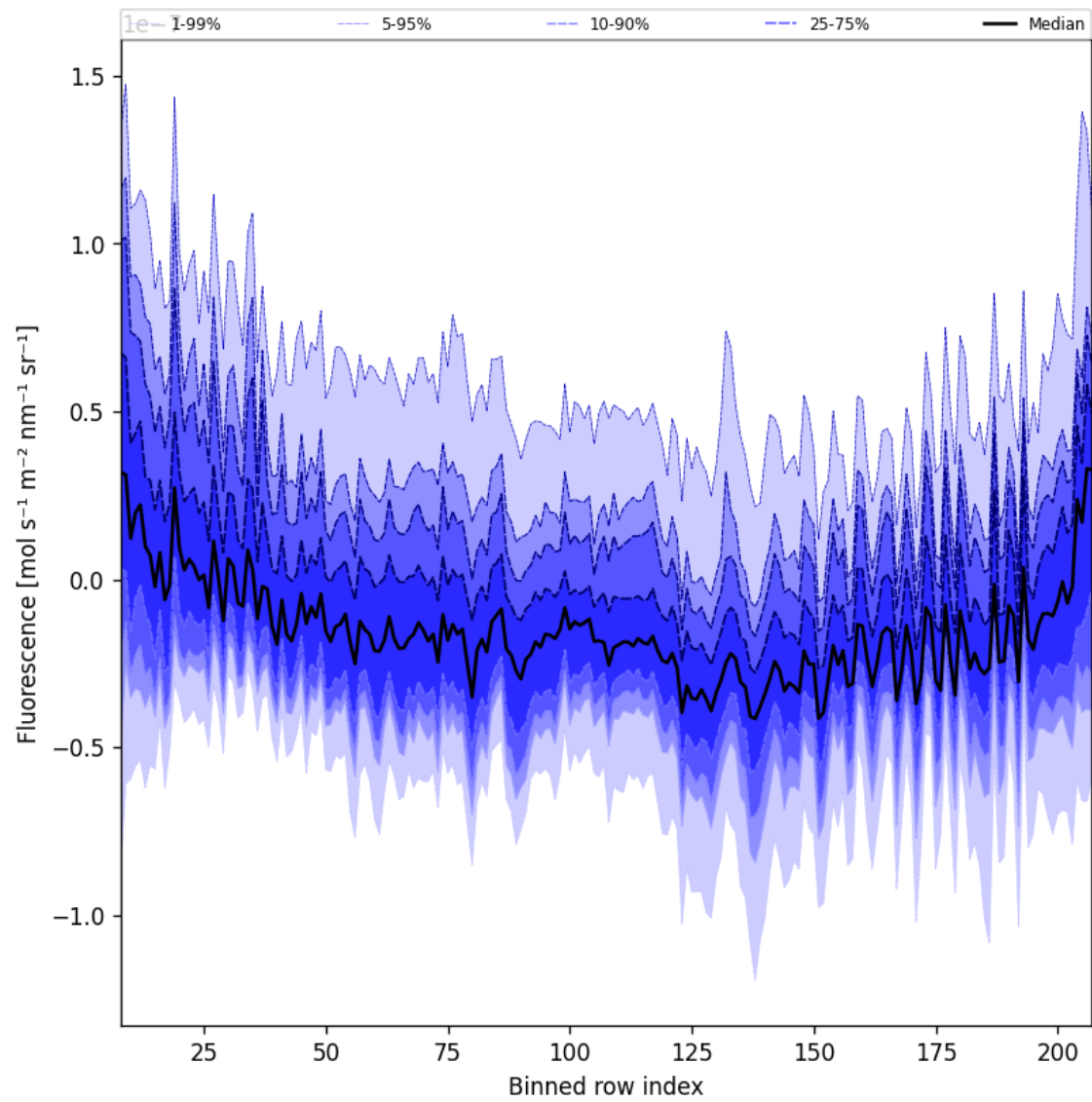
Figure 43: Along track statistics of "Fluorescence" for 2025-02-06 to 2025-02-08
