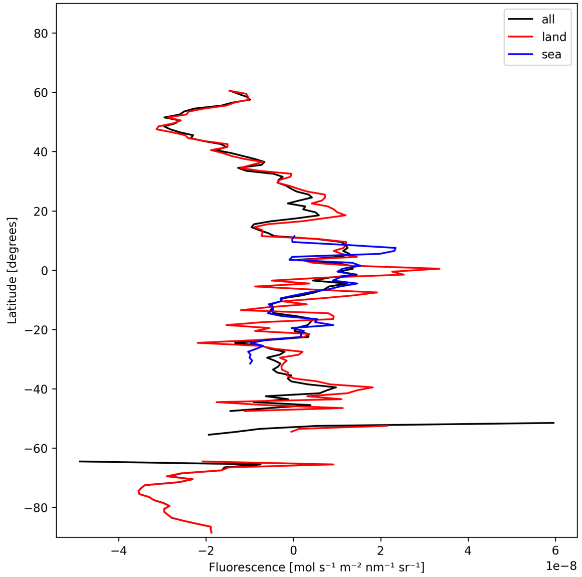
Figure 21: Zonal average of “Fluorescence” for 2025-02-06 to 2025-02-08.
