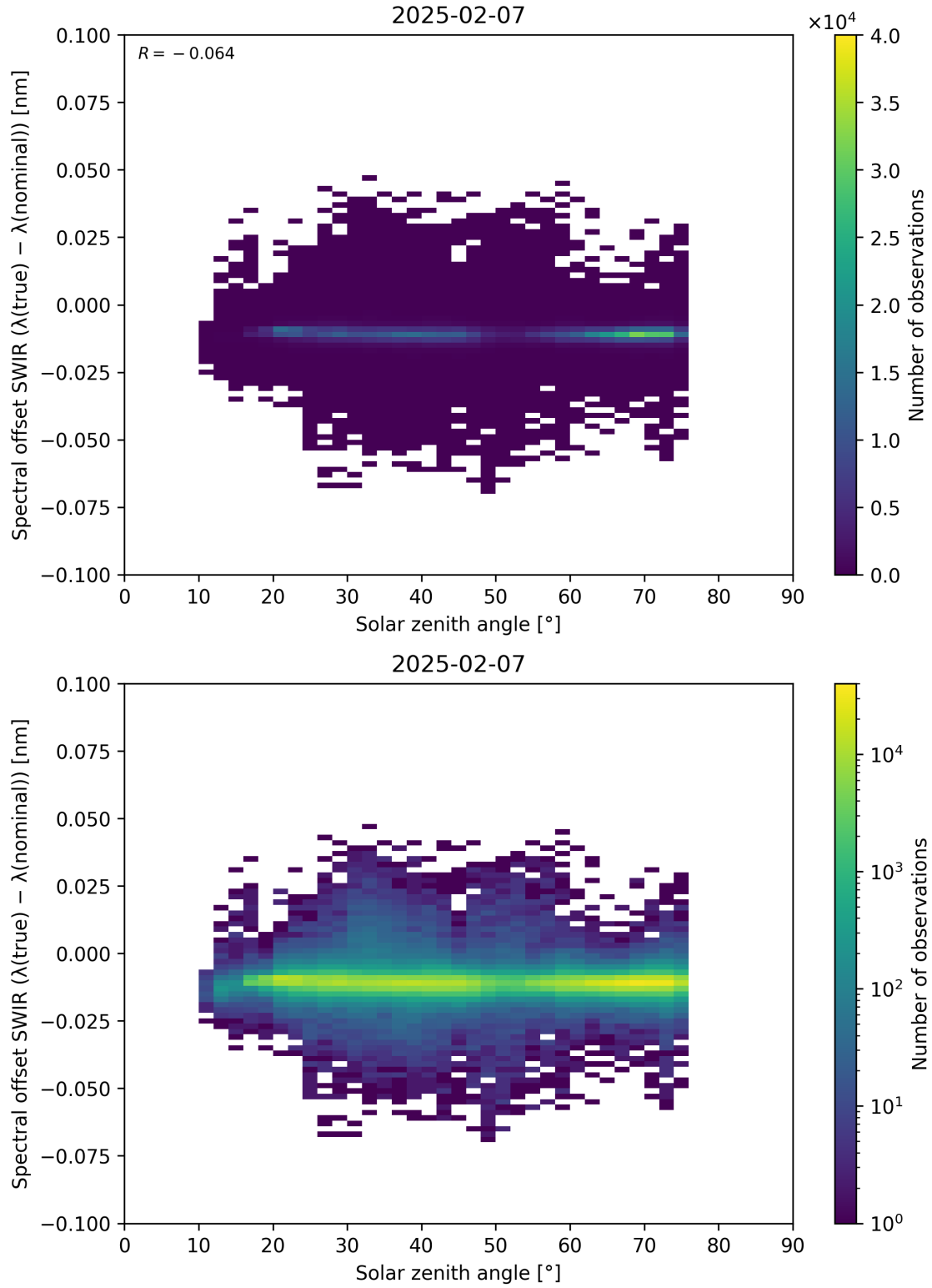
Figure 104: Scatter density plot of “Solar zenith angle” against “Spectral offset SWIR ( \lambda_{\text{true}} - \lambda_{\text{nominal}} )” for 2025-02-06 to 2025-02-08.
