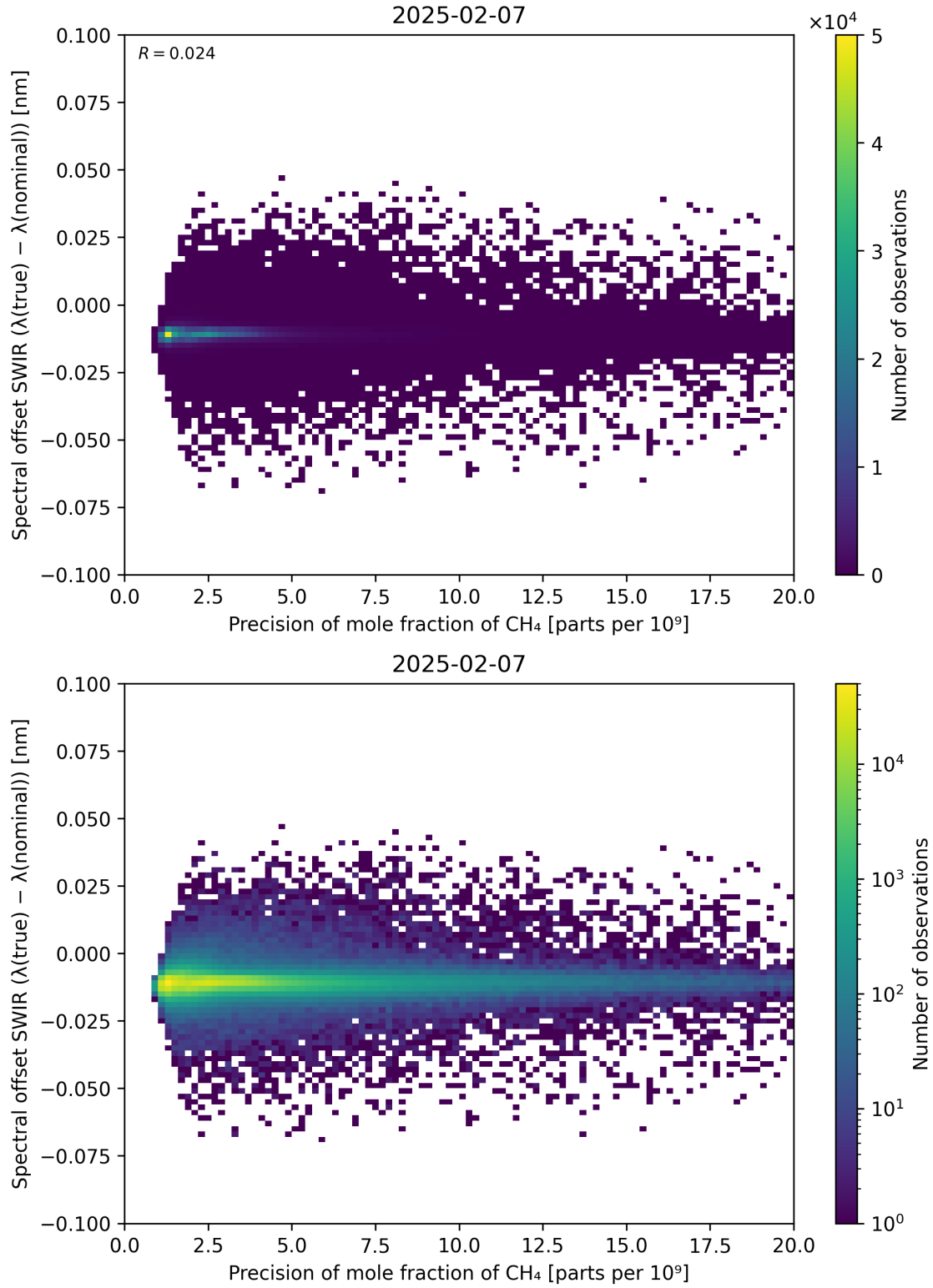
Figure 85: Scatter density plot of “Precision of mole fraction of CH 4 ” against “Spectral offset SWIR ( \lambda_{\text{true}} - \lambda_{\text{nominal}} )” for 2025-02-06 to 2025-02-08.
