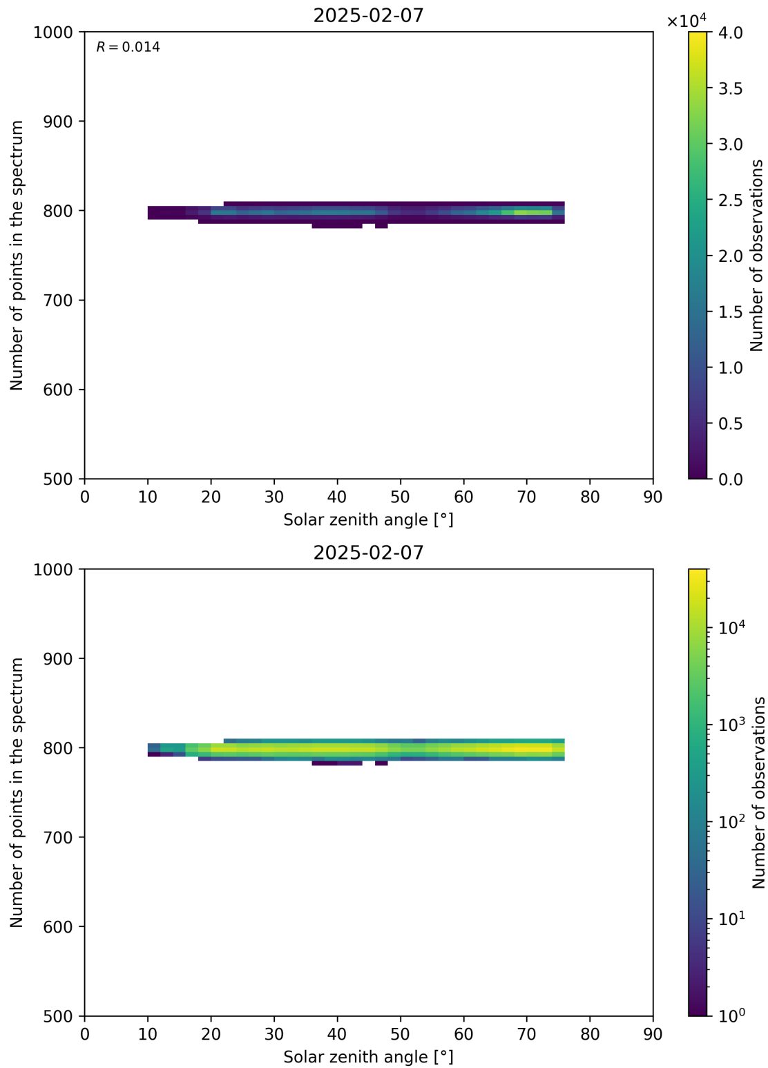
Figure 103: Scatter density plot of “Solar zenith angle” against “Number of points in the spectrum” for 2025-02-06 to 2025-02-08.
