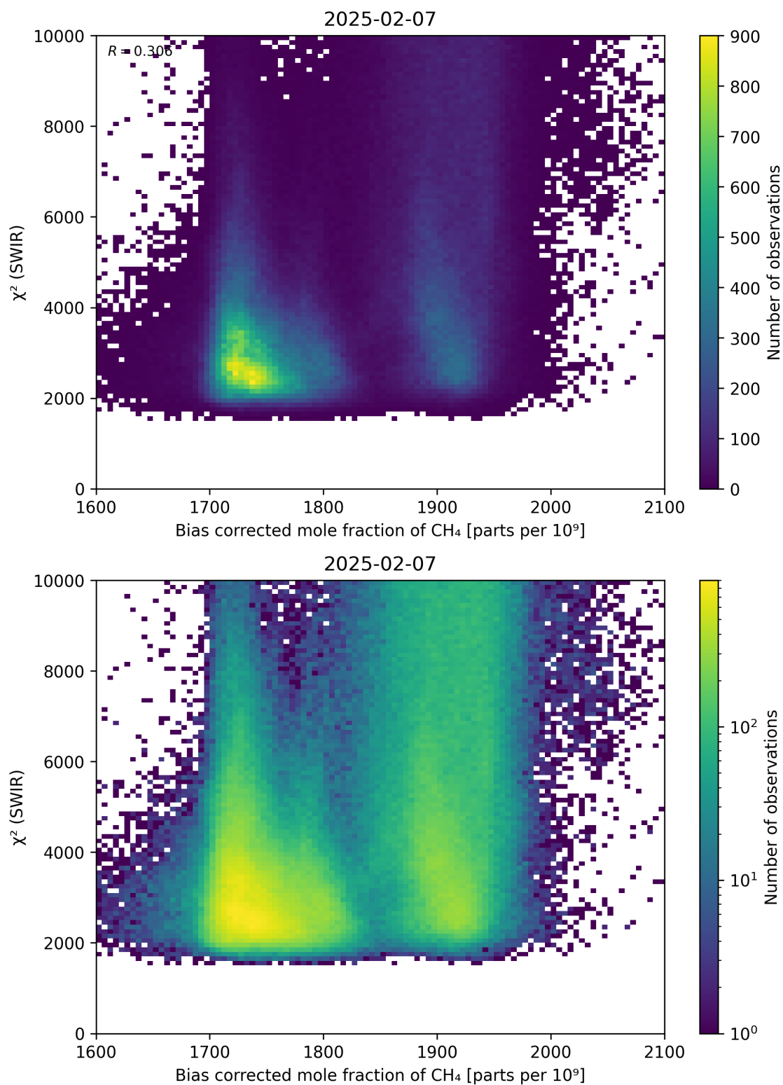
Figure 64: Scatter density plot of “Bias corrected mole fraction of \text{CH}_4 ” against “ \chi^2 (SWIR)” for 2025-02-06 to 2025-02-08.
