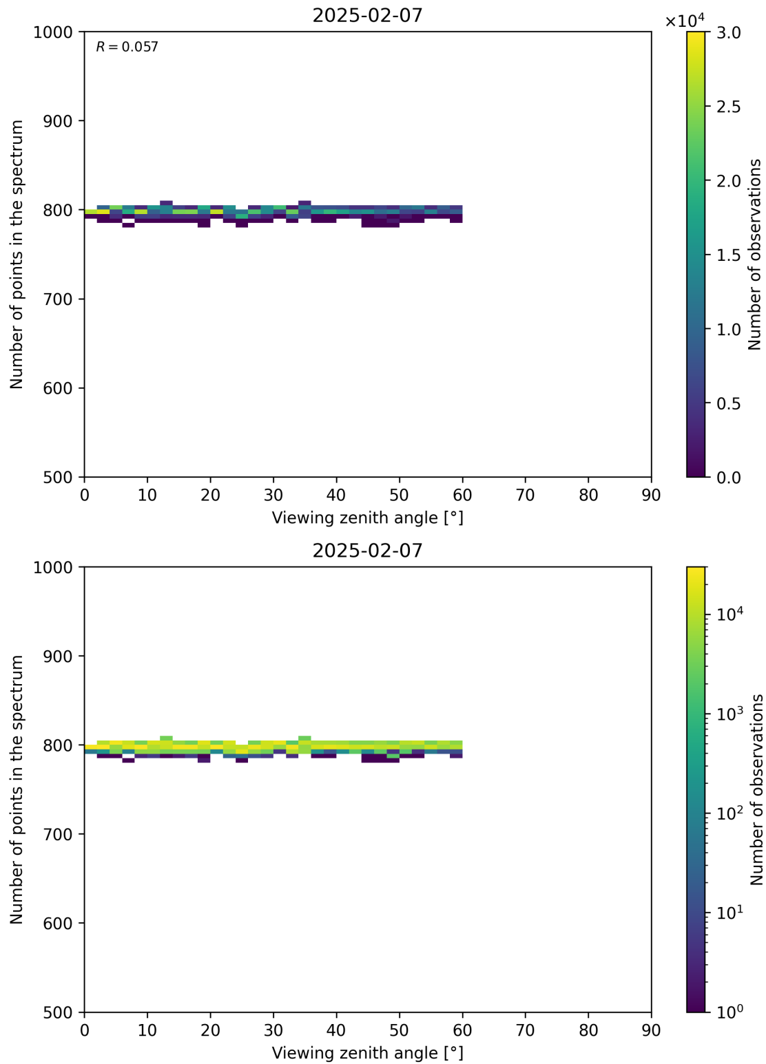
Figure 114: Scatter density plot of “Viewing zenith angle” against “Number of points in the spectrum” for 2025-02-06 to 2025-02-08.
