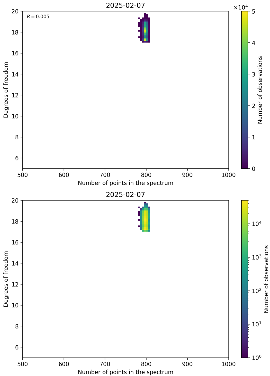
Figure 90: Scatter density plot of “Number of points in the spectrum” against “Degrees of freedom” for 2025-02-06 to 2025-02-08.
