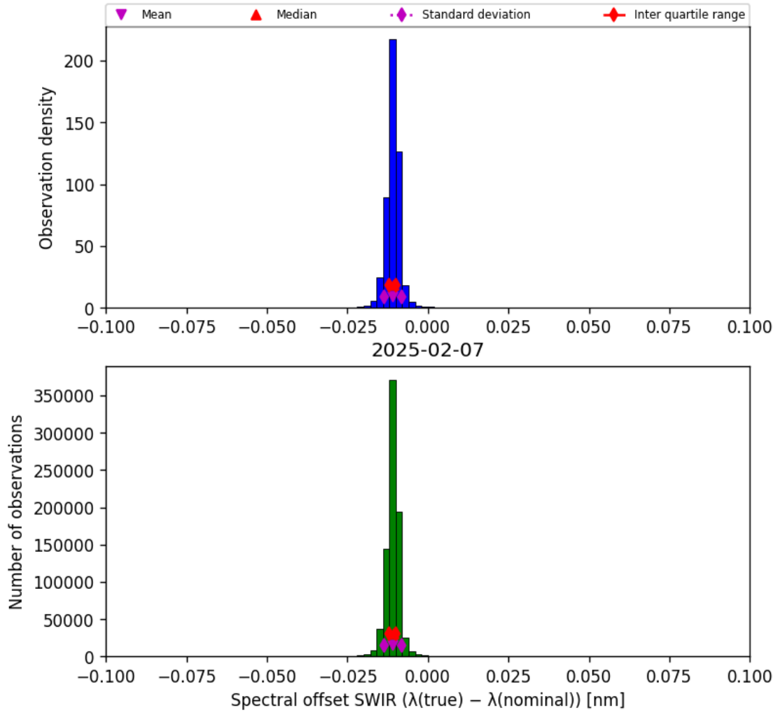
Figure 27: Histogram of “Spectral offset SWIR ( \lambda_{\text{true}} - \lambda_{\text{nominal}} )” for 2025-02-06 to 2025-02-08
