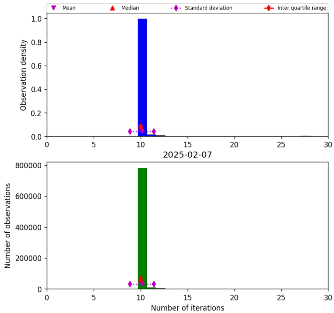
Figure 31: Histogram of “Number of iterations” for 2025-02-06 to 2025-02-08
