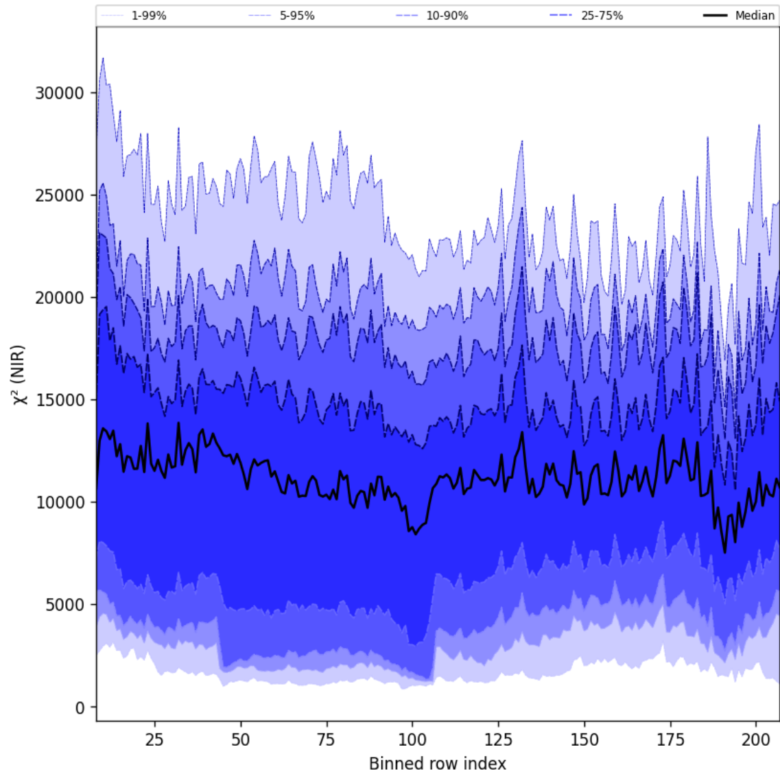
Figure 40: Along track statistics of “ \chi^2 (NIR)” for 2025-02-06 to 2025-02-08
