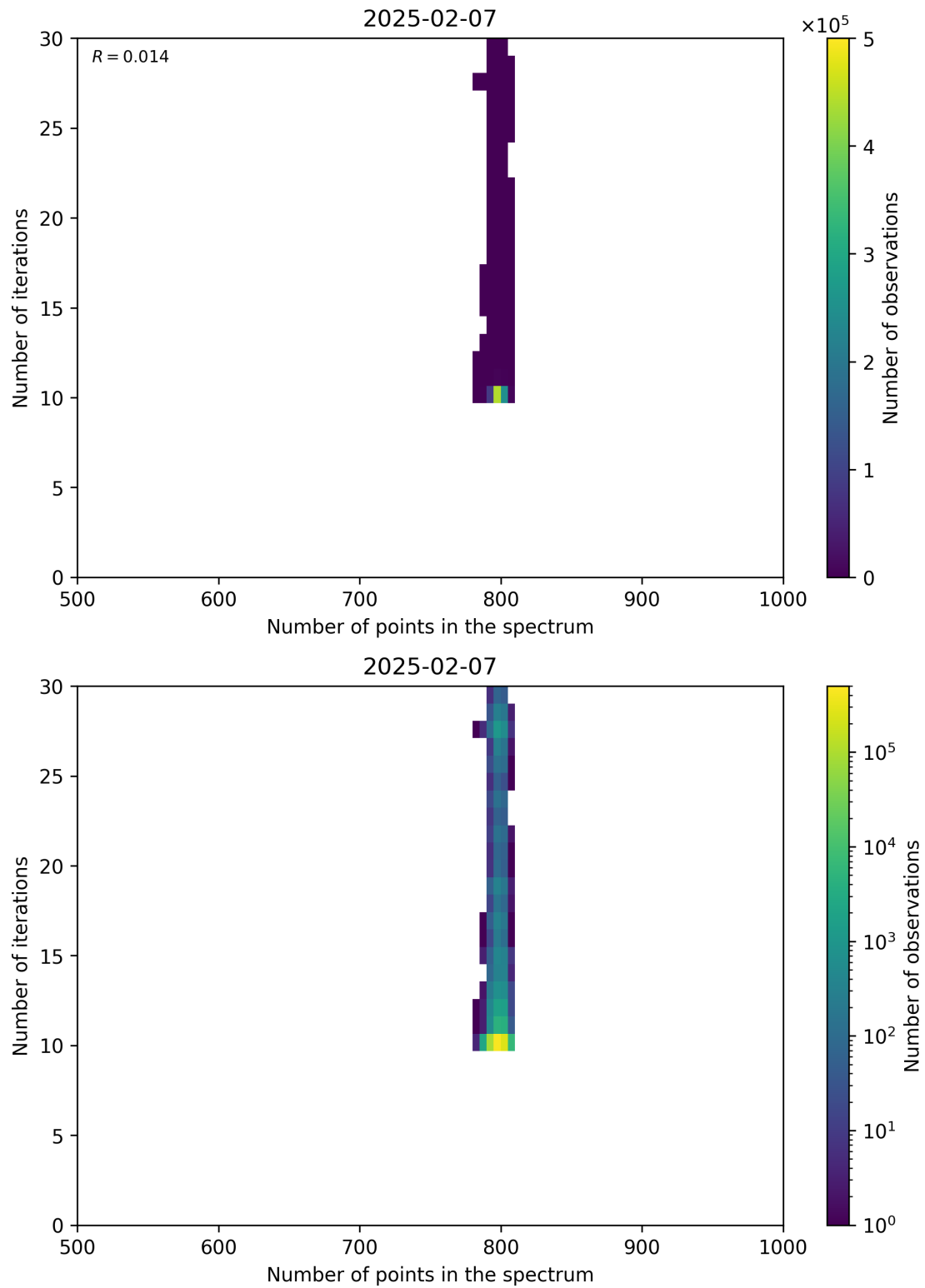
Figure 92: Scatter density plot of “Number of points in the spectrum” against “Number of iterations” for 2025-02-06 to 2025-02-08.
