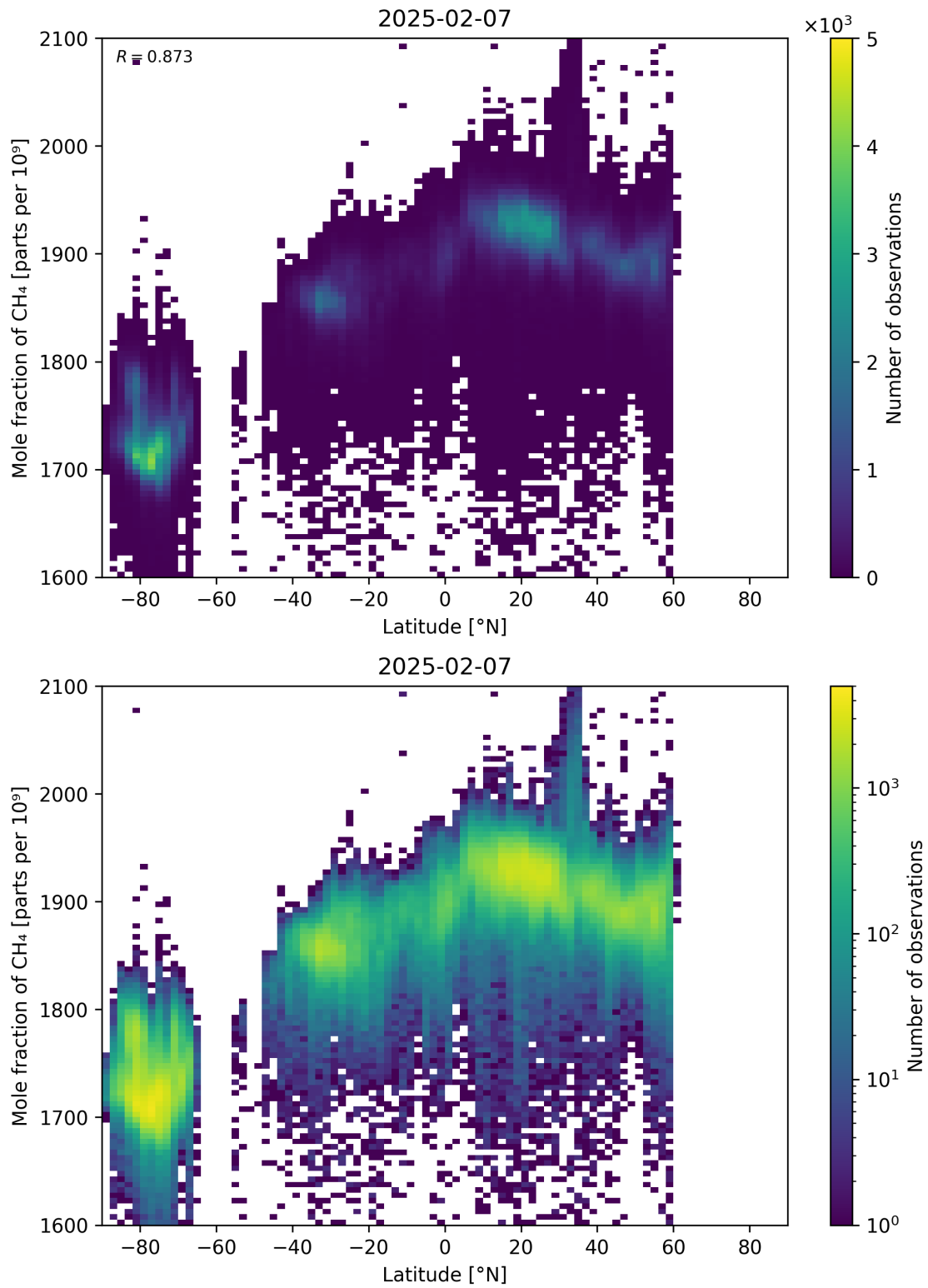
Figure 57: Scatter density plot of “Latitude” against “Mole fraction of CH 4 ” for 2025-02-06 to 2025-02-08.
