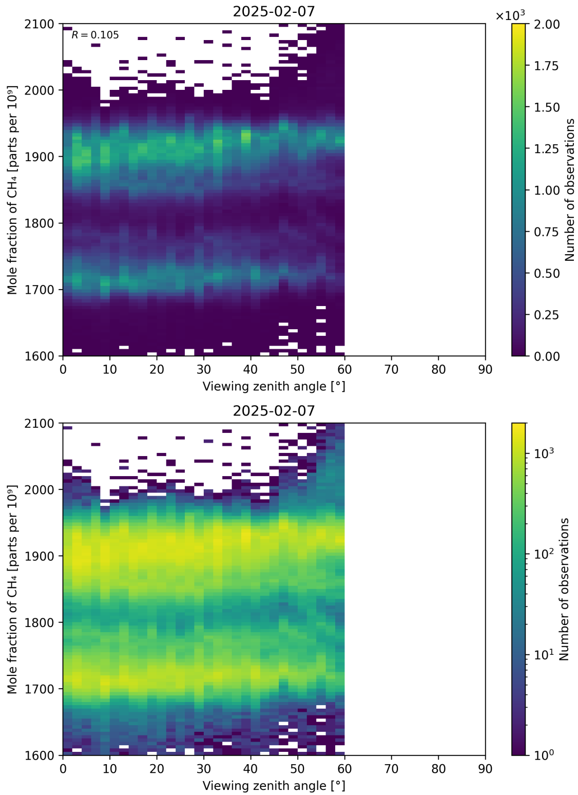
Figure 110: Scatter density plot of “Viewing zenith angle” against “Mole fraction of CH 4 ” for 2025-02-06 to 2025-02-08.
