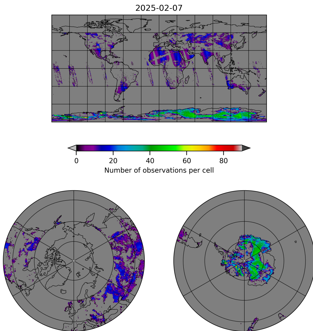
Figure 10: Map of the number of observations for 2025-02-06 to 2025-02-08
