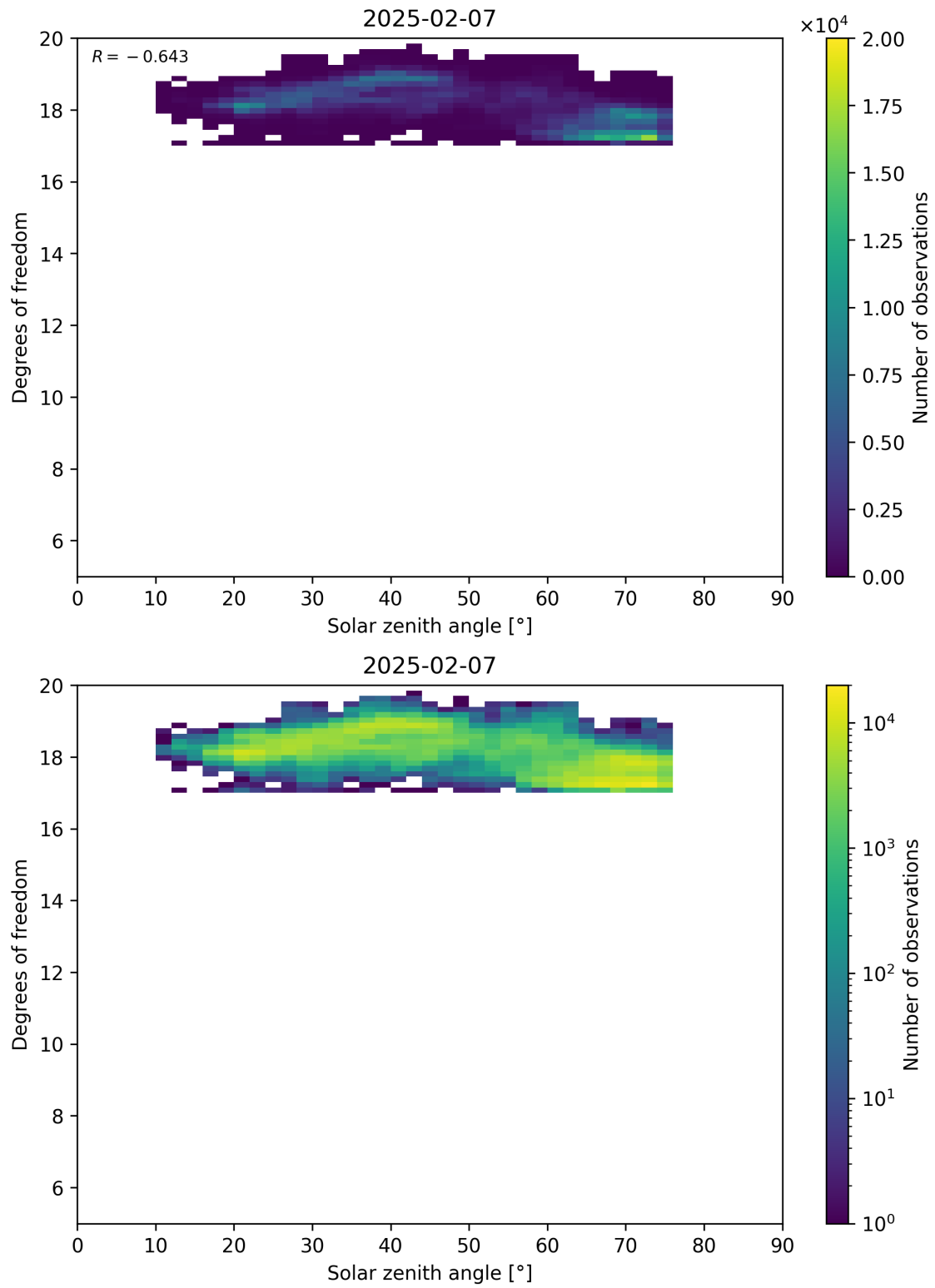
Figure 96: Scatter density plot of “Solar zenith angle” against “Degrees of freedom” for 2025-02-06 to 2025-02-08.
