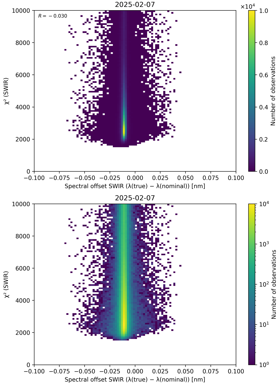
Figure 118: Scatter density plot of “Spectral offset SWIR ( \lambda_{\text{true}} - \lambda_{\text{nominal}} )” against “ \chi^2 (SWIR)” for 2025-02-06 to 2025-02-08.
