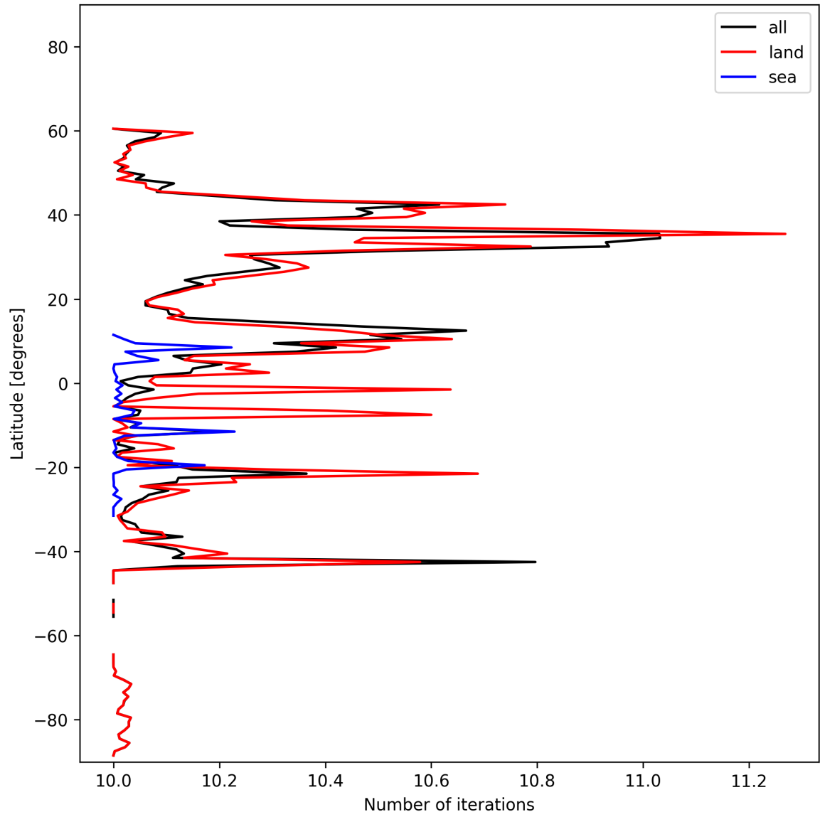
Figure 20: Zonal average of “Number of iterations” for 2025-02-06 to 2025-02-08.
