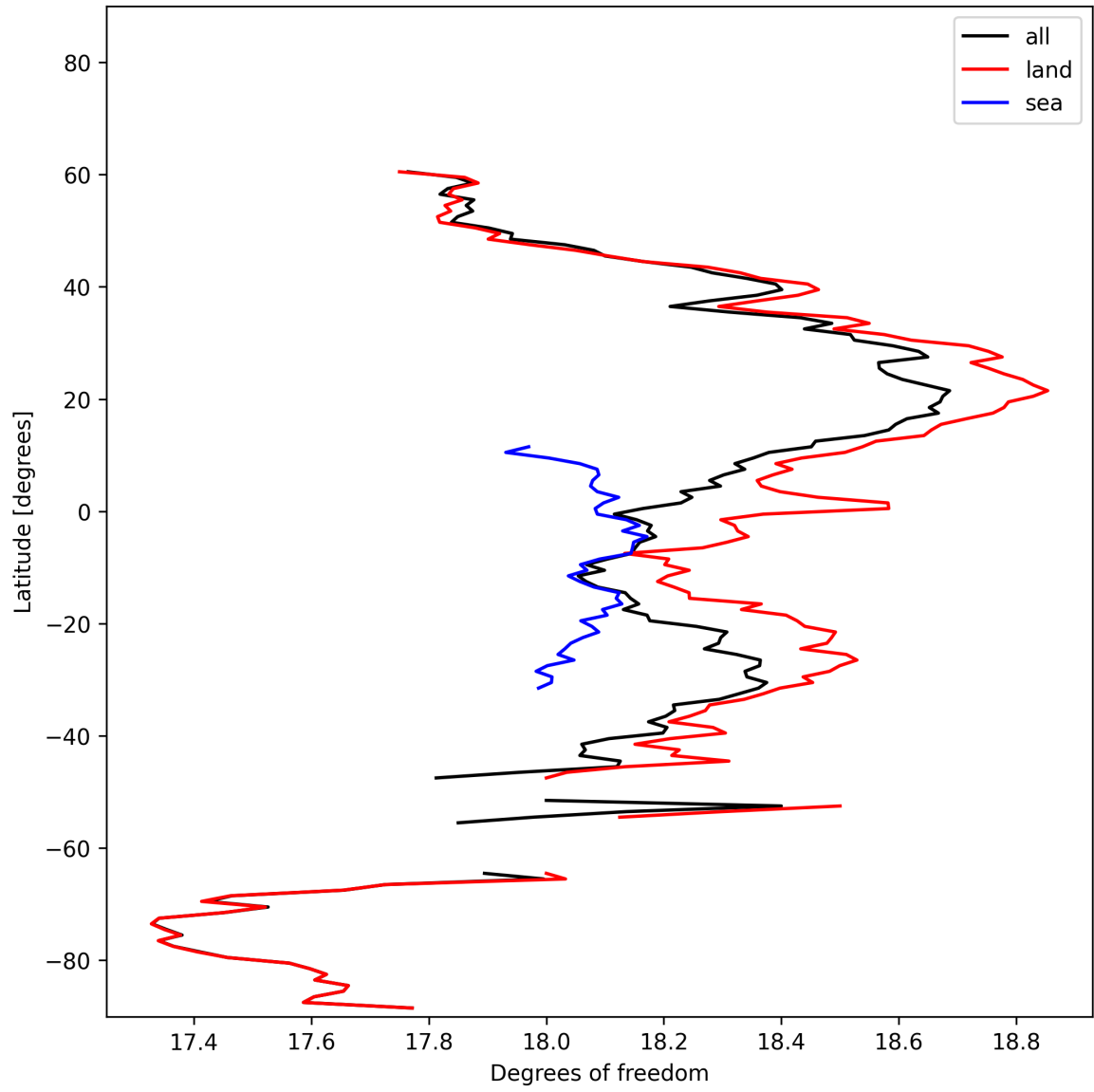
Figure 19: Zonal average of “Degrees of freedom” for 2025-02-06 to 2025-02-08.
