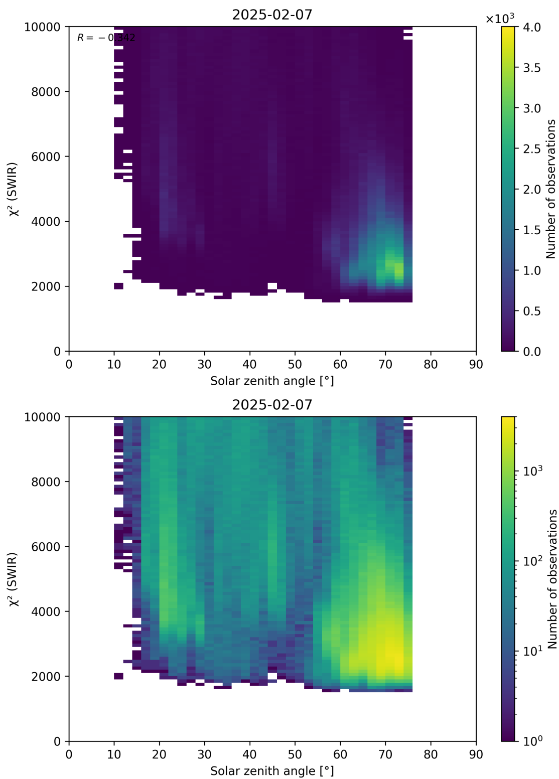
Figure 95: Scatter density plot of “Solar zenith angle” against “ \chi^2 (SWIR)” for 2025-02-06 to 2025-02-08.
