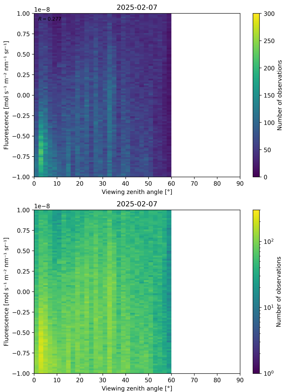
Figure 108: Scatter density plot of “Viewing zenith angle” against “Fluorescence” for 2025-02-06 to 2025-02-08.
