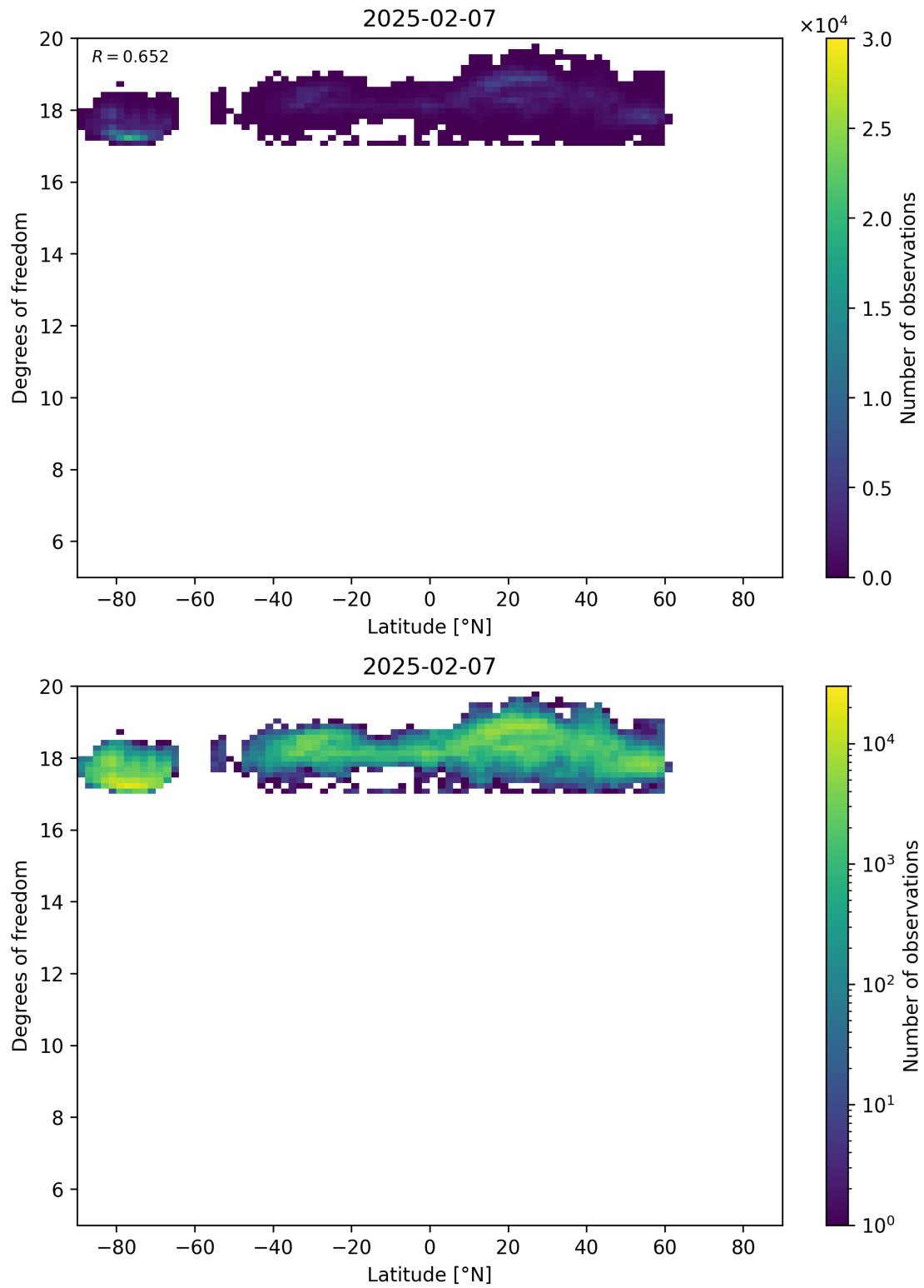
Figure 55: Scatter density plot of “Latitude” against “Degrees of freedom” for 2025-02-06 to 2025-02-08.
