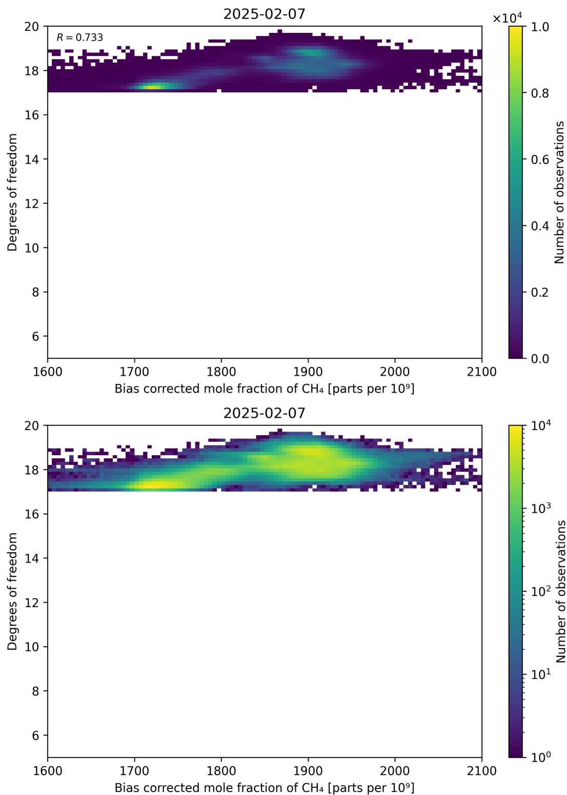
Figure 65: Scatter density plot of “Bias corrected mole fraction of CH 4 ” against “Degrees of freedom” for 2025-02-06 to 2025-02-08.
