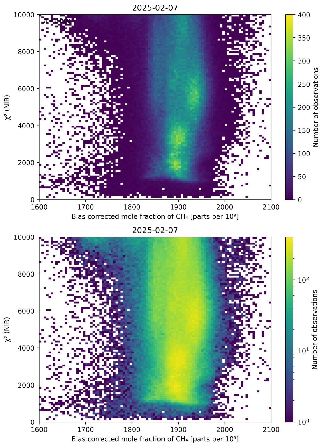
Figure 63: Scatter density plot of “Bias corrected mole fraction of CH 4 ” against “ \chi^2 (NIR)” for 2025-02-06 to 2025-02-08.
