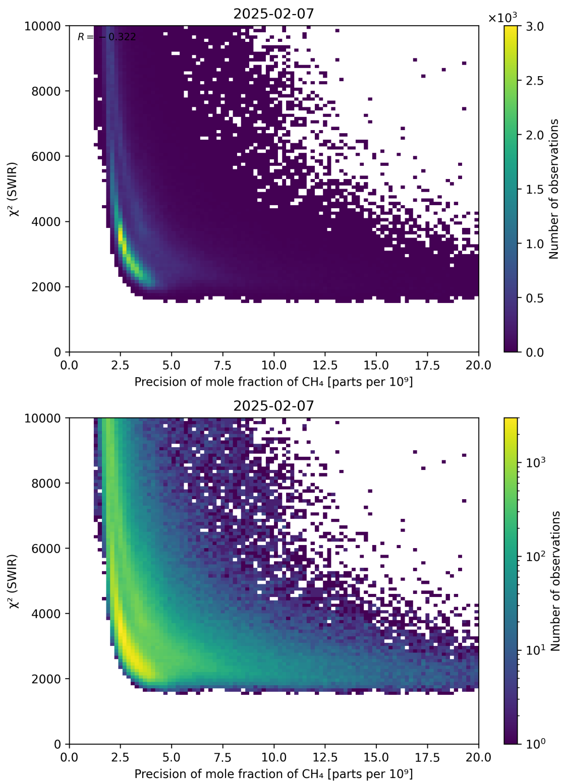
Figure 79: Scatter density plot of “Precision of mole fraction of CH 4 ” against “ \chi^2 (SWIR)” for 2025-02-06 to 2025-02-08.
