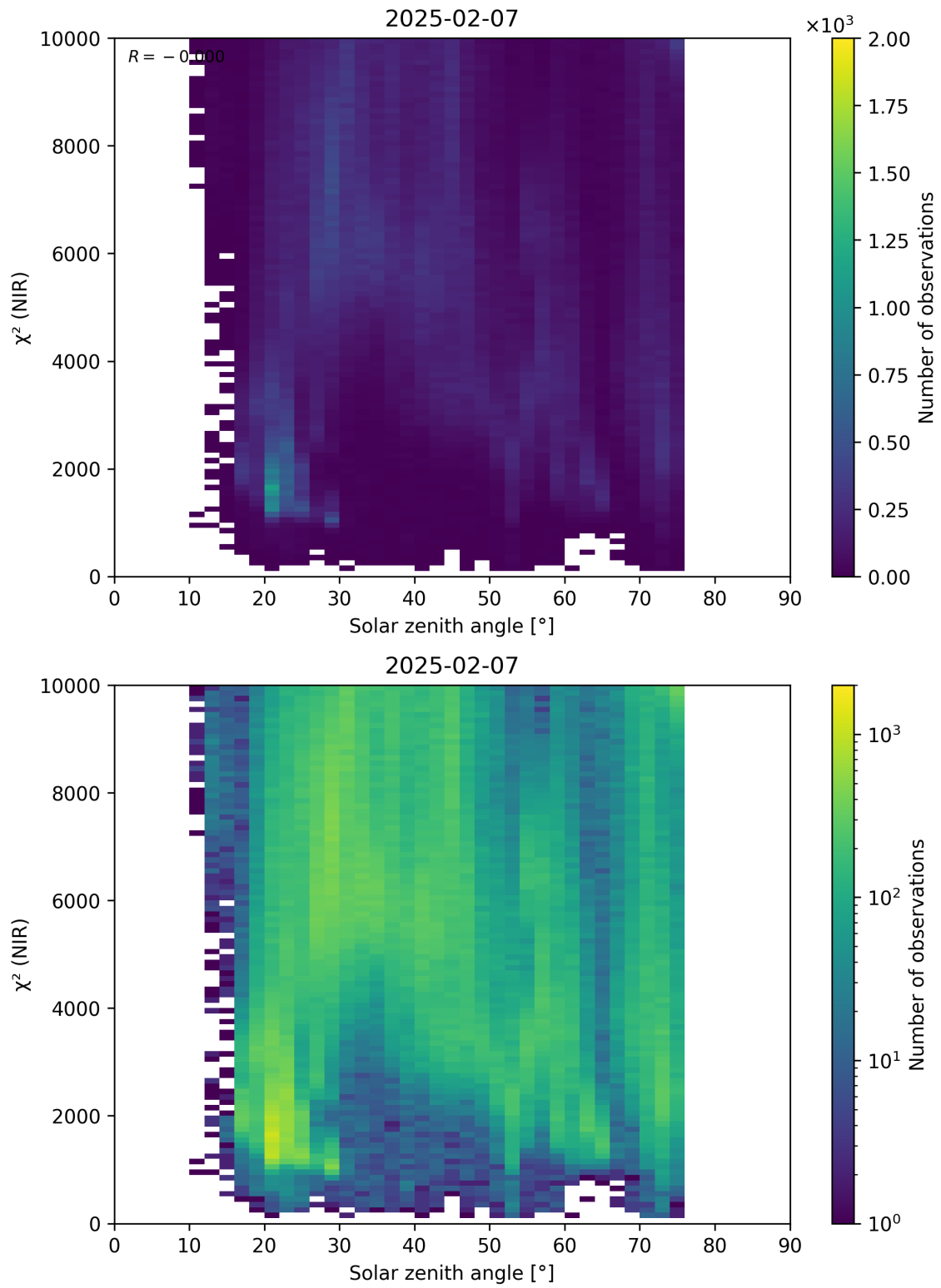
Figure 94: Scatter density plot of “Solar zenith angle” against “ \chi^2 (NIR)” for 2025-02-06 to 2025-02-08.
