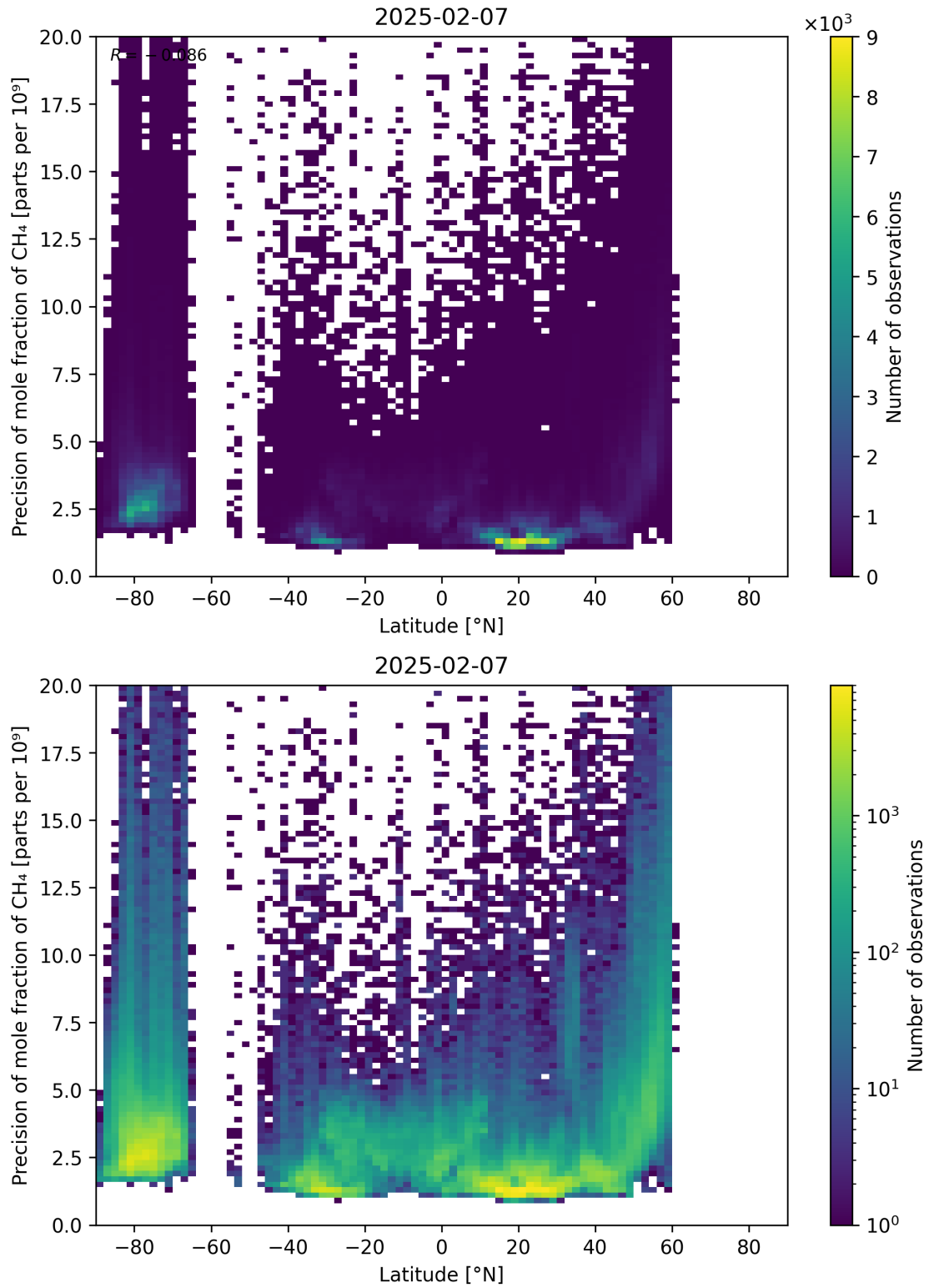
Figure 59: Scatter density plot of “Latitude” against “Precision of mole fraction of CH 4 ” for 2025-02-06 to 2025-02-08.
