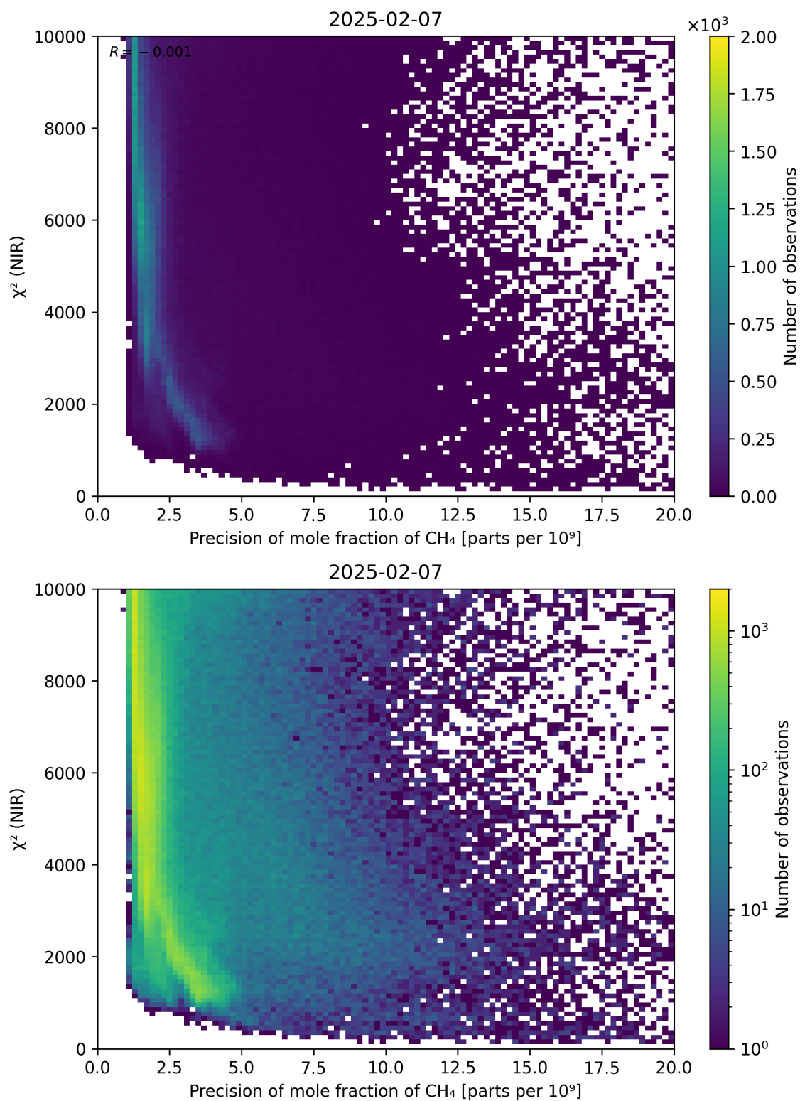
Figure 78: Scatter density plot of “Precision of mole fraction of CH 4 ” against “ \chi^2 (NIR)” for 2025-02-06 to 2025-02-08.
