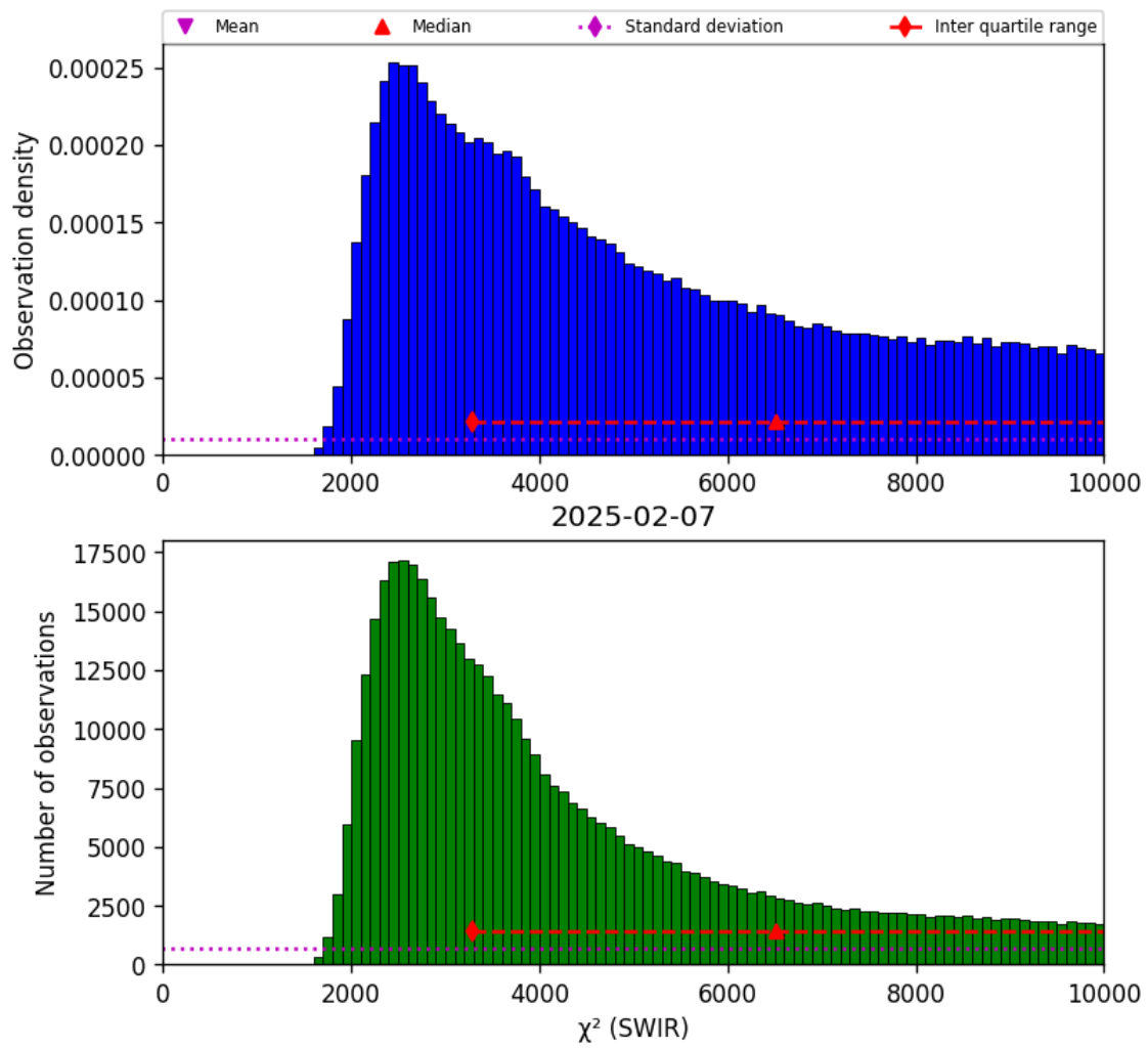
Figure 28: Histogram of “ \chi^2 (SWIR)” for 2025-02-06 to 2025-02-08
