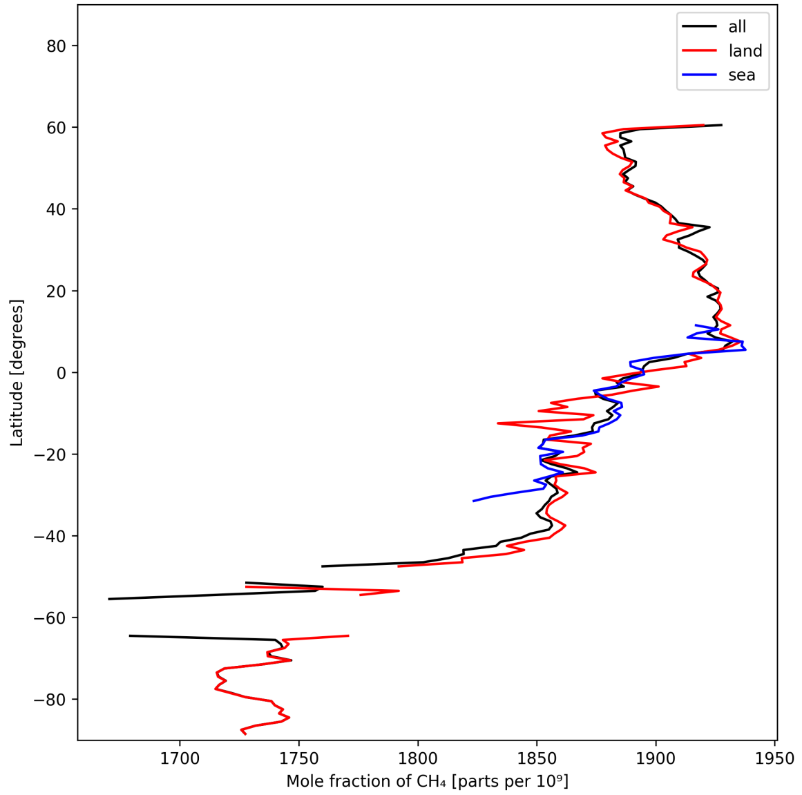
Figure 12: Zonal average of “Mole fraction of \text{CH}_4 ” for 2025-02-06 to 2025-02-08.
