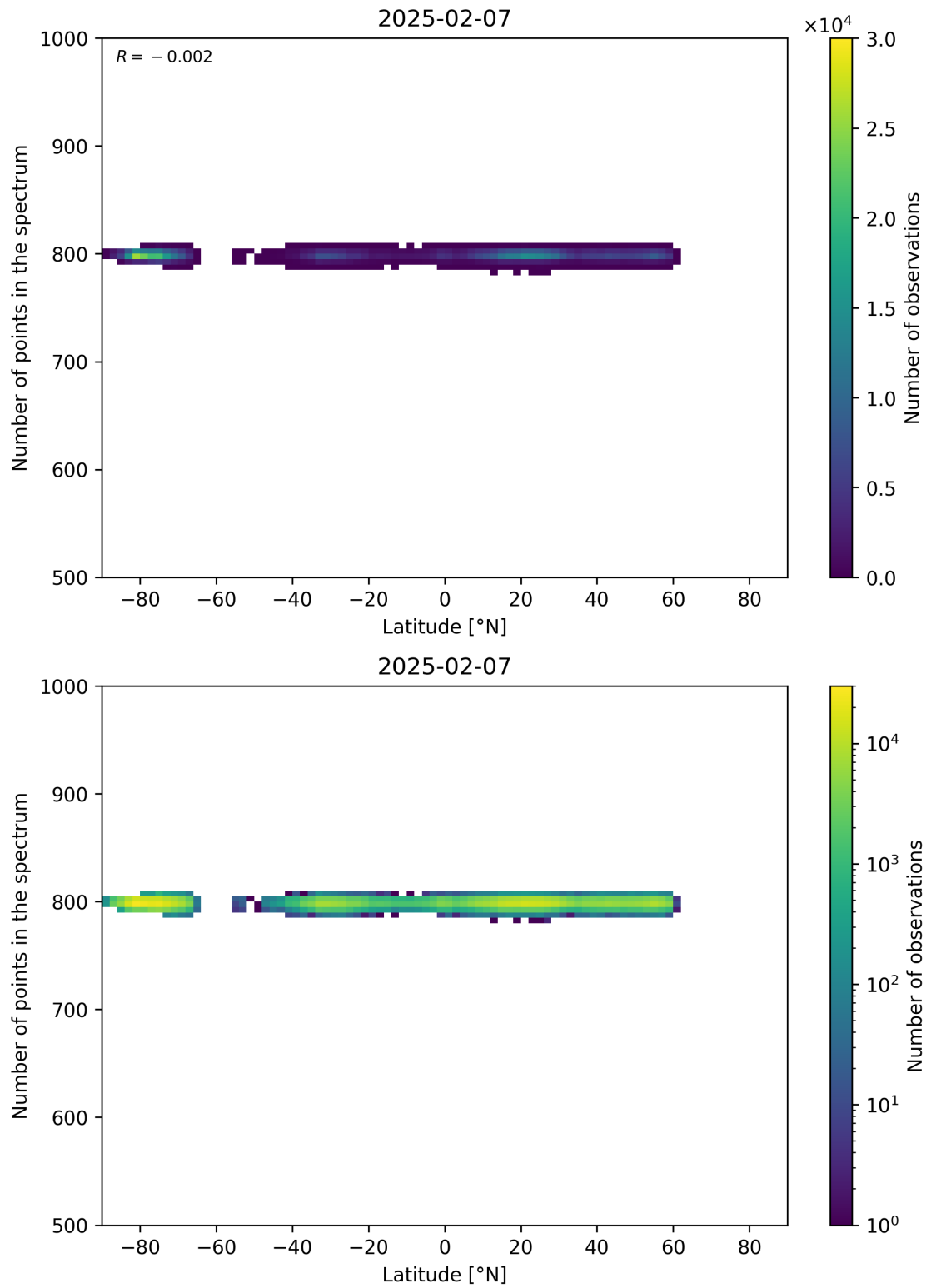
Figure 61: Scatter density plot of “Latitude” against “Number of points in the spectrum” for 2025-02-06 to 2025-02-08.
