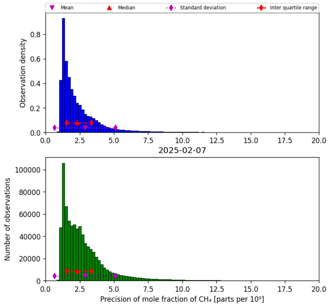
Figure 24: Histogram of “Precision of mole fraction of CH 4 ” for 2025-02-06 to 2025-02-08
