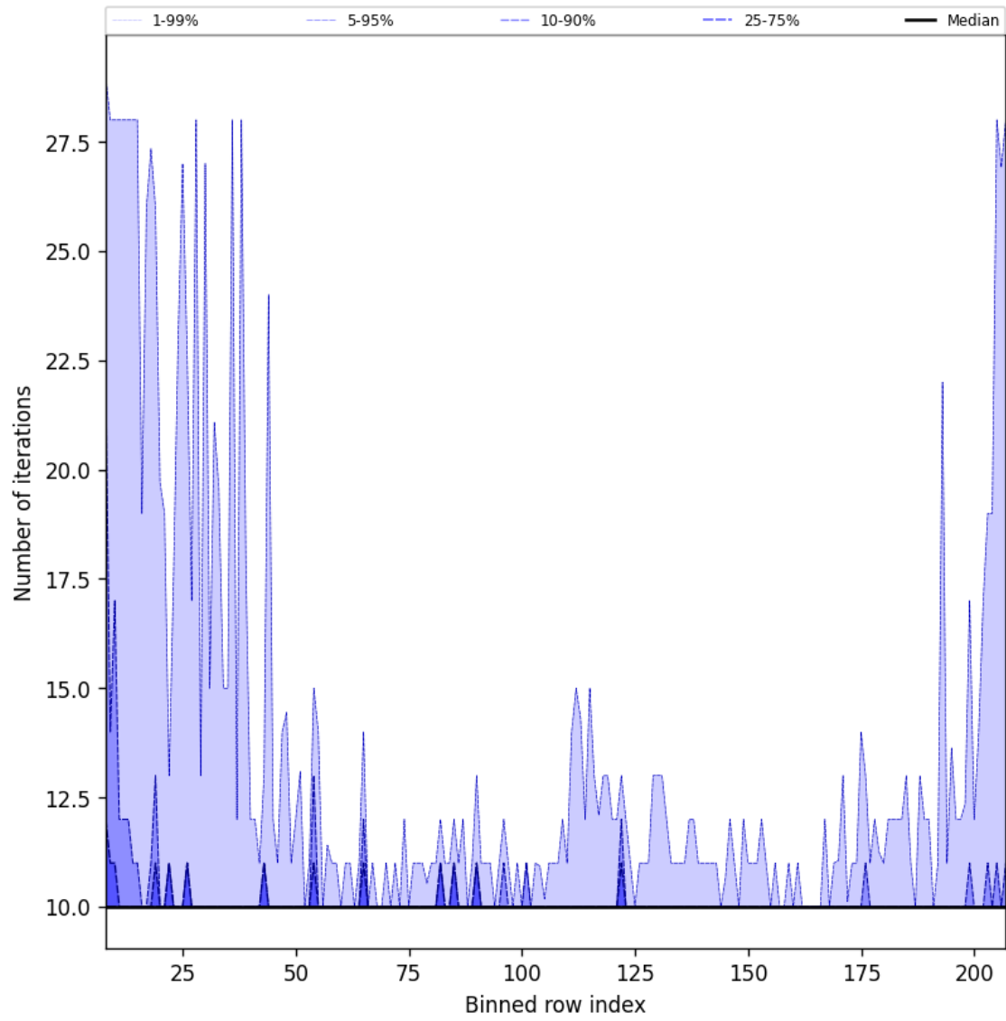
Figure 42: Along track statistics of “Number of iterations” for 2025-02-06 to 2025-02-08
