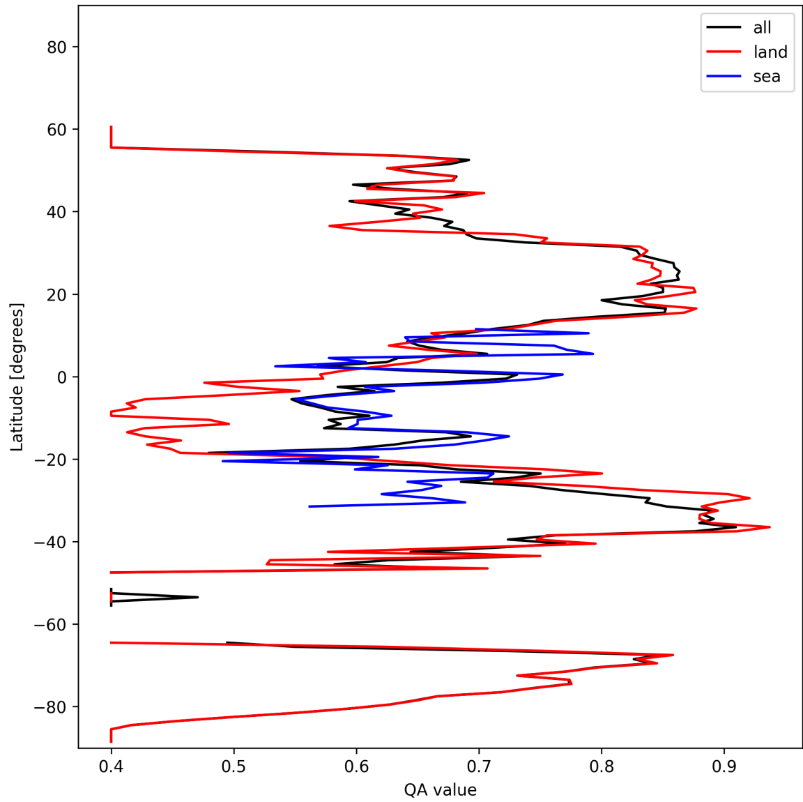
Figure 11: Zonal average of “QA value” for 2025-02-06 to 2025-02-08.
