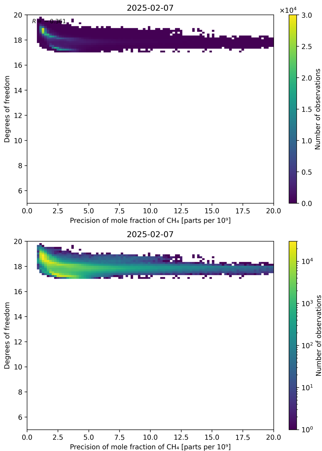
Figure 80: Scatter density plot of “Precision of mole fraction of CH 4 ” against “Degrees of freedom” for 2025-02-06 to 2025-02-08.
