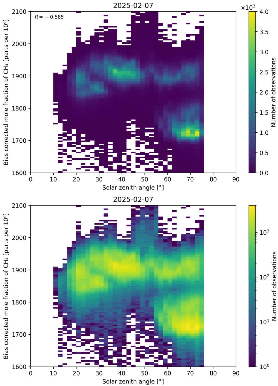
Figure 100: Scatter density plot of “Solar zenith angle” against “Bias corrected mole fraction of CH 4 ” for 2025-02-06 to 2025-02-08.
