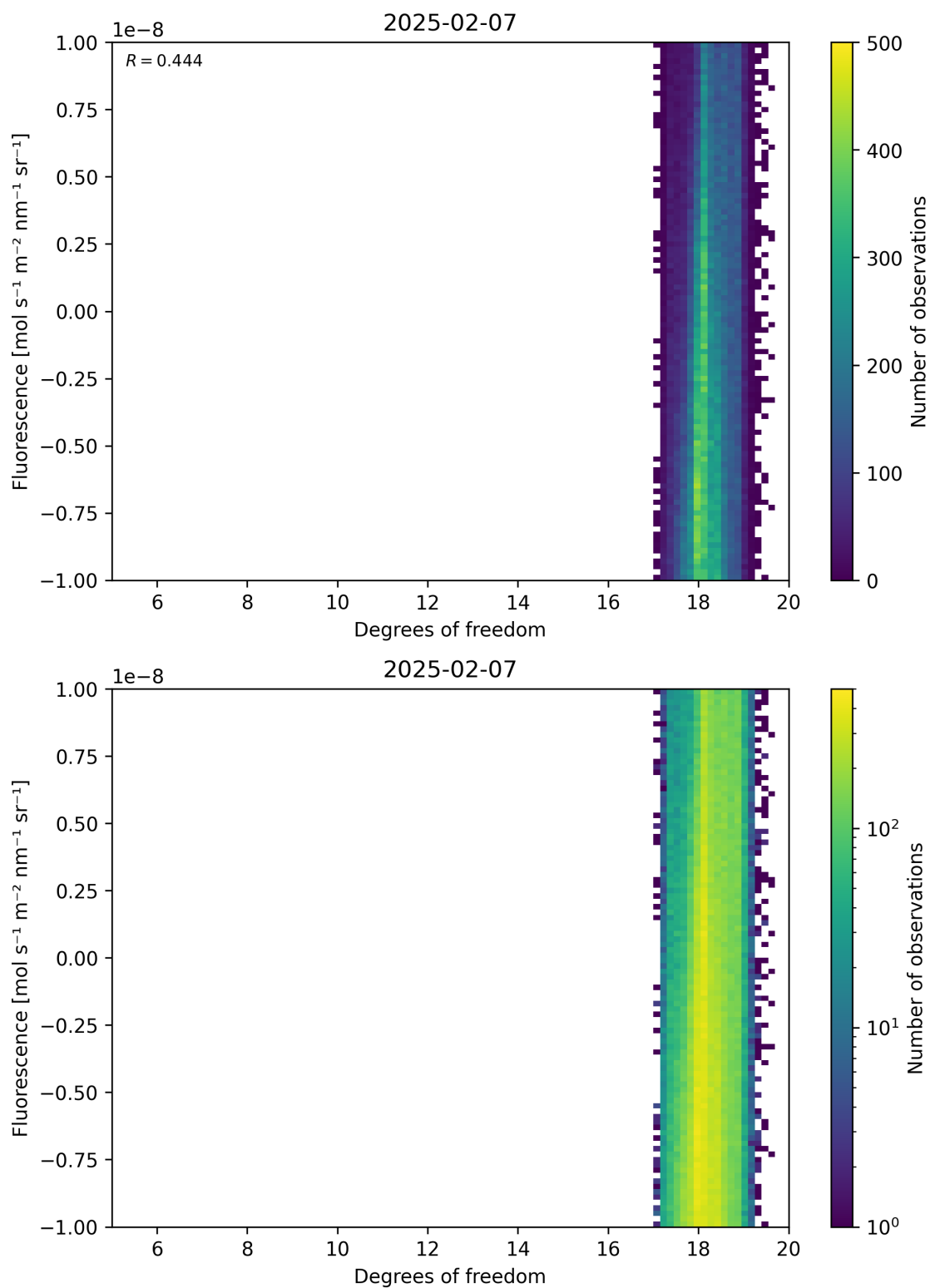
Figure 51: Scatter density plot of “Degrees of freedom” against “Fluorescence” for 2025-02-06 to 2025-02-08.
