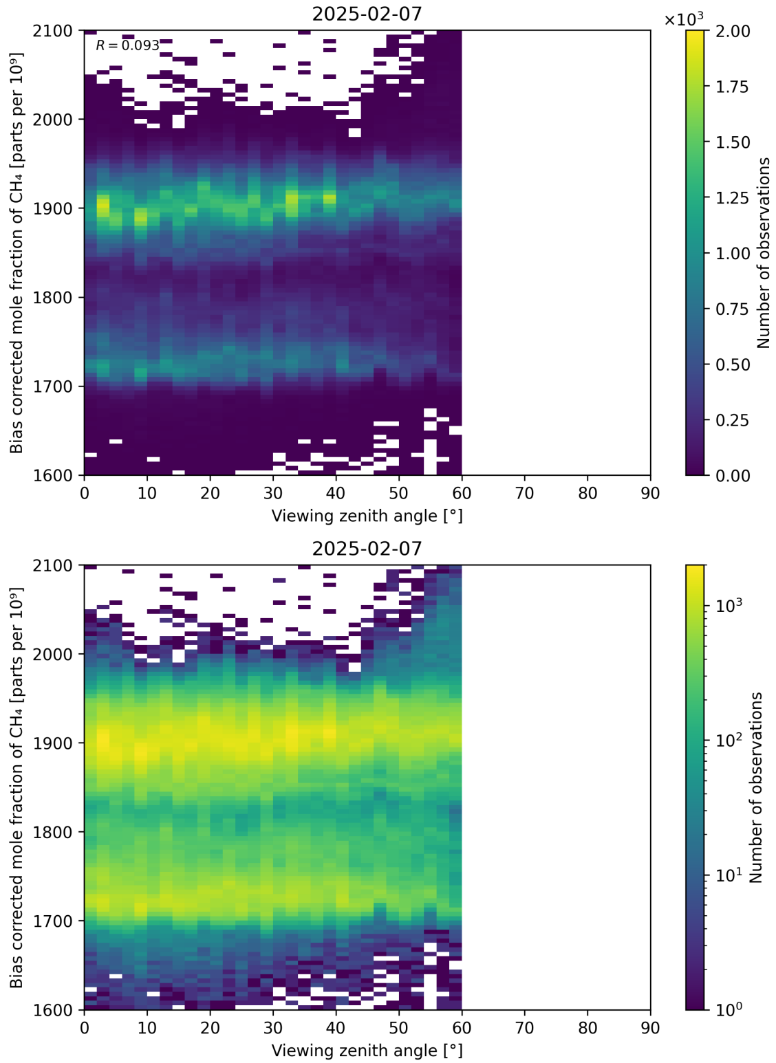
Figure 111: Scatter density plot of “Viewing zenith angle” against “Bias corrected mole fraction of CH 4 ” for 2025-02-06 to 2025-02-08.
