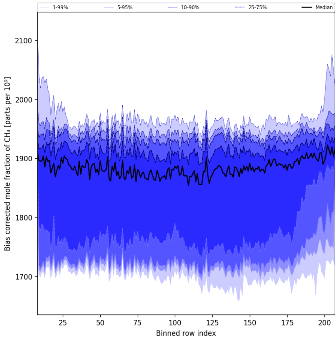
Figure 36: Along track statistics of “Bias corrected mole fraction of CH 4 ” for 2025-02-06 to 2025-02-08
