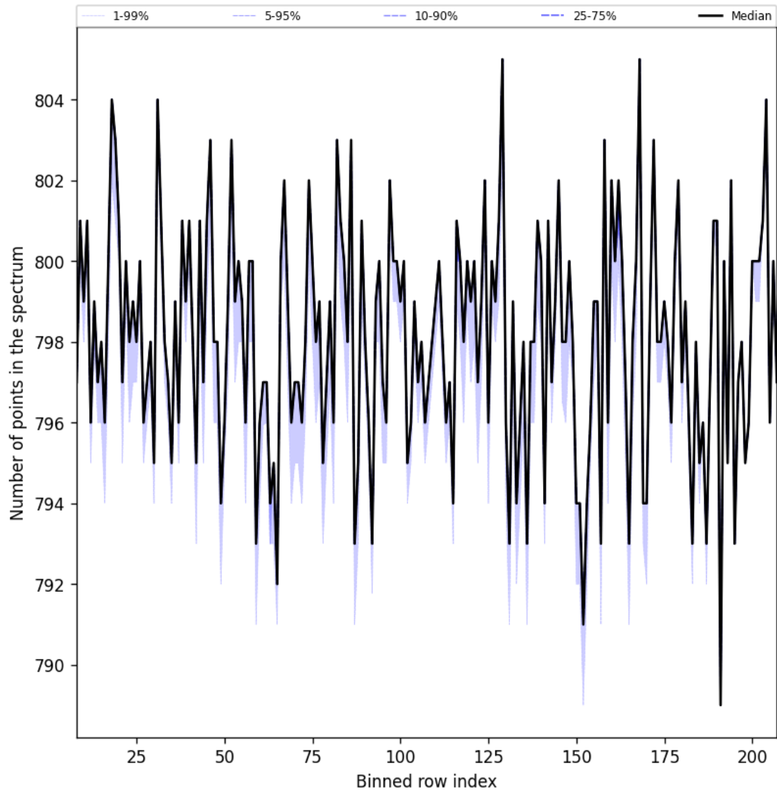
Figure 37: Along track statistics of “Number of points in the spectrum” for 2025-02-06 to 2025-02-08
