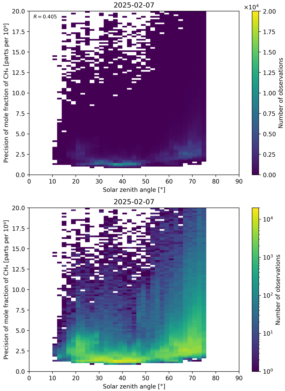
Figure 101: Scatter density plot of “Solar zenith angle” against “Precision of mole fraction of CH 4 ” for 2025-02-06 to 2025-02-08.
