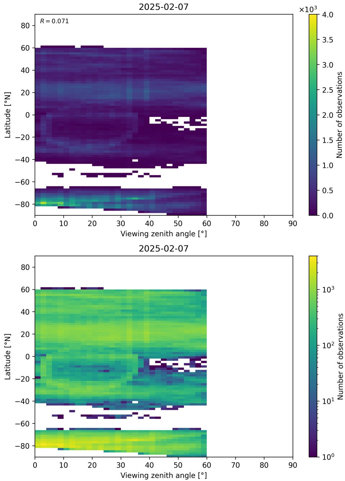
Figure 109: Scatter density plot of “Viewing zenith angle” against “Latitude” for 2025-02-06 to 2025-02-08.
