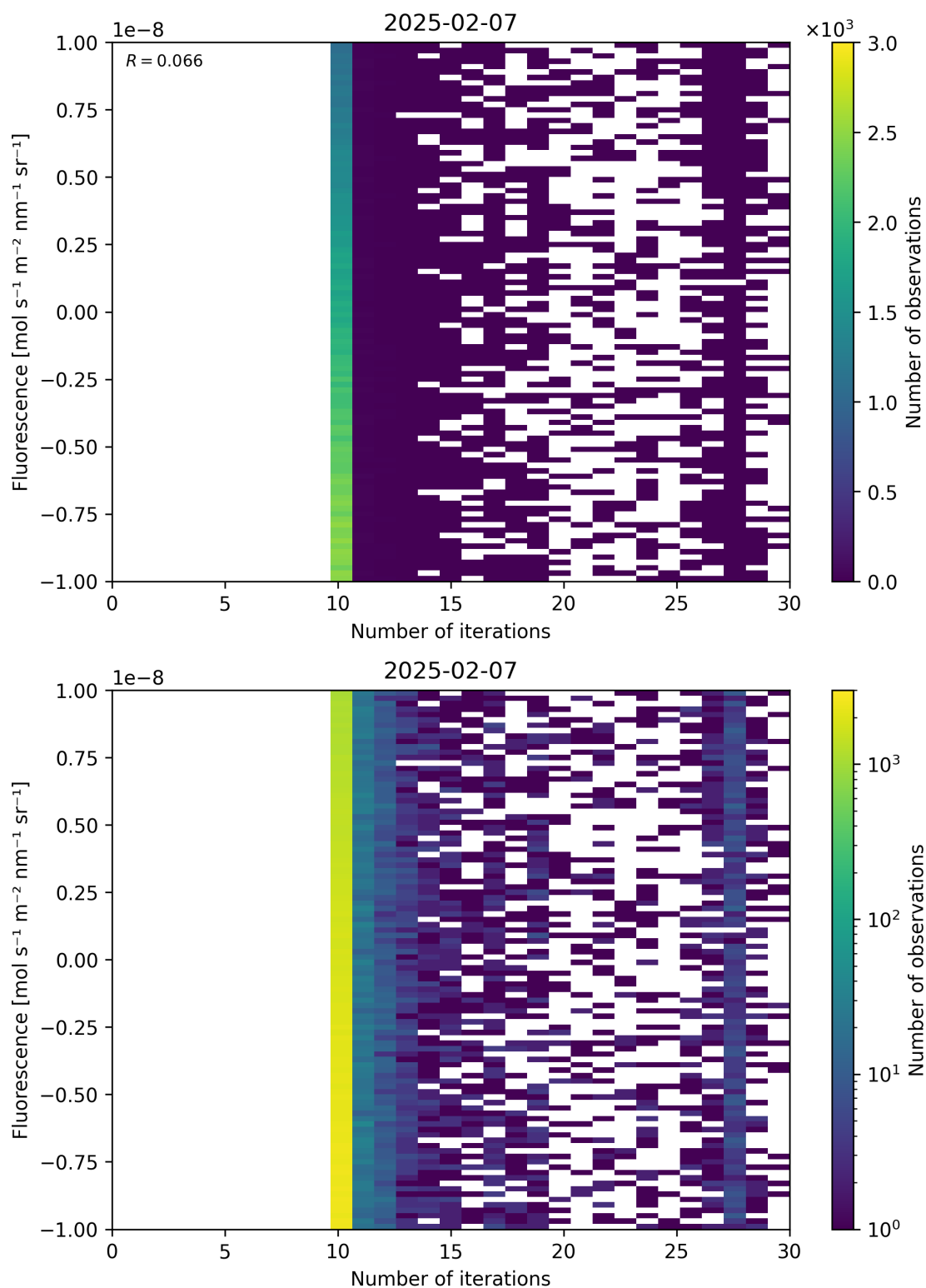
Figure 87: Scatter density plot of “Number of iterations” against “Fluorescence” for 2025-02-06 to 2025-02-08.
