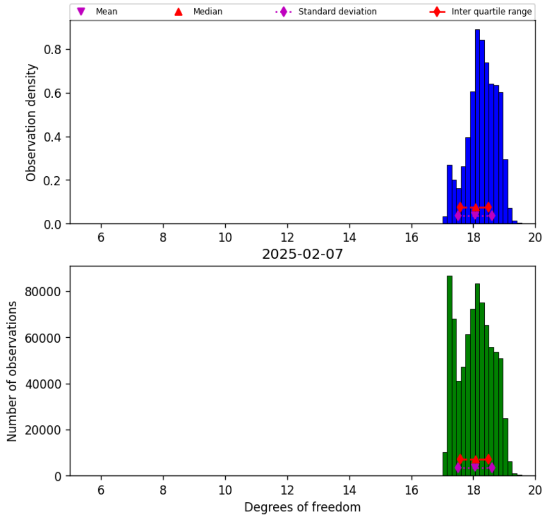
Figure 30: Histogram of “Degrees of freedom” for 2025-02-06 to 2025-02-08
