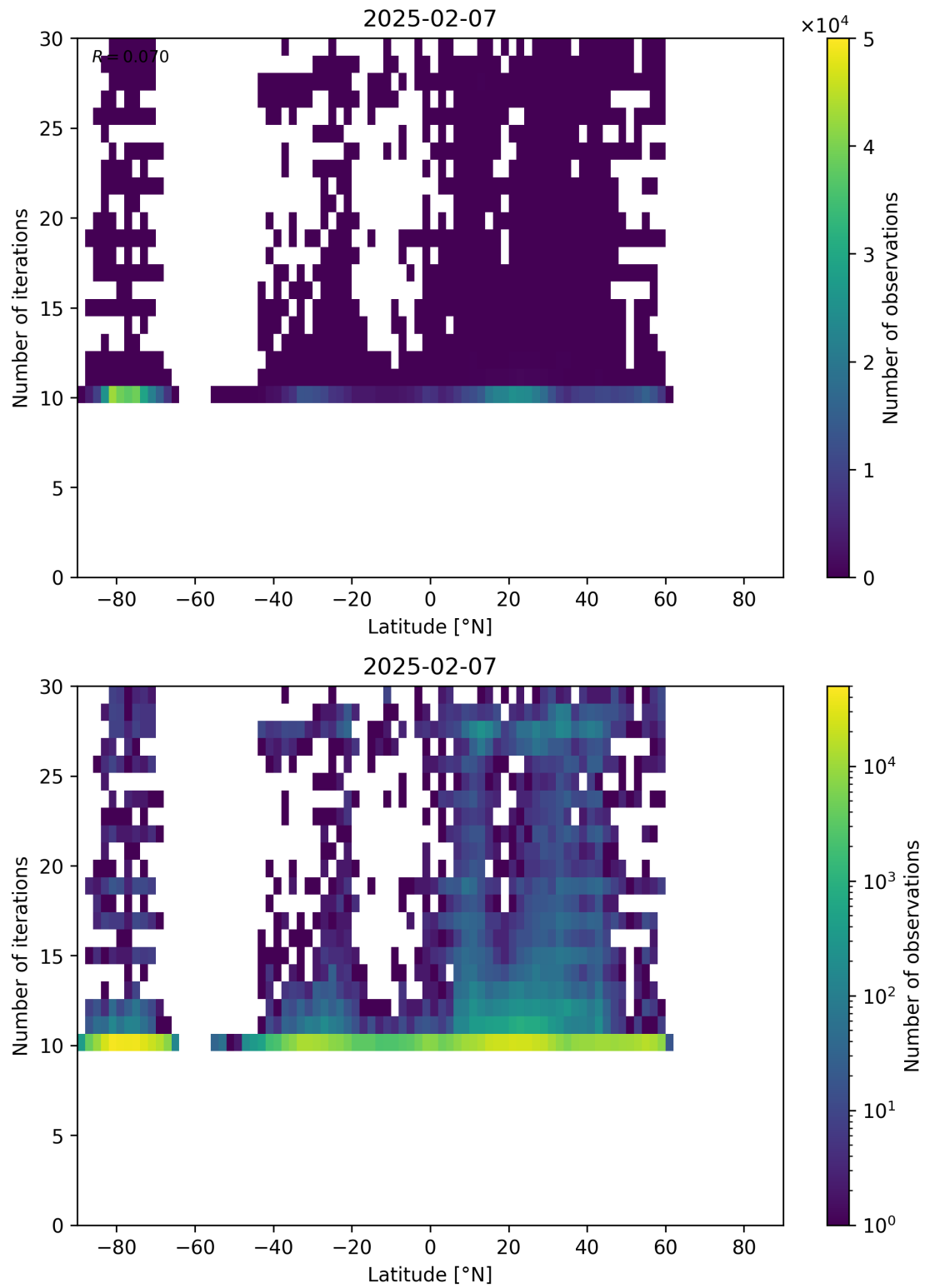
Figure 60: Scatter density plot of “Latitude” against “Number of iterations” for 2025-02-06 to 2025-02-08.
