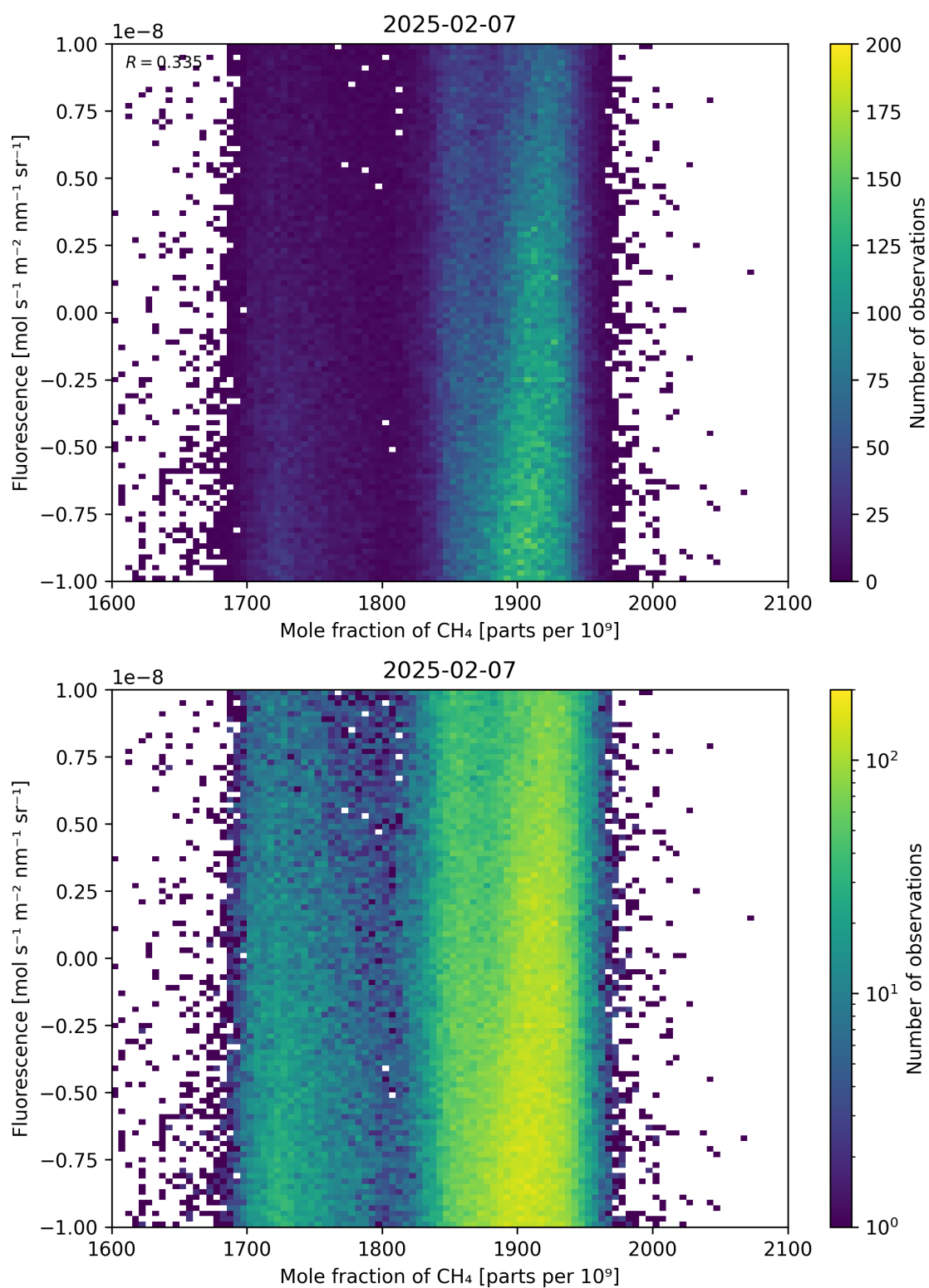
Figure 73: Scatter density plot of “Mole fraction of \text{CH}_4 ” against “Fluorescence” for 2025-02-06 to 2025-02-08.
