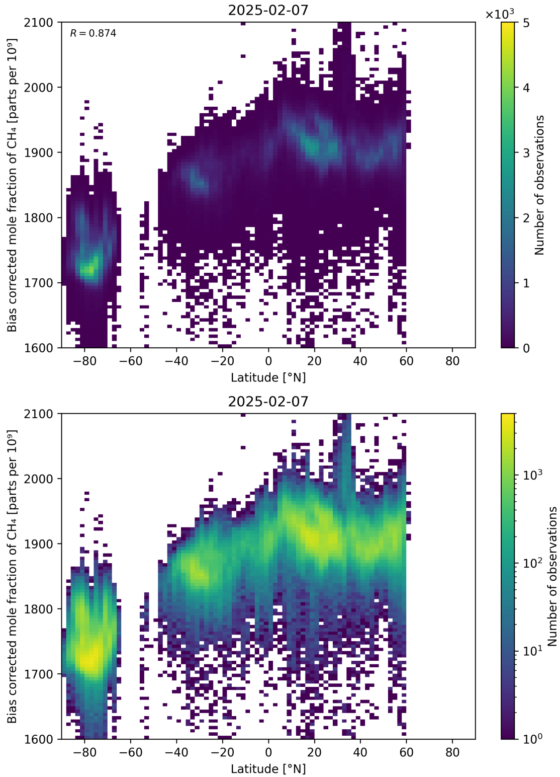
Figure 58: Scatter density plot of “Latitude” against “Bias corrected mole fraction of CH 4 ” for 2025-02-06 to 2025-02-08.
