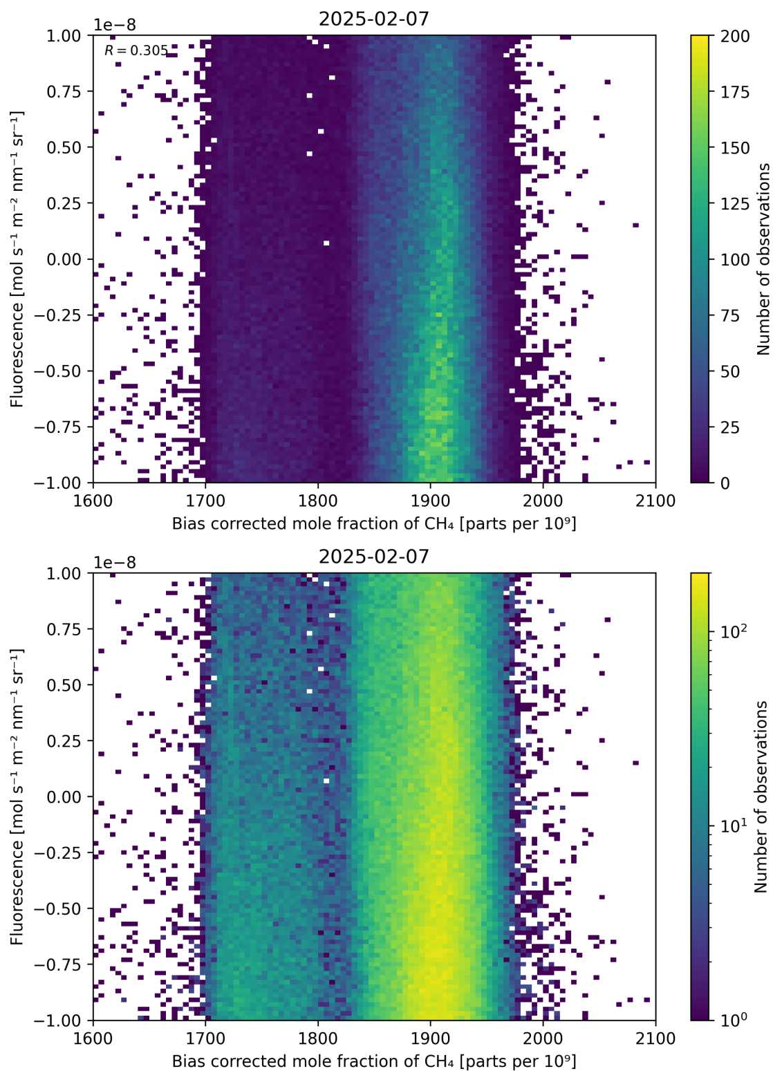
Figure 66: Scatter density plot of “Bias corrected mole fraction of \text{CH}_4 ” against “Fluorescence” for 2025-02-06 to 2025-02-08.
