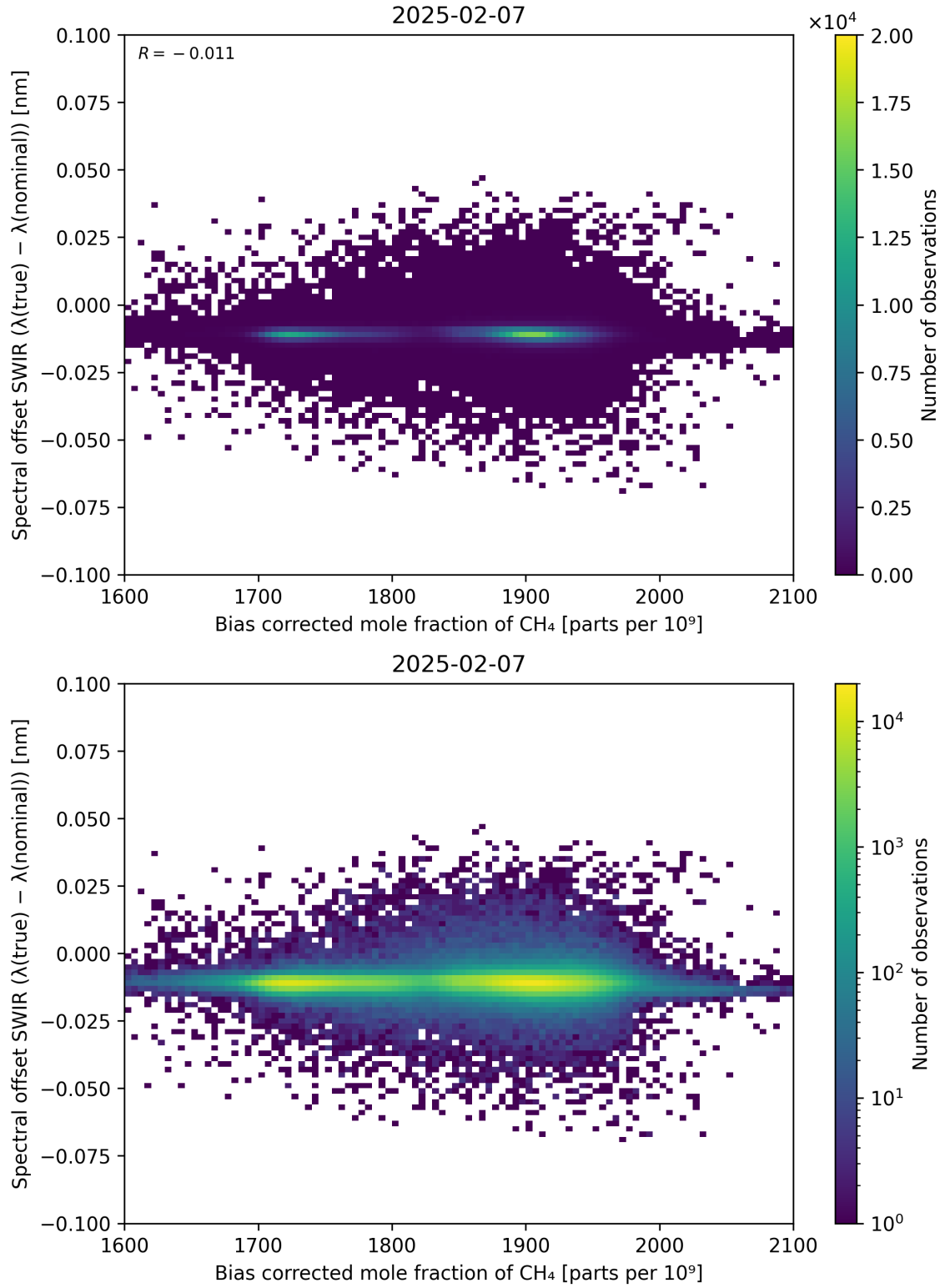
Figure 69: Scatter density plot of “Bias corrected mole fraction of \text{CH}_4 ” against “Spectral offset SWIR ( \lambda_{\text{true}} - \lambda_{\text{nominal}} )” for 2025-02-06 to 2025-02-08.
