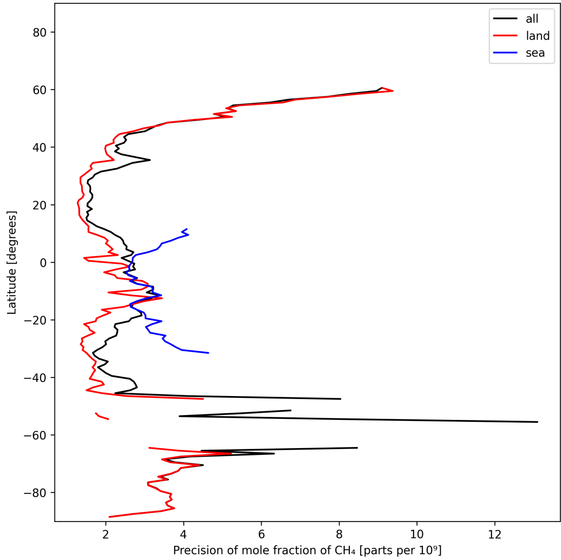
Figure 13: Zonal average of “Precision of mole fraction of CH 4 ” for 2025-02-06 to 2025-02-08.
