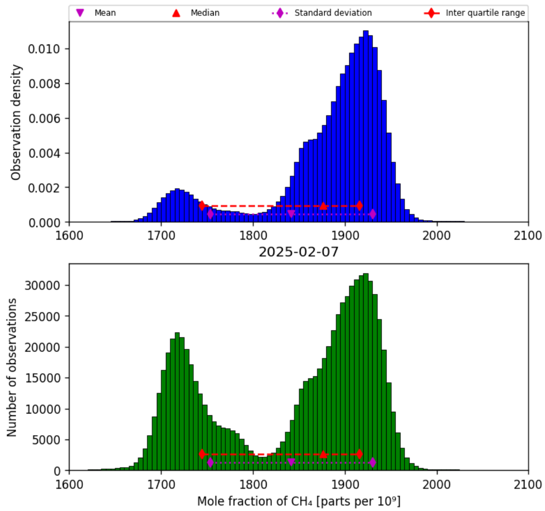
Figure 23: Histogram of “Mole fraction of CH 4 ” for 2025-02-06 to 2025-02-08
