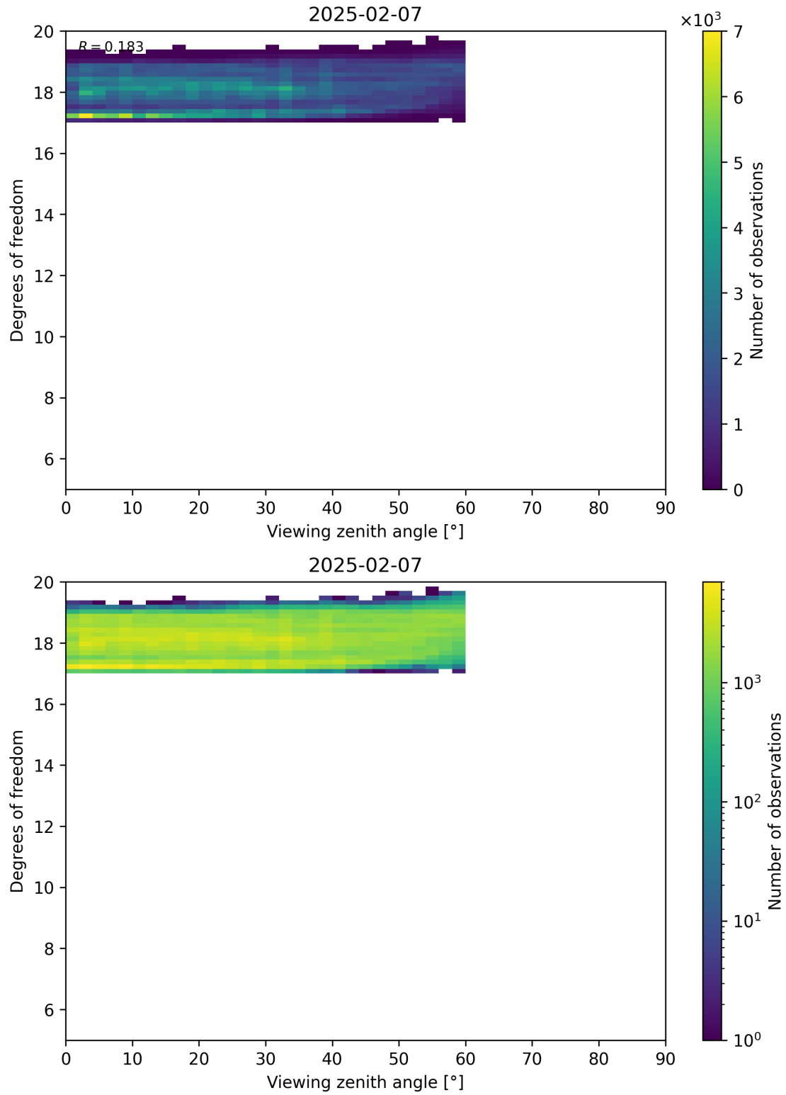
Figure 107: Scatter density plot of “Viewing zenith angle” against “Degrees of freedom” for 2025-02-06 to 2025-02-08.
