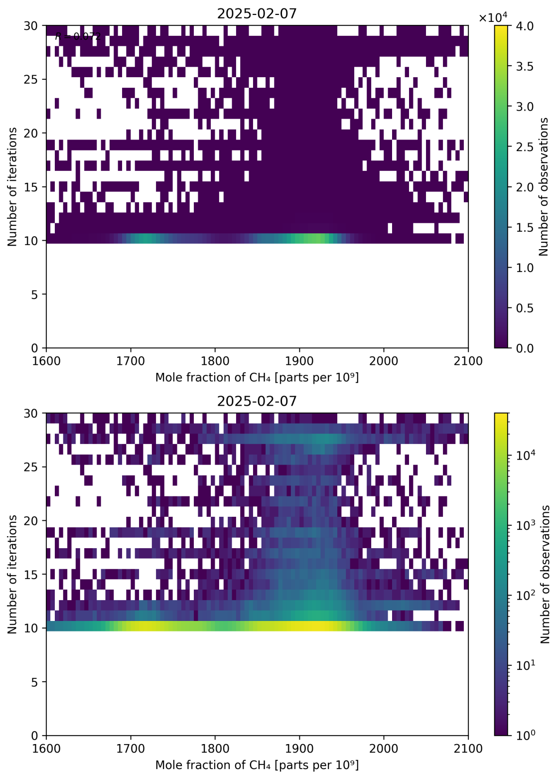
Figure 76: Scatter density plot of “Mole fraction of CH 4 ” against “Number of iterations” for 2025-02-06 to 2025-02-08.
