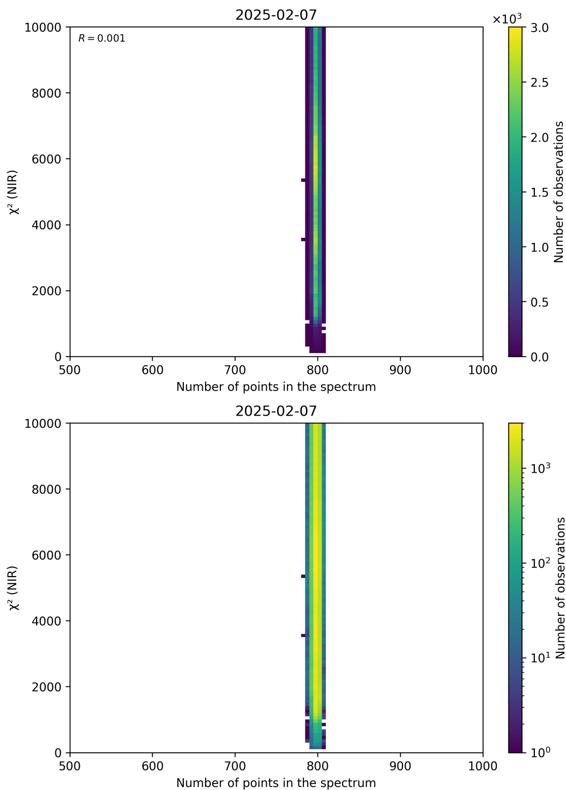
Figure 88: Scatter density plot of “Number of points in the spectrum” against “ \chi^2 (NIR)” for 2025-02-06 to 2025-02-08.
