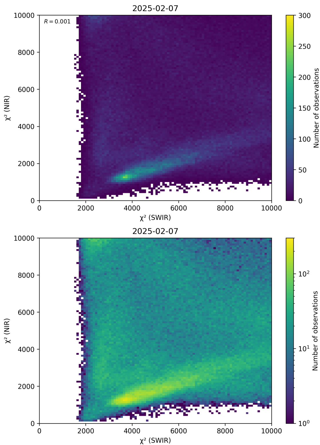
Figure 47: Scatter density plot of “ \chi^2 (SWIR)” against “ \chi^2 (NIR)” for 2025-02-06 to 2025-02-08.
