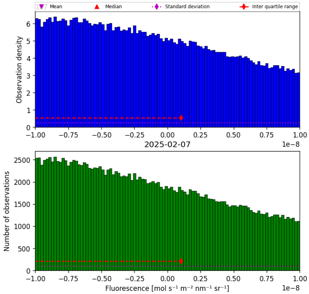
Figure 32: Histogram of “Fluorescence” for 2025-02-06 to 2025-02-08
