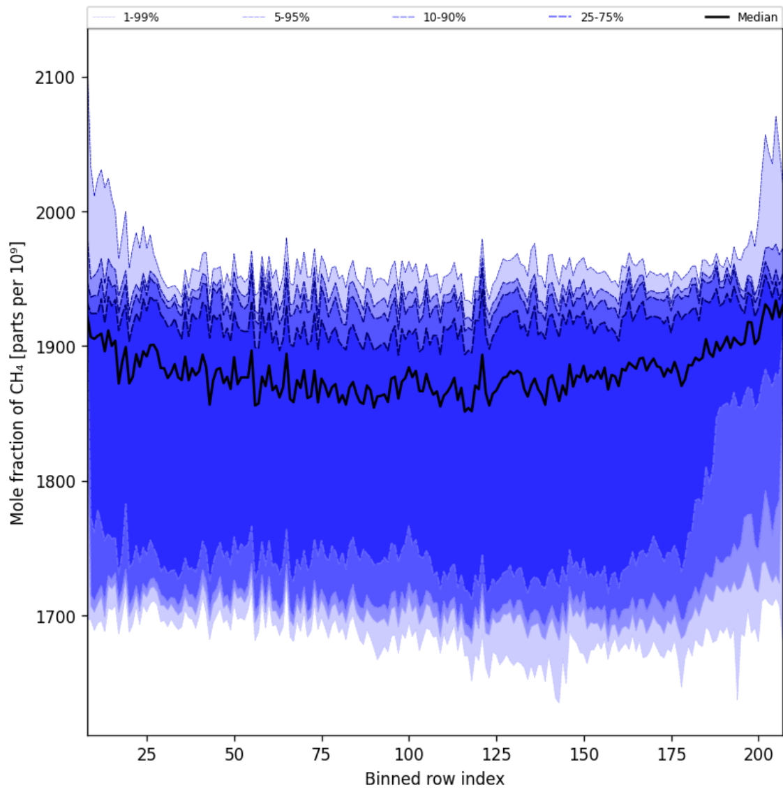
Figure 34: Along track statistics of “Mole fraction of CH 4 ” for 2025-02-06 to 2025-02-08
