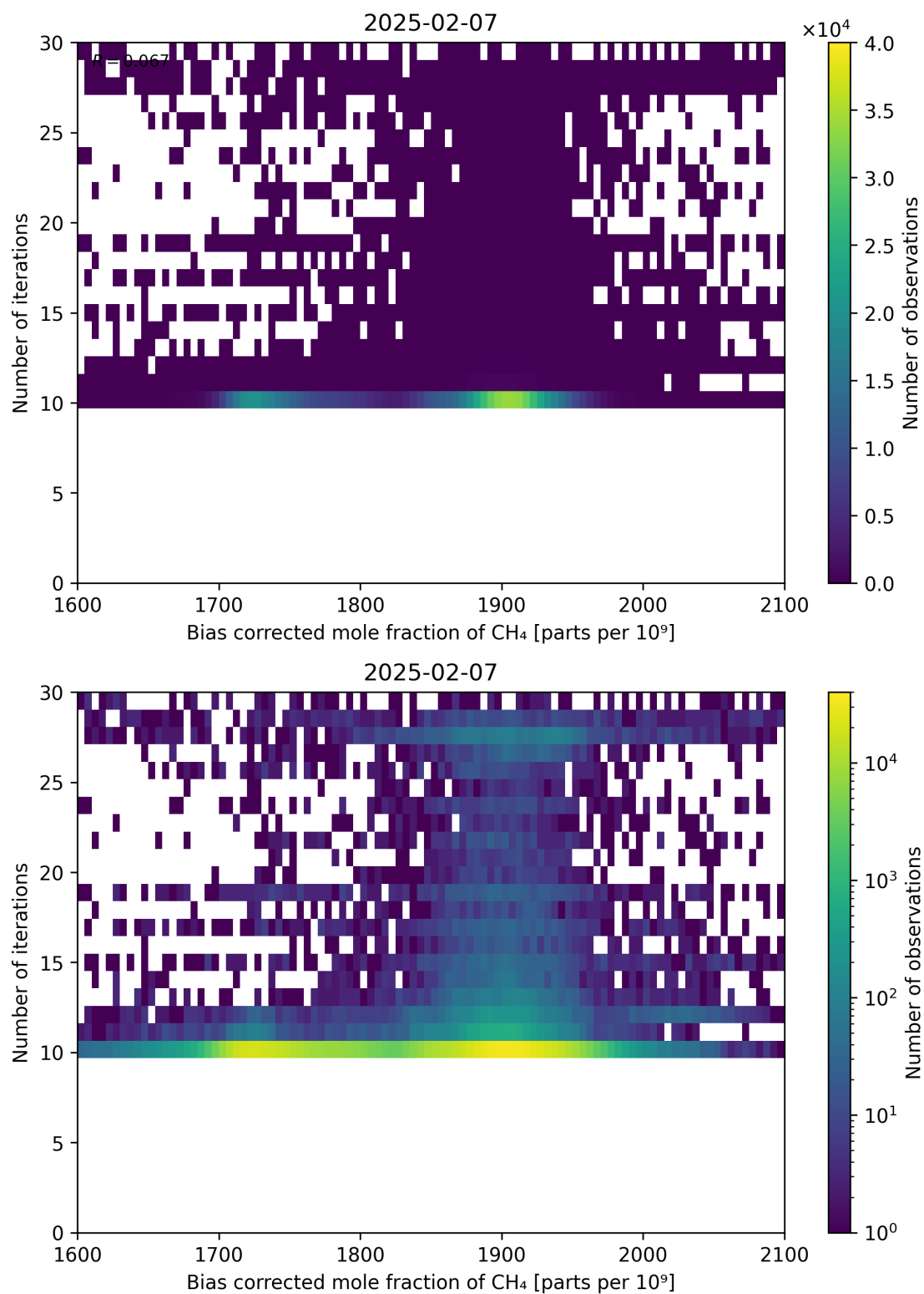
Figure 67: Scatter density plot of “Bias corrected mole fraction of CH 4 ” against “Number of iterations” for 2025-02-06 to 2025-02-08.
