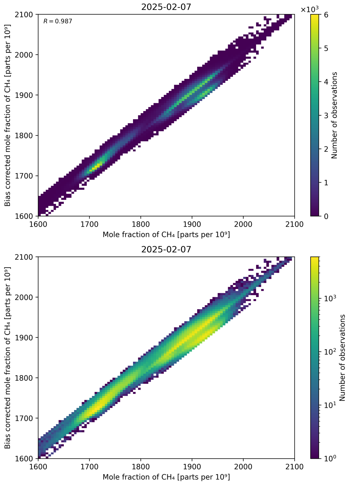
Figure 74: Scatter density plot of “Mole fraction of CH 4 ” against “Bias corrected mole fraction of CH 4 ” for 2025-02-06 to 2025-02-08.
