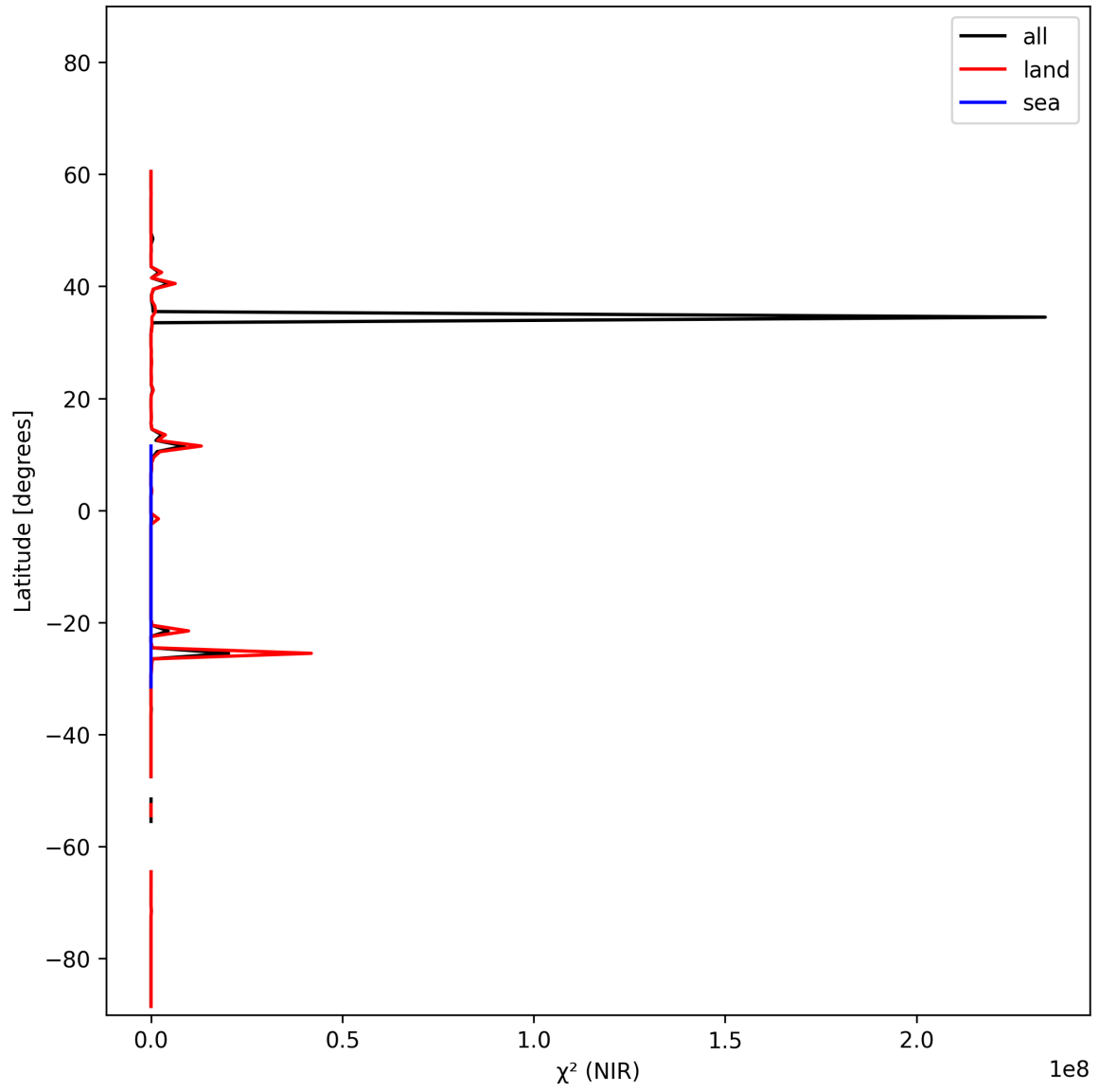
Figure 18: Zonal average of “ \chi^2 (NIR)” for 2025-02-06 to 2025-02-08.
