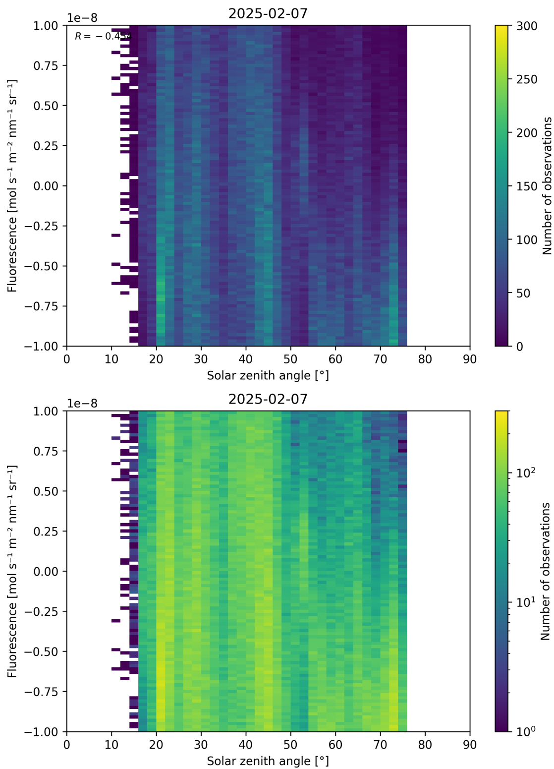
Figure 97: Scatter density plot of “Solar zenith angle” against “Fluorescence” for 2025-02-06 to 2025-02-08.
