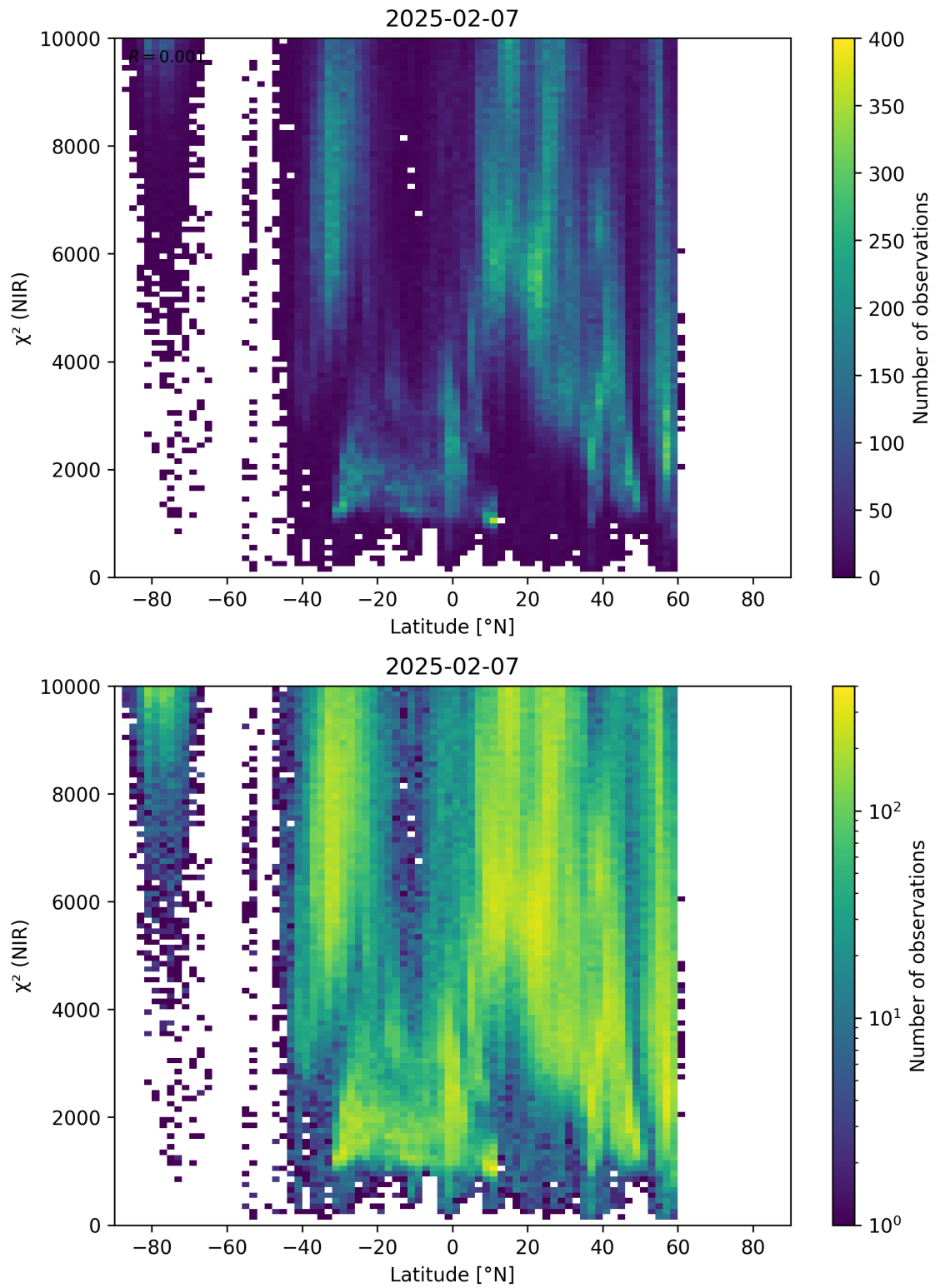
Figure 53: Scatter density plot of “Latitude” against “ \chi^2 (NIR)” for 2025-02-06 to 2025-02-08.
