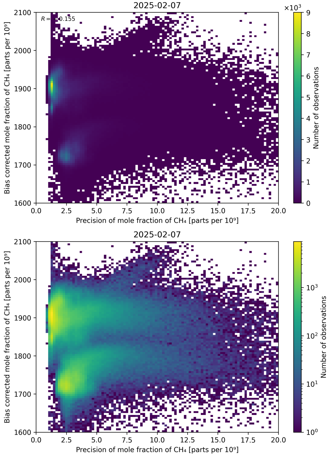
Figure 82: Scatter density plot of “Precision of mole fraction of CH 4 ” against “Bias corrected mole fraction of CH 4 ” for 2025-02-06 to 2025-02-08.
