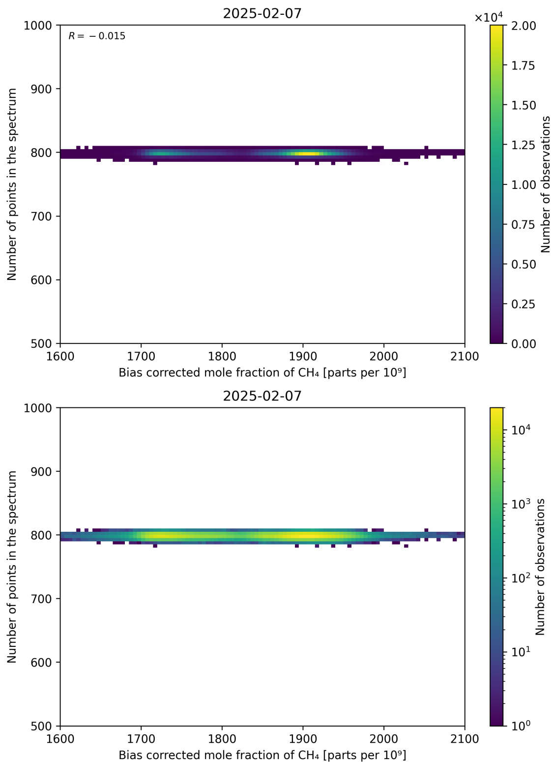
Figure 68: Scatter density plot of “Bias corrected mole fraction of CH 4 ” against “Number of points in the spectrum” for 2025-02-06 to 2025-02-08.
