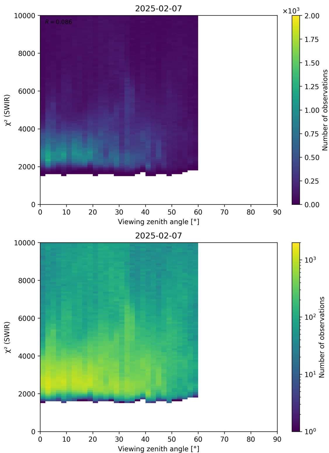
Figure 106: Scatter density plot of “Viewing zenith angle” against “ \chi^2 (SWIR)” for 2025-02-06 to 2025-02-08.
