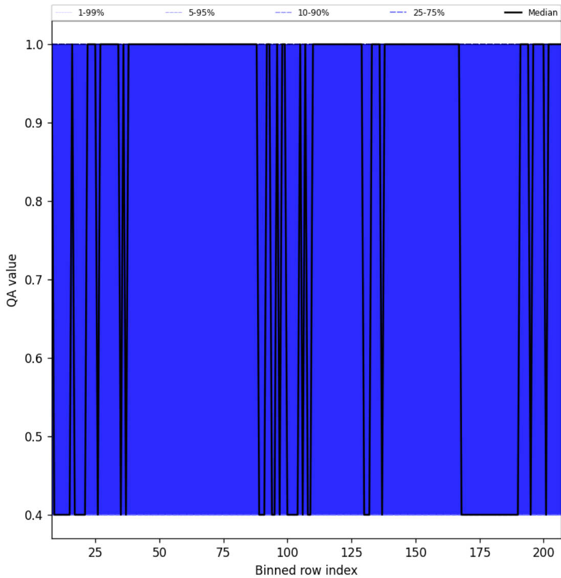
Figure 33: Along track statistics of “QA value” for 2025-02-06 to 2025-02-08
