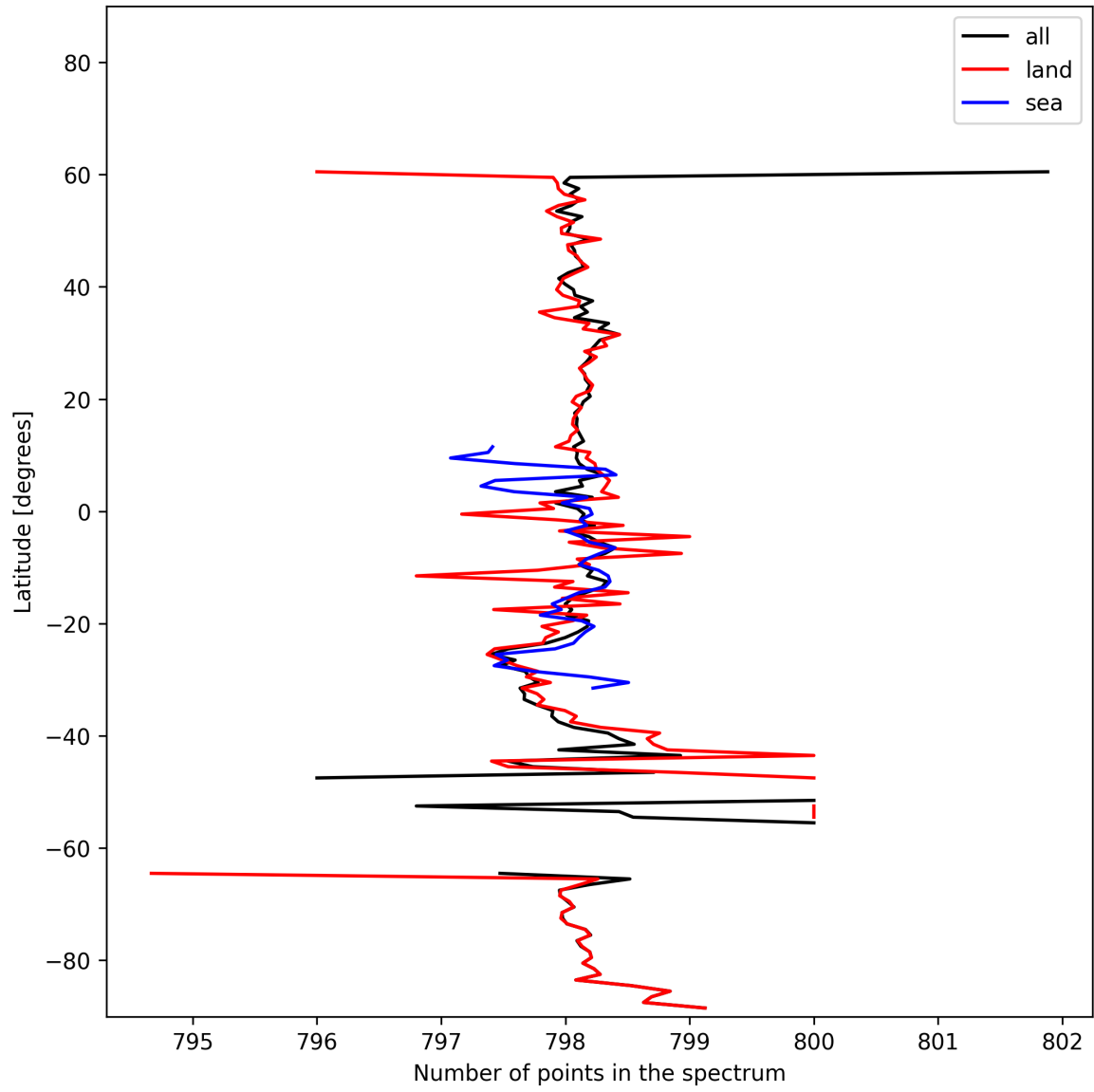
Figure 15: Zonal average of “Number of points in the spectrum” for 2025-02-06 to 2025-02-08.
