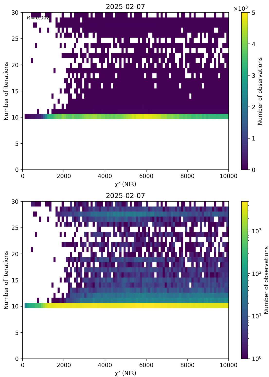
Figure 46: Scatter density plot of “ \chi^2 (NIR)” against “Number of iterations” for 2025-02-06 to 2025-02-08.
