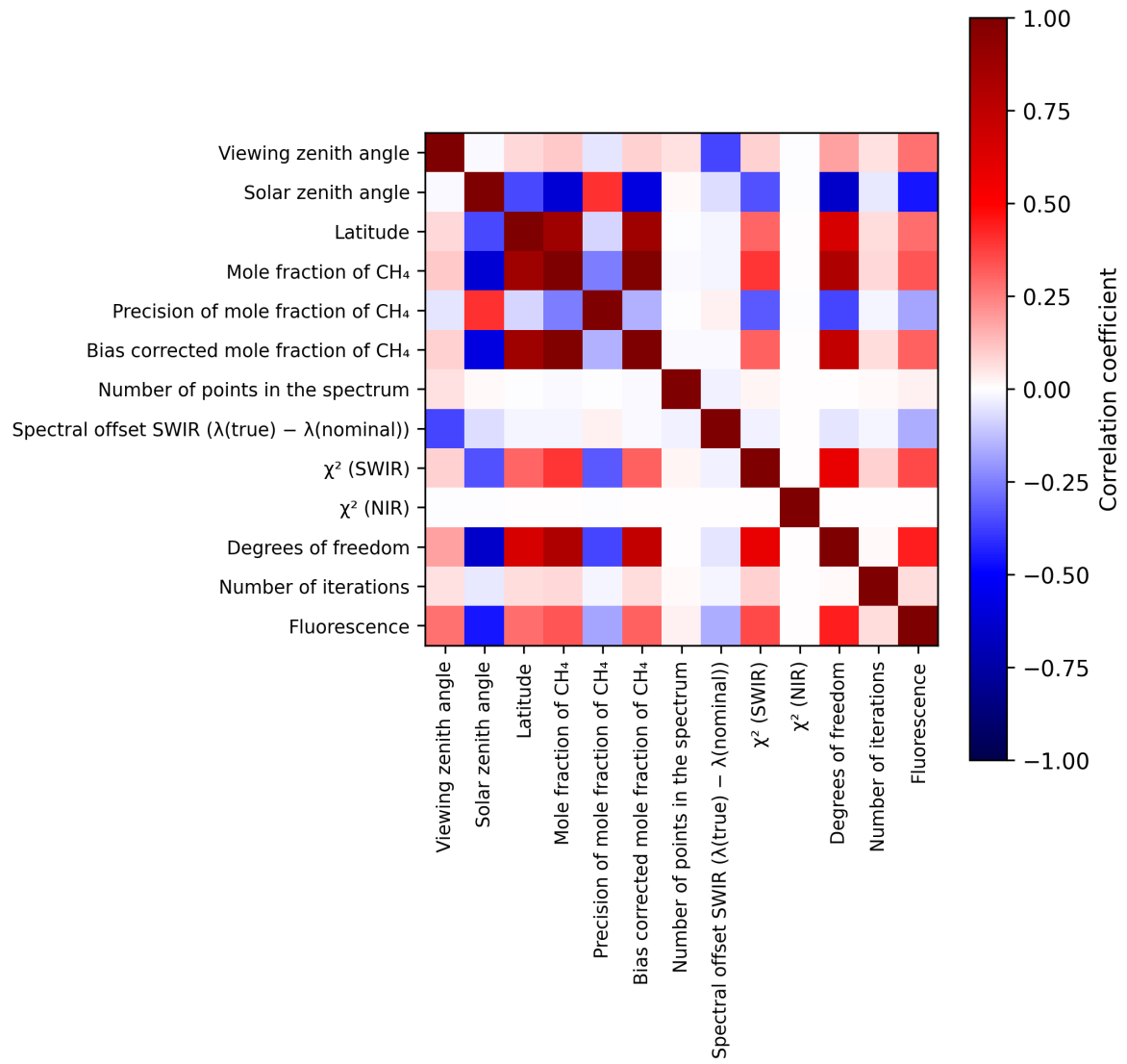
Figure 2: Map of correlation matrix for 2025-02-06 to 2025-02-08.
