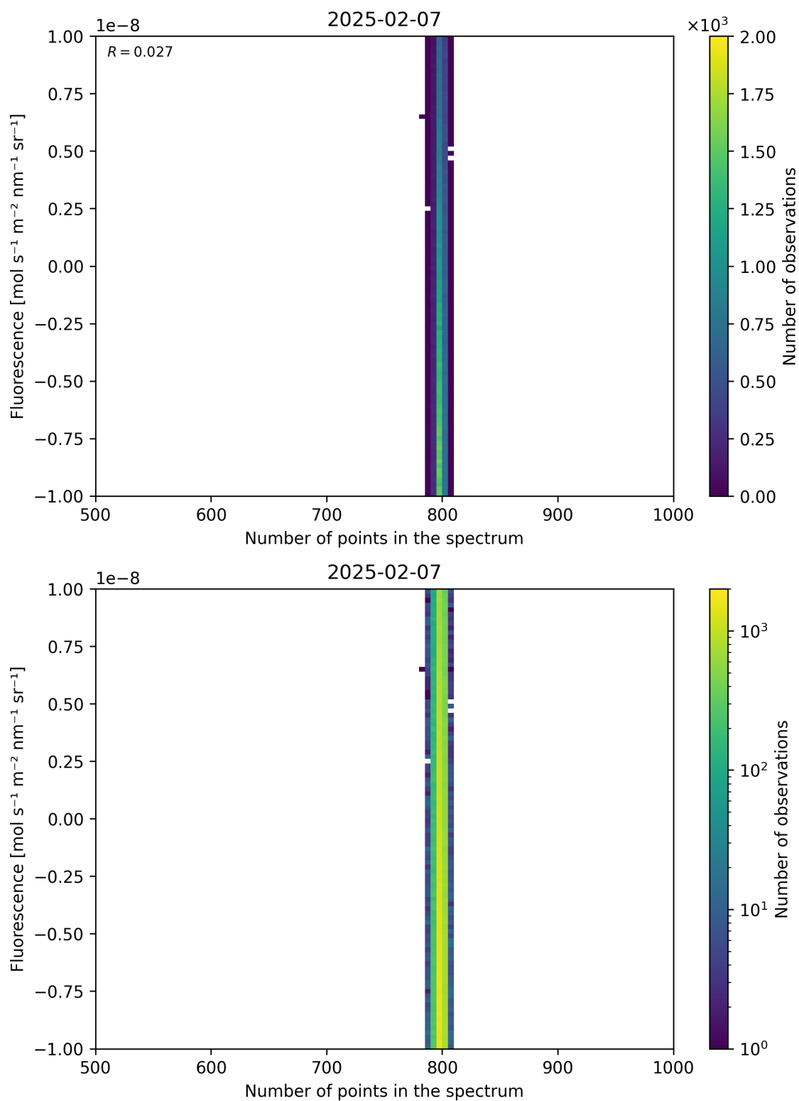
Figure 91: Scatter density plot of “Number of points in the spectrum” against “Fluorescence” for 2025-02-06 to 2025-02-08.
