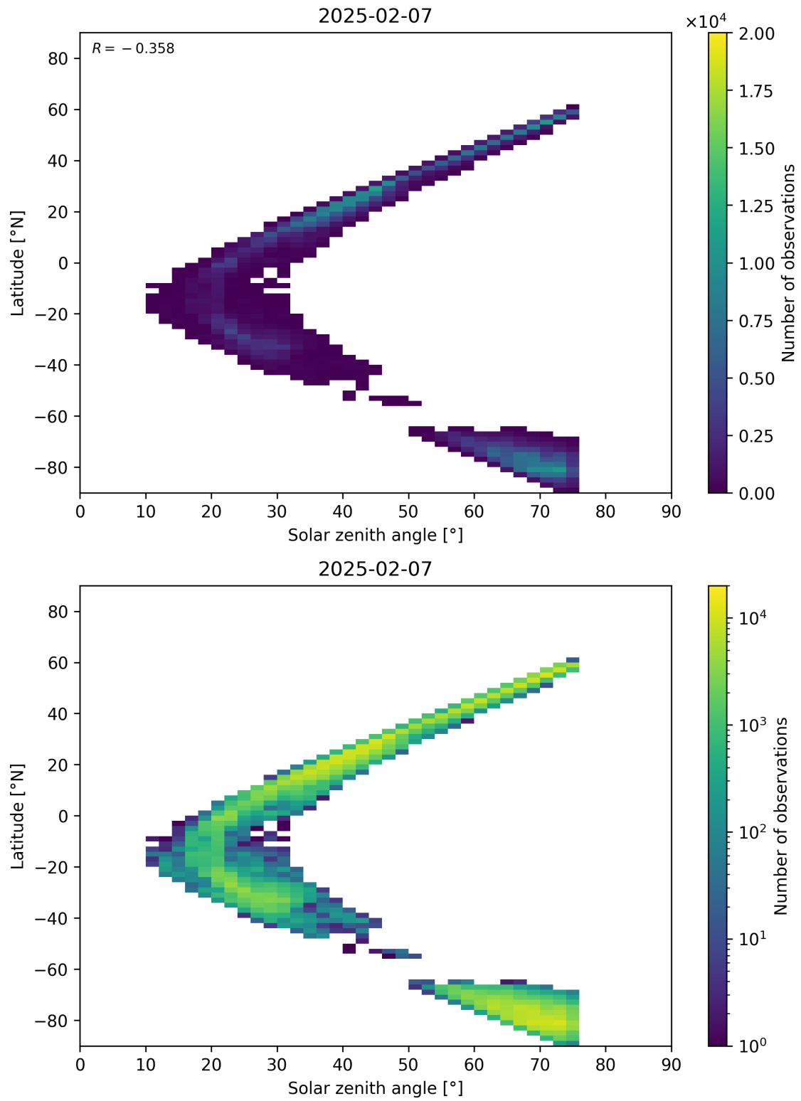
Figure 98: Scatter density plot of “Solar zenith angle” against “Latitude” for 2025-02-06 to 2025-02-08.
