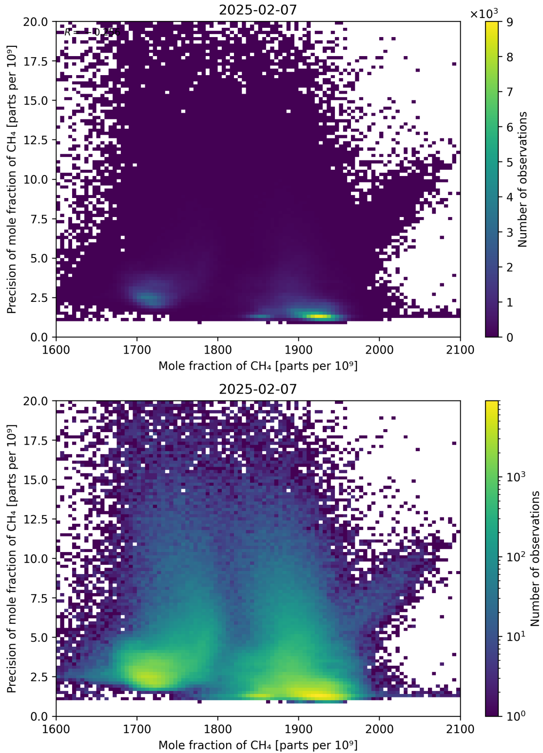
Figure 75: Scatter density plot of “Mole fraction of CH 4 ” against “Precision of mole fraction of CH 4 ” for 2025-02-06 to 2025-02-08.
