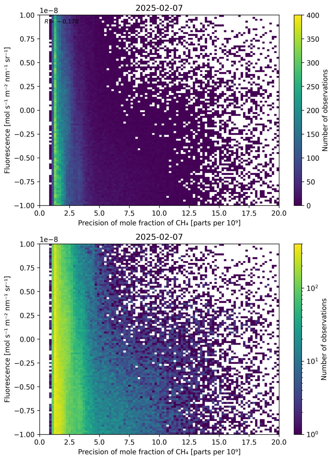
Figure 81: Scatter density plot of “Precision of mole fraction of CH 4 ” against “Fluorescence” for 2025-02-06 to 2025-02-08.
