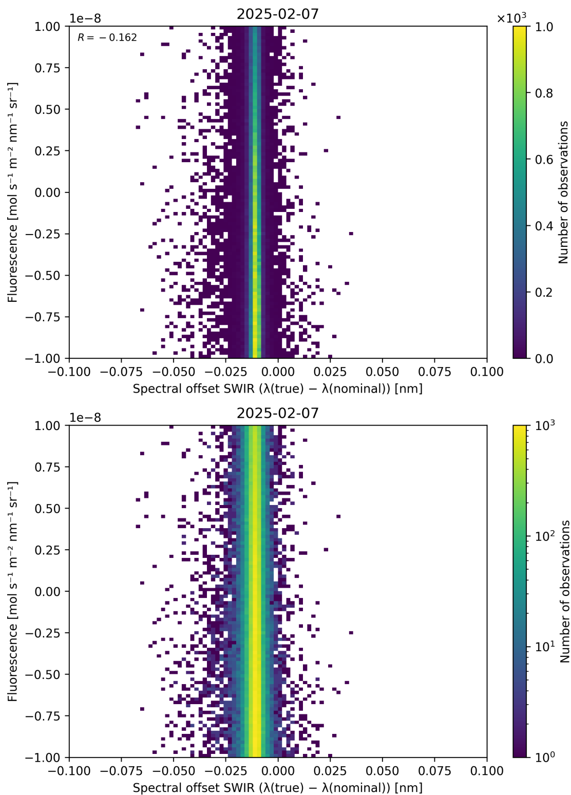
Figure 120: Scatter density plot of “Spectral offset SWIR ( \lambda_{\text{true}} - \lambda_{\text{nominal}} )” against “Fluorescence” for 2025-02-06 to 2025-02-08.
