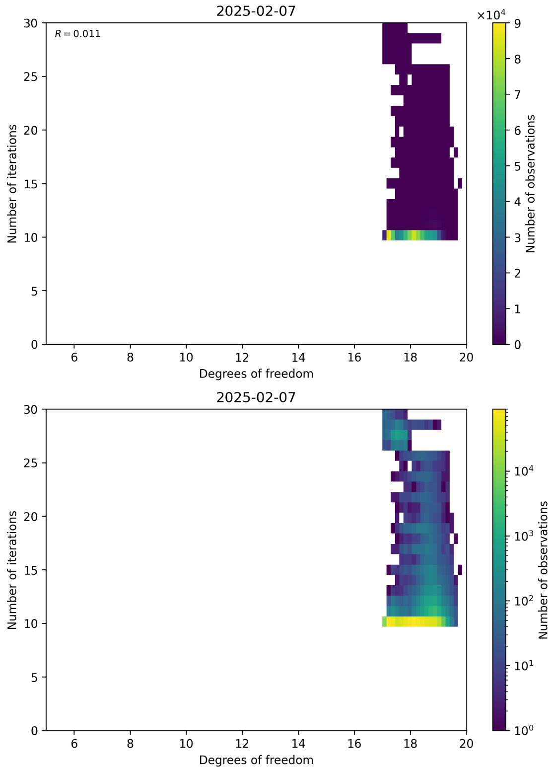
Figure 52: Scatter density plot of “Degrees of freedom” against “Number of iterations” for 2025-02-06 to 2025-02-08.
