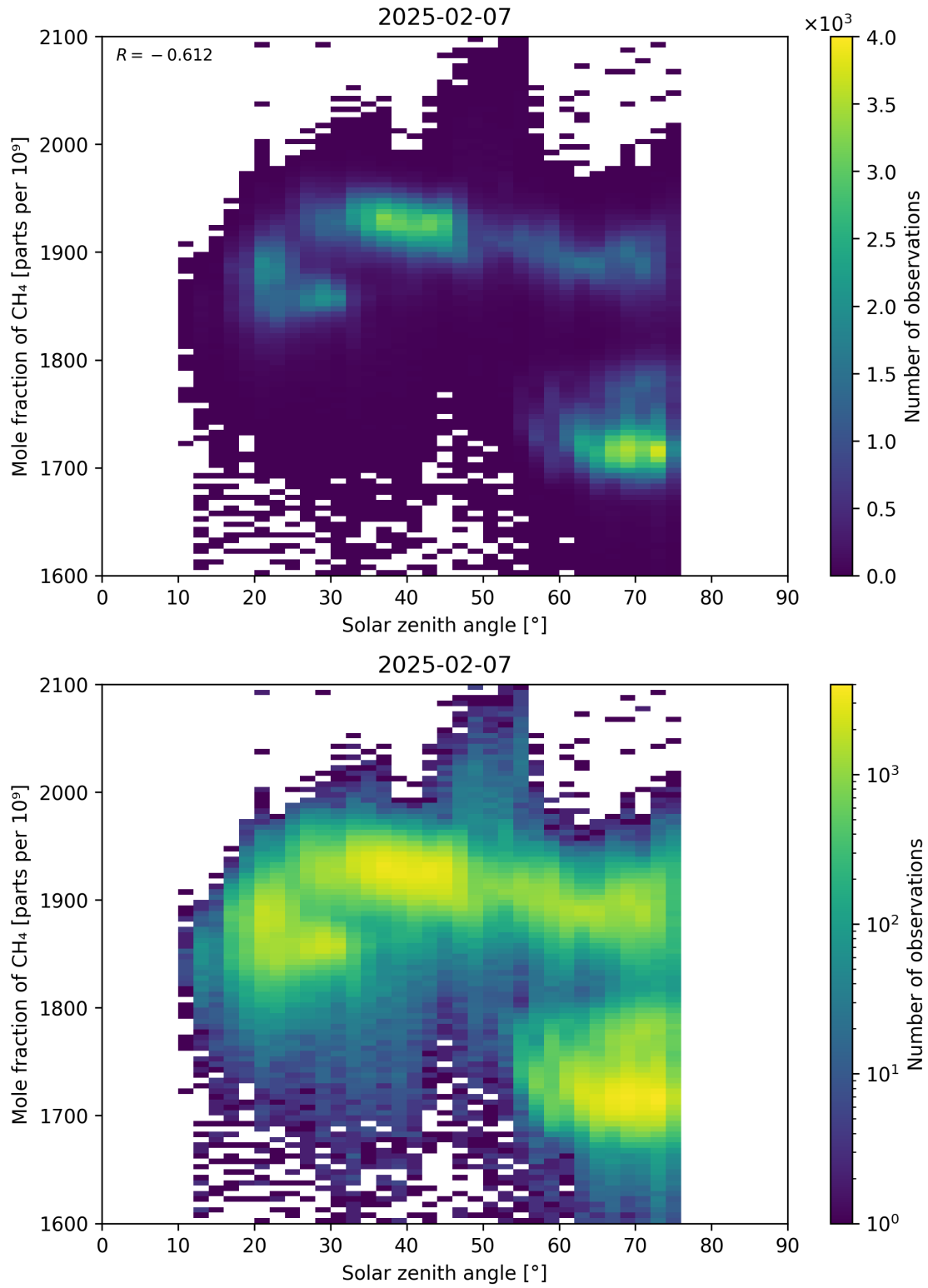
Figure 99: Scatter density plot of “Solar zenith angle” against “Mole fraction of CH 4 ” for 2025-02-06 to 2025-02-08.
