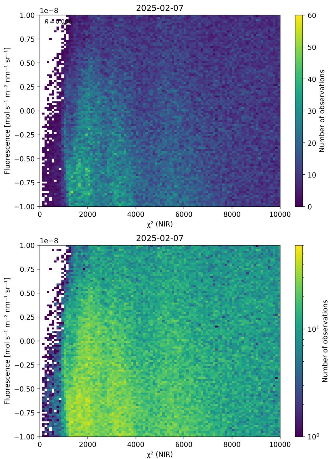
Figure 45: Scatter density plot of “ \chi^2 (NIR)” against “Fluorescence” for 2025-02-06 to 2025-02-08.
