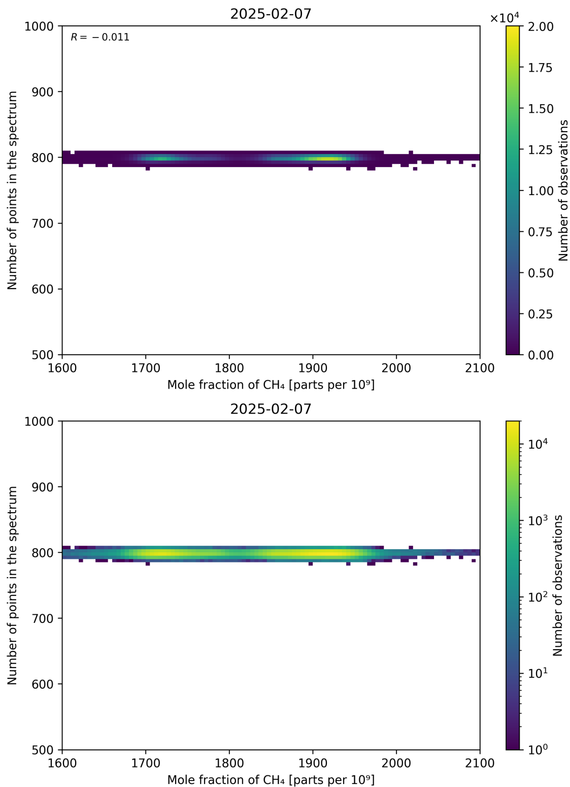
Figure 77: Scatter density plot of “Mole fraction of CH 4 ” against “Number of points in the spectrum” for 2025-02-06 to 2025-02-08.
