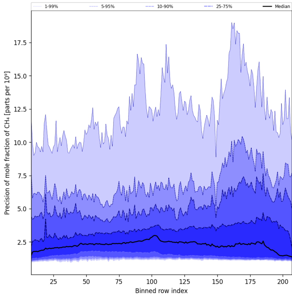
Figure 35: Along track statistics of “Precision of mole fraction of CH 4 ” for 2025-02-06 to 2025-02-08
