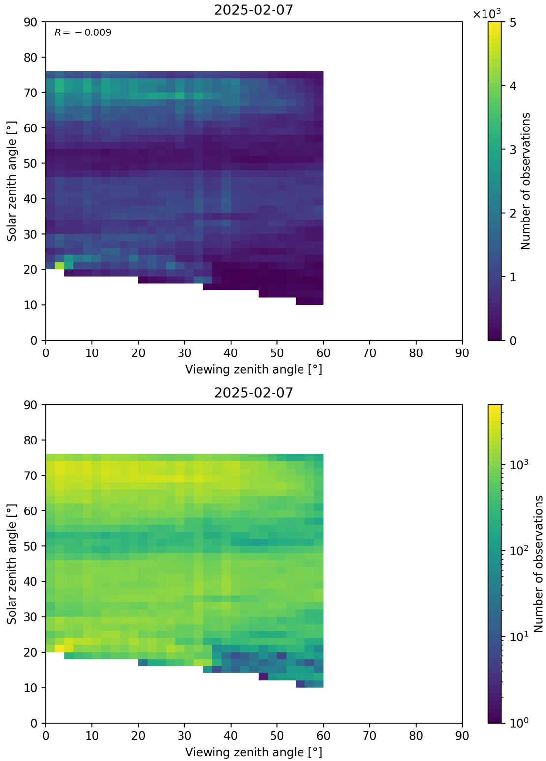
Figure 115: Scatter density plot of “Viewing zenith angle” against “Solar zenith angle” for 2025-02-06 to 2025-02-08.
