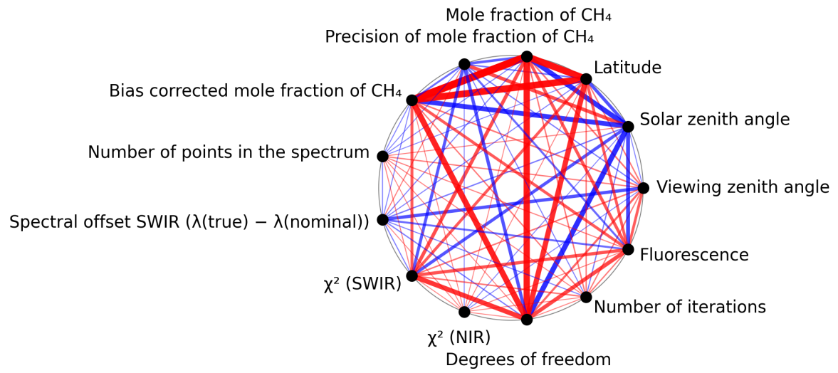
Figure 1: Map of correlation graph for 2025-02-06 to 2025-02-08.
