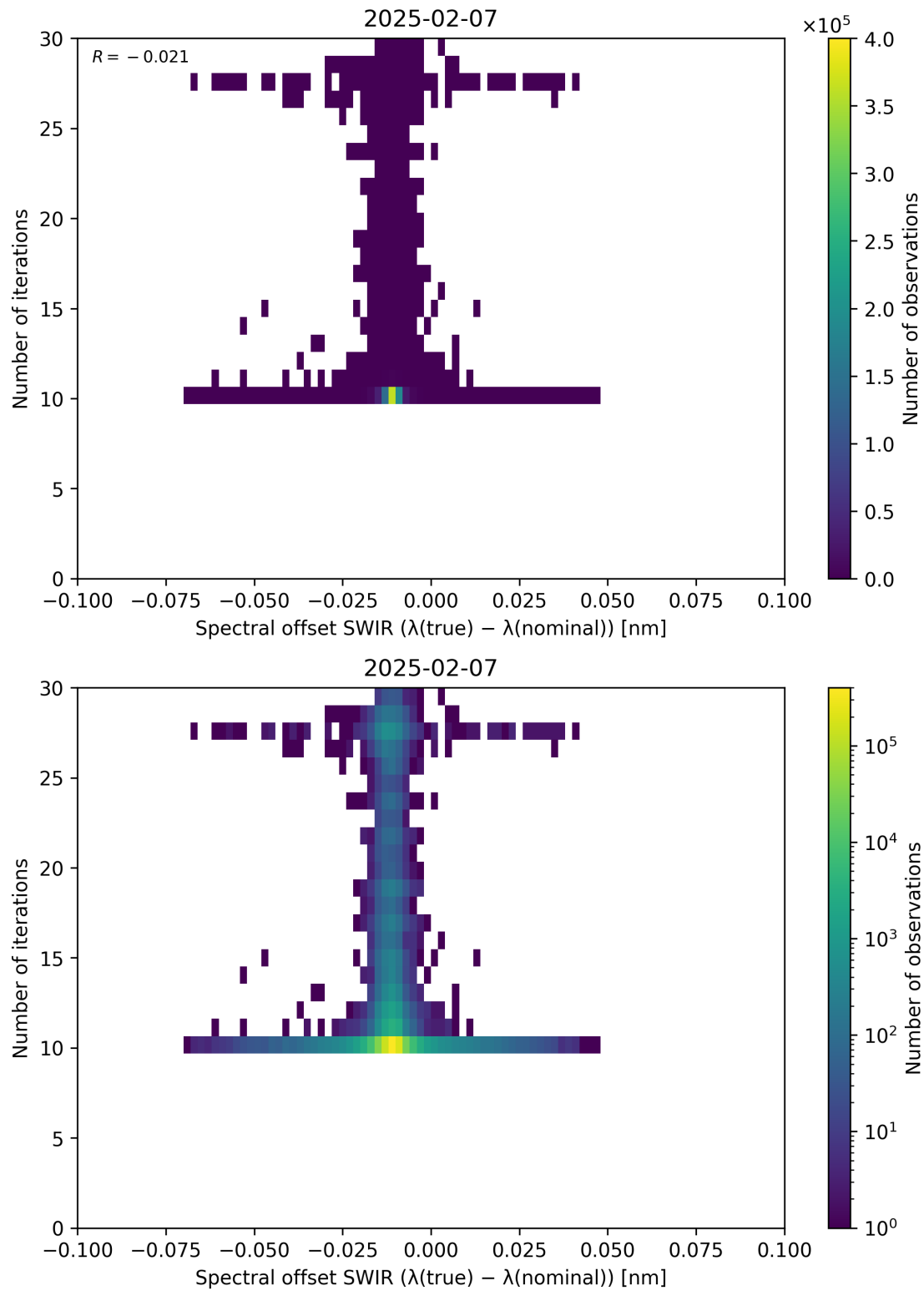
Figure 121: Scatter density plot of “Spectral offset SWIR ( \lambda_{\text{true}} - \lambda_{\text{nominal}} )” against “Number of iterations” for 2025-02-06 to 2025-02-08.
