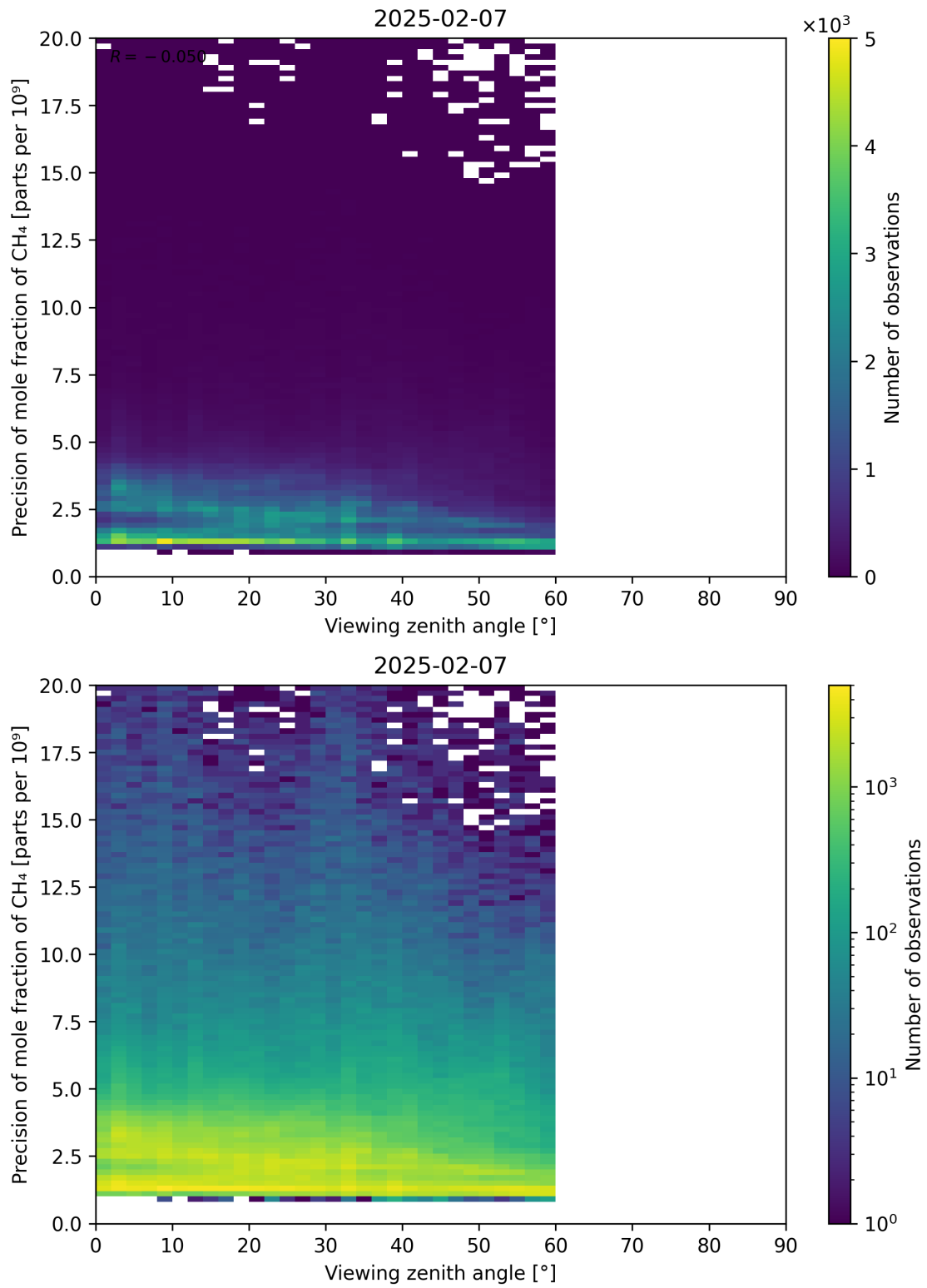
Figure 112: Scatter density plot of “Viewing zenith angle” against “Precision of mole fraction of CH 4 ” for 2025-02-06 to 2025-02-08.
