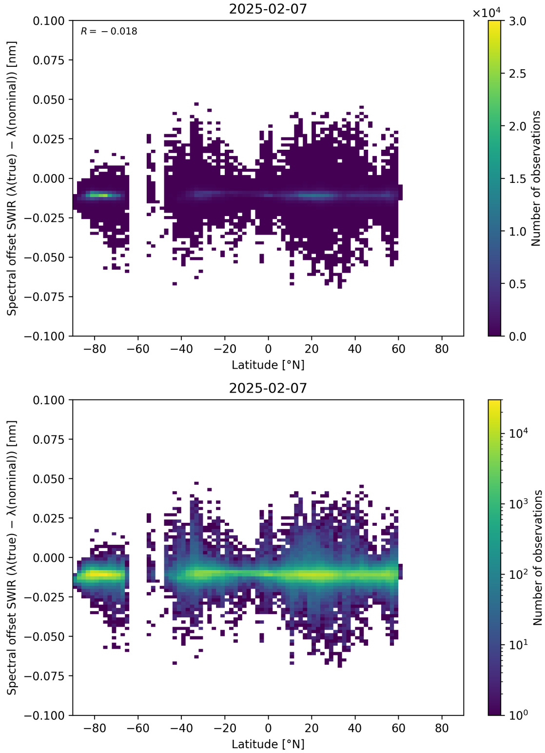
Figure 62: Scatter density plot of “Latitude” against “Spectral offset SWIR ( \lambda_{\text{true}} - \lambda_{\text{nominal}} )” for 2025-02-06 to 2025-02-08.
