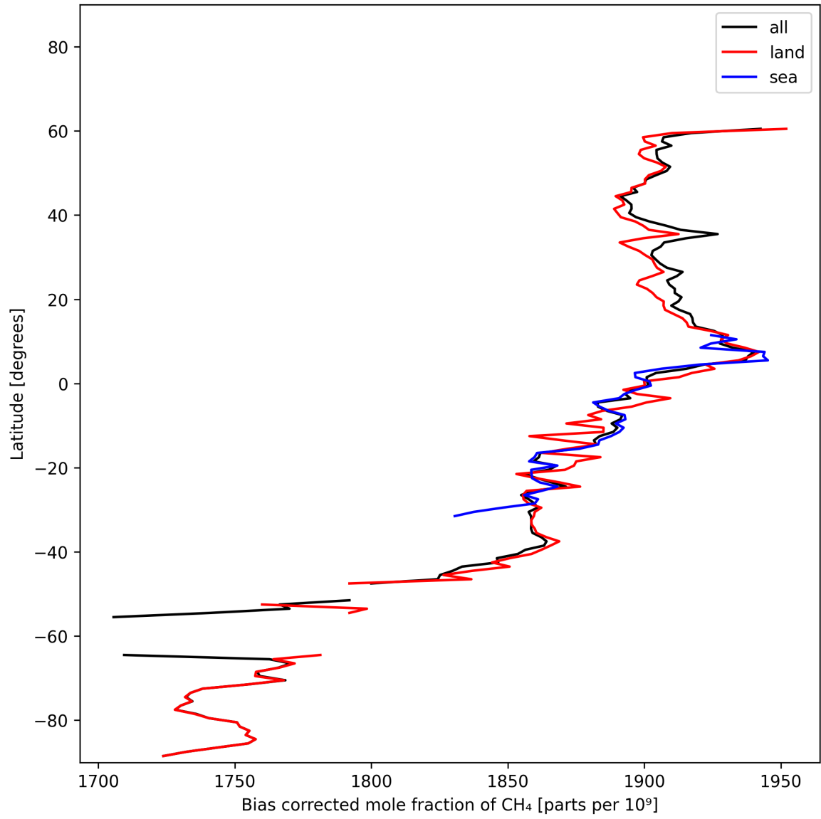
Figure 14: Zonal average of “Bias corrected mole fraction of CH 4 ” for 2025-02-06 to 2025-02-08.
