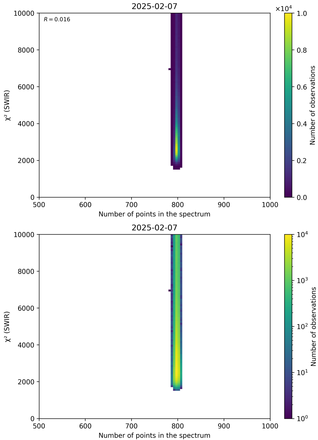
Figure 89: Scatter density plot of “Number of points in the spectrum” against “ \chi^2 (SWIR)” for 2025-02-06 to 2025-02-08.
