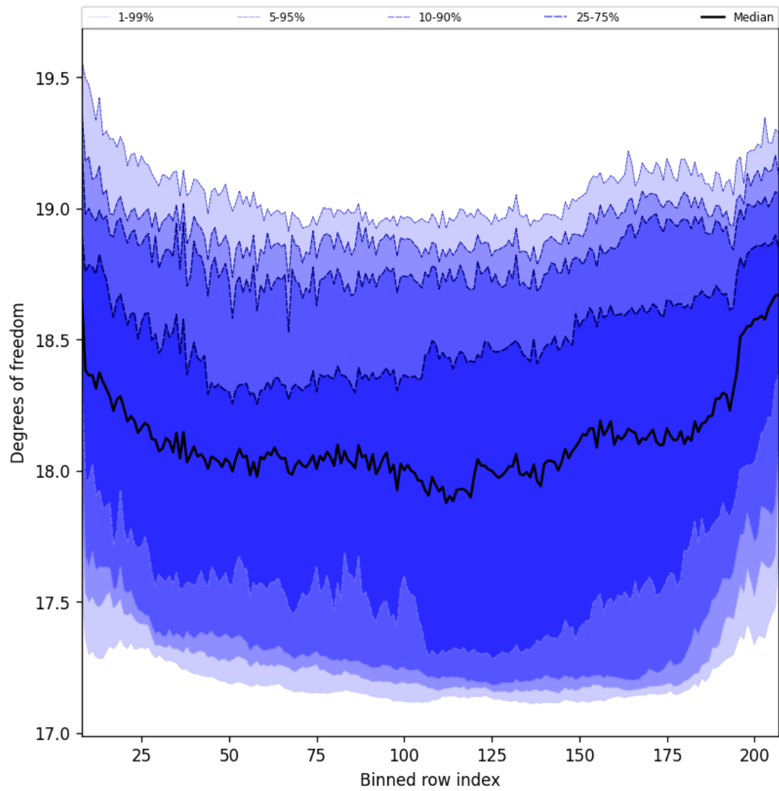
Figure 41: Along track statistics of “Degrees of freedom” for 2025-02-06 to 2025-02-08
