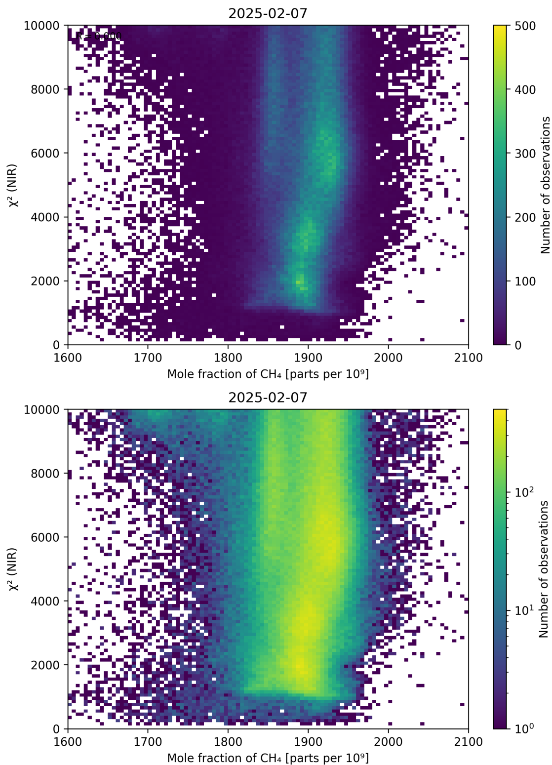
Figure 70: Scatter density plot of “Mole fraction of CH 4 ” against “ \chi^2 (NIR)” for 2025-02-06 to 2025-02-08.
