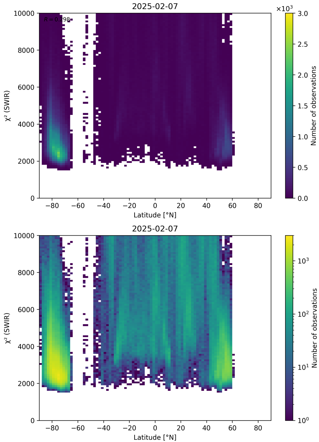
Figure 54: Scatter density plot of “Latitude” against “ \chi^2 (SWIR)” for 2025-02-06 to 2025-02-08.
