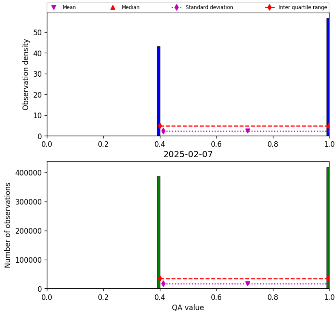
Figure 22: Histogram of “QA value” for 2025-02-06 to 2025-02-08
