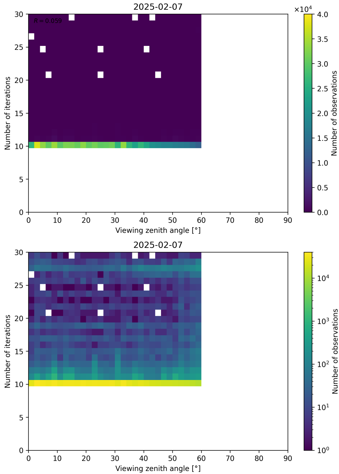
Figure 113: Scatter density plot of “Viewing zenith angle” against “Number of iterations” for 2025-02-06 to 2025-02-08.
