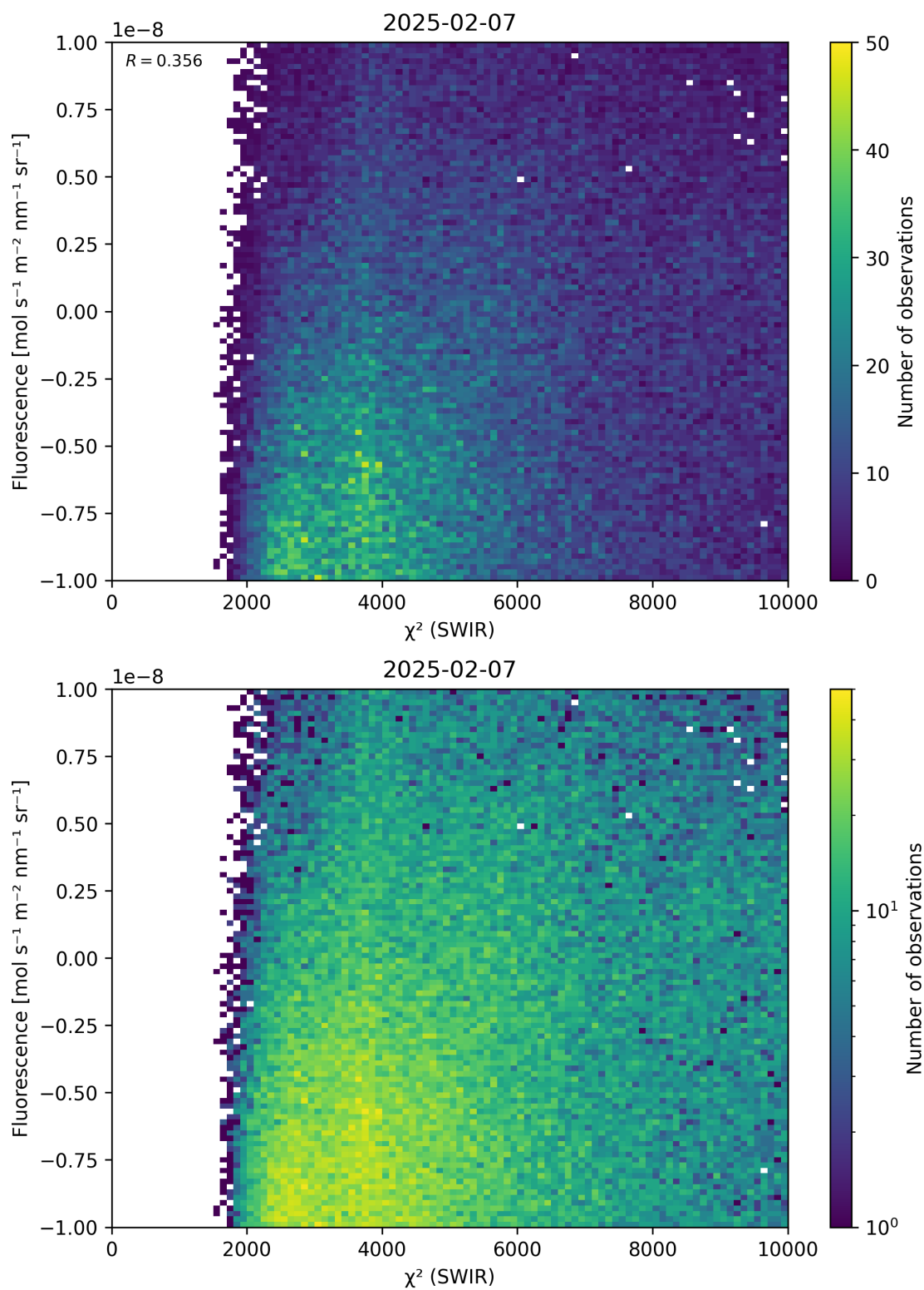
Figure 49: Scatter density plot of “ \chi^2 (SWIR)” against “Fluorescence” for 2025-02-06 to 2025-02-08.
