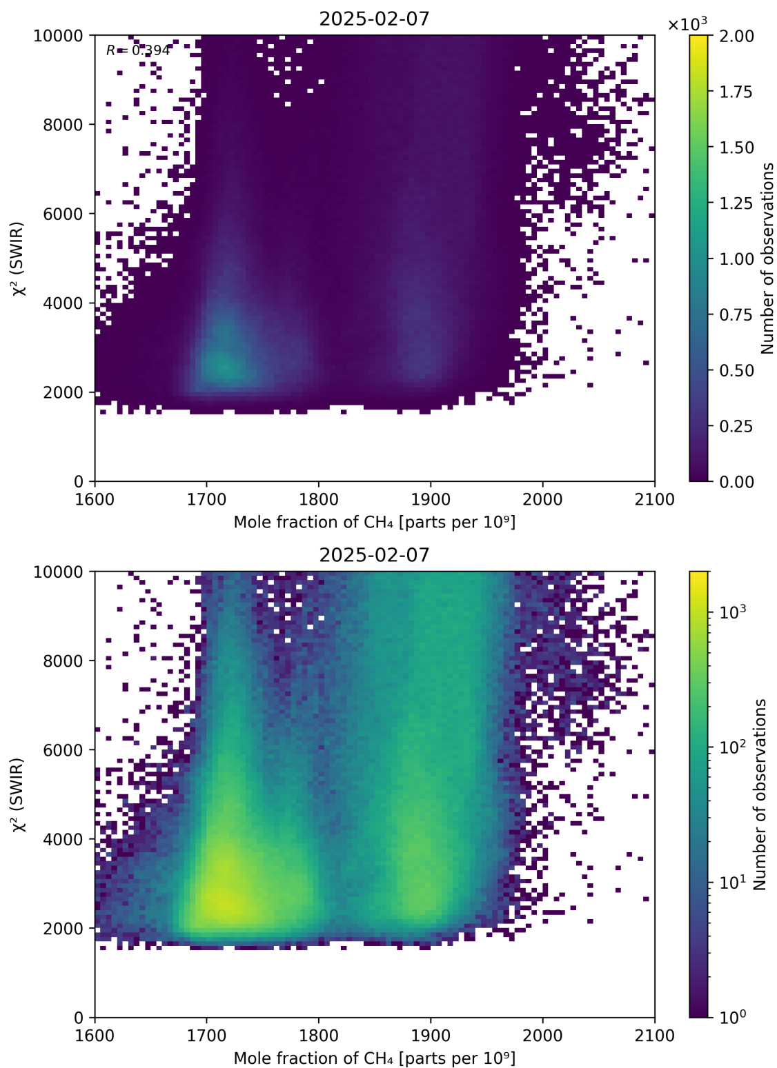
Figure 71: Scatter density plot of “Mole fraction of \text{CH}_4 ” against “ \chi^2 (SWIR)” for 2025-02-06 to 2025-02-08.
