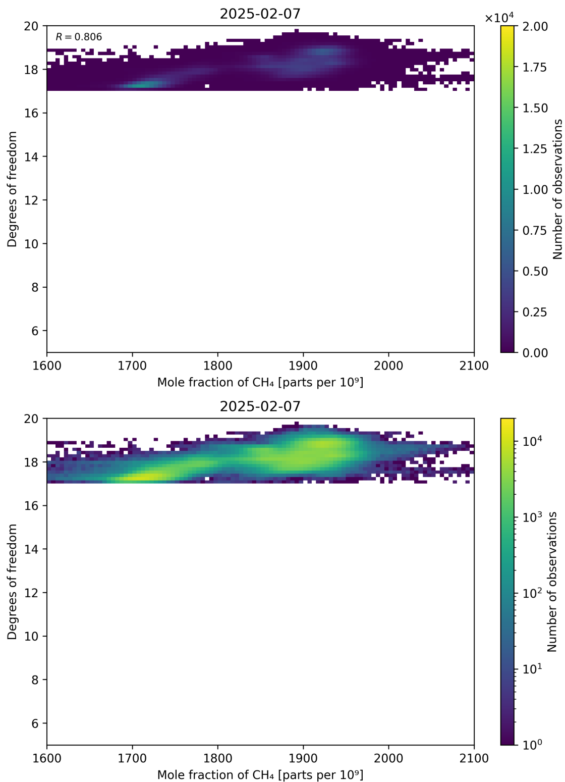
Figure 72: Scatter density plot of “Mole fraction of CH 4 ” against “Degrees of freedom” for 2025-02-06 to 2025-02-08.
