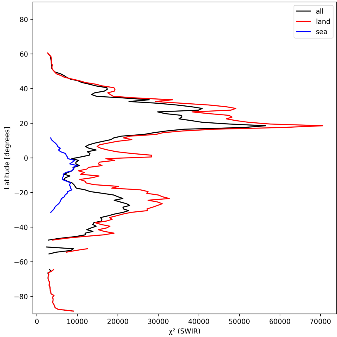
Figure 17: Zonal average of “ \chi^2 (SWIR)” for 2025-02-06 to 2025-02-08.
