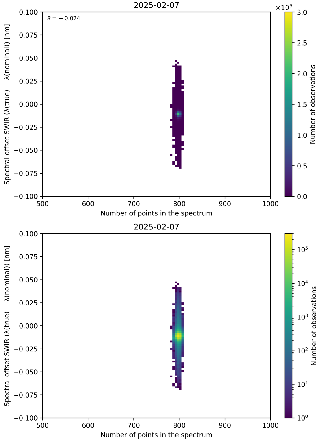
Figure 93: Scatter density plot of “Number of points in the spectrum” against “Spectral offset SWIR ( \lambda_{\text{true}} - \lambda_{\text{nominal}} )” for 2025-02-06 to 2025-02-08.
