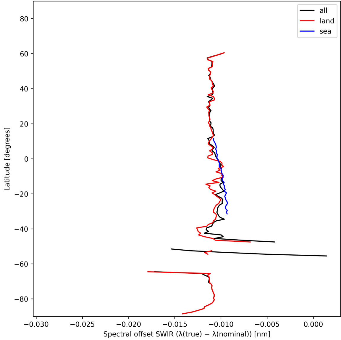
Figure 16: Zonal average of “Spectral offset SWIR ( \lambda_{\text{true}} - \lambda_{\text{nominal}} )” for 2025-02-06 to 2025-02-08.
