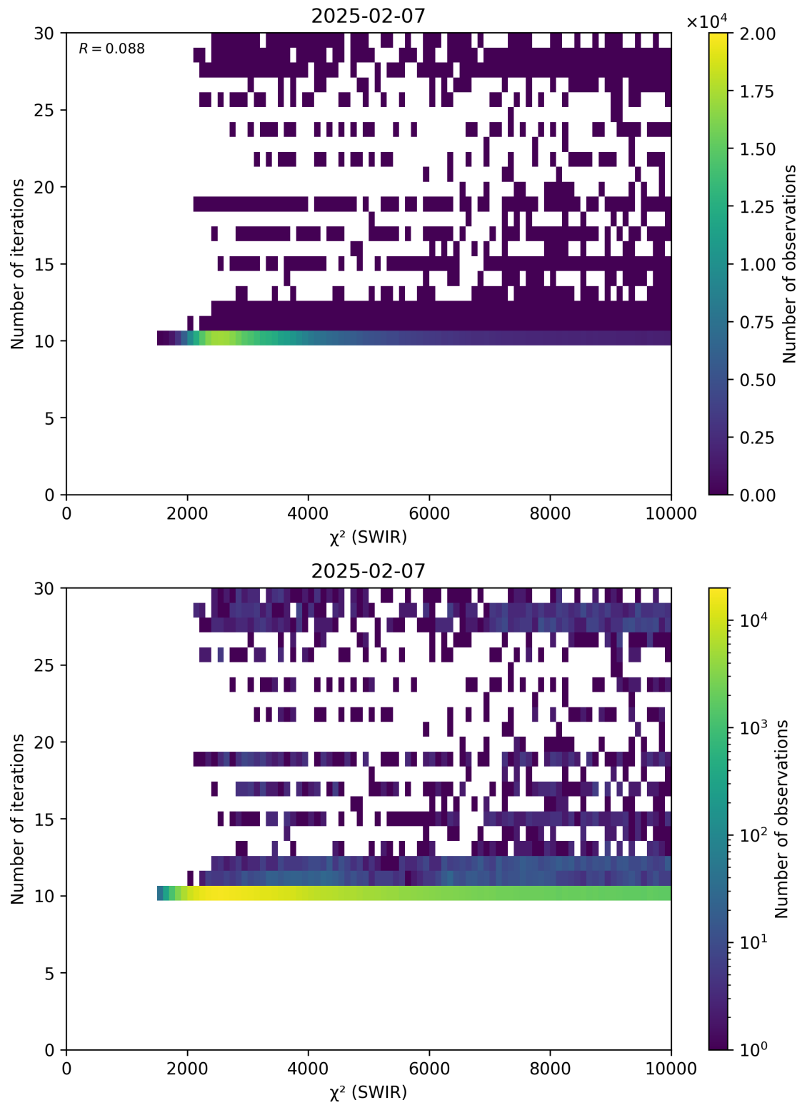
Figure 50: Scatter density plot of “ \chi^2 (SWIR)” against “Number of iterations” for 2025-02-06 to 2025-02-08.
