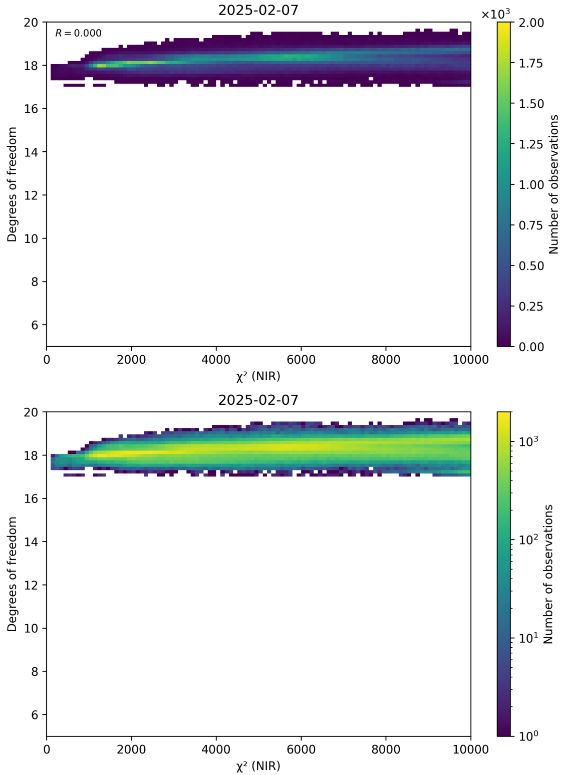
Figure 44: Scatter density plot of “ \chi^2 (NIR)” against “Degrees of freedom” for 2025-02-06 to 2025-02-08.
