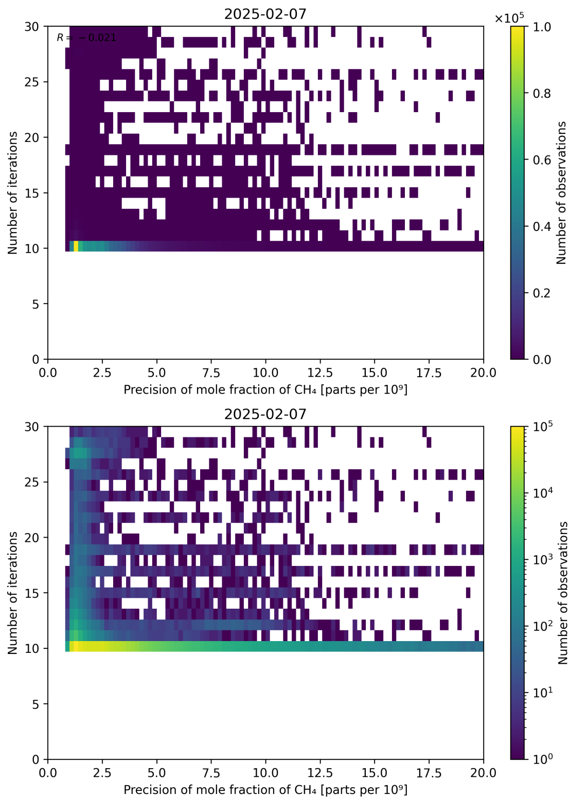
Figure 83: Scatter density plot of “Precision of mole fraction of CH 4 ” against “Number of iterations” for 2025-02-06 to 2025-02-08.
