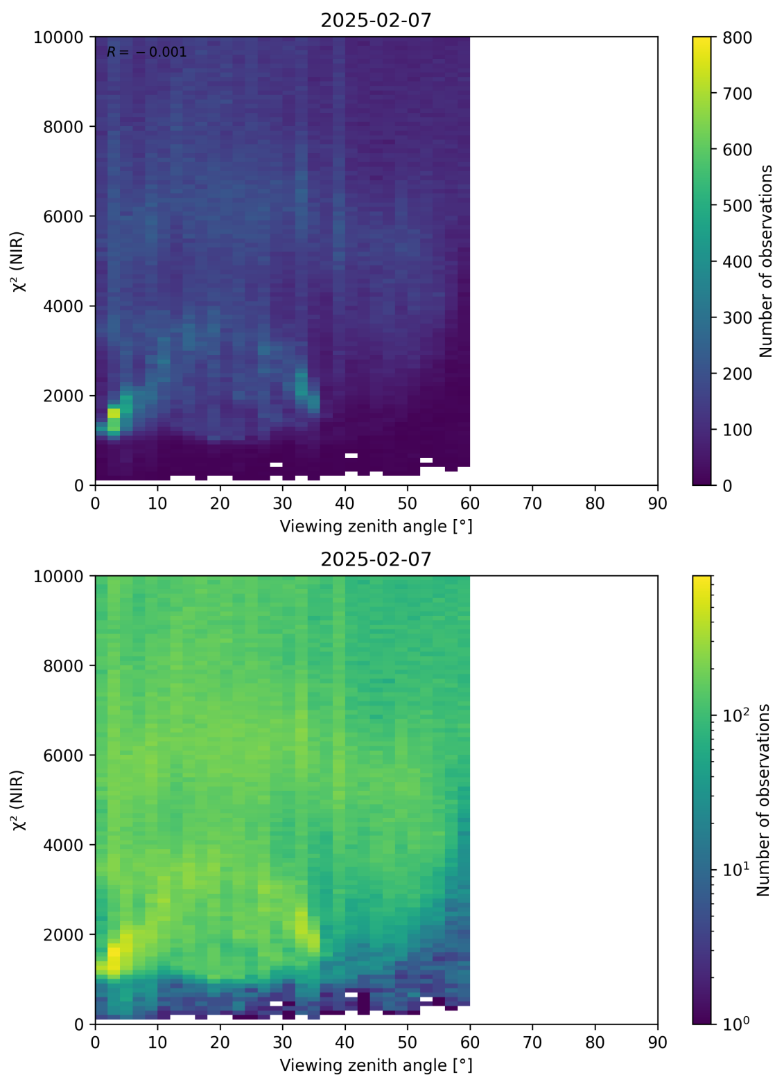
Figure 105: Scatter density plot of “Viewing zenith angle” against “ \chi^2 (NIR)” for 2025-02-06 to 2025-02-08.
