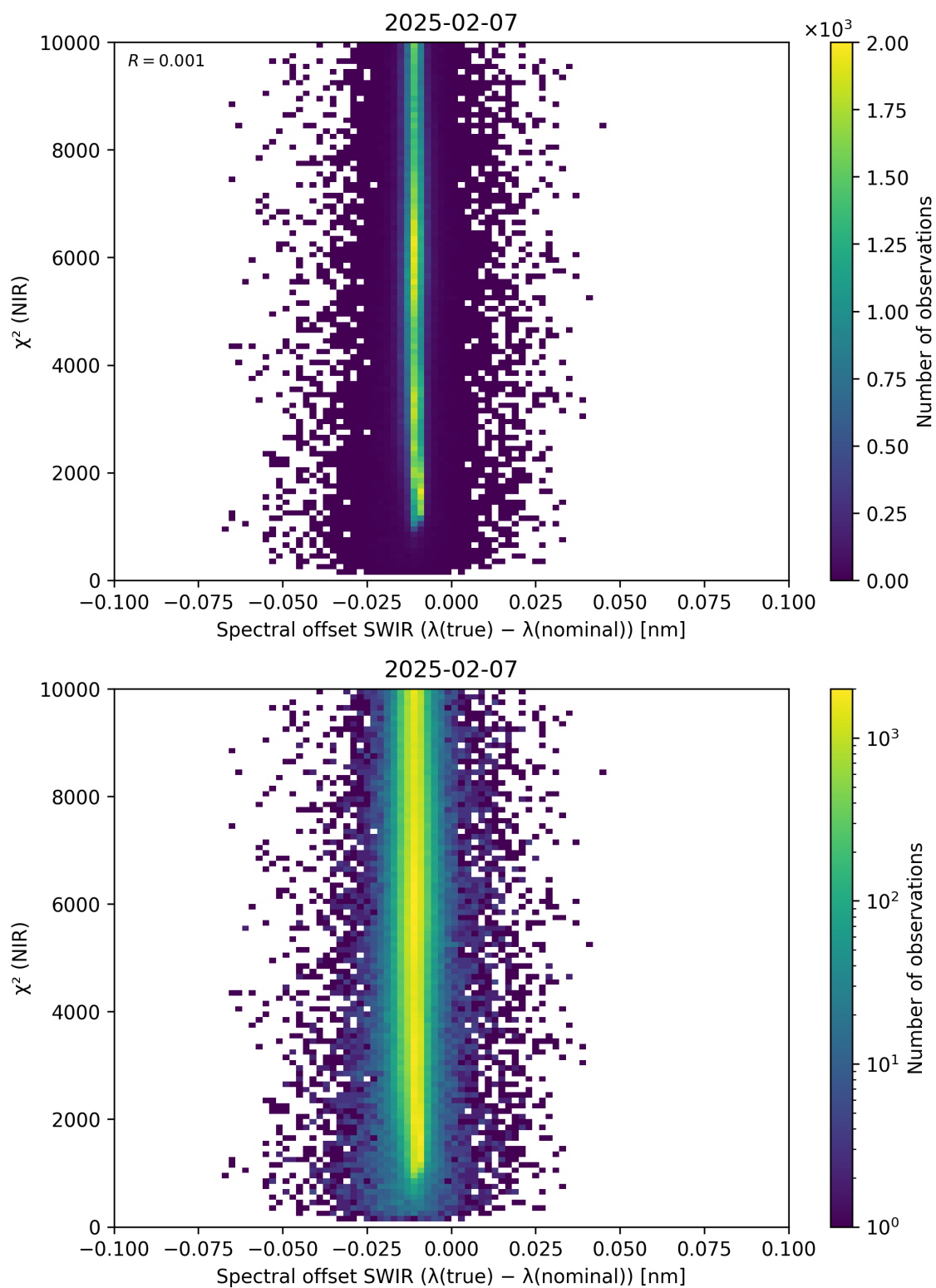
Figure 117: Scatter density plot of “Spectral offset SWIR ( \lambda_{\text{true}} - \lambda_{\text{nominal}} )” against “ \chi^2 (NIR)” for 2025-02-06 to 2025-02-08.
