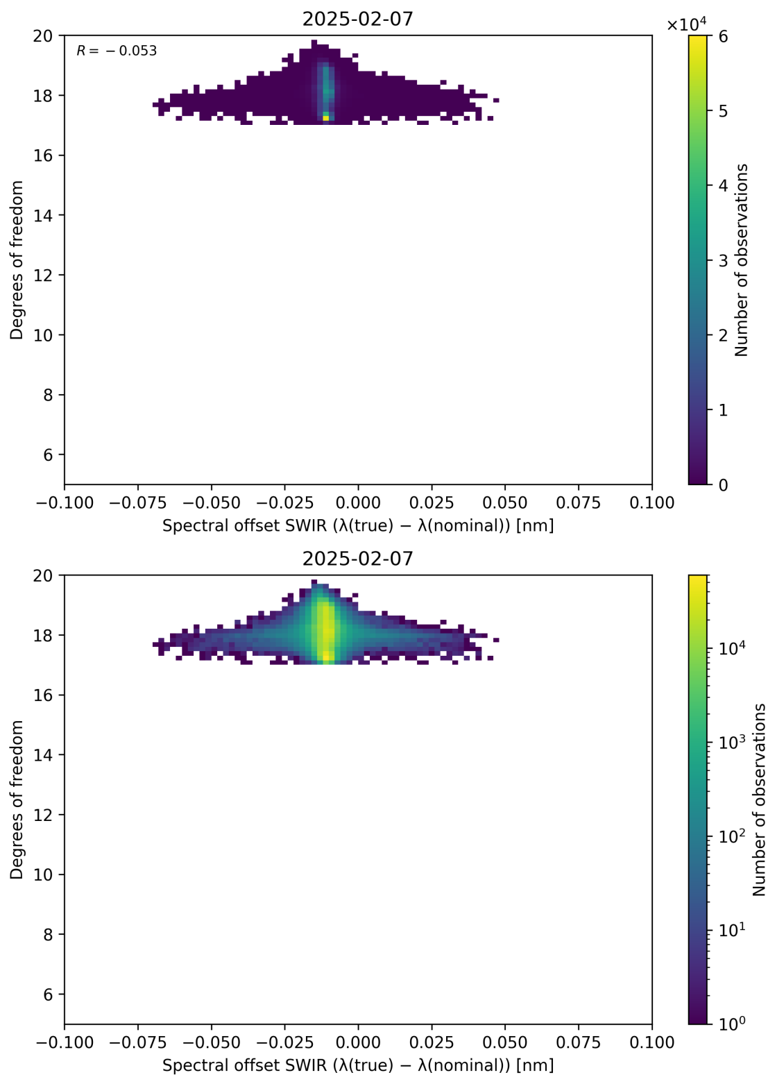
Figure 119: Scatter density plot of “Spectral offset SWIR ( \lambda_{\text{true}} - \lambda_{\text{nominal}} )” against “Degrees of freedom” for 2025-02-06 to 2025-02-08.
