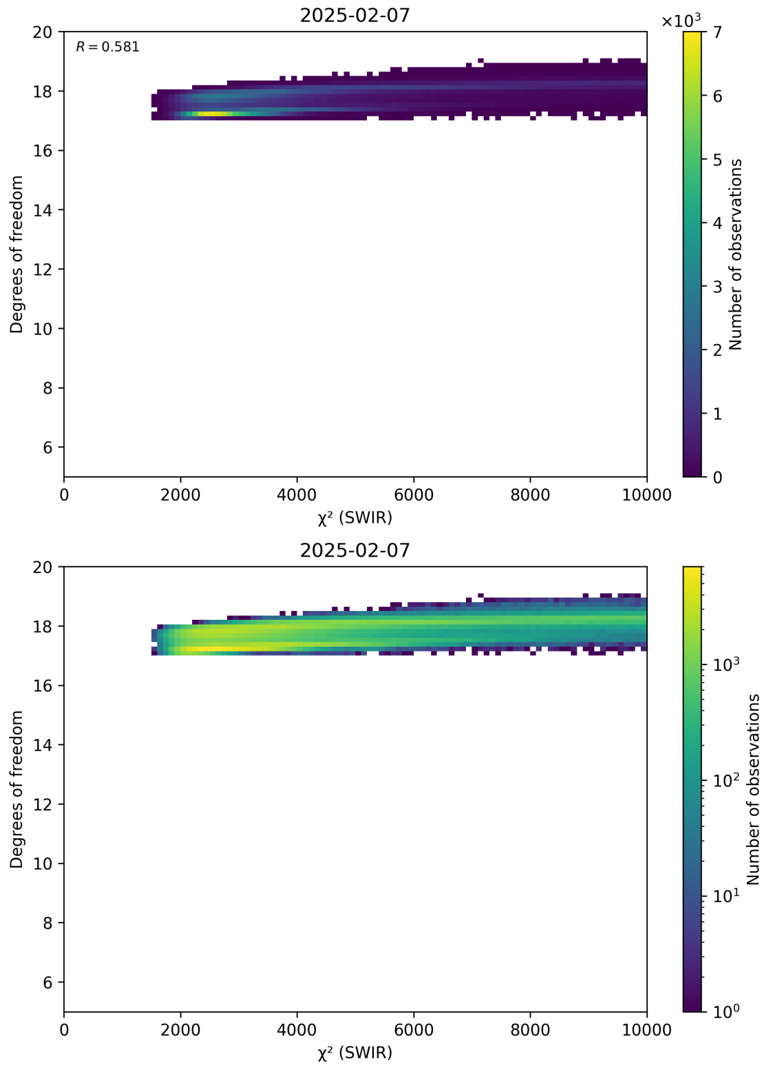
Figure 48: Scatter density plot of “ \chi^2 (SWIR)” against “Degrees of freedom” for 2025-02-06 to 2025-02-08.
