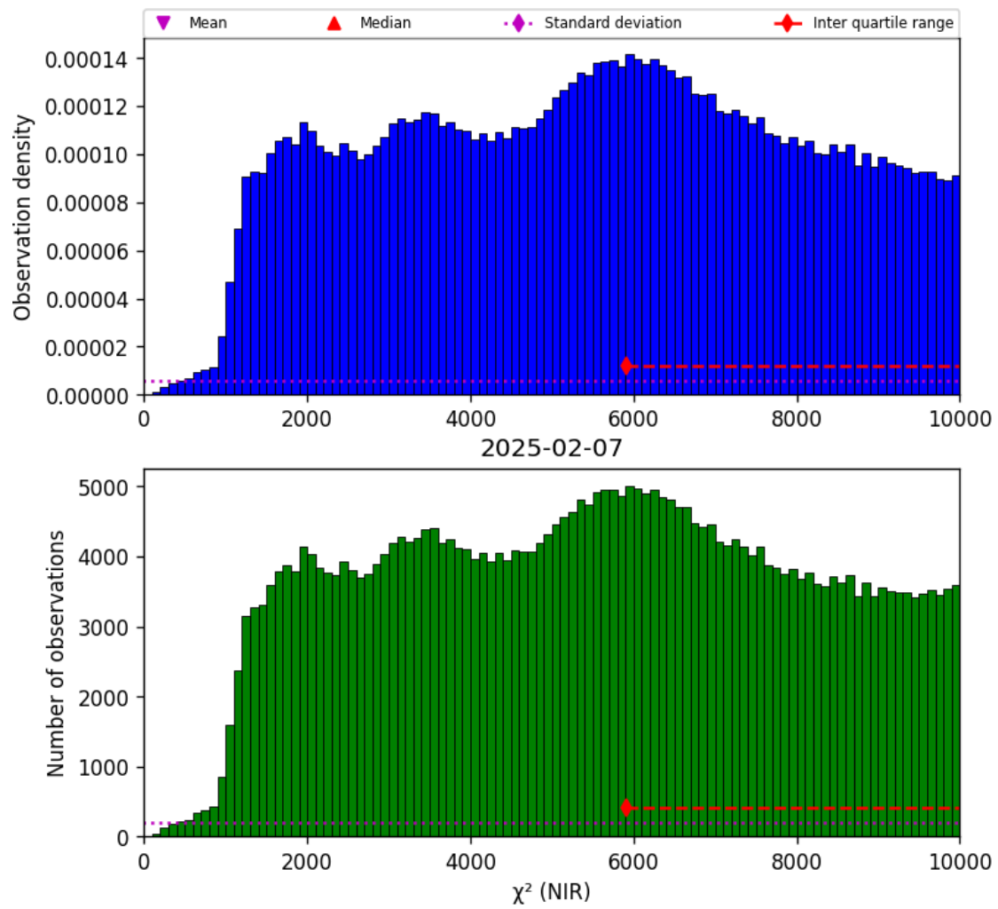
Figure 29: Histogram of “ \chi^2 (NIR)” for 2025-02-06 to 2025-02-08
