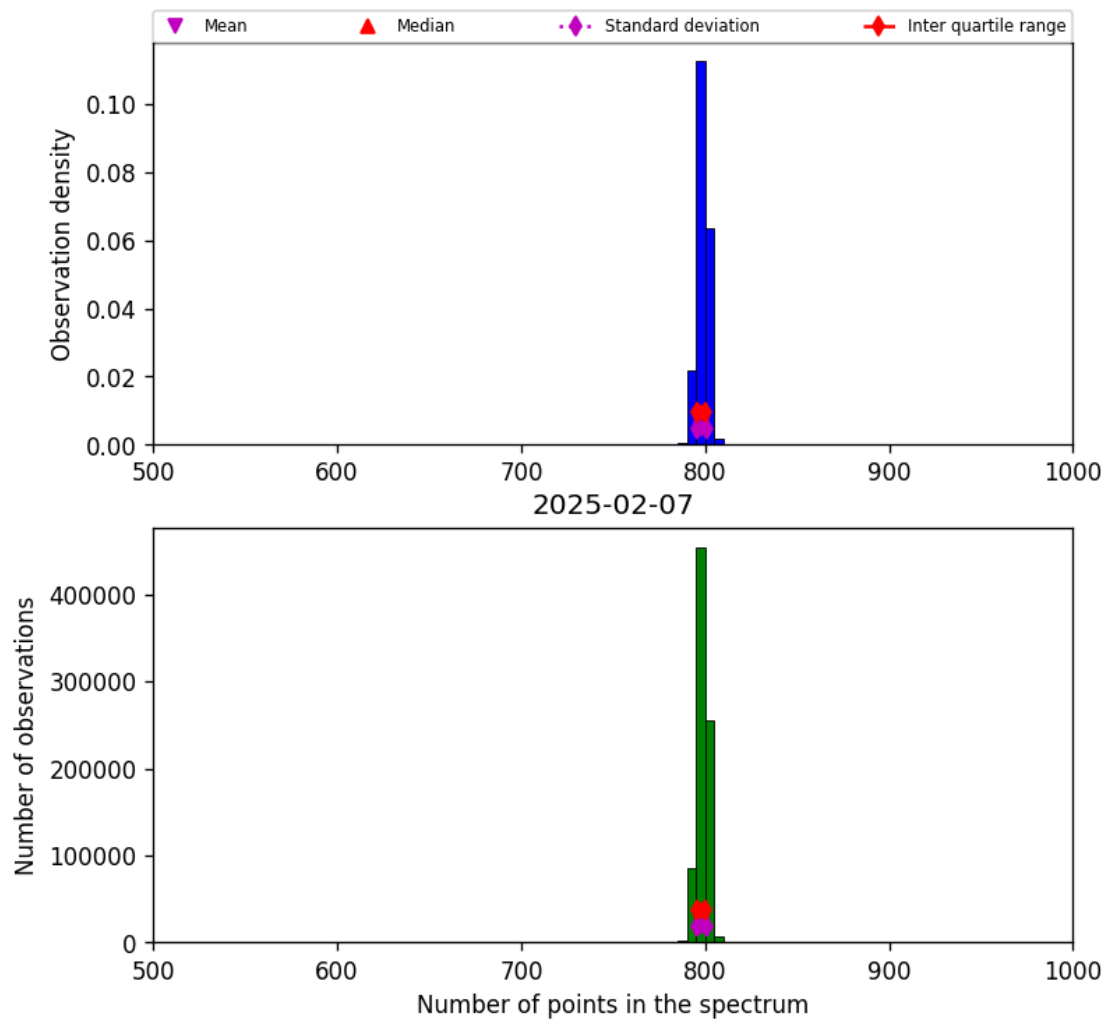
Figure 26: Histogram of “Number of points in the spectrum” for 2025-02-06 to 2025-02-08
