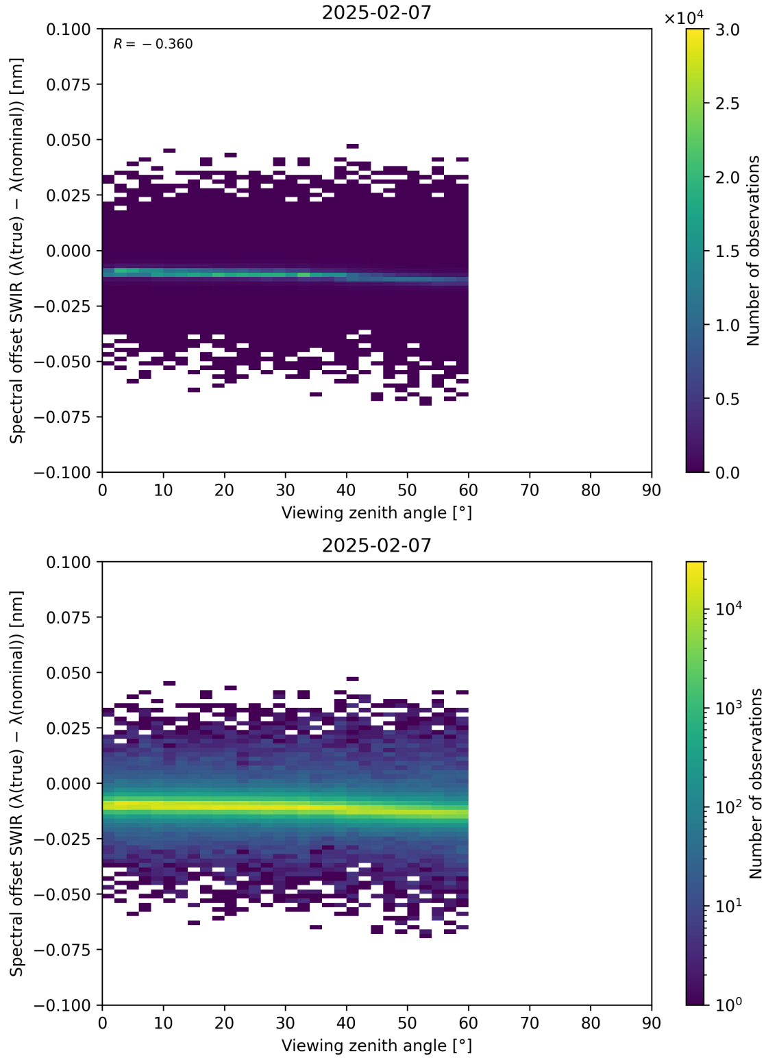
Figure 116: Scatter density plot of “Viewing zenith angle” against “Spectral offset SWIR ( \lambda_{\text{true}} - \lambda_{\text{nominal}} )” for 2025-02-06 to 2025-02-08.
