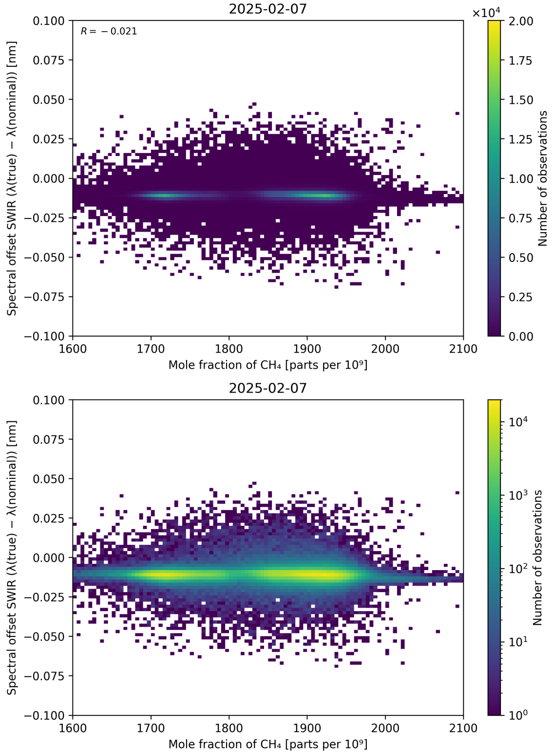
Figure 86: Scatter density plot of “Mole fraction of CH 4 ” against “Spectral offset SWIR ( \lambda_{\text{true}} - \lambda_{\text{nominal}} )” for 2025-02-06 to 2025-02-08.
