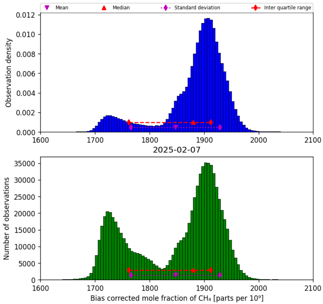
Figure 25: Histogram of “Bias corrected mole fraction of CH 4 ” for 2025-02-06 to 2025-02-08
