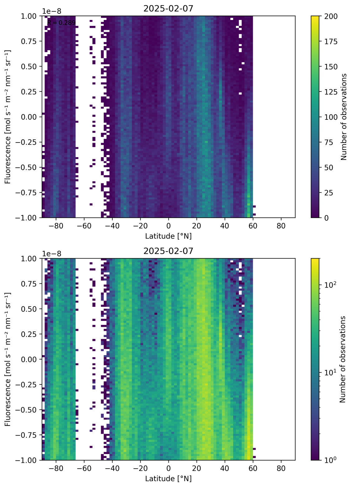
Figure 56: Scatter density plot of “Latitude” against “Fluorescence” for 2025-02-06 to 2025-02-08.
