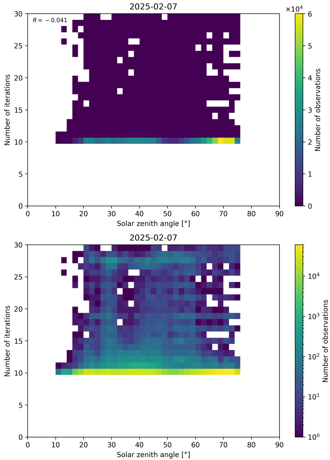
Figure 102: Scatter density plot of “Solar zenith angle” against “Number of iterations” for 2025-02-06 to 2025-02-08.
