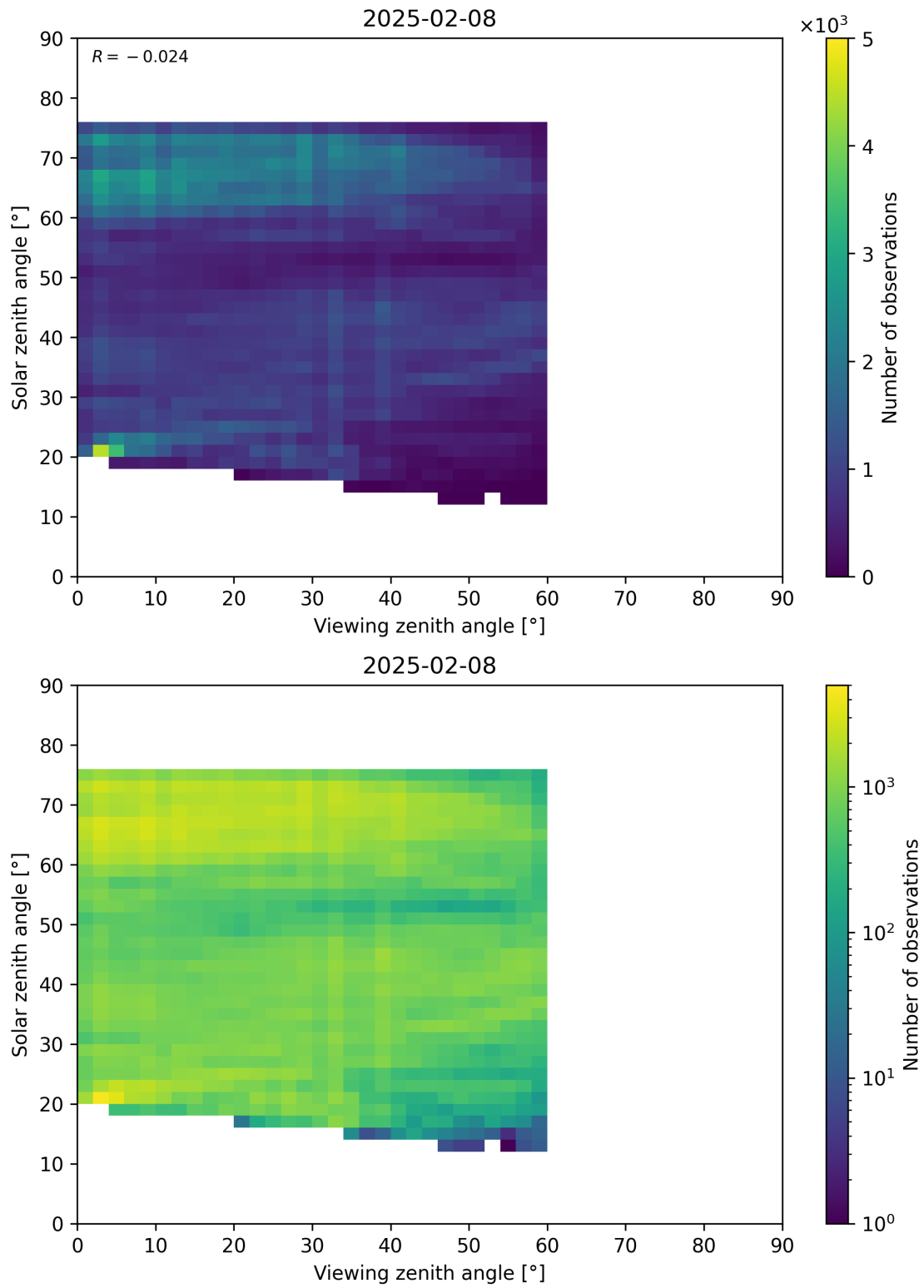
Figure 115: Scatter density plot of “Viewing zenith angle” against “Solar zenith angle” for 2025-02-08 to 2025-02-09.
