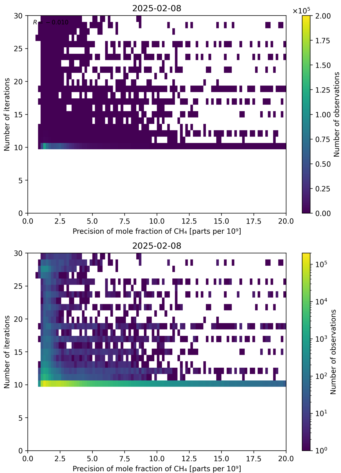
Figure 83: Scatter density plot of “Precision of mole fraction of CH 4 ” against “Number of iterations” for 2025-02-08 to 2025-02-09.
