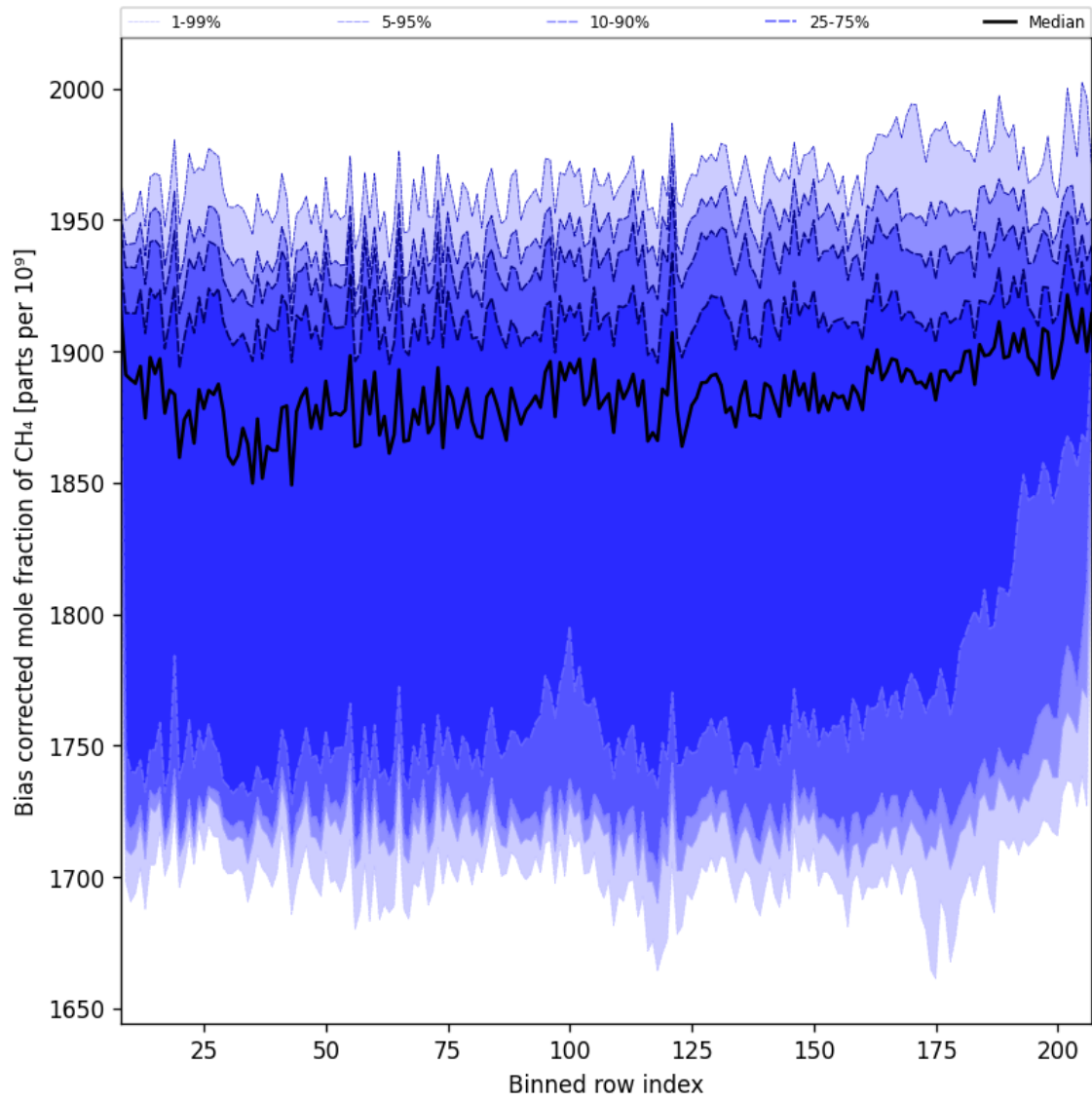
Figure 36: Along track statistics of “Bias corrected mole fraction of CH 4 ” for 2025-02-08 to 2025-02-09
