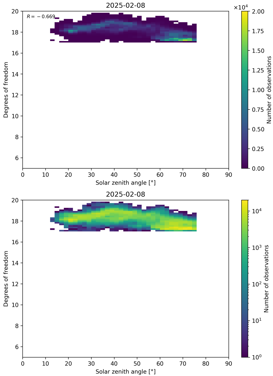
Figure 96: Scatter density plot of “Solar zenith angle” against “Degrees of freedom” for 2025-02-08 to 2025-02-09.
