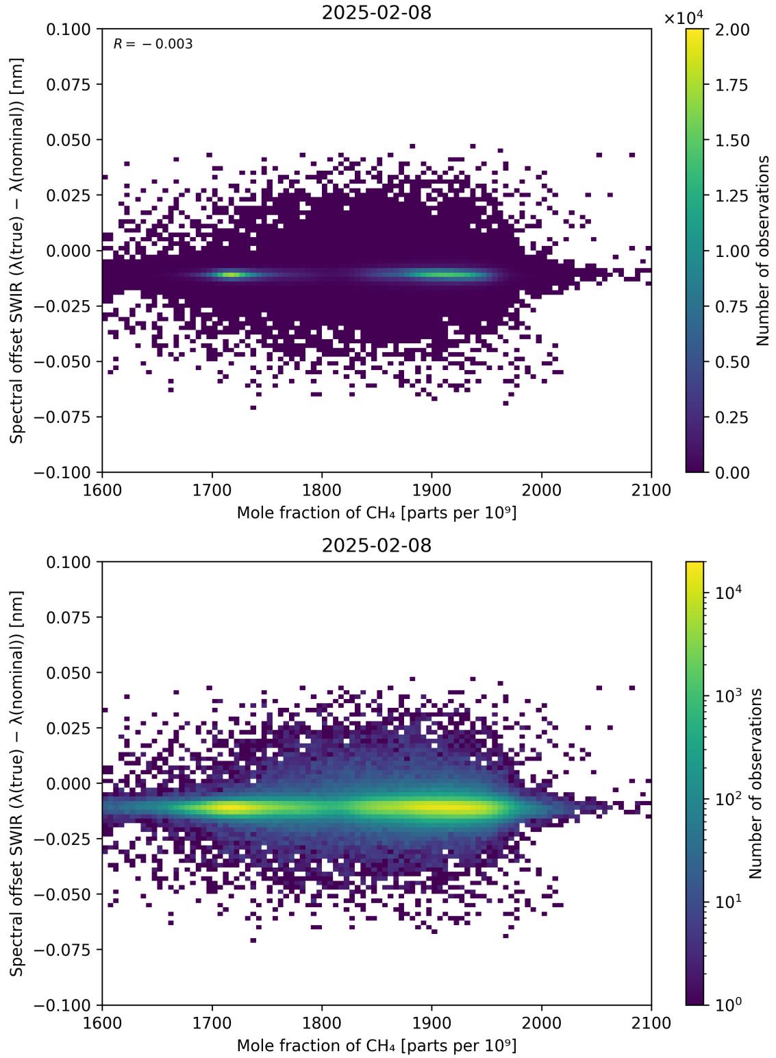
Figure 86: Scatter density plot of “Mole fraction of CH 4 ” against “Spectral offset SWIR ( \lambda_{\text{true}} - \lambda_{\text{nominal}} )” for 2025-02-08 to 2025-02-09.
