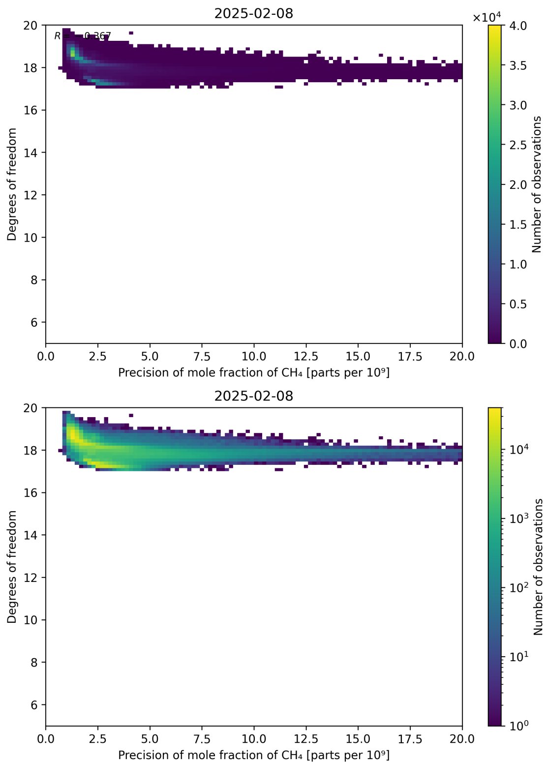
Figure 80: Scatter density plot of “Precision of mole fraction of CH 4 ” against “Degrees of freedom” for 2025-02-08 to 2025-02-09.
