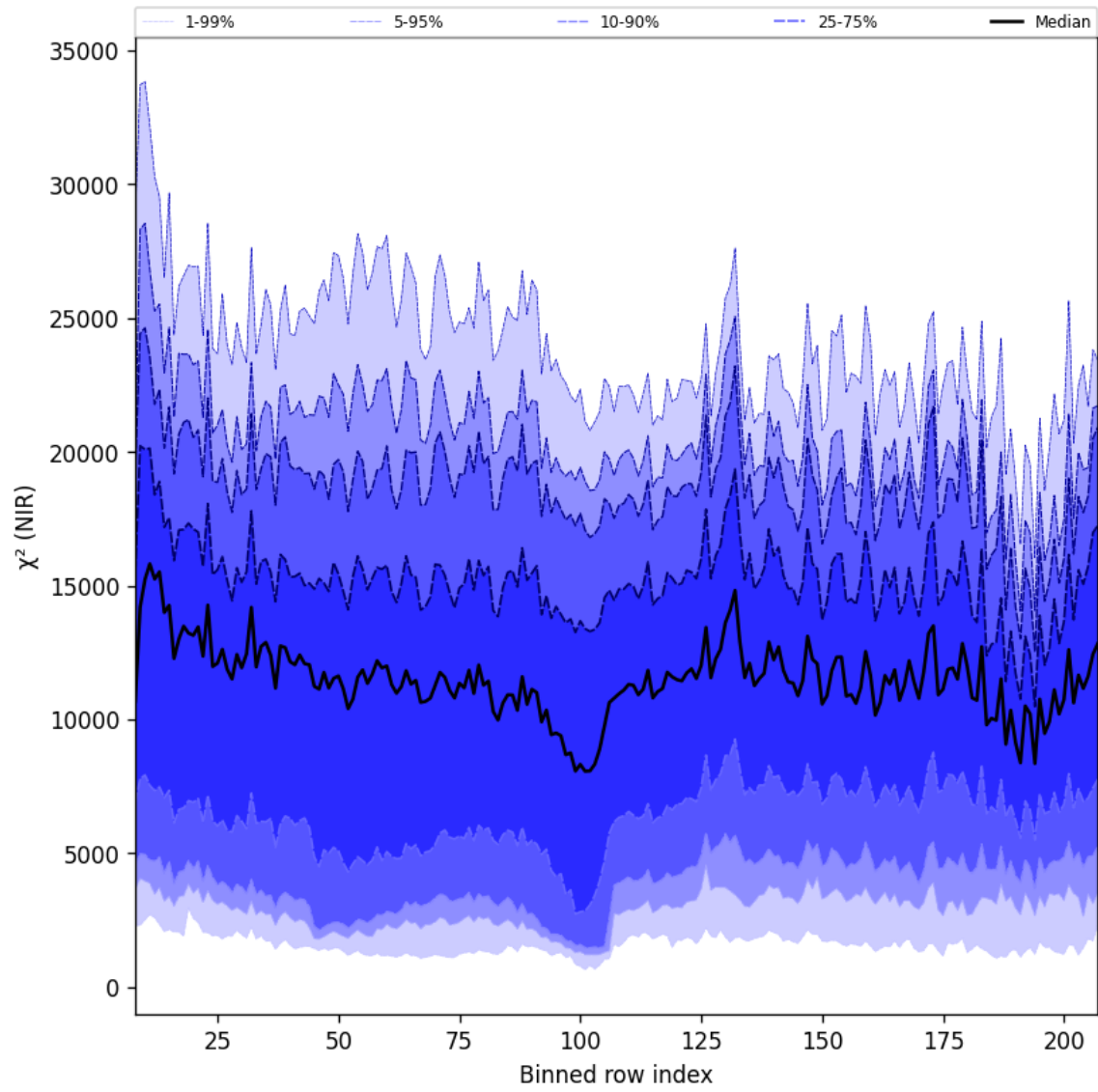
Figure 40: Along track statistics of “ \chi^2 (NIR)” for 2025-02-08 to 2025-02-09
