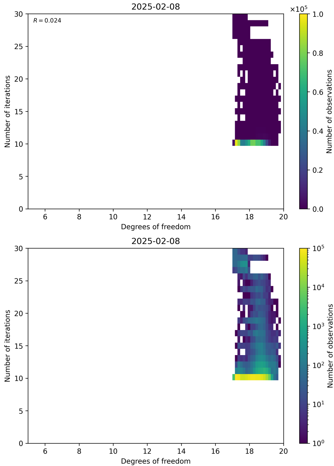
Figure 52: Scatter density plot of “Degrees of freedom” against “Number of iterations” for 2025-02-08 to 2025-02-09.
