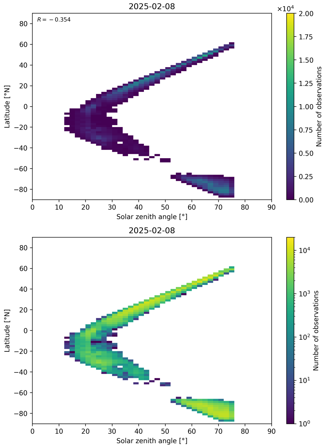
Figure 98: Scatter density plot of “Solar zenith angle” against “Latitude” for 2025-02-08 to 2025-02-09.
