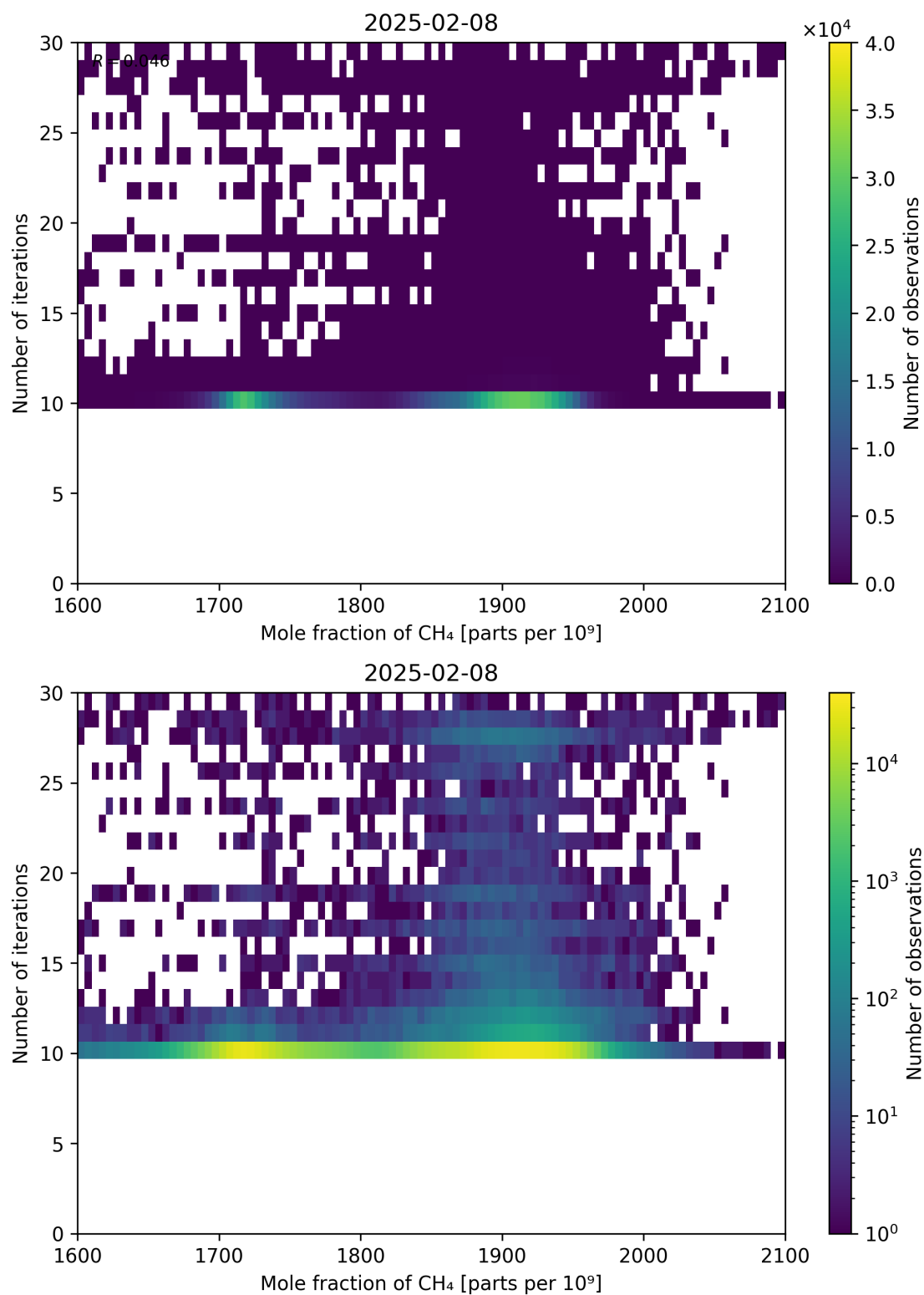
Figure 76: Scatter density plot of “Mole fraction of CH 4 ” against “Number of iterations” for 2025-02-08 to 2025-02-09.
