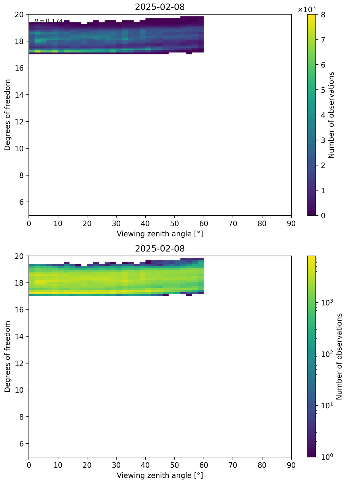
Figure 107: Scatter density plot of “Viewing zenith angle” against “Degrees of freedom” for 2025-02-08 to 2025-02-09.
