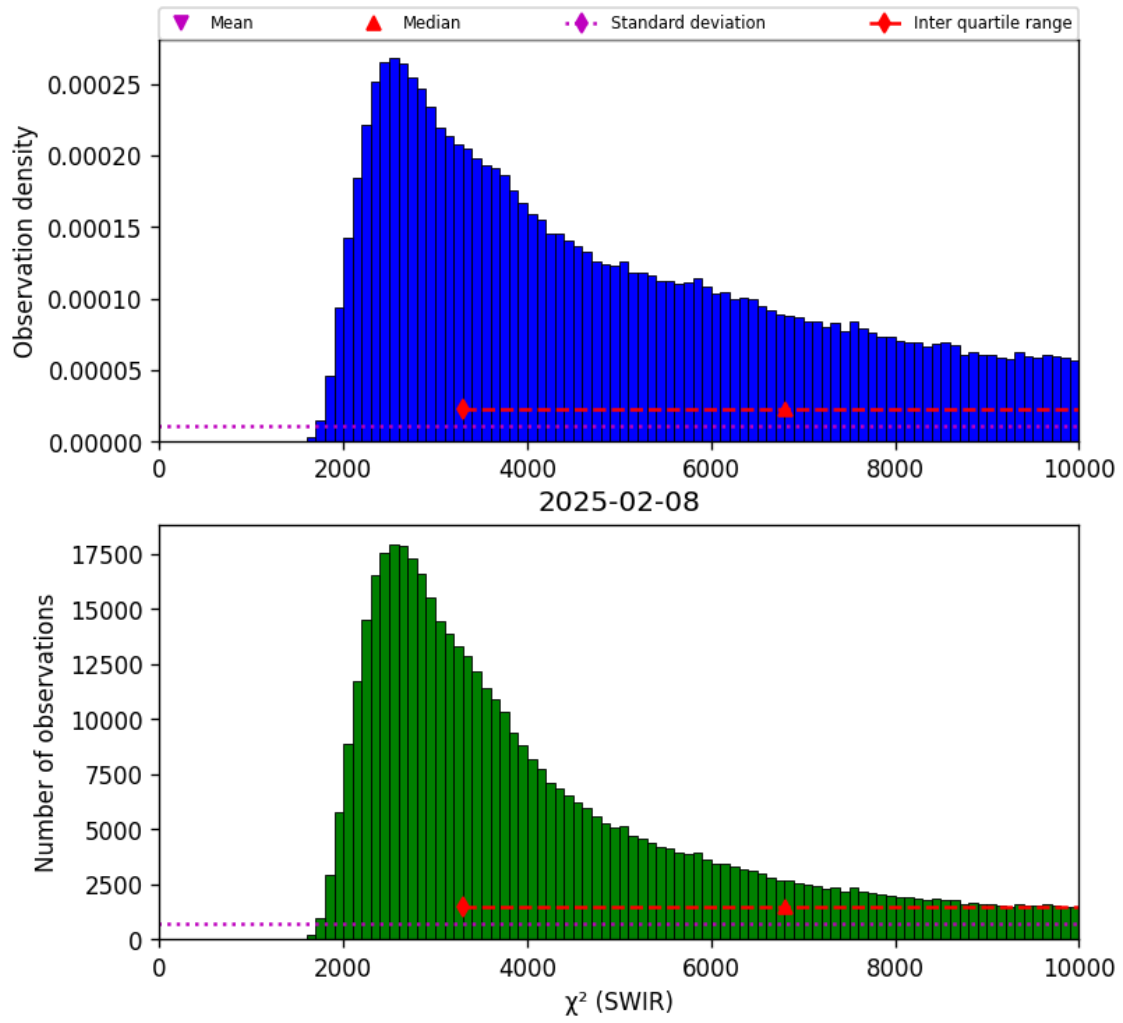
Figure 28: Histogram of “ \chi^2 (SWIR)” for 2025-02-08 to 2025-02-09
