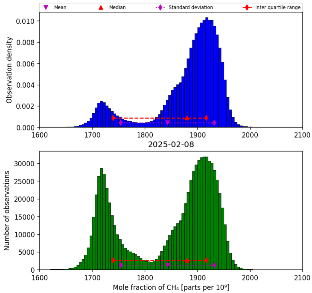
Figure 23: Histogram of “Mole fraction of CH 4 ” for 2025-02-08 to 2025-02-09
