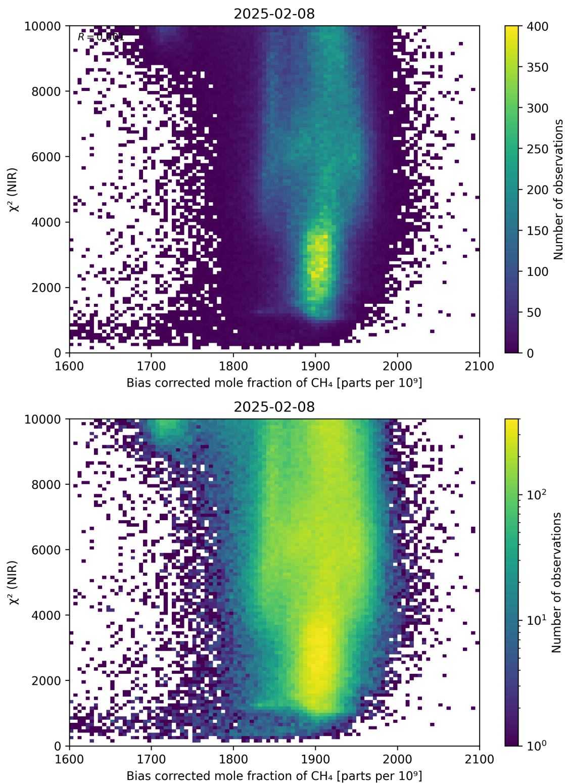
Figure 63: Scatter density plot of “Bias corrected mole fraction of \text{CH}_4 ” against “ \chi^2 (NIR)” for 2025-02-08 to 2025-02-09.
