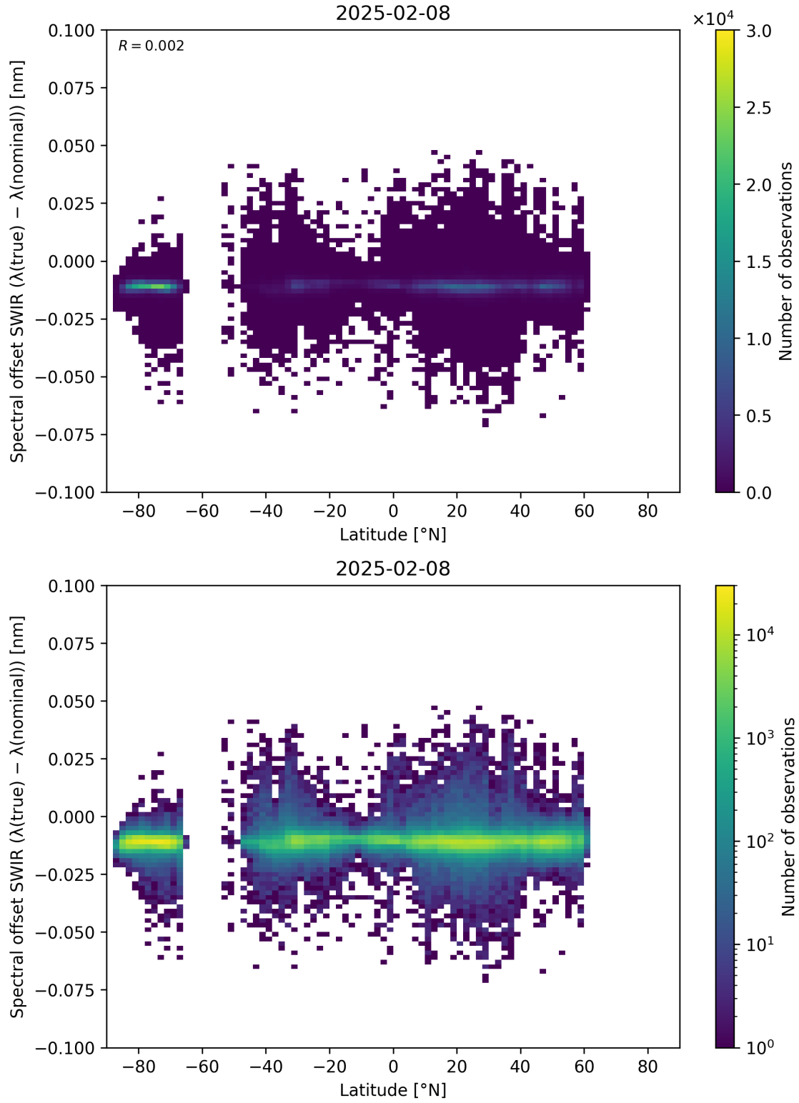
Figure 62: Scatter density plot of “Latitude” against “Spectral offset SWIR ( \lambda_{\text{true}} - \lambda_{\text{nominal}} )” for 2025-02-08 to 2025-02-09.
