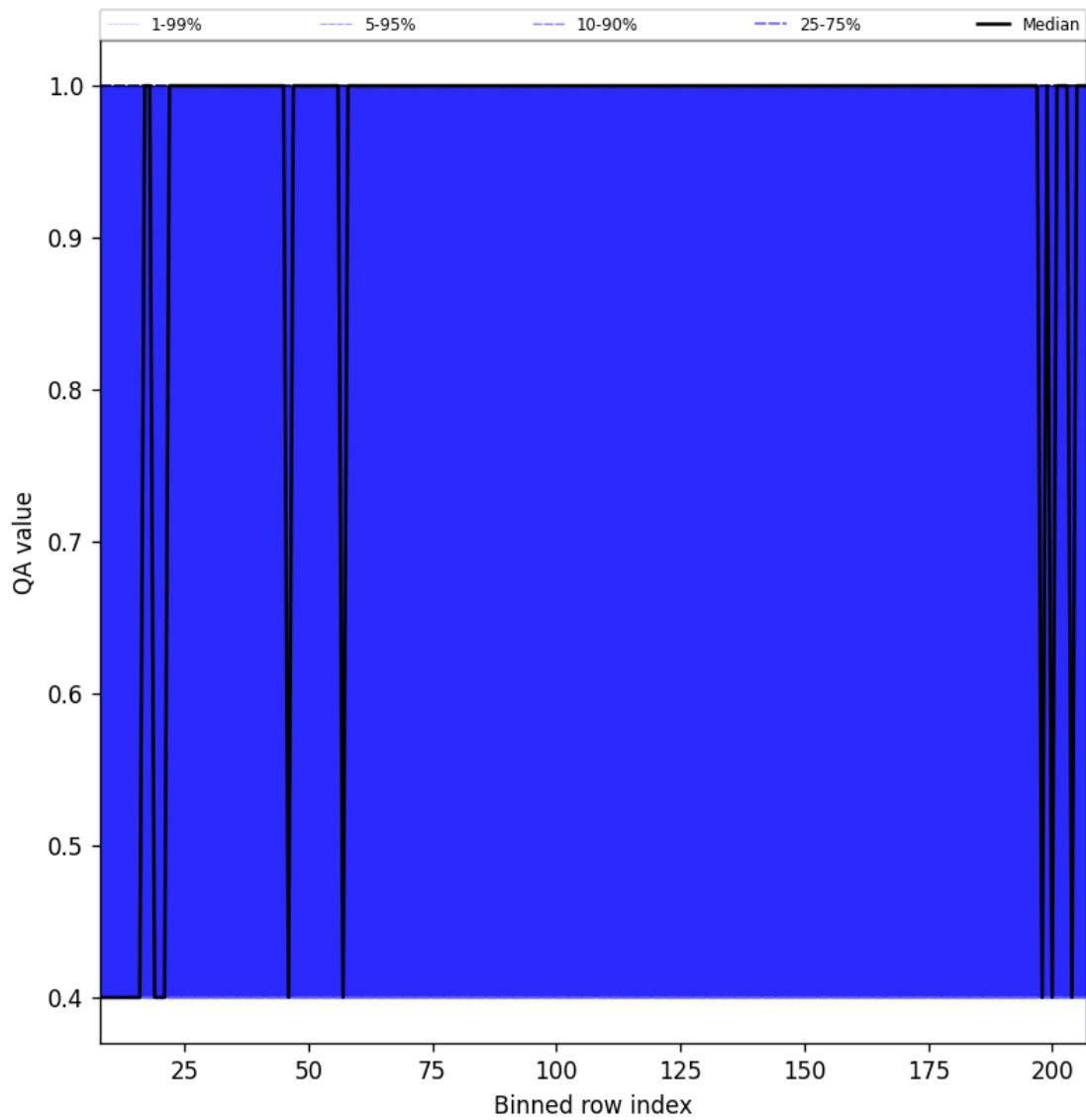
Figure 33: Along track statistics of “QA value” for 2025-02-08 to 2025-02-09
