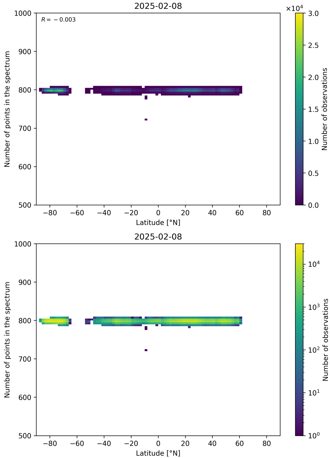
Figure 61: Scatter density plot of “Latitude” against “Number of points in the spectrum” for 2025-02-08 to 2025-02-09.
