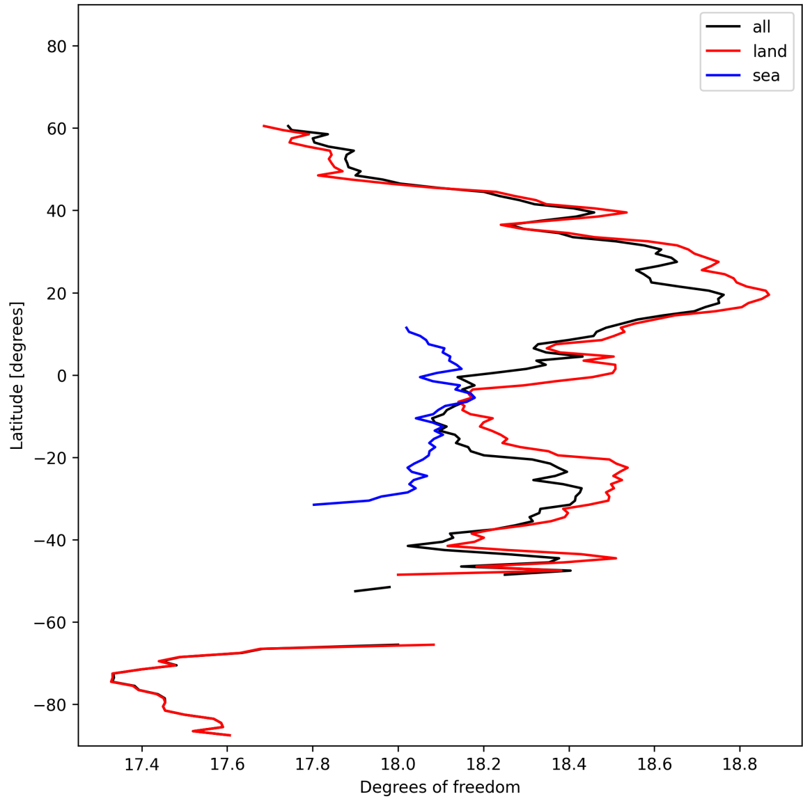
Figure 19: Zonal average of “Degrees of freedom” for 2025-02-08 to 2025-02-09.
