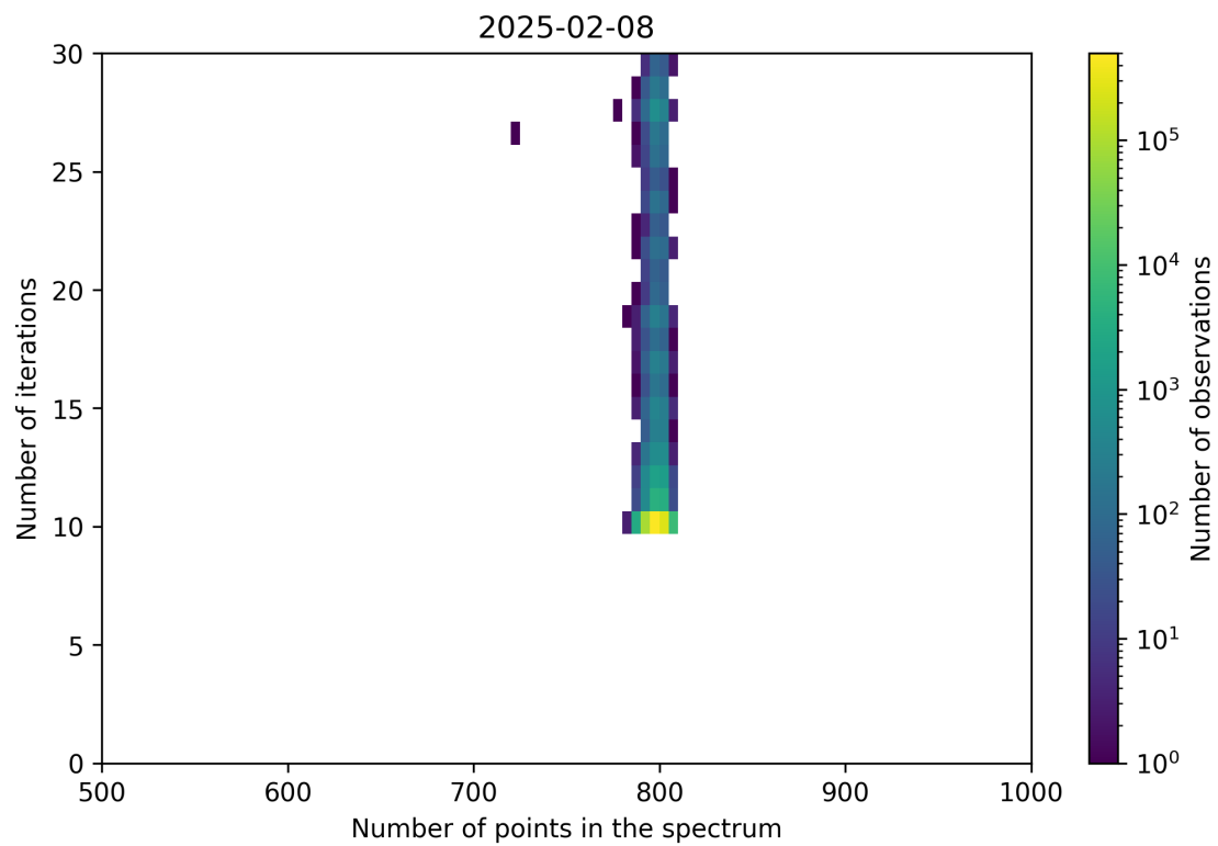
Figure 92: Scatter density plot of “Number of points in the spectrum” against “Number of iterations” for 2025-02-08 to 2025-02-09.
