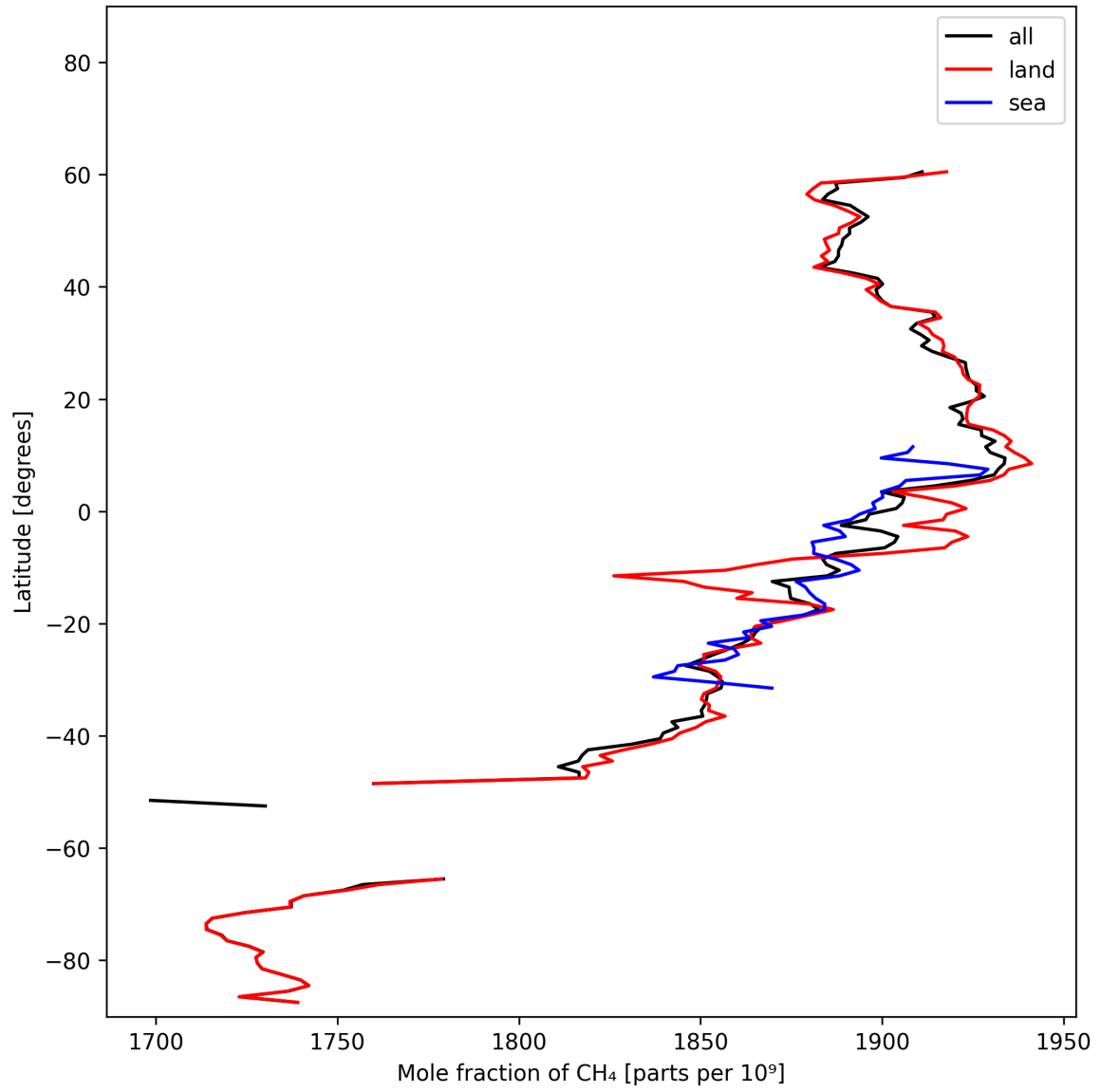
Figure 12: Zonal average of “Mole fraction of CH 4 ” for 2025-02-08 to 2025-02-09.
