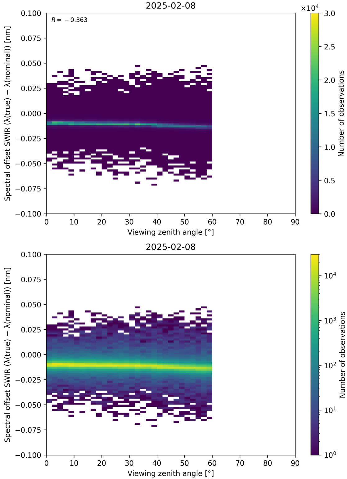
Figure 116: Scatter density plot of “Viewing zenith angle” against “Spectral offset SWIR ( \lambda_{\text{true}} - \lambda_{\text{nominal}} )” for 2025-02-08 to 2025-02-09.
