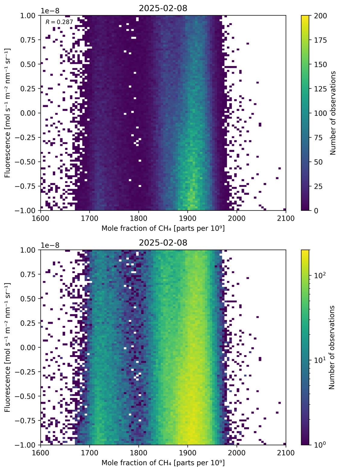
Figure 73: Scatter density plot of “Mole fraction of CH 4 ” against “Fluorescence” for 2025-02-08 to 2025-02-09.
