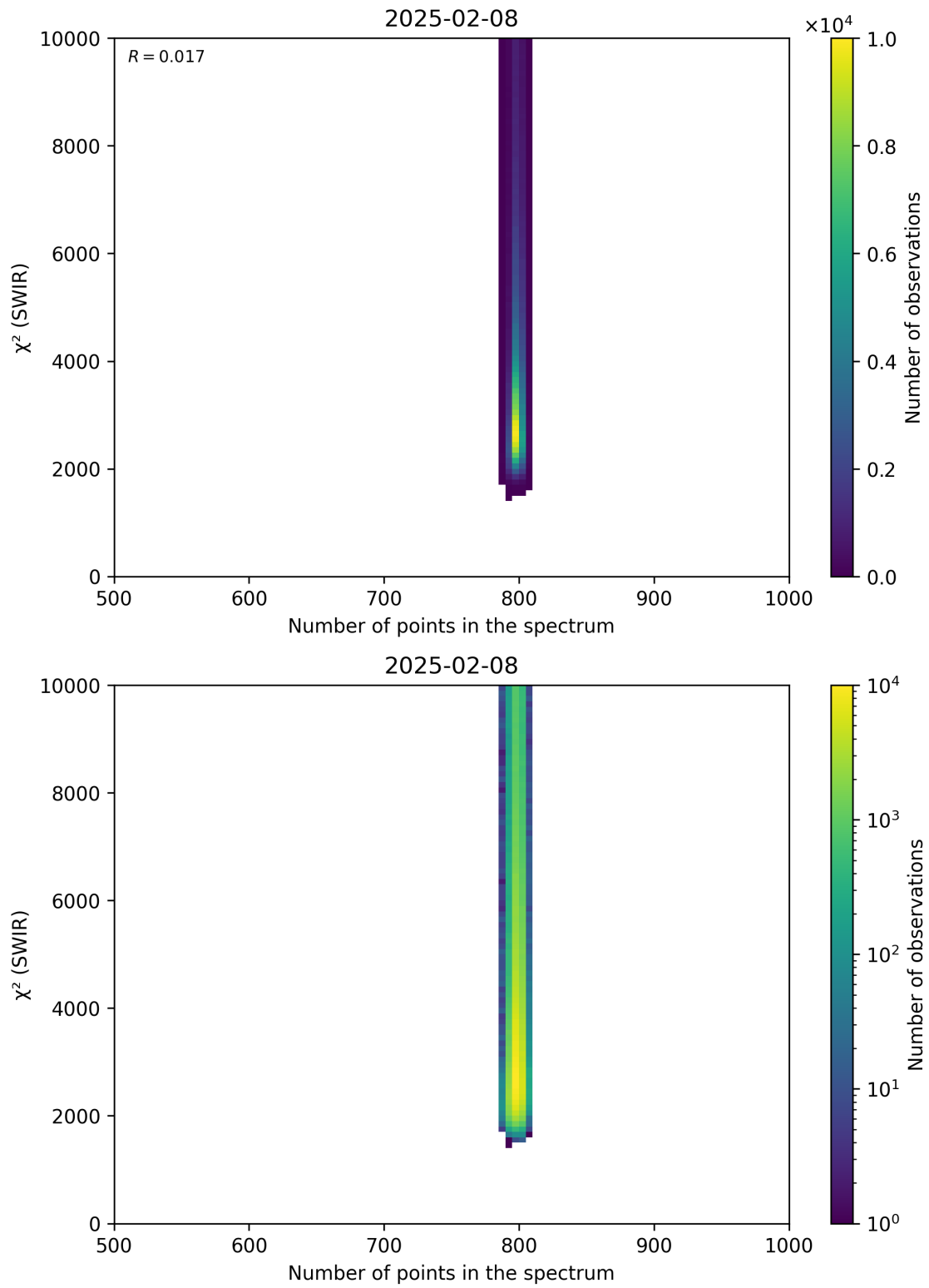
Figure 89: Scatter density plot of “Number of points in the spectrum” against “ \chi^2 (SWIR)” for 2025-02-08 to 2025-02-09.
