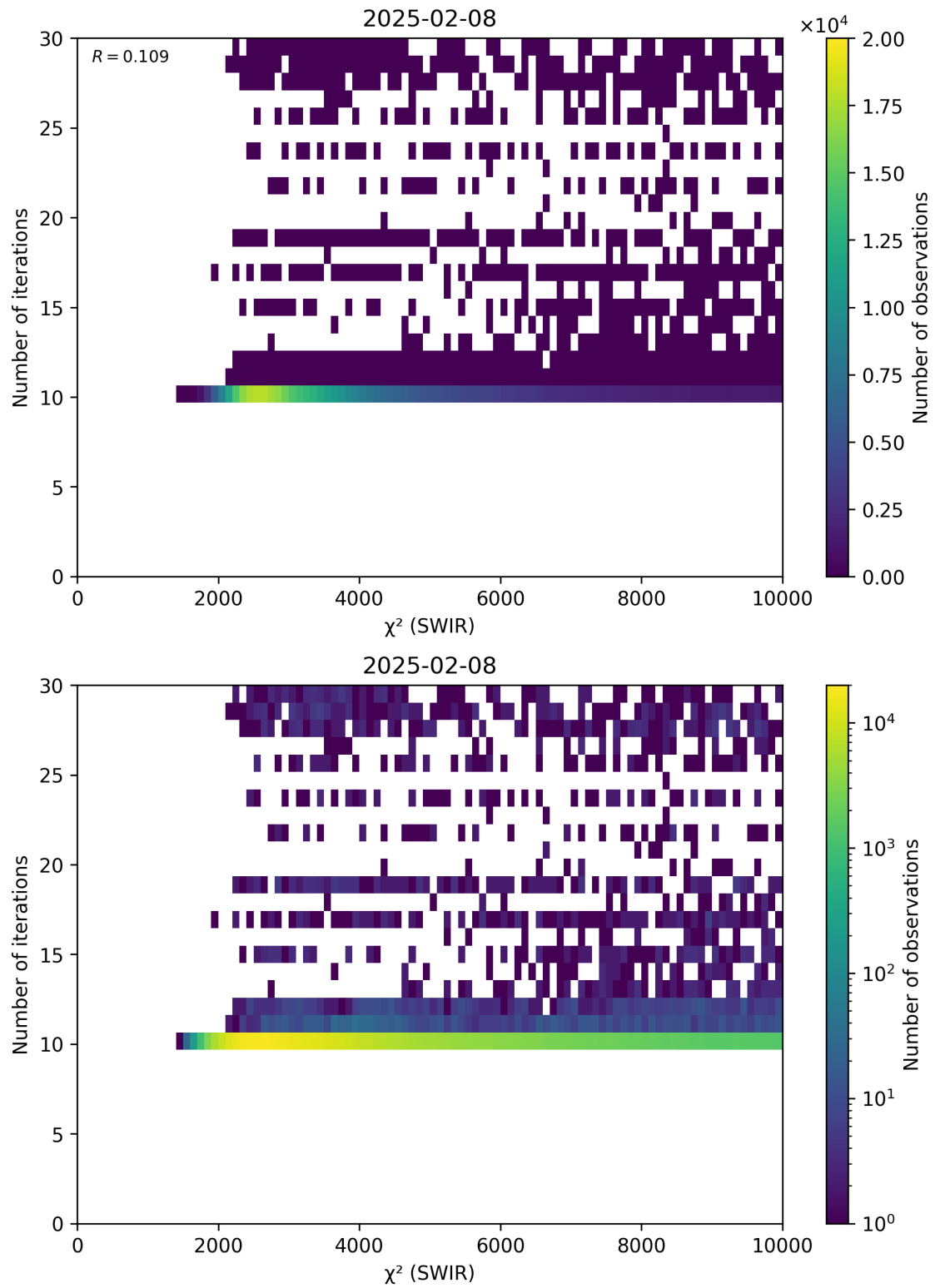
Figure 50: Scatter density plot of “ \chi^2 (SWIR)” against “Number of iterations” for 2025-02-08 to 2025-02-09.
