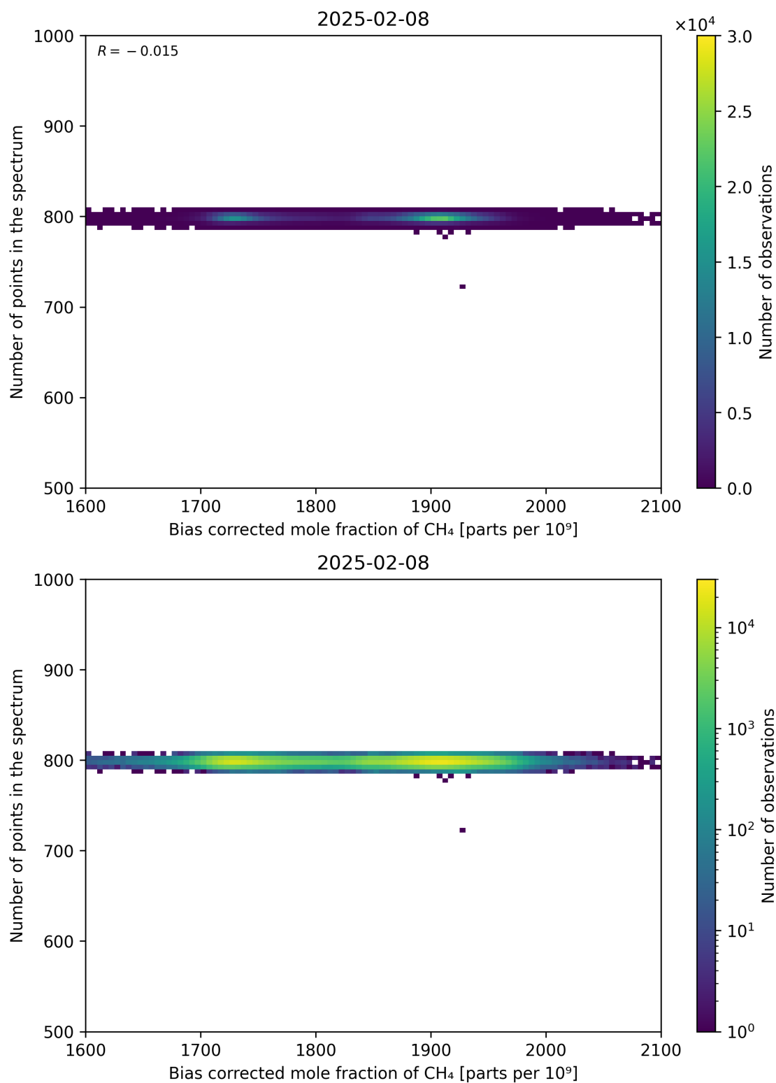
Figure 68: Scatter density plot of “Bias corrected mole fraction of CH 4 ” against “Number of points in the spectrum” for 2025-02-08 to 2025-02-09.
