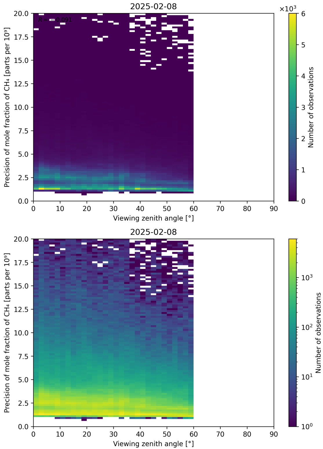
Figure 112: Scatter density plot of “Viewing zenith angle” against “Precision of mole fraction of CH 4 ” for 2025-02-08 to 2025-02-09.
