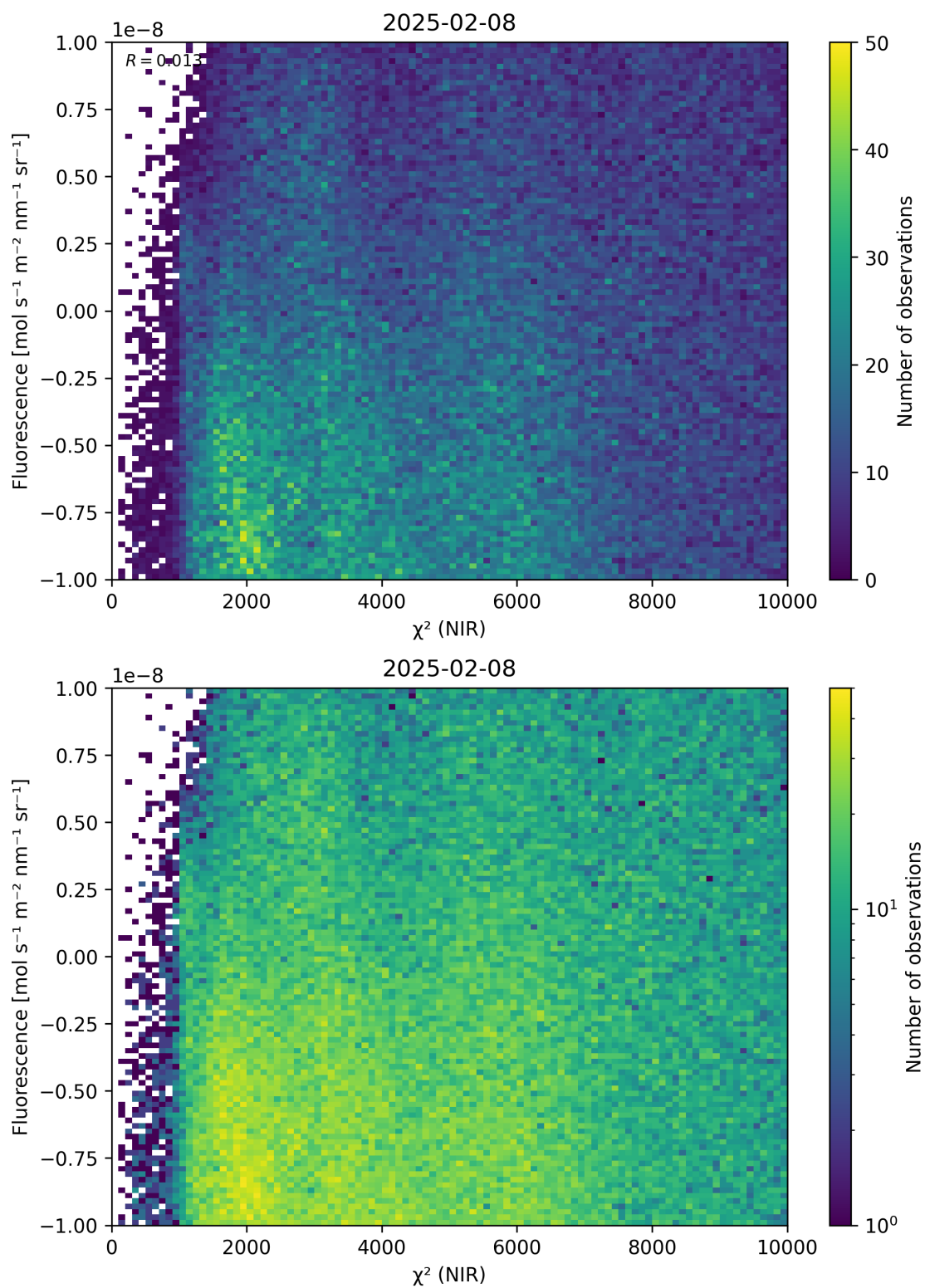
Figure 45: Scatter density plot of “ \chi^2 (NIR)” against “Fluorescence” for 2025-02-08 to 2025-02-09.
