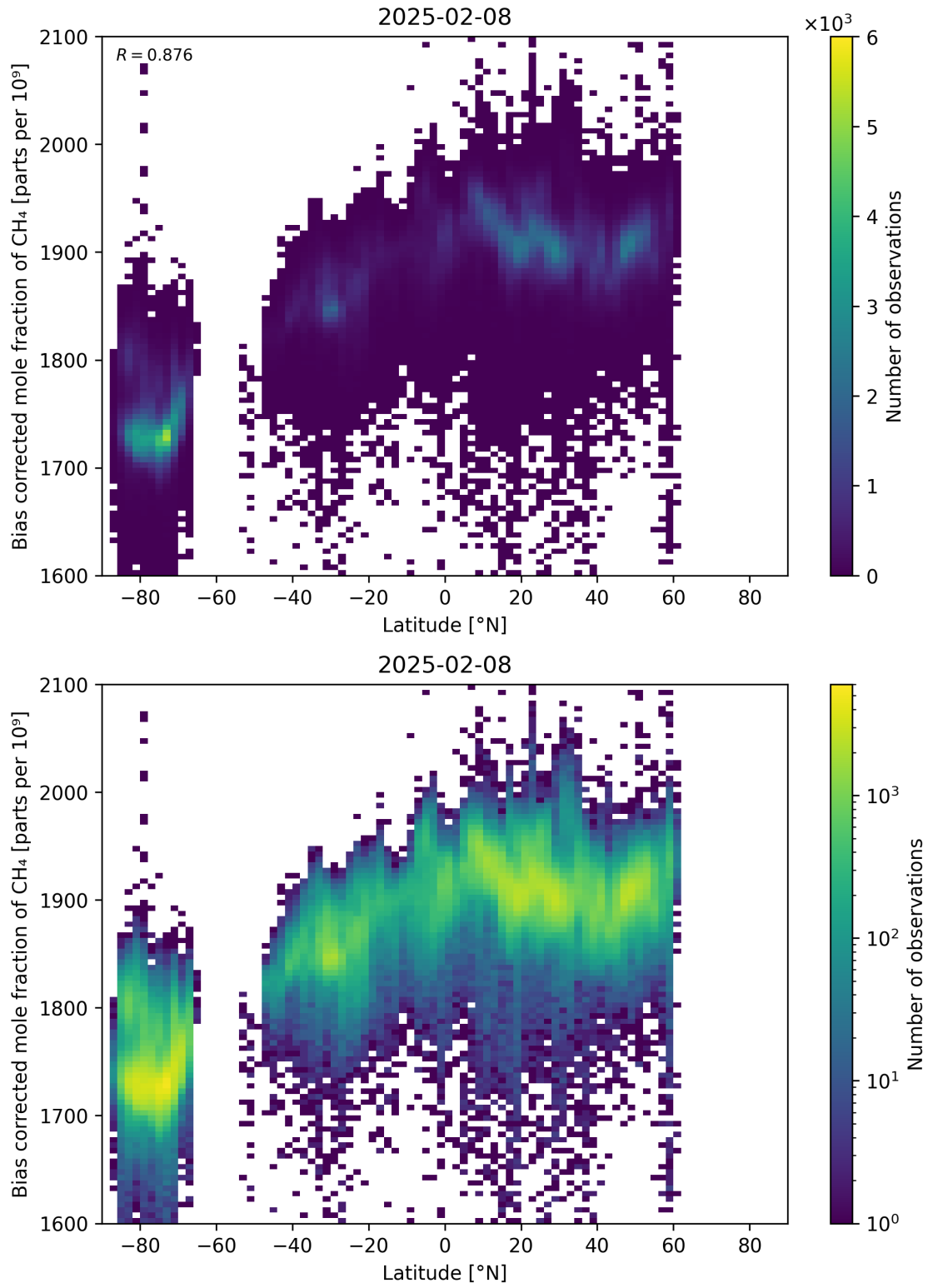
Figure 58: Scatter density plot of “Latitude” against “Bias corrected mole fraction of CH 4 ” for 2025-02-08 to 2025-02-09.
