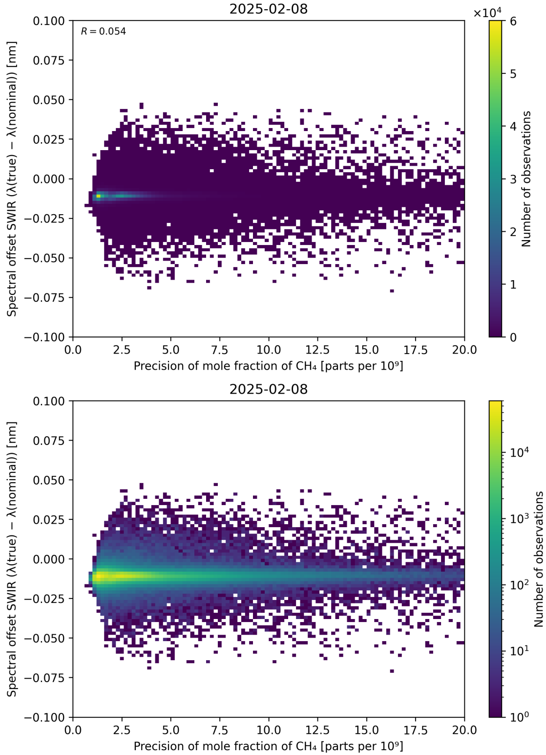
Figure 85: Scatter density plot of “Precision of mole fraction of \text{CH}_4 ” against “Spectral offset SWIR ( \lambda_{\text{true}} - \lambda_{\text{nominal}} )” for 2025-02-08 to 2025-02-09.
