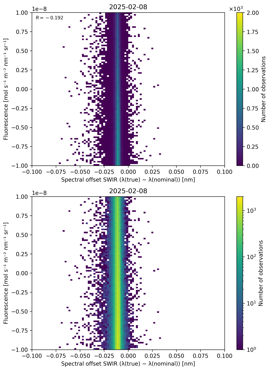
Figure 120: Scatter density plot of “Spectral offset SWIR ( \lambda_{\text{true}} - \lambda_{\text{nominal}} )” against “Fluorescence” for 2025-02-08 to 2025-02-09.
