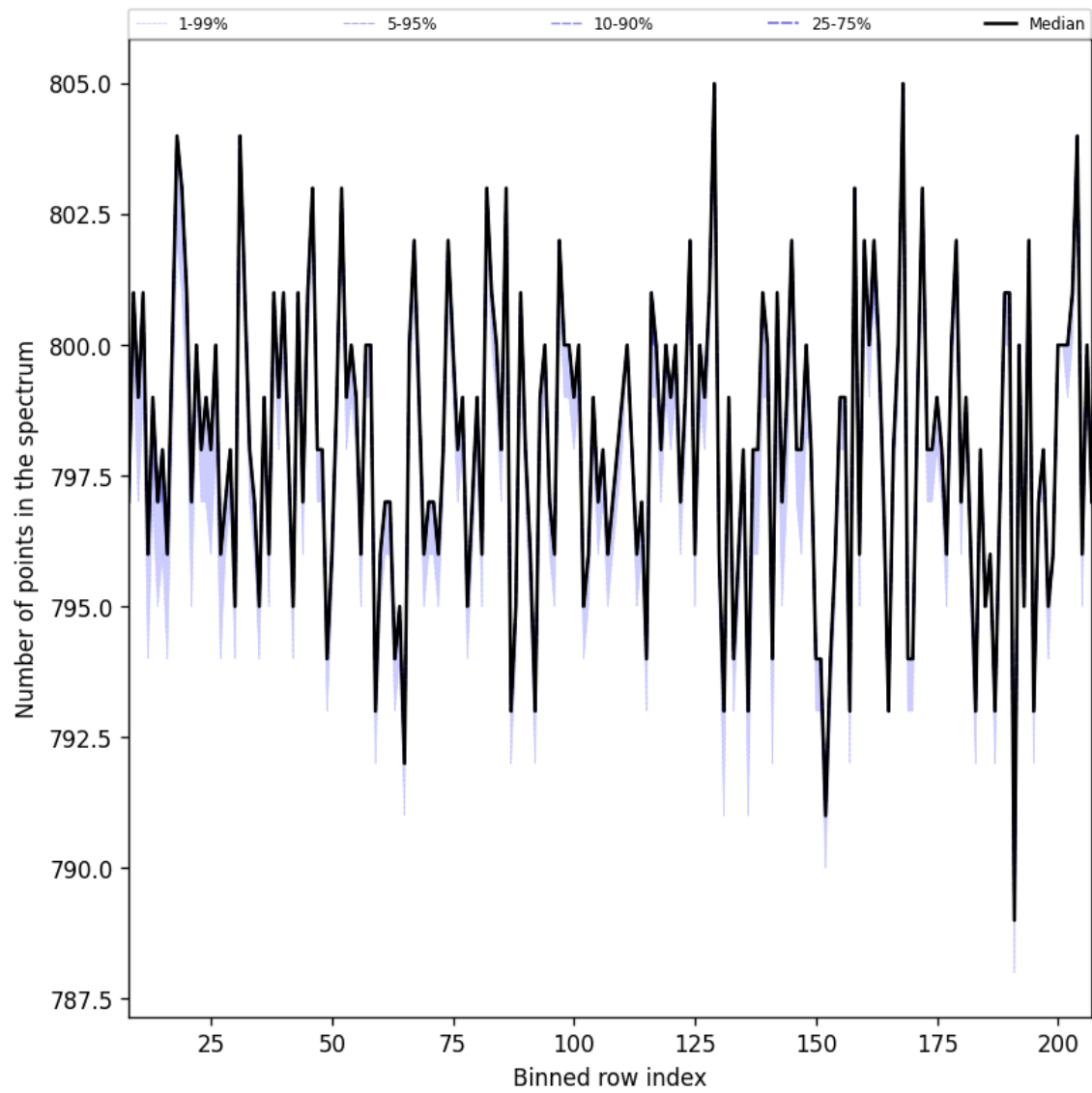
Figure 37: Along track statistics of “Number of points in the spectrum” for 2025-02-08 to 2025-02-09
