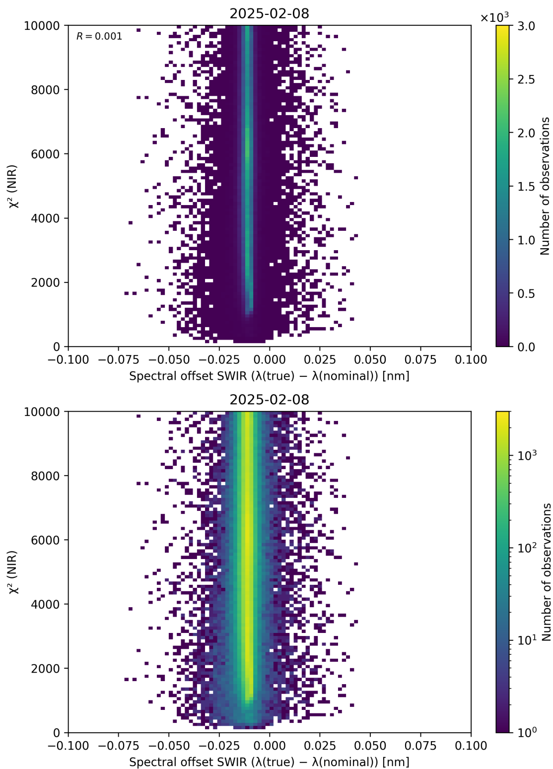
Figure 117: Scatter density plot of “Spectral offset SWIR ( \lambda_{\text{true}} - \lambda_{\text{nominal}} )” against “ \chi^2 (NIR)” for 2025-02-08 to 2025-02-09.
