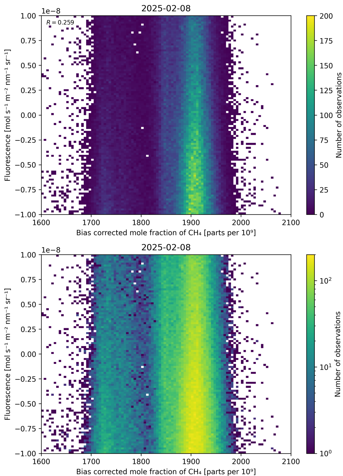
Figure 66: Scatter density plot of “Bias corrected mole fraction of \text{CH}_4 ” against “Fluorescence” for 2025-02-08 to 2025-02-09.
