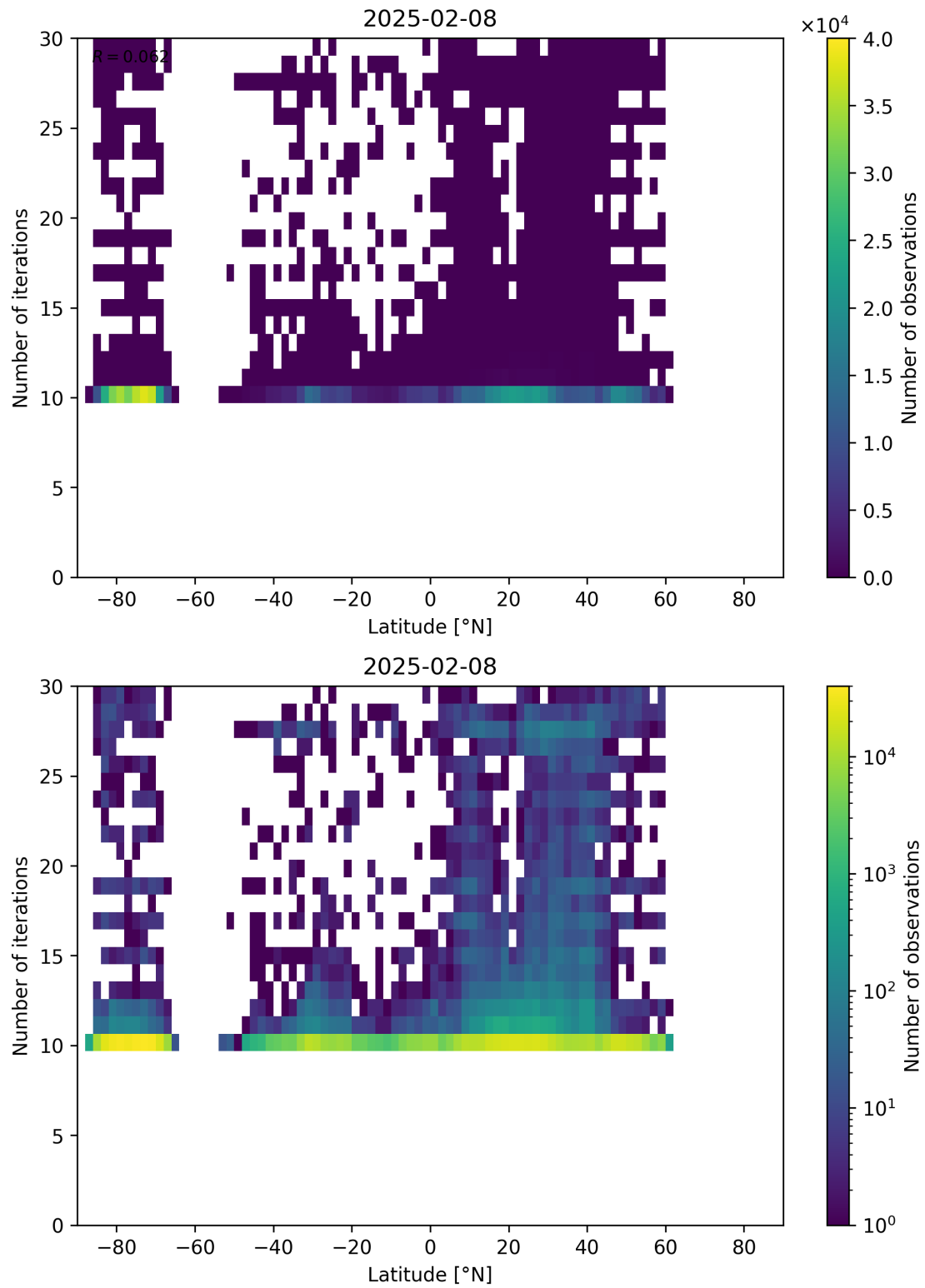
Figure 60: Scatter density plot of “Latitude” against “Number of iterations” for 2025-02-08 to 2025-02-09.
