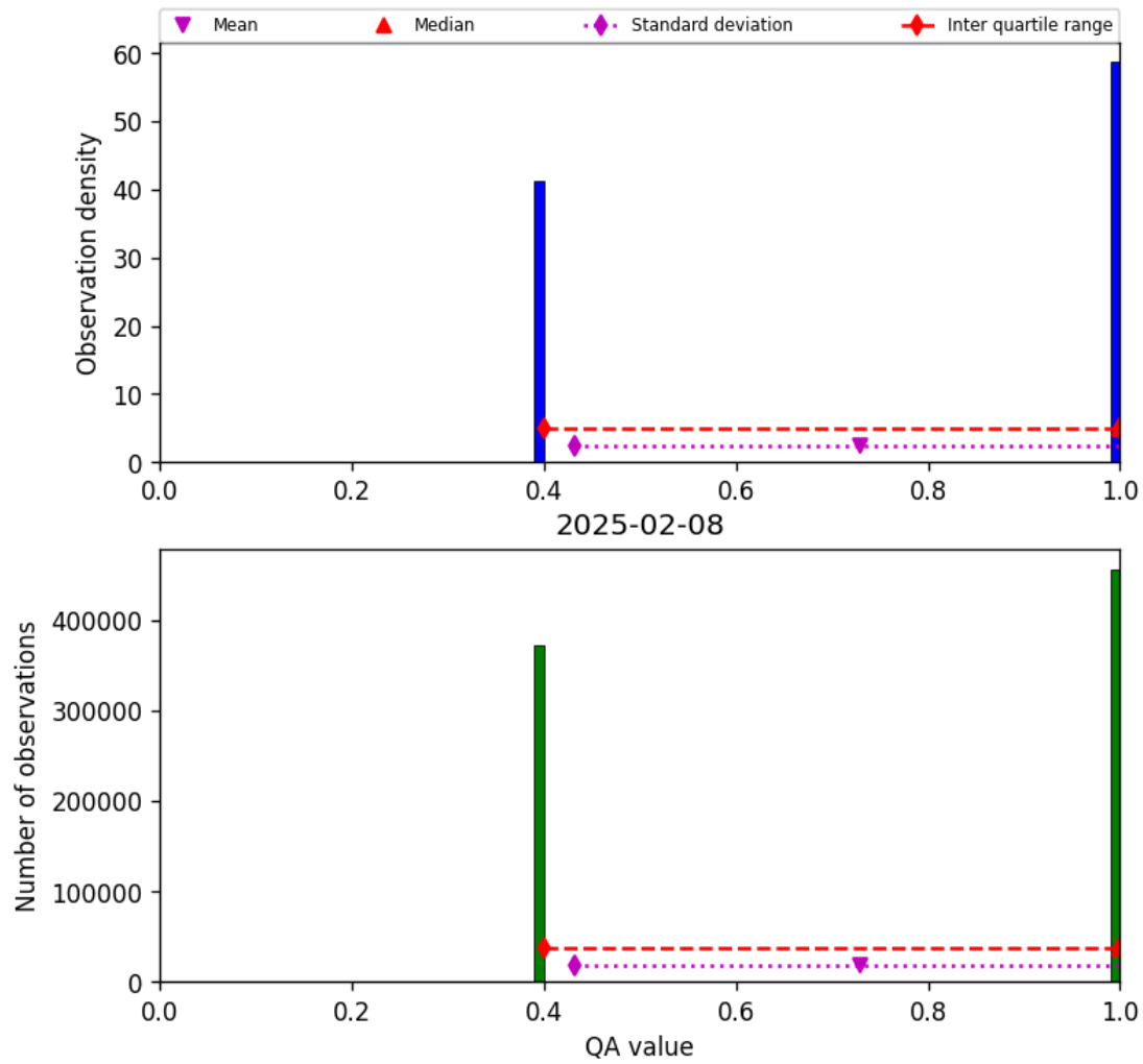
Figure 22: Histogram of “QA value” for 2025-02-08 to 2025-02-09
