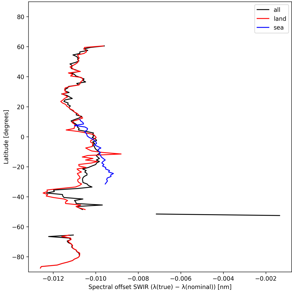
Figure 16: Zonal average of “Spectral offset SWIR ( \lambda_{\text{true}} - \lambda_{\text{nominal}} )” for 2025-02-08 to 2025-02-09.
