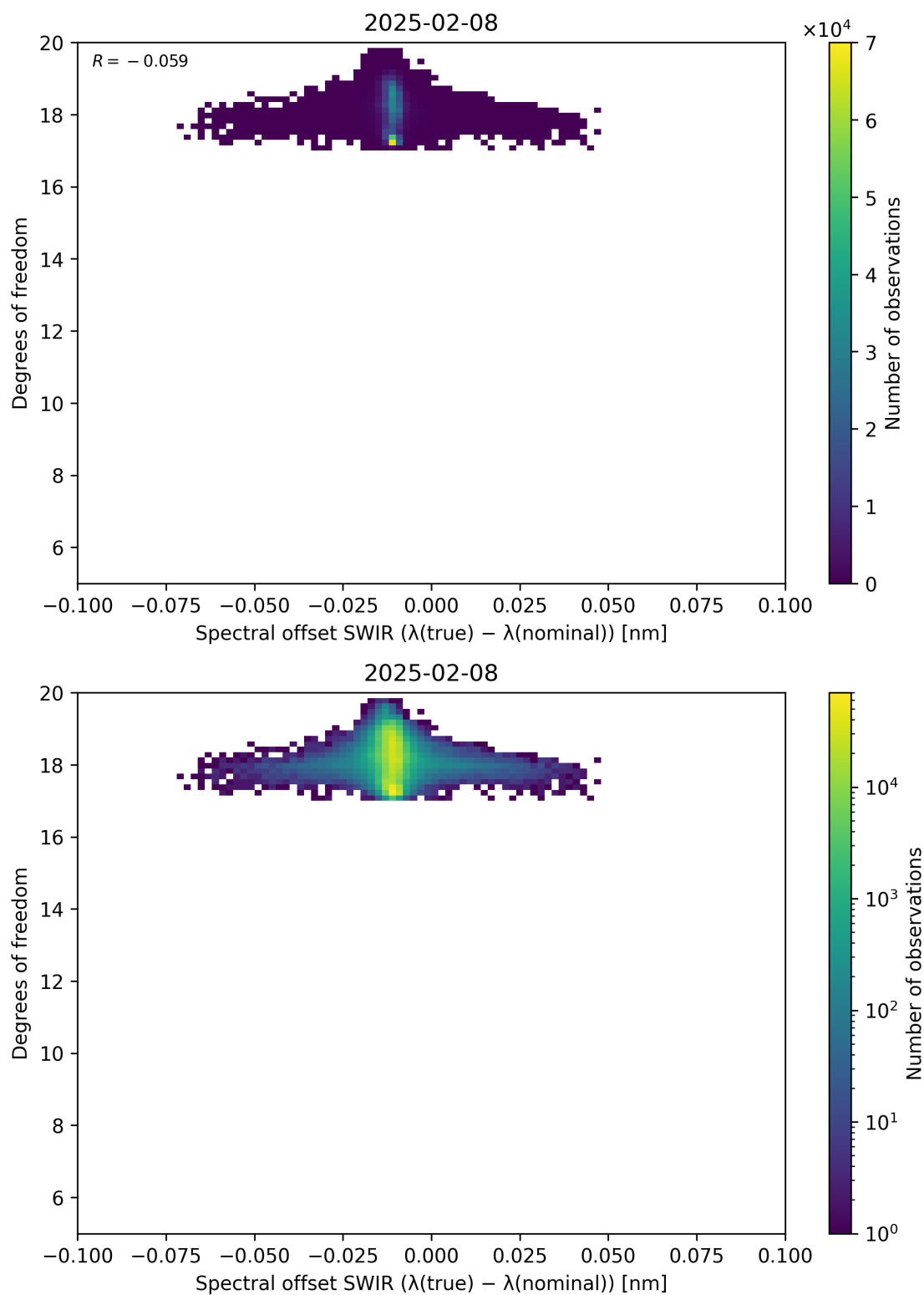
Figure 119: Scatter density plot of “Spectral offset SWIR ( \lambda_{\text{true}} - \lambda_{\text{nominal}} )” against “Degrees of freedom” for 2025-02-08 to 2025-02-09.
