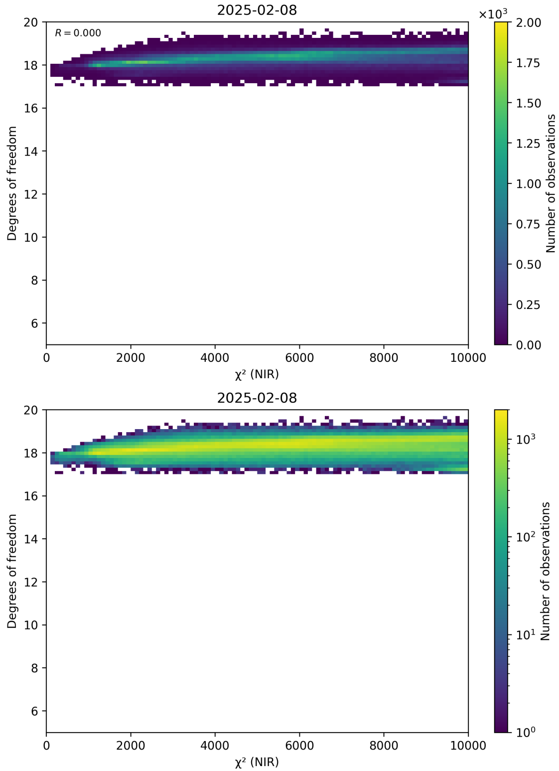
Figure 44: Scatter density plot of “ \chi^2 (NIR)” against “Degrees of freedom” for 2025-02-08 to 2025-02-09.
