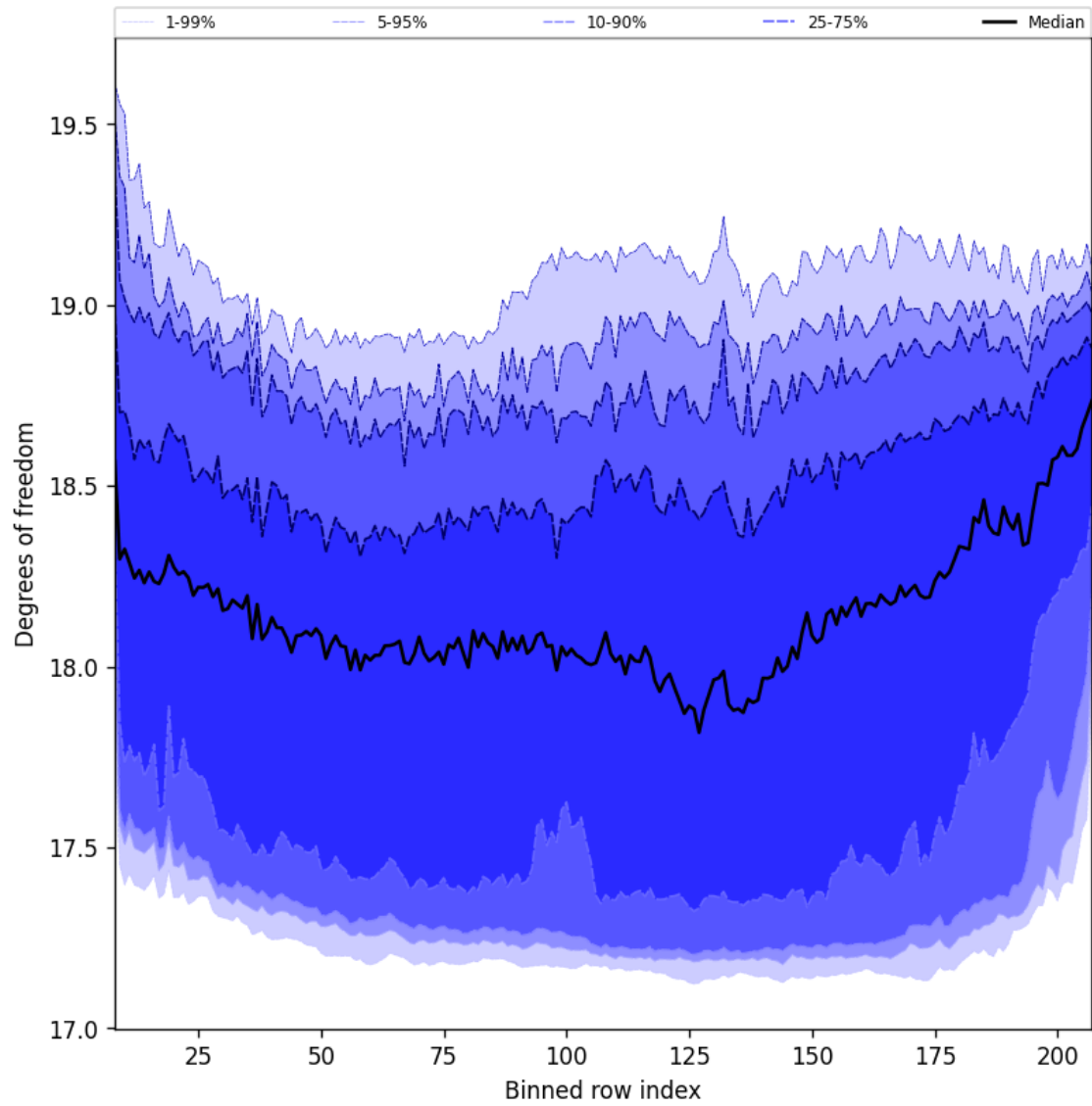
Figure 41: Along track statistics of “Degrees of freedom” for 2025-02-08 to 2025-02-09
