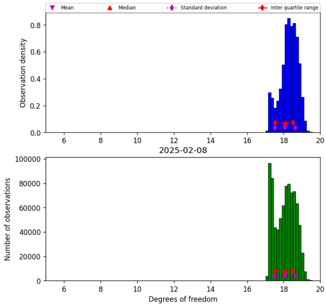
Figure 30: Histogram of “Degrees of freedom” for 2025-02-08 to 2025-02-09
