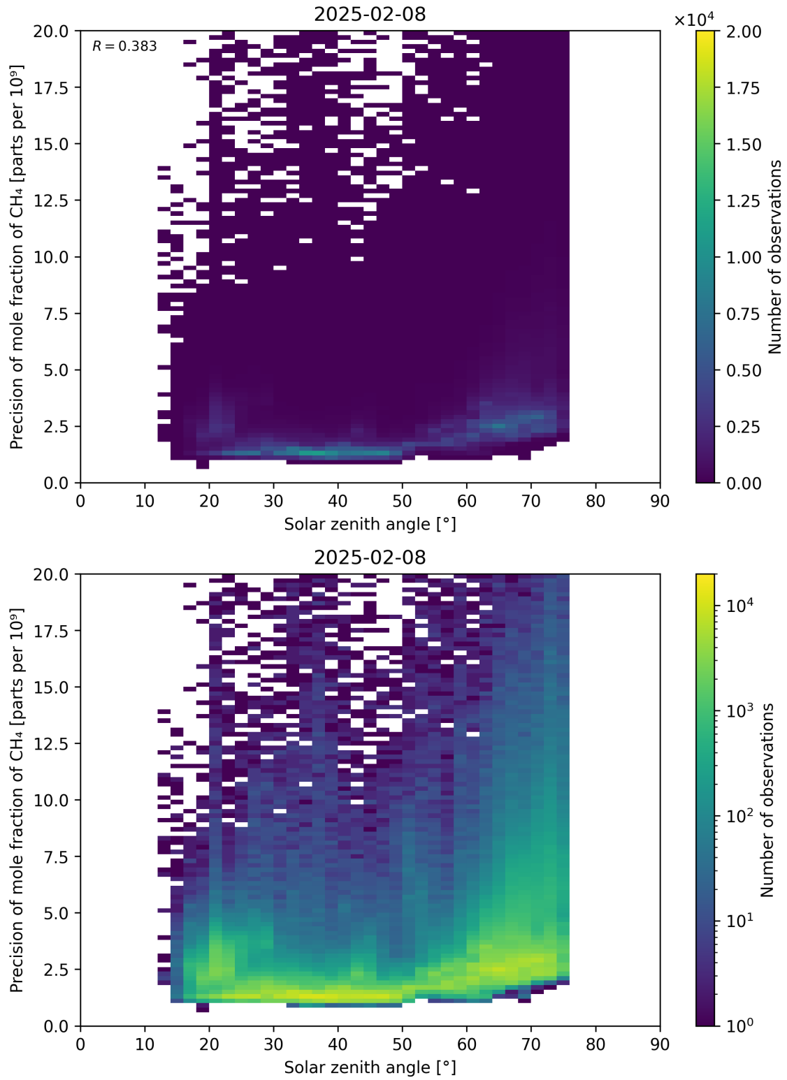
Figure 101: Scatter density plot of “Solar zenith angle” against “Precision of mole fraction of CH 4 ” for 2025-02-08 to 2025-02-09.
