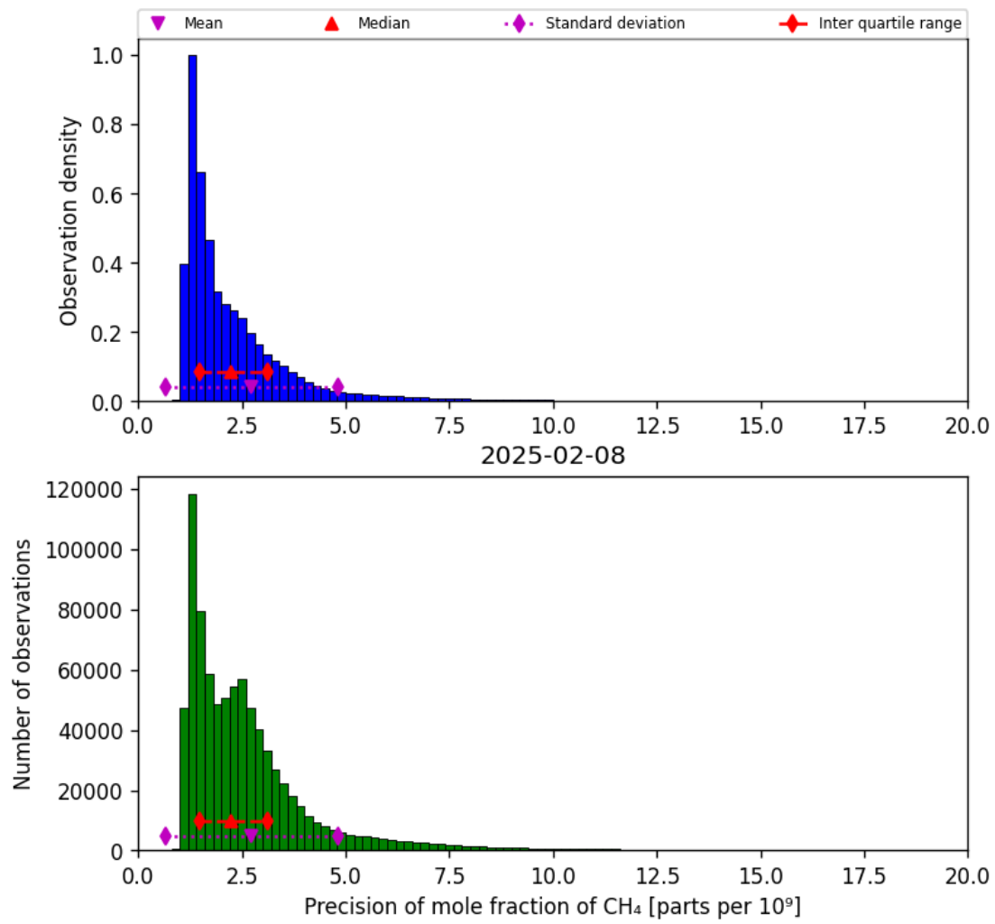
Figure 24: Histogram of “Precision of mole fraction of CH 4 ” for 2025-02-08 to 2025-02-09
