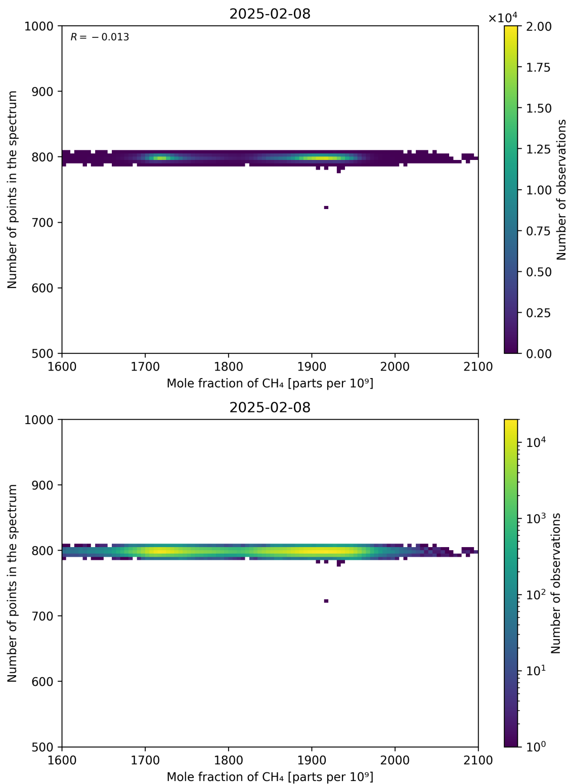
Figure 77: Scatter density plot of “Mole fraction of CH 4 ” against “Number of points in the spectrum” for 2025-02-08 to 2025-02-09.
