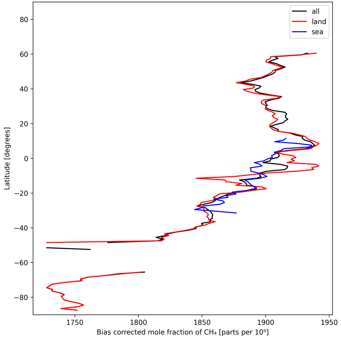
Figure 14: Zonal average of “Bias corrected mole fraction of CH 4 ” for 2025-02-08 to 2025-02-09.
