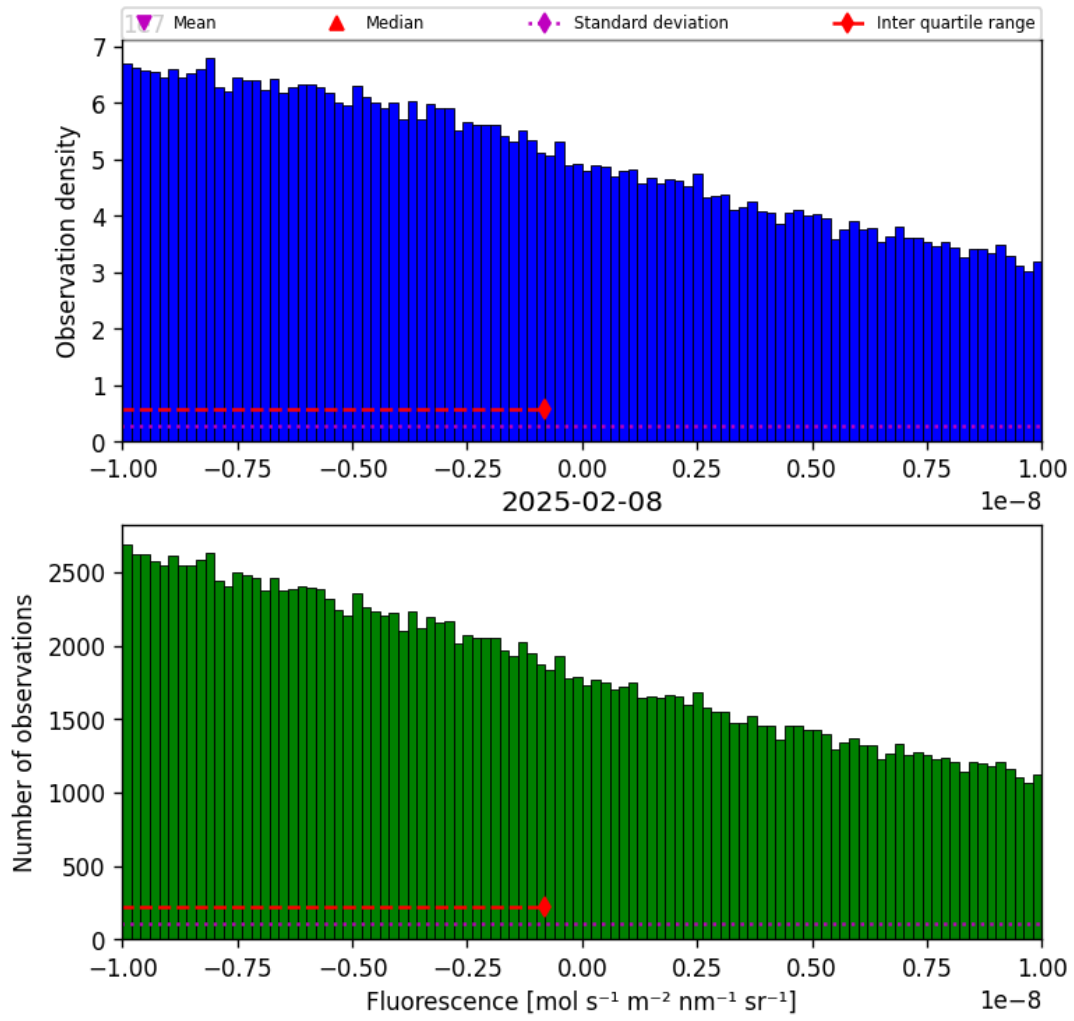
Figure 32: Histogram of “Fluorescence” for 2025-02-08 to 2025-02-09
