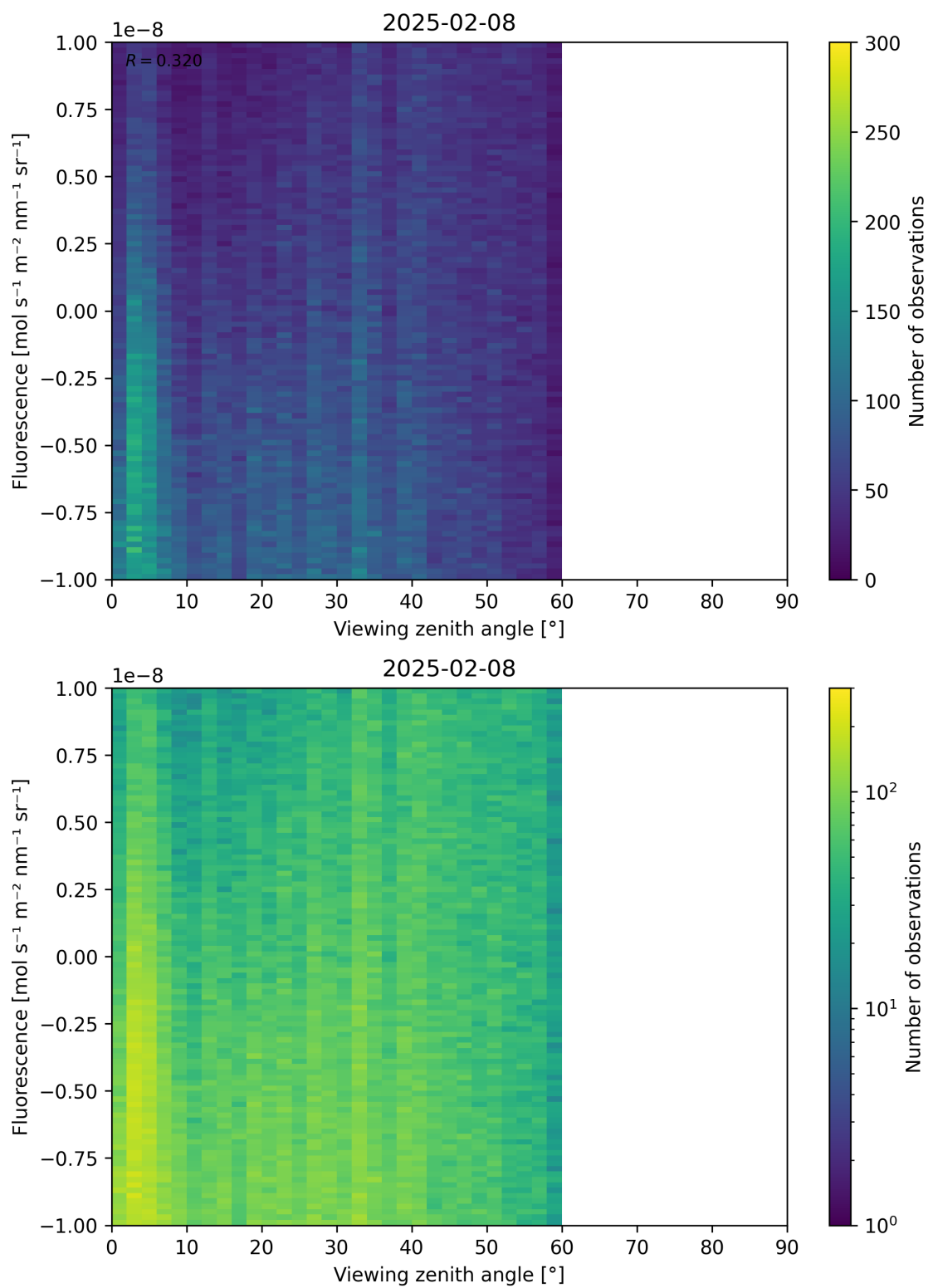
Figure 108: Scatter density plot of “Viewing zenith angle” against “Fluorescence” for 2025-02-08 to 2025-02-09.
