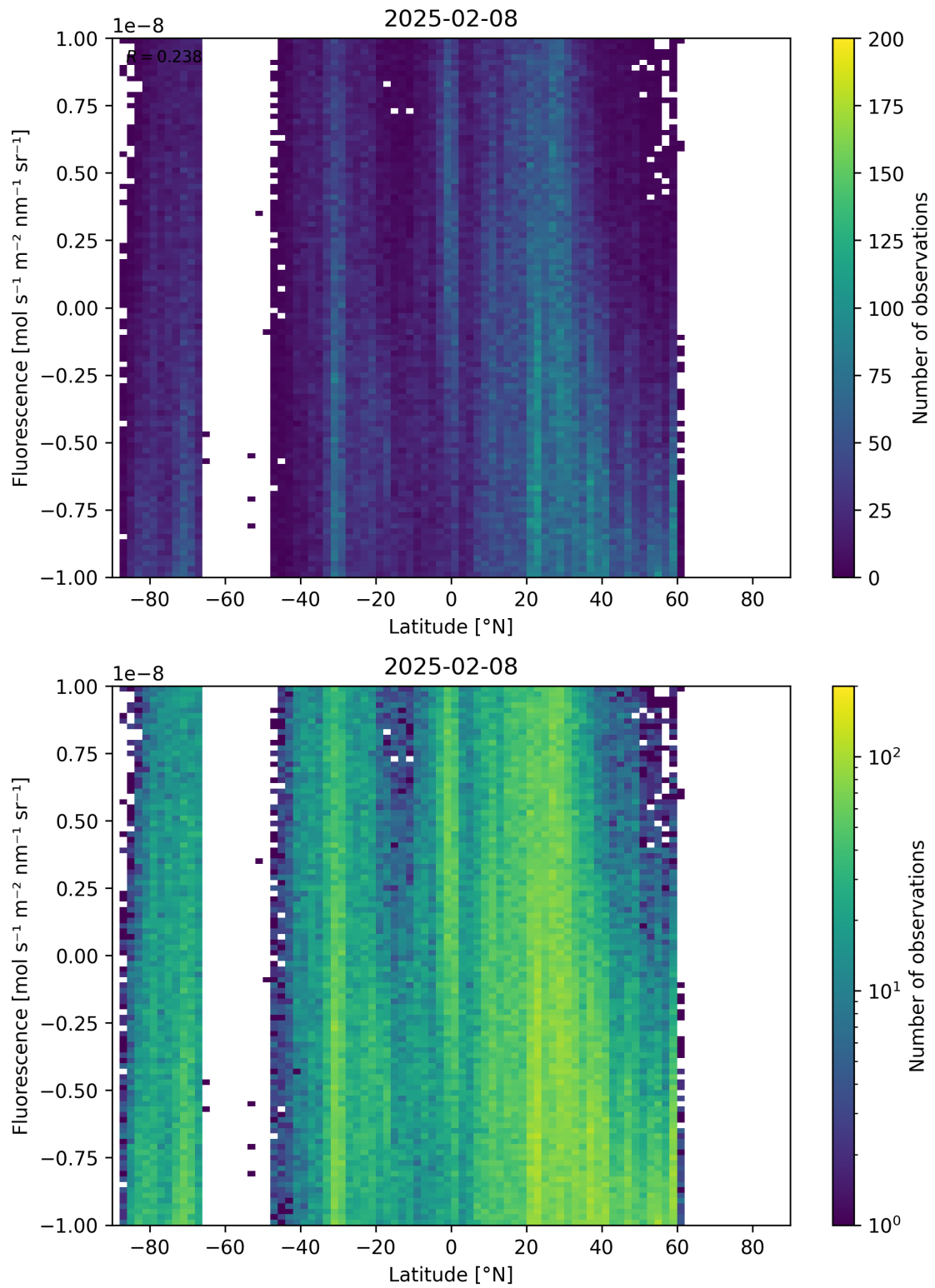
Figure 56: Scatter density plot of “Latitude” against “Fluorescence” for 2025-02-08 to 2025-02-09.
