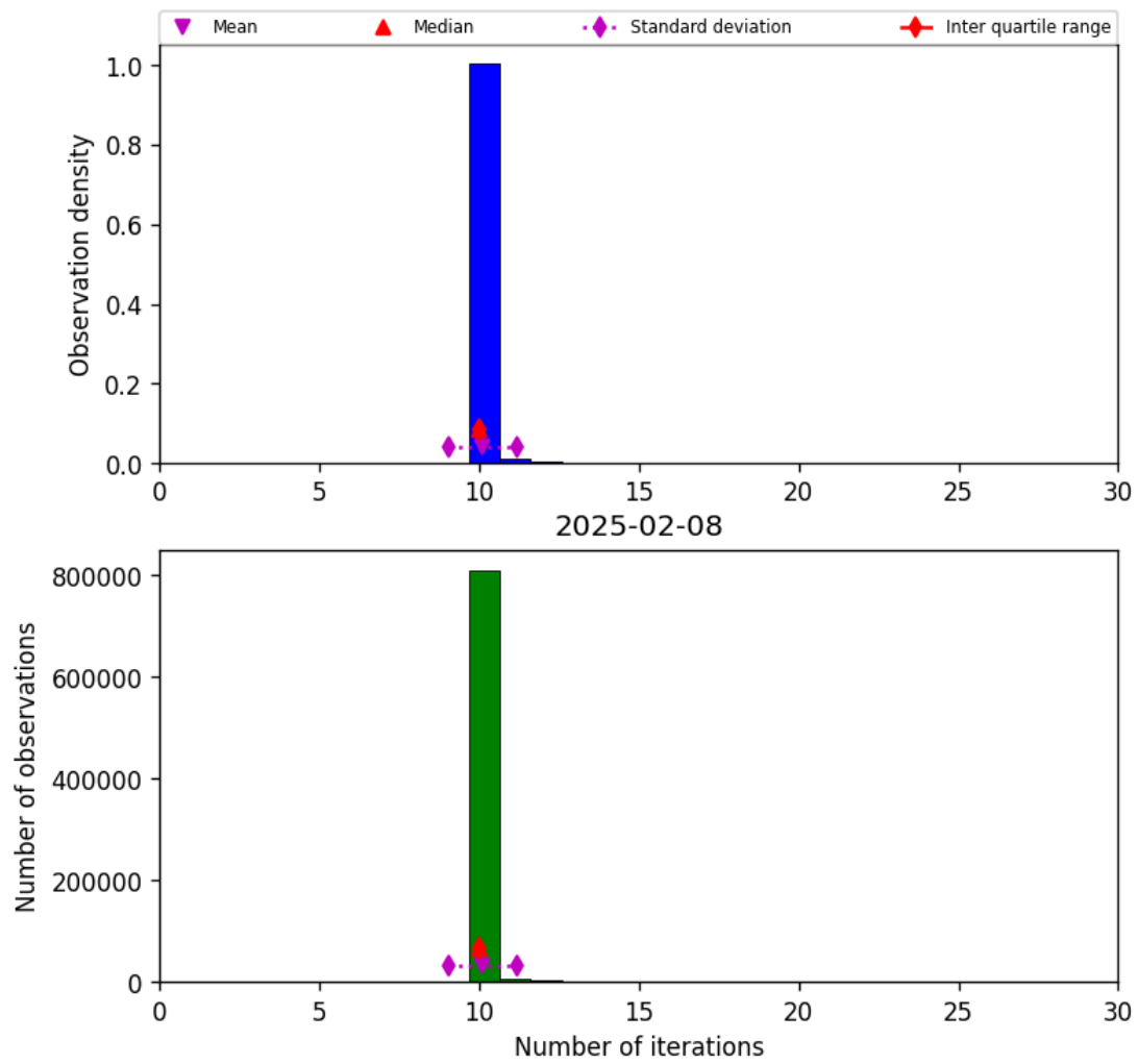
Figure 31: Histogram of “Number of iterations” for 2025-02-08 to 2025-02-09
