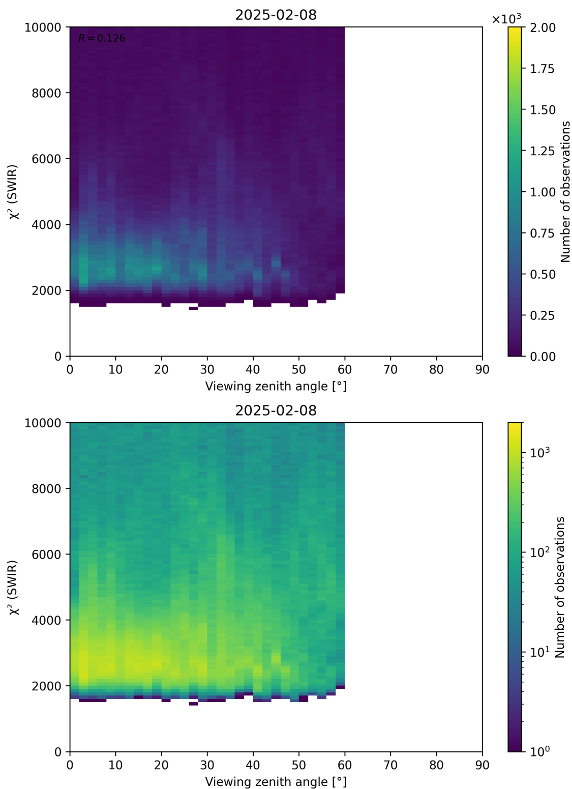
Figure 106: Scatter density plot of “Viewing zenith angle” against “ \chi^2 (SWIR)” for 2025-02-08 to 2025-02-09.
