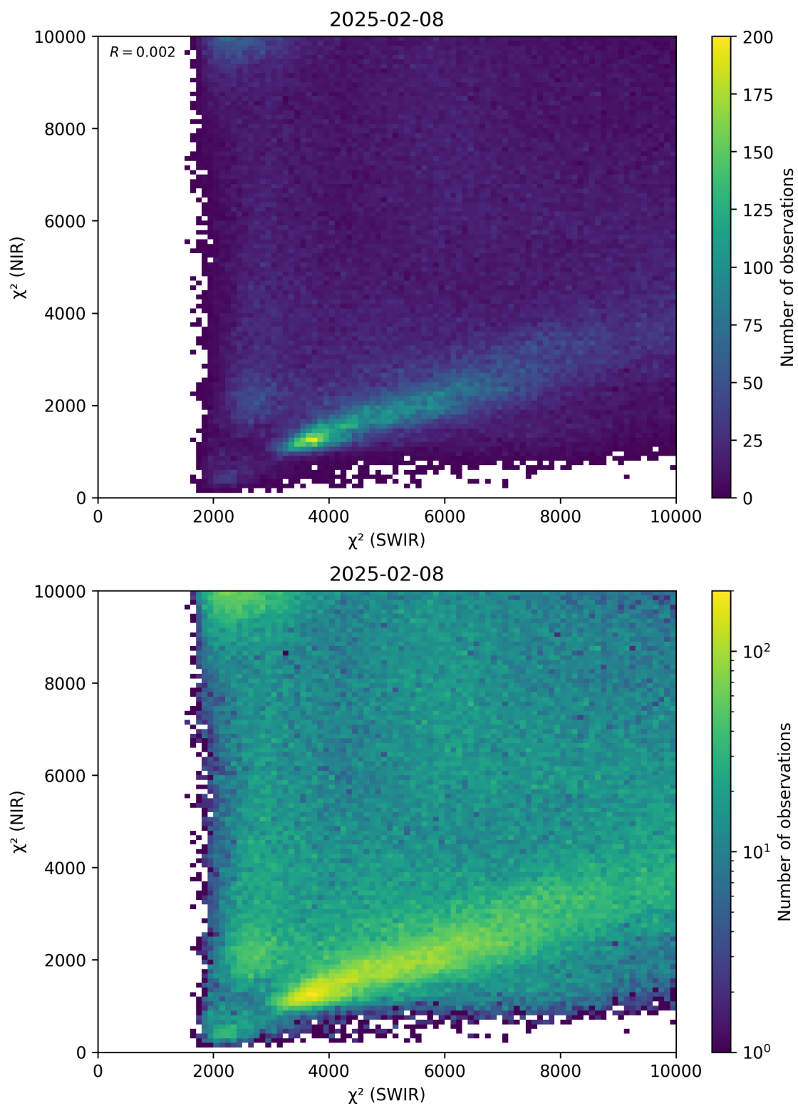
Figure 47: Scatter density plot of “ \chi^2 (SWIR)” against “ \chi^2 (NIR)” for 2025-02-08 to 2025-02-09.
