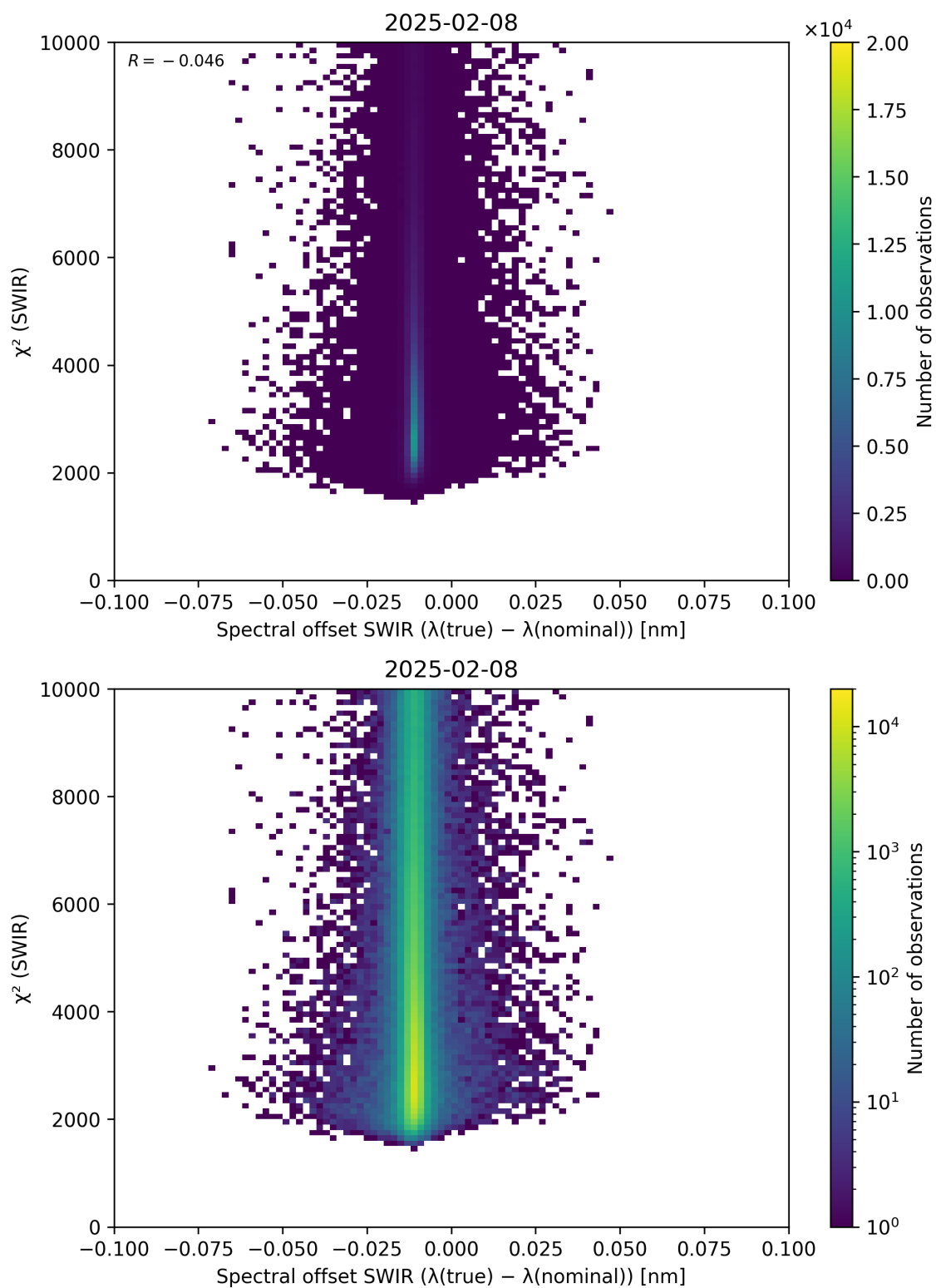
Figure 118: Scatter density plot of “Spectral offset SWIR ( \lambda_{\text{true}} - \lambda_{\text{nominal}} )” against “ \chi^2 (SWIR)” for 2025-02-08 to 2025-02-09.
