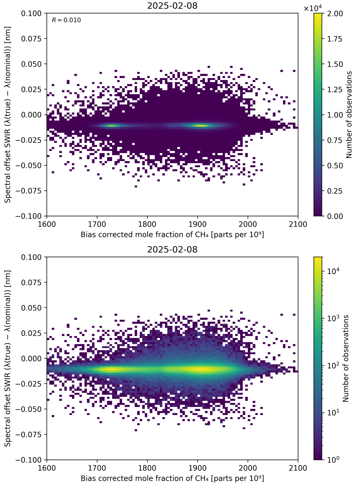
Figure 69: Scatter density plot of “Bias corrected mole fraction of \text{CH}_4 ” against “Spectral offset SWIR ( \lambda_{\text{true}} - \lambda_{\text{nominal}} )” for 2025-02-08 to 2025-02-09.
