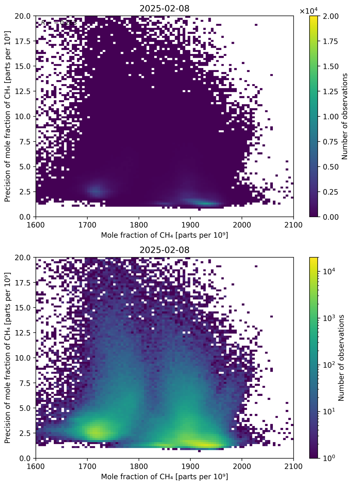
Figure 75: Scatter density plot of “Mole fraction of CH 4 ” against “Precision of mole fraction of CH 4 ” for 2025-02-08 to 2025-02-09.
