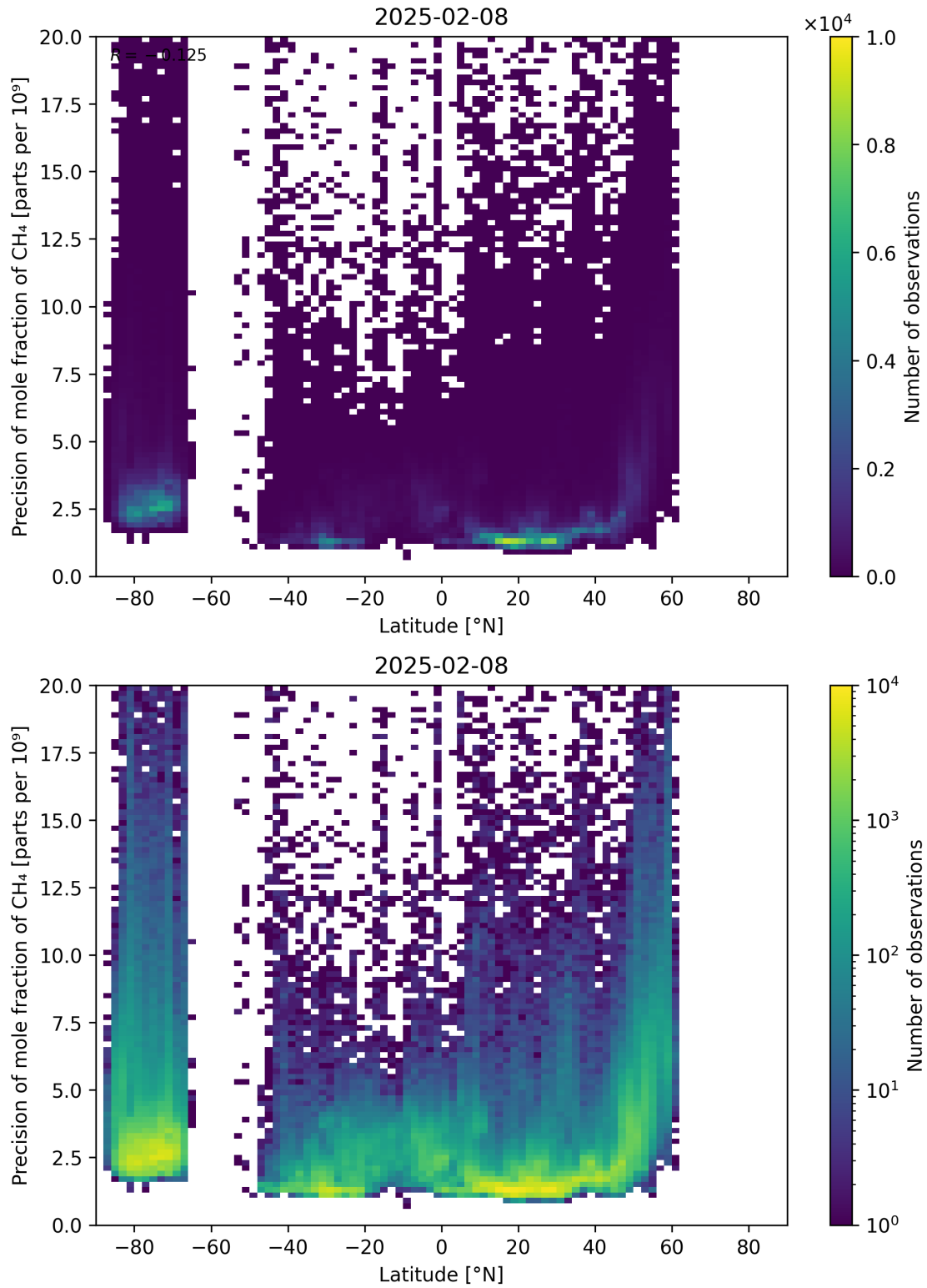
Figure 59: Scatter density plot of “Latitude” against “Precision of mole fraction of \text{CH}_4 ” for 2025-02-08 to 2025-02-09.
