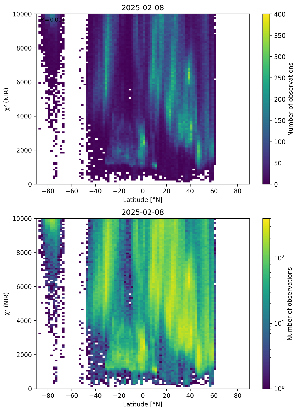
Figure 53: Scatter density plot of “Latitude” against “ \chi^2 (NIR)” for 2025-02-08 to 2025-02-09.
