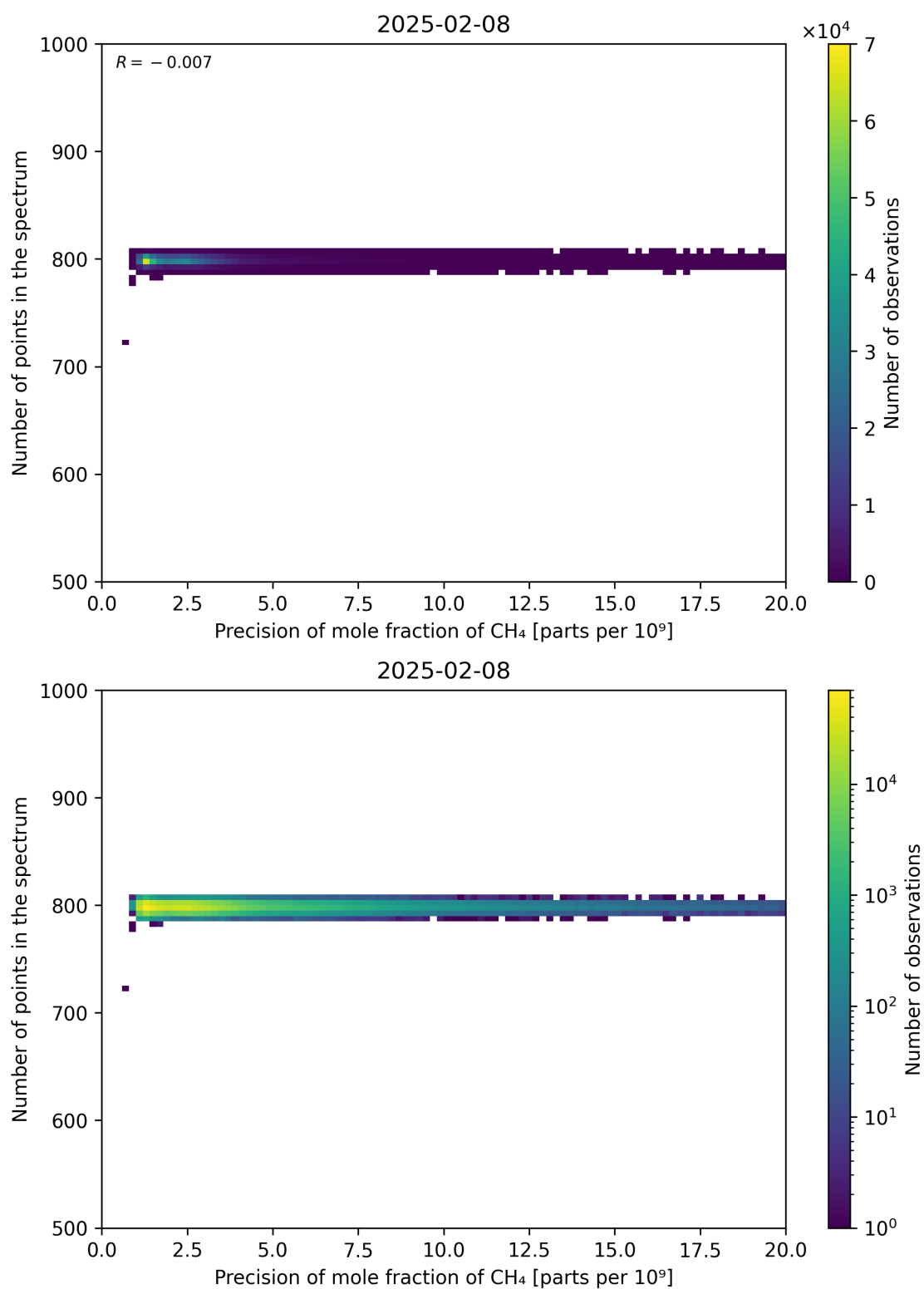
Figure 84: Scatter density plot of “Precision of mole fraction of CH 4 ” against “Number of points in the spectrum” for 2025-02-08 to 2025-02-09.
