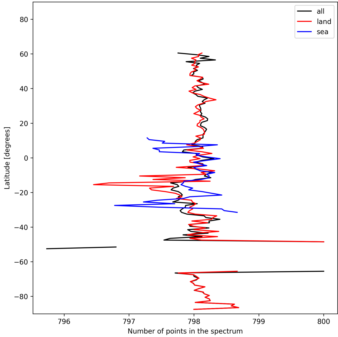
Figure 15: Zonal average of “Number of points in the spectrum” for 2025-02-08 to 2025-02-09.
