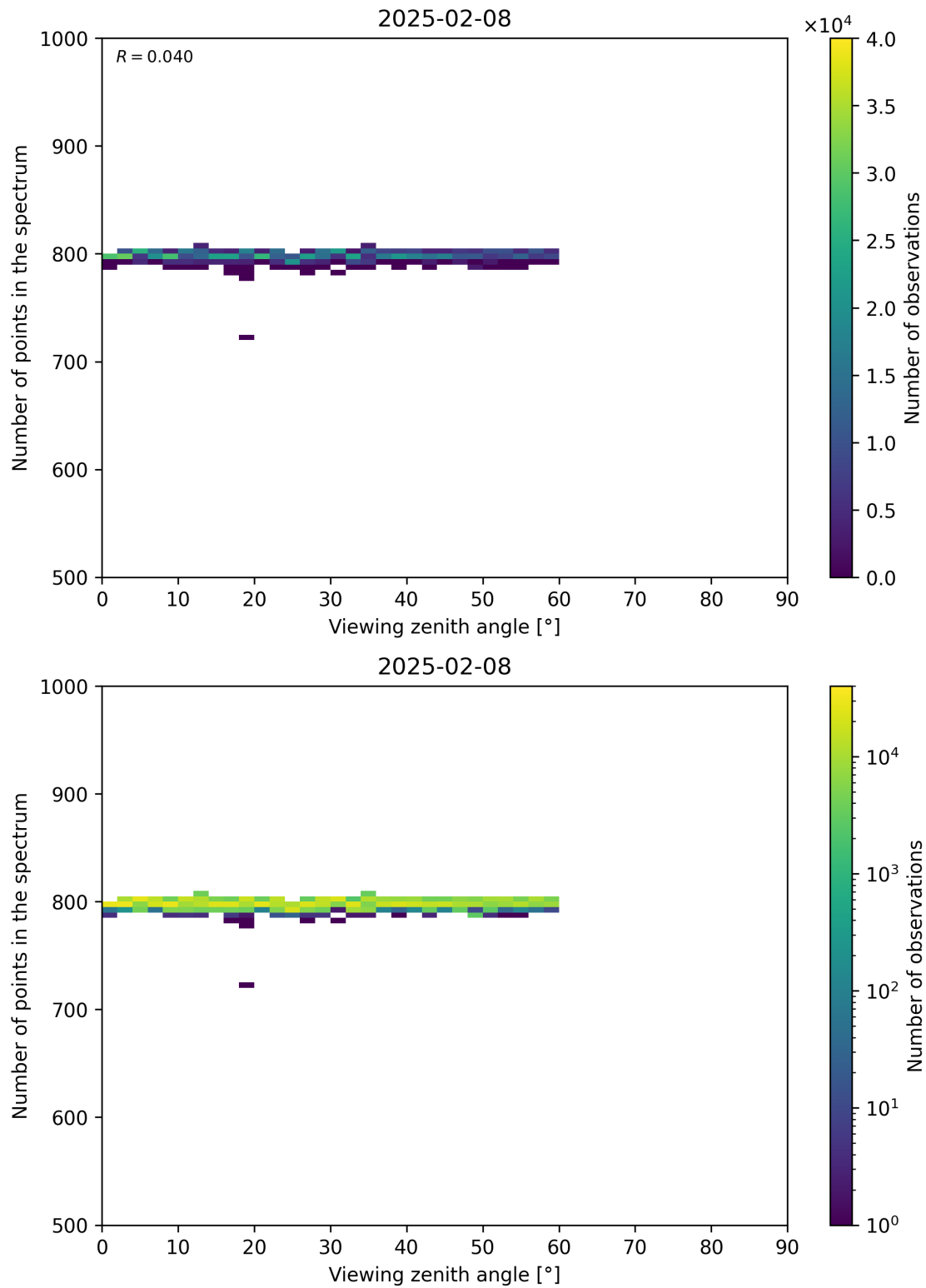
Figure 114: Scatter density plot of “Viewing zenith angle” against “Number of points in the spectrum” for 2025-02-08 to 2025-02-09.
