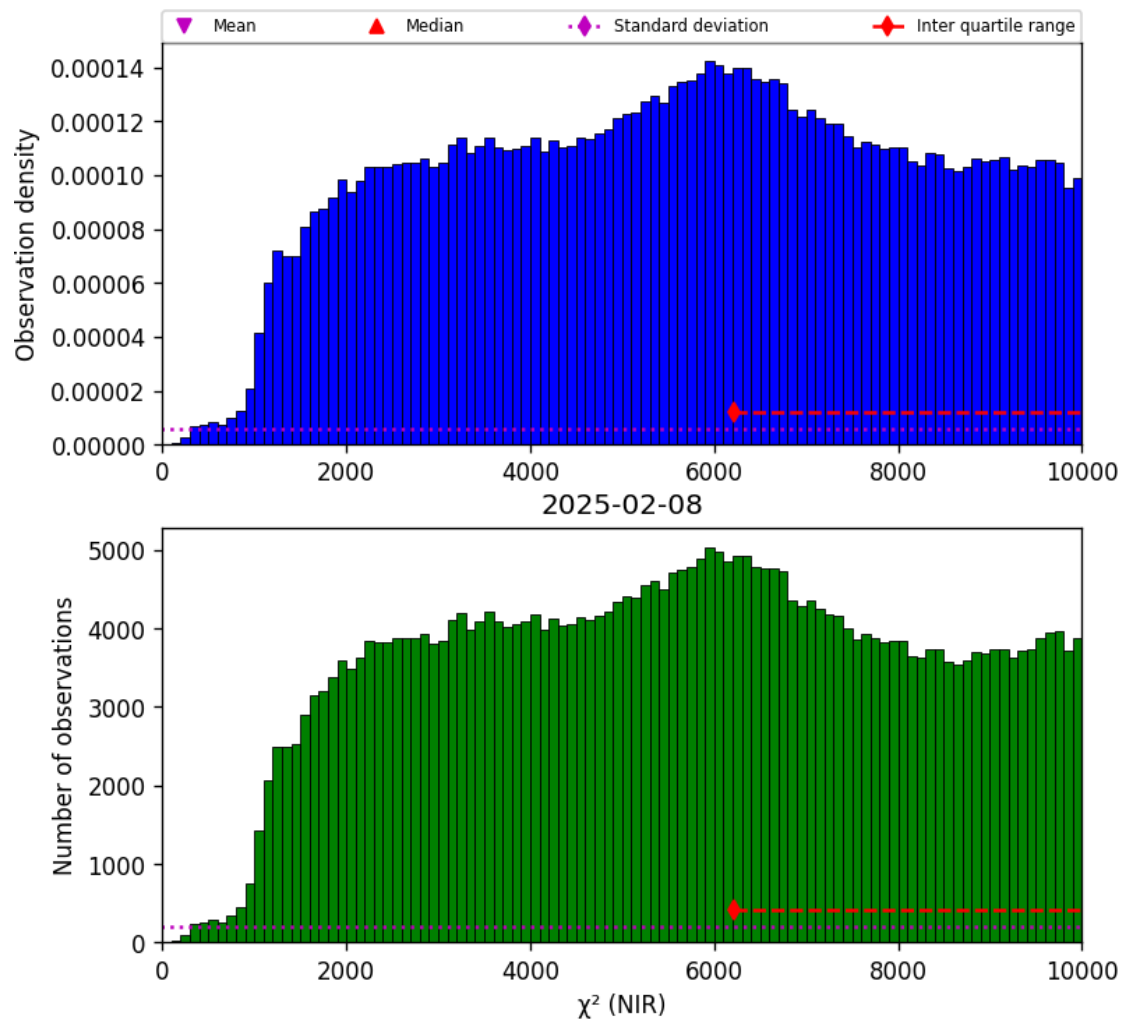
Figure 29: Histogram of “ \chi^2 (NIR)” for 2025-02-08 to 2025-02-09
