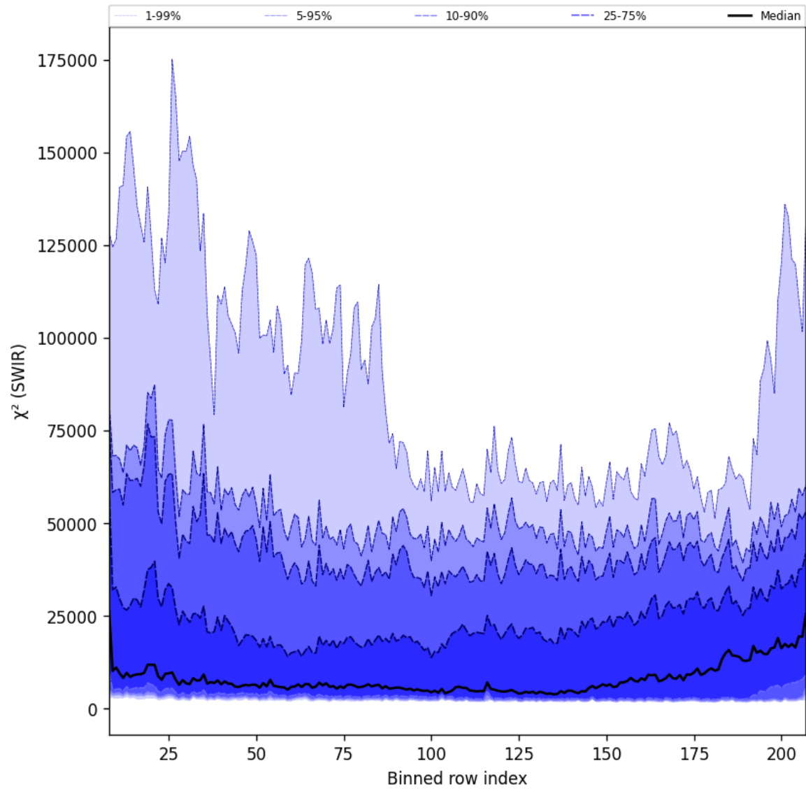
Figure 39: Along track statistics of “ \chi^2 (SWIR)” for 2025-02-08 to 2025-02-09
