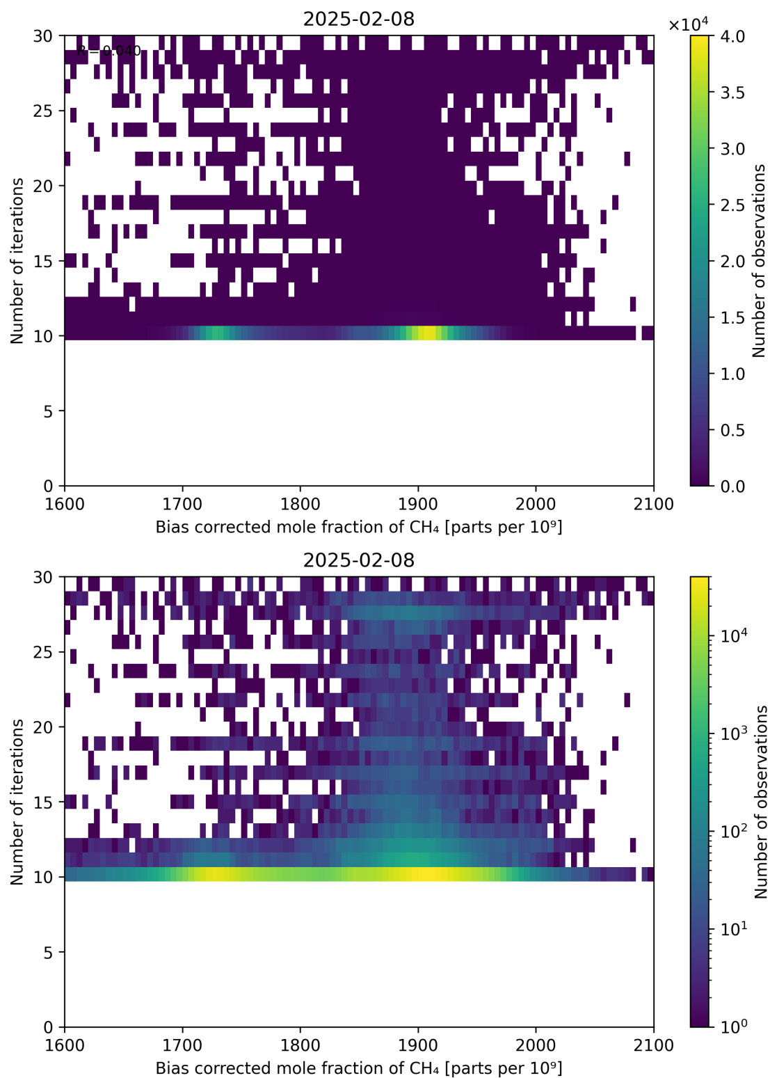
Figure 67: Scatter density plot of “Bias corrected mole fraction of \text{CH}_4 ” against “Number of iterations” for 2025-02-08 to 2025-02-09.
