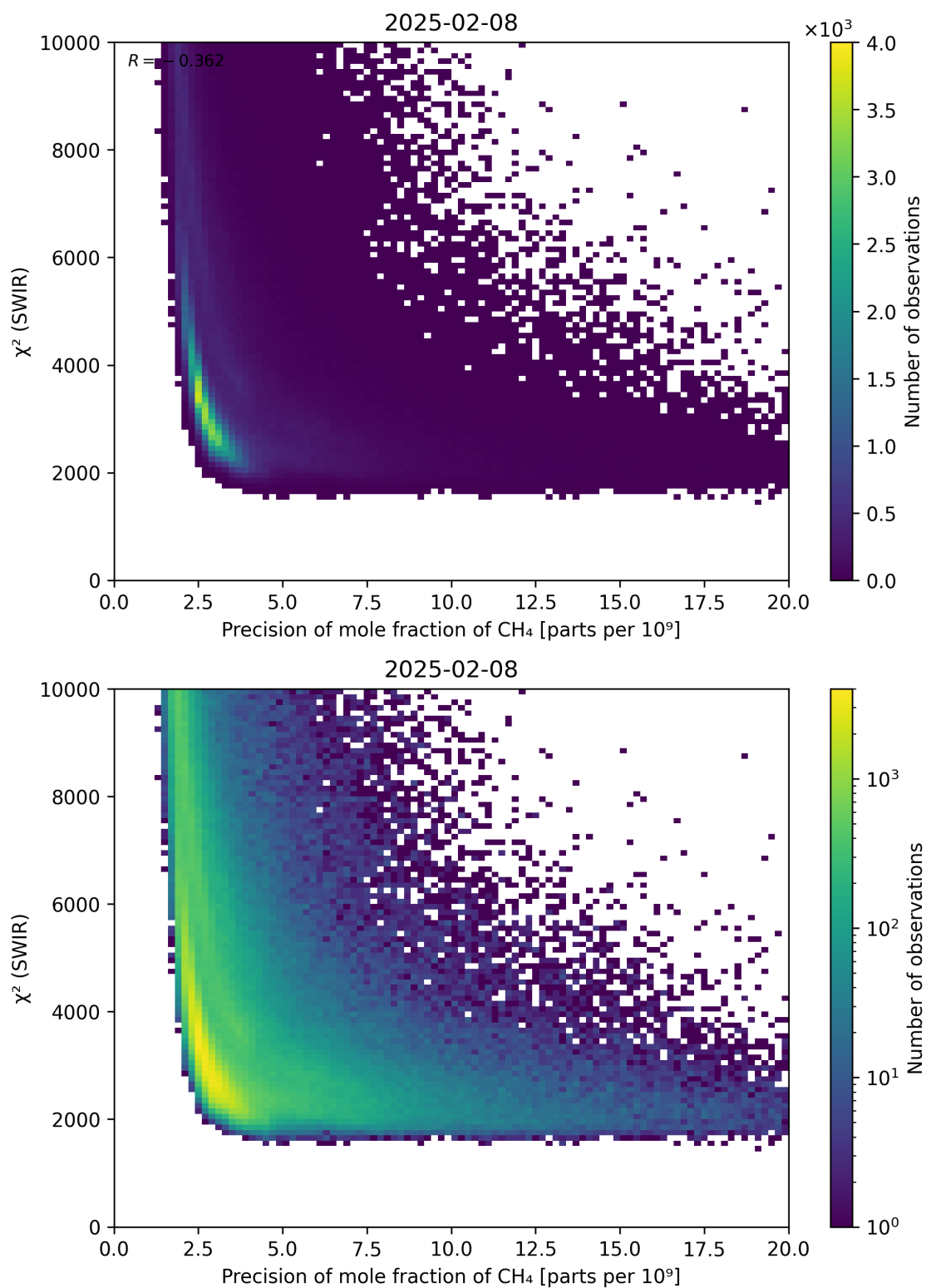
Figure 79: Scatter density plot of “Precision of mole fraction of \text{CH}_4 ” against “ \chi^2 (SWIR)” for 2025-02-08 to 2025-02-09.
