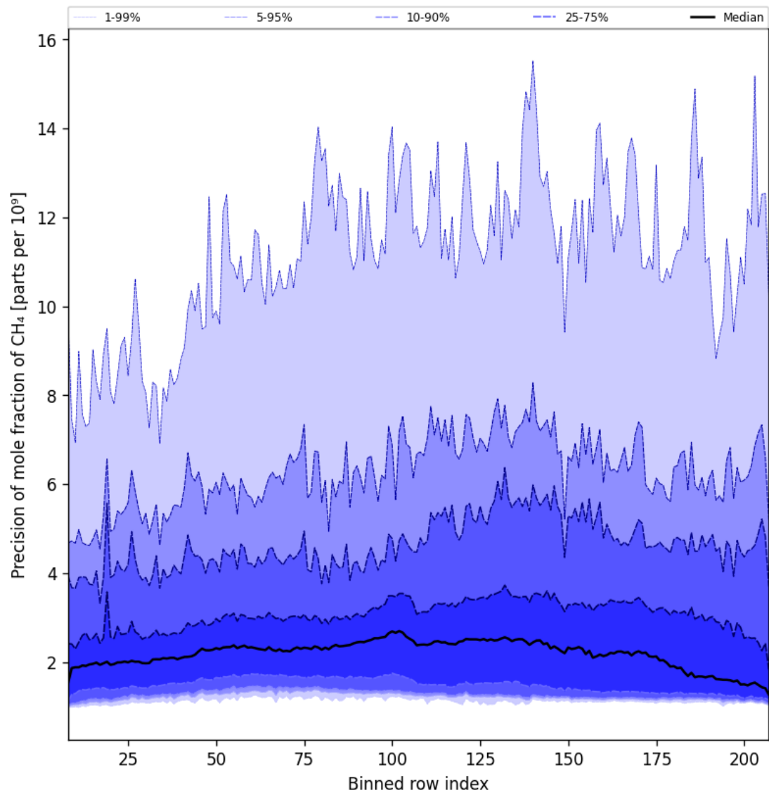
Figure 35: Along track statistics of “Precision of mole fraction of CH 4 ” for 2025-02-08 to 2025-02-09
