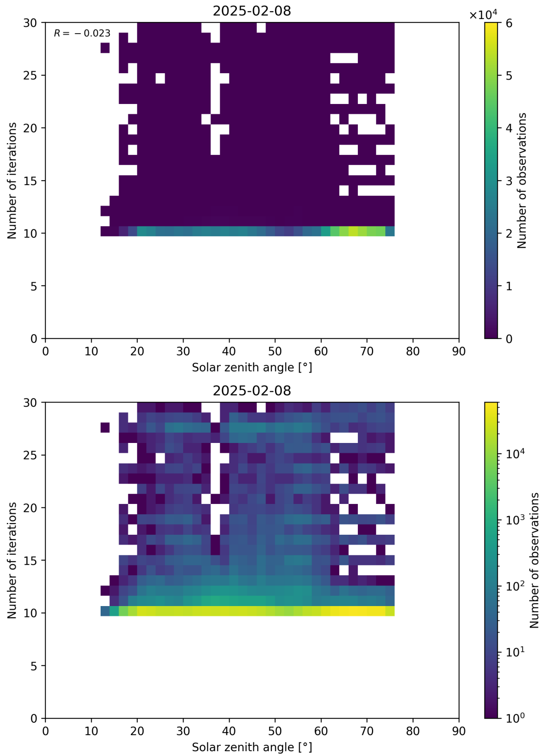
Figure 102: Scatter density plot of “Solar zenith angle” against “Number of iterations” for 2025-02-08 to 2025-02-09.
