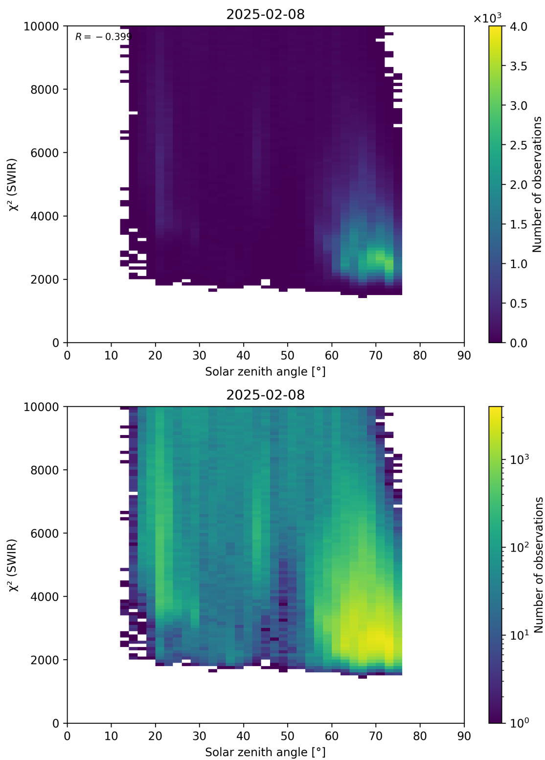
Figure 95: Scatter density plot of “Solar zenith angle” against “ \chi^2 (SWIR)” for 2025-02-08 to 2025-02-09.
