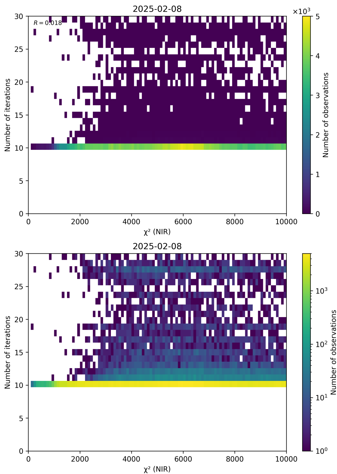
Figure 46: Scatter density plot of “ \chi^2 (NIR)” against “Number of iterations” for 2025-02-08 to 2025-02-09.
