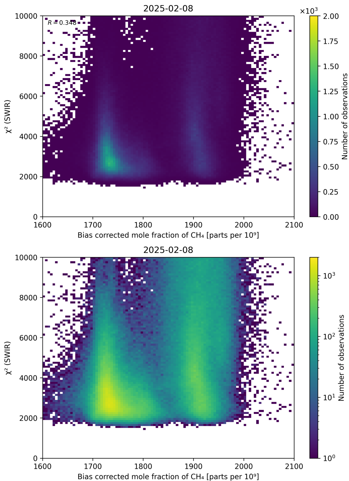
Figure 64: Scatter density plot of “Bias corrected mole fraction of \text{CH}_4 ” against “ \chi^2 (SWIR)” for 2025-02-08 to 2025-02-09.
