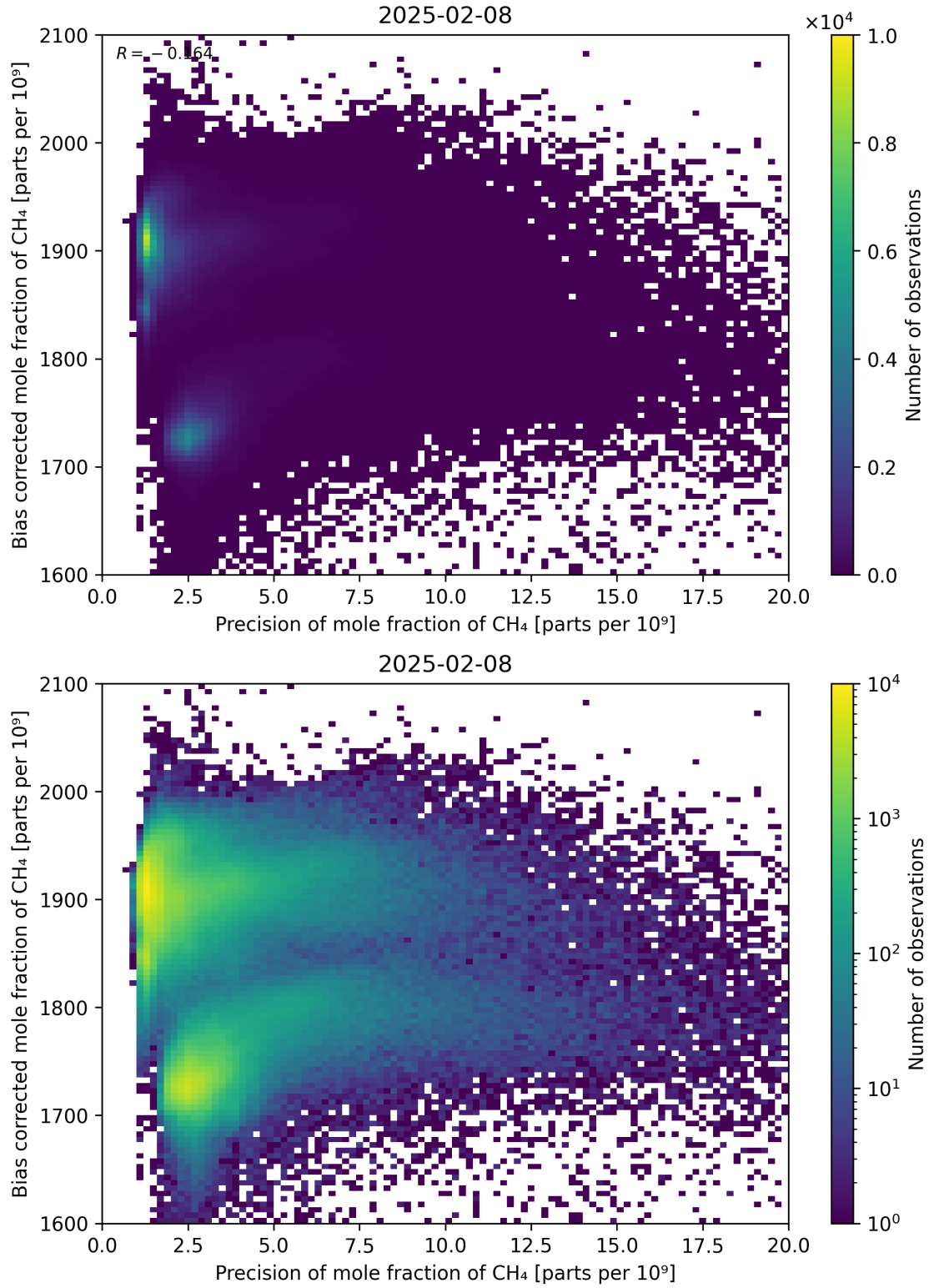
Figure 82: Scatter density plot of “Precision of mole fraction of CH 4 ” against “Bias corrected mole fraction of CH 4 ” for 2025-02-08 to 2025-02-09.
