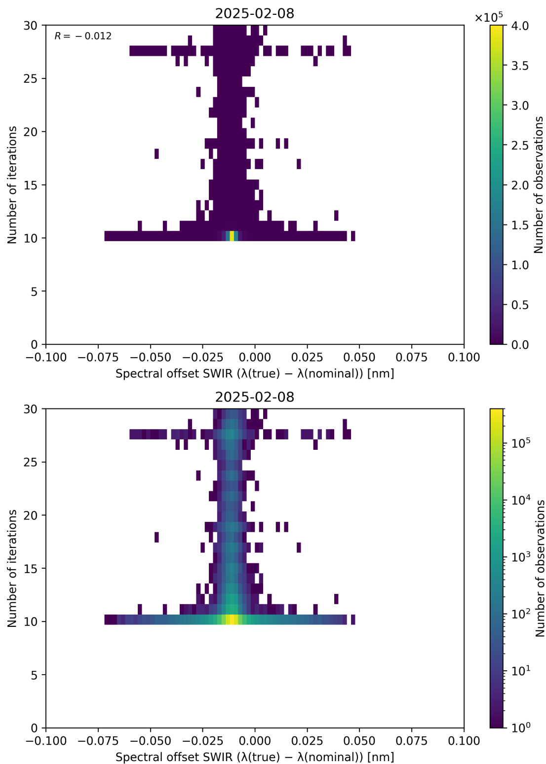
Figure 121: Scatter density plot of “Spectral offset SWIR ( \lambda_{\text{true}} - \lambda_{\text{nominal}} )” against “Number of iterations” for 2025-02-08 to 2025-02-09.
