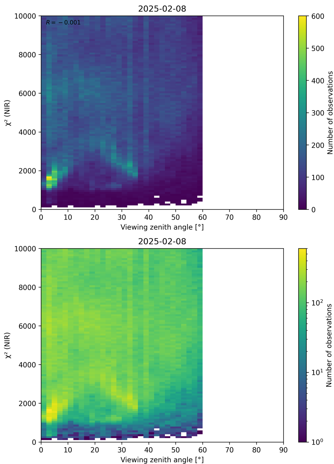
Figure 105: Scatter density plot of “Viewing zenith angle” against “ \chi^2 (NIR)” for 2025-02-08 to 2025-02-09.
