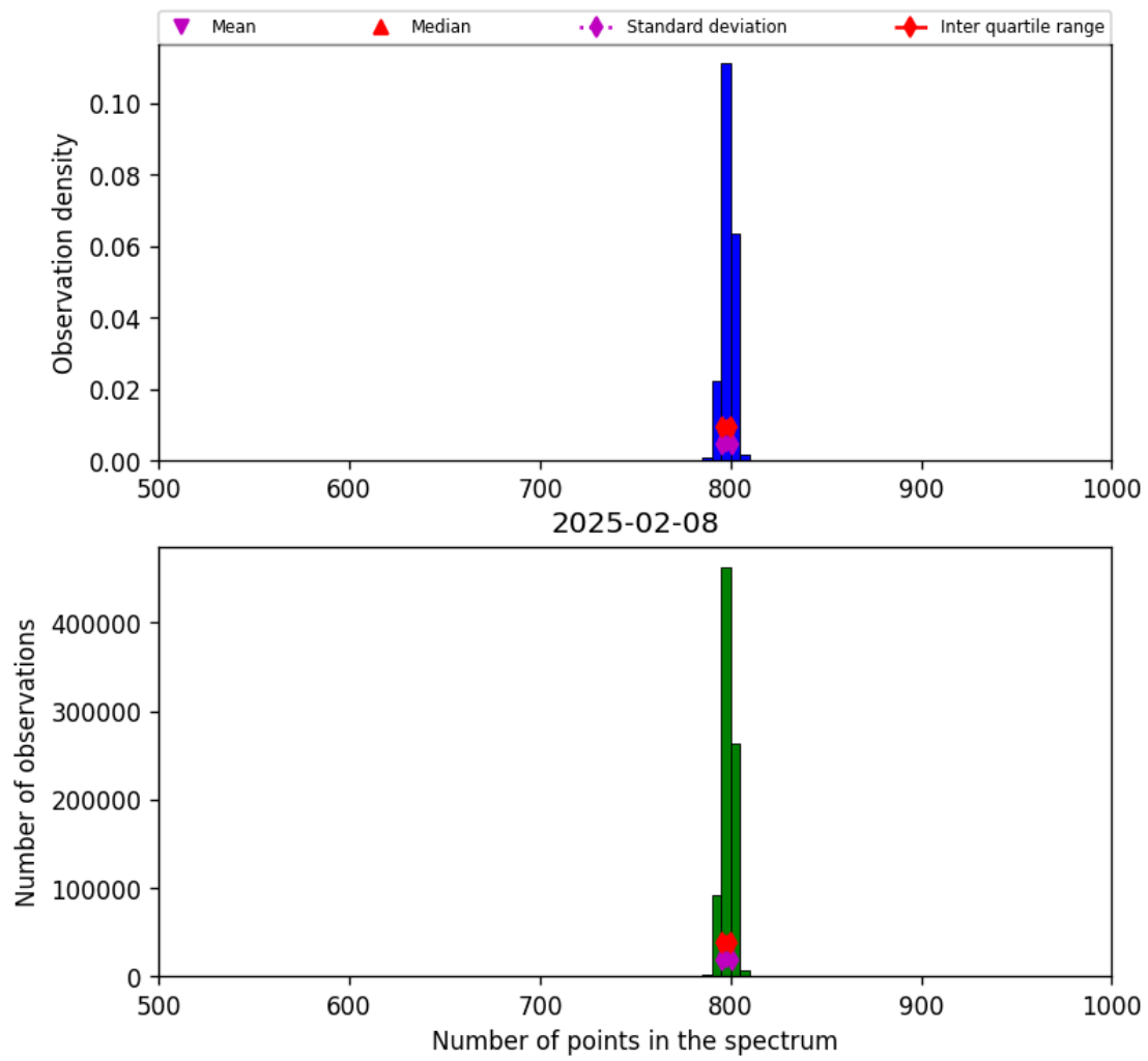
Figure 26: Histogram of “Number of points in the spectrum” for 2025-02-08 to 2025-02-09
