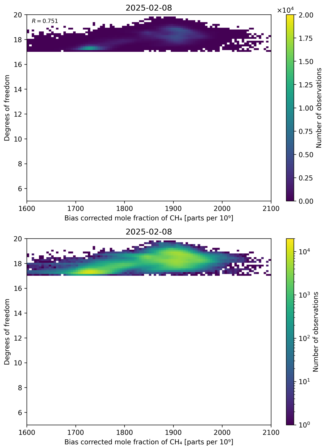
Figure 65: Scatter density plot of “Bias corrected mole fraction of CH 4 ” against “Degrees of freedom” for 2025-02-08 to 2025-02-09.
