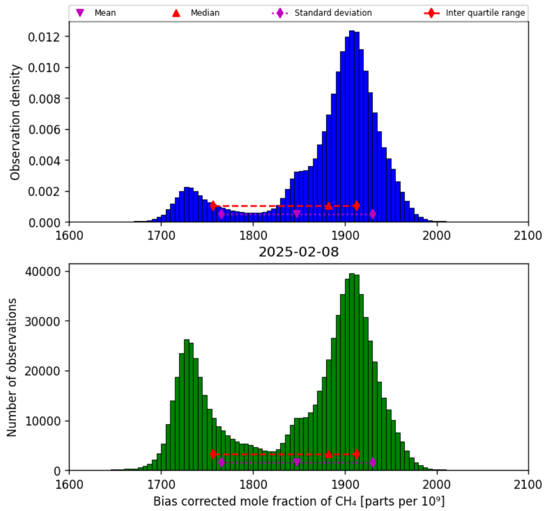
Figure 25: Histogram of “Bias corrected mole fraction of CH 4 ” for 2025-02-08 to 2025-02-09
