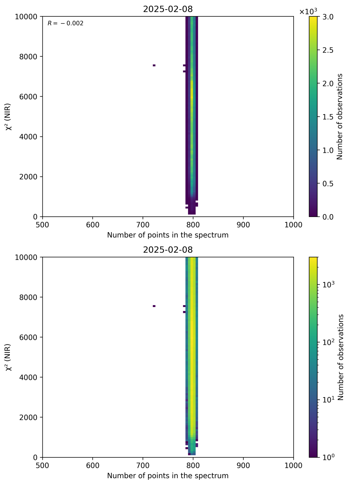
Figure 88: Scatter density plot of “Number of points in the spectrum” against “ \chi^2 (NIR)” for 2025-02-08 to 2025-02-09.
