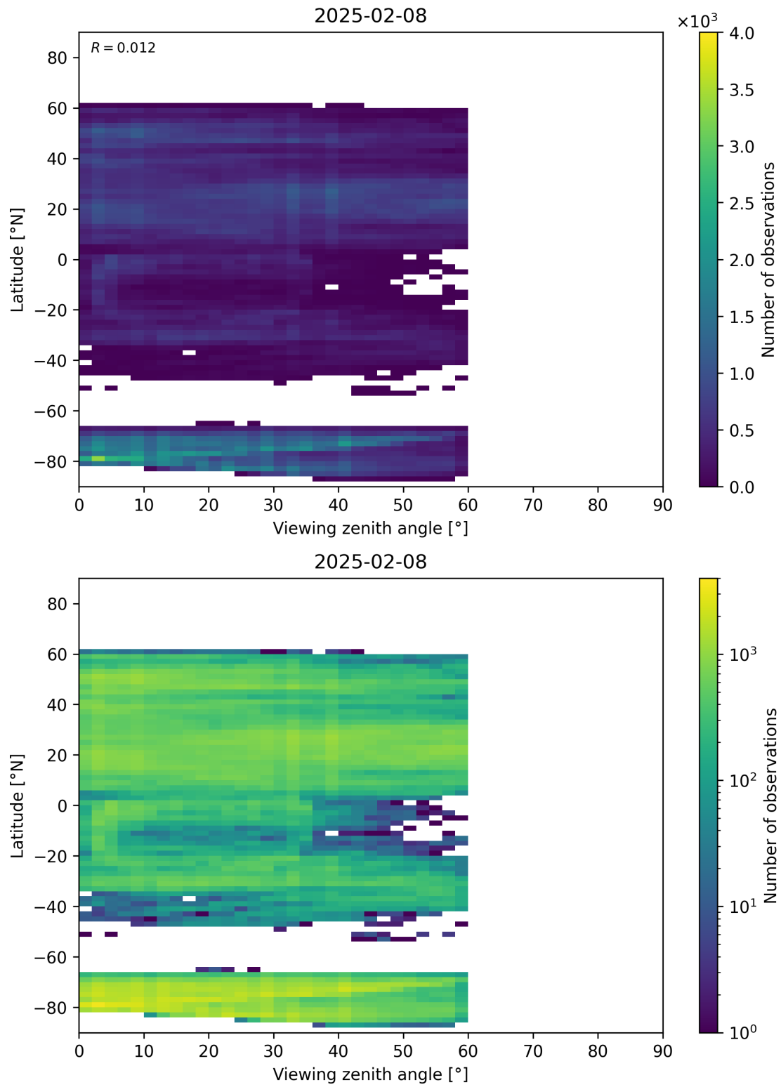
Figure 109: Scatter density plot of “Viewing zenith angle” against “Latitude” for 2025-02-08 to 2025-02-09.
