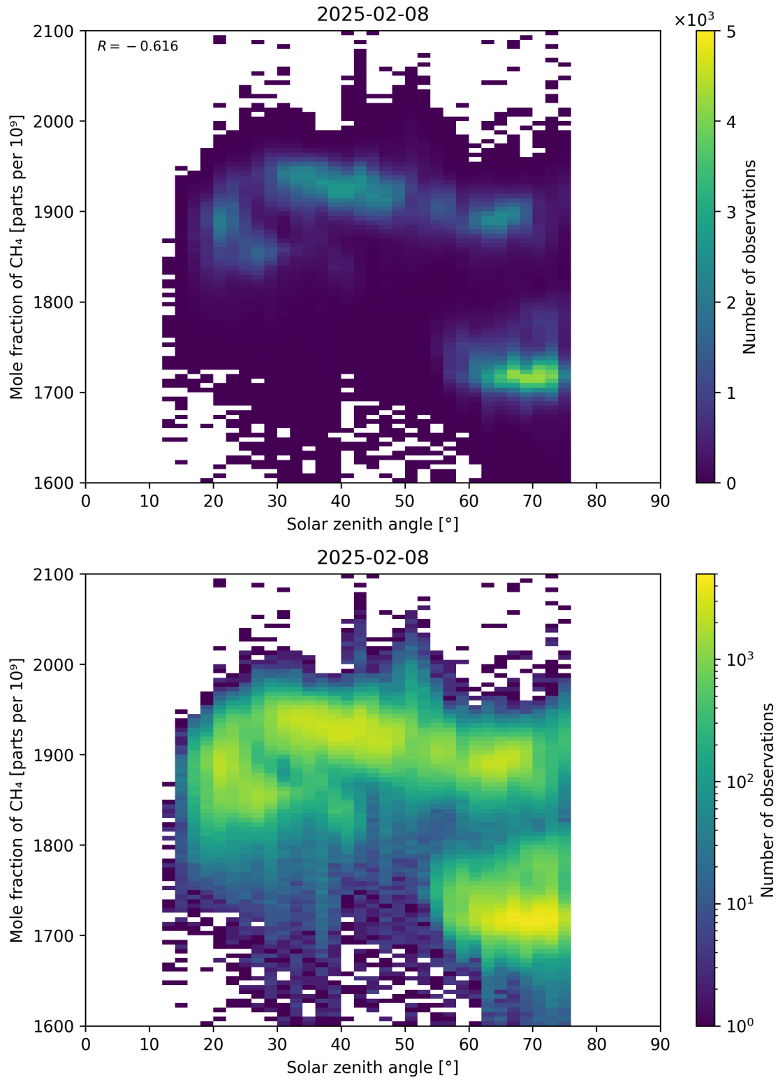
Figure 99: Scatter density plot of “Solar zenith angle” against “Mole fraction of CH 4 ” for 2025-02-08 to 2025-02-09.
