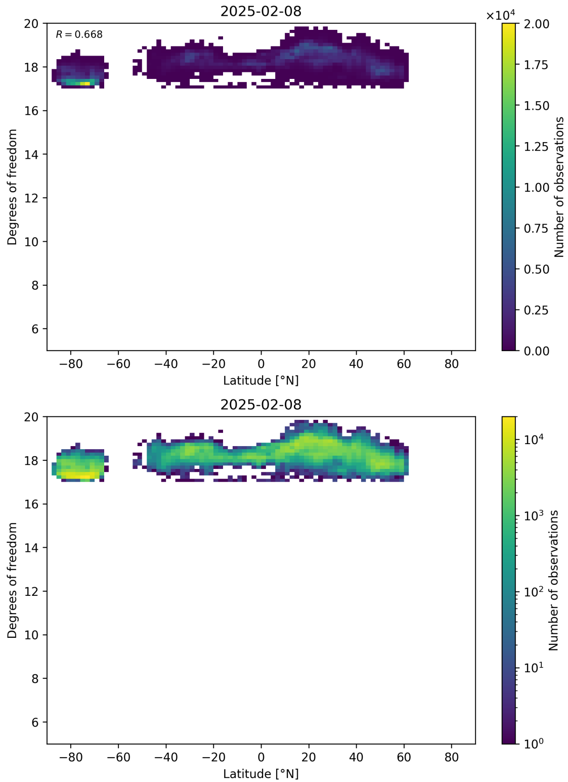
Figure 55: Scatter density plot of “Latitude” against “Degrees of freedom” for 2025-02-08 to 2025-02-09.
