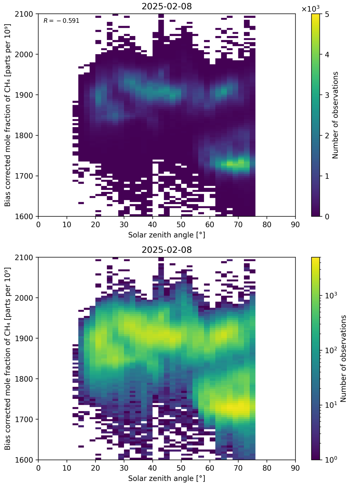
Figure 100: Scatter density plot of “Solar zenith angle” against “Bias corrected mole fraction of CH 4 ” for 2025-02-08 to 2025-02-09.
