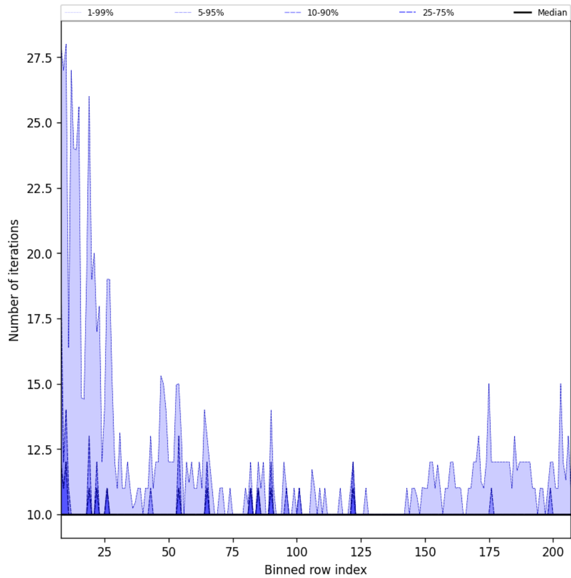
Figure 42: Along track statistics of “Number of iterations” for 2025-02-08 to 2025-02-09
