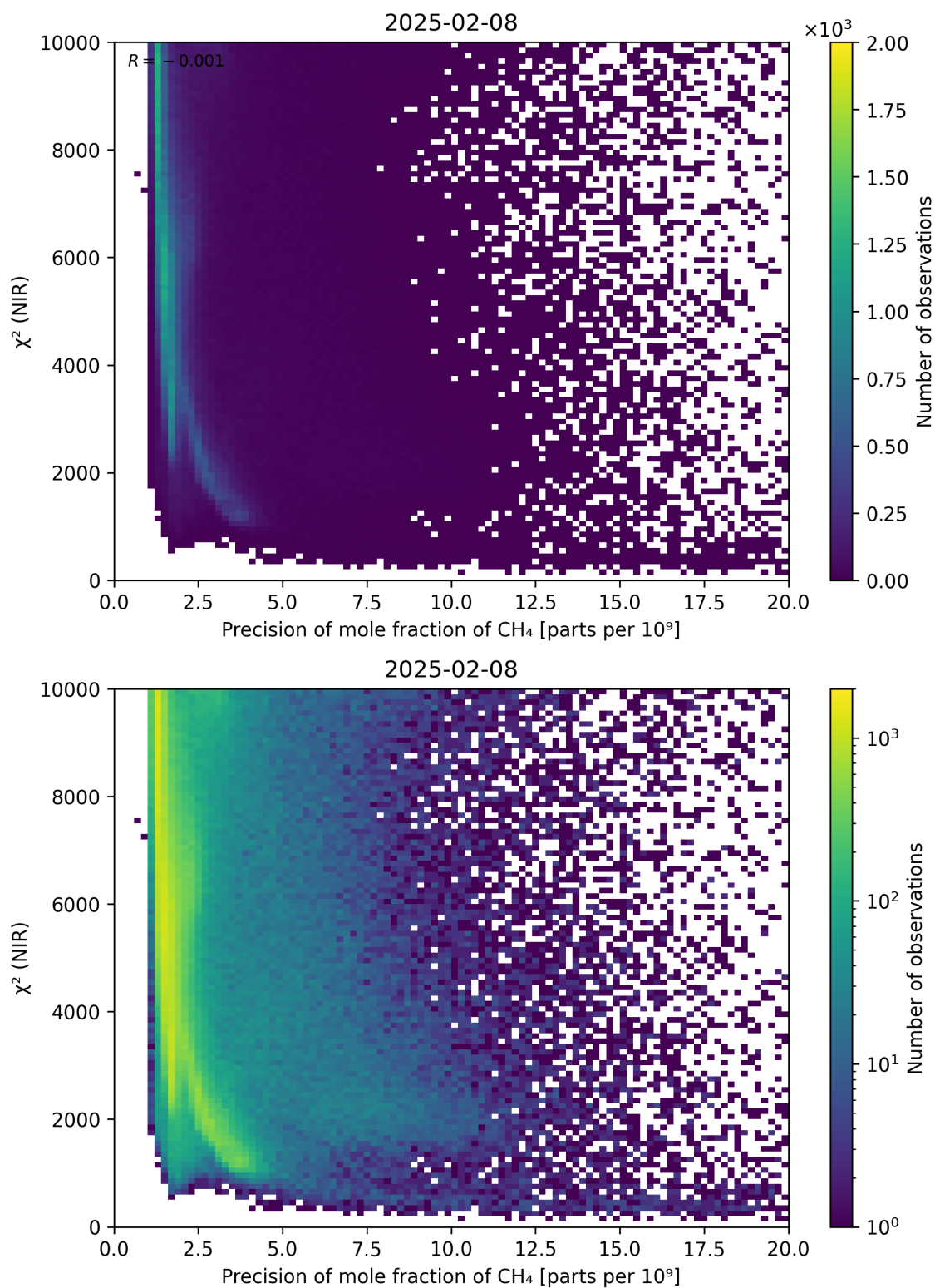
Figure 78: Scatter density plot of “Precision of mole fraction of CH 4 ” against “ \chi^2 (NIR)” for 2025-02-08 to 2025-02-09.
