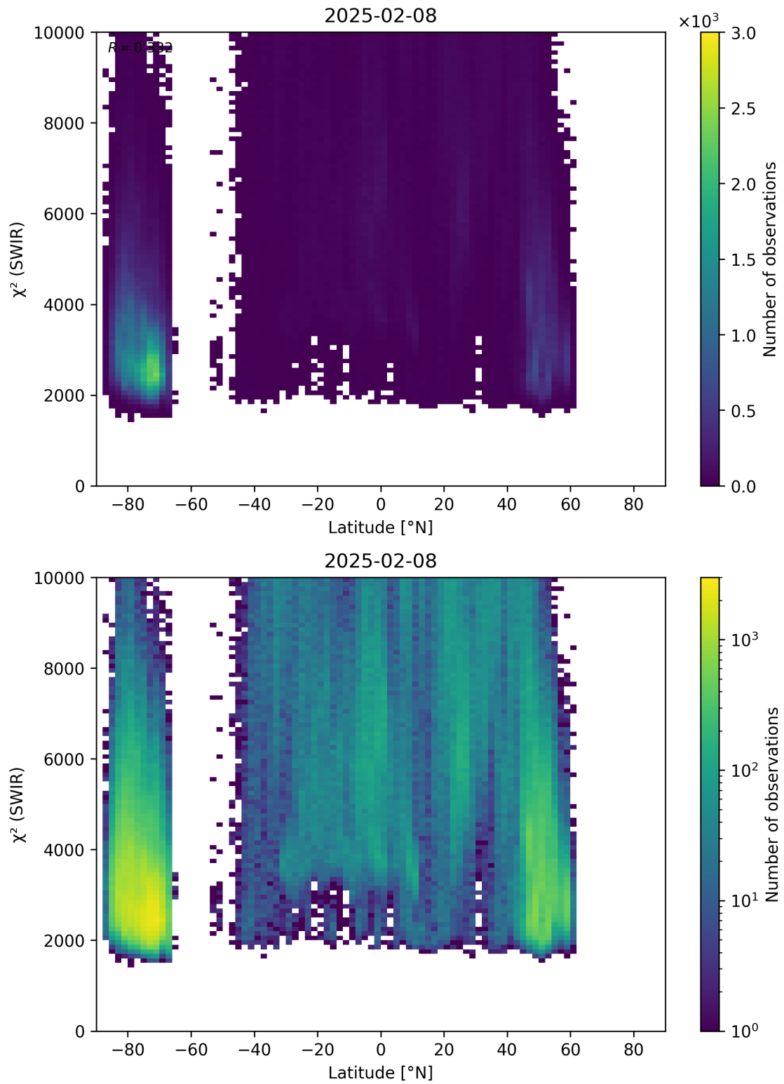
Figure 54: Scatter density plot of “Latitude” against “ \chi^2 (SWIR)” for 2025-02-08 to 2025-02-09.
