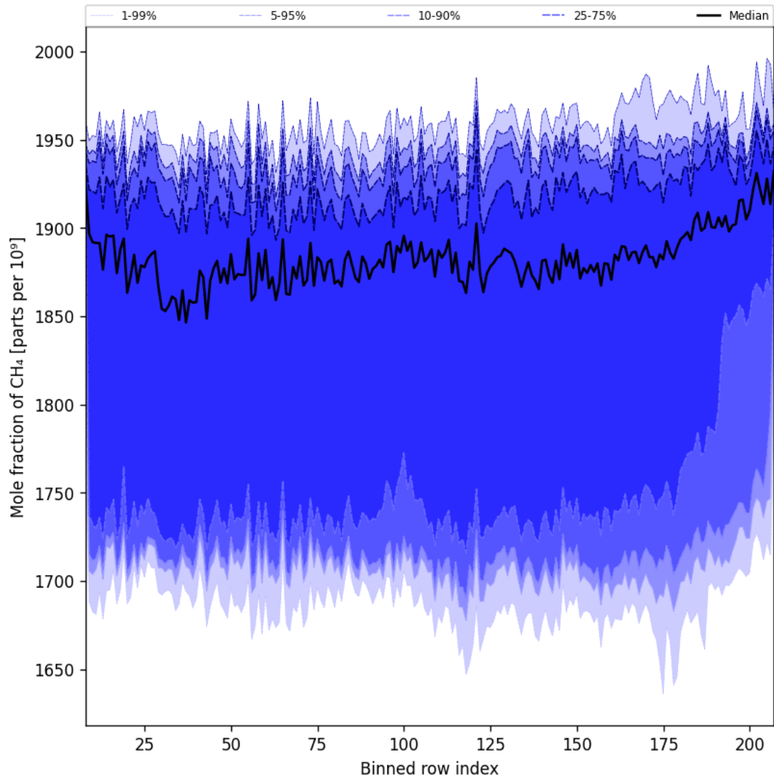
Figure 34: Along track statistics of “Mole fraction of CH 4 ” for 2025-02-08 to 2025-02-09
