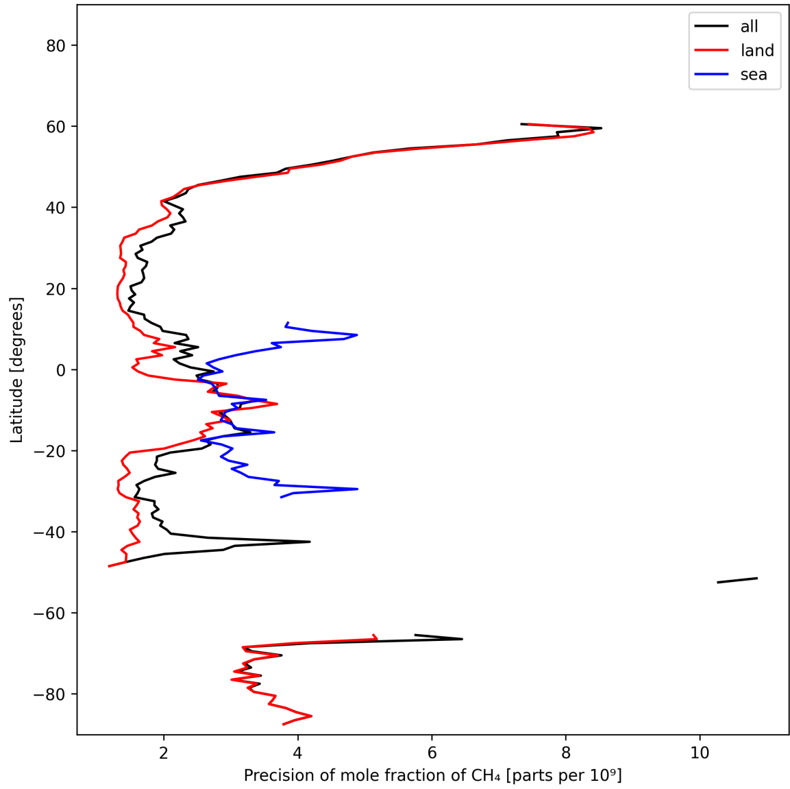
Figure 13: Zonal average of “Precision of mole fraction of CH 4 ” for 2025-02-08 to 2025-02-09.
