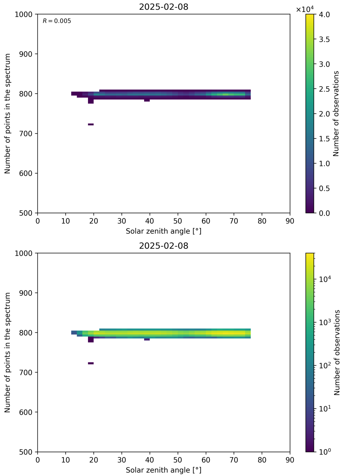
Figure 103: Scatter density plot of “Solar zenith angle” against “Number of points in the spectrum” for 2025-02-08 to 2025-02-09.
