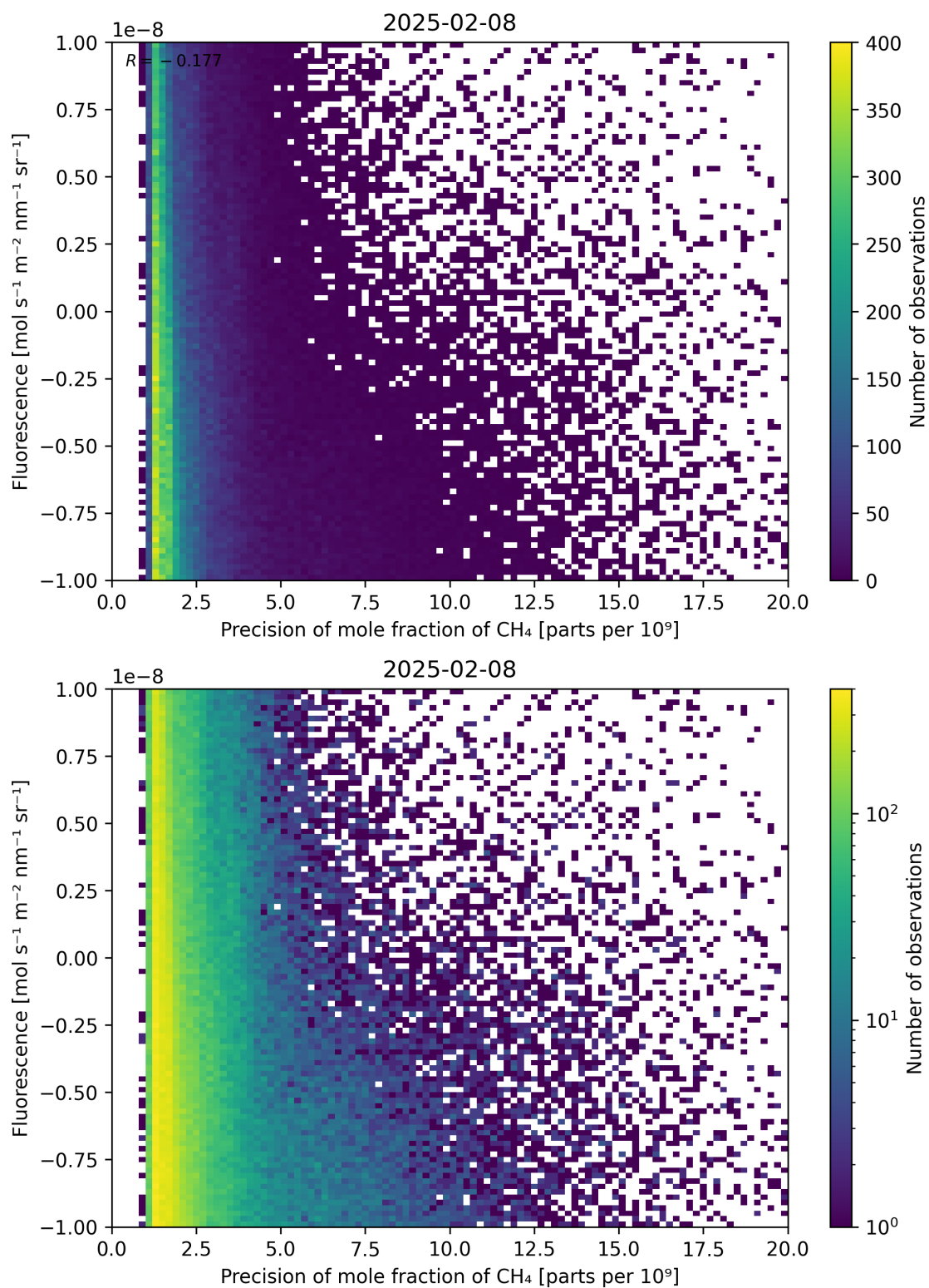
Figure 81: Scatter density plot of “Precision of mole fraction of \text{CH}_4 ” against “Fluorescence” for 2025-02-08 to 2025-02-09.
