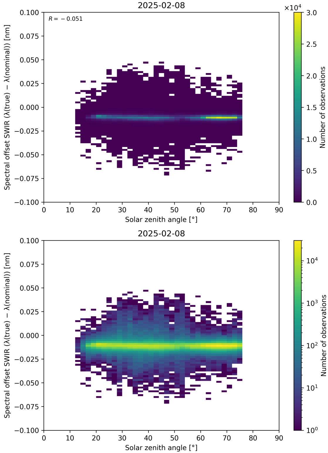
Figure 104: Scatter density plot of “Solar zenith angle” against “Spectral offset SWIR ( \lambda_{\text{true}} - \lambda_{\text{nominal}} )” for 2025-02-08 to 2025-02-09.
