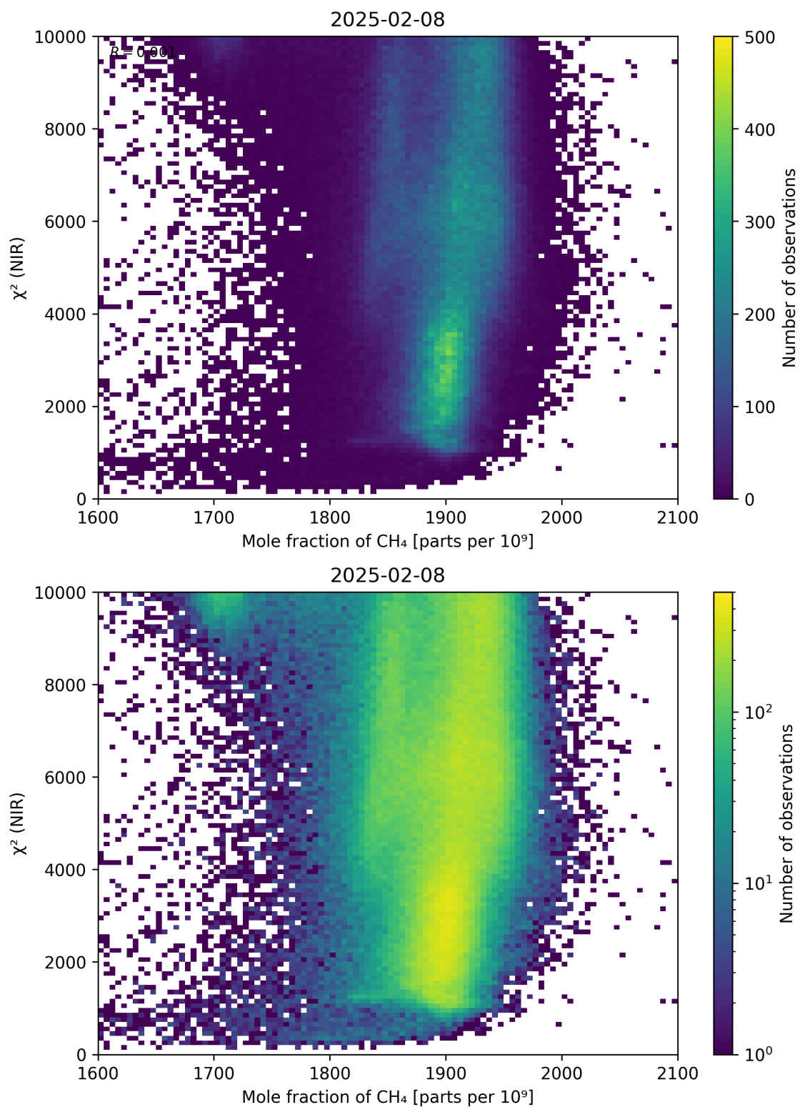
Figure 70: Scatter density plot of “Mole fraction of CH 4 ” against “ \chi^2 (NIR)” for 2025-02-08 to 2025-02-09.
