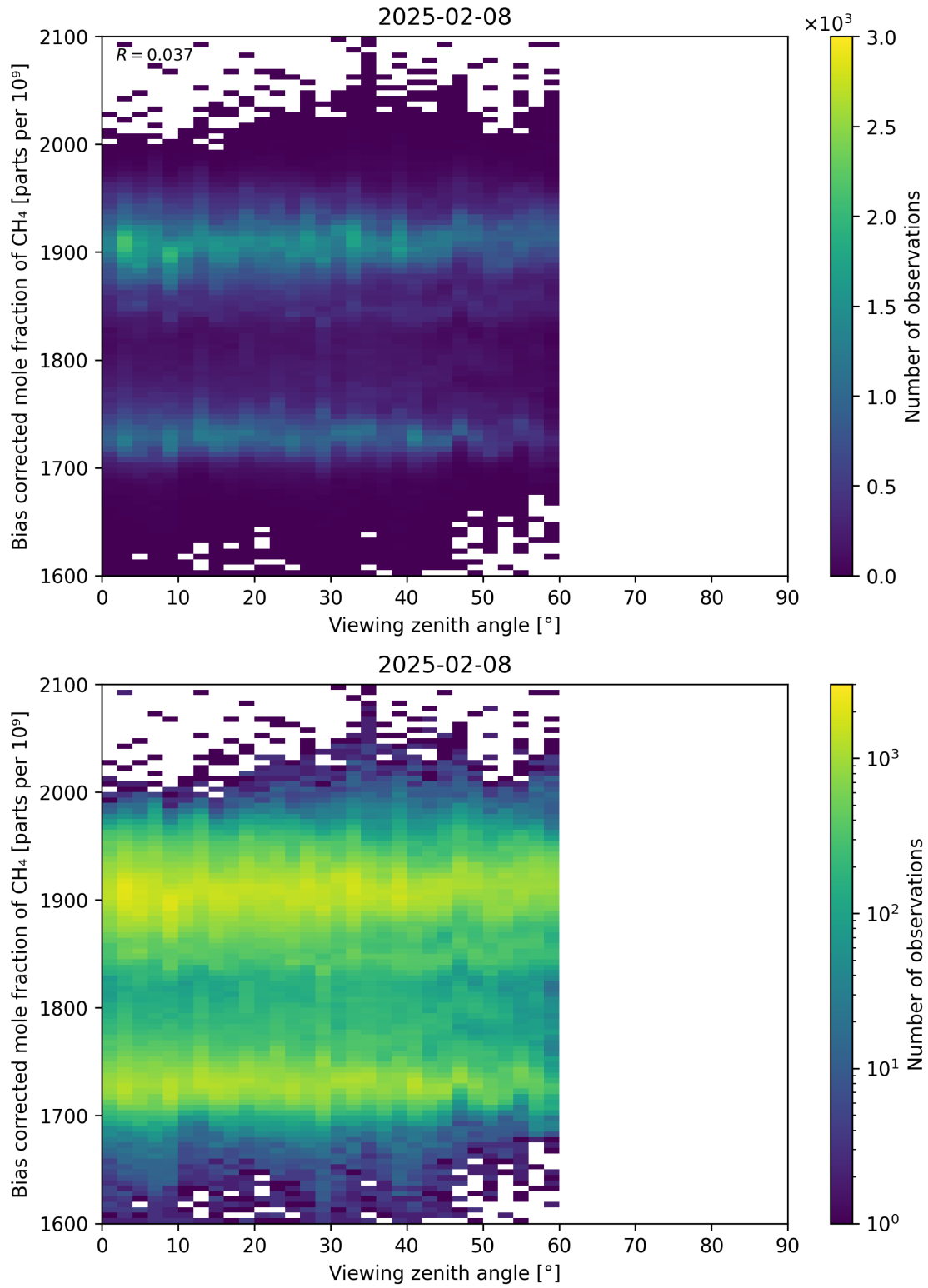
Figure 111: Scatter density plot of “Viewing zenith angle” against “Bias corrected mole fraction of CH 4 ” for 2025-02-08 to 2025-02-09.
