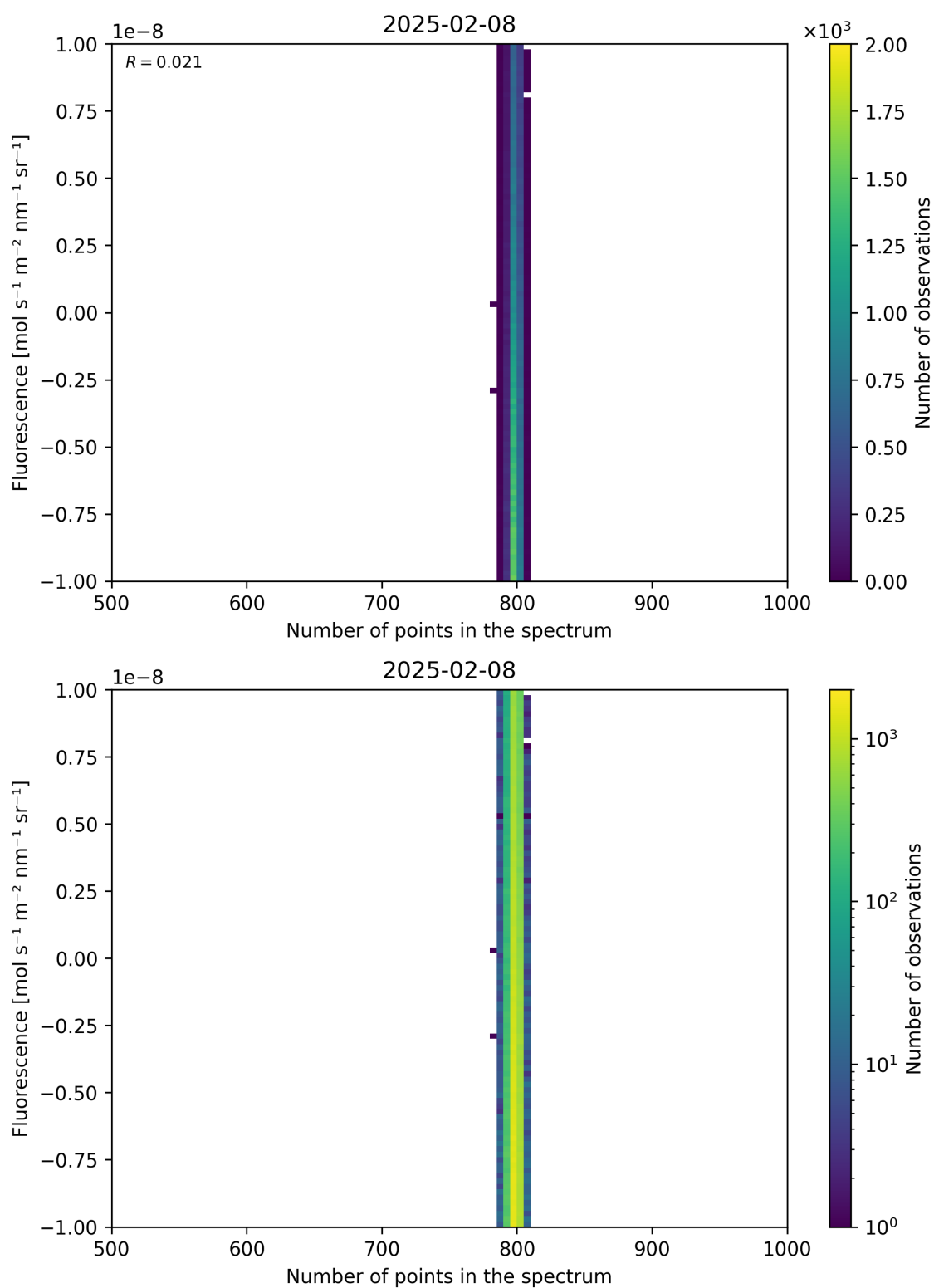
Figure 91: Scatter density plot of “Number of points in the spectrum” against “Fluorescence” for 2025-02-08 to 2025-02-09.
