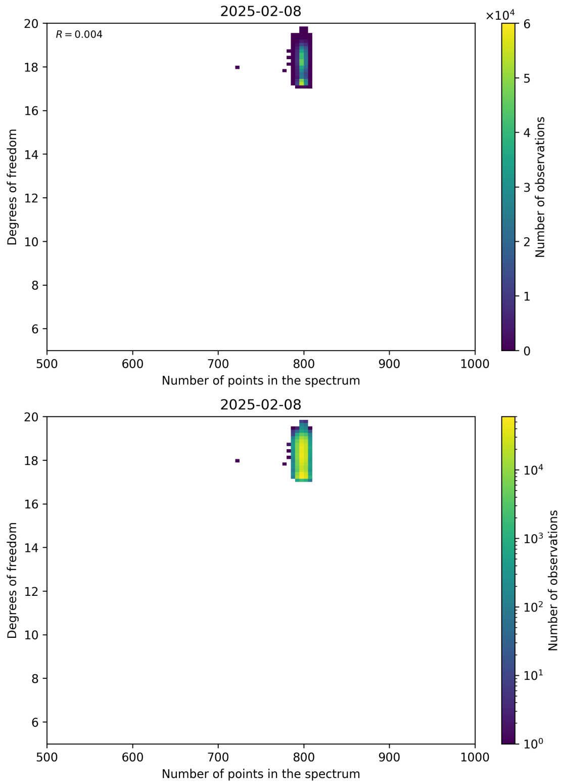
Figure 90: Scatter density plot of “Number of points in the spectrum” against “Degrees of freedom” for 2025-02-08 to 2025-02-09.
