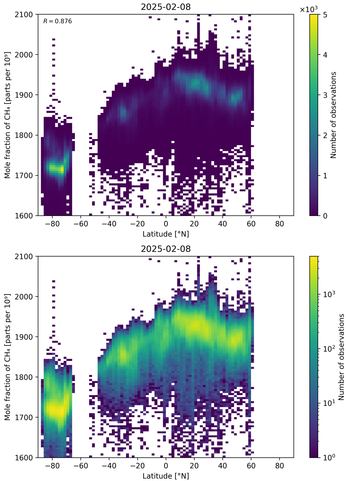
Figure 57: Scatter density plot of “Latitude” against “Mole fraction of CH 4 ” for 2025-02-08 to 2025-02-09.
