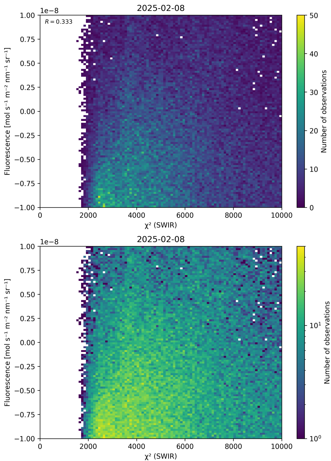
Figure 49: Scatter density plot of “ \chi^2 (SWIR)” against “Fluorescence” for 2025-02-08 to 2025-02-09.
