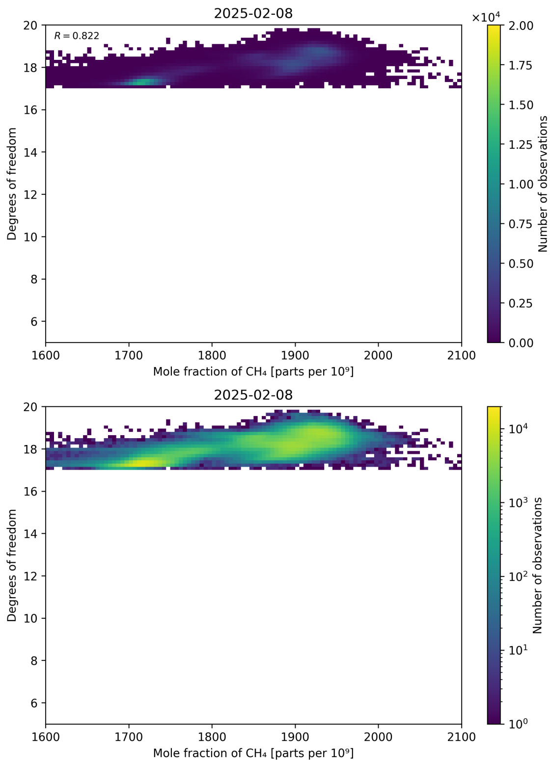
Figure 72: Scatter density plot of “Mole fraction of CH 4 ” against “Degrees of freedom” for 2025-02-08 to 2025-02-09.
