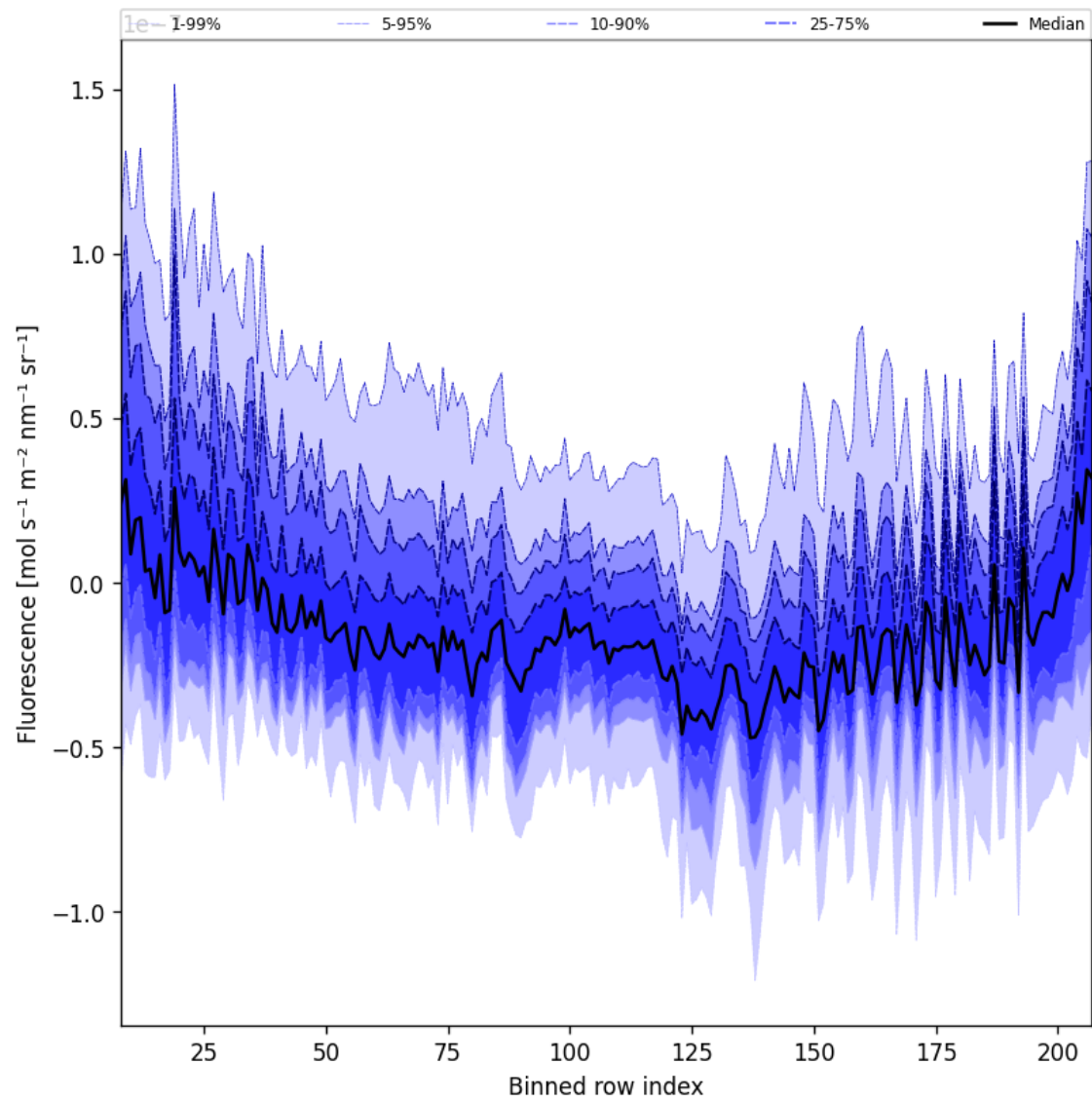
Figure 43: Along track statistics of “Fluorescence” for 2025-02-08 to 2025-02-09
