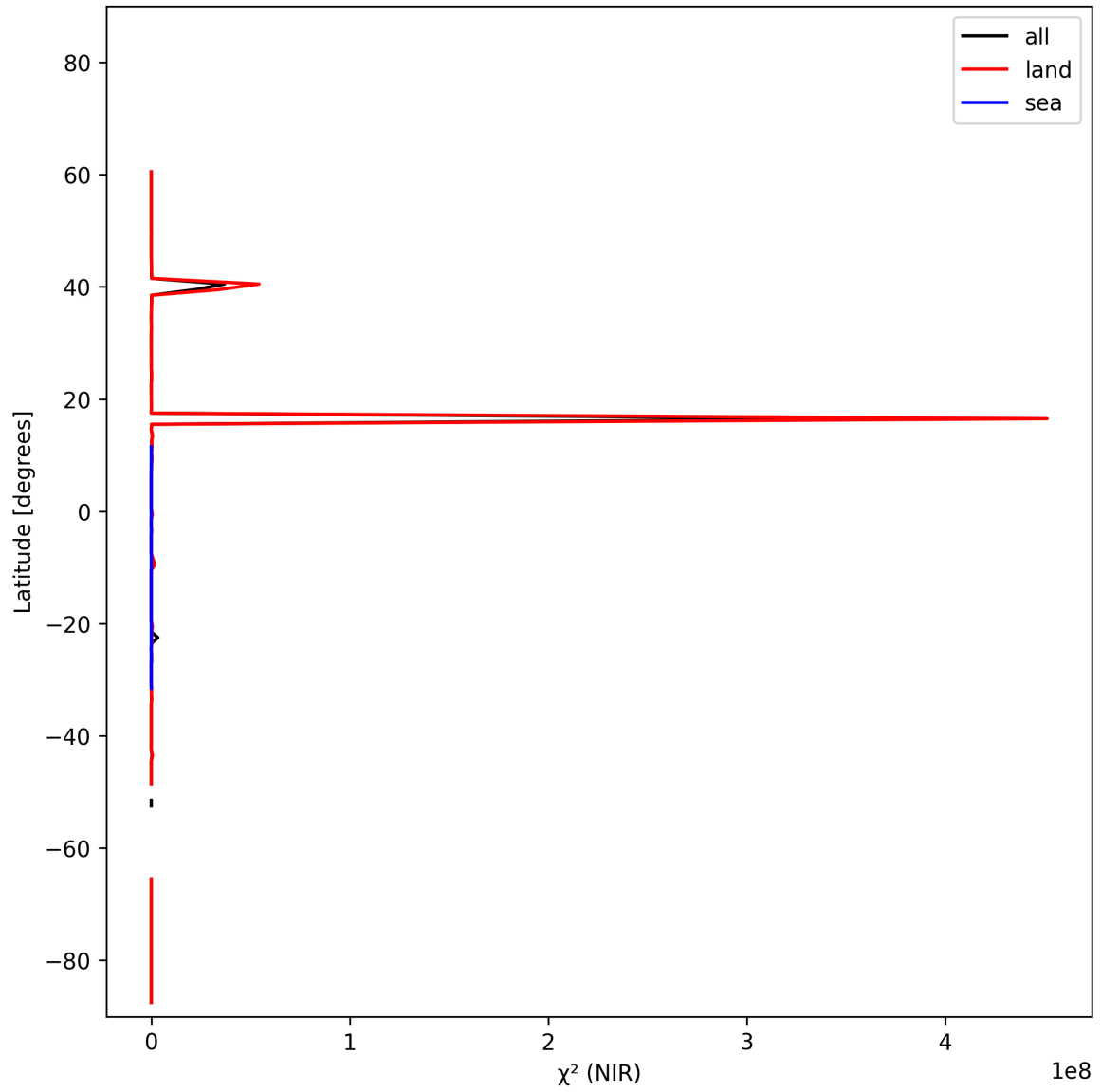
Figure 18: Zonal average of “ \chi^2 (NIR)” for 2025-02-08 to 2025-02-09.
