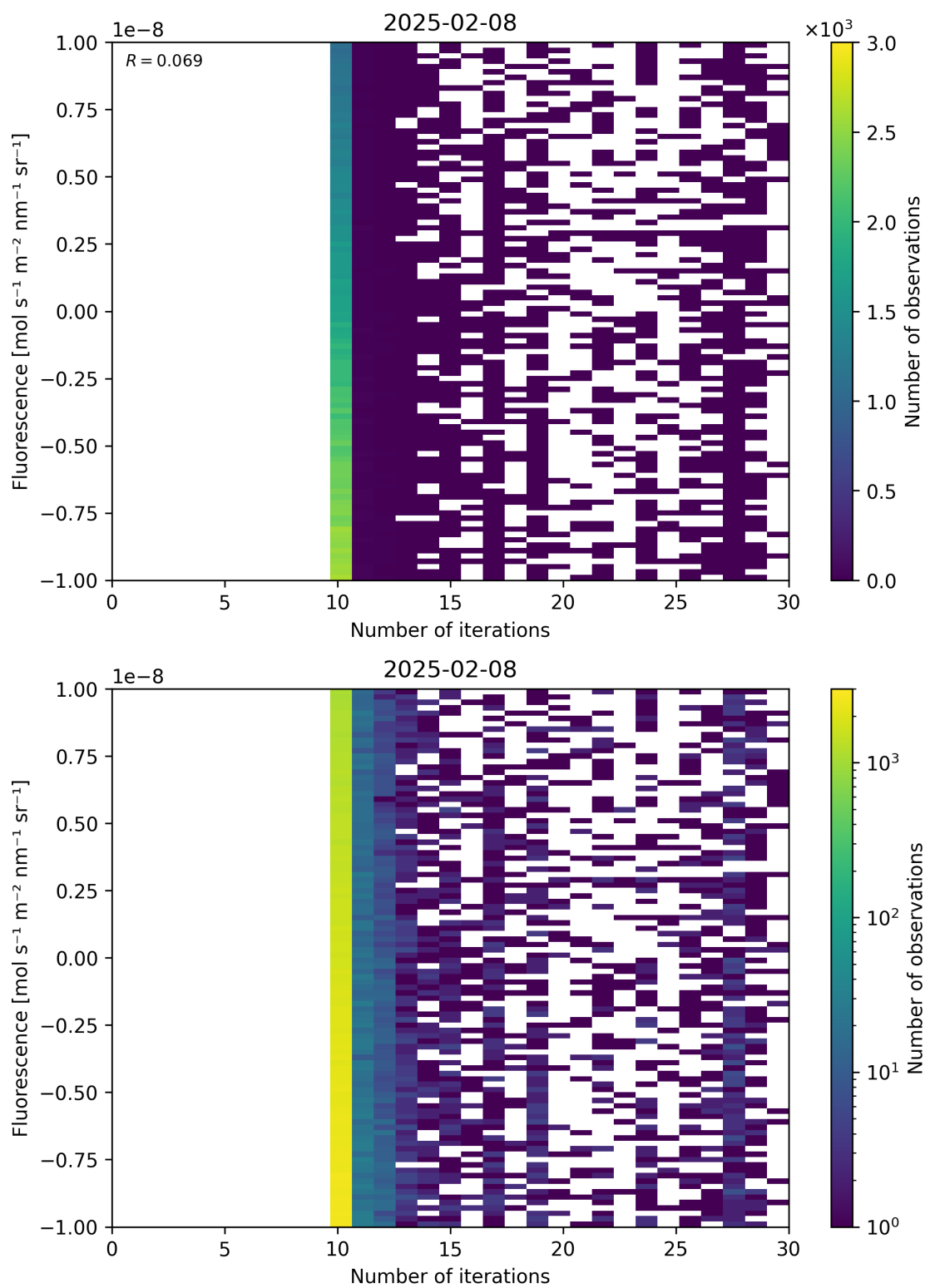
Figure 87: Scatter density plot of “Number of iterations” against “Fluorescence” for 2025-02-08 to 2025-02-09.
