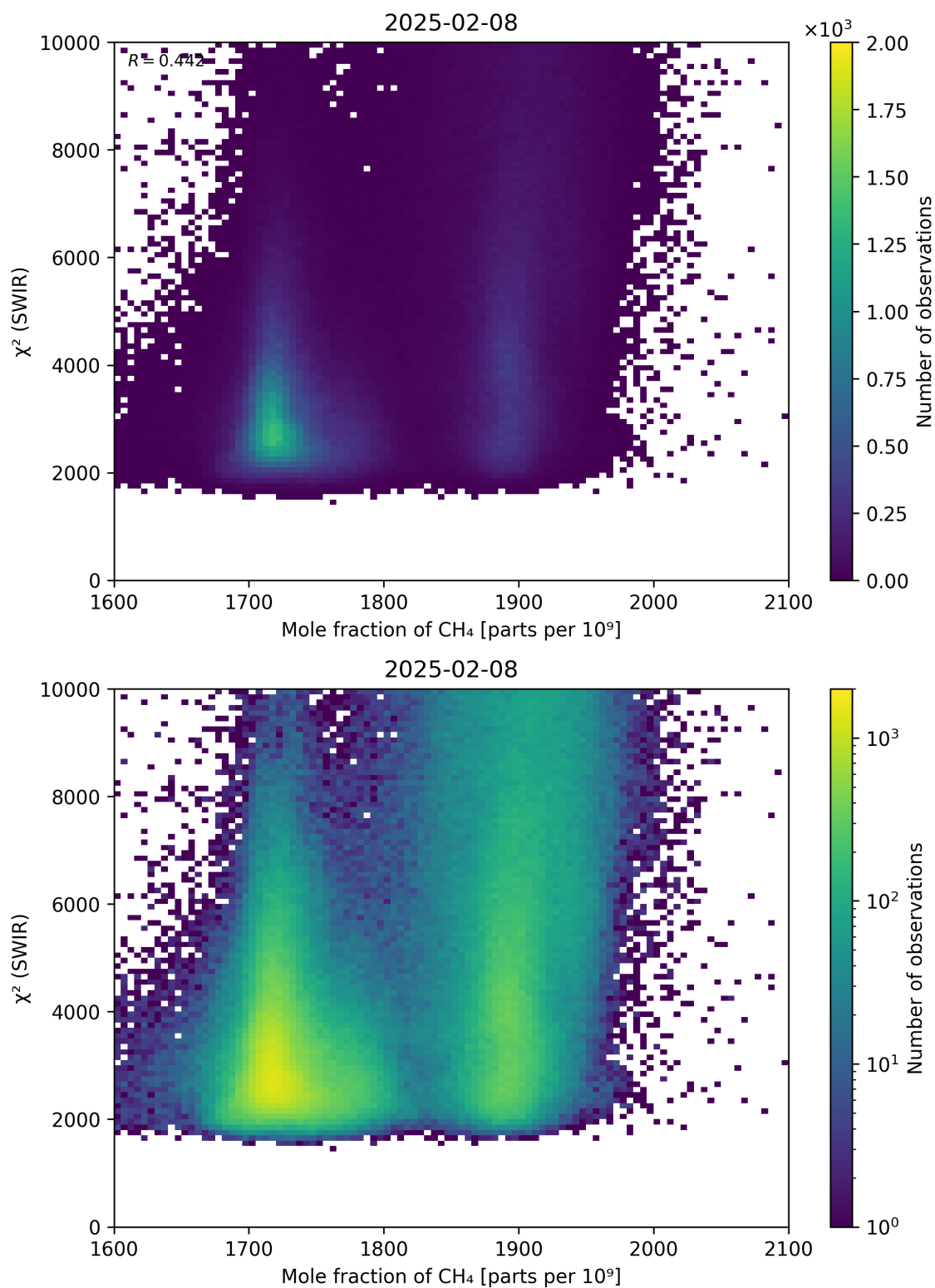
Figure 71: Scatter density plot of “Mole fraction of \text{CH}_4 ” against “ \chi^2 (SWIR)” for 2025-02-08 to 2025-02-09.
