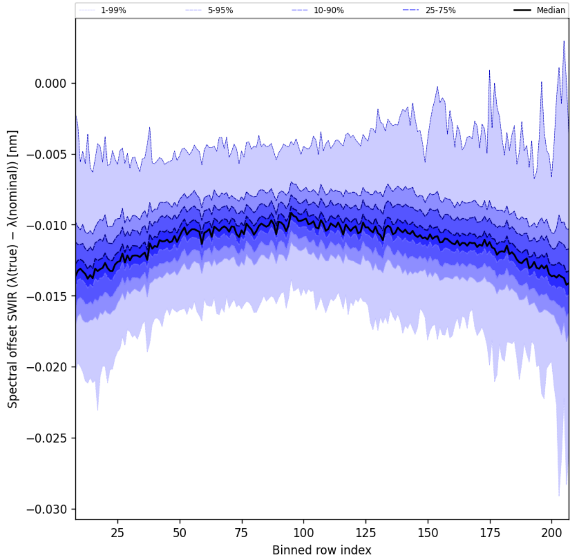
Figure 38: Along track statistics of “Spectral offset SWIR ( \lambda_{\text{true}} - \lambda_{\text{nominal}} )” for 2025-02-08 to 2025-02-09
