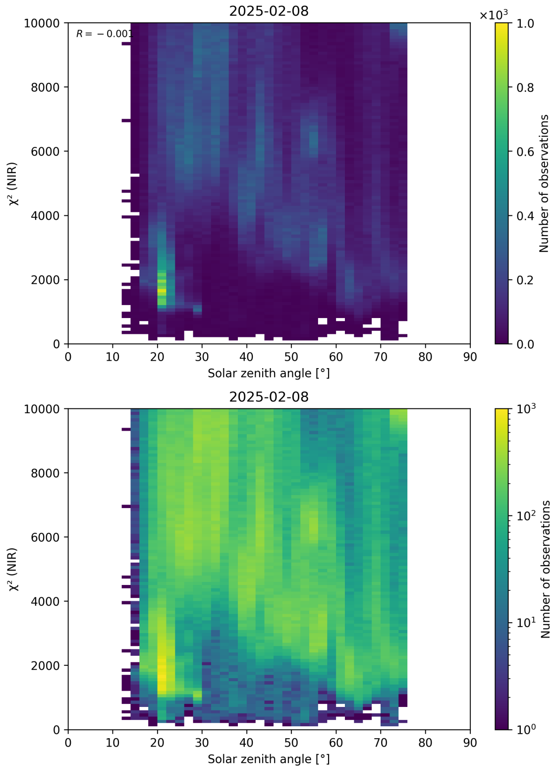
Figure 94: Scatter density plot of “Solar zenith angle” against “ \chi^2 (NIR)” for 2025-02-08 to 2025-02-09.
