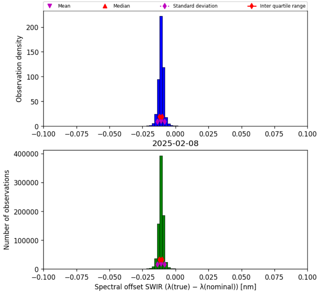
Figure 27: Histogram of “Spectral offset SWIR ( \lambda_{\text{true}} - \lambda_{\text{nominal}} )” for 2025-02-08 to 2025-02-09
