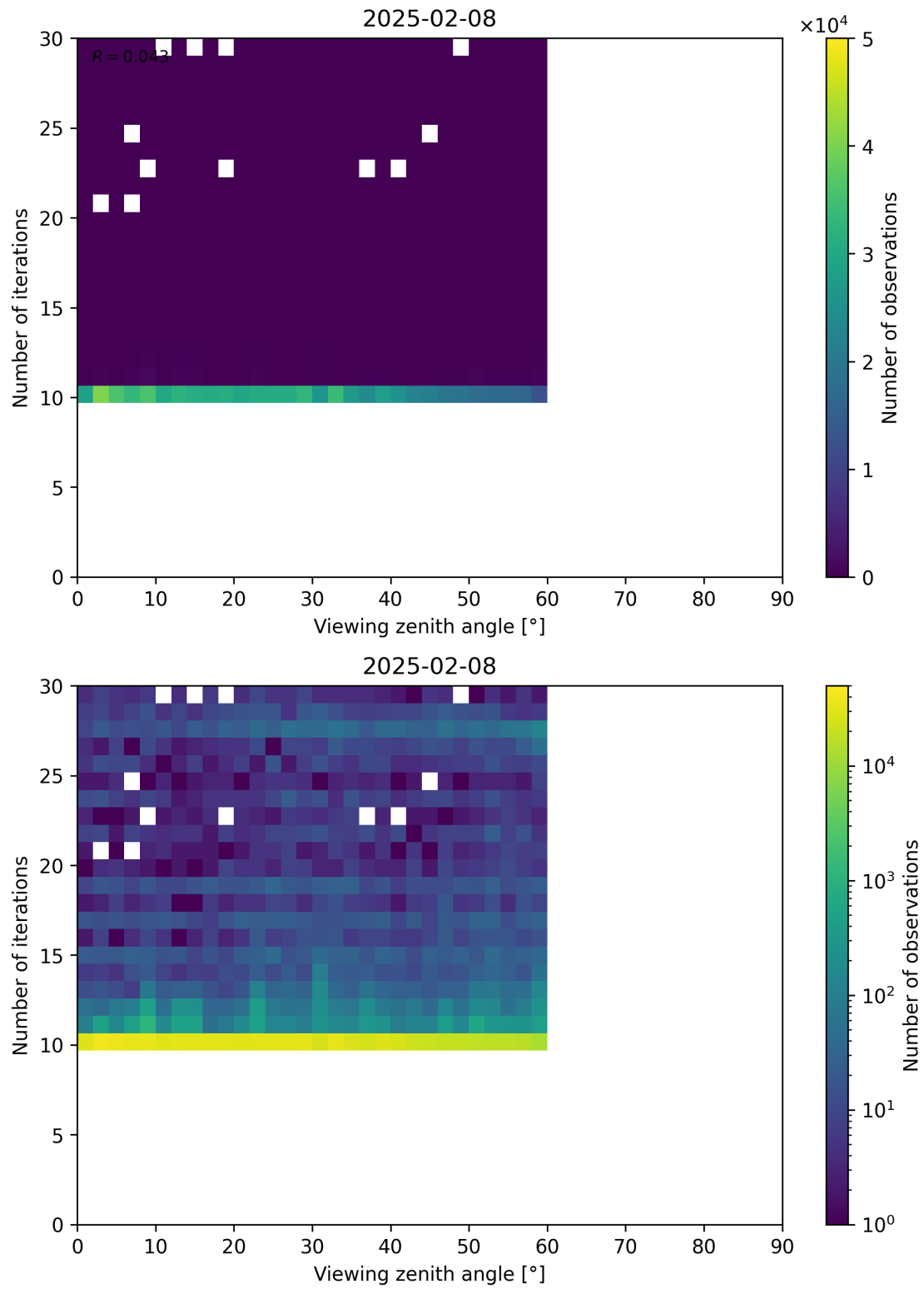
Figure 113: Scatter density plot of “Viewing zenith angle” against “Number of iterations” for 2025-02-08 to 2025-02-09.
