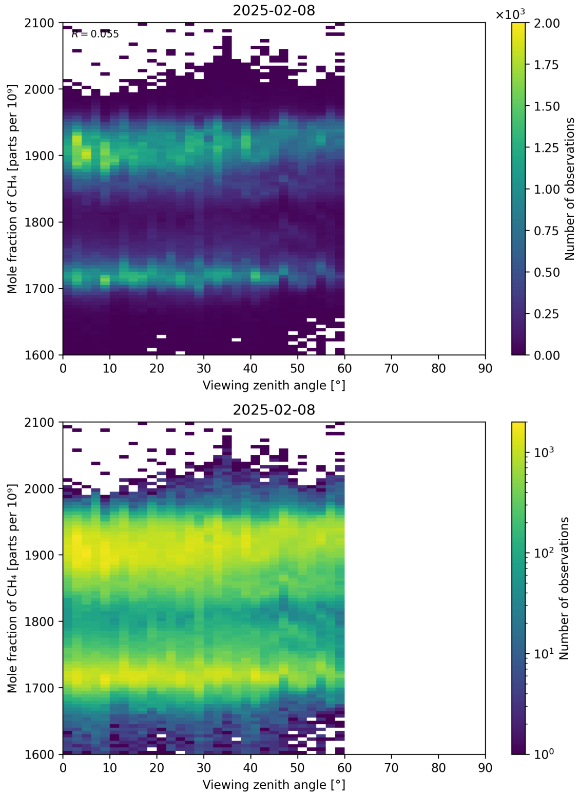
Figure 110: Scatter density plot of “Viewing zenith angle” against “Mole fraction of CH 4 ” for 2025-02-08 to 2025-02-09.
