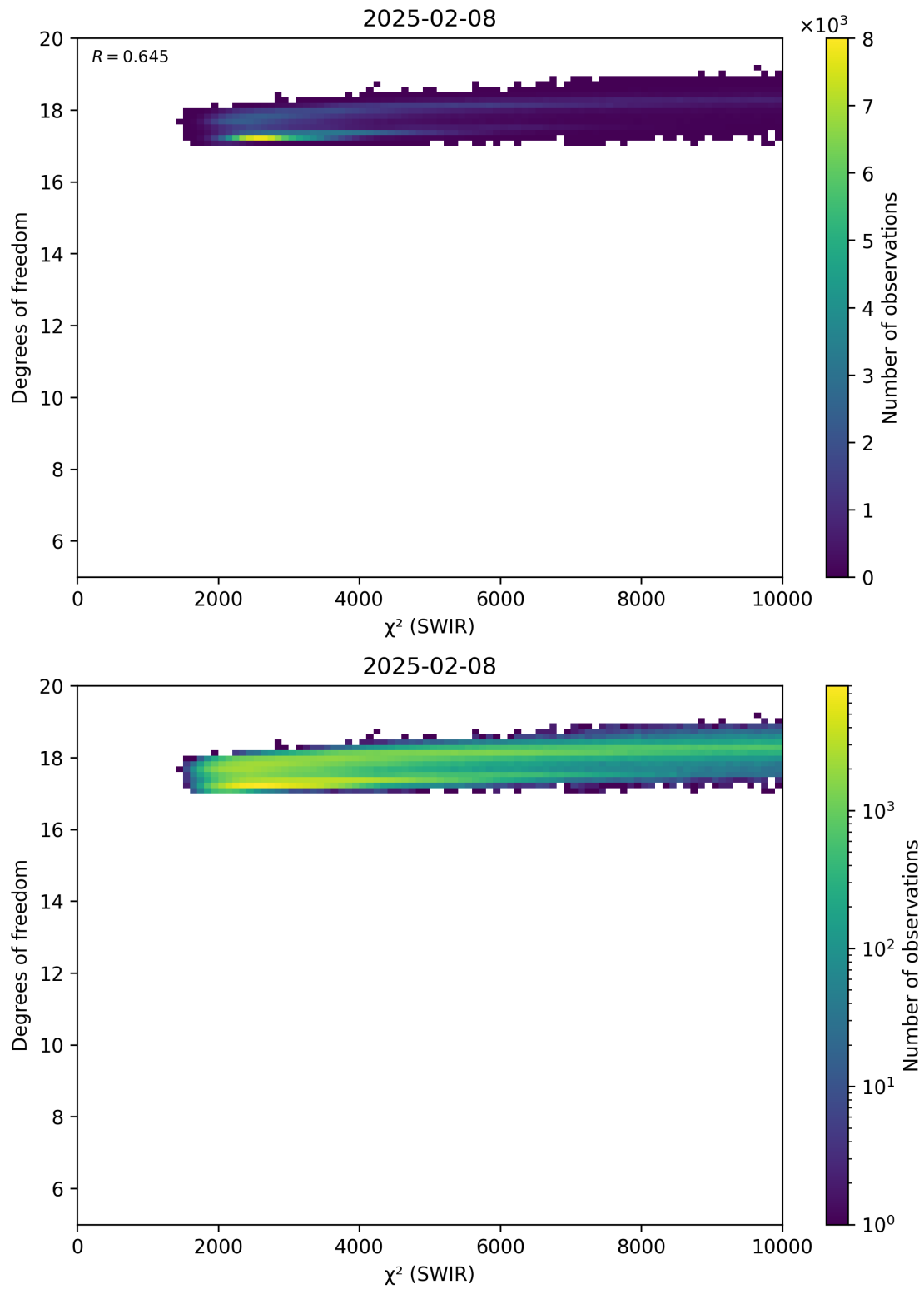
Figure 48: Scatter density plot of “ \chi^2 (SWIR)” against “Degrees of freedom” for 2025-02-08 to 2025-02-09.
