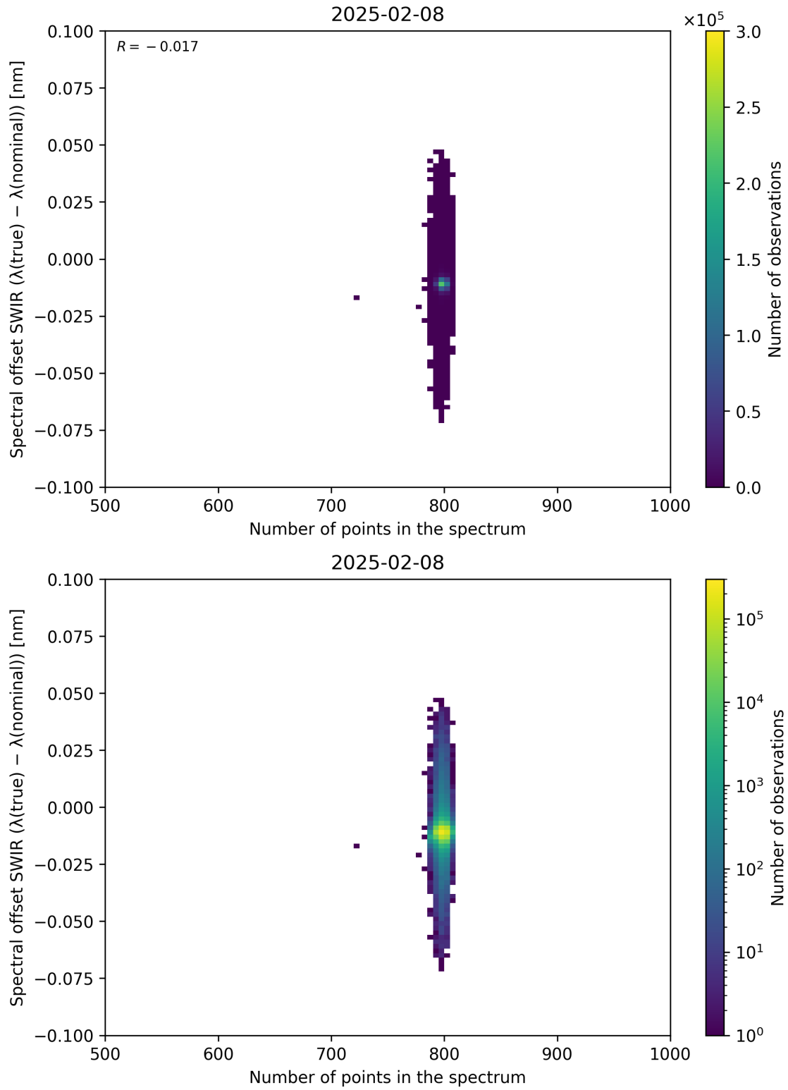
Figure 93: Scatter density plot of “Number of points in the spectrum” against “Spectral offset SWIR ( \lambda_{\text{true}} - \lambda_{\text{nominal}} )” for 2025-02-08 to 2025-02-09.
