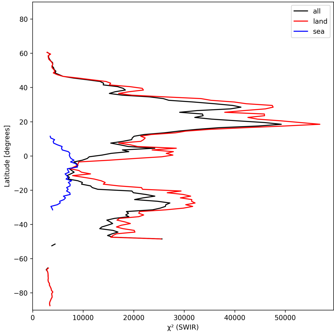
Figure 17: Zonal average of “ \chi^2 (SWIR)” for 2025-02-08 to 2025-02-09.
