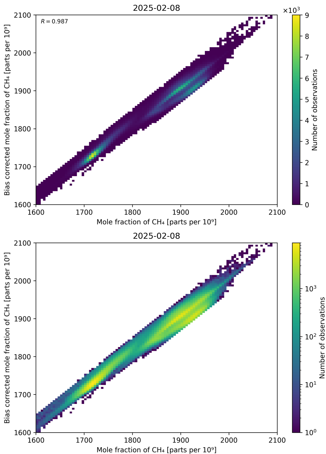
Figure 74: Scatter density plot of “Mole fraction of CH 4 ” against “Bias corrected mole fraction of CH 4 ” for 2025-02-08 to 2025-02-09.
