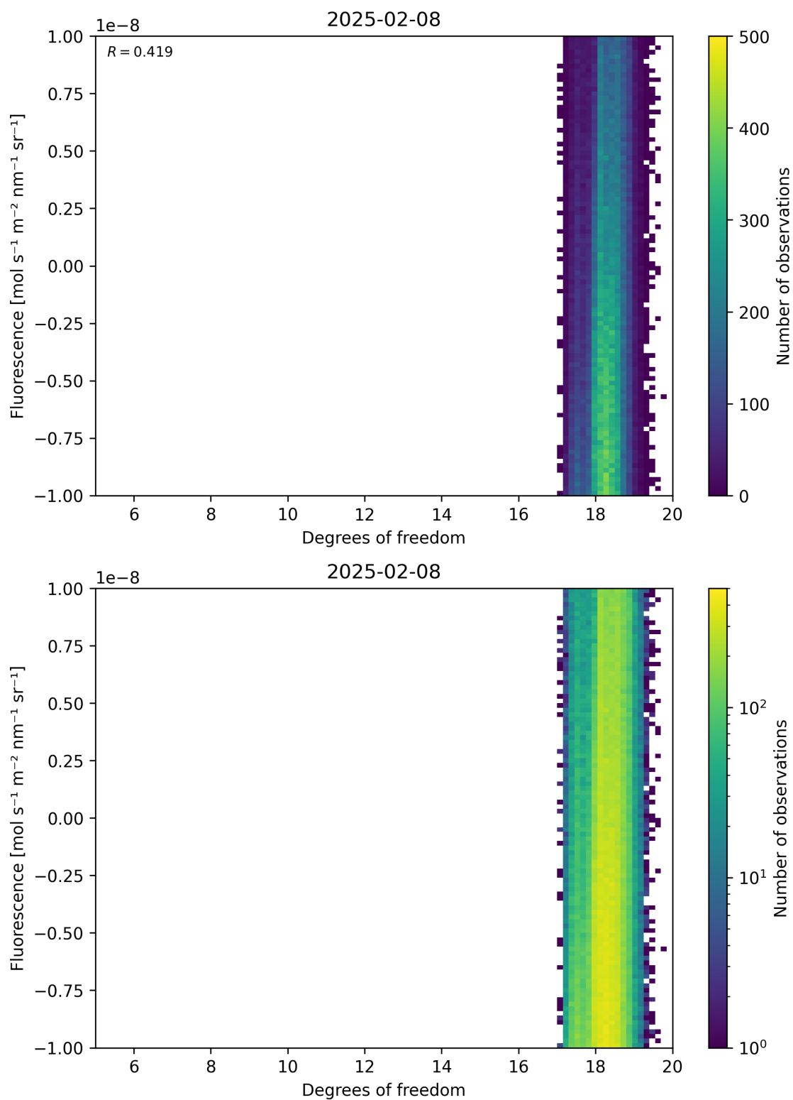
Figure 51: Scatter density plot of “Degrees of freedom” against “Fluorescence” for 2025-02-08 to 2025-02-09.
