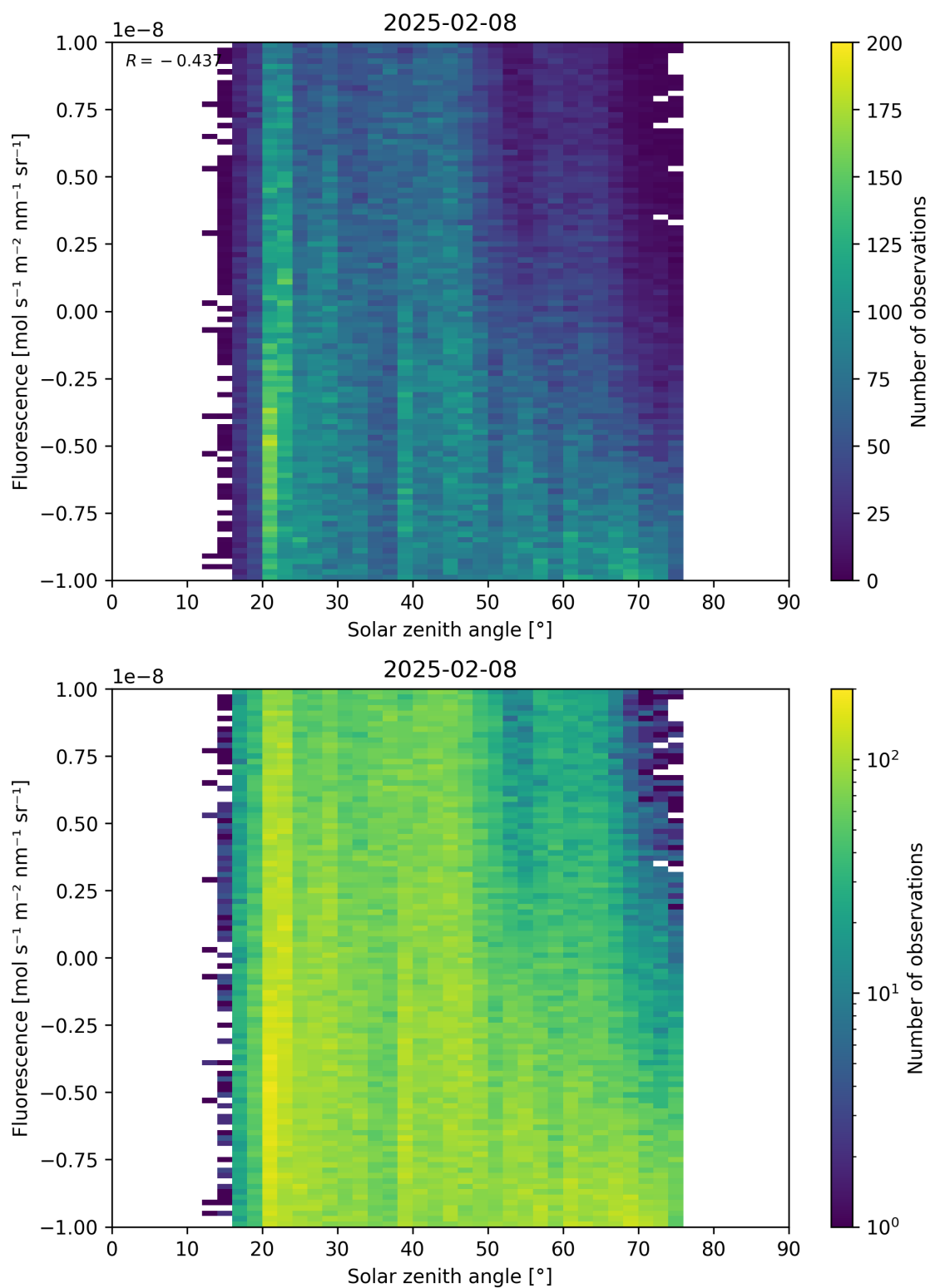
Figure 97: Scatter density plot of “Solar zenith angle” against “Fluorescence” for 2025-02-08 to 2025-02-09.
