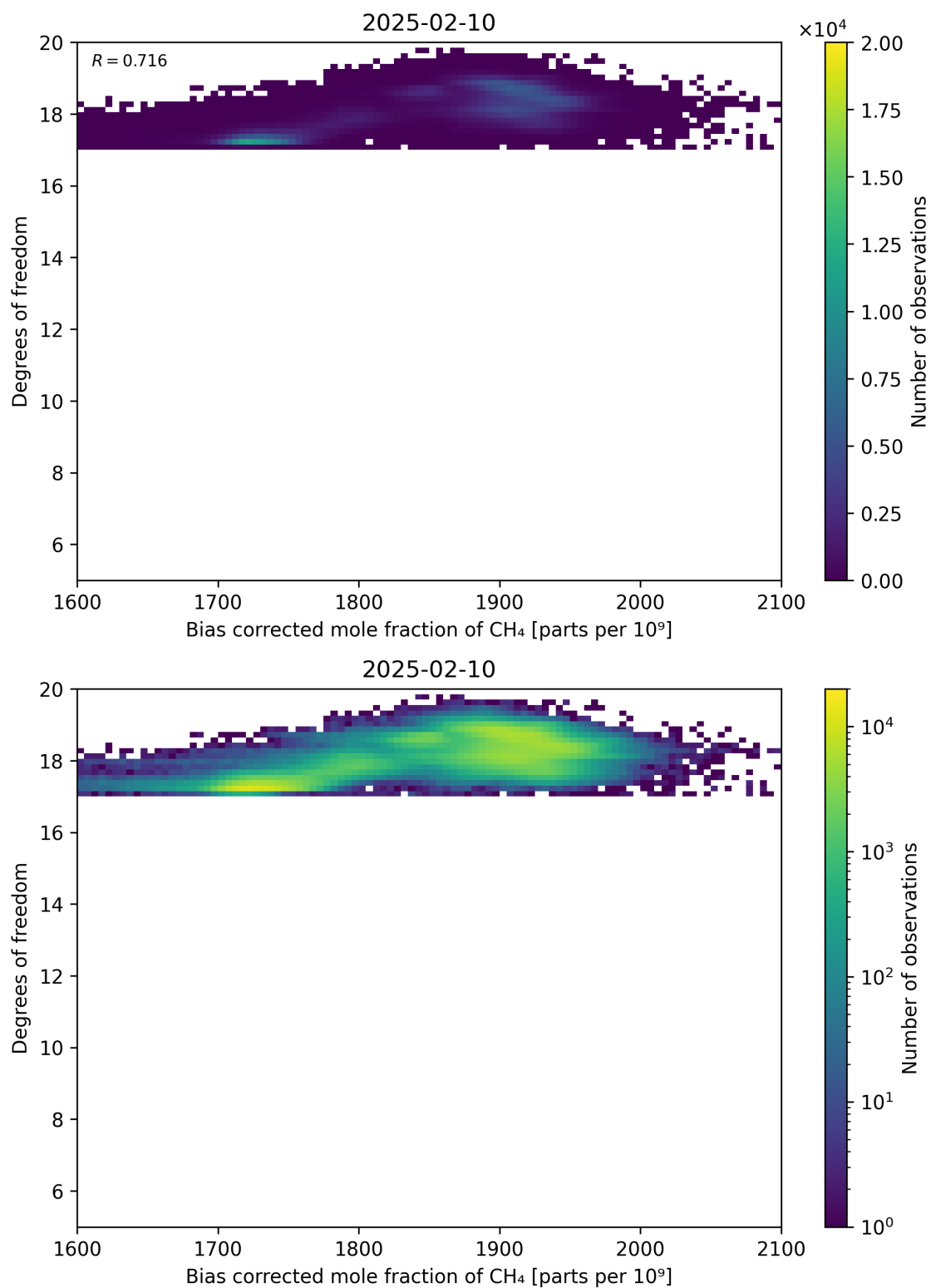
Figure 65: Scatter density plot of “Bias corrected mole fraction of CH 4 ” against “Degrees of freedom” for 2025-02-09 to 2025-02-11.
