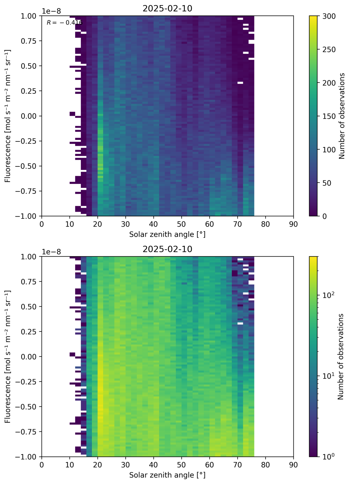
Figure 97: Scatter density plot of “Solar zenith angle” against “Fluorescence” for 2025-02-09 to 2025-02-11.
