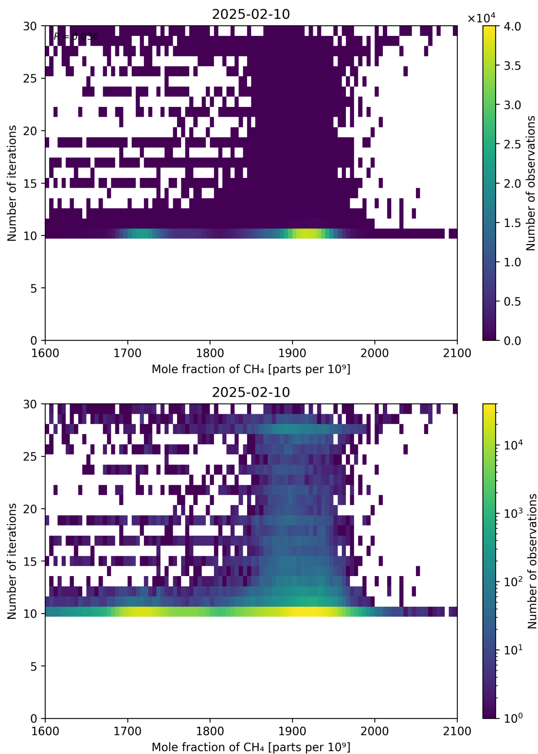
Figure 76: Scatter density plot of “Mole fraction of CH 4 ” against “Number of iterations” for 2025-02-09 to 2025-02-11.
