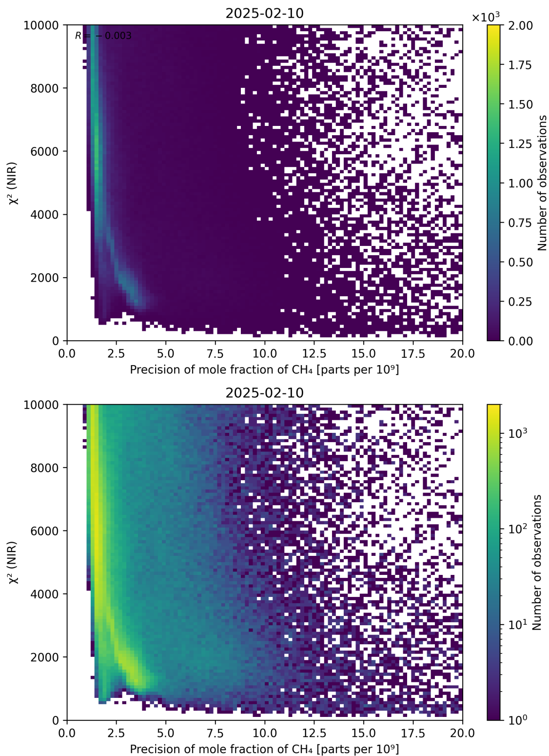
Figure 78: Scatter density plot of “Precision of mole fraction of CH 4 ” against “ \chi^2 (NIR)” for 2025-02-09 to 2025-02-11.
