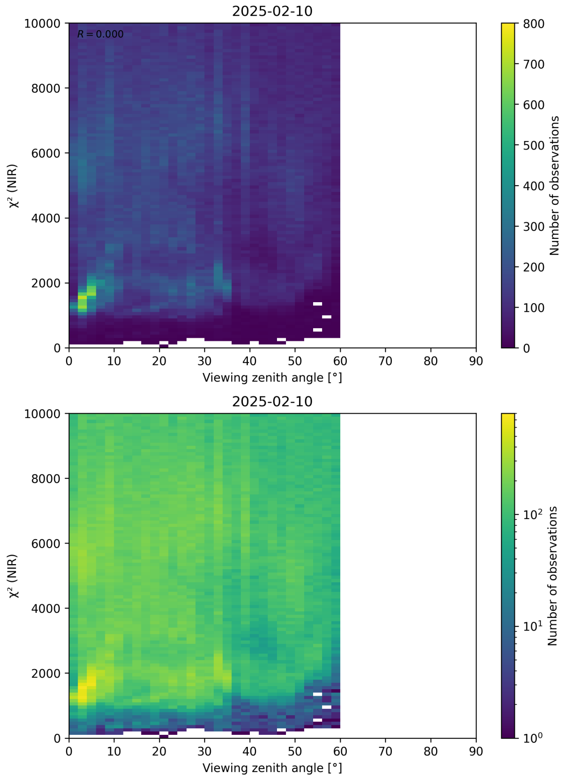
Figure 105: Scatter density plot of “Viewing zenith angle” against “ \chi^2 (NIR)” for 2025-02-09 to 2025-02-11.
