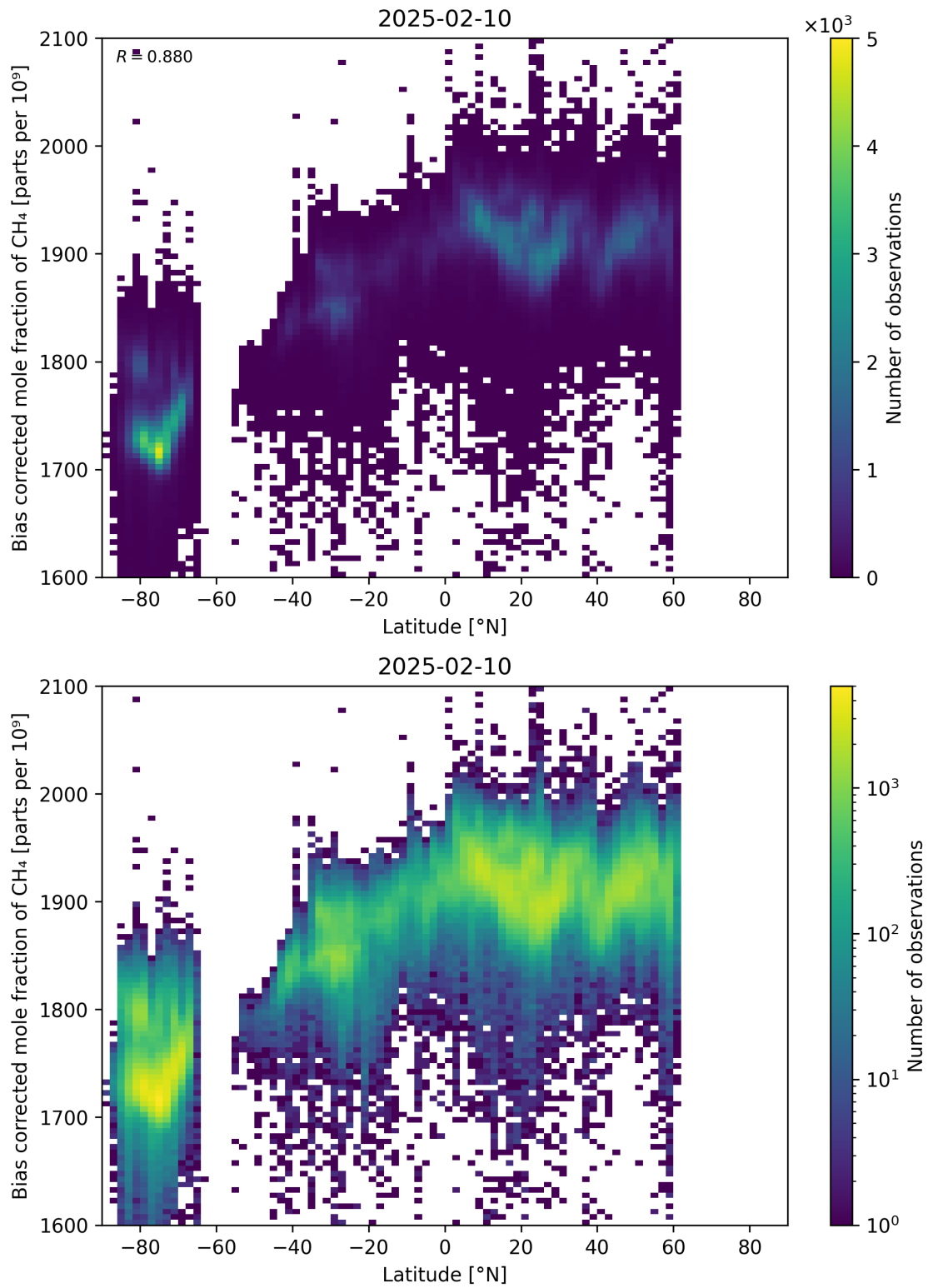
Figure 58: Scatter density plot of “Latitude” against “Bias corrected mole fraction of CH 4 ” for 2025-02-09 to 2025-02-11.
