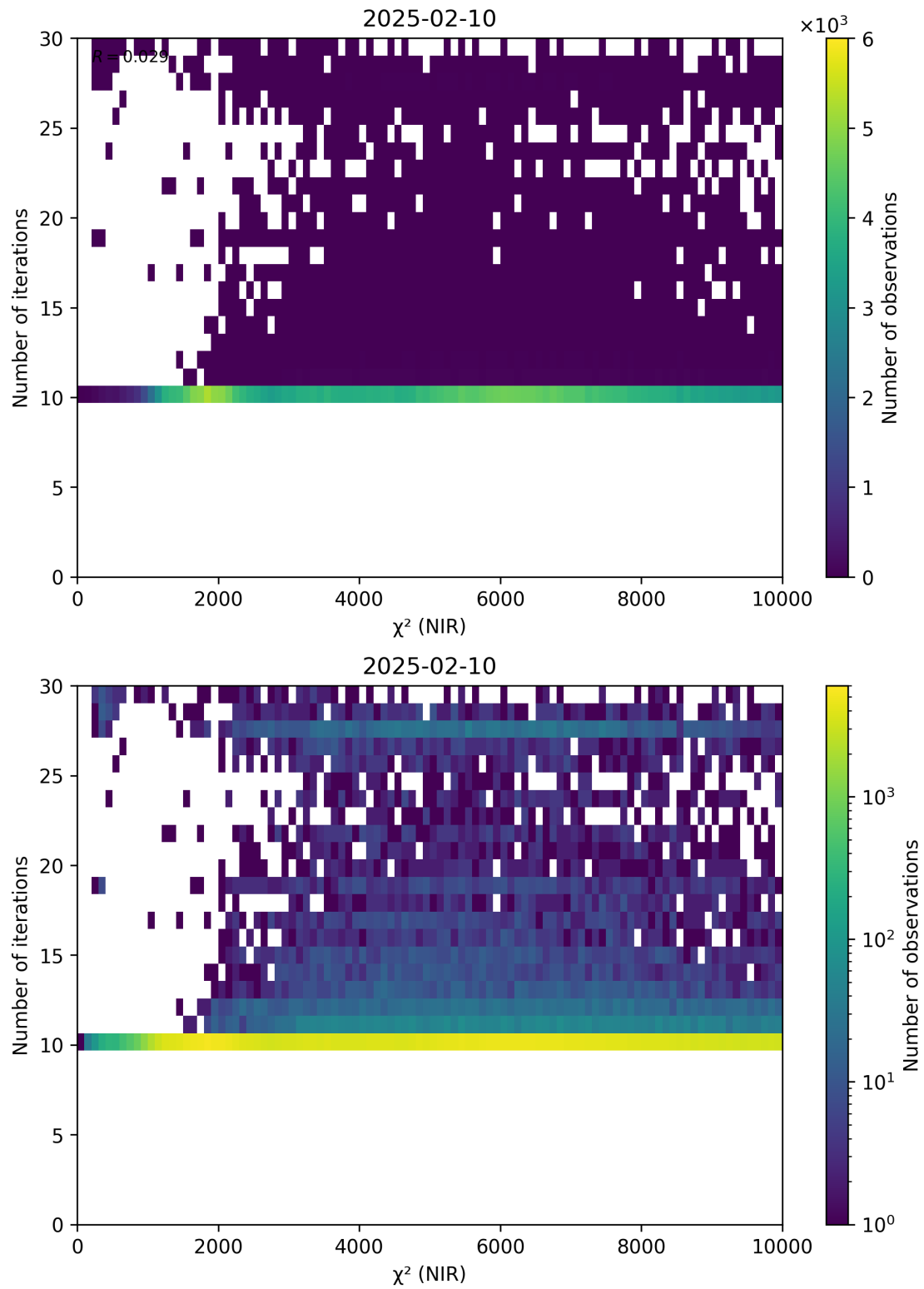
Figure 46: Scatter density plot of “ \chi^2 (NIR)” against “Number of iterations” for 2025-02-09 to 2025-02-11.
