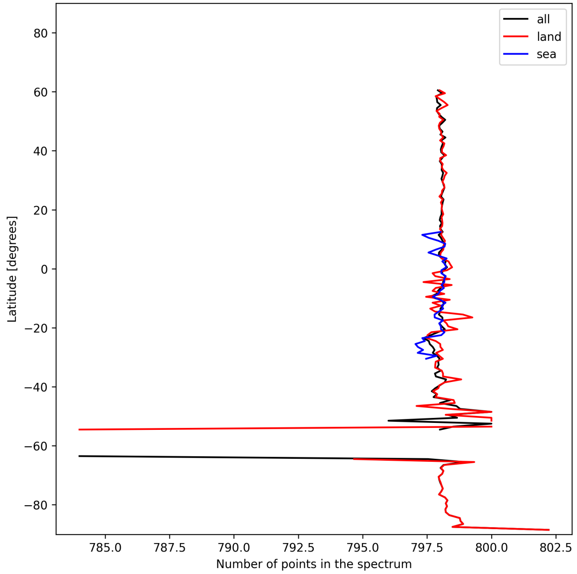
Figure 15: Zonal average of “Number of points in the spectrum” for 2025-02-09 to 2025-02-11.
