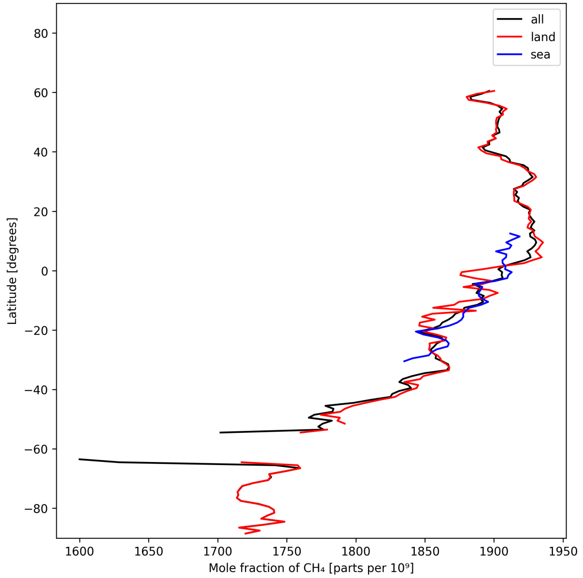
Figure 12: Zonal average of “Mole fraction of \text{CH}_4 ” for 2025-02-09 to 2025-02-11.
