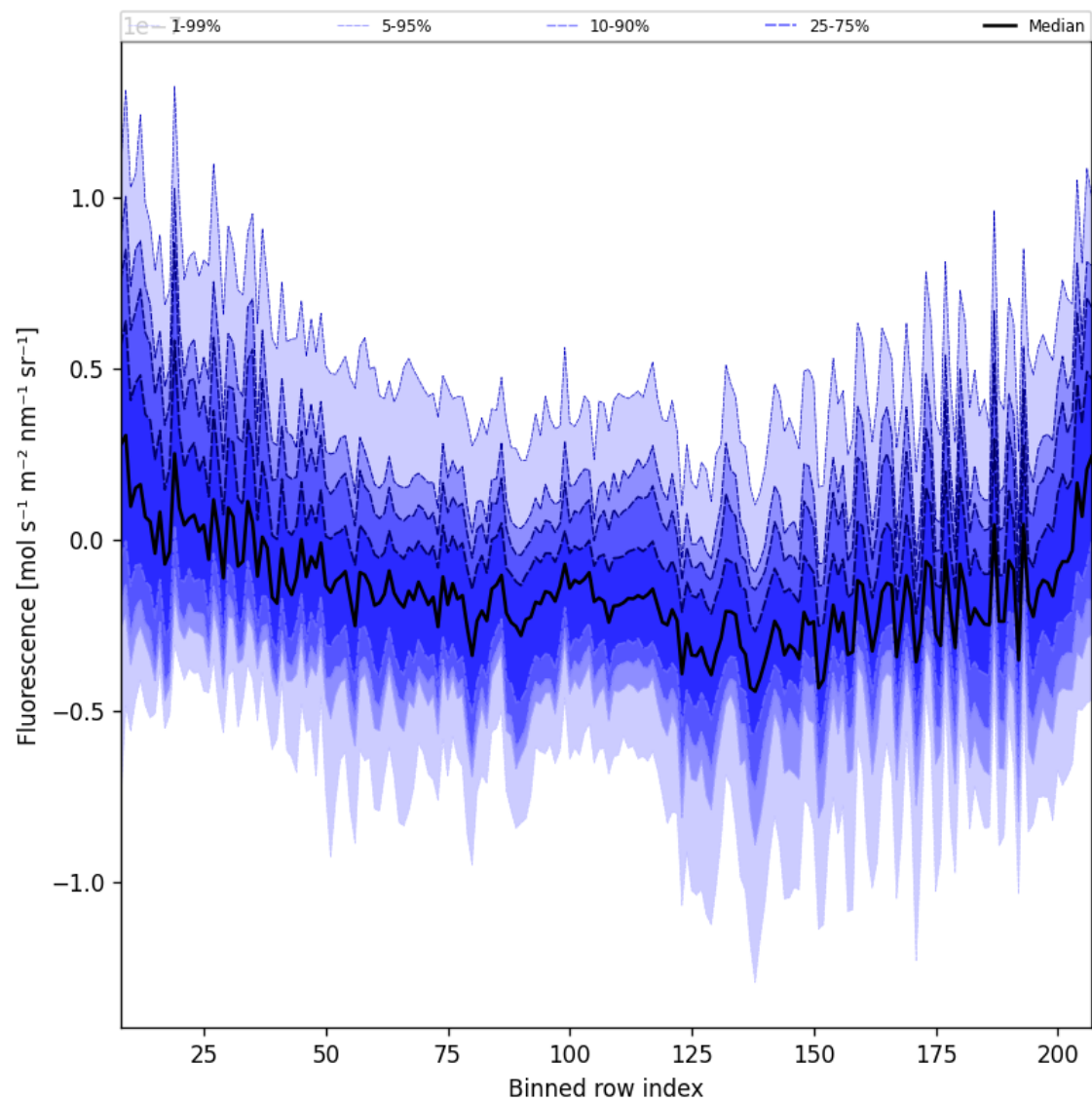
Figure 43: Along track statistics of “Fluorescence” for 2025-02-09 to 2025-02-11
