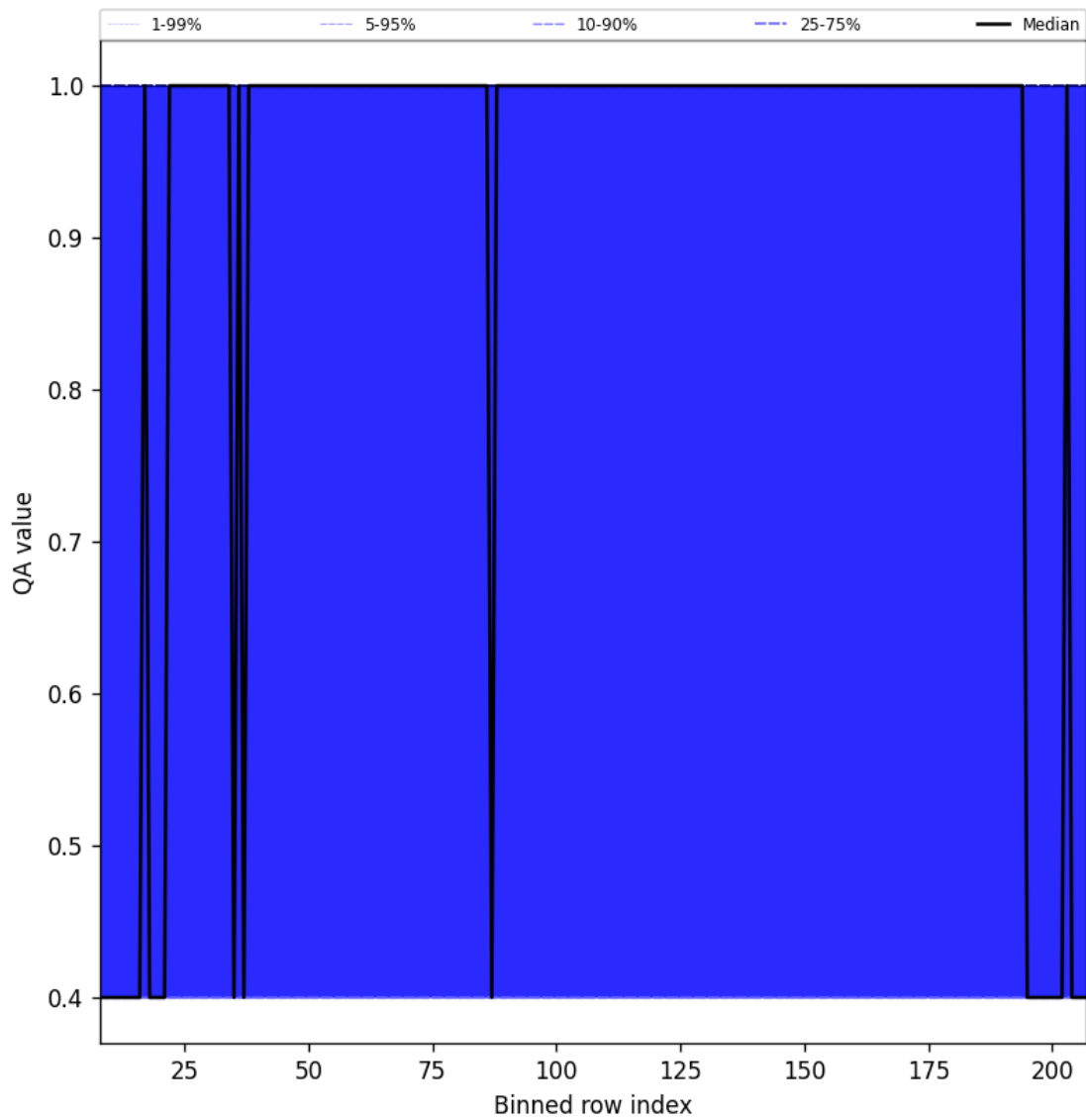
Figure 33: Along track statistics of “QA value” for 2025-02-09 to 2025-02-11
