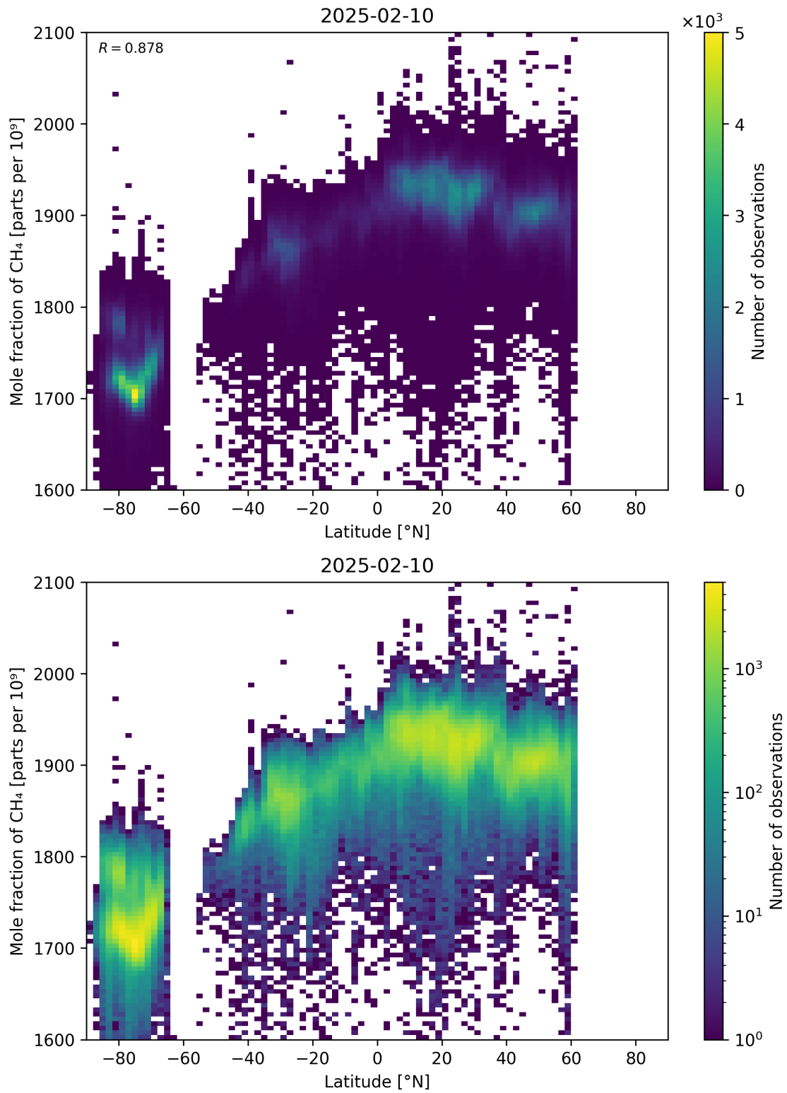
Figure 57: Scatter density plot of “Latitude” against “Mole fraction of CH 4 ” for 2025-02-09 to 2025-02-11.
