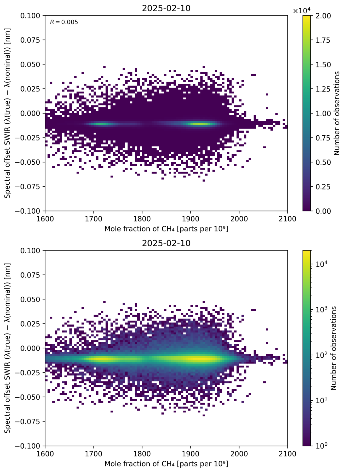
Figure 86: Scatter density plot of “Mole fraction of \text{CH}_4 ” against “Spectral offset SWIR ( \lambda_{\text{true}} - \lambda_{\text{nominal}} )” for 2025-02-09 to 2025-02-11.
