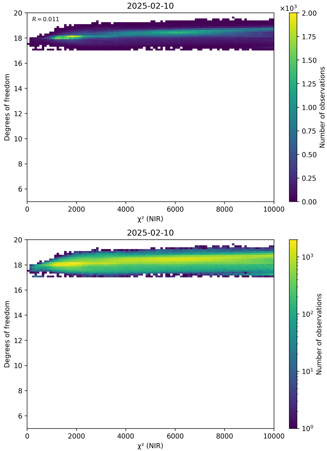
Figure 44: Scatter density plot of “ \chi^2 (NIR)” against “Degrees of freedom” for 2025-02-09 to 2025-02-11.
