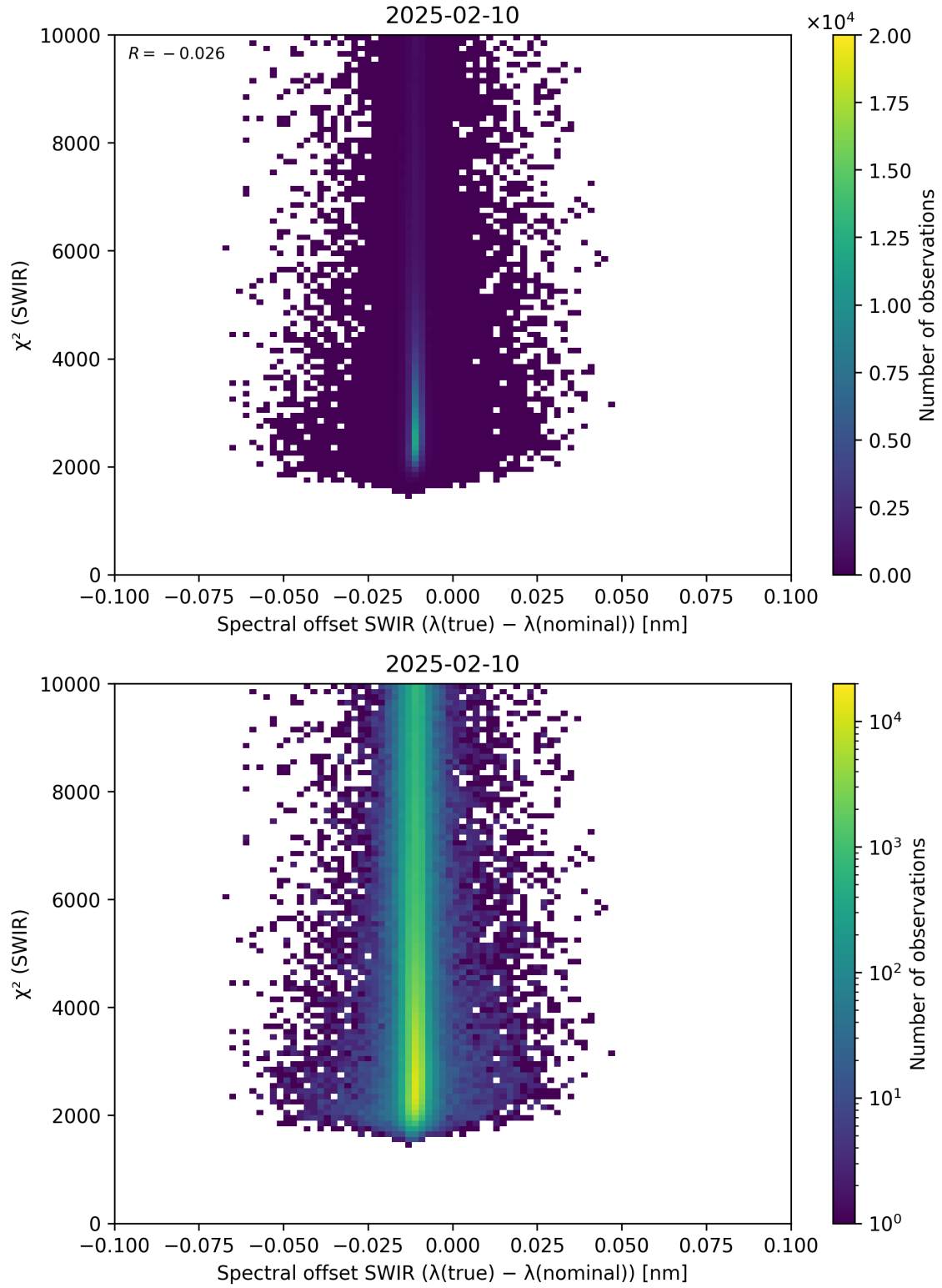
Figure 118: Scatter density plot of “Spectral offset SWIR ( \lambda_{\text{true}} - \lambda_{\text{nominal}} )” against “ \chi^2 (SWIR)” for 2025-02-09 to 2025-02-11.
