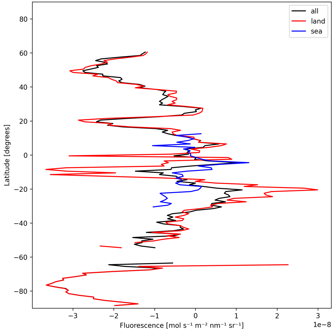
Figure 21: Zonal average of “Fluorescence” for 2025-02-09 to 2025-02-11.
