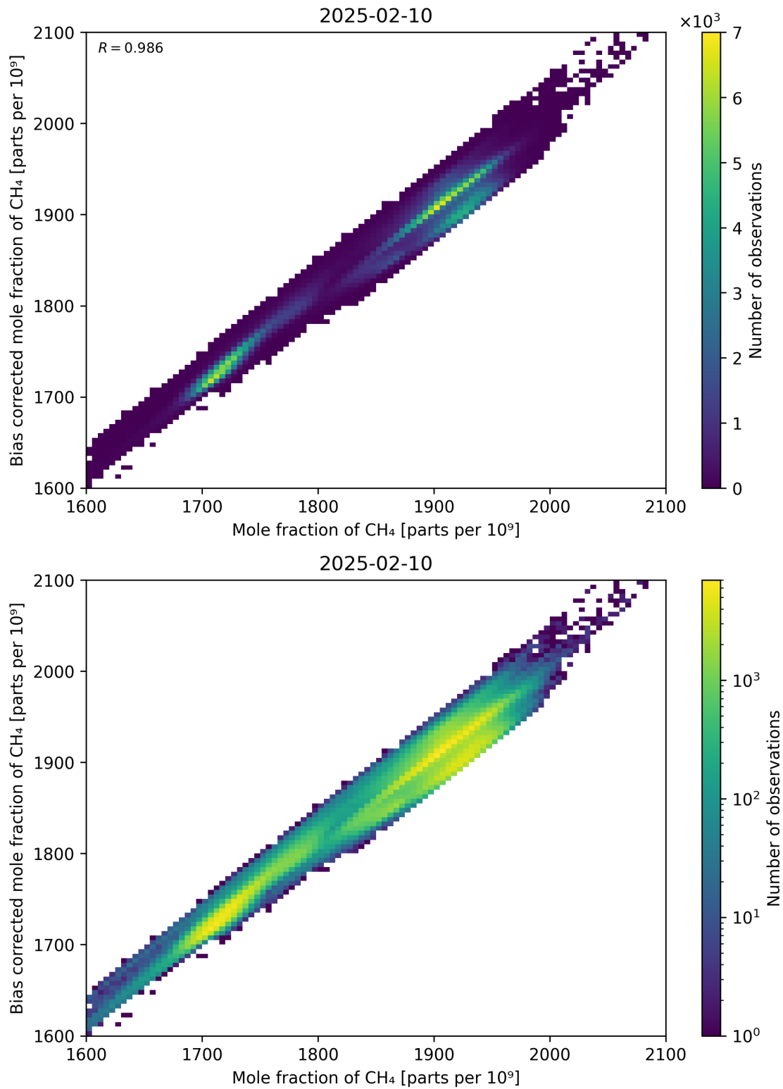
Figure 74: Scatter density plot of “Mole fraction of CH 4 ” against “Bias corrected mole fraction of CH 4 ” for 2025-02-09 to 2025-02-11.
