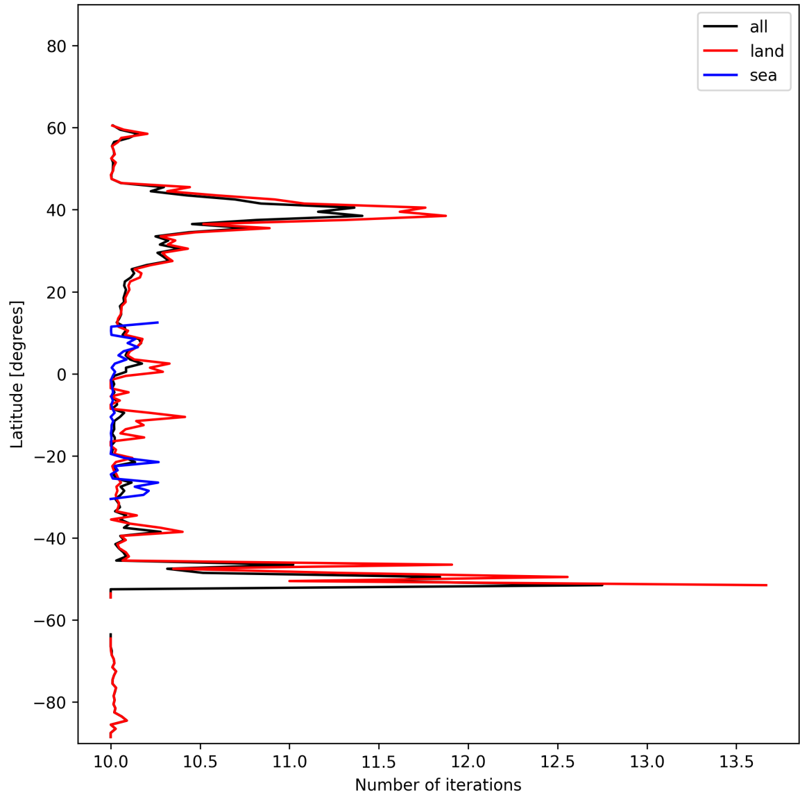
Figure 20: Zonal average of “Number of iterations” for 2025-02-09 to 2025-02-11.
