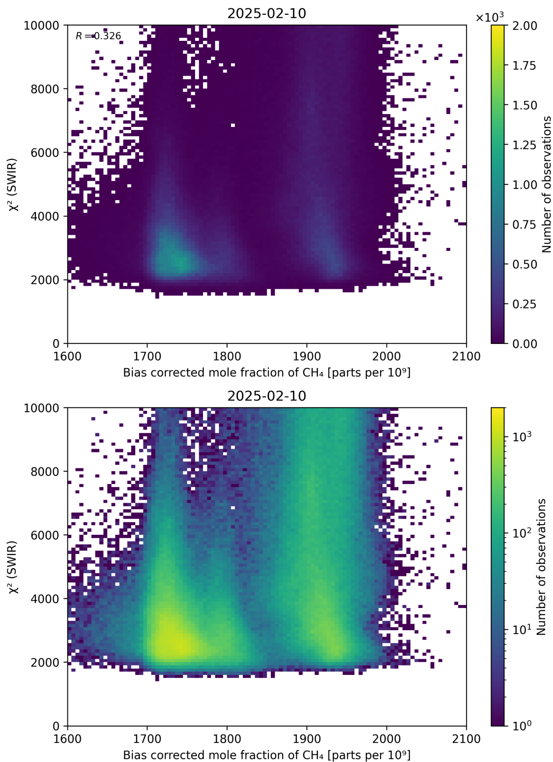
Figure 64: Scatter density plot of “Bias corrected mole fraction of \text{CH}_4 ” against “ \chi^2 (SWIR)” for 2025-02-09 to 2025-02-11.
