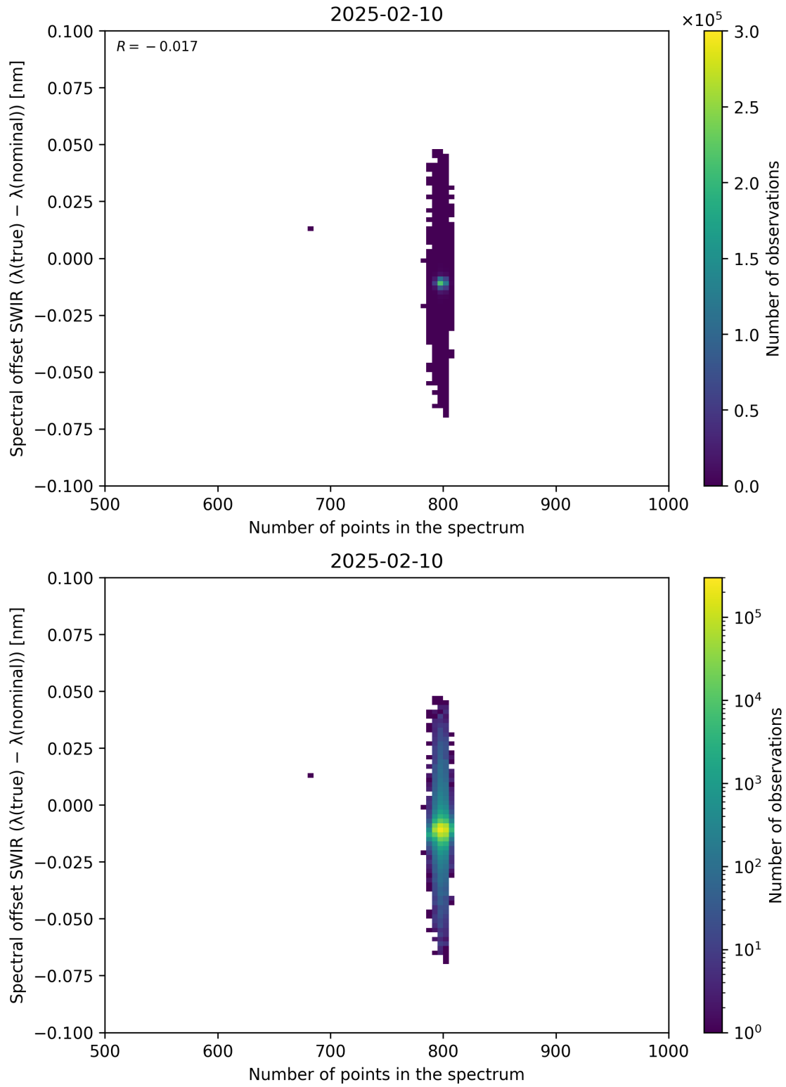
Figure 93: Scatter density plot of “Number of points in the spectrum” against “Spectral offset SWIR ( \lambda_{\text{true}} - \lambda_{\text{nominal}} )” for 2025-02-09 to 2025-02-11.
