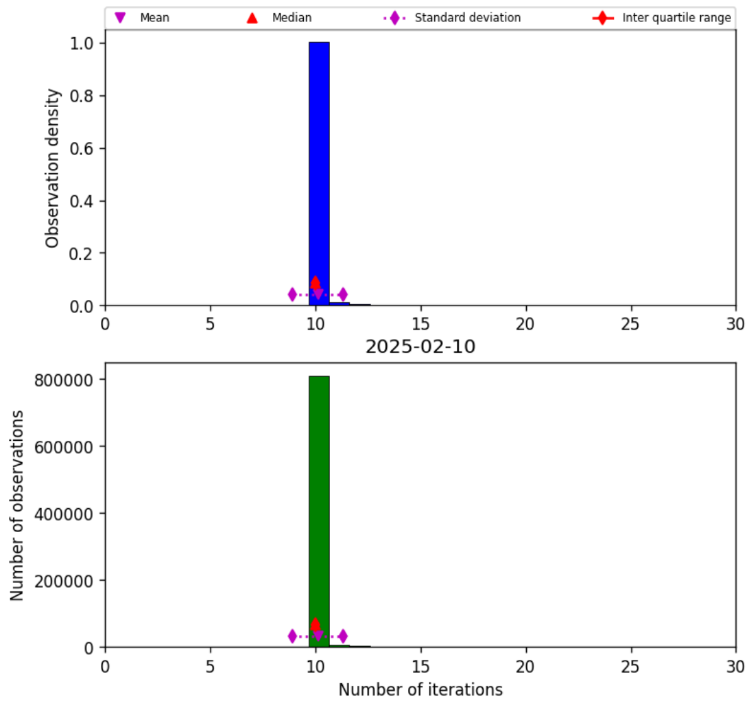
Figure 31: Histogram of “Number of iterations” for 2025-02-09 to 2025-02-11
