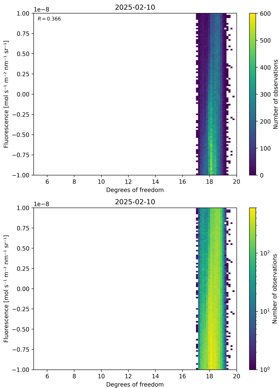
Figure 51: Scatter density plot of “Degrees of freedom” against “Fluorescence” for 2025-02-09 to 2025-02-11.
