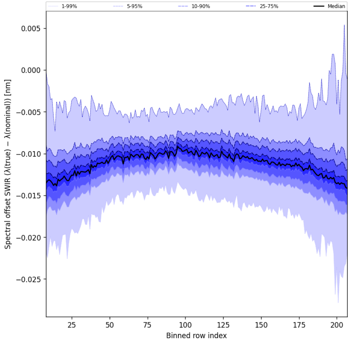
Figure 38: Along track statistics of “Spectral offset SWIR ( \lambda_{\text{true}} - \lambda_{\text{nominal}} )” for 2025-02-09 to 2025-02-11
