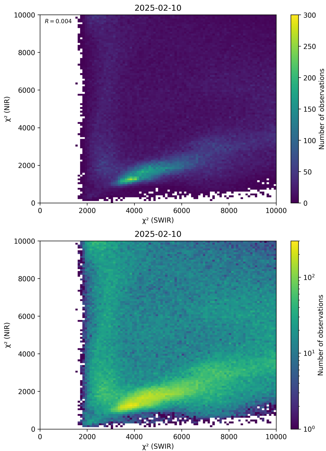
Figure 47: Scatter density plot of “ \chi^2 (SWIR)” against “ \chi^2 (NIR)” for 2025-02-09 to 2025-02-11.
