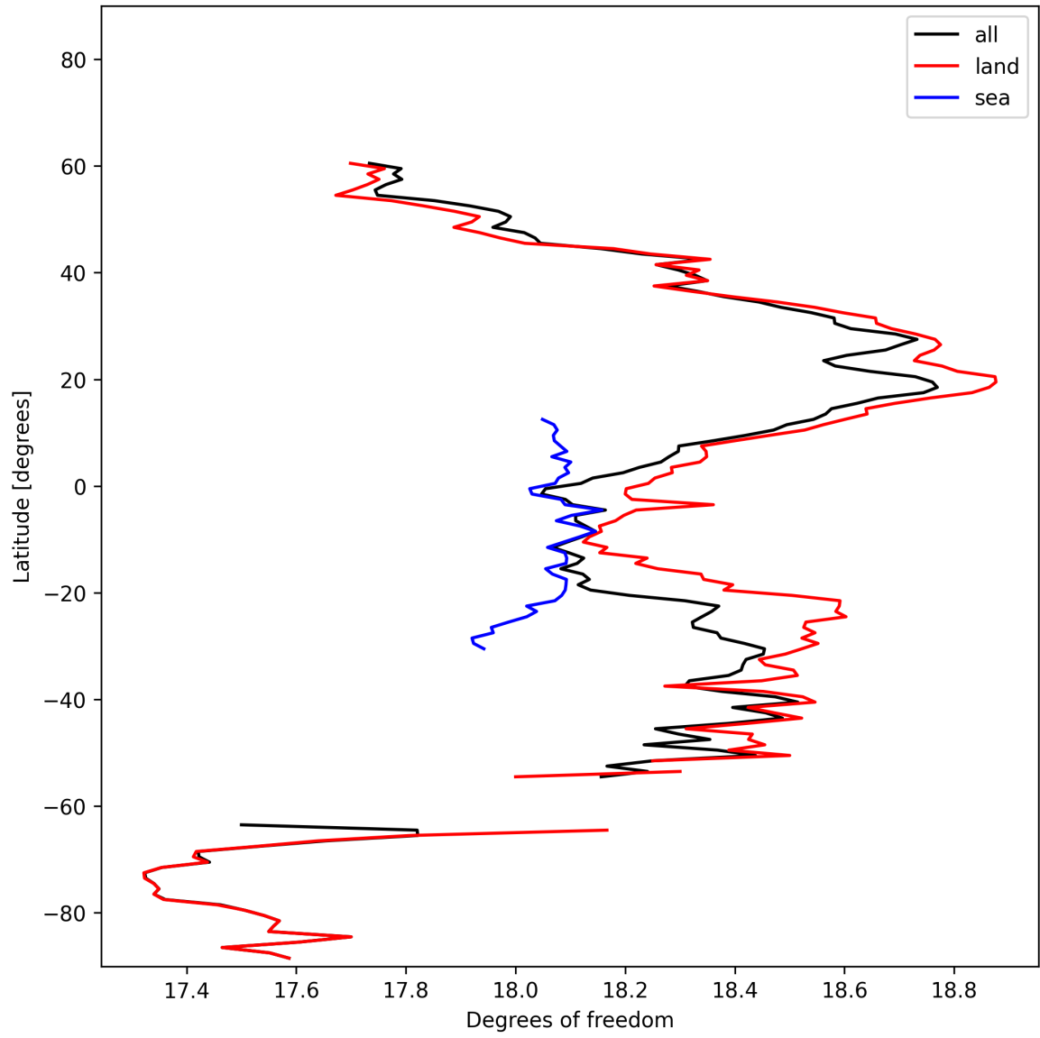
Figure 19: Zonal average of “Degrees of freedom” for 2025-02-09 to 2025-02-11.
