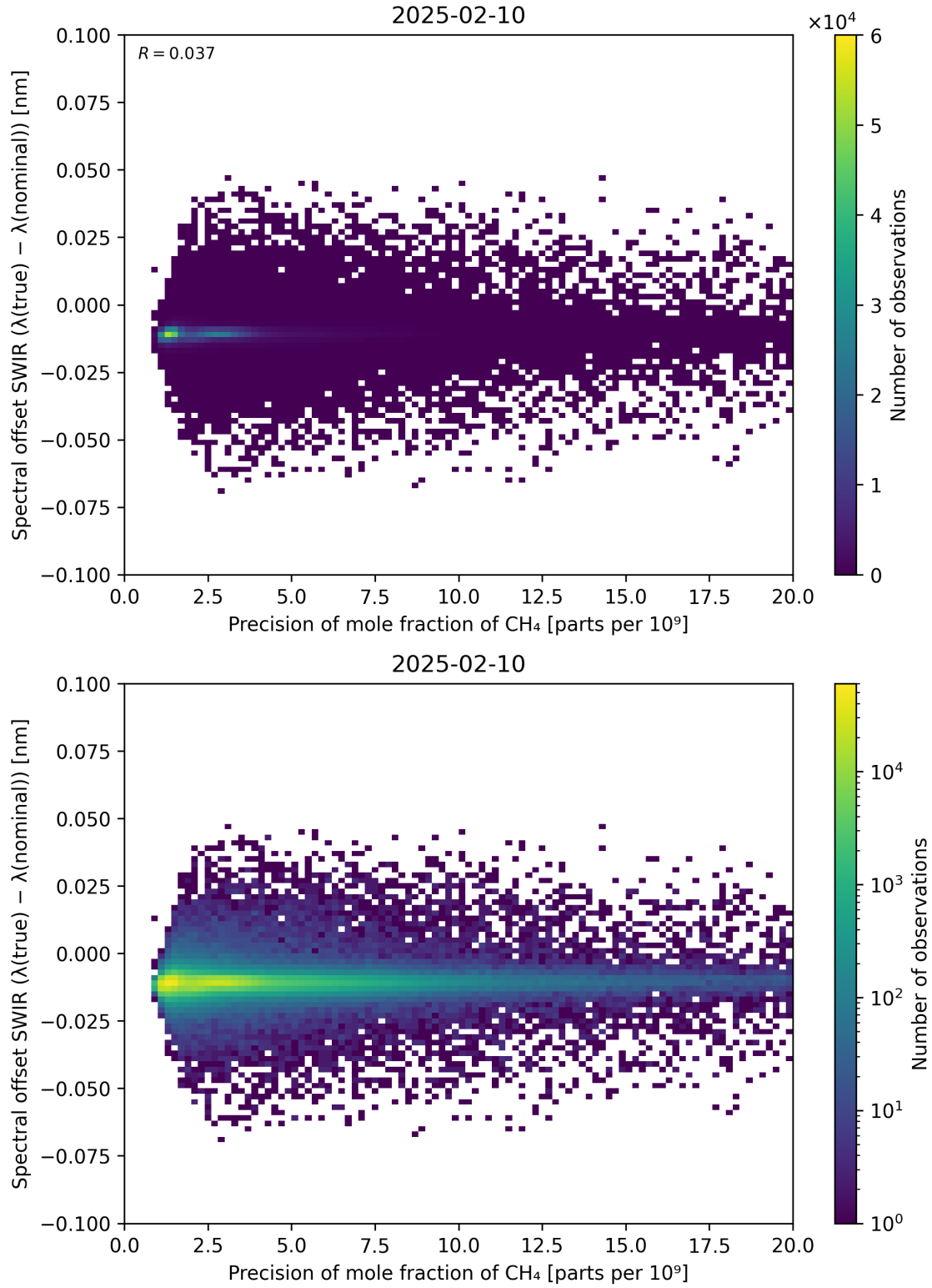
Figure 85: Scatter density plot of “Precision of mole fraction of \text{CH}_4 ” against “Spectral offset SWIR ( \lambda_{\text{true}} - \lambda_{\text{nominal}} )” for 2025-02-09 to 2025-02-11.
