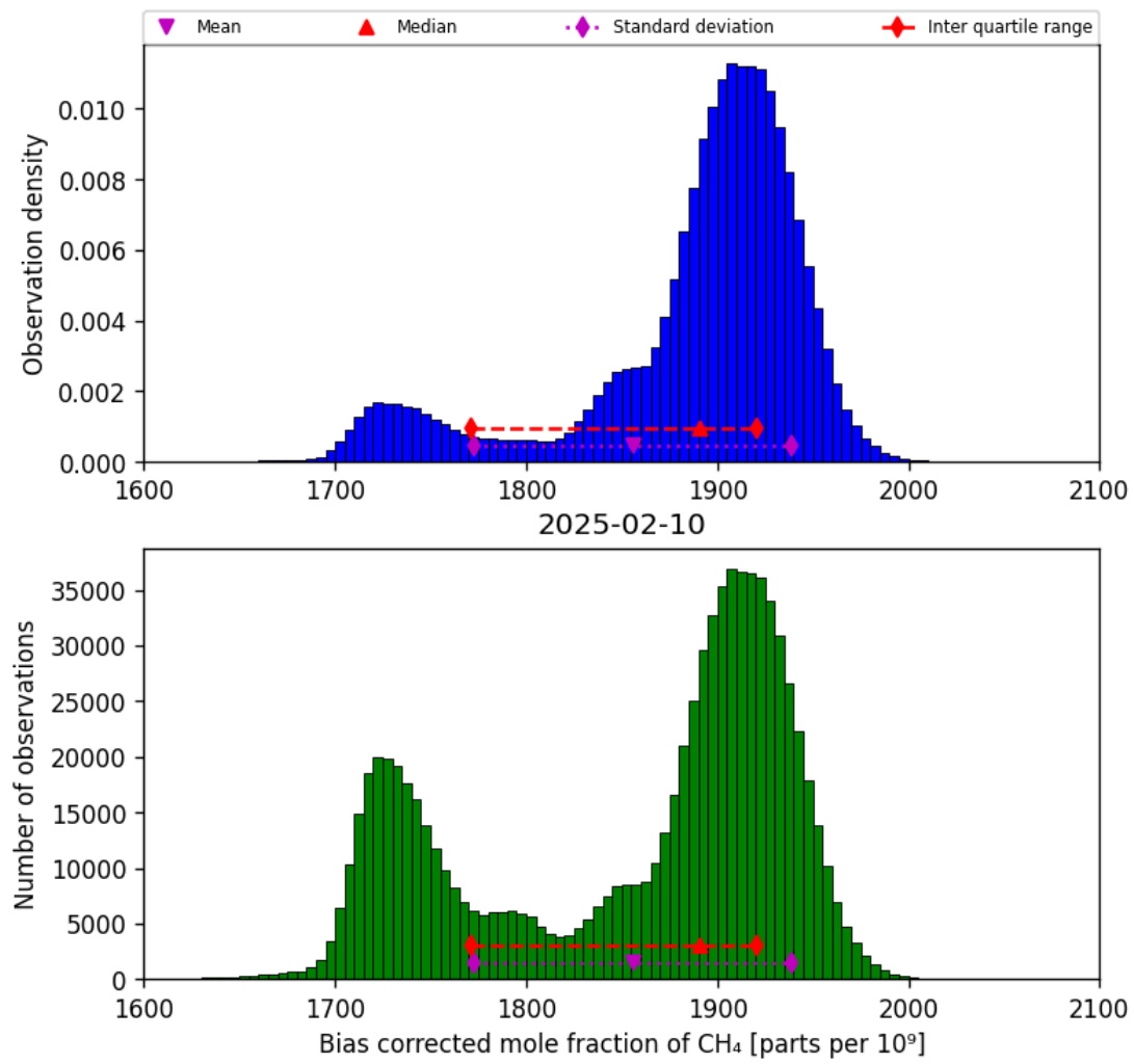
Figure 25: Histogram of “Bias corrected mole fraction of CH 4 ” for 2025-02-09 to 2025-02-11
