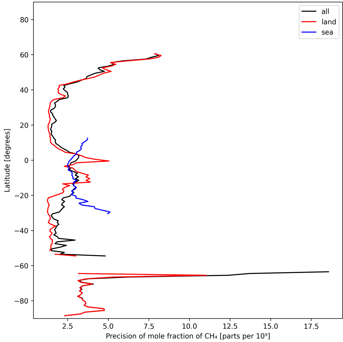
Figure 13: Zonal average of “Precision of mole fraction of CH 4 ” for 2025-02-09 to 2025-02-11.
