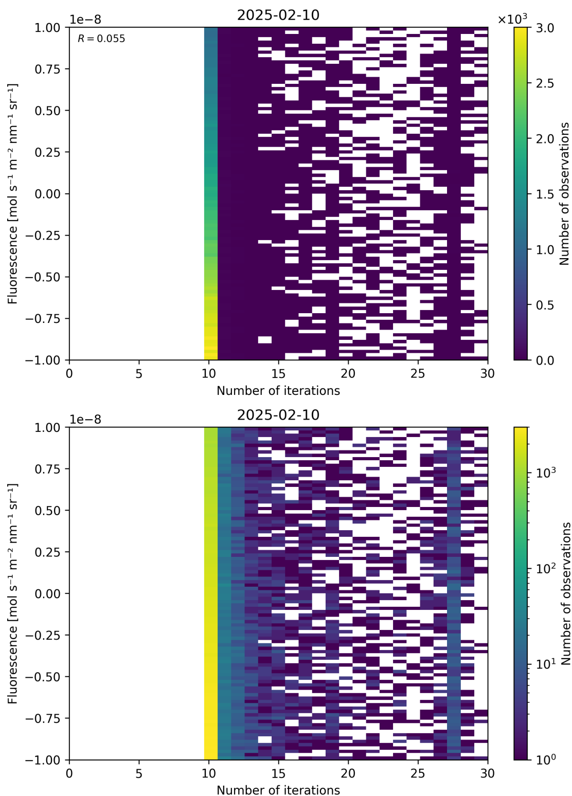
Figure 87: Scatter density plot of “Number of iterations” against “Fluorescence” for 2025-02-09 to 2025-02-11.
