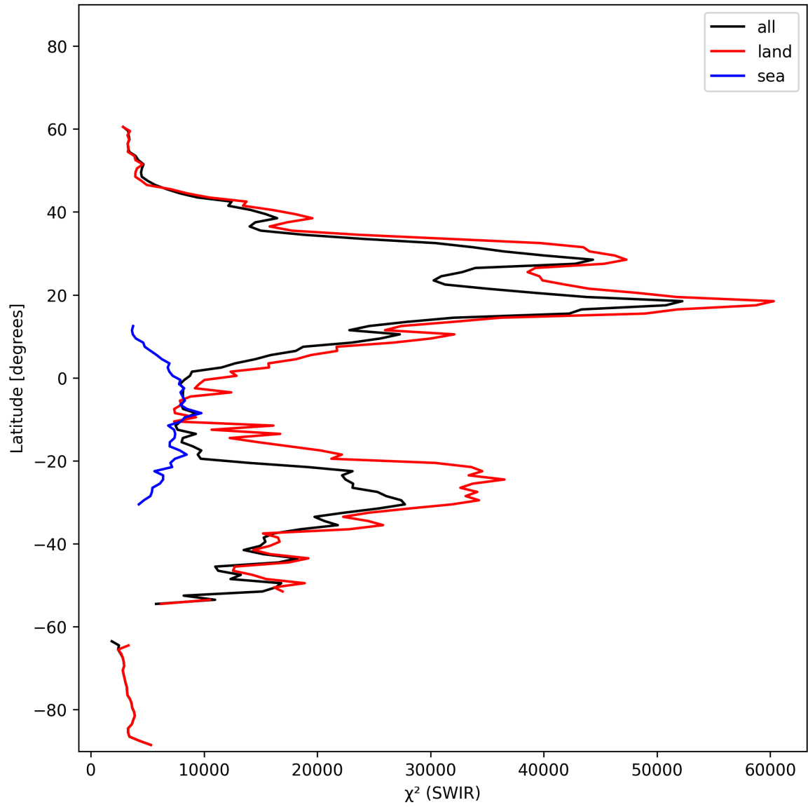
Figure 17: Zonal average of “ \chi^2 (SWIR)” for 2025-02-09 to 2025-02-11.
