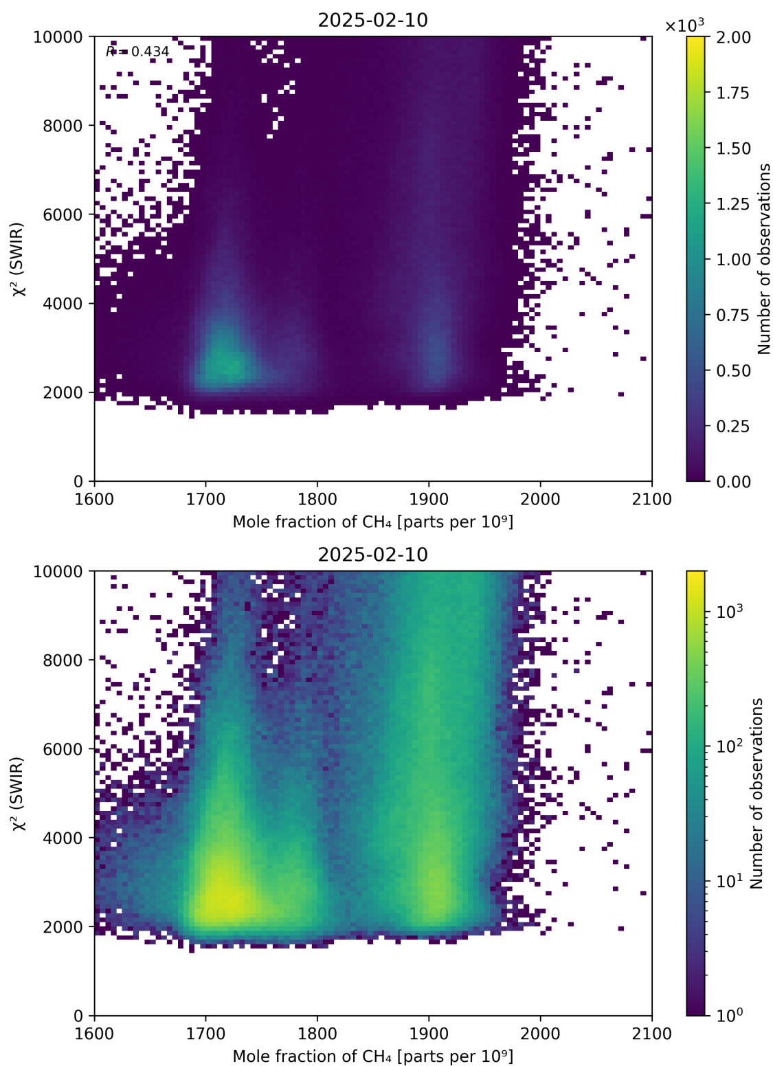
Figure 71: Scatter density plot of “Mole fraction of CH 4 ” against “ \chi^2 (SWIR)” for 2025-02-09 to 2025-02-11.
