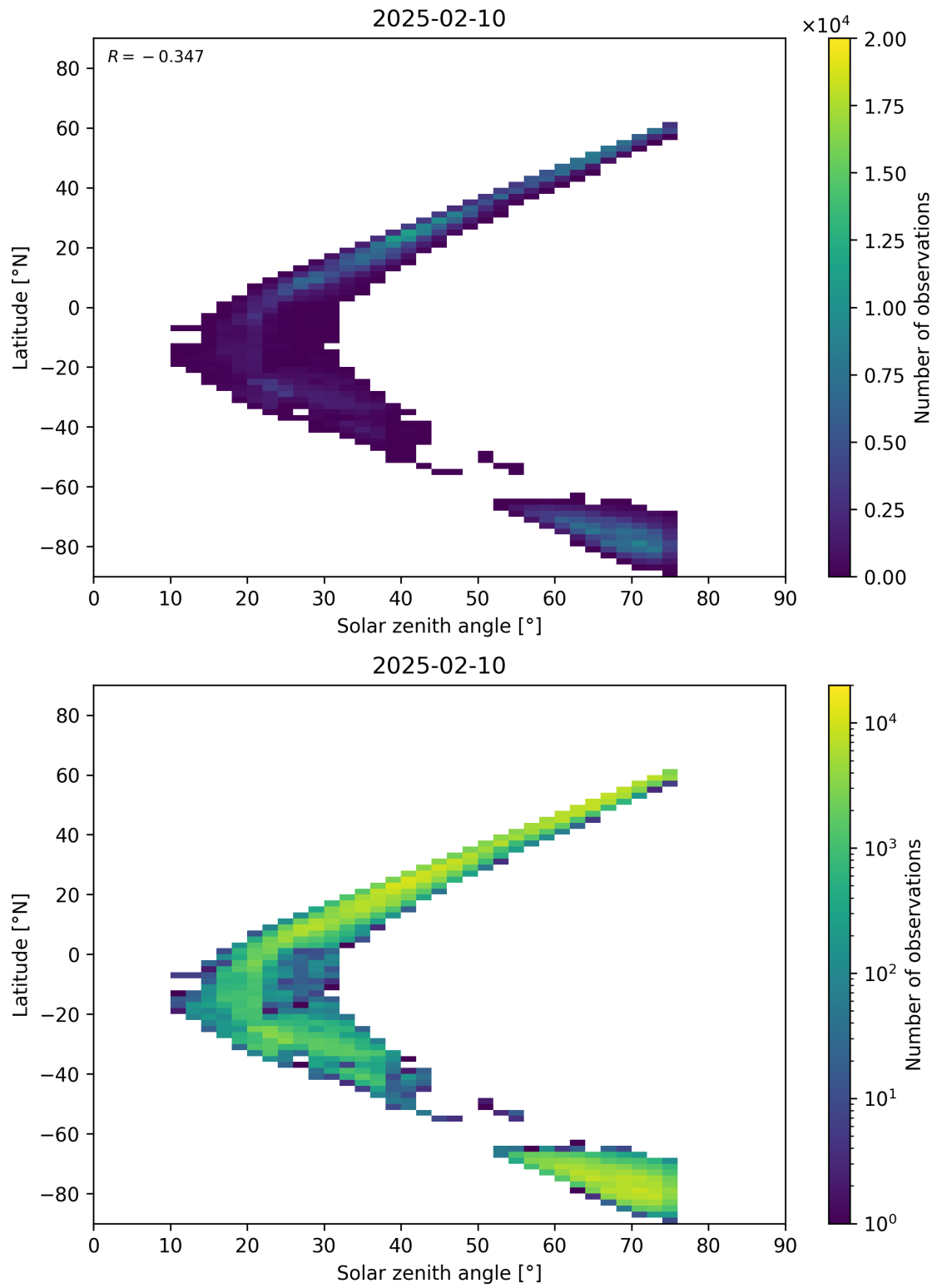
Figure 98: Scatter density plot of “Solar zenith angle” against “Latitude” for 2025-02-09 to 2025-02-11.
