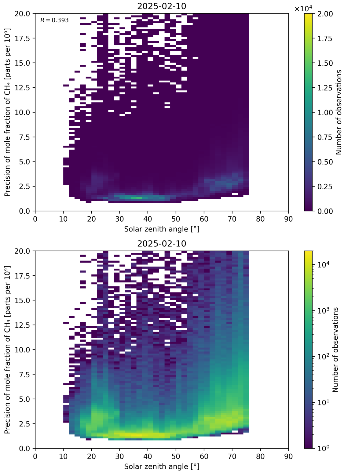
Figure 101: Scatter density plot of “Solar zenith angle” against “Precision of mole fraction of CH 4 ” for 2025-02-09 to 2025-02-11.
