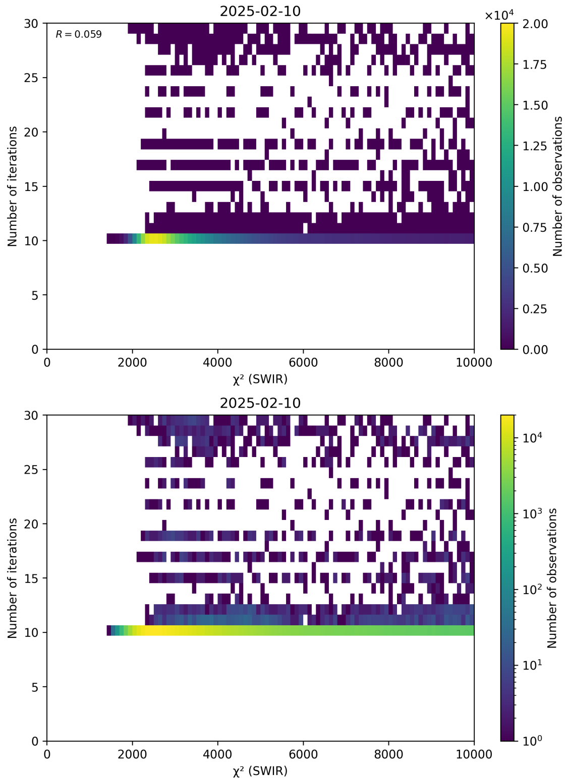
Figure 50: Scatter density plot of “ \chi^2 (SWIR)” against “Number of iterations” for 2025-02-09 to 2025-02-11.
