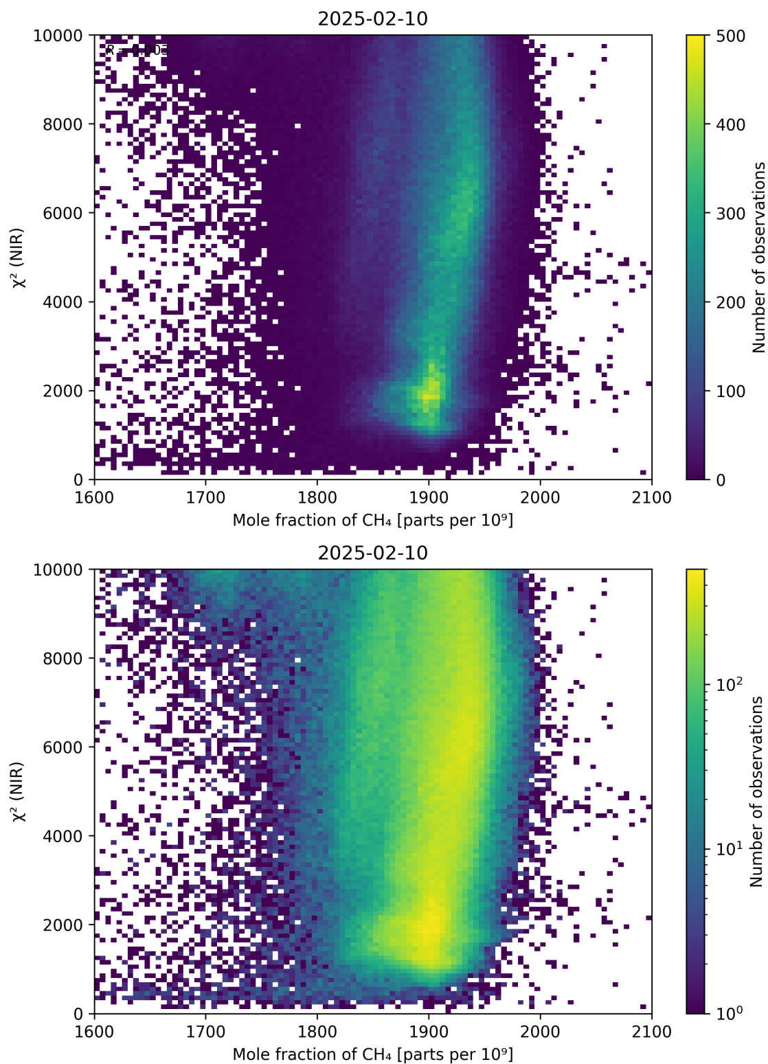
Figure 70: Scatter density plot of “Mole fraction of CH 4 ” against “ \chi^2 (NIR)” for 2025-02-09 to 2025-02-11.
