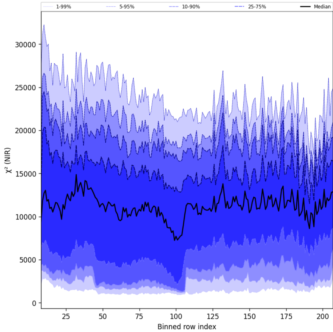
Figure 40: Along track statistics of “ \chi^2 (NIR)” for 2025-02-09 to 2025-02-11
