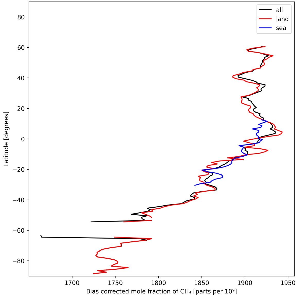
Figure 14: Zonal average of “Bias corrected mole fraction of \text{CH}_4 ” for 2025-02-09 to 2025-02-11.
