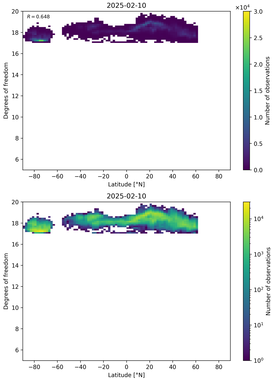
Figure 55: Scatter density plot of “Latitude” against “Degrees of freedom” for 2025-02-09 to 2025-02-11.
