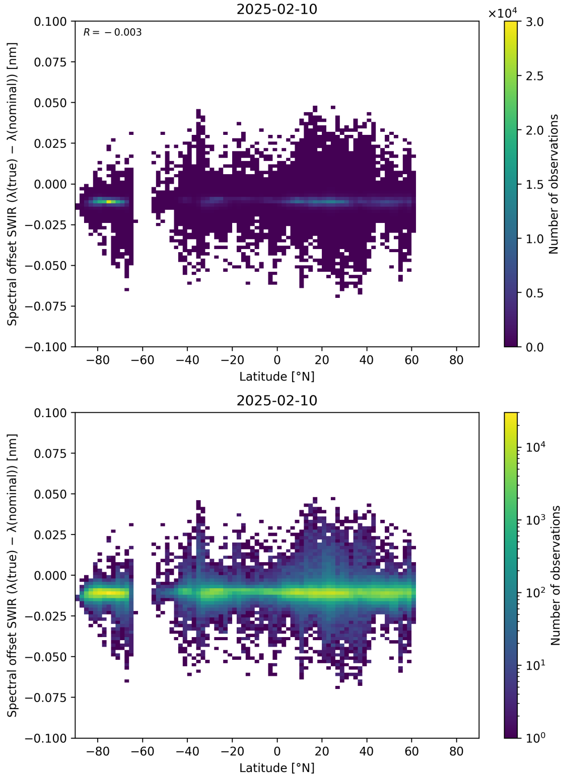
Figure 62: Scatter density plot of “Latitude” against “Spectral offset SWIR ( \lambda_{\text{true}} - \lambda_{\text{nominal}} )” for 2025-02-09 to 2025-02-11.
