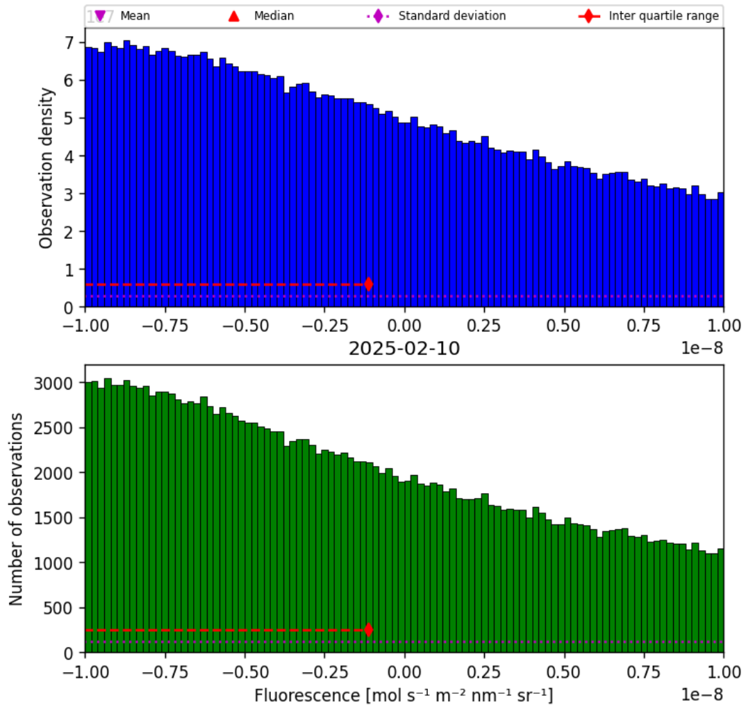
Figure 32: Histogram of “Fluorescence” for 2025-02-09 to 2025-02-11
