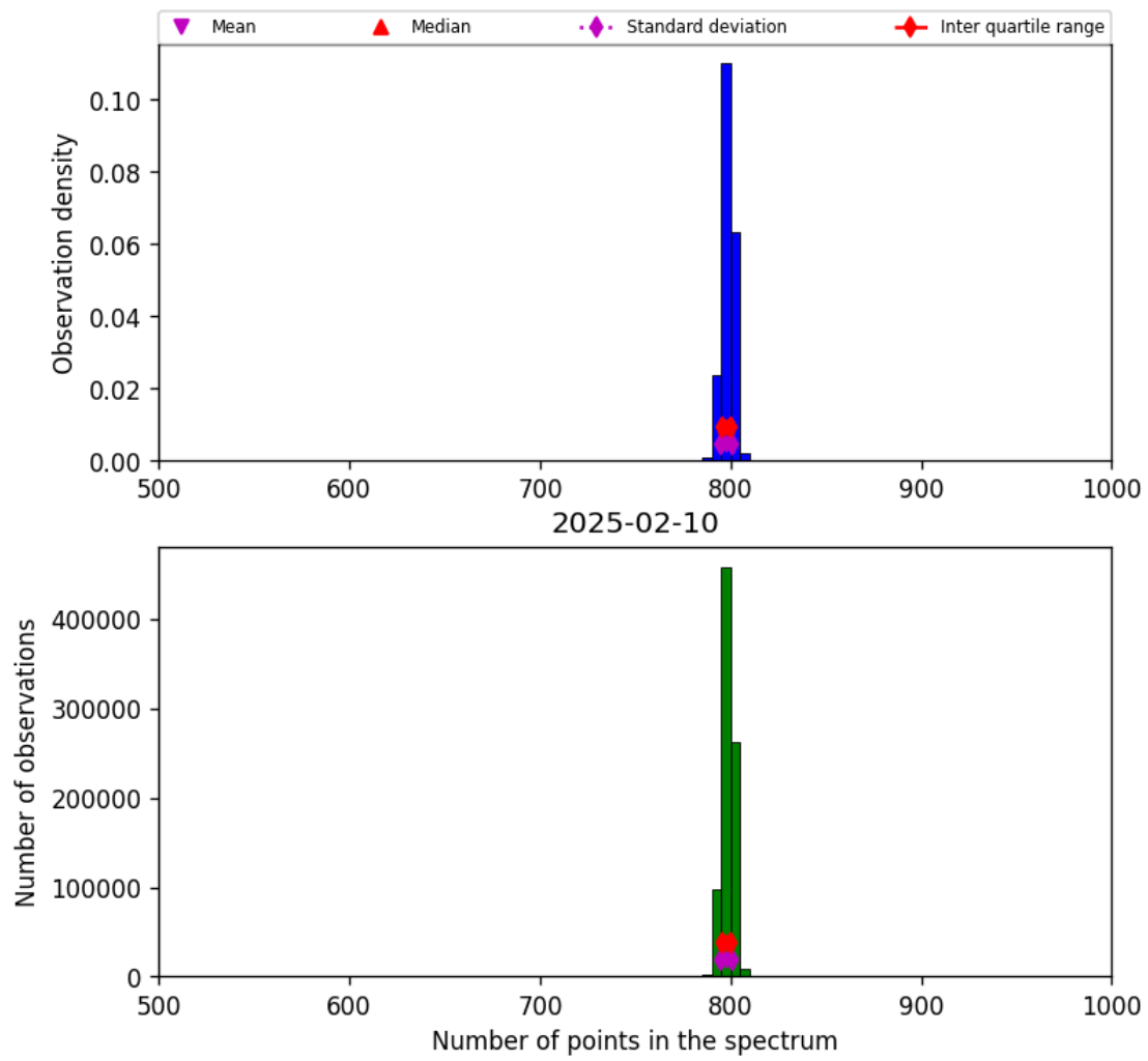
Figure 26: Histogram of “Number of points in the spectrum” for 2025-02-09 to 2025-02-11
