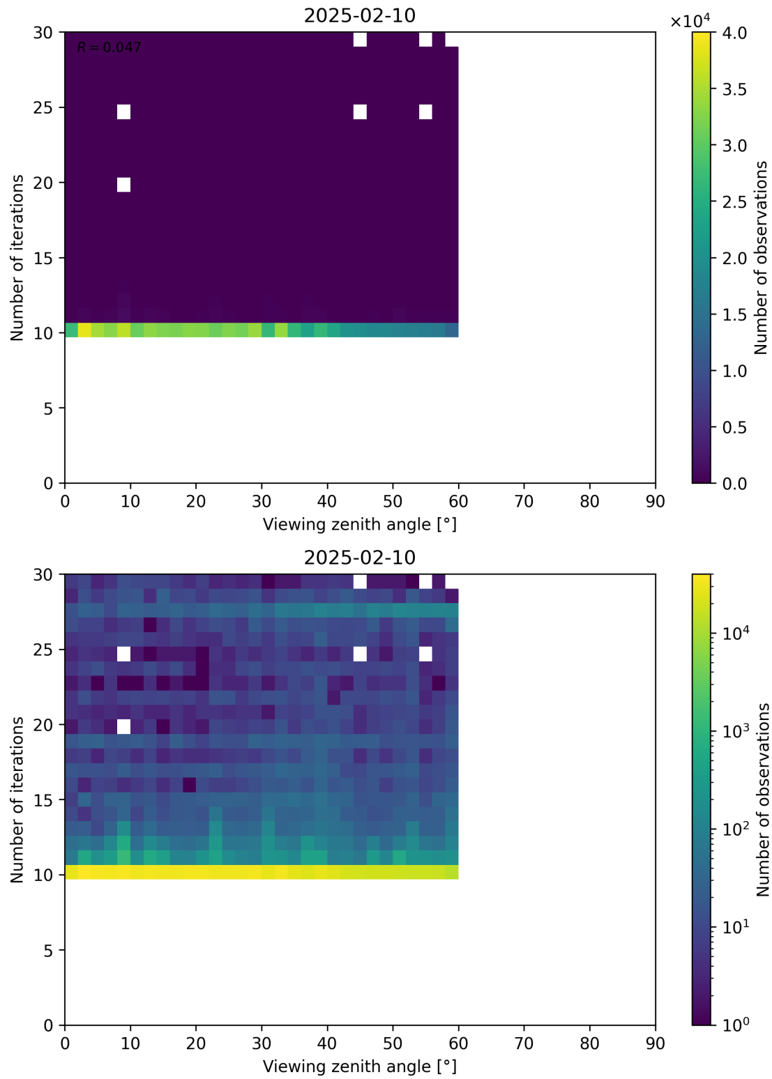
Figure 113: Scatter density plot of “Viewing zenith angle” against “Number of iterations” for 2025-02-09 to 2025-02-11.
