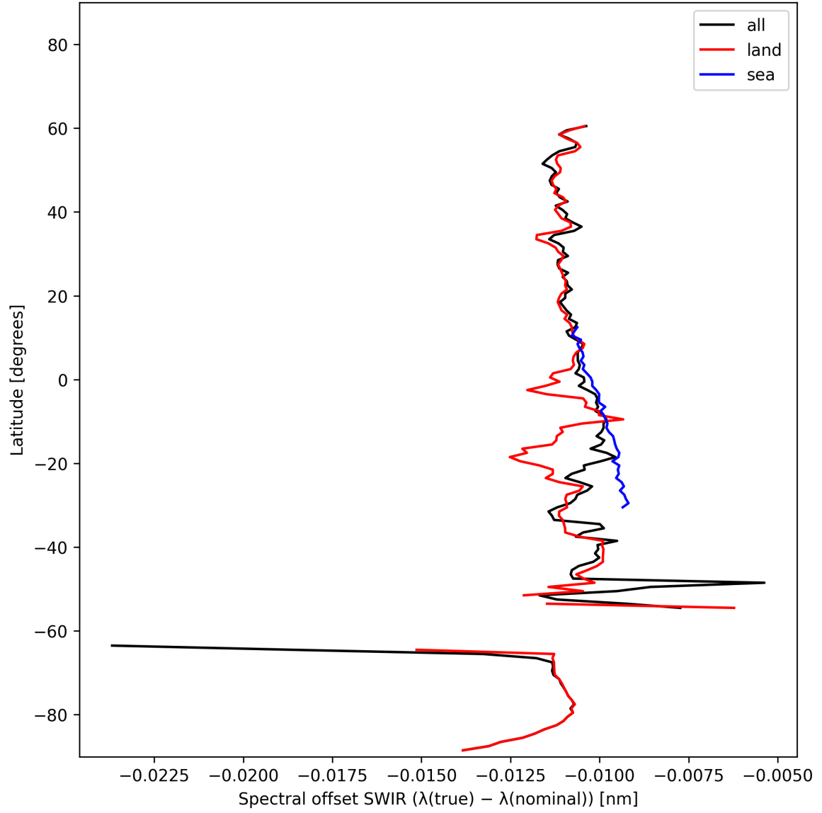
Figure 16: Zonal average of “Spectral offset SWIR ( \lambda_{\text{true}} - \lambda_{\text{nominal}} )” for 2025-02-09 to 2025-02-11.
