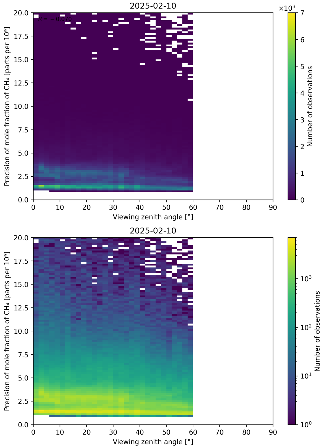
Figure 112: Scatter density plot of “Viewing zenith angle” against “Precision of mole fraction of CH 4 ” for 2025-02-09 to 2025-02-11.
