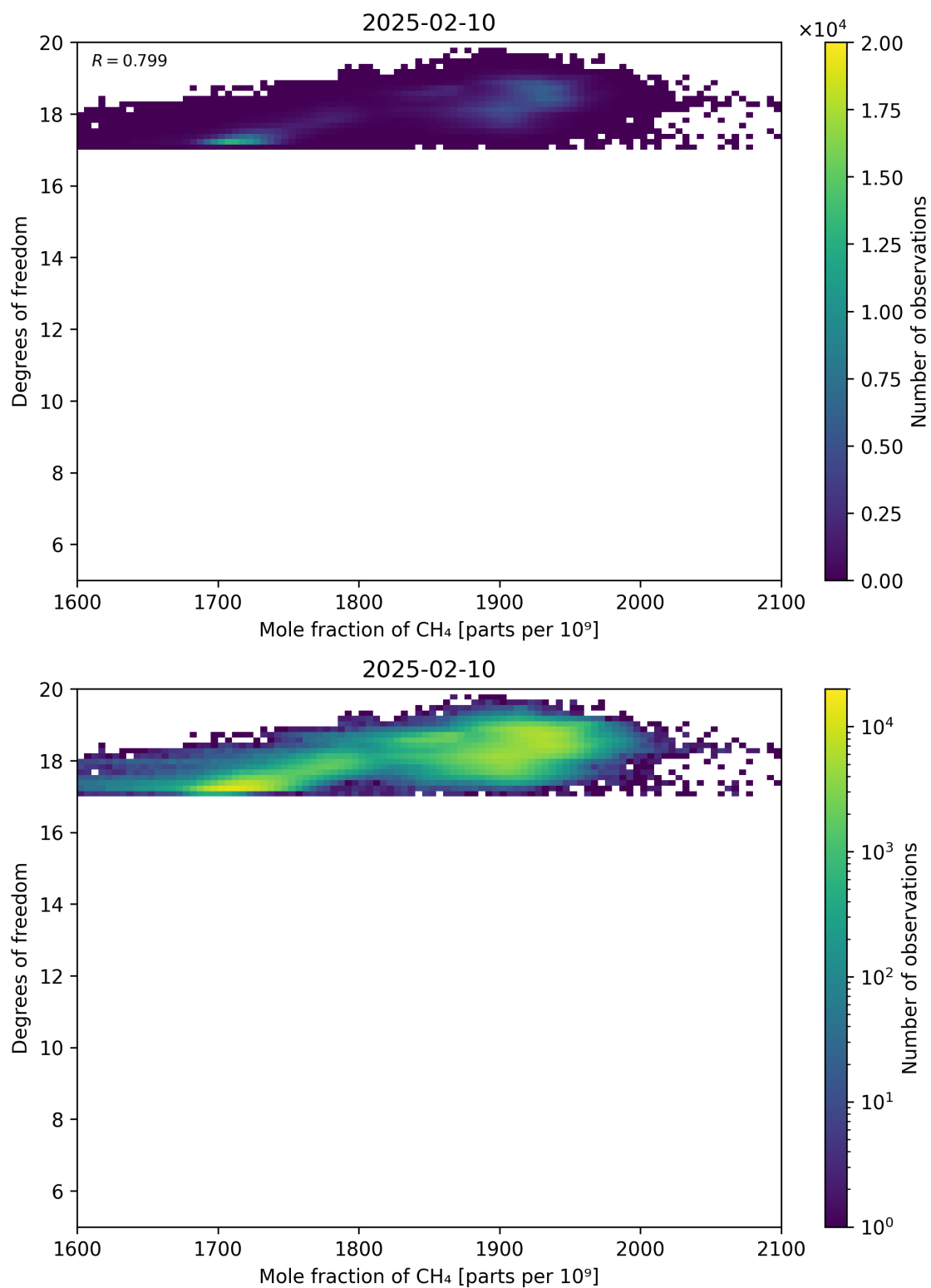
Figure 72: Scatter density plot of “Mole fraction of CH 4 ” against “Degrees of freedom” for 2025-02-09 to 2025-02-11.
