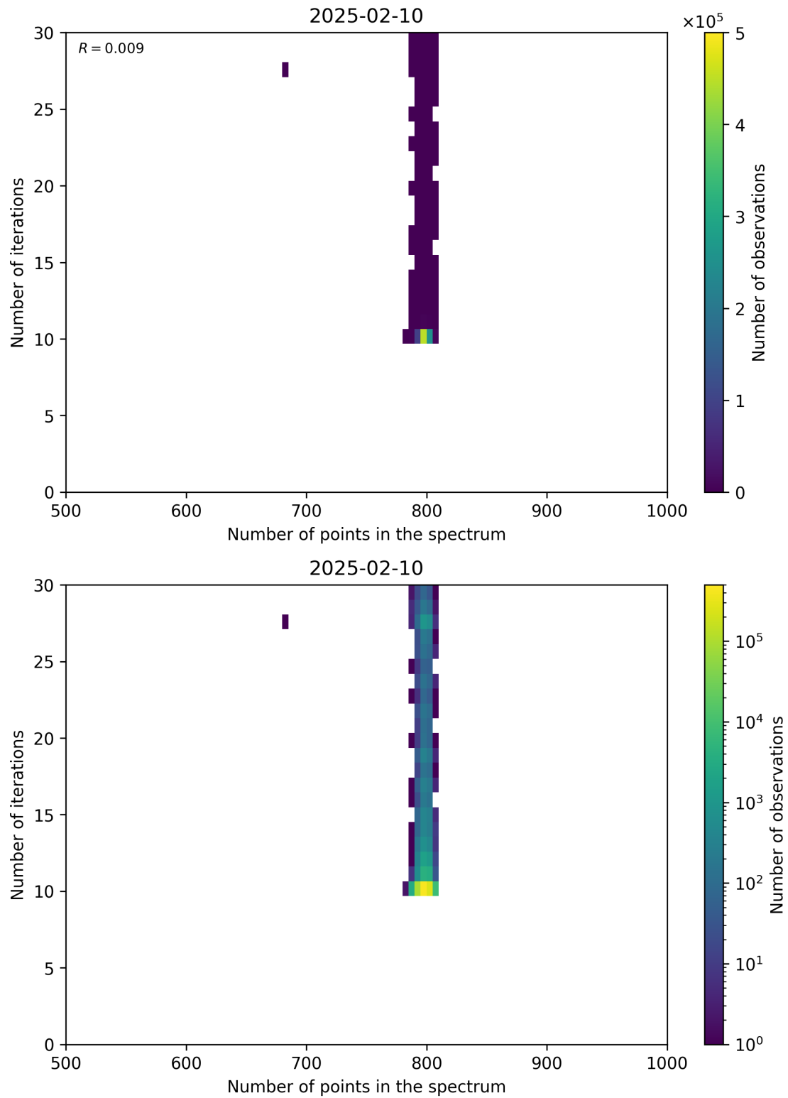
Figure 92: Scatter density plot of “Number of points in the spectrum” against “Number of iterations” for 2025-02-09 to 2025-02-11.
