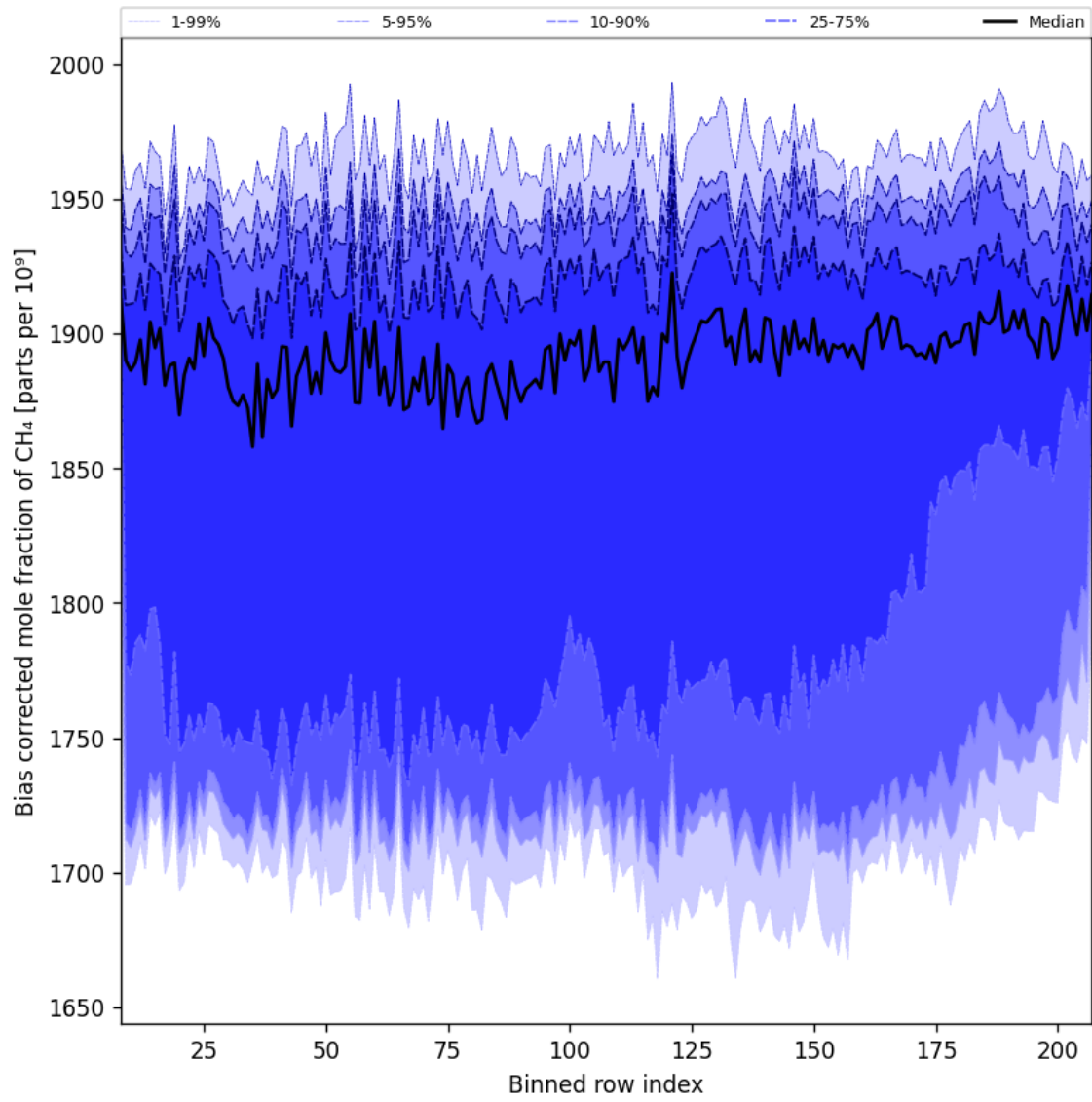
Figure 36: Along track statistics of “Bias corrected mole fraction of CH 4 ” for 2025-02-09 to 2025-02-11
