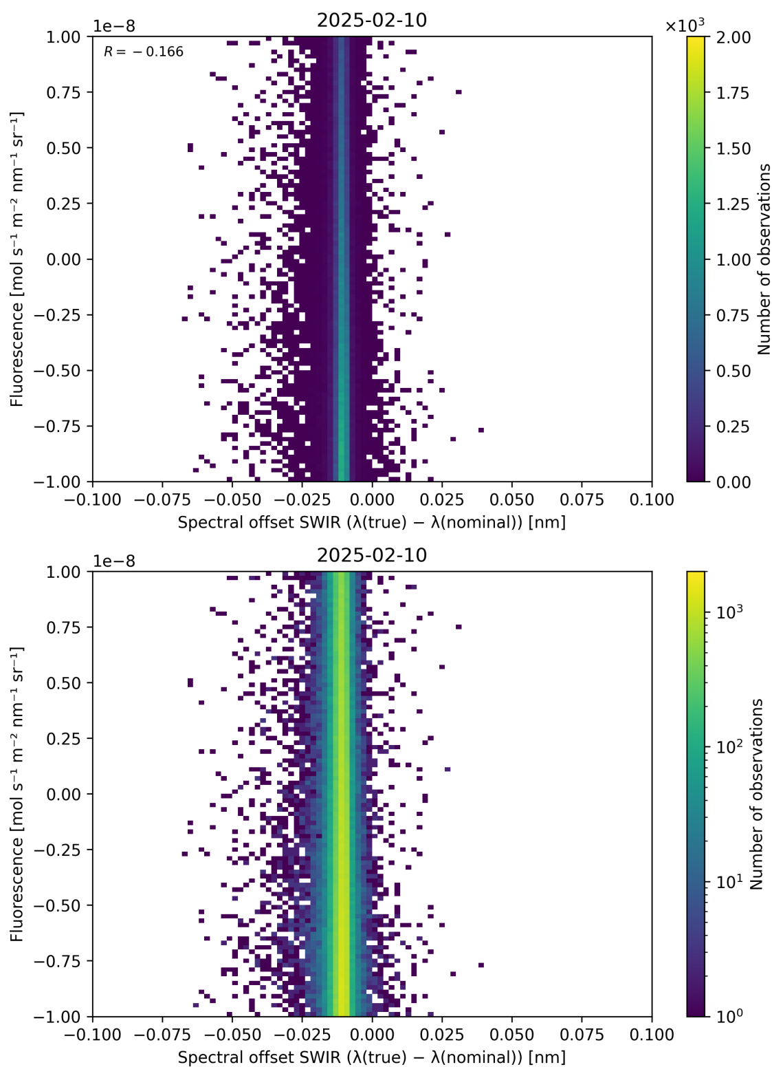
Figure 120: Scatter density plot of “Spectral offset SWIR ( \lambda_{\text{true}} - \lambda_{\text{nominal}} )” against “Fluorescence” for 2025-02-09 to 2025-02-11.
