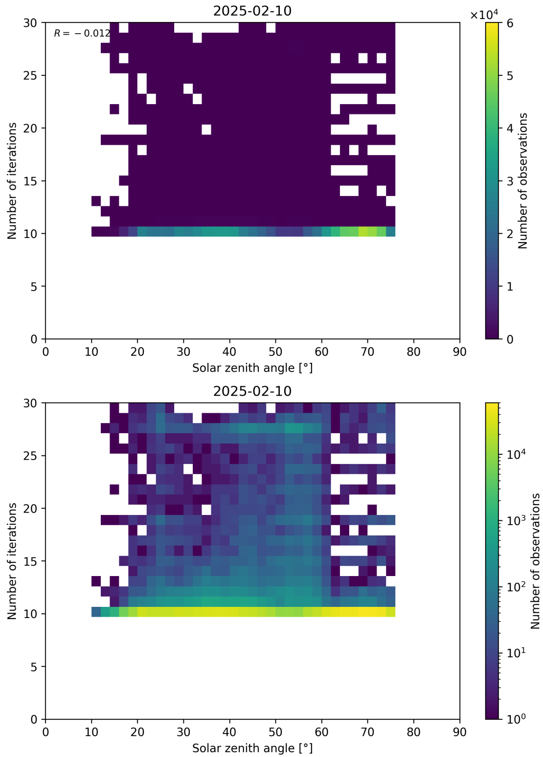
Figure 102: Scatter density plot of “Solar zenith angle” against “Number of iterations” for 2025-02-09 to 2025-02-11.
