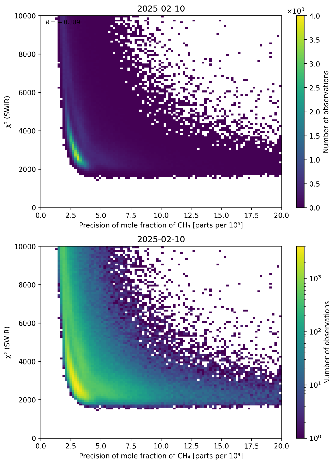
Figure 79: Scatter density plot of “Precision of mole fraction of \text{CH}_4 ” against “ \chi^2 (SWIR)” for 2025-02-09 to 2025-02-11.
