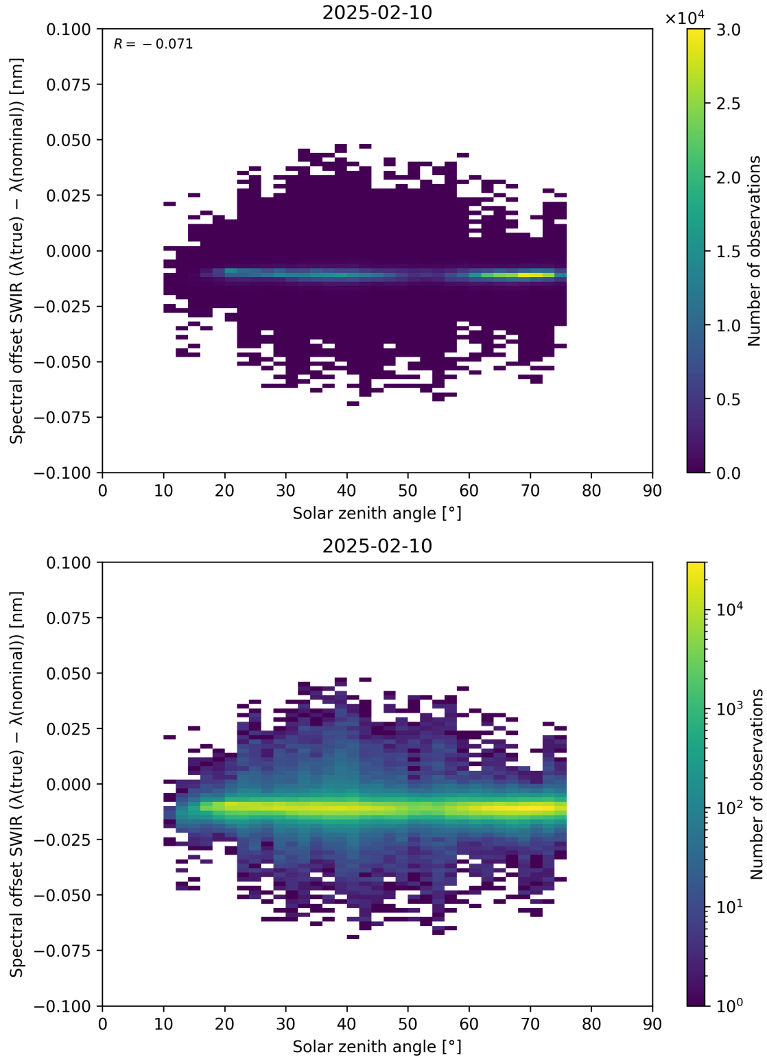
Figure 104: Scatter density plot of “Solar zenith angle” against “Spectral offset SWIR ( \lambda_{\text{true}} - \lambda_{\text{nominal}} )” for 2025-02-09 to 2025-02-11.
