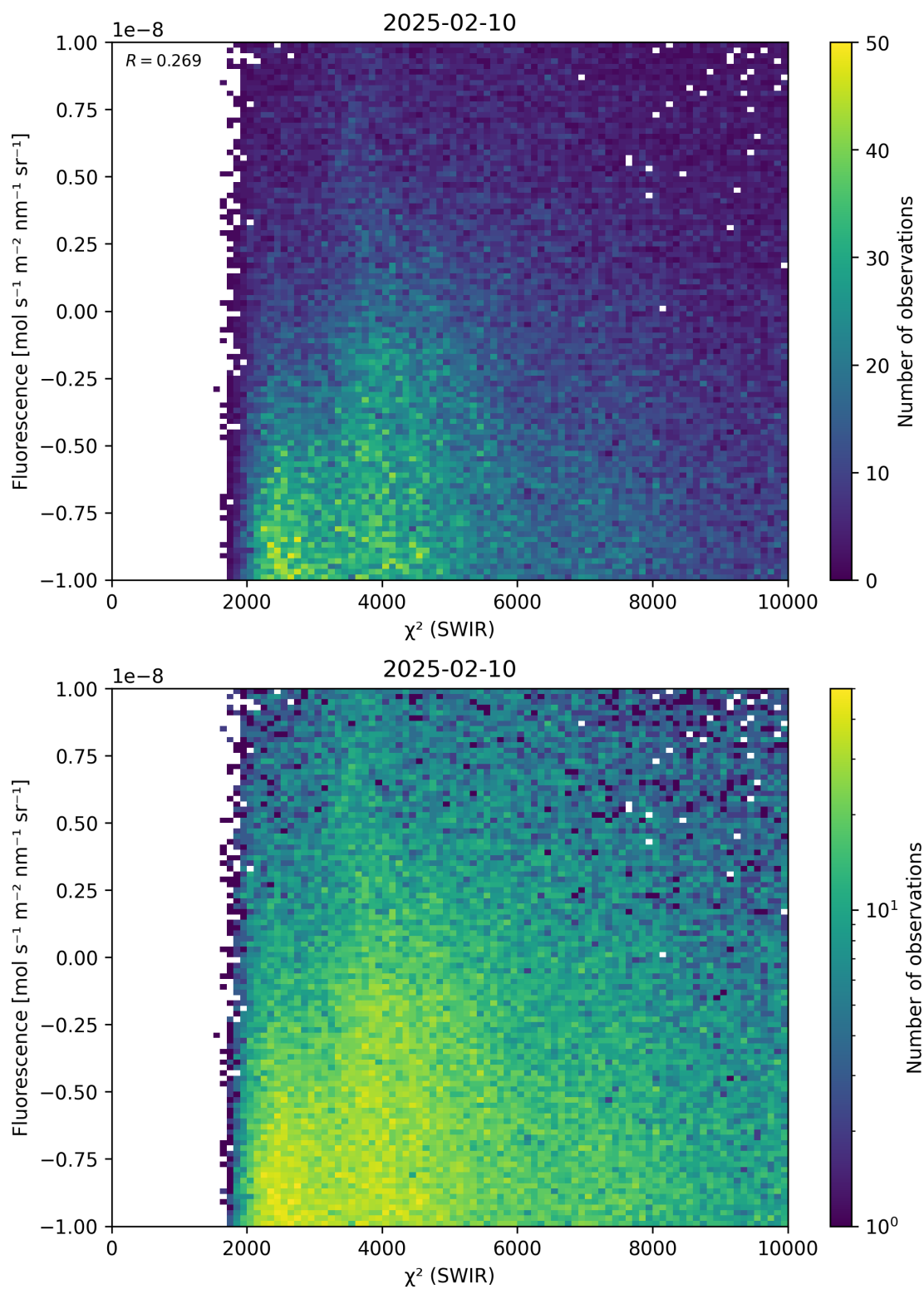
Figure 49: Scatter density plot of “ \chi^2 (SWIR)” against “Fluorescence” for 2025-02-09 to 2025-02-11.
