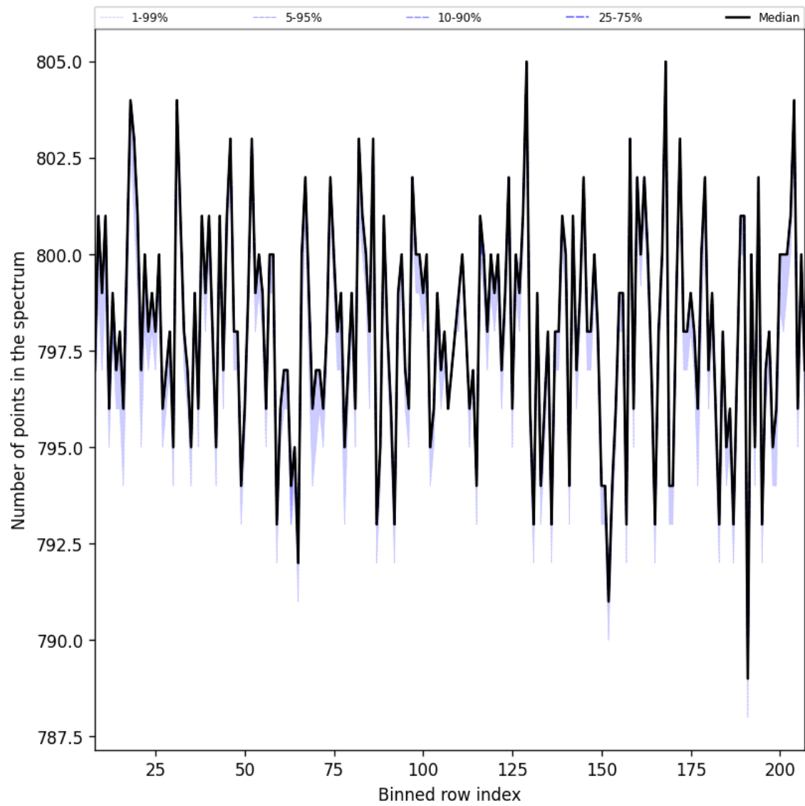
Figure 37: Along track statistics of “Number of points in the spectrum” for 2025-02-09 to 2025-02-11
