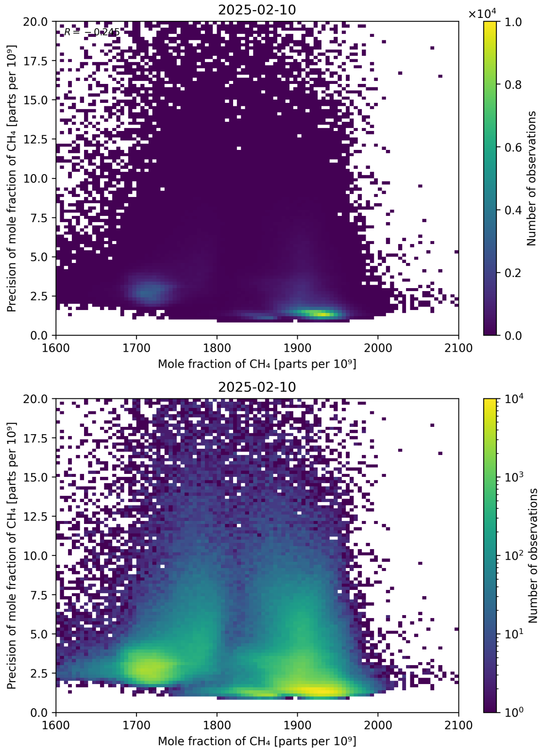
Figure 75: Scatter density plot of “Mole fraction of CH 4 ” against “Precision of mole fraction of CH 4 ” for 2025-02-09 to 2025-02-11.
