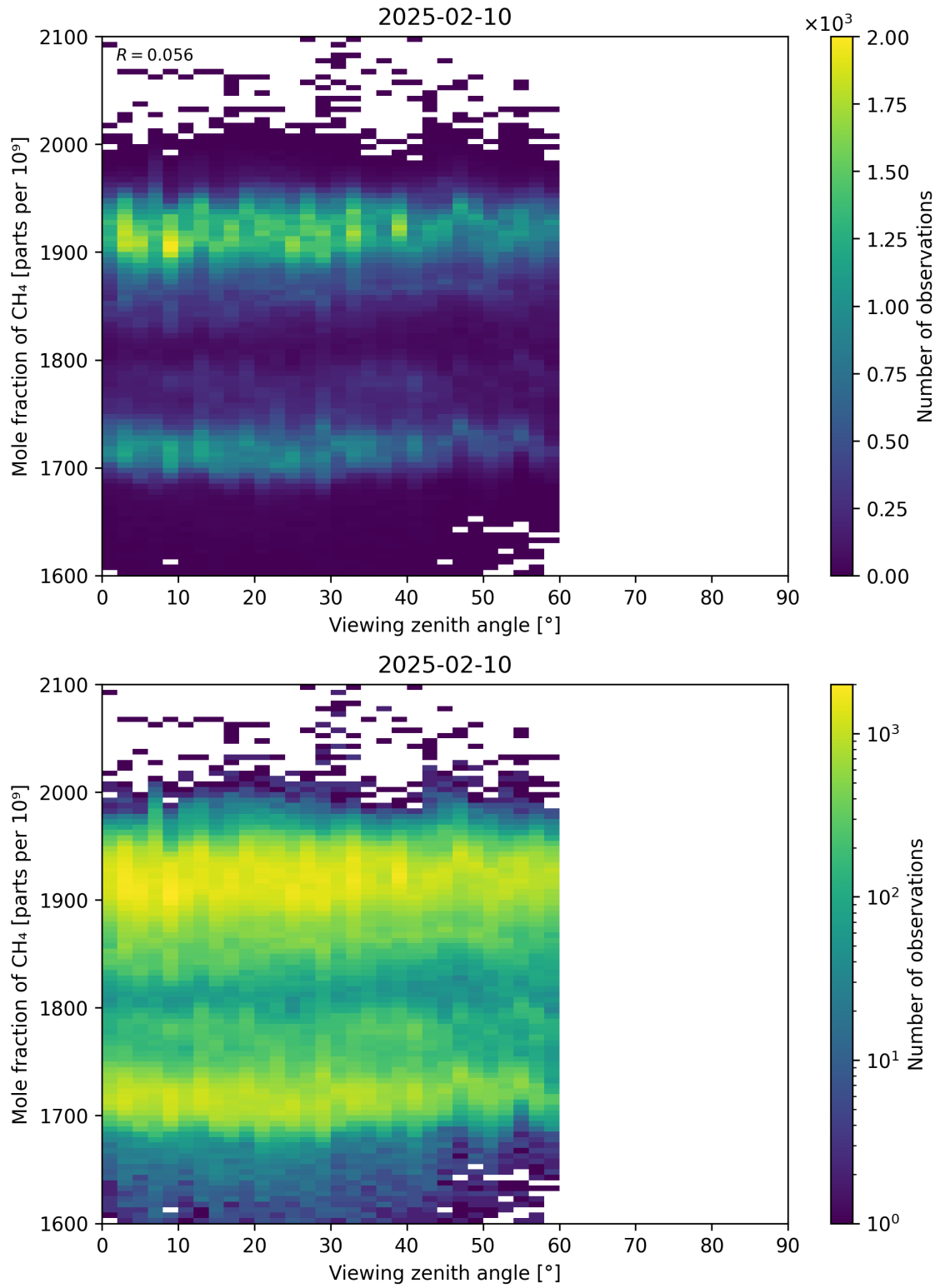
Figure 110: Scatter density plot of “Viewing zenith angle” against “Mole fraction of CH 4 ” for 2025-02-09 to 2025-02-11.
