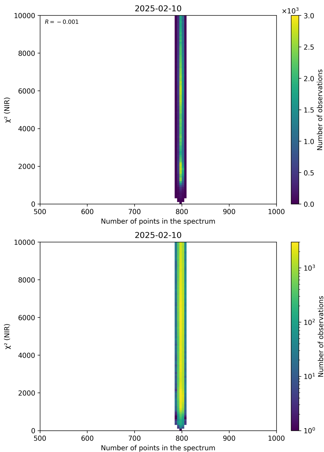
Figure 88: Scatter density plot of “Number of points in the spectrum” against “ \chi^2 (NIR)” for 2025-02-09 to 2025-02-11.
