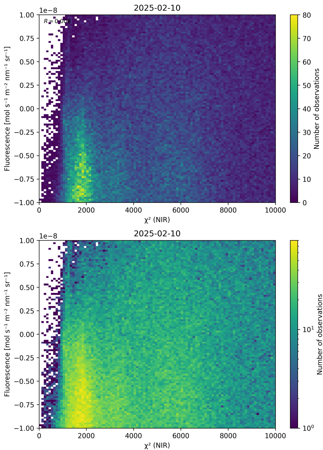
Figure 45: Scatter density plot of “ \chi^2 (NIR)” against “Fluorescence” for 2025-02-09 to 2025-02-11.
