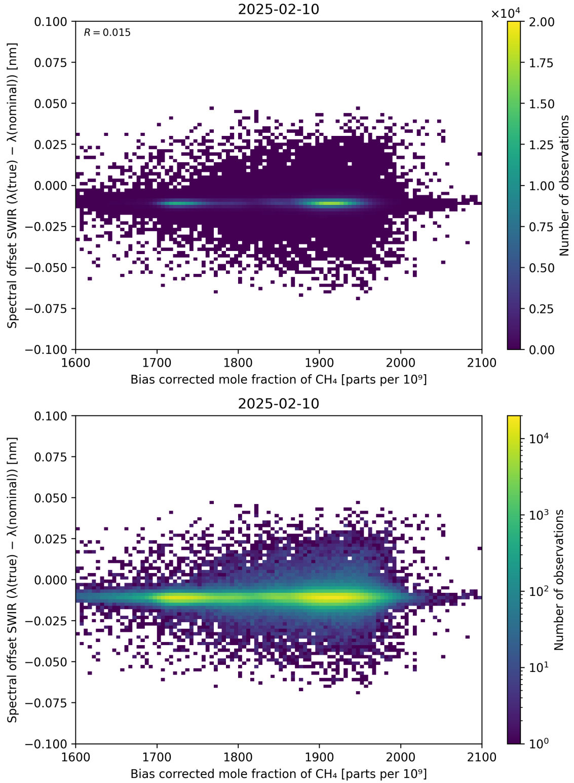
Figure 69: Scatter density plot of “Bias corrected mole fraction of \text{CH}_4 ” against “Spectral offset SWIR ( \lambda_{\text{true}} - \lambda_{\text{nominal}} )” for 2025-02-09 to 2025-02-11.
