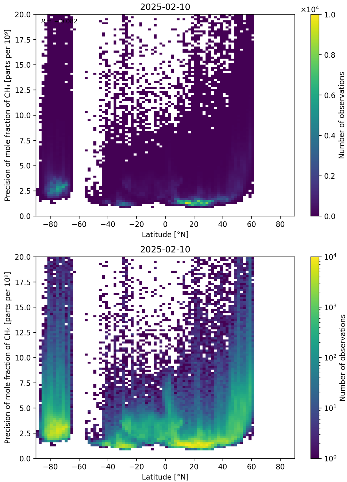
Figure 59: Scatter density plot of “Latitude” against “Precision of mole fraction of CH 4 ” for 2025-02-09 to 2025-02-11.
