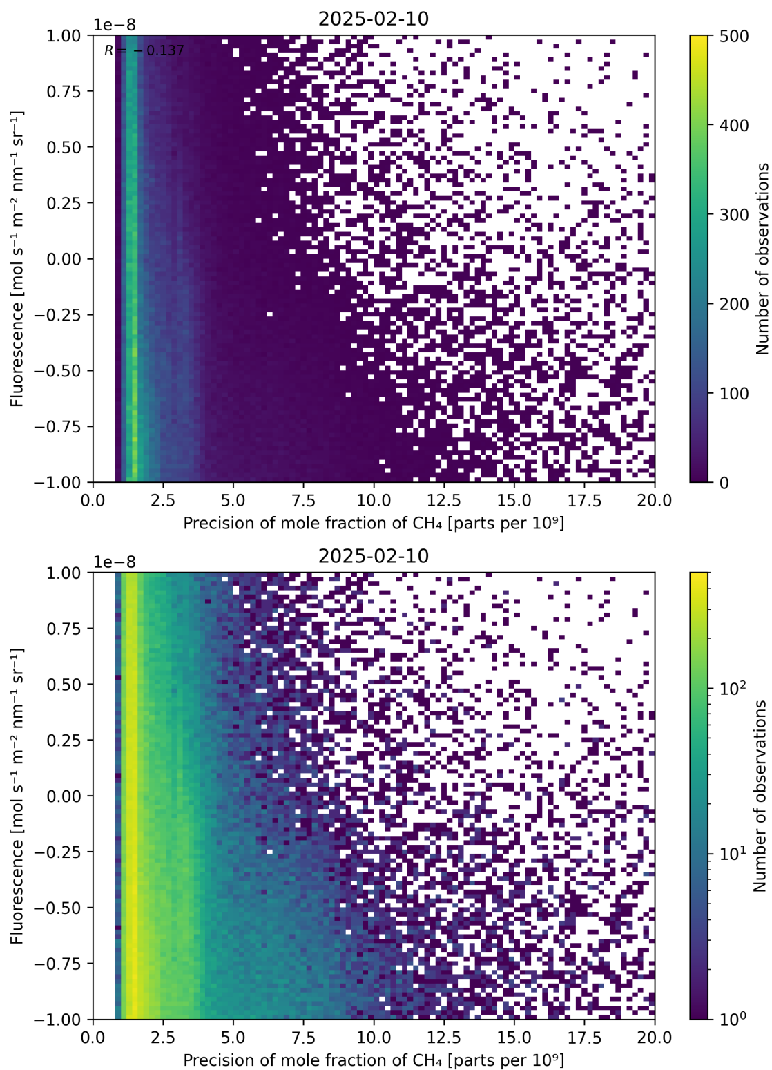
Figure 81: Scatter density plot of “Precision of mole fraction of CH 4 ” against “Fluorescence” for 2025-02-09 to 2025-02-11.
