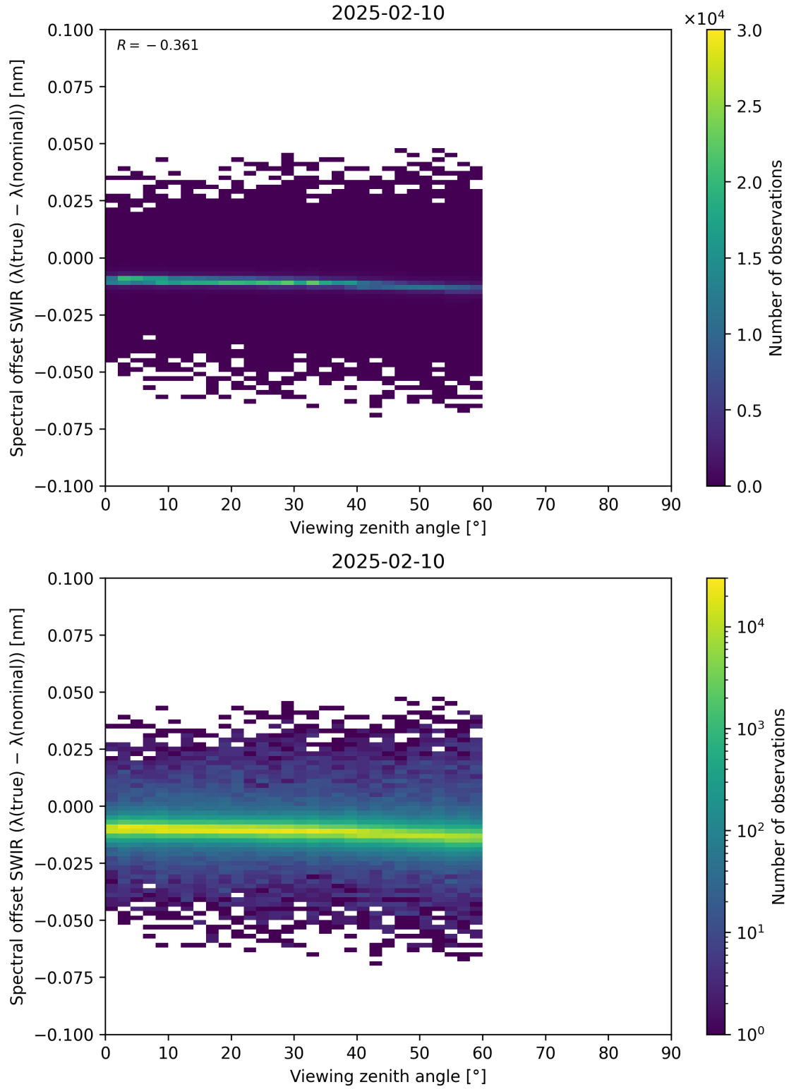
Figure 116: Scatter density plot of “Viewing zenith angle” against “Spectral offset SWIR ( \lambda_{\text{true}} - \lambda_{\text{nominal}} )” for 2025-02-09 to 2025-02-11.
