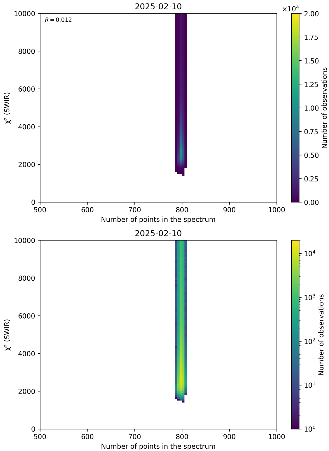
Figure 89: Scatter density plot of “Number of points in the spectrum” against “ \chi^2 (SWIR)” for 2025-02-09 to 2025-02-11.
