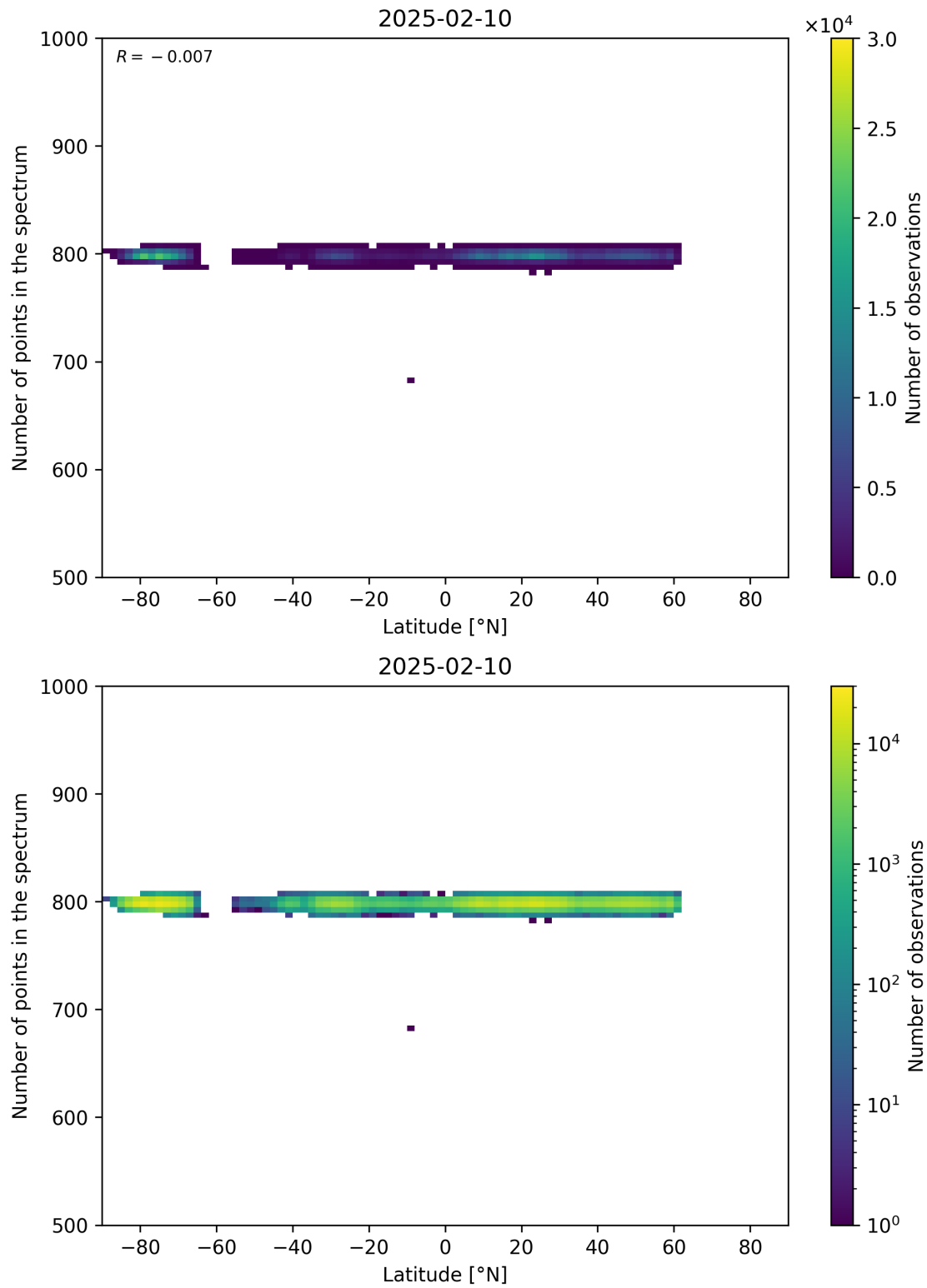
Figure 61: Scatter density plot of “Latitude” against “Number of points in the spectrum” for 2025-02-09 to 2025-02-11.
