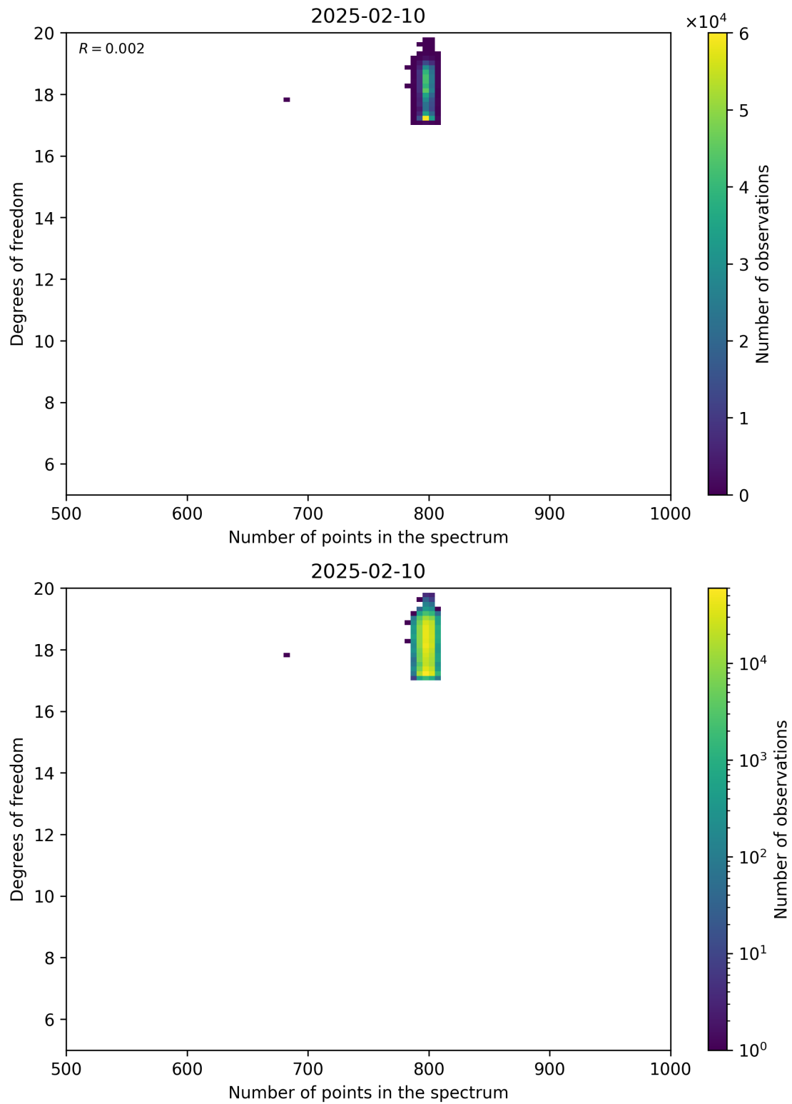
Figure 90: Scatter density plot of “Number of points in the spectrum” against “Degrees of freedom” for 2025-02-09 to 2025-02-11.
