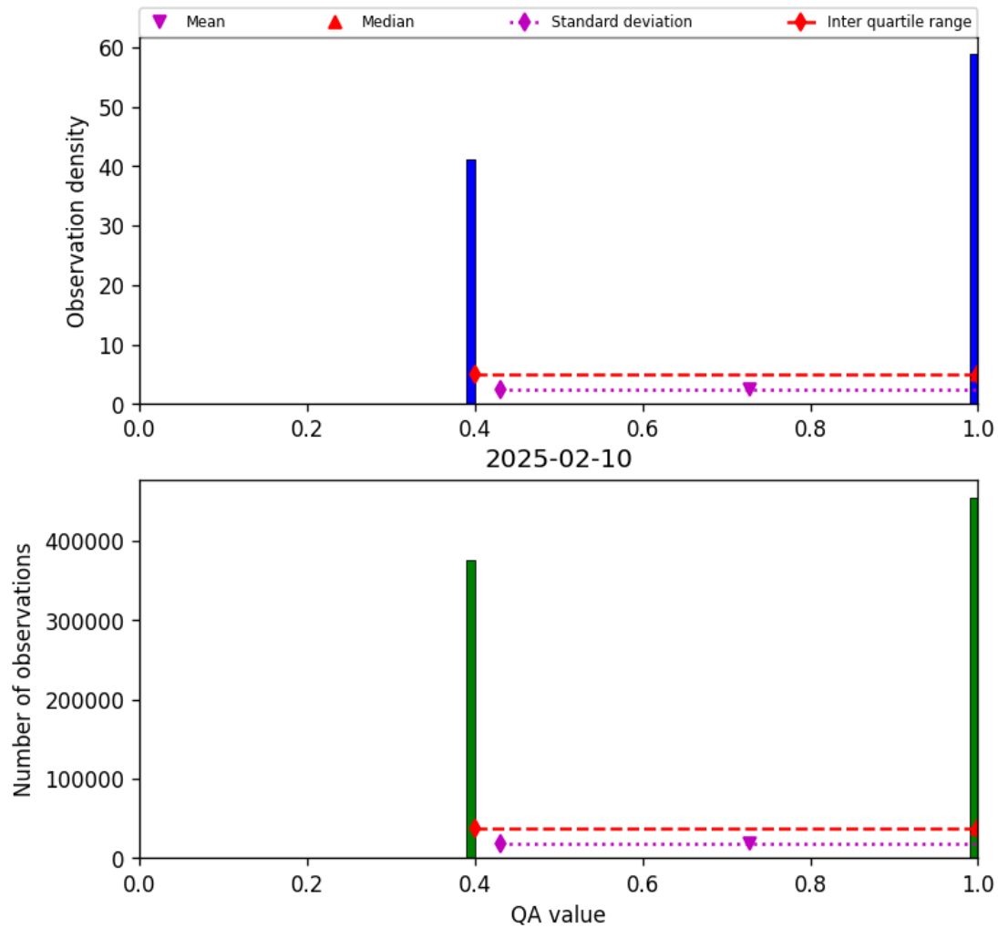
Figure 22: Histogram of “QA value” for 2025-02-09 to 2025-02-11
