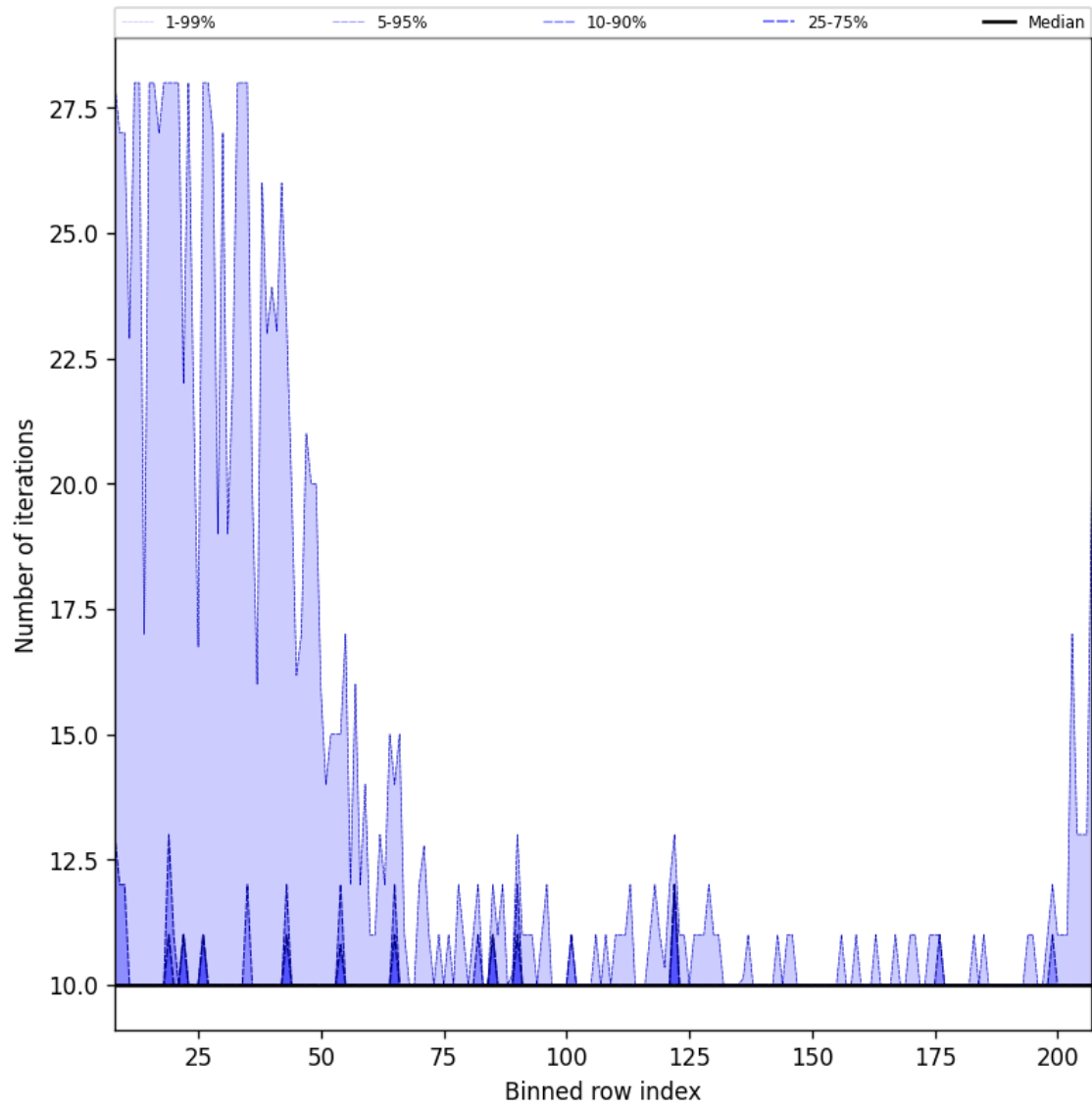
Figure 42: Along track statistics of “Number of iterations” for 2025-02-09 to 2025-02-11
