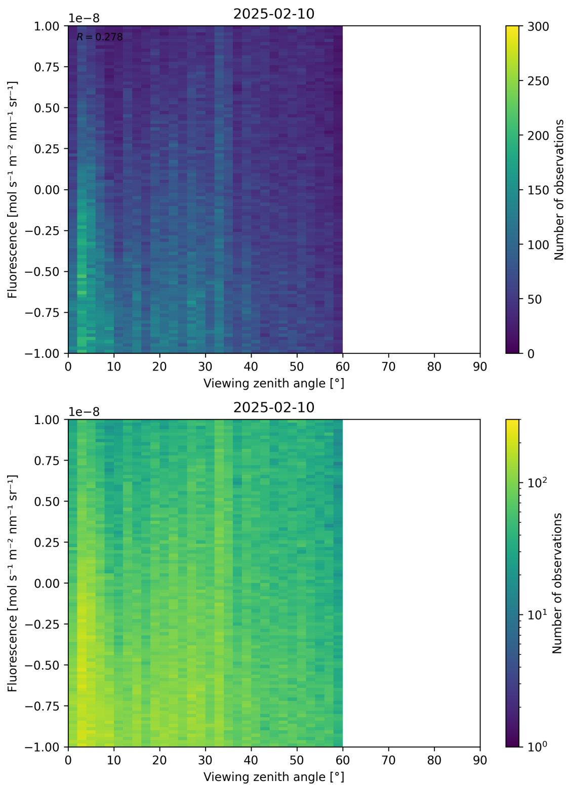
Figure 108: Scatter density plot of “Viewing zenith angle” against “Fluorescence” for 2025-02-09 to 2025-02-11.
