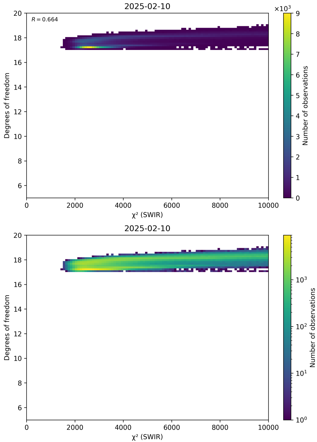
Figure 48: Scatter density plot of “ \chi^2 (SWIR)” against “Degrees of freedom” for 2025-02-09 to 2025-02-11.
