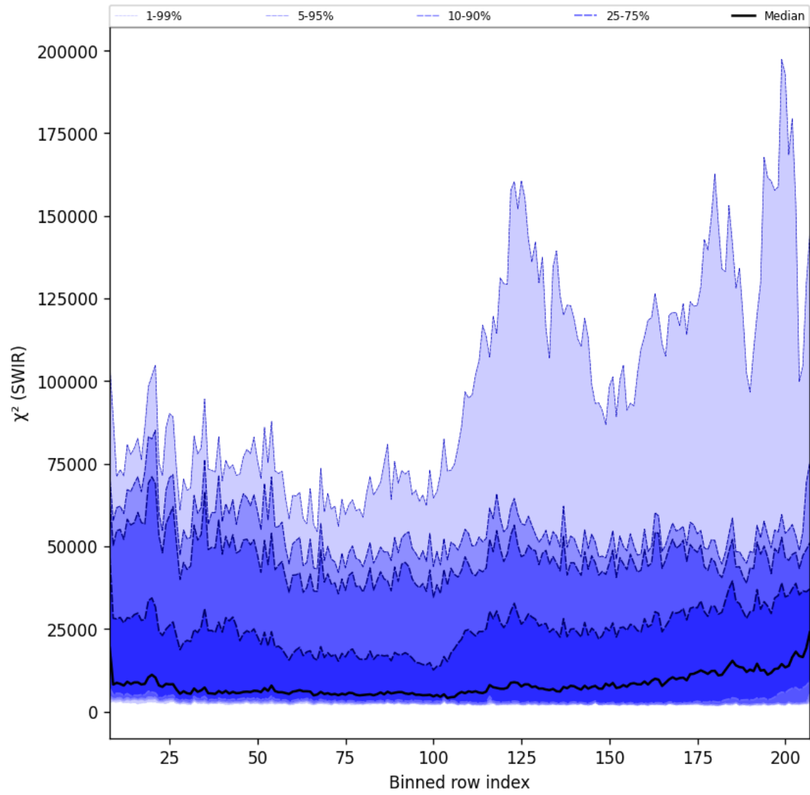
Figure 39: Along track statistics of " \chi^2 (SWIR)" for 2025-02-09 to 2025-02-11
