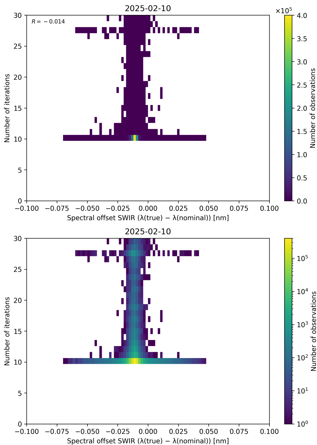
Figure 121: Scatter density plot of “Spectral offset SWIR ( \lambda_{\text{true}} - \lambda_{\text{nominal}} )” against “Number of iterations” for 2025-02-09 to 2025-02-11.
