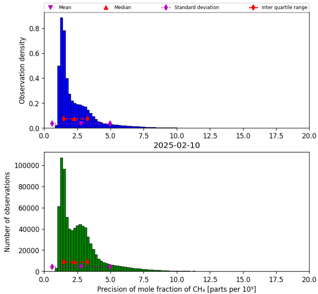
Figure 24: Histogram of “Precision of mole fraction of CH 4 ” for 2025-02-09 to 2025-02-11
