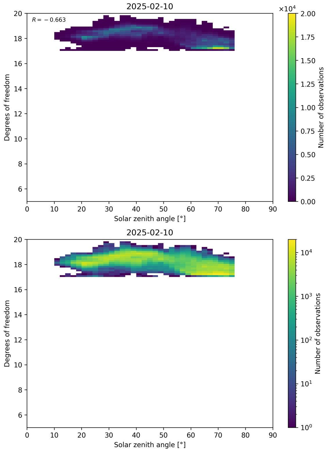
Figure 96: Scatter density plot of “Solar zenith angle” against “Degrees of freedom” for 2025-02-09 to 2025-02-11.
