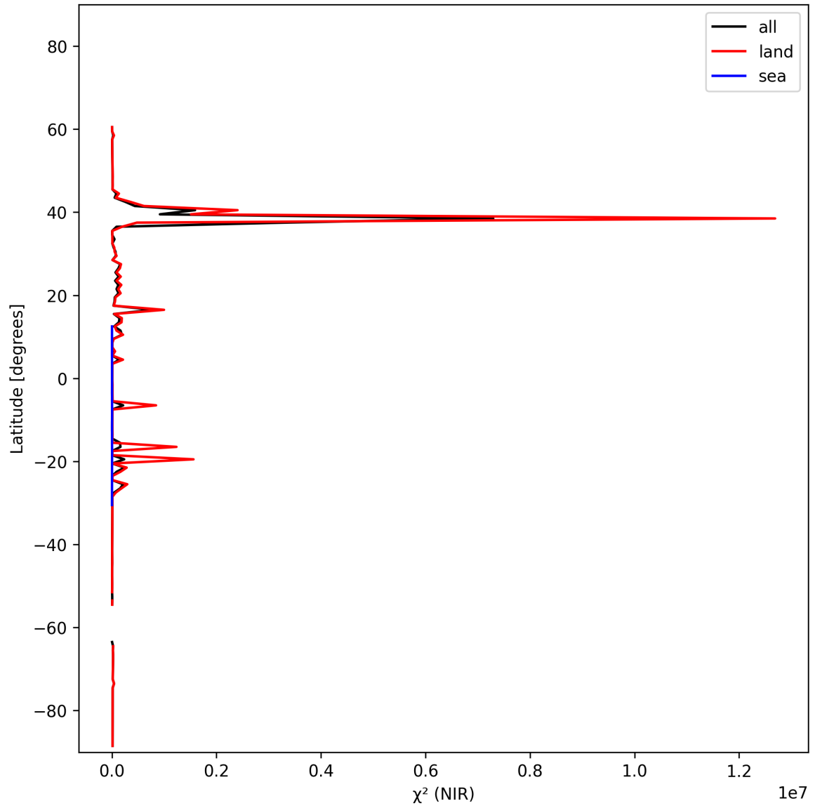
Figure 18: Zonal average of “ \chi^2 (NIR)” for 2025-02-09 to 2025-02-11.
