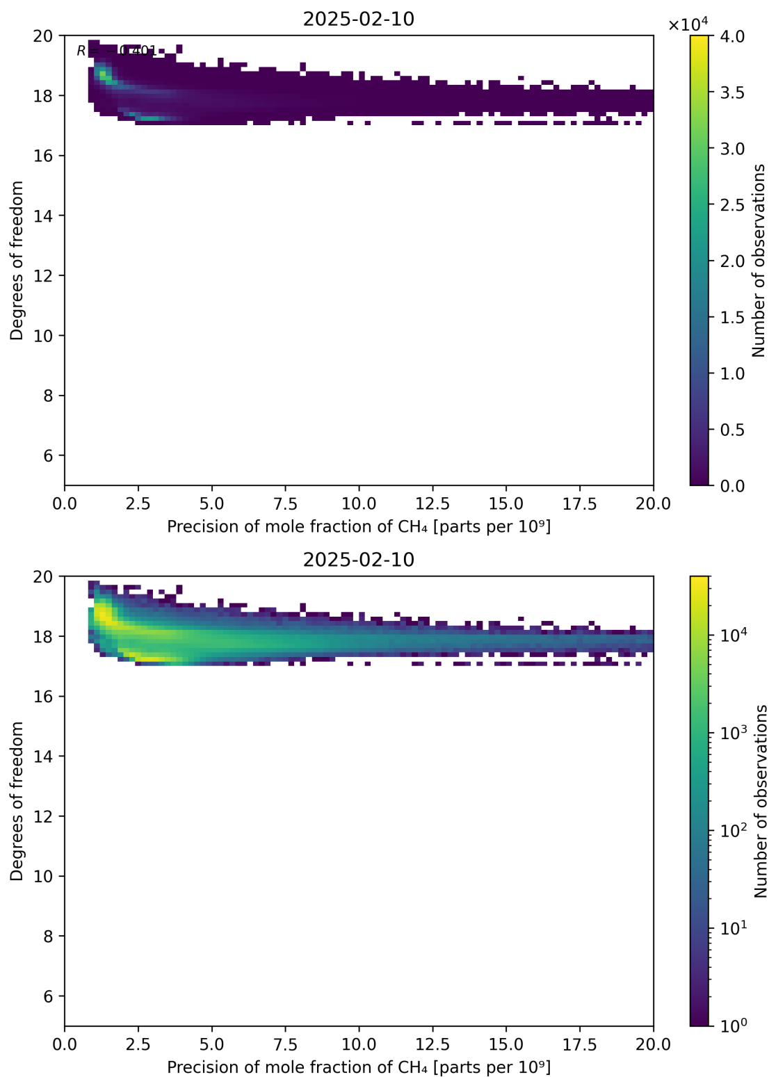
Figure 80: Scatter density plot of “Precision of mole fraction of CH 4 ” against “Degrees of freedom” for 2025-02-09 to 2025-02-11.
