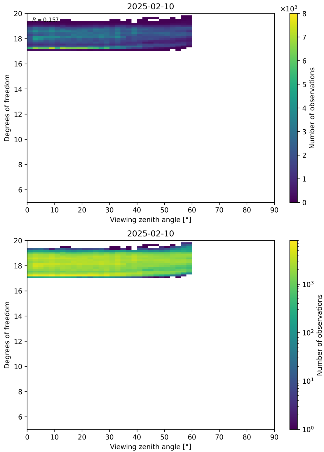
Figure 107: Scatter density plot of “Viewing zenith angle” against “Degrees of freedom” for 2025-02-09 to 2025-02-11.
