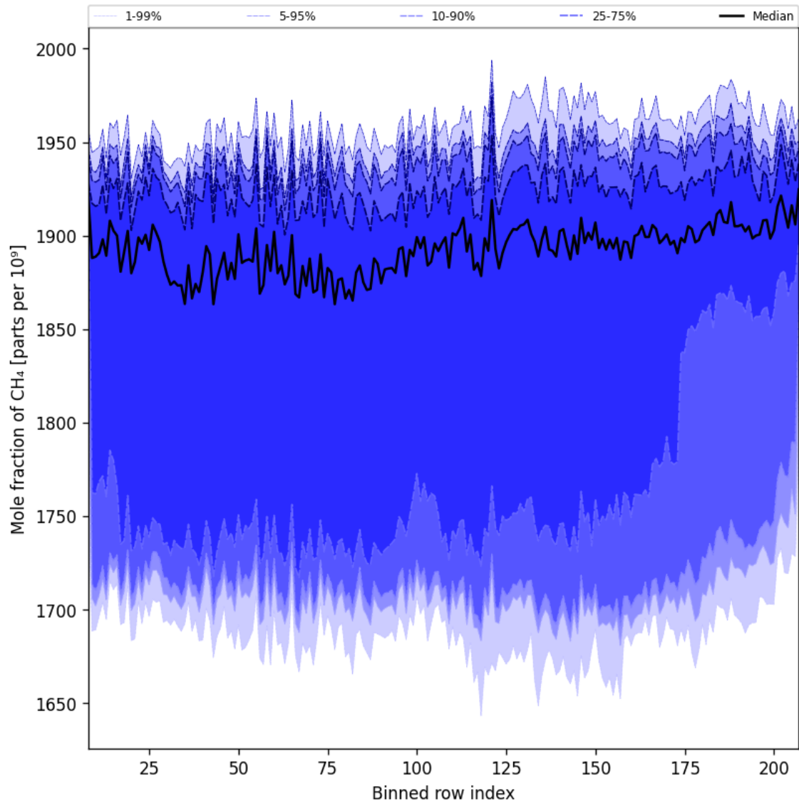
Figure 34: Along track statistics of “Mole fraction of CH 4 ” for 2025-02-09 to 2025-02-11
