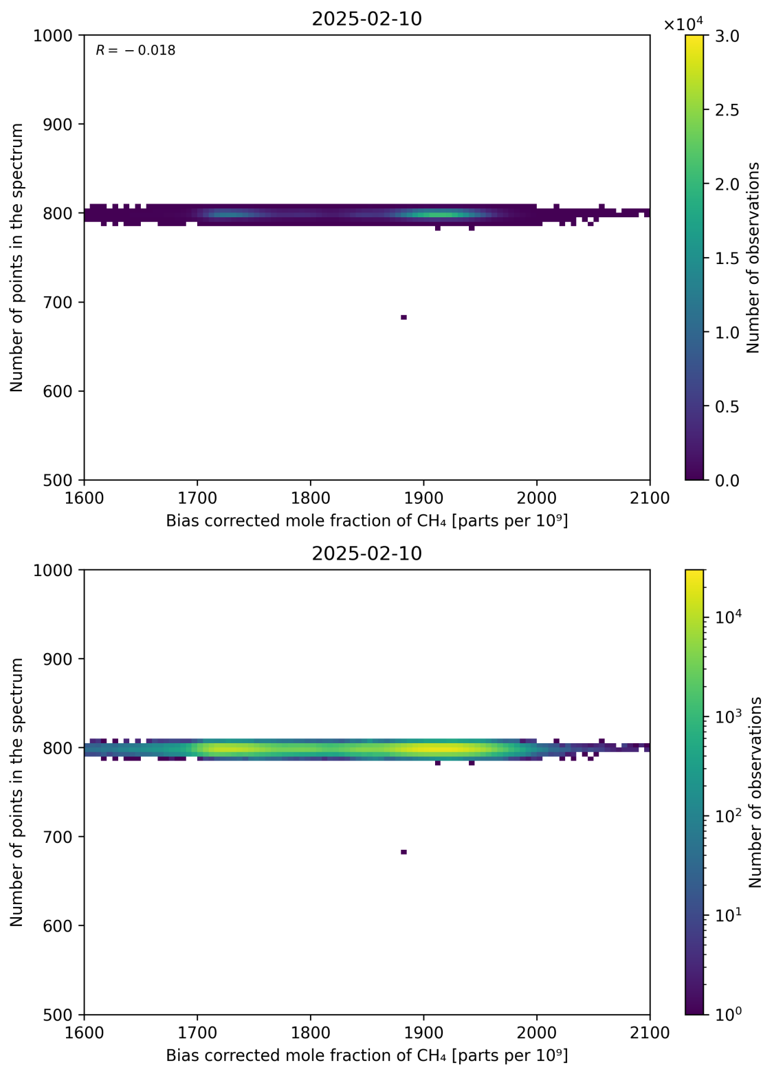
Figure 68: Scatter density plot of “Bias corrected mole fraction of CH 4 ” against “Number of points in the spectrum” for 2025-02-09 to 2025-02-11.
