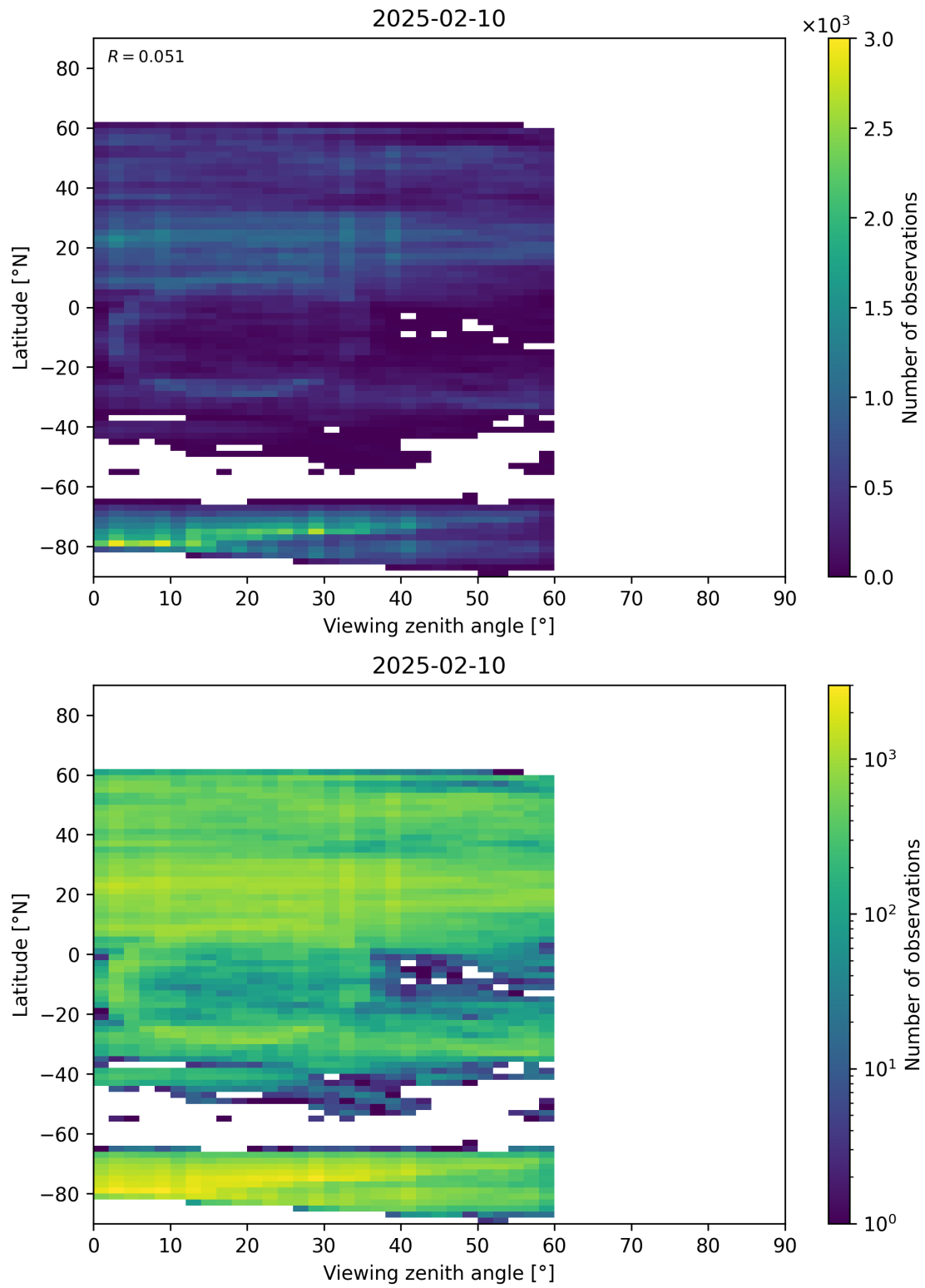
Figure 109: Scatter density plot of “Viewing zenith angle” against “Latitude” for 2025-02-09 to 2025-02-11.
