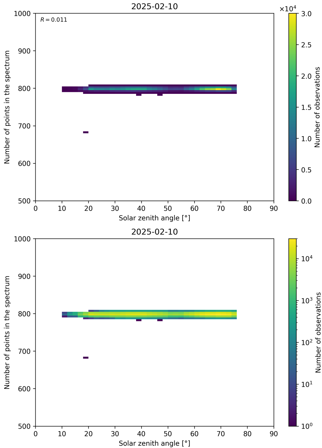
Figure 103: Scatter density plot of “Solar zenith angle” against “Number of points in the spectrum” for 2025-02-09 to 2025-02-11.
