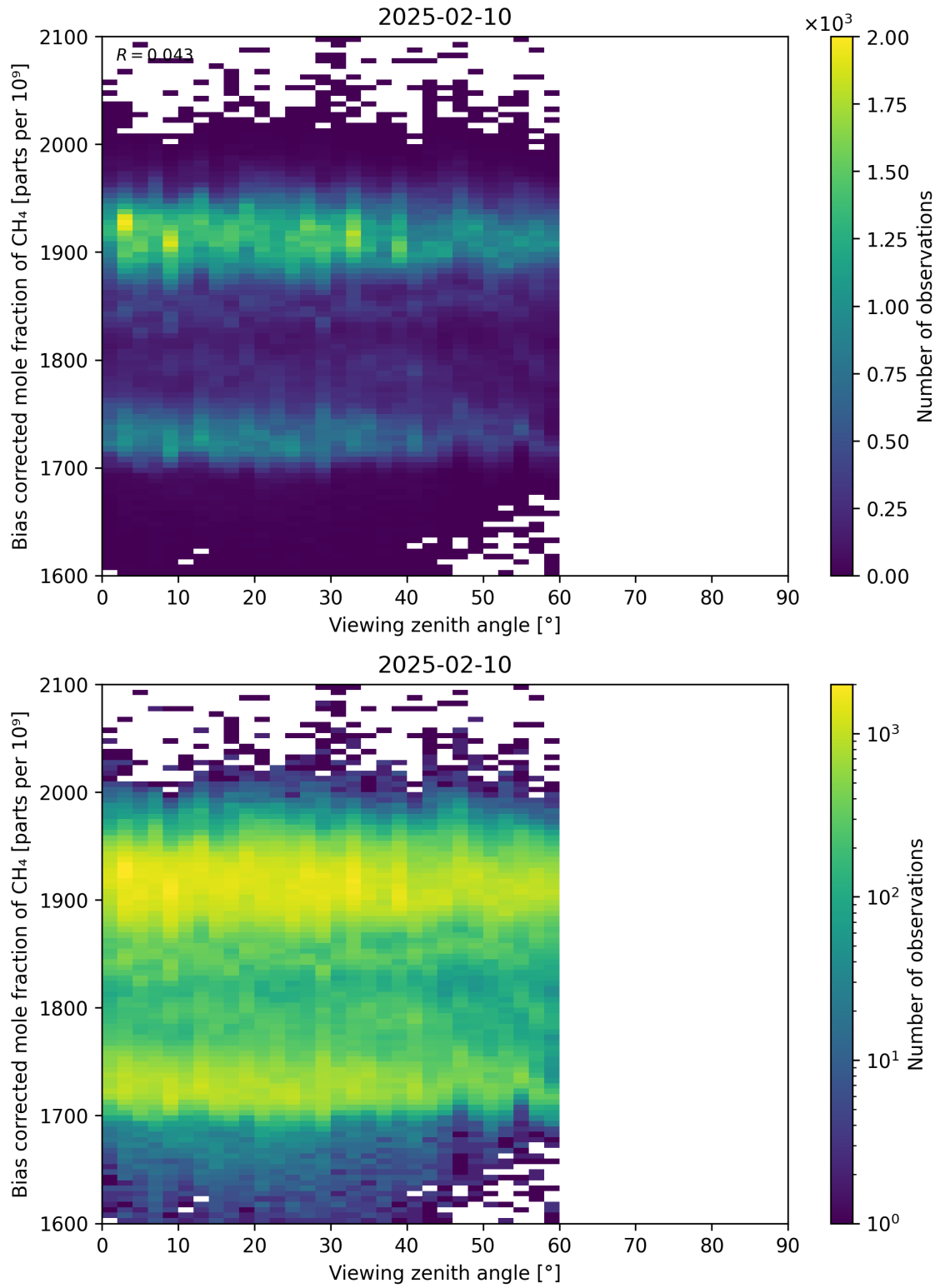
Figure 111: Scatter density plot of “Viewing zenith angle” against “Bias corrected mole fraction of CH 4 ” for 2025-02-09 to 2025-02-11.
