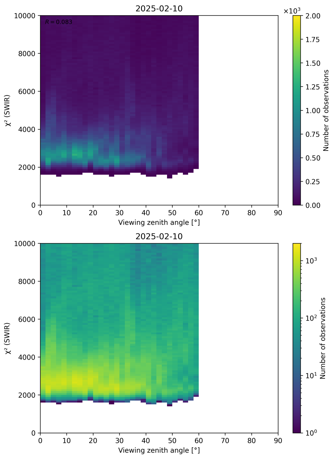
Figure 106: Scatter density plot of “Viewing zenith angle” against “ \chi^2 (SWIR)” for 2025-02-09 to 2025-02-11.
