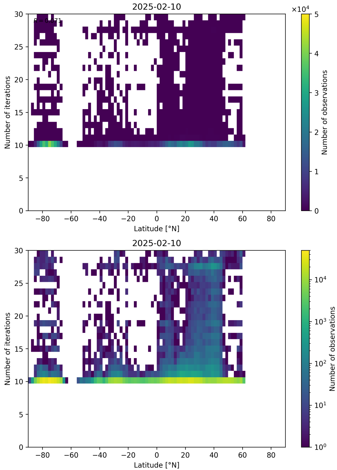
Figure 60: Scatter density plot of “Latitude” against “Number of iterations” for 2025-02-09 to 2025-02-11.
