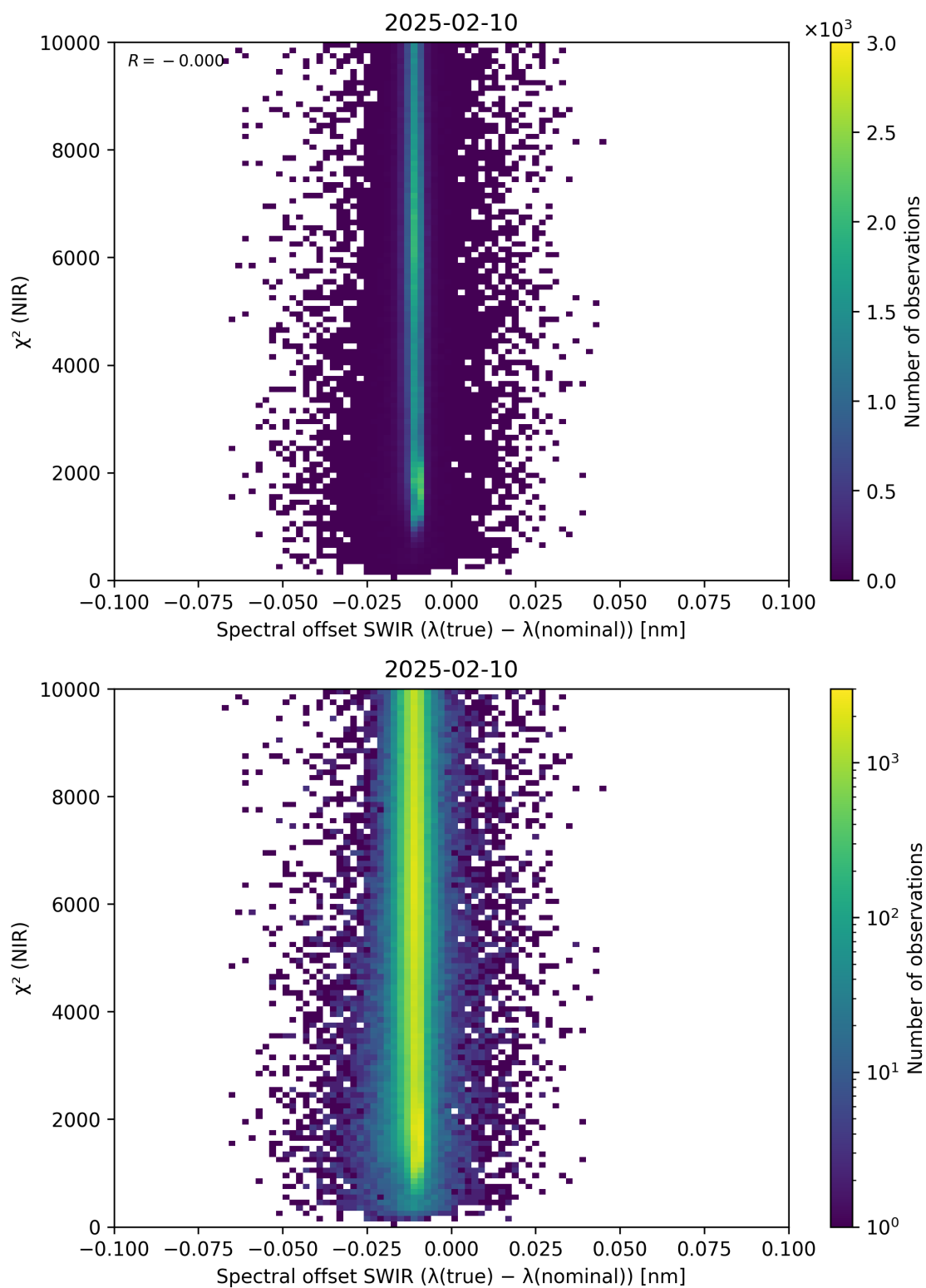
Figure 117: Scatter density plot of “Spectral offset SWIR ( \lambda_{\text{true}} - \lambda_{\text{nominal}} )” against “ \chi^2 (NIR)” for 2025-02-09 to 2025-02-11.
