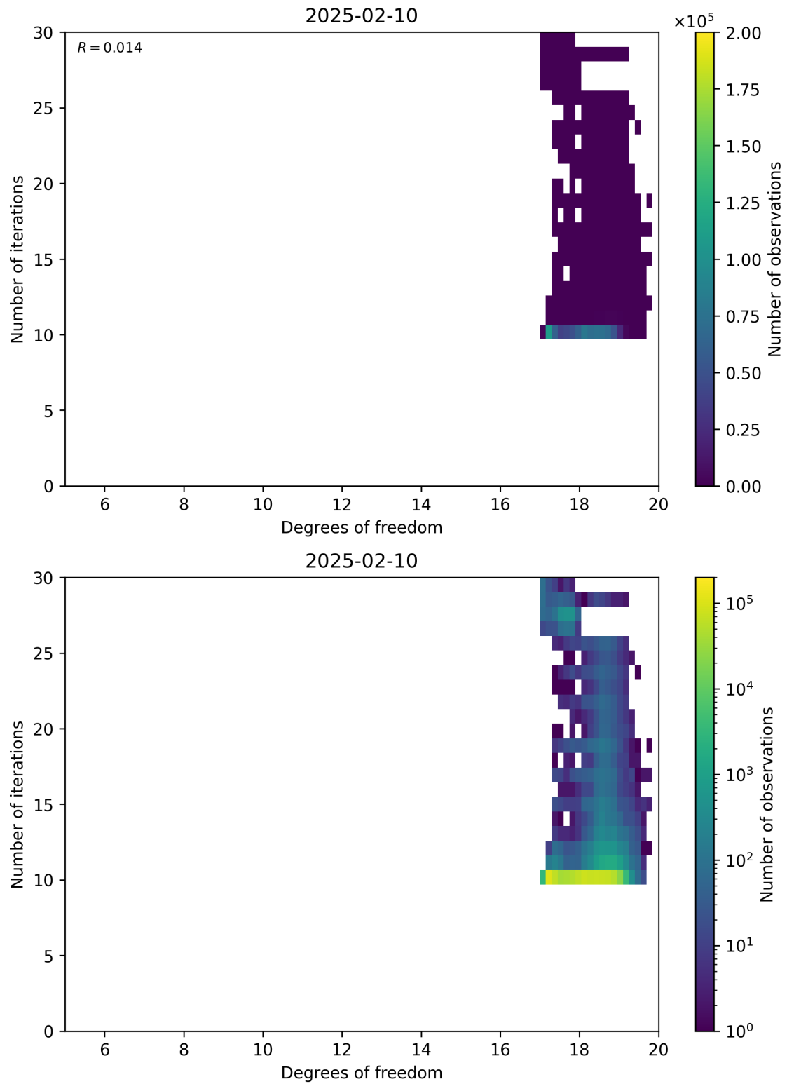
Figure 52: Scatter density plot of “Degrees of freedom” against “Number of iterations” for 2025-02-09 to 2025-02-11.
