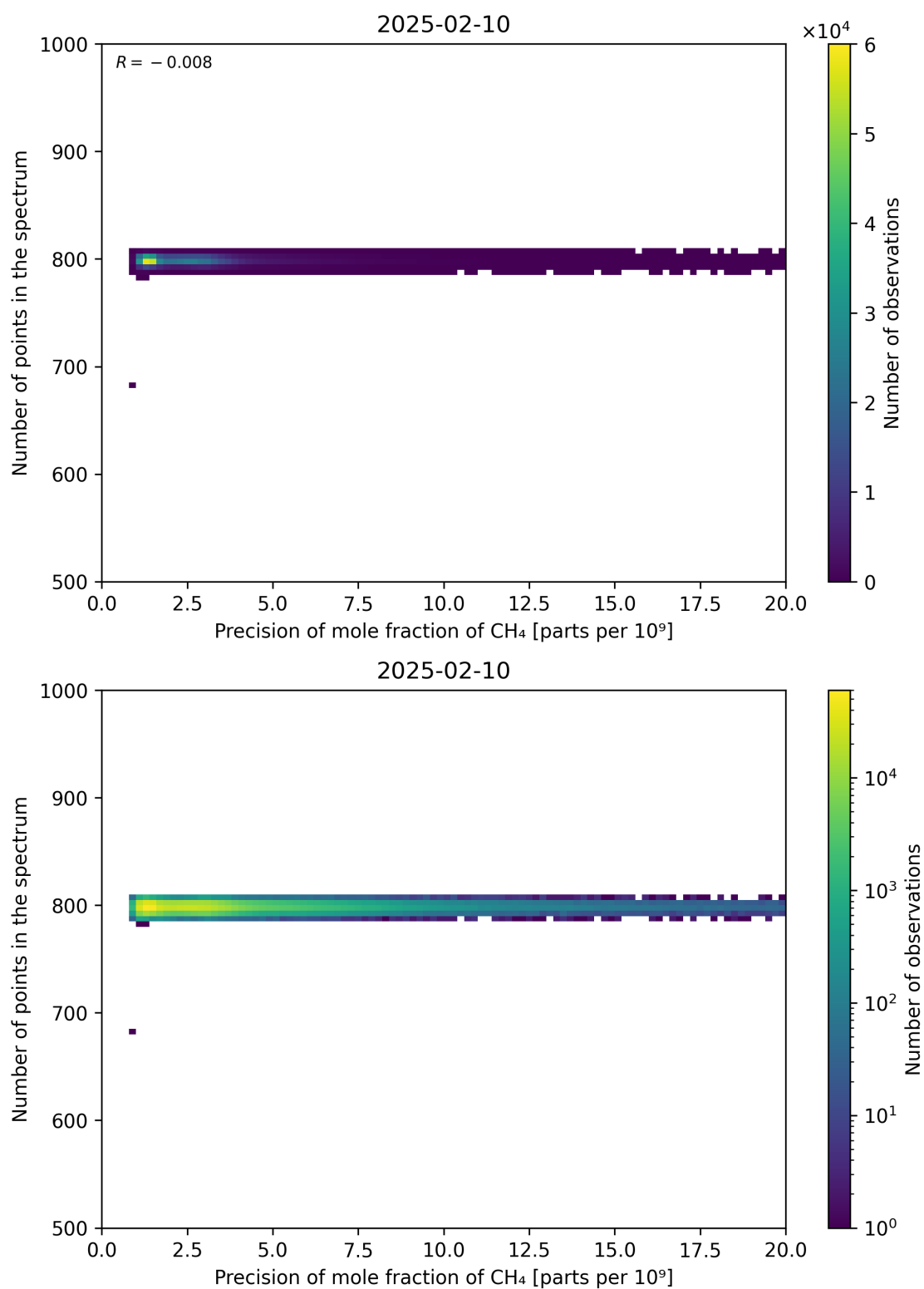
Figure 84: Scatter density plot of “Precision of mole fraction of CH 4 ” against “Number of points in the spectrum” for 2025-02-09 to 2025-02-11.
