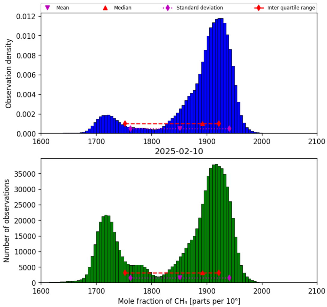
Figure 23: Histogram of “Mole fraction of CH 4 ” for 2025-02-09 to 2025-02-11
