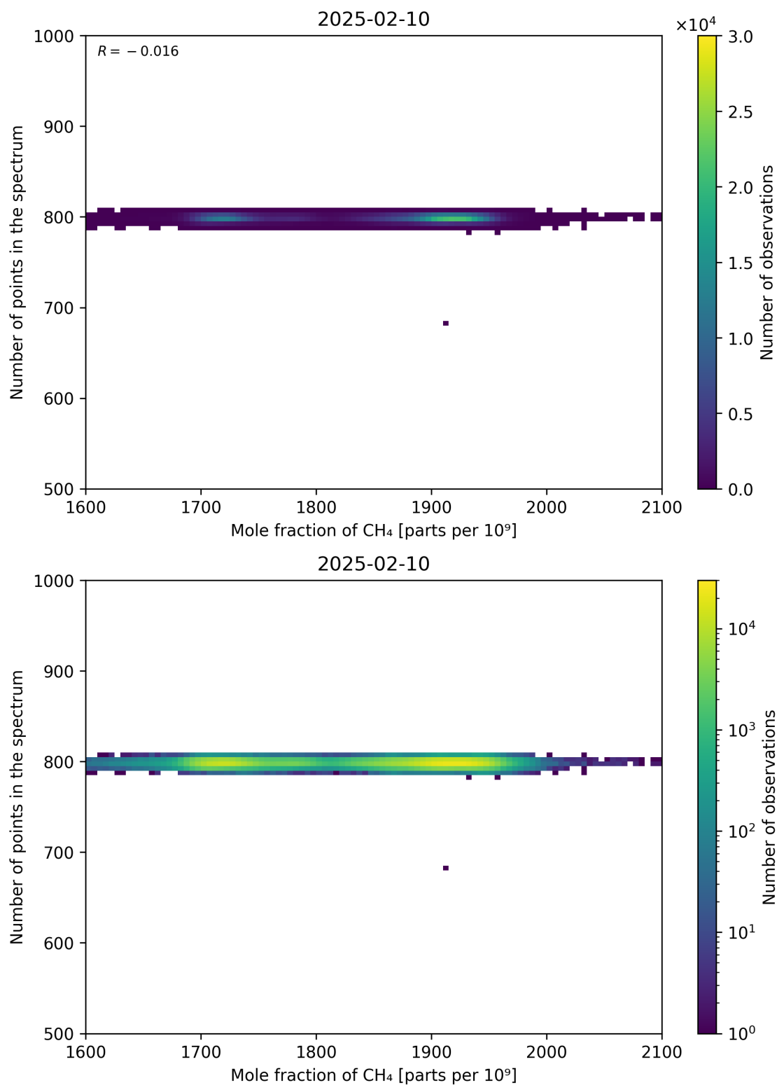
Figure 77: Scatter density plot of “Mole fraction of CH 4 ” against “Number of points in the spectrum” for 2025-02-09 to 2025-02-11.
