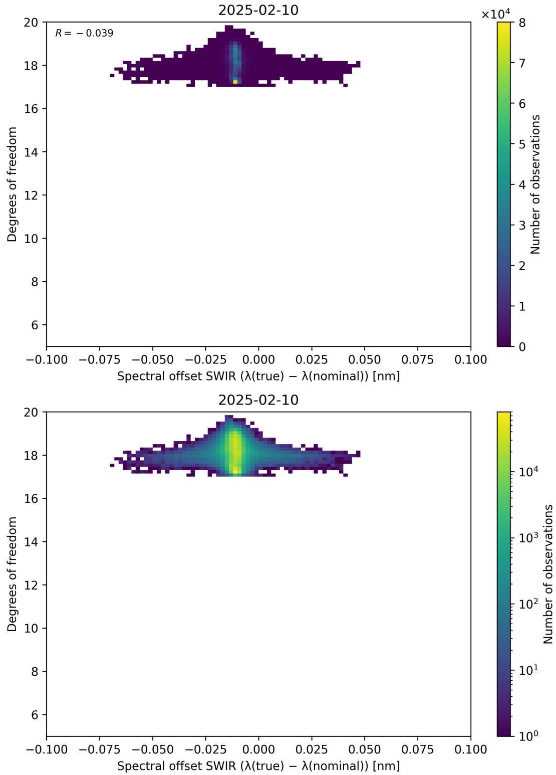
Figure 119: Scatter density plot of “Spectral offset SWIR ( \lambda_{\text{true}} - \lambda_{\text{nominal}} )” against “Degrees of freedom” for 2025-02-09 to 2025-02-11.
