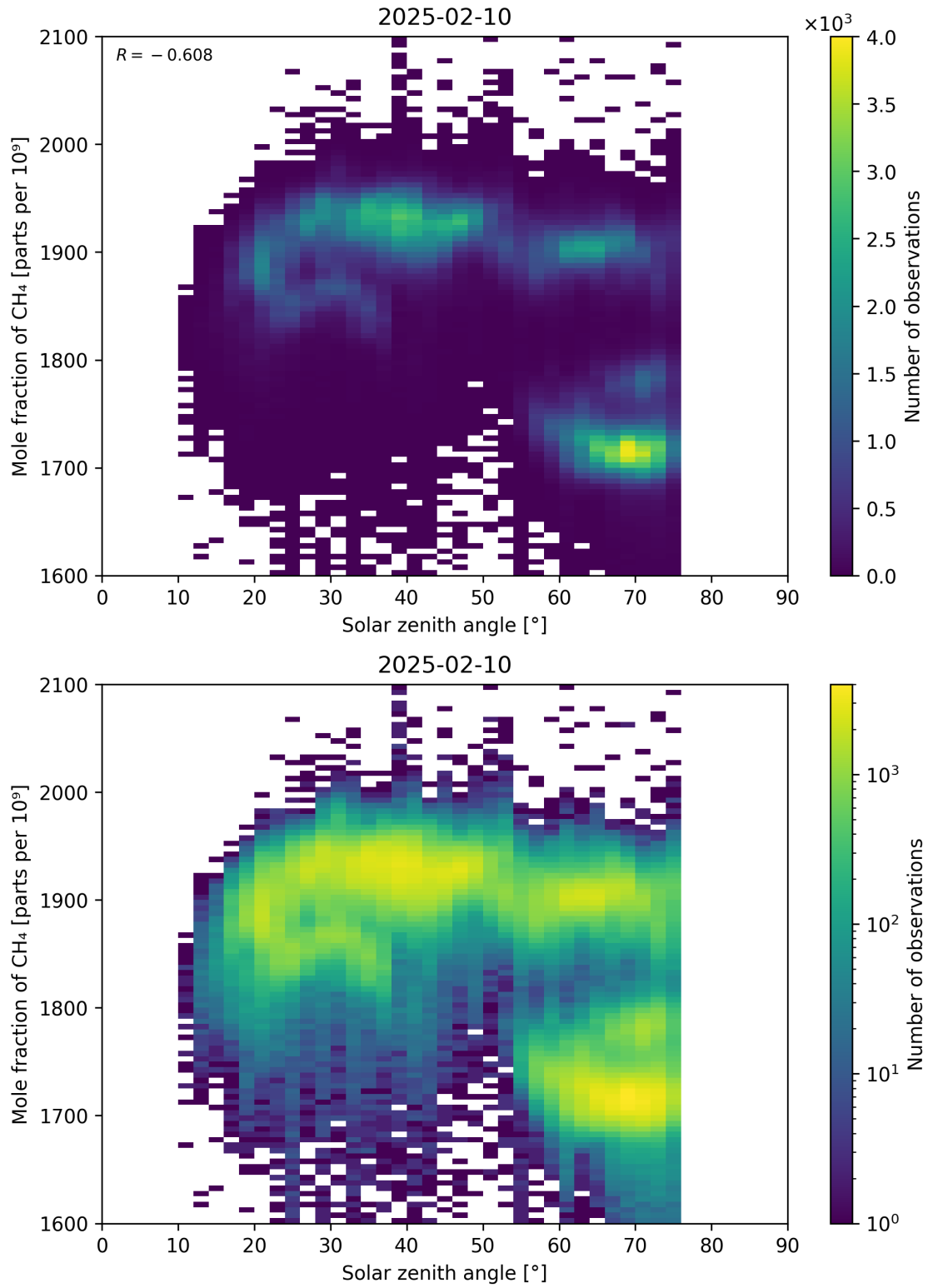
Figure 99: Scatter density plot of “Solar zenith angle” against “Mole fraction of CH 4 ” for 2025-02-09 to 2025-02-11.
