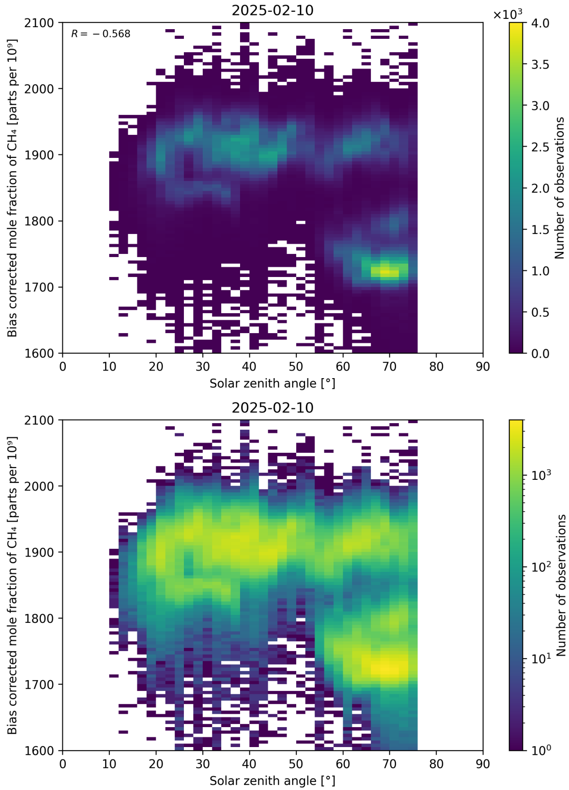
Figure 100: Scatter density plot of “Solar zenith angle” against “Bias corrected mole fraction of \text{CH}_4 ” for 2025-02-09 to 2025-02-11.
