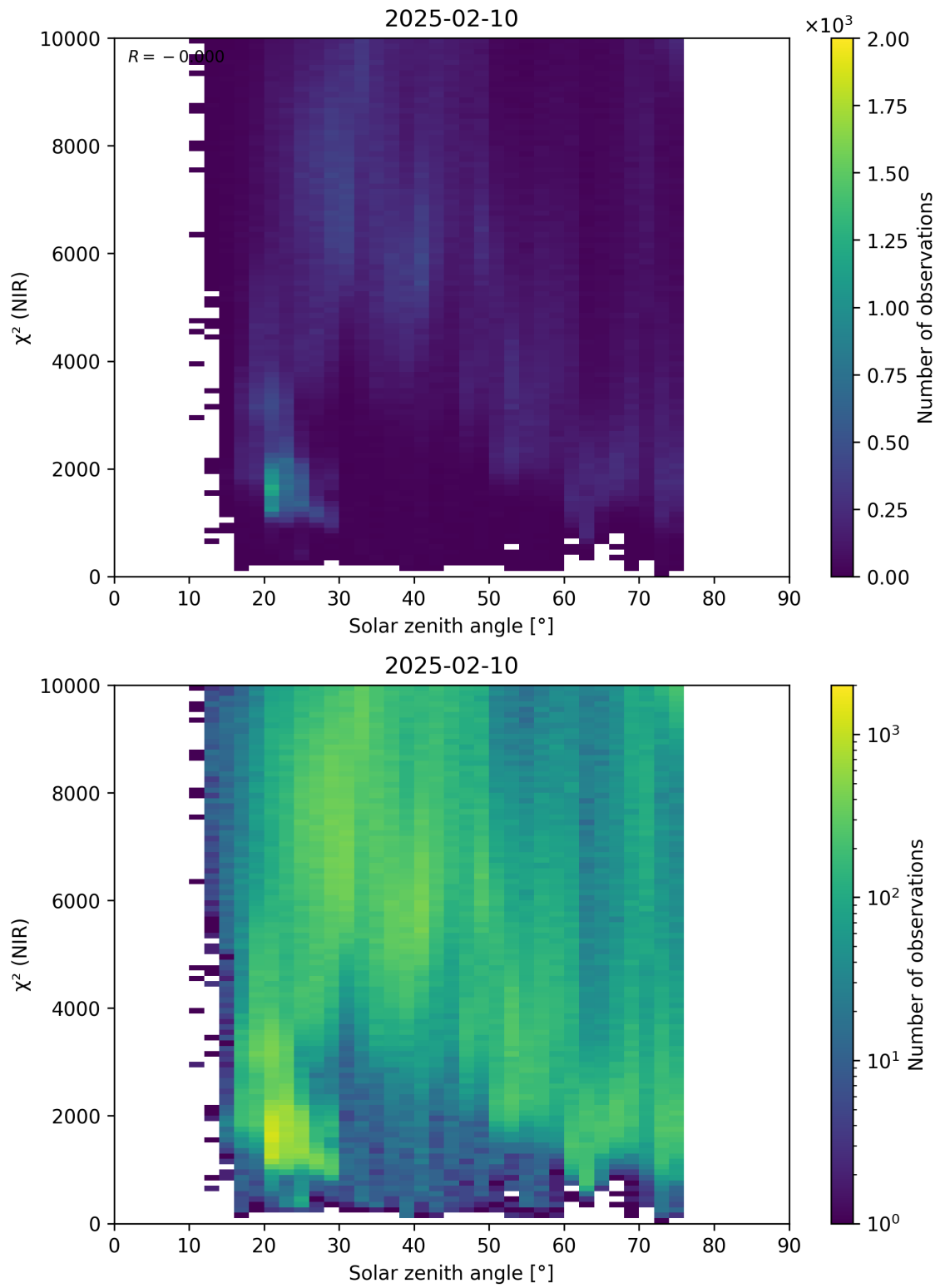
Figure 94: Scatter density plot of “Solar zenith angle” against “ \chi^2 (NIR)” for 2025-02-09 to 2025-02-11.
