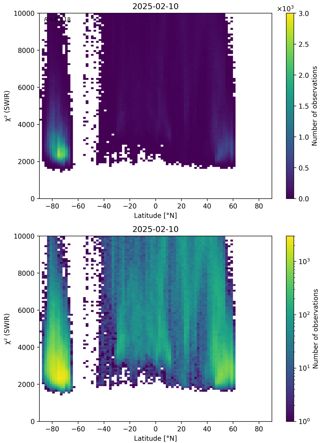
Figure 54: Scatter density plot of “Latitude” against “ \chi^2 (SWIR)” for 2025-02-09 to 2025-02-11.
