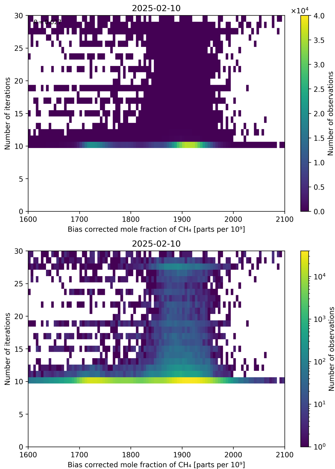
Figure 67: Scatter density plot of “Bias corrected mole fraction of \text{CH}_4 ” against “Number of iterations” for 2025-02-09 to 2025-02-11.
