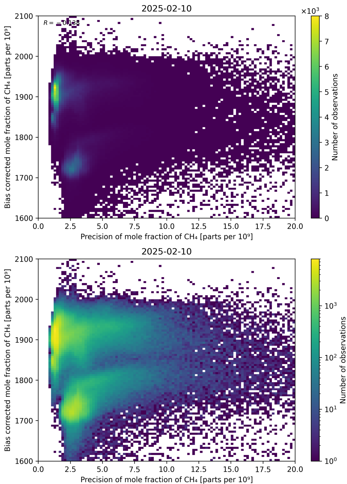
Figure 82: Scatter density plot of “Precision of mole fraction of CH 4 ” against “Bias corrected mole fraction of CH 4 ” for 2025-02-09 to 2025-02-11.
