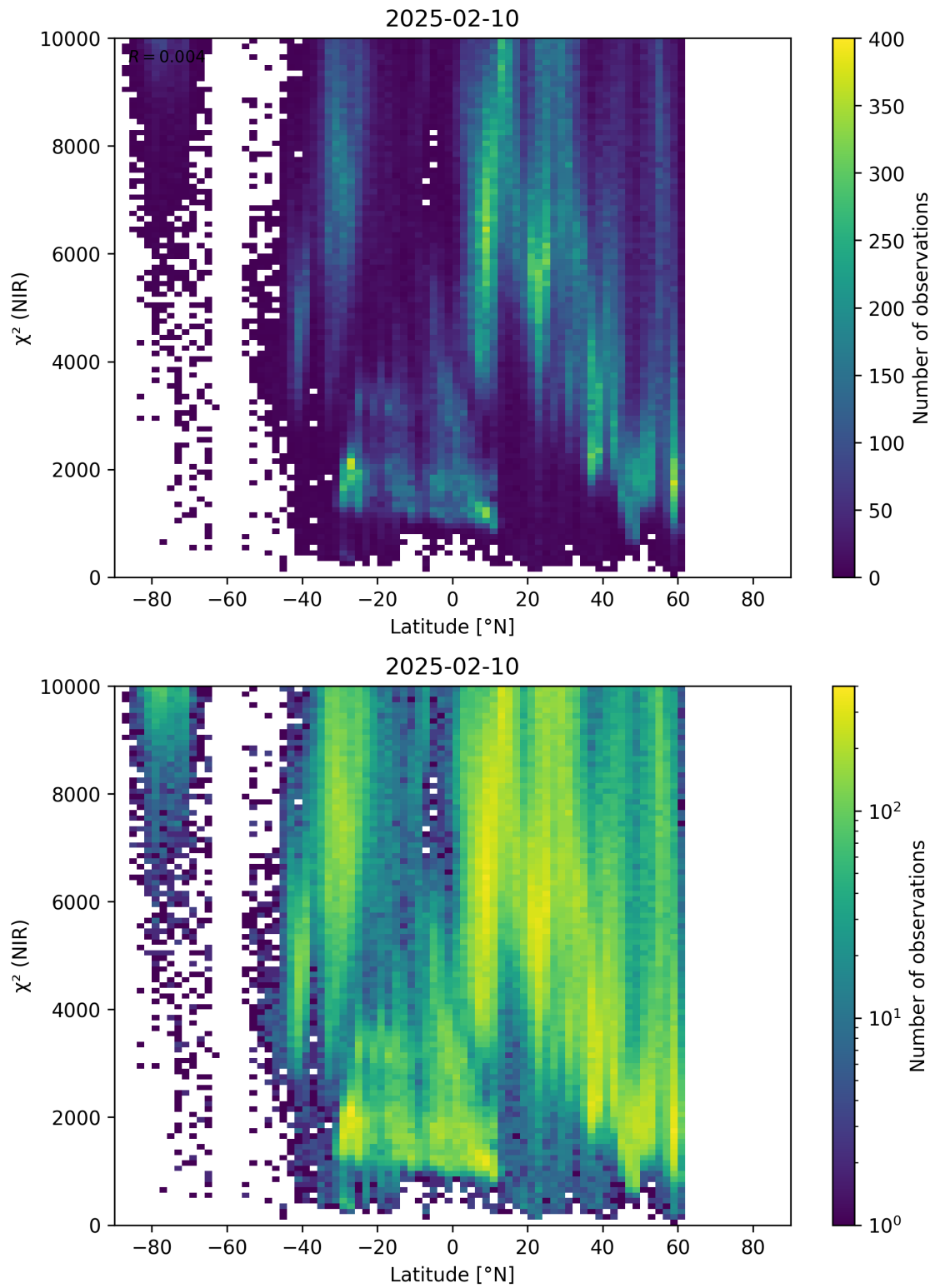
Figure 53: Scatter density plot of “Latitude” against “ \chi^2 (NIR)” for 2025-02-09 to 2025-02-11.
