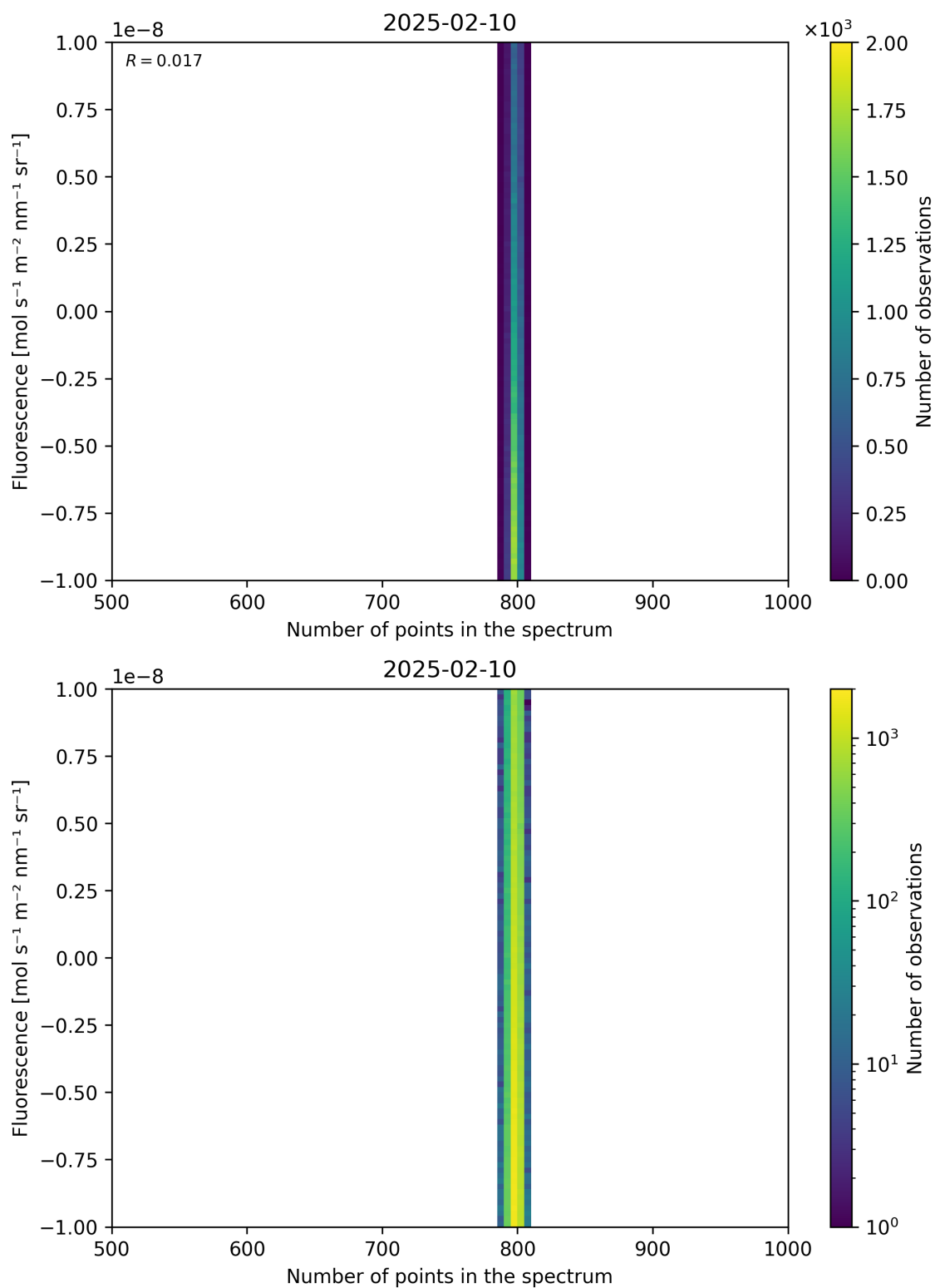
Figure 91: Scatter density plot of “Number of points in the spectrum” against “Fluorescence” for 2025-02-09 to 2025-02-11.
