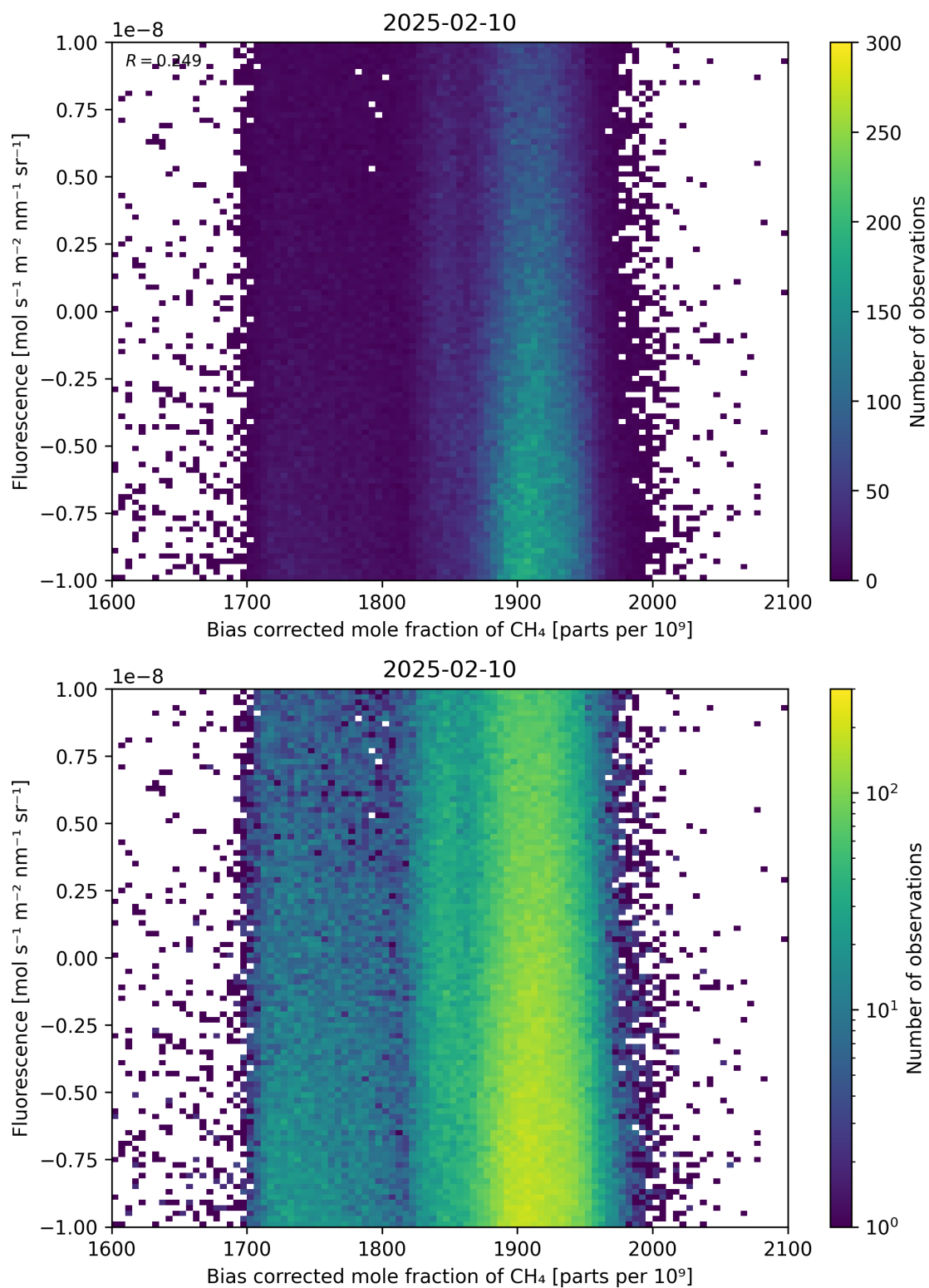
Figure 66: Scatter density plot of “Bias corrected mole fraction of CH 4 ” against “Fluorescence” for 2025-02-09 to 2025-02-11.
