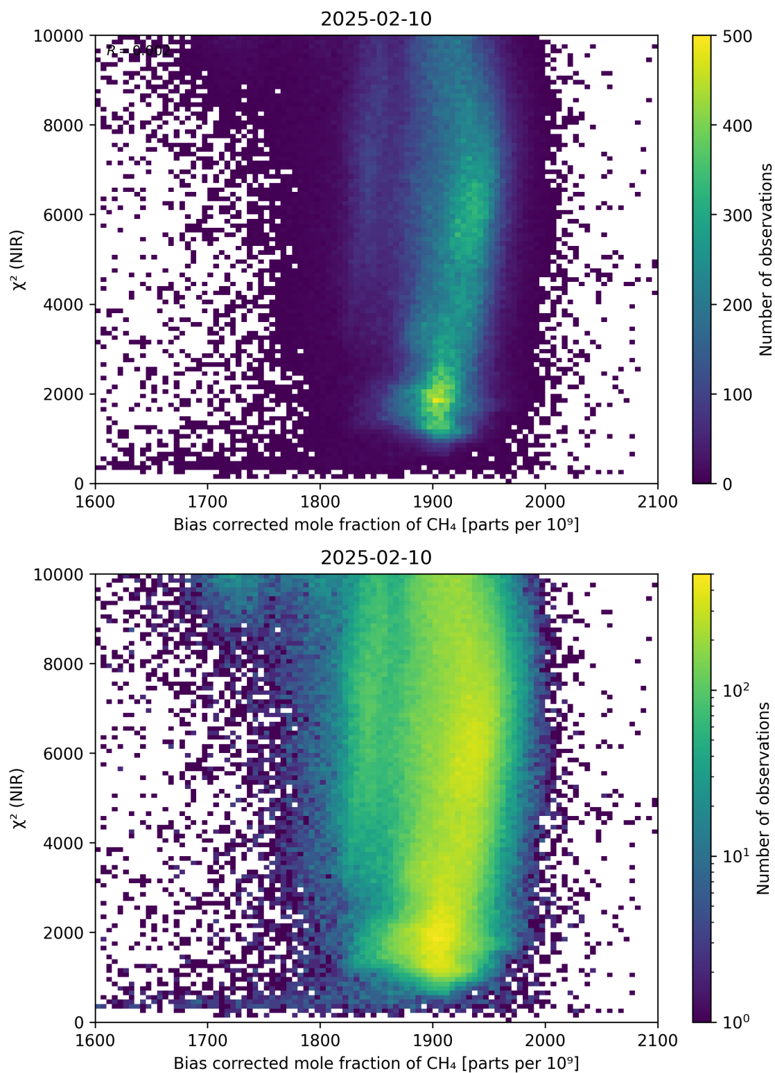
Figure 63: Scatter density plot of “Bias corrected mole fraction of \text{CH}_4 ” against “ \chi^2 (NIR)” for 2025-02-09 to 2025-02-11.
