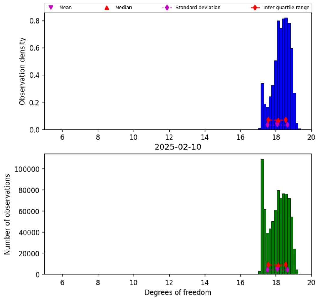
Figure 30: Histogram of “Degrees of freedom” for 2025-02-09 to 2025-02-11
