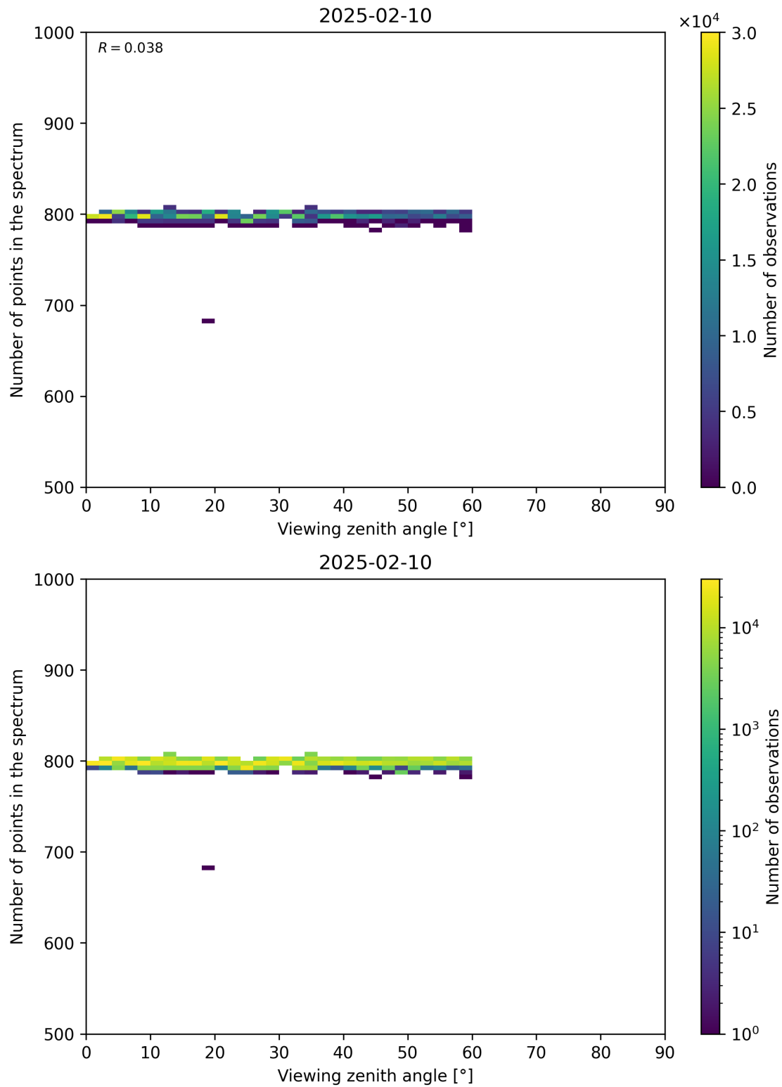
Figure 114: Scatter density plot of “Viewing zenith angle” against “Number of points in the spectrum” for 2025-02-09 to 2025-02-11.
