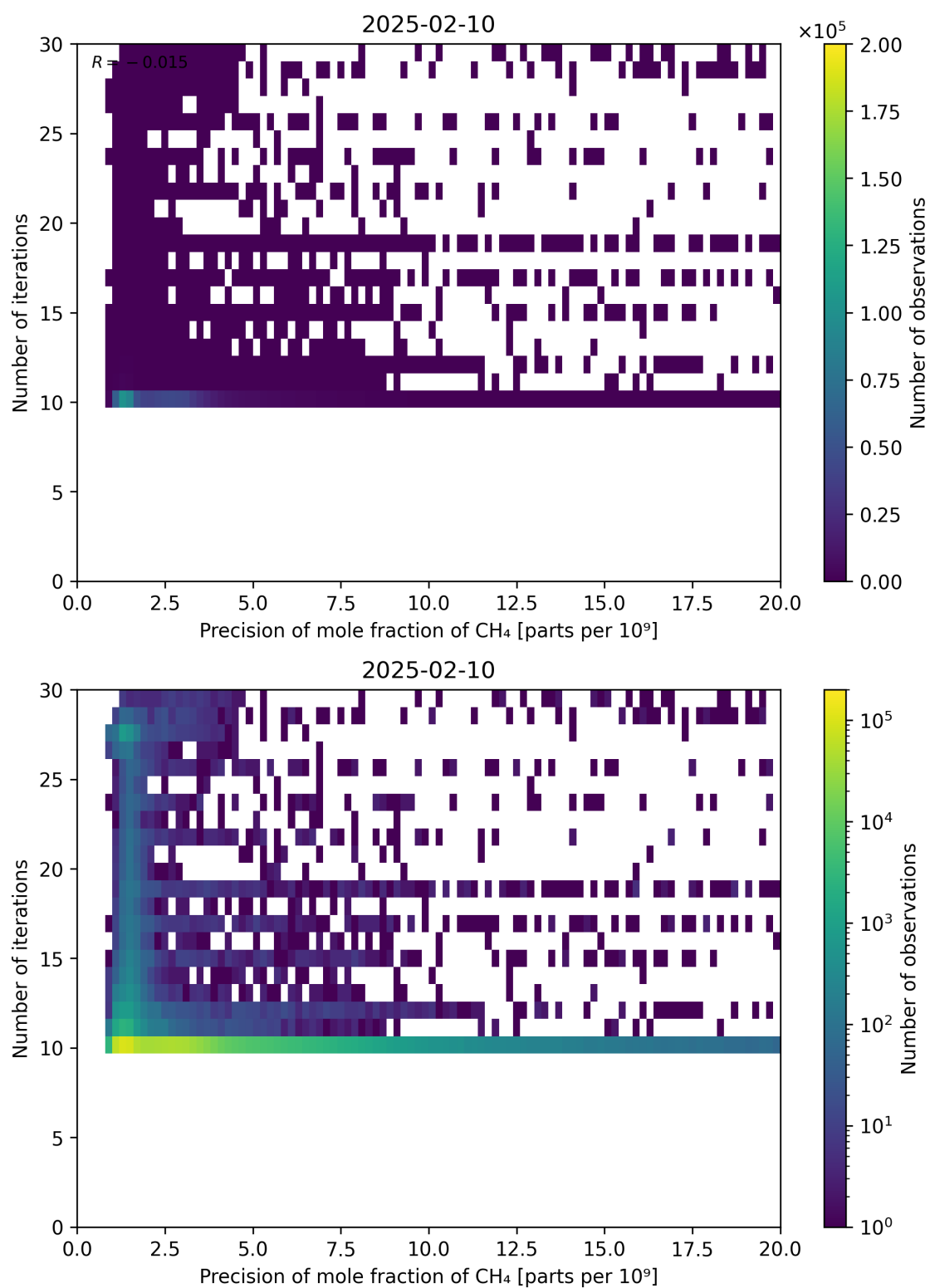
Figure 83: Scatter density plot of “Precision of mole fraction of CH 4 ” against “Number of iterations” for 2025-02-09 to 2025-02-11.
