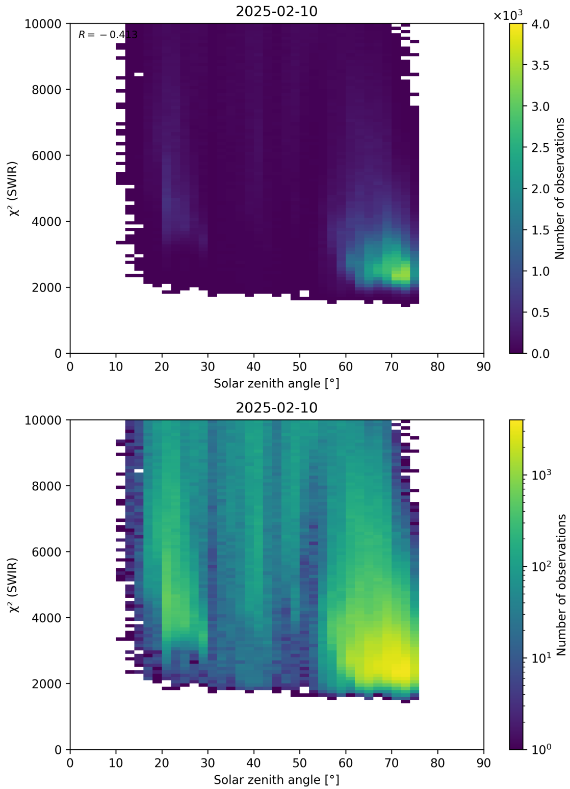
Figure 95: Scatter density plot of “Solar zenith angle” against “ \chi^2 (SWIR)” for 2025-02-09 to 2025-02-11.
