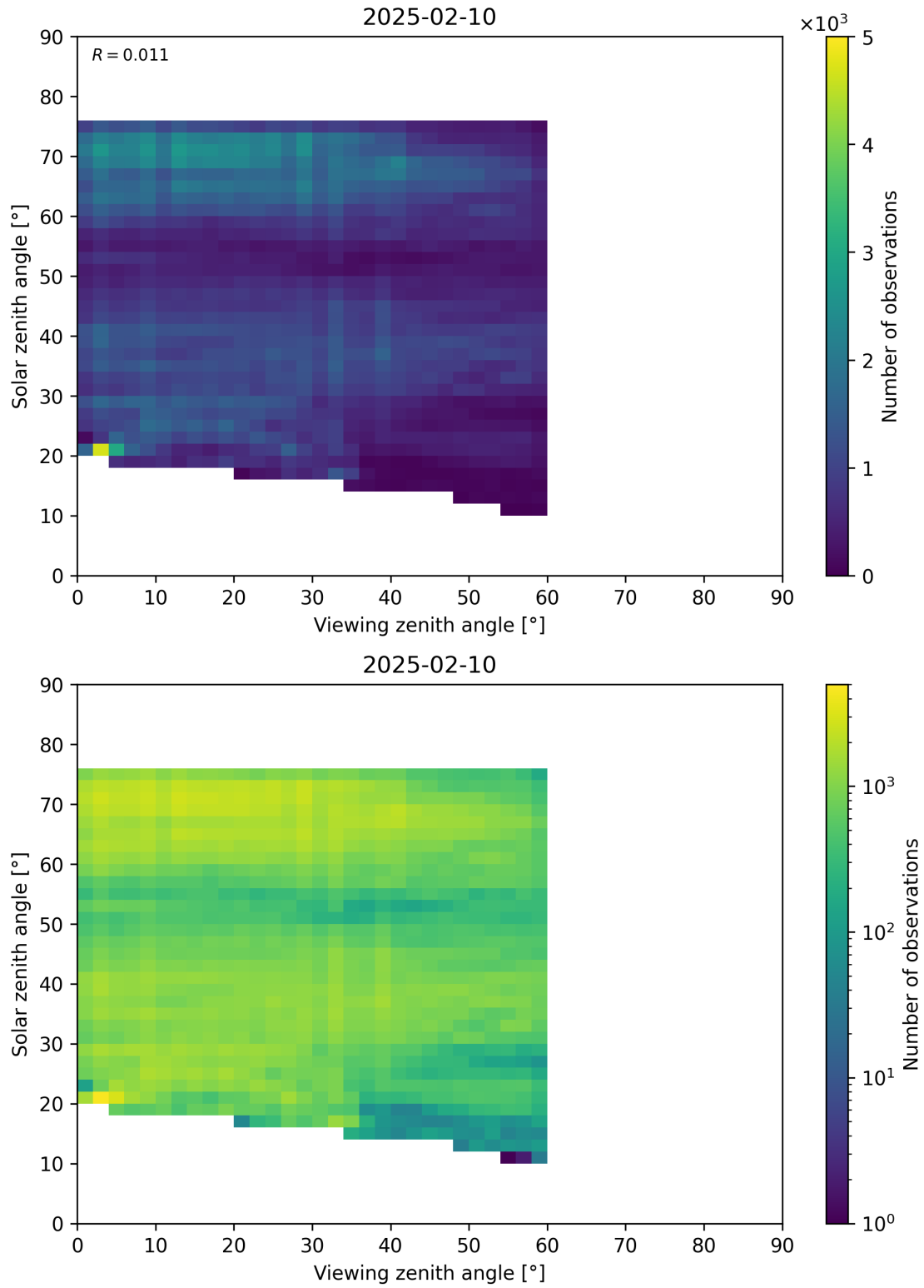
Figure 115: Scatter density plot of “Viewing zenith angle” against “Solar zenith angle” for 2025-02-09 to 2025-02-11.
