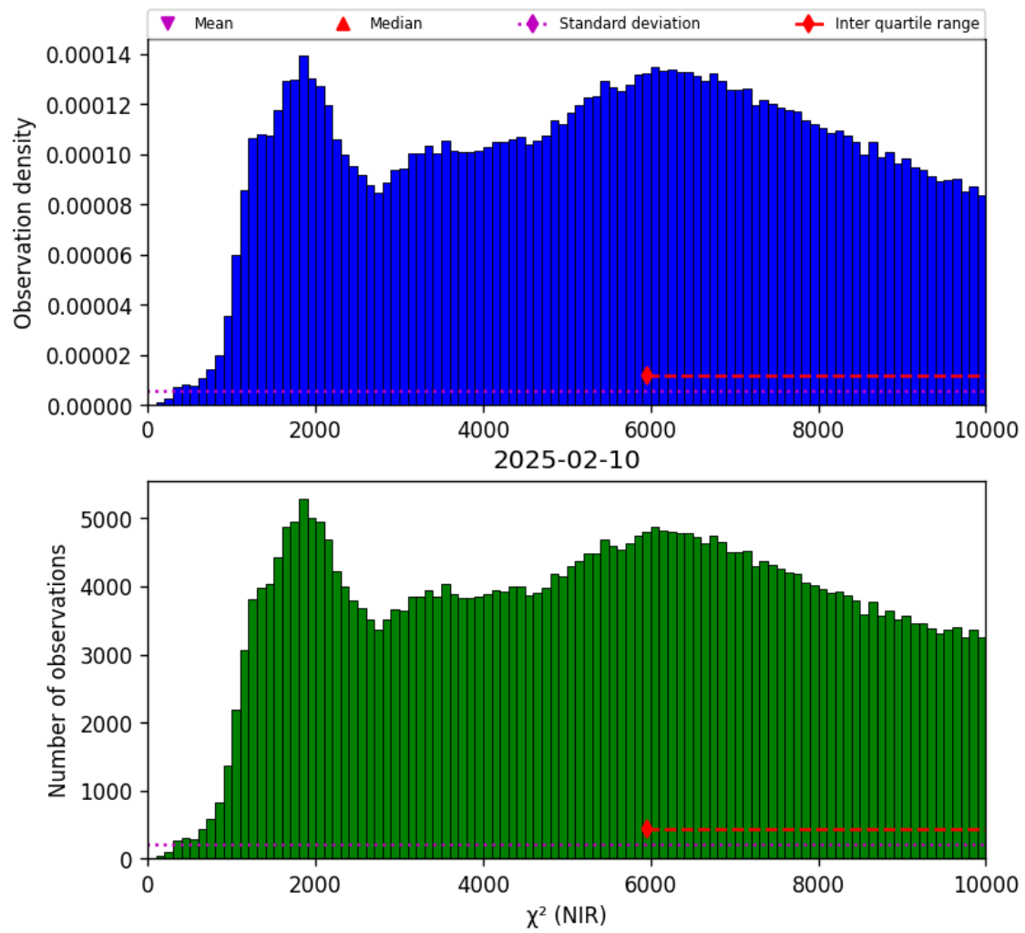
Figure 29: Histogram of “ \chi^2 (NIR)” for 2025-02-09 to 2025-02-11
