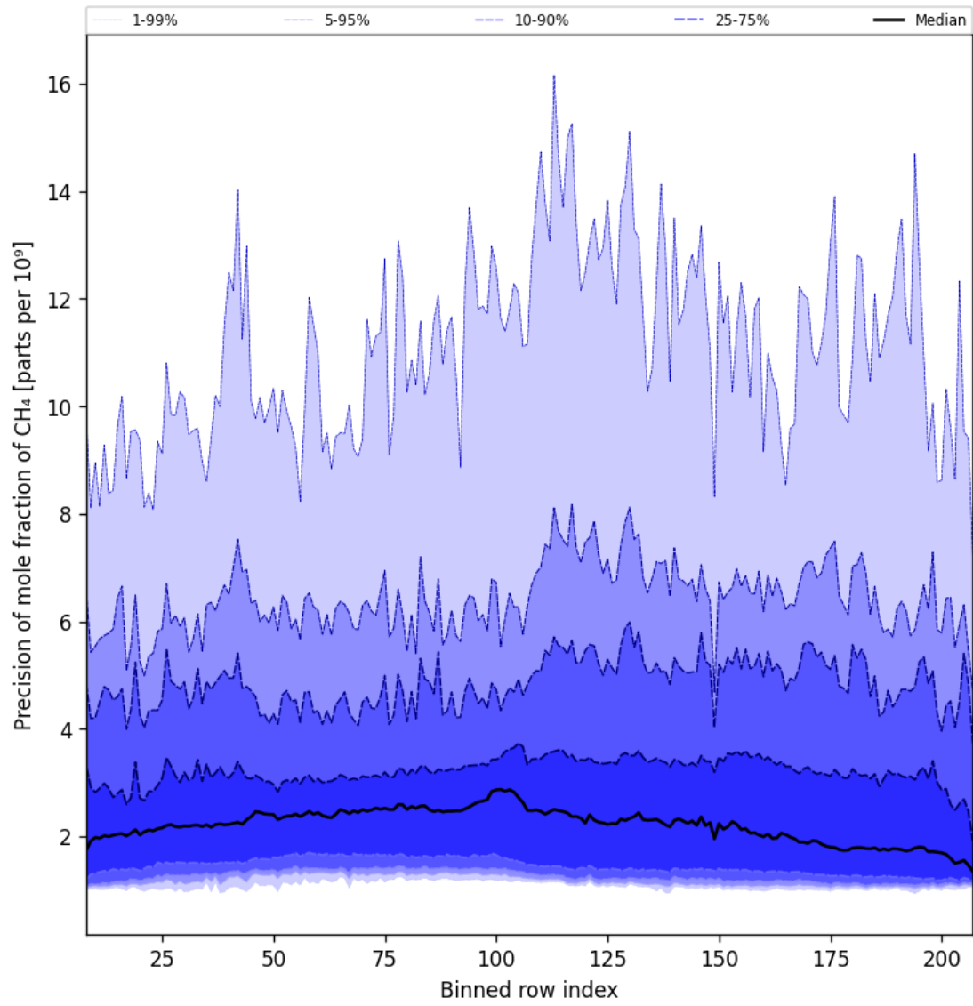
Figure 35: Along track statistics of “Precision of mole fraction of CH 4 ” for 2025-02-09 to 2025-02-11
