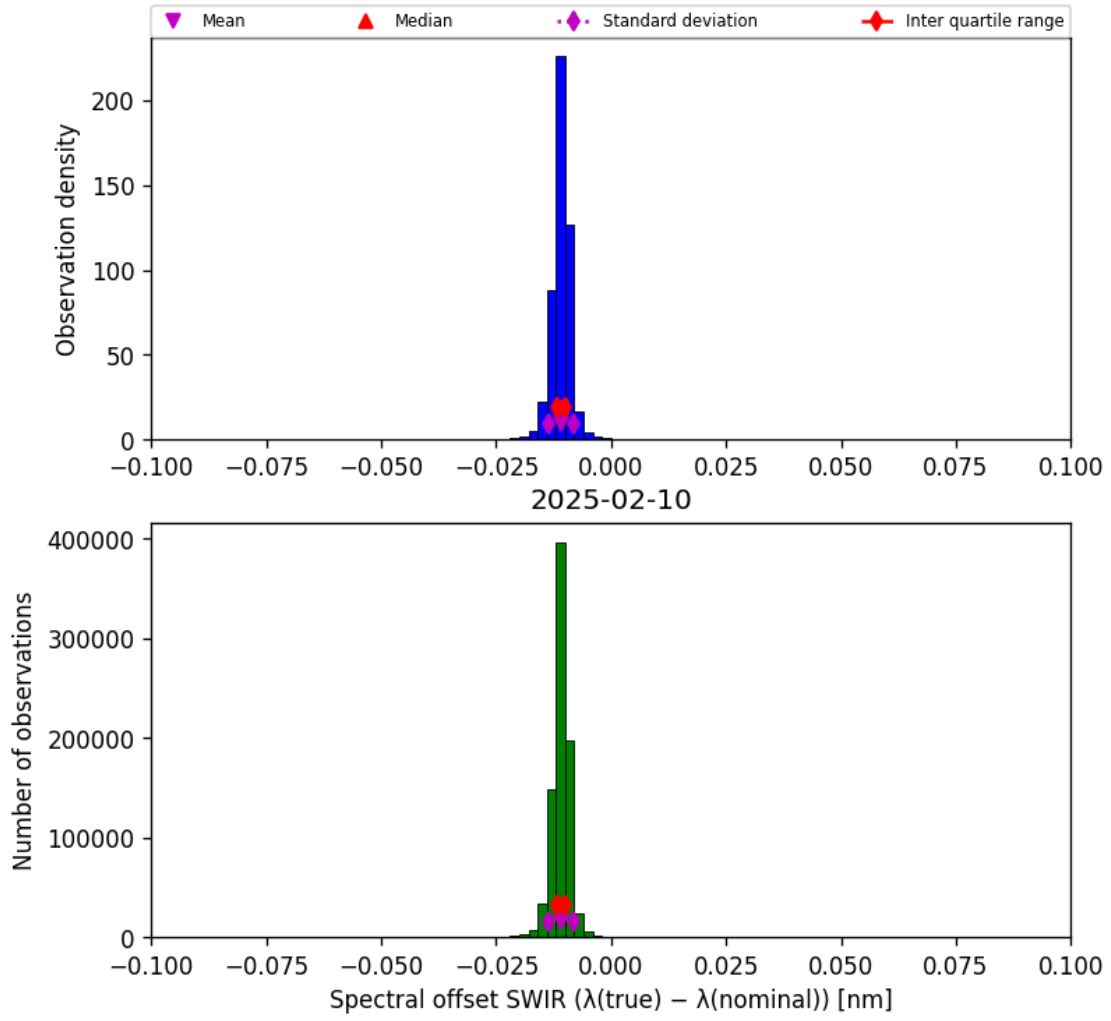
Figure 27: Histogram of “Spectral offset SWIR ( \lambda_{\text{true}} - \lambda_{\text{nominal}} )” for 2025-02-09 to 2025-02-11
