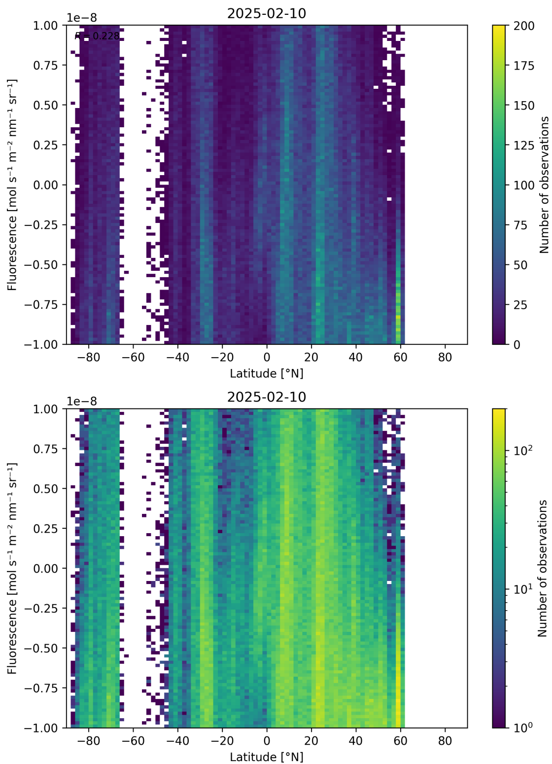
Figure 56: Scatter density plot of “Latitude” against “Fluorescence” for 2025-02-09 to 2025-02-11.
