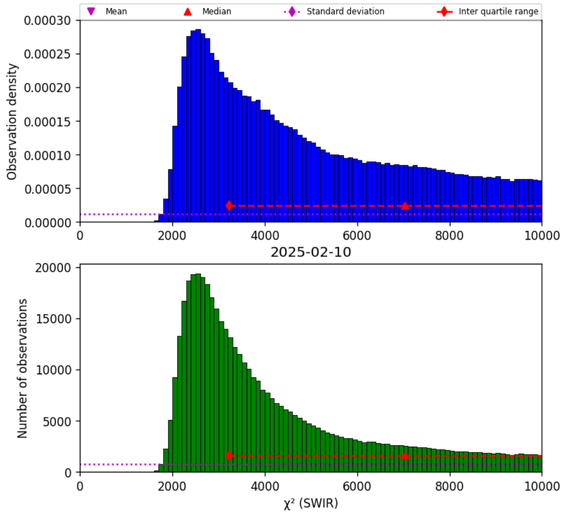
Figure 28: Histogram of “ \chi^2 (SWIR)” for 2025-02-09 to 2025-02-11
