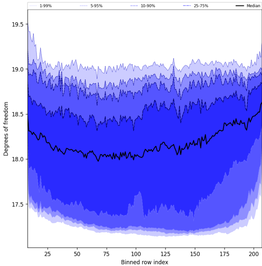
Figure 41: Along track statistics of “Degrees of freedom” for 2025-02-09 to 2025-02-11
