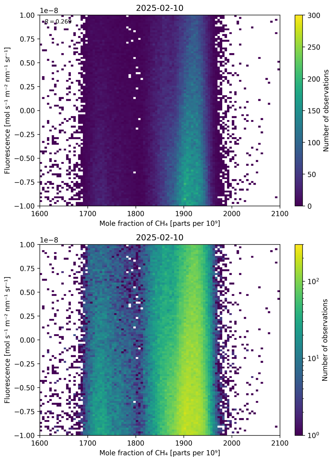
Figure 73: Scatter density plot of “Mole fraction of \text{CH}_4 ” against “Fluorescence” for 2025-02-09 to 2025-02-11.
