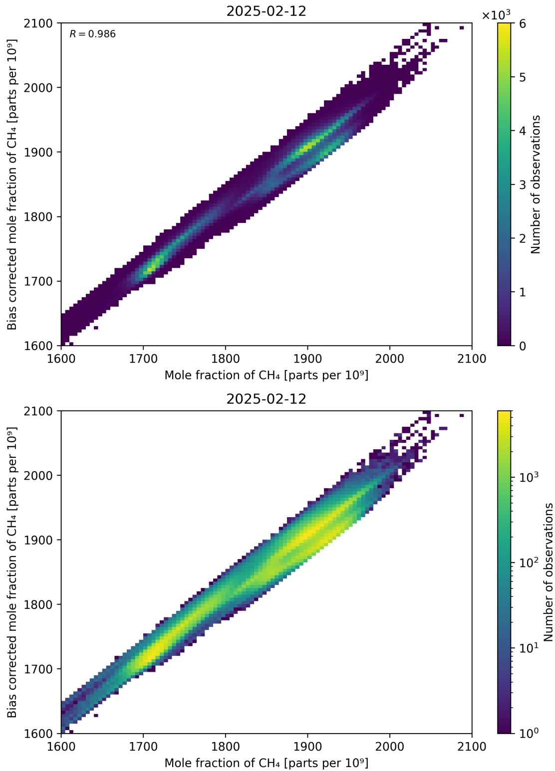
Figure 74: Scatter density plot of “Mole fraction of CH 4 ” against “Bias corrected mole fraction of CH 4 ” for 2025-02-11 to 2025-02-13.
