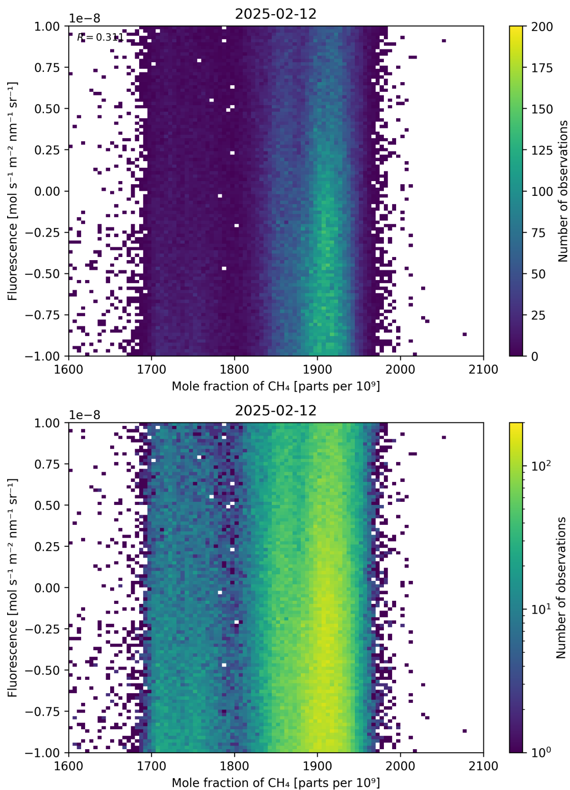
Figure 73: Scatter density plot of “Mole fraction of \text{CH}_4 ” against “Fluorescence” for 2025-02-11 to 2025-02-13.
