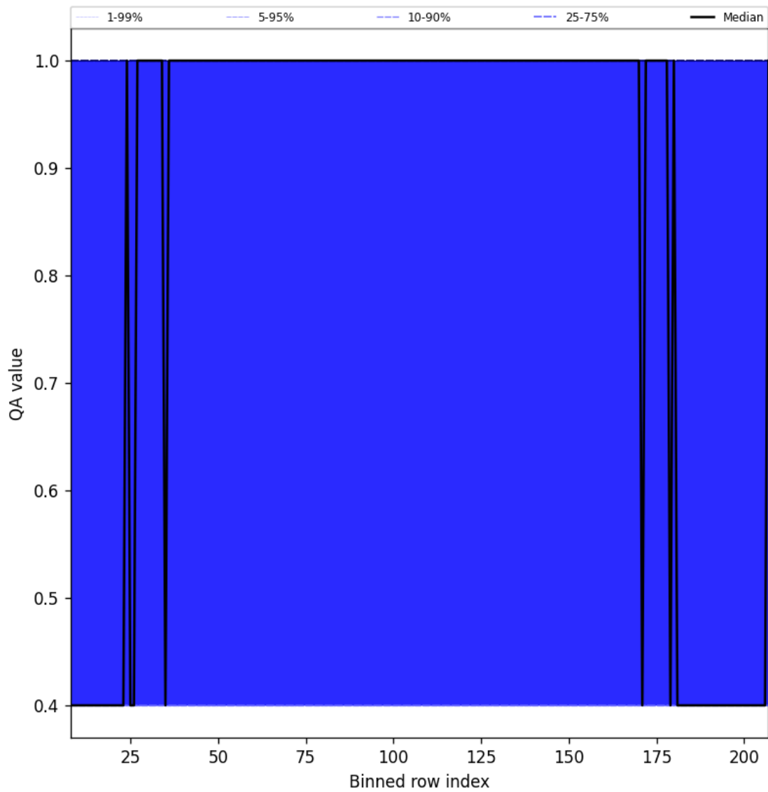
Figure 33: Along track statistics of “QA value” for 2025-02-11 to 2025-02-13
