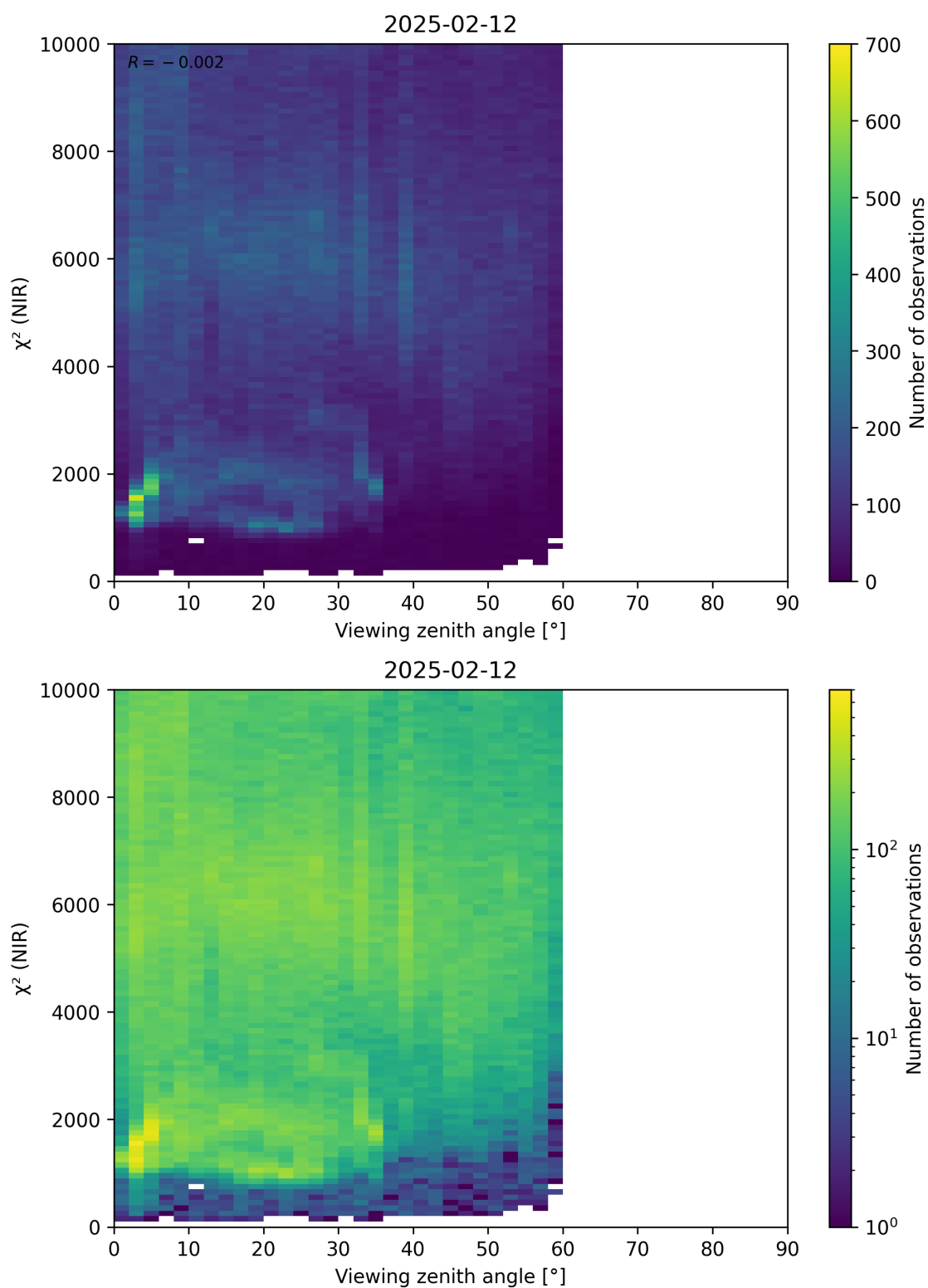
Figure 105: Scatter density plot of “Viewing zenith angle” against “ \chi^2 (NIR)” for 2025-02-11 to 2025-02-13.
