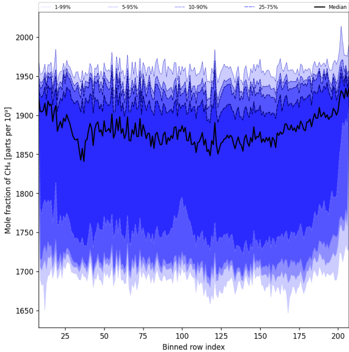
Figure 34: Along track statistics of “Mole fraction of CH 4 ” for 2025-02-11 to 2025-02-13
