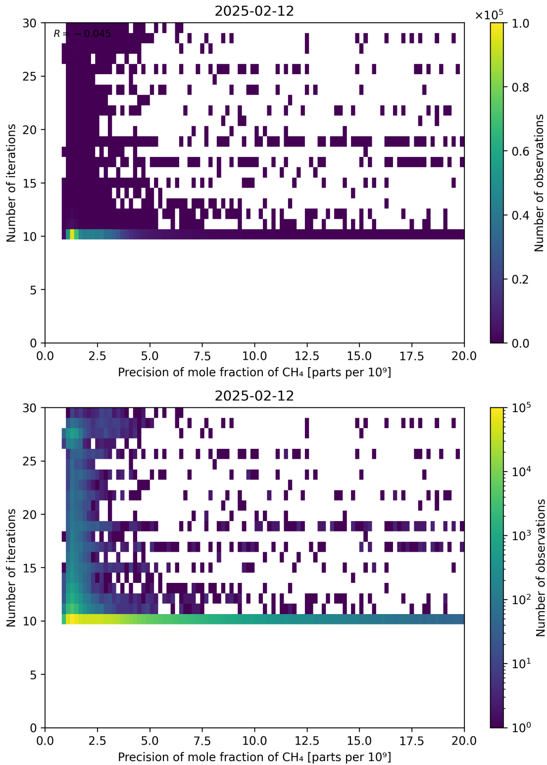
Figure 83: Scatter density plot of “Precision of mole fraction of CH 4 ” against “Number of iterations” for 2025-02-11 to 2025-02-13.
