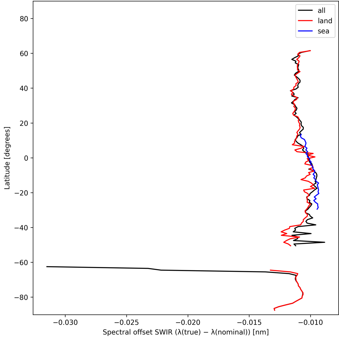
Figure 16: Zonal average of “Spectral offset SWIR ( \lambda_{\text{true}} - \lambda_{\text{nominal}} )” for 2025-02-11 to 2025-02-13.
