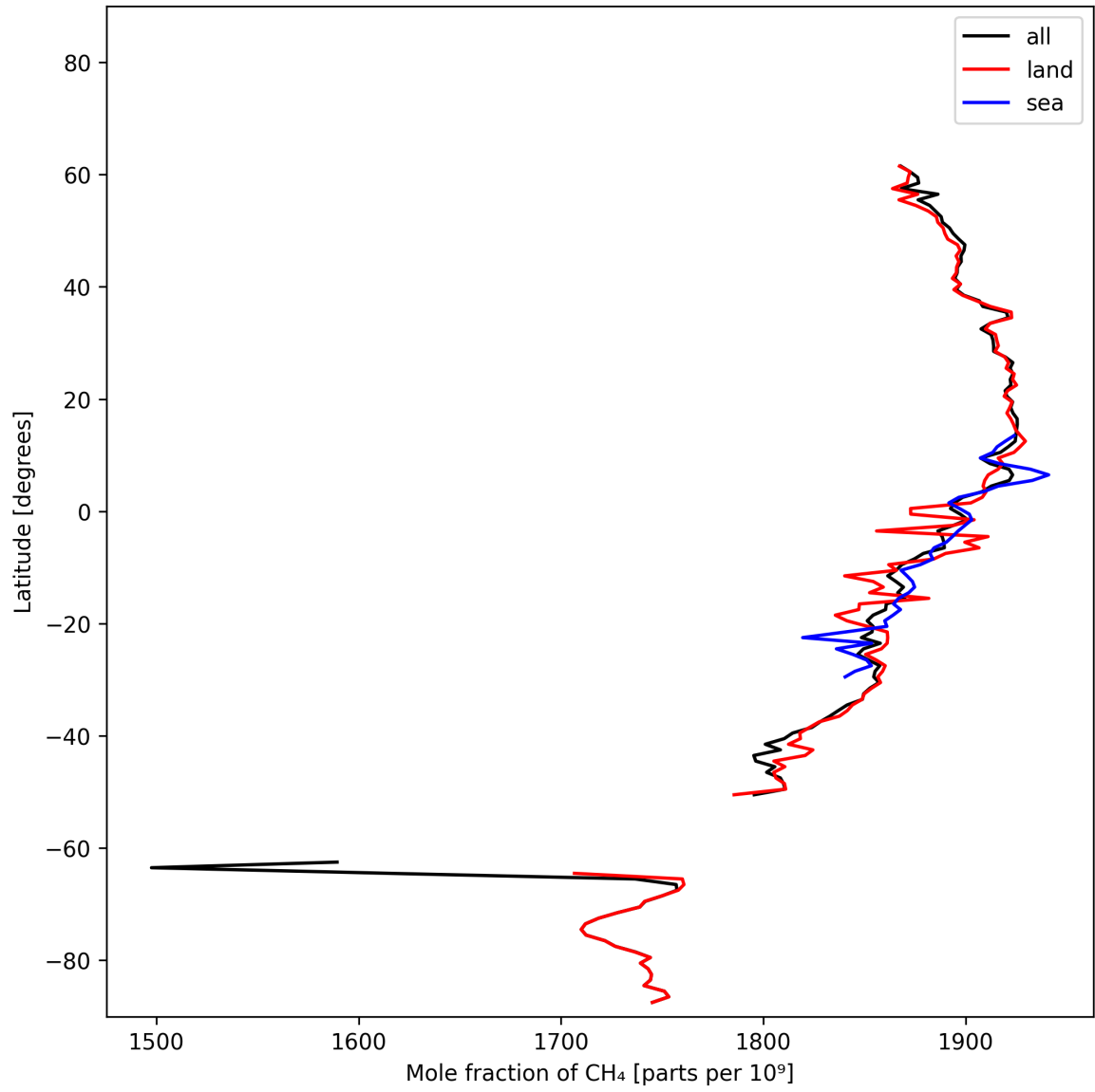
Figure 12: Zonal average of “Mole fraction of \text{CH}_4 ” for 2025-02-11 to 2025-02-13.
