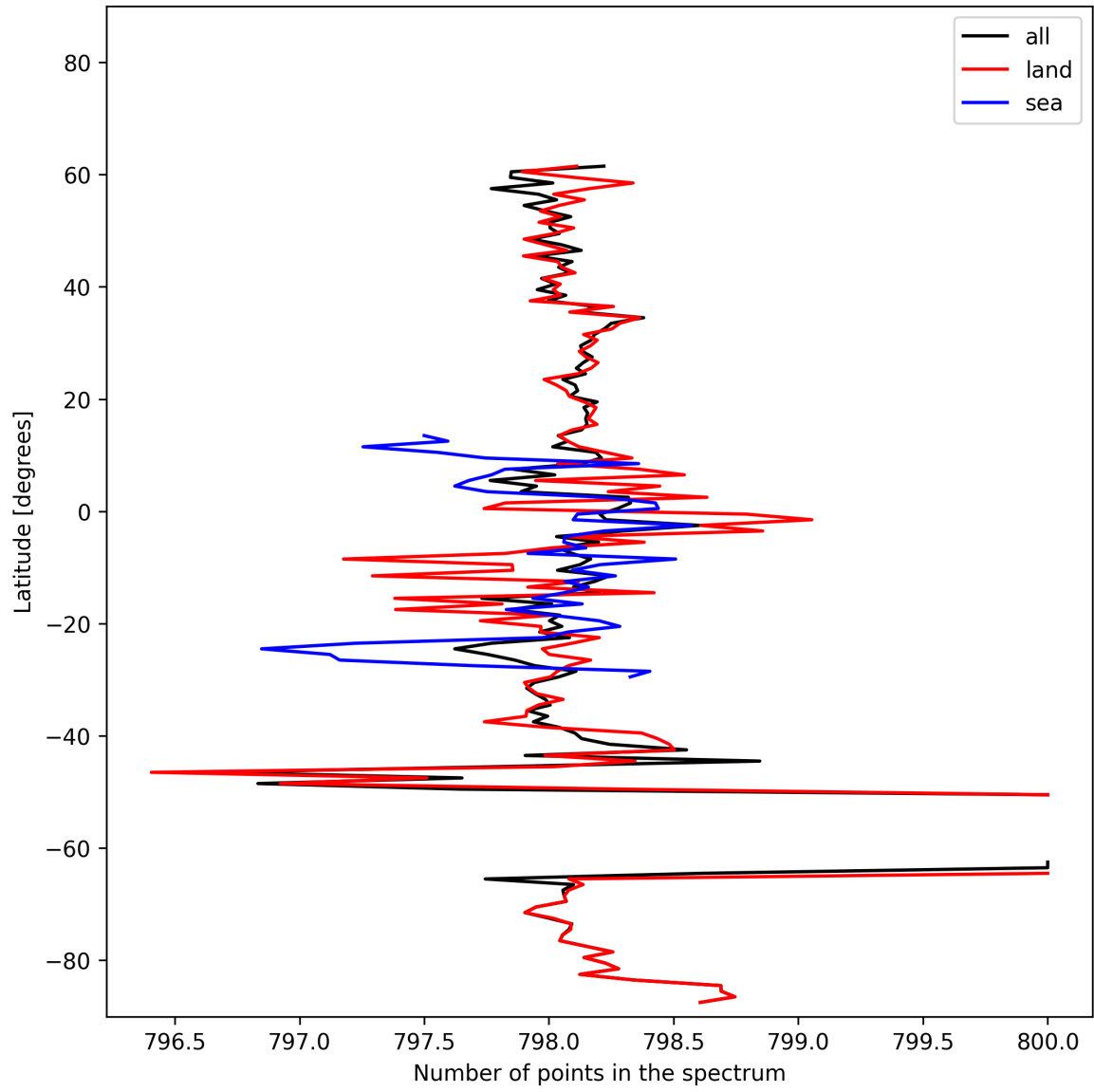
Figure 15: Zonal average of “Number of points in the spectrum” for 2025-02-11 to 2025-02-13.
