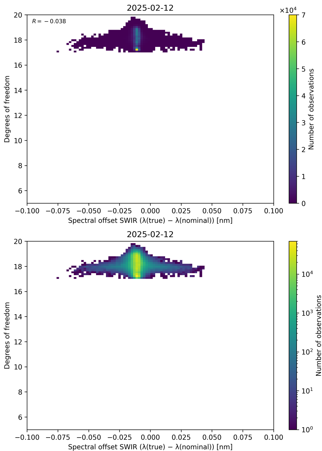
Figure 119: Scatter density plot of “Spectral offset SWIR ( \lambda_{\text{true}} - \lambda_{\text{nominal}} )” against “Degrees of freedom” for 2025-02-11 to 2025-02-13.
