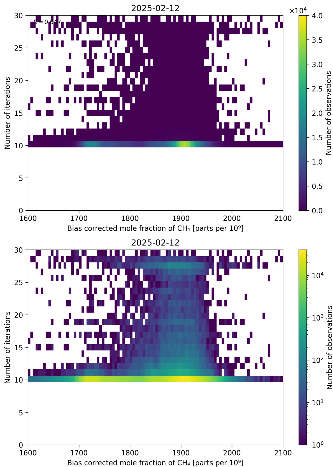
Figure 67: Scatter density plot of “Bias corrected mole fraction of \text{CH}_4 ” against “Number of iterations” for 2025-02-11 to 2025-02-13.
