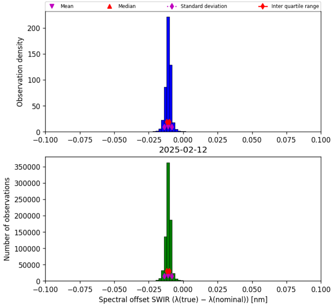
Figure 27: Histogram of “Spectral offset SWIR ( \lambda_{\text{true}} - \lambda_{\text{nominal}} )” for 2025-02-11 to 2025-02-13
