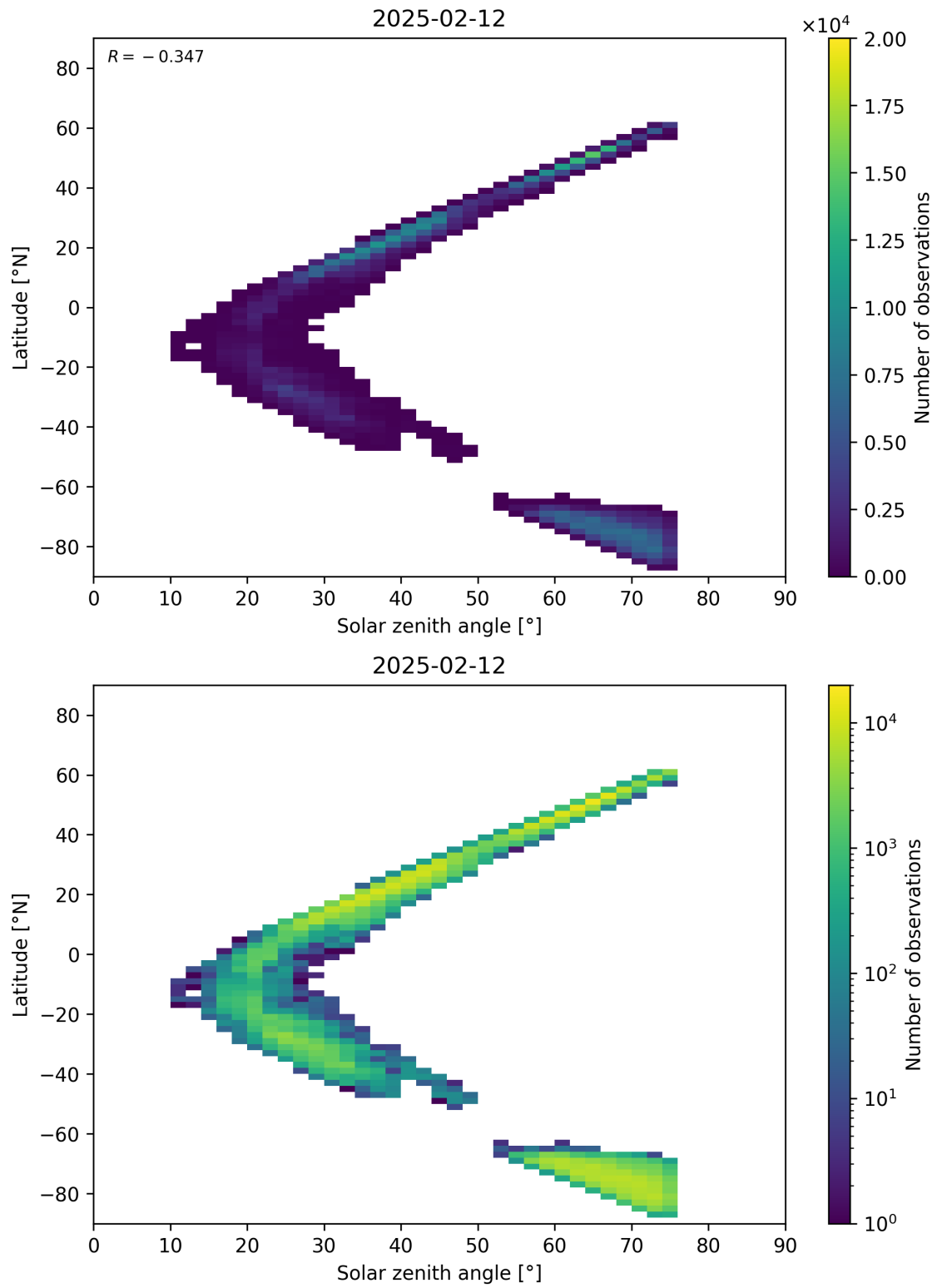
Figure 98: Scatter density plot of “Solar zenith angle” against “Latitude” for 2025-02-11 to 2025-02-13.
