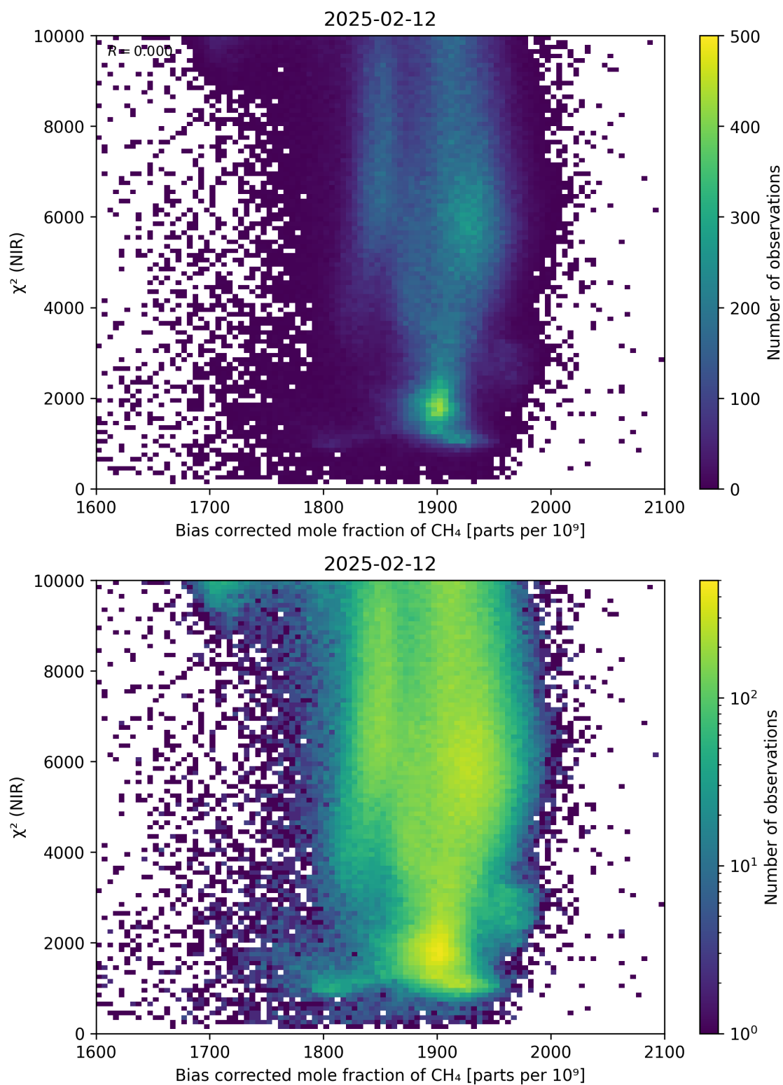
Figure 63: Scatter density plot of “Bias corrected mole fraction of \text{CH}_4 ” against “ \chi^2 (NIR)” for 2025-02-11 to 2025-02-13.
