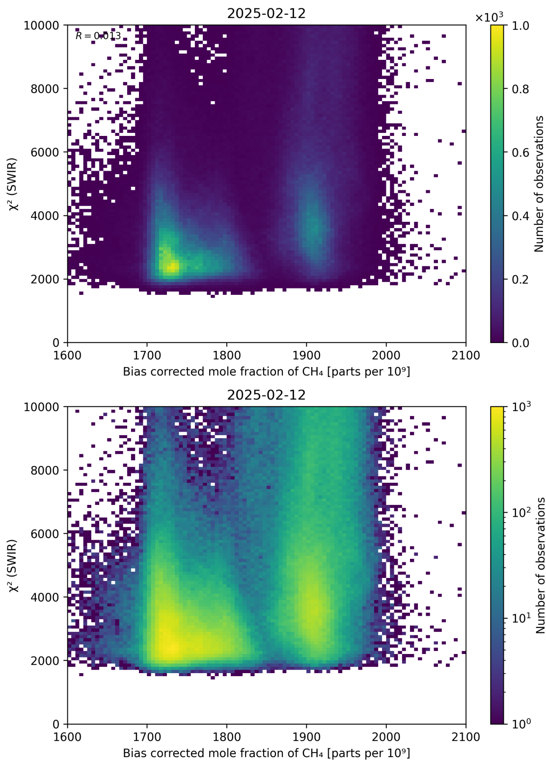
Figure 64: Scatter density plot of “Bias corrected mole fraction of \text{CH}_4 ” against “ \chi^2 (SWIR)” for 2025-02-11 to 2025-02-13.
