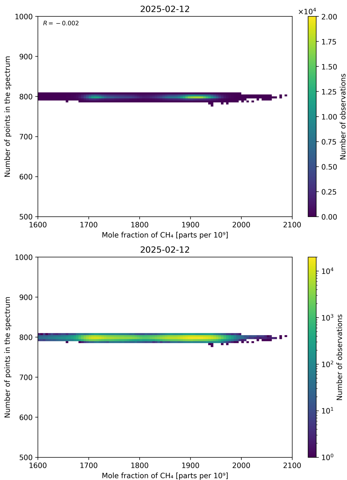
Figure 77: Scatter density plot of “Mole fraction of CH 4 ” against “Number of points in the spectrum” for 2025-02-11 to 2025-02-13.
