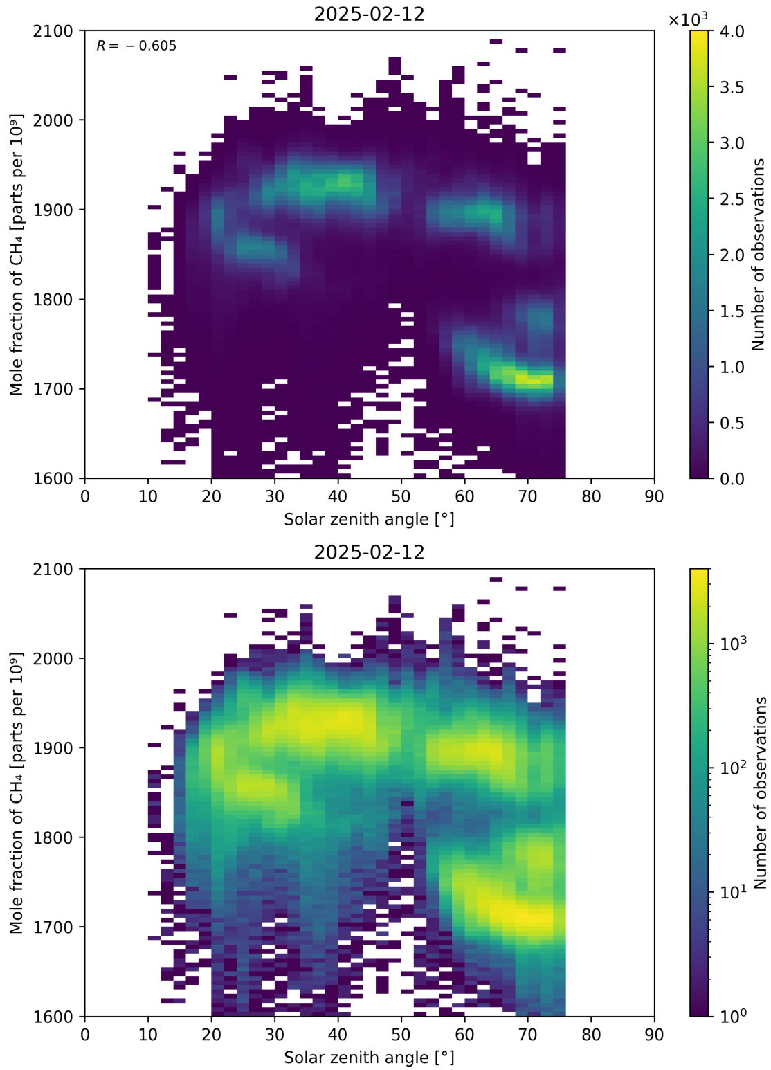
Figure 99: Scatter density plot of “Solar zenith angle” against “Mole fraction of CH 4 ” for 2025-02-11 to 2025-02-13.
