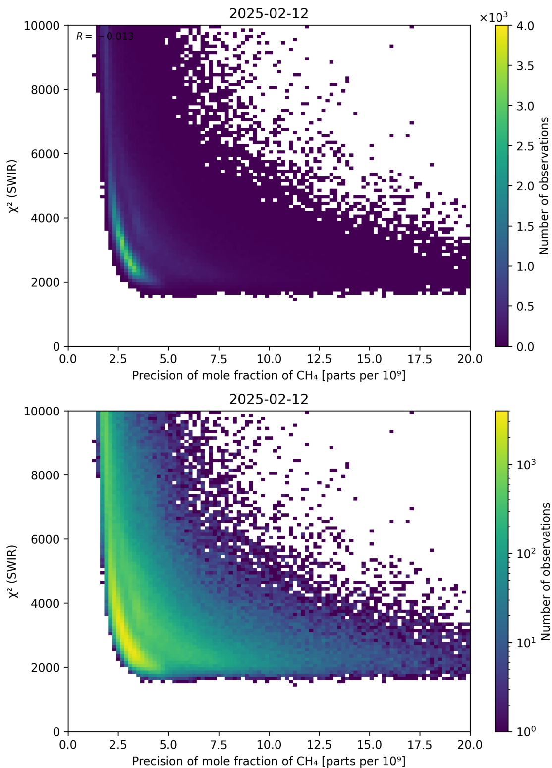
Figure 79: Scatter density plot of “Precision of mole fraction of CH 4 ” against “ \chi^2 (SWIR)” for 2025-02-11 to 2025-02-13.
