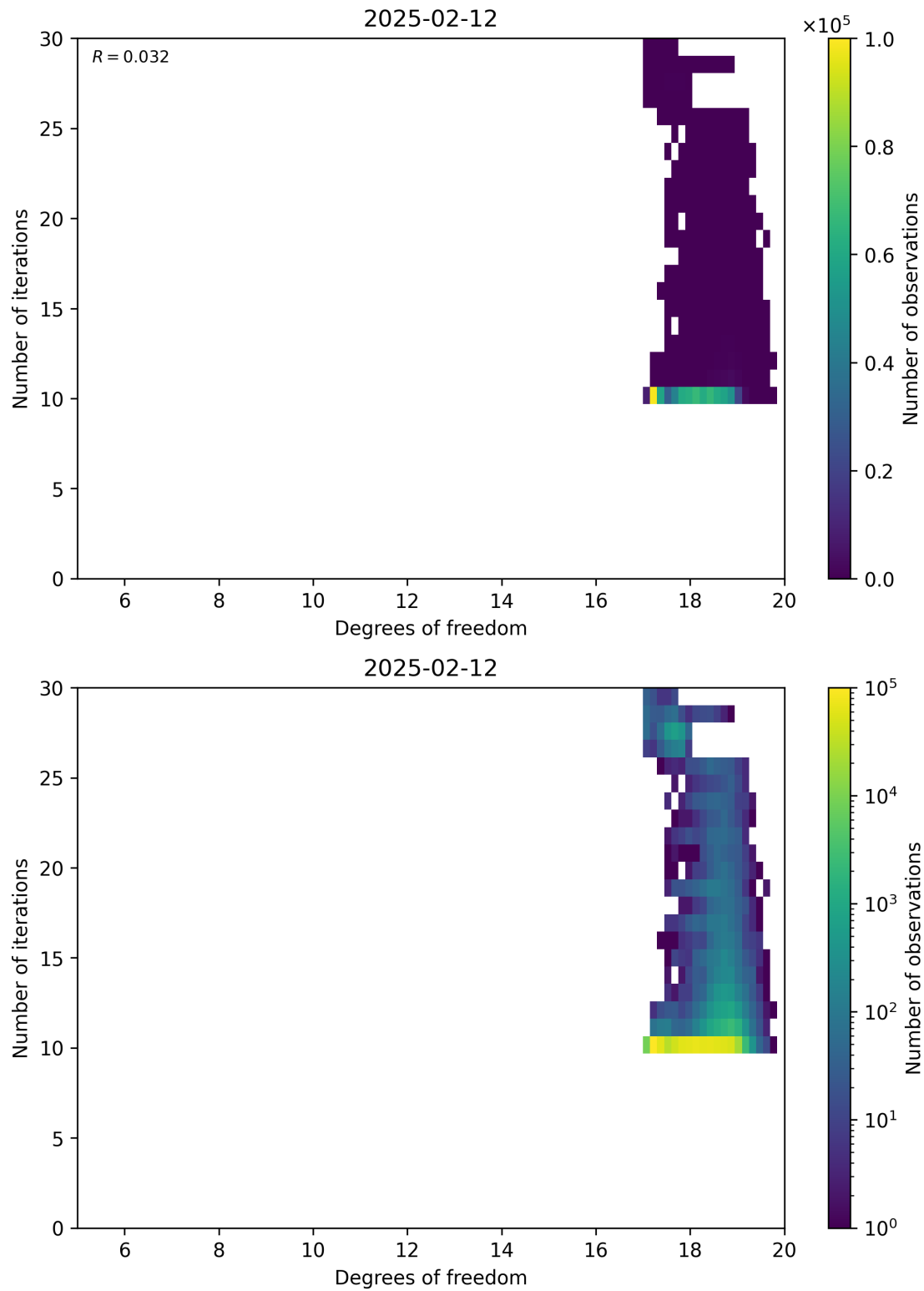
Figure 52: Scatter density plot of “Degrees of freedom” against “Number of iterations” for 2025-02-11 to 2025-02-13.
