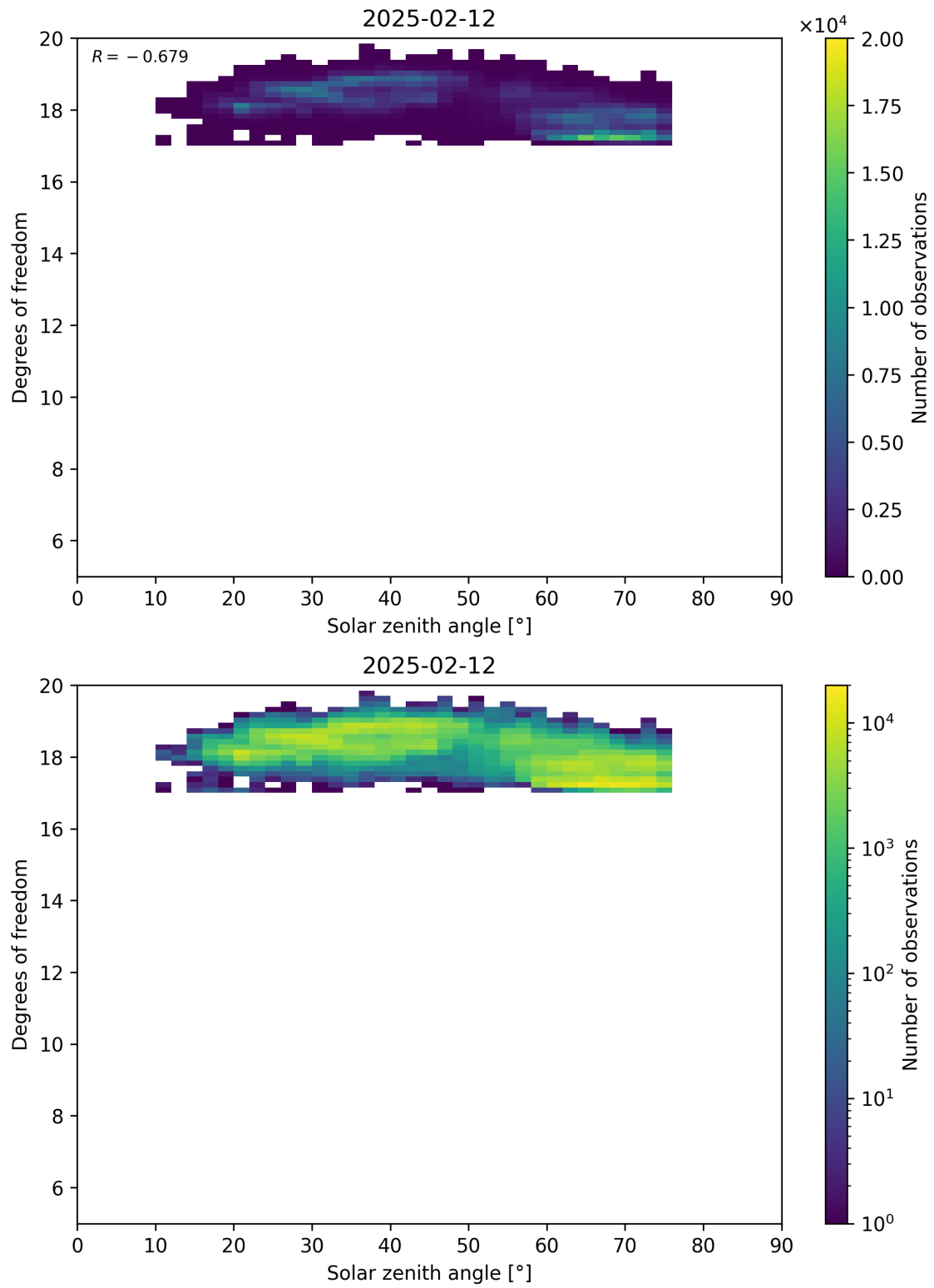
Figure 96: Scatter density plot of “Solar zenith angle” against “Degrees of freedom” for 2025-02-11 to 2025-02-13.
