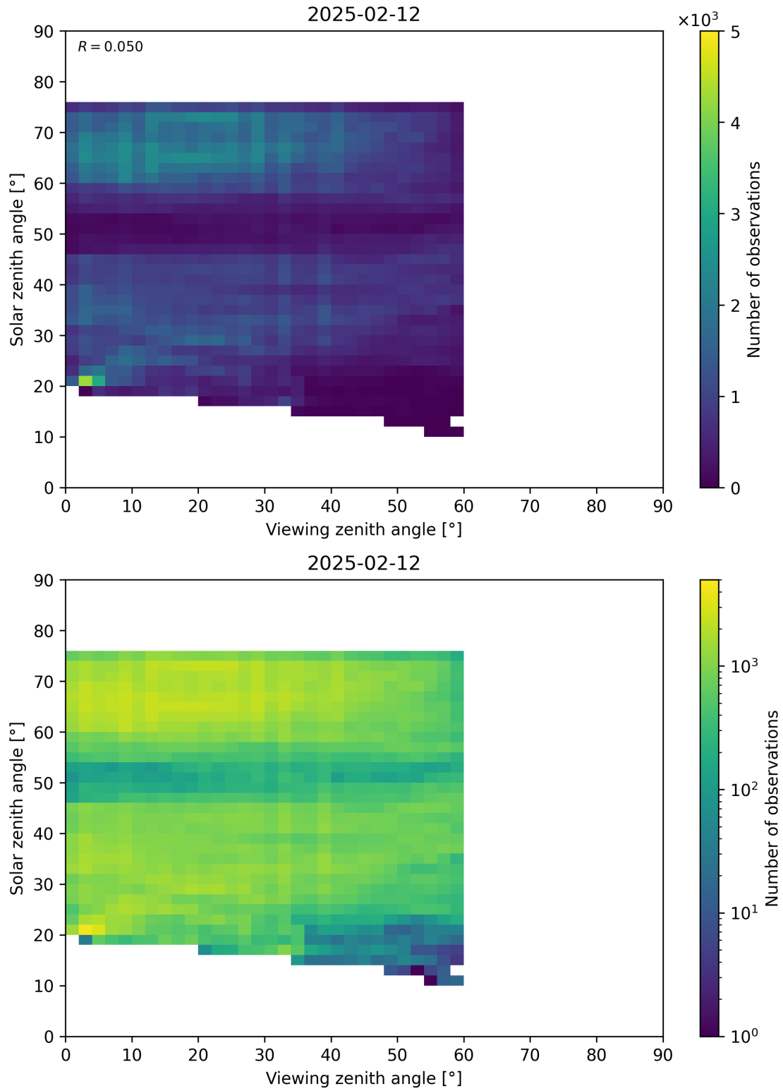
Figure 115: Scatter density plot of “Viewing zenith angle” against “Solar zenith angle” for 2025-02-11 to 2025-02-13.
