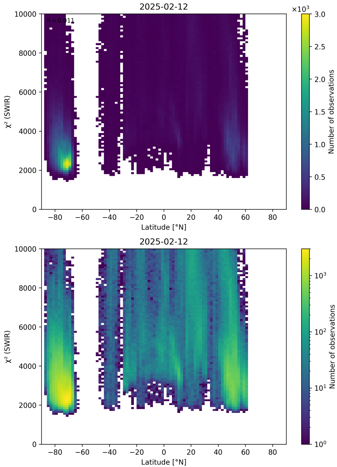
Figure 54: Scatter density plot of “Latitude” against “ \chi^2 (SWIR)” for 2025-02-11 to 2025-02-13.
