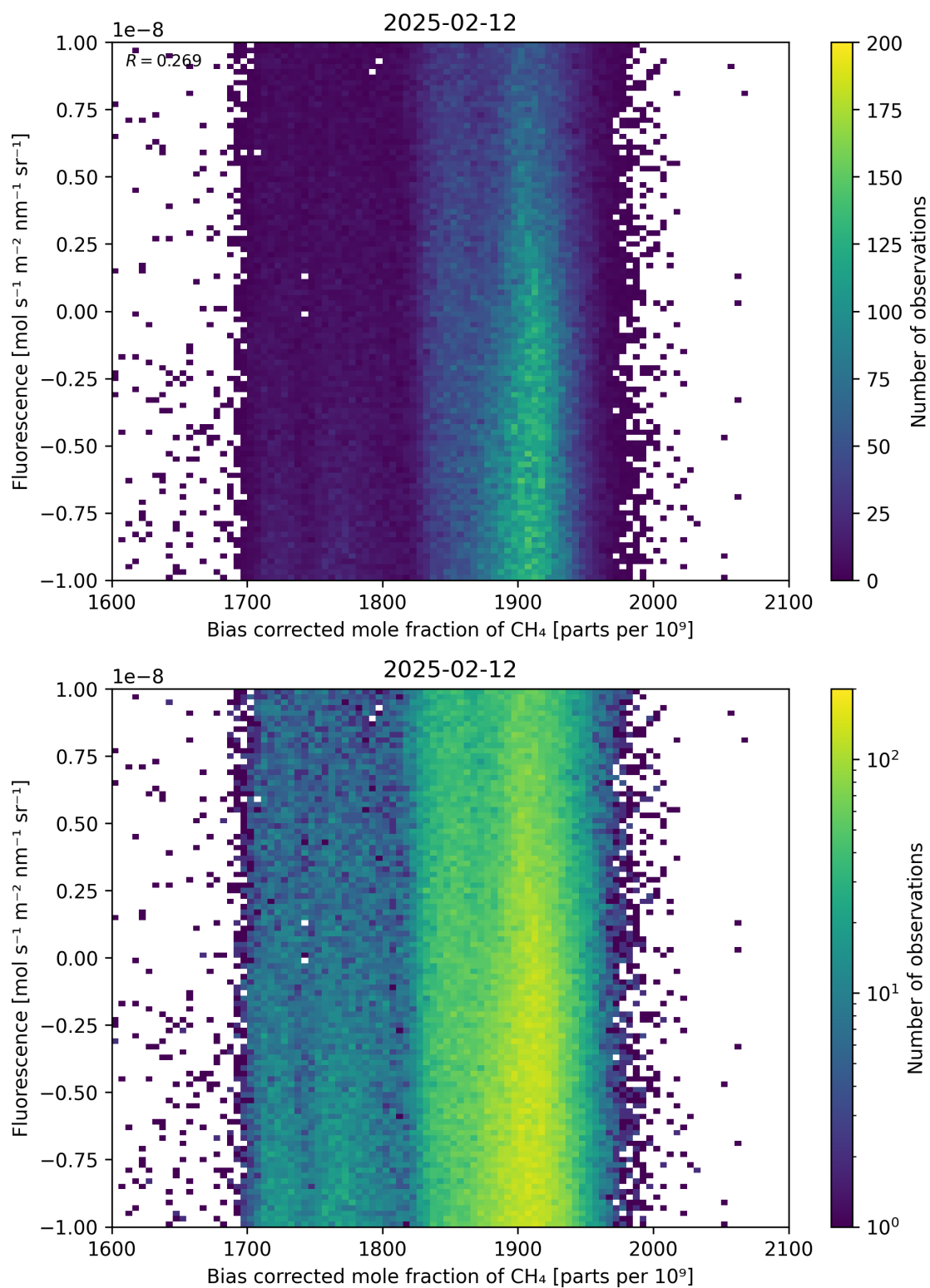
Figure 66: Scatter density plot of “Bias corrected mole fraction of \text{CH}_4 ” against “Fluorescence” for 2025-02-11 to 2025-02-13.
