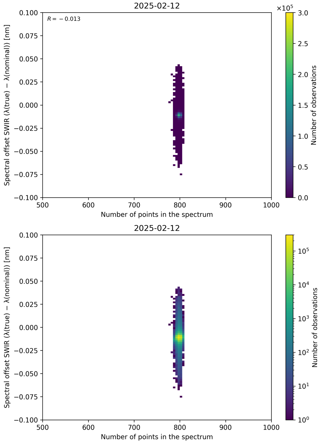
Figure 93: Scatter density plot of “Number of points in the spectrum” against “Spectral offset SWIR ( \lambda_{\text{true}} - \lambda_{\text{nominal}} )” for 2025-02-11 to 2025-02-13.
