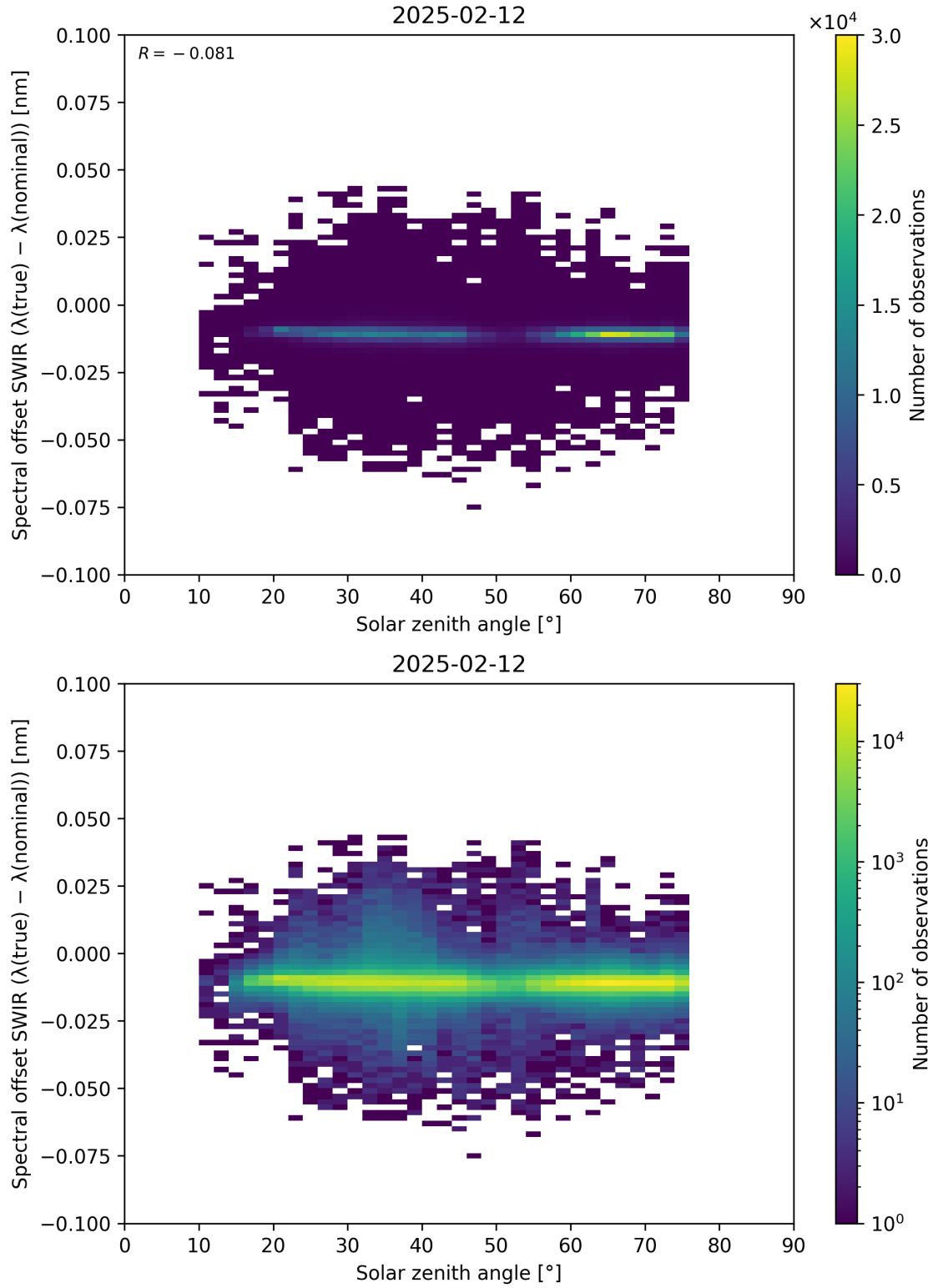
Figure 104: Scatter density plot of “Solar zenith angle” against “Spectral offset SWIR ( \lambda_{\text{true}} - \lambda_{\text{nominal}} )” for 2025-02-11 to 2025-02-13.
