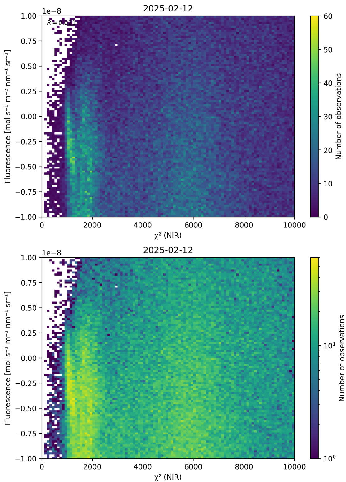
Figure 45: Scatter density plot of “ \chi^2 (NIR)” against “Fluorescence” for 2025-02-11 to 2025-02-13.
