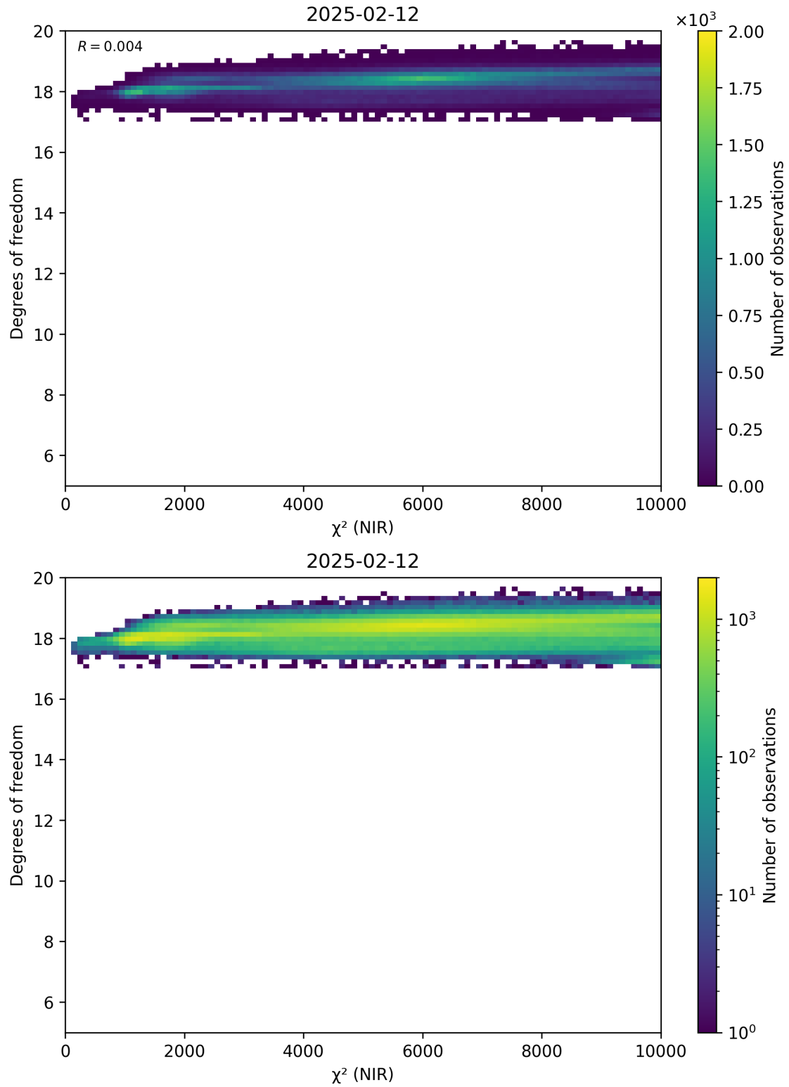
Figure 44: Scatter density plot of “ \chi^2 (NIR)” against “Degrees of freedom” for 2025-02-11 to 2025-02-13.
