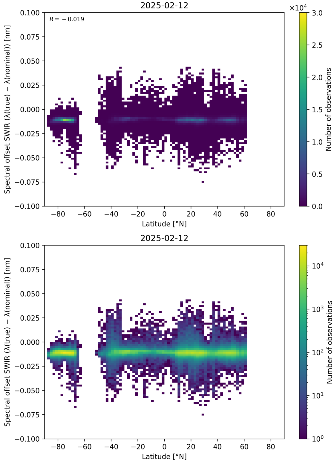
Figure 62: Scatter density plot of “Latitude” against “Spectral offset SWIR ( \lambda_{\text{true}} - \lambda_{\text{nominal}} )” for 2025-02-11 to 2025-02-13.
