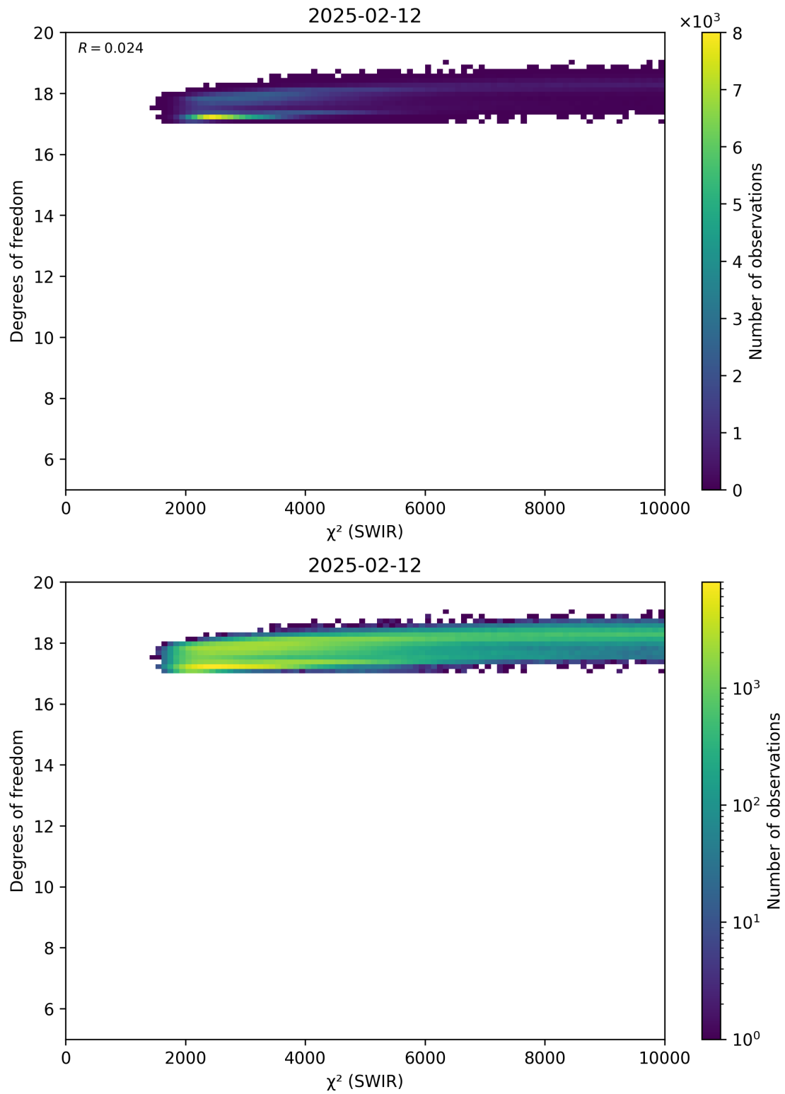
Figure 48: Scatter density plot of “ \chi^2 (SWIR)” against “Degrees of freedom” for 2025-02-11 to 2025-02-13.
