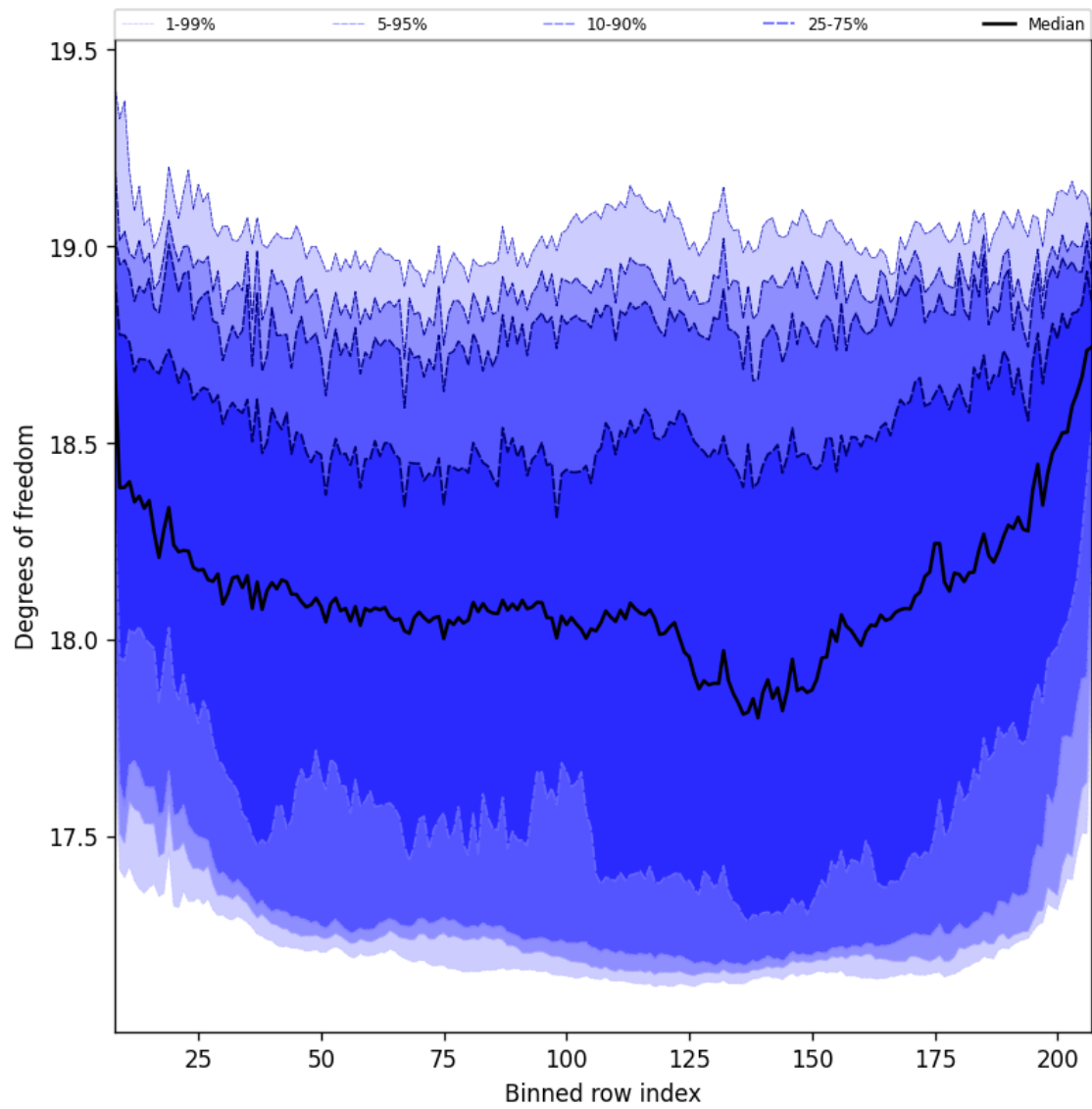
Figure 41: Along track statistics of “Degrees of freedom” for 2025-02-11 to 2025-02-13
