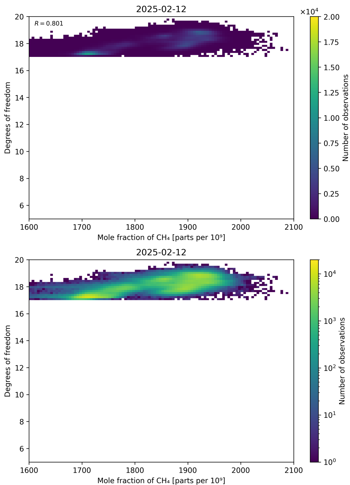
Figure 72: Scatter density plot of “Mole fraction of CH 4 ” against “Degrees of freedom” for 2025-02-11 to 2025-02-13.
