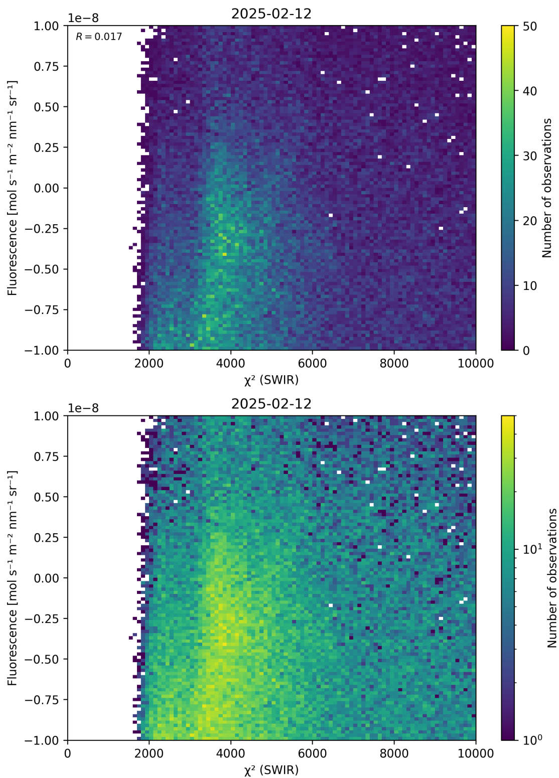
Figure 49: Scatter density plot of “ \chi^2 (SWIR)” against “Fluorescence” for 2025-02-11 to 2025-02-13.
