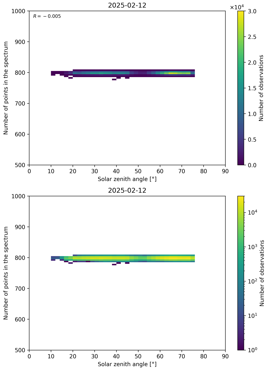
Figure 103: Scatter density plot of “Solar zenith angle” against “Number of points in the spectrum” for 2025-02-11 to 2025-02-13.
