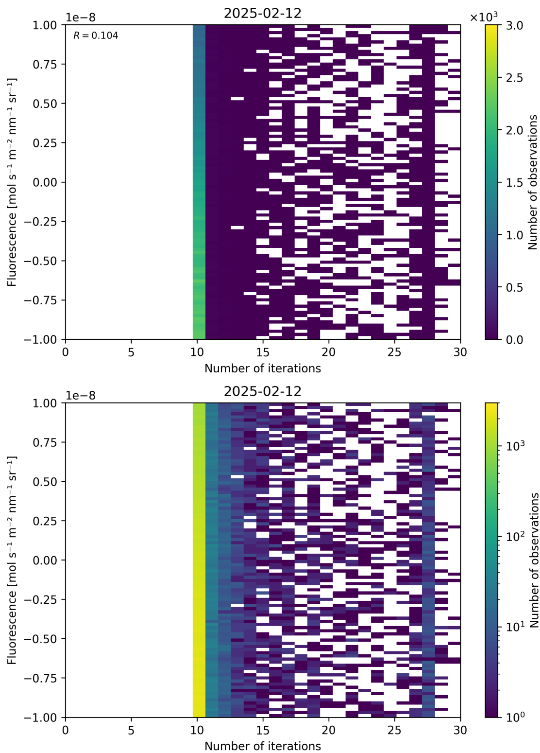
Figure 87: Scatter density plot of “Number of iterations” against “Fluorescence” for 2025-02-11 to 2025-02-13.
