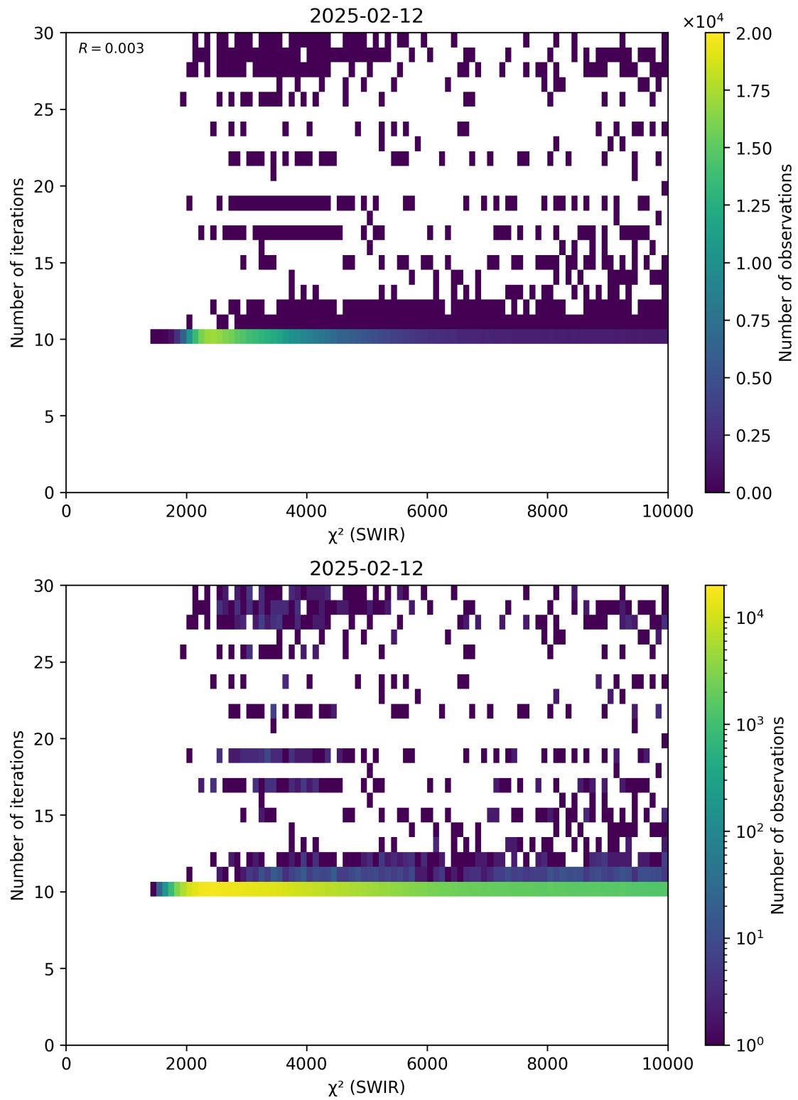
Figure 50: Scatter density plot of “ \chi^2 (SWIR)” against “Number of iterations” for 2025-02-11 to 2025-02-13.
