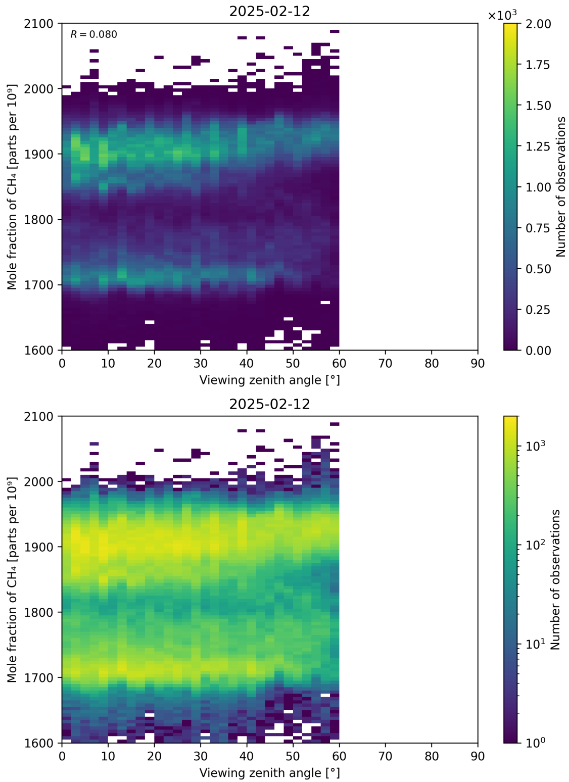
Figure 110: Scatter density plot of “Viewing zenith angle” against “Mole fraction of CH 4 ” for 2025-02-11 to 2025-02-13.
