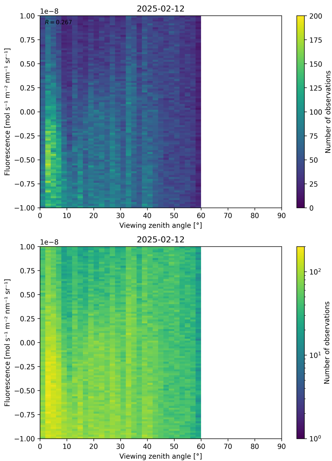
Figure 108: Scatter density plot of “Viewing zenith angle” against “Fluorescence” for 2025-02-11 to 2025-02-13.
