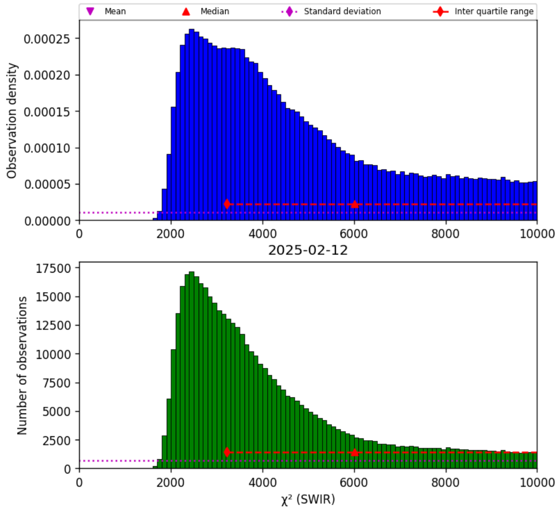
Figure 28: Histogram of “ \chi^2 (SWIR)” for 2025-02-11 to 2025-02-13
