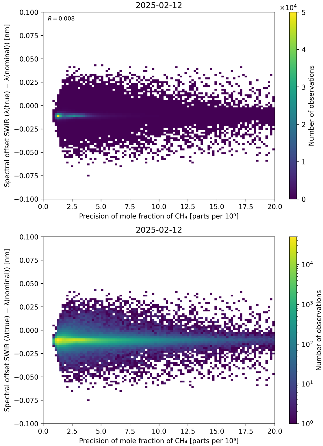
Figure 85: Scatter density plot of “Precision of mole fraction of \text{CH}_4 ” against “Spectral offset SWIR ( \lambda_{\text{true}} - \lambda_{\text{nominal}} )” for 2025-02-11 to 2025-02-13.
