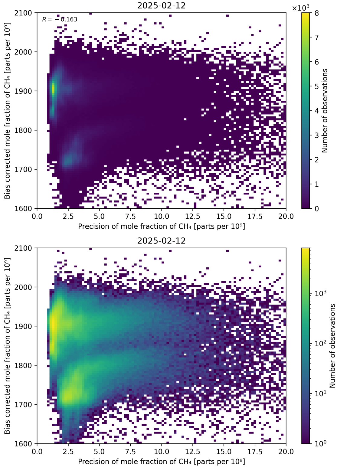
Figure 82: Scatter density plot of “Precision of mole fraction of CH 4 ” against “Bias corrected mole fraction of CH 4 ” for 2025-02-11 to 2025-02-13.
