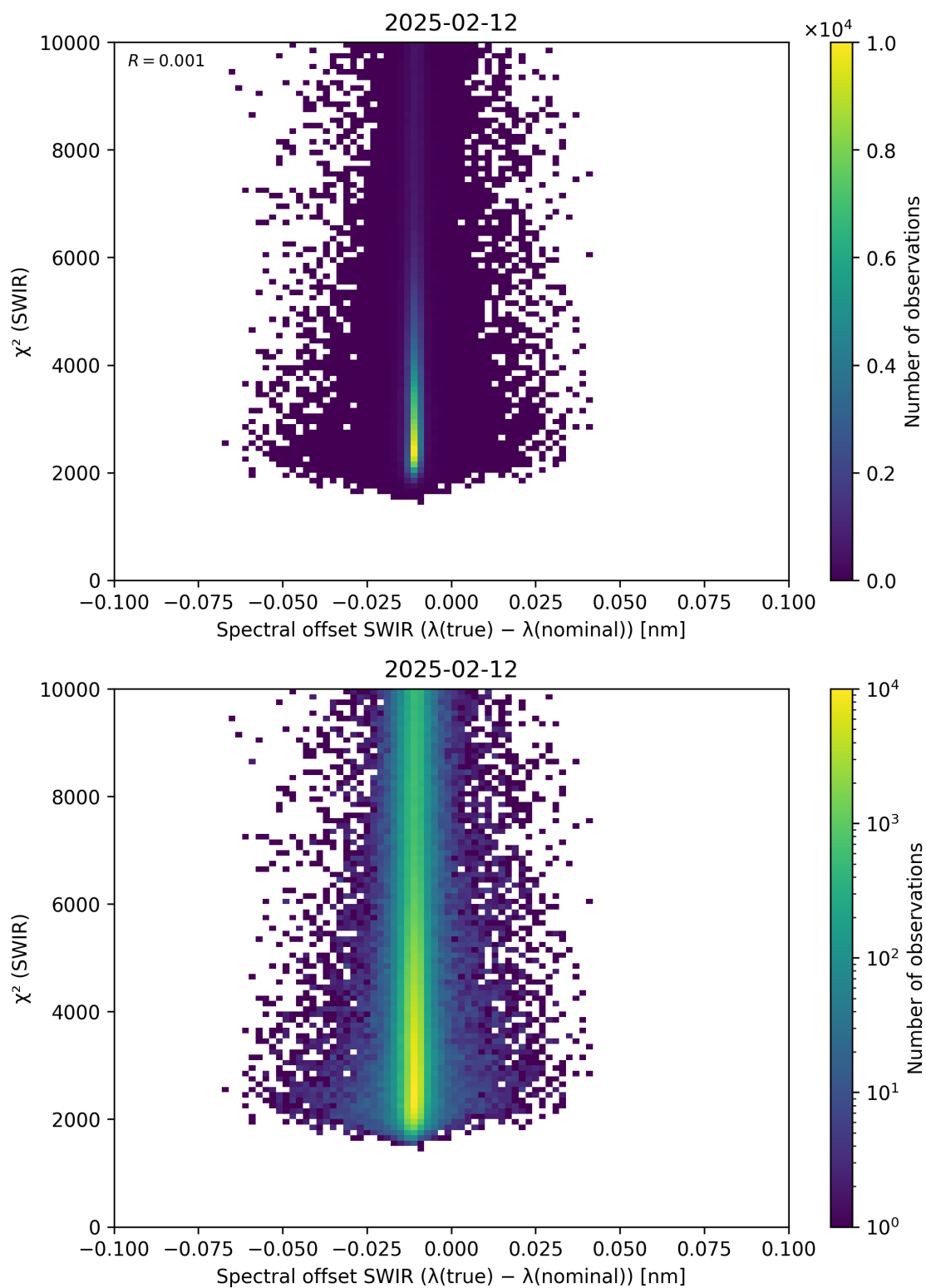
Figure 118: Scatter density plot of “Spectral offset SWIR ( \lambda_{\text{true}} - \lambda_{\text{nominal}} )” against “ \chi^2 (SWIR)” for 2025-02-11 to 2025-02-13.
