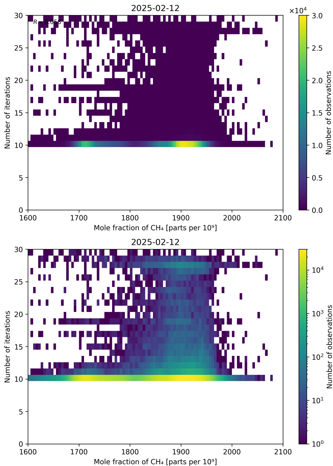
Figure 76: Scatter density plot of “Mole fraction of CH 4 ” against “Number of iterations” for 2025-02-11 to 2025-02-13.
