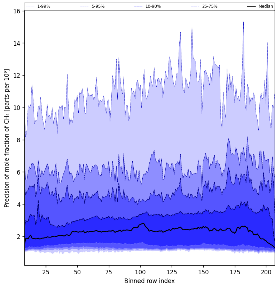
Figure 35: Along track statistics of “Precision of mole fraction of CH 4 ” for 2025-02-11 to 2025-02-13
