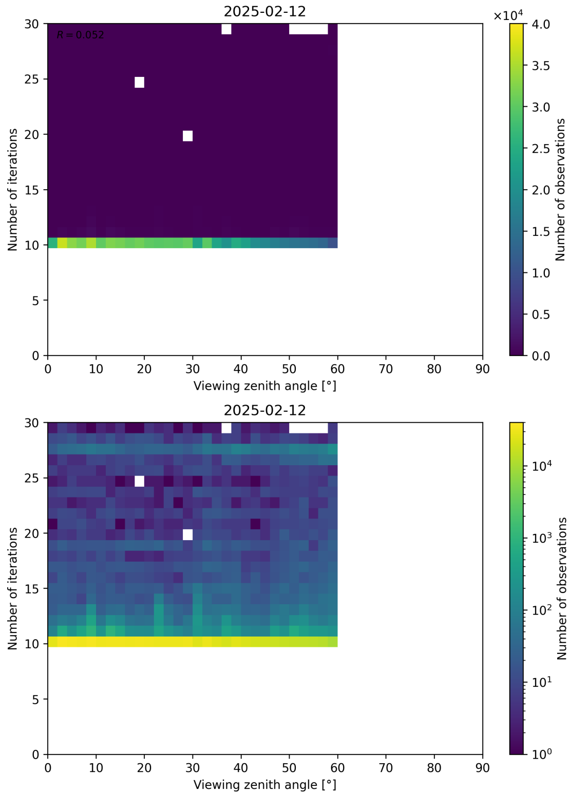
Figure 113: Scatter density plot of “Viewing zenith angle” against “Number of iterations” for 2025-02-11 to 2025-02-13.
