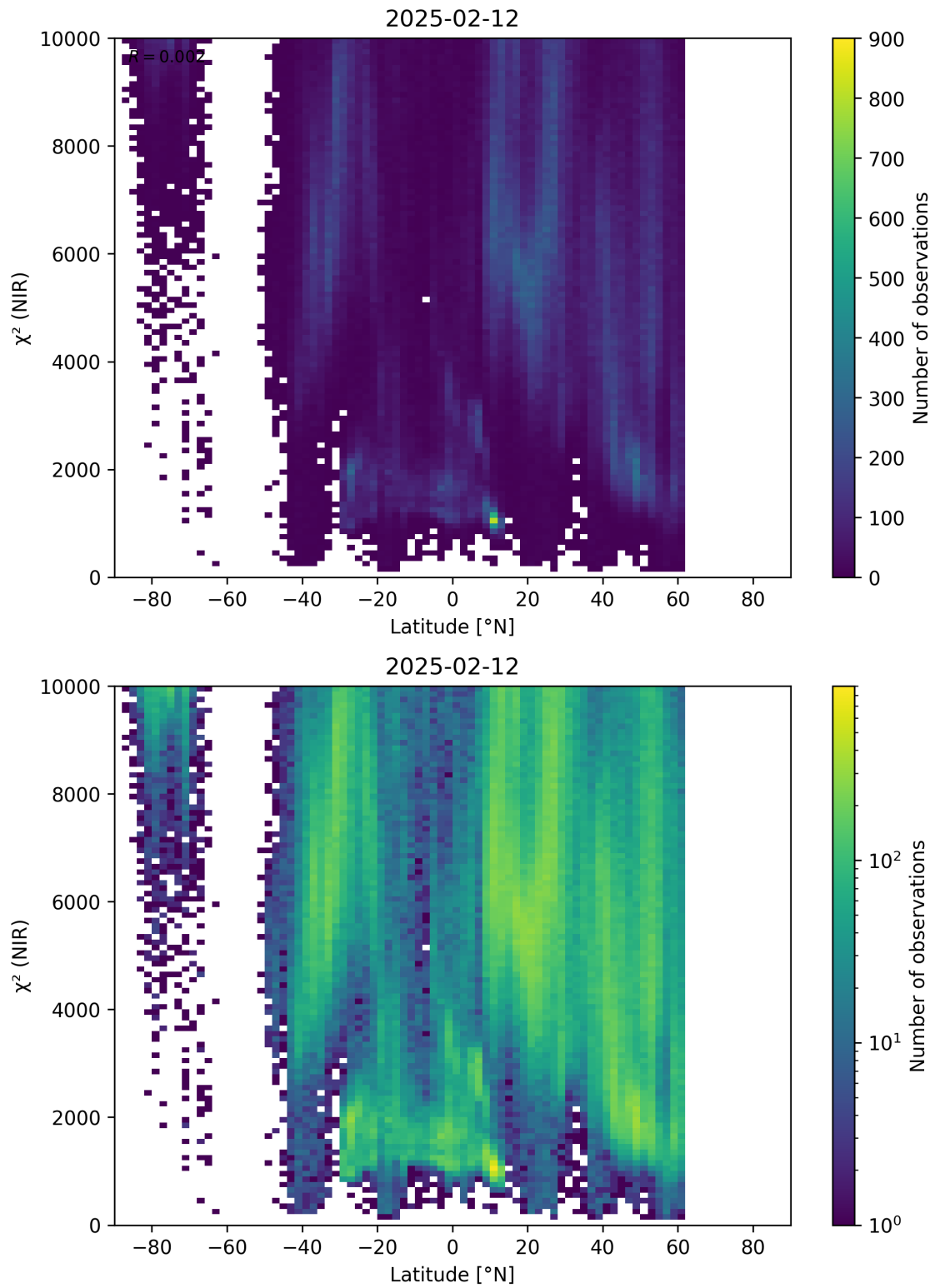
Figure 53: Scatter density plot of “Latitude” against “ \chi^2 (NIR)” for 2025-02-11 to 2025-02-13.
