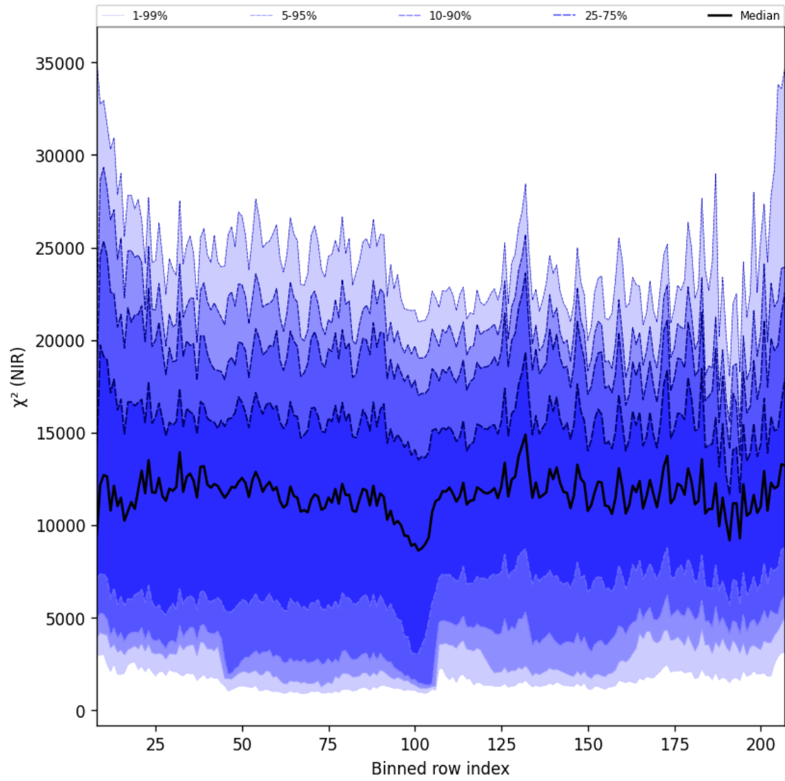
Figure 40: Along track statistics of “ \chi^2 (NIR)” for 2025-02-11 to 2025-02-13
