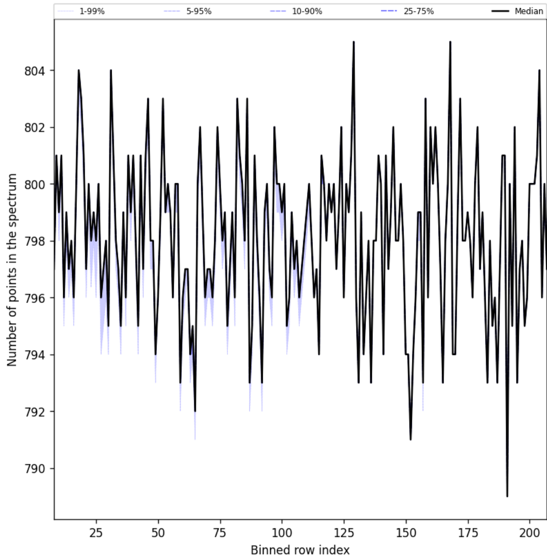
Figure 37: Along track statistics of “Number of points in the spectrum” for 2025-02-11 to 2025-02-13
