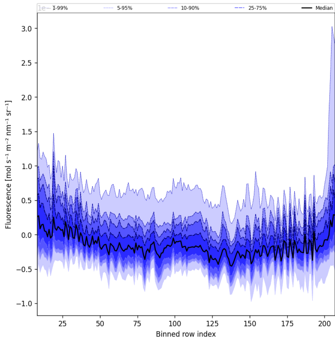
Figure 43: Along track statistics of “Fluorescence” for 2025-02-11 to 2025-02-13
