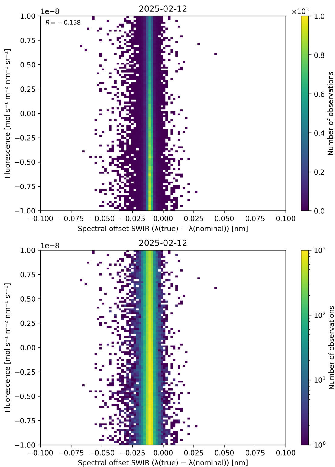
Figure 120: Scatter density plot of “Spectral offset SWIR ( \lambda_{\text{true}} - \lambda_{\text{nominal}} )” against “Fluorescence” for 2025-02-11 to 2025-02-13.
