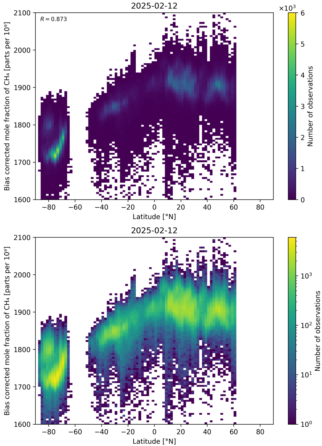
Figure 58: Scatter density plot of “Latitude” against “Bias corrected mole fraction of \text{CH}_4 ” for 2025-02-11 to 2025-02-13.
