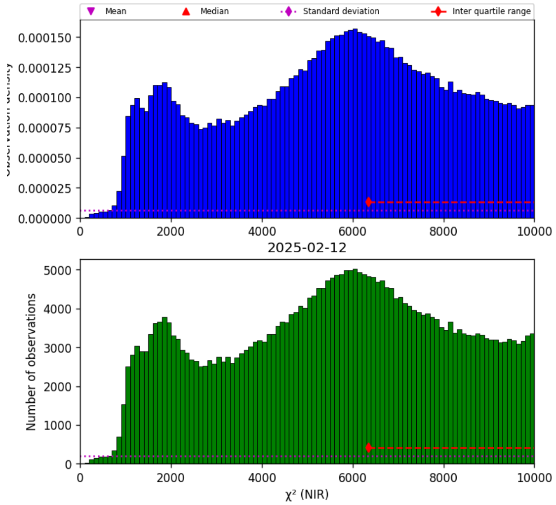
Figure 29: Histogram of “ \chi^2 (NIR)” for 2025-02-11 to 2025-02-13
