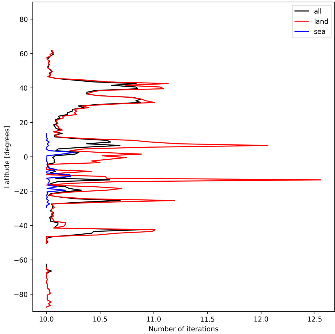
Figure 20: Zonal average of “Number of iterations” for 2025-02-11 to 2025-02-13.
