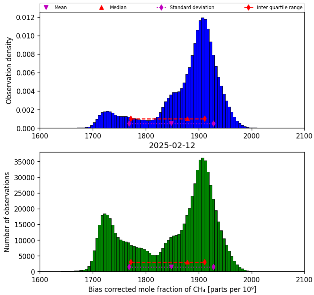
Figure 25: Histogram of “Bias corrected mole fraction of CH 4 ” for 2025-02-11 to 2025-02-13
