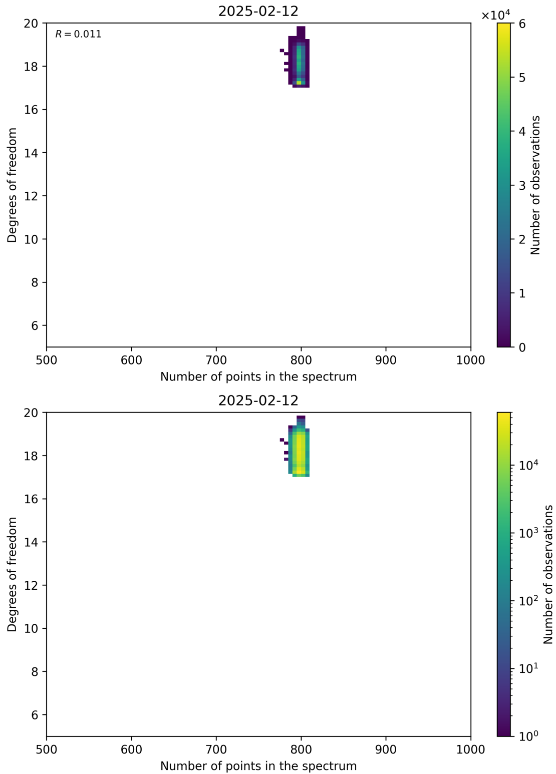
Figure 90: Scatter density plot of “Number of points in the spectrum” against “Degrees of freedom” for 2025-02-11 to 2025-02-13.
