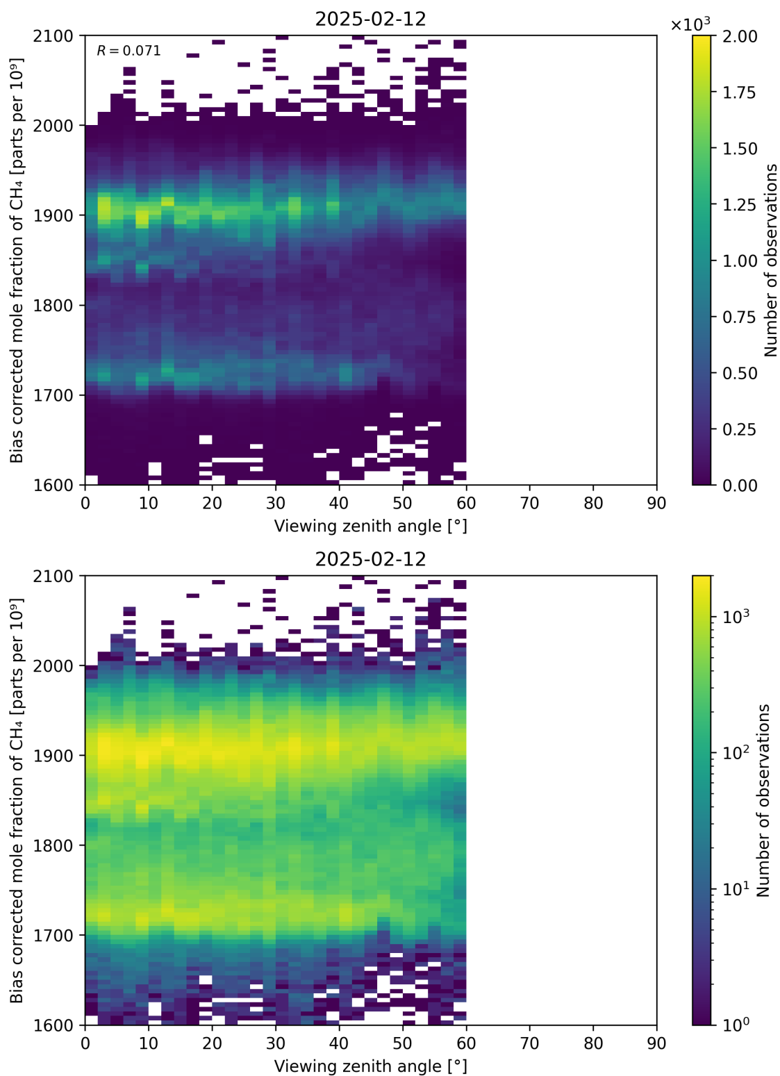
Figure 111: Scatter density plot of “Viewing zenith angle” against “Bias corrected mole fraction of CH 4 ” for 2025-02-11 to 2025-02-13.
