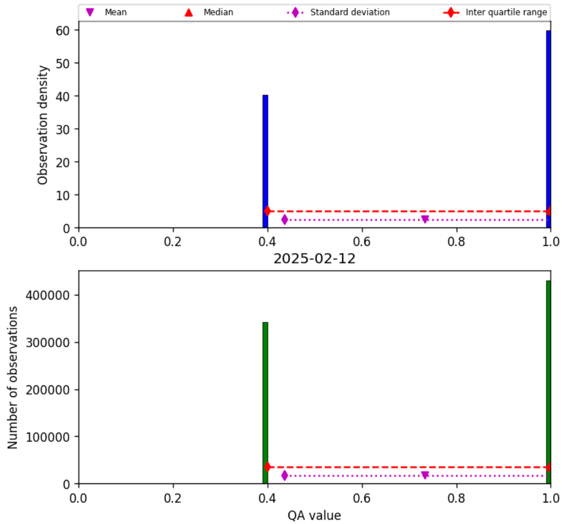
Figure 22: Histogram of “QA value” for 2025-02-11 to 2025-02-13
