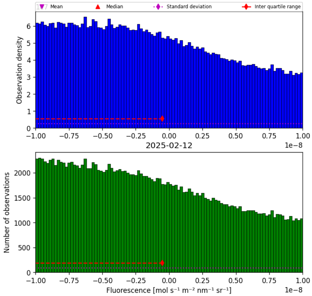
Figure 32: Histogram of “Fluorescence” for 2025-02-11 to 2025-02-13
