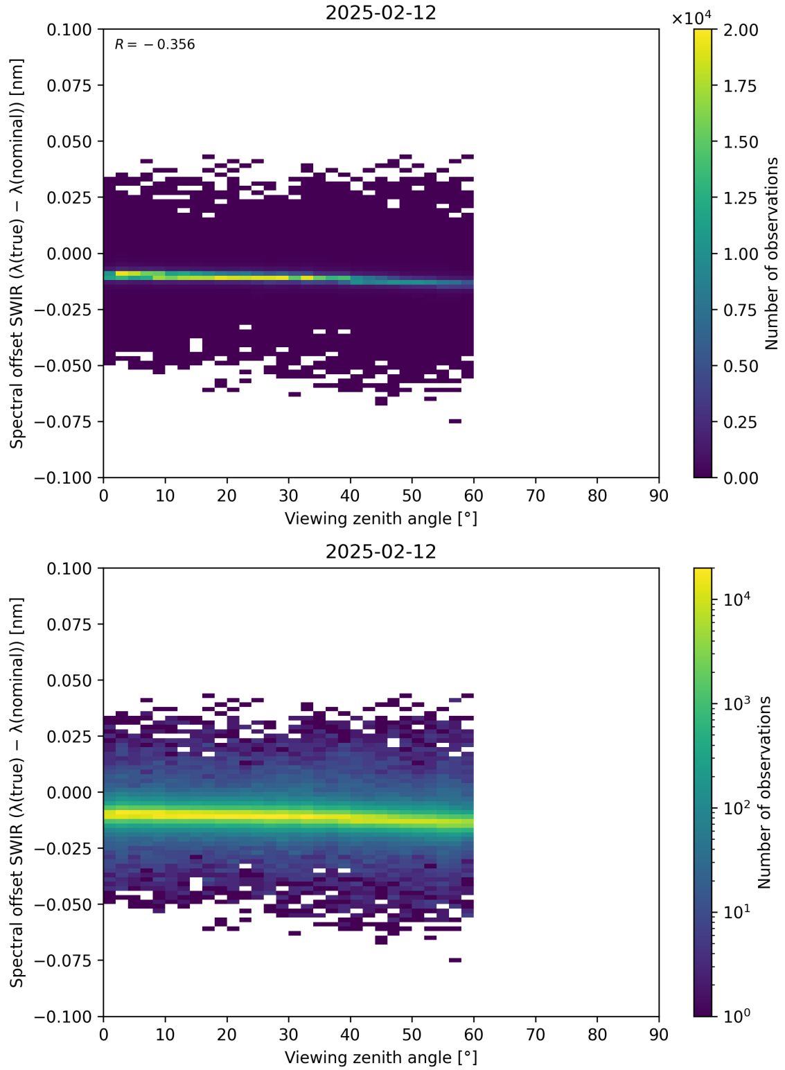
Figure 116: Scatter density plot of “Viewing zenith angle” against “Spectral offset SWIR ( \lambda_{\text{true}} - \lambda_{\text{nominal}} )” for 2025-02-11 to 2025-02-13.
