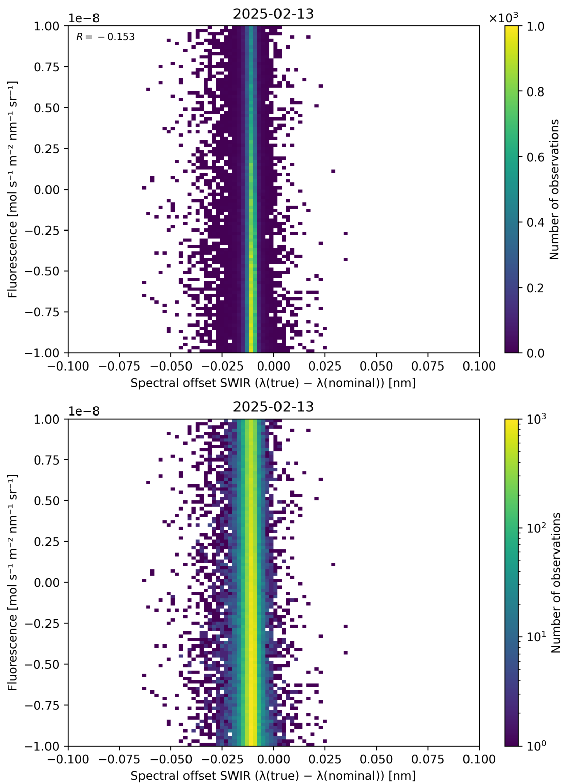
Figure 120: Scatter density plot of “Spectral offset SWIR ( \lambda_{\text{true}} - \lambda_{\text{nominal}} )” against “Fluorescence” for 2025-02-13 to 2025-02-14.
