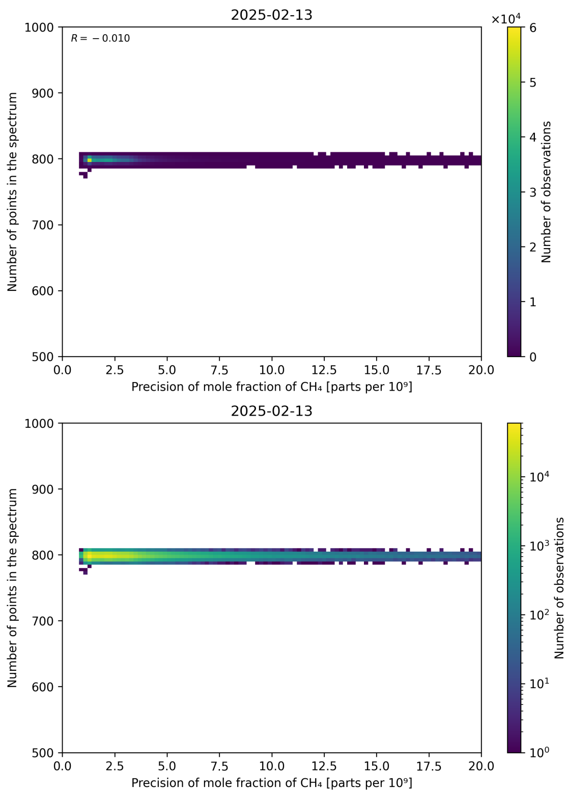
Figure 84: Scatter density plot of “Precision of mole fraction of CH 4 ” against “Number of points in the spectrum” for 2025-02-13 to 2025-02-14.
