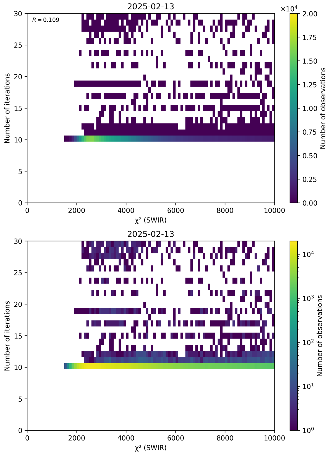
Figure 50: Scatter density plot of “ \chi^2 (SWIR)” against “Number of iterations” for 2025-02-13 to 2025-02-14.
