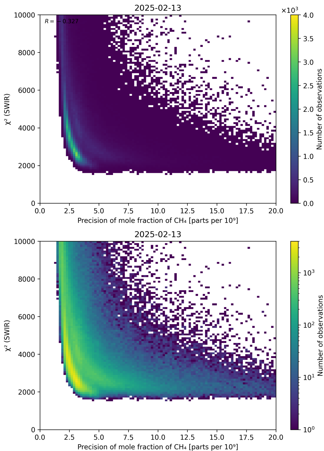
Figure 79: Scatter density plot of “Precision of mole fraction of \text{CH}_4 ” against “ \chi^2 (SWIR)” for 2025-02-13 to 2025-02-14.
