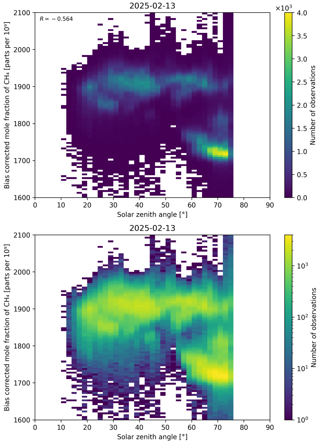
Figure 100: Scatter density plot of “Solar zenith angle” against “Bias corrected mole fraction of CH 4 ” for 2025-02-13 to 2025-02-14.
