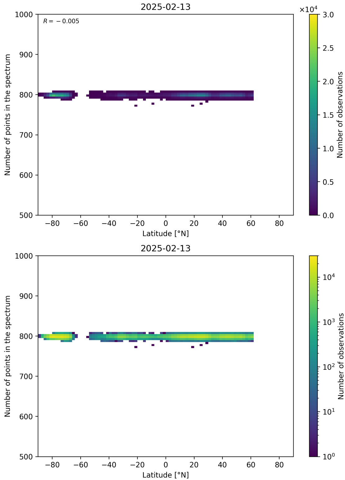
Figure 61: Scatter density plot of “Latitude” against “Number of points in the spectrum” for 2025-02-13 to 2025-02-14.
