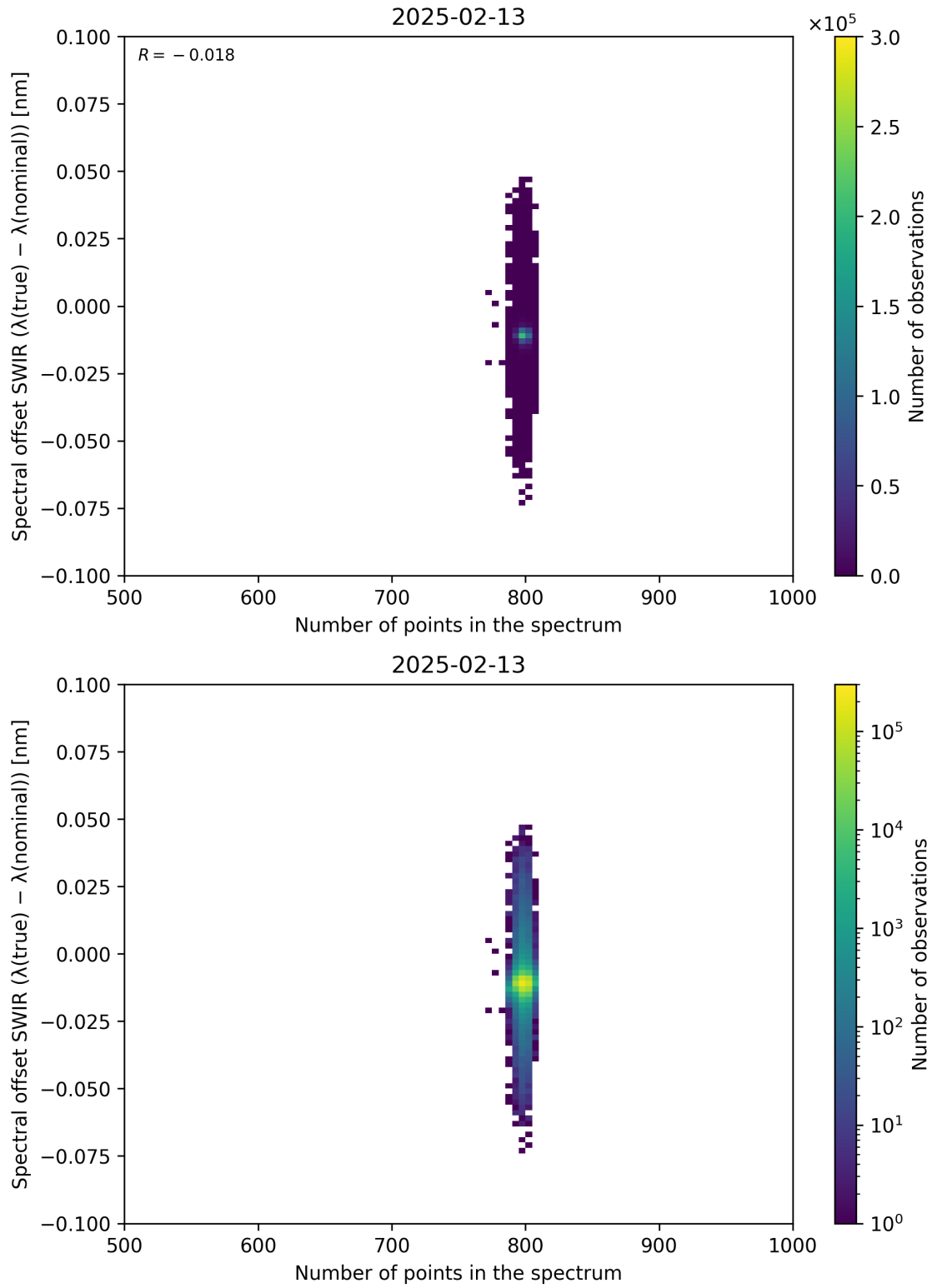
Figure 93: Scatter density plot of “Number of points in the spectrum” against “Spectral offset SWIR ( \lambda_{\text{true}} - \lambda_{\text{nominal}} )” for 2025-02-13 to 2025-02-14.
