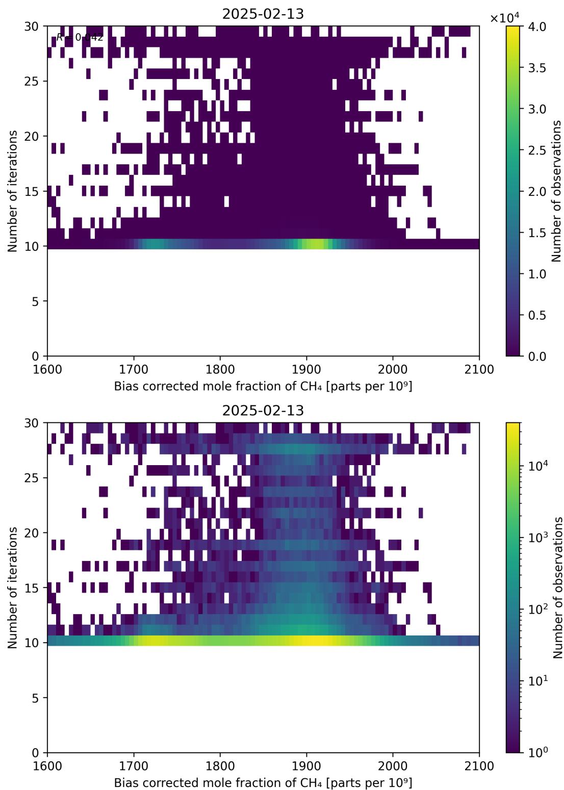
Figure 67: Scatter density plot of “Bias corrected mole fraction of CH 4 ” against “Number of iterations” for 2025-02-13 to 2025-02-14.
