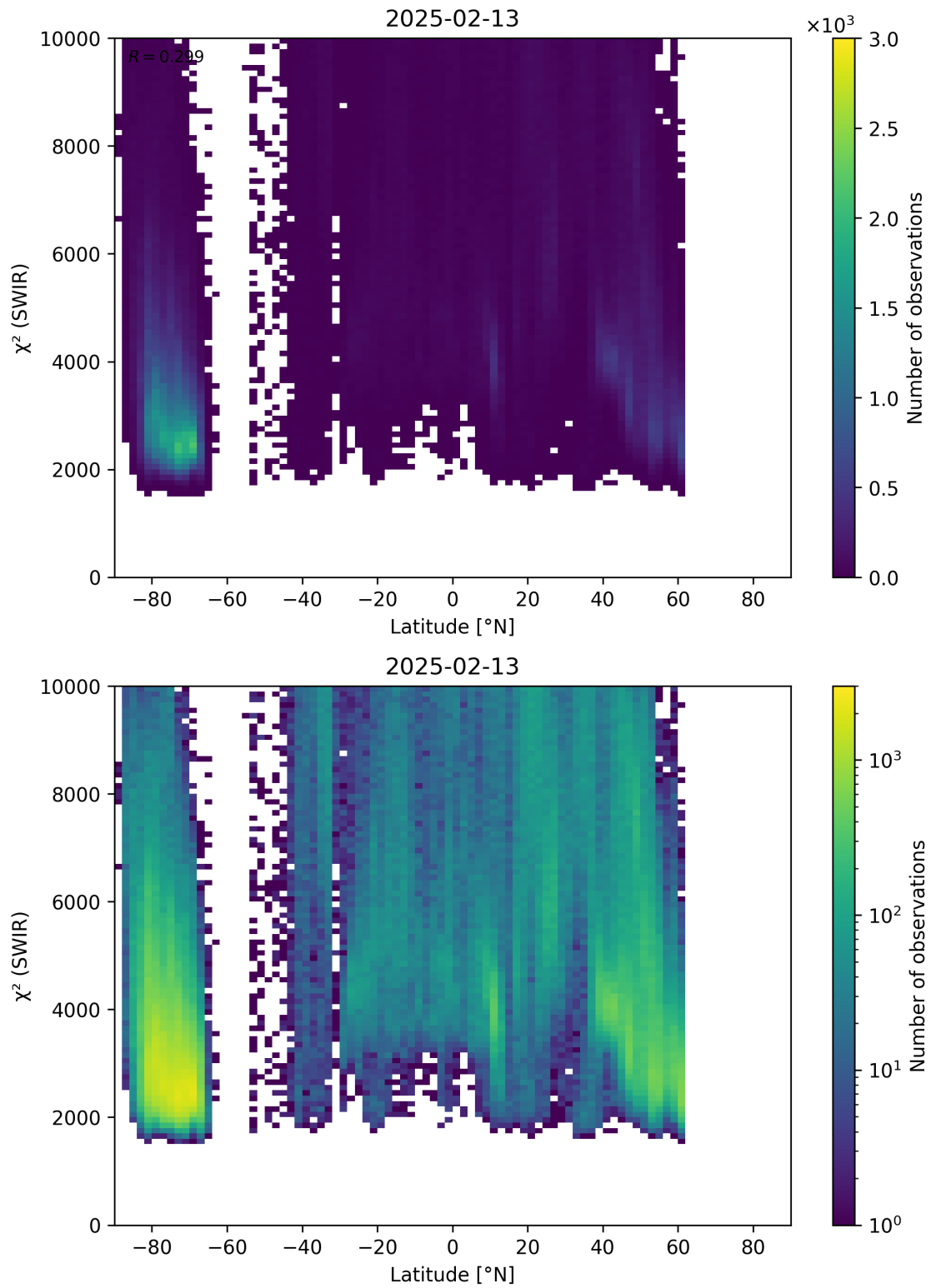
Figure 54: Scatter density plot of “Latitude” against “ \chi^2 (SWIR)” for 2025-02-13 to 2025-02-14.
