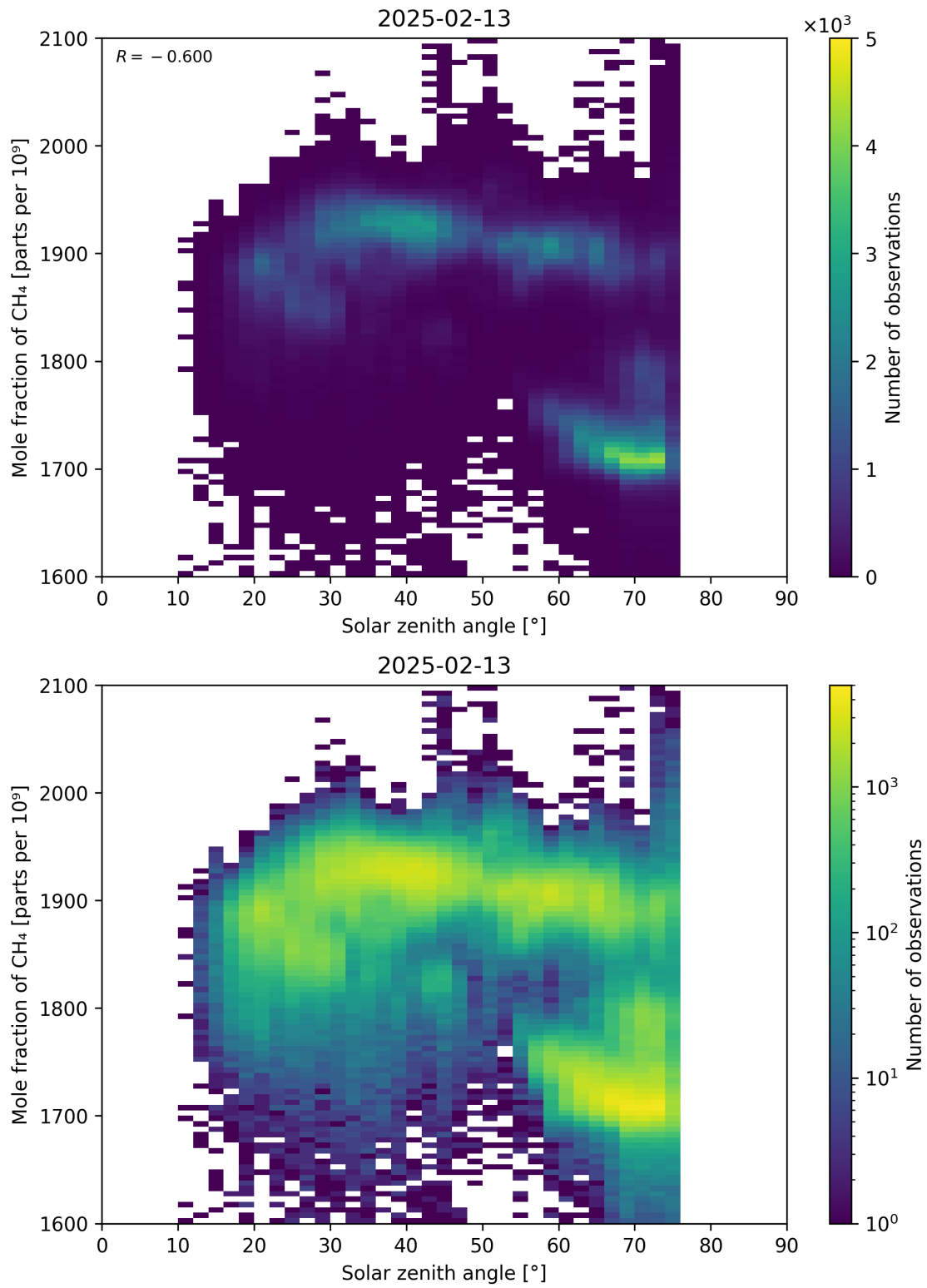
Figure 99: Scatter density plot of “Solar zenith angle” against “Mole fraction of CH 4 ” for 2025-02-13 to 2025-02-14.
