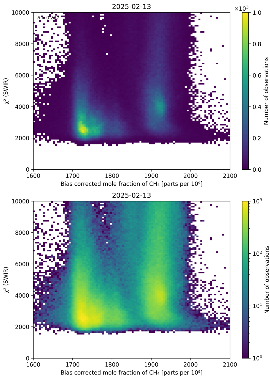
Figure 64: Scatter density plot of “Bias corrected mole fraction of \text{CH}_4 ” against “ \chi^2 (SWIR)” for 2025-02-13 to 2025-02-14.
