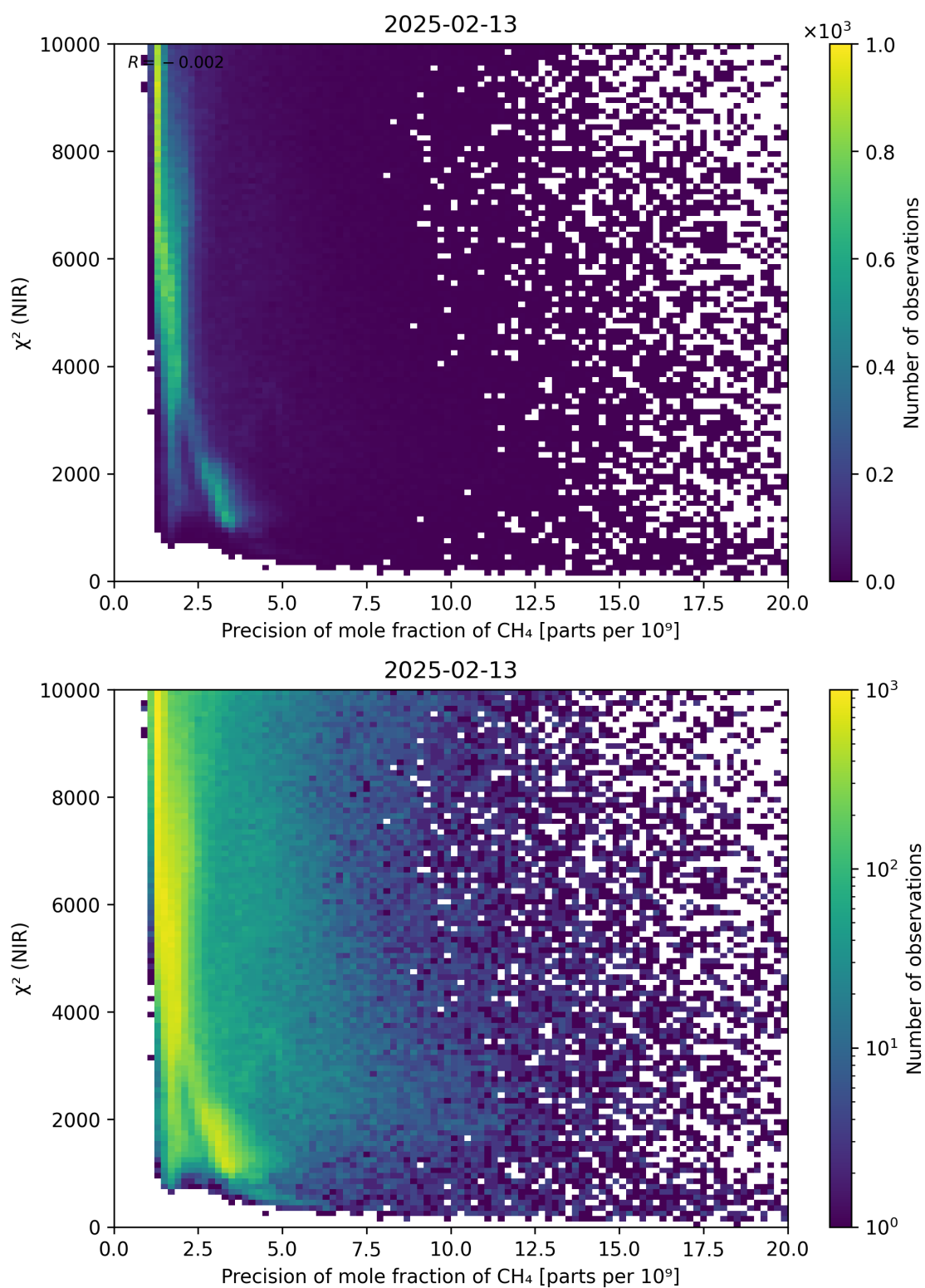
Figure 78: Scatter density plot of “Precision of mole fraction of \text{CH}_4 ” against “ \chi^2 (NIR)” for 2025-02-13 to 2025-02-14.
