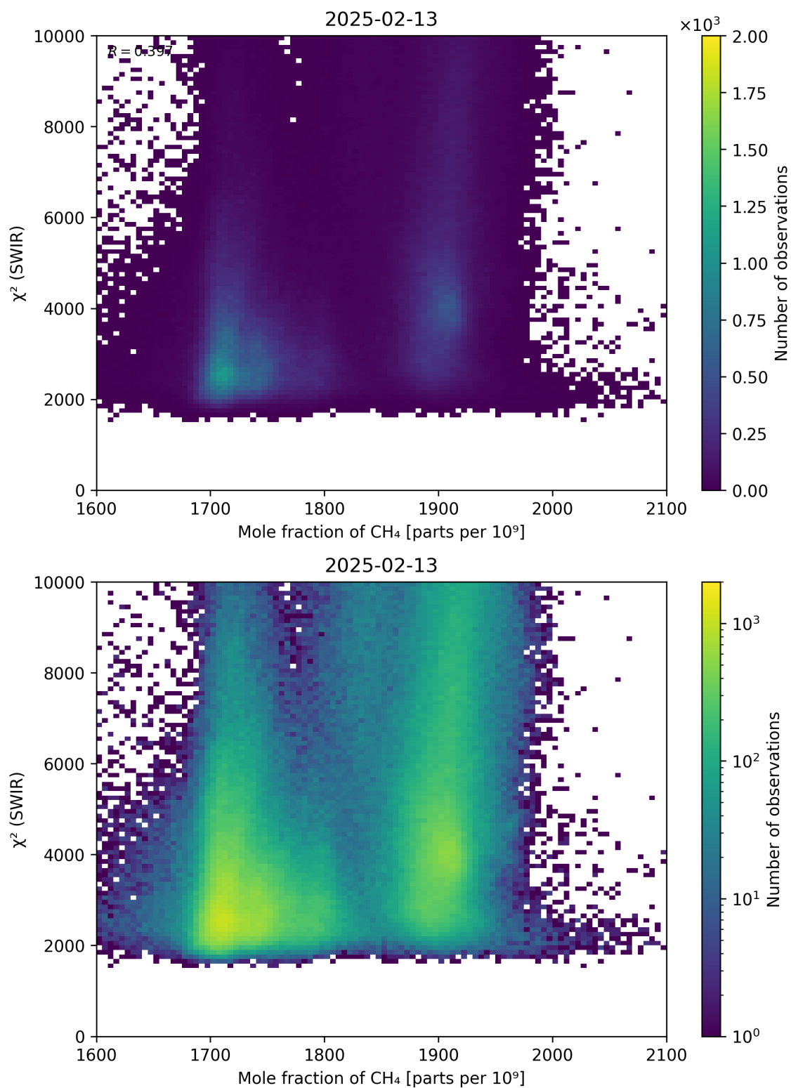
Figure 71: Scatter density plot of “Mole fraction of \text{CH}_4 ” against “ \chi^2 (SWIR)” for 2025-02-13 to 2025-02-14.
