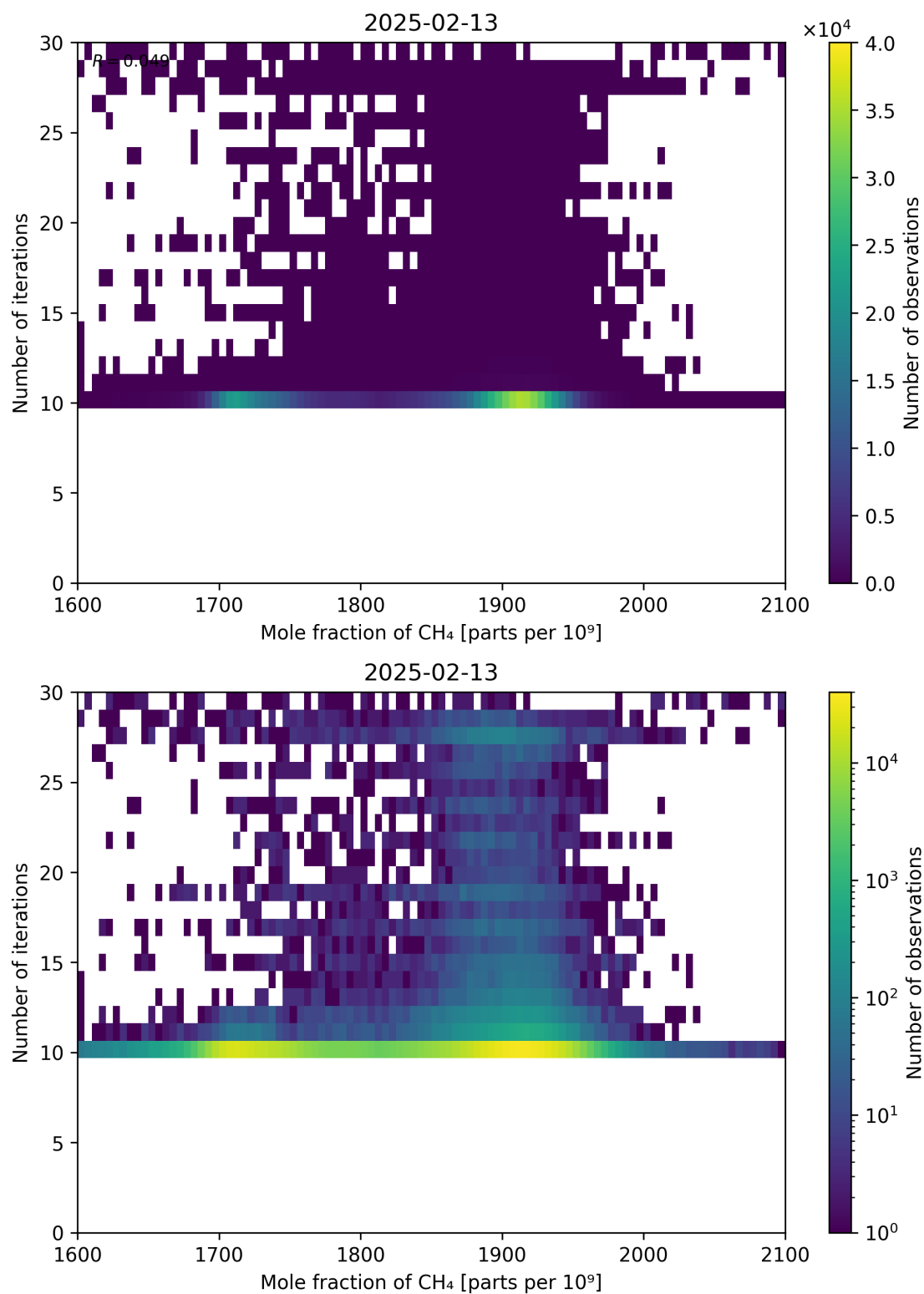
Figure 76: Scatter density plot of “Mole fraction of CH 4 ” against “Number of iterations” for 2025-02-13 to 2025-02-14.
