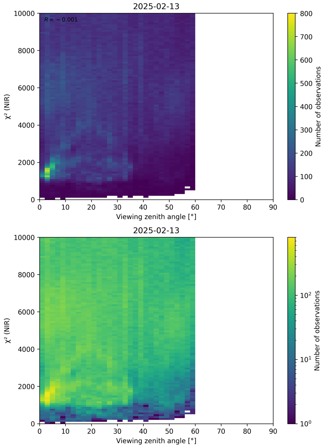
Figure 105: Scatter density plot of “Viewing zenith angle” against “ \chi^2 (NIR)” for 2025-02-13 to 2025-02-14.
