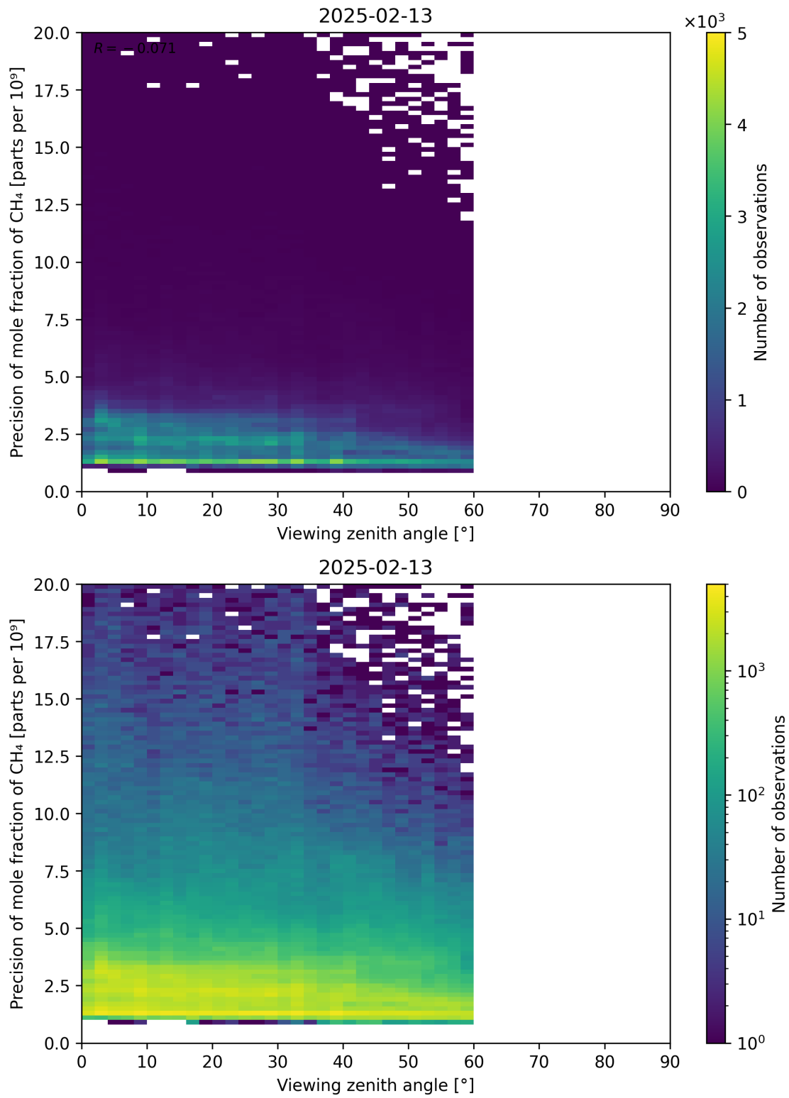
Figure 112: Scatter density plot of “Viewing zenith angle” against “Precision of mole fraction of \text{CH}_4 ” for 2025-02-13 to 2025-02-14.
