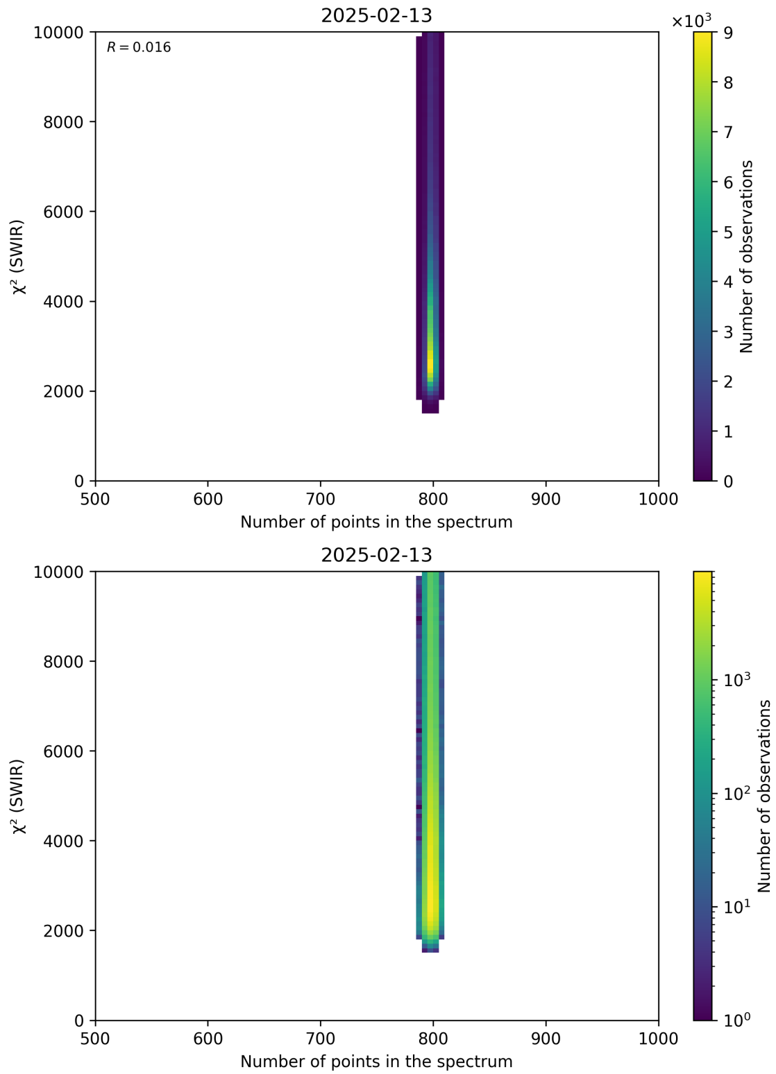
Figure 89: Scatter density plot of “Number of points in the spectrum” against “ \chi^2 (SWIR)” for 2025-02-13 to 2025-02-14.
