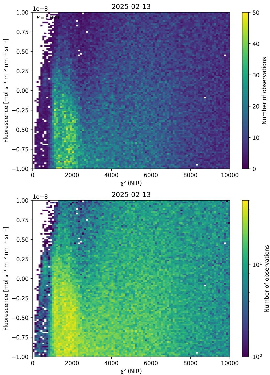
Figure 45: Scatter density plot of “ \chi^2 (NIR)” against “Fluorescence” for 2025-02-13 to 2025-02-14.
