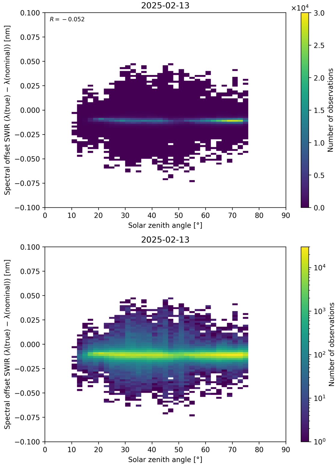
Figure 104: Scatter density plot of “Solar zenith angle” against “Spectral offset SWIR ( \lambda_{\text{true}} - \lambda_{\text{nominal}} )” for 2025-02-13 to 2025-02-14.
