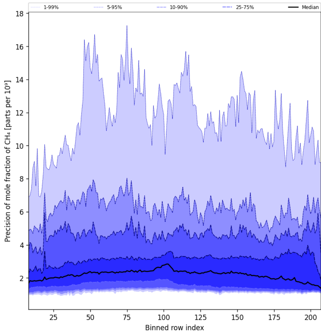
Figure 35: Along track statistics of “Precision of mole fraction of CH 4 ” for 2025-02-13 to 2025-02-14
