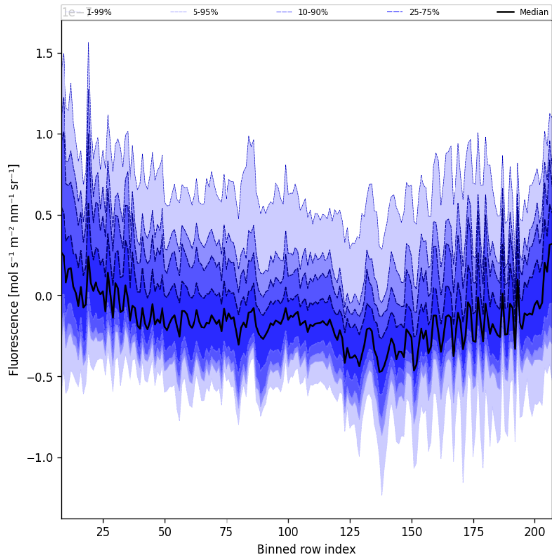
Figure 43: Along track statistics of “Fluorescence” for 2025-02-13 to 2025-02-14
