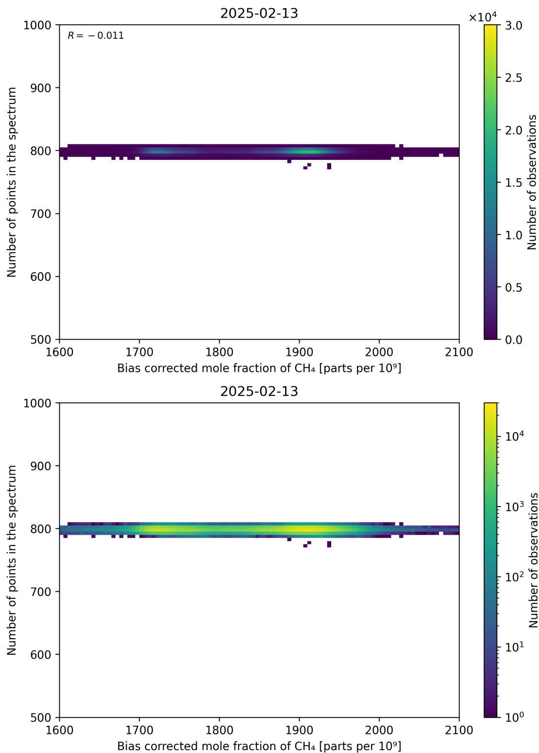
Figure 68: Scatter density plot of “Bias corrected mole fraction of CH 4 ” against “Number of points in the spectrum” for 2025-02-13 to 2025-02-14.
