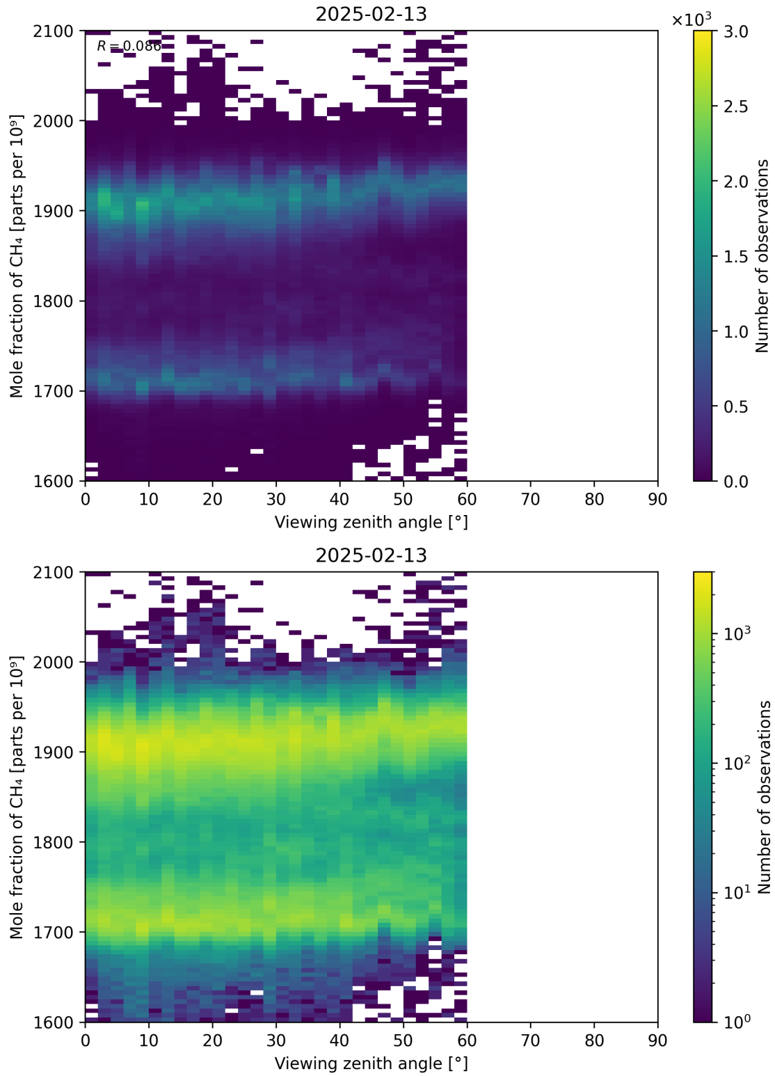
Figure 110: Scatter density plot of “Viewing zenith angle” against “Mole fraction of CH 4 ” for 2025-02-13 to 2025-02-14.
