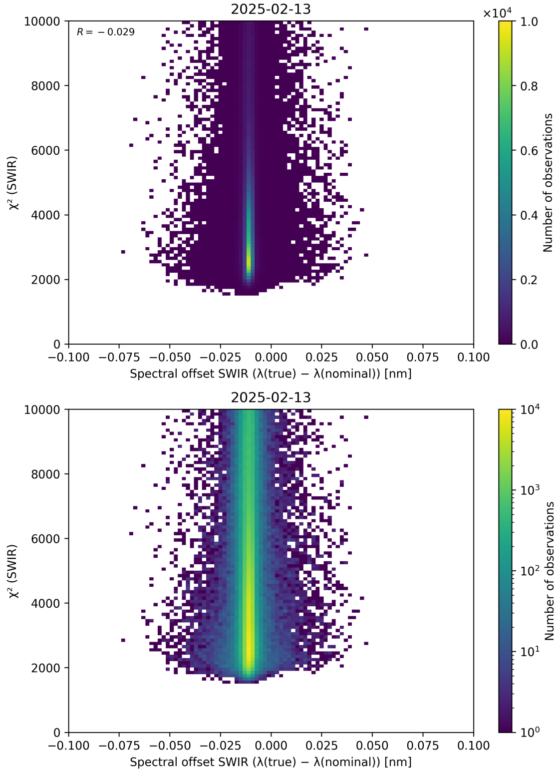
Figure 118: Scatter density plot of “Spectral offset SWIR ( \lambda_{\text{true}} - \lambda_{\text{nominal}} )” against “ \chi^2 (SWIR)” for 2025-02-13 to 2025-02-14.
