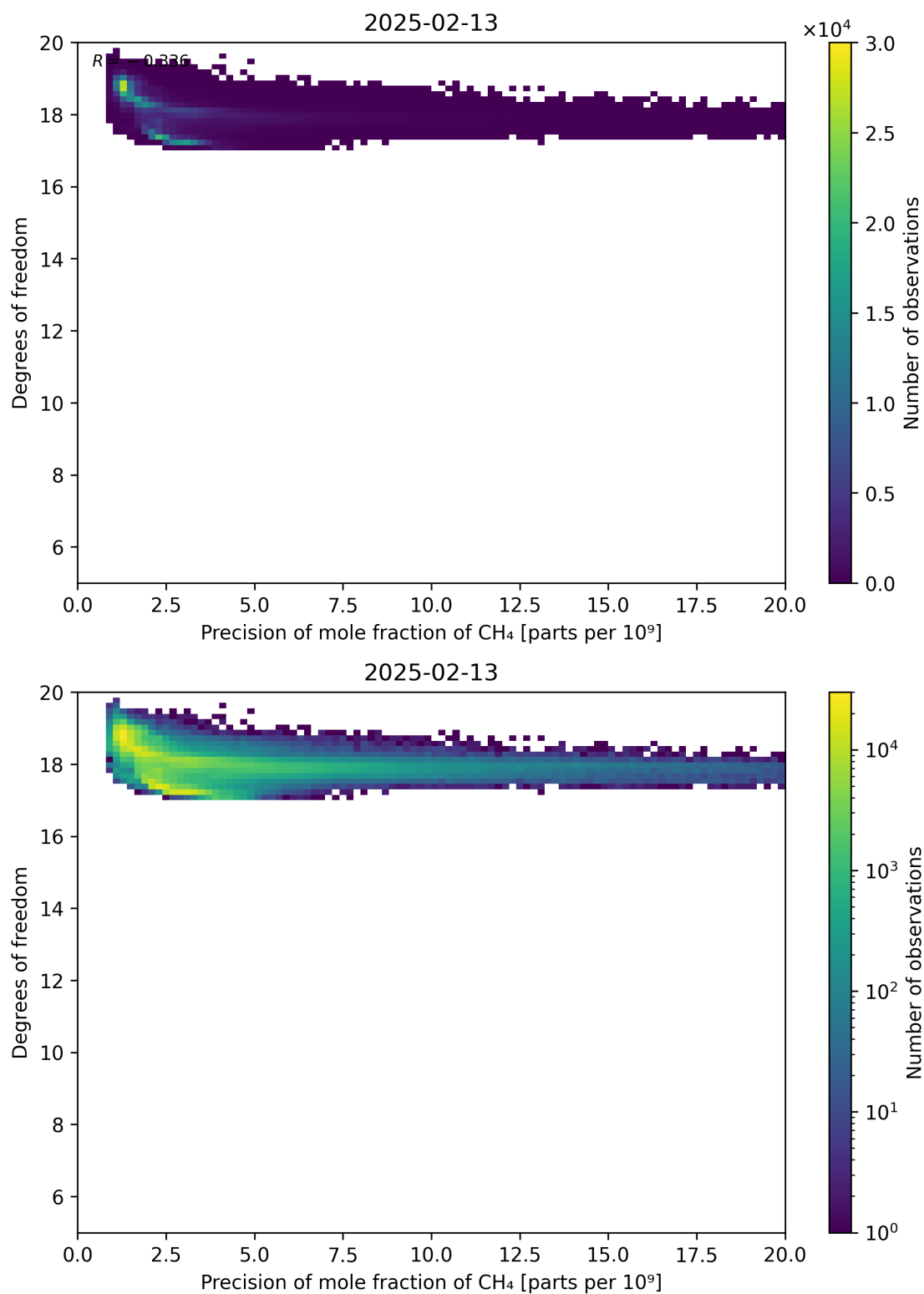
Figure 80: Scatter density plot of “Precision of mole fraction of CH 4 ” against “Degrees of freedom” for 2025-02-13 to 2025-02-14.
