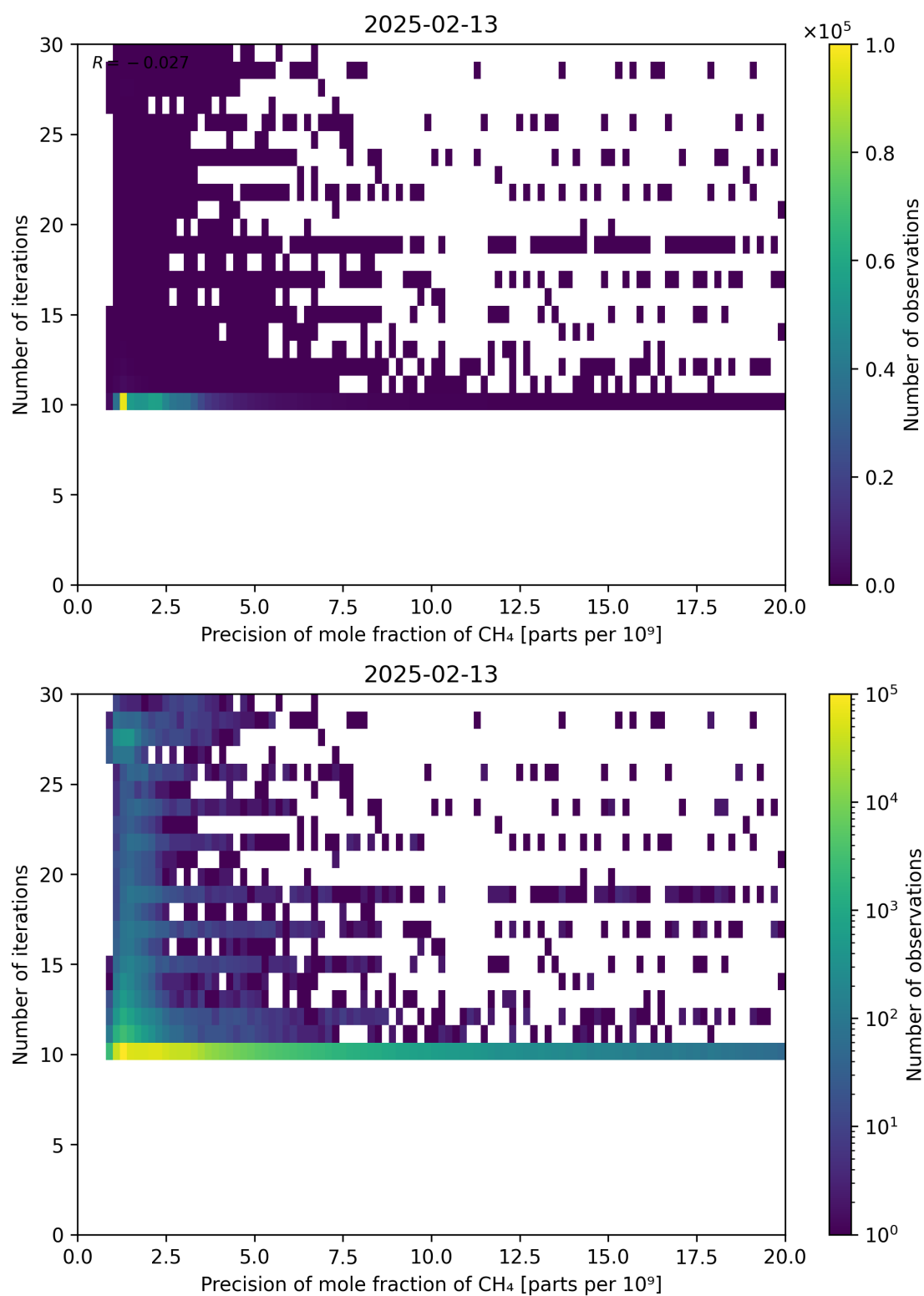
Figure 83: Scatter density plot of “Precision of mole fraction of CH 4 ” against “Number of iterations” for 2025-02-13 to 2025-02-14.
