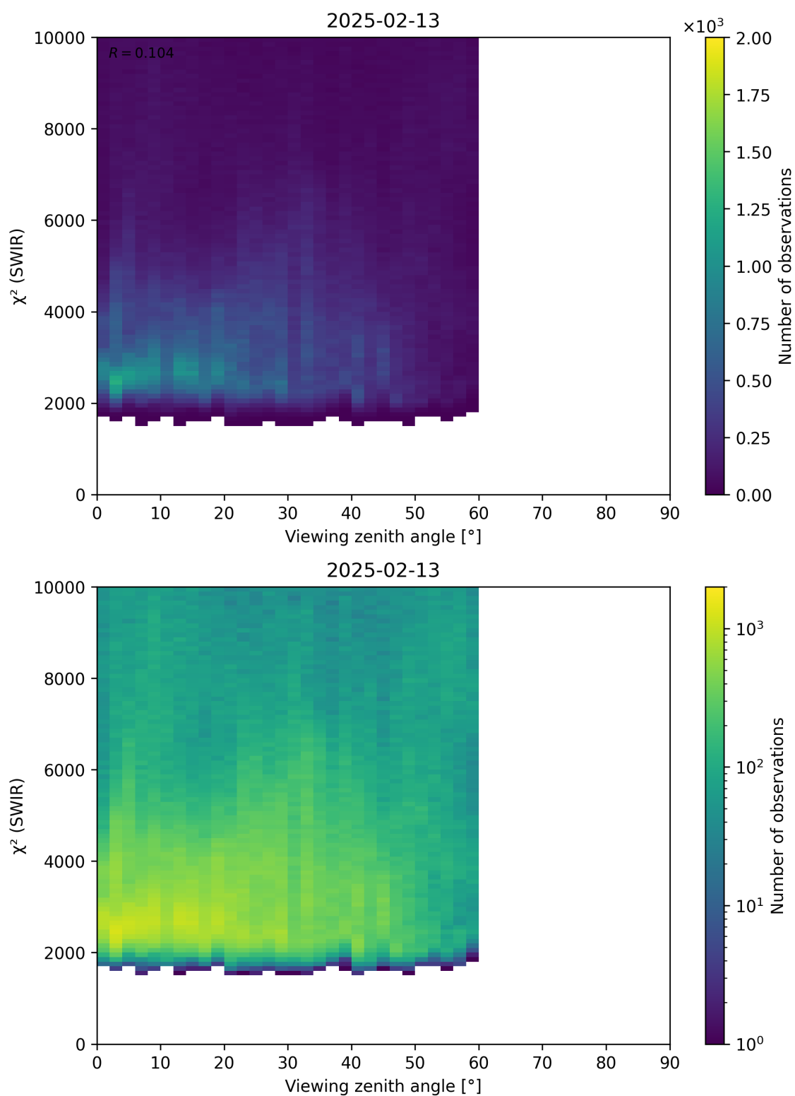
Figure 106: Scatter density plot of “Viewing zenith angle” against “ \chi^2 (SWIR)” for 2025-02-13 to 2025-02-14.
