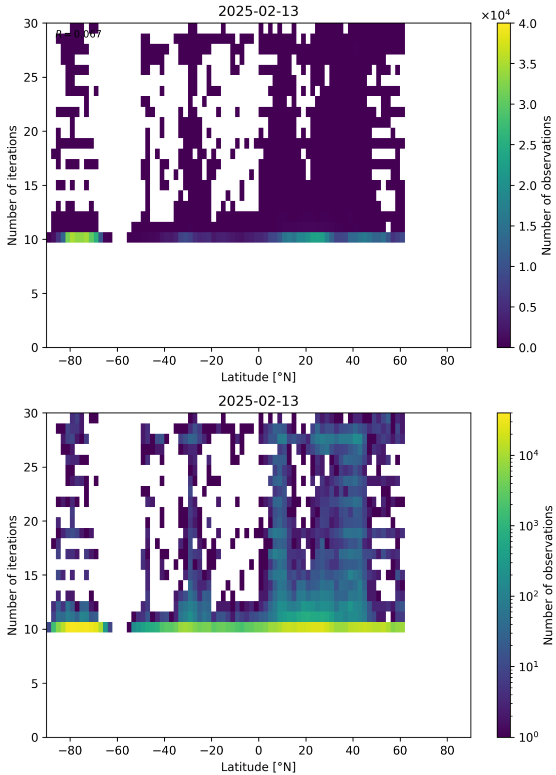
Figure 60: Scatter density plot of “Latitude” against “Number of iterations” for 2025-02-13 to 2025-02-14.
