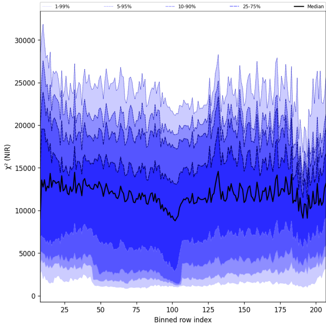
Figure 40: Along track statistics of " \chi^2 (NIR)" for 2025-02-13 to 2025-02-14
