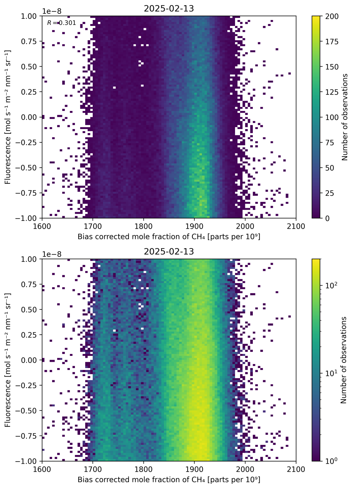
Figure 66: Scatter density plot of “Bias corrected mole fraction of \text{CH}_4 ” against “Fluorescence” for 2025-02-13 to 2025-02-14.
