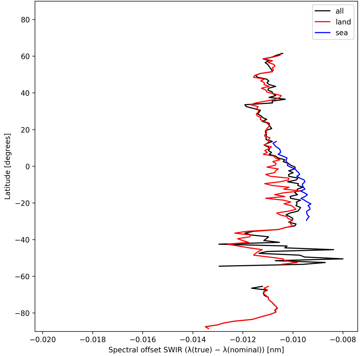
Figure 16: Zonal average of “Spectral offset SWIR ( \lambda_{\text{true}} - \lambda_{\text{nominal}} )” for 2025-02-13 to 2025-02-14.
