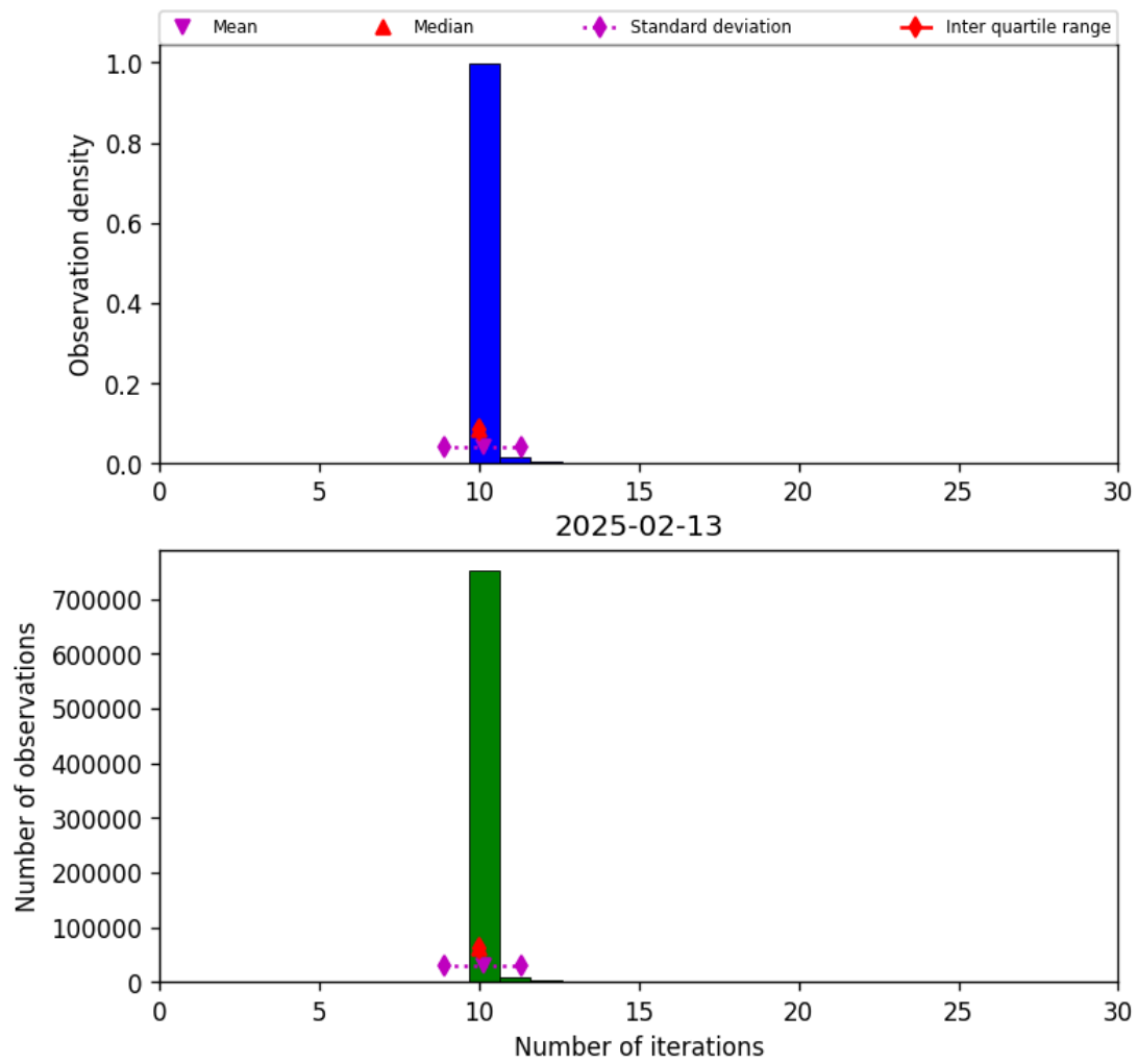
Figure 31: Histogram of “Number of iterations” for 2025-02-13 to 2025-02-14
