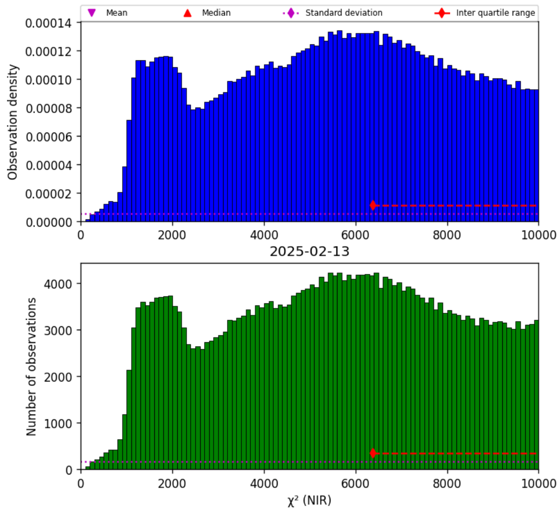
Figure 29: Histogram of “ \chi^2 (NIR)” for 2025-02-13 to 2025-02-14
