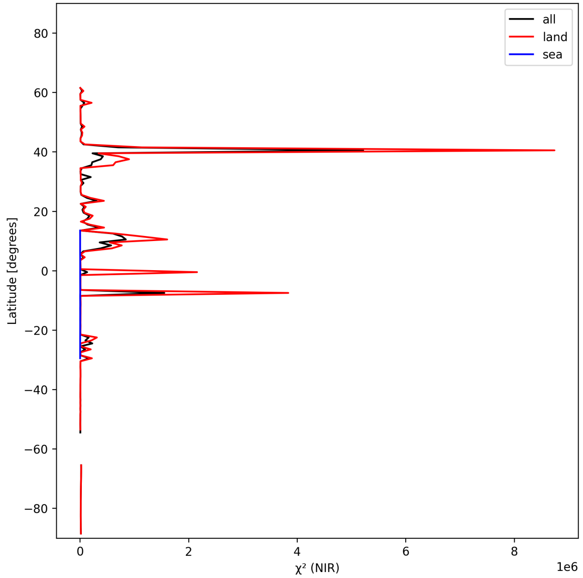
Figure 18: Zonal average of “ \chi^2 (NIR)” for 2025-02-13 to 2025-02-14.
