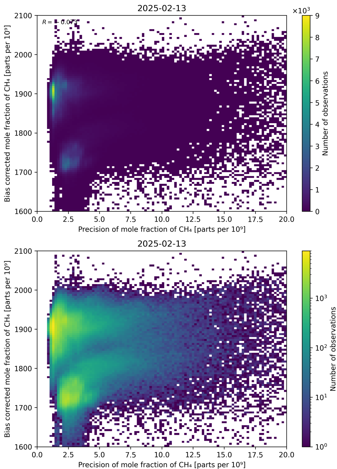
Figure 82: Scatter density plot of “Precision of mole fraction of CH 4 ” against “Bias corrected mole fraction of CH 4 ” for 2025-02-13 to 2025-02-14.
