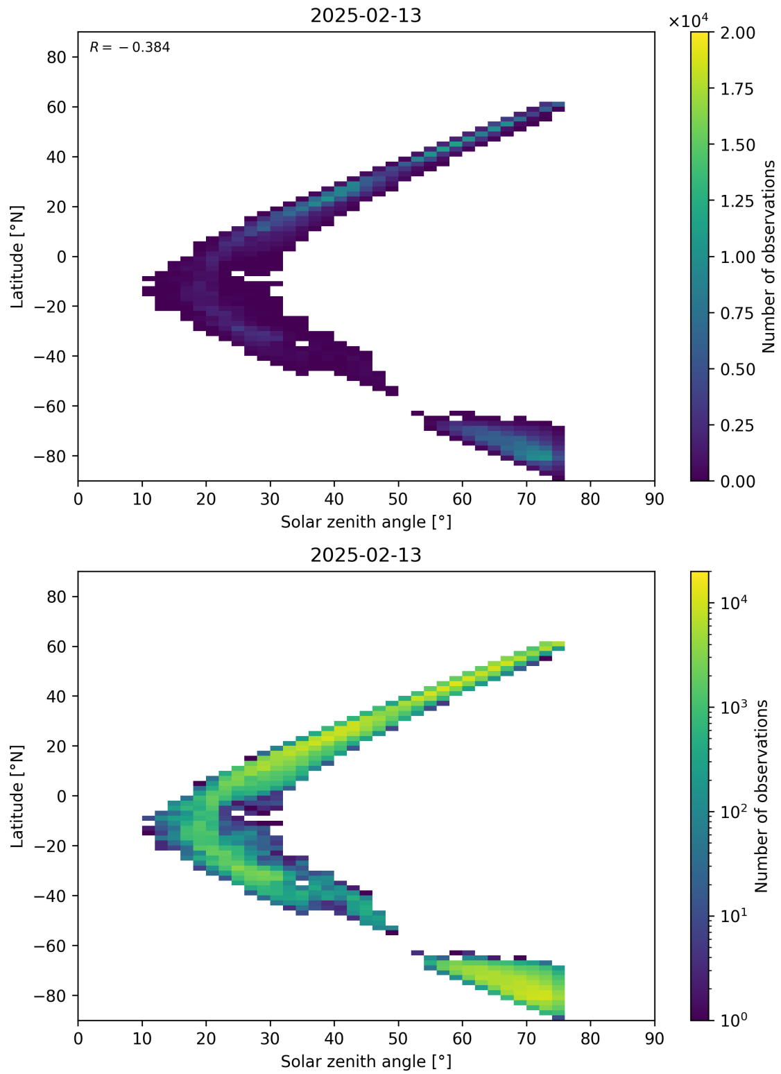
Figure 98: Scatter density plot of “Solar zenith angle” against “Latitude” for 2025-02-13 to 2025-02-14.
