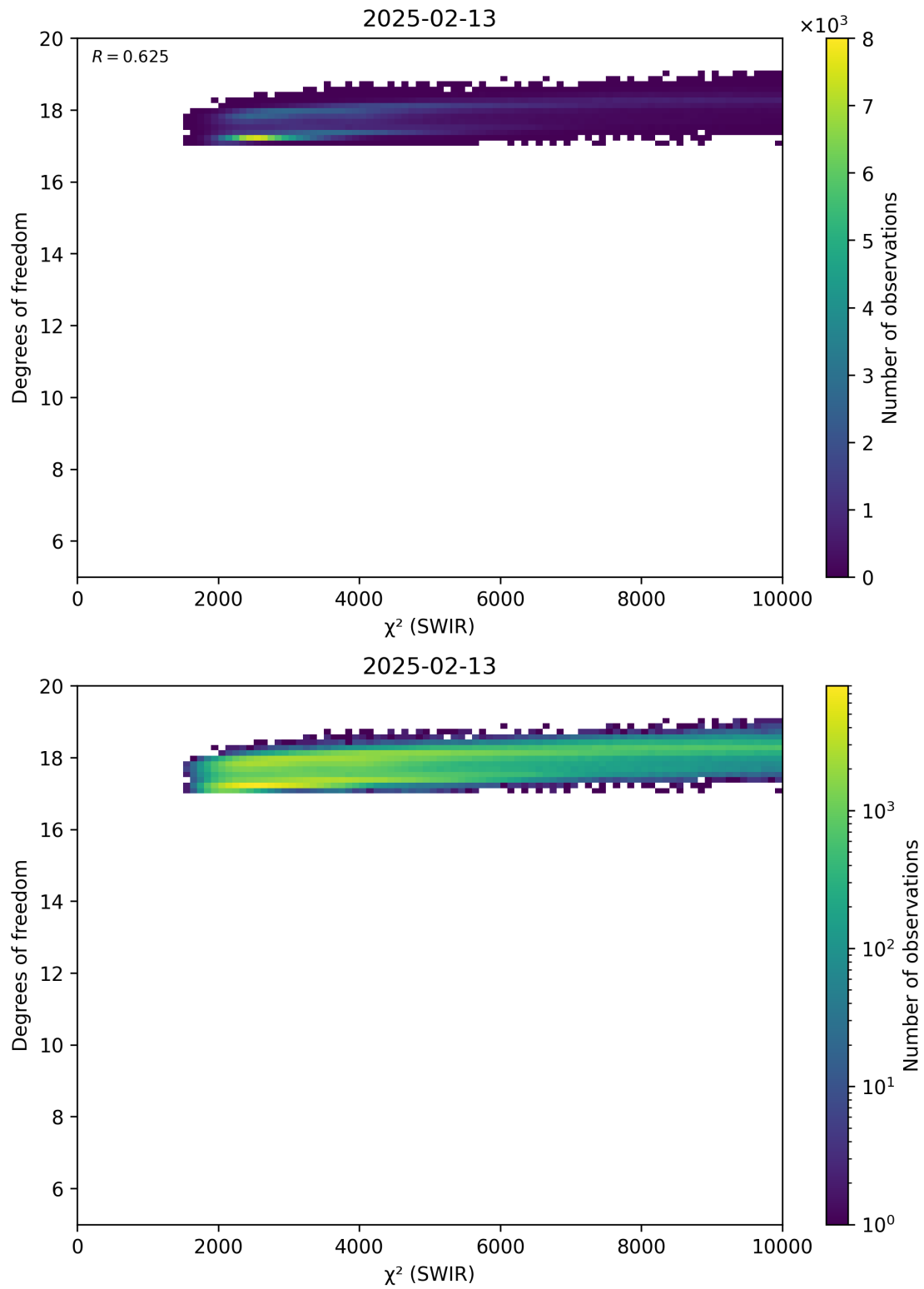
Figure 48: Scatter density plot of “ \chi^2 (SWIR)” against “Degrees of freedom” for 2025-02-13 to 2025-02-14.
