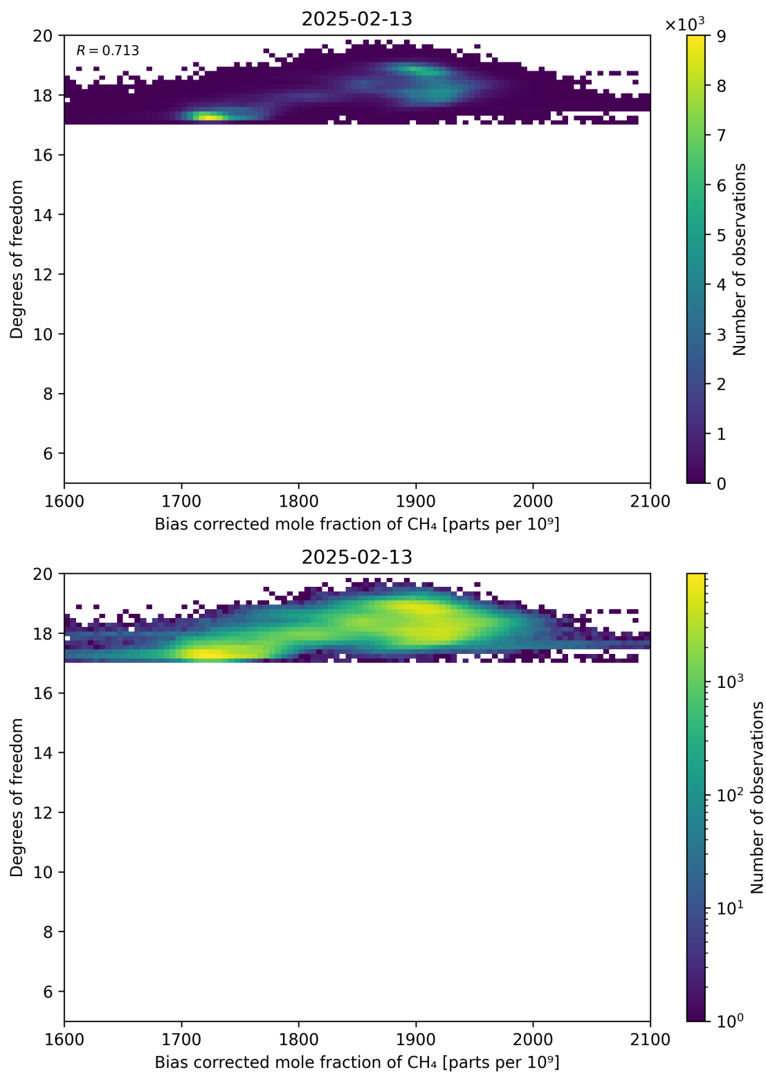
Figure 65: Scatter density plot of “Bias corrected mole fraction of CH 4 ” against “Degrees of freedom” for 2025-02-13 to 2025-02-14.
