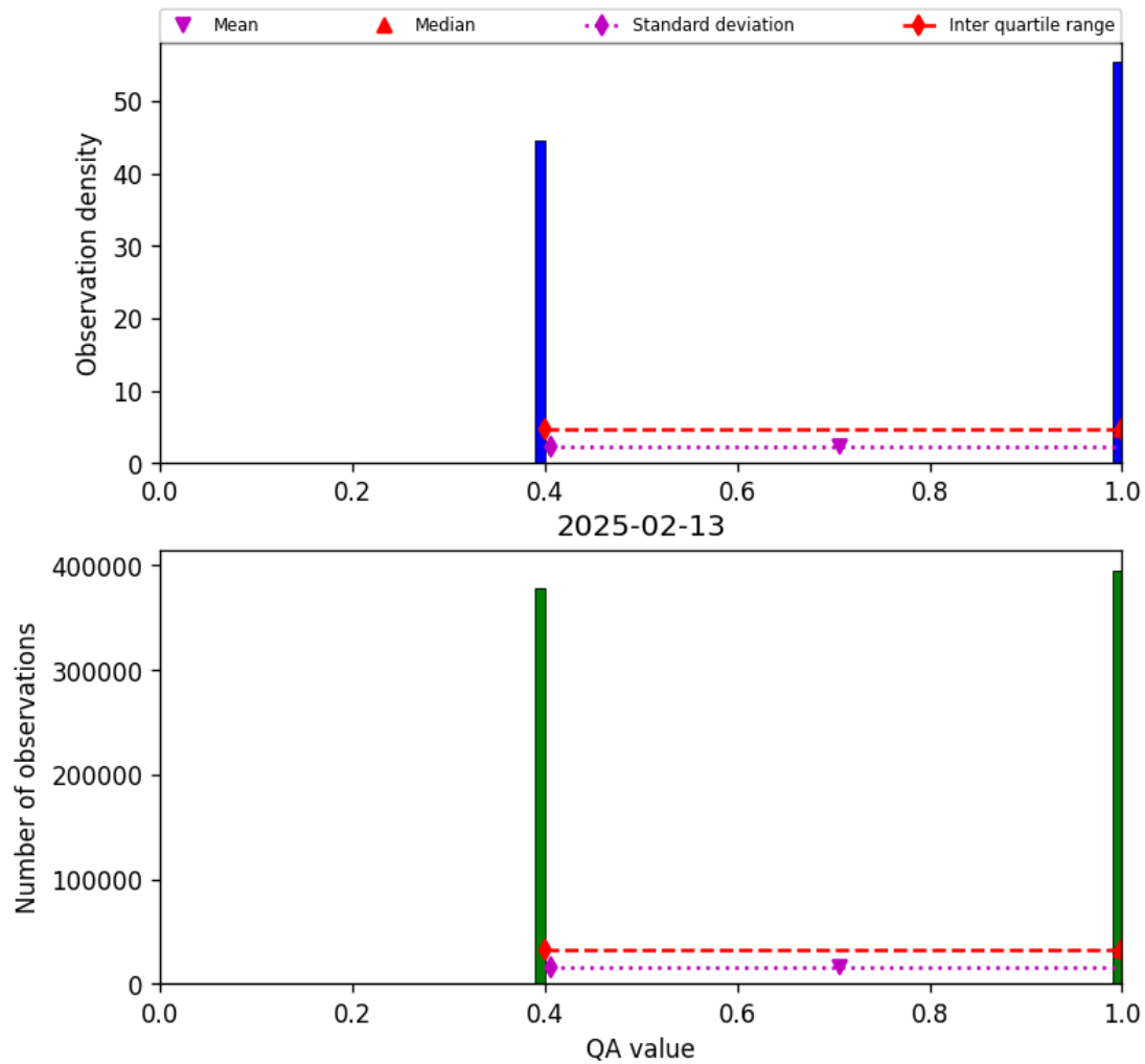
Figure 22: Histogram of “QA value” for 2025-02-13 to 2025-02-14
