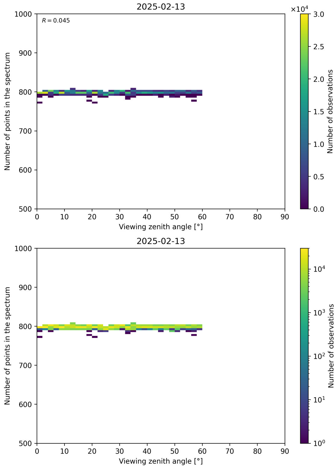
Figure 114: Scatter density plot of “Viewing zenith angle” against “Number of points in the spectrum” for 2025-02-13 to 2025-02-14.
