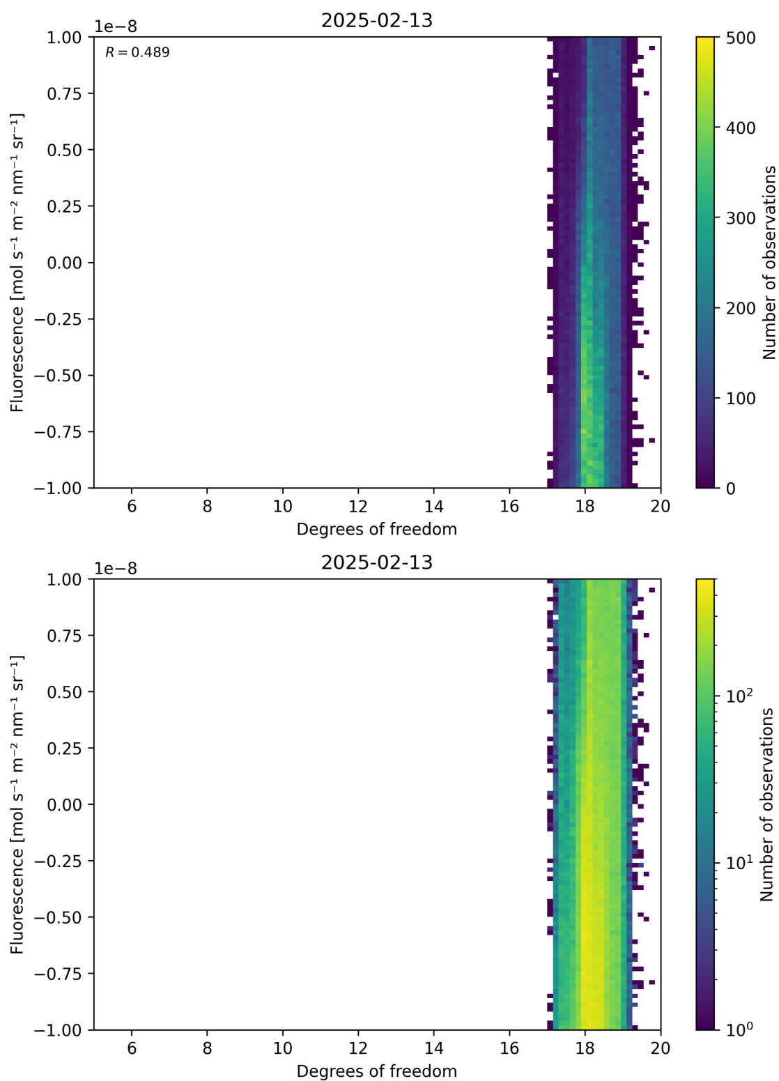
Figure 51: Scatter density plot of “Degrees of freedom” against “Fluorescence” for 2025-02-13 to 2025-02-14.
