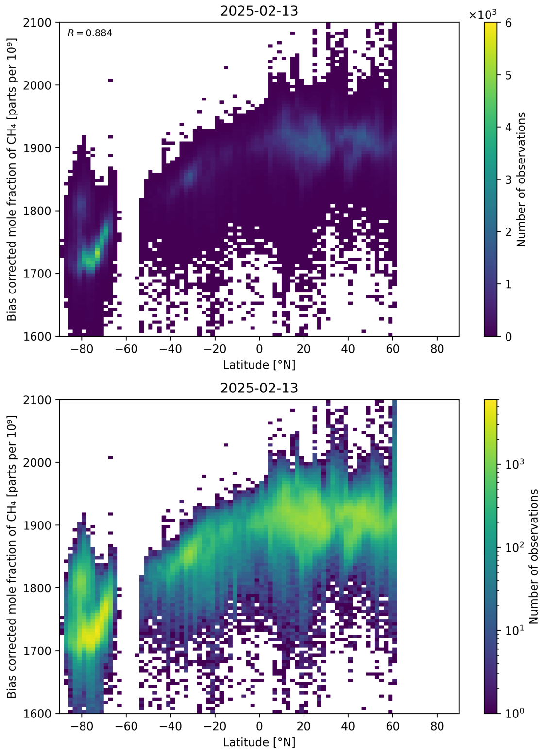
Figure 58: Scatter density plot of “Latitude” against “Bias corrected mole fraction of CH 4 ” for 2025-02-13 to 2025-02-14.
