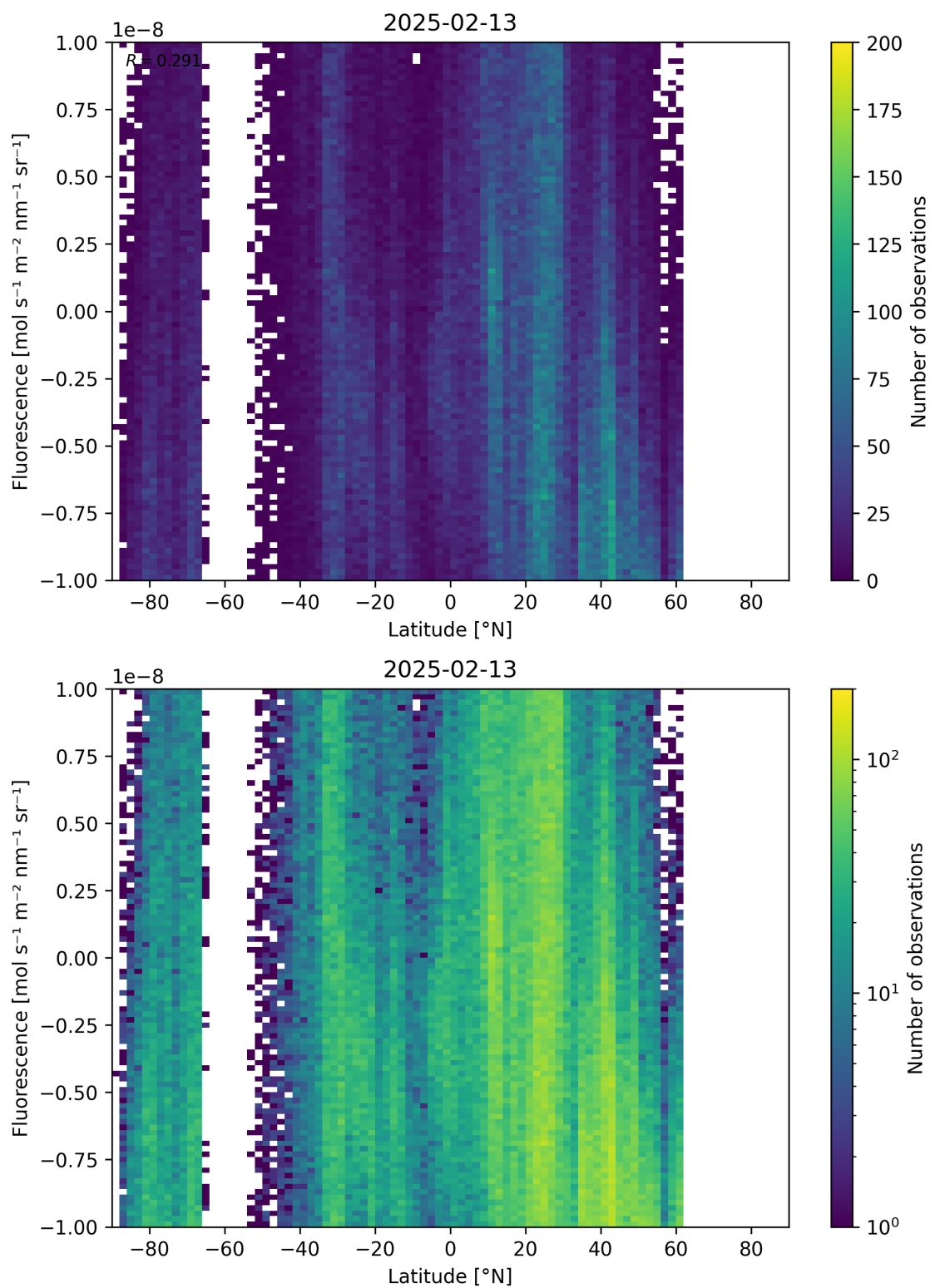
Figure 56: Scatter density plot of “Latitude” against “Fluorescence” for 2025-02-13 to 2025-02-14.
