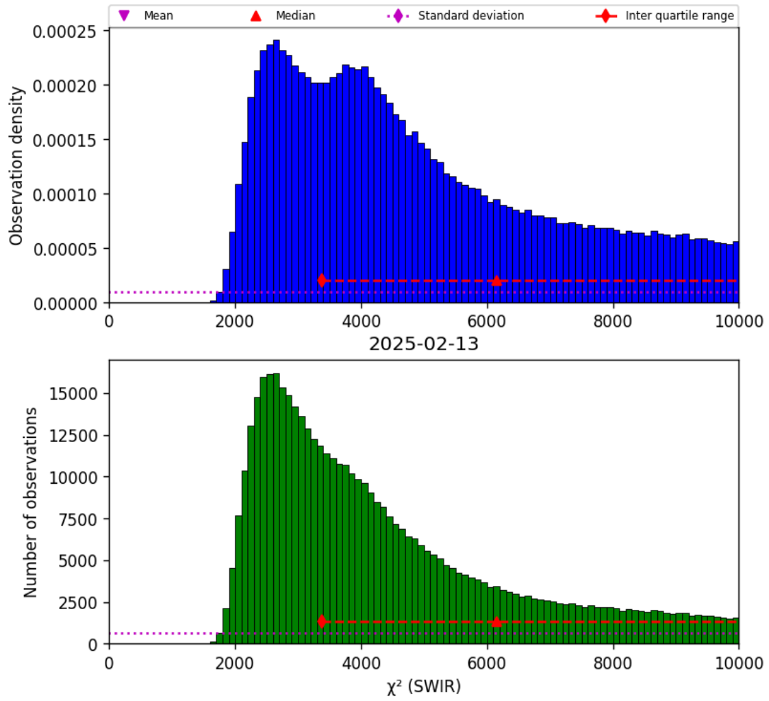
Figure 28: Histogram of “ \chi^2 (SWIR)” for 2025-02-13 to 2025-02-14
