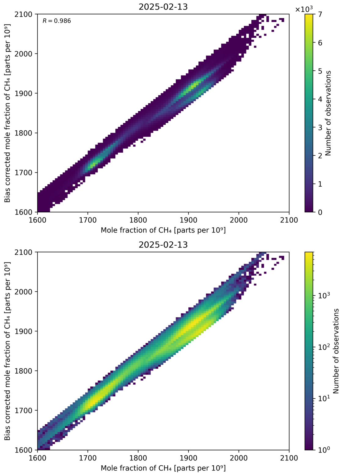
Figure 74: Scatter density plot of “Mole fraction of CH 4 ” against “Bias corrected mole fraction of CH 4 ” for 2025-02-13 to 2025-02-14.
