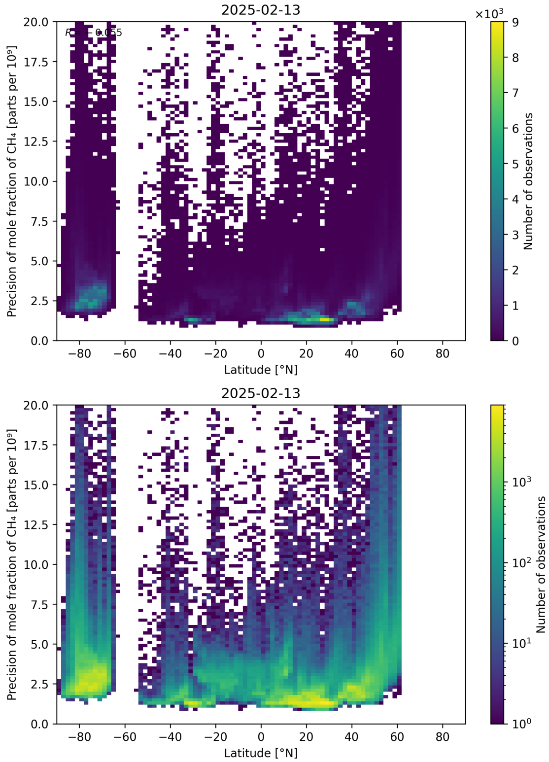
Figure 59: Scatter density plot of “Latitude” against “Precision of mole fraction of CH 4 ” for 2025-02-13 to 2025-02-14.
