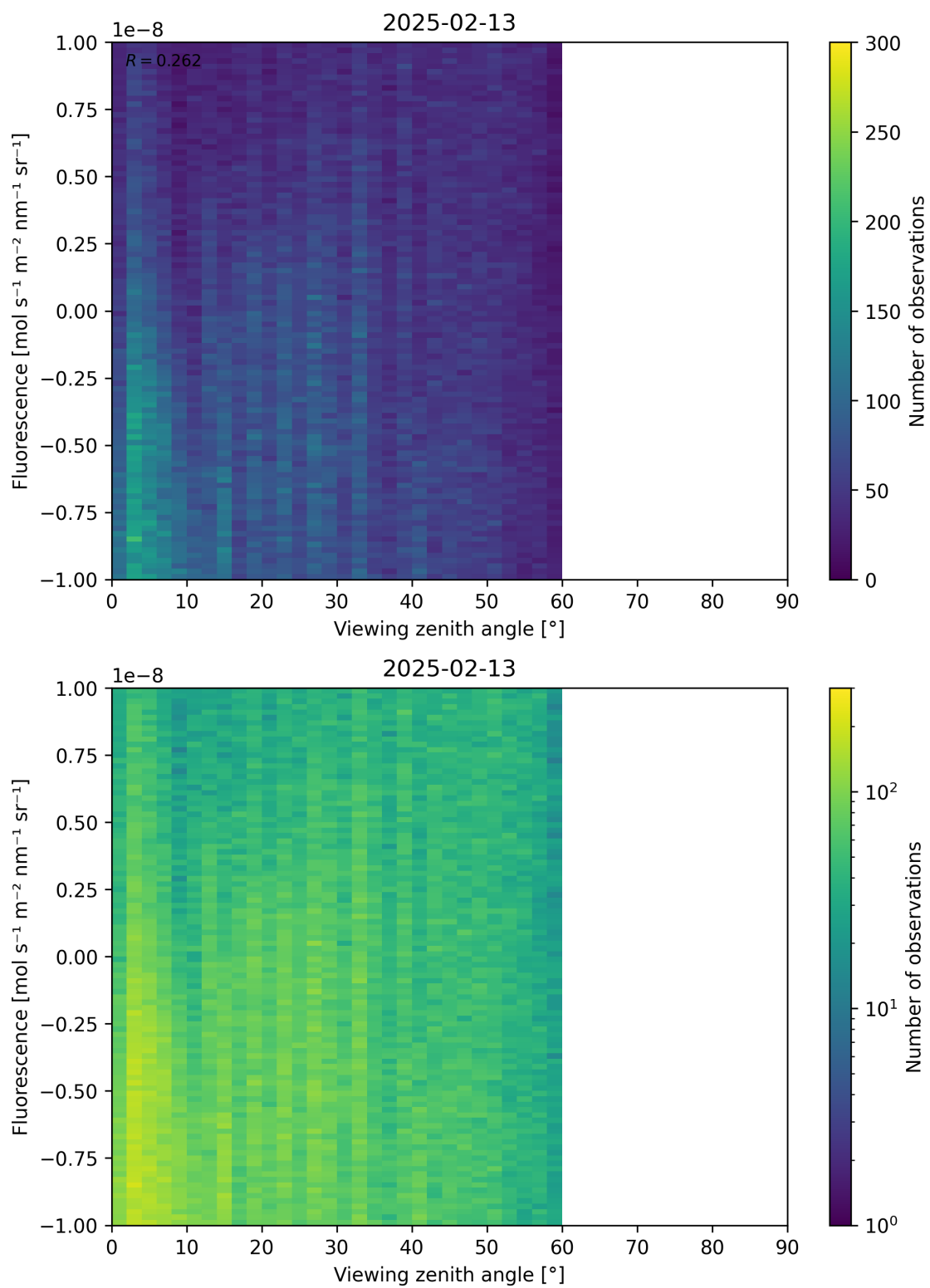
Figure 108: Scatter density plot of “Viewing zenith angle” against “Fluorescence” for 2025-02-13 to 2025-02-14.
