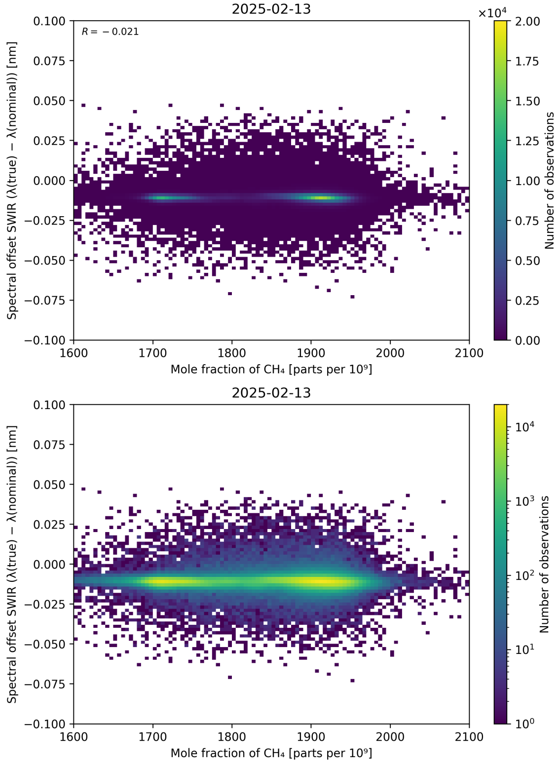
Figure 86: Scatter density plot of “Mole fraction of \text{CH}_4 ” against “Spectral offset SWIR ( \lambda_{\text{true}} - \lambda_{\text{nominal}} )” for 2025-02-13 to 2025-02-14.
