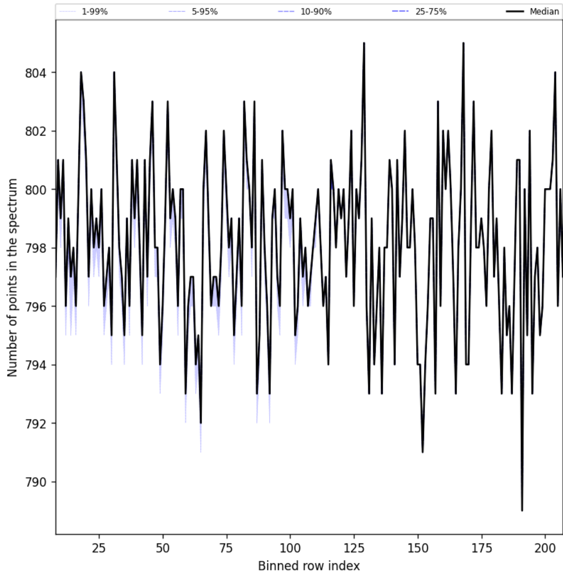
Figure 37: Along track statistics of “Number of points in the spectrum” for 2025-02-13 to 2025-02-14
