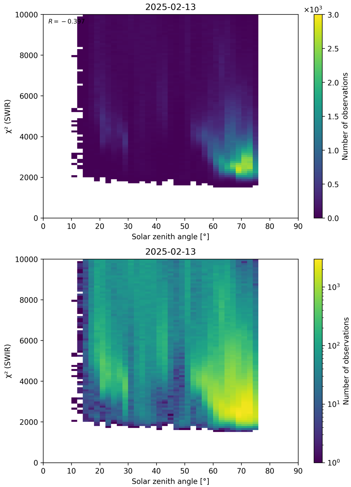
Figure 95: Scatter density plot of “Solar zenith angle” against “ \chi^2 (SWIR)” for 2025-02-13 to 2025-02-14.
