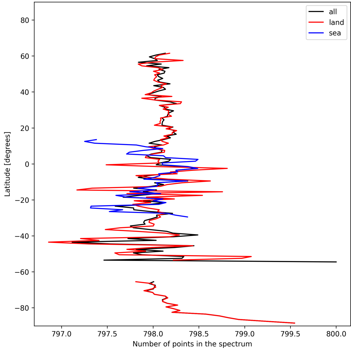
Figure 15: Zonal average of “Number of points in the spectrum” for 2025-02-13 to 2025-02-14.
