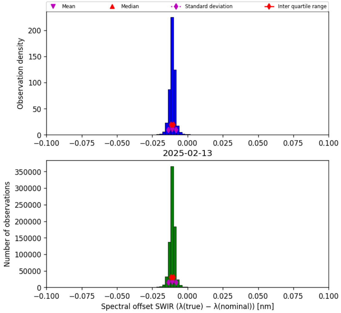
Figure 27: Histogram of “Spectral offset SWIR ( \lambda_{\text{true}} - \lambda_{\text{nominal}} )” for 2025-02-13 to 2025-02-14
