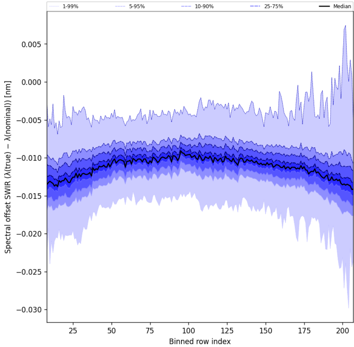
Figure 38: Along track statistics of “Spectral offset SWIR ( \lambda_{\text{true}} - \lambda_{\text{nominal}} )” for 2025-02-13 to 2025-02-14
