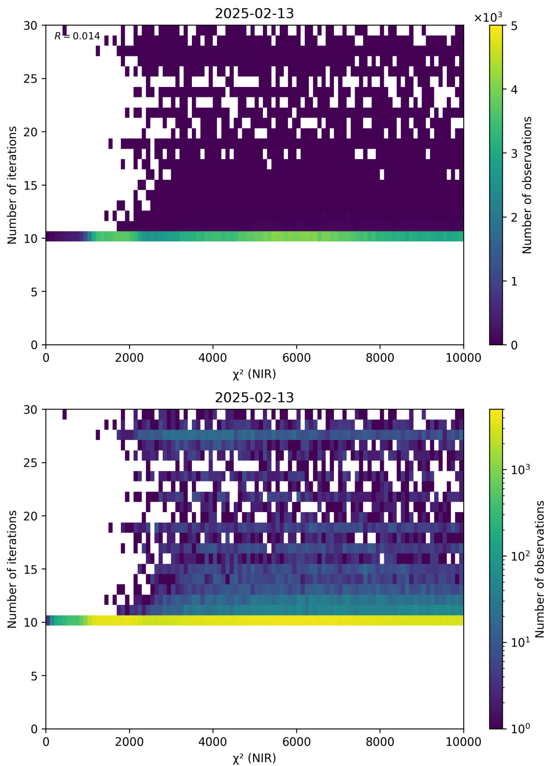
Figure 46: Scatter density plot of “ \chi^2 (NIR)” against “Number of iterations” for 2025-02-13 to 2025-02-14.
