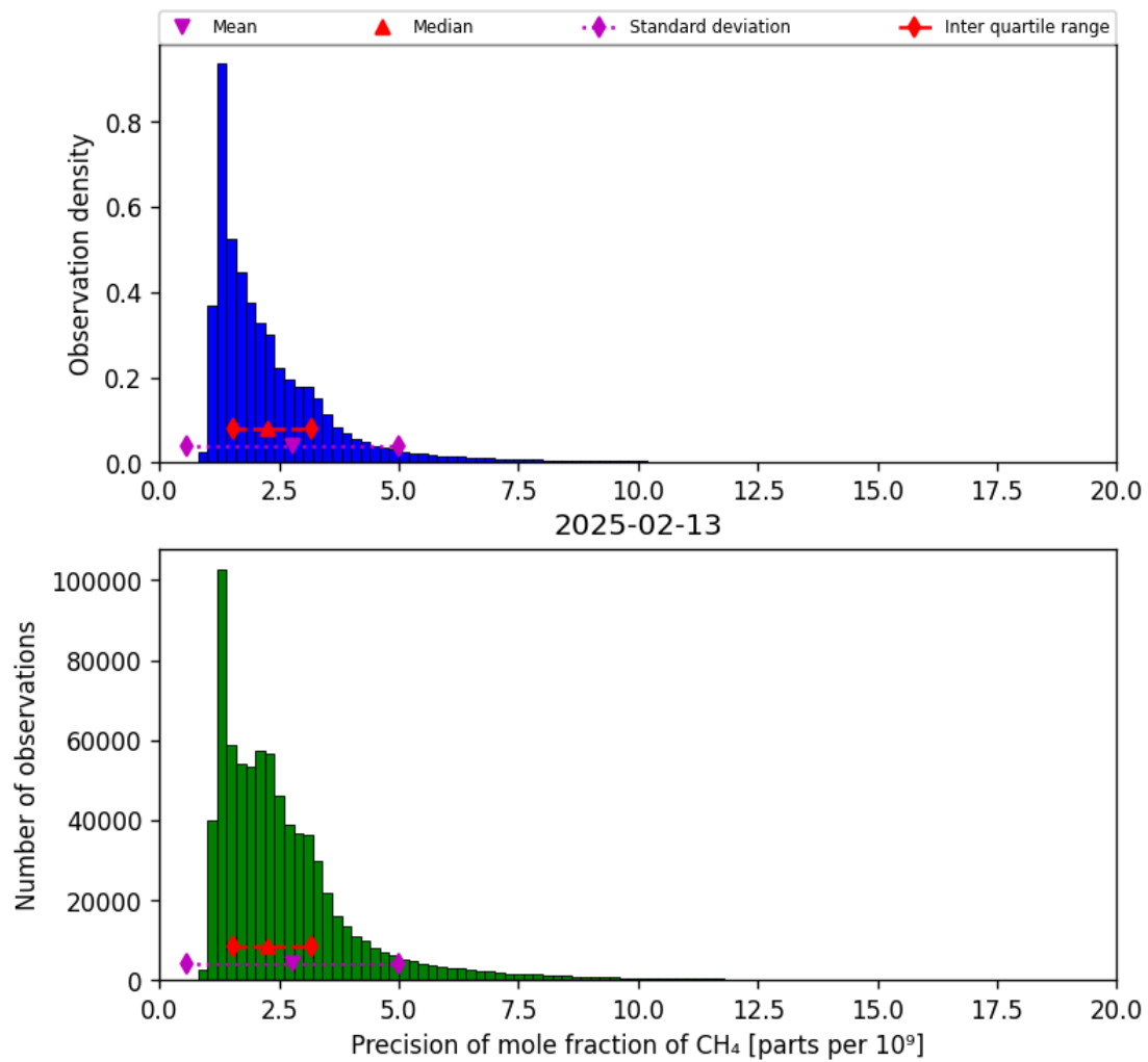
Figure 24: Histogram of “Precision of mole fraction of CH 4 ” for 2025-02-13 to 2025-02-14
