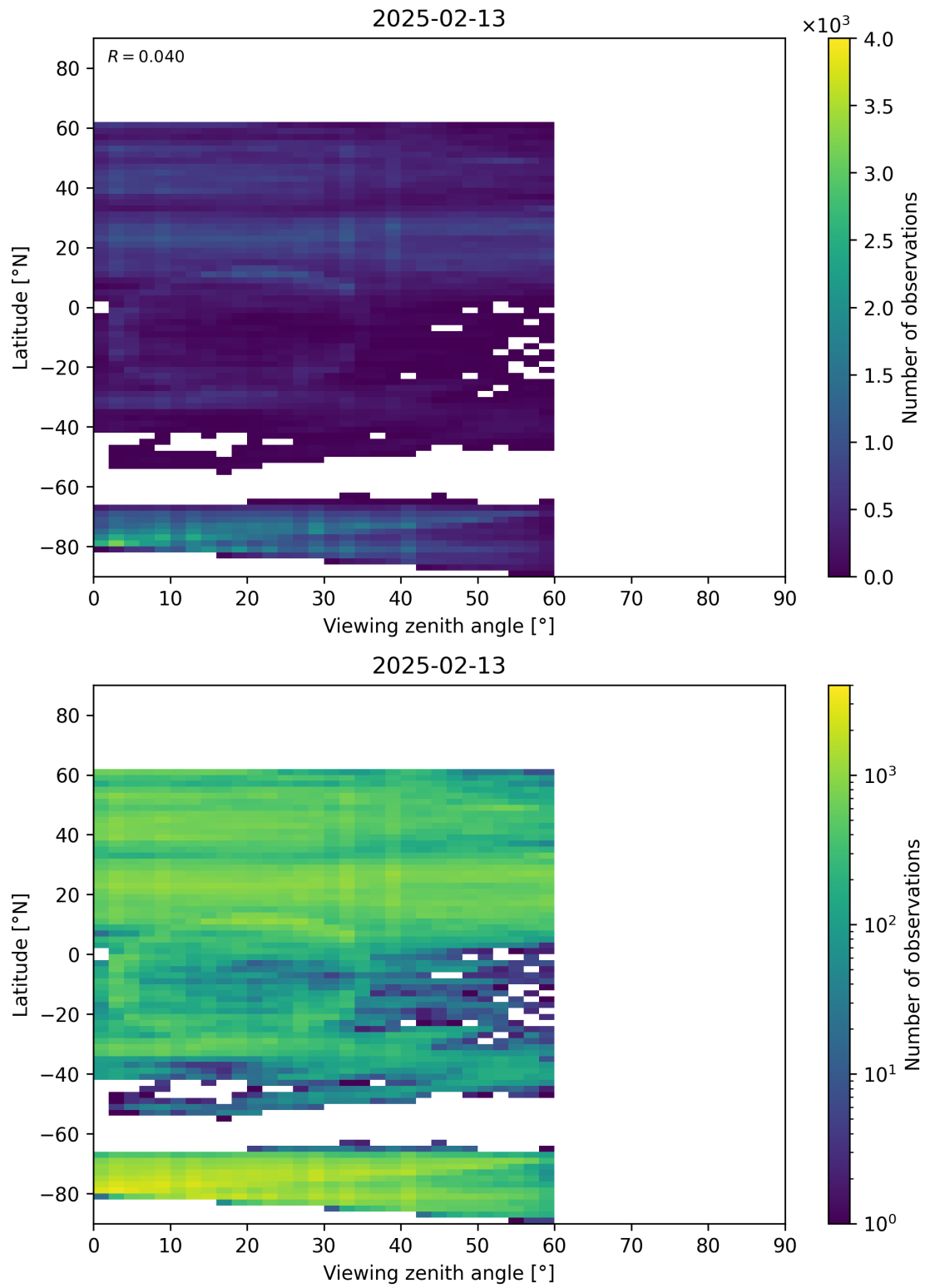
Figure 109: Scatter density plot of “Viewing zenith angle” against “Latitude” for 2025-02-13 to 2025-02-14.
