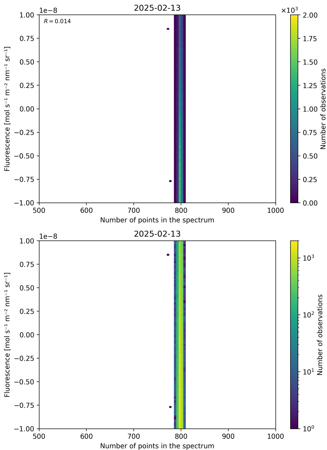
Figure 91: Scatter density plot of “Number of points in the spectrum” against “Fluorescence” for 2025-02-13 to 2025-02-14.
