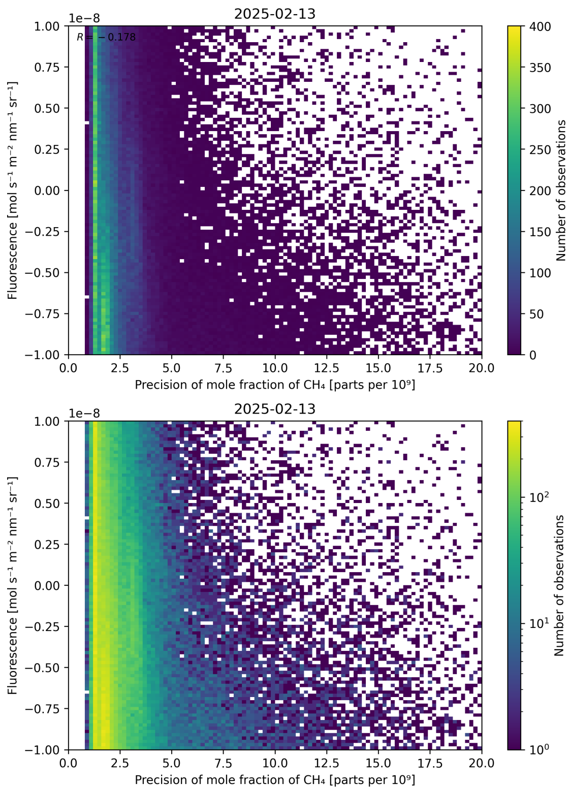
Figure 81: Scatter density plot of “Precision of mole fraction of \text{CH}_4 ” against “Fluorescence” for 2025-02-13 to 2025-02-14.
