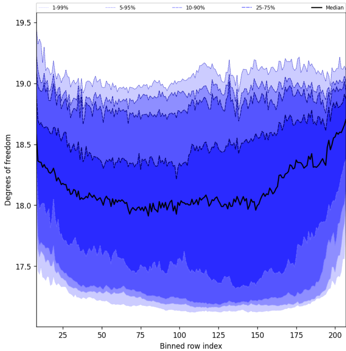
Figure 41: Along track statistics of “Degrees of freedom” for 2025-02-13 to 2025-02-14
