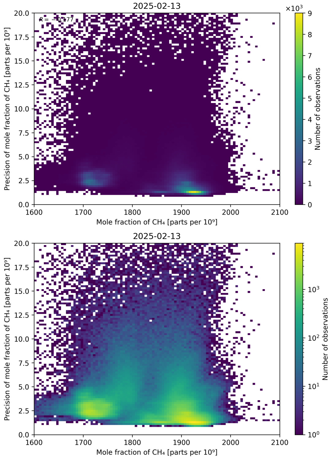
Figure 75: Scatter density plot of “Mole fraction of CH 4 ” against “Precision of mole fraction of CH 4 ” for 2025-02-13 to 2025-02-14.
