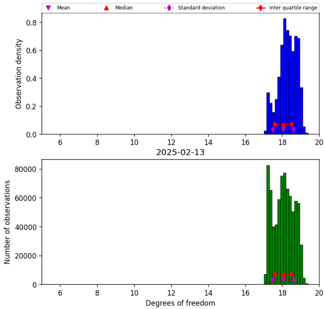
Figure 30: Histogram of “Degrees of freedom” for 2025-02-13 to 2025-02-14
