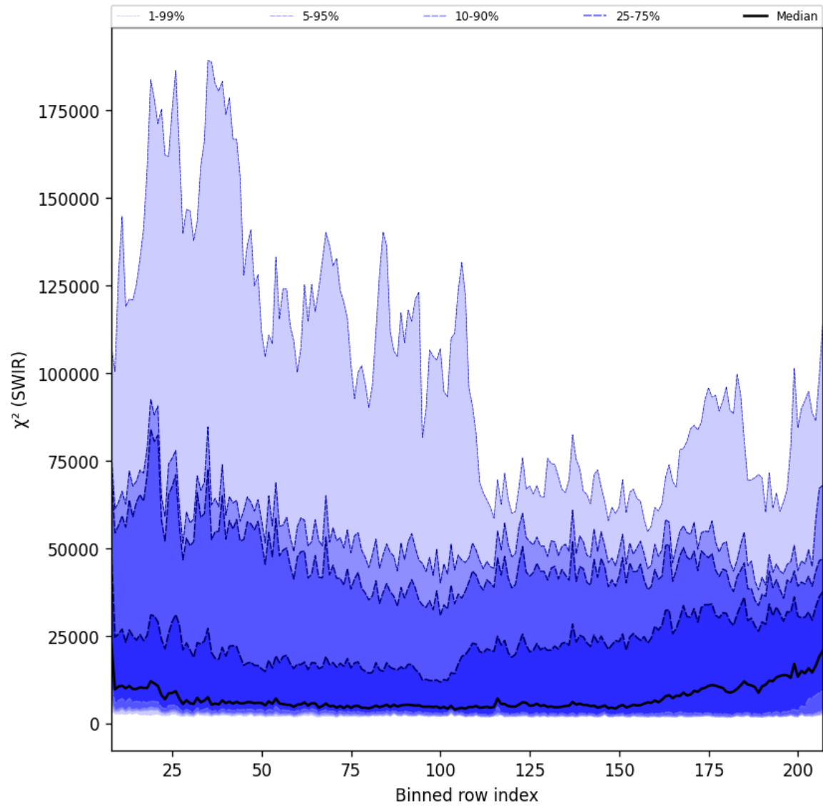
Figure 39: Along track statistics of " \chi^2 (SWIR)" for 2025-02-13 to 2025-02-14
