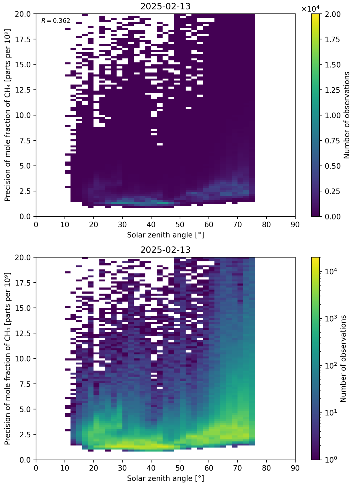
Figure 101: Scatter density plot of “Solar zenith angle” against “Precision of mole fraction of CH 4 ” for 2025-02-13 to 2025-02-14.
