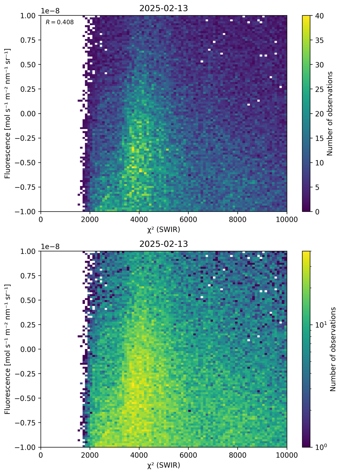
Figure 49: Scatter density plot of “ \chi^2 (SWIR)” against “Fluorescence” for 2025-02-13 to 2025-02-14.
