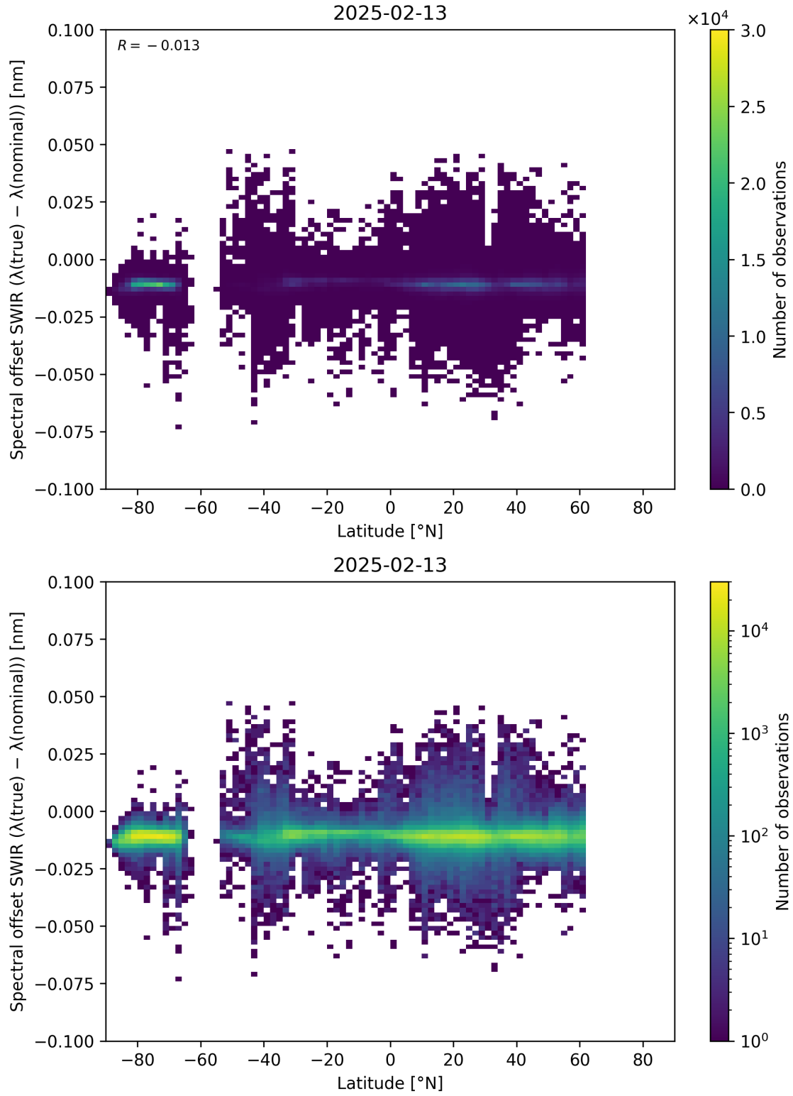
Figure 62: Scatter density plot of “Latitude” against “Spectral offset SWIR ( \lambda_{\text{true}} - \lambda_{\text{nominal}} )” for 2025-02-13 to 2025-02-14.
