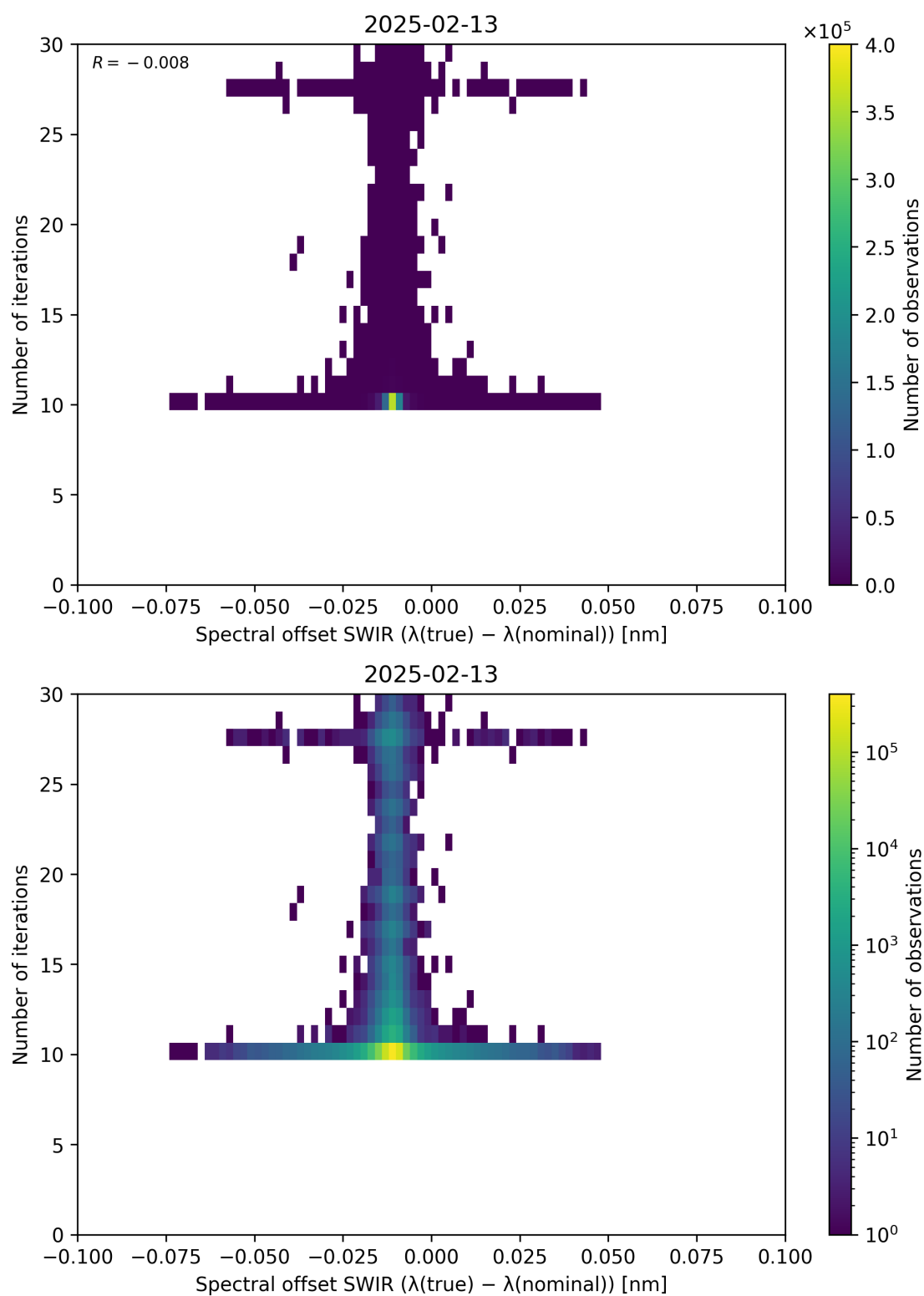
Figure 121: Scatter density plot of “Spectral offset SWIR ( \lambda_{\text{true}} - \lambda_{\text{nominal}} )” against “Number of iterations” for 2025-02-13 to 2025-02-14.
