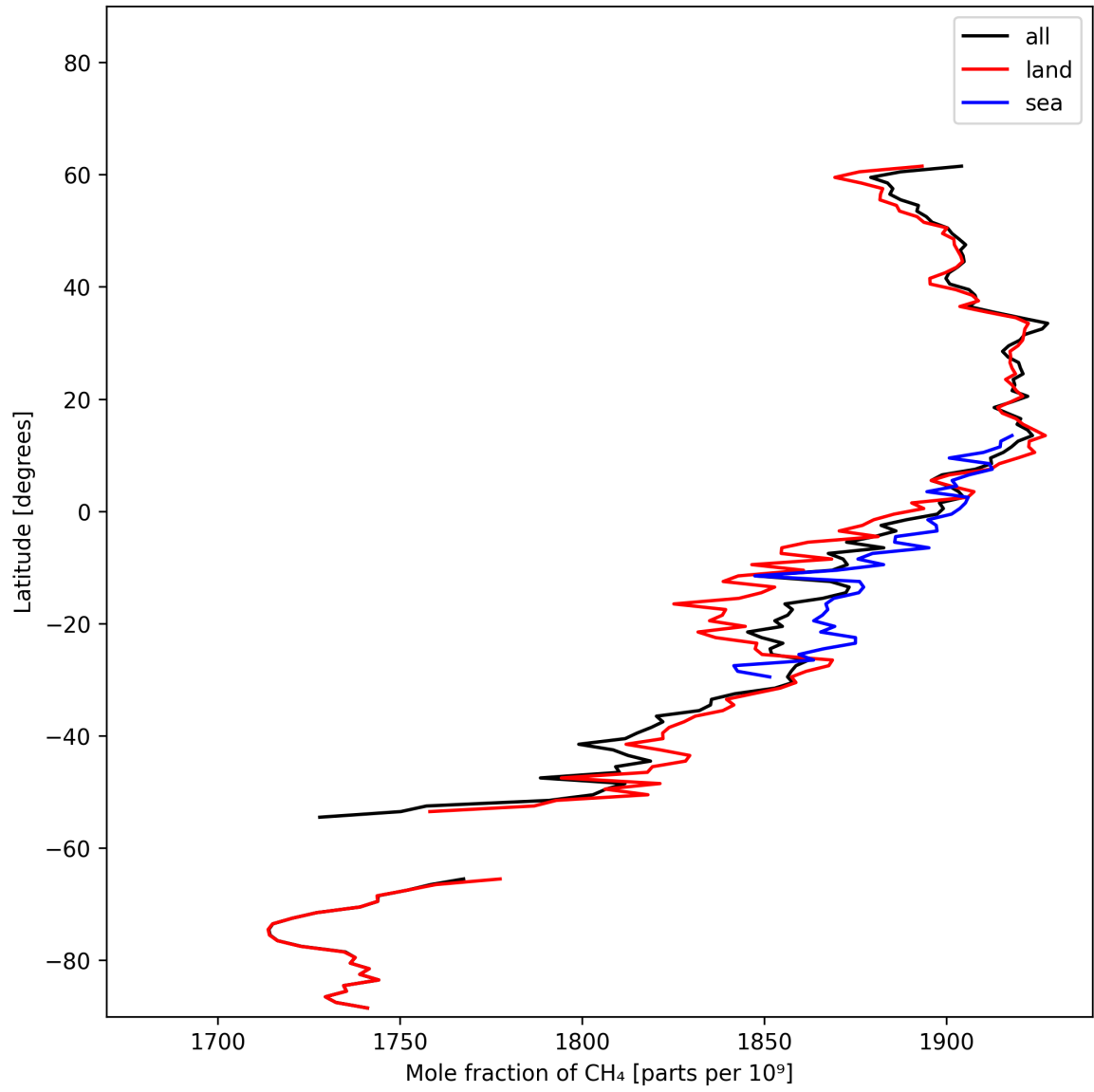
Figure 12: Zonal average of “Mole fraction of CH 4 ” for 2025-02-13 to 2025-02-14.
