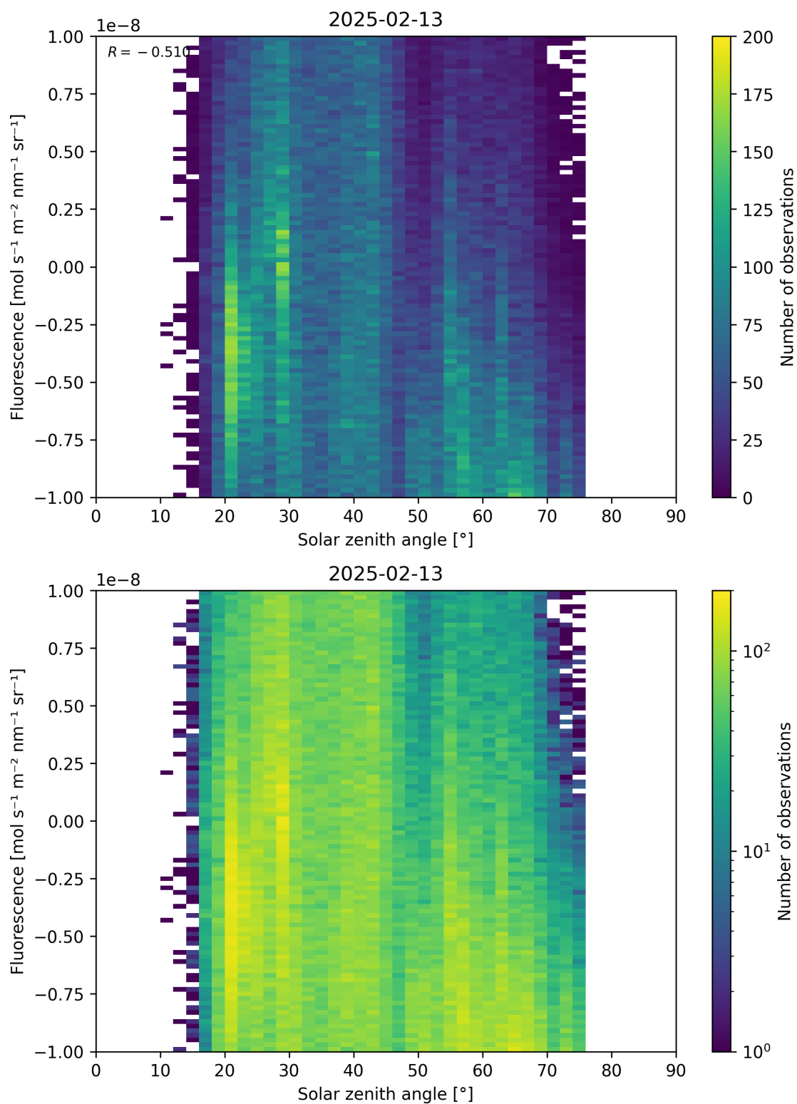
Figure 97: Scatter density plot of “Solar zenith angle” against “Fluorescence” for 2025-02-13 to 2025-02-14.
