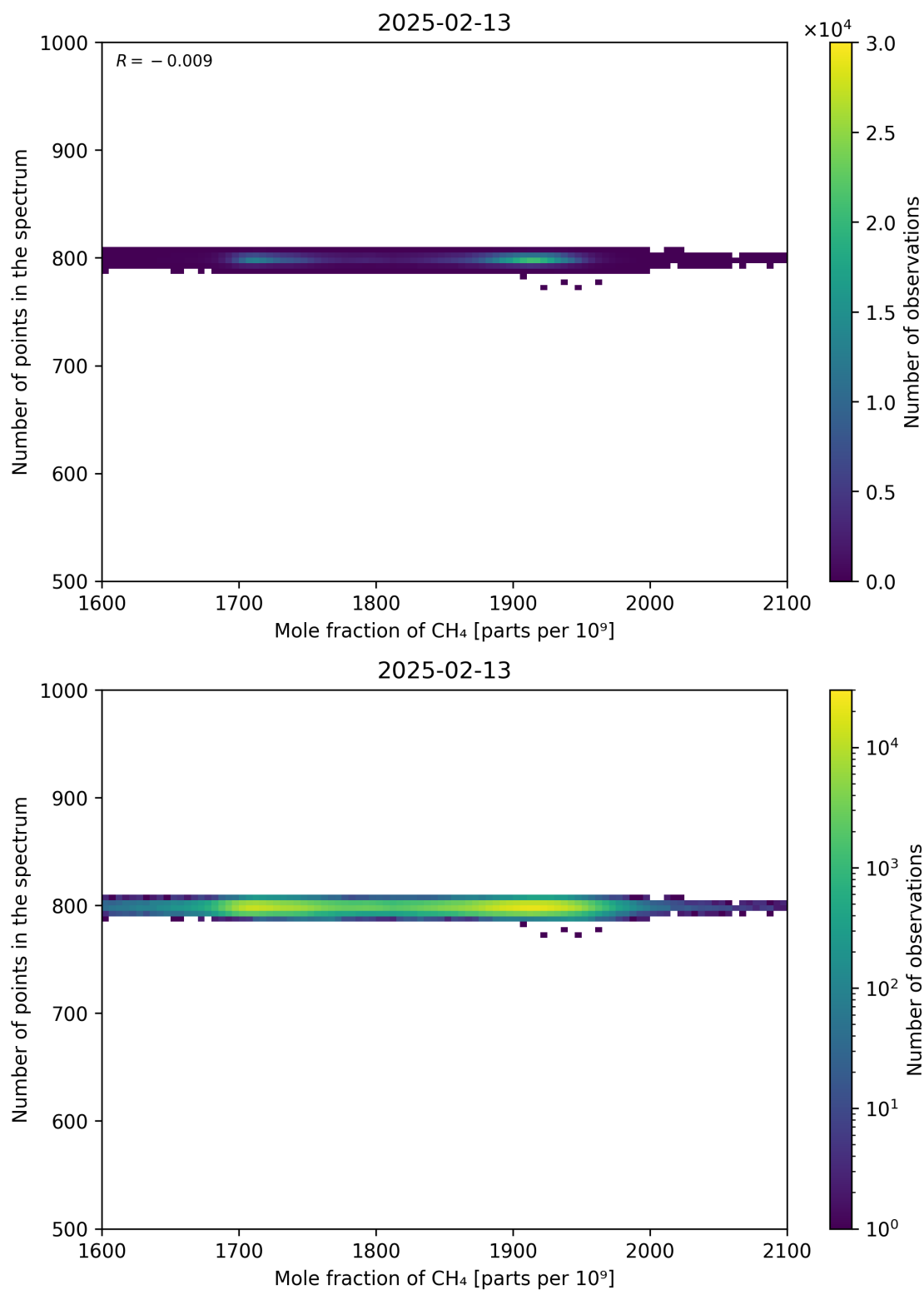
Figure 77: Scatter density plot of “Mole fraction of CH 4 ” against “Number of points in the spectrum” for 2025-02-13 to 2025-02-14.
