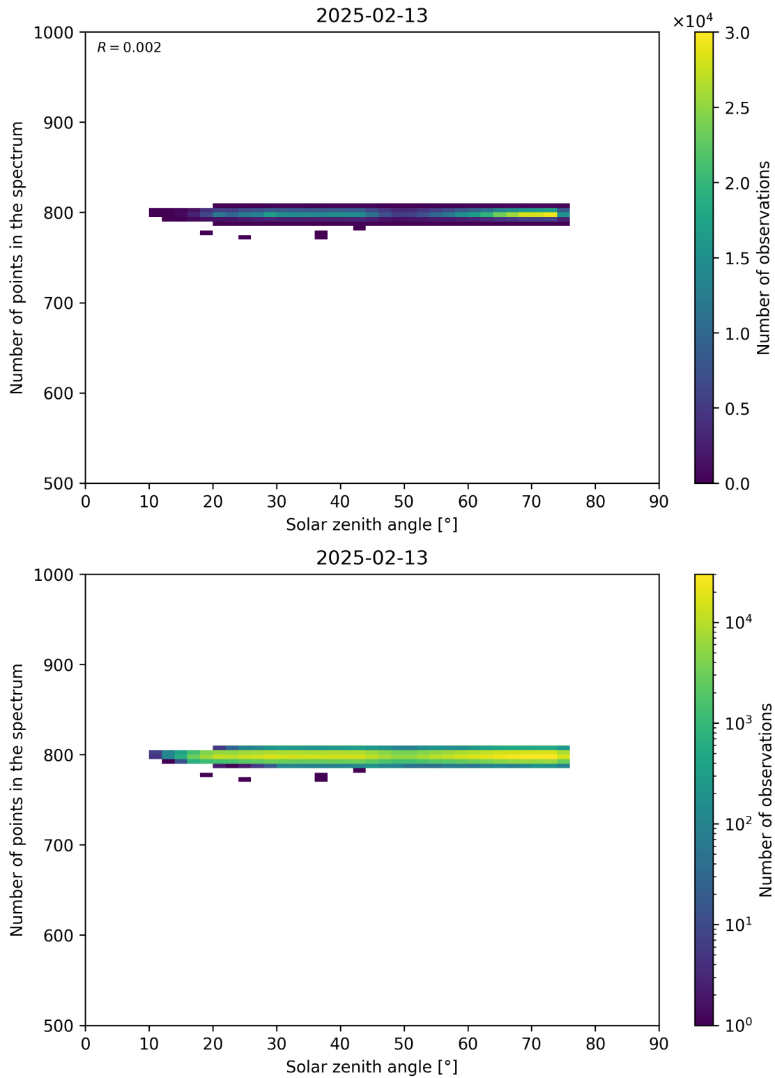
Figure 103: Scatter density plot of “Solar zenith angle” against “Number of points in the spectrum” for 2025-02-13 to 2025-02-14.
