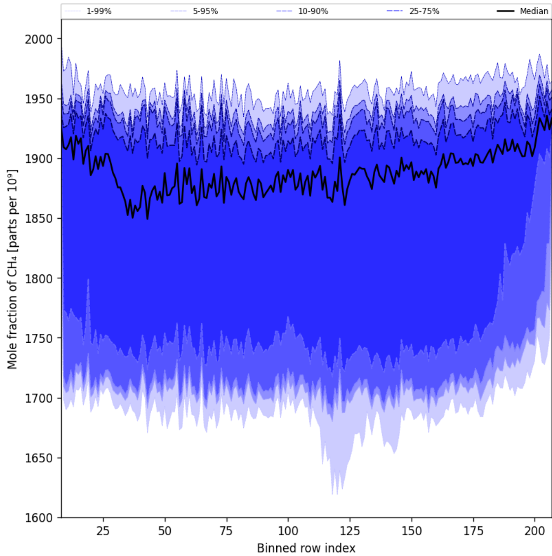
Figure 34: Along track statistics of “Mole fraction of CH 4 ” for 2025-02-13 to 2025-02-14
