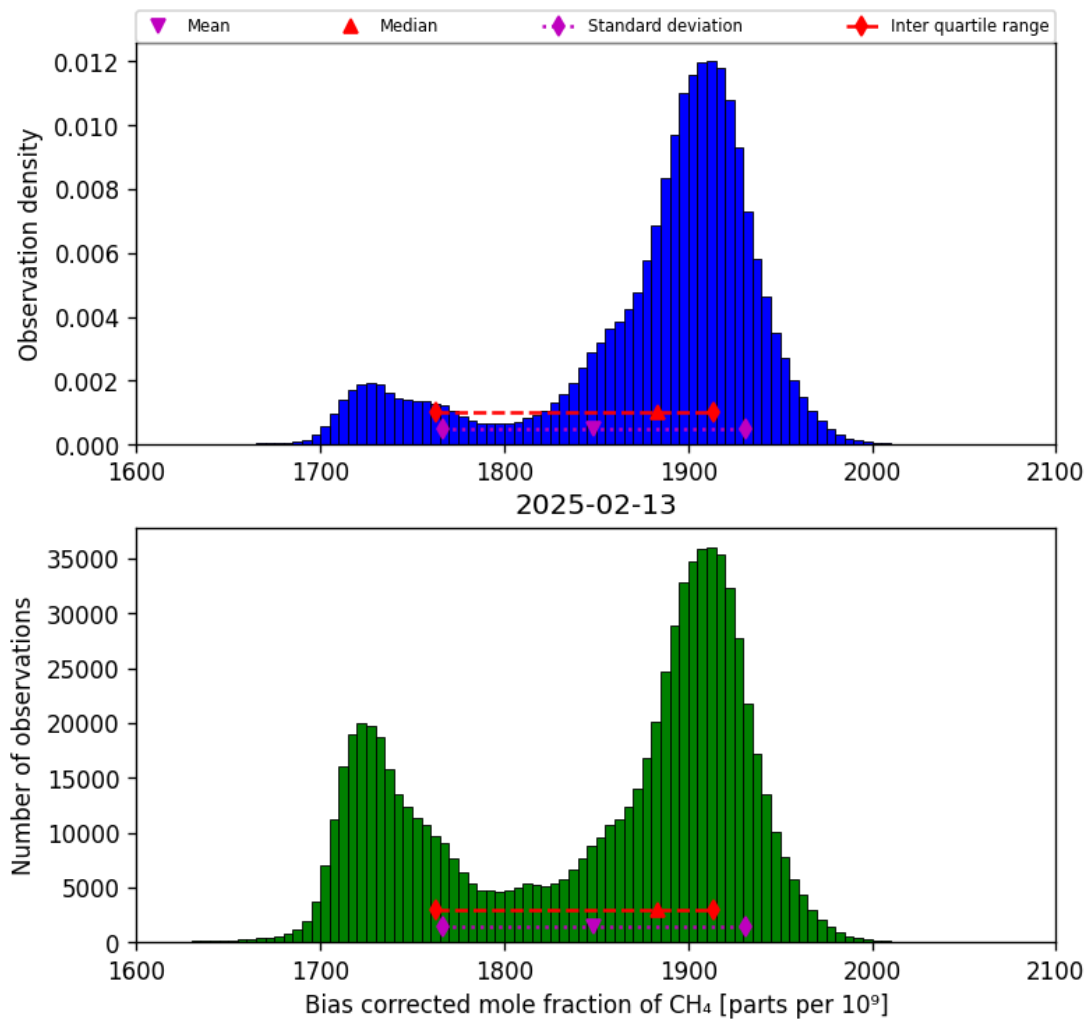
Figure 25: Histogram of “Bias corrected mole fraction of CH 4 ” for 2025-02-13 to 2025-02-14
