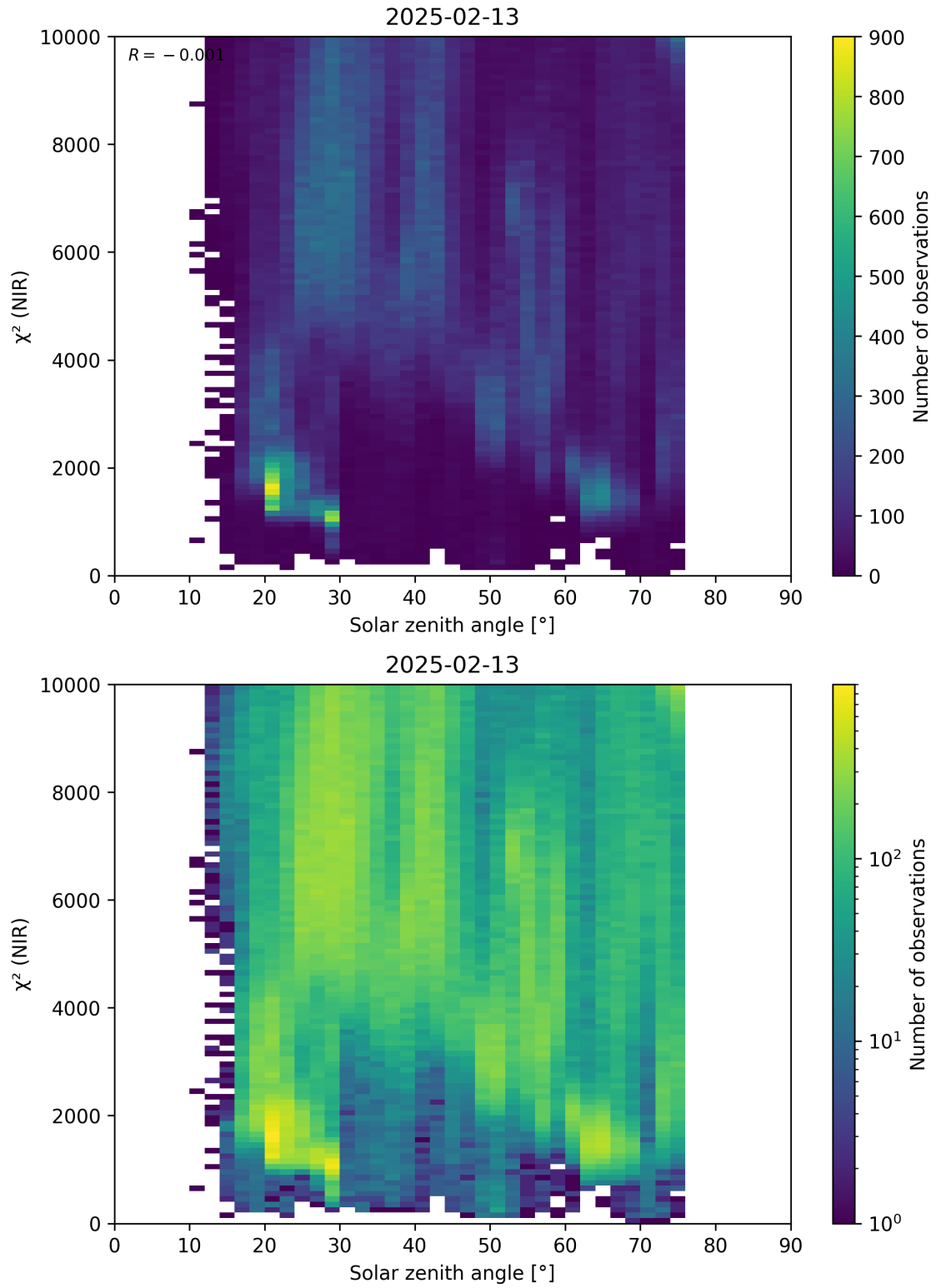
Figure 94: Scatter density plot of “Solar zenith angle” against “ \chi^2 (NIR)” for 2025-02-13 to 2025-02-14.
