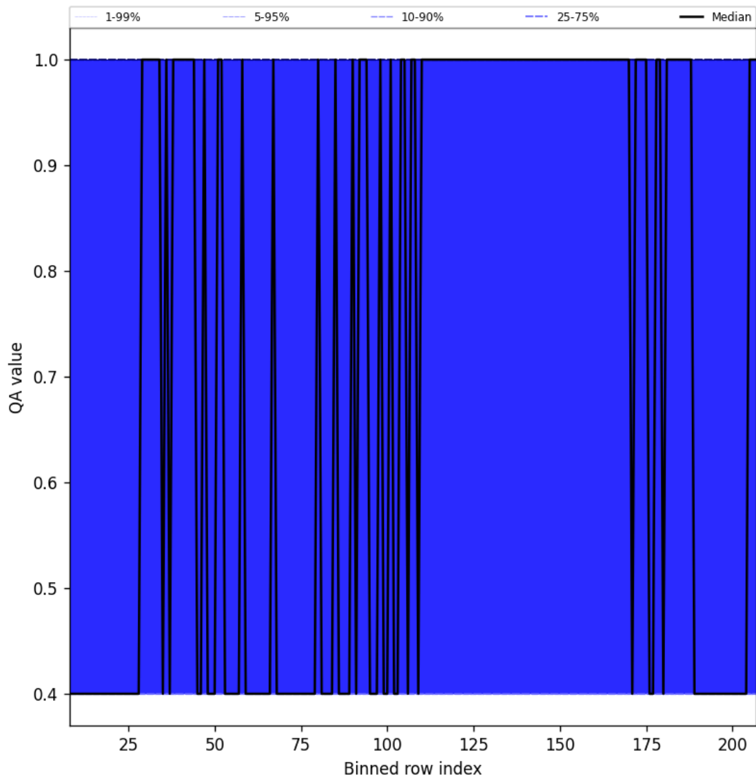
Figure 33: Along track statistics of “QA value” for 2025-02-13 to 2025-02-14
