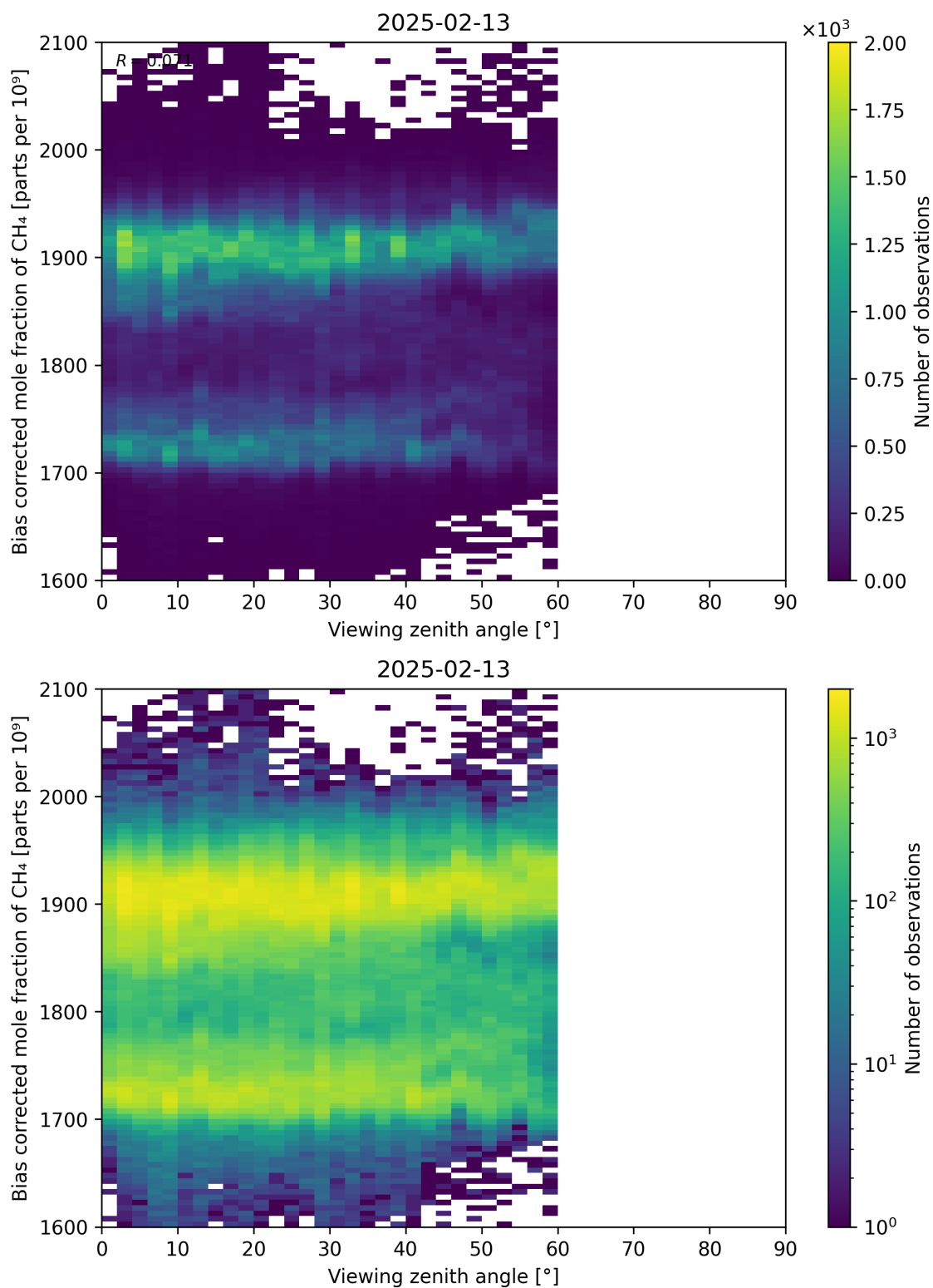
Figure 111: Scatter density plot of “Viewing zenith angle” against “Bias corrected mole fraction of CH 4 ” for 2025-02-13 to 2025-02-14.
