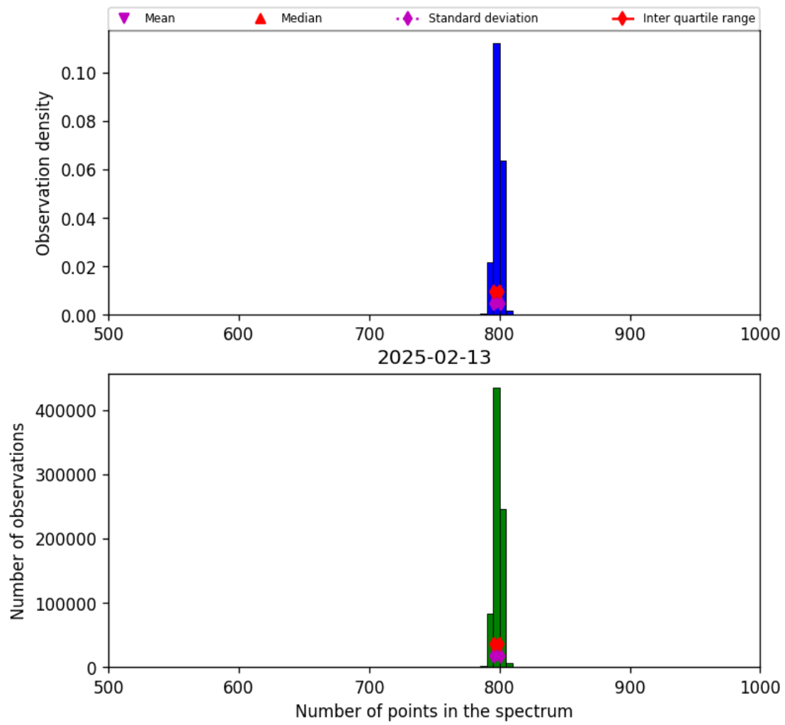
Figure 26: Histogram of “Number of points in the spectrum” for 2025-02-13 to 2025-02-14
