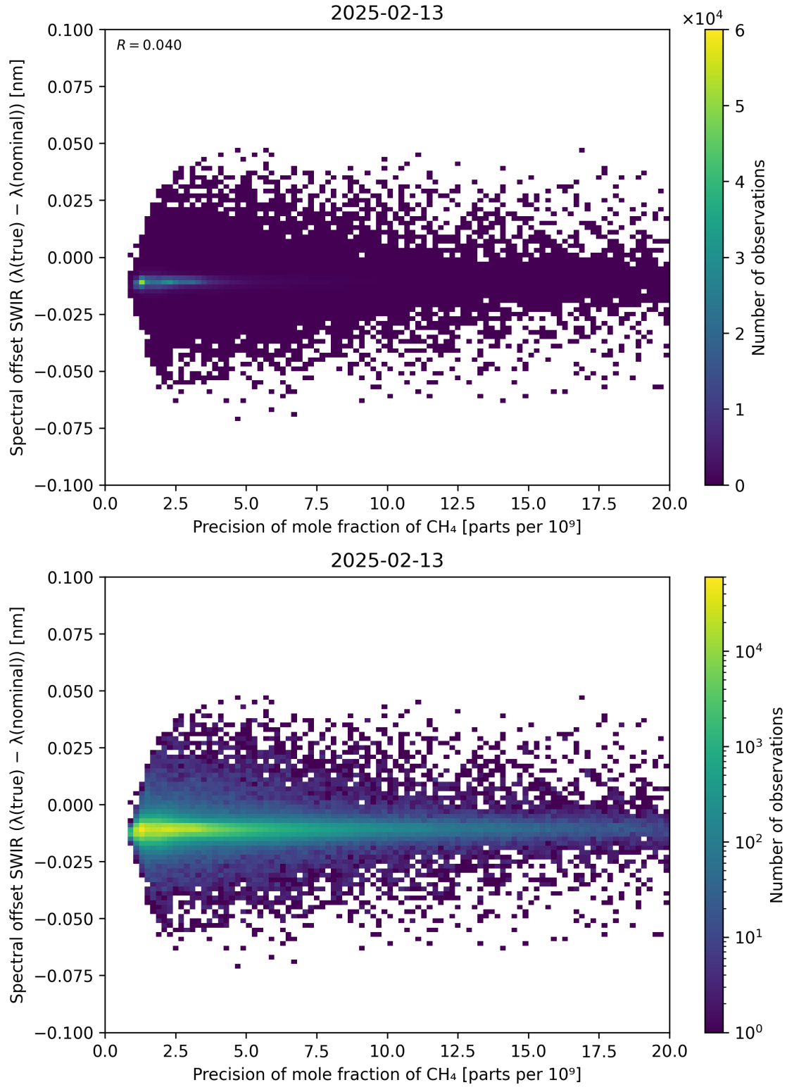
Figure 85: Scatter density plot of “Precision of mole fraction of CH 4 ” against “Spectral offset SWIR ( \lambda_{\text{true}} - \lambda_{\text{nominal}} )” for 2025-02-13 to 2025-02-14.
