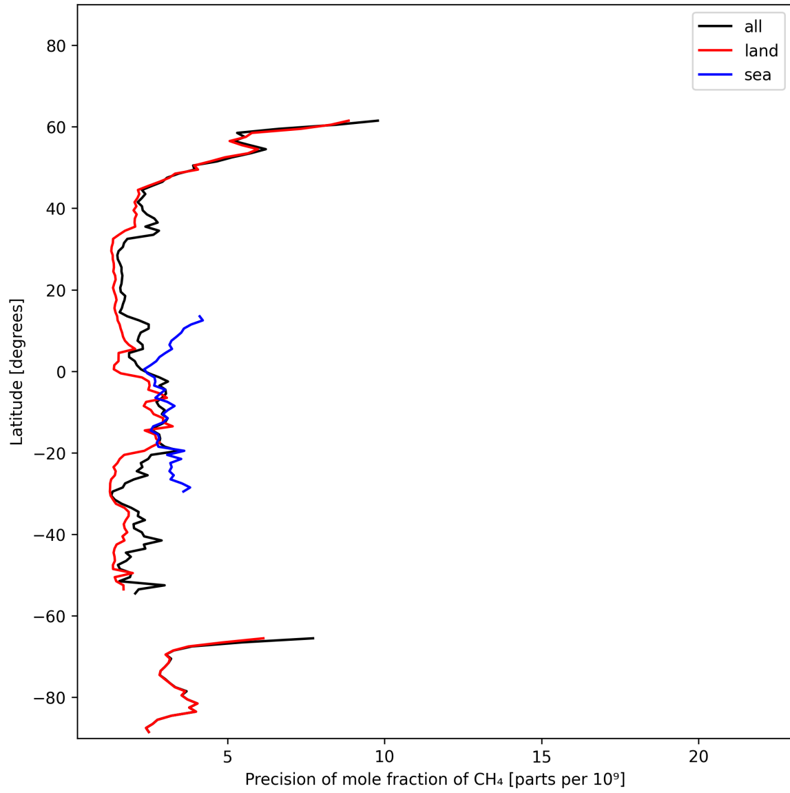
Figure 13: Zonal average of “Precision of mole fraction of CH 4 ” for 2025-02-13 to 2025-02-14.
