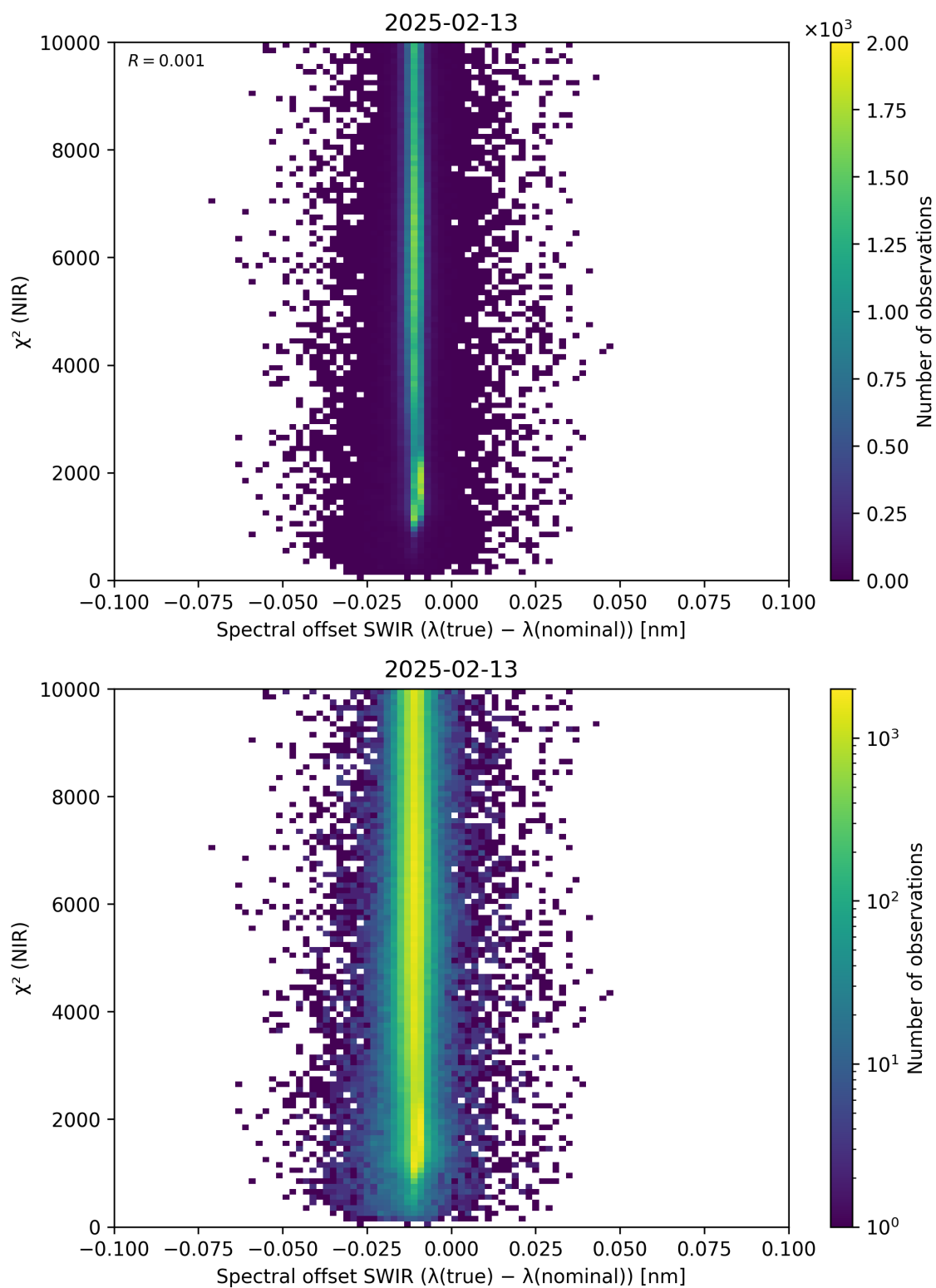
Figure 117: Scatter density plot of “Spectral offset SWIR ( \lambda_{\text{true}} - \lambda_{\text{nominal}} )” against “ \chi^2 (NIR)” for 2025-02-13 to 2025-02-14.
