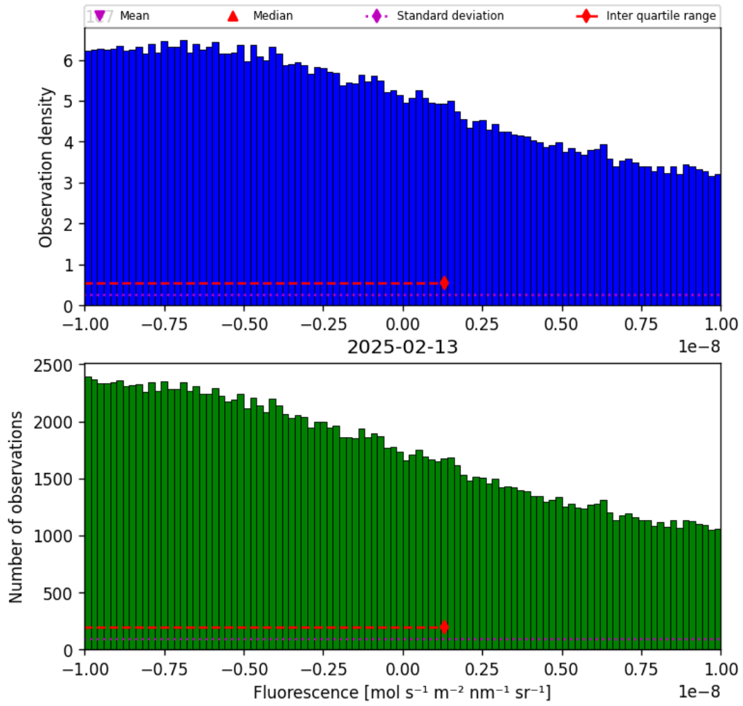
Figure 32: Histogram of “Fluorescence” for 2025-02-13 to 2025-02-14
