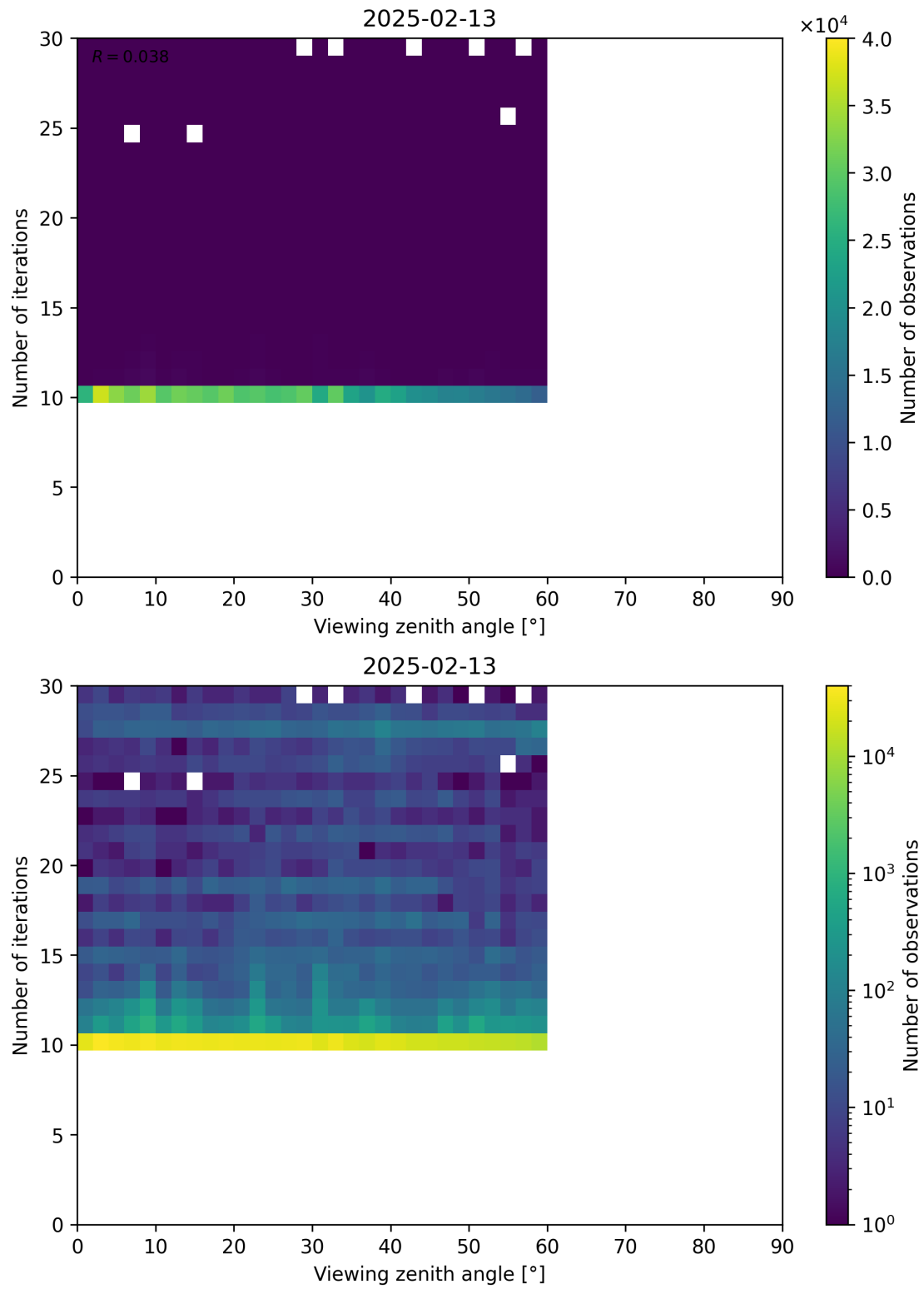
Figure 113: Scatter density plot of “Viewing zenith angle” against “Number of iterations” for 2025-02-13 to 2025-02-14.
