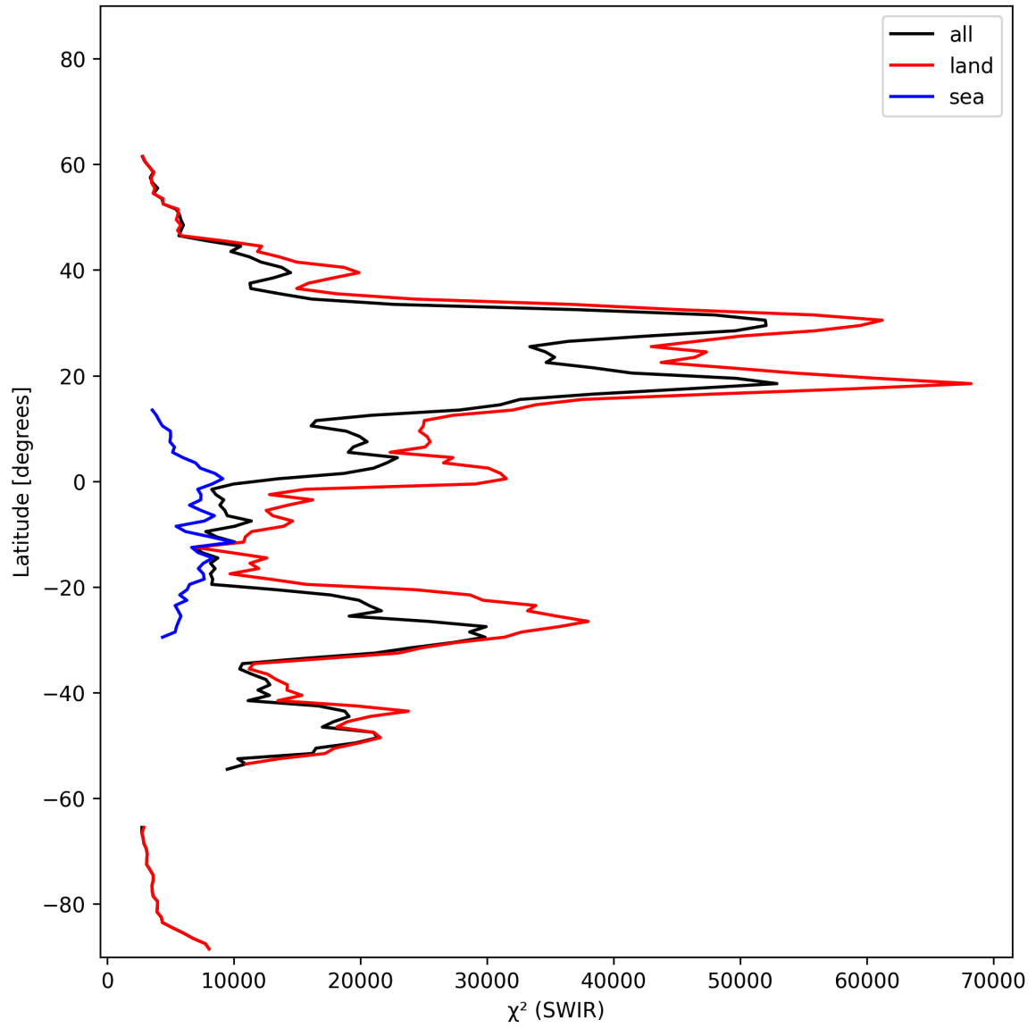
Figure 17: Zonal average of “ \chi^2 (SWIR)” for 2025-02-13 to 2025-02-14.
