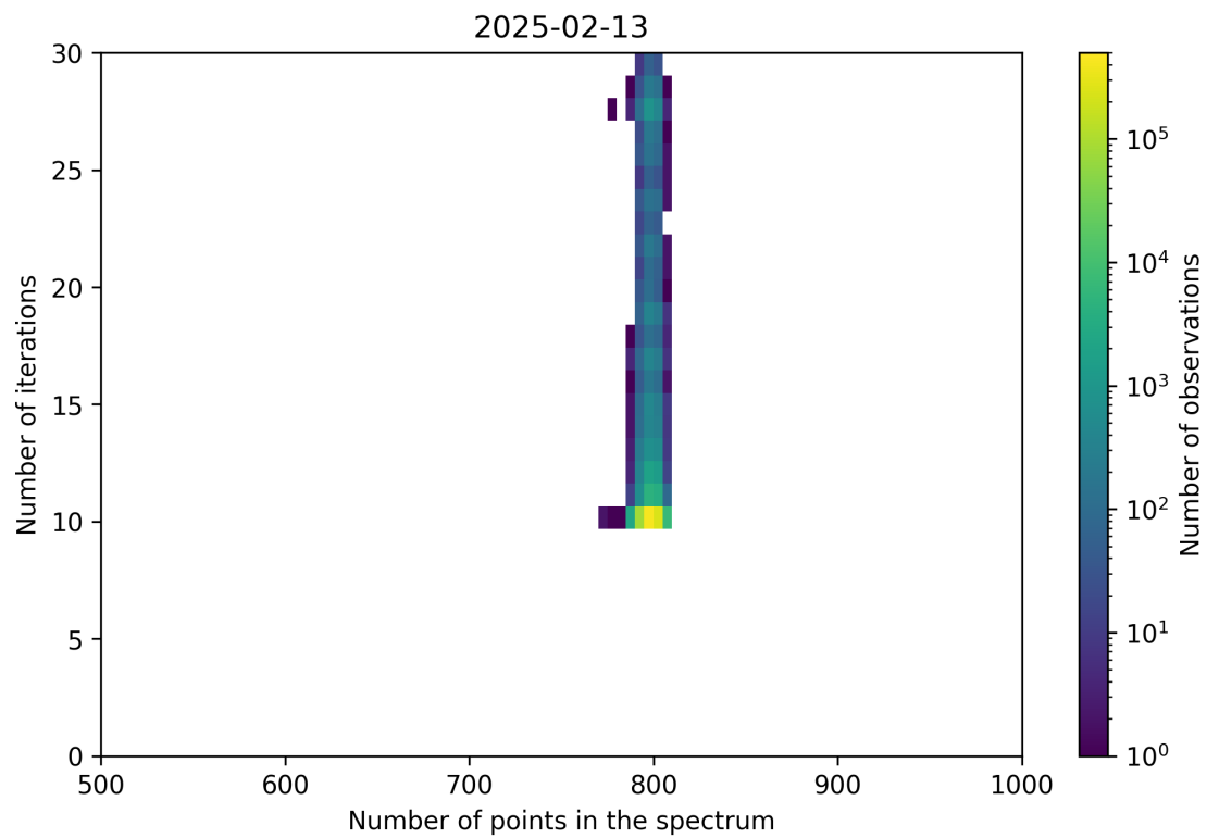
Figure 92: Scatter density plot of “Number of points in the spectrum” against “Number of iterations” for 2025-02-13 to 2025-02-14.
