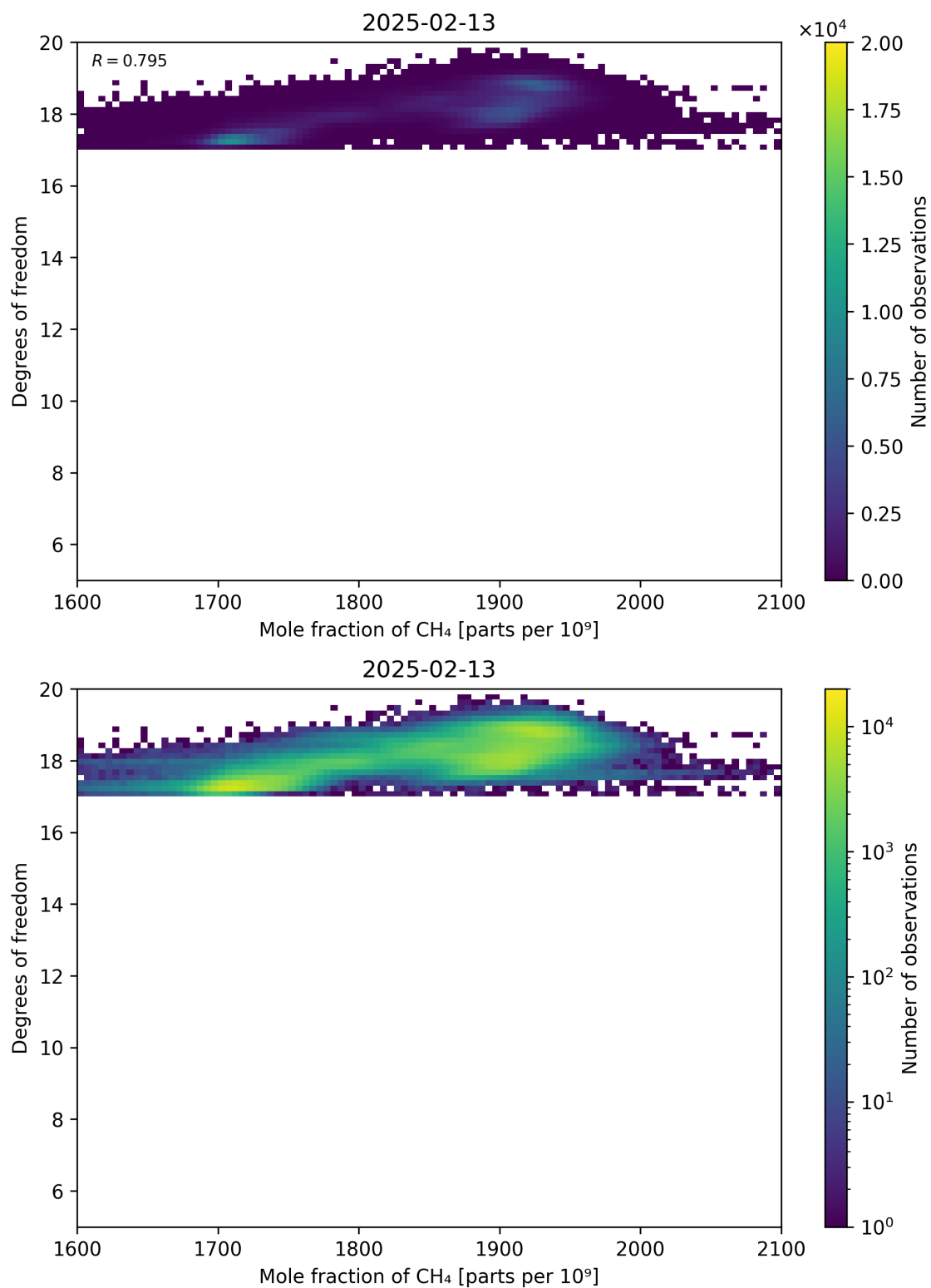
Figure 72: Scatter density plot of “Mole fraction of CH 4 ” against “Degrees of freedom” for 2025-02-13 to 2025-02-14.
