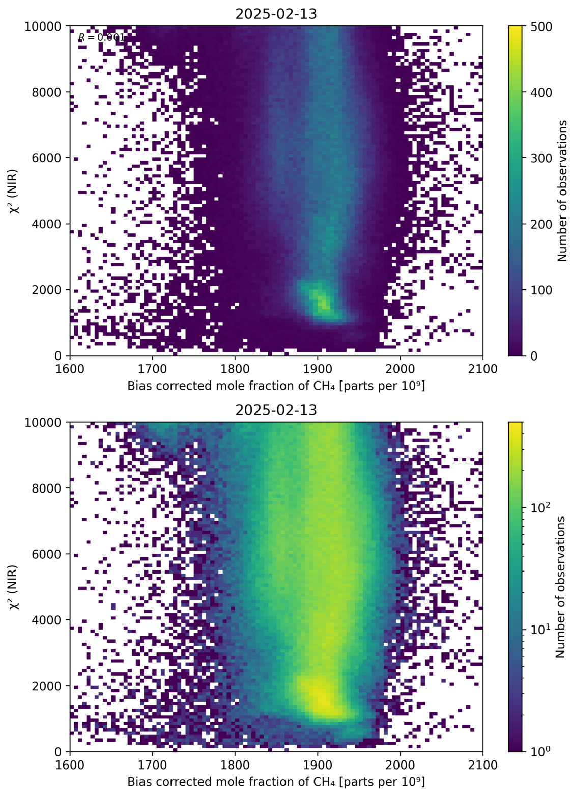
Figure 63: Scatter density plot of “Bias corrected mole fraction of \text{CH}_4 ” against “ \chi^2 (NIR)” for 2025-02-13 to 2025-02-14.
