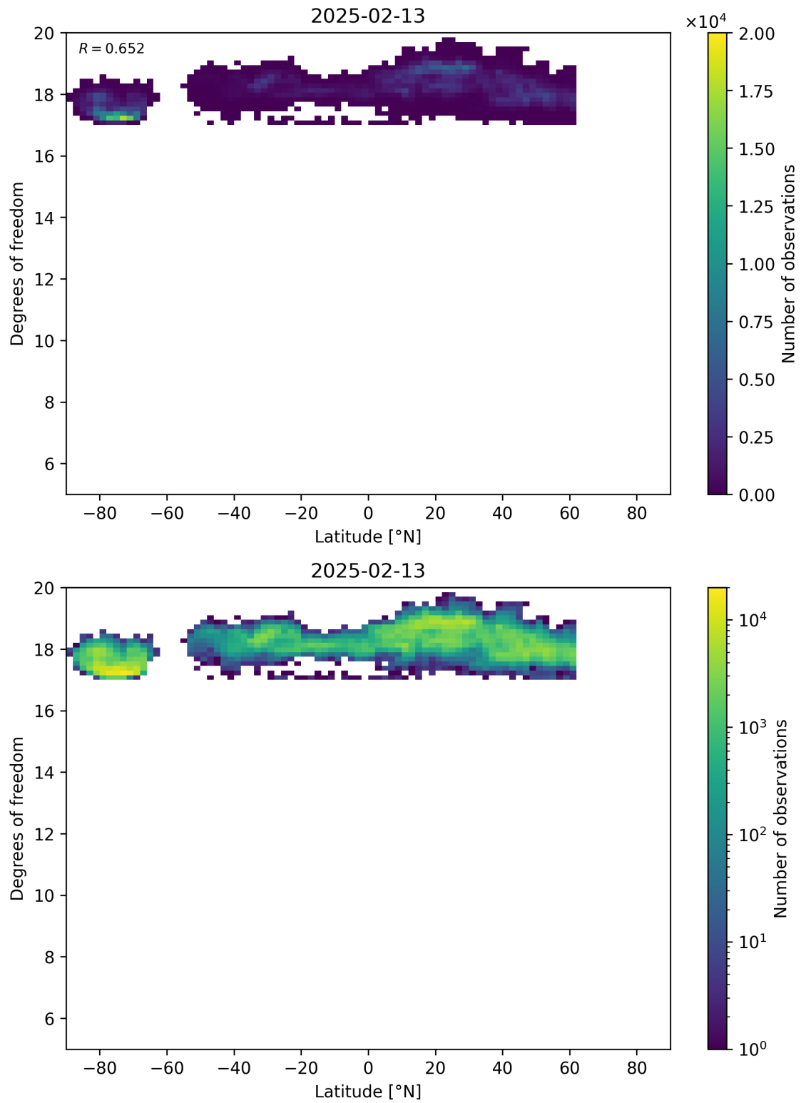
Figure 55: Scatter density plot of “Latitude” against “Degrees of freedom” for 2025-02-13 to 2025-02-14.
