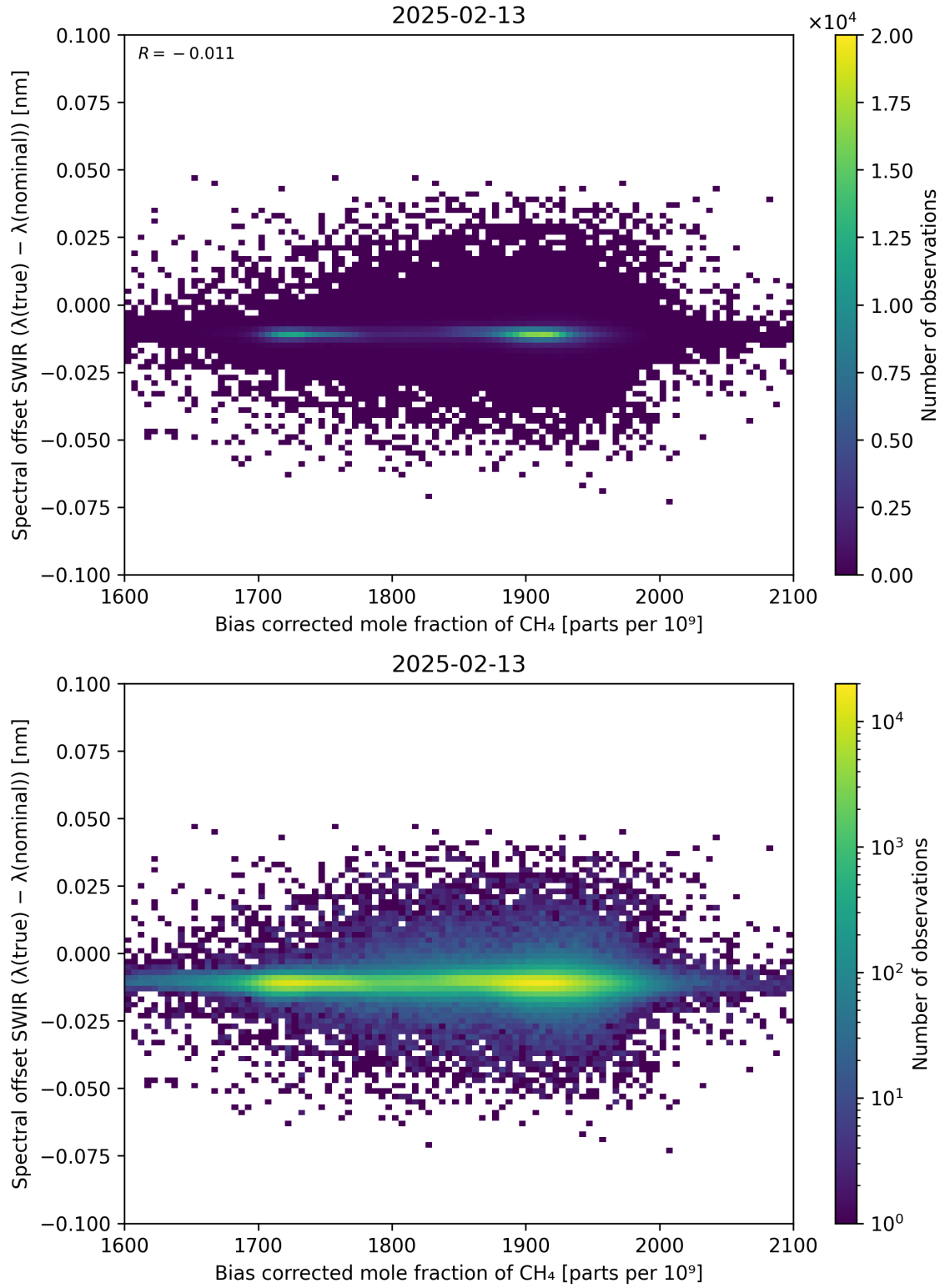
Figure 69: Scatter density plot of “Bias corrected mole fraction of \text{CH}_4 ” against “Spectral offset SWIR ( \lambda_{\text{true}} - \lambda_{\text{nominal}} )” for 2025-02-13 to 2025-02-14.
