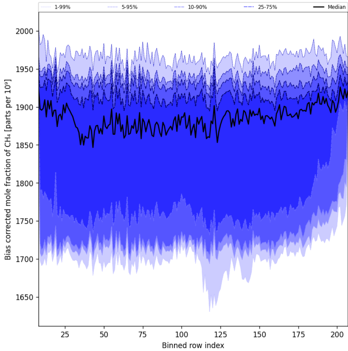
Figure 36: Along track statistics of “Bias corrected mole fraction of CH 4 ” for 2025-02-13 to 2025-02-14
