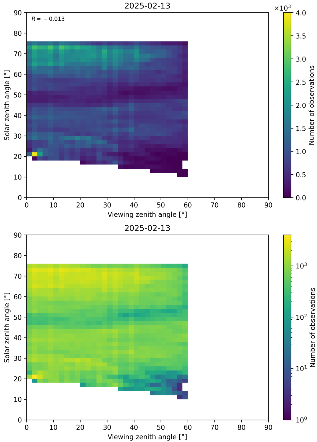
Figure 115: Scatter density plot of “Viewing zenith angle” against “Solar zenith angle” for 2025-02-13 to 2025-02-14.
