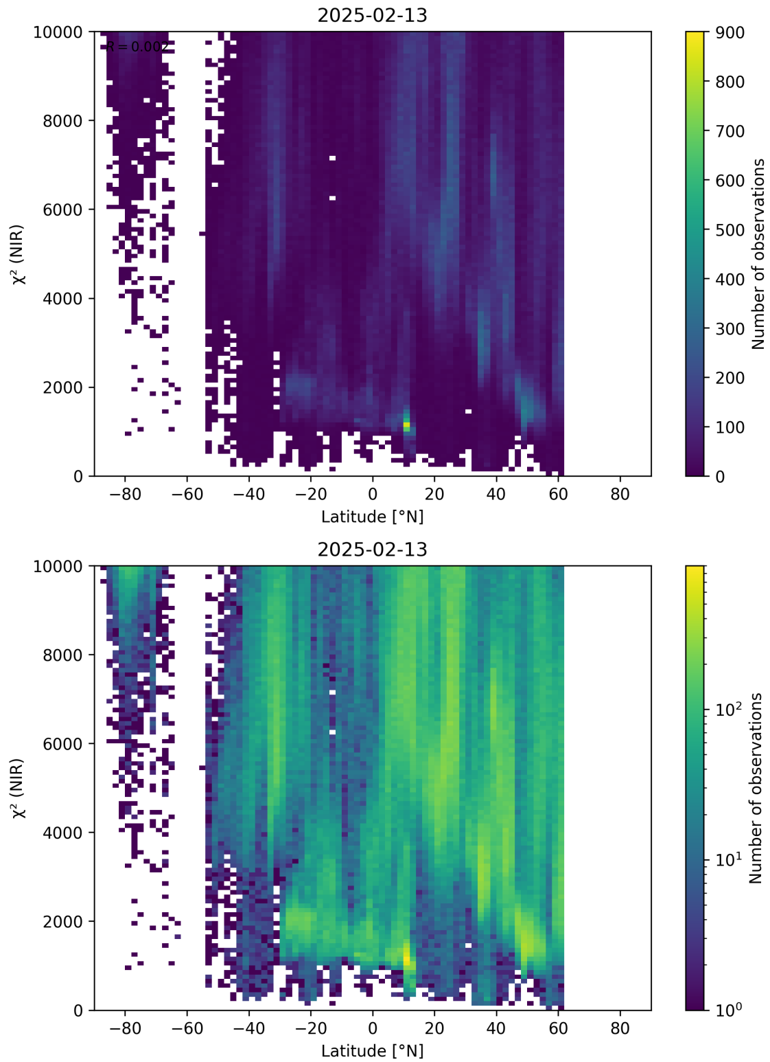
Figure 53: Scatter density plot of “Latitude” against “ \chi^2 (NIR)” for 2025-02-13 to 2025-02-14.
