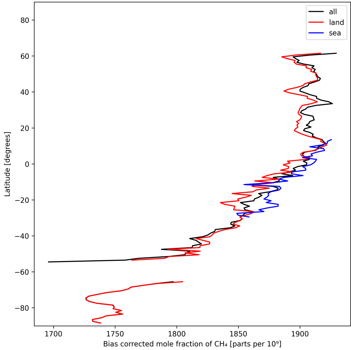
Figure 14: Zonal average of “Bias corrected mole fraction of CH 4 ” for 2025-02-13 to 2025-02-14.
