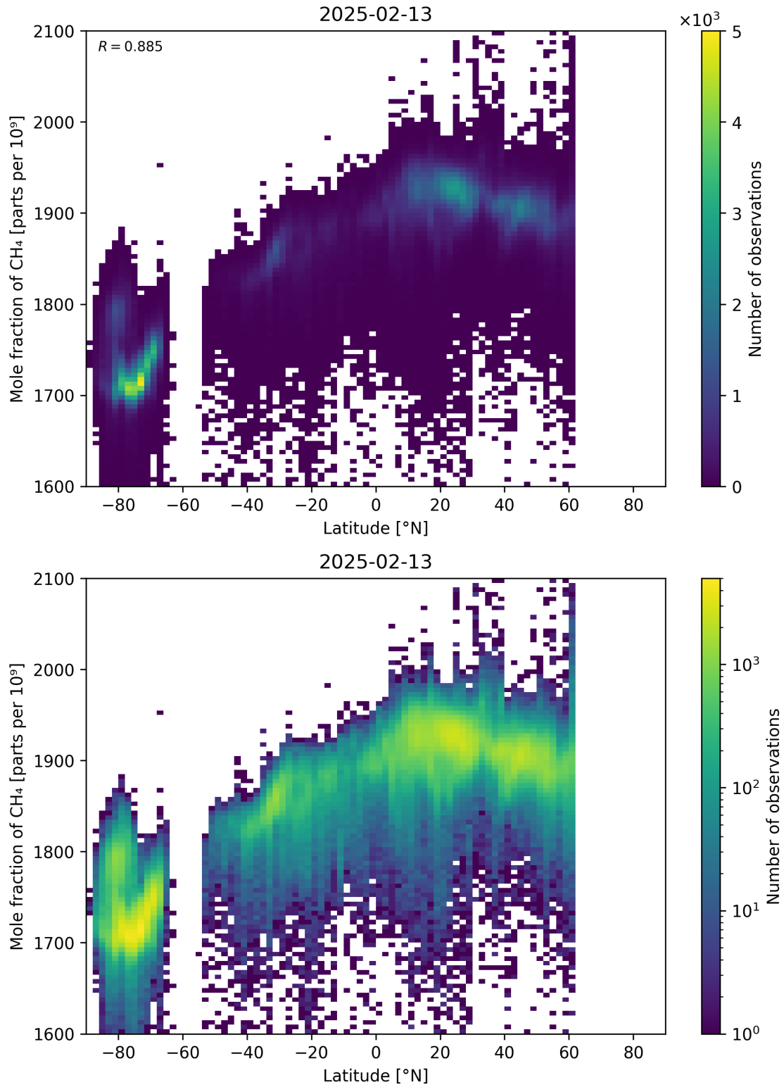
Figure 57: Scatter density plot of “Latitude” against “Mole fraction of CH 4 ” for 2025-02-13 to 2025-02-14.
