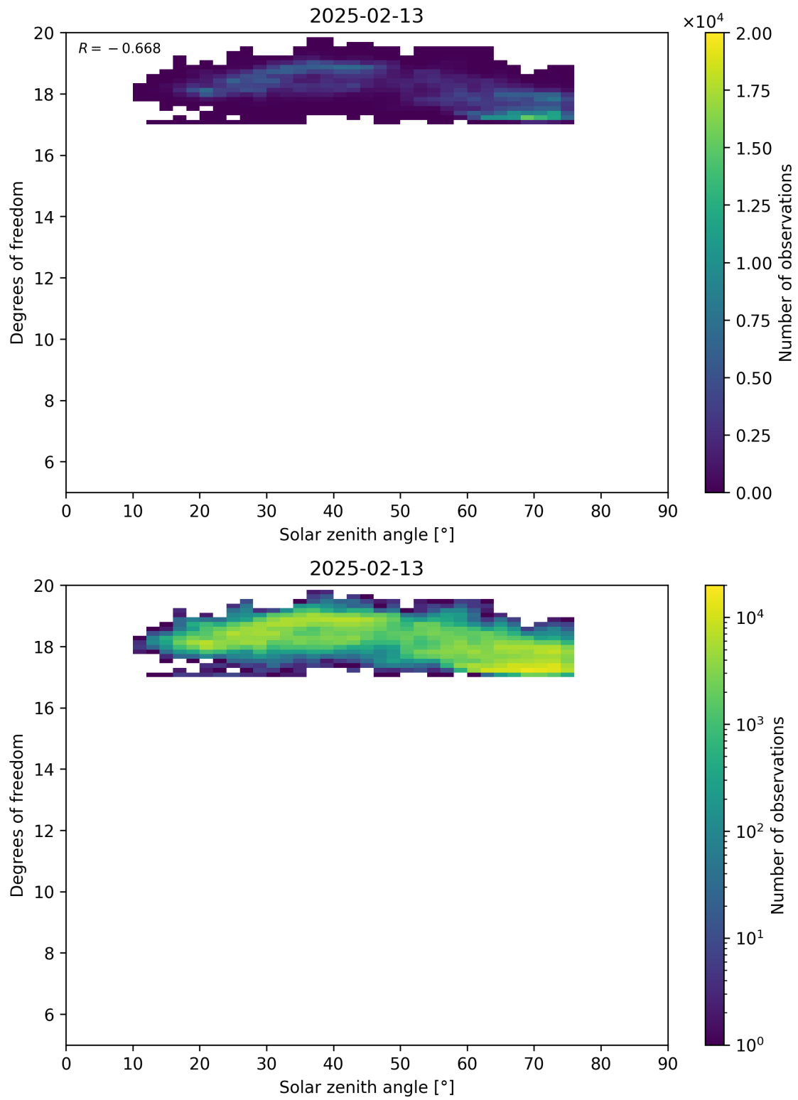
Figure 96: Scatter density plot of “Solar zenith angle” against “Degrees of freedom” for 2025-02-13 to 2025-02-14.
