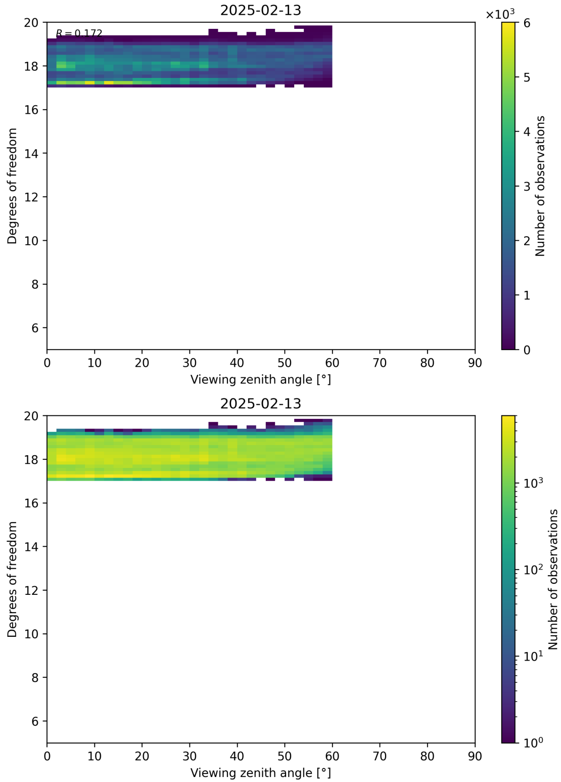
Figure 107: Scatter density plot of “Viewing zenith angle” against “Degrees of freedom” for 2025-02-13 to 2025-02-14.
