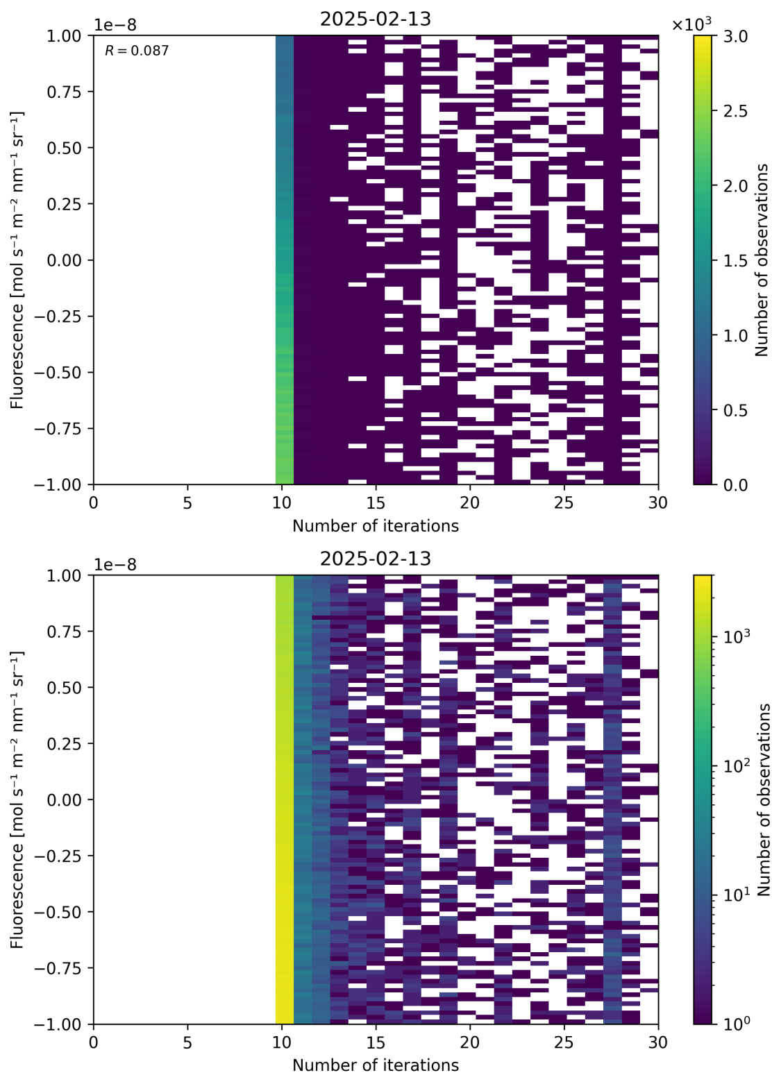
Figure 87: Scatter density plot of “Number of iterations” against “Fluorescence” for 2025-02-13 to 2025-02-14.
