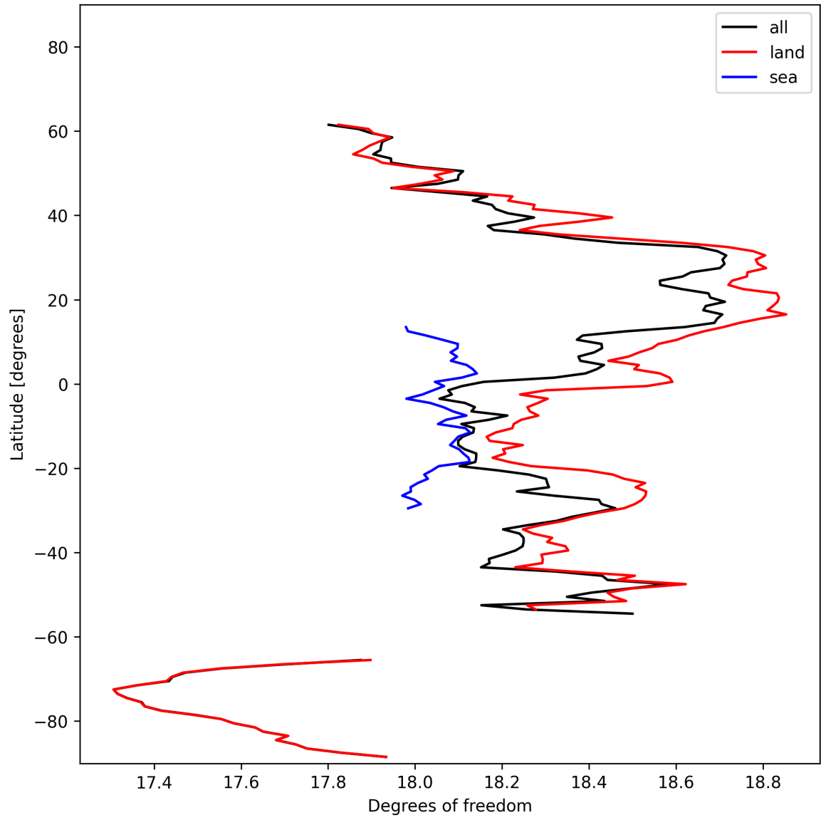
Figure 19: Zonal average of “Degrees of freedom” for 2025-02-13 to 2025-02-14.
