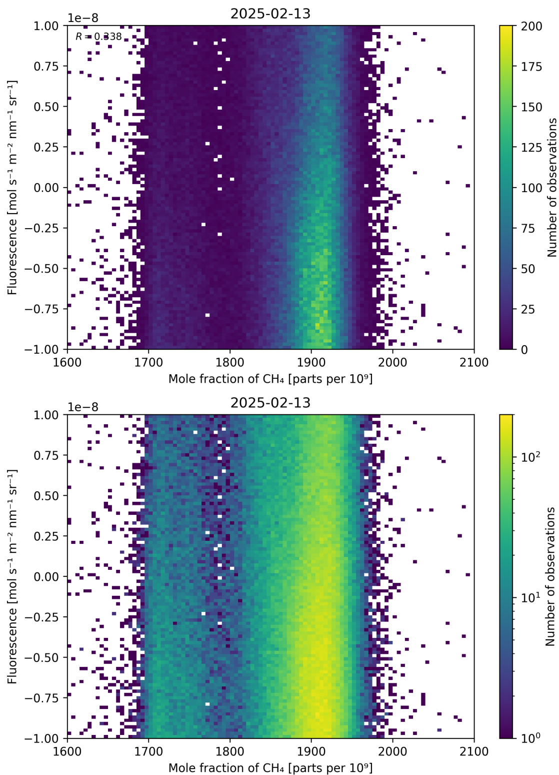
Figure 73: Scatter density plot of “Mole fraction of \text{CH}_4 ” against “Fluorescence” for 2025-02-13 to 2025-02-14.
