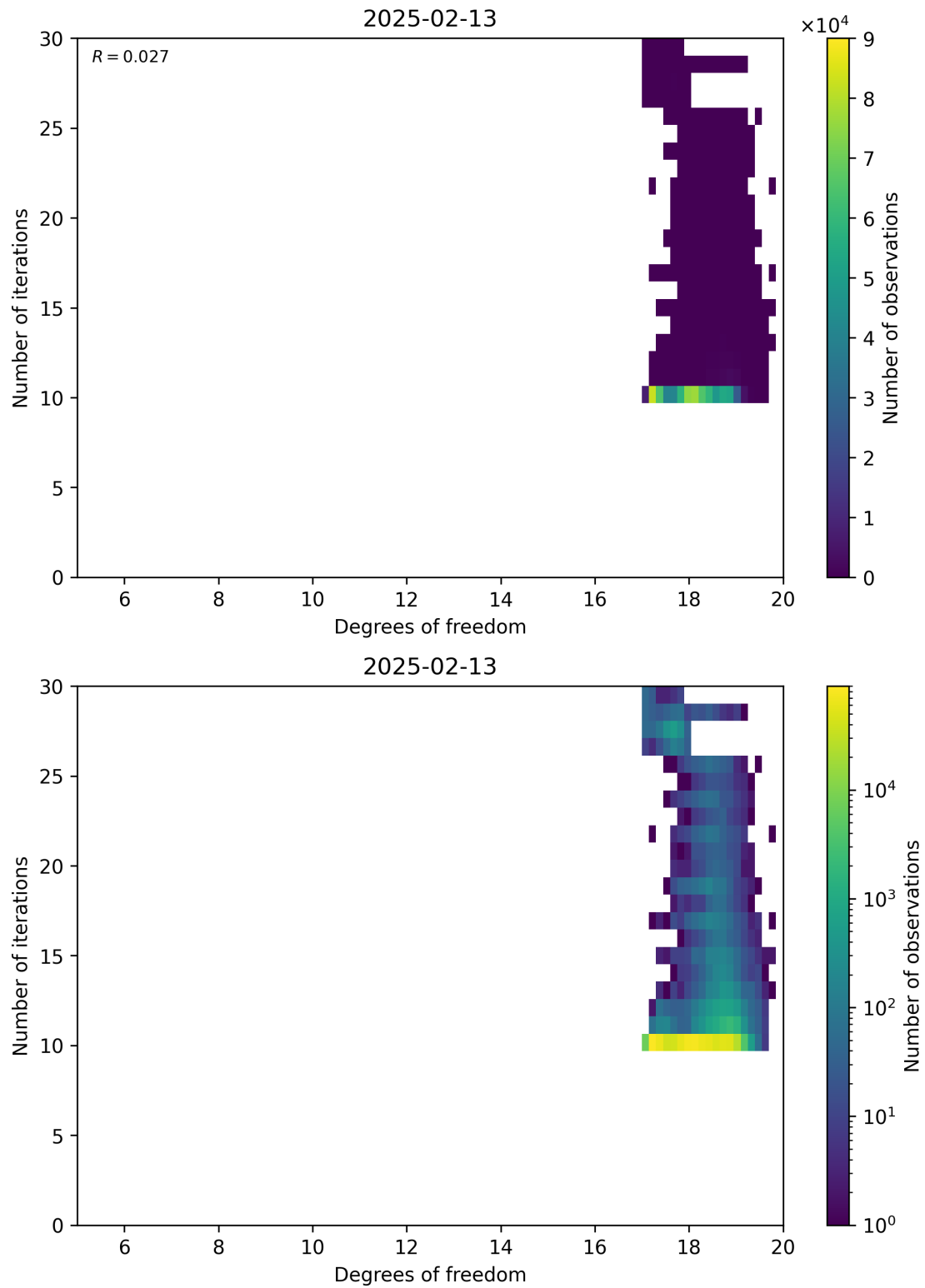
Figure 52: Scatter density plot of “Degrees of freedom” against “Number of iterations” for 2025-02-13 to 2025-02-14.
