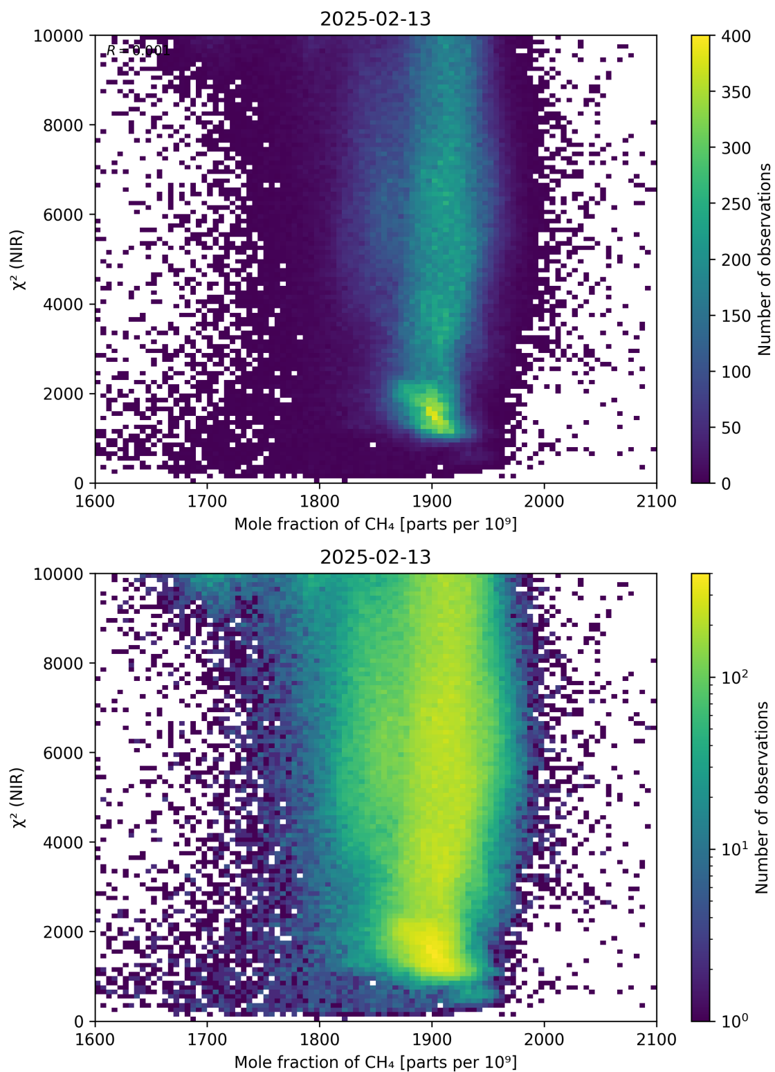
Figure 70: Scatter density plot of “Mole fraction of \text{CH}_4 ” against “ \chi^2 (NIR)” for 2025-02-13 to 2025-02-14.
