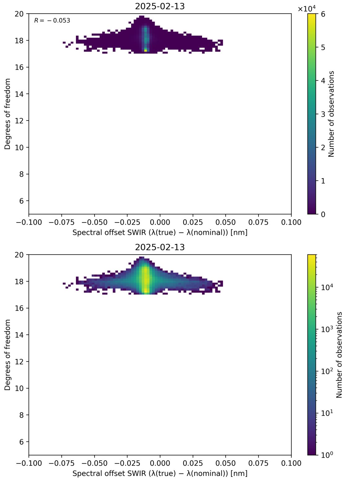
Figure 119: Scatter density plot of “Spectral offset SWIR ( \lambda_{\text{true}} - \lambda_{\text{nominal}} )” against “Degrees of freedom” for 2025-02-13 to 2025-02-14.
