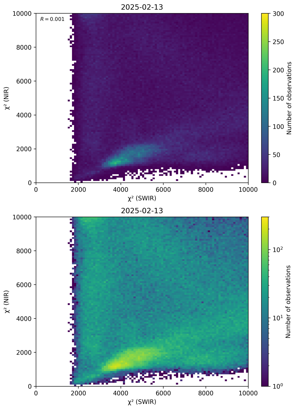
Figure 47: Scatter density plot of “ \chi^2 (SWIR)” against “ \chi^2 (NIR)” for 2025-02-13 to 2025-02-14.
