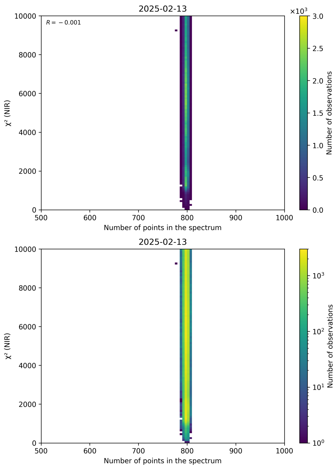
Figure 88: Scatter density plot of “Number of points in the spectrum” against “ \chi^2 (NIR)” for 2025-02-13 to 2025-02-14.
