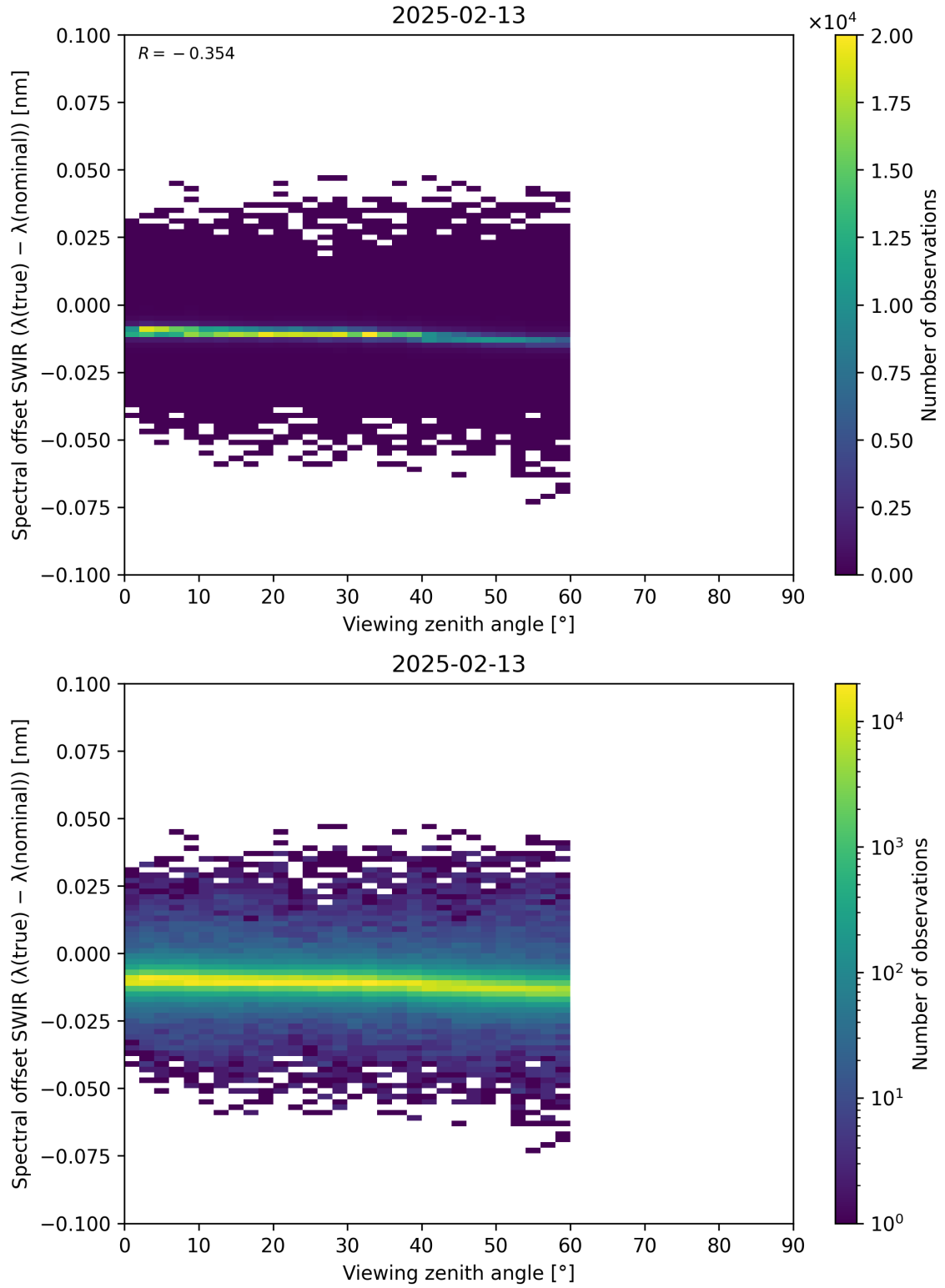
Figure 116: Scatter density plot of “Viewing zenith angle” against “Spectral offset SWIR ( \lambda_{\text{true}} - \lambda_{\text{nominal}} )” for 2025-02-13 to 2025-02-14.
