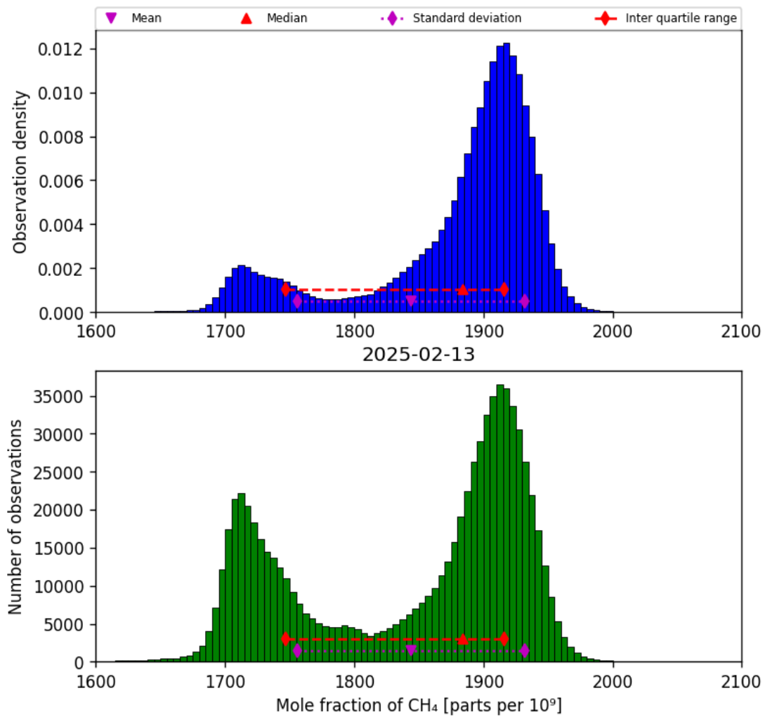
Figure 23: Histogram of “Mole fraction of CH 4 ” for 2025-02-13 to 2025-02-14
