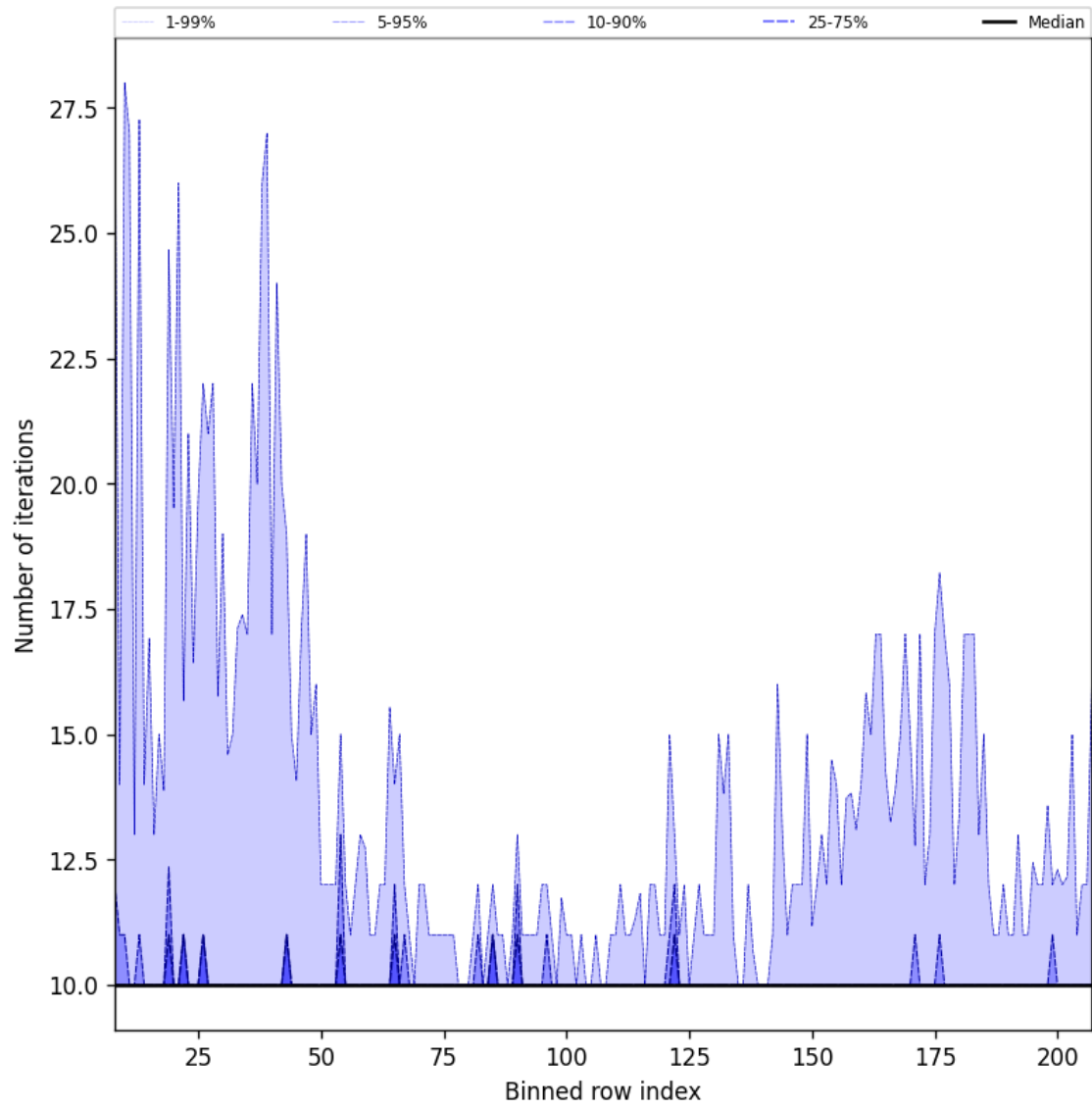
Figure 42: Along track statistics of “Number of iterations” for 2025-02-13 to 2025-02-14
