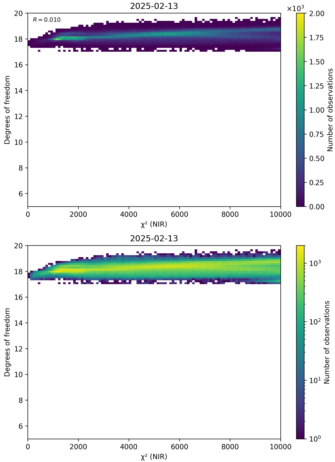
Figure 44: Scatter density plot of “ \chi^2 (NIR)” against “Degrees of freedom” for 2025-02-13 to 2025-02-14.
