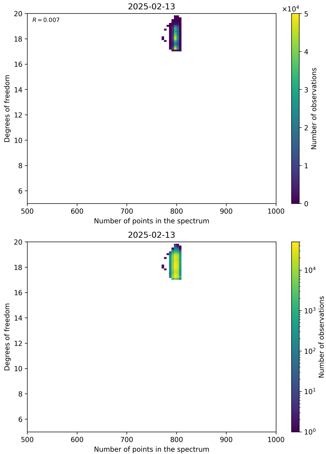
Figure 90: Scatter density plot of “Number of points in the spectrum” against “Degrees of freedom” for 2025-02-13 to 2025-02-14.
