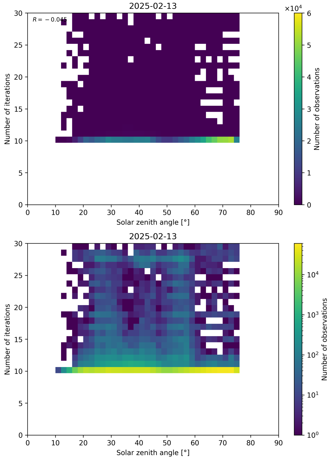
Figure 102: Scatter density plot of “Solar zenith angle” against “Number of iterations” for 2025-02-13 to 2025-02-14.
