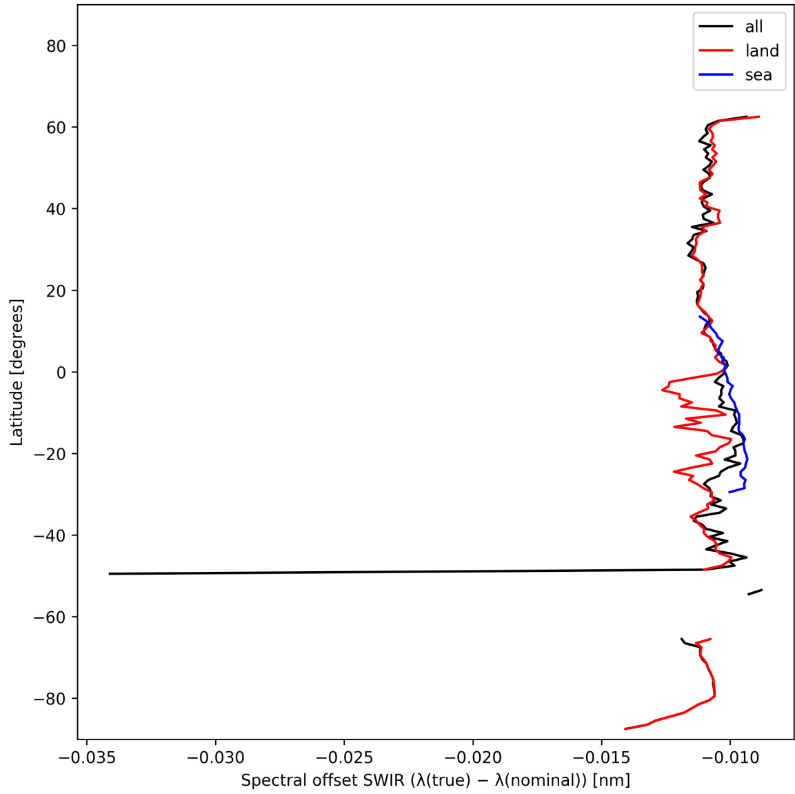
Figure 16: Zonal average of “Spectral offset SWIR ( \lambda_{\text{true}} - \lambda_{\text{nominal}} )” for 2025-02-13 to 2025-02-15.
