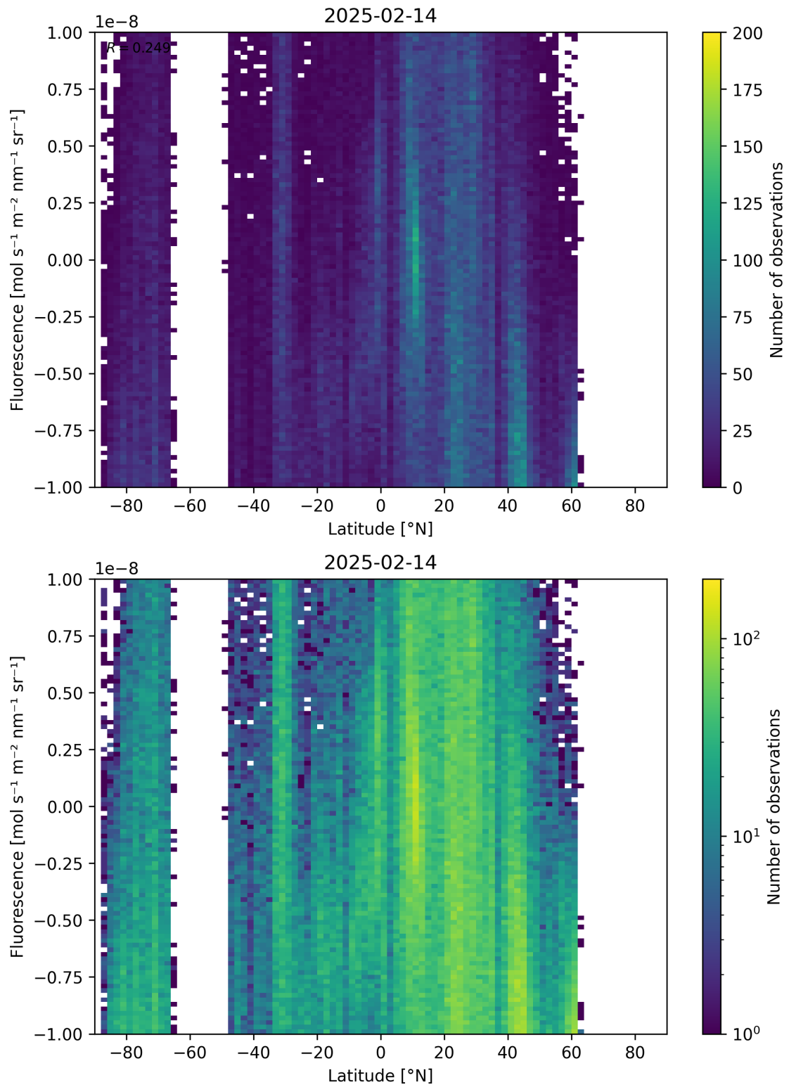
Figure 56: Scatter density plot of “Latitude” against “Fluorescence” for 2025-02-13 to 2025-02-15.
