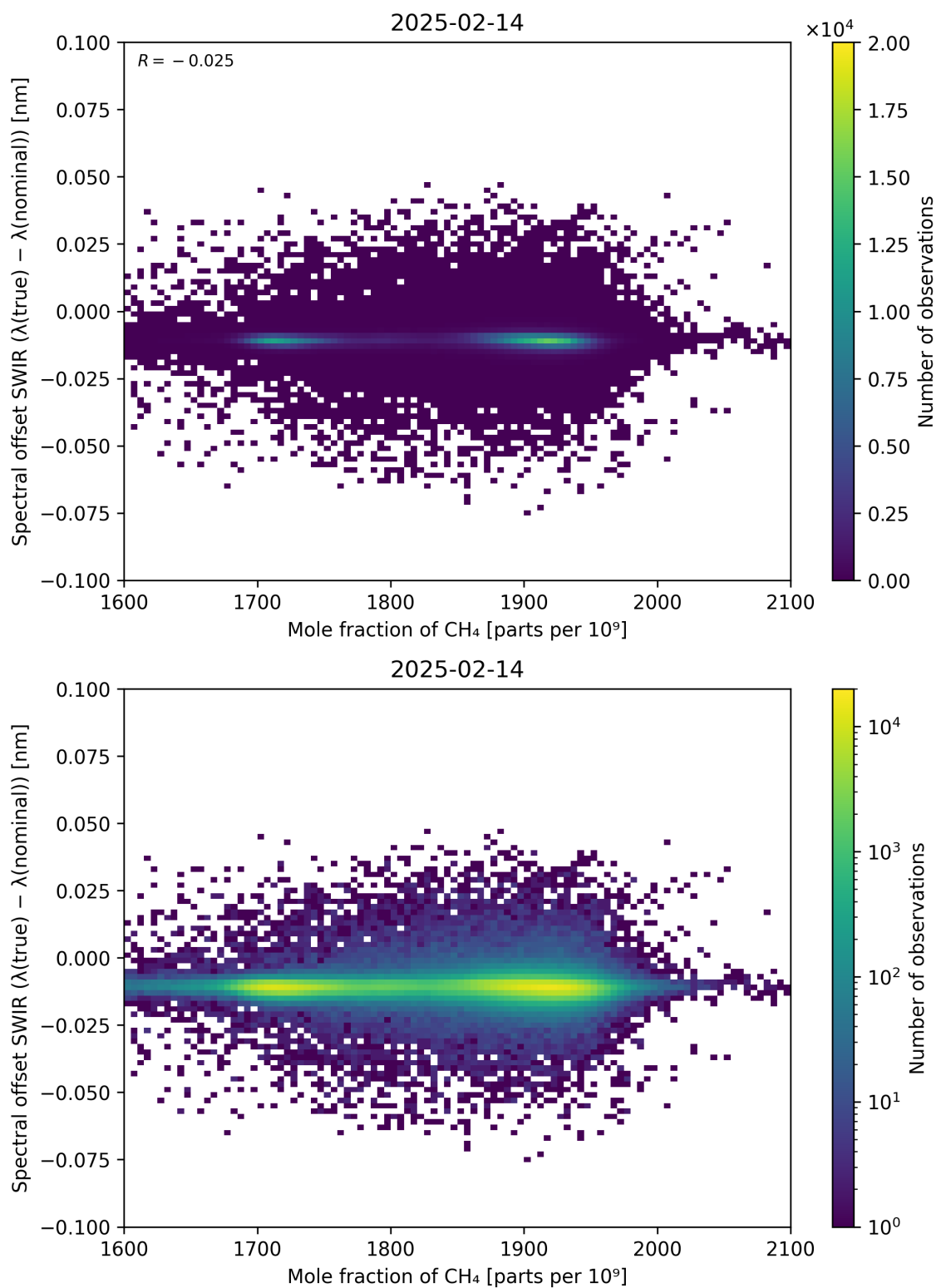
Figure 86: Scatter density plot of “Mole fraction of CH 4 ” against “Spectral offset SWIR ( \lambda_{\text{true}} - \lambda_{\text{nominal}} )” for 2025-02-13 to 2025-02-15.
