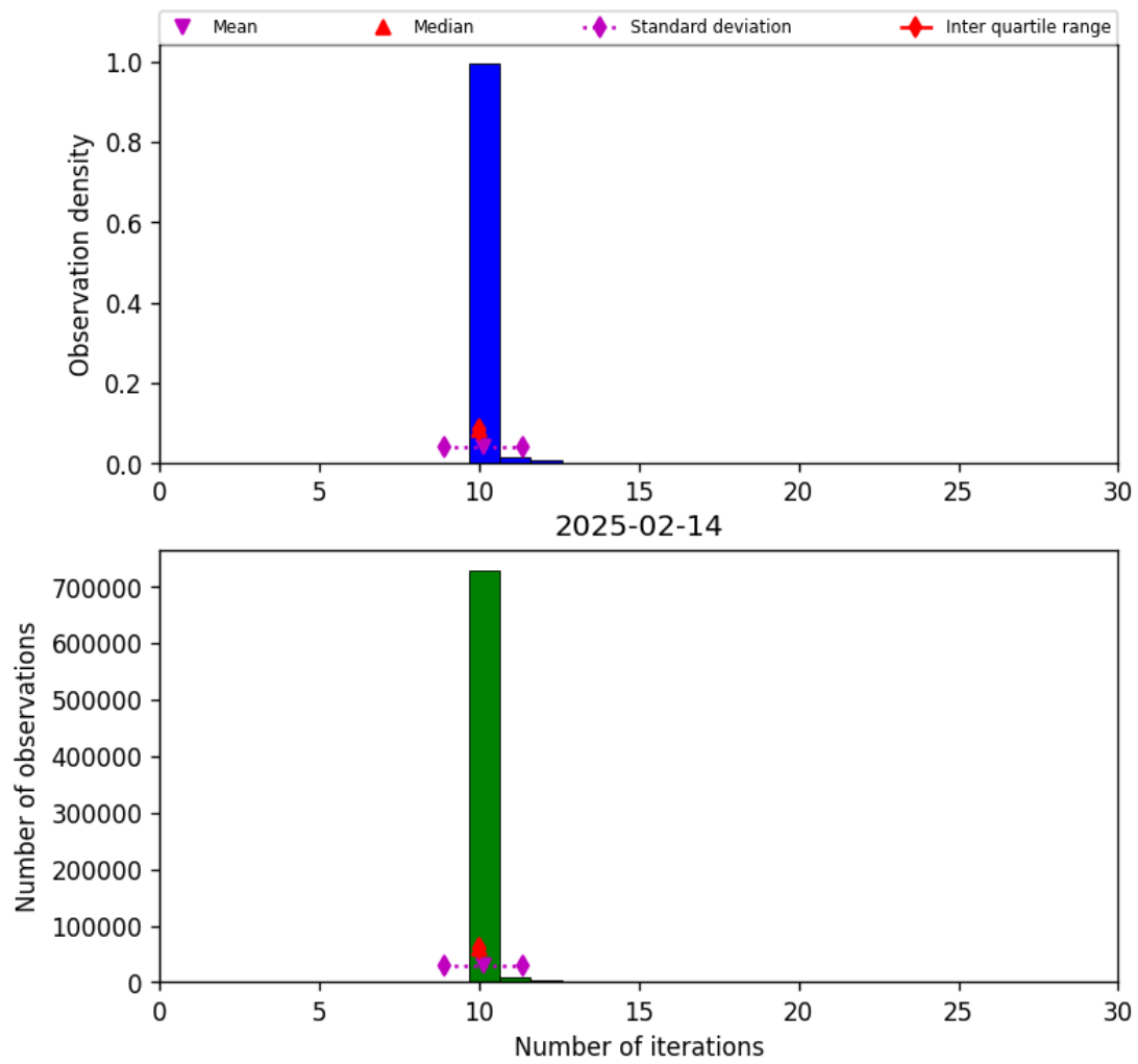
Figure 31: Histogram of “Number of iterations” for 2025-02-13 to 2025-02-15
