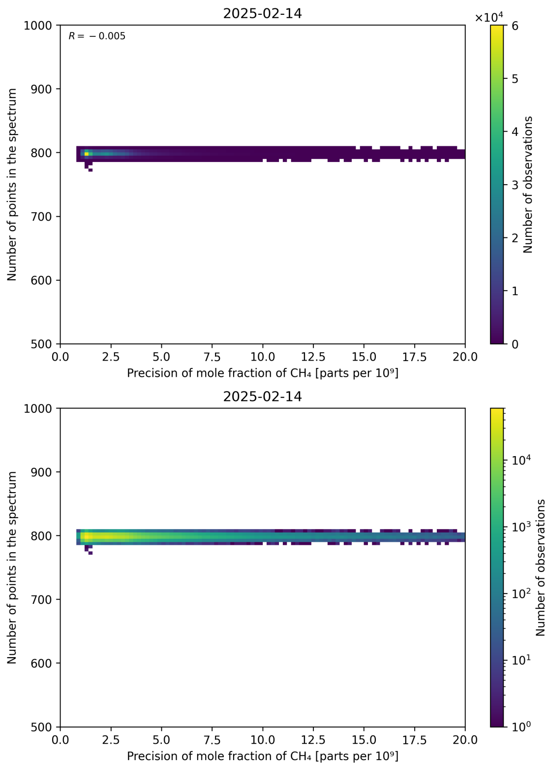
Figure 84: Scatter density plot of “Precision of mole fraction of CH 4 ” against “Number of points in the spectrum” for 2025-02-13 to 2025-02-15.
