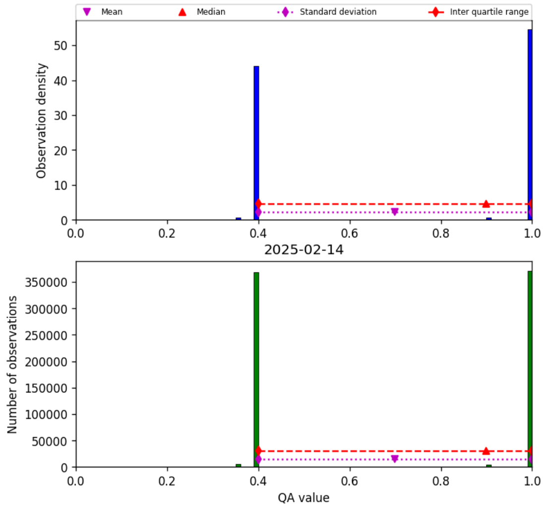
Figure 22: Histogram of “QA value” for 2025-02-13 to 2025-02-15
