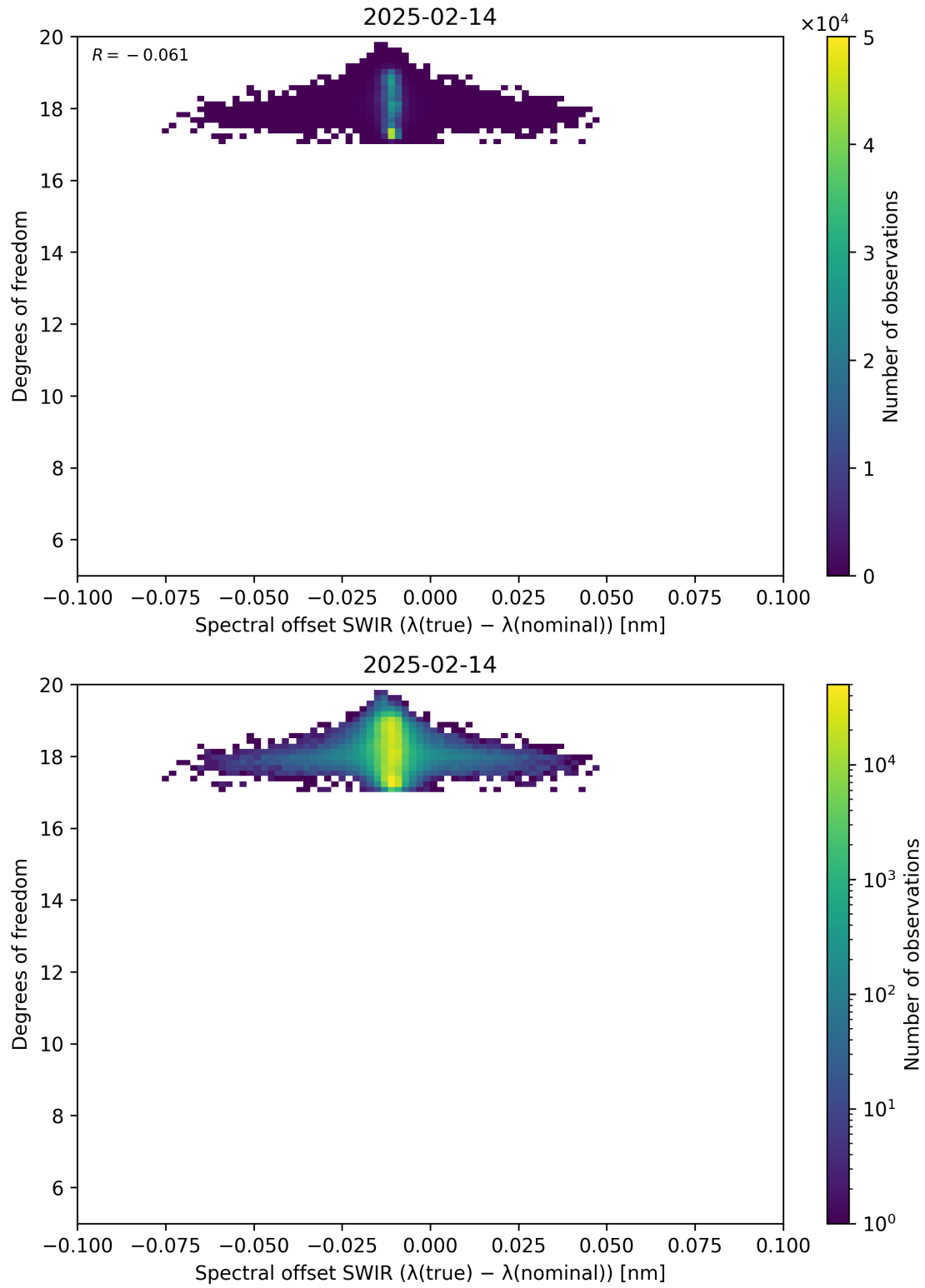
Figure 119: Scatter density plot of “Spectral offset SWIR ( \lambda_{\text{true}} - \lambda_{\text{nominal}} )” against “Degrees of freedom” for 2025-02-13 to 2025-02-15.
