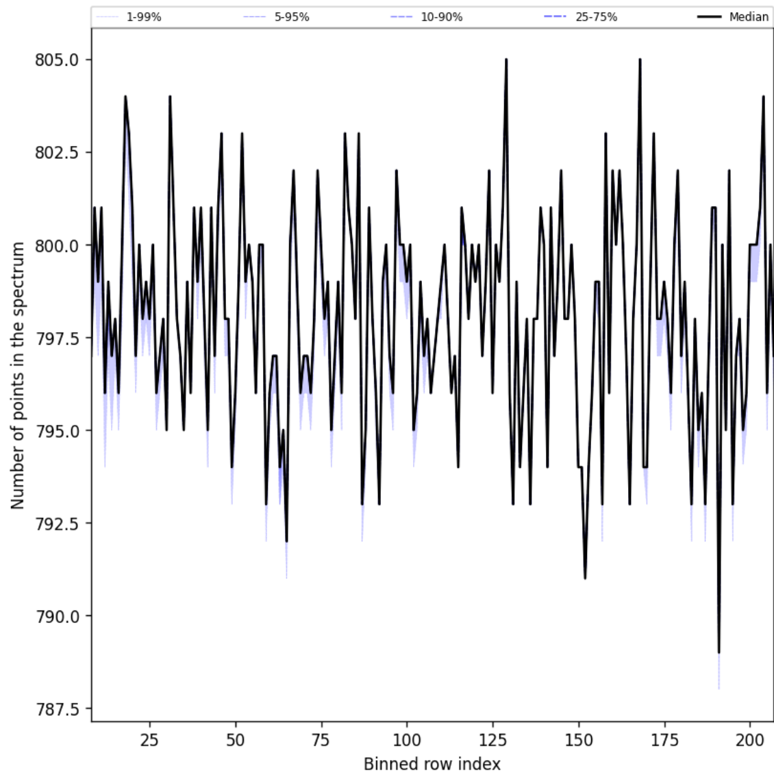
Figure 37: Along track statistics of “Number of points in the spectrum” for 2025-02-13 to 2025-02-15
