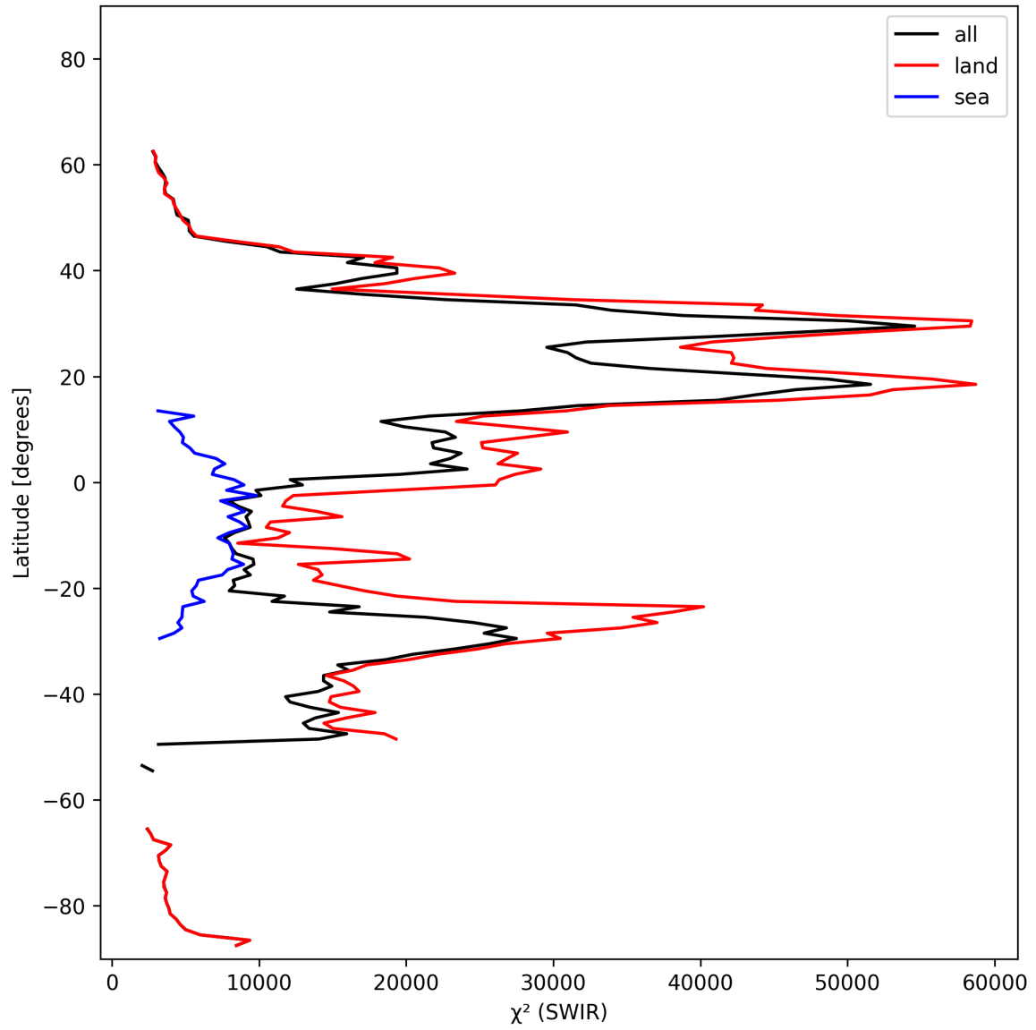
Figure 17: Zonal average of “ \chi^2 (SWIR)” for 2025-02-13 to 2025-02-15.
