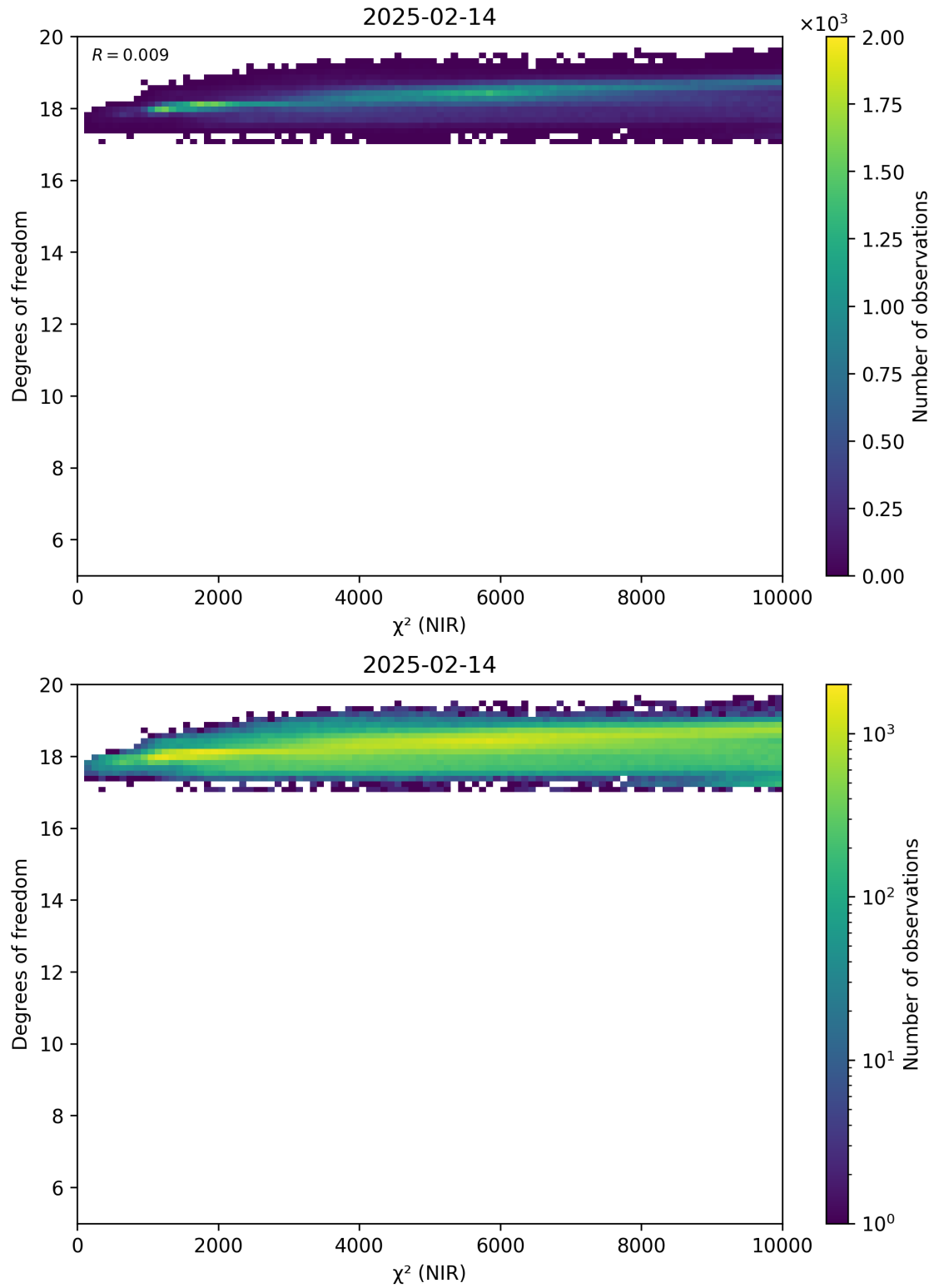
Figure 44: Scatter density plot of “ \chi^2 (NIR)” against “Degrees of freedom” for 2025-02-13 to 2025-02-15.
