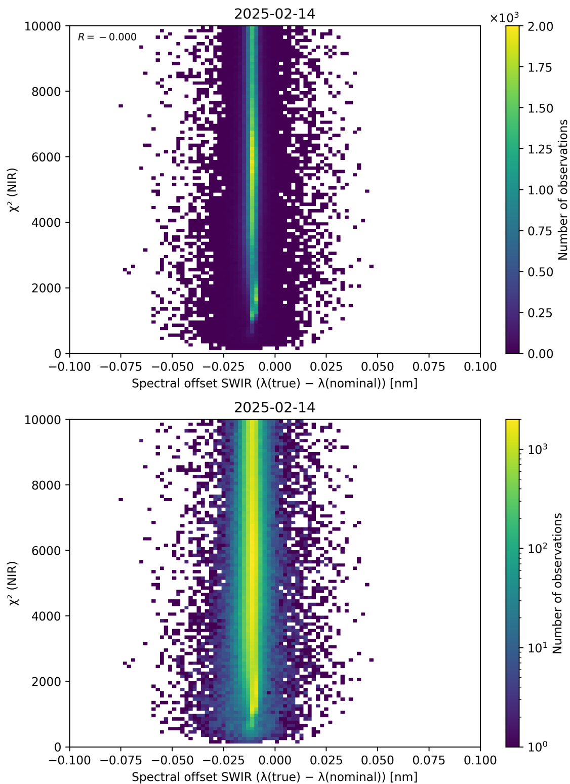
Figure 117: Scatter density plot of “Spectral offset SWIR ( \lambda_{\text{true}} - \lambda_{\text{nominal}} )” against “ \chi^2 (NIR)” for 2025-02-13 to 2025-02-15.
