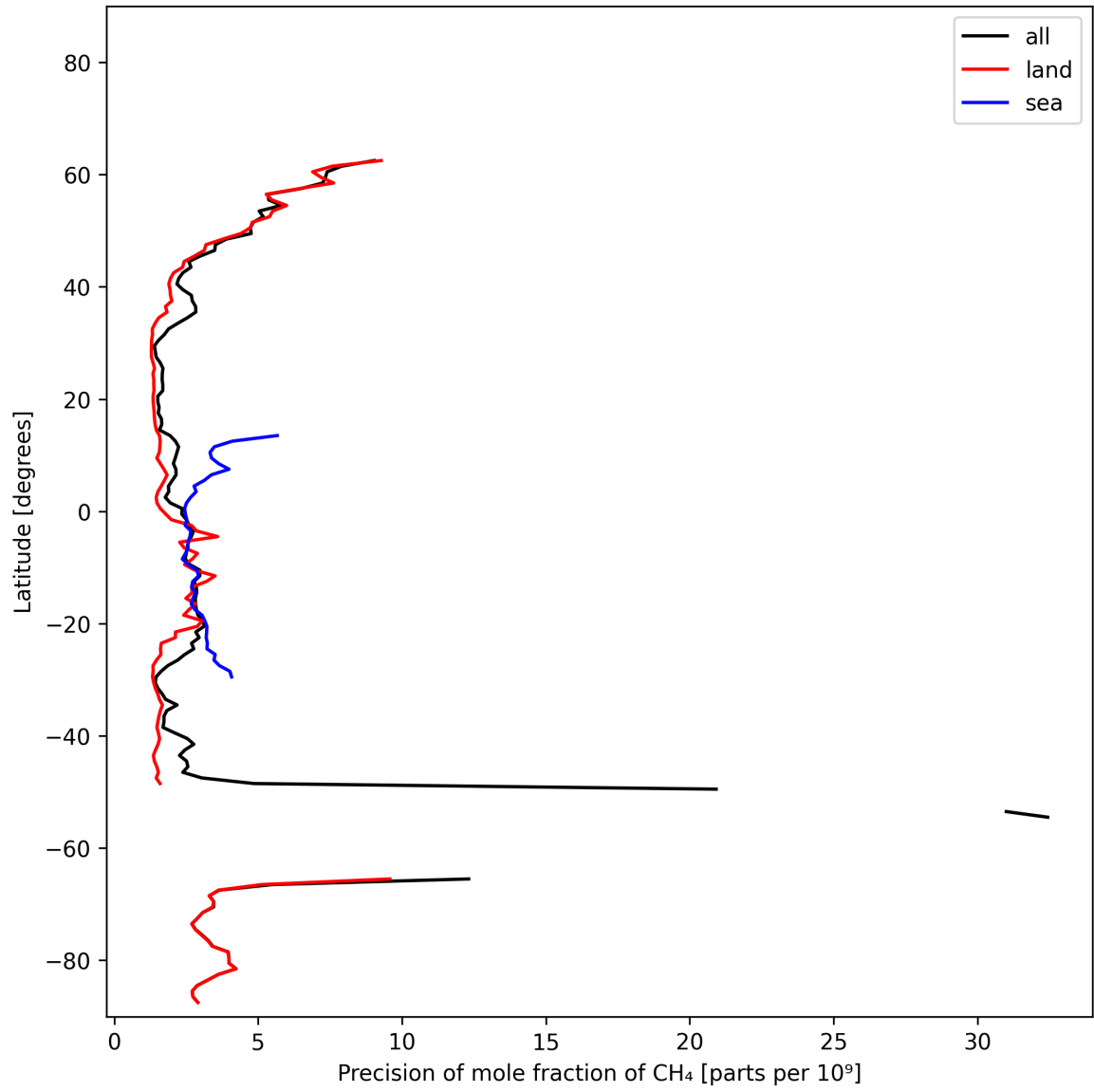
Figure 13: Zonal average of “Precision of mole fraction of CH 4 ” for 2025-02-13 to 2025-02-15.
