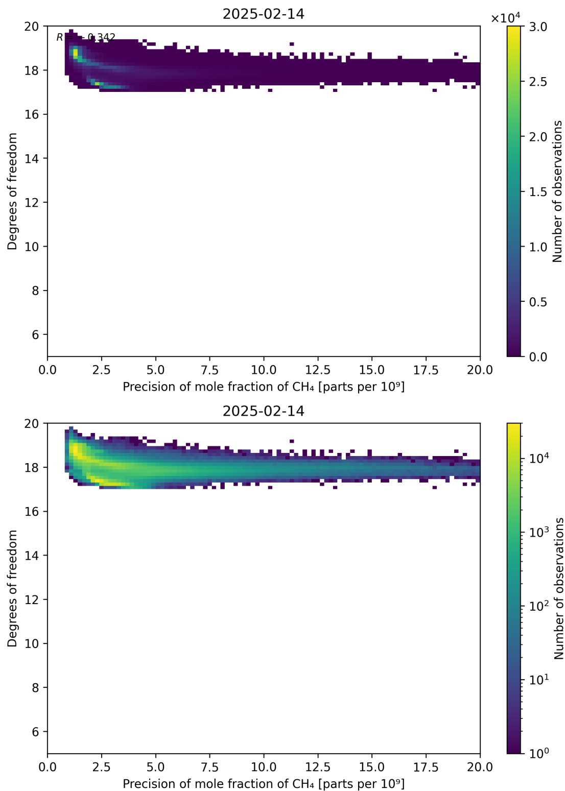
Figure 80: Scatter density plot of “Precision of mole fraction of CH 4 ” against “Degrees of freedom” for 2025-02-13 to 2025-02-15.
