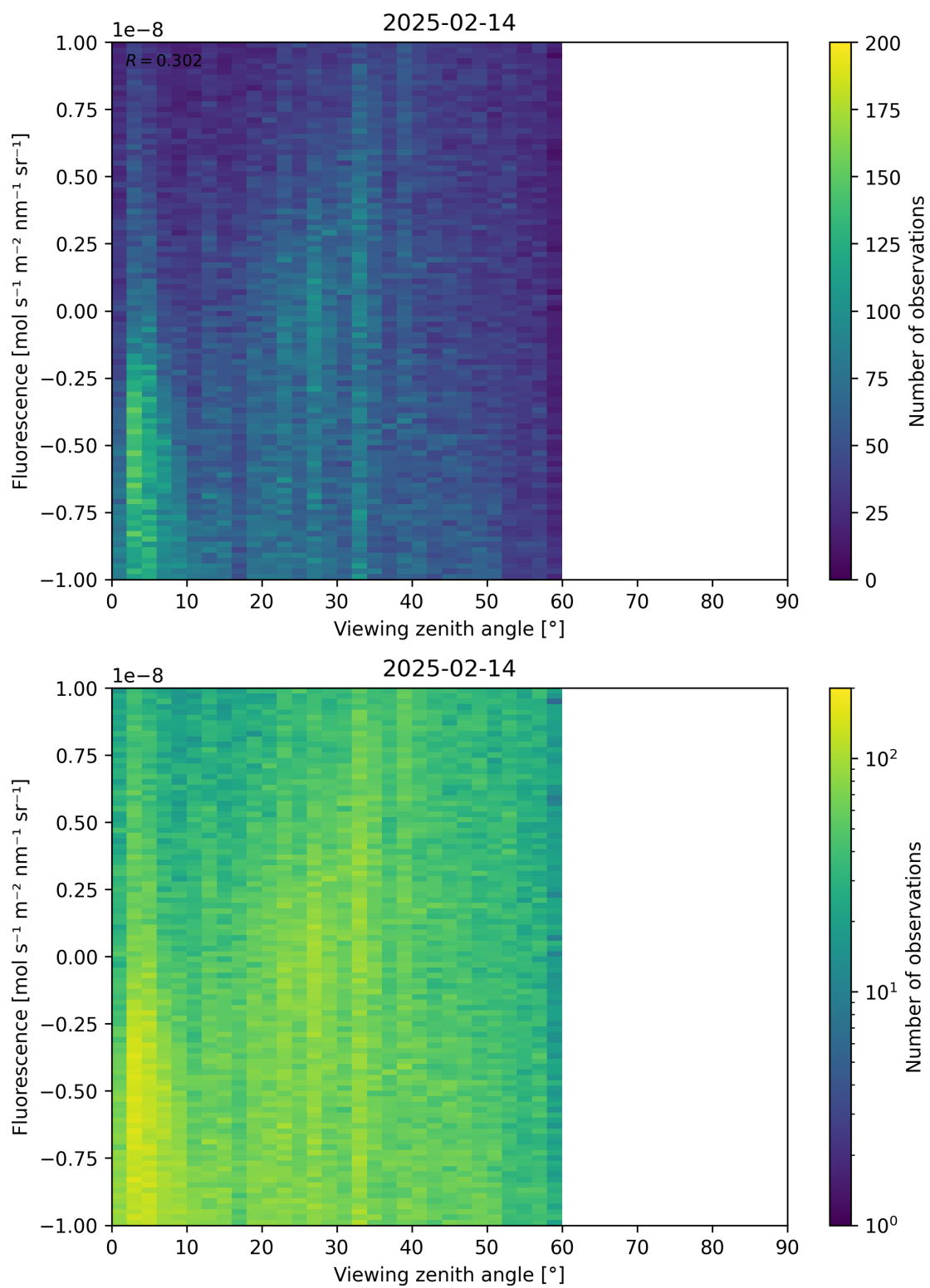
Figure 108: Scatter density plot of “Viewing zenith angle” against “Fluorescence” for 2025-02-13 to 2025-02-15.
