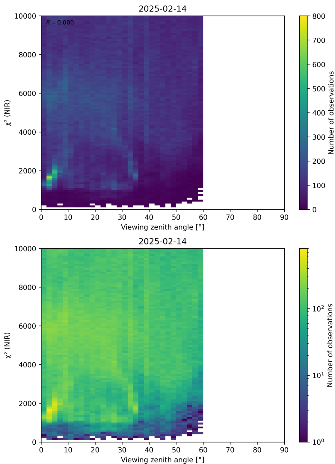
Figure 105: Scatter density plot of “Viewing zenith angle” against “ \chi^2 (NIR)” for 2025-02-13 to 2025-02-15.
