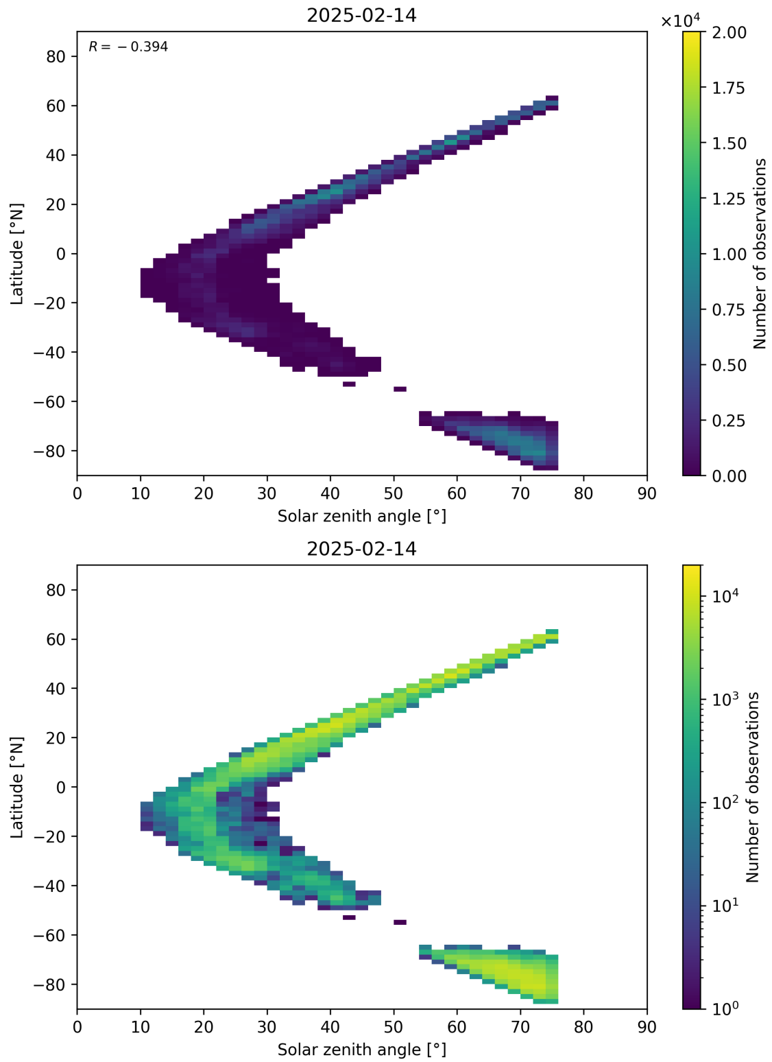
Figure 98: Scatter density plot of “Solar zenith angle” against “Latitude” for 2025-02-13 to 2025-02-15.
