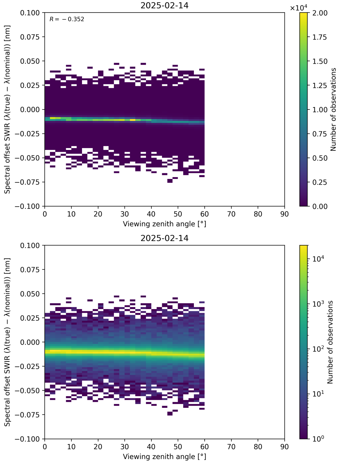
Figure 116: Scatter density plot of “Viewing zenith angle” against “Spectral offset SWIR ( \lambda_{\text{true}} - \lambda_{\text{nominal}} )” for 2025-02-13 to 2025-02-15.
