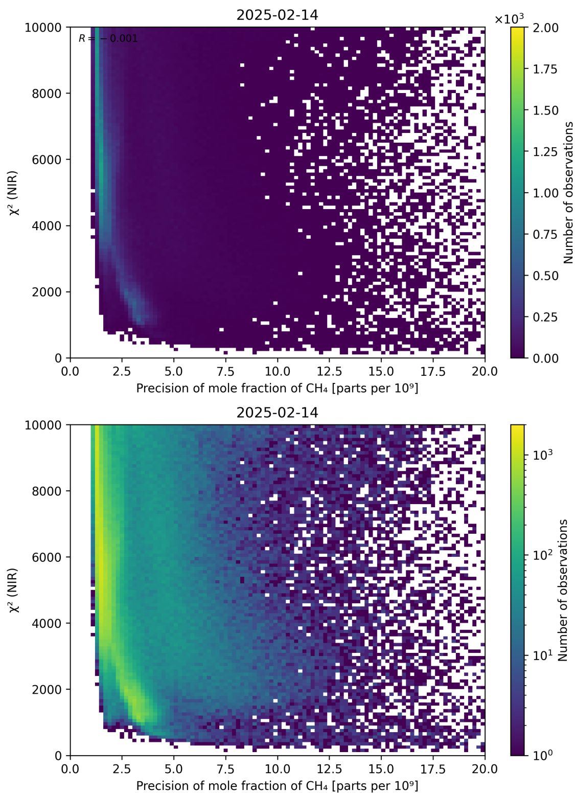
Figure 78: Scatter density plot of “Precision of mole fraction of CH 4 ” against “ \chi^2 (NIR)” for 2025-02-13 to 2025-02-15.
