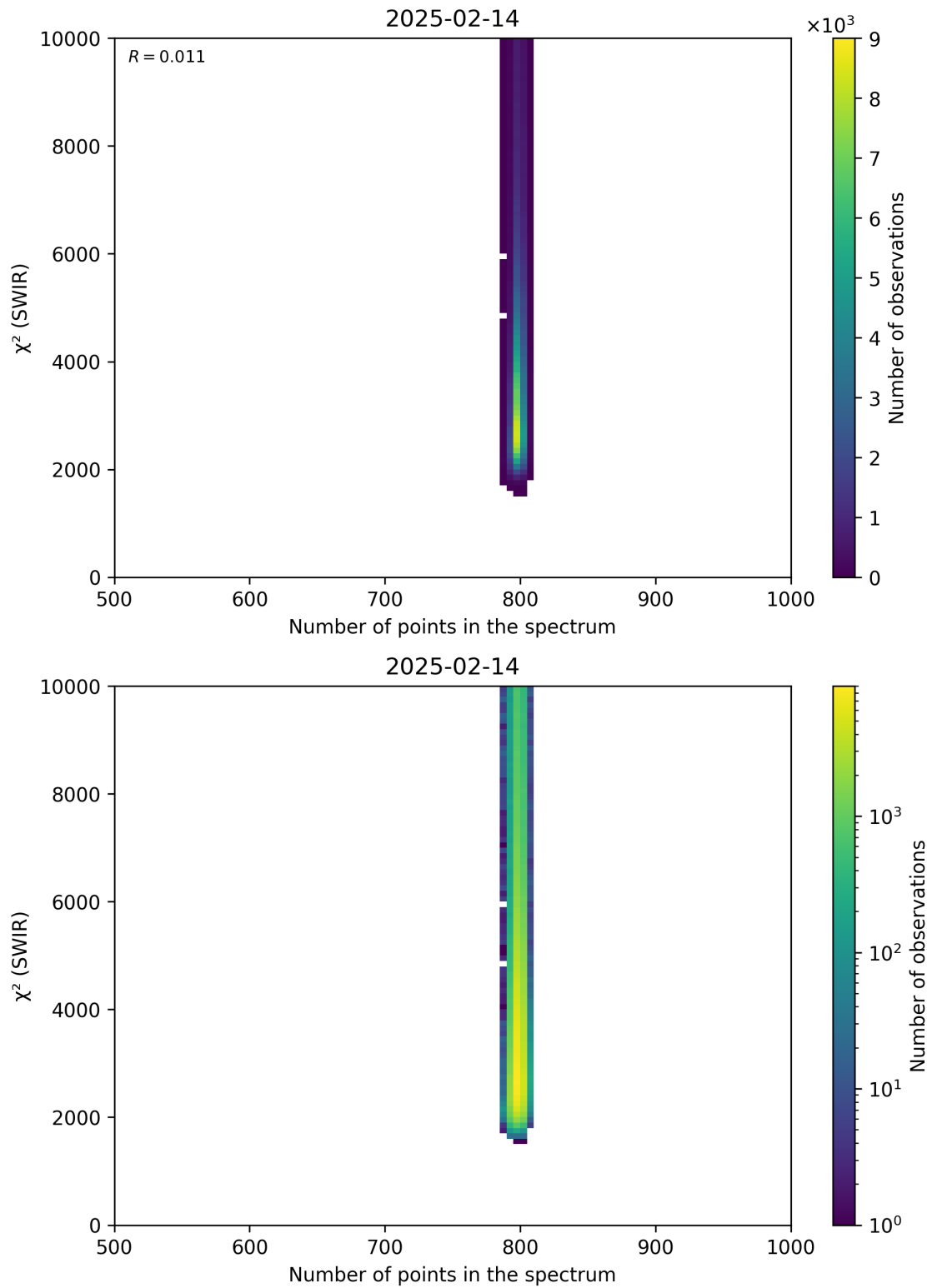
Figure 89: Scatter density plot of “Number of points in the spectrum” against “ \chi^2 (SWIR)” for 2025-02-13 to 2025-02-15.
