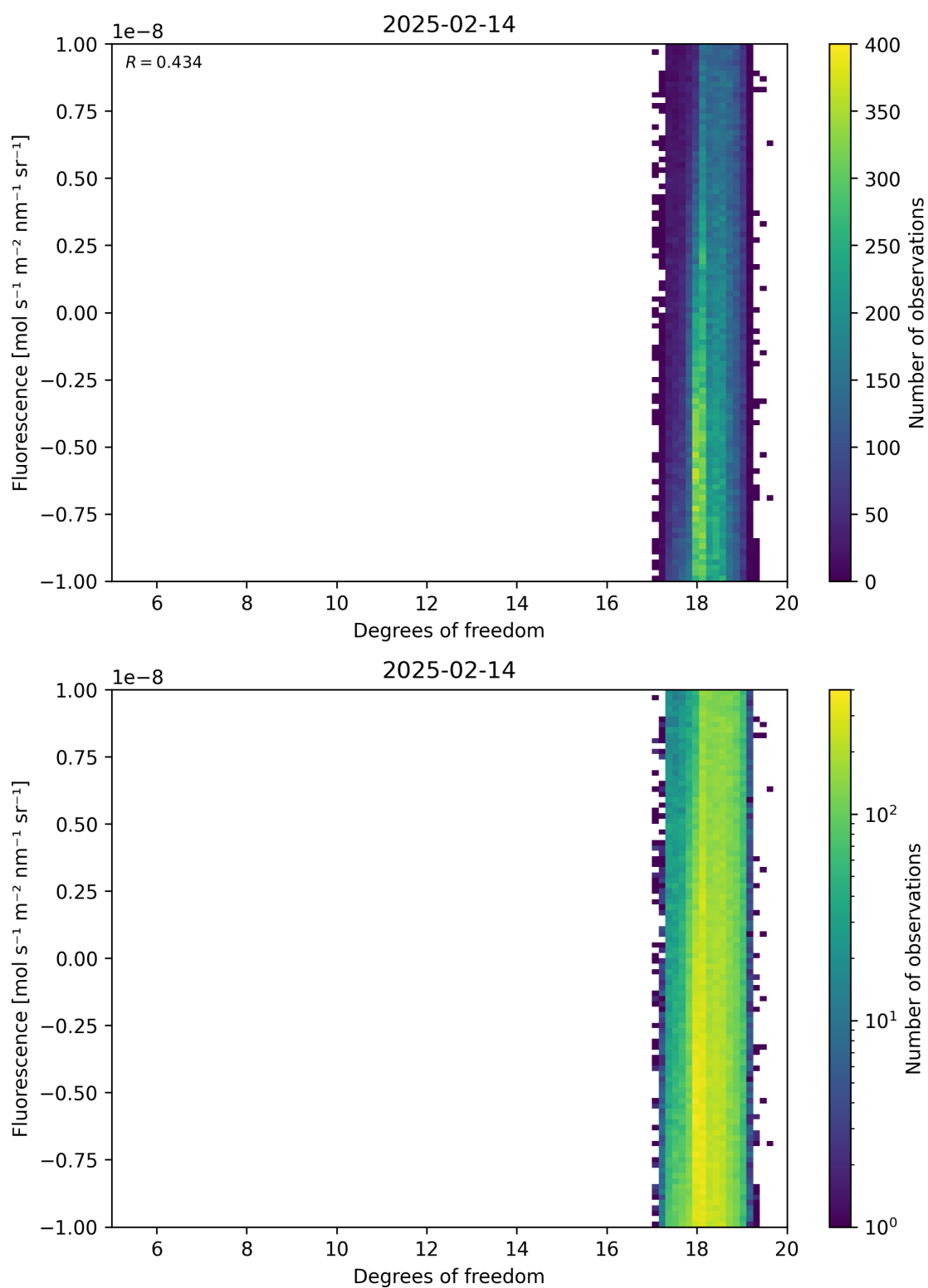
Figure 51: Scatter density plot of “Degrees of freedom” against “Fluorescence” for 2025-02-13 to 2025-02-15.
