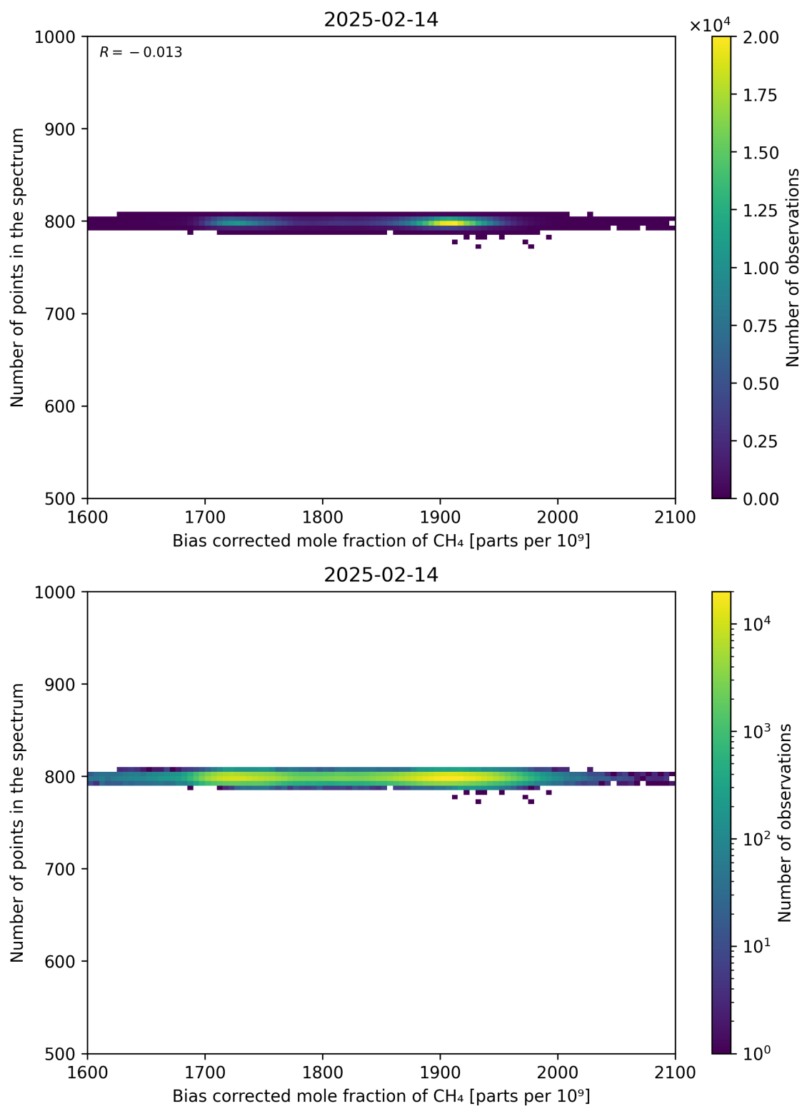
Figure 68: Scatter density plot of “Bias corrected mole fraction of CH 4 ” against “Number of points in the spectrum” for 2025-02-13 to 2025-02-15.
