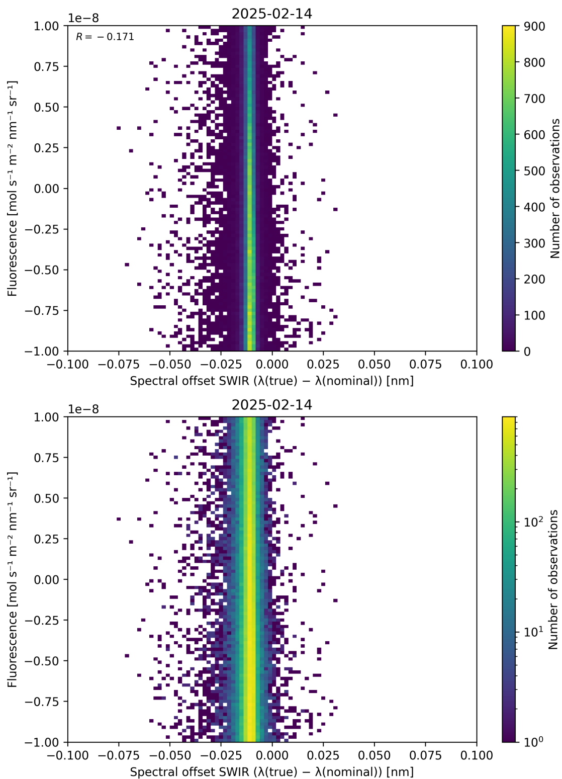
Figure 120: Scatter density plot of “Spectral offset SWIR ( \lambda_{\text{true}} - \lambda_{\text{nominal}} )” against “Fluorescence” for 2025-02-13 to 2025-02-15.
