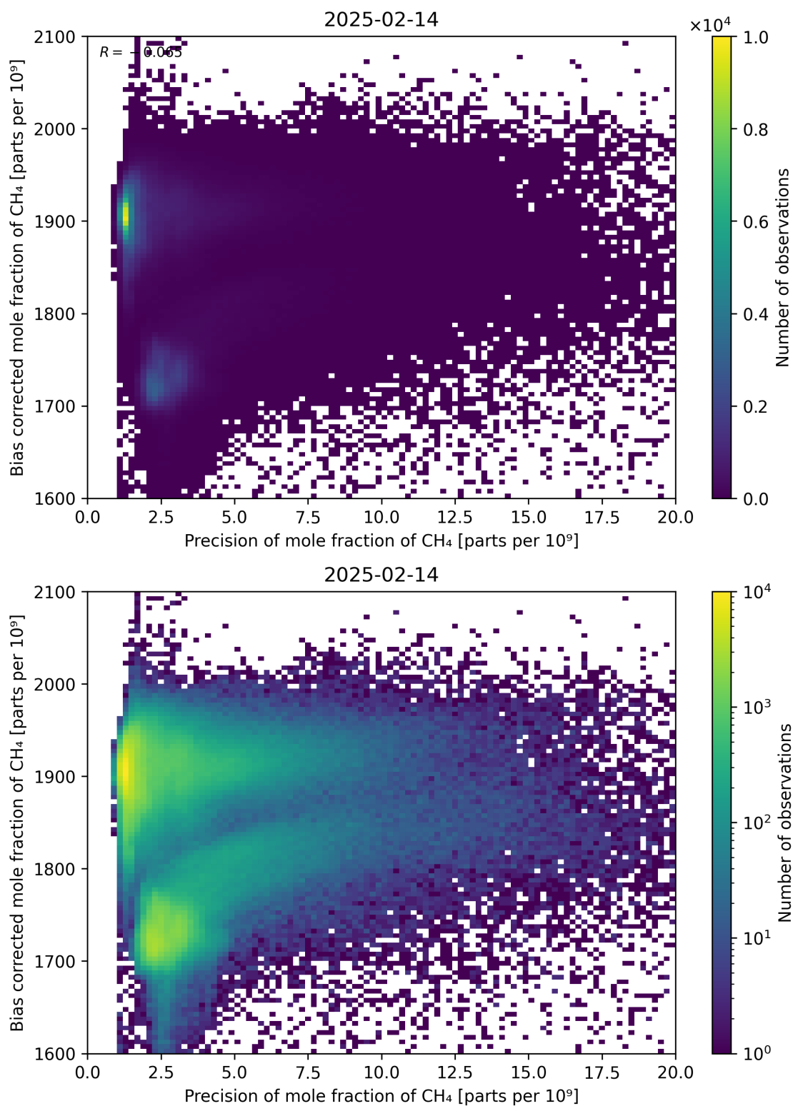
Figure 82: Scatter density plot of “Precision of mole fraction of CH 4 ” against “Bias corrected mole fraction of CH 4 ” for 2025-02-13 to 2025-02-15.
