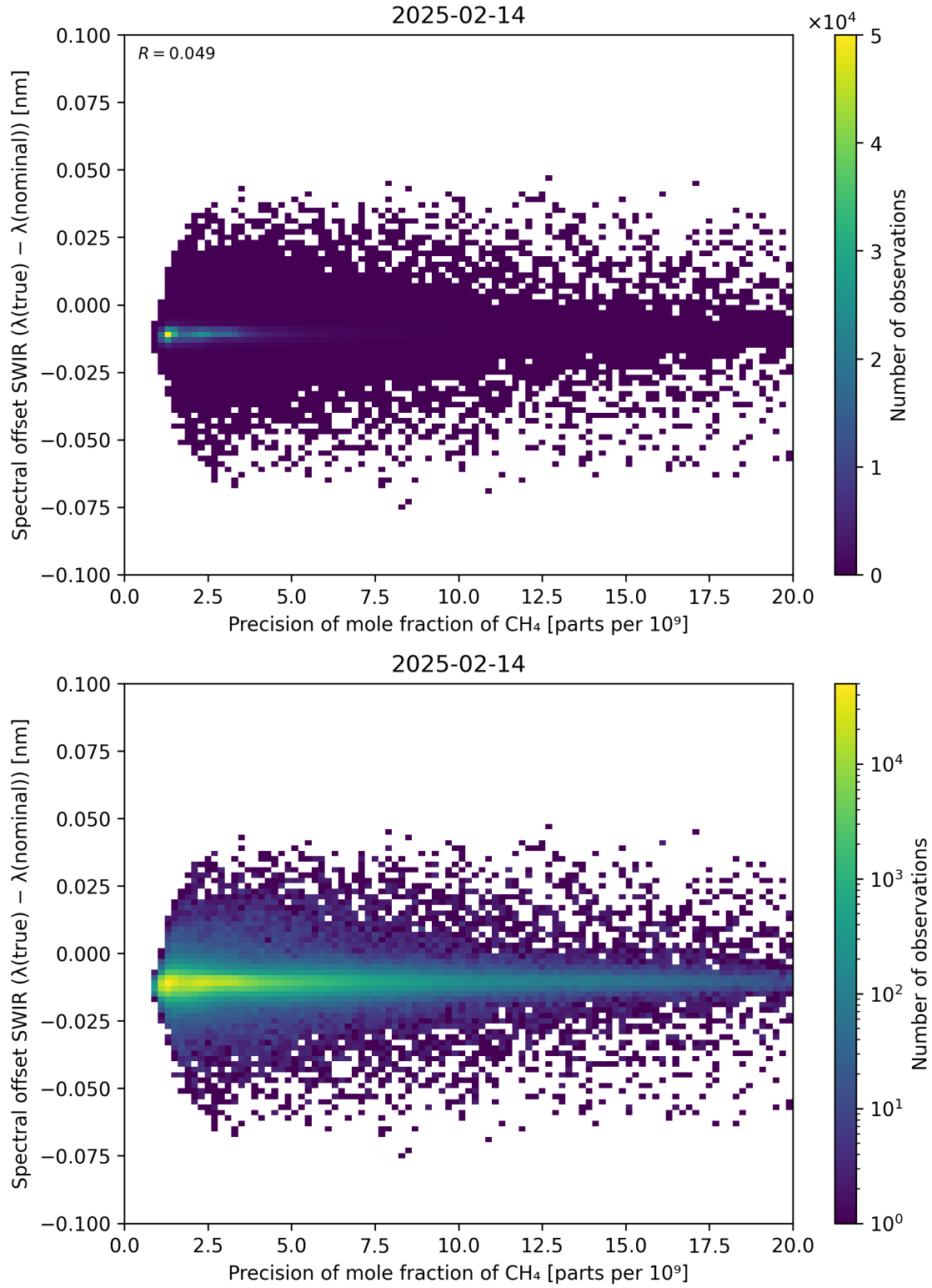
Figure 85: Scatter density plot of “Precision of mole fraction of CH 4 ” against “Spectral offset SWIR ( \lambda_{\text{true}} - \lambda_{\text{nominal}} )” for 2025-02-13 to 2025-02-15.
