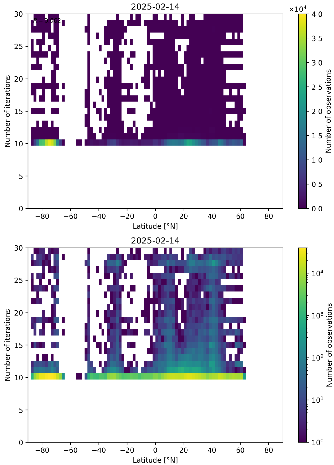
Figure 60: Scatter density plot of “Latitude” against “Number of iterations” for 2025-02-13 to 2025-02-15.
