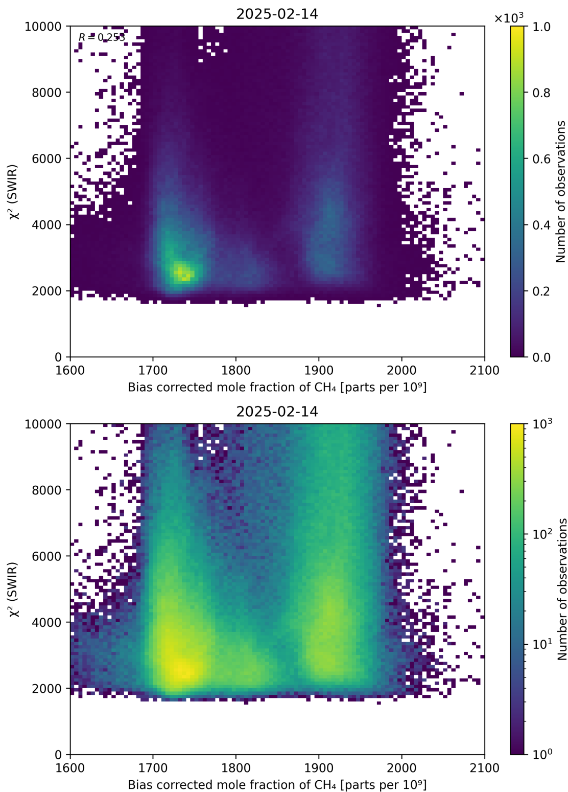
Figure 64: Scatter density plot of “Bias corrected mole fraction of \text{CH}_4 ” against “ \chi^2 (SWIR)” for 2025-02-13 to 2025-02-15.
