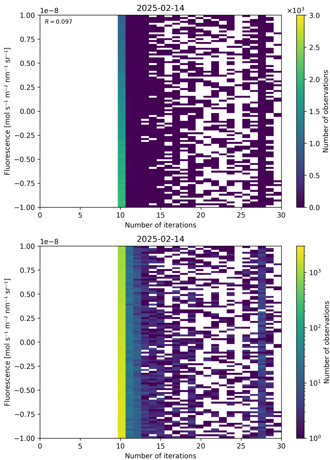
Figure 87: Scatter density plot of “Number of iterations” against “Fluorescence” for 2025-02-13 to 2025-02-15.
