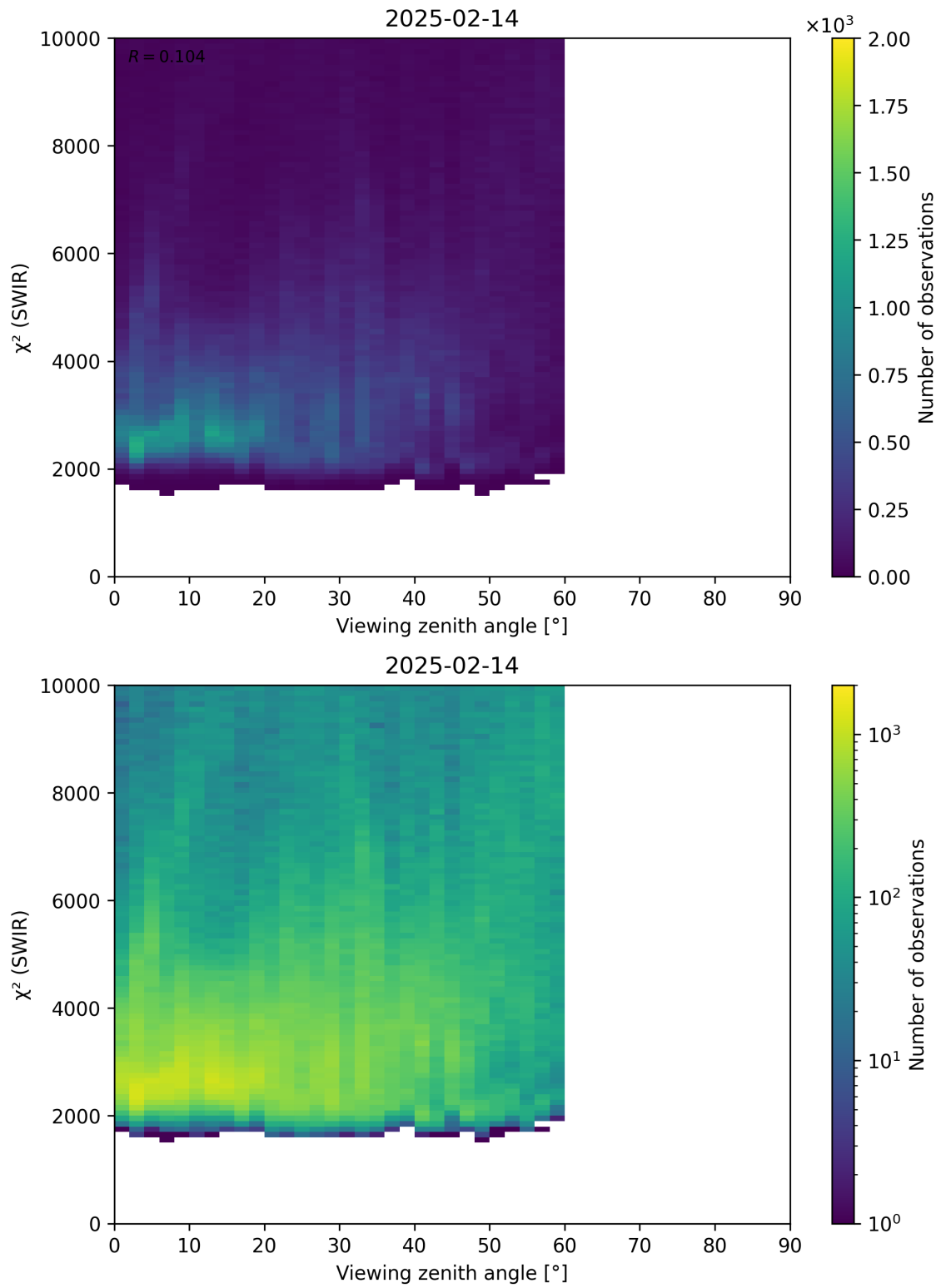
Figure 106: Scatter density plot of “Viewing zenith angle” against “ \chi^2 (SWIR)” for 2025-02-13 to 2025-02-15.
