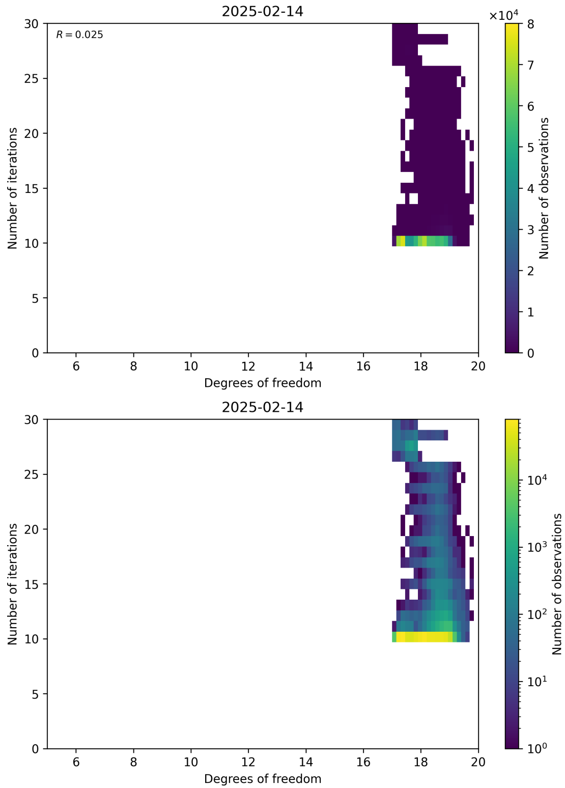
Figure 52: Scatter density plot of “Degrees of freedom” against “Number of iterations” for 2025-02-13 to 2025-02-15.
