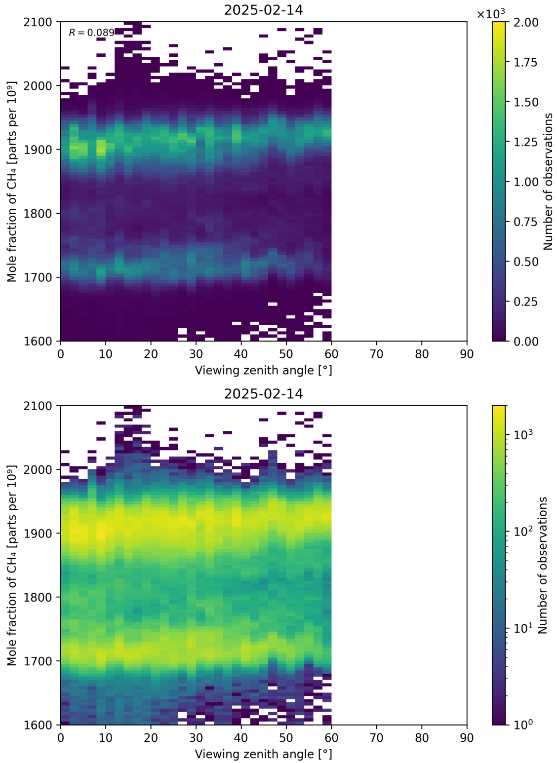
Figure 110: Scatter density plot of “Viewing zenith angle” against “Mole fraction of CH 4 ” for 2025-02-13 to 2025-02-15.
