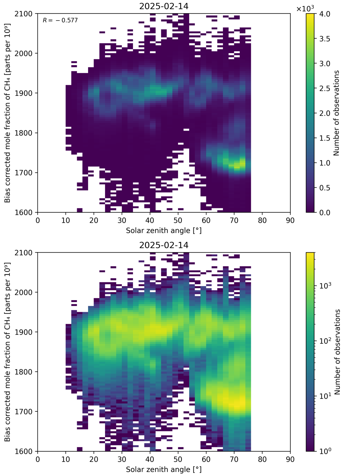
Figure 100: Scatter density plot of “Solar zenith angle” against “Bias corrected mole fraction of CH 4 ” for 2025-02-13 to 2025-02-15.
