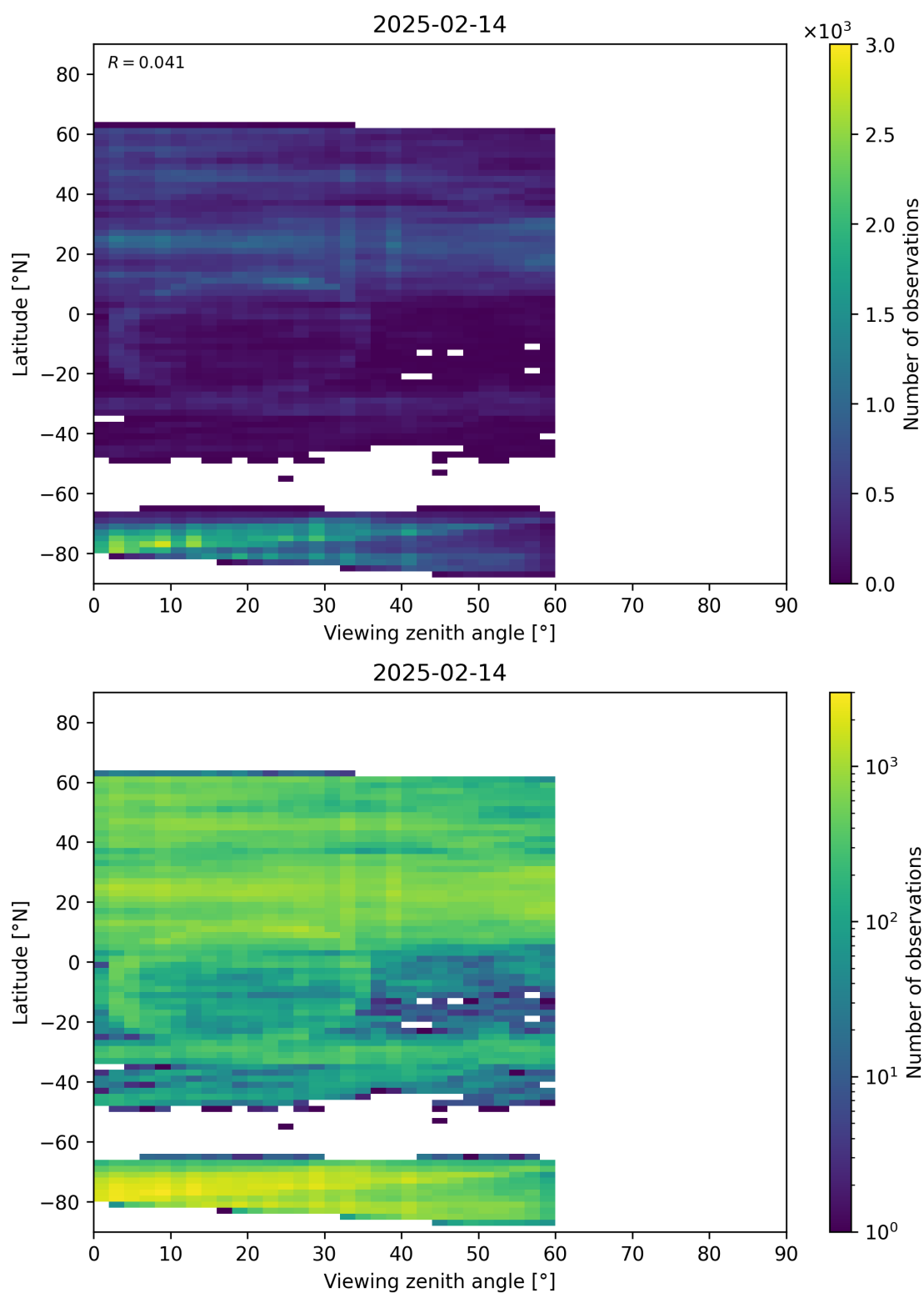
Figure 109: Scatter density plot of “Viewing zenith angle” against “Latitude” for 2025-02-13 to 2025-02-15.
