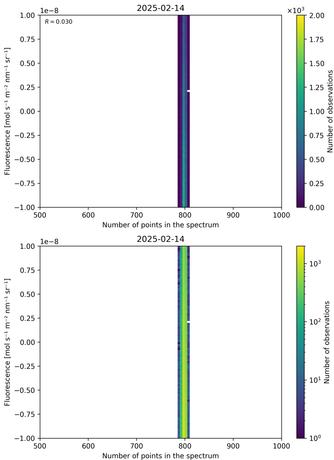
Figure 91: Scatter density plot of “Number of points in the spectrum” against “Fluorescence” for 2025-02-13 to 2025-02-15.
