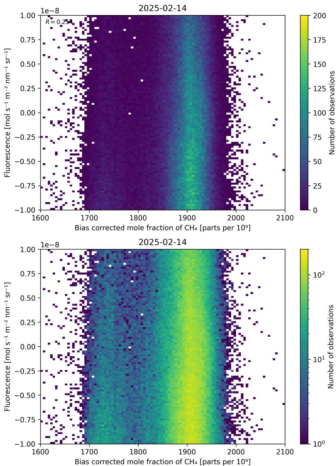
Figure 66: Scatter density plot of “Bias corrected mole fraction of \text{CH}_4 ” against “Fluorescence” for 2025-02-13 to 2025-02-15.
