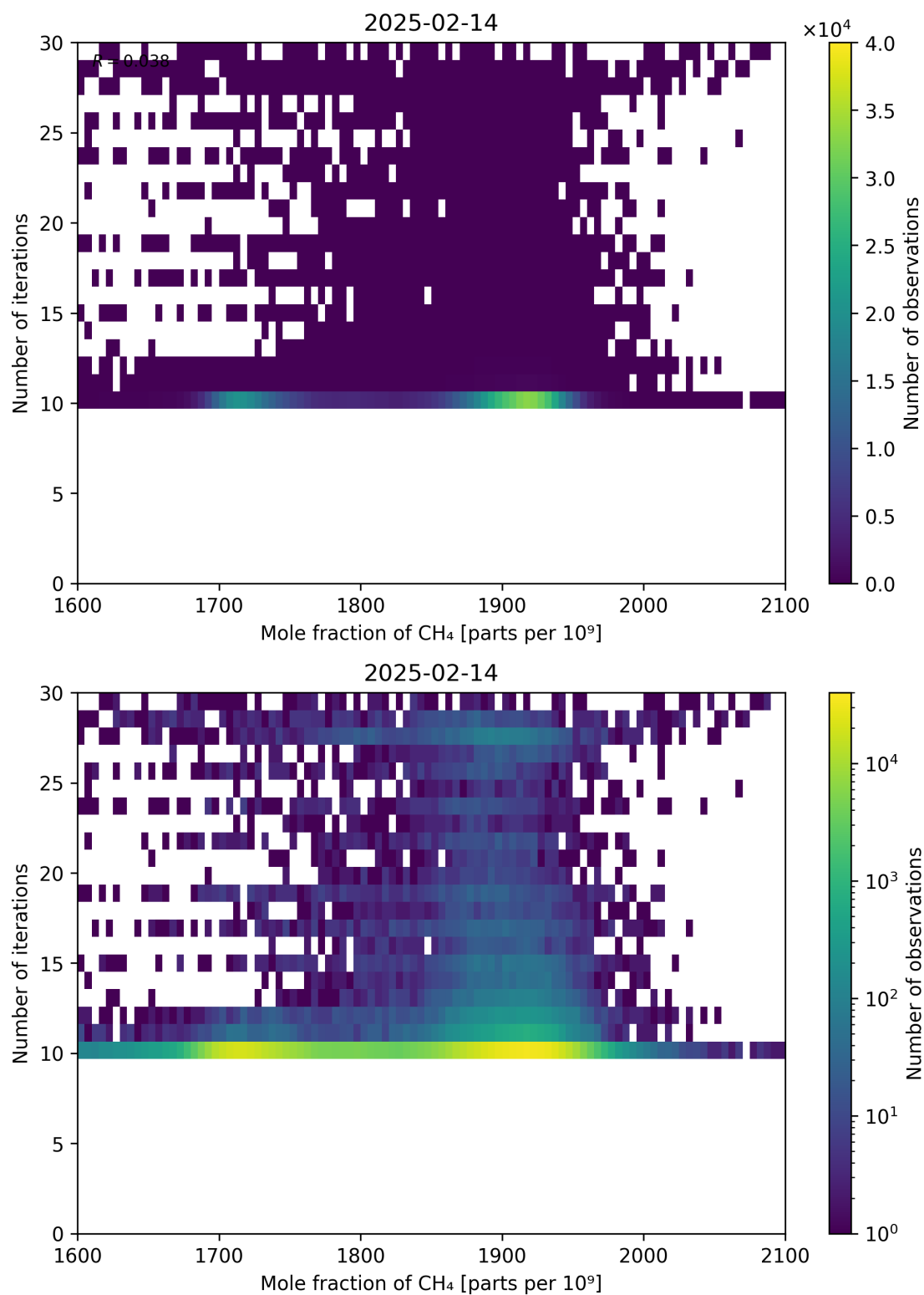
Figure 76: Scatter density plot of “Mole fraction of CH 4 ” against “Number of iterations” for 2025-02-13 to 2025-02-15.
