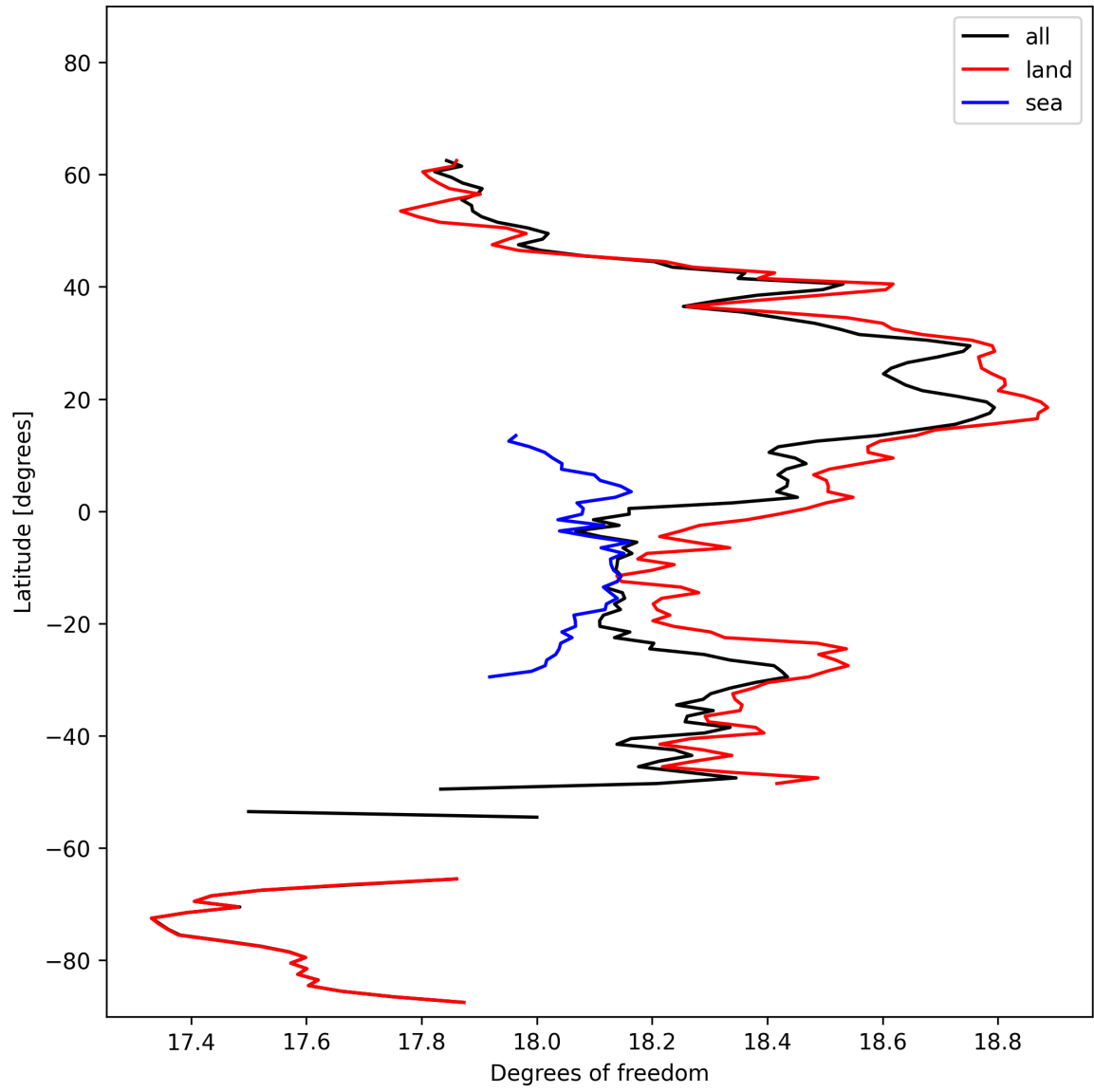
Figure 19: Zonal average of “Degrees of freedom” for 2025-02-13 to 2025-02-15.
