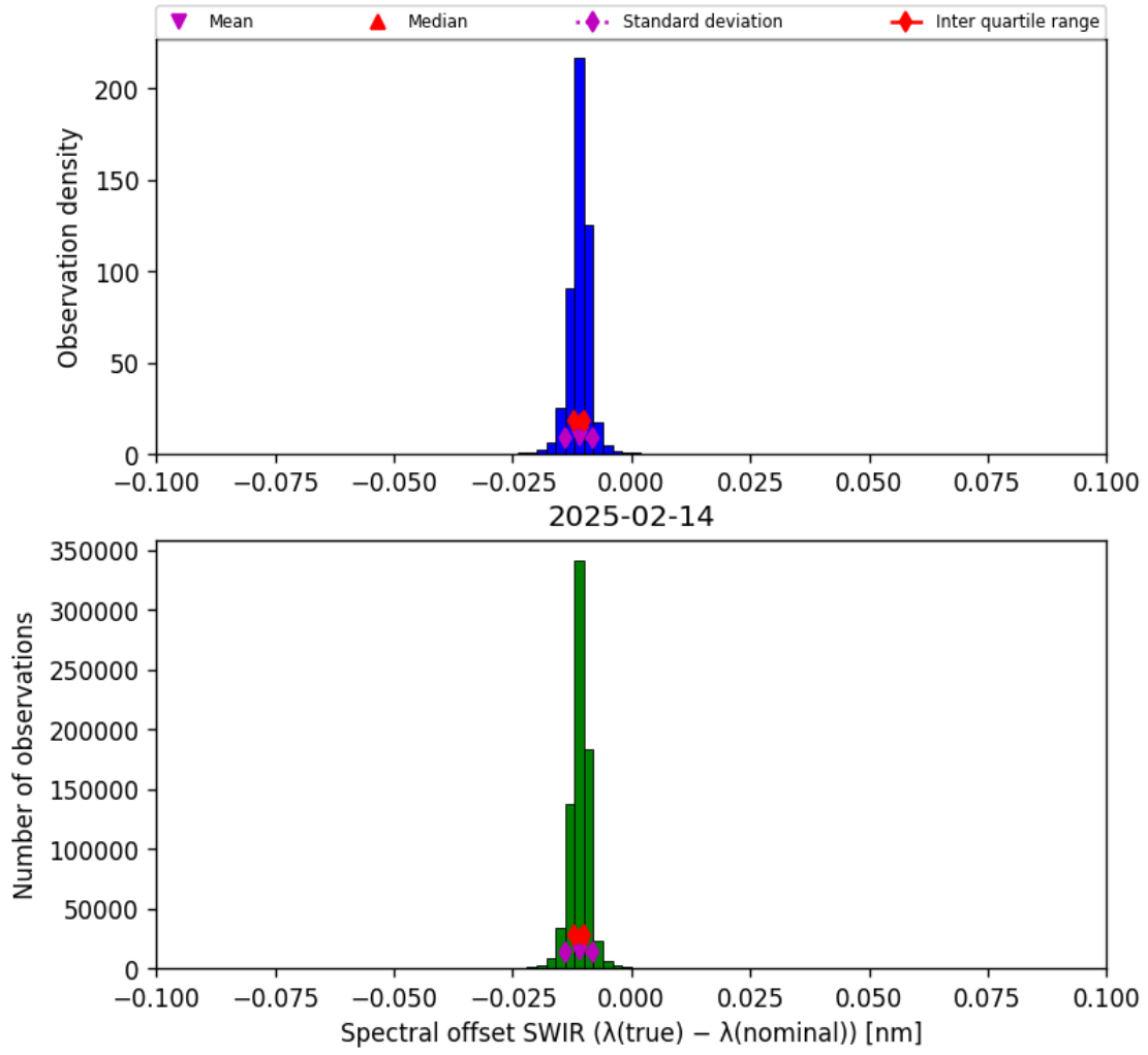
Figure 27: Histogram of “Spectral offset SWIR ( \lambda_{\text{true}} - \lambda_{\text{nominal}} )” for 2025-02-13 to 2025-02-15
