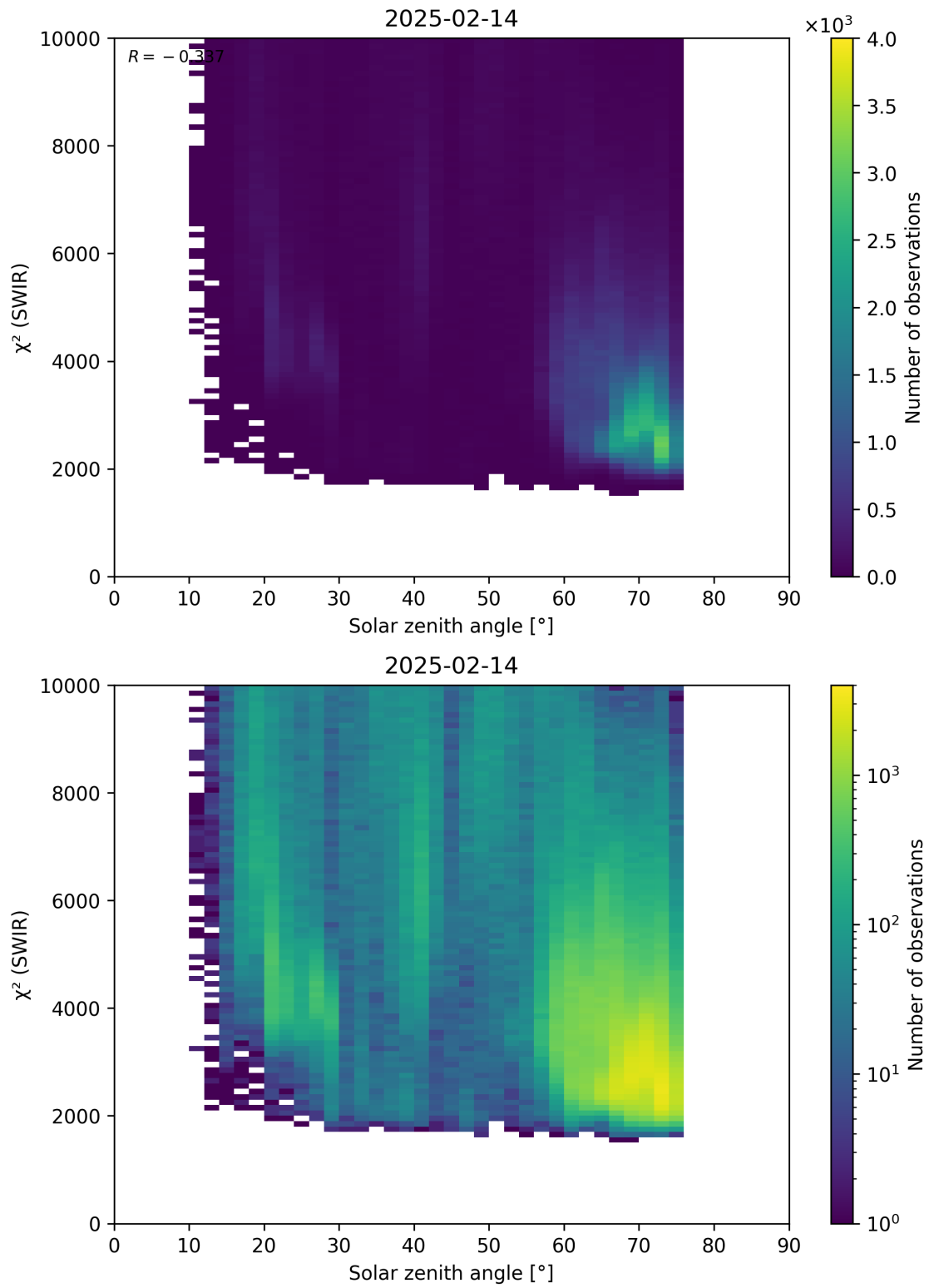
Figure 95: Scatter density plot of “Solar zenith angle” against “ \chi^2 (SWIR)” for 2025-02-13 to 2025-02-15.
