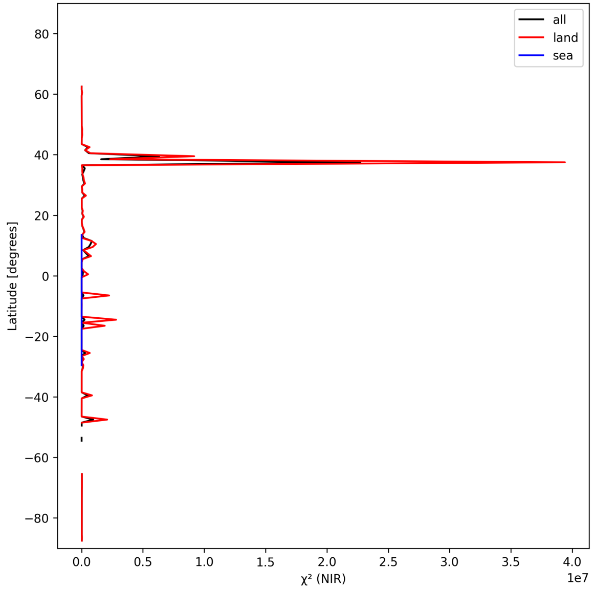
Figure 18: Zonal average of “ \chi^2 (NIR)” for 2025-02-13 to 2025-02-15.
