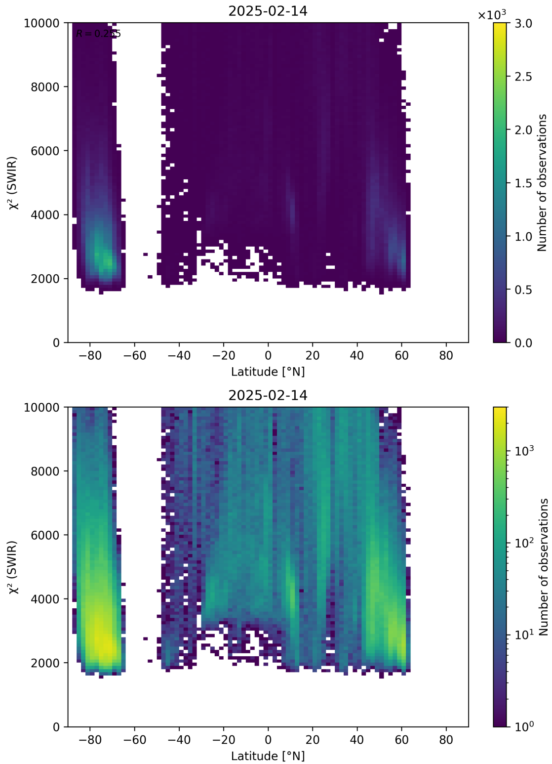
Figure 54: Scatter density plot of “Latitude” against “ \chi^2 (SWIR)” for 2025-02-13 to 2025-02-15.
