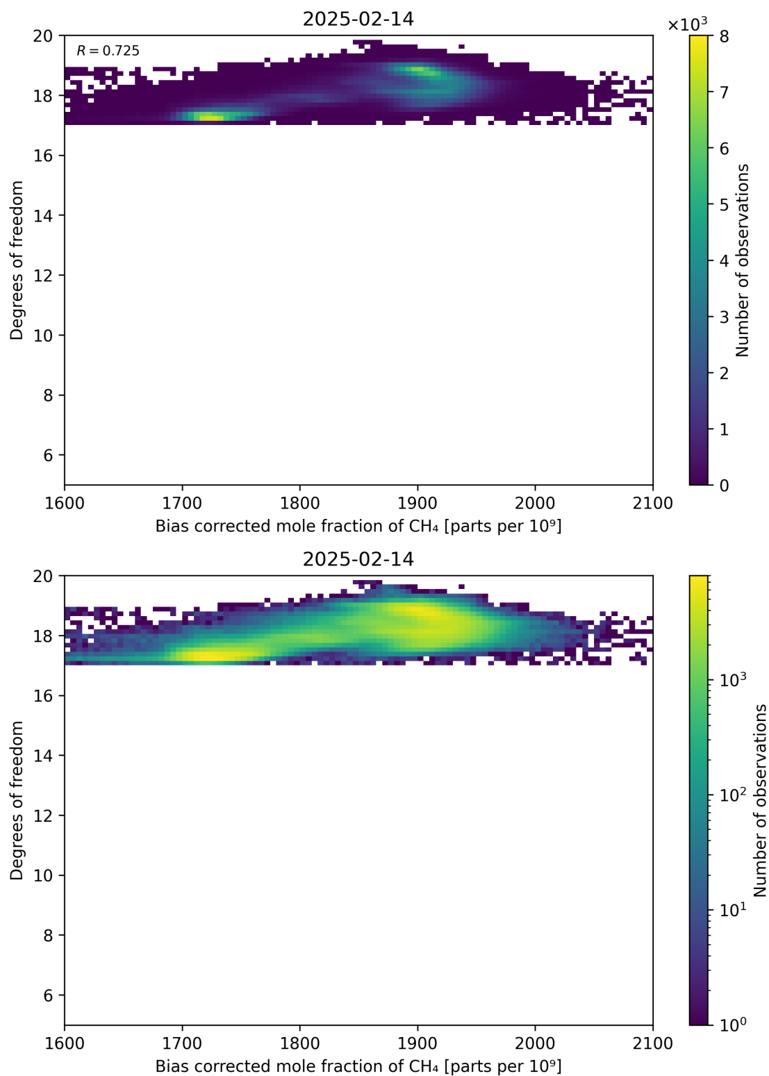
Figure 65: Scatter density plot of “Bias corrected mole fraction of CH 4 ” against “Degrees of freedom” for 2025-02-13 to 2025-02-15.
