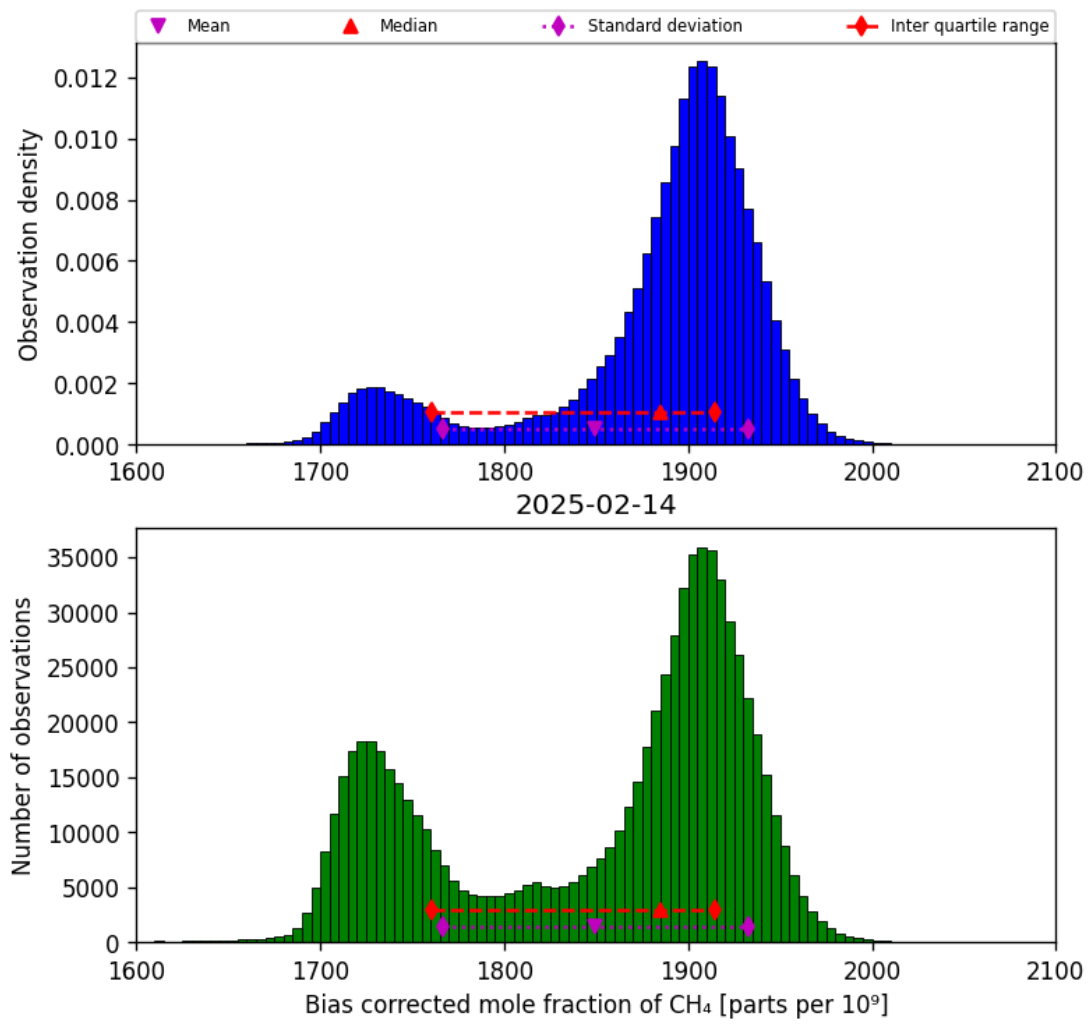
Figure 25: Histogram of “Bias corrected mole fraction of CH 4 ” for 2025-02-13 to 2025-02-15
