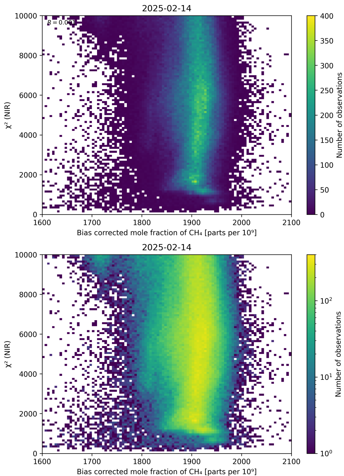
Figure 63: Scatter density plot of “Bias corrected mole fraction of \text{CH}_4 ” against “ \chi^2 (NIR)” for 2025-02-13 to 2025-02-15.
