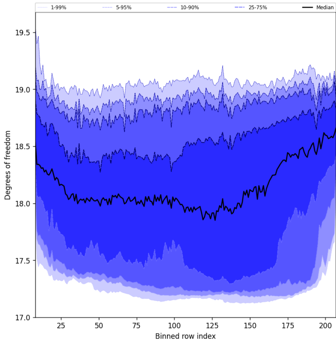
Figure 41: Along track statistics of “Degrees of freedom” for 2025-02-13 to 2025-02-15
