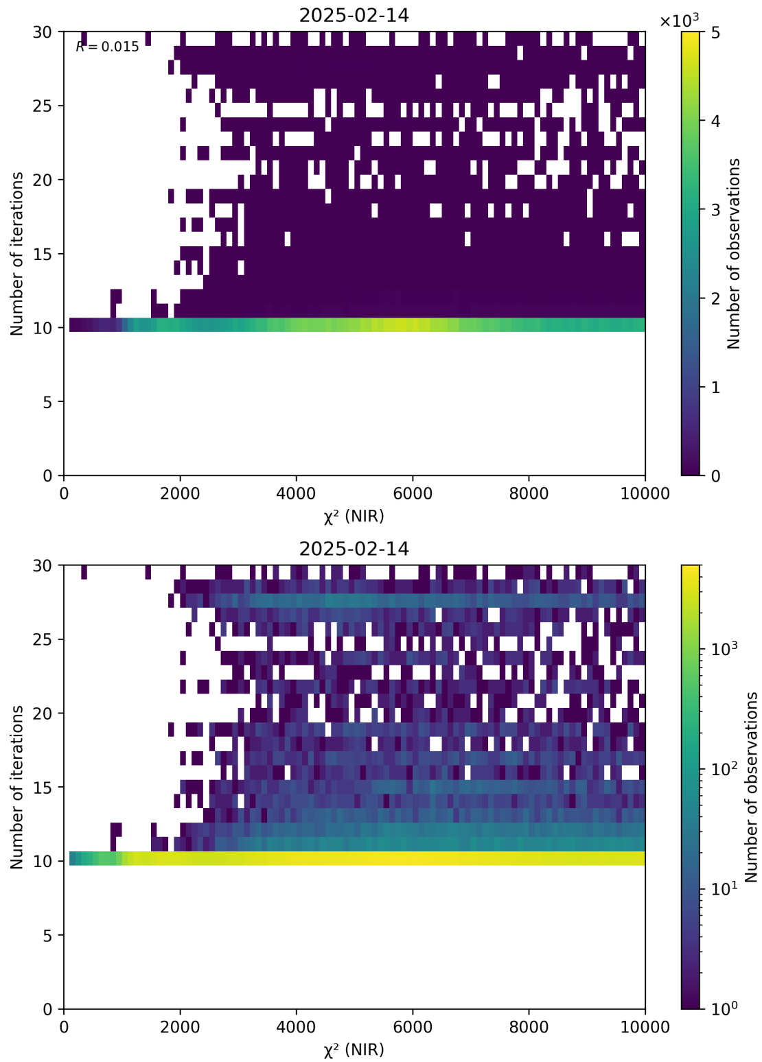
Figure 46: Scatter density plot of “ \chi^2 (NIR)” against “Number of iterations” for 2025-02-13 to 2025-02-15.
