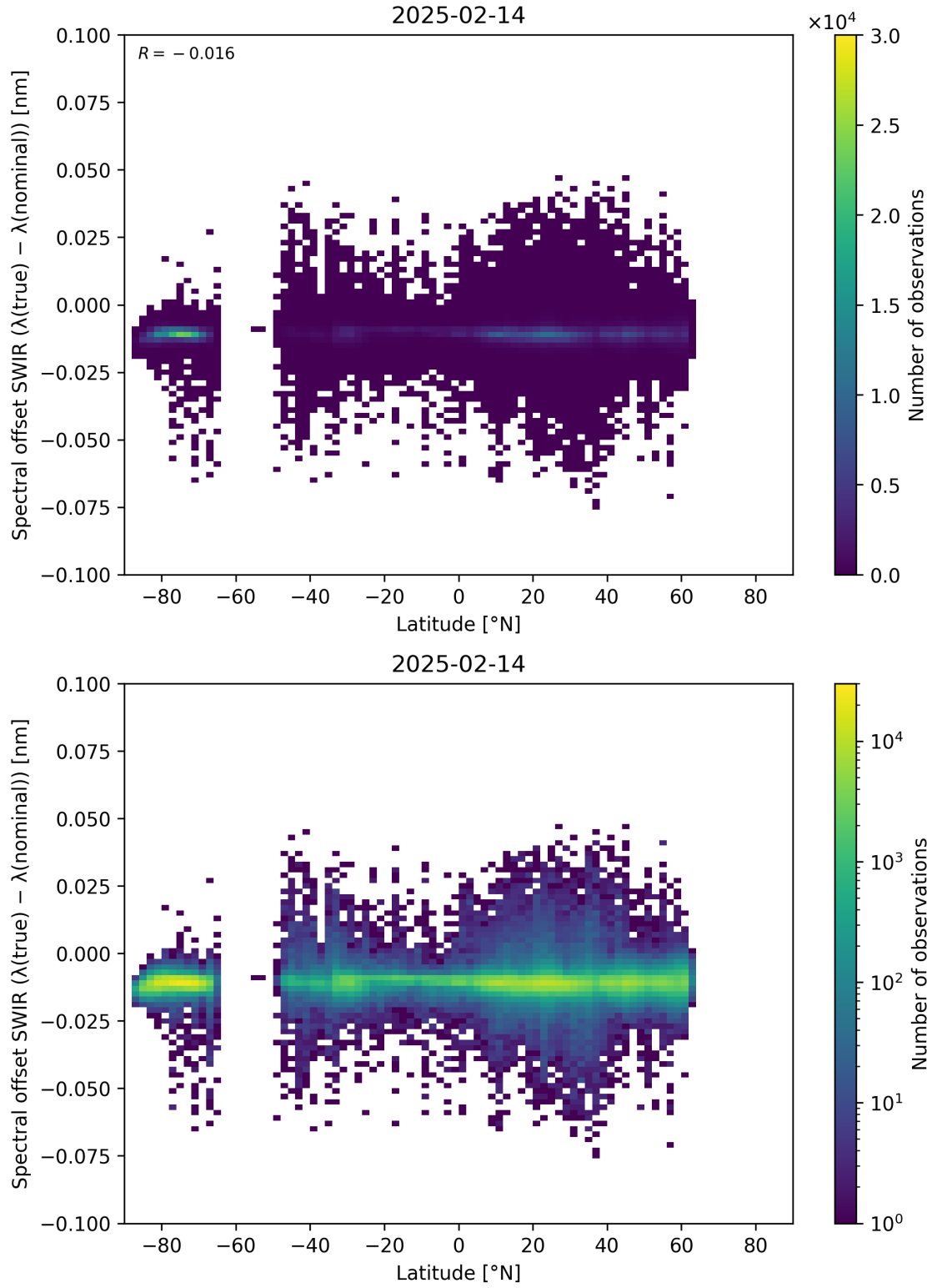
Figure 62: Scatter density plot of “Latitude” against “Spectral offset SWIR ( \lambda_{\text{true}} - \lambda_{\text{nominal}} )” for 2025-02-13 to 2025-02-15.
