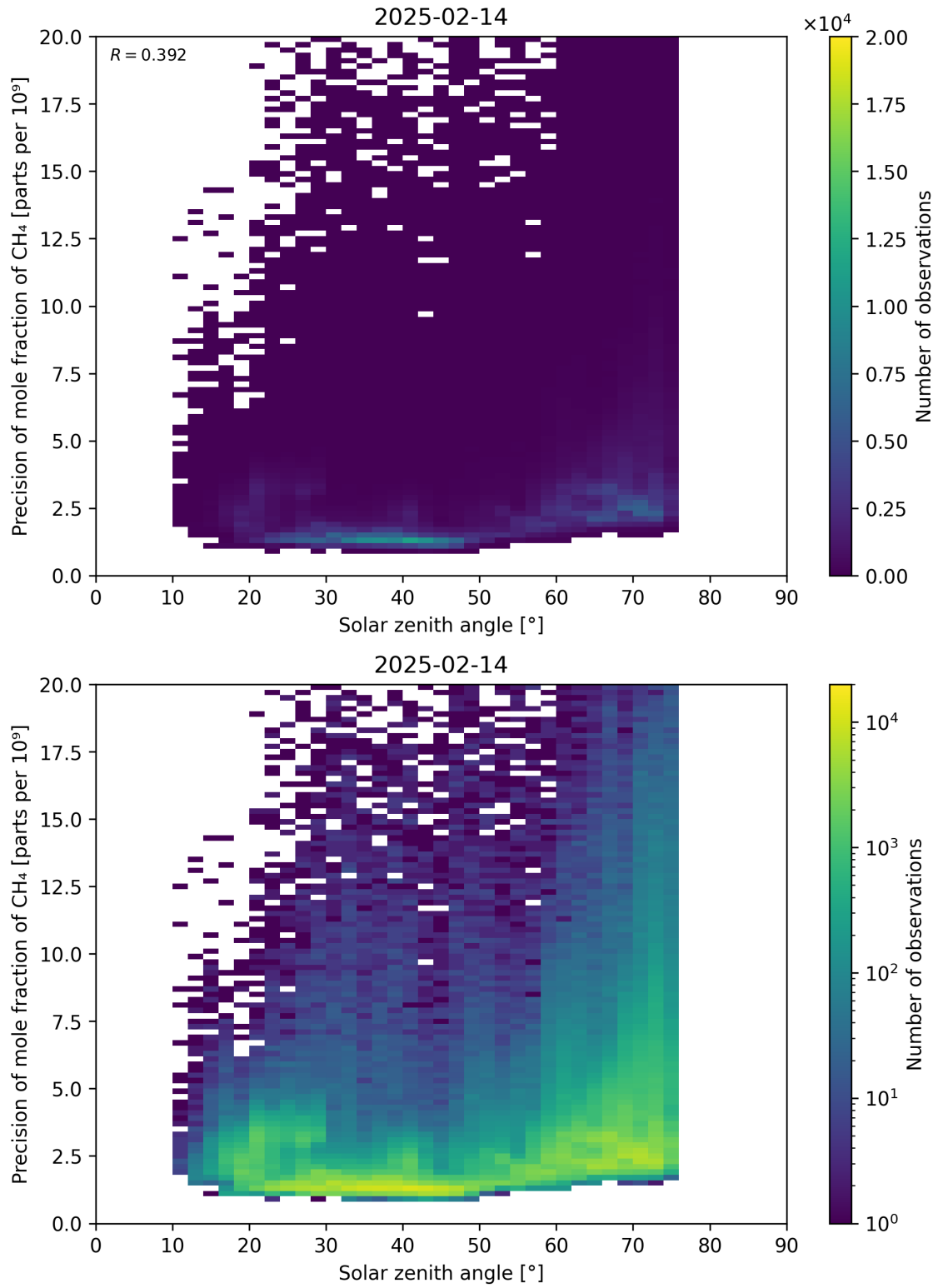
Figure 101: Scatter density plot of “Solar zenith angle” against “Precision of mole fraction of \text{CH}_4 ” for 2025-02-13 to 2025-02-15.
