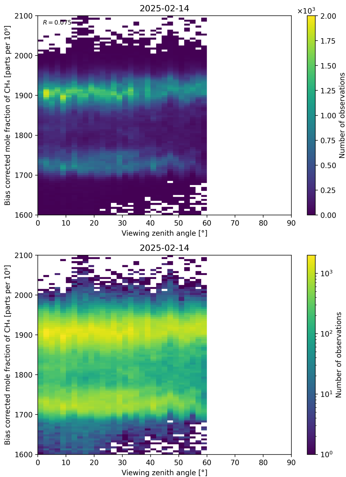
Figure 111: Scatter density plot of “Viewing zenith angle” against “Bias corrected mole fraction of CH 4 ” for 2025-02-13 to 2025-02-15.
