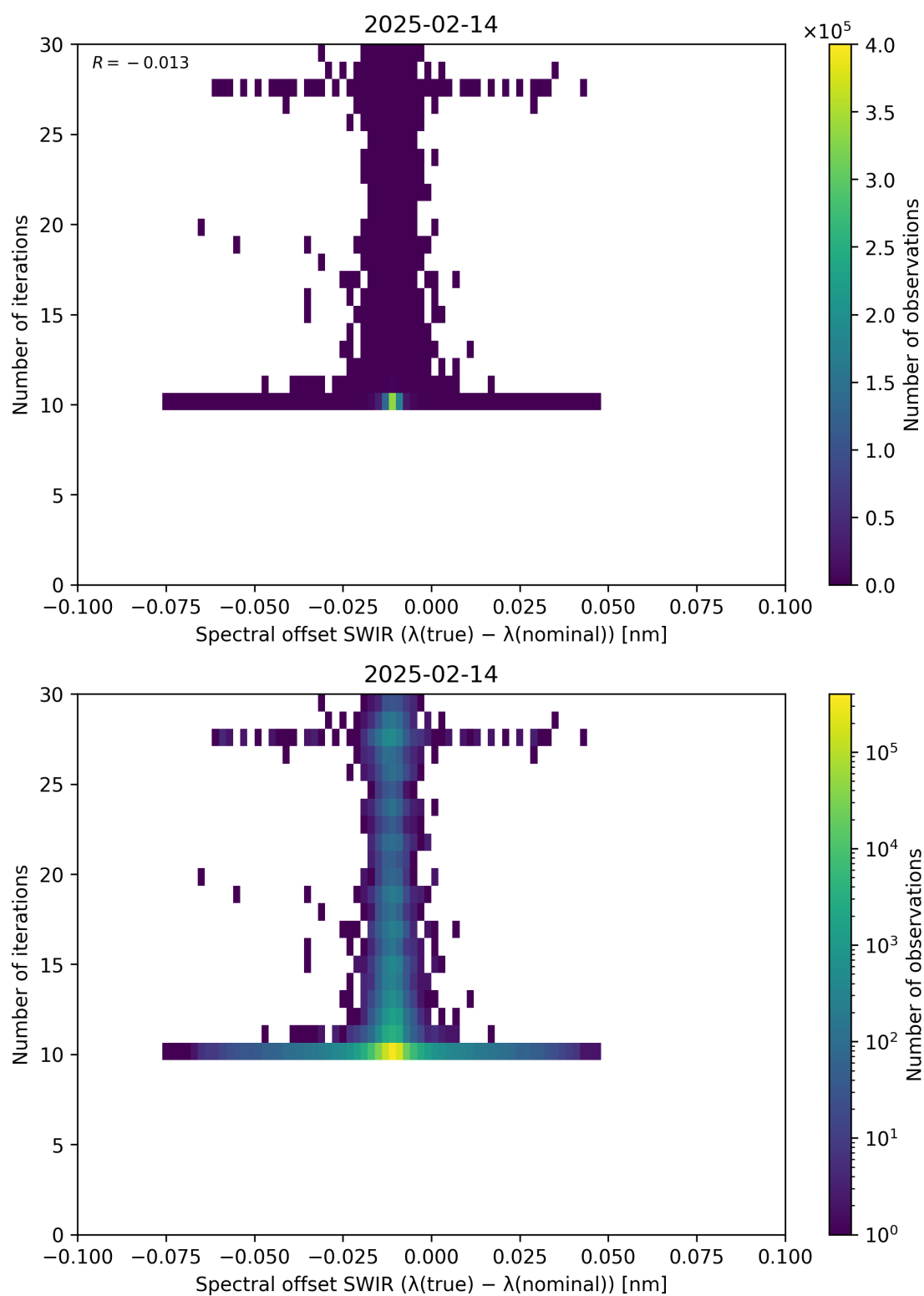
Figure 121: Scatter density plot of “Spectral offset SWIR ( \lambda_{\text{true}} - \lambda_{\text{nominal}} )” against “Number of iterations” for 2025-02-13 to 2025-02-15.
