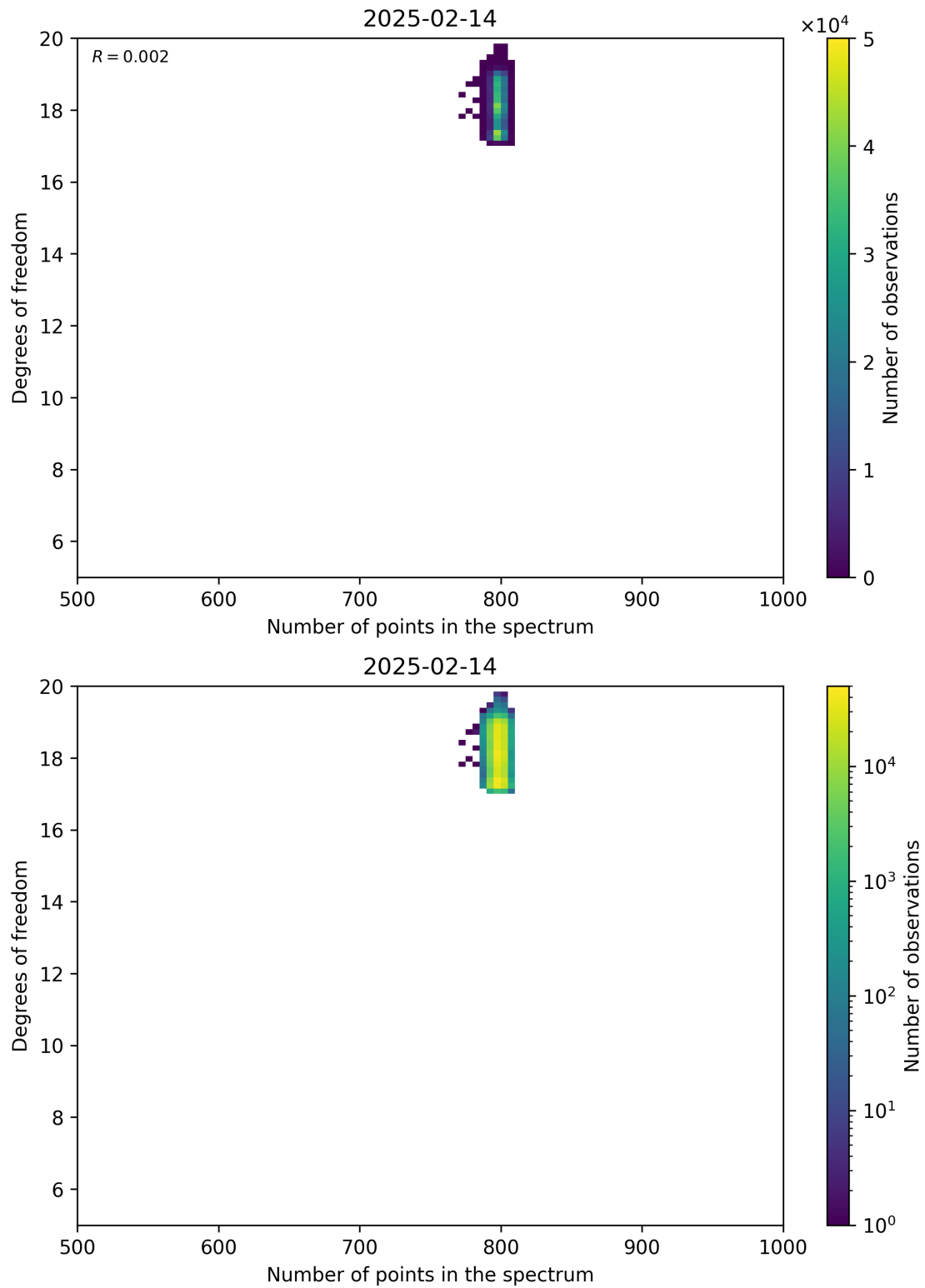
Figure 90: Scatter density plot of “Number of points in the spectrum” against “Degrees of freedom” for 2025-02-13 to 2025-02-15.
