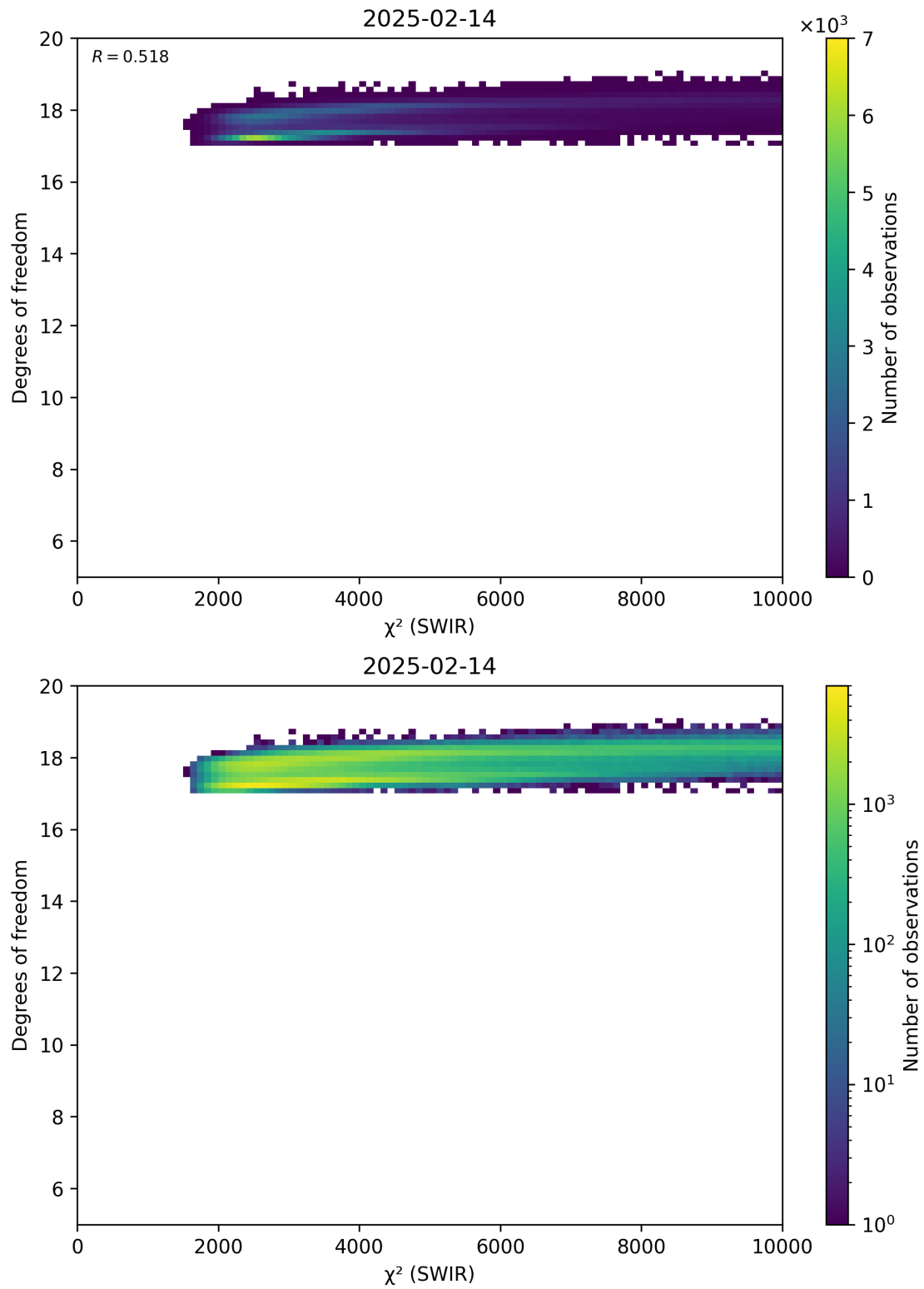
Figure 48: Scatter density plot of “ \chi^2 (SWIR)” against “Degrees of freedom” for 2025-02-13 to 2025-02-15.
