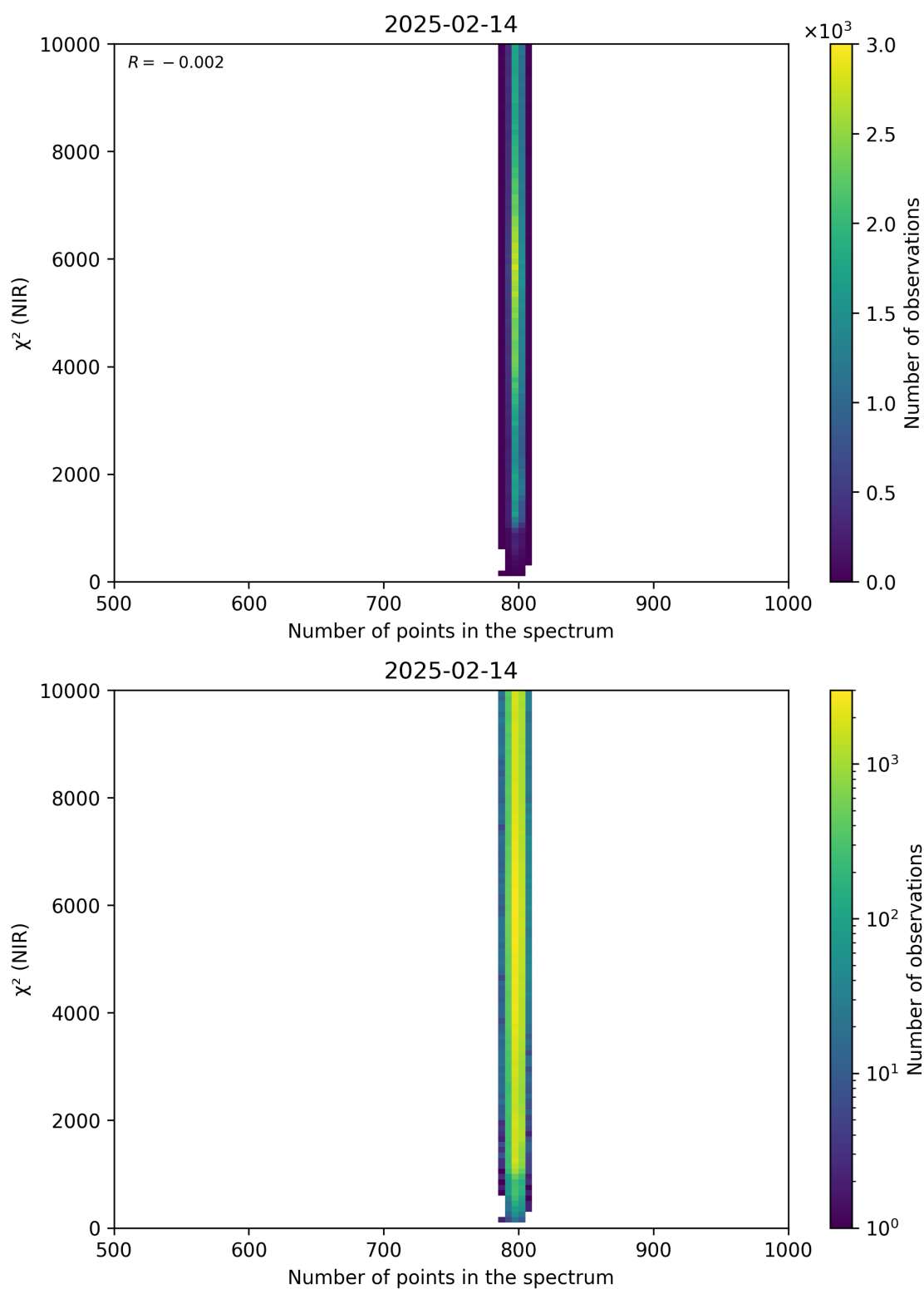
Figure 88: Scatter density plot of “Number of points in the spectrum” against “ \chi^2 (NIR)” for 2025-02-13 to 2025-02-15.
