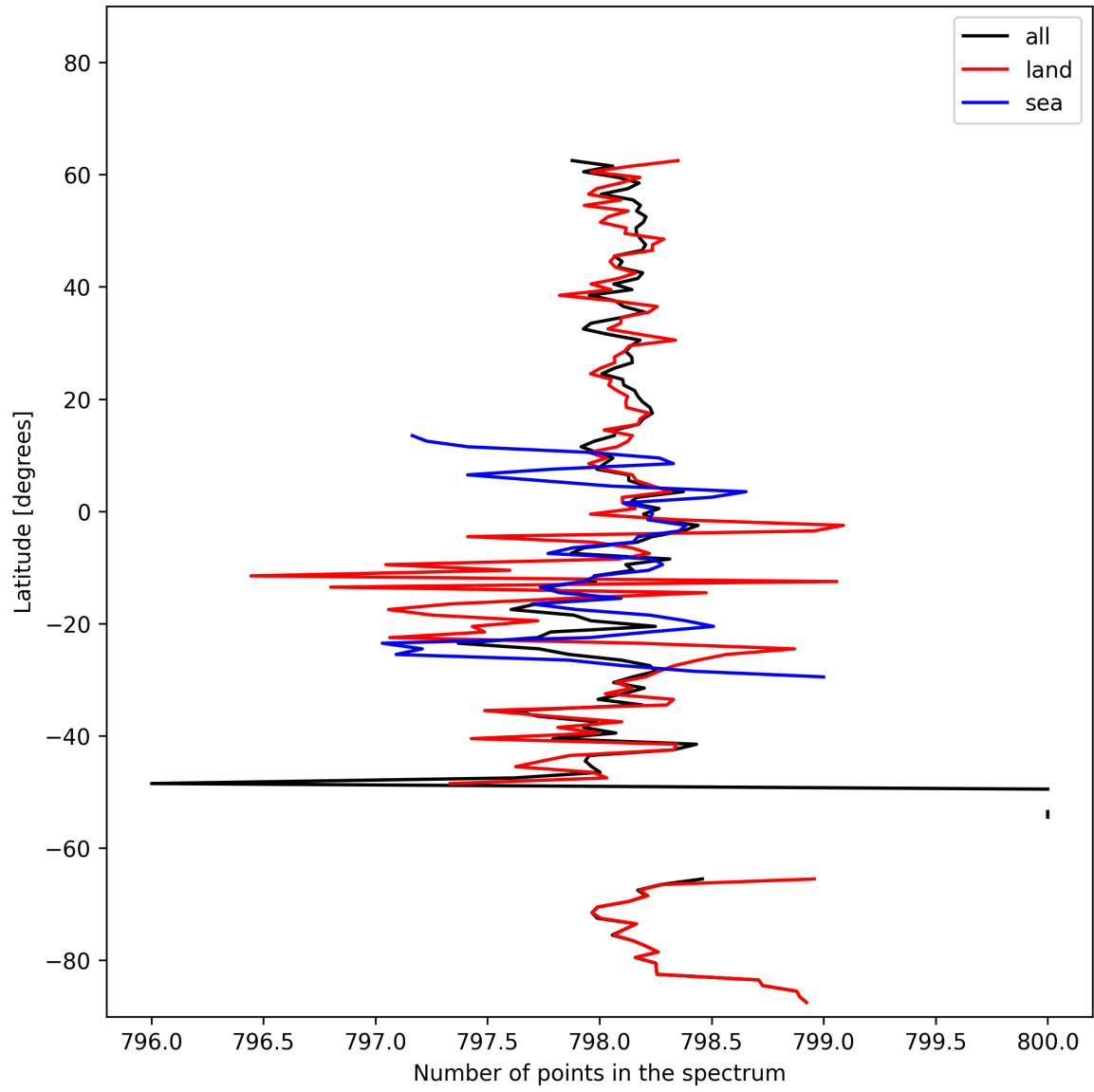
Figure 15: Zonal average of “Number of points in the spectrum” for 2025-02-13 to 2025-02-15.
