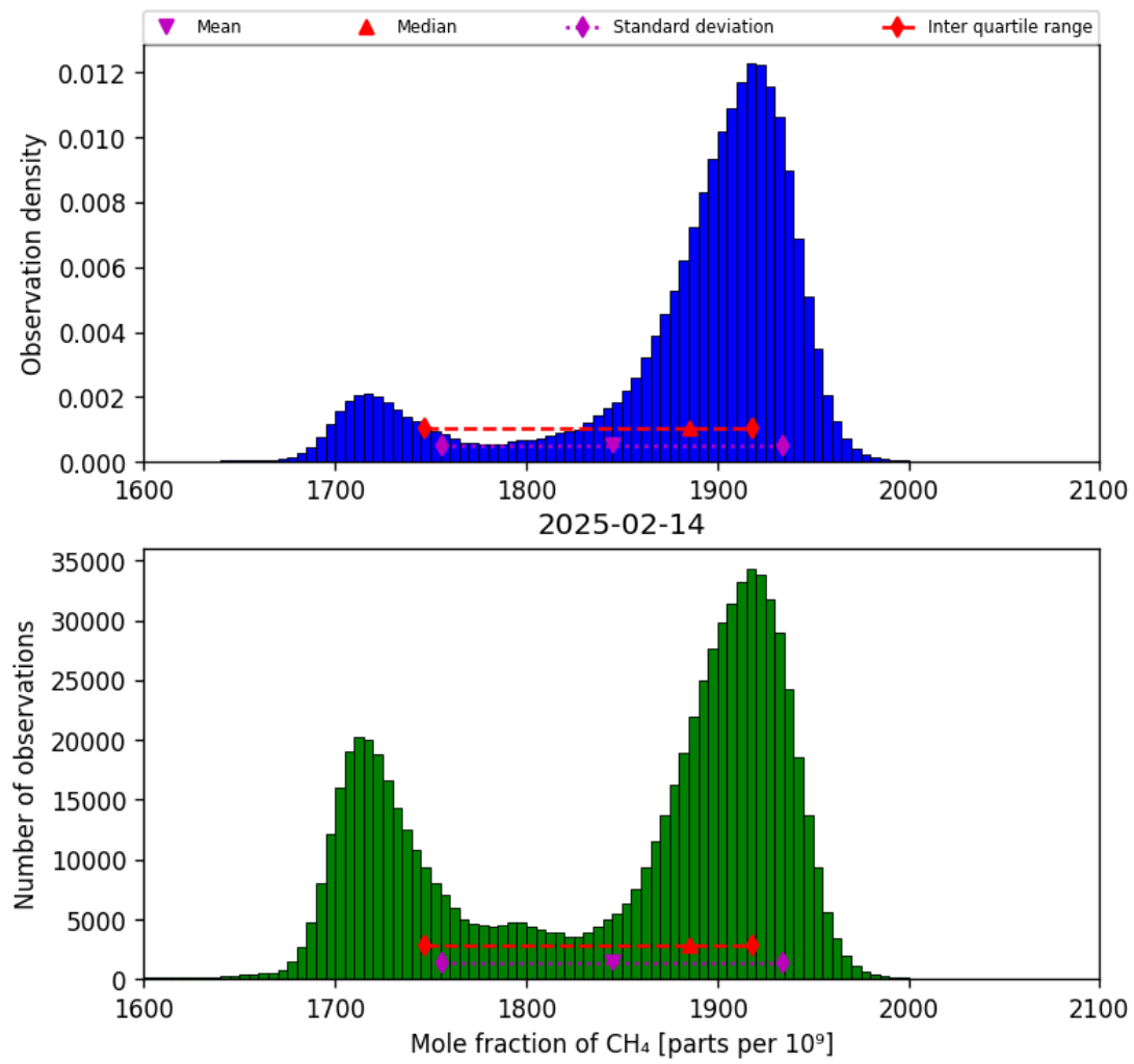
Figure 23: Histogram of “Mole fraction of CH 4 ” for 2025-02-13 to 2025-02-15
