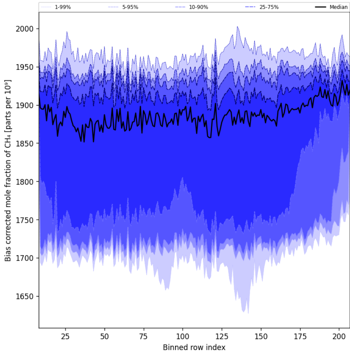
Figure 36: Along track statistics of “Bias corrected mole fraction of CH 4 ” for 2025-02-13 to 2025-02-15
