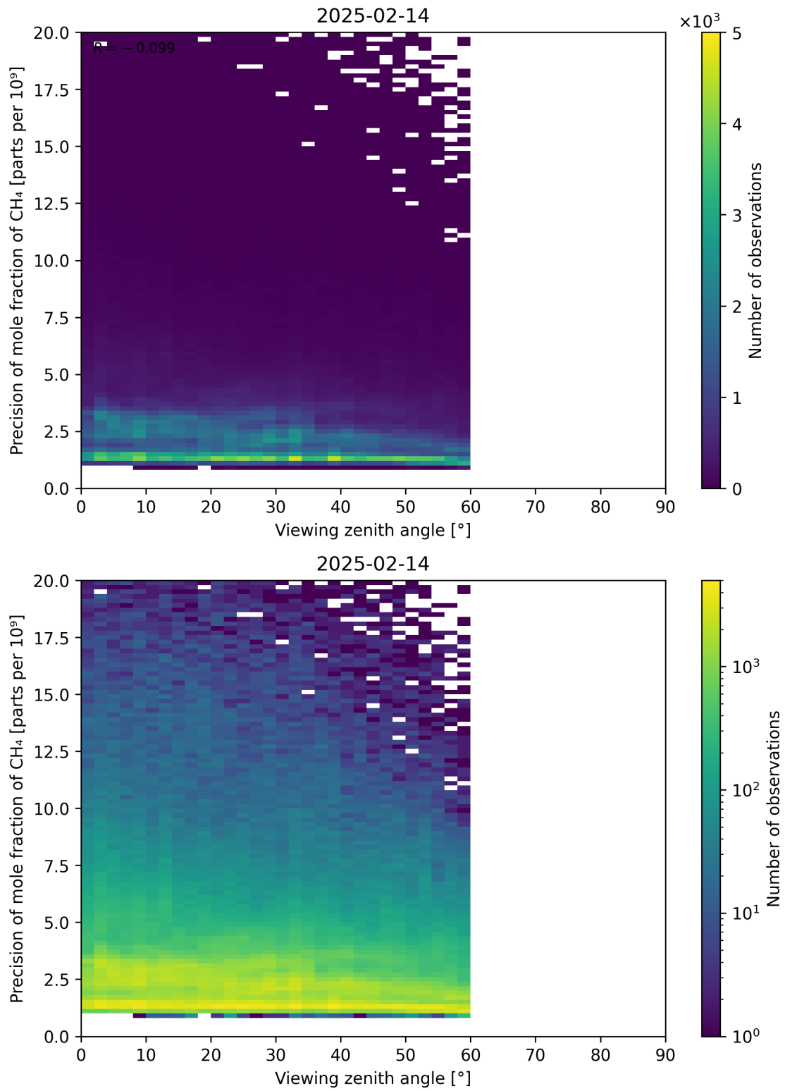
Figure 112: Scatter density plot of “Viewing zenith angle” against “Precision of mole fraction of CH 4 ” for 2025-02-13 to 2025-02-15.
