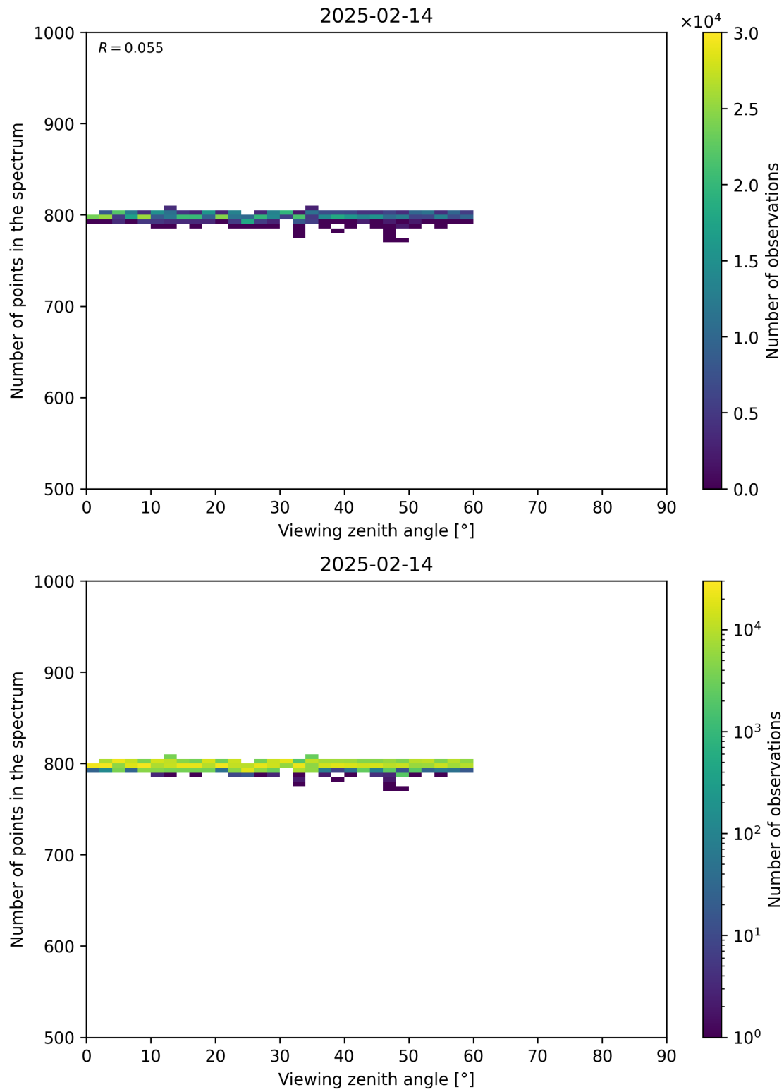
Figure 114: Scatter density plot of “Viewing zenith angle” against “Number of points in the spectrum” for 2025-02-13 to 2025-02-15.
