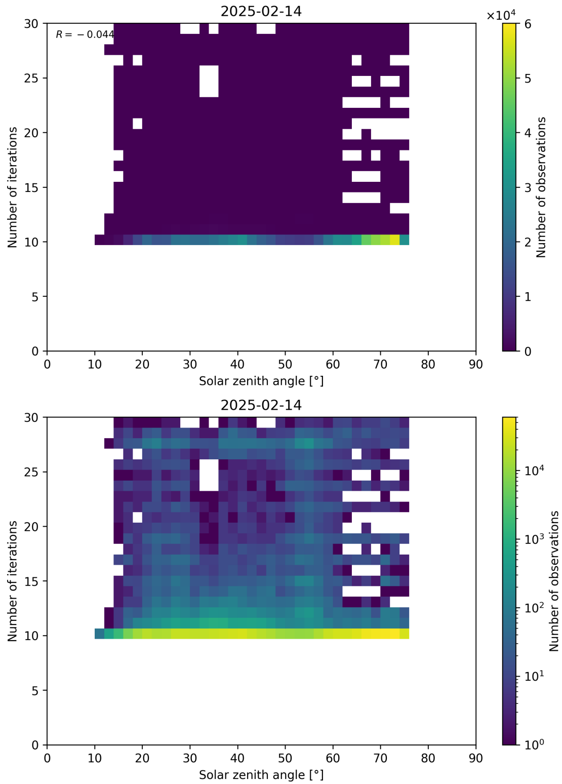
Figure 102: Scatter density plot of “Solar zenith angle” against “Number of iterations” for 2025-02-13 to 2025-02-15.
