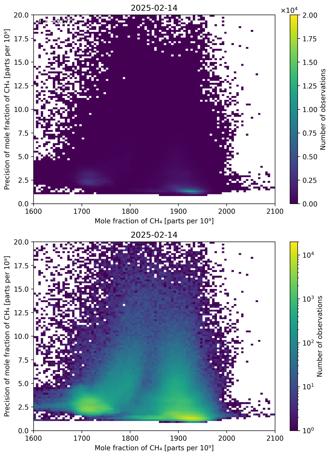
Figure 75: Scatter density plot of “Mole fraction of CH 4 ” against “Precision of mole fraction of CH 4 ” for 2025-02-13 to 2025-02-15.
