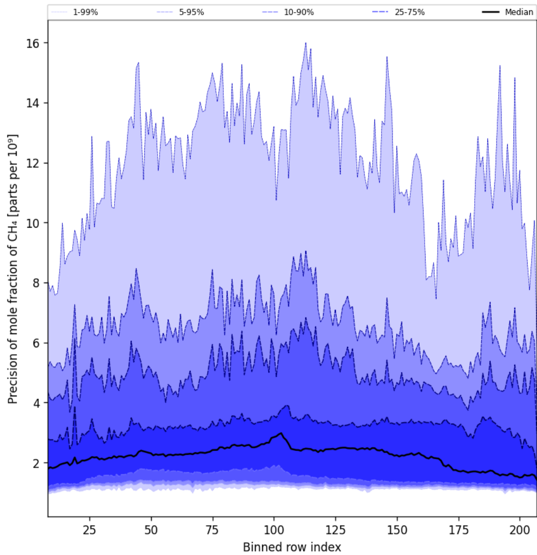
Figure 35: Along track statistics of “Precision of mole fraction of CH 4 ” for 2025-02-13 to 2025-02-15
