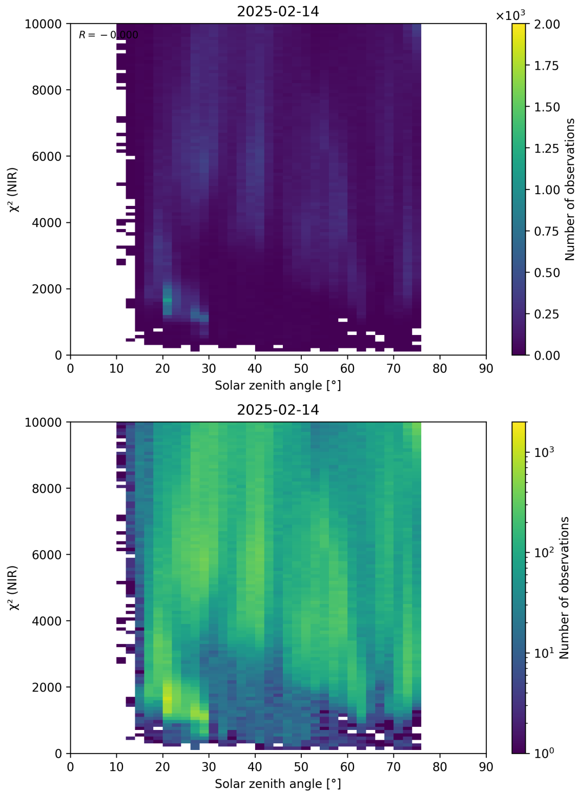
Figure 94: Scatter density plot of “Solar zenith angle” against “ \chi^2 (NIR)” for 2025-02-13 to 2025-02-15.
