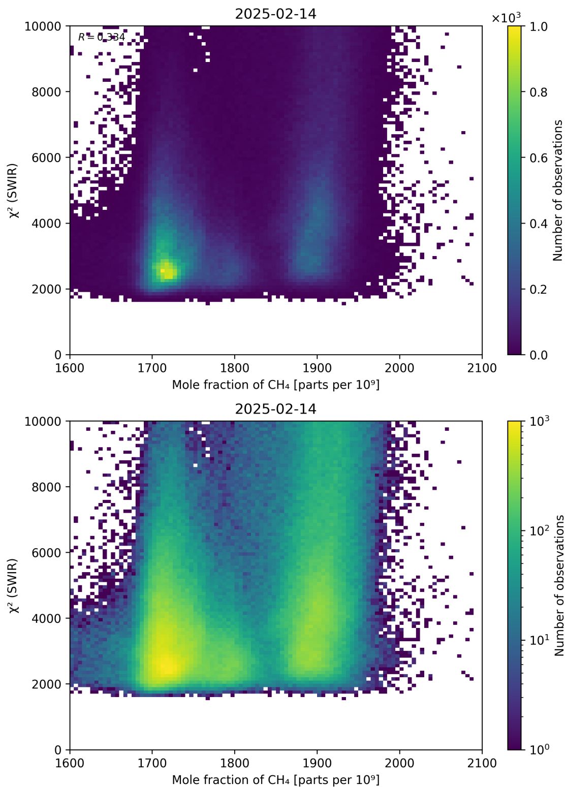
Figure 71: Scatter density plot of “Mole fraction of \text{CH}_4 ” against “ \chi^2 (SWIR)” for 2025-02-13 to 2025-02-15.
