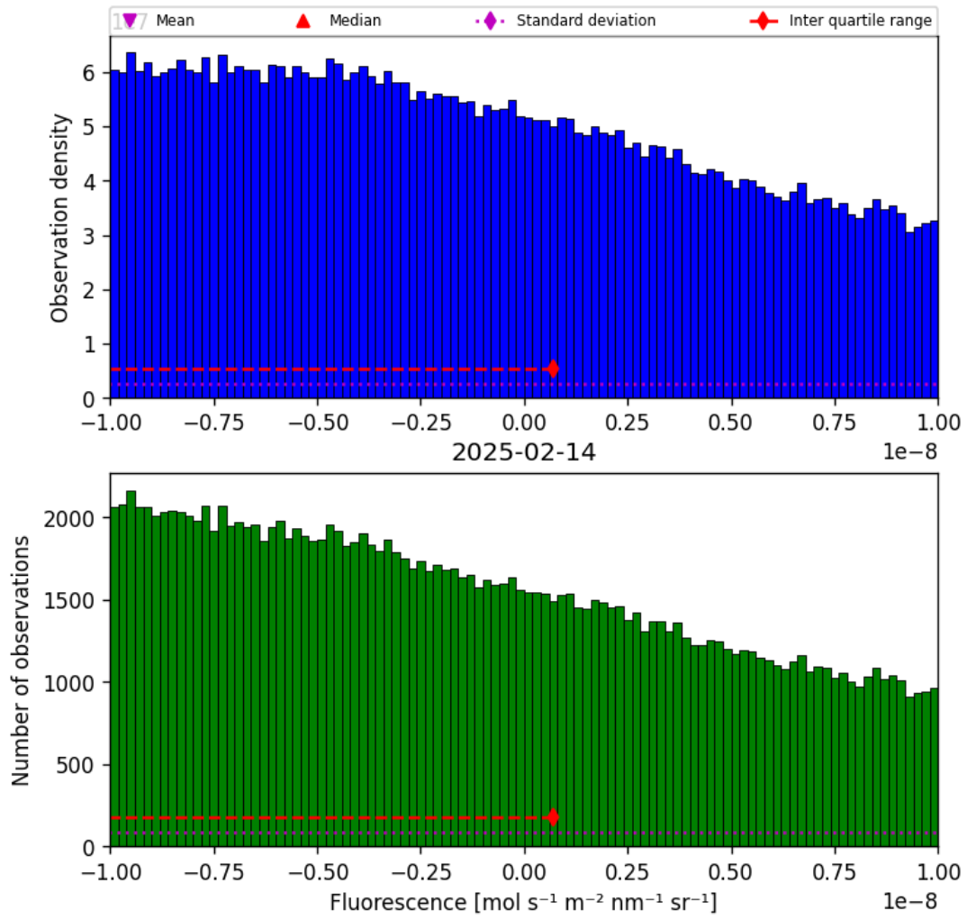
Figure 32: Histogram of “Fluorescence” for 2025-02-13 to 2025-02-15
