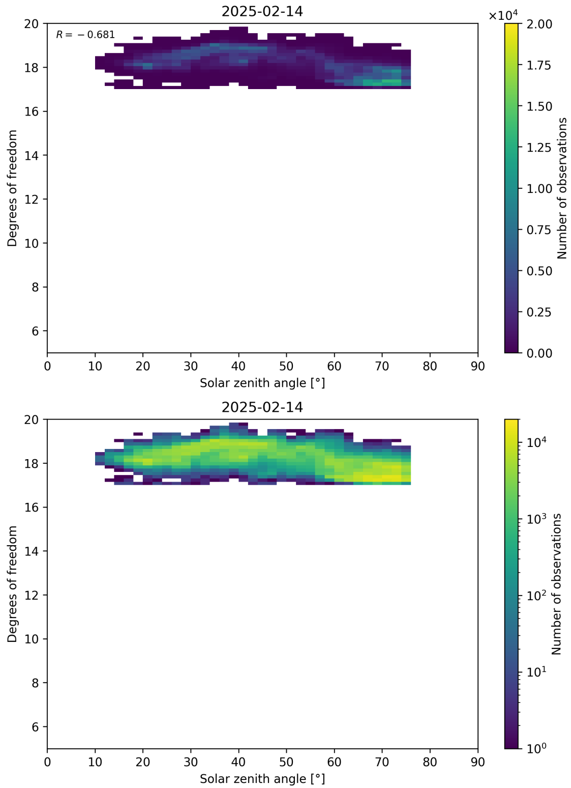
Figure 96: Scatter density plot of “Solar zenith angle” against “Degrees of freedom” for 2025-02-13 to 2025-02-15.
