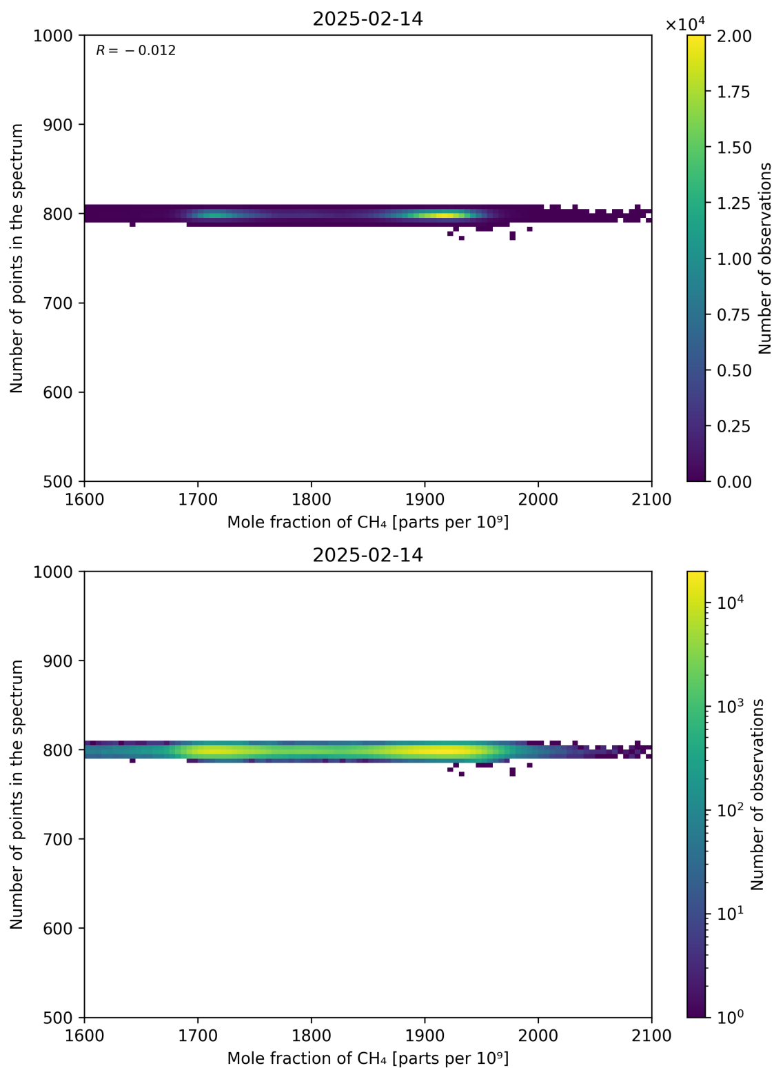
Figure 77: Scatter density plot of “Mole fraction of CH 4 ” against “Number of points in the spectrum” for 2025-02-13 to 2025-02-15.
