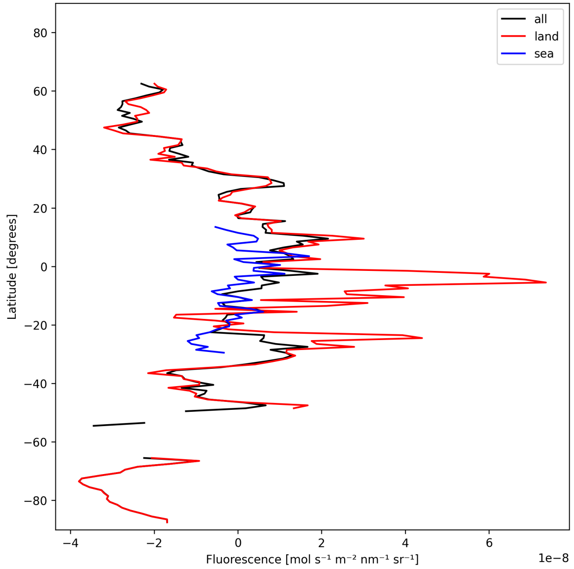
Figure 21: Zonal average of “Fluorescence” for 2025-02-13 to 2025-02-15.
