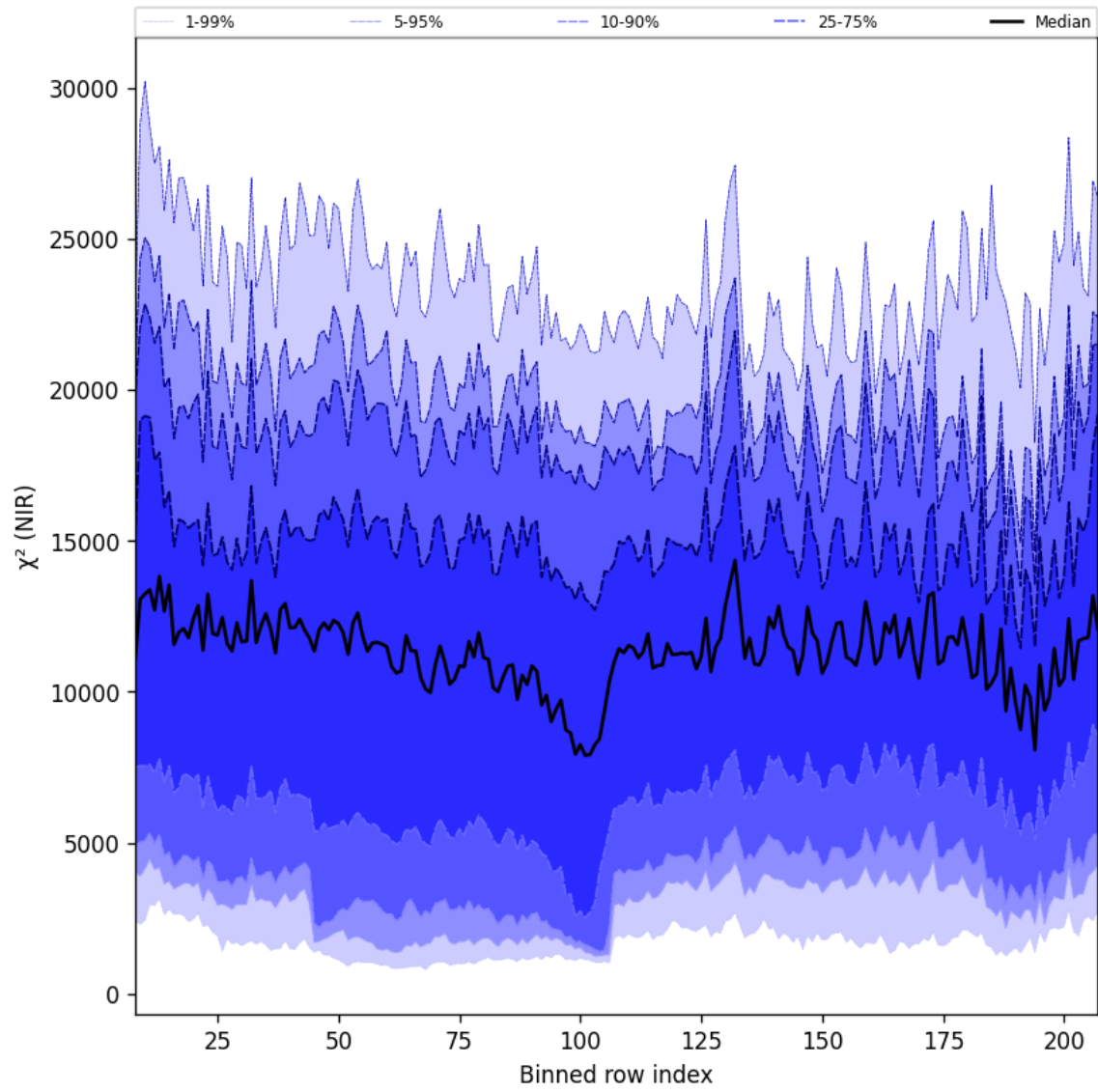
Figure 40: Along track statistics of “ \chi^2 (NIR)” for 2025-02-13 to 2025-02-15
