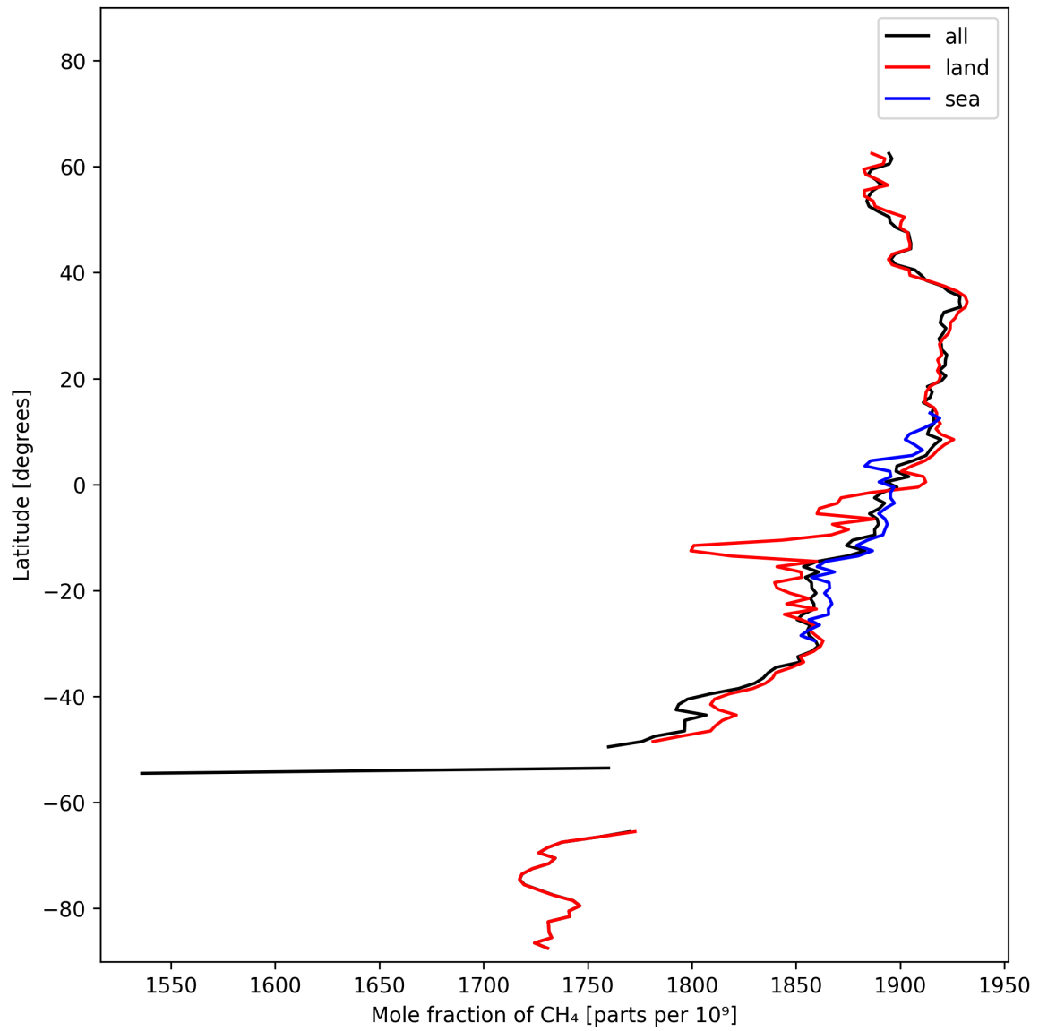
Figure 12: Zonal average of “Mole fraction of \text{CH}_4 ” for 2025-02-13 to 2025-02-15.
