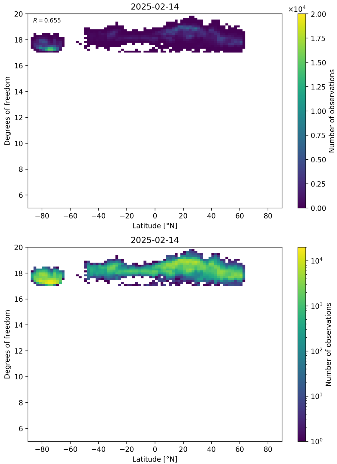
Figure 55: Scatter density plot of “Latitude” against “Degrees of freedom” for 2025-02-13 to 2025-02-15.
