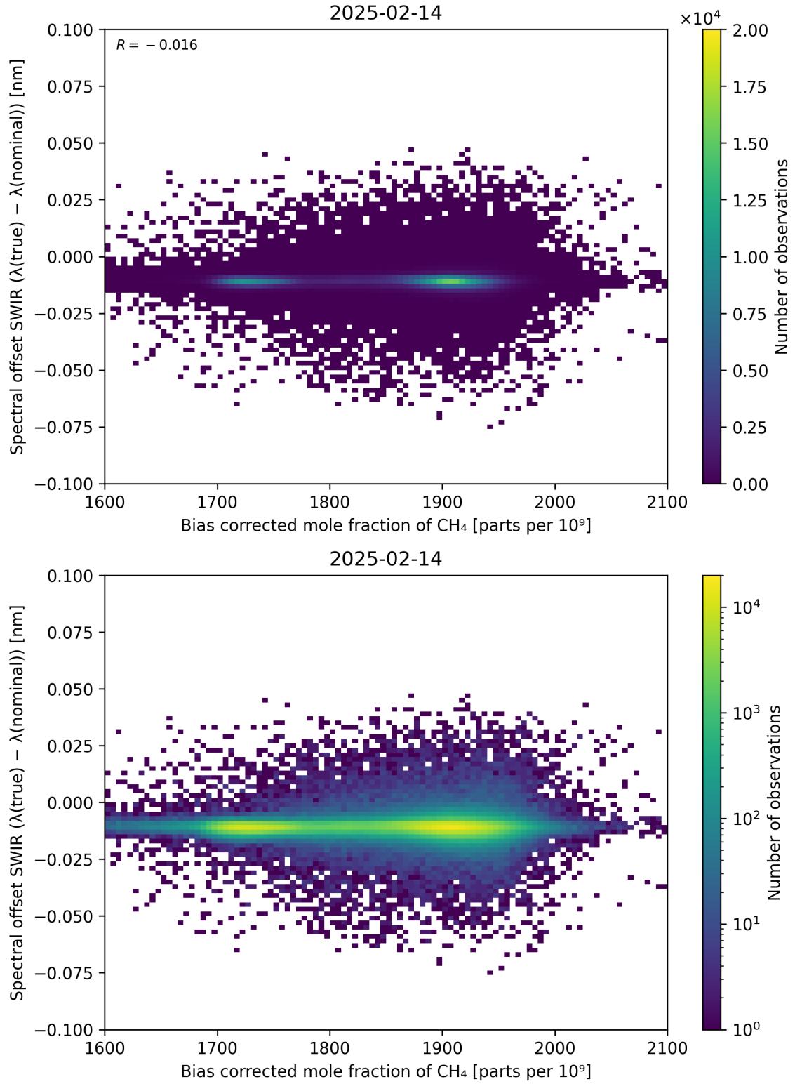
Figure 69: Scatter density plot of “Bias corrected mole fraction of \text{CH}_4 ” against “Spectral offset SWIR ( \lambda_{\text{true}} - \lambda_{\text{nominal}} )” for 2025-02-13 to 2025-02-15.
