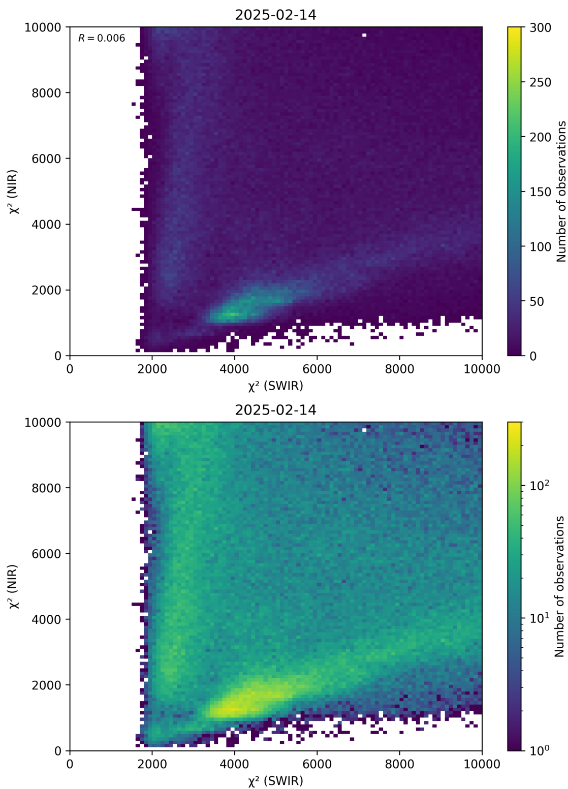
Figure 47: Scatter density plot of “ \chi^2 (SWIR)” against “ \chi^2 (NIR)” for 2025-02-13 to 2025-02-15.
