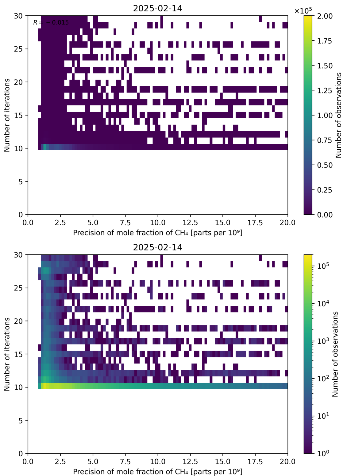
Figure 83: Scatter density plot of “Precision of mole fraction of CH 4 ” against “Number of iterations” for 2025-02-13 to 2025-02-15.
