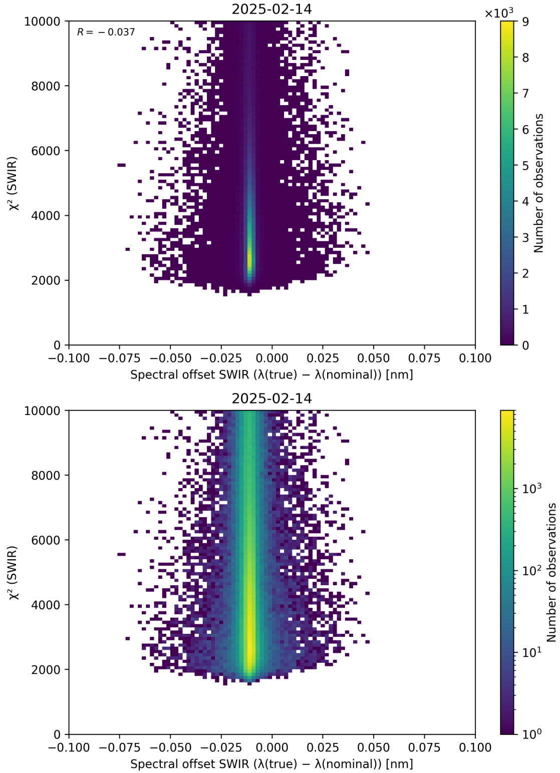
Figure 118: Scatter density plot of “Spectral offset SWIR ( \lambda_{\text{true}} - \lambda_{\text{nominal}} )” against “ \chi^2 (SWIR)” for 2025-02-13 to 2025-02-15.
