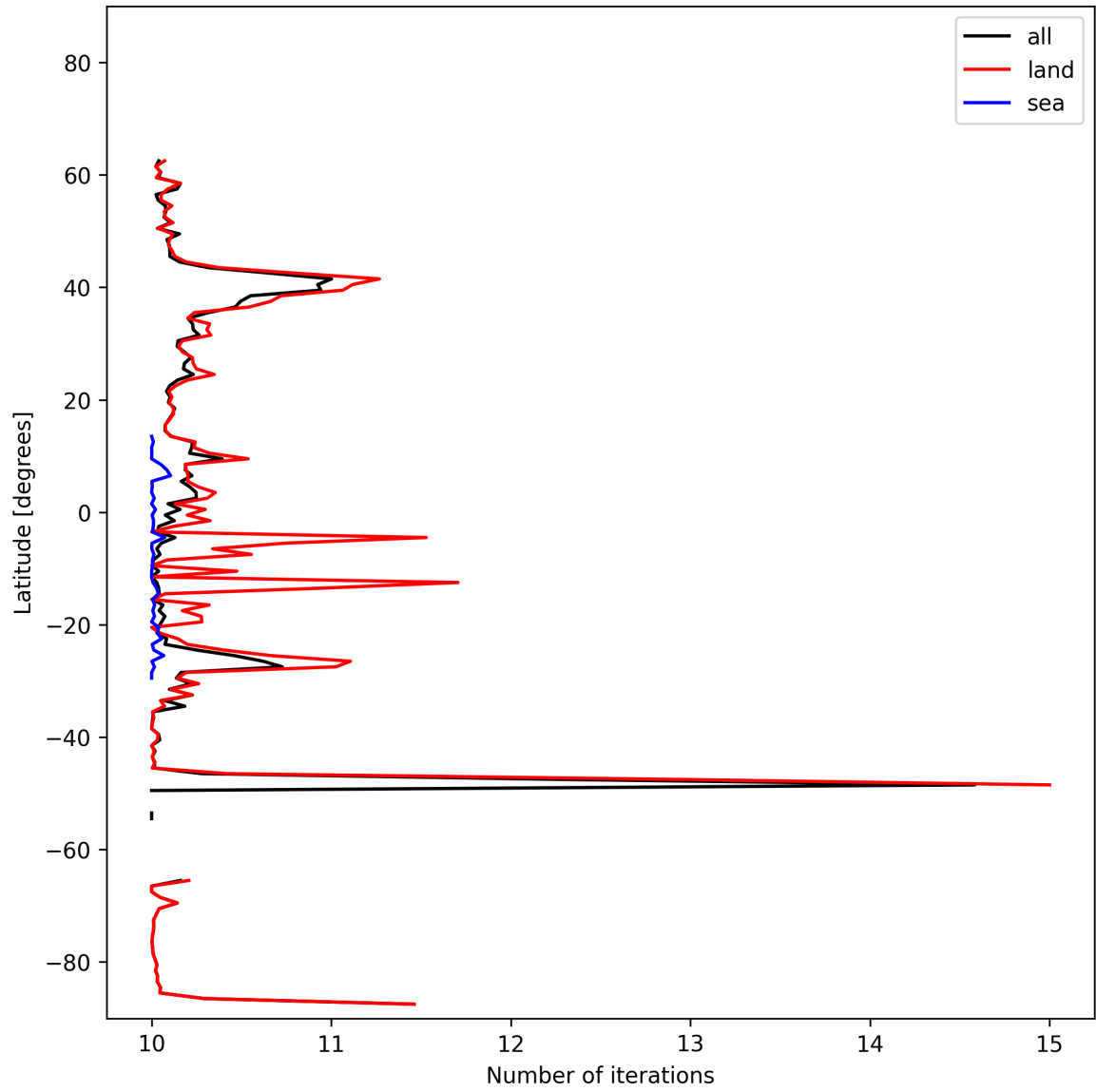
Figure 20: Zonal average of “Number of iterations” for 2025-02-13 to 2025-02-15.
