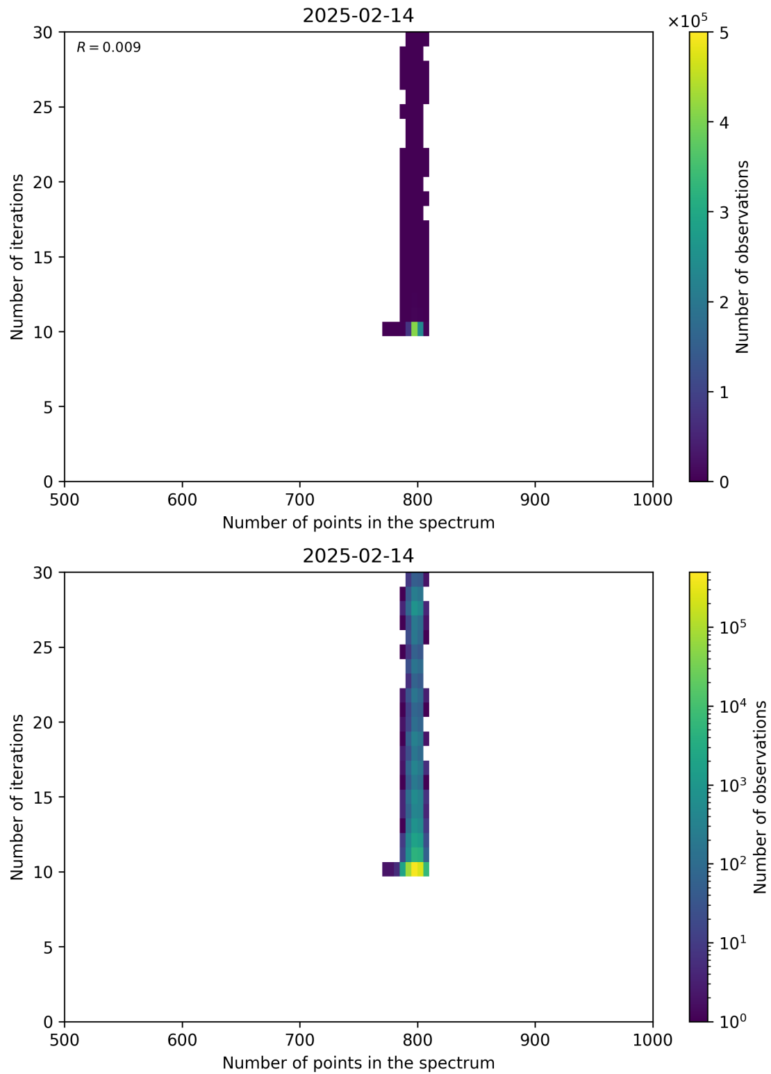
Figure 92: Scatter density plot of “Number of points in the spectrum” against “Number of iterations” for 2025-02-13 to 2025-02-15.
