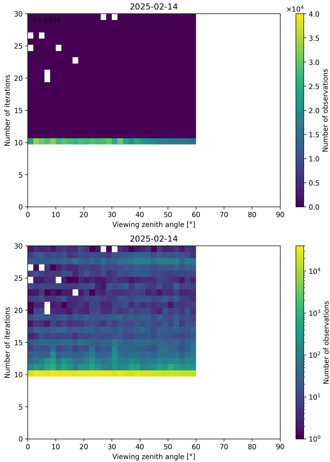
Figure 113: Scatter density plot of “Viewing zenith angle” against “Number of iterations” for 2025-02-13 to 2025-02-15.
