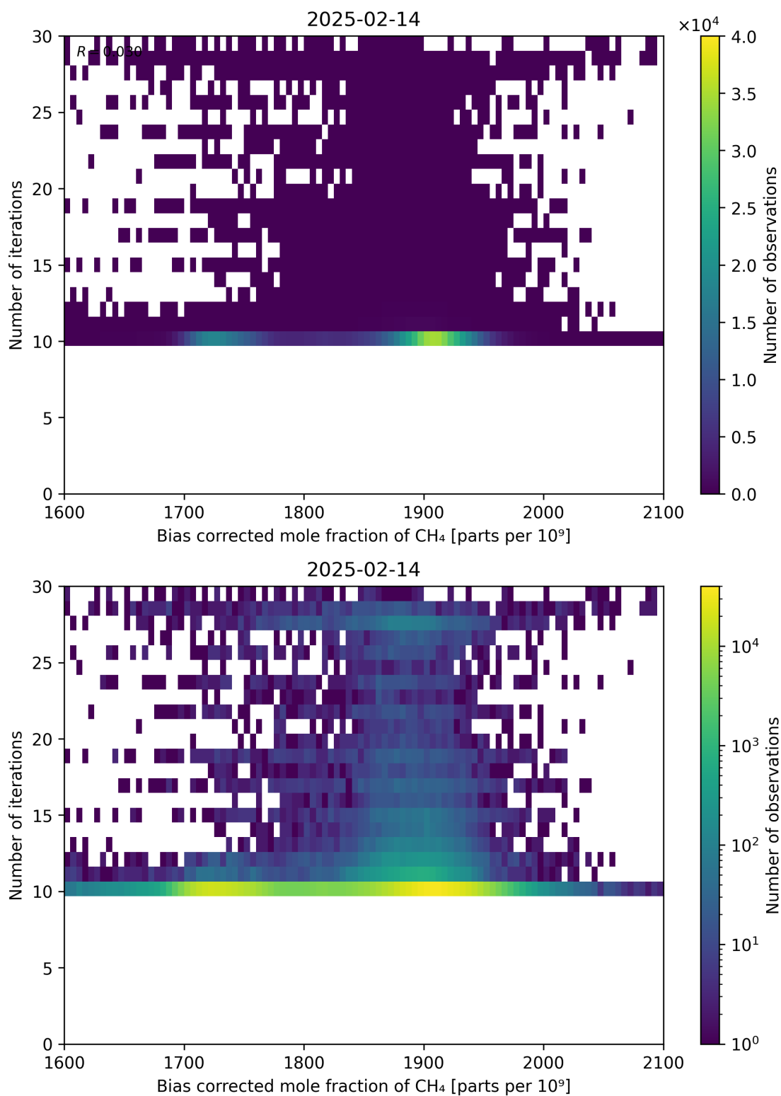
Figure 67: Scatter density plot of “Bias corrected mole fraction of \text{CH}_4 ” against “Number of iterations” for 2025-02-13 to 2025-02-15.
