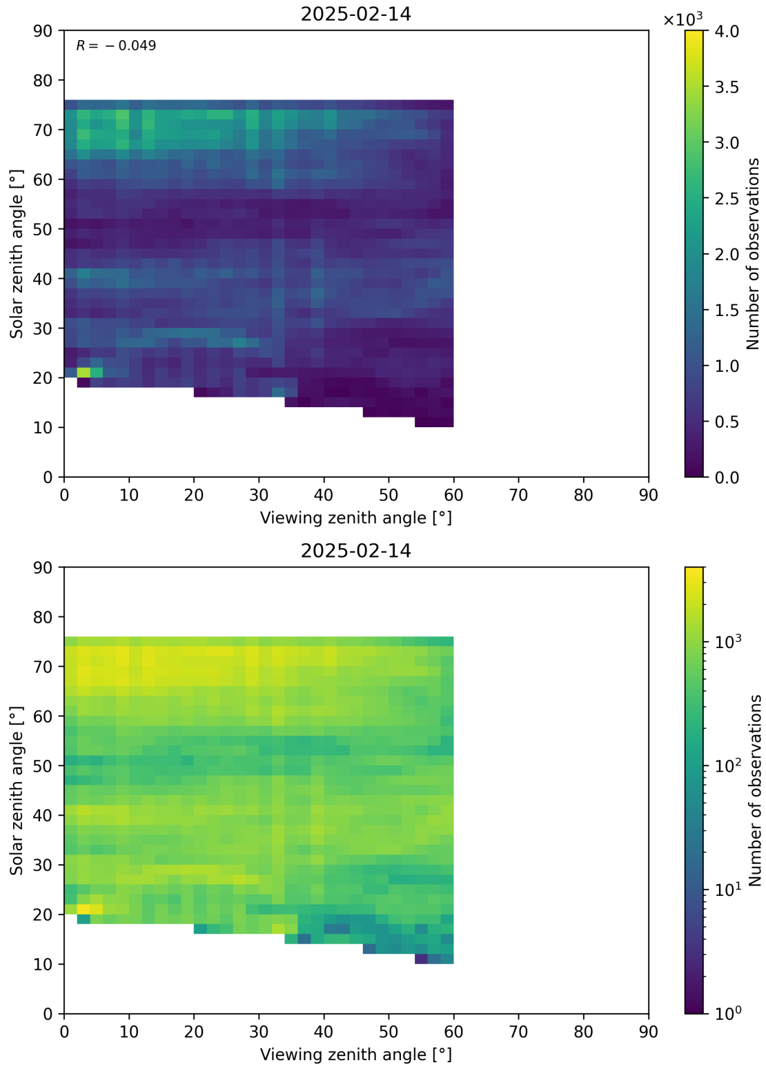
Figure 115: Scatter density plot of “Viewing zenith angle” against “Solar zenith angle” for 2025-02-13 to 2025-02-15.
