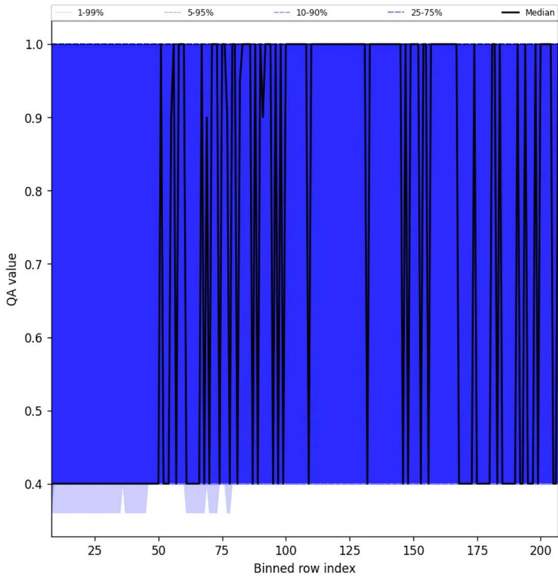
Figure 33: Along track statistics of “QA value” for 2025-02-13 to 2025-02-15
