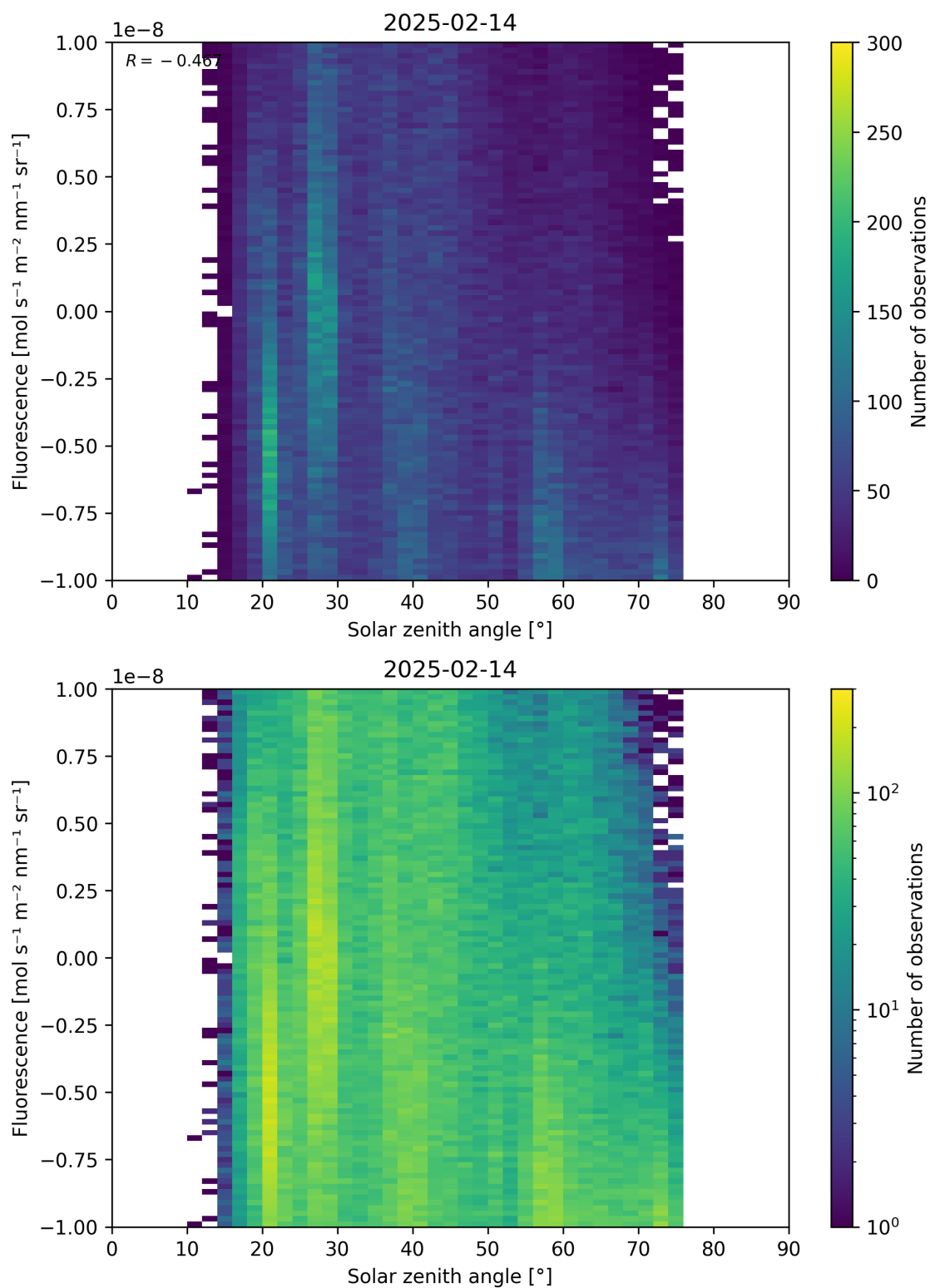
Figure 97: Scatter density plot of “Solar zenith angle” against “Fluorescence” for 2025-02-13 to 2025-02-15.
