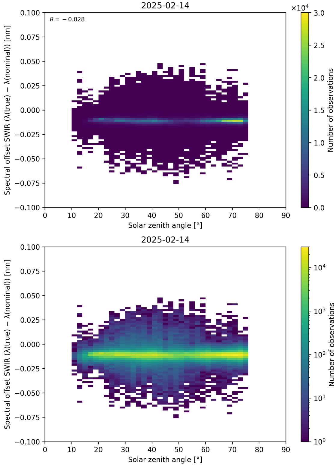
Figure 104: Scatter density plot of “Solar zenith angle” against “Spectral offset SWIR ( \lambda_{\text{true}} - \lambda_{\text{nominal}} )” for 2025-02-13 to 2025-02-15.
