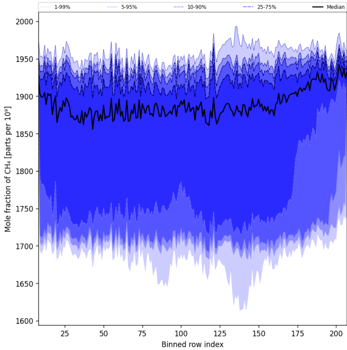
Figure 34: Along track statistics of “Mole fraction of CH 4 ” for 2025-02-13 to 2025-02-15
