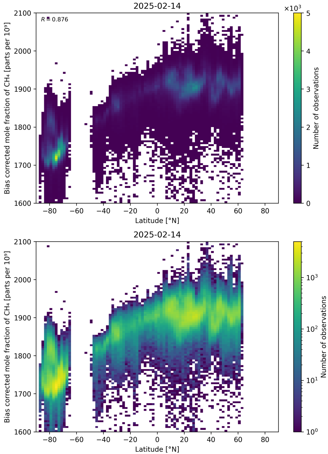
Figure 58: Scatter density plot of “Latitude” against “Bias corrected mole fraction of CH 4 ” for 2025-02-13 to 2025-02-15.
