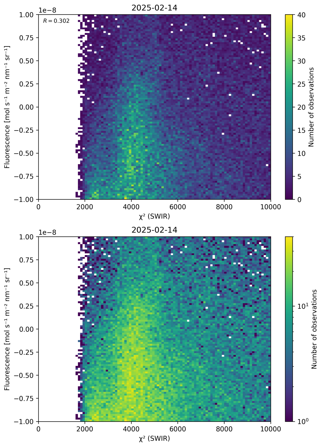
Figure 49: Scatter density plot of “ \chi^2 (SWIR)” against “Fluorescence” for 2025-02-13 to 2025-02-15.
