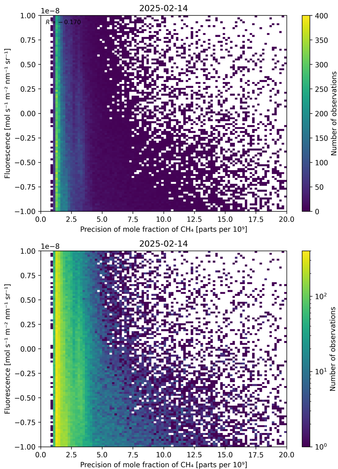
Figure 81: Scatter density plot of “Precision of mole fraction of CH 4 ” against “Fluorescence” for 2025-02-13 to 2025-02-15.
