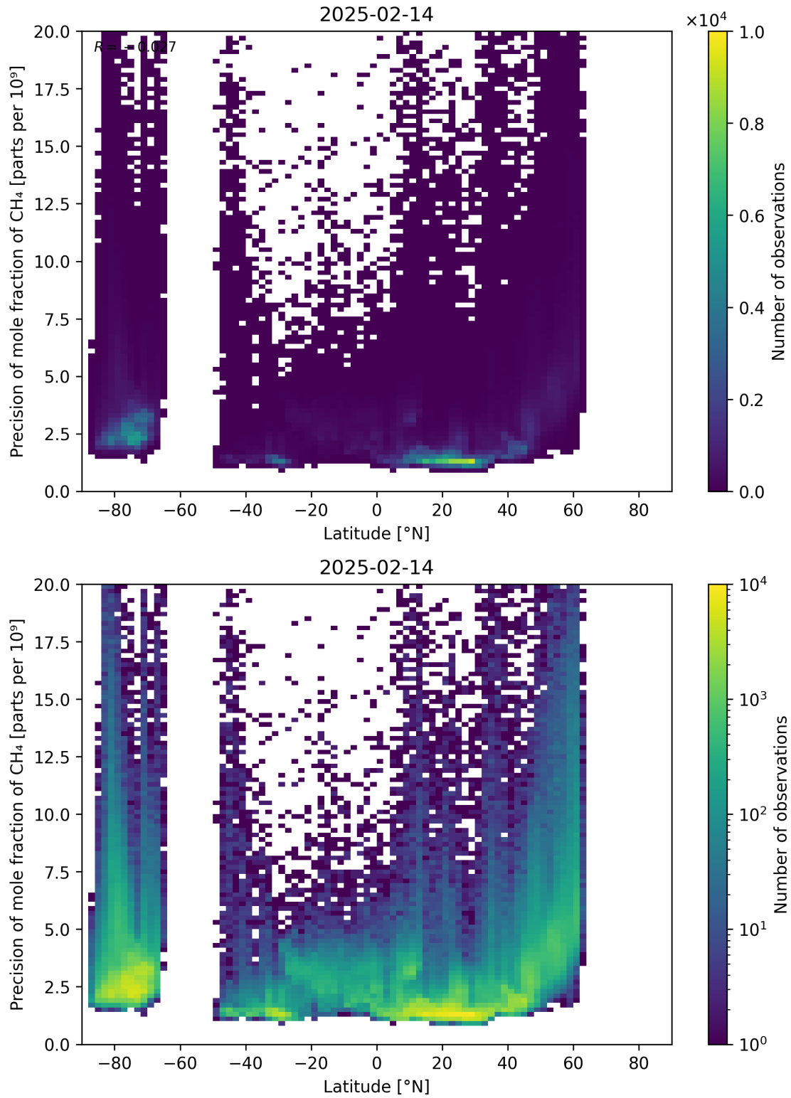
Figure 59: Scatter density plot of “Latitude” against “Precision of mole fraction of CH 4 ” for 2025-02-13 to 2025-02-15.
