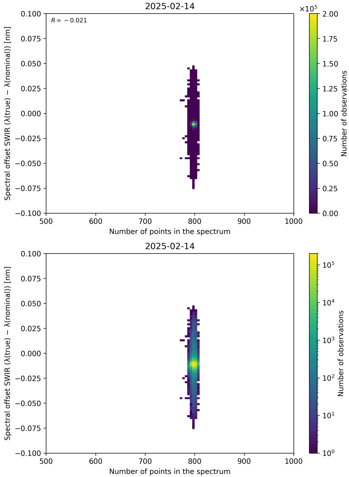
Figure 93: Scatter density plot of “Number of points in the spectrum” against “Spectral offset SWIR ( \lambda_{\text{true}} - \lambda_{\text{nominal}} )” for 2025-02-13 to 2025-02-15.
