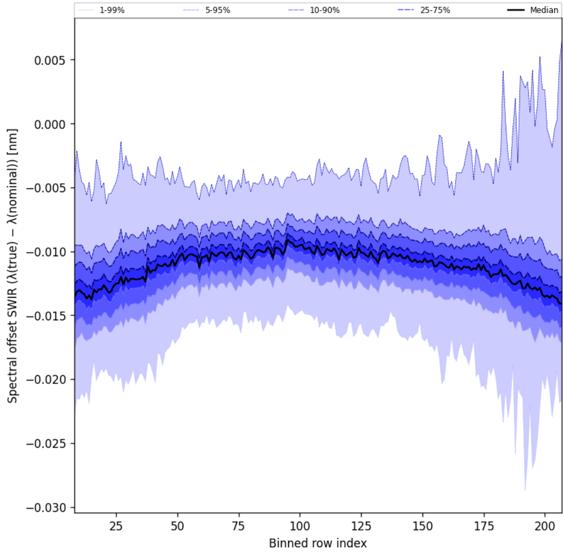
Figure 38: Along track statistics of “Spectral offset SWIR ( \lambda_{\text{true}} - \lambda_{\text{nominal}} )” for 2025-02-13 to 2025-02-15
