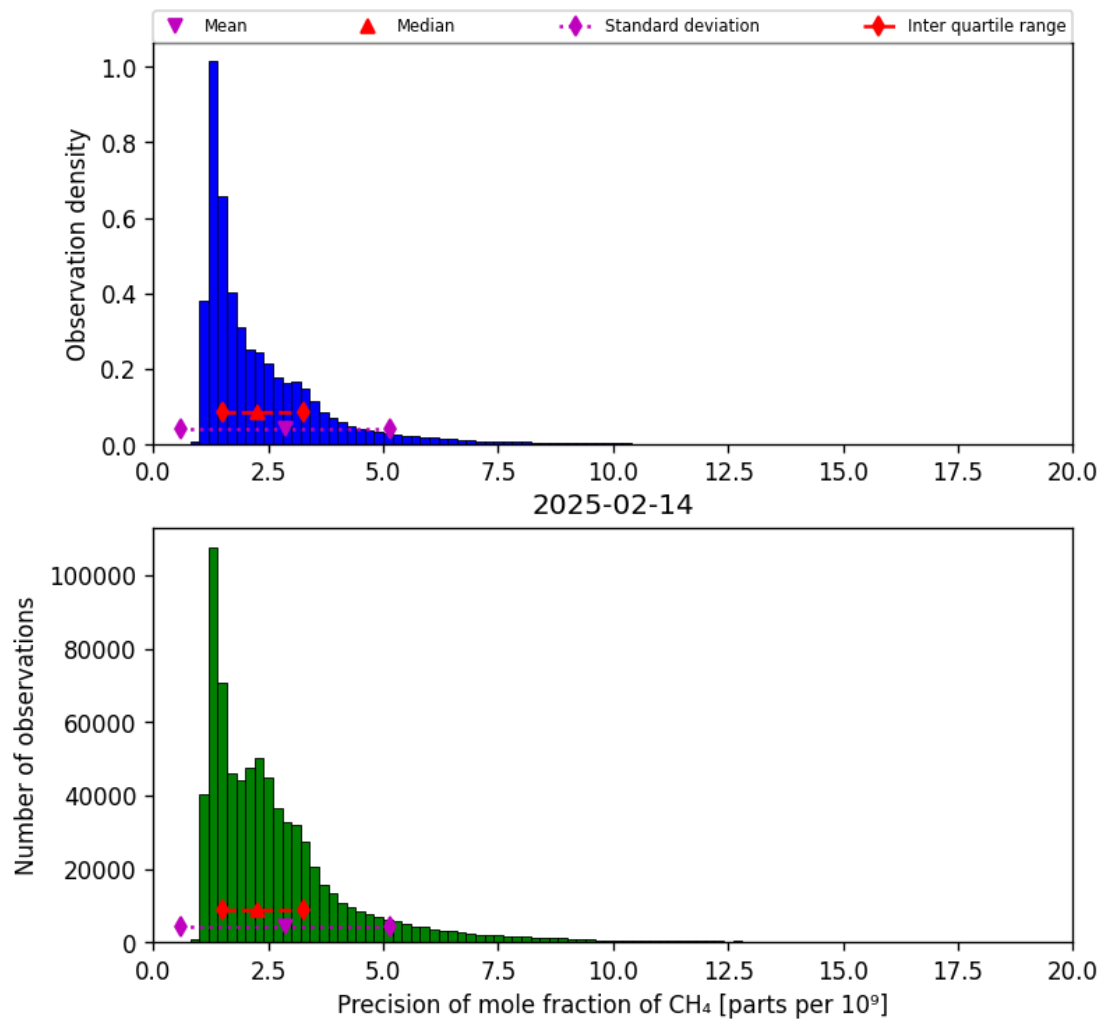
Figure 24: Histogram of “Precision of mole fraction of CH 4 ” for 2025-02-13 to 2025-02-15
