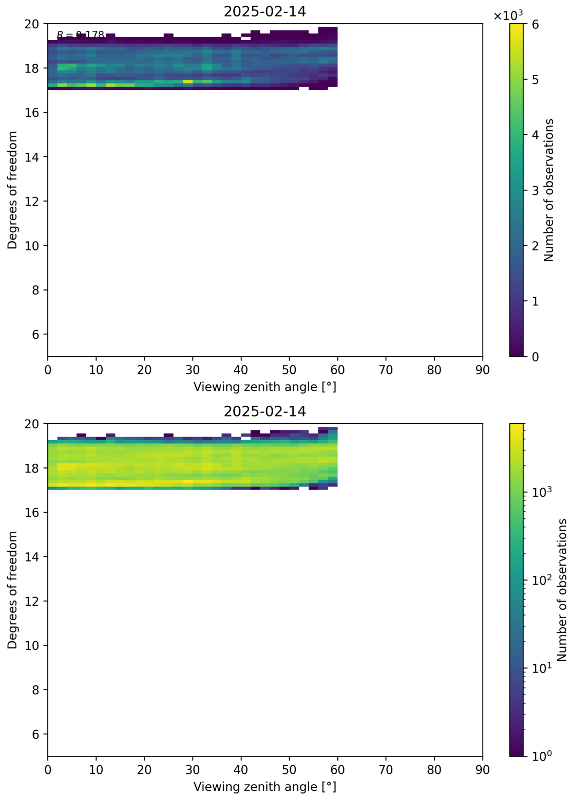
Figure 107: Scatter density plot of “Viewing zenith angle” against “Degrees of freedom” for 2025-02-13 to 2025-02-15.
