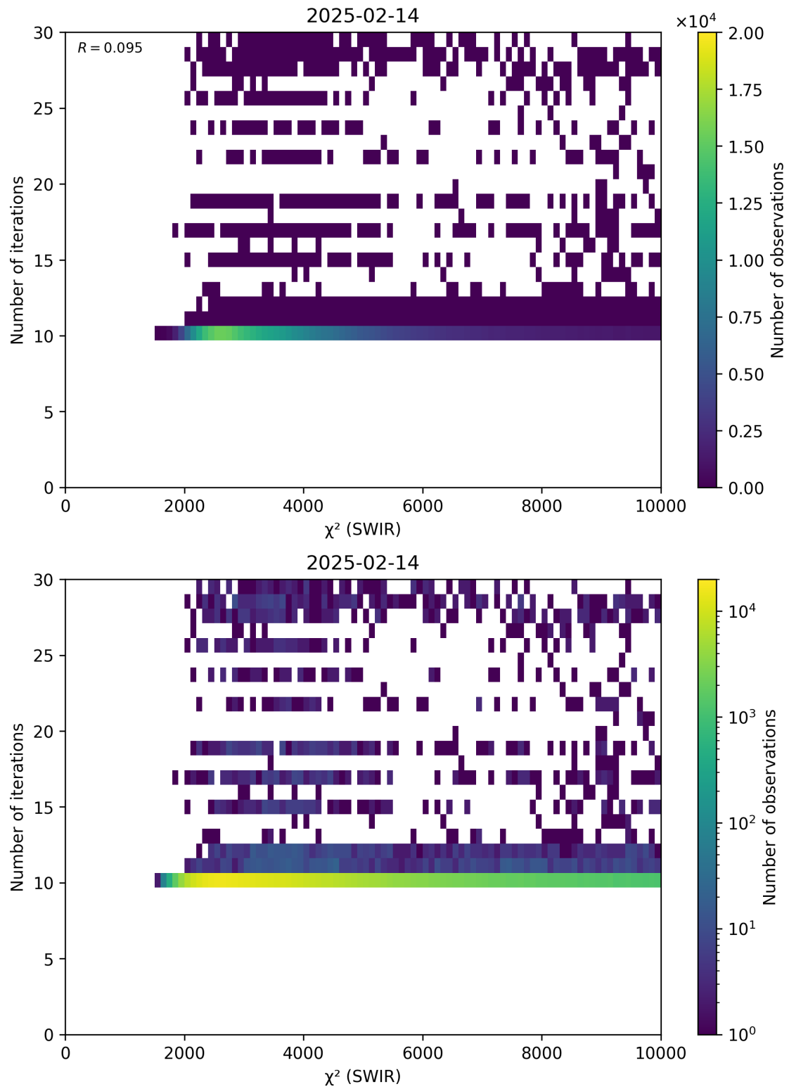
Figure 50: Scatter density plot of “ \chi^2 (SWIR)” against “Number of iterations” for 2025-02-13 to 2025-02-15.
