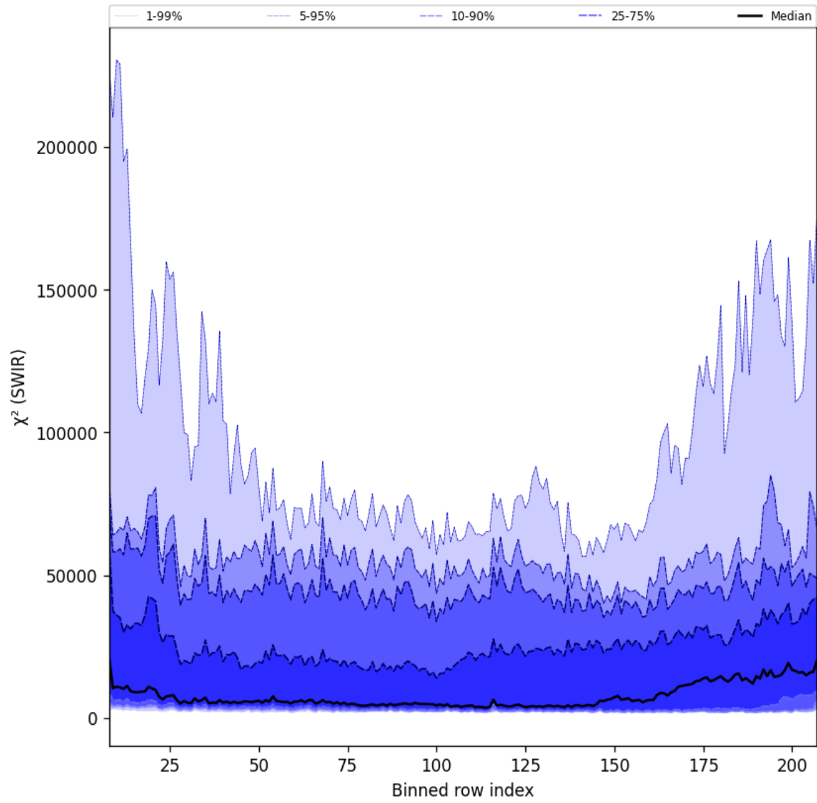
Figure 39: Along track statistics of “ \chi^2 (SWIR)” for 2025-02-13 to 2025-02-15
