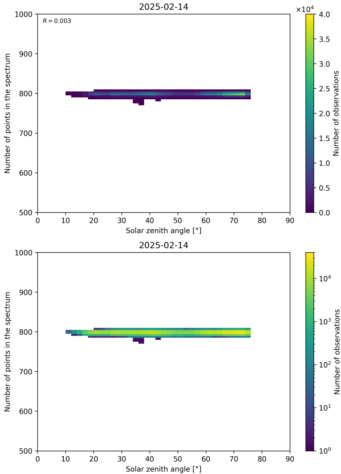
Figure 103: Scatter density plot of “Solar zenith angle” against “Number of points in the spectrum” for 2025-02-13 to 2025-02-15.
