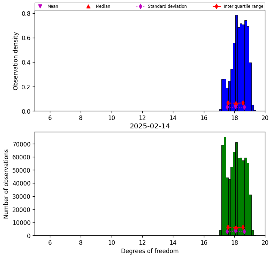
Figure 30: Histogram of “Degrees of freedom” for 2025-02-13 to 2025-02-15
