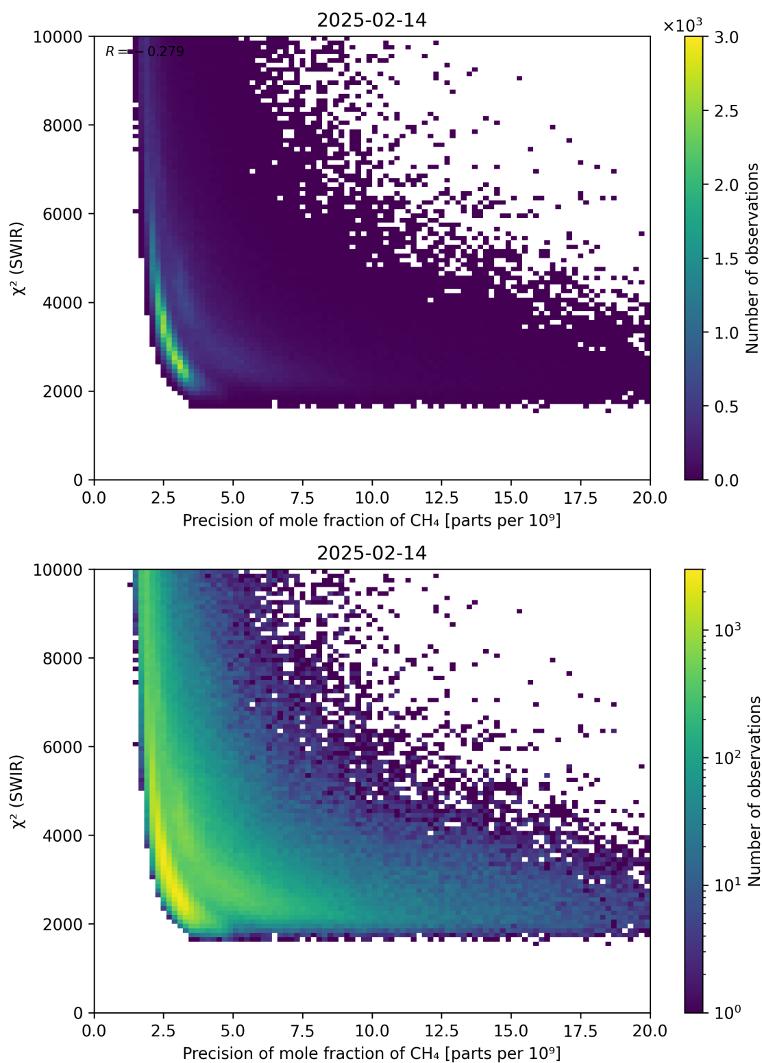
Figure 79: Scatter density plot of “Precision of mole fraction of \text{CH}_4 ” against “ \chi^2 (SWIR)” for 2025-02-13 to 2025-02-15.
