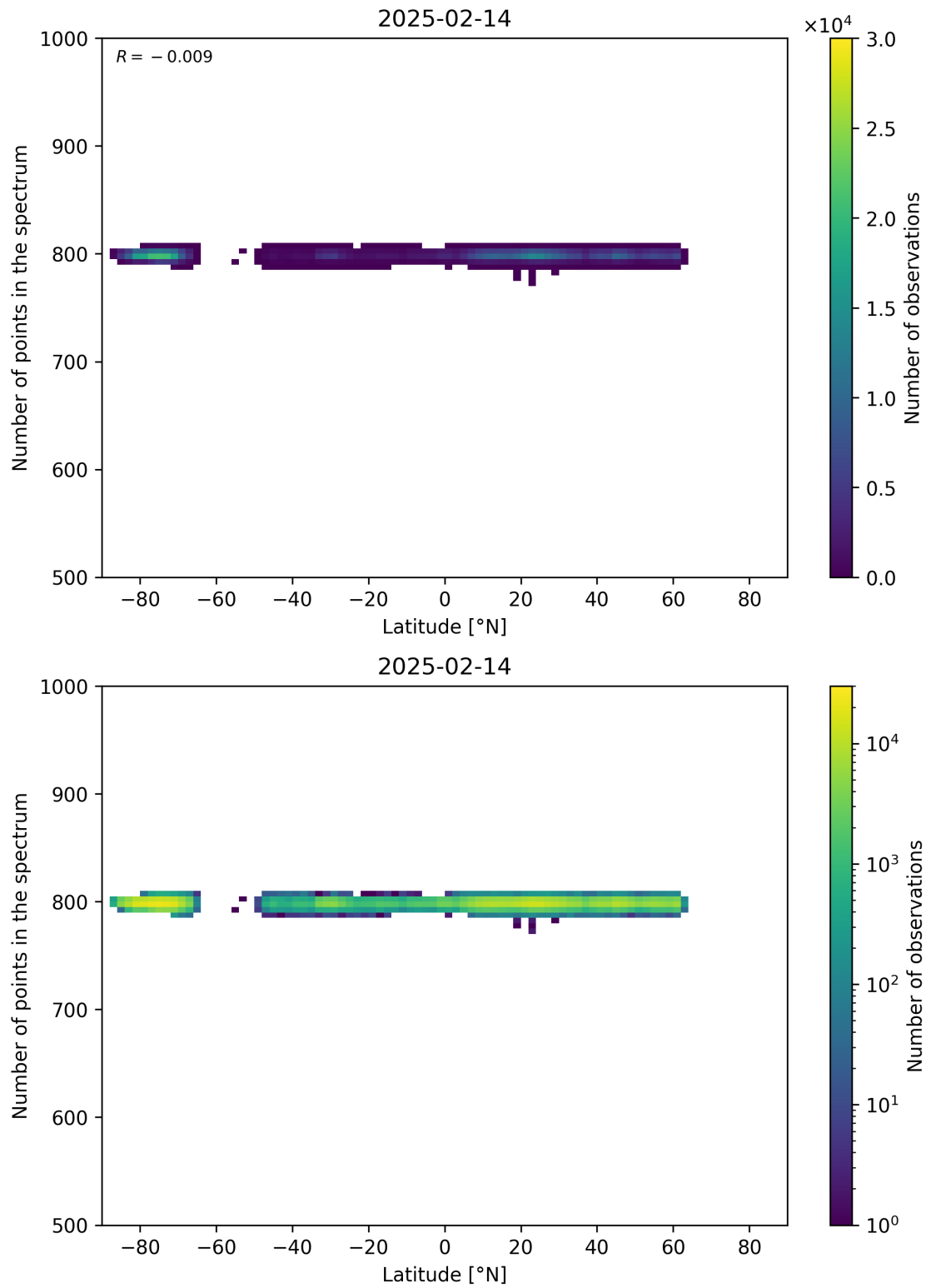
Figure 61: Scatter density plot of “Latitude” against “Number of points in the spectrum” for 2025-02-13 to 2025-02-15.
