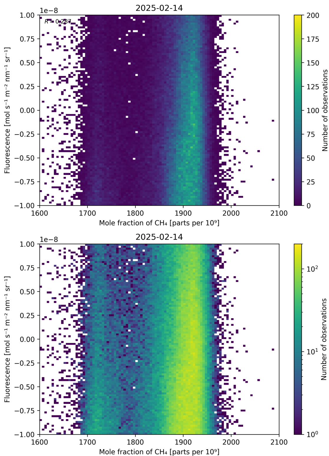
Figure 73: Scatter density plot of “Mole fraction of \text{CH}_4 ” against “Fluorescence” for 2025-02-13 to 2025-02-15.
