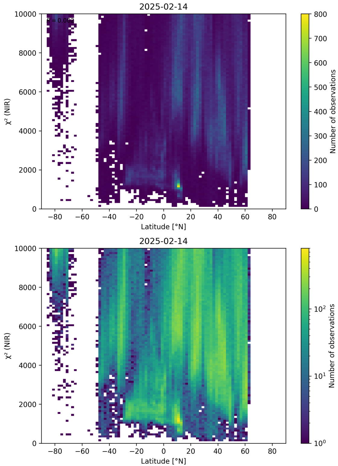
Figure 53: Scatter density plot of “Latitude” against “ \chi^2 (NIR)” for 2025-02-13 to 2025-02-15.
