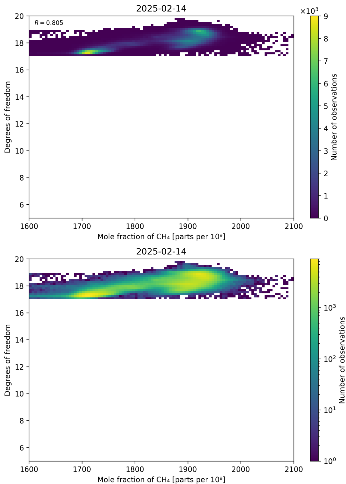
Figure 72: Scatter density plot of “Mole fraction of CH 4 ” against “Degrees of freedom” for 2025-02-13 to 2025-02-15.
