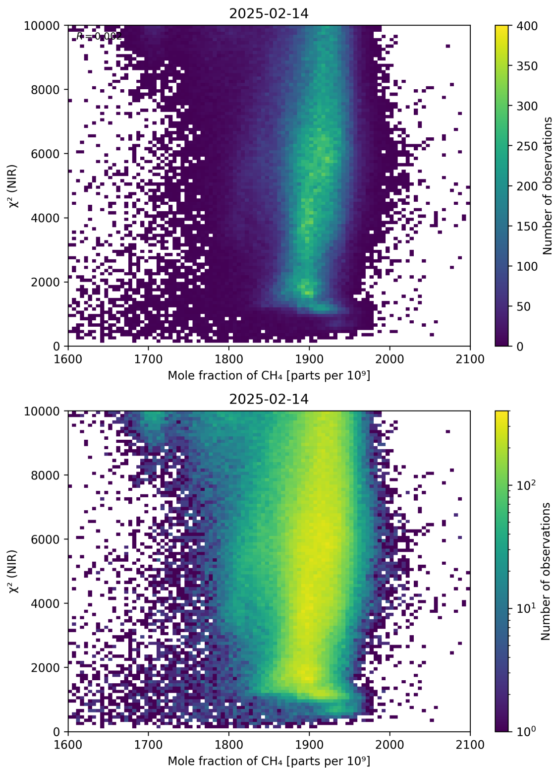
Figure 70: Scatter density plot of “Mole fraction of \text{CH}_4 ” against “ \chi^2 (NIR)” for 2025-02-13 to 2025-02-15.
