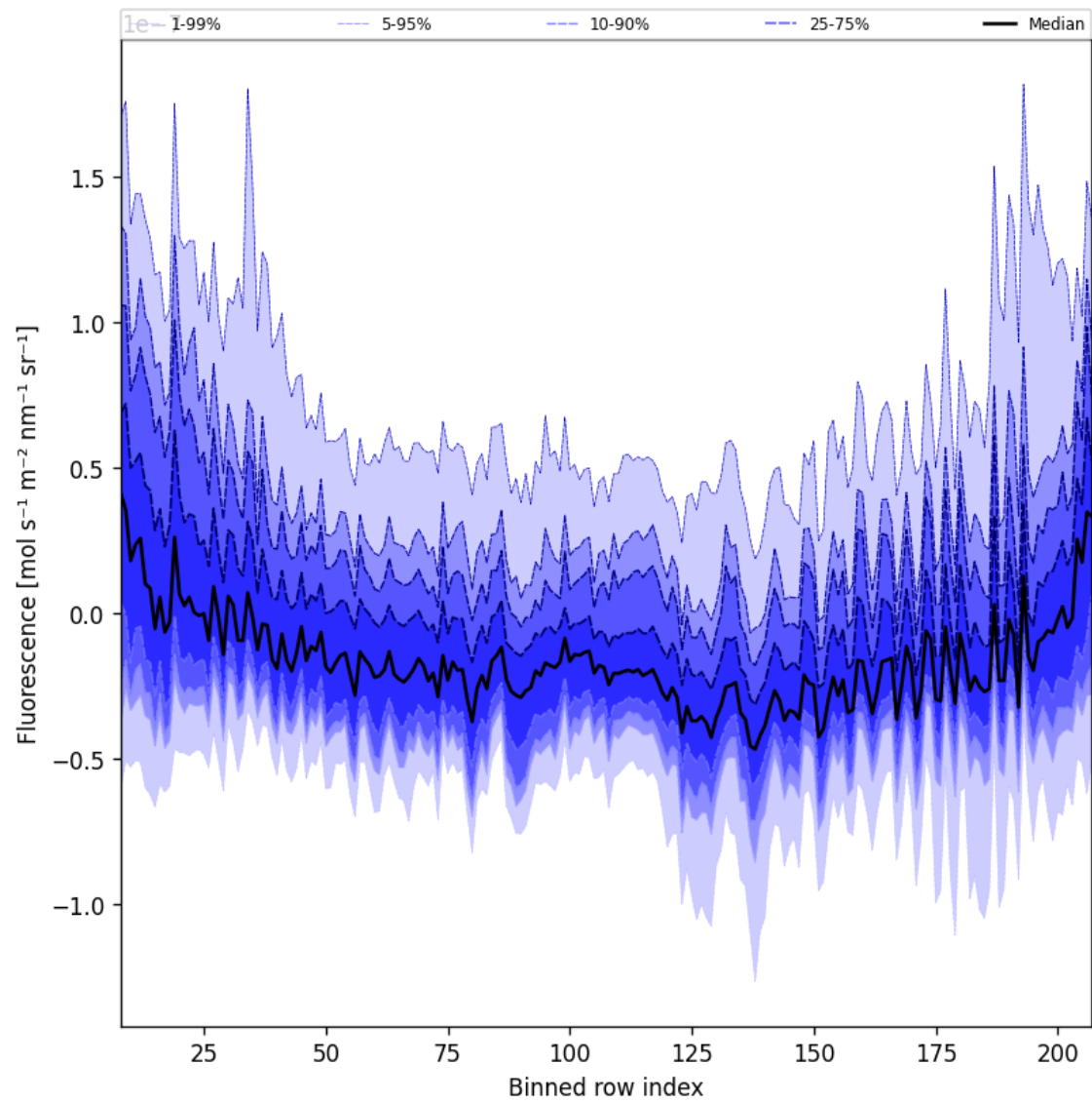
Figure 43: Along track statistics of "Fluorescence" for 2025-02-13 to 2025-02-15
