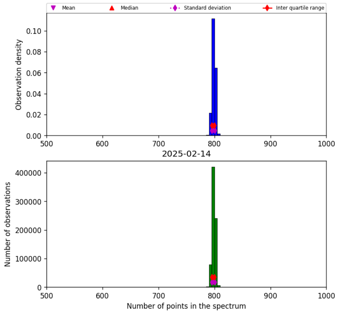
Figure 26: Histogram of “Number of points in the spectrum” for 2025-02-13 to 2025-02-15
