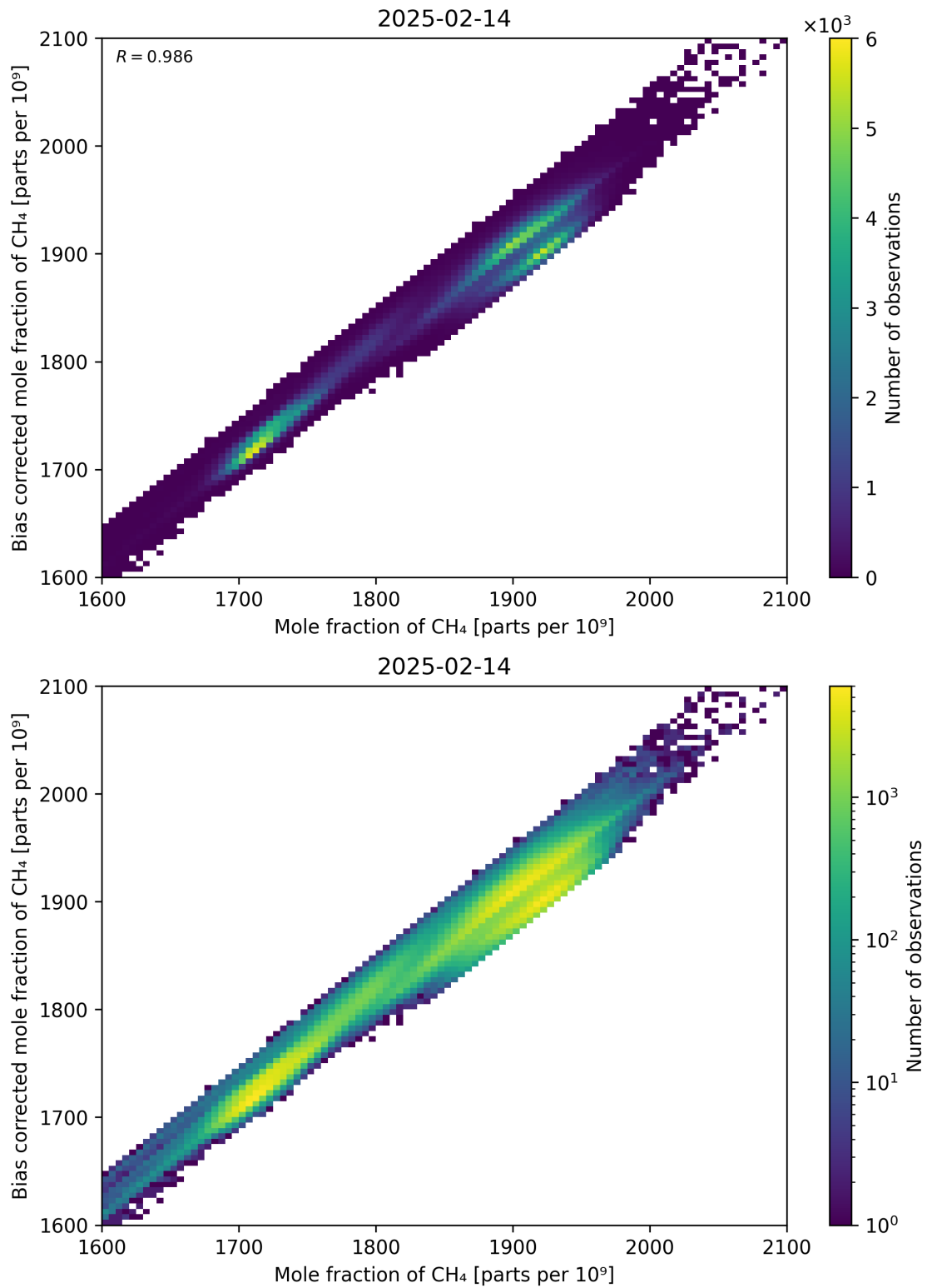
Figure 74: Scatter density plot of “Mole fraction of CH 4 ” against “Bias corrected mole fraction of CH 4 ” for 2025-02-13 to 2025-02-15.
