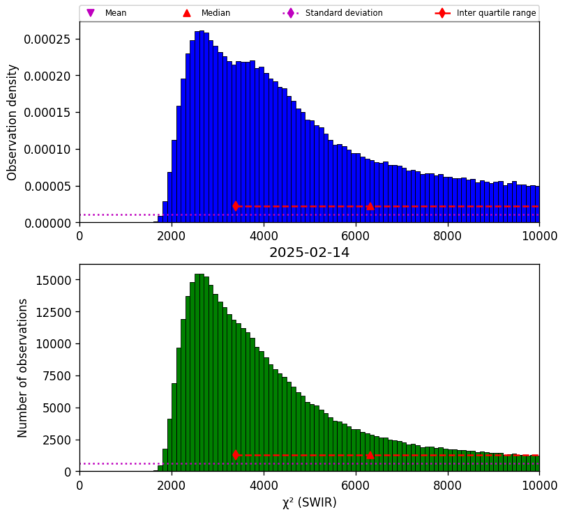
Figure 28: Histogram of “ \chi^2 (SWIR)” for 2025-02-13 to 2025-02-15
