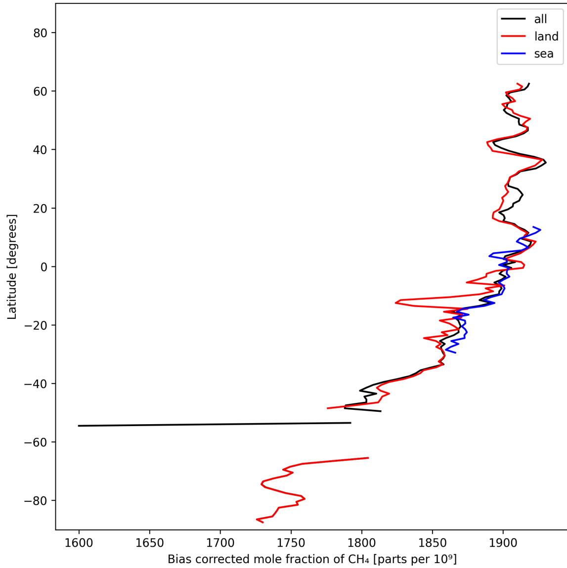
Figure 14: Zonal average of “Bias corrected mole fraction of CH 4 ” for 2025-02-13 to 2025-02-15.
