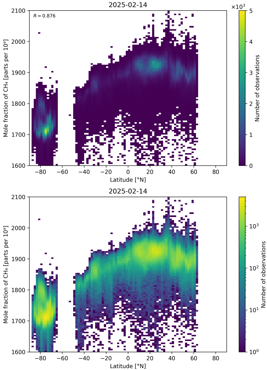
Figure 57: Scatter density plot of “Latitude” against “Mole fraction of CH 4 ” for 2025-02-13 to 2025-02-15.
