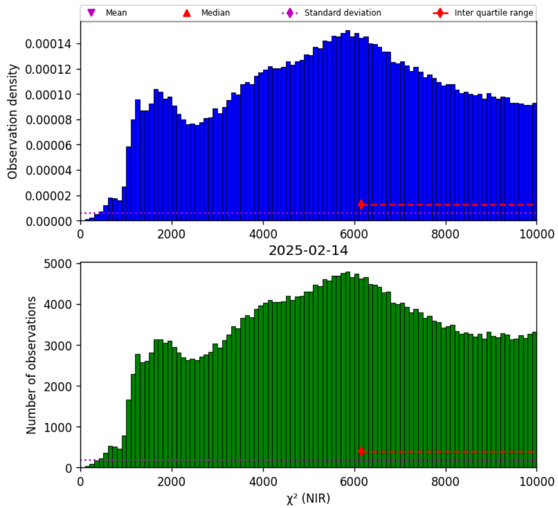
Figure 29: Histogram of “ \chi^2 (NIR)” for 2025-02-13 to 2025-02-15
