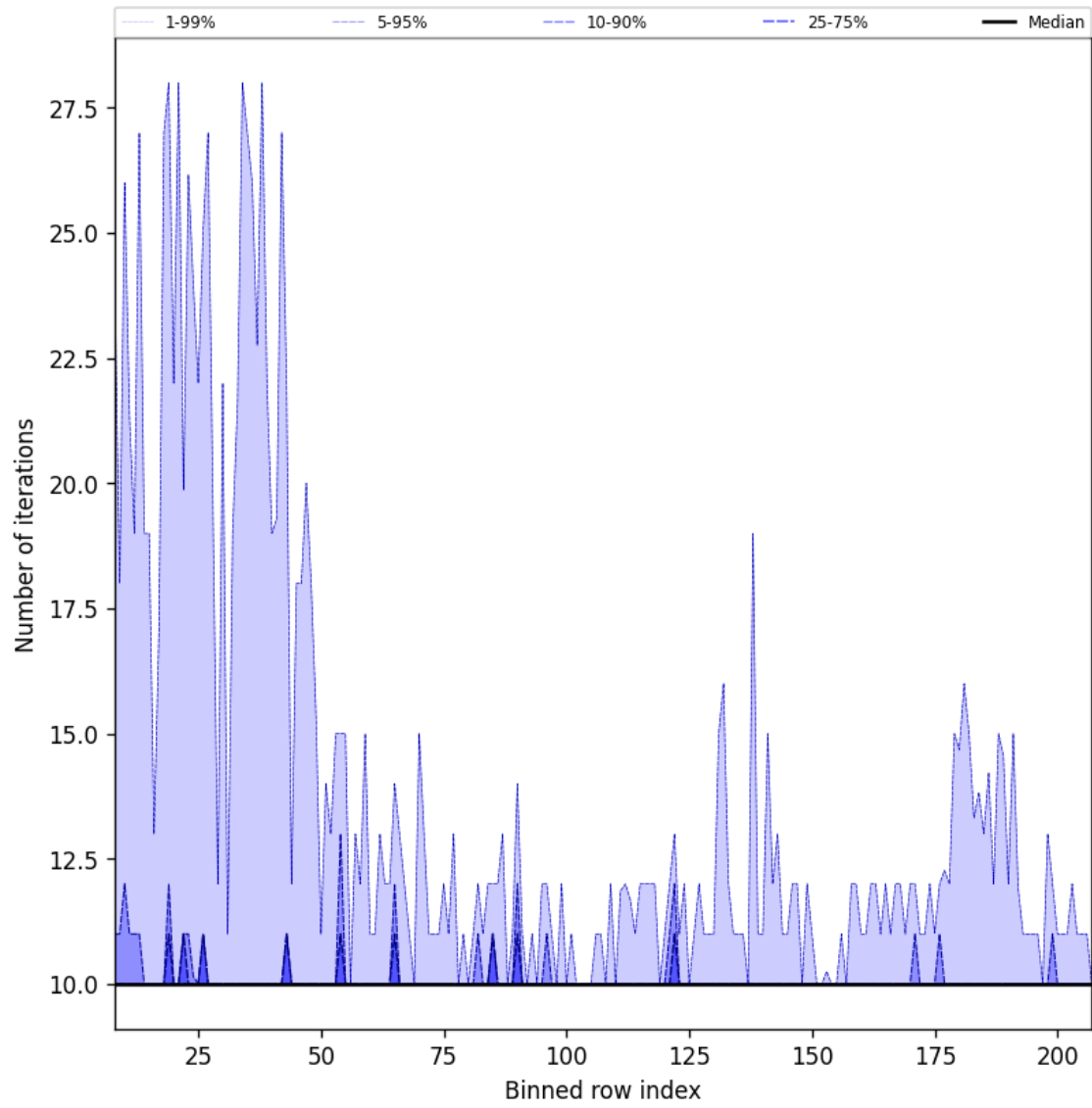
Figure 42: Along track statistics of “Number of iterations” for 2025-02-13 to 2025-02-15
