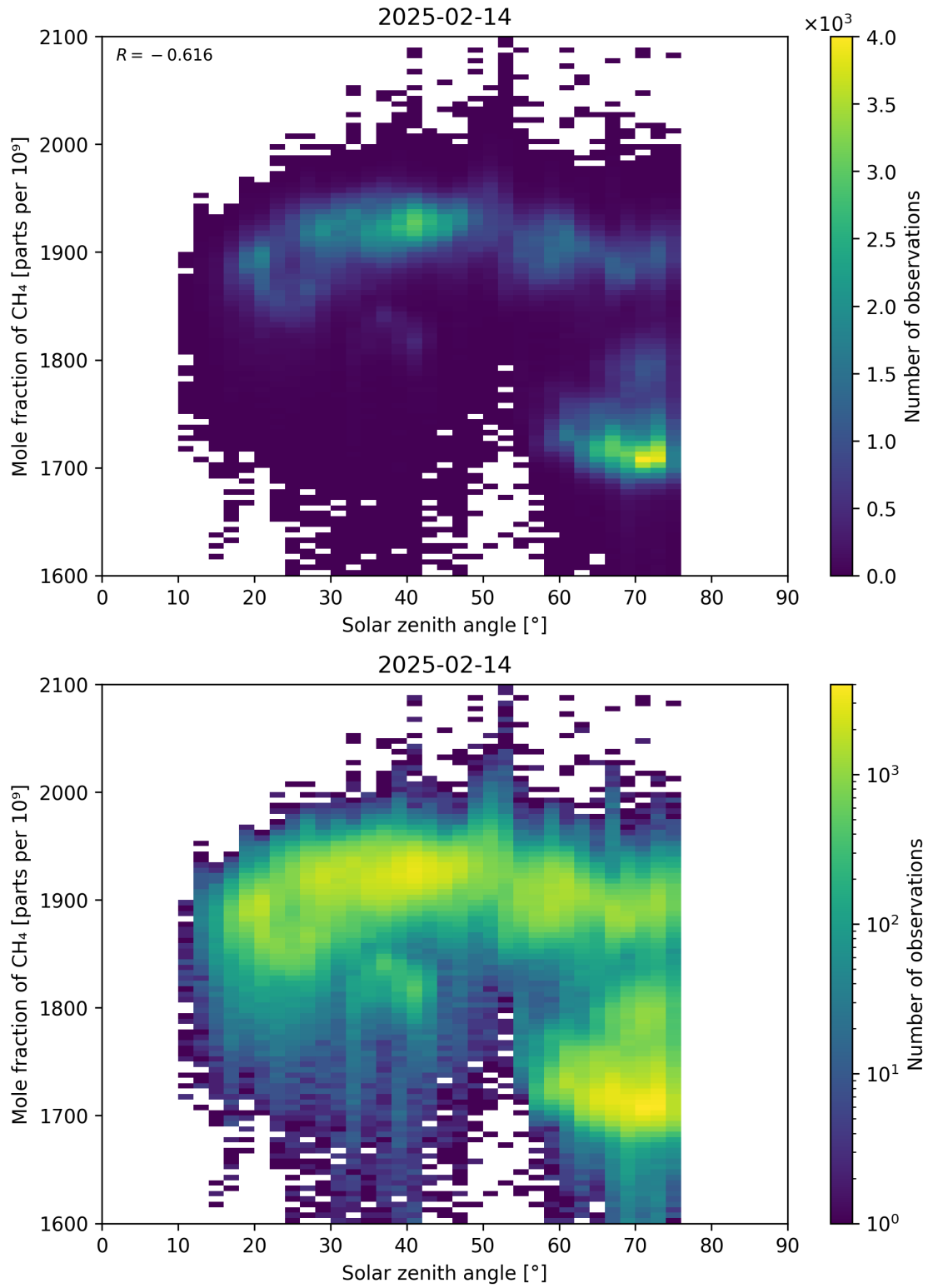
Figure 99: Scatter density plot of “Solar zenith angle” against “Mole fraction of CH 4 ” for 2025-02-13 to 2025-02-15.
