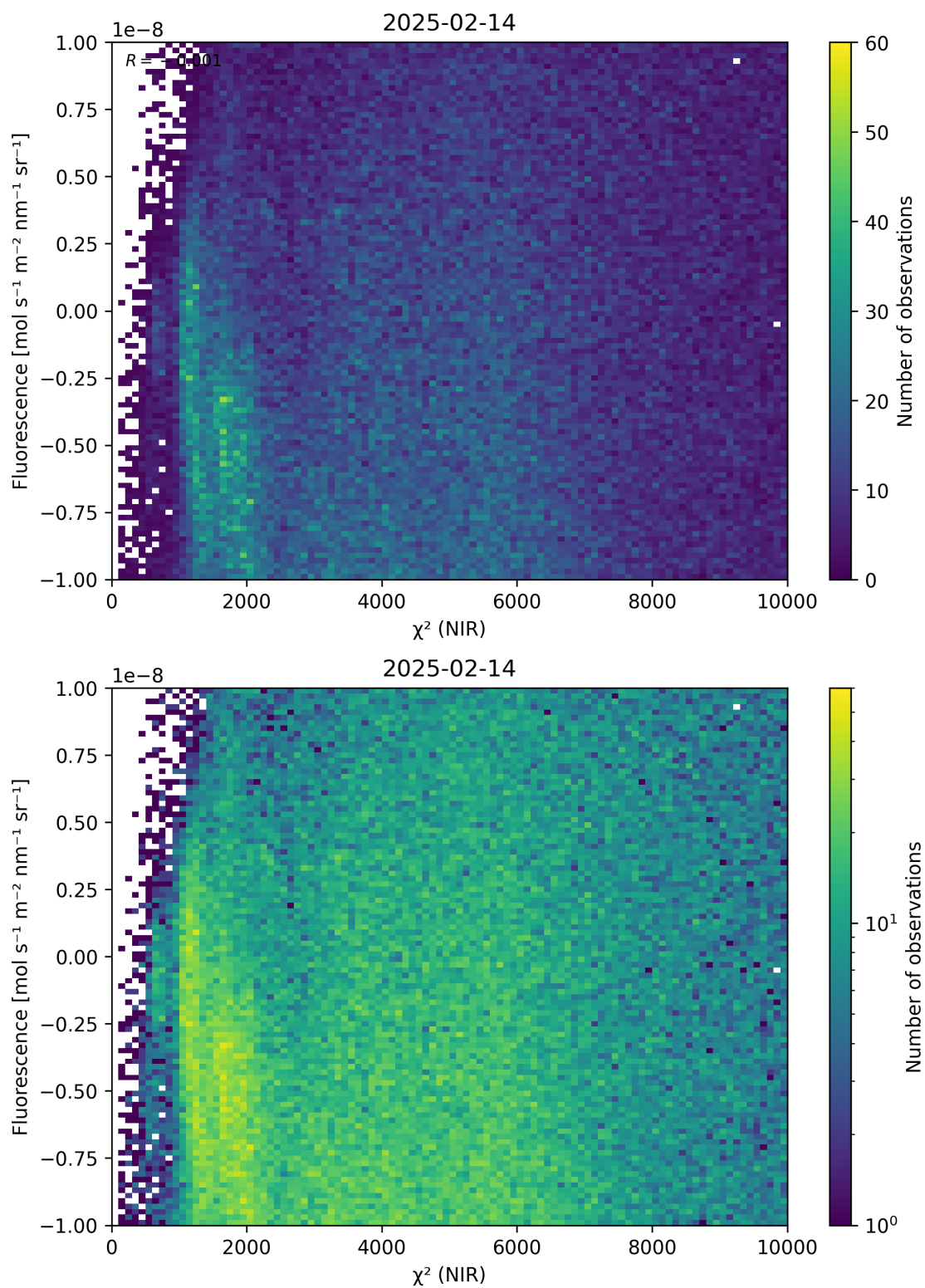
Figure 45: Scatter density plot of “ \chi^2 (NIR)” against “Fluorescence” for 2025-02-13 to 2025-02-15.
