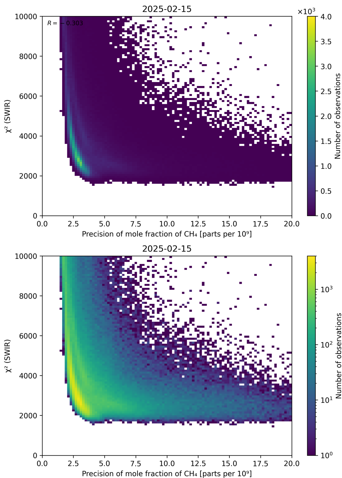
Figure 79: Scatter density plot of “Precision of mole fraction of \text{CH}_4 ” against “ \chi^2 (SWIR)” for 2025-02-14 to 2025-02-16.
