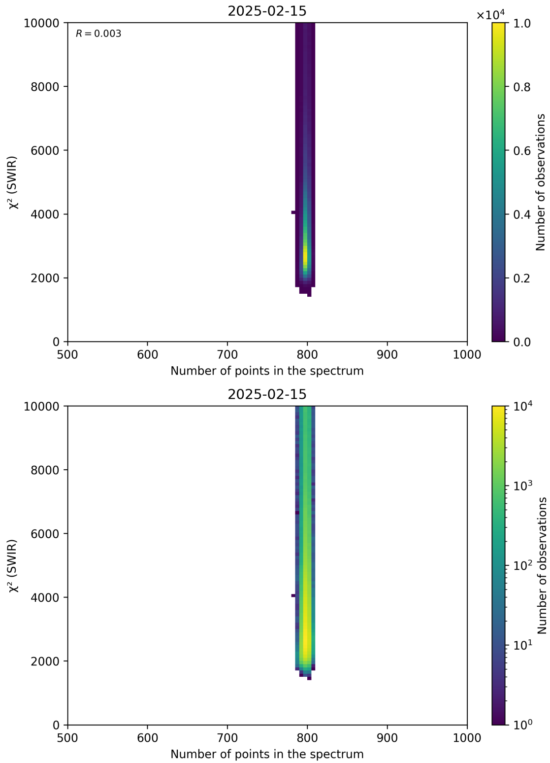
Figure 89: Scatter density plot of “Number of points in the spectrum” against “ \chi^2 (SWIR)” for 2025-02-14 to 2025-02-16.
