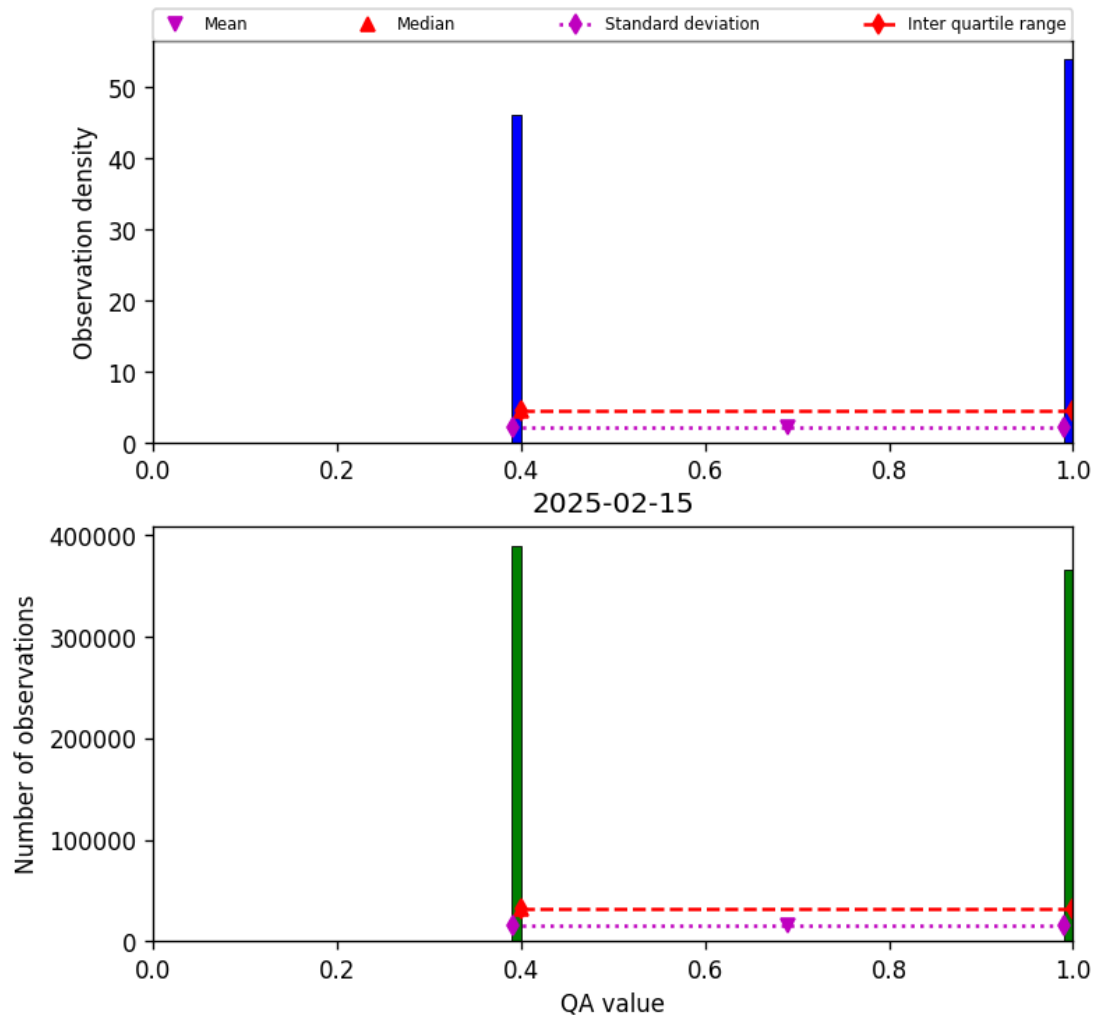
Figure 22: Histogram of “QA value” for 2025-02-14 to 2025-02-16
