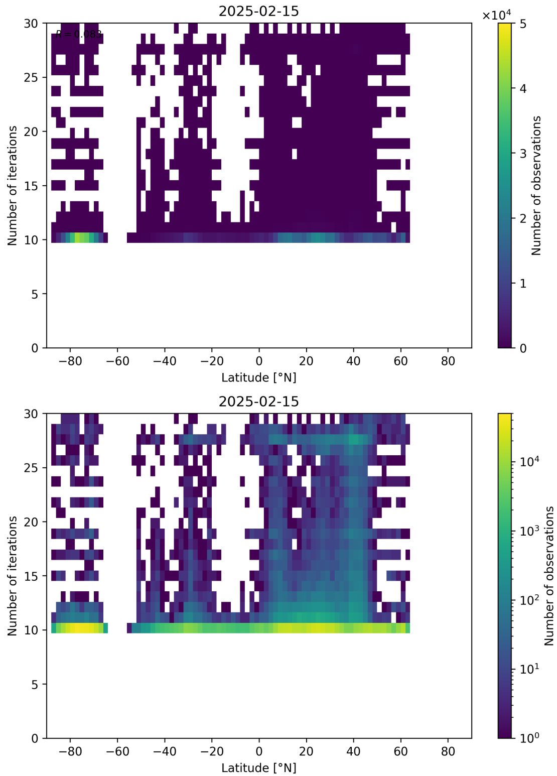
Figure 60: Scatter density plot of “Latitude” against “Number of iterations” for 2025-02-14 to 2025-02-16.
