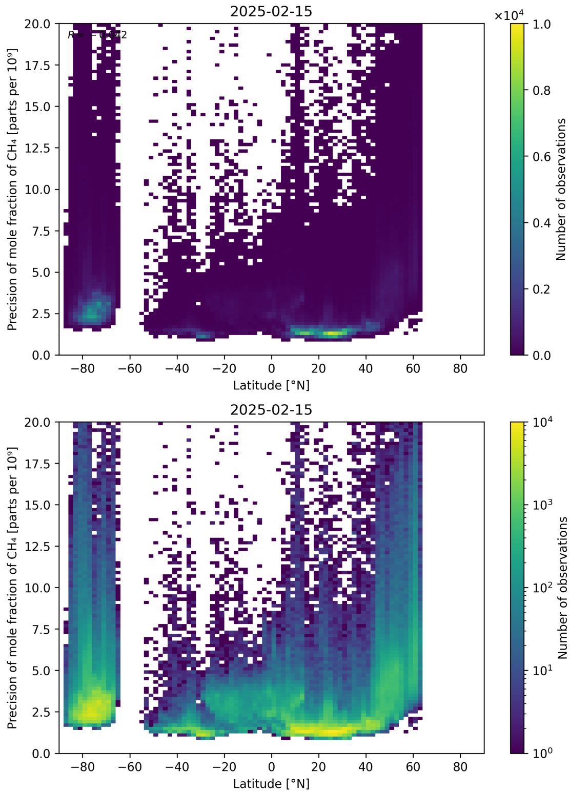
Figure 59: Scatter density plot of “Latitude” against “Precision of mole fraction of CH 4 ” for 2025-02-14 to 2025-02-16.
