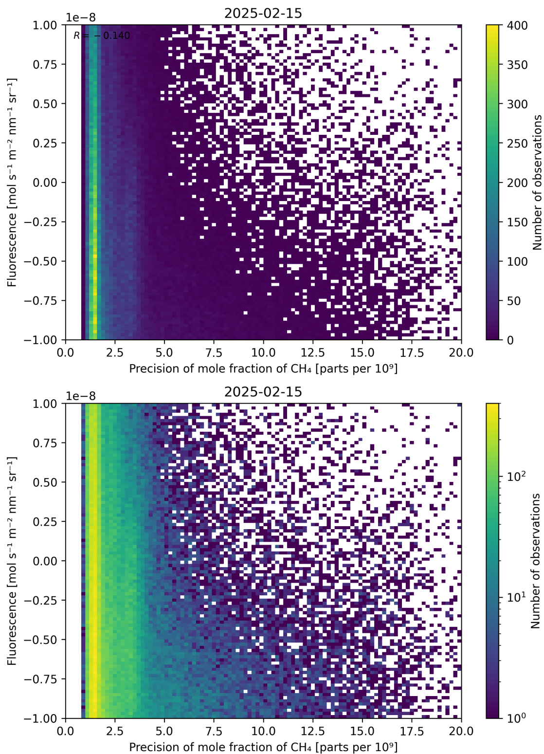
Figure 81: Scatter density plot of “Precision of mole fraction of \text{CH}_4 ” against “Fluorescence” for 2025-02-14 to 2025-02-16.
