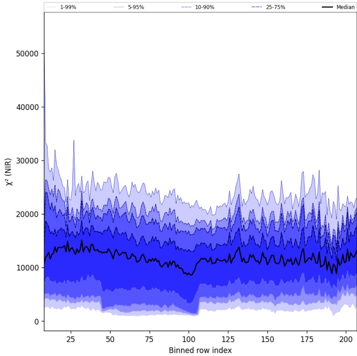
Figure 40: Along track statistics of “ \chi^2 (NIR)” for 2025-02-14 to 2025-02-16
