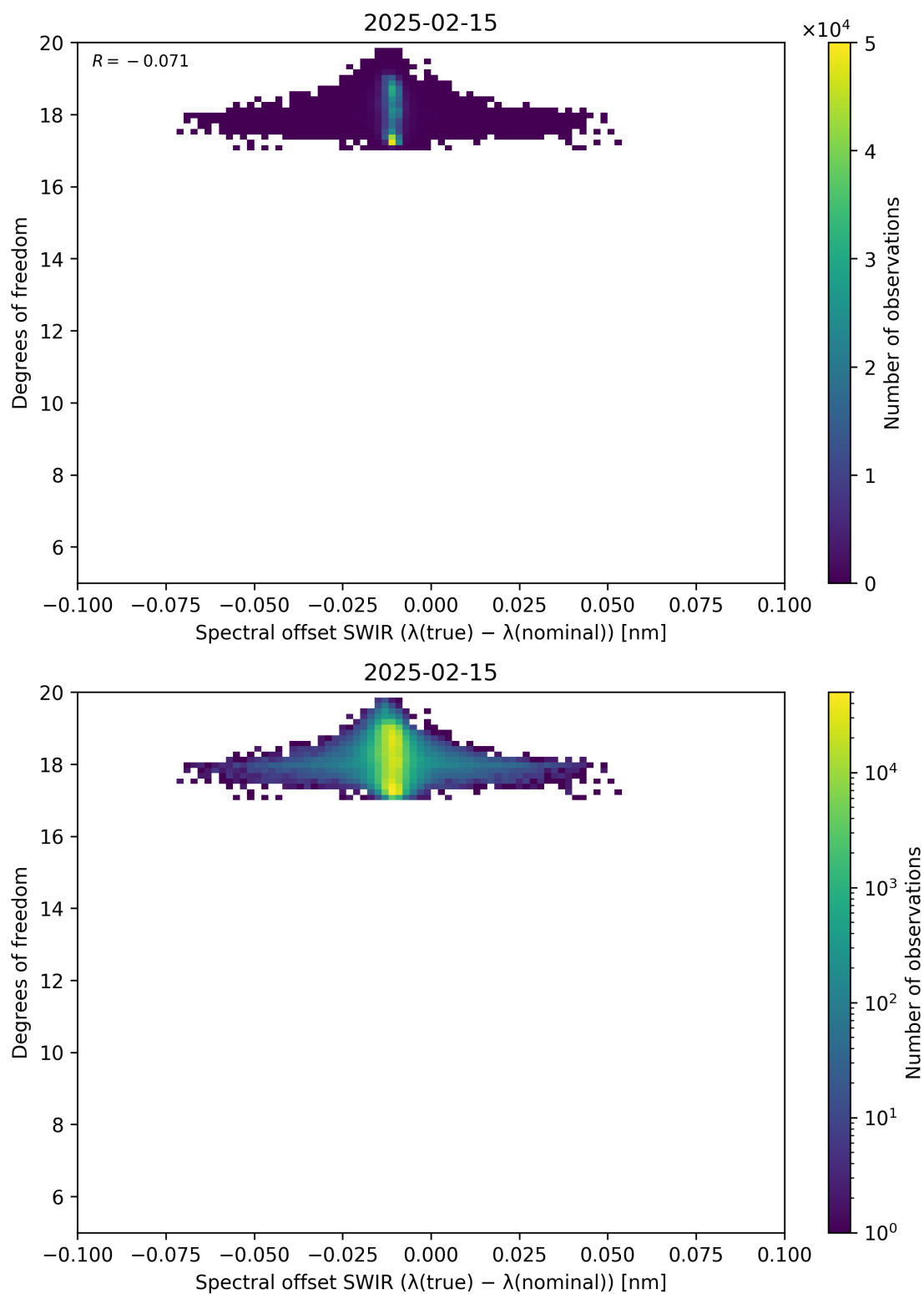
Figure 119: Scatter density plot of “Spectral offset SWIR ( \lambda_{\text{true}} - \lambda_{\text{nominal}} )” against “Degrees of freedom” for 2025-02-14 to 2025-02-16.
