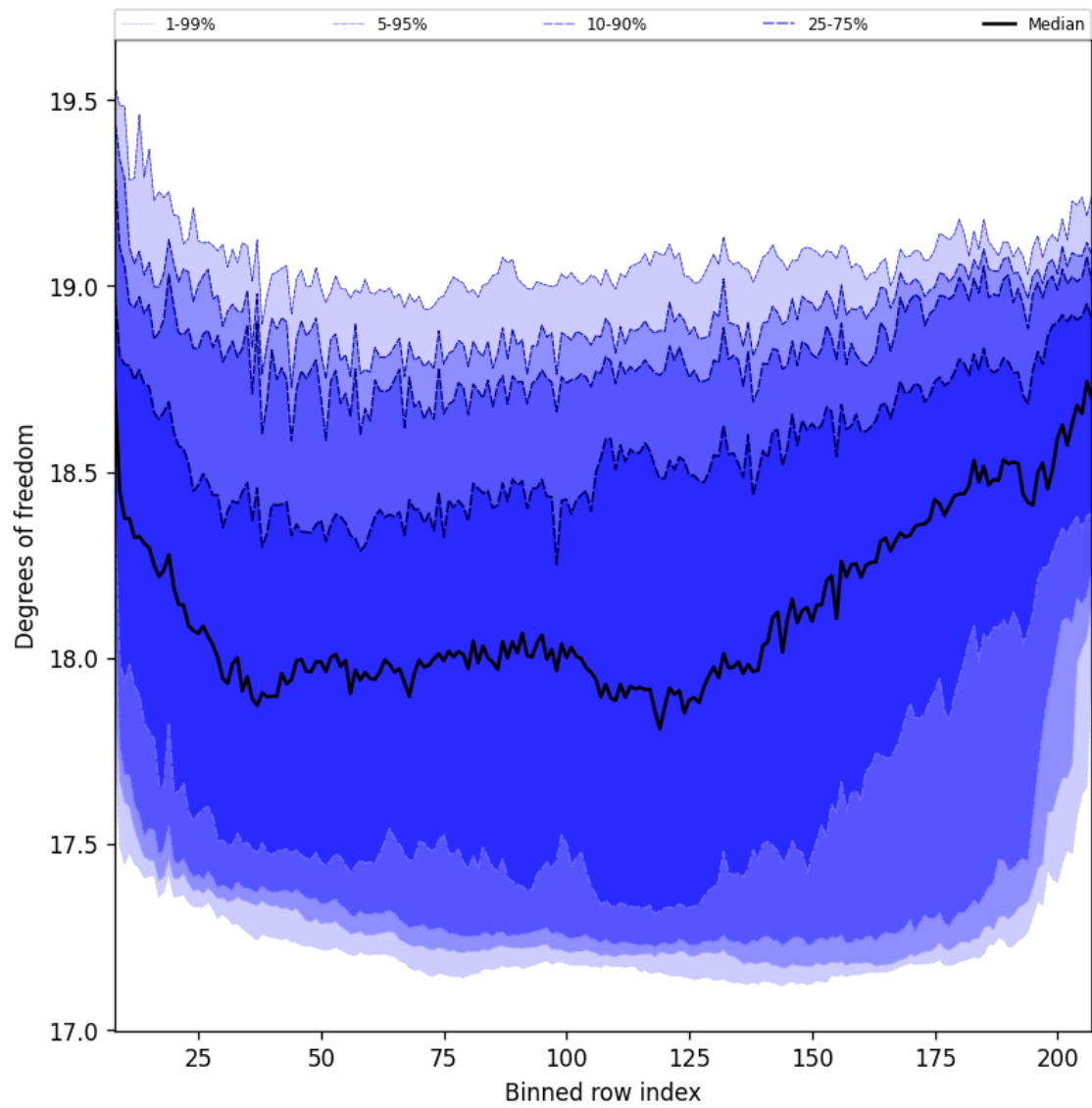
Figure 41: Along track statistics of “Degrees of freedom” for 2025-02-14 to 2025-02-16
