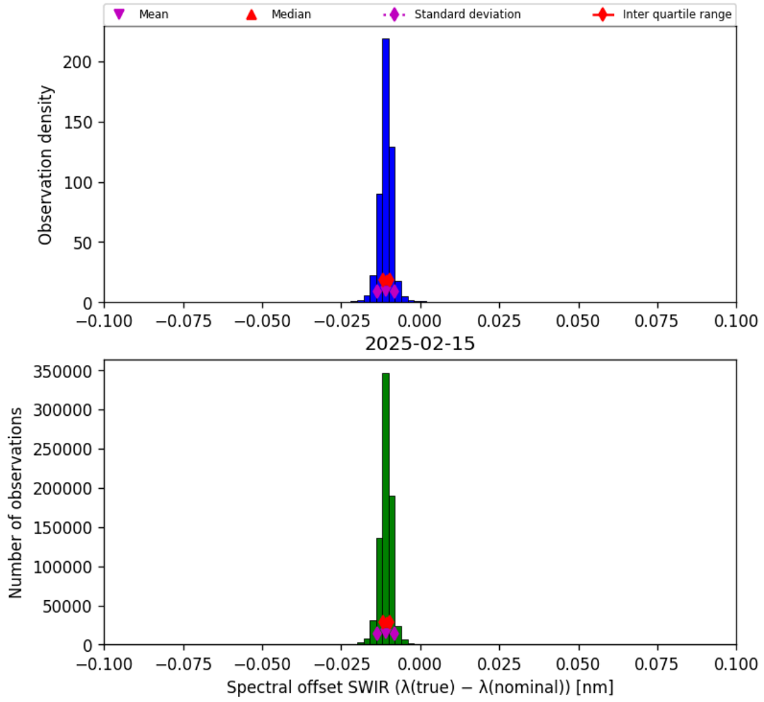
Figure 27: Histogram of “Spectral offset SWIR ( \lambda_{\text{true}} - \lambda_{\text{nominal}} )” for 2025-02-14 to 2025-02-16
