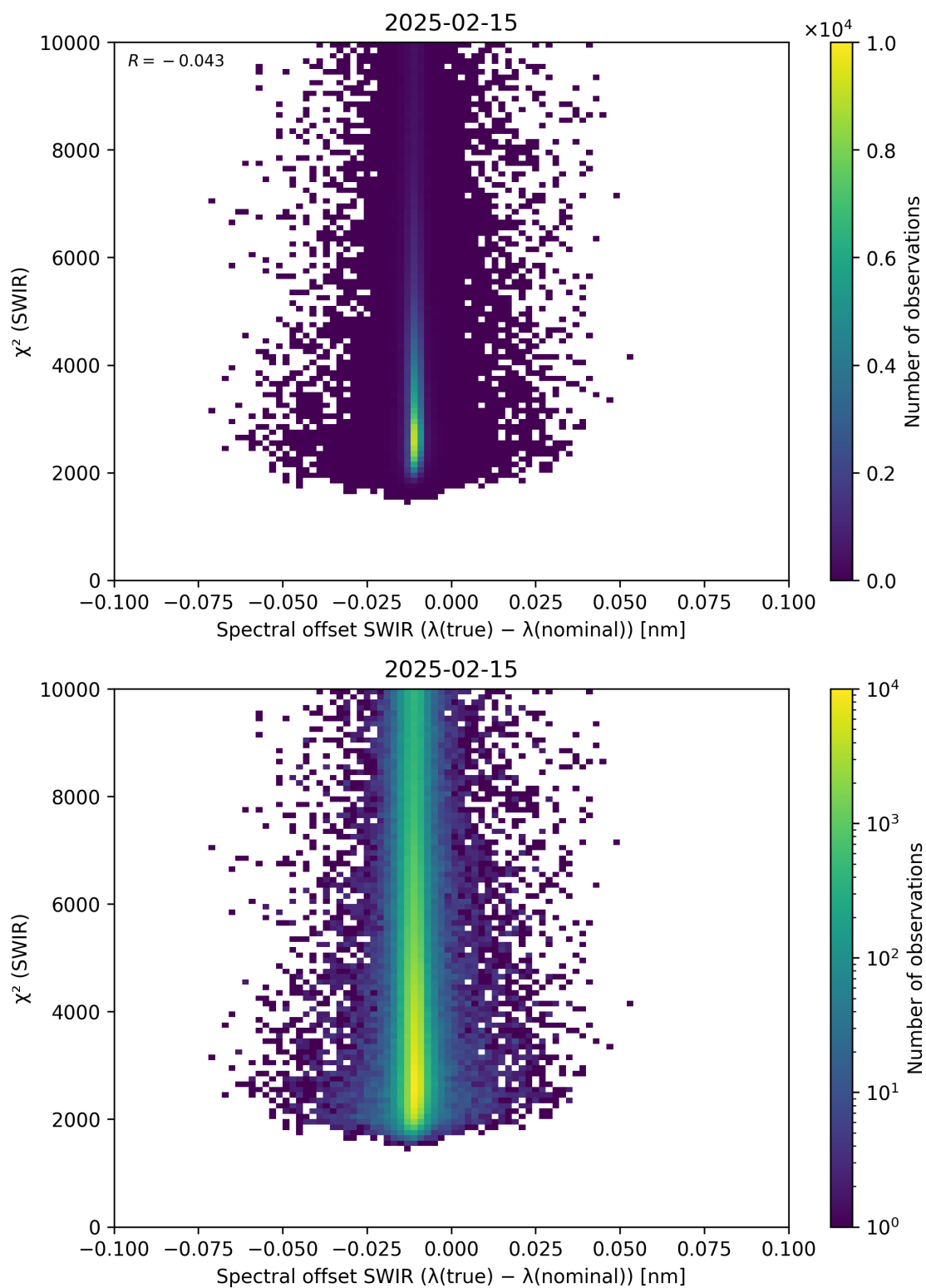
Figure 118: Scatter density plot of “Spectral offset SWIR ( \lambda_{\text{true}} - \lambda_{\text{nominal}} )” against “ \chi^2 (SWIR)” for 2025-02-14 to 2025-02-16.
