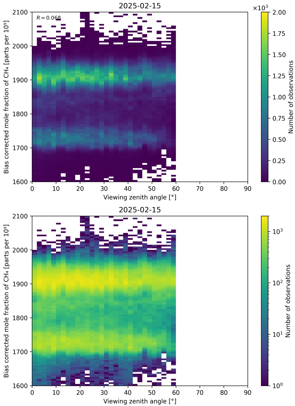
Figure 111: Scatter density plot of “Viewing zenith angle” against “Bias corrected mole fraction of CH 4 ” for 2025-02-14 to 2025-02-16.
