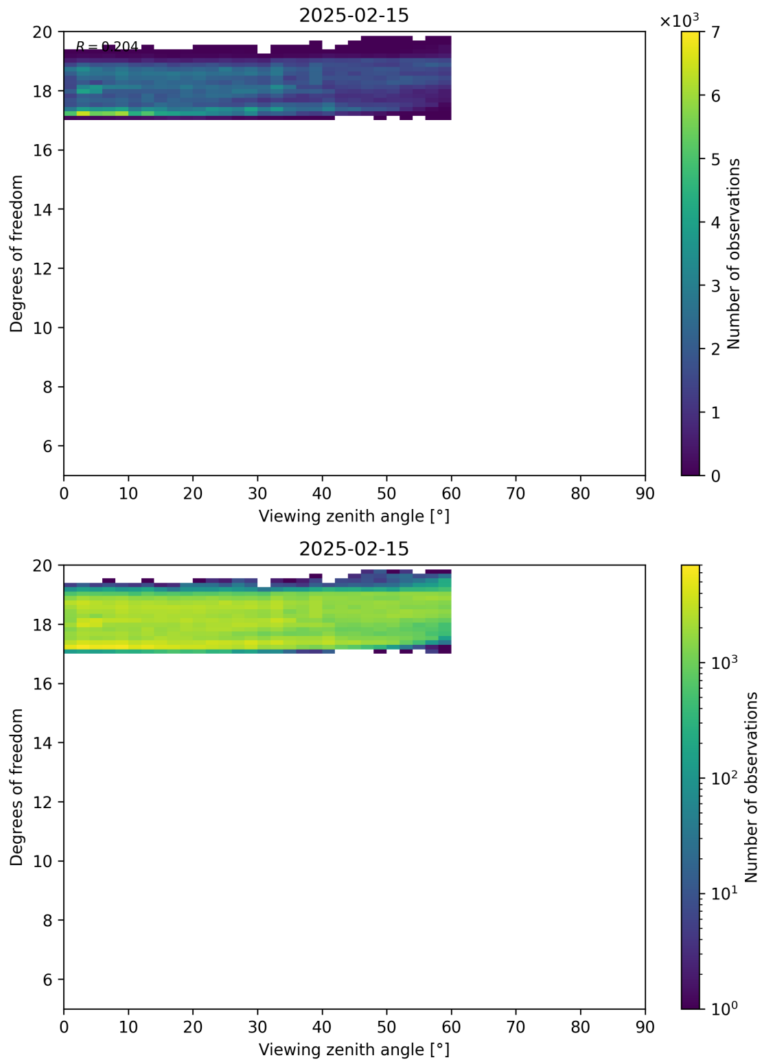
Figure 107: Scatter density plot of “Viewing zenith angle” against “Degrees of freedom” for 2025-02-14 to 2025-02-16.
