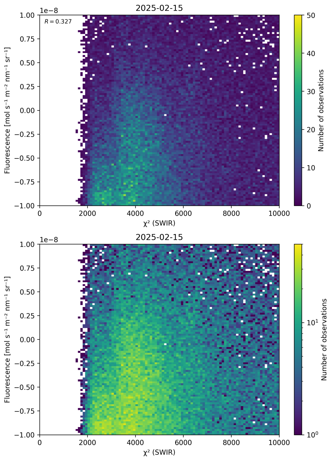
Figure 49: Scatter density plot of “ \chi^2 (SWIR)” against “Fluorescence” for 2025-02-14 to 2025-02-16.
