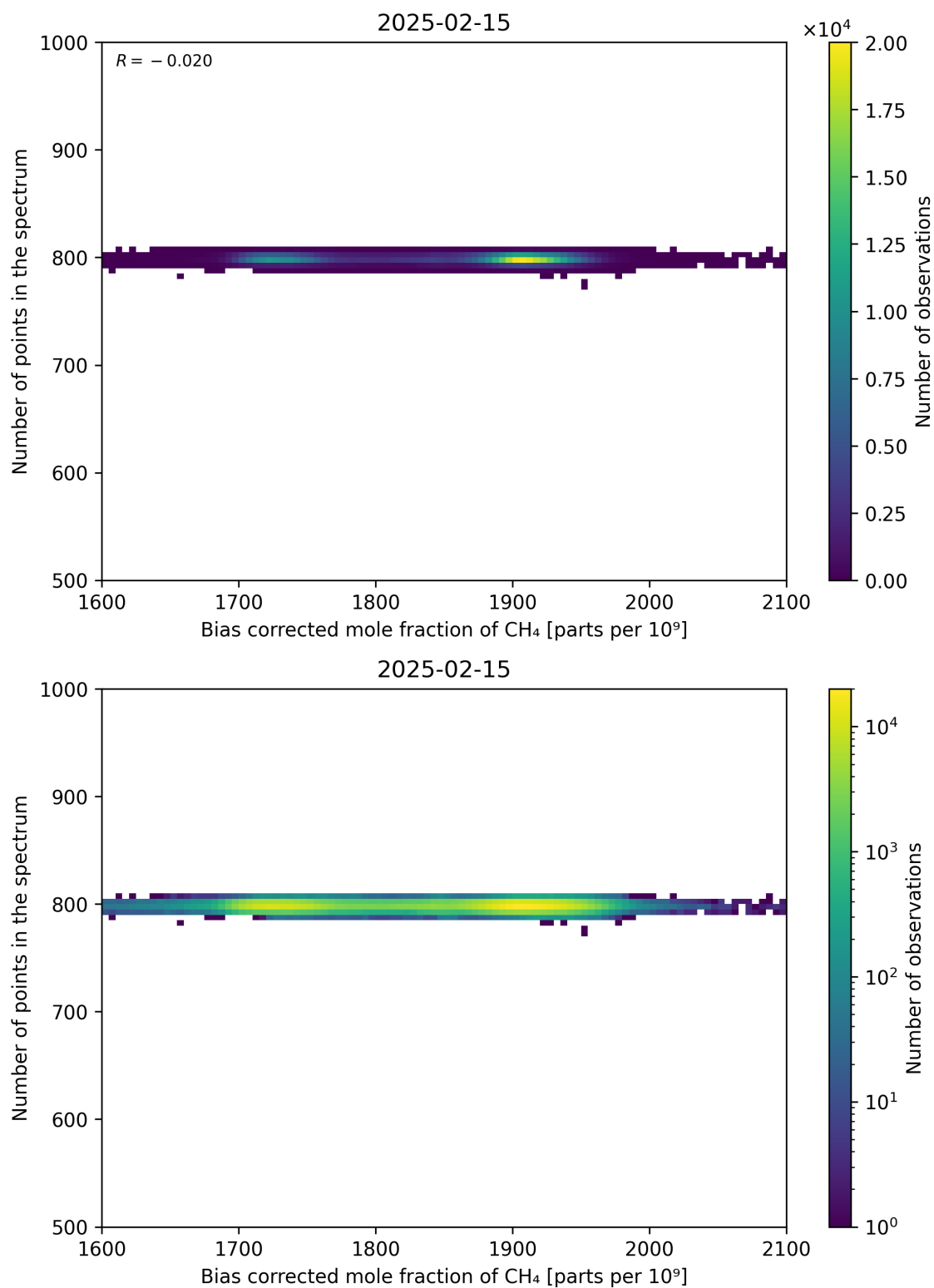
Figure 68: Scatter density plot of “Bias corrected mole fraction of CH 4 ” against “Number of points in the spectrum” for 2025-02-14 to 2025-02-16.
