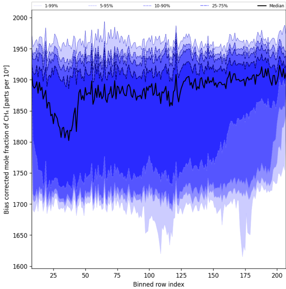
Figure 36: Along track statistics of “Bias corrected mole fraction of CH 4 ” for 2025-02-14 to 2025-02-16
