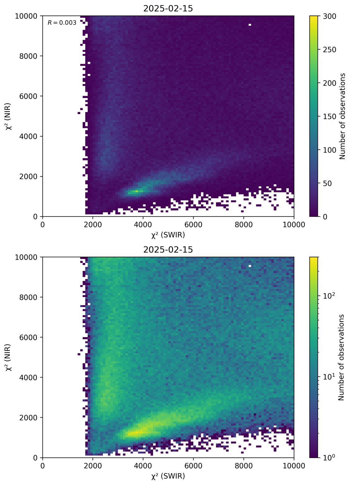
Figure 47: Scatter density plot of “ \chi^2 (SWIR)” against “ \chi^2 (NIR)” for 2025-02-14 to 2025-02-16.
