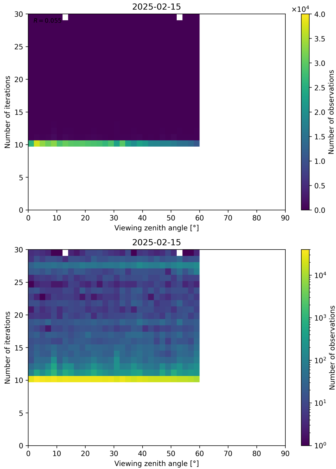
Figure 113: Scatter density plot of “Viewing zenith angle” against “Number of iterations” for 2025-02-14 to 2025-02-16.
