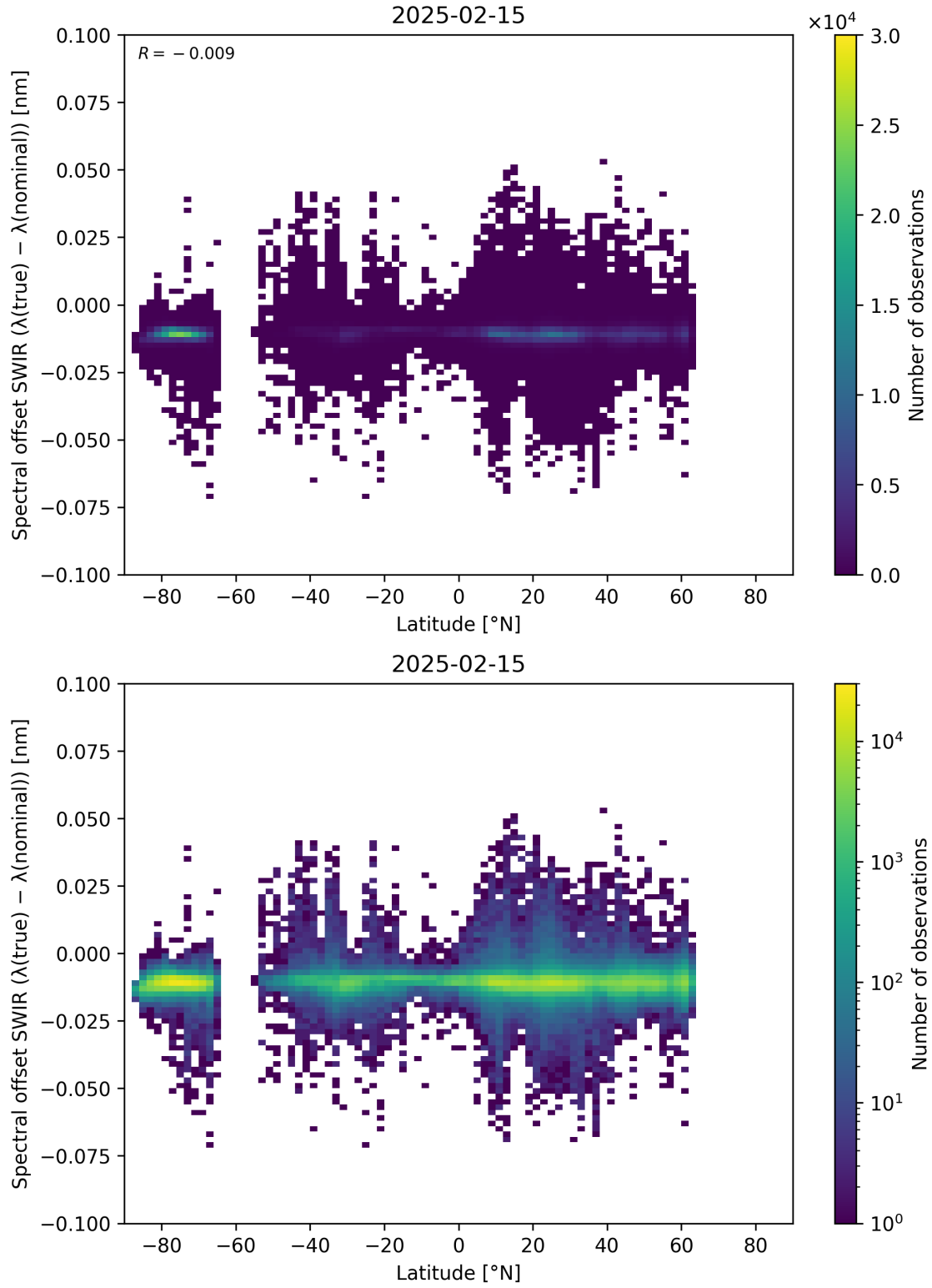
Figure 62: Scatter density plot of “Latitude” against “Spectral offset SWIR ( \lambda_{\text{true}} - \lambda_{\text{nominal}} )” for 2025-02-14 to 2025-02-16.
