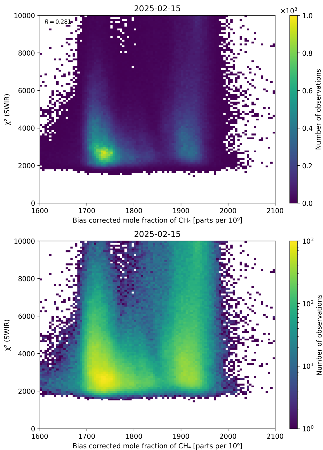
Figure 64: Scatter density plot of “Bias corrected mole fraction of \text{CH}_4 ” against “ \chi^2 (SWIR)” for 2025-02-14 to 2025-02-16.
