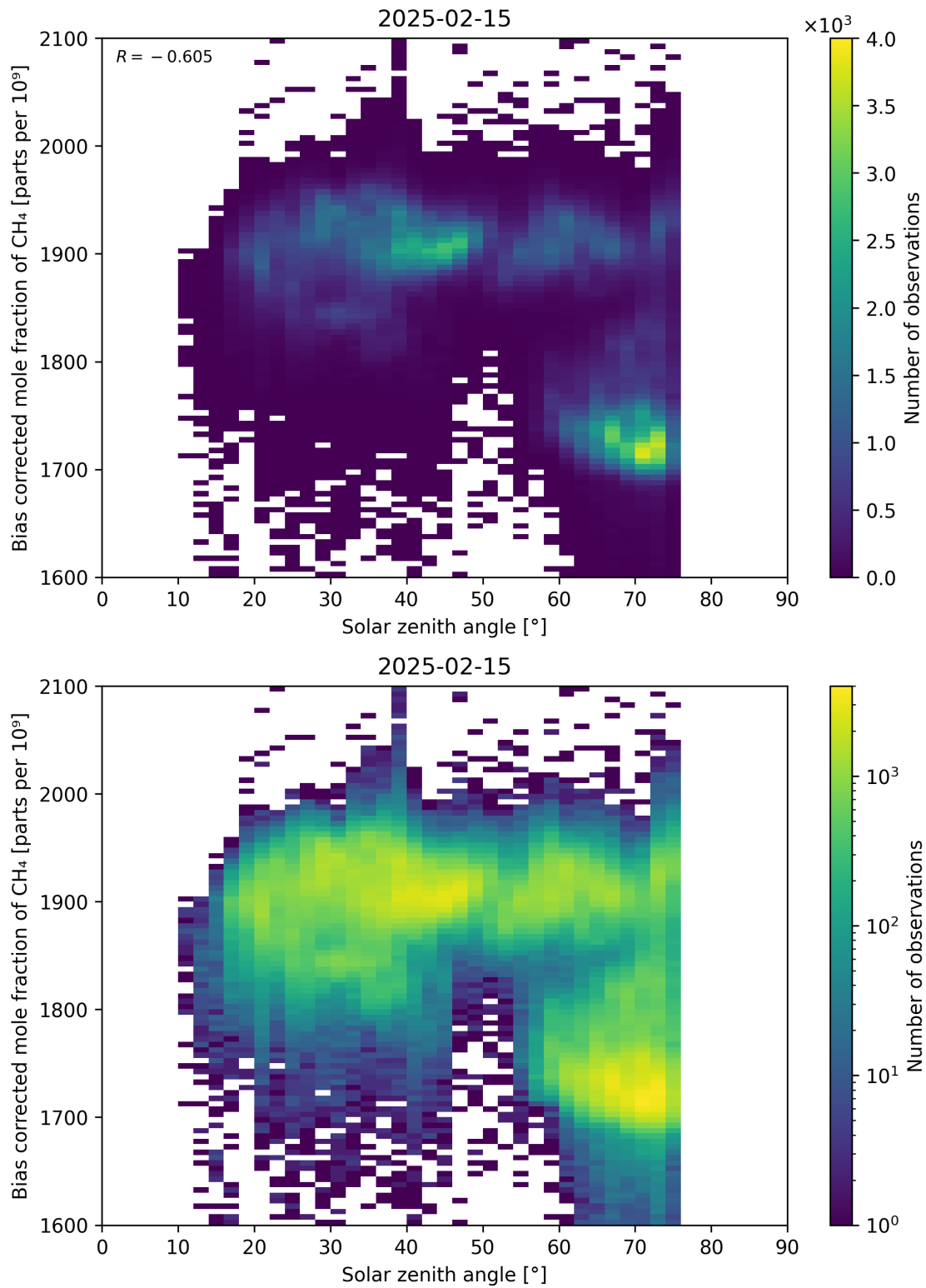
Figure 100: Scatter density plot of “Solar zenith angle” against “Bias corrected mole fraction of CH 4 ” for 2025-02-14 to 2025-02-16.
