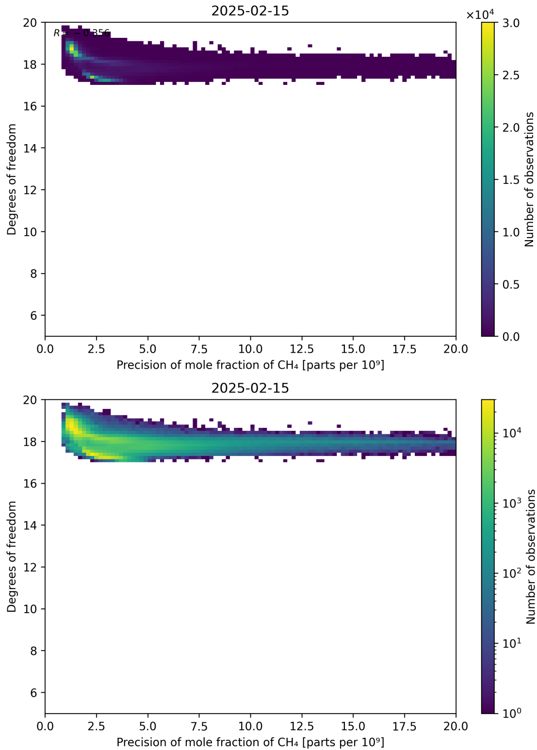
Figure 80: Scatter density plot of “Precision of mole fraction of CH 4 ” against “Degrees of freedom” for 2025-02-14 to 2025-02-16.
