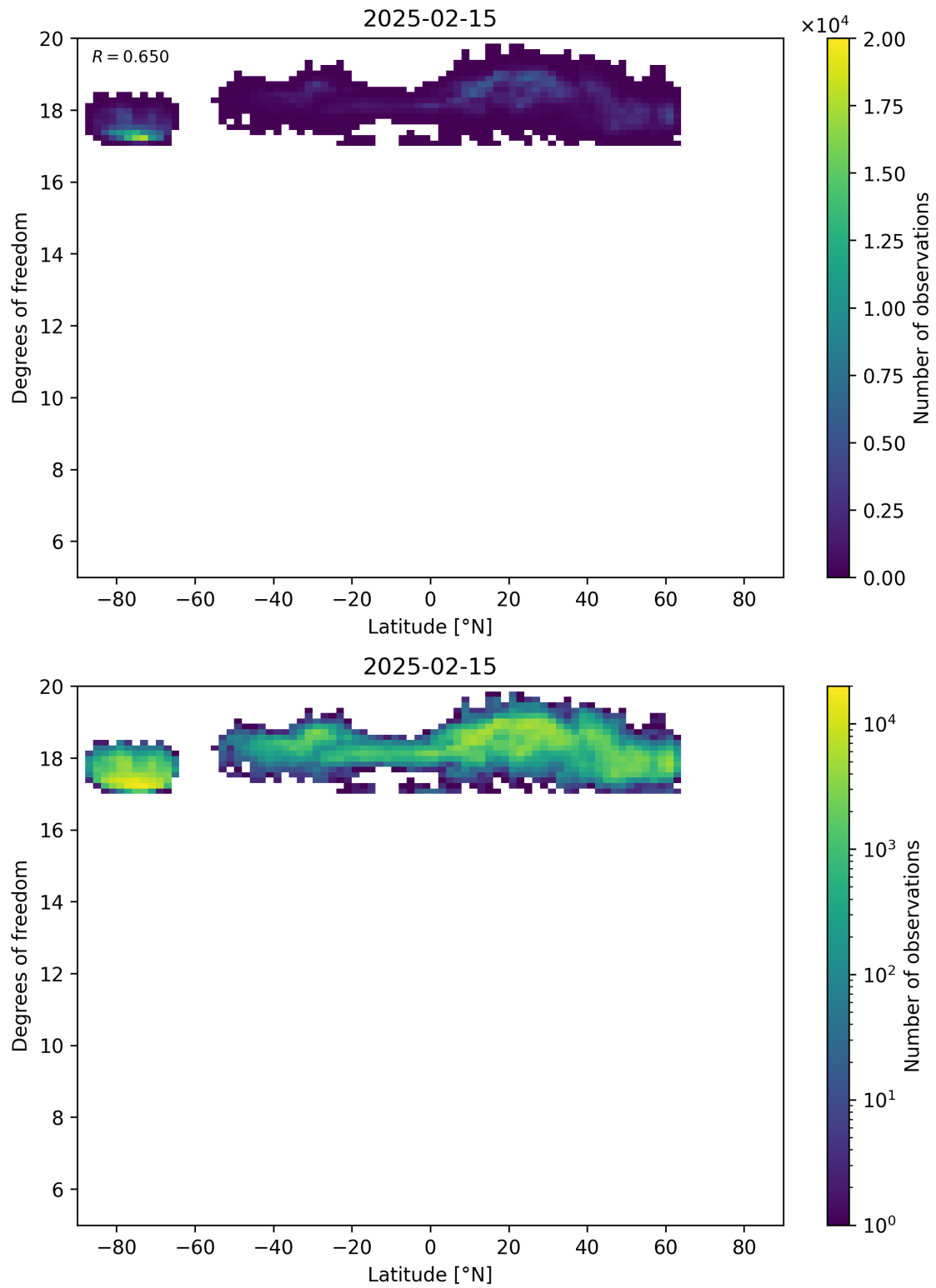
Figure 55: Scatter density plot of “Latitude” against “Degrees of freedom” for 2025-02-14 to 2025-02-16.
