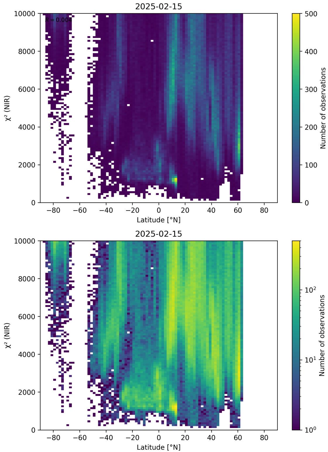
Figure 53: Scatter density plot of “Latitude” against “ \chi^2 (NIR)” for 2025-02-14 to 2025-02-16.
