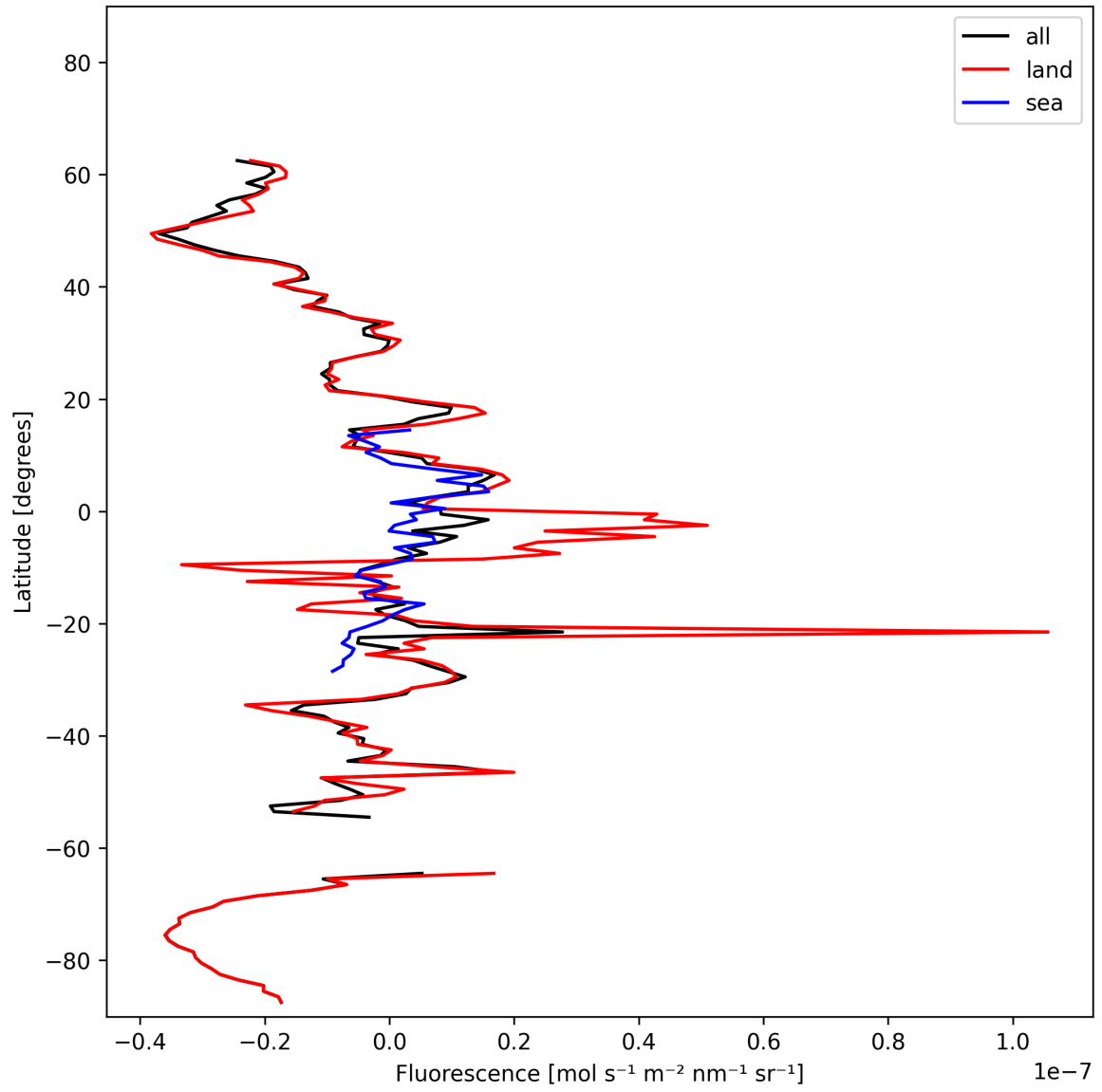
Figure 21: Zonal average of “Fluorescence” for 2025-02-14 to 2025-02-16.
