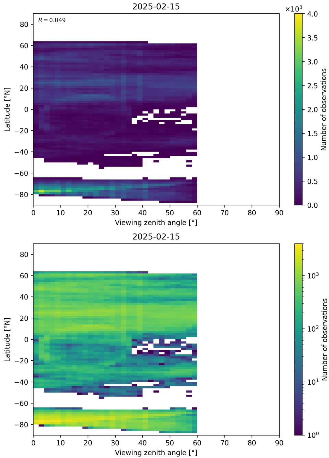
Figure 109: Scatter density plot of “Viewing zenith angle” against “Latitude” for 2025-02-14 to 2025-02-16.
