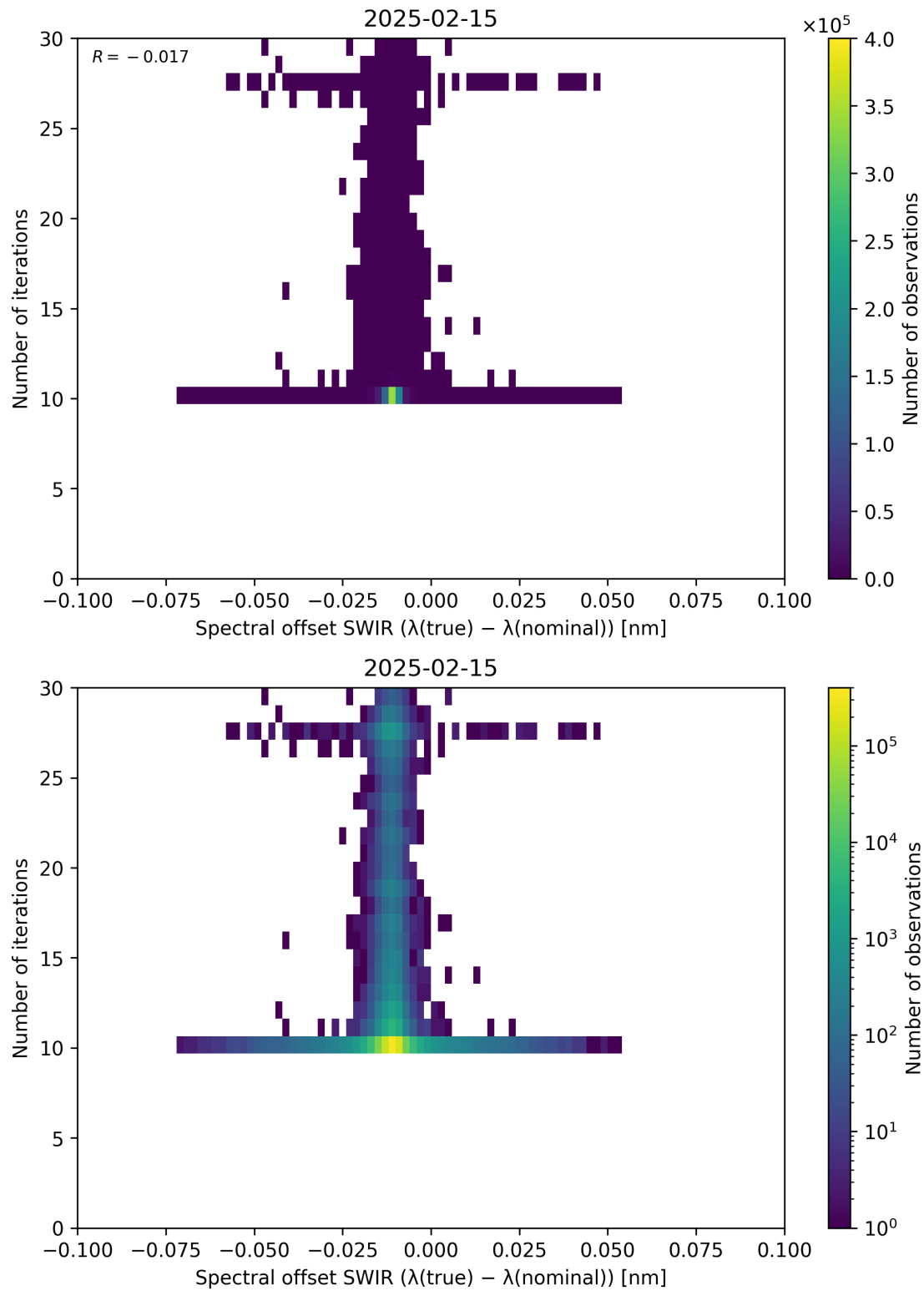
Figure 121: Scatter density plot of “Spectral offset SWIR ( \lambda_{\text{true}} - \lambda_{\text{nominal}} )” against “Number of iterations” for 2025-02-14 to 2025-02-16.
