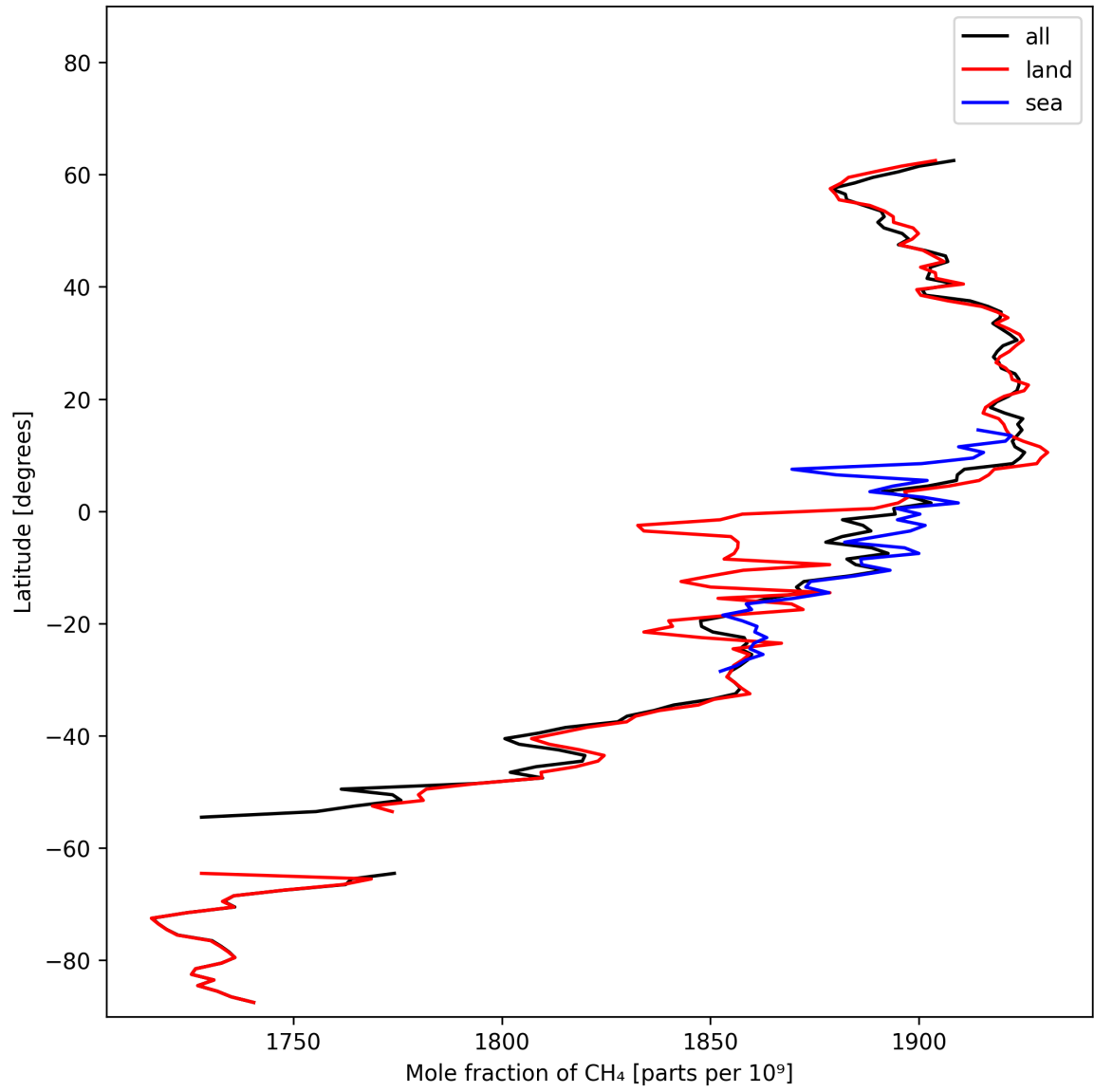
Figure 12: Zonal average of “Mole fraction of \text{CH}_4 ” for 2025-02-14 to 2025-02-16.
