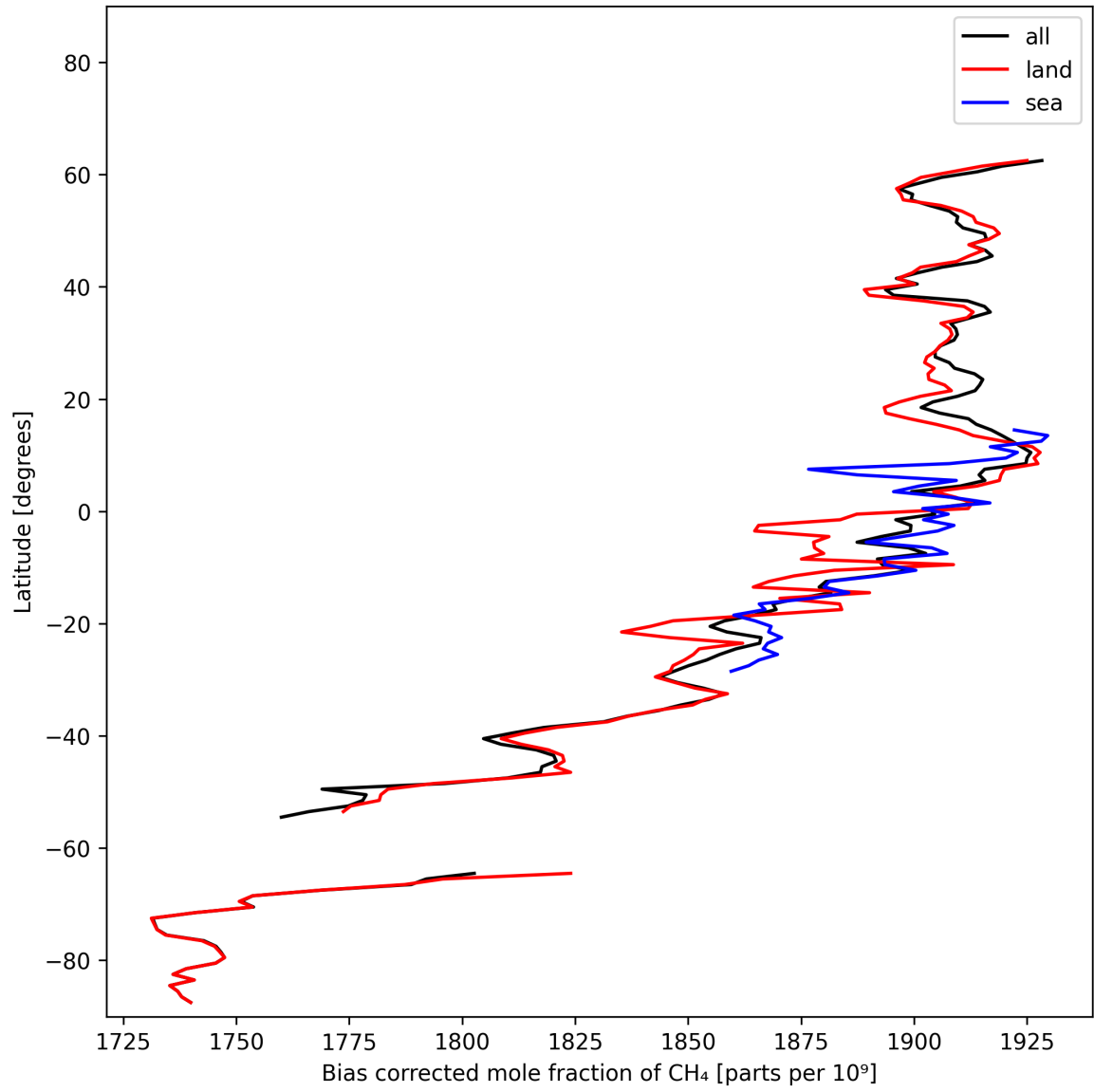
Figure 14: Zonal average of “Bias corrected mole fraction of CH 4 ” for 2025-02-14 to 2025-02-16.
