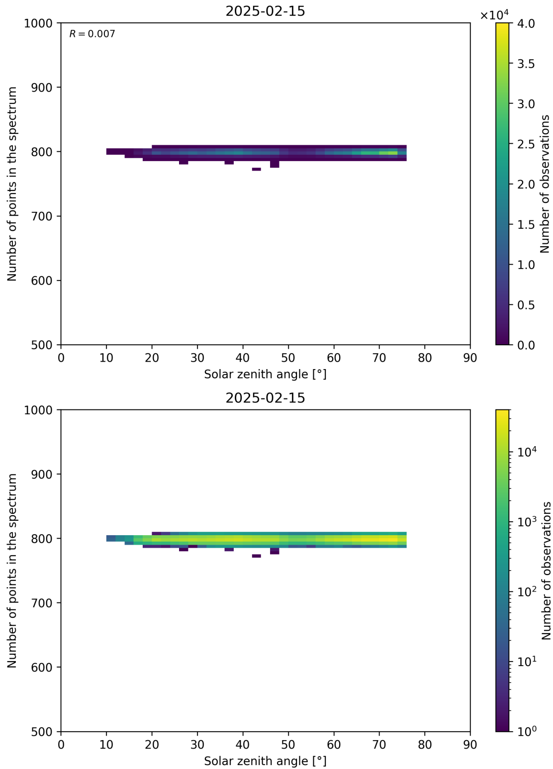
Figure 103: Scatter density plot of “Solar zenith angle” against “Number of points in the spectrum” for 2025-02-14 to 2025-02-16.
