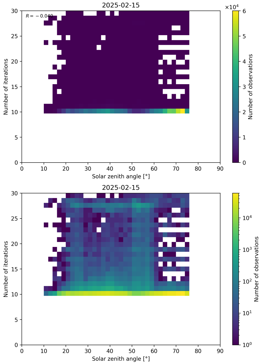
Figure 102: Scatter density plot of “Solar zenith angle” against “Number of iterations” for 2025-02-14 to 2025-02-16.
