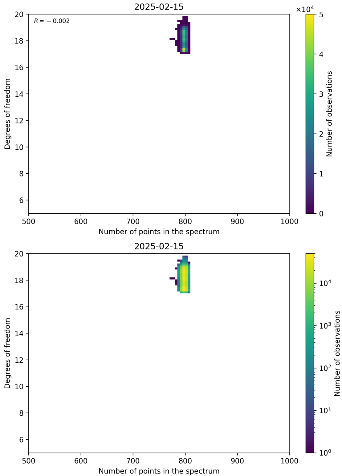
Figure 90: Scatter density plot of “Number of points in the spectrum” against “Degrees of freedom” for 2025-02-14 to 2025-02-16.
