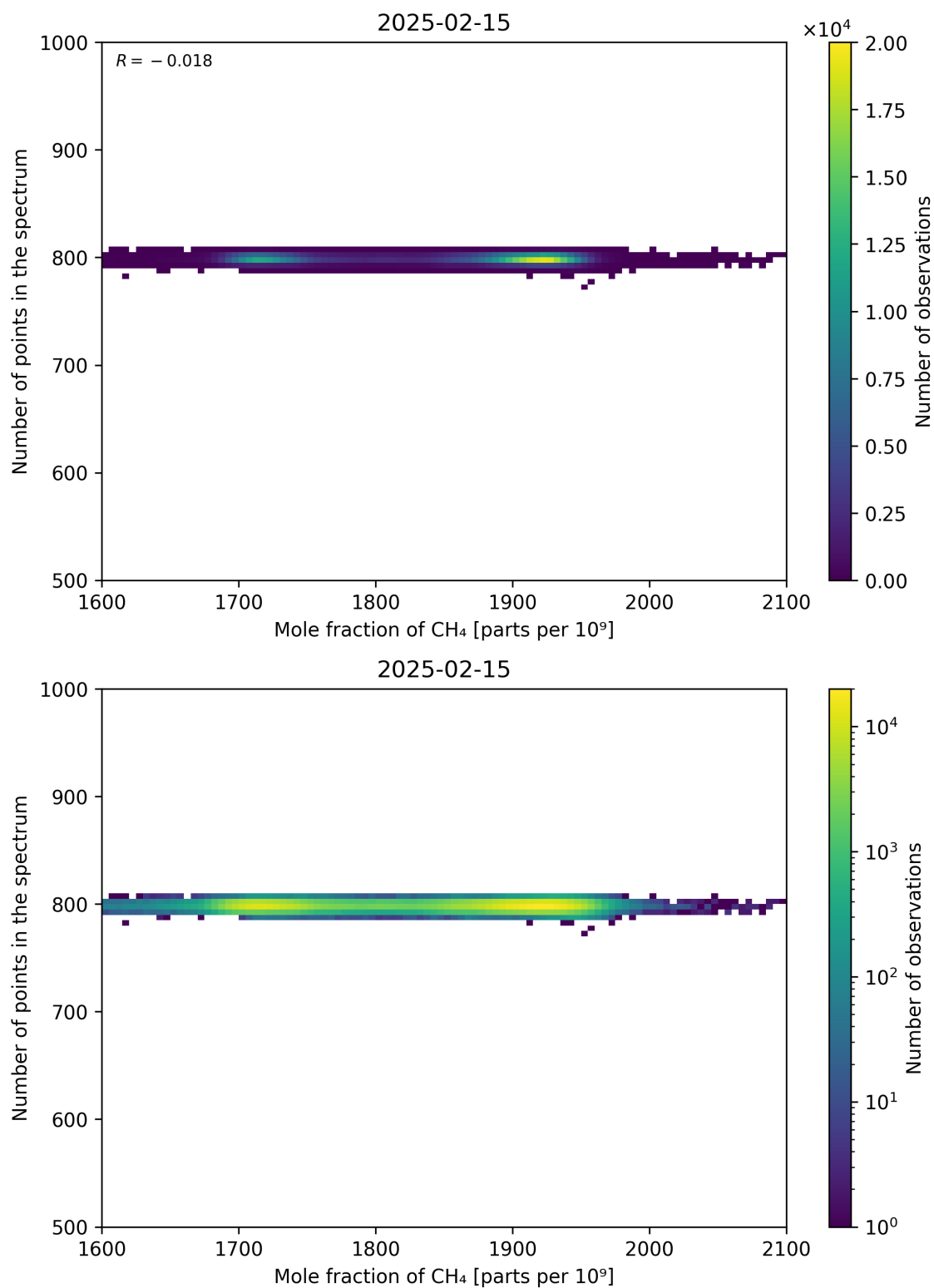
Figure 77: Scatter density plot of “Mole fraction of CH 4 ” against “Number of points in the spectrum” for 2025-02-14 to 2025-02-16.
