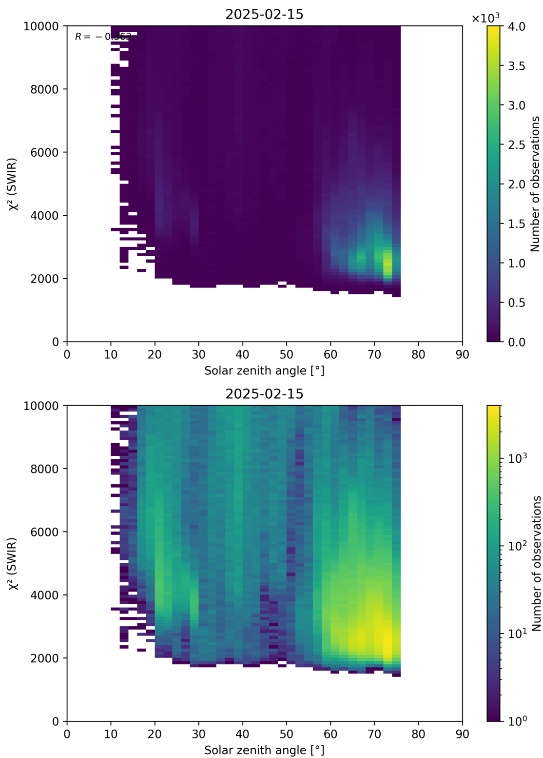
Figure 95: Scatter density plot of “Solar zenith angle” against “ \chi^2 (SWIR)” for 2025-02-14 to 2025-02-16.
