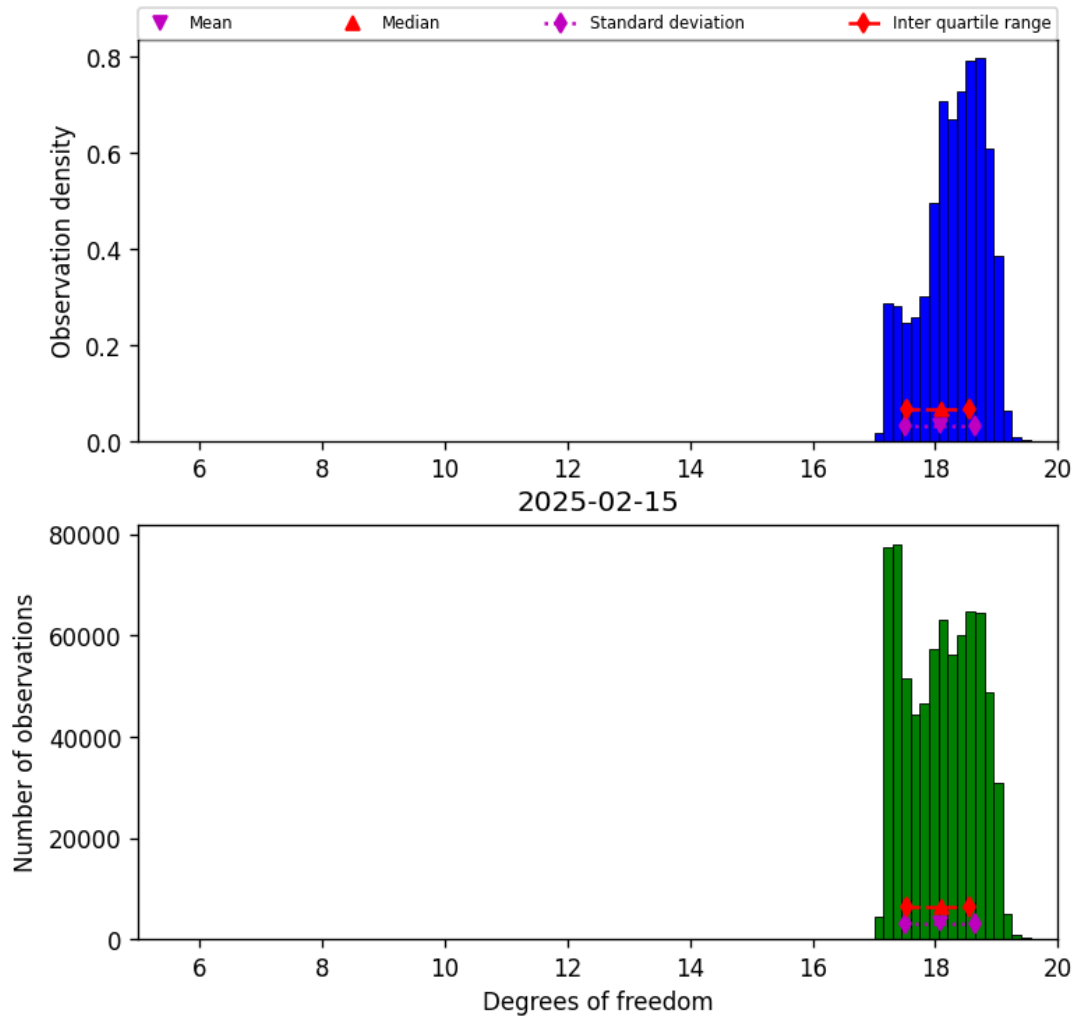
Figure 30: Histogram of “Degrees of freedom” for 2025-02-14 to 2025-02-16
