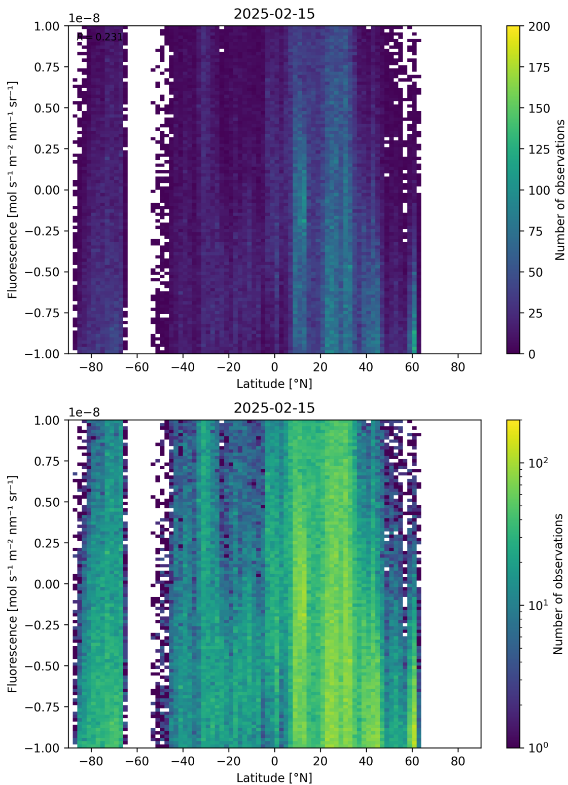
Figure 56: Scatter density plot of “Latitude” against “Fluorescence” for 2025-02-14 to 2025-02-16.
