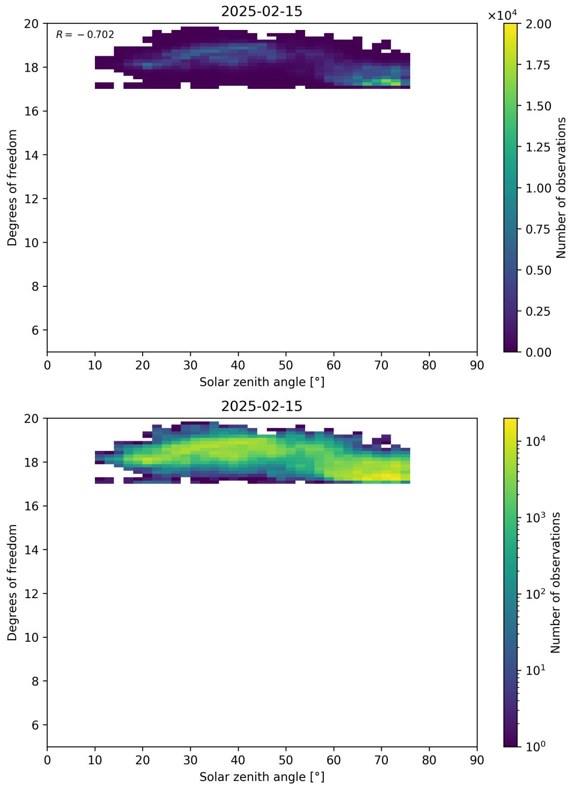
Figure 96: Scatter density plot of “Solar zenith angle” against “Degrees of freedom” for 2025-02-14 to 2025-02-16.
