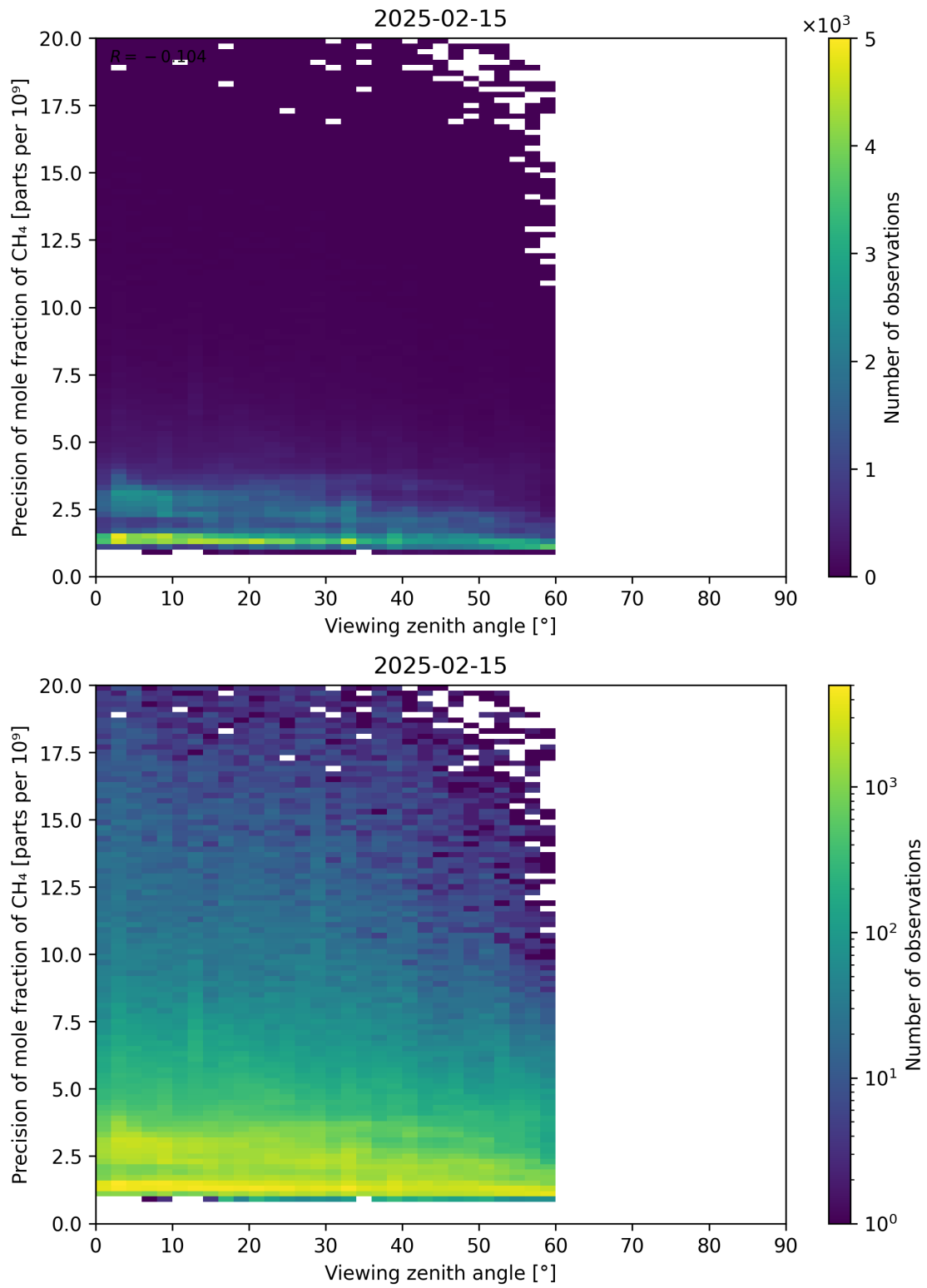
Figure 112: Scatter density plot of “Viewing zenith angle” against “Precision of mole fraction of CH 4 ” for 2025-02-14 to 2025-02-16.
