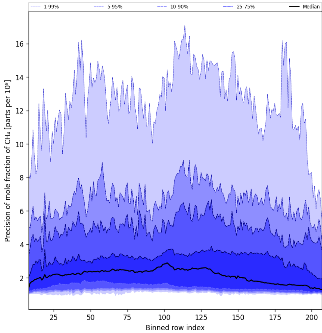
Figure 35: Along track statistics of “Precision of mole fraction of CH 4 ” for 2025-02-14 to 2025-02-16
