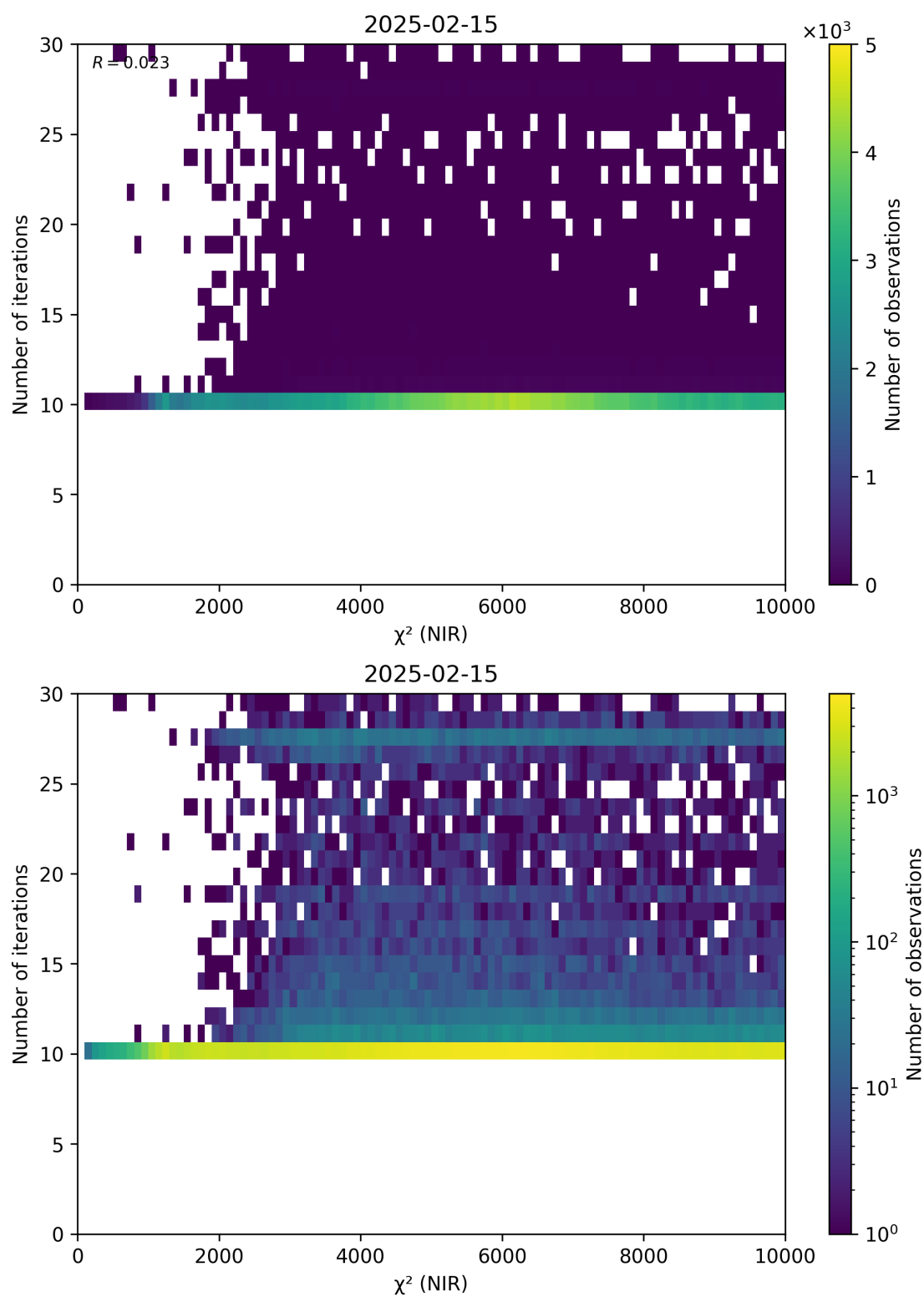
Figure 46: Scatter density plot of “ \chi^2 (NIR)” against “Number of iterations” for 2025-02-14 to 2025-02-16.
