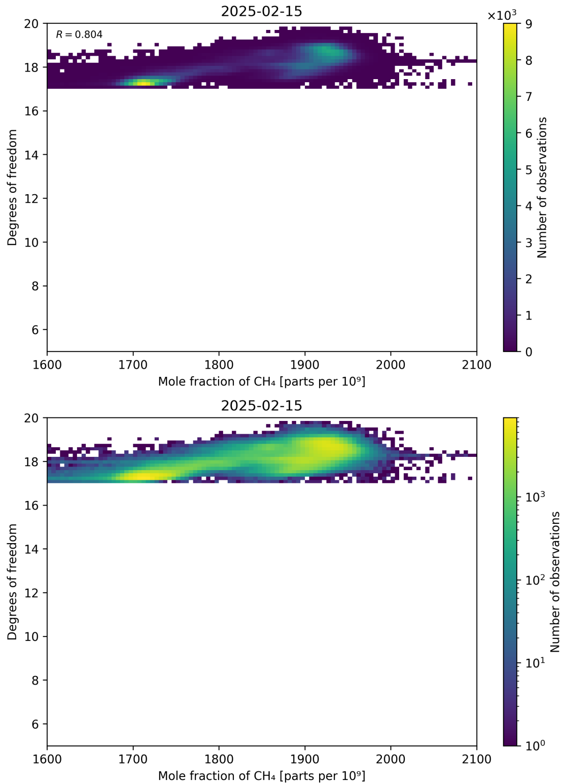
Figure 72: Scatter density plot of “Mole fraction of CH 4 ” against “Degrees of freedom” for 2025-02-14 to 2025-02-16.
