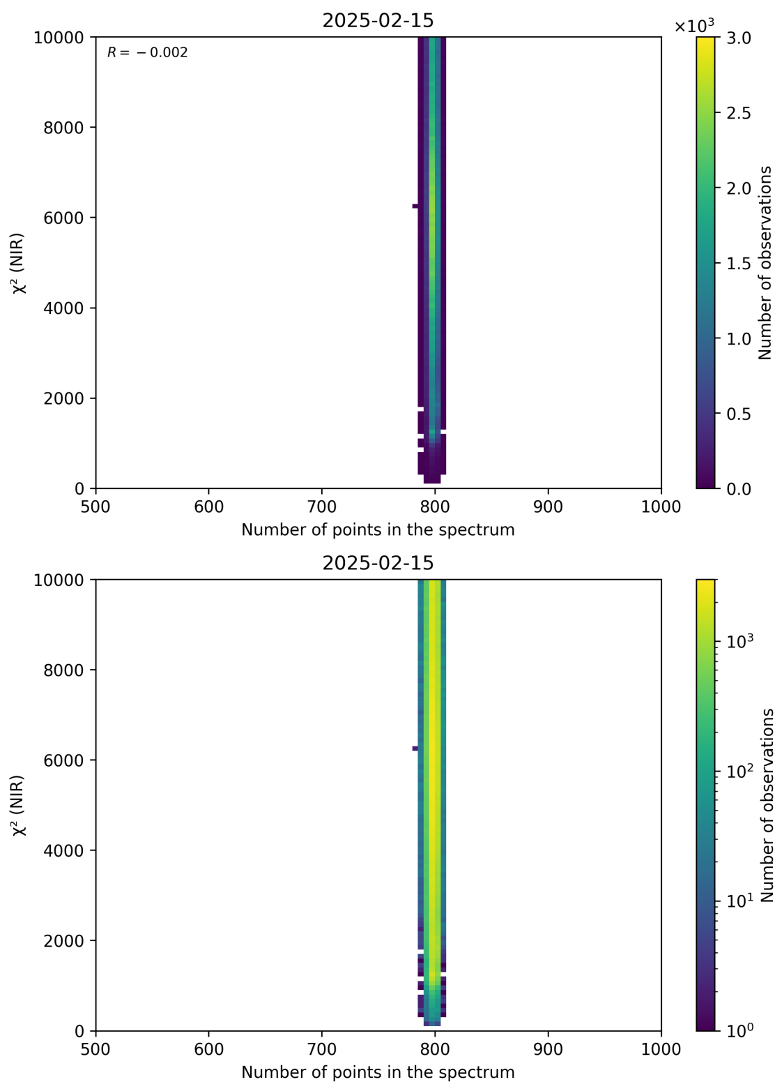
Figure 88: Scatter density plot of “Number of points in the spectrum” against “ \chi^2 (NIR)” for 2025-02-14 to 2025-02-16.
