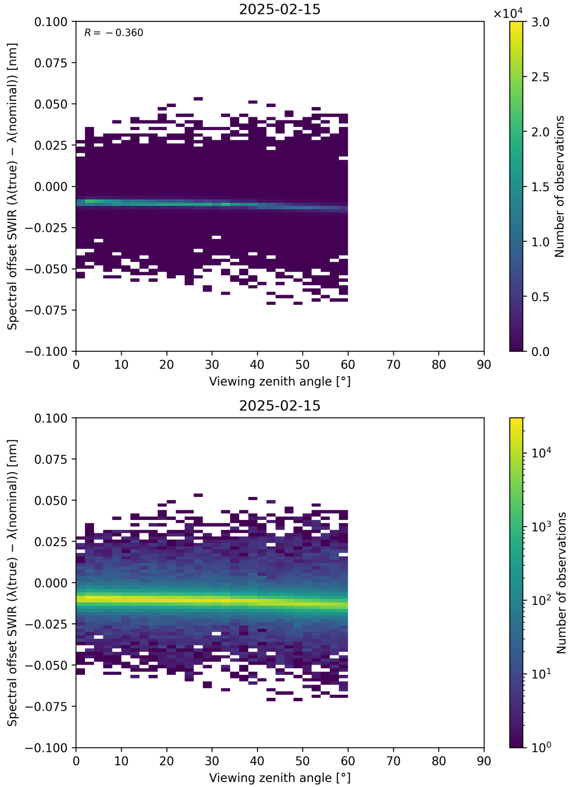
Figure 116: Scatter density plot of “Viewing zenith angle” against “Spectral offset SWIR ( \lambda_{\text{true}} - \lambda_{\text{nominal}} )” for 2025-02-14 to 2025-02-16.
