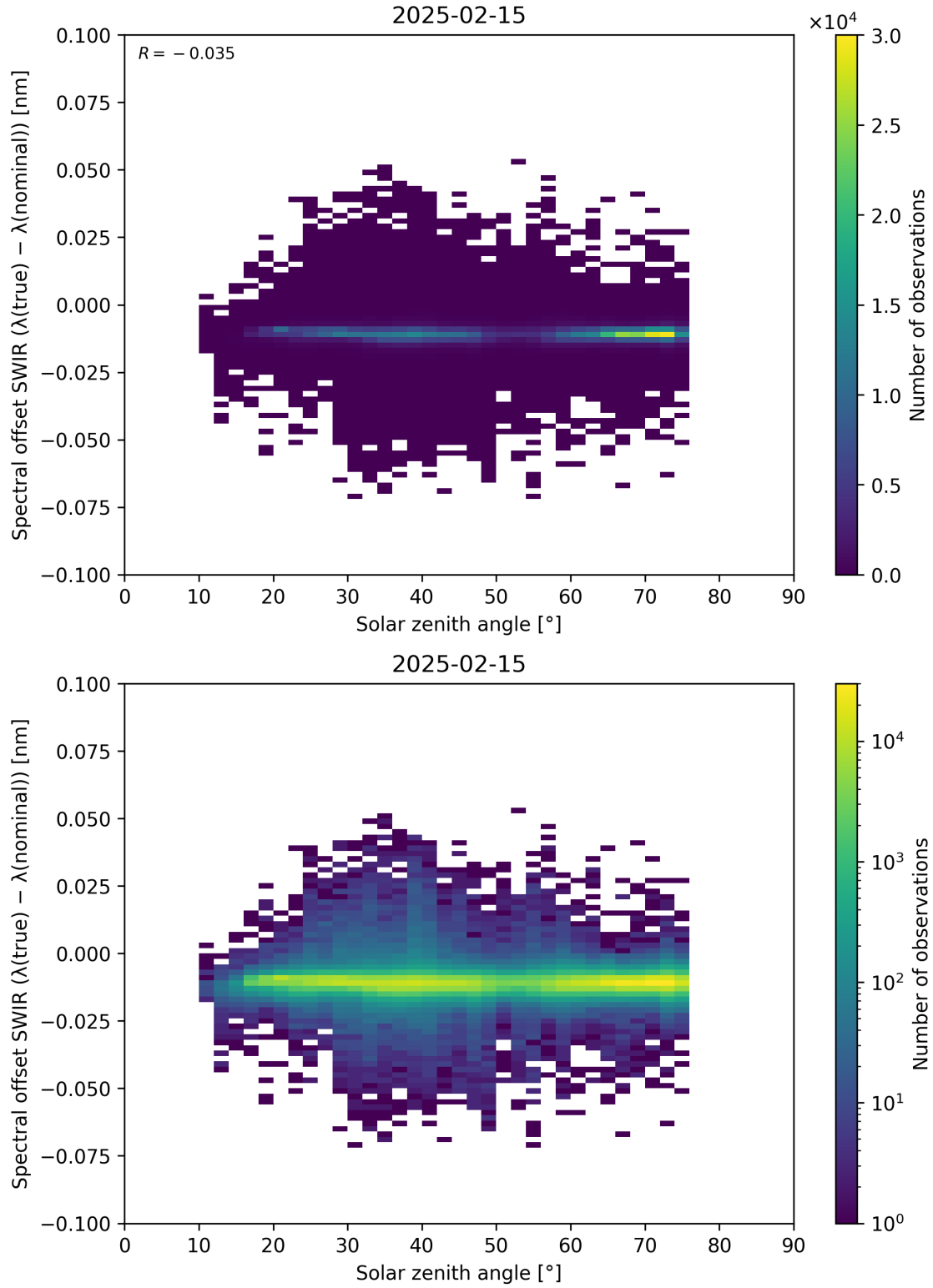
Figure 104: Scatter density plot of “Solar zenith angle” against “Spectral offset SWIR ( \lambda_{\text{true}} - \lambda_{\text{nominal}} )” for 2025-02-14 to 2025-02-16.
