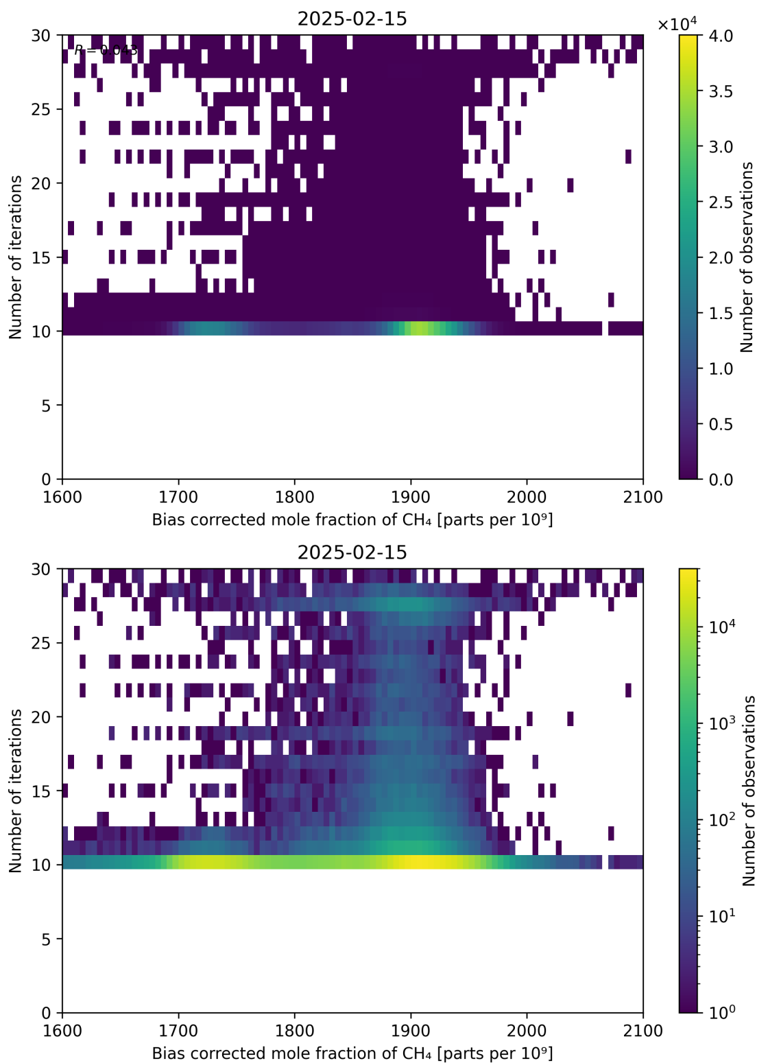
Figure 67: Scatter density plot of “Bias corrected mole fraction of CH 4 ” against “Number of iterations” for 2025-02-14 to 2025-02-16.
