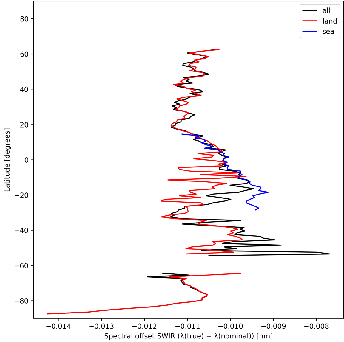
Figure 16: Zonal average of “Spectral offset SWIR ( \lambda_{\text{true}} - \lambda_{\text{nominal}} )” for 2025-02-14 to 2025-02-16.
