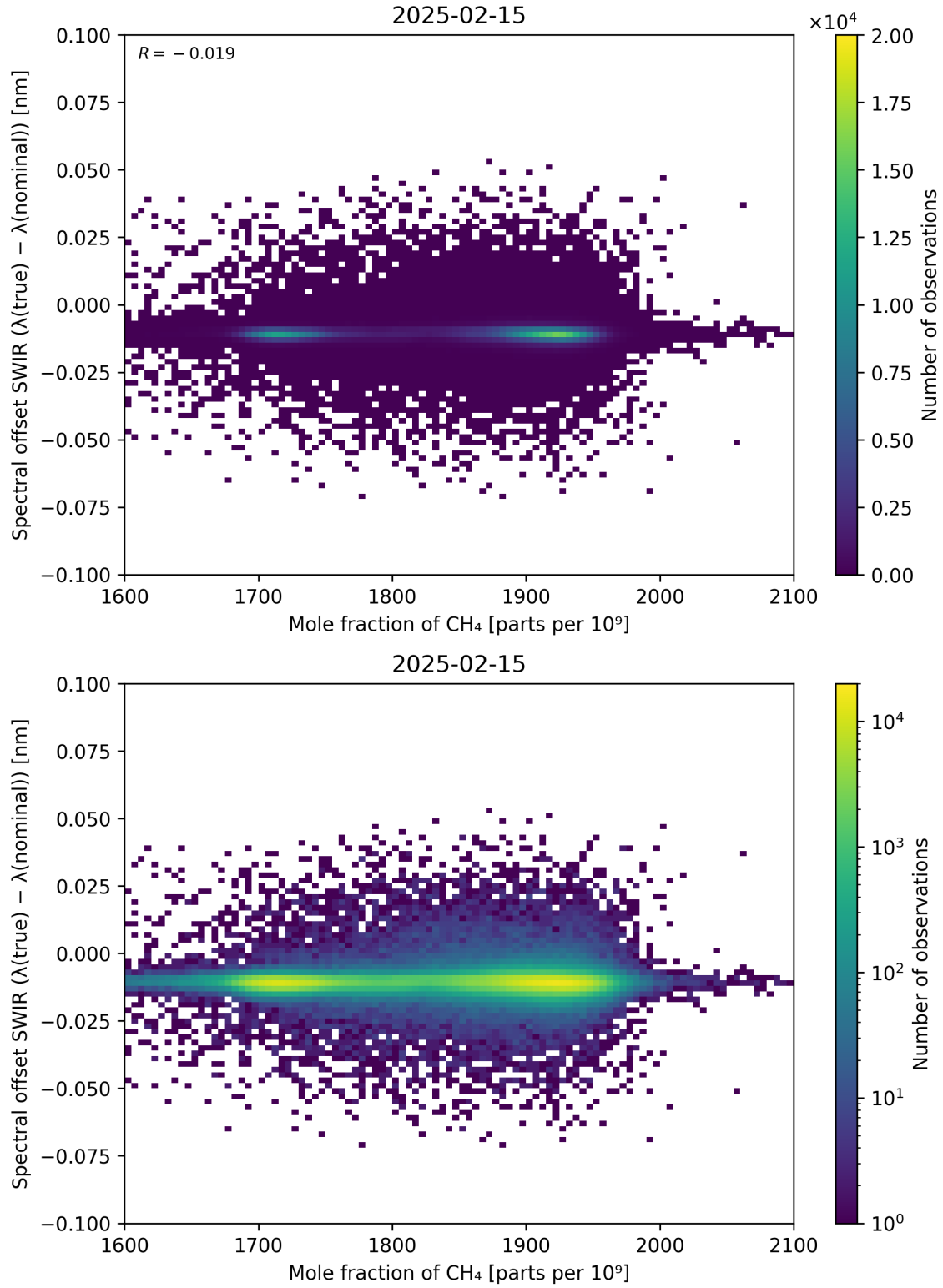
Figure 86: Scatter density plot of “Mole fraction of CH 4 ” against “Spectral offset SWIR ( \lambda_{\text{true}} - \lambda_{\text{nominal}} )” for 2025-02-14 to 2025-02-16.
