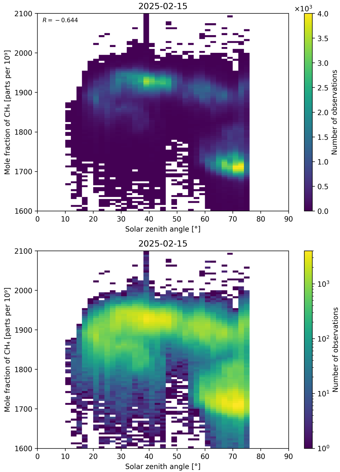
Figure 99: Scatter density plot of “Solar zenith angle” against “Mole fraction of CH 4 ” for 2025-02-14 to 2025-02-16.
