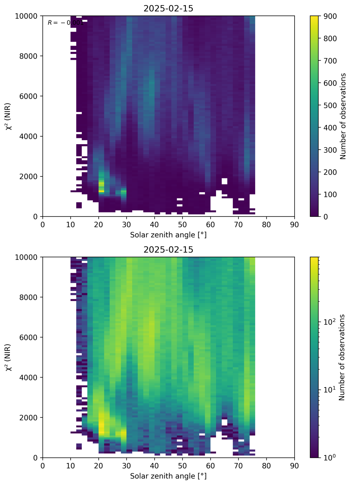
Figure 94: Scatter density plot of “Solar zenith angle” against “ \chi^2 (NIR)” for 2025-02-14 to 2025-02-16.
