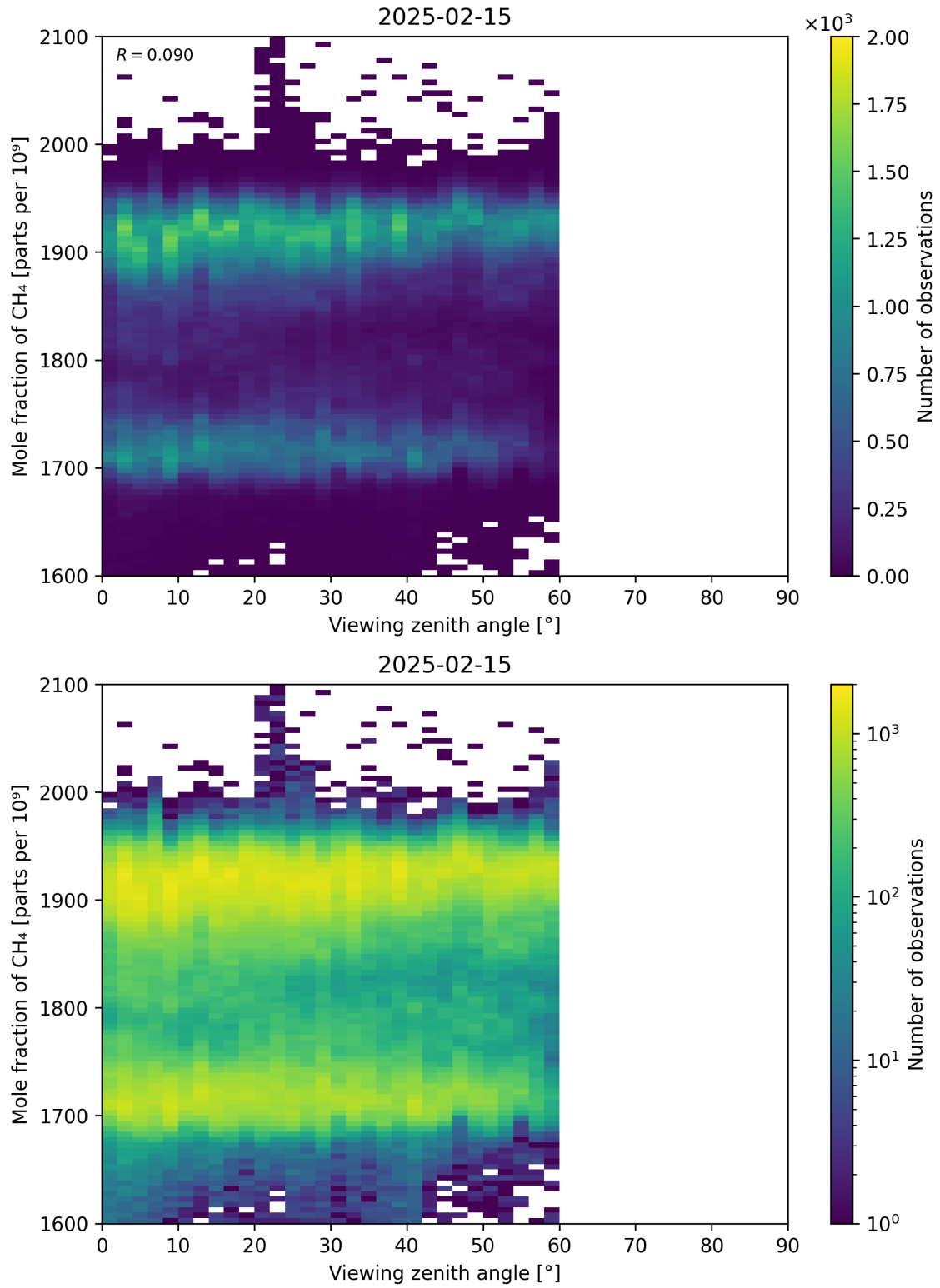
Figure 110: Scatter density plot of “Viewing zenith angle” against “Mole fraction of \text{CH}_4 ” for 2025-02-14 to 2025-02-16.
