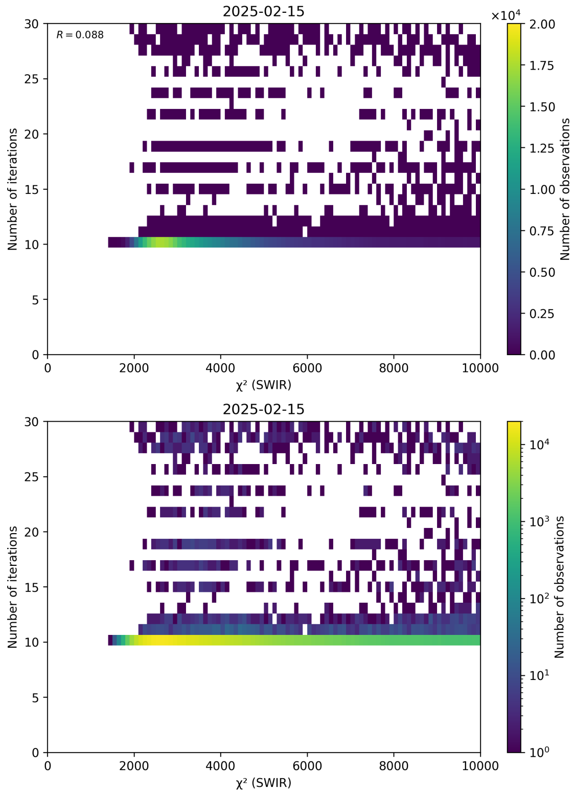
Figure 50: Scatter density plot of “ \chi^2 (SWIR)” against “Number of iterations” for 2025-02-14 to 2025-02-16.
