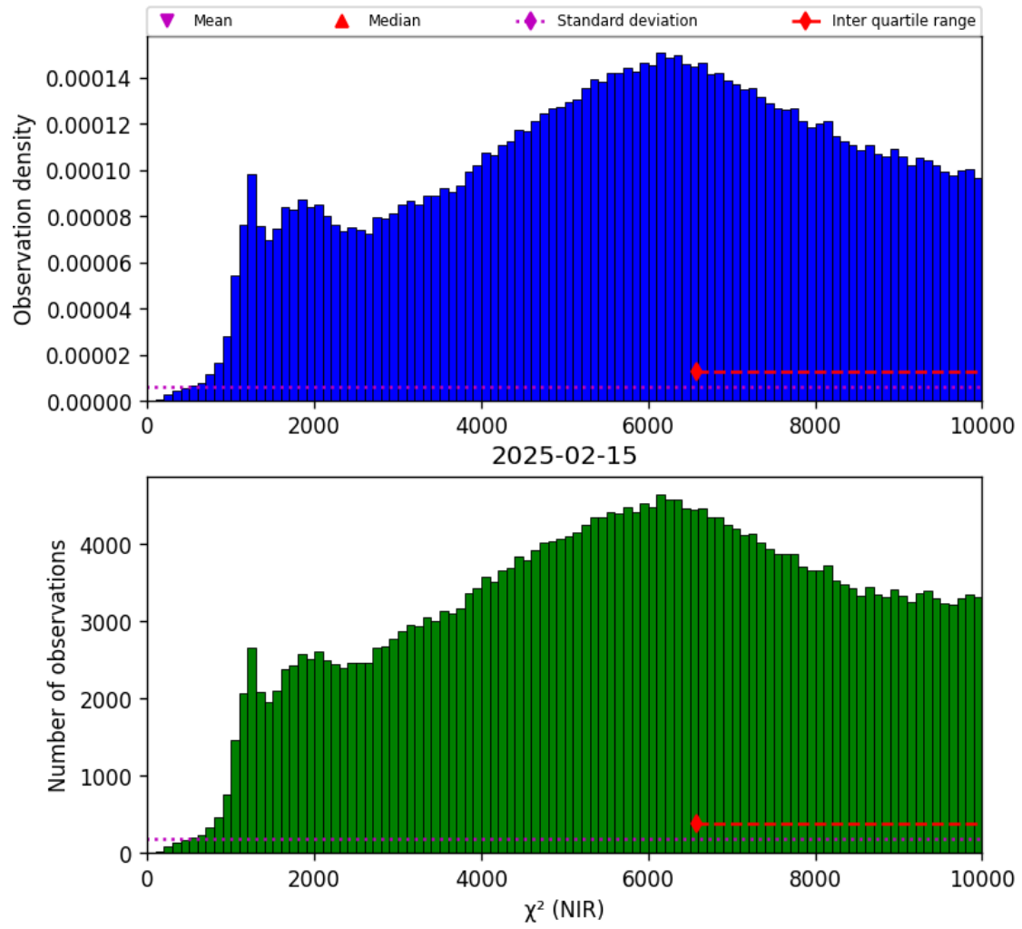
Figure 29: Histogram of “ \chi^2 (NIR)” for 2025-02-14 to 2025-02-16
