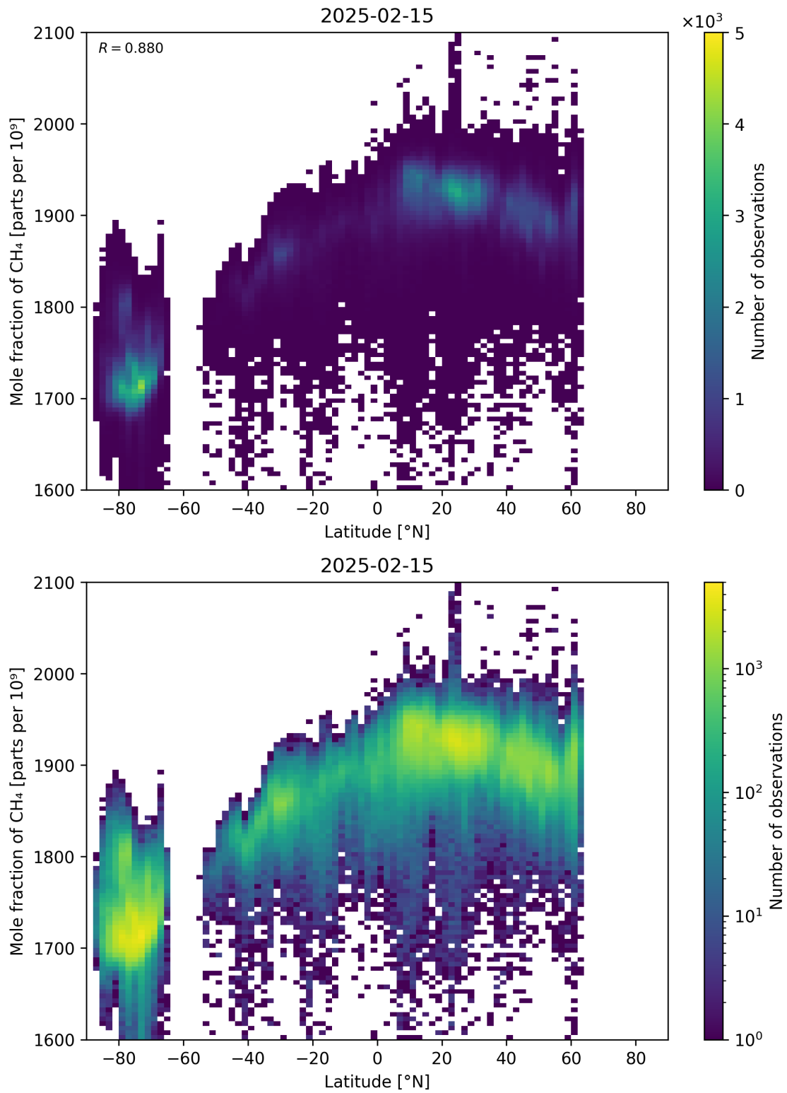
Figure 57: Scatter density plot of “Latitude” against “Mole fraction of CH 4 ” for 2025-02-14 to 2025-02-16.
