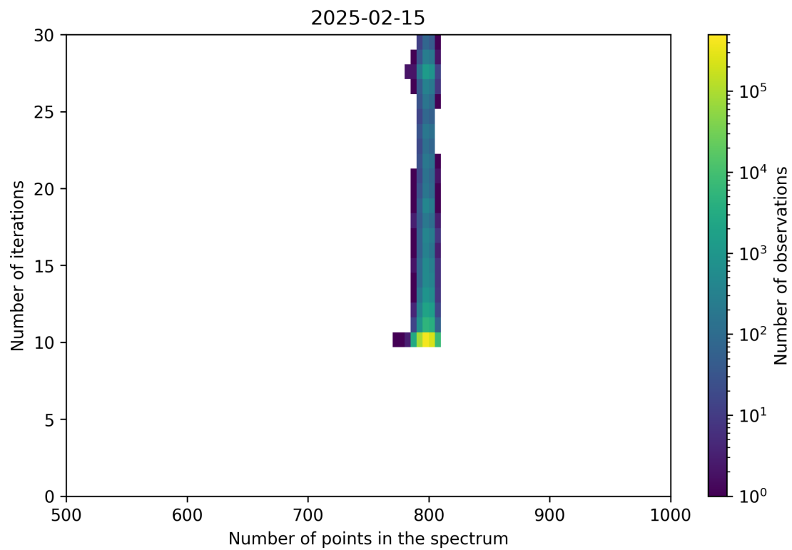
Figure 92: Scatter density plot of “Number of points in the spectrum” against “Number of iterations” for 2025-02-14 to 2025-02-16.
