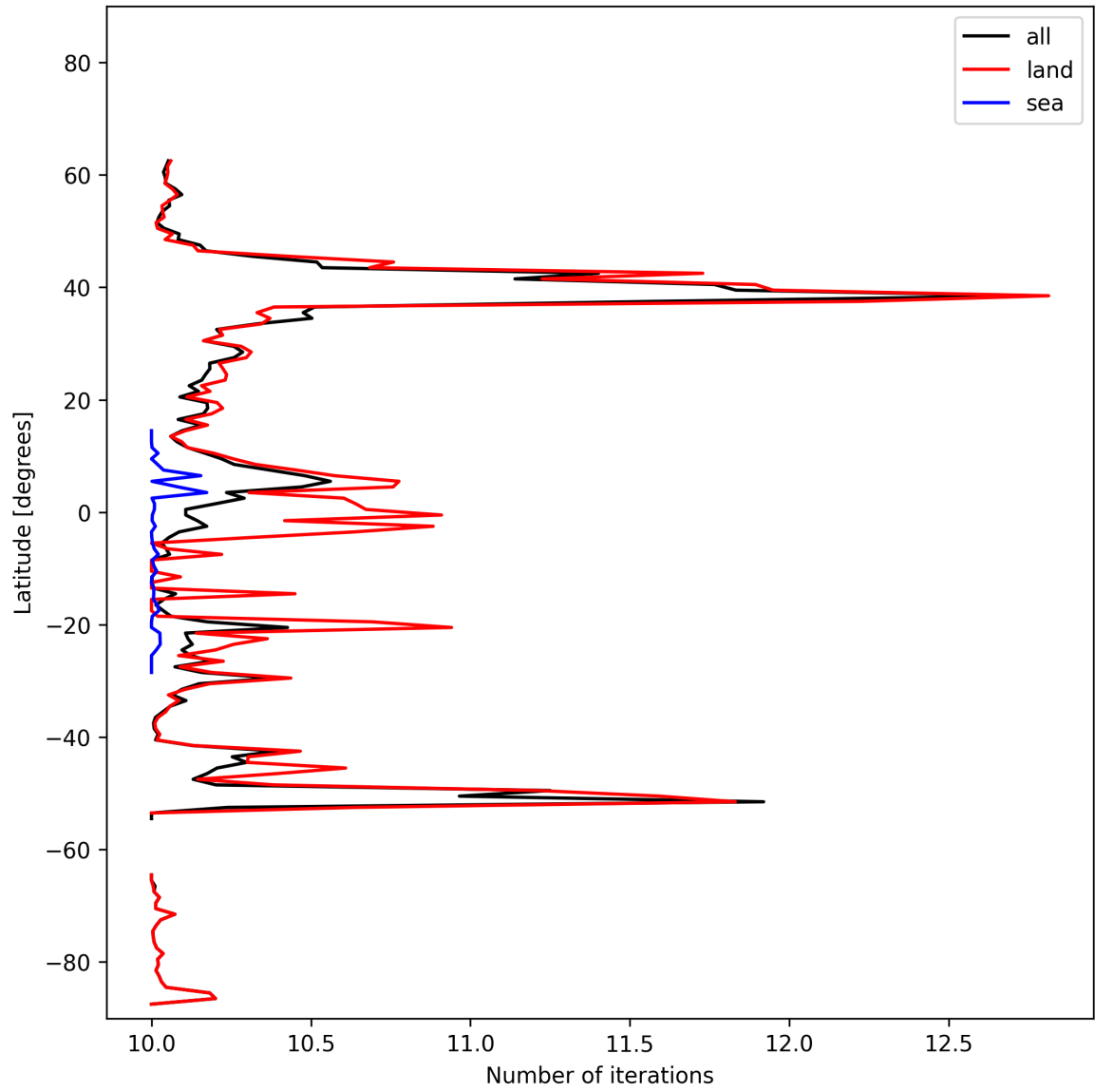
Figure 20: Zonal average of “Number of iterations” for 2025-02-14 to 2025-02-16.
