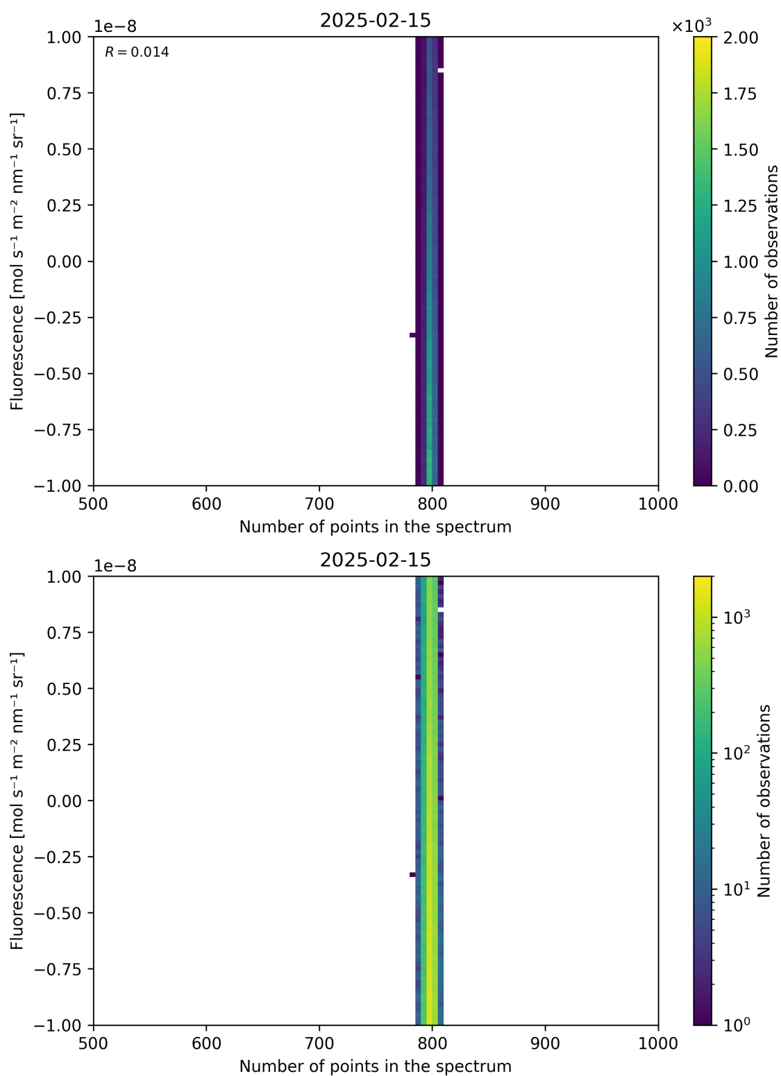
Figure 91: Scatter density plot of “Number of points in the spectrum” against “Fluorescence” for 2025-02-14 to 2025-02-16.
