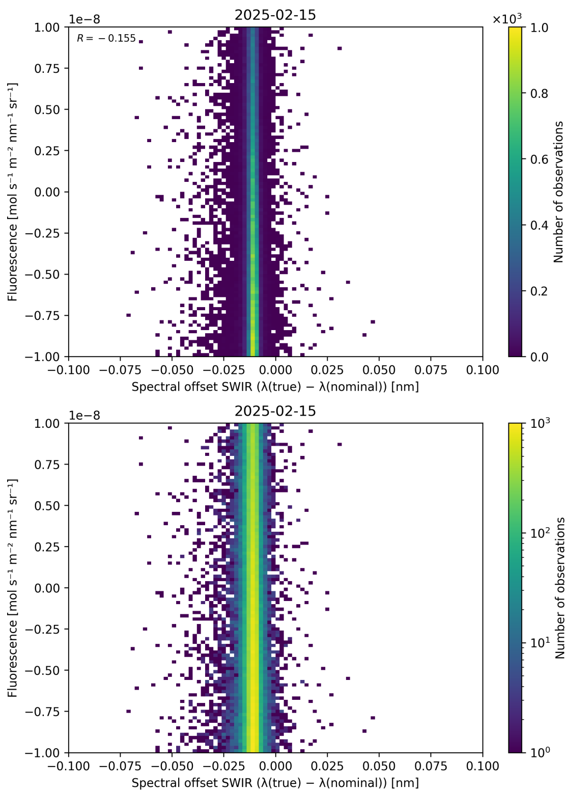
Figure 120: Scatter density plot of “Spectral offset SWIR ( \lambda_{\text{true}} - \lambda_{\text{nominal}} )” against “Fluorescence” for 2025-02-14 to 2025-02-16.
