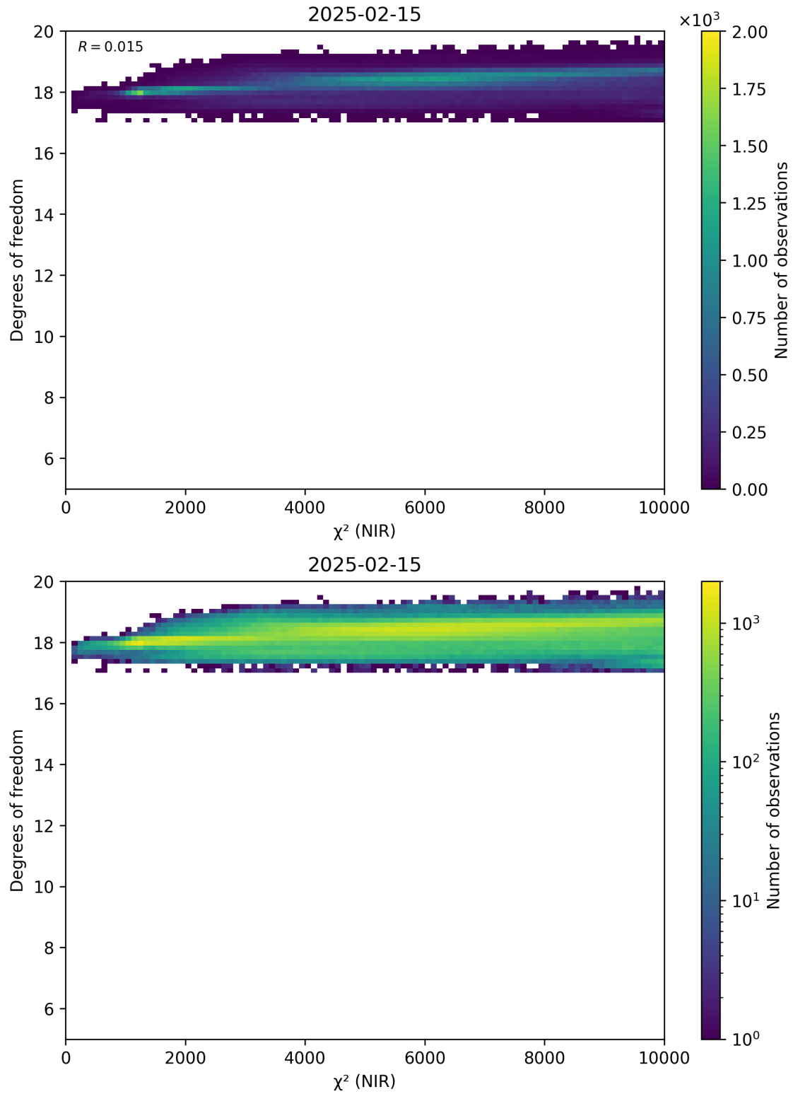
Figure 44: Scatter density plot of “ \chi^2 (NIR)” against “Degrees of freedom” for 2025-02-14 to 2025-02-16.
