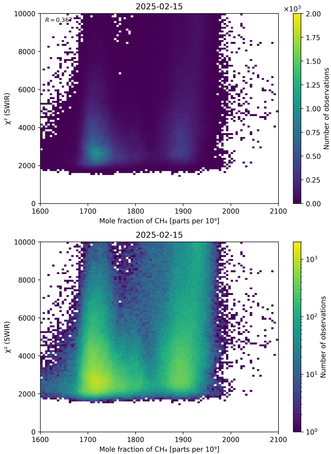
Figure 71: Scatter density plot of “Mole fraction of \text{CH}_4 ” against “ \chi^2 (SWIR)” for 2025-02-14 to 2025-02-16.
