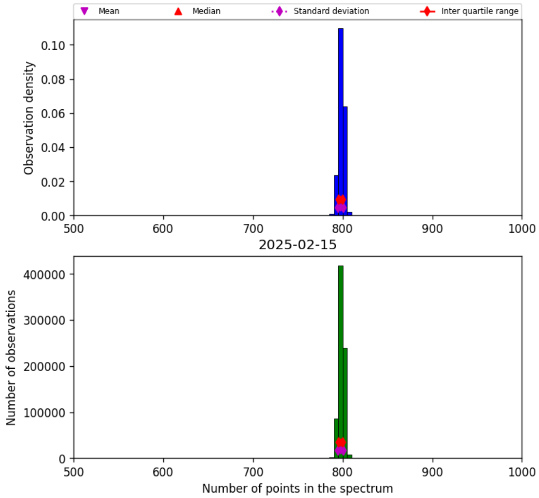
Figure 26: Histogram of “Number of points in the spectrum” for 2025-02-14 to 2025-02-16
