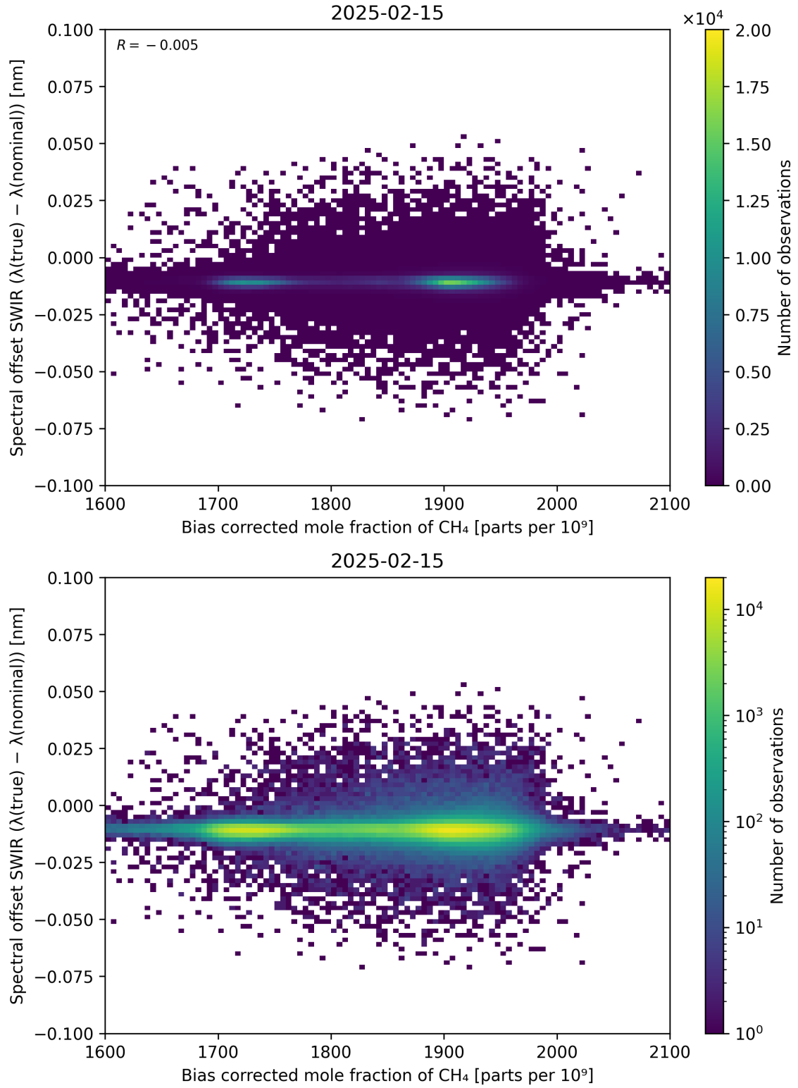
Figure 69: Scatter density plot of “Bias corrected mole fraction of \text{CH}_4 ” against “Spectral offset SWIR ( \lambda_{\text{true}} - \lambda_{\text{nominal}} )” for 2025-02-14 to 2025-02-16.
