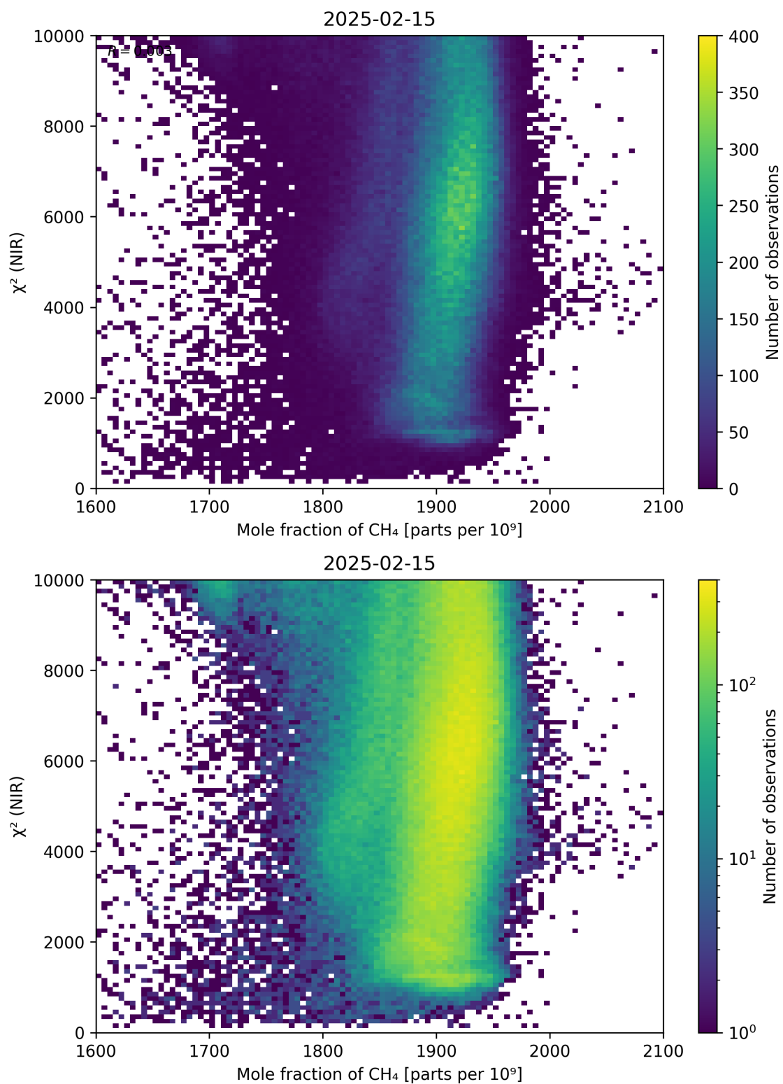
Figure 70: Scatter density plot of “Mole fraction of \text{CH}_4 ” against “ \chi^2 (NIR)” for 2025-02-14 to 2025-02-16.
