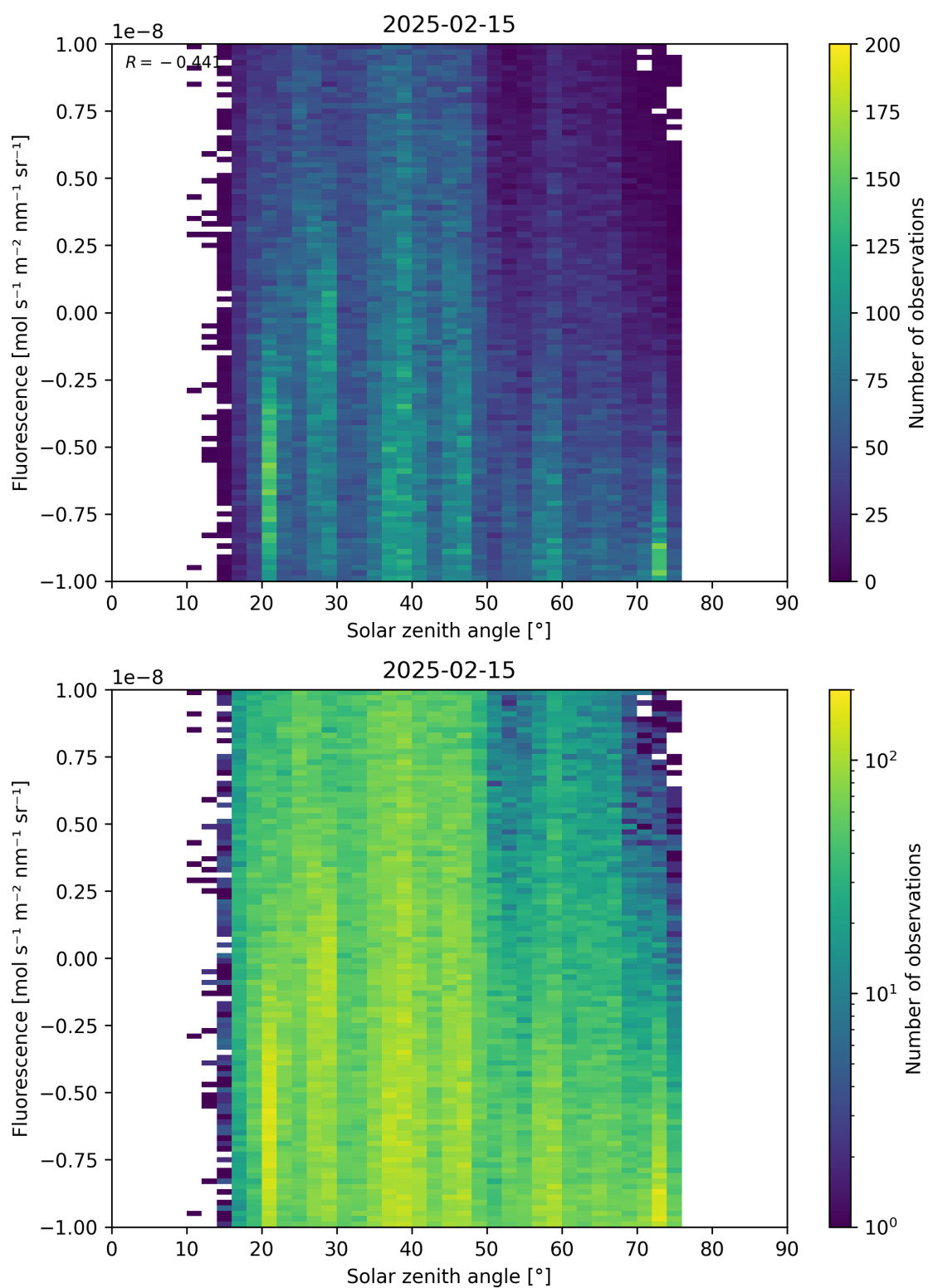
Figure 97: Scatter density plot of “Solar zenith angle” against “Fluorescence” for 2025-02-14 to 2025-02-16.
