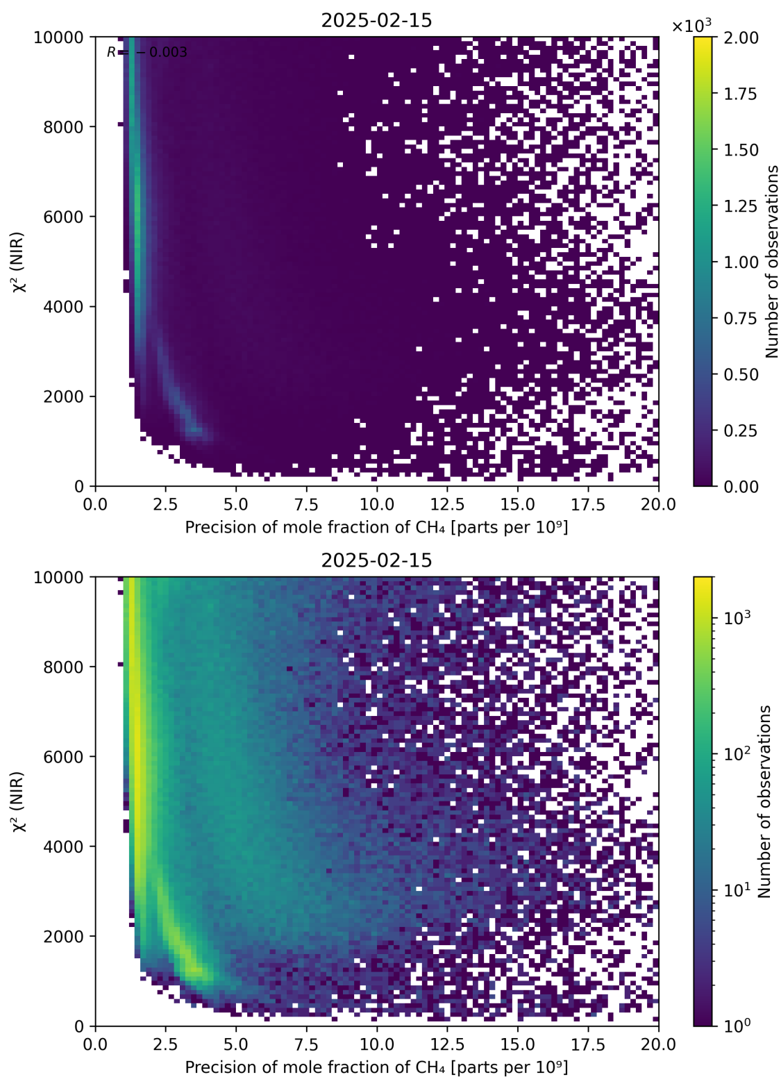
Figure 78: Scatter density plot of “Precision of mole fraction of CH 4 ” against “ \chi^2 (NIR)” for 2025-02-14 to 2025-02-16.
