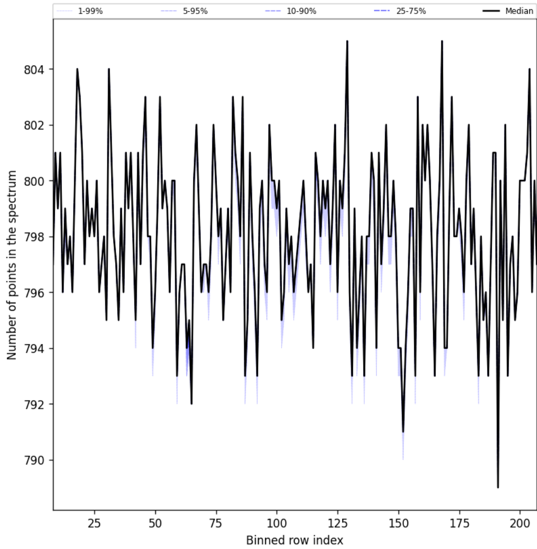
Figure 37: Along track statistics of “Number of points in the spectrum” for 2025-02-14 to 2025-02-16
