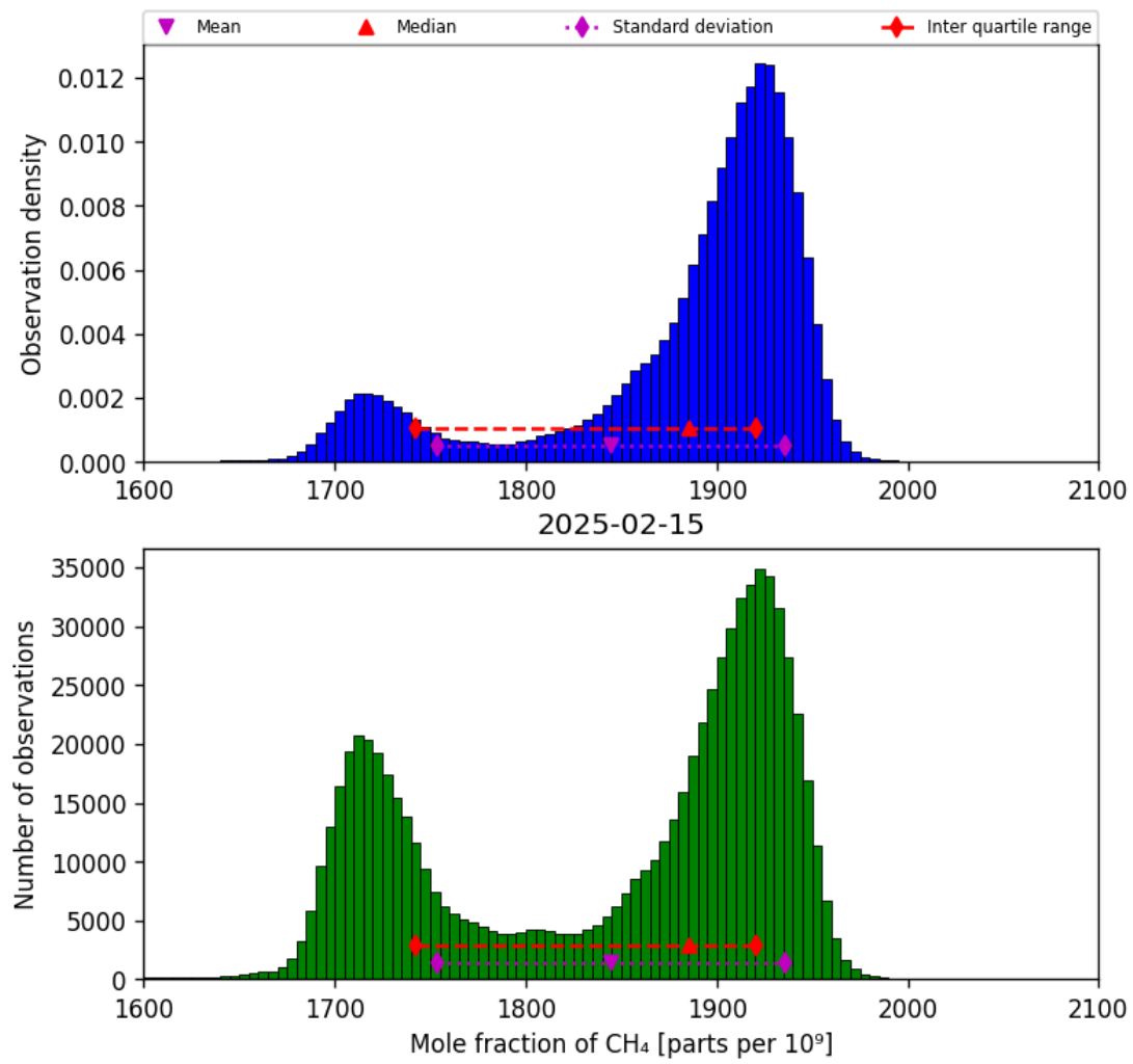
Figure 23: Histogram of “Mole fraction of CH 4 ” for 2025-02-14 to 2025-02-16
