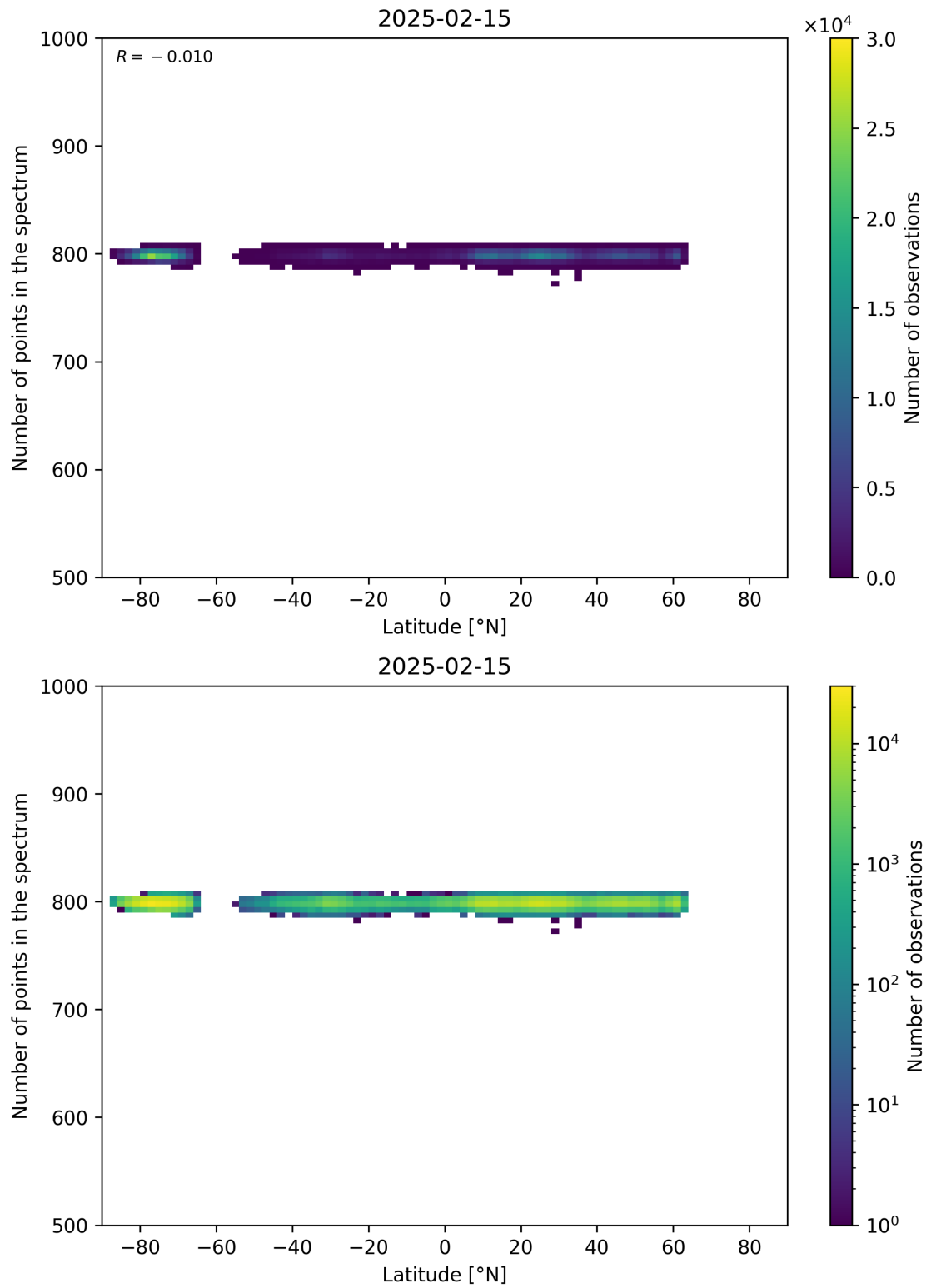
Figure 61: Scatter density plot of “Latitude” against “Number of points in the spectrum” for 2025-02-14 to 2025-02-16.
