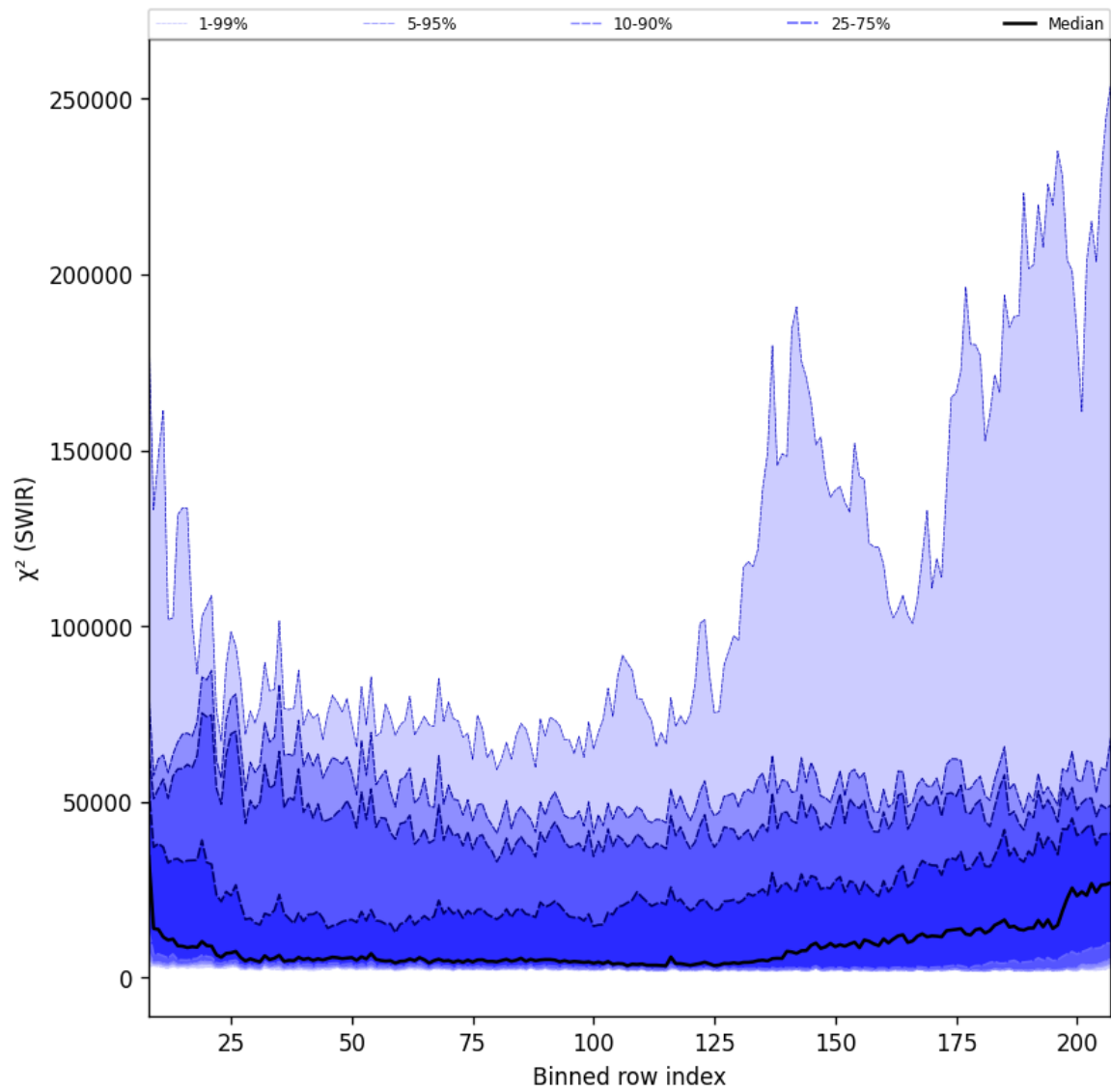
Figure 39: Along track statistics of “ \chi^2 (SWIR)” for 2025-02-14 to 2025-02-16
