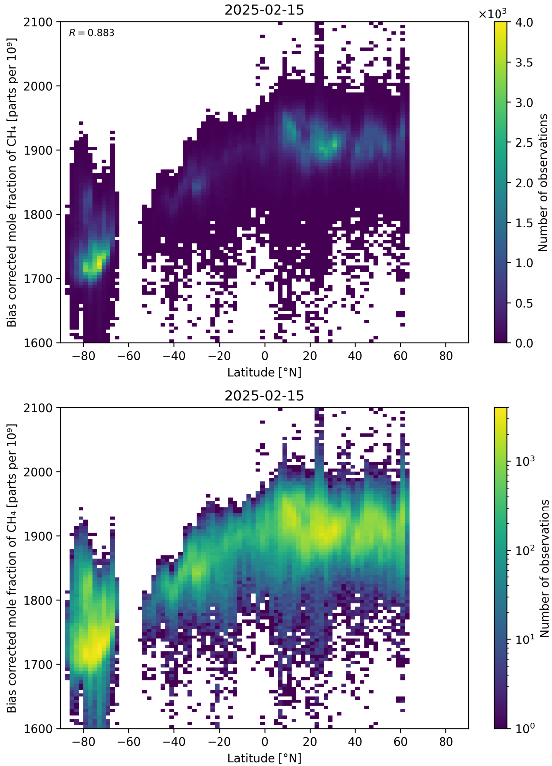
Figure 58: Scatter density plot of “Latitude” against “Bias corrected mole fraction of \text{CH}_4 ” for 2025-02-14 to 2025-02-16.
