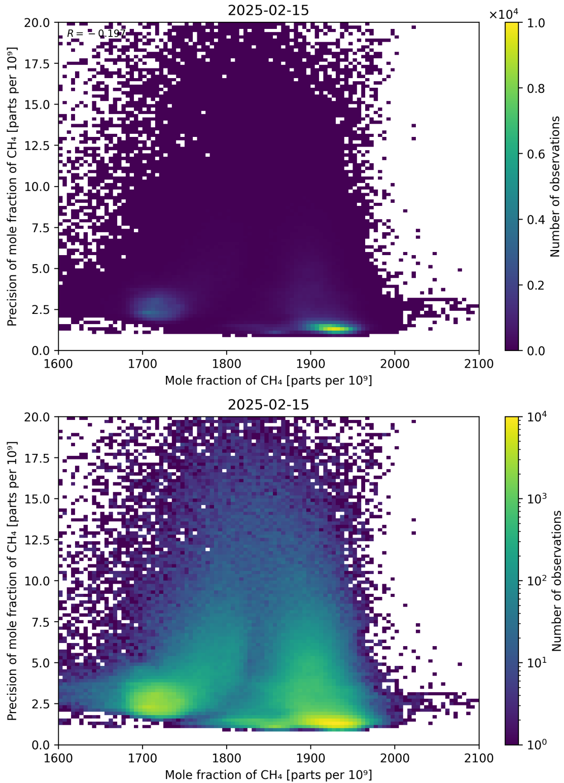
Figure 75: Scatter density plot of “Mole fraction of CH 4 ” against “Precision of mole fraction of CH 4 ” for 2025-02-14 to 2025-02-16.
