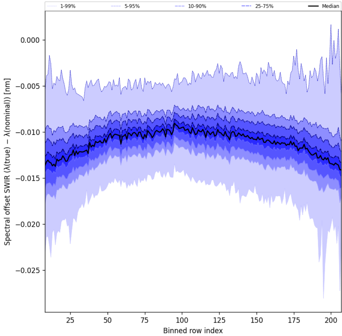
Figure 38: Along track statistics of “Spectral offset SWIR ( \lambda_{\text{true}} - \lambda_{\text{nominal}} )” for 2025-02-14 to 2025-02-16
