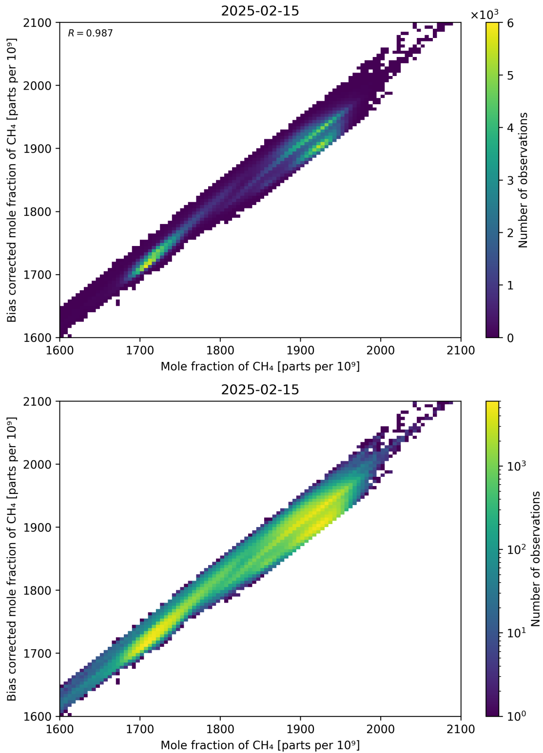
Figure 74: Scatter density plot of “Mole fraction of CH 4 ” against “Bias corrected mole fraction of CH 4 ” for 2025-02-14 to 2025-02-16.
