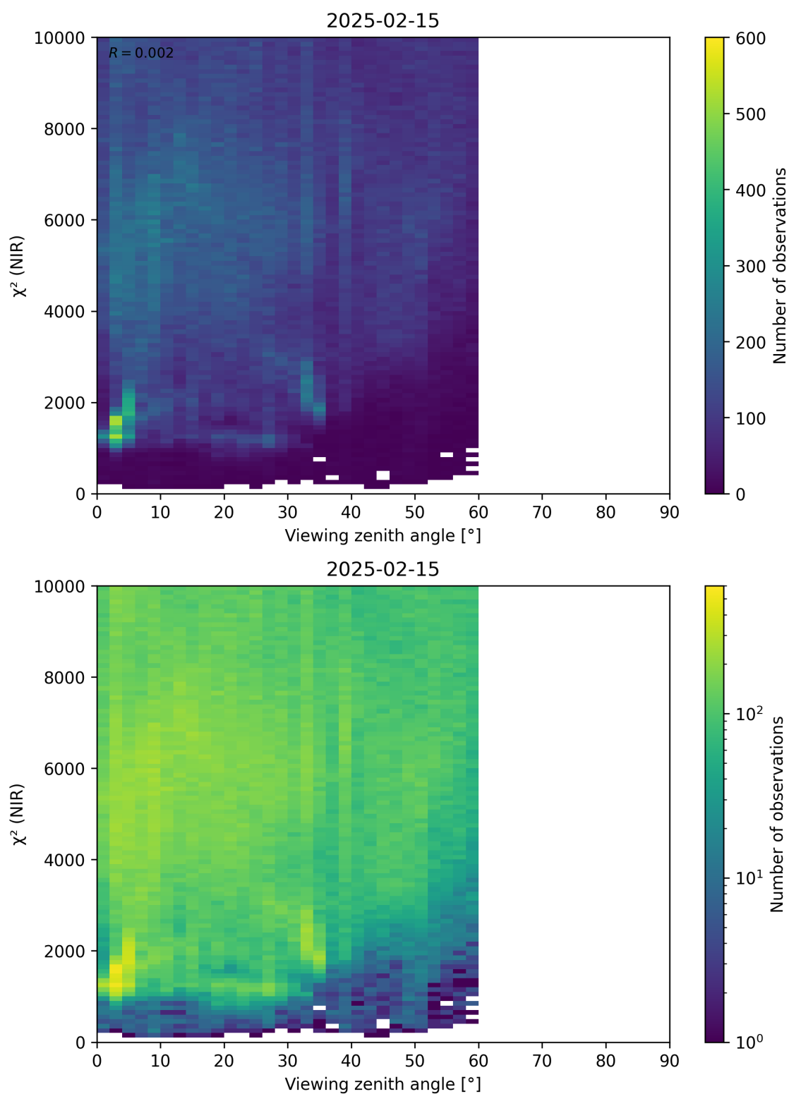
Figure 105: Scatter density plot of “Viewing zenith angle” against “ \chi^2 (NIR)” for 2025-02-14 to 2025-02-16.
