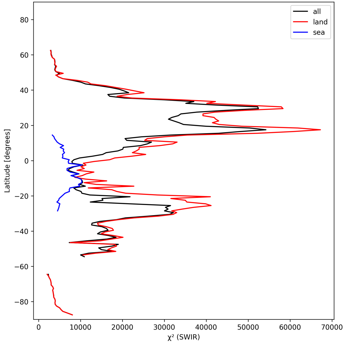
Figure 17: Zonal average of “ \chi^2 (SWIR)” for 2025-02-14 to 2025-02-16.
