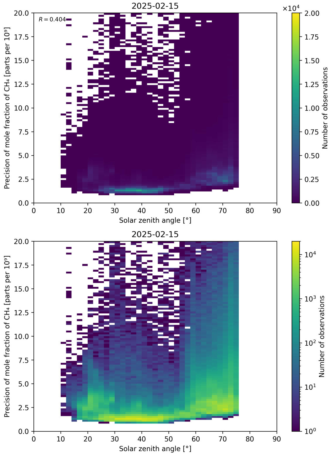
Figure 101: Scatter density plot of “Solar zenith angle” against “Precision of mole fraction of CH 4 ” for 2025-02-14 to 2025-02-16.
