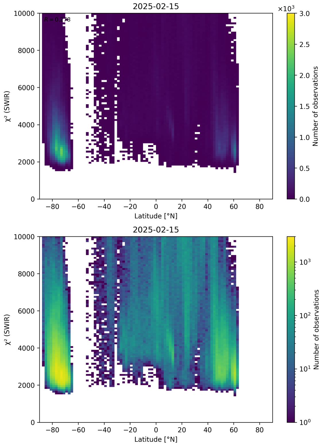
Figure 54: Scatter density plot of “Latitude” against “ \chi^2 (SWIR)” for 2025-02-14 to 2025-02-16.
