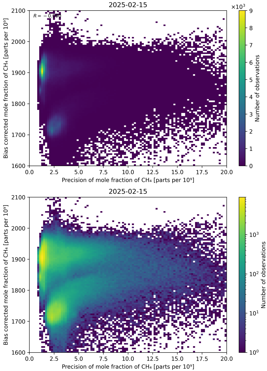
Figure 82: Scatter density plot of “Precision of mole fraction of CH 4 ” against “Bias corrected mole fraction of CH 4 ” for 2025-02-14 to 2025-02-16.
