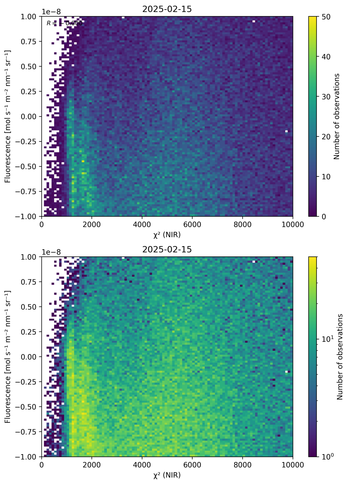
Figure 45: Scatter density plot of “ \chi^2 (NIR)” against “Fluorescence” for 2025-02-14 to 2025-02-16.
