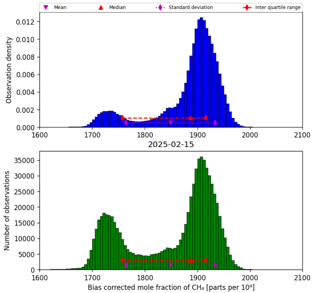
Figure 25: Histogram of “Bias corrected mole fraction of CH 4 ” for 2025-02-14 to 2025-02-16
