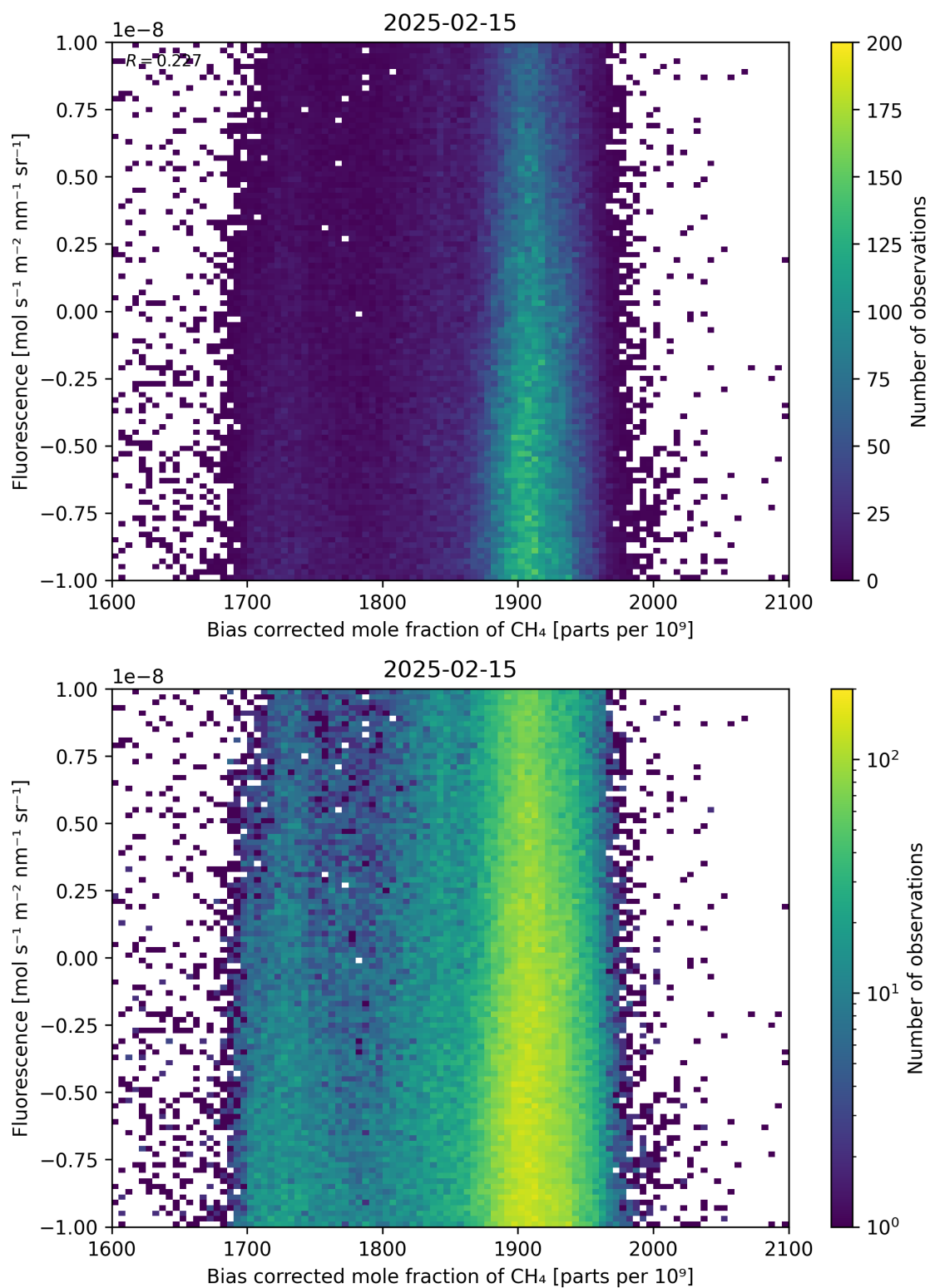
Figure 66: Scatter density plot of “Bias corrected mole fraction of \text{CH}_4 ” against “Fluorescence” for 2025-02-14 to 2025-02-16.
