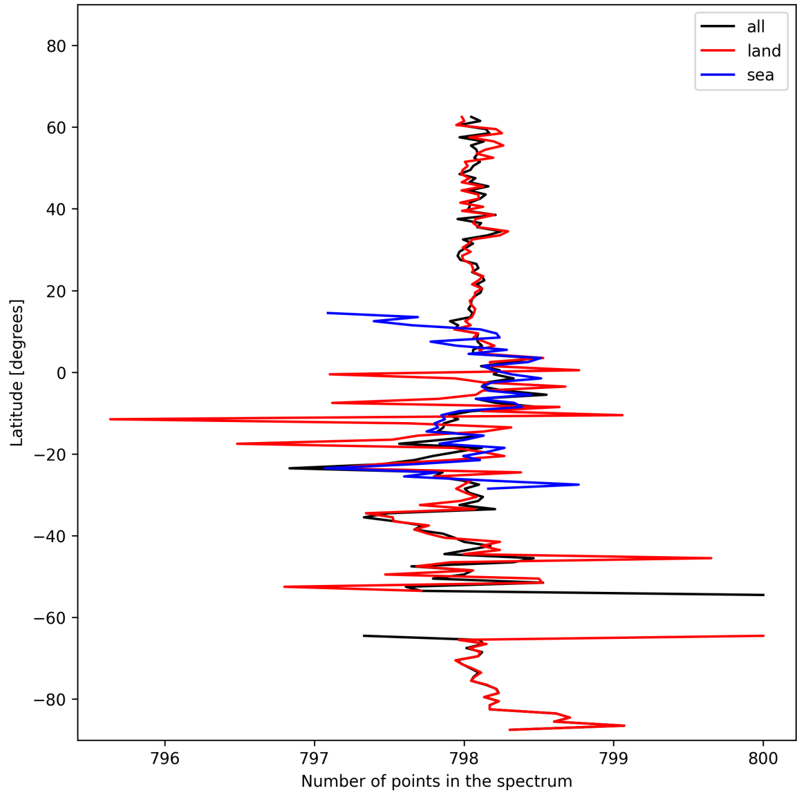
Figure 15: Zonal average of “Number of points in the spectrum” for 2025-02-14 to 2025-02-16.
