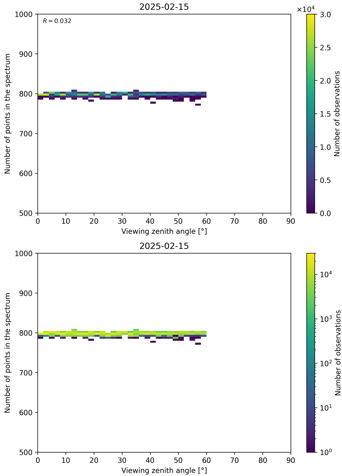
Figure 114: Scatter density plot of “Viewing zenith angle” against “Number of points in the spectrum” for 2025-02-14 to 2025-02-16.
