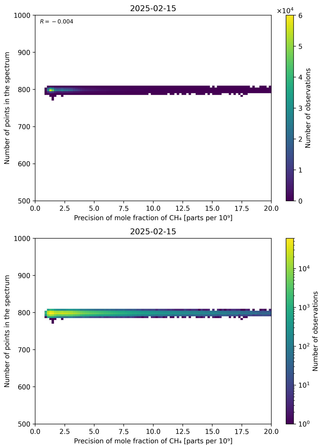
Figure 84: Scatter density plot of “Precision of mole fraction of CH 4 ” against “Number of points in the spectrum” for 2025-02-14 to 2025-02-16.
