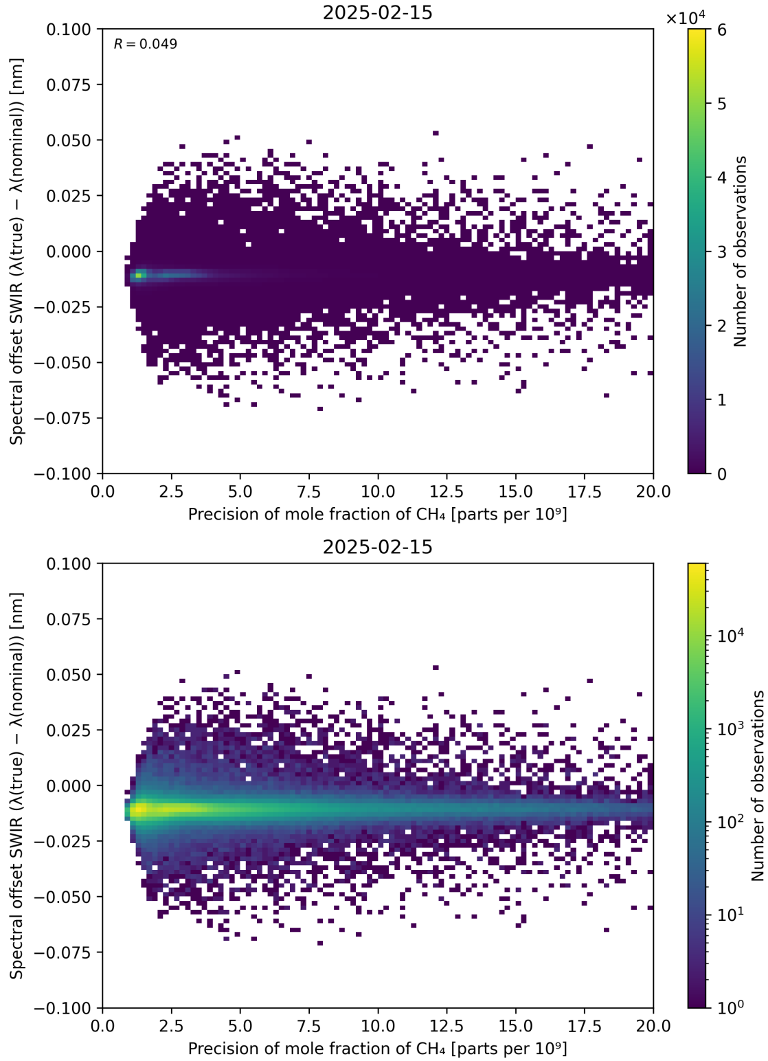
Figure 85: Scatter density plot of “Precision of mole fraction of \text{CH}_4 ” against “Spectral offset SWIR ( \lambda_{\text{true}} - \lambda_{\text{nominal}} )” for 2025-02-14 to 2025-02-16.
