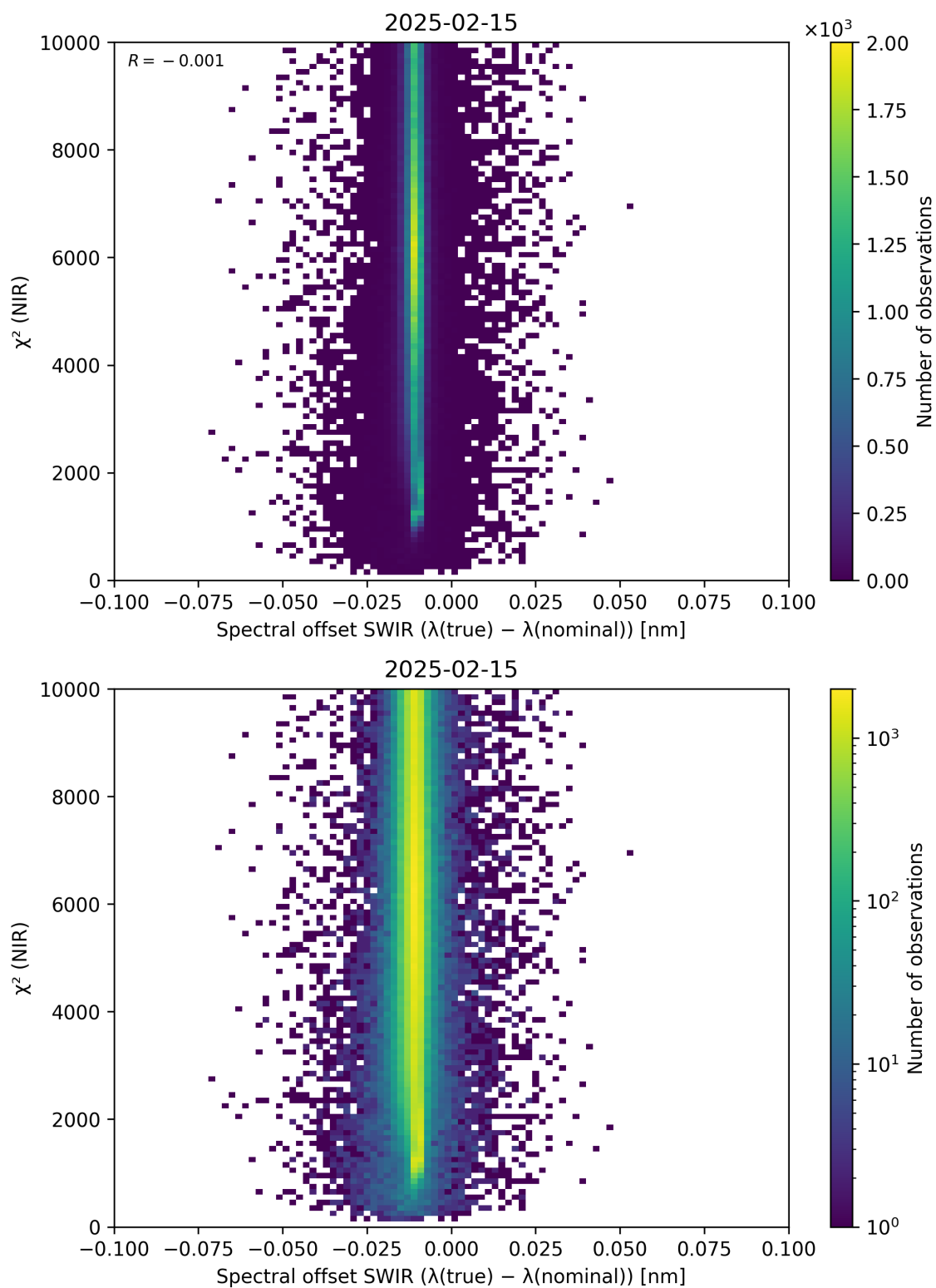
Figure 117: Scatter density plot of “Spectral offset SWIR ( \lambda_{\text{true}} - \lambda_{\text{nominal}} )” against “ \chi^2 (NIR)” for 2025-02-14 to 2025-02-16.
