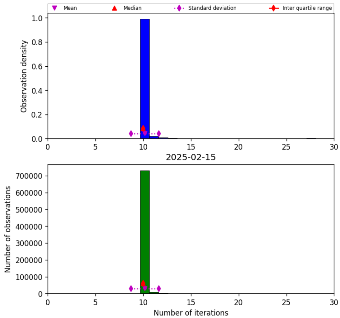
Figure 31: Histogram of “Number of iterations” for 2025-02-14 to 2025-02-16
