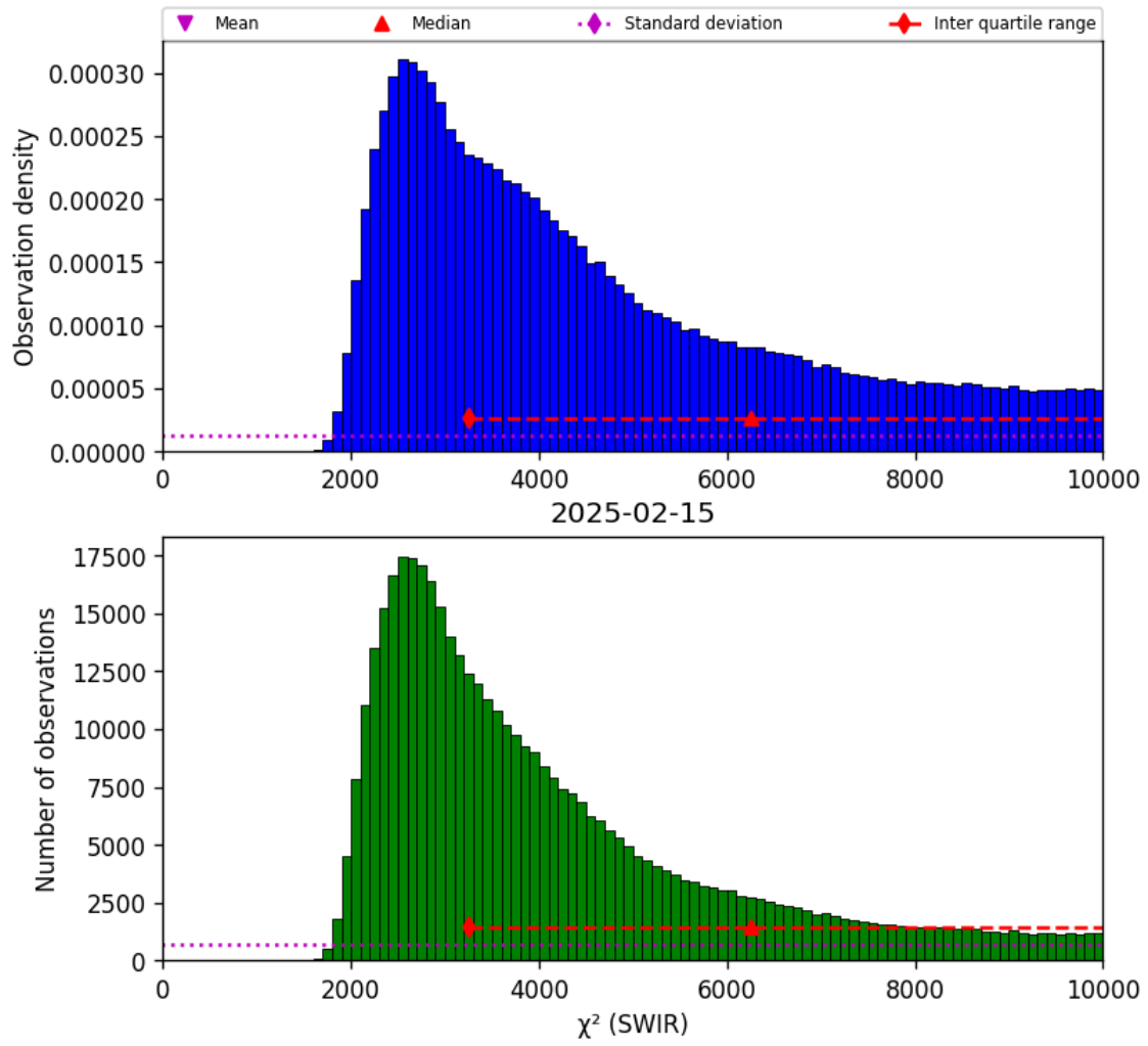
Figure 28: Histogram of “ \chi^2 (SWIR)” for 2025-02-14 to 2025-02-16
