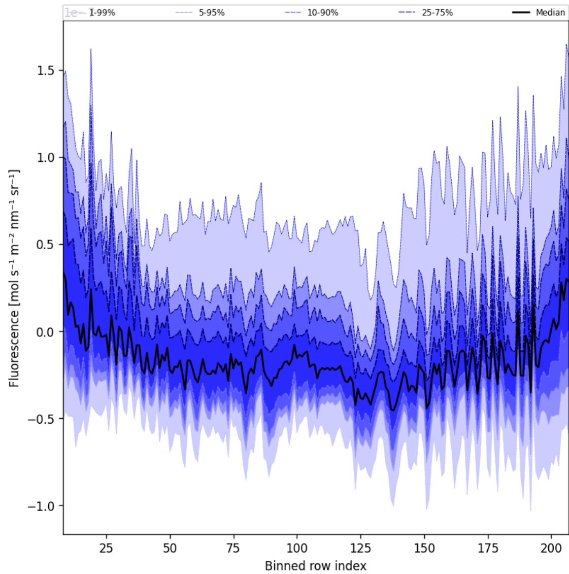
Figure 43: Along track statistics of “Fluorescence” for 2025-02-14 to 2025-02-16
