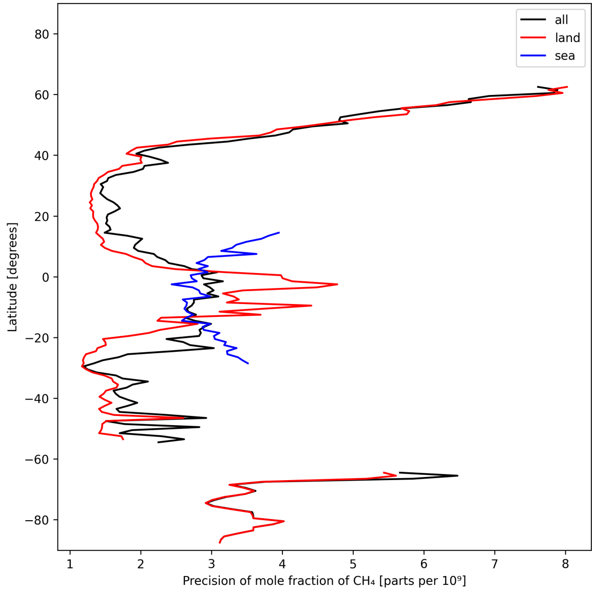
Figure 13: Zonal average of “Precision of mole fraction of CH 4 ” for 2025-02-14 to 2025-02-16.
