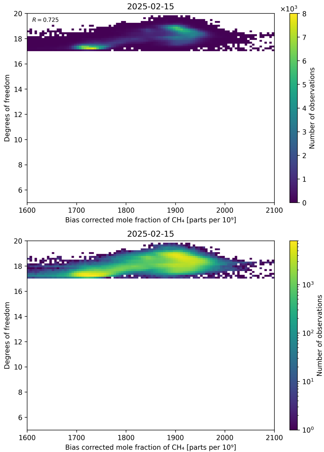
Figure 65: Scatter density plot of “Bias corrected mole fraction of CH 4 ” against “Degrees of freedom” for 2025-02-14 to 2025-02-16.
