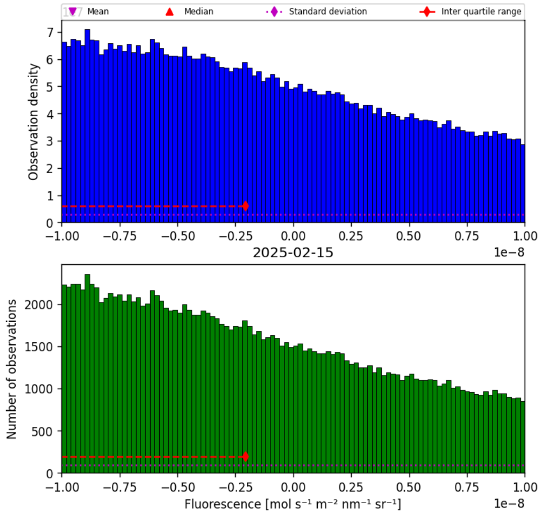
Figure 32: Histogram of “Fluorescence” for 2025-02-14 to 2025-02-16
