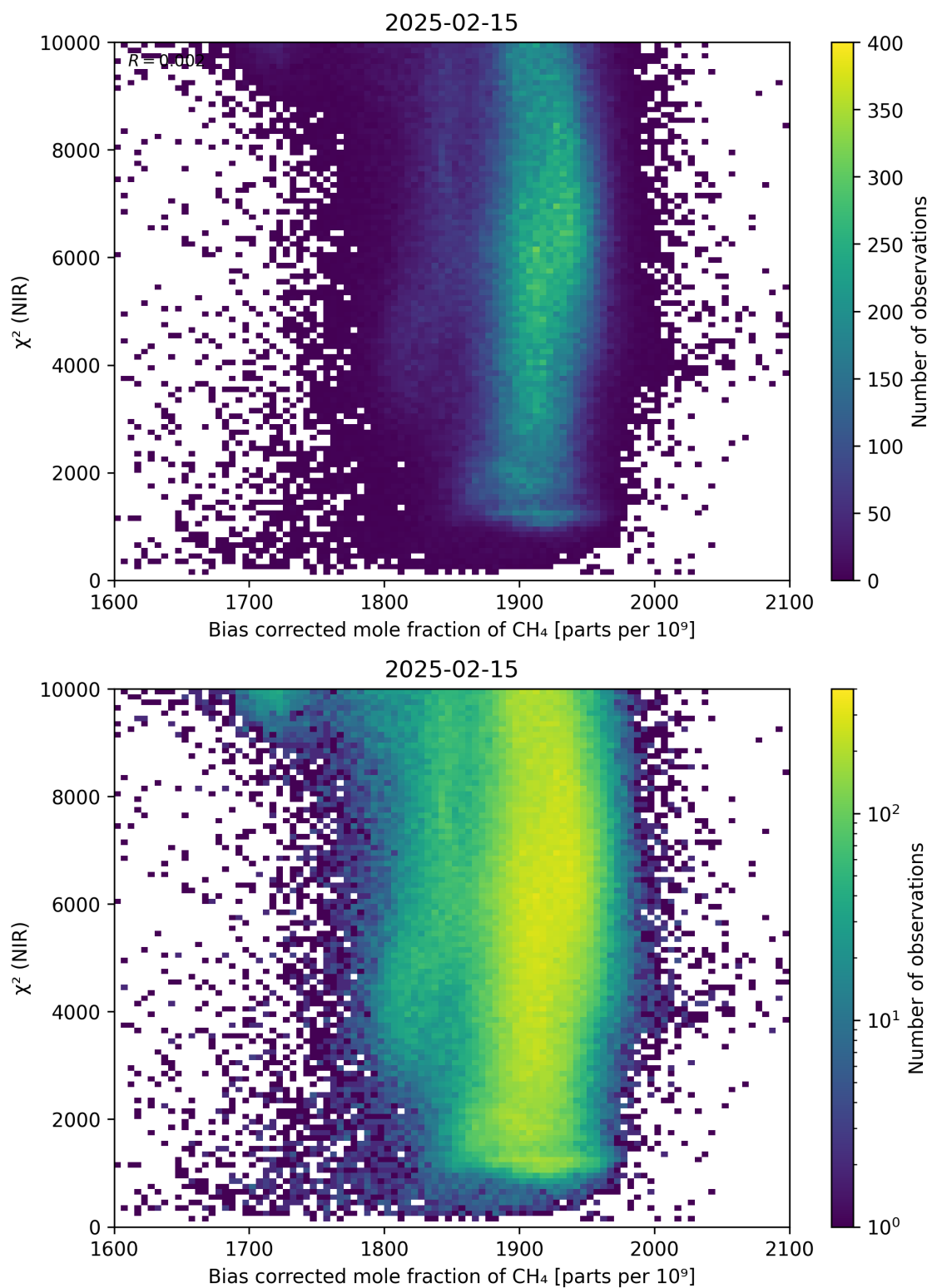
Figure 63: Scatter density plot of “Bias corrected mole fraction of \text{CH}_4 ” against “ \chi^2 (NIR)” for 2025-02-14 to 2025-02-16.
