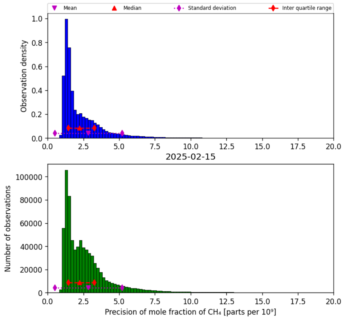
Figure 24: Histogram of “Precision of mole fraction of CH 4 ” for 2025-02-14 to 2025-02-16
