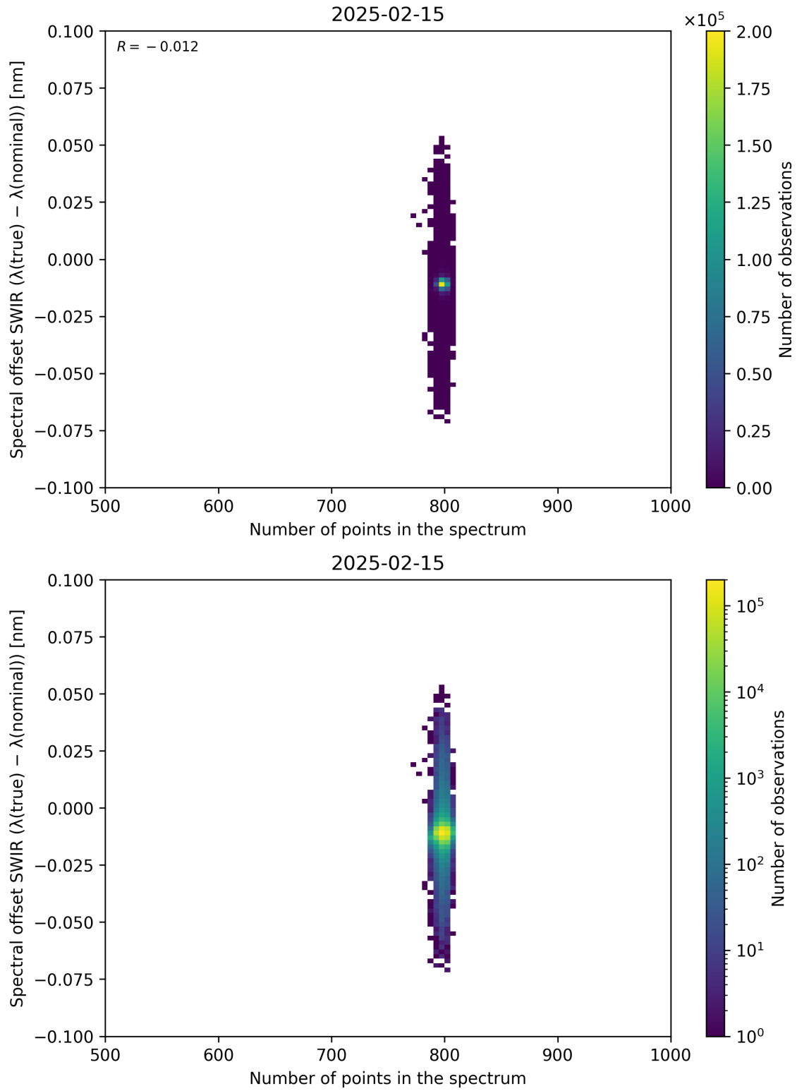
Figure 93: Scatter density plot of “Number of points in the spectrum” against “Spectral offset SWIR ( \lambda_{\text{true}} - \lambda_{\text{nominal}} )” for 2025-02-14 to 2025-02-16.
