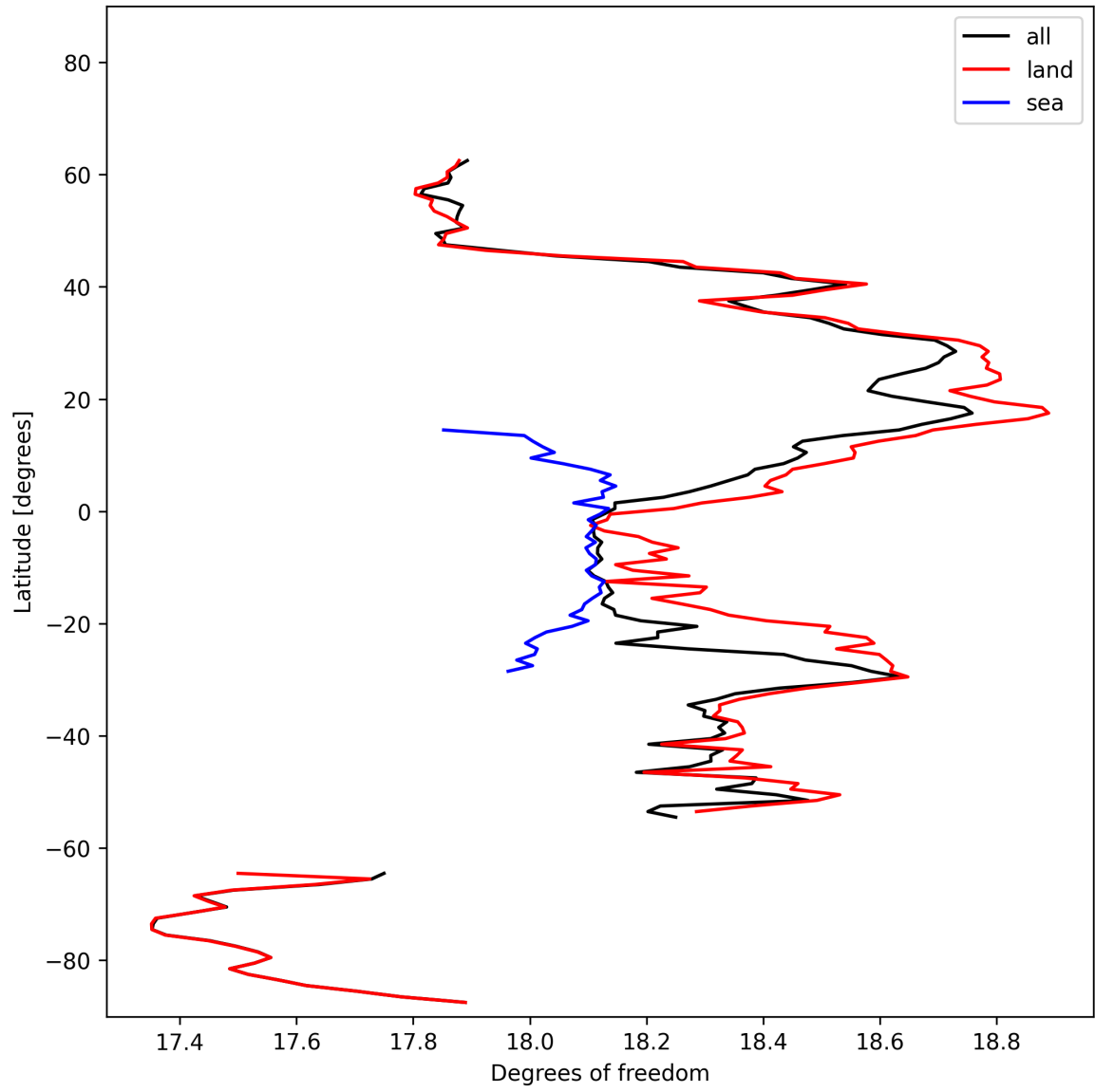
Figure 19: Zonal average of “Degrees of freedom” for 2025-02-14 to 2025-02-16.
