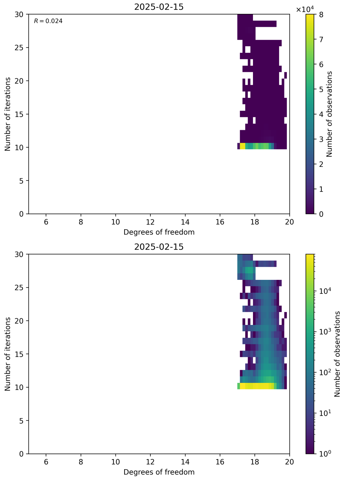
Figure 52: Scatter density plot of “Degrees of freedom” against “Number of iterations” for 2025-02-14 to 2025-02-16.
