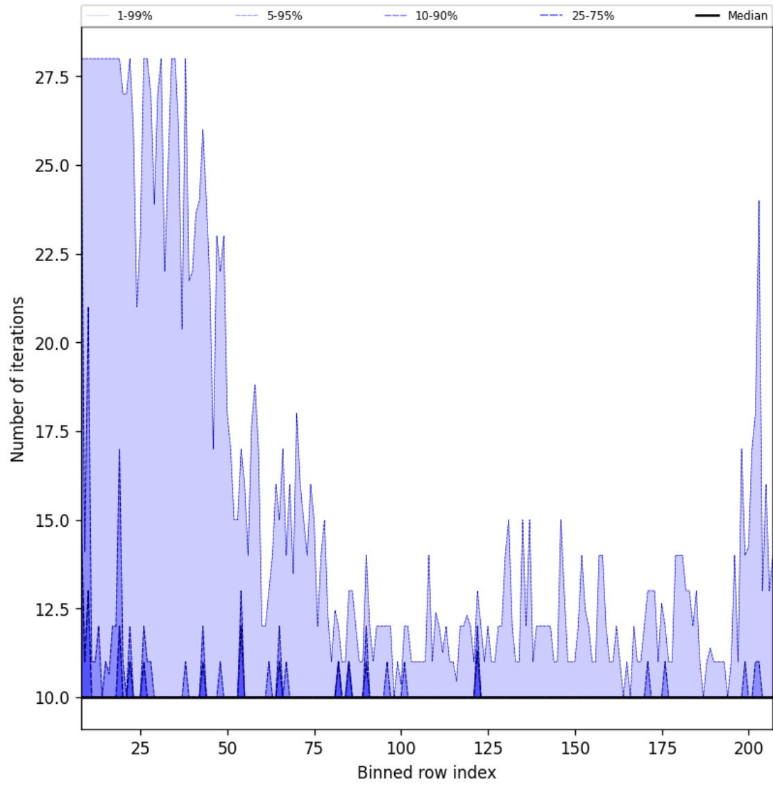
Figure 42: Along track statistics of “Number of iterations” for 2025-02-14 to 2025-02-16
