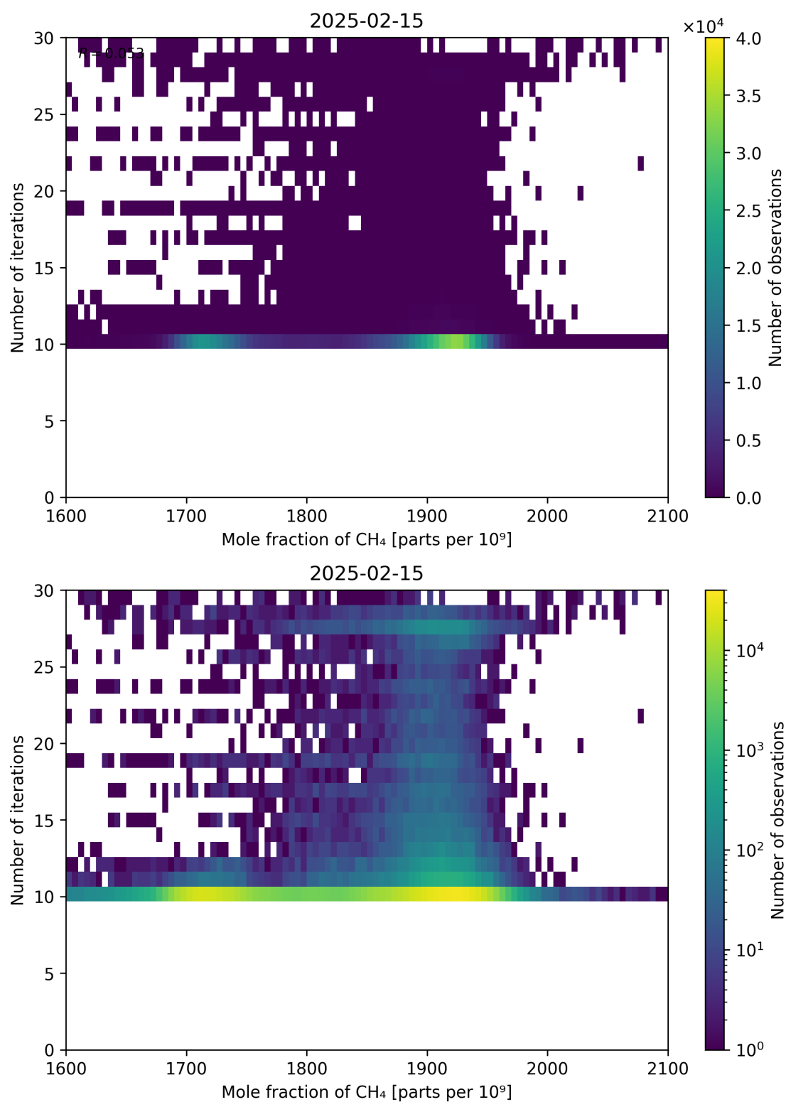
Figure 76: Scatter density plot of “Mole fraction of CH 4 ” against “Number of iterations” for 2025-02-14 to 2025-02-16.
