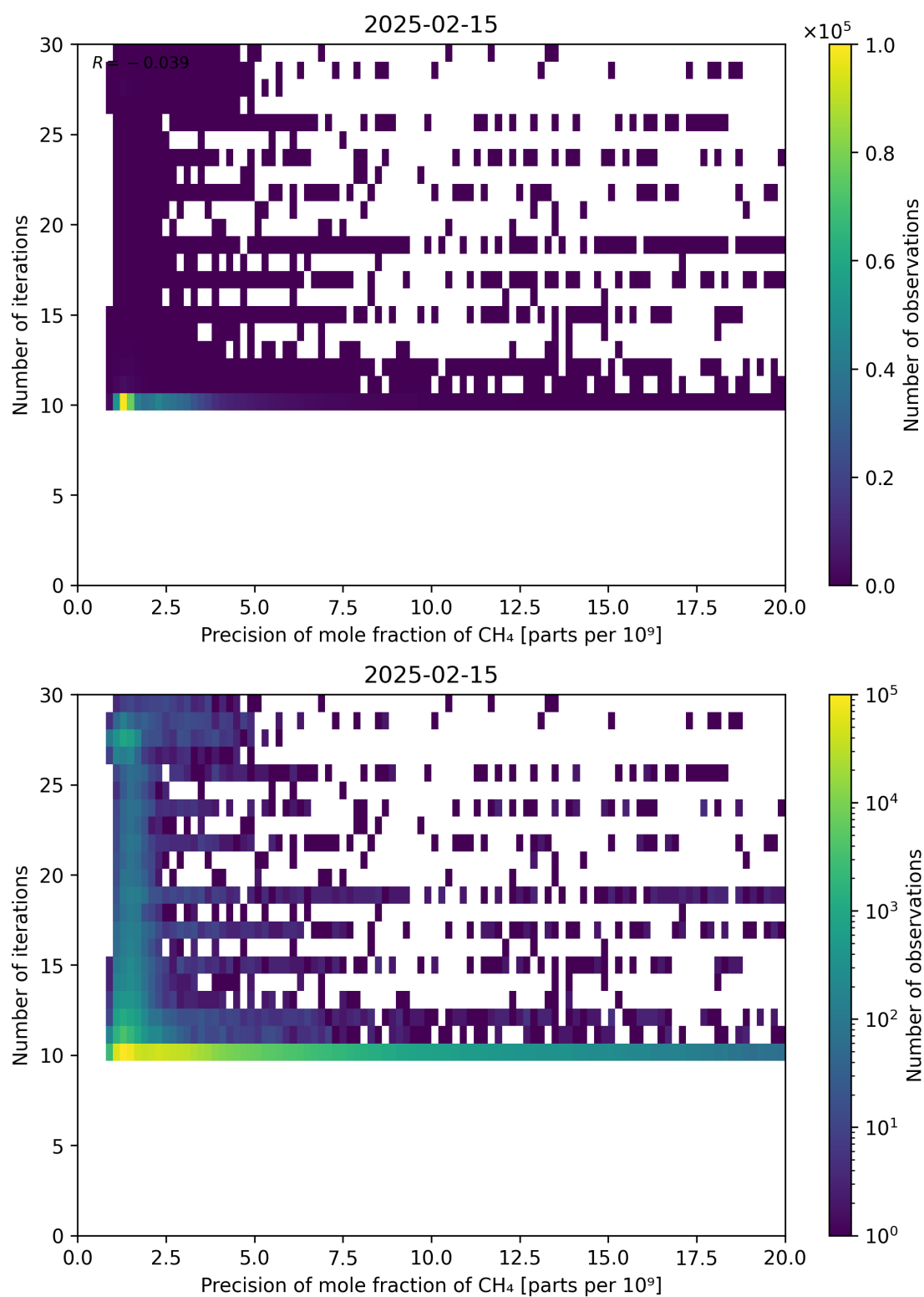
Figure 83: Scatter density plot of “Precision of mole fraction of CH 4 ” against “Number of iterations” for 2025-02-14 to 2025-02-16.
