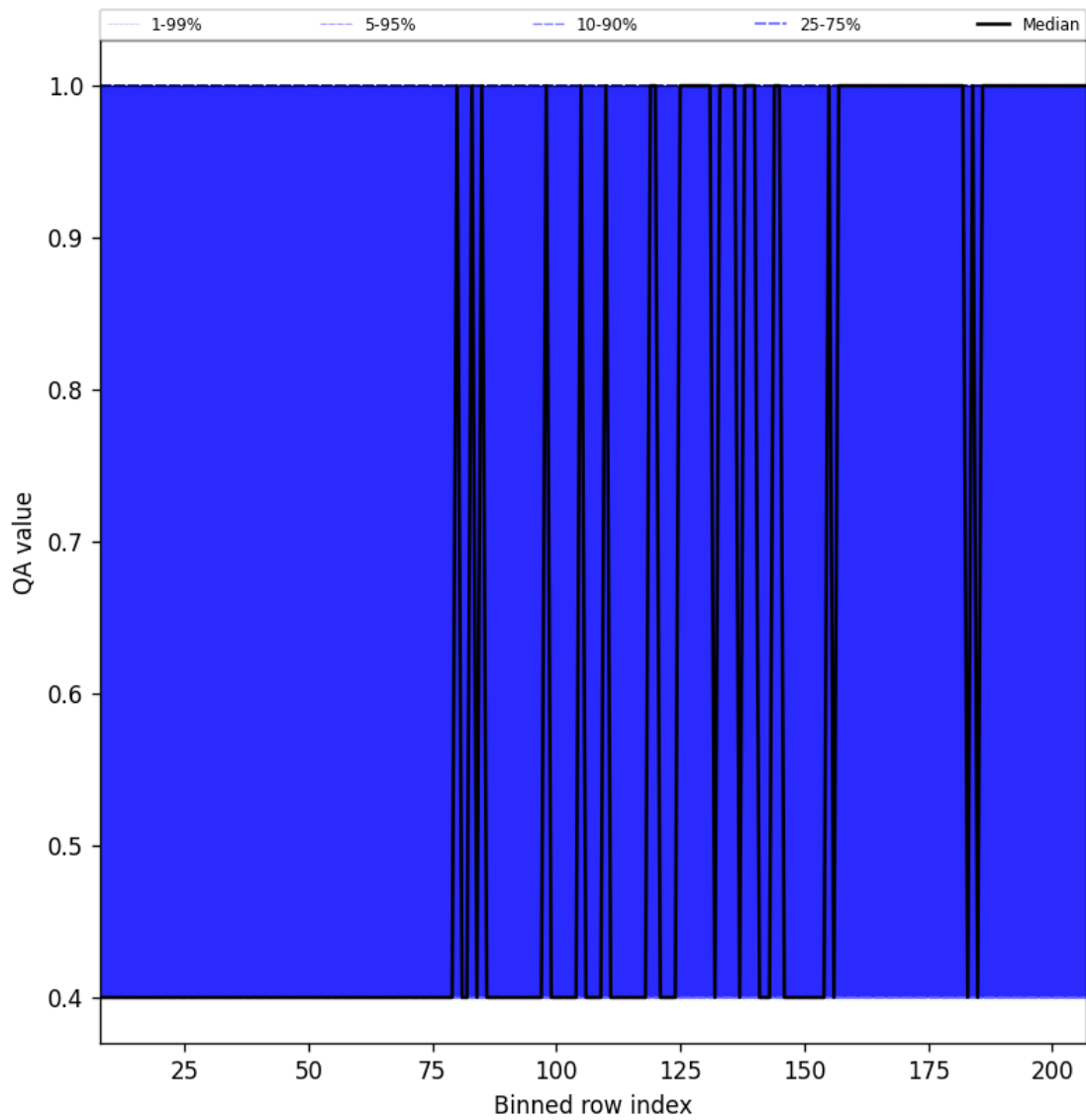
Figure 33: Along track statistics of “QA value” for 2025-02-14 to 2025-02-16
