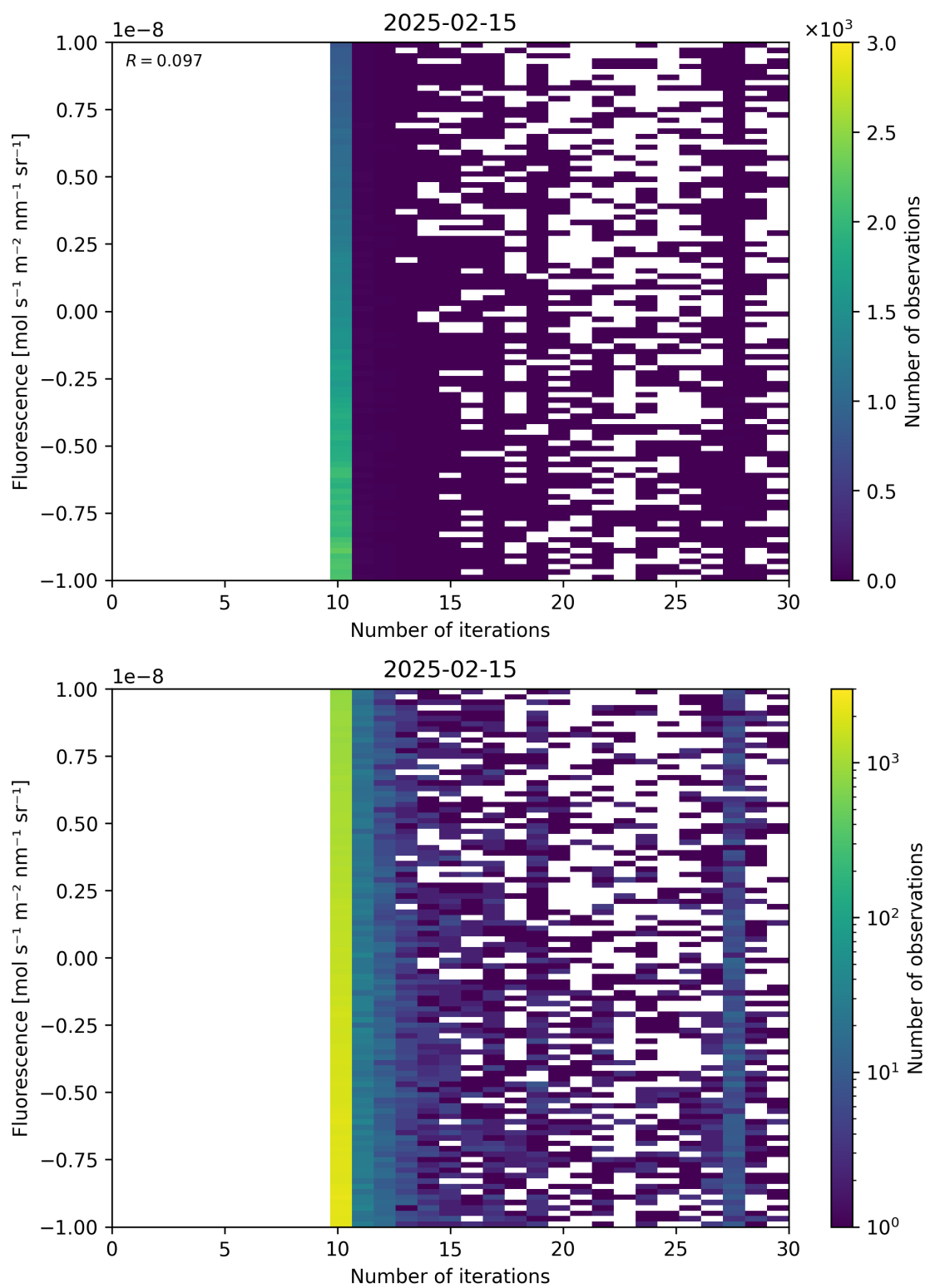
Figure 87: Scatter density plot of “Number of iterations” against “Fluorescence” for 2025-02-14 to 2025-02-16.
