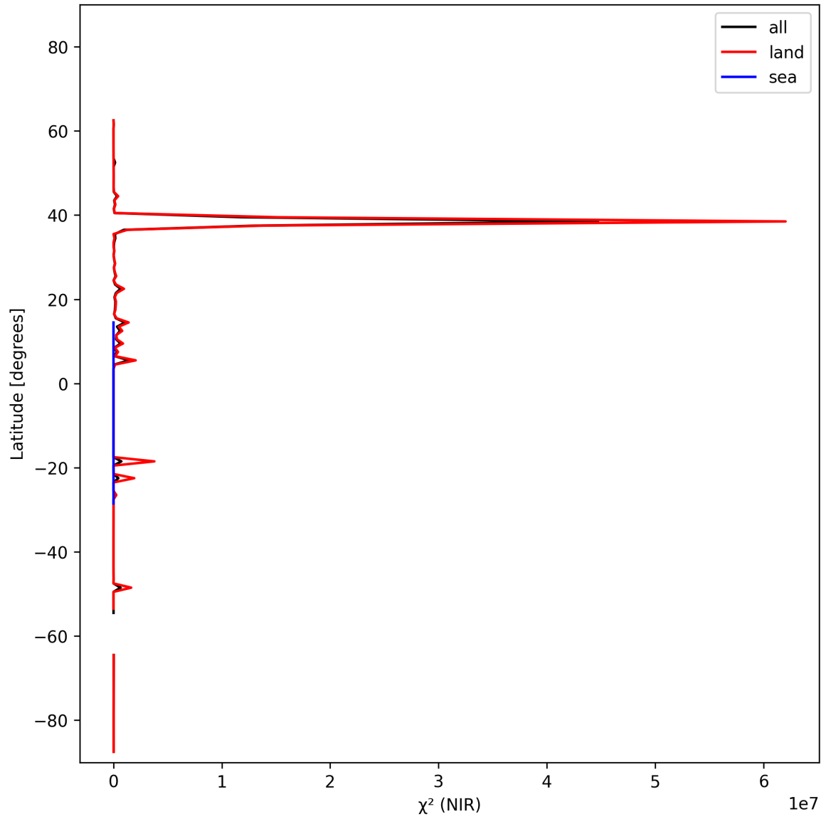
Figure 18: Zonal average of “ \chi^2 (NIR)” for 2025-02-14 to 2025-02-16.
