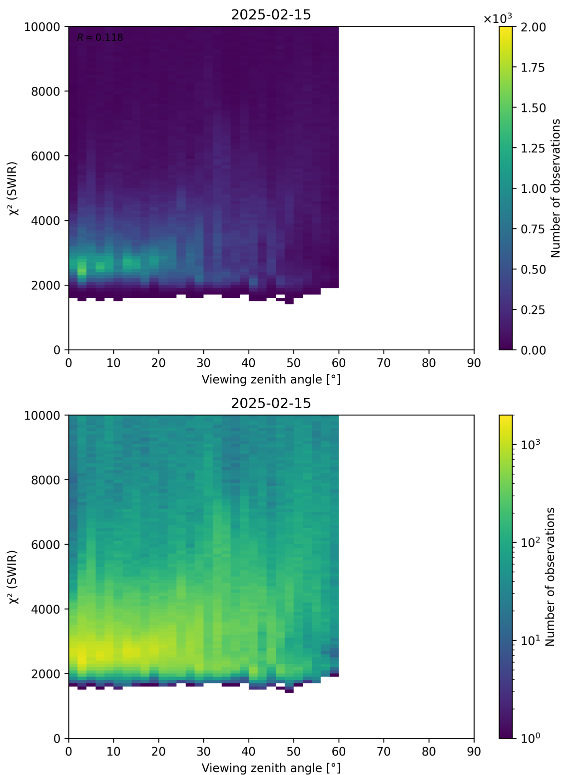
Figure 106: Scatter density plot of “Viewing zenith angle” against “ \chi^2 (SWIR)” for 2025-02-14 to 2025-02-16.
