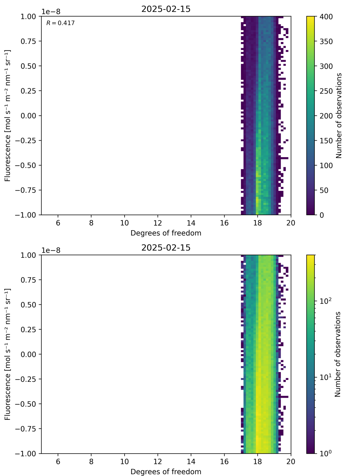
Figure 51: Scatter density plot of “Degrees of freedom” against “Fluorescence” for 2025-02-14 to 2025-02-16.
