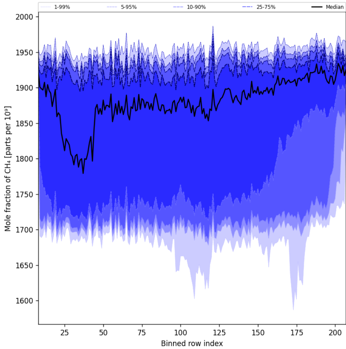
Figure 34: Along track statistics of “Mole fraction of CH 4 ” for 2025-02-14 to 2025-02-16
