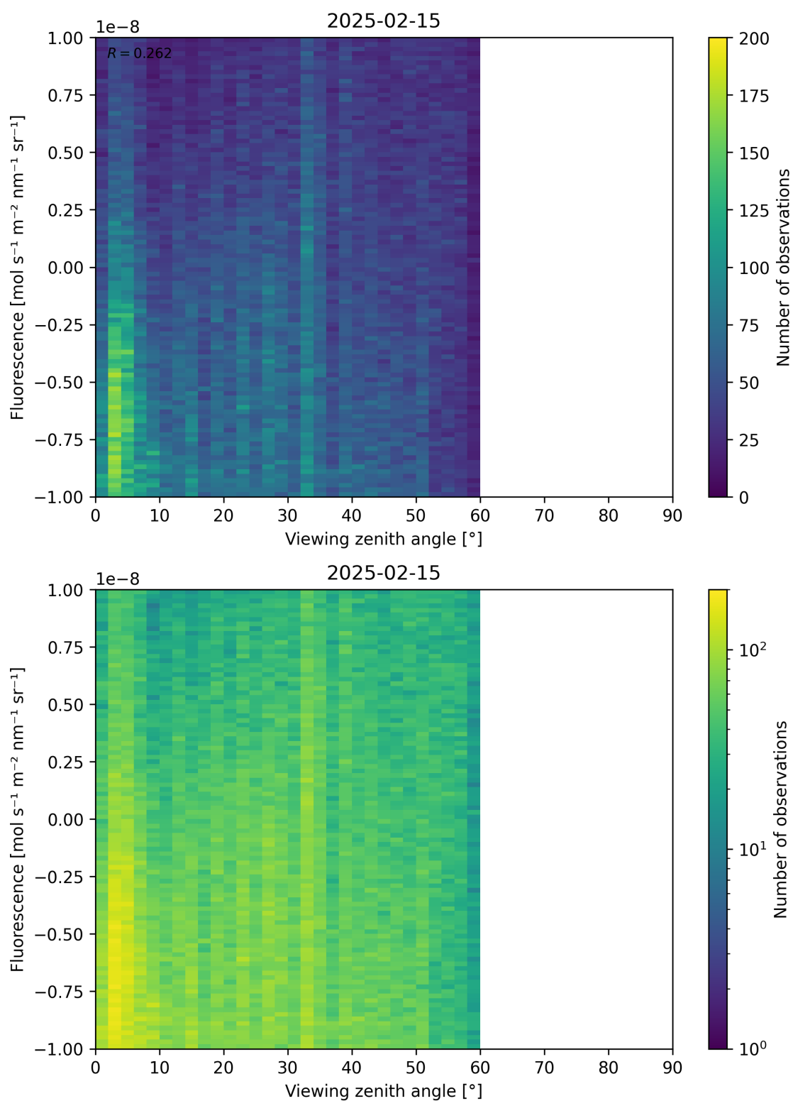
Figure 108: Scatter density plot of “Viewing zenith angle” against “Fluorescence” for 2025-02-14 to 2025-02-16.
