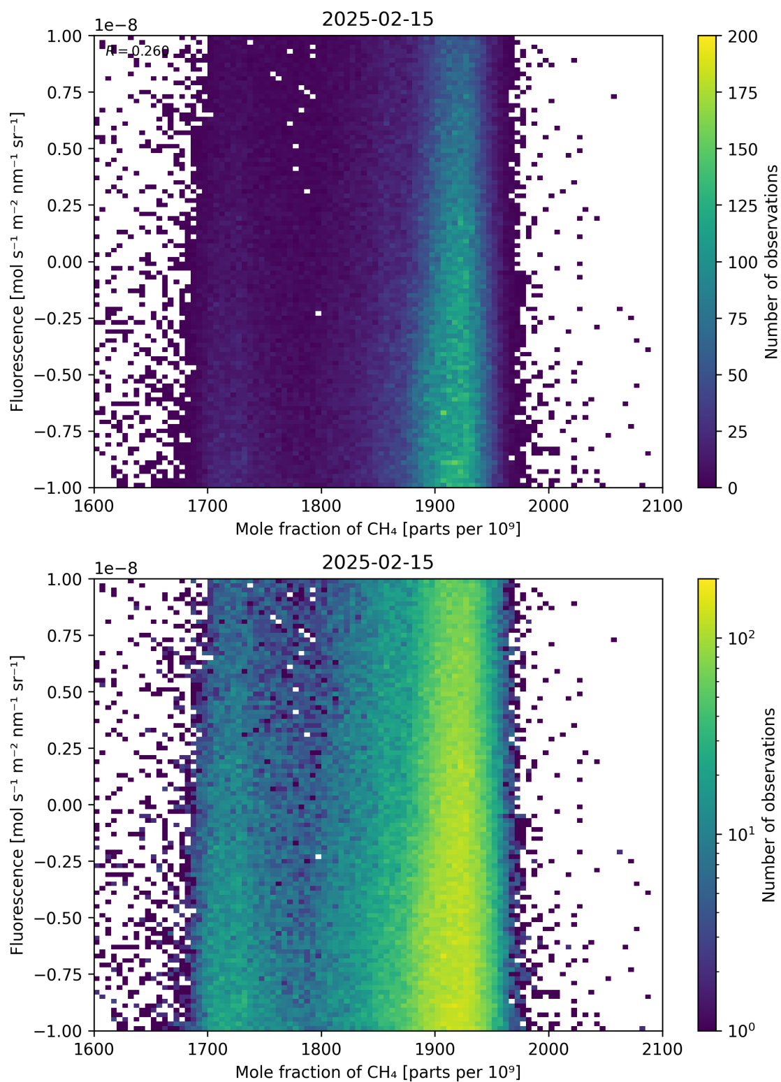
Figure 73: Scatter density plot of “Mole fraction of CH 4 ” against “Fluorescence” for 2025-02-14 to 2025-02-16.
