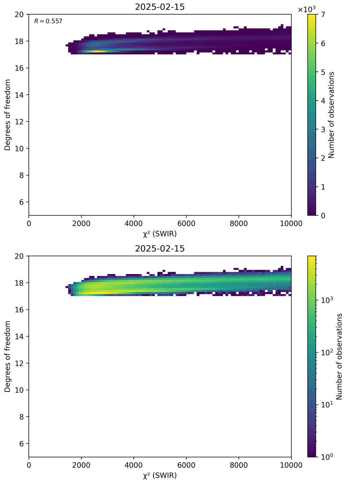
Figure 48: Scatter density plot of “ \chi^2 (SWIR)” against “Degrees of freedom” for 2025-02-14 to 2025-02-16.
