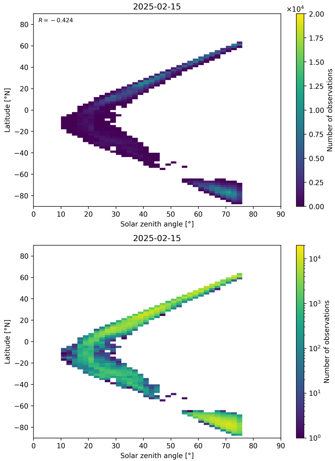
Figure 98: Scatter density plot of “Solar zenith angle” against “Latitude” for 2025-02-14 to 2025-02-16.
