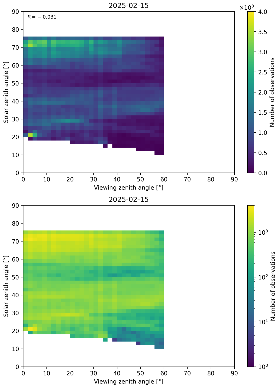
Figure 115: Scatter density plot of “Viewing zenith angle” against “Solar zenith angle” for 2025-02-14 to 2025-02-16.
