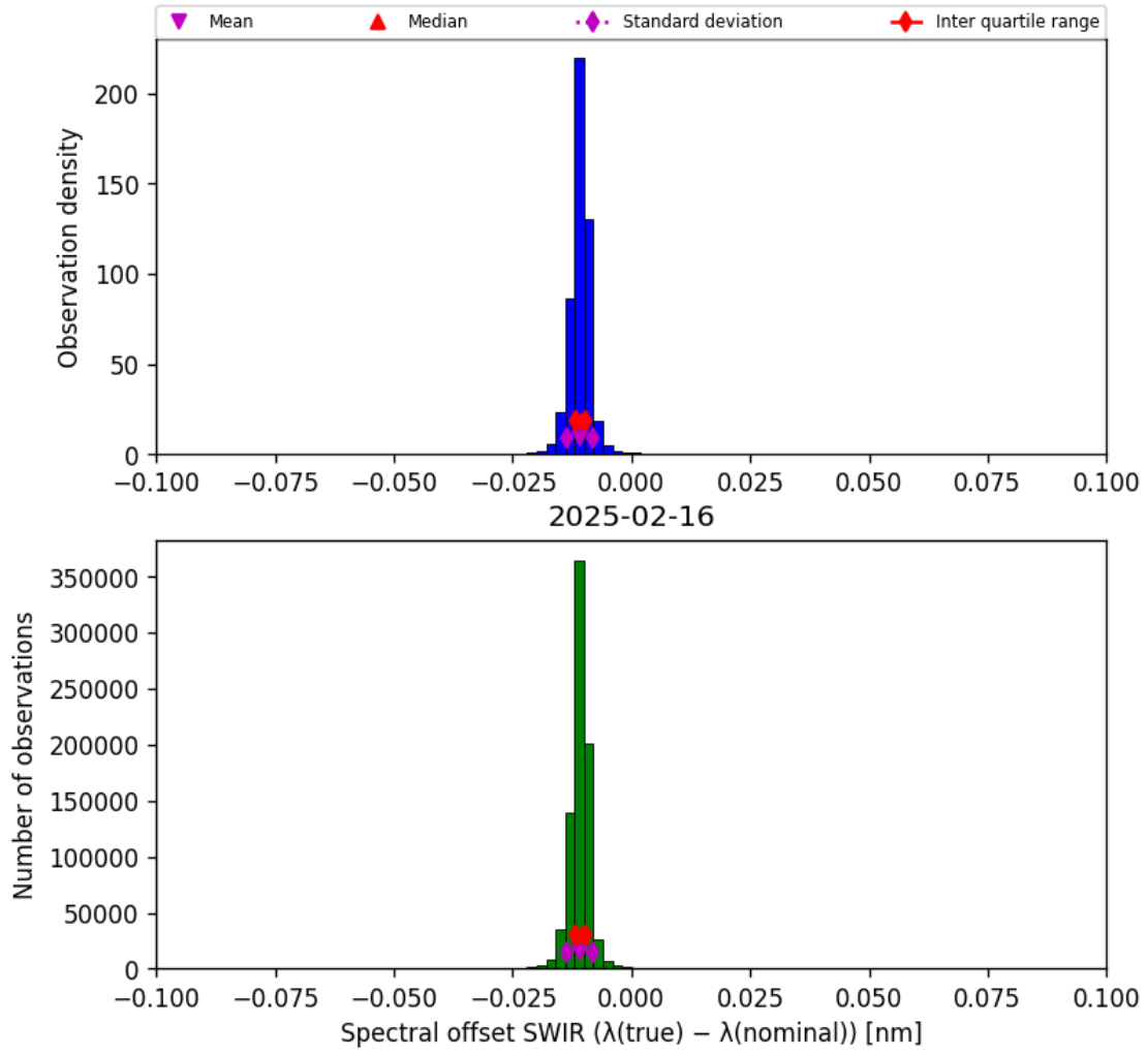
Figure 27: Histogram of “Spectral offset SWIR ( \lambda_{\text{true}} - \lambda_{\text{nominal}} )” for 2025-02-15 to 2025-02-17
