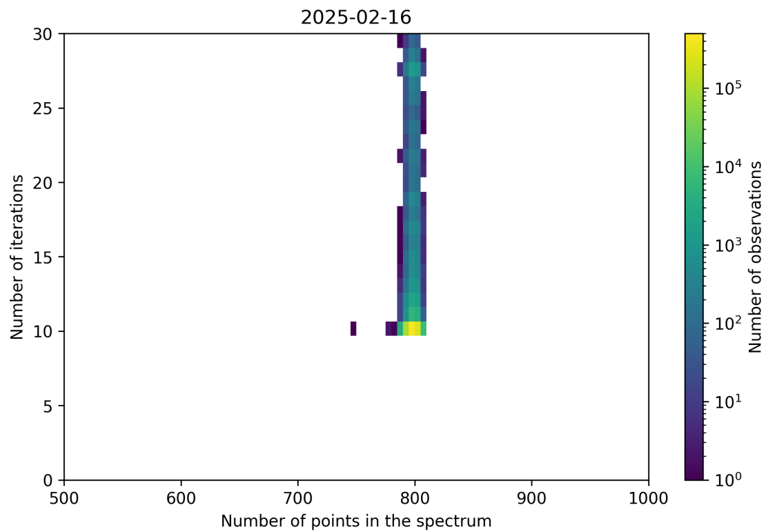
Figure 92: Scatter density plot of “Number of points in the spectrum” against “Number of iterations” for 2025-02-15 to 2025-02-17.
