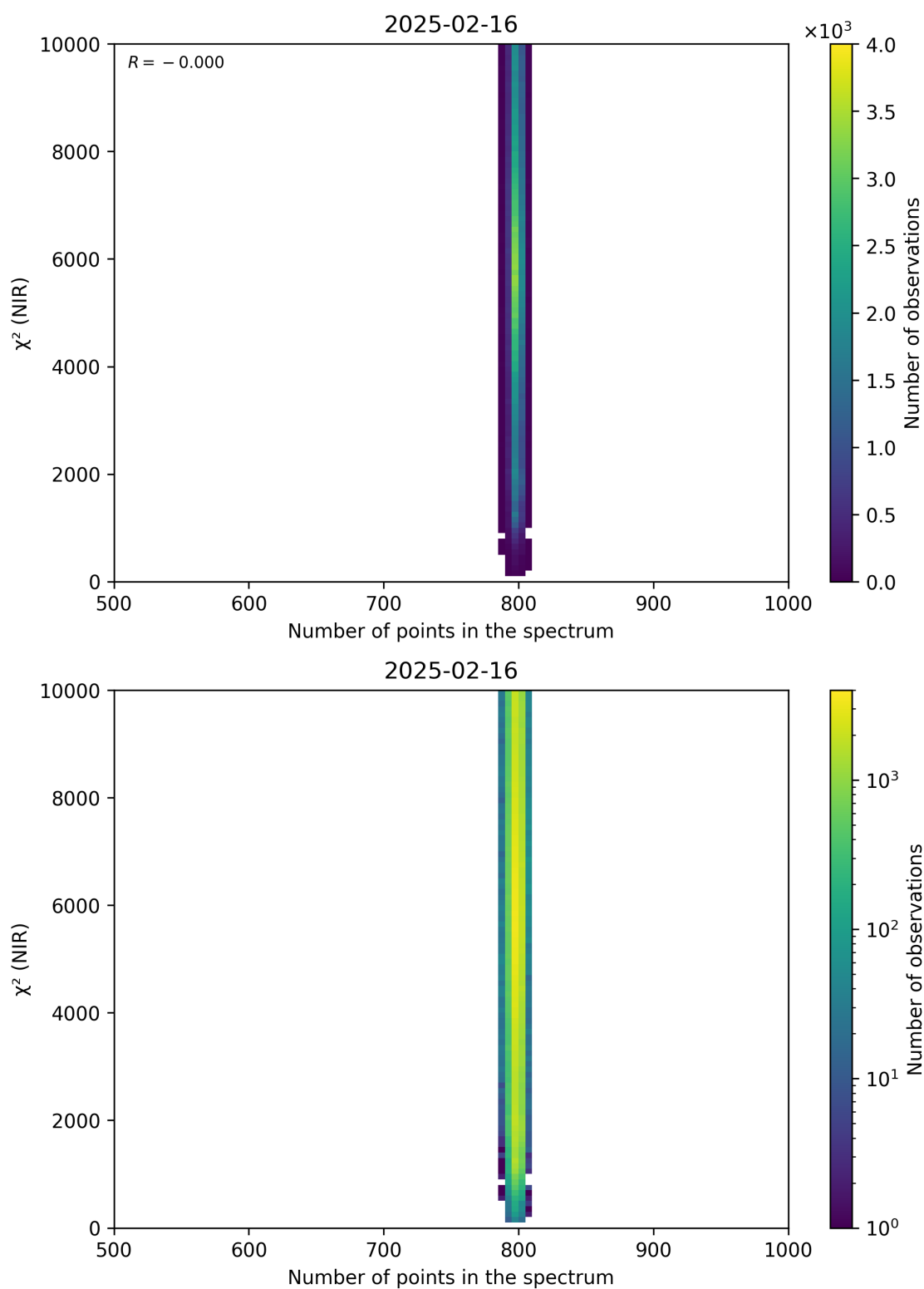
Figure 88: Scatter density plot of “Number of points in the spectrum” against “ \chi^2 (NIR)” for 2025-02-15 to 2025-02-17.
