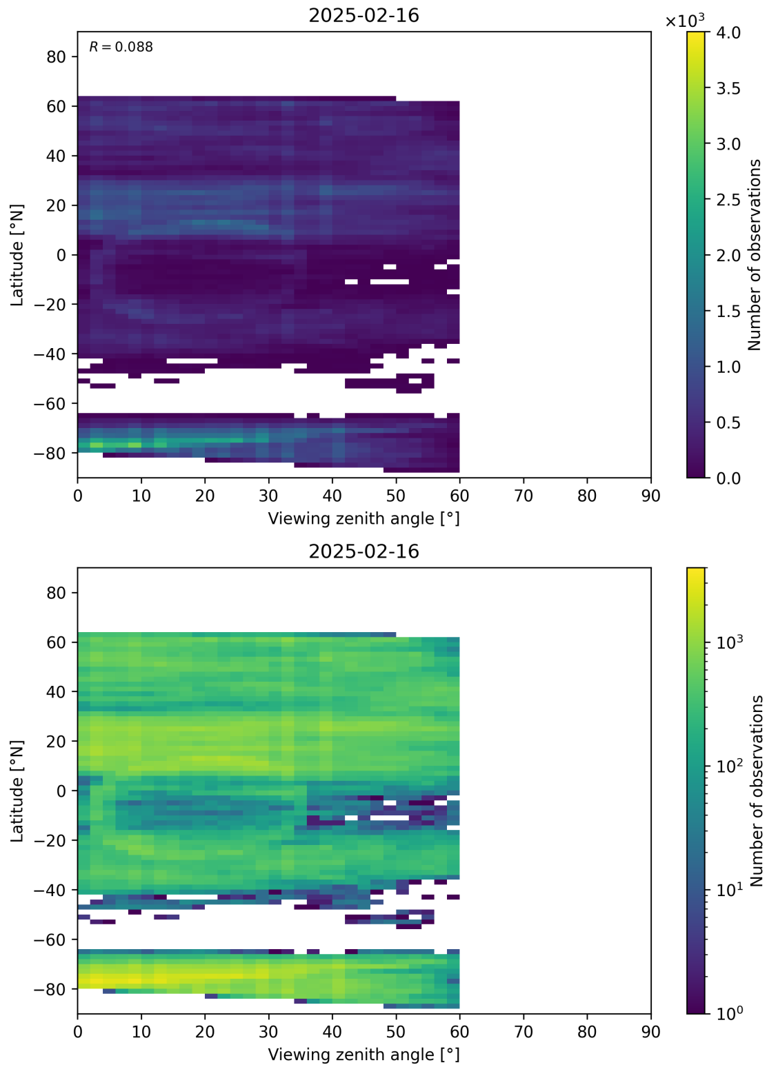
Figure 109: Scatter density plot of “Viewing zenith angle” against “Latitude” for 2025-02-15 to 2025-02-17.
