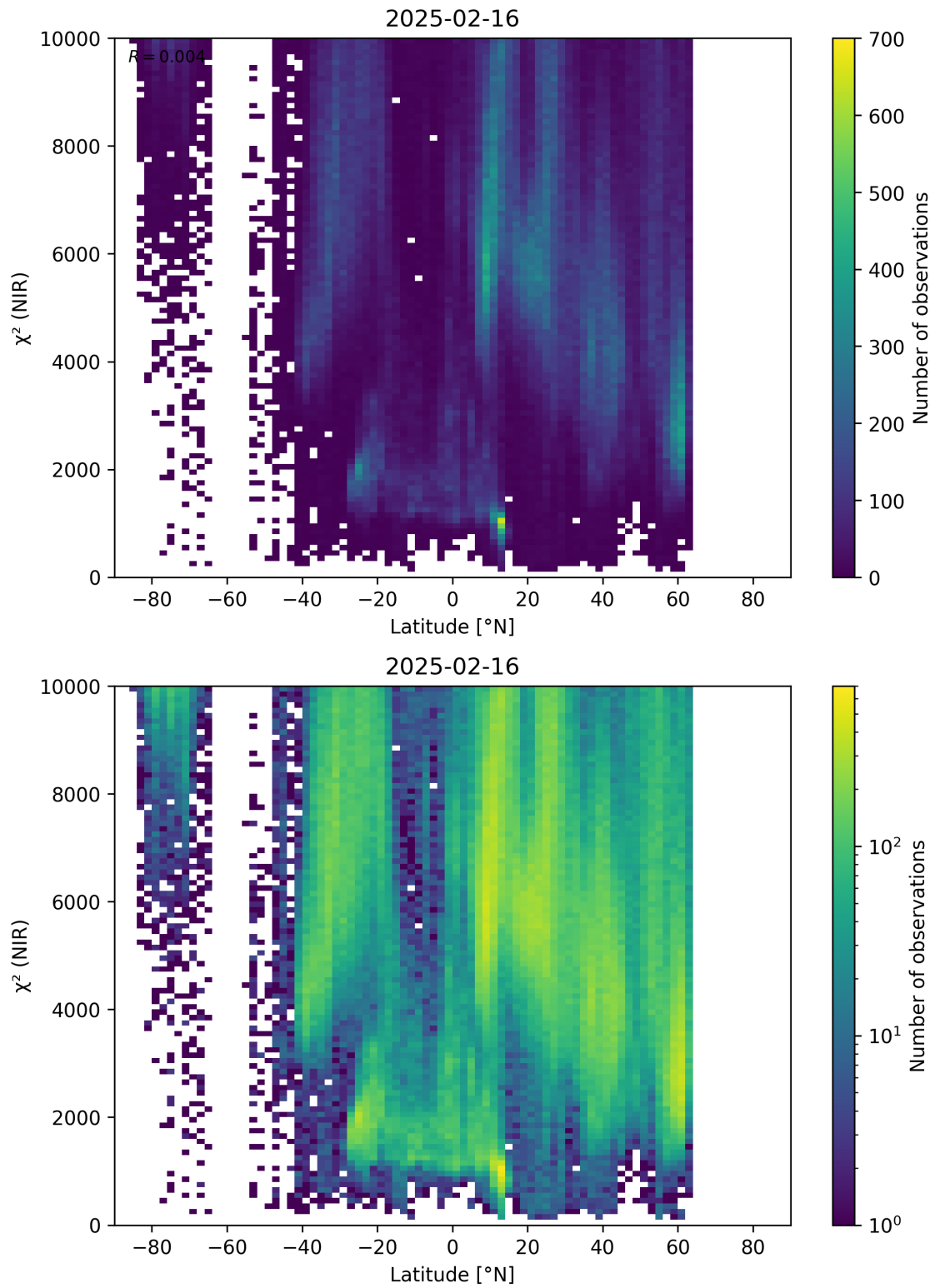
Figure 53: Scatter density plot of “Latitude” against “ \chi^2 (NIR)” for 2025-02-15 to 2025-02-17.
