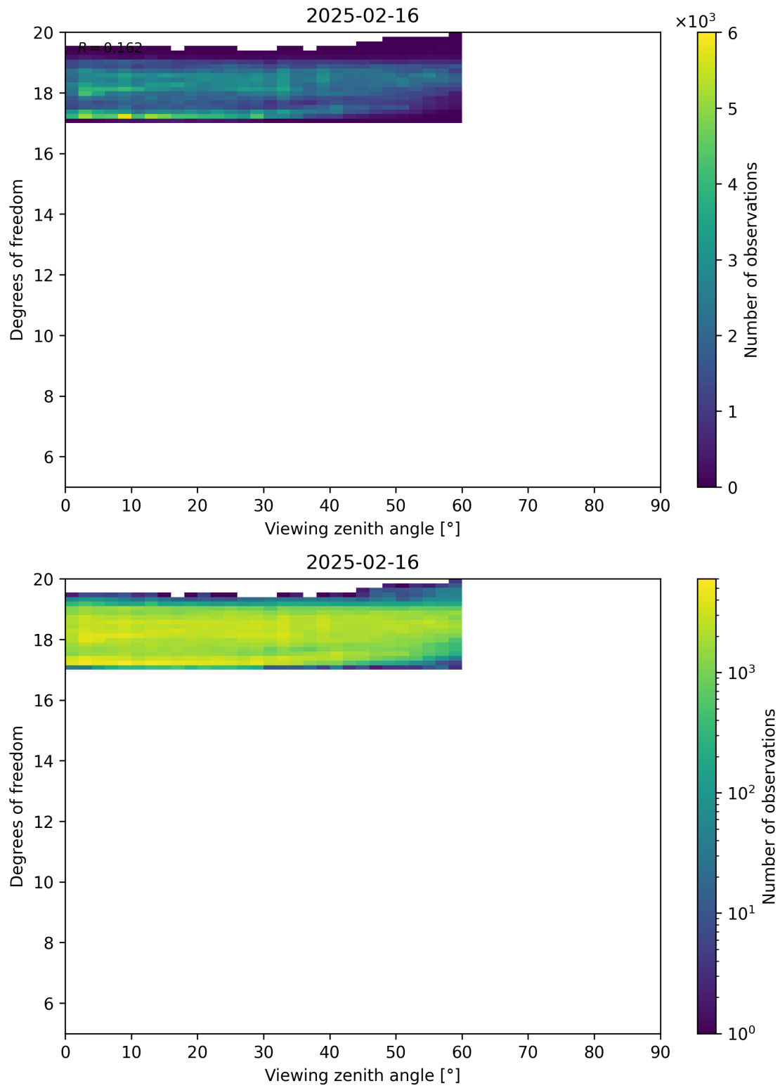
Figure 107: Scatter density plot of “Viewing zenith angle” against “Degrees of freedom” for 2025-02-15 to 2025-02-17.
