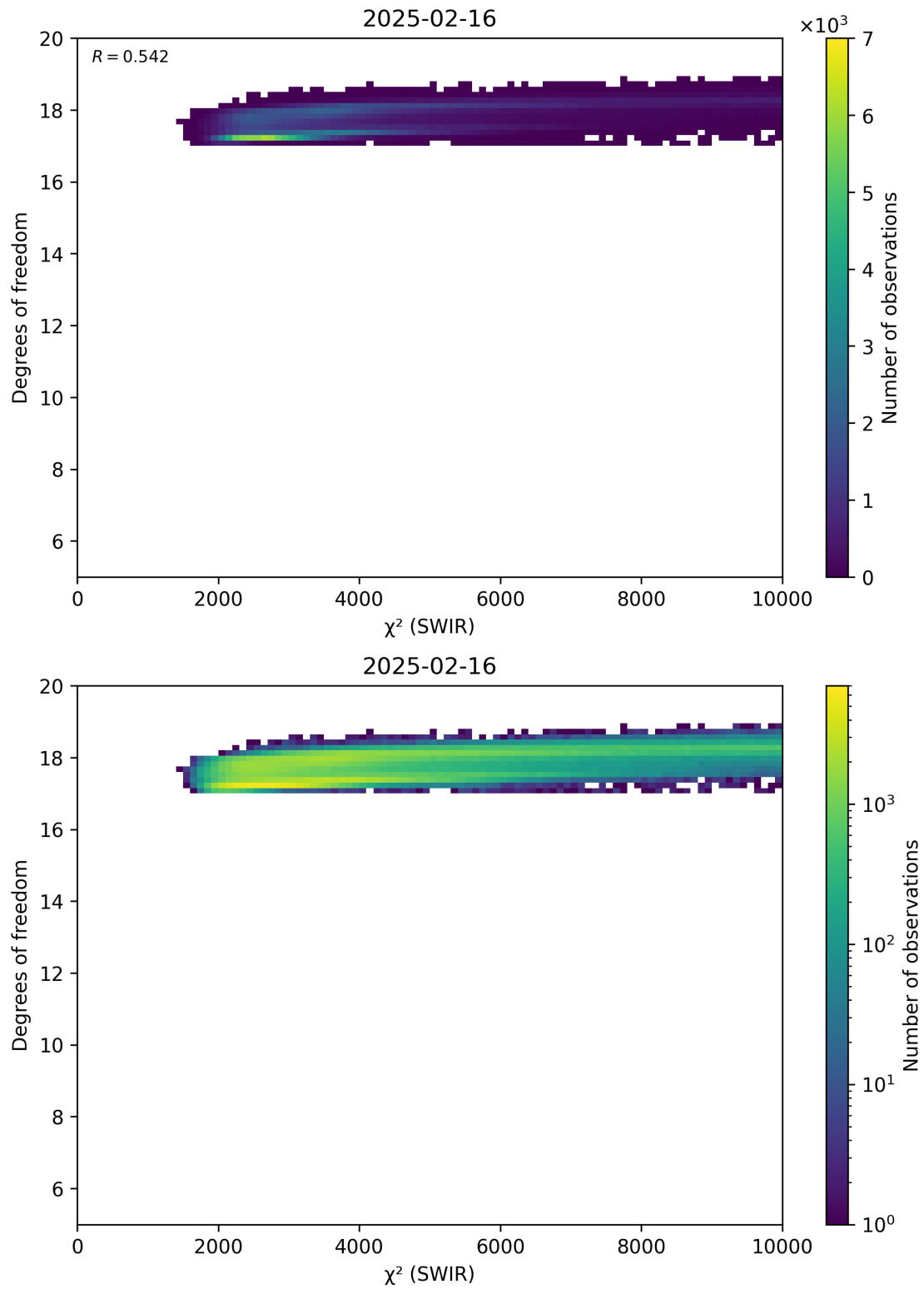
Figure 48: Scatter density plot of “ \chi^2 (SWIR)” against “Degrees of freedom” for 2025-02-15 to 2025-02-17.
