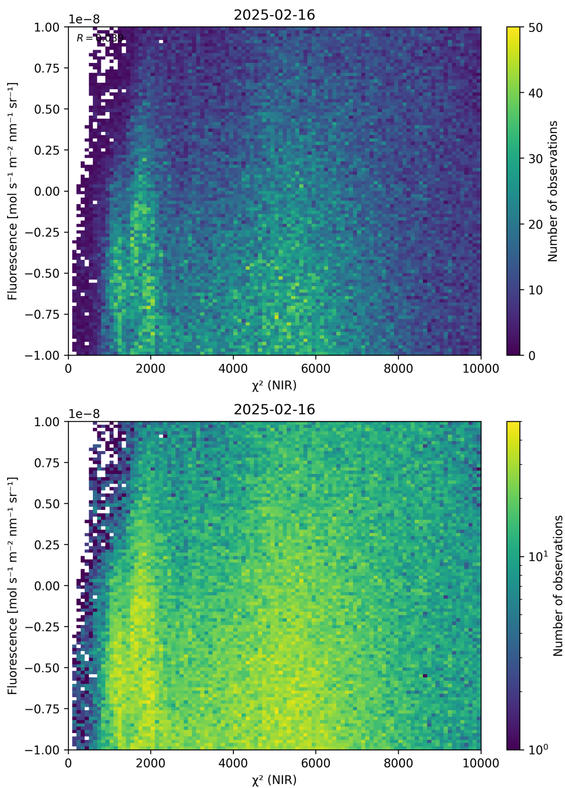
Figure 45: Scatter density plot of “ \chi^2 (NIR)” against “Fluorescence” for 2025-02-15 to 2025-02-17.
