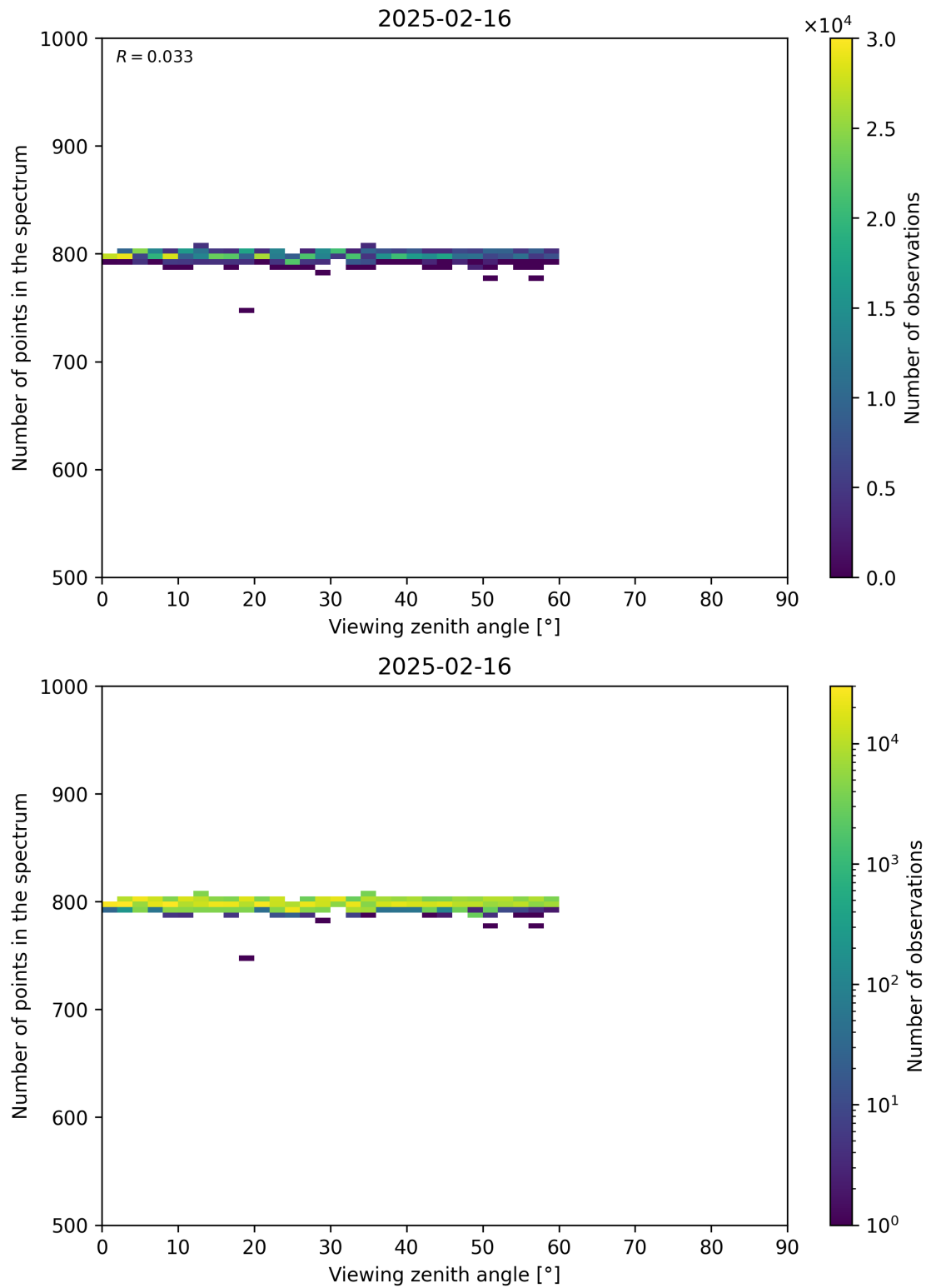
Figure 114: Scatter density plot of “Viewing zenith angle” against “Number of points in the spectrum” for 2025-02-15 to 2025-02-17.
