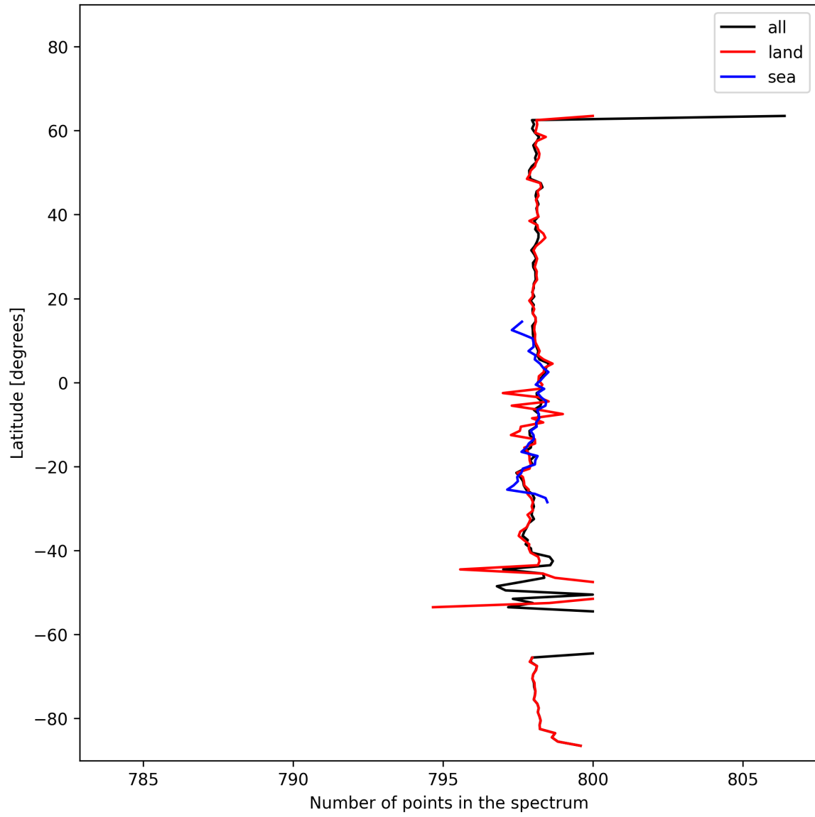
Figure 15: Zonal average of “Number of points in the spectrum” for 2025-02-15 to 2025-02-17.
