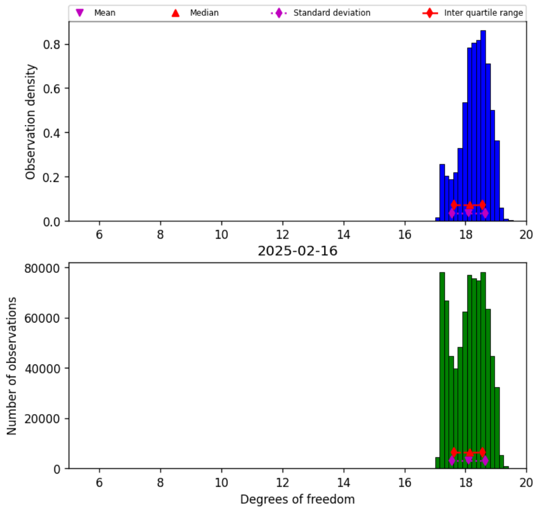
Figure 30: Histogram of “Degrees of freedom” for 2025-02-15 to 2025-02-17
