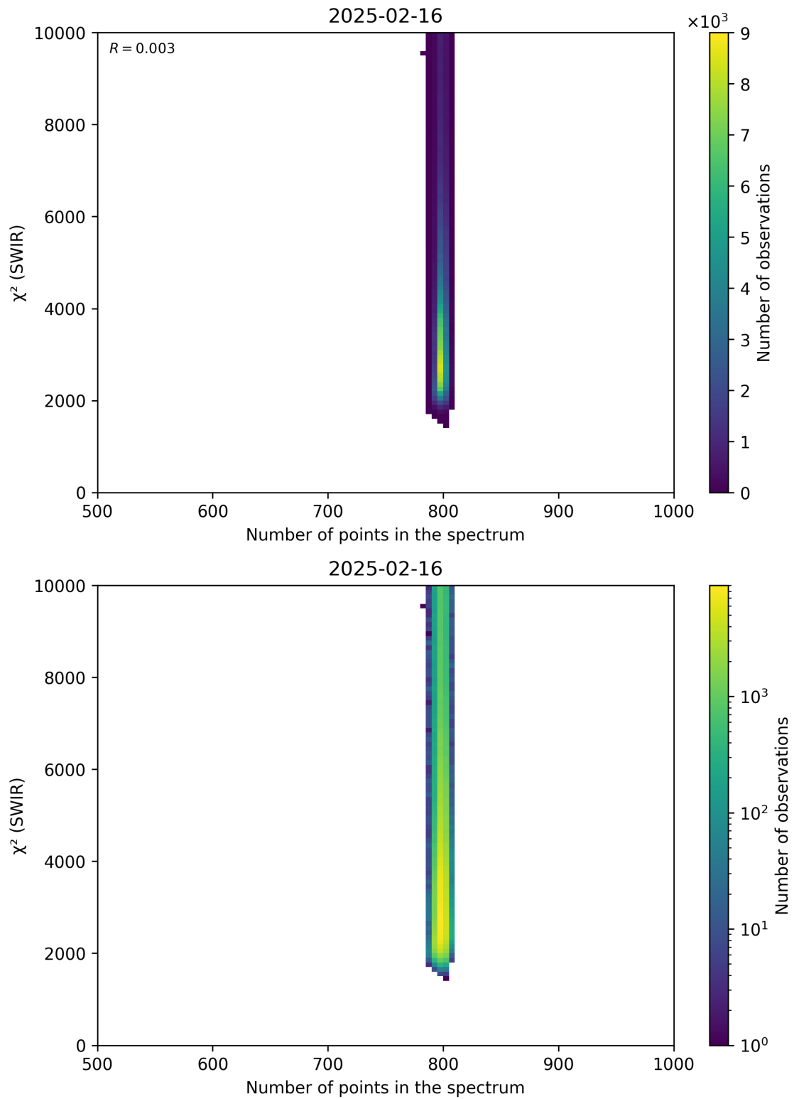
Figure 89: Scatter density plot of “Number of points in the spectrum” against “ \chi^2 (SWIR)” for 2025-02-15 to 2025-02-17.
