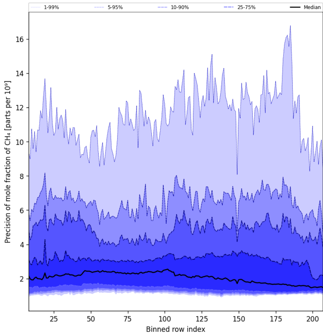
Figure 35: Along track statistics of “Precision of mole fraction of CH 4 ” for 2025-02-15 to 2025-02-17
