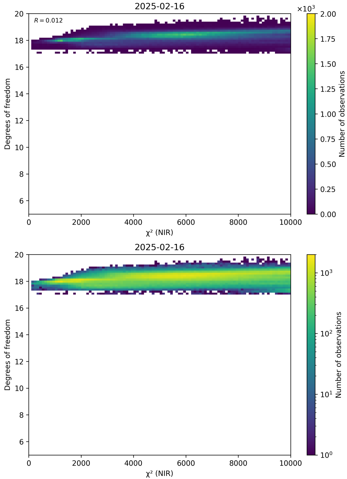
Figure 44: Scatter density plot of “ \chi^2 (NIR)” against “Degrees of freedom” for 2025-02-15 to 2025-02-17.
