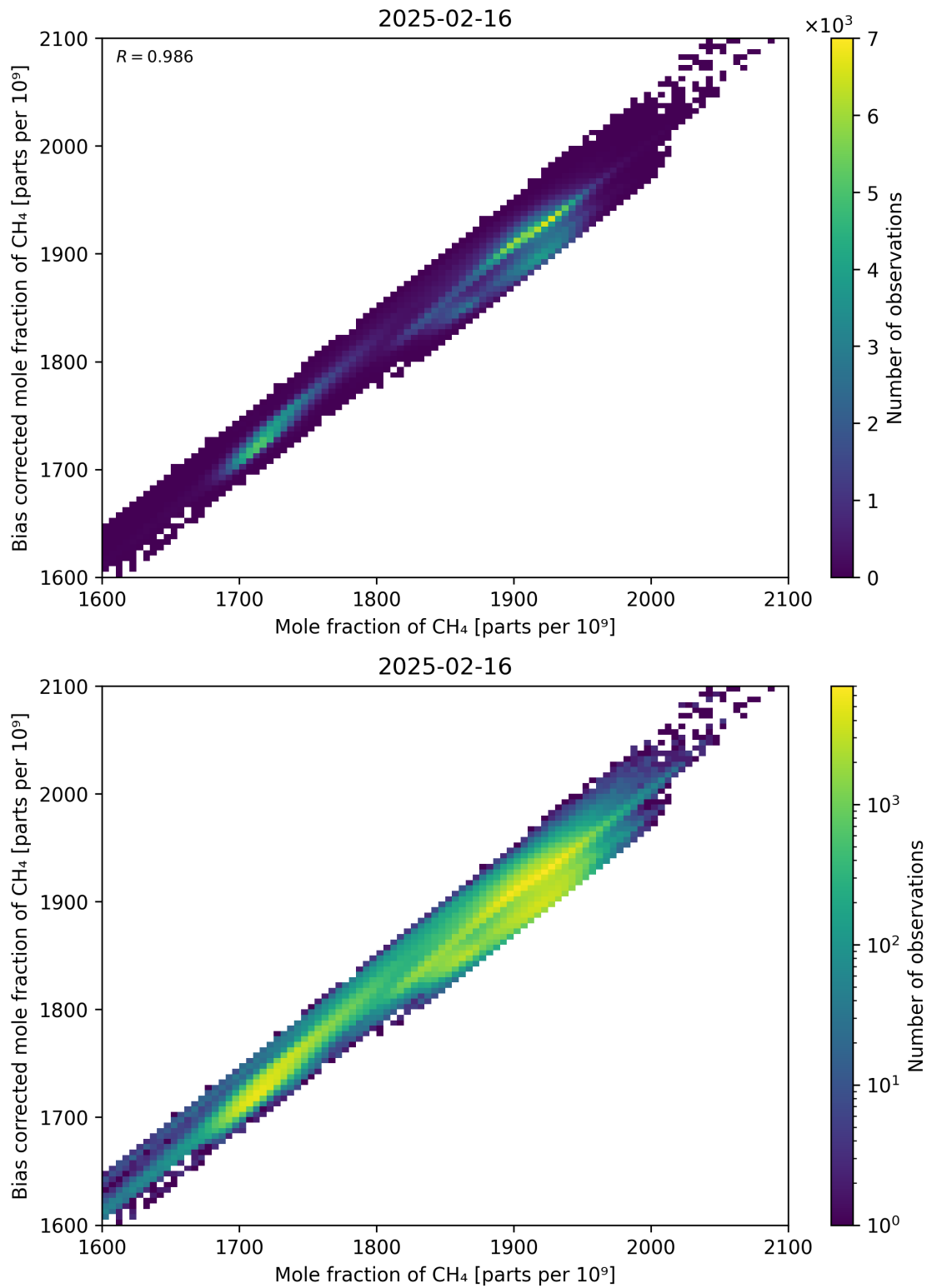
Figure 74: Scatter density plot of “Mole fraction of CH 4 ” against “Bias corrected mole fraction of CH 4 ” for 2025-02-15 to 2025-02-17.
