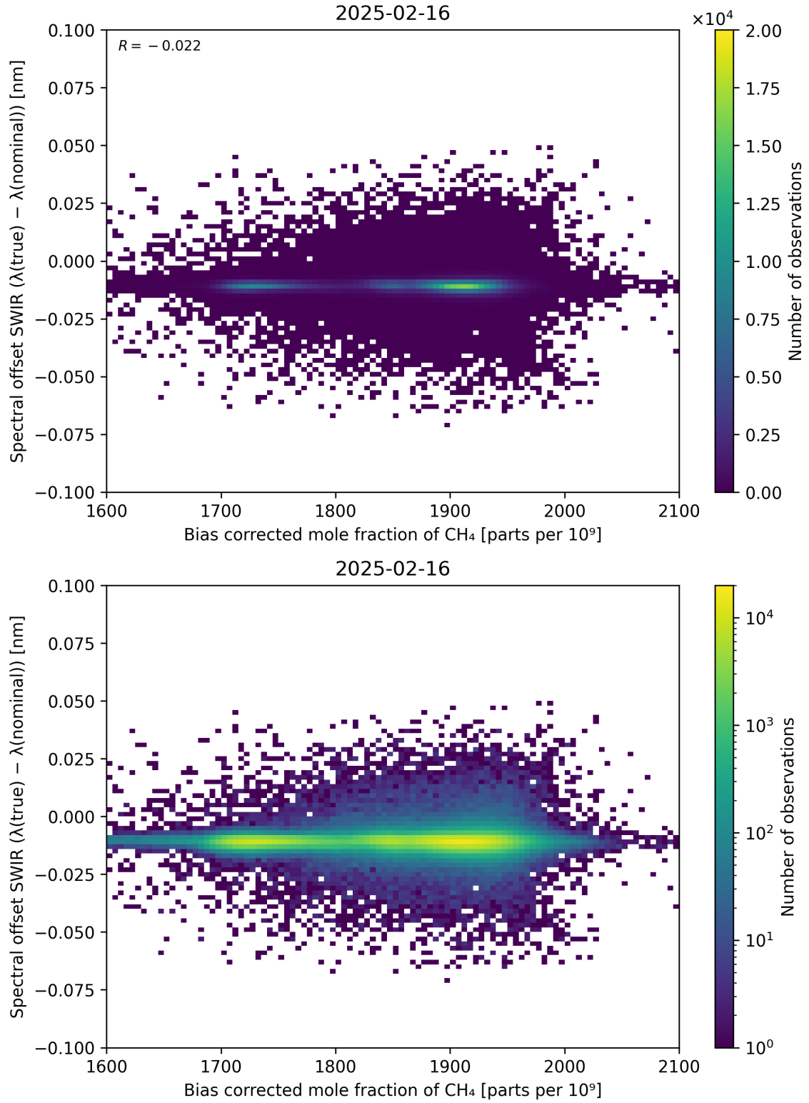
Figure 69: Scatter density plot of “Bias corrected mole fraction of \text{CH}_4 ” against “Spectral offset SWIR ( \lambda_{\text{true}} - \lambda_{\text{nominal}} )” for 2025-02-15 to 2025-02-17.
