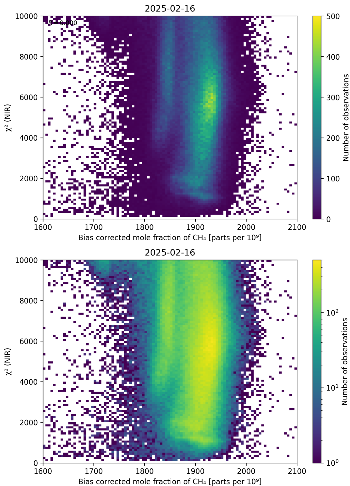
Figure 63: Scatter density plot of “Bias corrected mole fraction of \text{CH}_4 ” against “ \chi^2 (NIR)” for 2025-02-15 to 2025-02-17.
