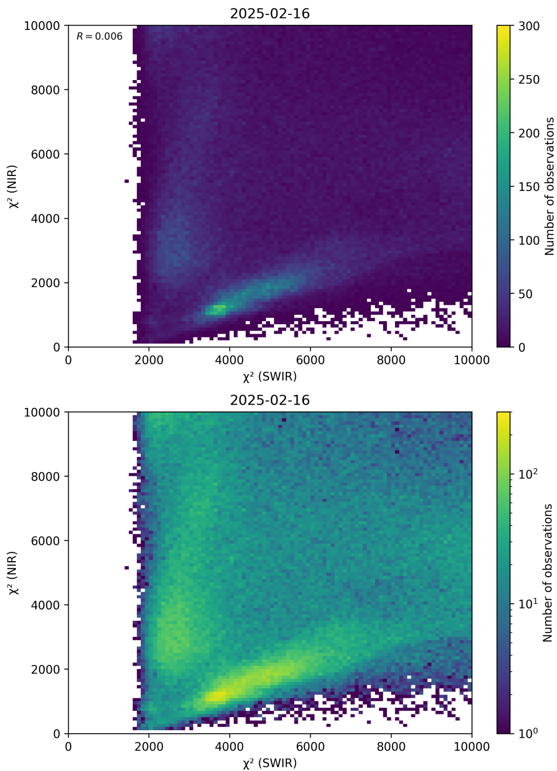
Figure 47: Scatter density plot of “ \chi^2 (SWIR)” against “ \chi^2 (NIR)” for 2025-02-15 to 2025-02-17.
