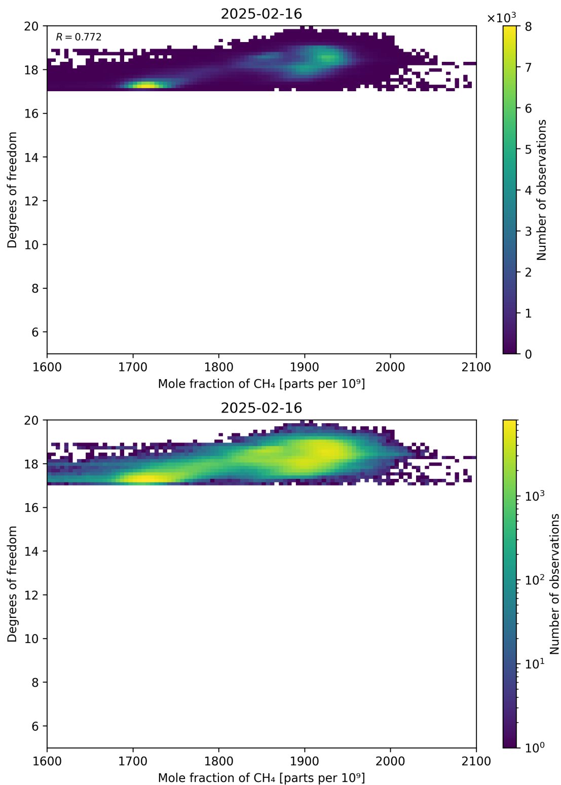
Figure 72: Scatter density plot of “Mole fraction of CH 4 ” against “Degrees of freedom” for 2025-02-15 to 2025-02-17.
