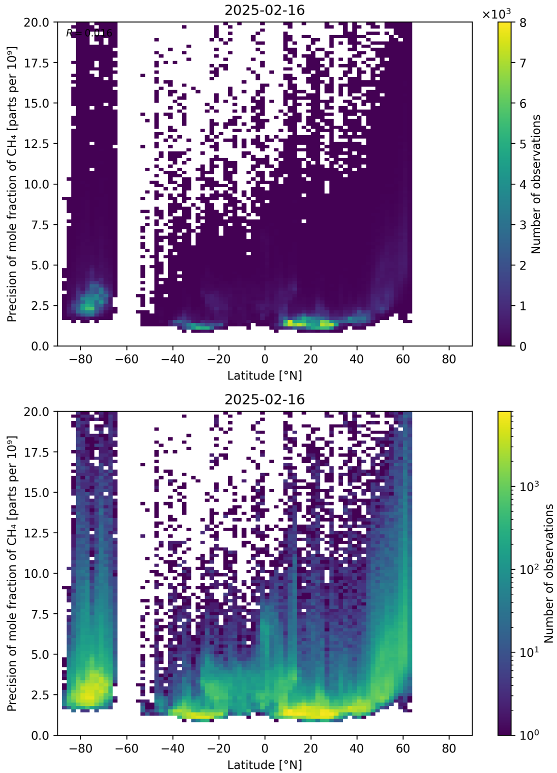
Figure 59: Scatter density plot of “Latitude” against “Precision of mole fraction of CH 4 ” for 2025-02-15 to 2025-02-17.
