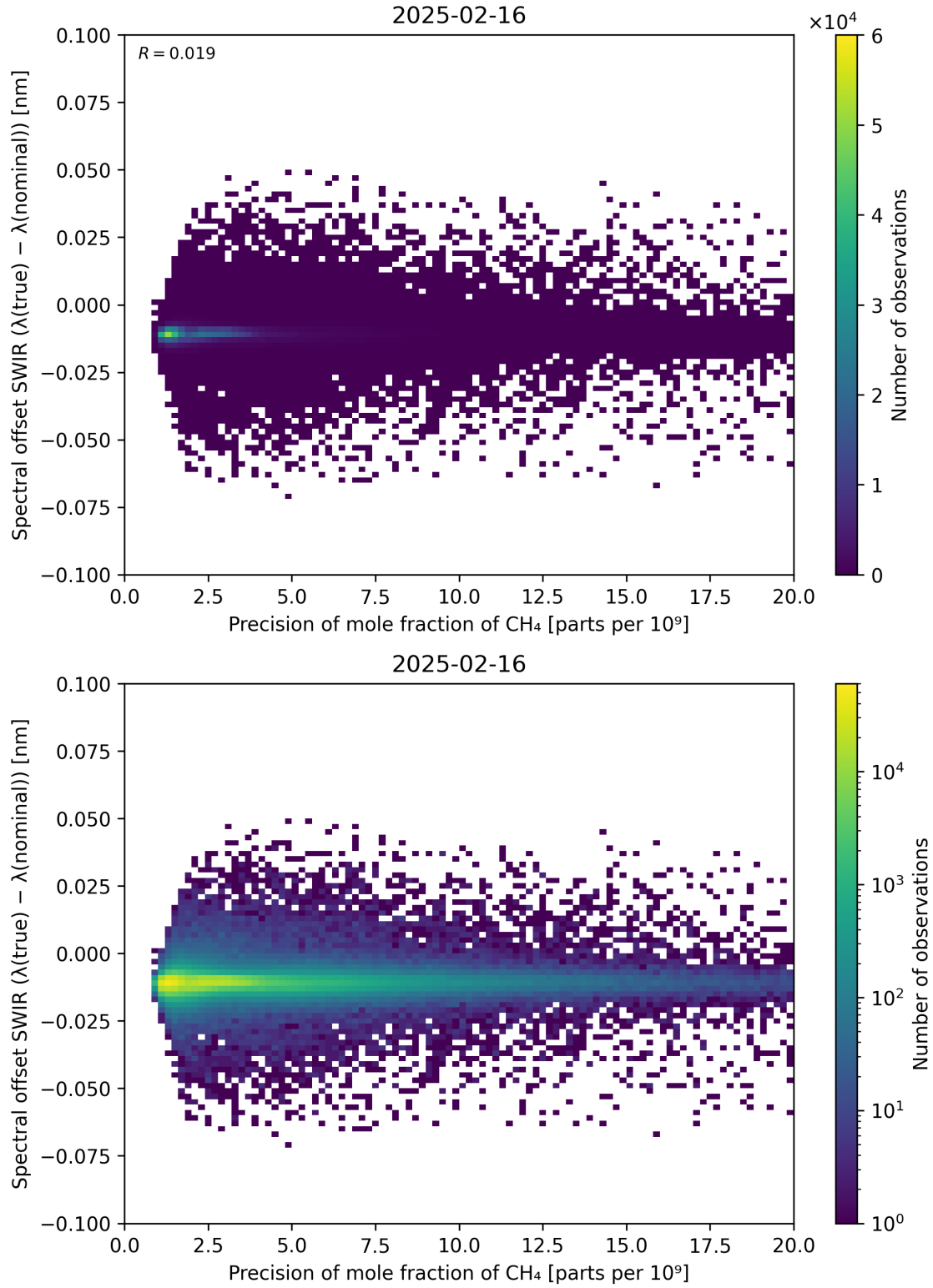
Figure 85: Scatter density plot of “Precision of mole fraction of CH 4 ” against “Spectral offset SWIR ( \lambda_{\text{true}} - \lambda_{\text{nominal}} )” for 2025-02-15 to 2025-02-17.
