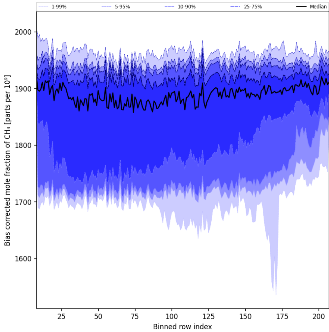
Figure 36: Along track statistics of “Bias corrected mole fraction of CH 4 ” for 2025-02-15 to 2025-02-17
