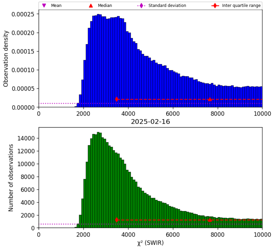
Figure 28: Histogram of “ \chi^2 (SWIR)” for 2025-02-15 to 2025-02-17
