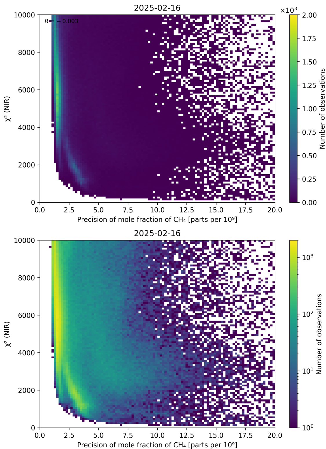
Figure 78: Scatter density plot of “Precision of mole fraction of CH 4 ” against “ \chi^2 (NIR)” for 2025-02-15 to 2025-02-17.
