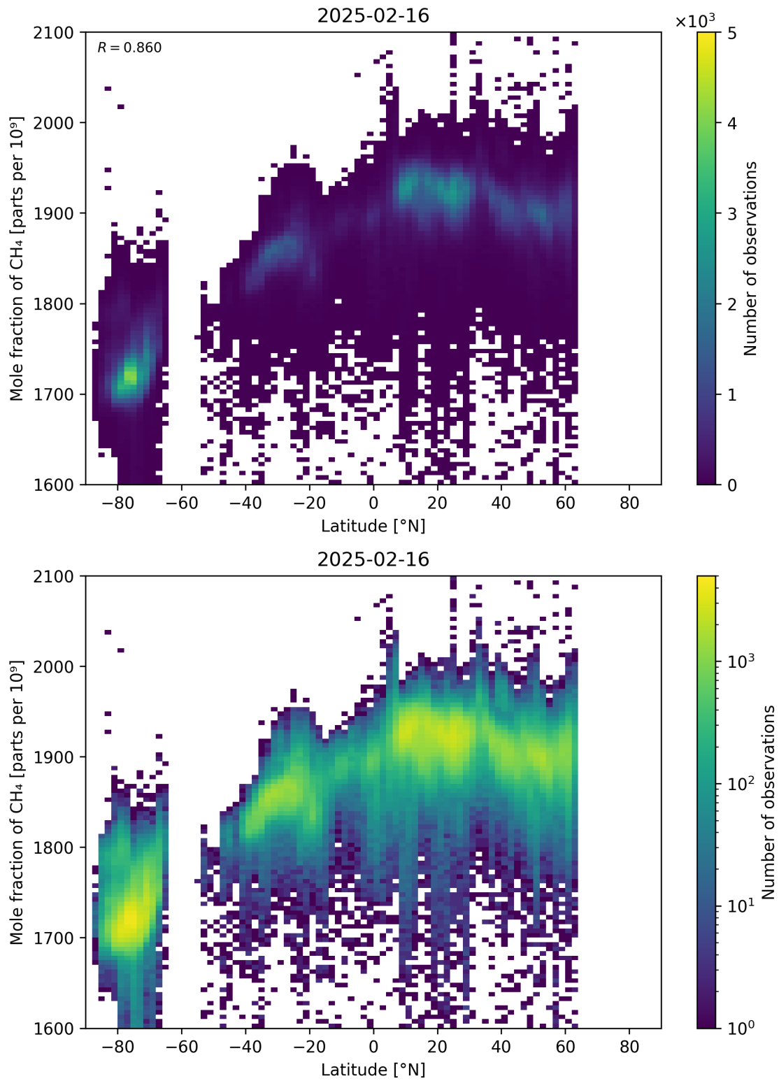
Figure 57: Scatter density plot of “Latitude” against “Mole fraction of CH 4 ” for 2025-02-15 to 2025-02-17.
