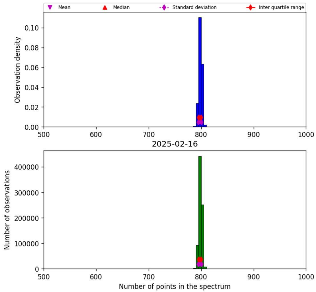
Figure 26: Histogram of “Number of points in the spectrum” for 2025-02-15 to 2025-02-17
