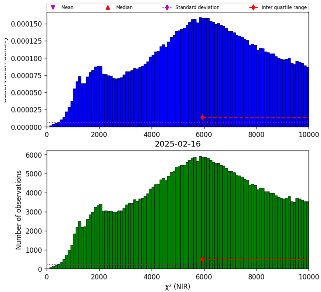
Figure 29: Histogram of “ \chi^2 (NIR)” for 2025-02-15 to 2025-02-17
