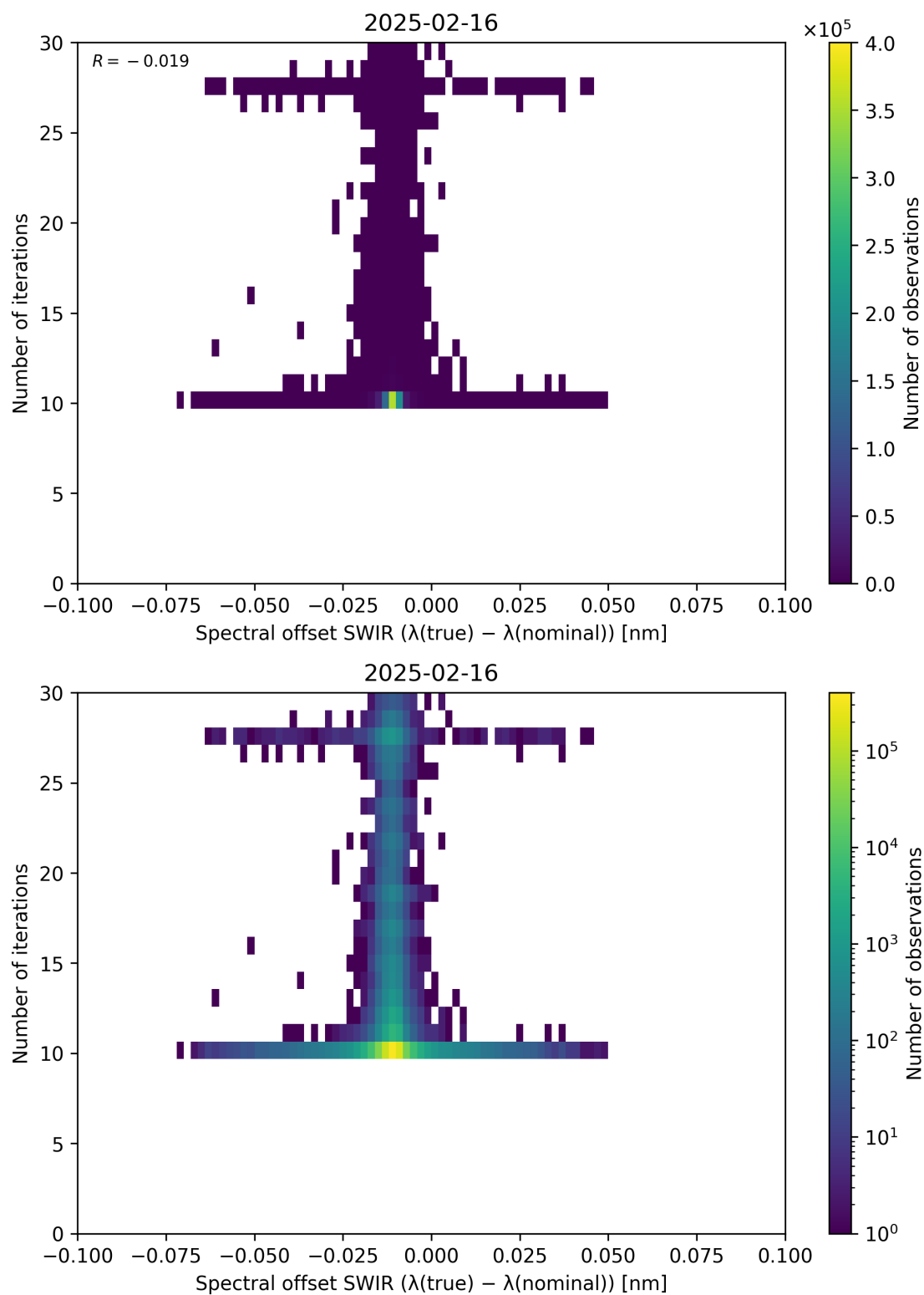
Figure 121: Scatter density plot of “Spectral offset SWIR ( \lambda_{\text{true}} - \lambda_{\text{nominal}} )” against “Number of iterations” for 2025-02-15 to 2025-02-17.
