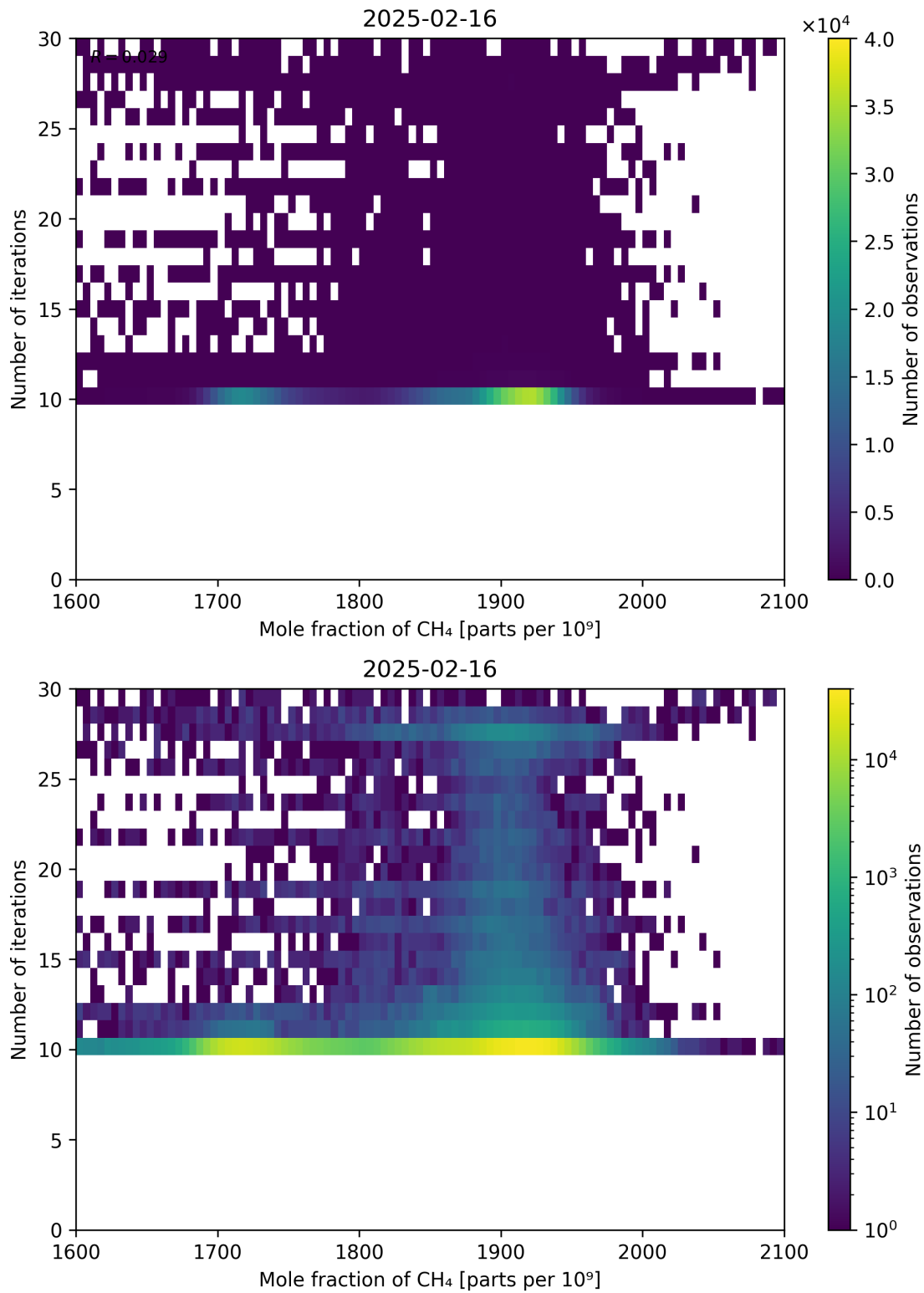
Figure 76: Scatter density plot of “Mole fraction of CH 4 ” against “Number of iterations” for 2025-02-15 to 2025-02-17.
