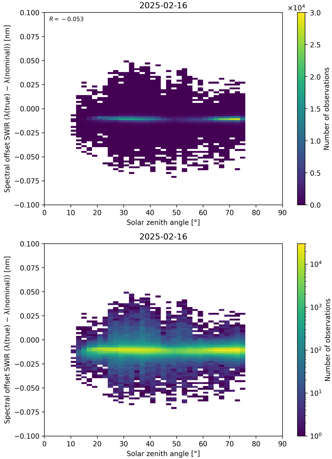
Figure 104: Scatter density plot of “Solar zenith angle” against “Spectral offset SWIR ( \lambda_{\text{true}} - \lambda_{\text{nominal}} )” for 2025-02-15 to 2025-02-17.
