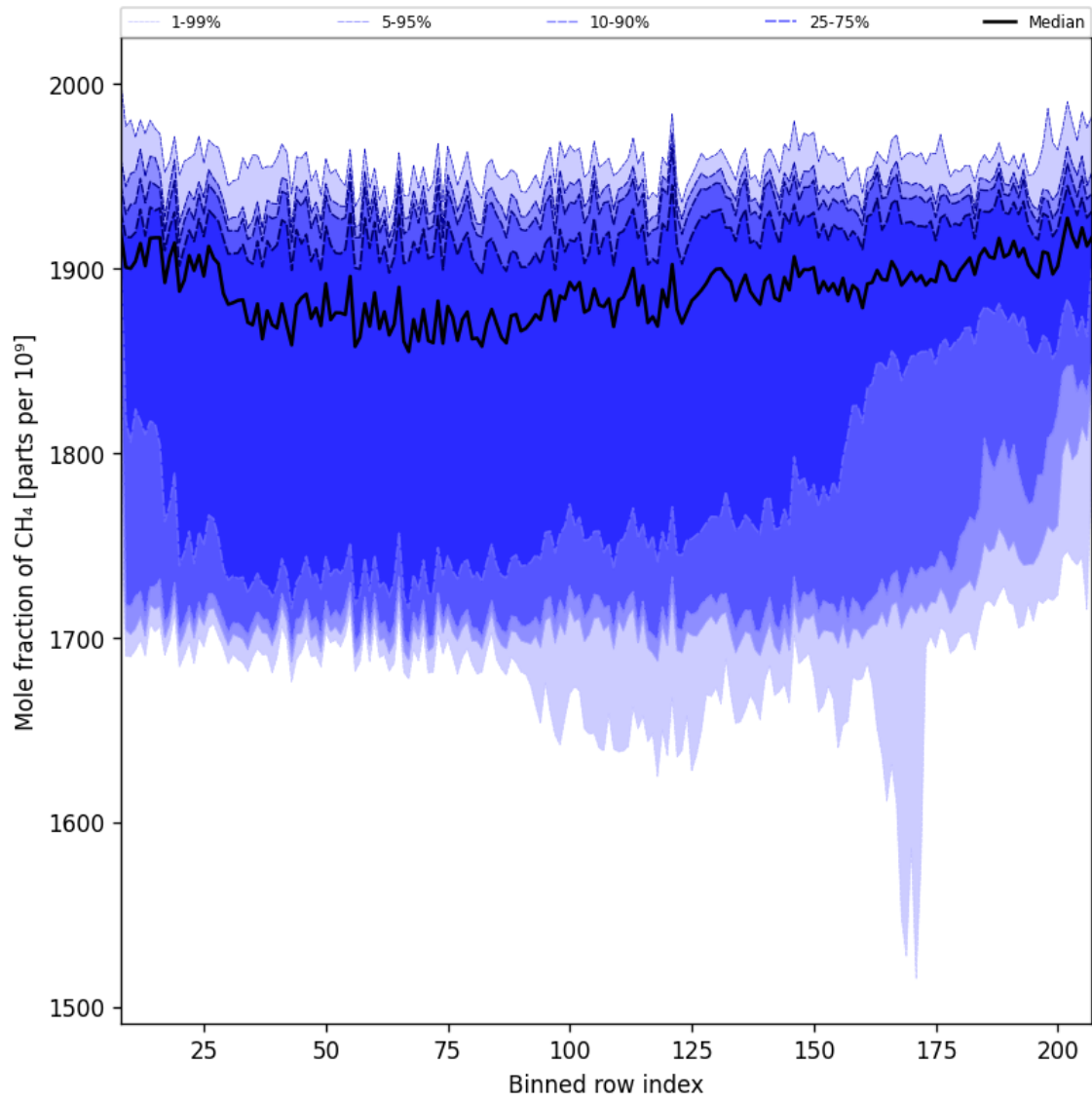
Figure 34: Along track statistics of “Mole fraction of CH 4 ” for 2025-02-15 to 2025-02-17
