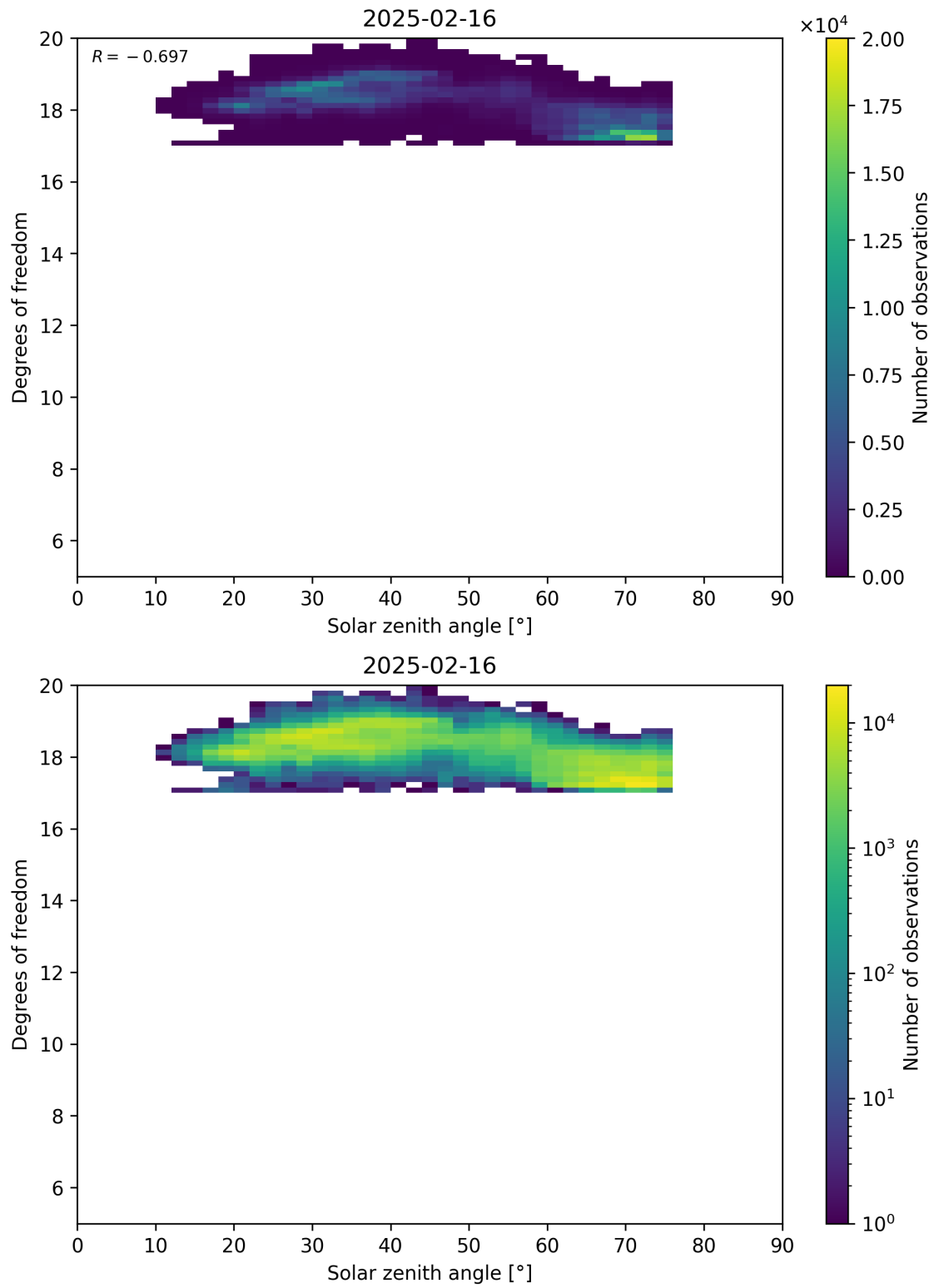
Figure 96: Scatter density plot of “Solar zenith angle” against “Degrees of freedom” for 2025-02-15 to 2025-02-17.
