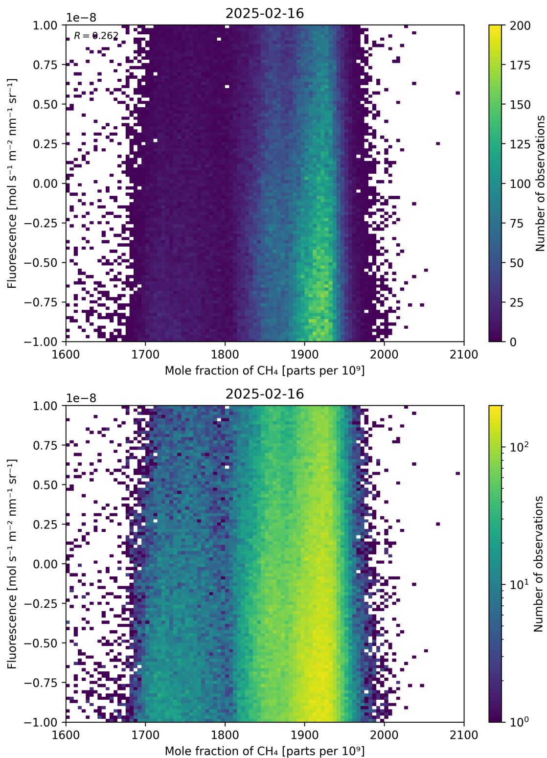
Figure 73: Scatter density plot of “Mole fraction of \text{CH}_4 ” against “Fluorescence” for 2025-02-15 to 2025-02-17.
