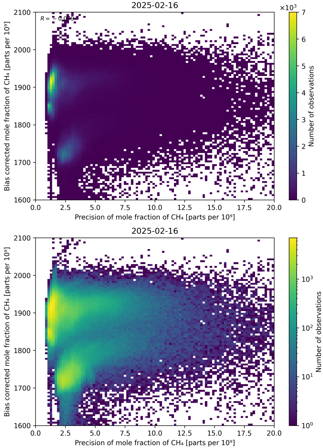
Figure 82: Scatter density plot of “Precision of mole fraction of CH 4 ” against “Bias corrected mole fraction of CH 4 ” for 2025-02-15 to 2025-02-17.
