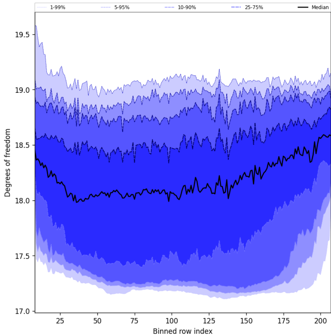
Figure 41: Along track statistics of “Degrees of freedom” for 2025-02-15 to 2025-02-17
