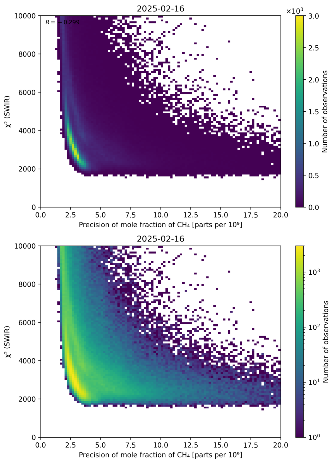
Figure 79: Scatter density plot of “Precision of mole fraction of \text{CH}_4 ” against “ \chi^2 (SWIR)” for 2025-02-15 to 2025-02-17.
