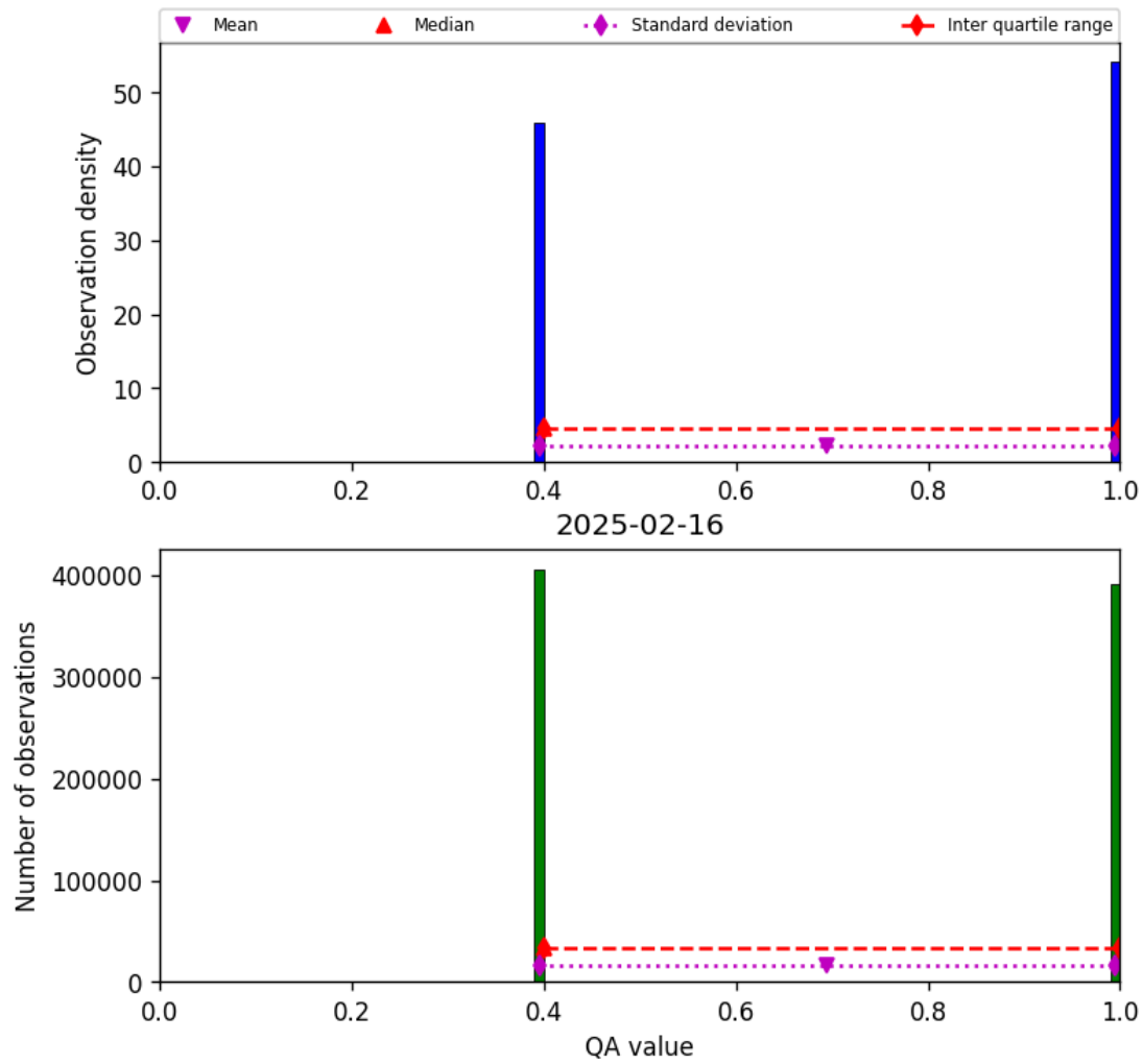
Figure 22: Histogram of “QA value” for 2025-02-15 to 2025-02-17
