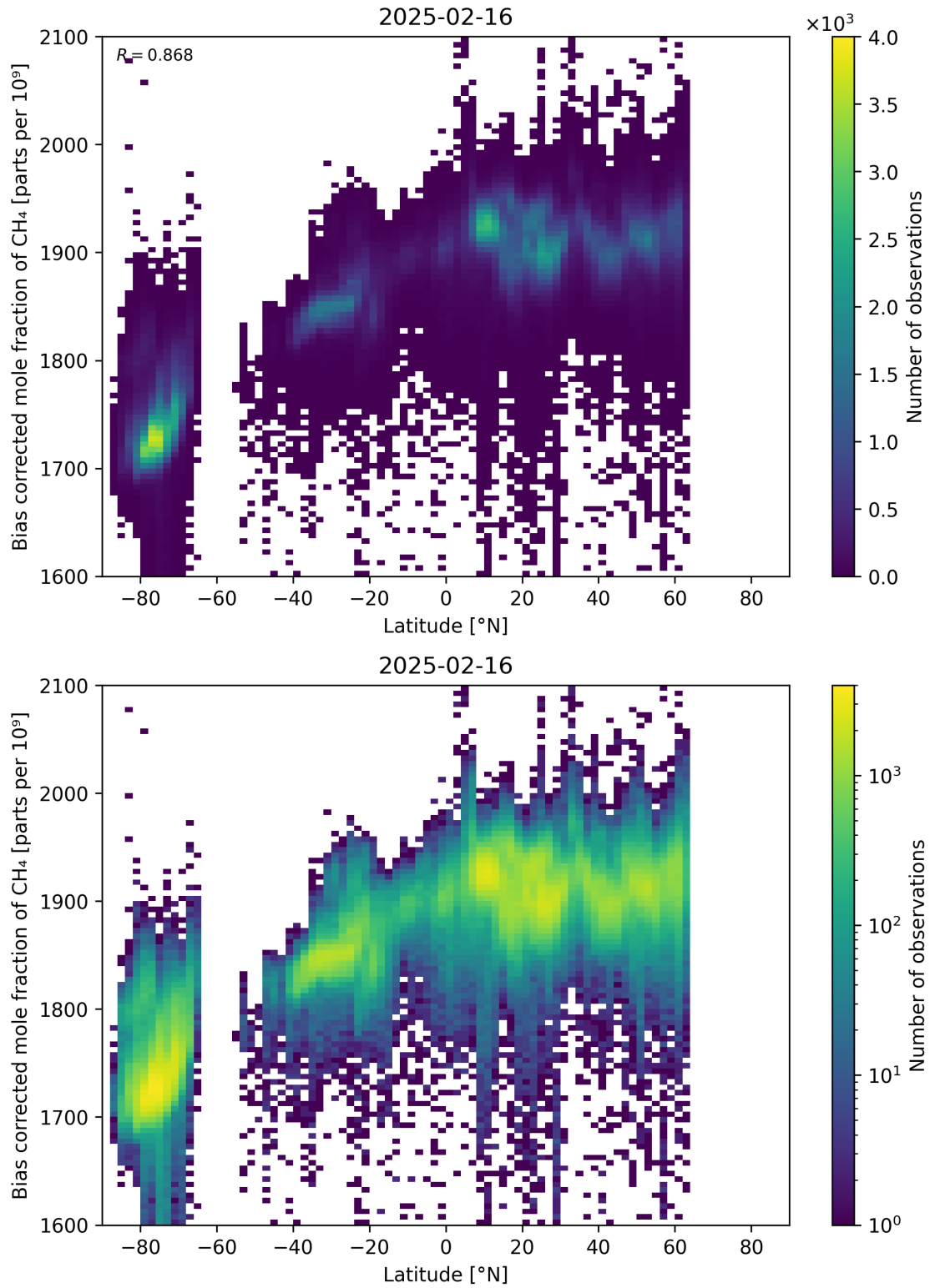
Figure 58: Scatter density plot of “Latitude” against “Bias corrected mole fraction of CH 4 ” for 2025-02-15 to 2025-02-17.
