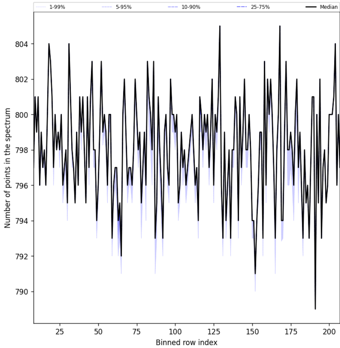
Figure 37: Along track statistics of “Number of points in the spectrum” for 2025-02-15 to 2025-02-17
