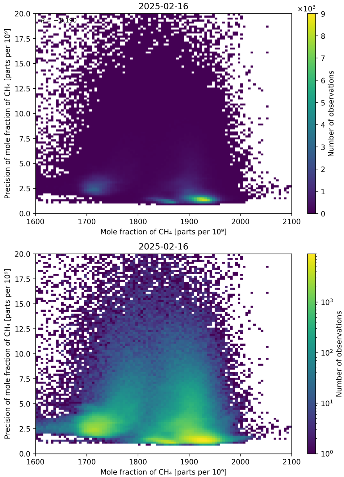
Figure 75: Scatter density plot of “Mole fraction of CH 4 ” against “Precision of mole fraction of CH 4 ” for 2025-02-15 to 2025-02-17.
