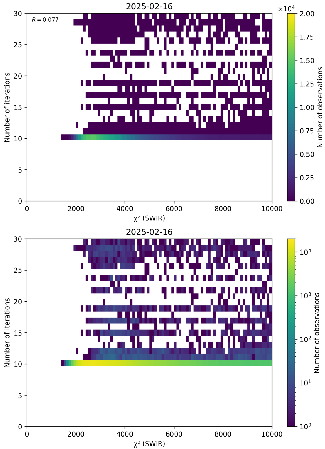
Figure 50: Scatter density plot of “ \chi^2 (SWIR)” against “Number of iterations” for 2025-02-15 to 2025-02-17.
