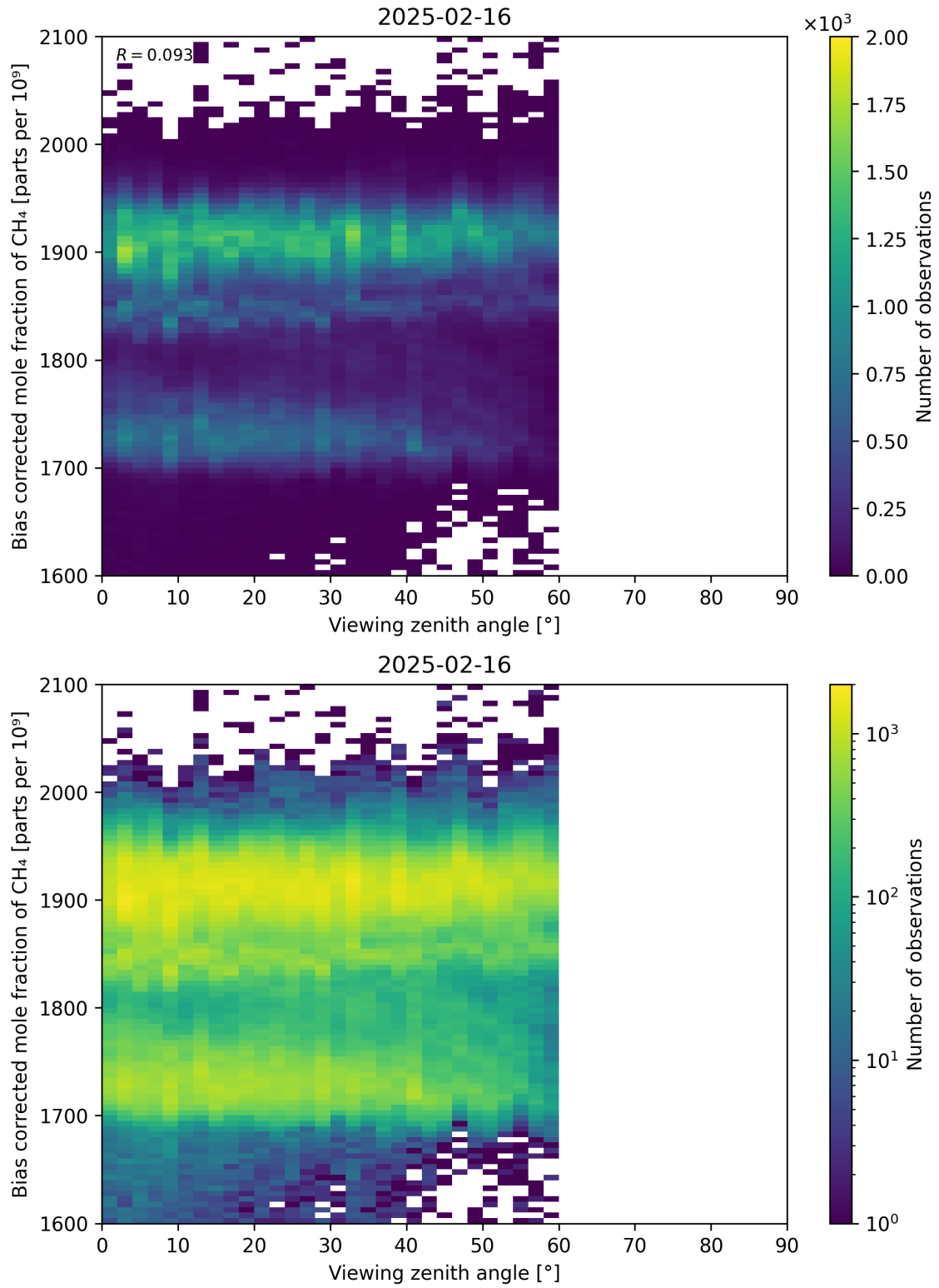
Figure 111: Scatter density plot of “Viewing zenith angle” against “Bias corrected mole fraction of CH 4 ” for 2025-02-15 to 2025-02-17.
