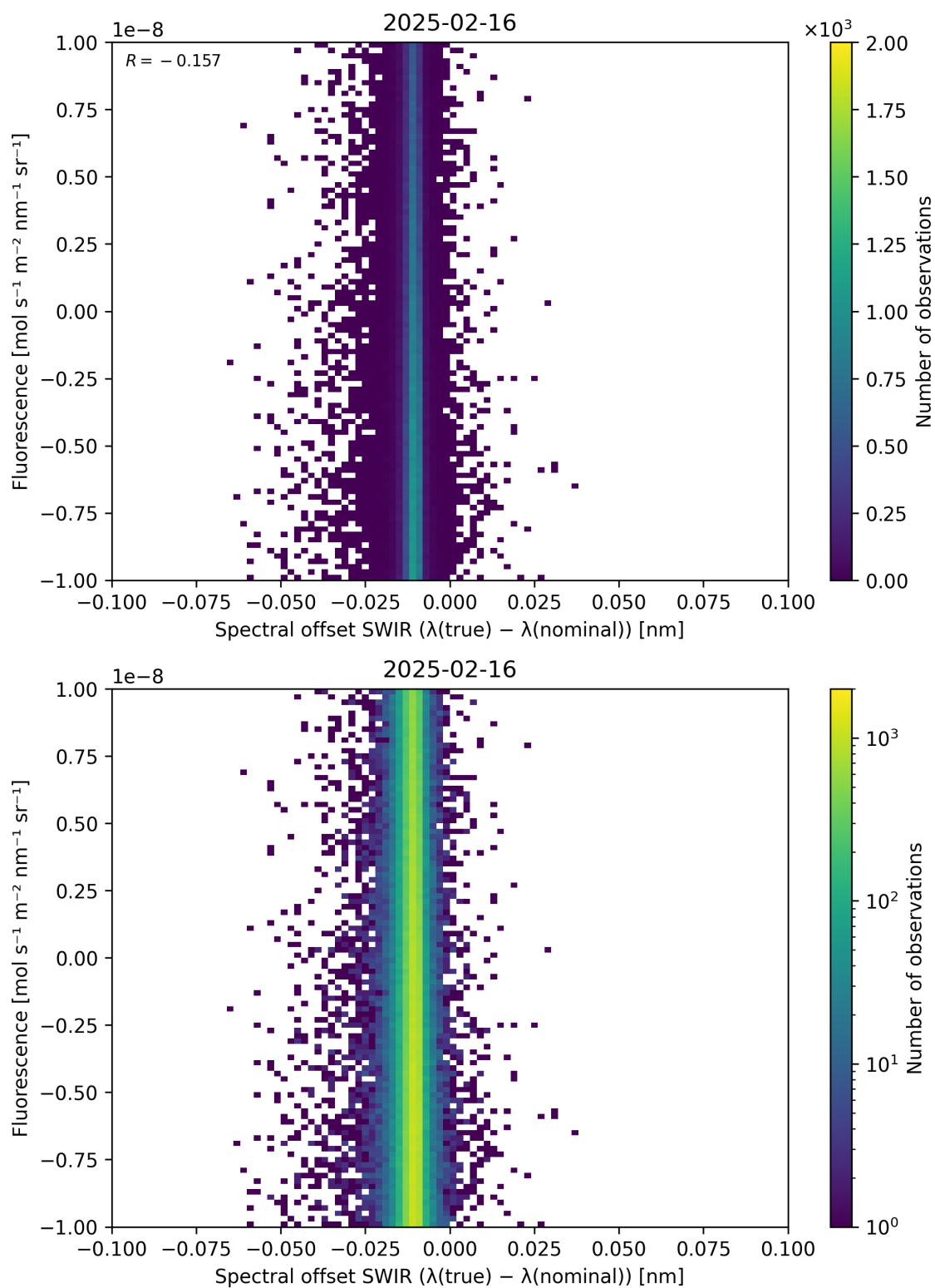
Figure 120: Scatter density plot of “Spectral offset SWIR ( \lambda_{\text{true}} - \lambda_{\text{nominal}} )” against “Fluorescence” for 2025-02-15 to 2025-02-17.
