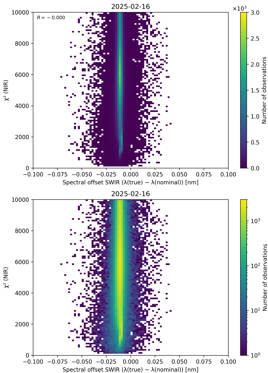
Figure 117: Scatter density plot of “Spectral offset SWIR ( \lambda_{\text{true}} - \lambda_{\text{nominal}} )” against “ \chi^2 (NIR)” for 2025-02-15 to 2025-02-17.
