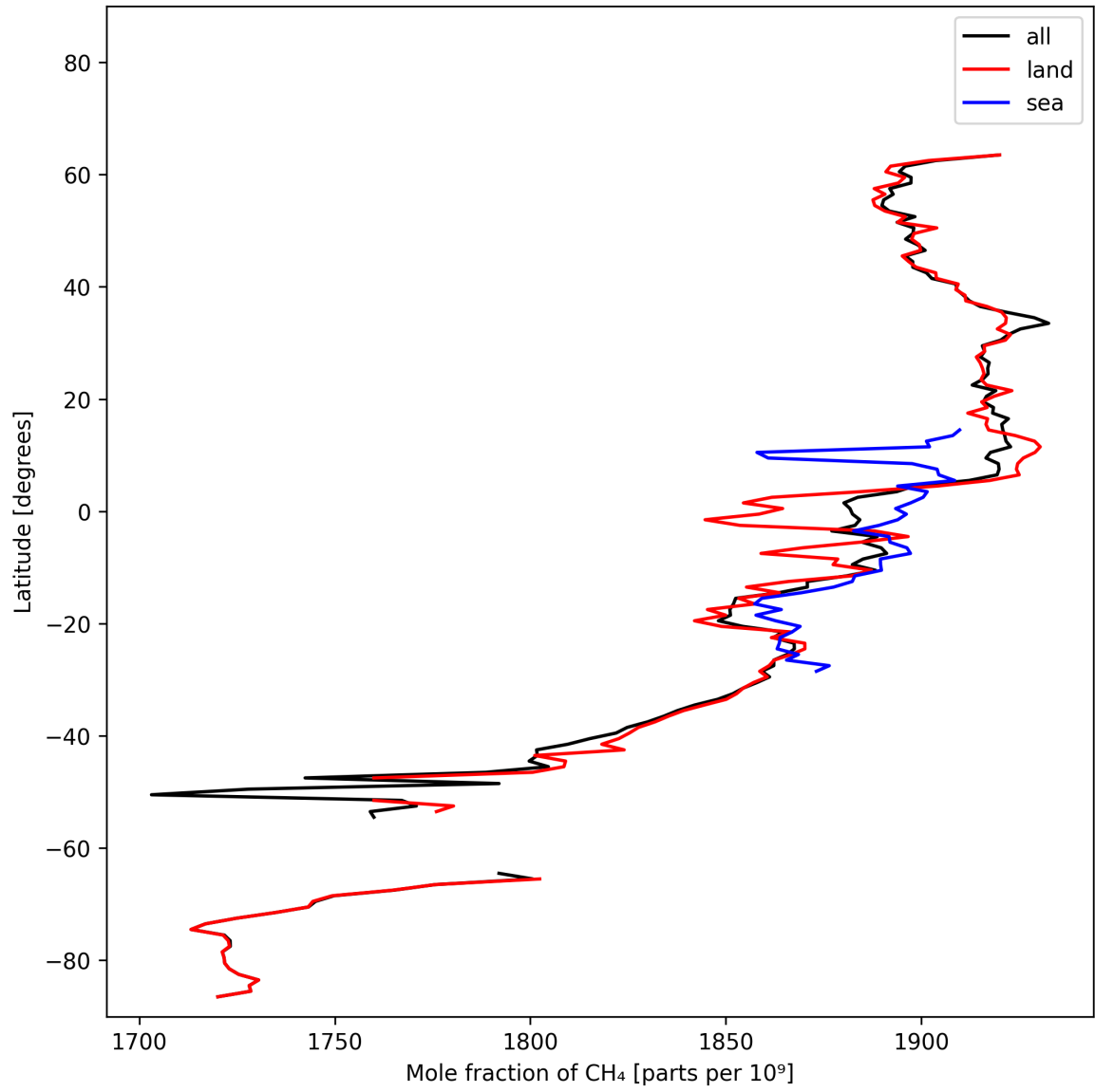
Figure 12: Zonal average of “Mole fraction of \text{CH}_4 ” for 2025-02-15 to 2025-02-17.
