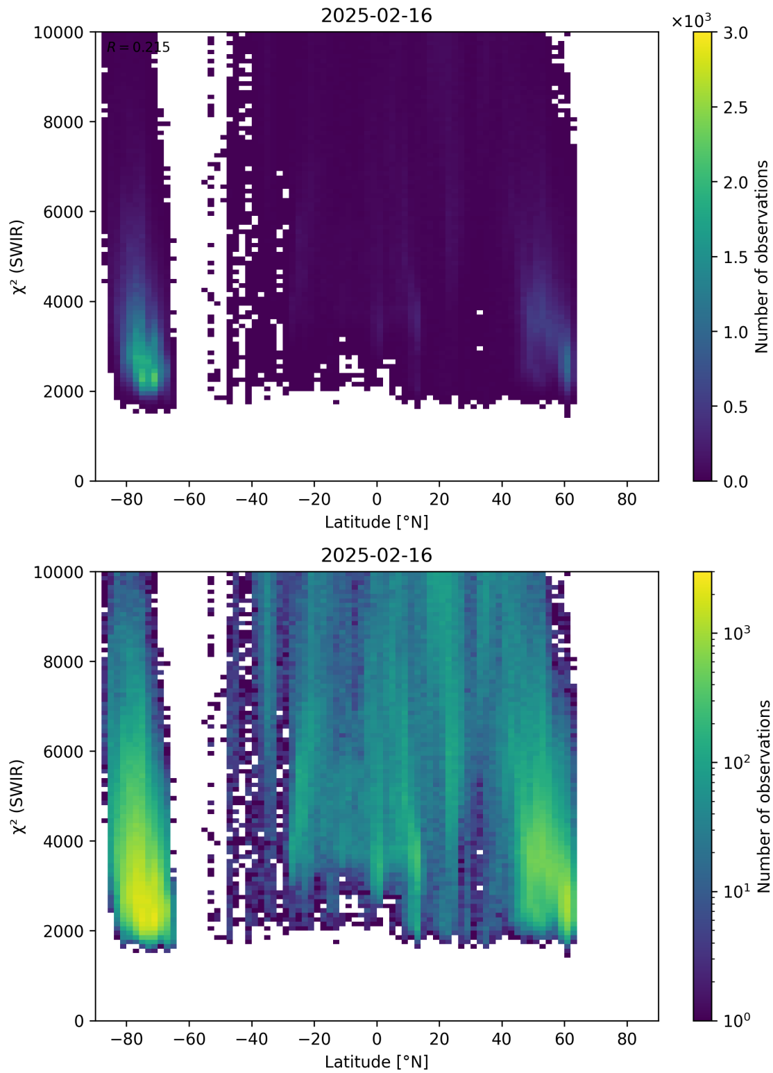
Figure 54: Scatter density plot of “Latitude” against “ \chi^2 (SWIR)” for 2025-02-15 to 2025-02-17.
