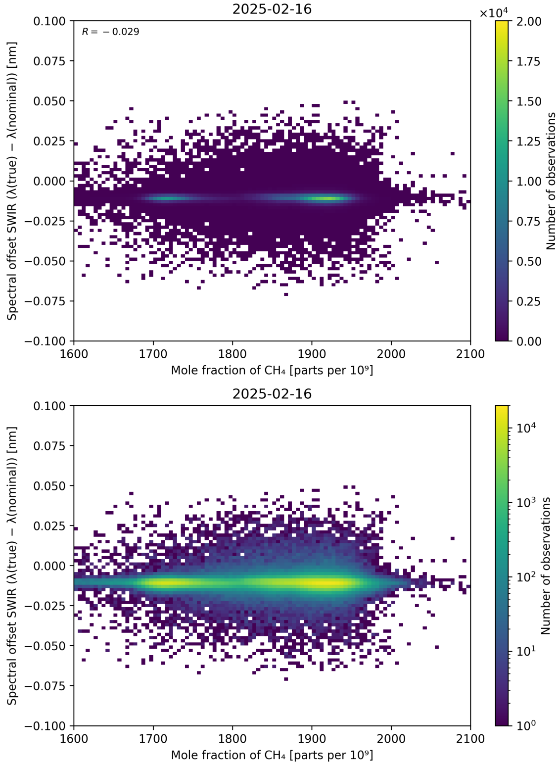
Figure 86: Scatter density plot of “Mole fraction of CH 4 ” against “Spectral offset SWIR ( \lambda_{\text{true}} - \lambda_{\text{nominal}} )” for 2025-02-15 to 2025-02-17.
