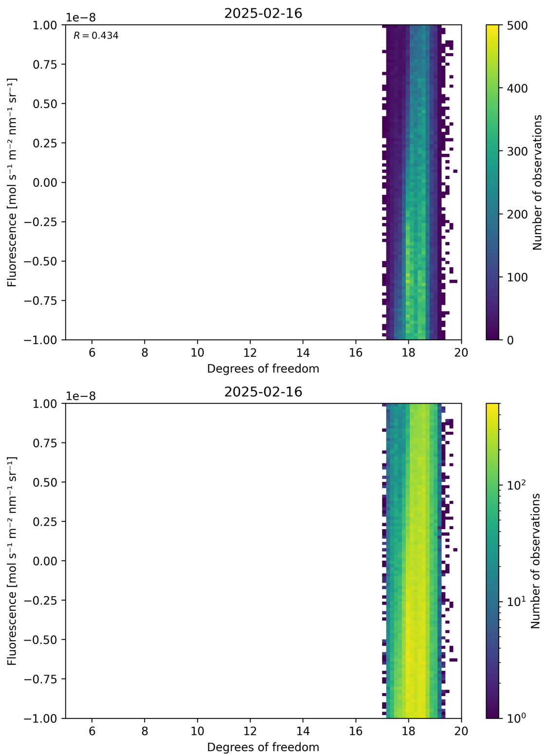
Figure 51: Scatter density plot of “Degrees of freedom” against “Fluorescence” for 2025-02-15 to 2025-02-17.
