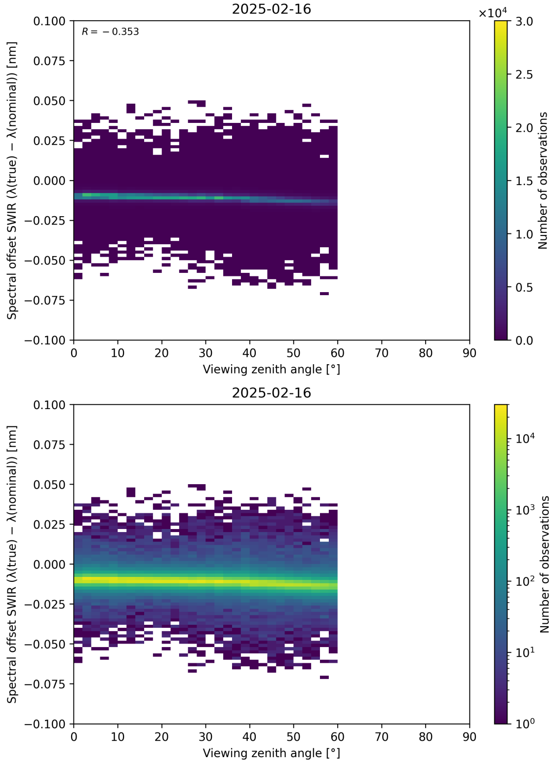
Figure 116: Scatter density plot of “Viewing zenith angle” against “Spectral offset SWIR ( \lambda_{\text{true}} - \lambda_{\text{nominal}} )” for 2025-02-15 to 2025-02-17.
