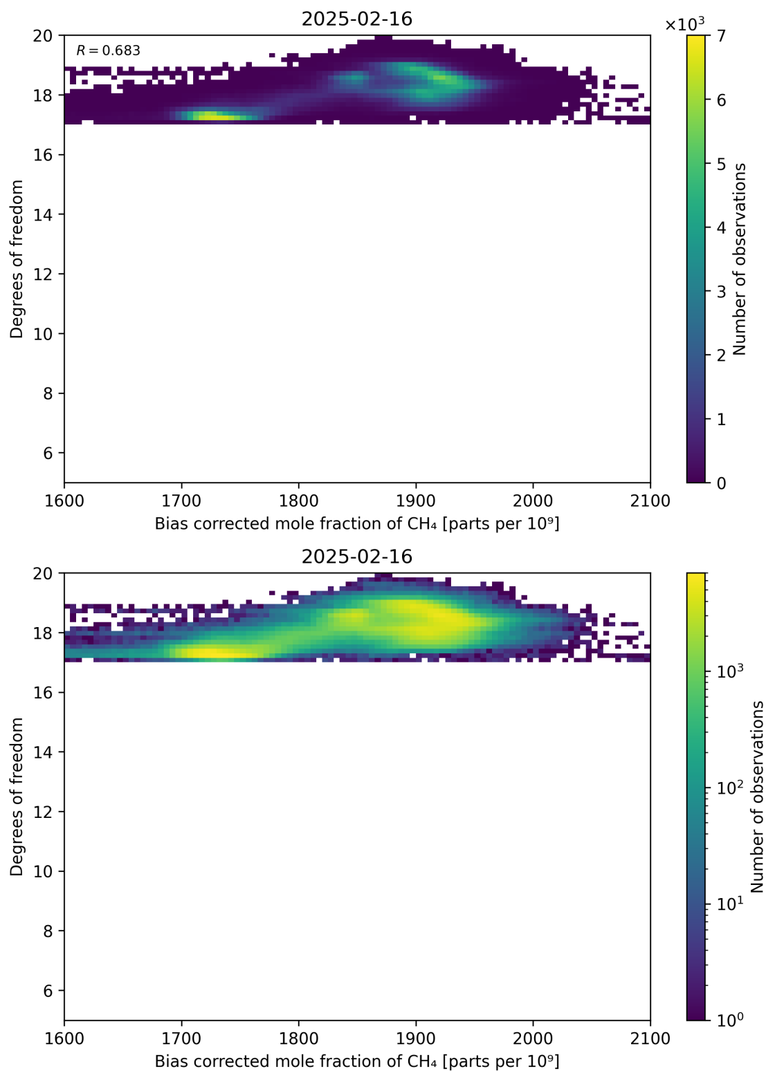
Figure 65: Scatter density plot of “Bias corrected mole fraction of CH 4 ” against “Degrees of freedom” for 2025-02-15 to 2025-02-17.
