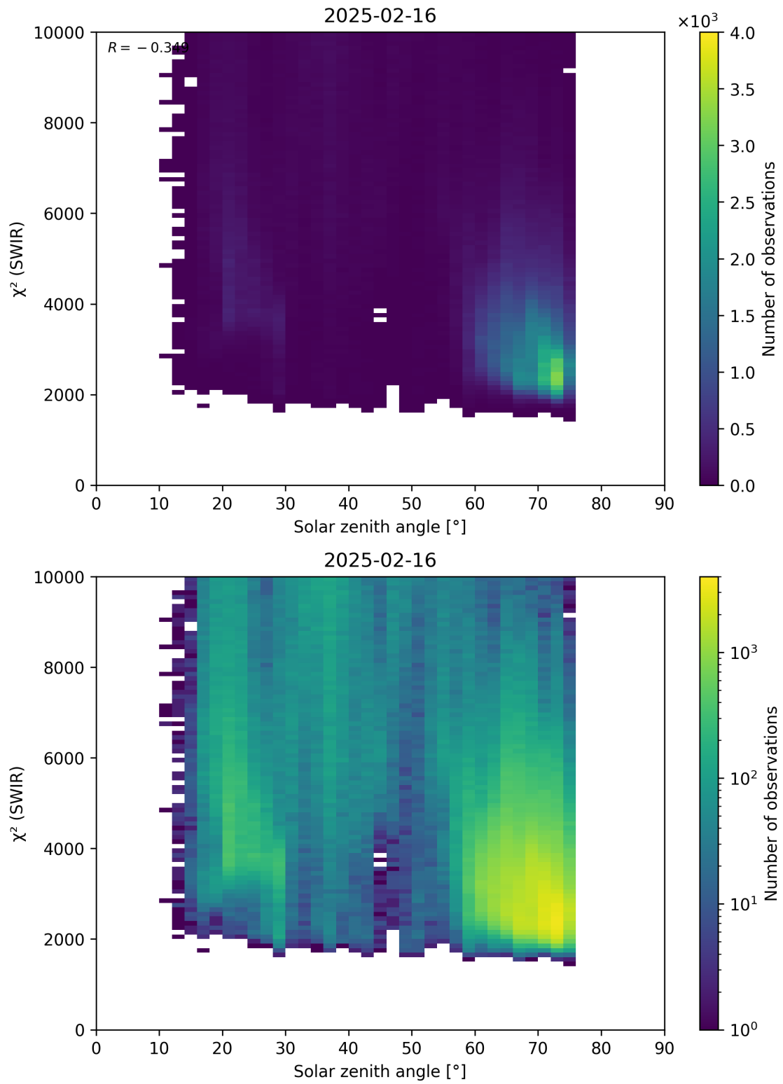
Figure 95: Scatter density plot of “Solar zenith angle” against “ \chi^2 (SWIR)” for 2025-02-15 to 2025-02-17.
