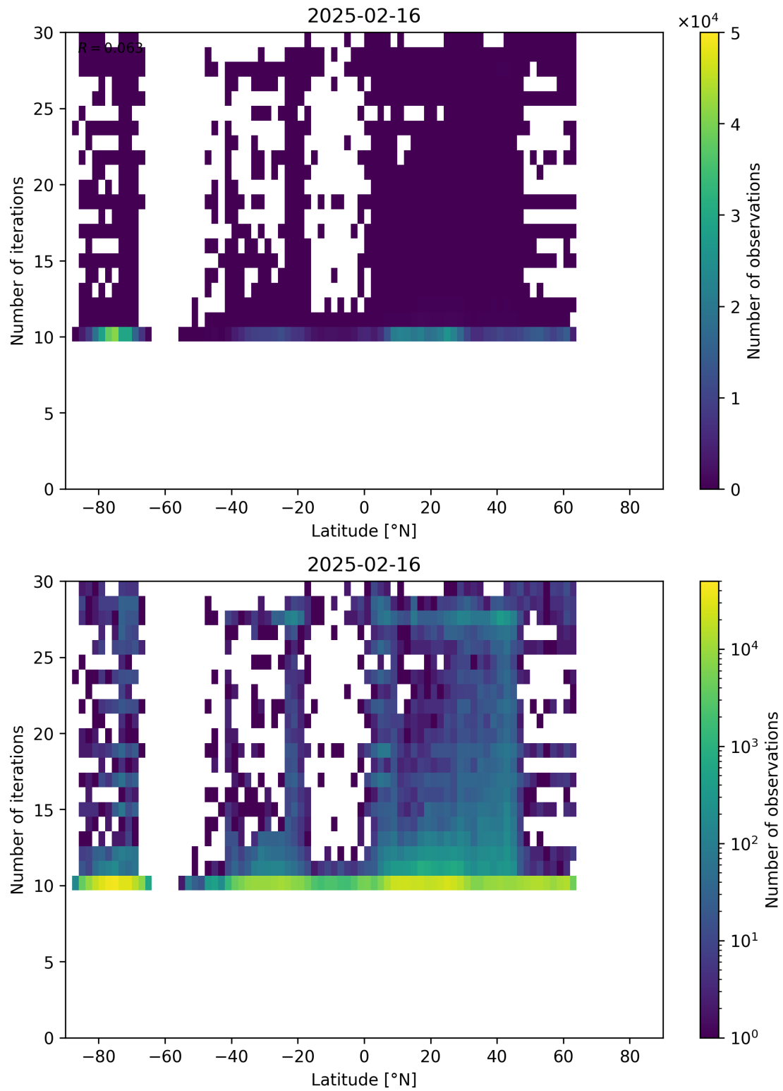
Figure 60: Scatter density plot of “Latitude” against “Number of iterations” for 2025-02-15 to 2025-02-17.
