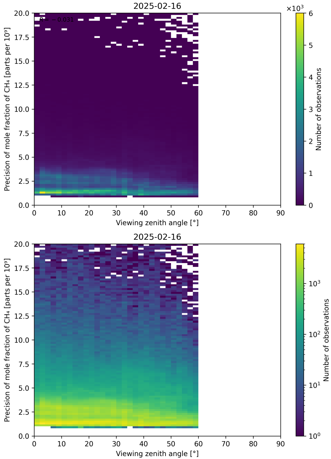
Figure 112: Scatter density plot of “Viewing zenith angle” against “Precision of mole fraction of CH 4 ” for 2025-02-15 to 2025-02-17.
