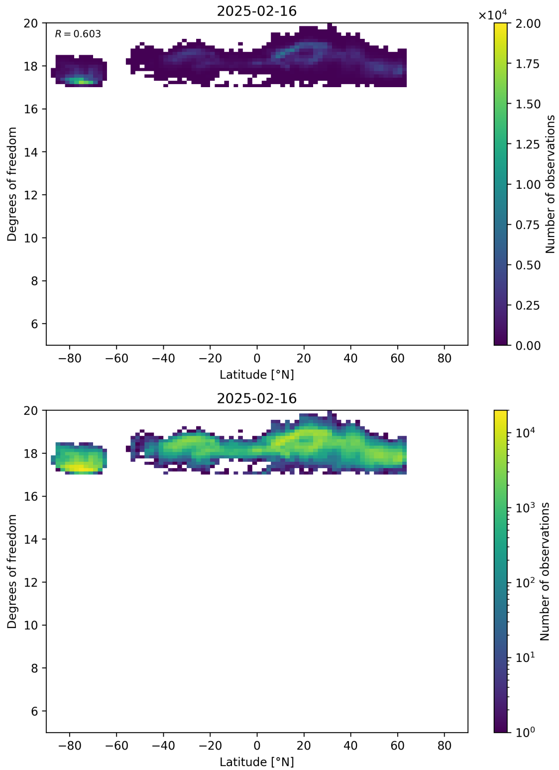
Figure 55: Scatter density plot of “Latitude” against “Degrees of freedom” for 2025-02-15 to 2025-02-17.
