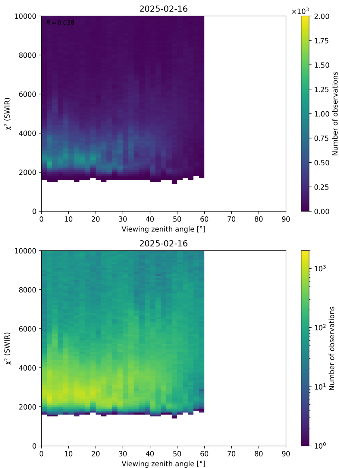
Figure 106: Scatter density plot of “Viewing zenith angle” against “ \chi^2 (SWIR)” for 2025-02-15 to 2025-02-17.
