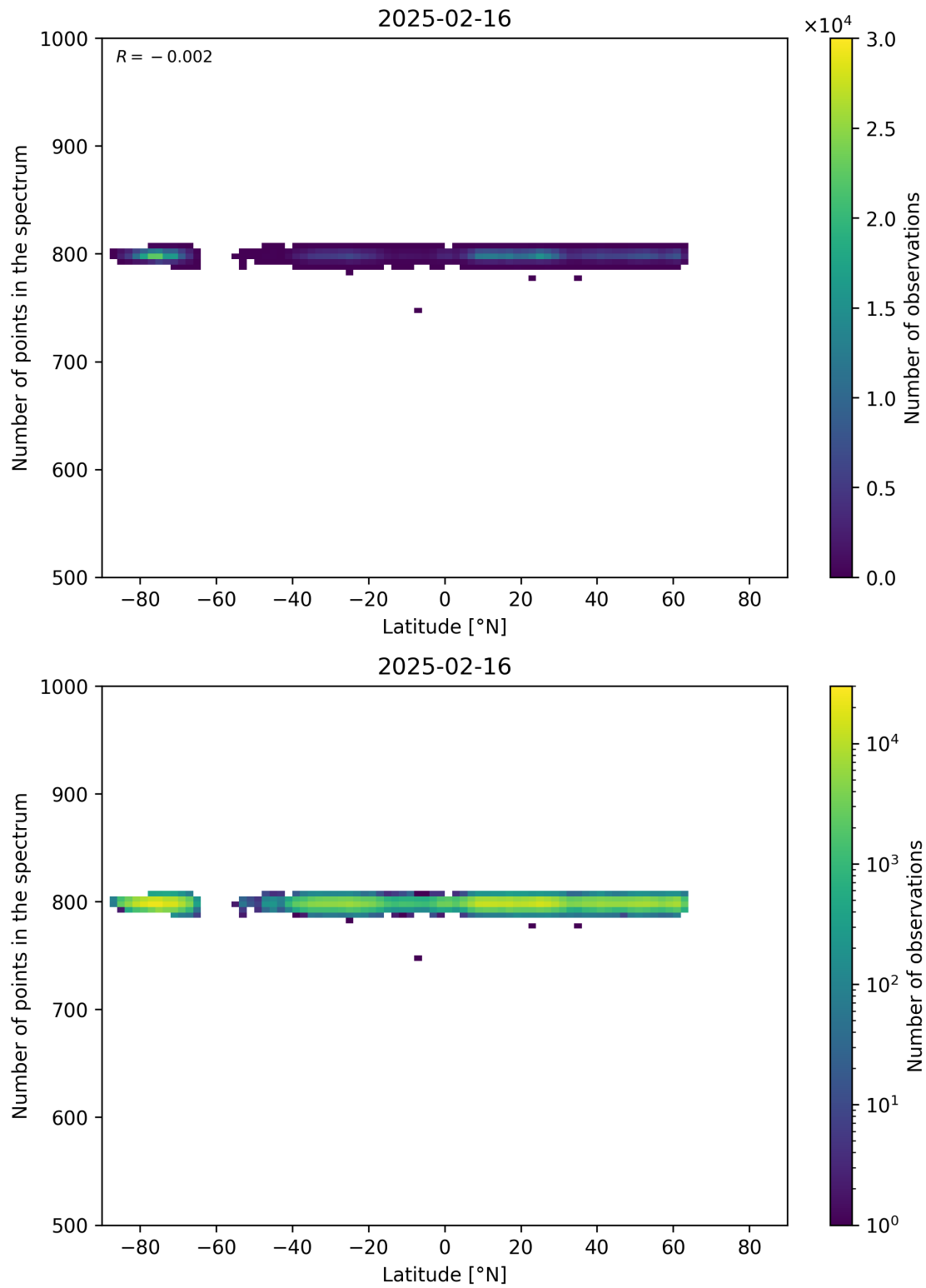
Figure 61: Scatter density plot of “Latitude” against “Number of points in the spectrum” for 2025-02-15 to 2025-02-17.
