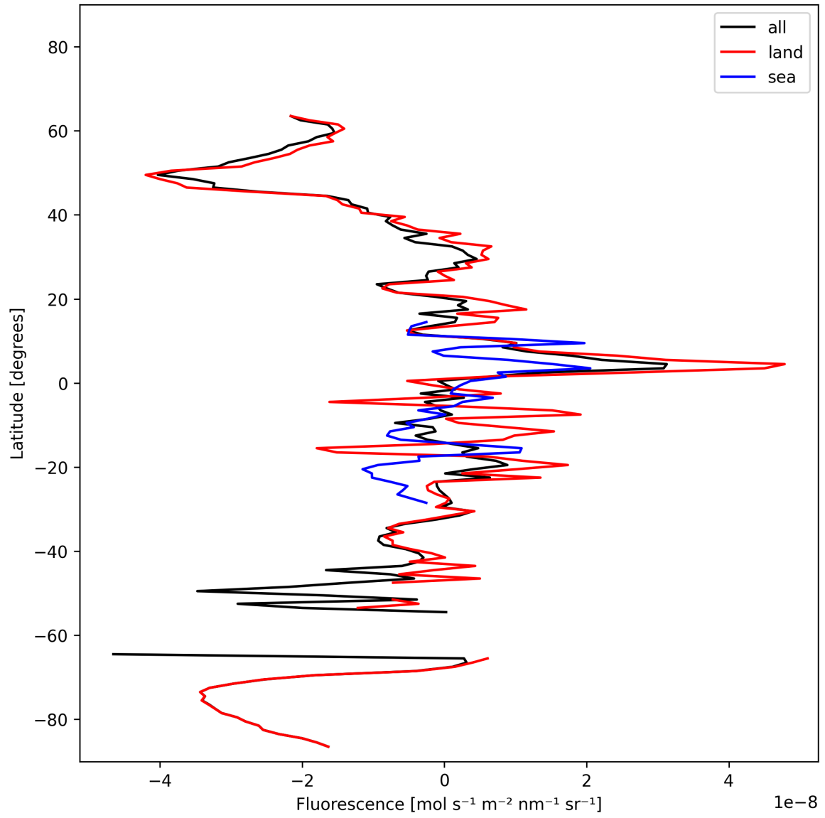
Figure 21: Zonal average of “Fluorescence” for 2025-02-15 to 2025-02-17.
