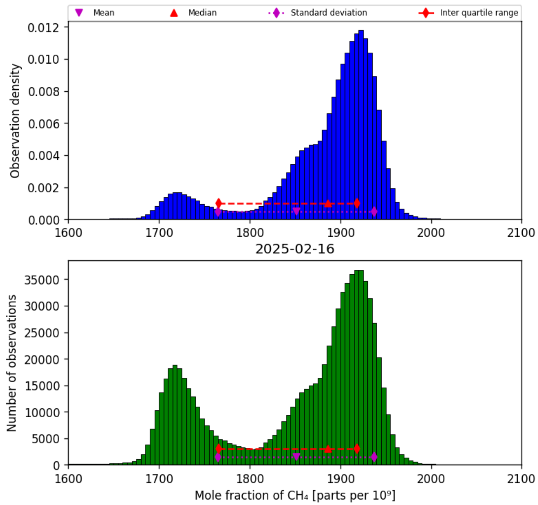
Figure 23: Histogram of “Mole fraction of CH 4 ” for 2025-02-15 to 2025-02-17
