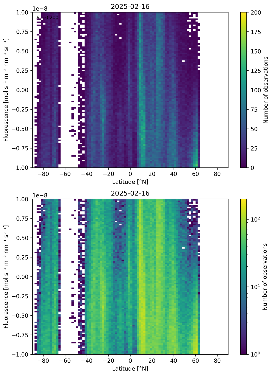
Figure 56: Scatter density plot of “Latitude” against “Fluorescence” for 2025-02-15 to 2025-02-17.
