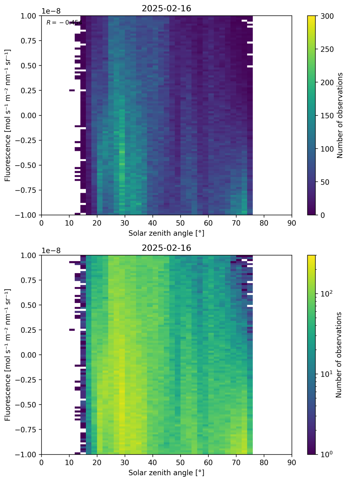
Figure 97: Scatter density plot of “Solar zenith angle” against “Fluorescence” for 2025-02-15 to 2025-02-17.
