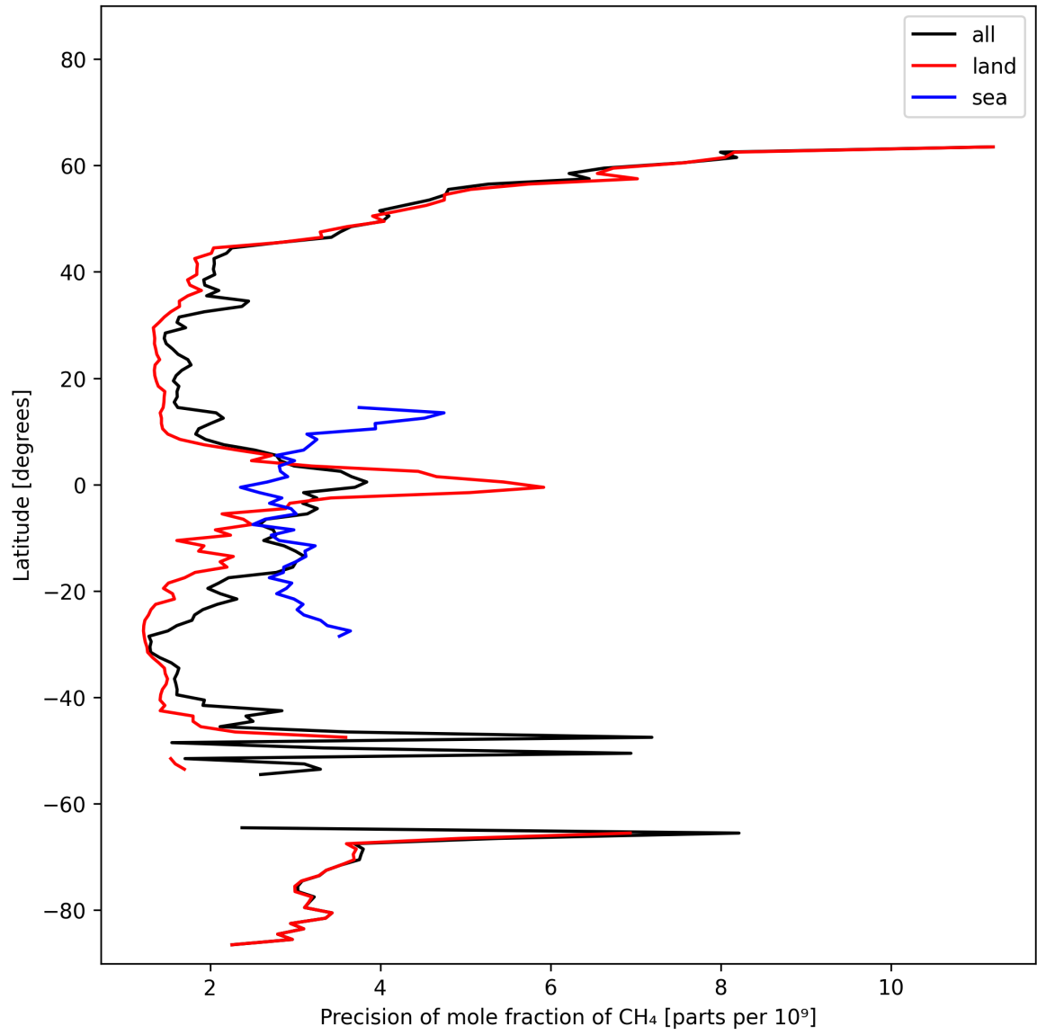
Figure 13: Zonal average of “Precision of mole fraction of CH 4 ” for 2025-02-15 to 2025-02-17.
