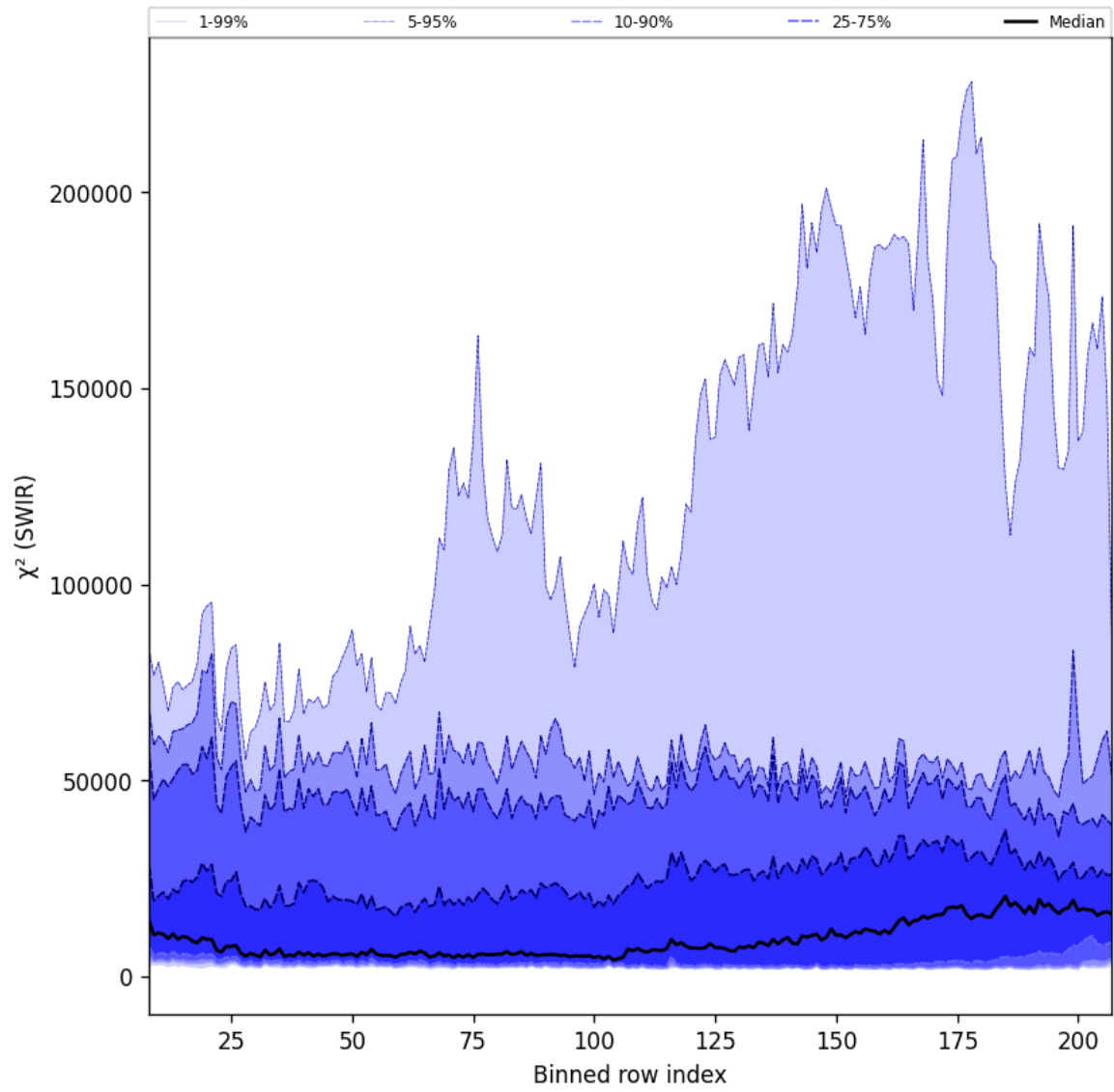
Figure 39: Along track statistics of “ \chi^2 (SWIR)” for 2025-02-15 to 2025-02-17
