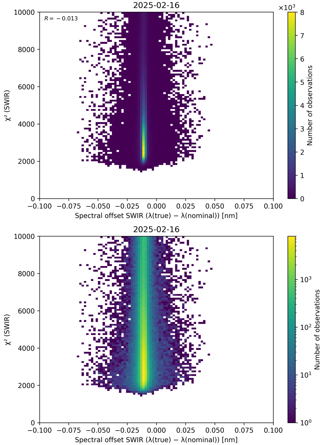
Figure 118: Scatter density plot of “Spectral offset SWIR ( \lambda_{\text{true}} - \lambda_{\text{nominal}} )” against “ \chi^2 (SWIR)” for 2025-02-15 to 2025-02-17.
