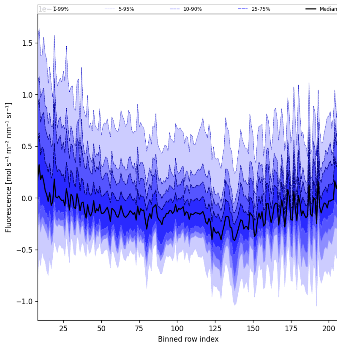
Figure 43: Along track statistics of "Fluorescence" for 2025-02-15 to 2025-02-17
