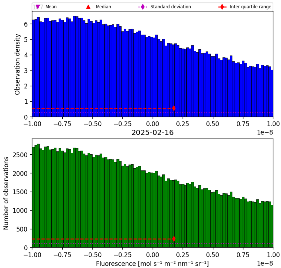
Figure 32: Histogram of “Fluorescence” for 2025-02-15 to 2025-02-17
