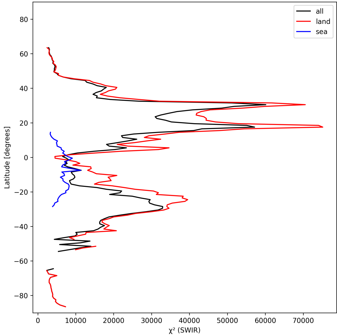
Figure 17: Zonal average of “ \chi^2 (SWIR)” for 2025-02-15 to 2025-02-17.
