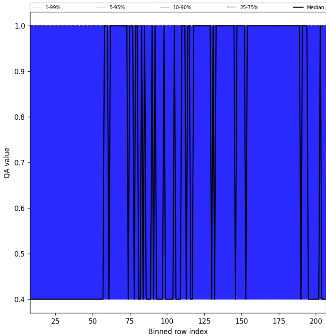
Figure 33: Along track statistics of “QA value” for 2025-02-15 to 2025-02-17
