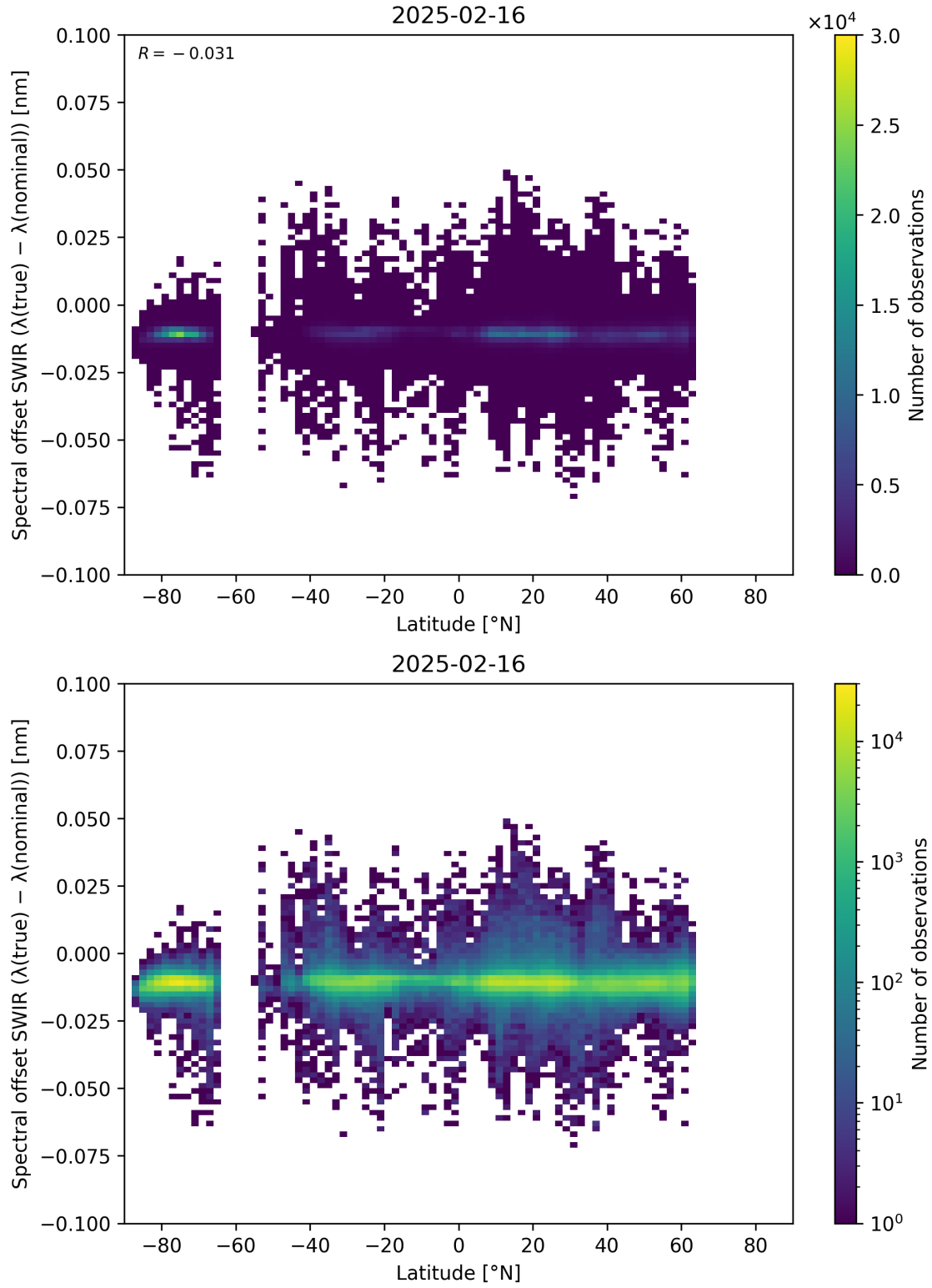
Figure 62: Scatter density plot of “Latitude” against “Spectral offset SWIR ( \lambda_{\text{true}} - \lambda_{\text{nominal}} )” for 2025-02-15 to 2025-02-17.
