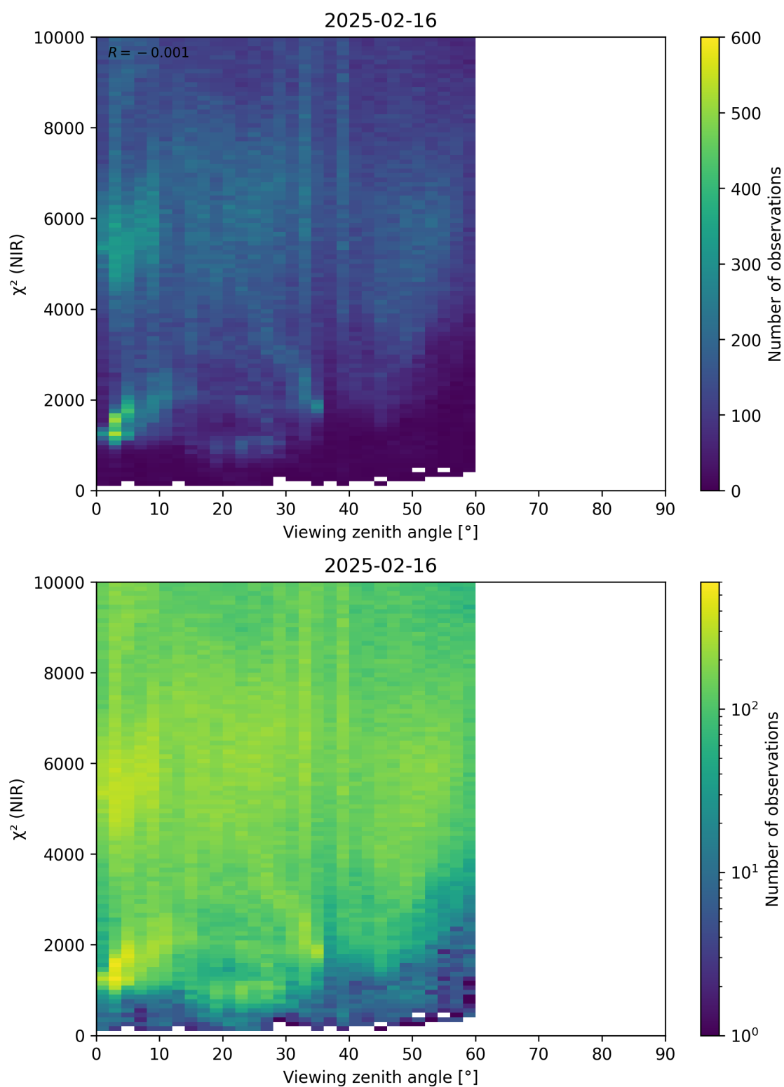
Figure 105: Scatter density plot of “Viewing zenith angle” against “ \chi^2 (NIR)” for 2025-02-15 to 2025-02-17.
