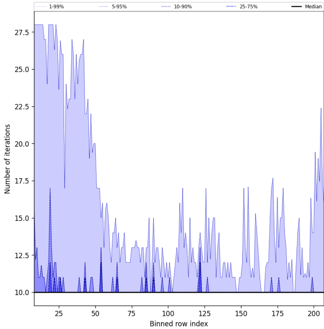
Figure 42: Along track statistics of “Number of iterations” for 2025-02-15 to 2025-02-17
