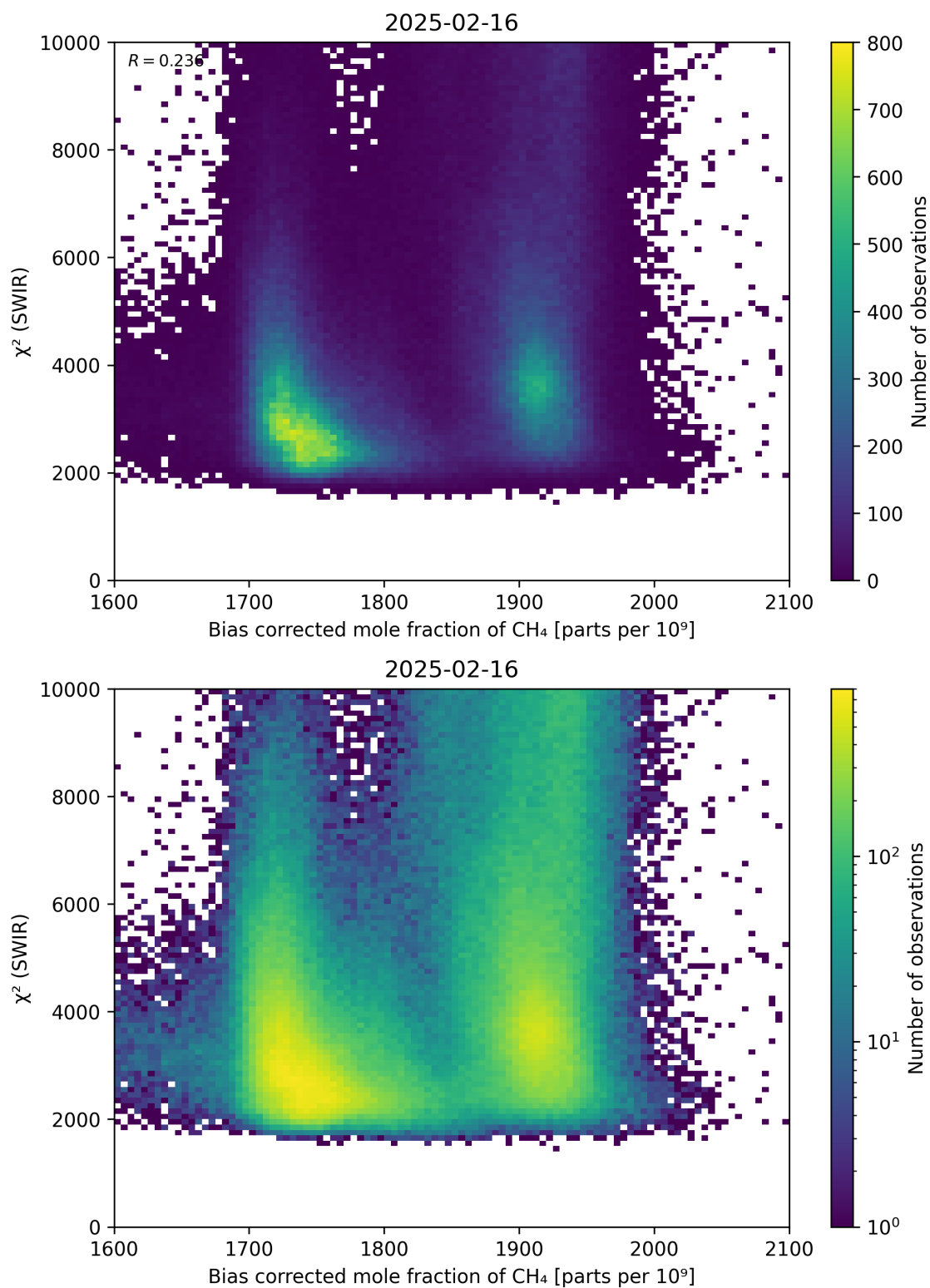
Figure 64: Scatter density plot of “Bias corrected mole fraction of \text{CH}_4 ” against “ \chi^2 (SWIR)” for 2025-02-15 to 2025-02-17.
