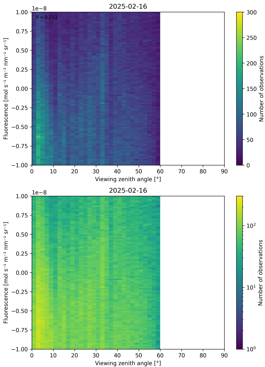
Figure 108: Scatter density plot of “Viewing zenith angle” against “Fluorescence” for 2025-02-15 to 2025-02-17.
