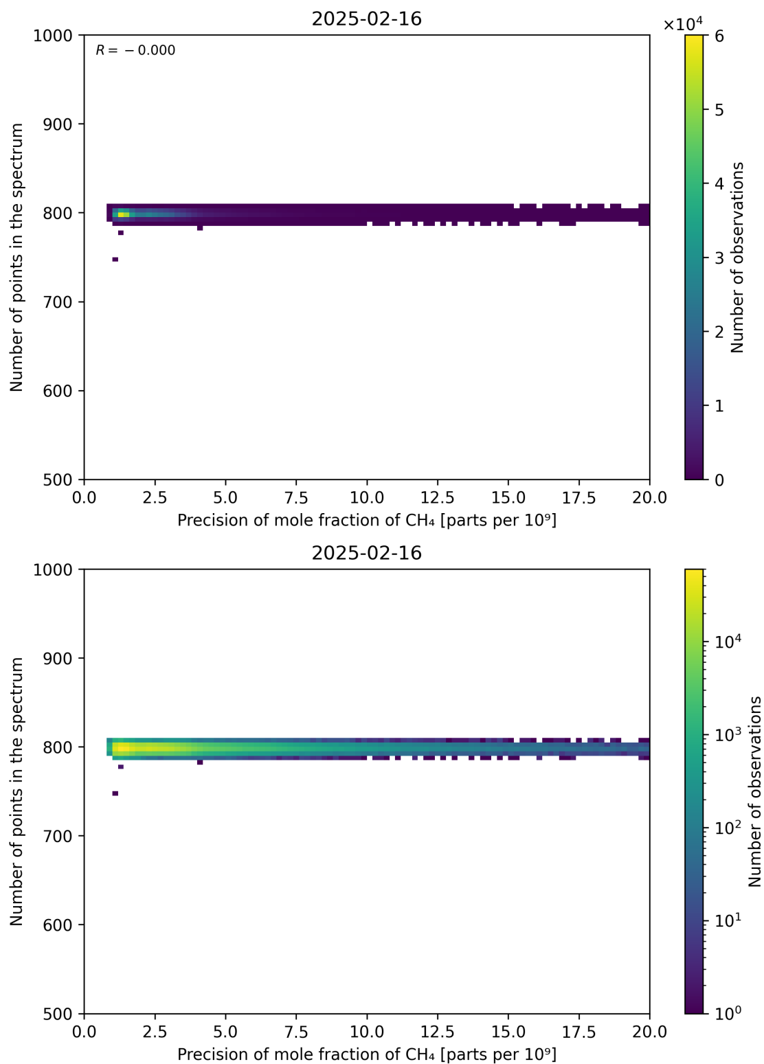
Figure 84: Scatter density plot of “Precision of mole fraction of CH 4 ” against “Number of points in the spectrum” for 2025-02-15 to 2025-02-17.
