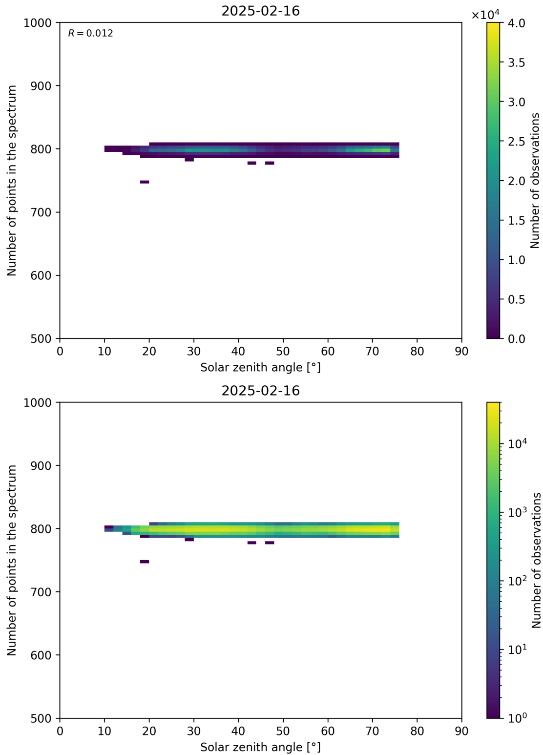
Figure 103: Scatter density plot of “Solar zenith angle” against “Number of points in the spectrum” for 2025-02-15 to 2025-02-17.
