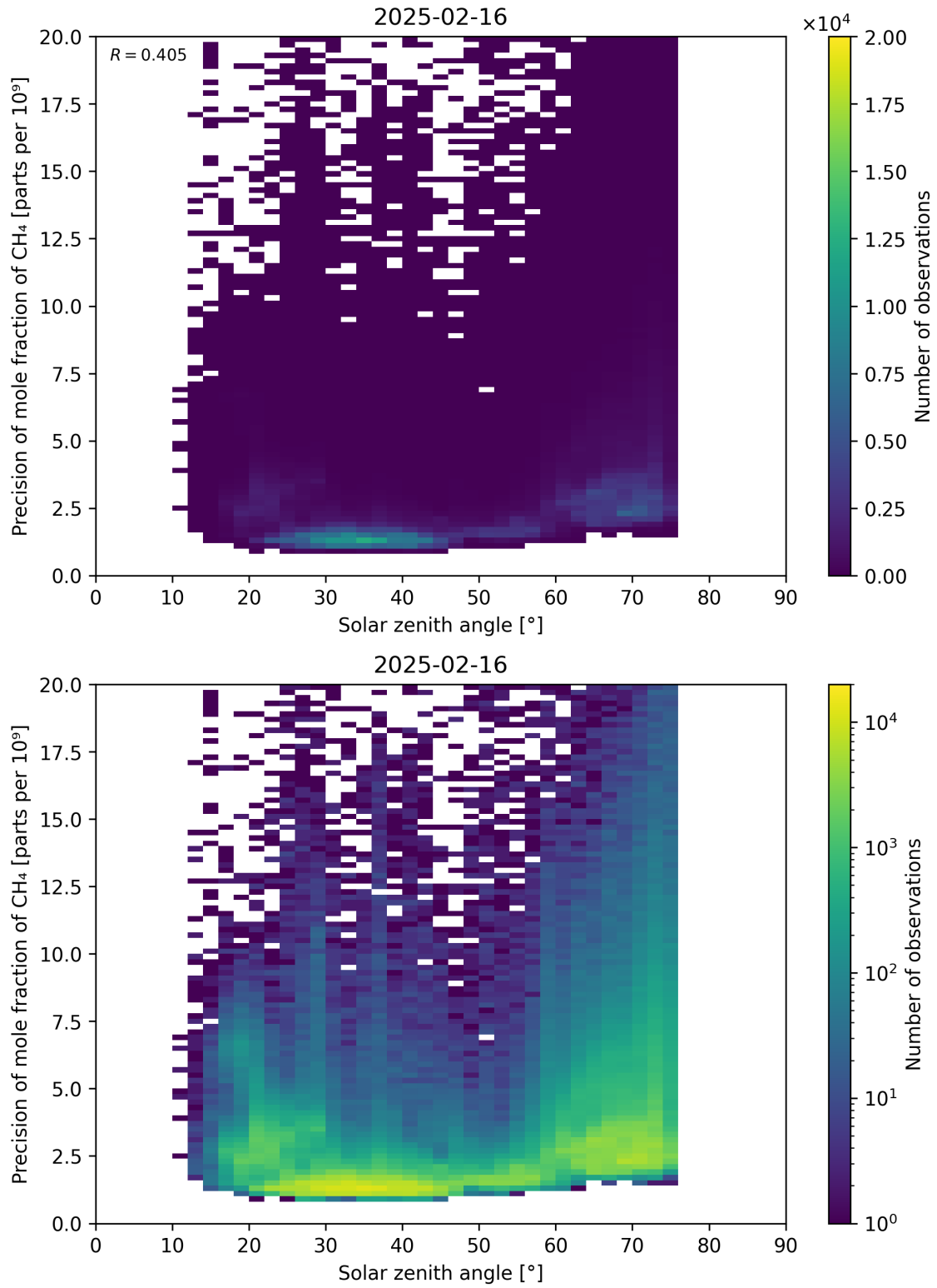
Figure 101: Scatter density plot of “Solar zenith angle” against “Precision of mole fraction of \text{CH}_4 ” for 2025-02-15 to 2025-02-17.
