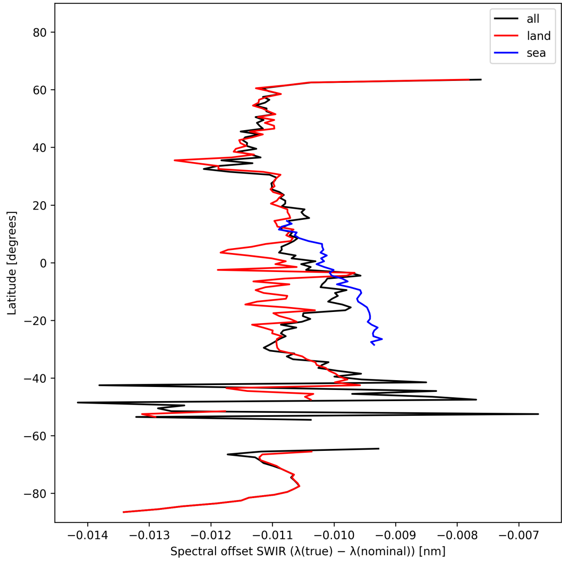
Figure 16: Zonal average of “Spectral offset SWIR ( \lambda_{\text{true}} - \lambda_{\text{nominal}} )” for 2025-02-15 to 2025-02-17.
