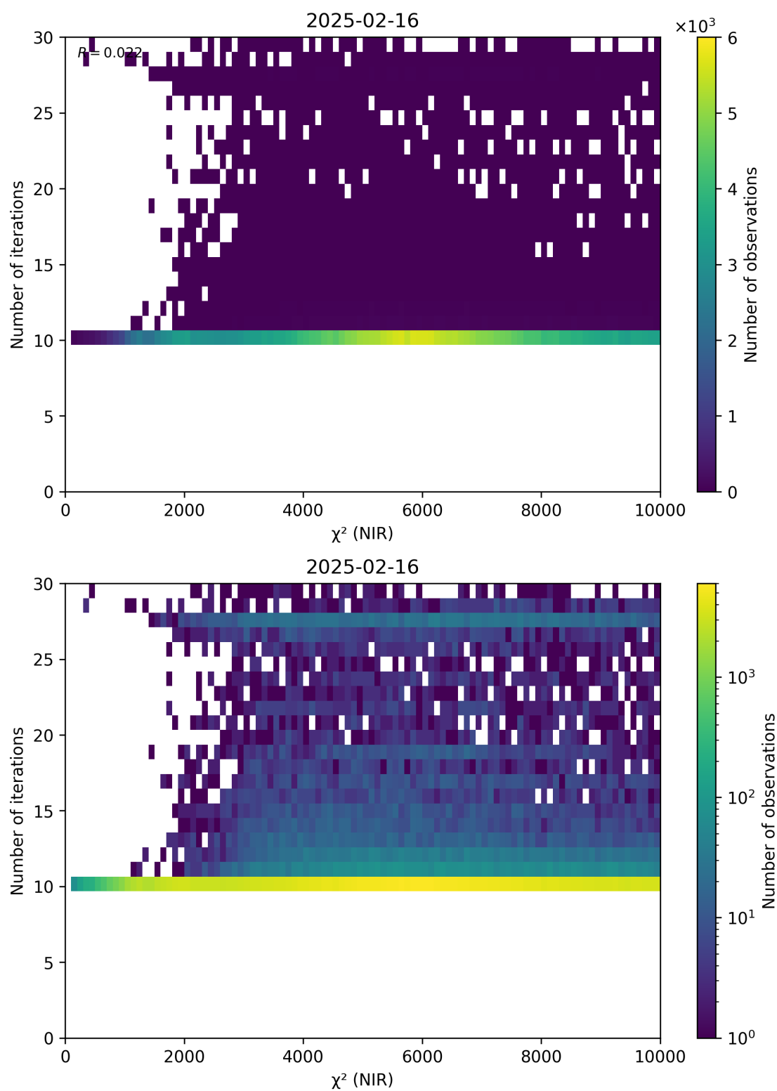
Figure 46: Scatter density plot of “ \chi^2 (NIR)” against “Number of iterations” for 2025-02-15 to 2025-02-17.
