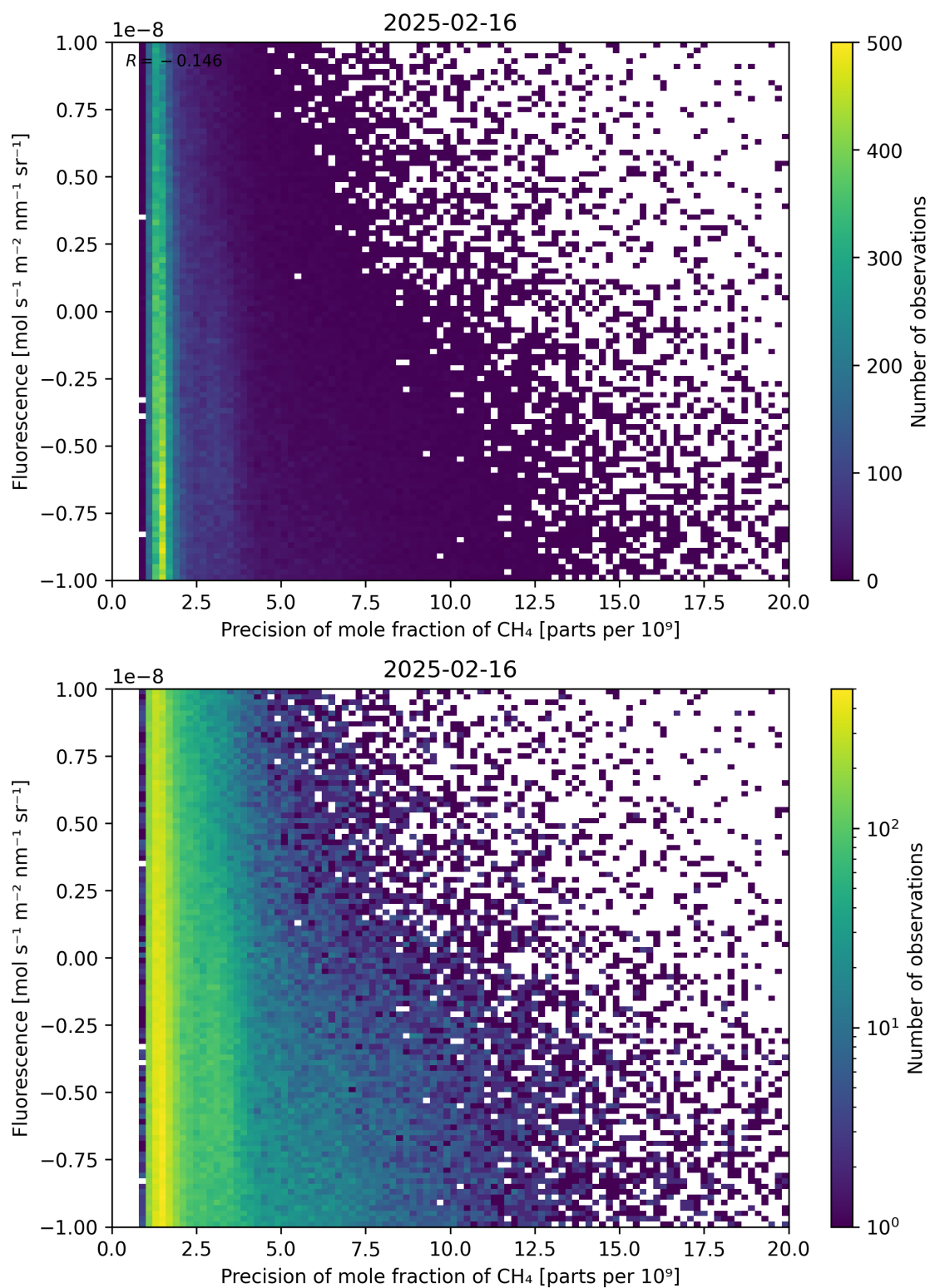
Figure 81: Scatter density plot of “Precision of mole fraction of CH 4 ” against “Fluorescence” for 2025-02-15 to 2025-02-17.
