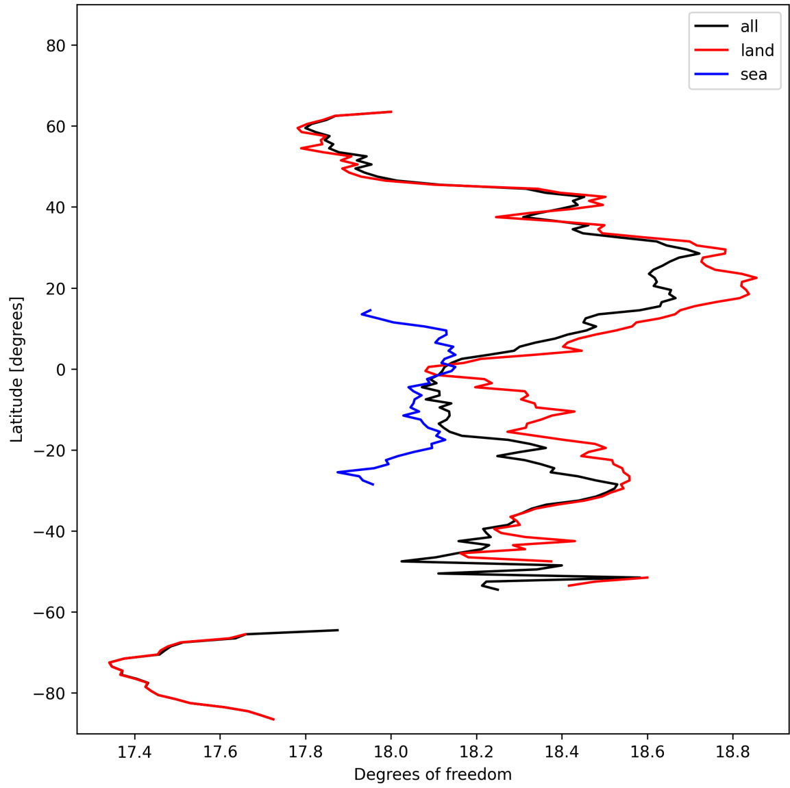
Figure 19: Zonal average of "Degrees of freedom" for 2025-02-15 to 2025-02-17.
