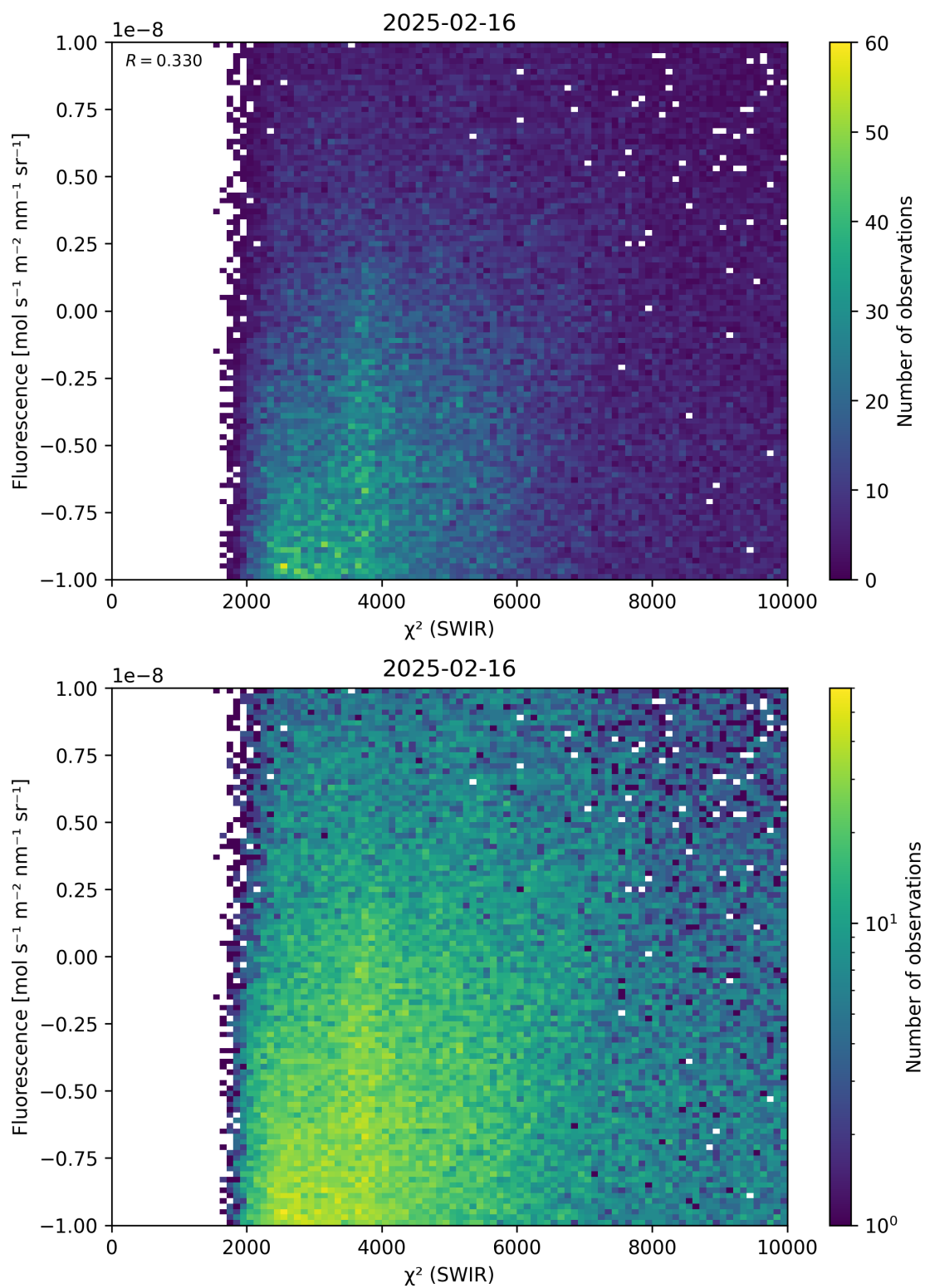
Figure 49: Scatter density plot of “ \chi^2 (SWIR)” against “Fluorescence” for 2025-02-15 to 2025-02-17.
