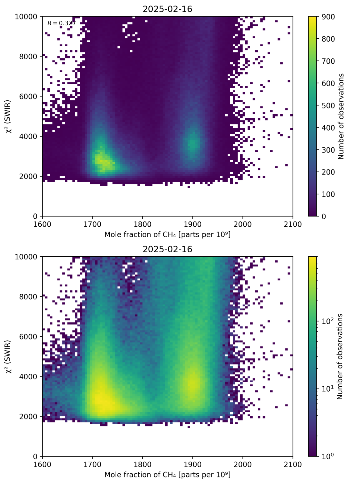
Figure 71: Scatter density plot of “Mole fraction of \text{CH}_4 ” against “ \chi^2 (SWIR)” for 2025-02-15 to 2025-02-17.
