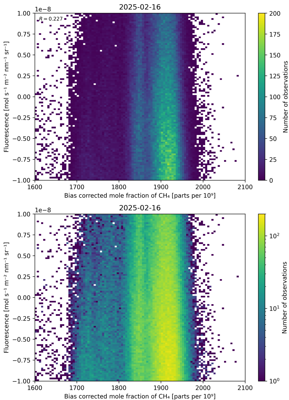
Figure 66: Scatter density plot of “Bias corrected mole fraction of \text{CH}_4 ” against “Fluorescence” for 2025-02-15 to 2025-02-17.
