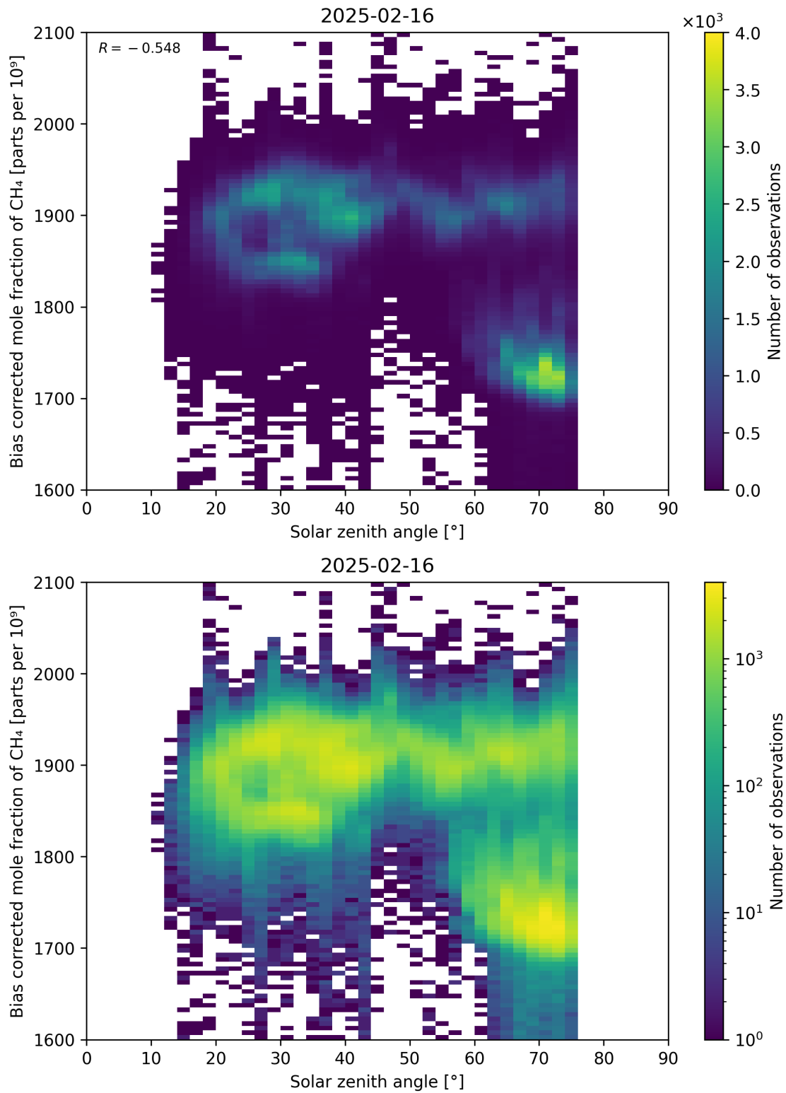
Figure 100: Scatter density plot of “Solar zenith angle” against “Bias corrected mole fraction of \text{CH}_4 ” for 2025-02-15 to 2025-02-17.
