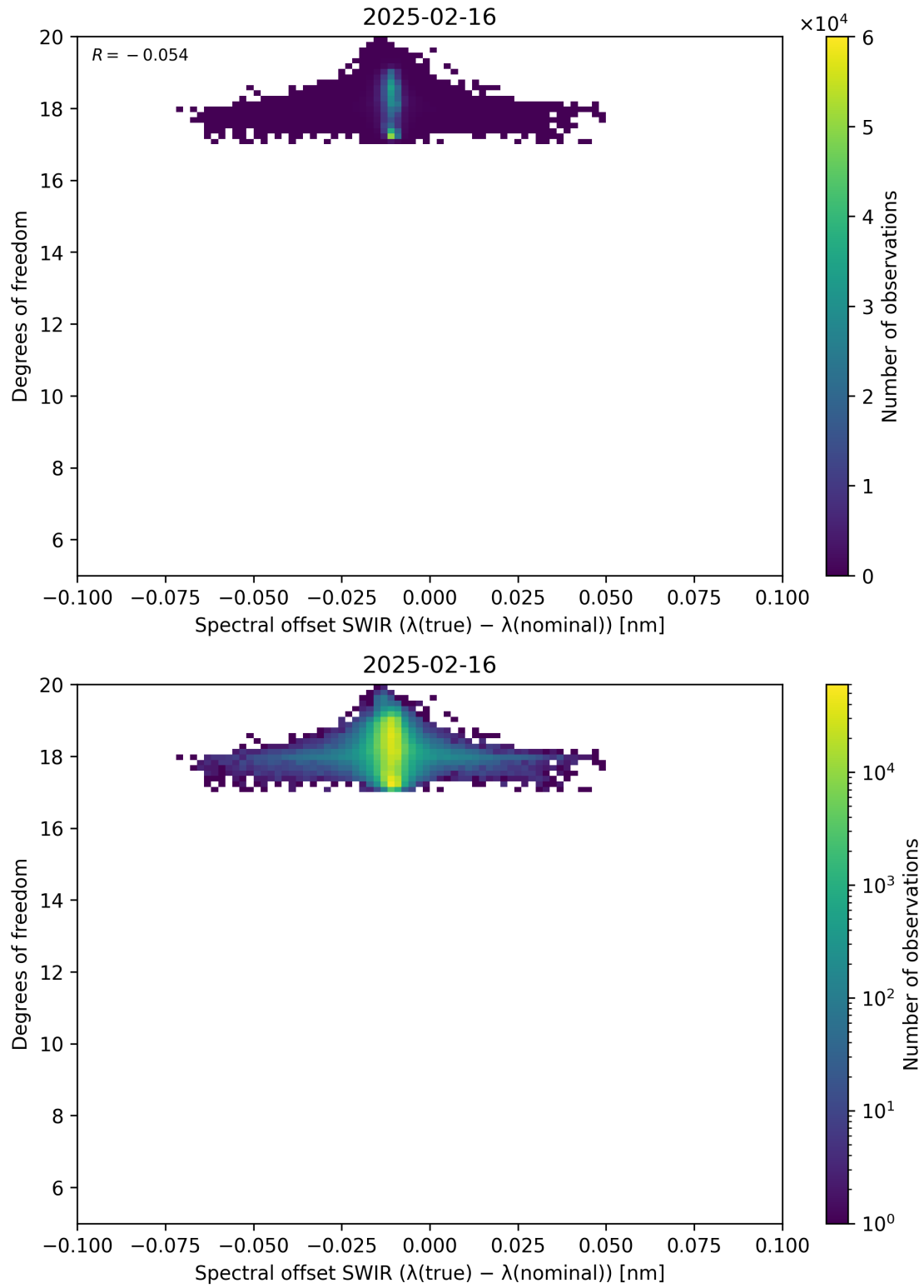
Figure 119: Scatter density plot of “Spectral offset SWIR ( \lambda_{\text{true}} - \lambda_{\text{nominal}} )” against “Degrees of freedom” for 2025-02-15 to 2025-02-17.
