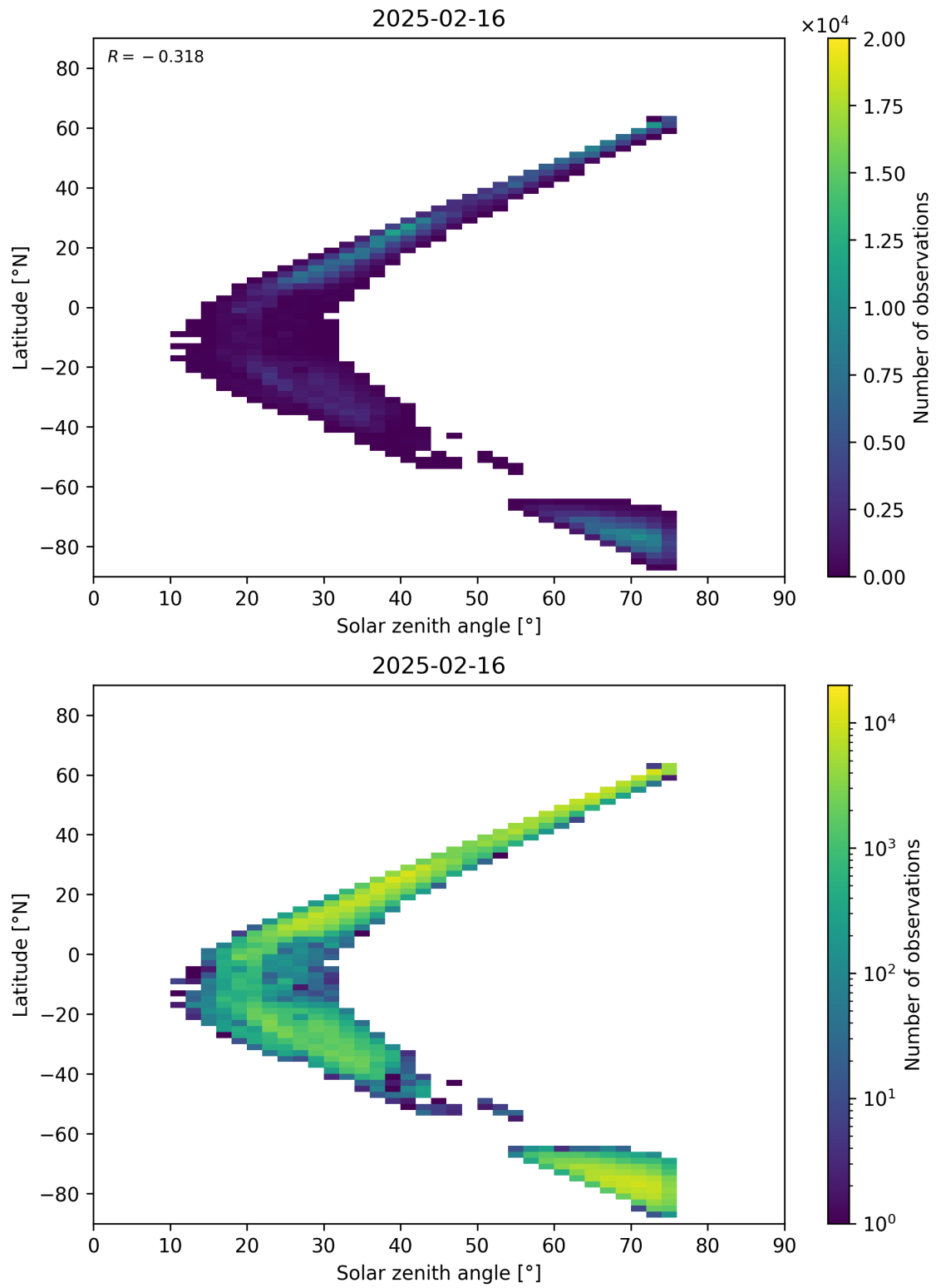
Figure 98: Scatter density plot of “Solar zenith angle” against “Latitude” for 2025-02-15 to 2025-02-17.
