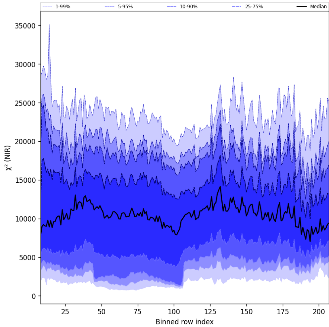
Figure 40: Along track statistics of " \chi^2 (NIR)" for 2025-02-15 to 2025-02-17
