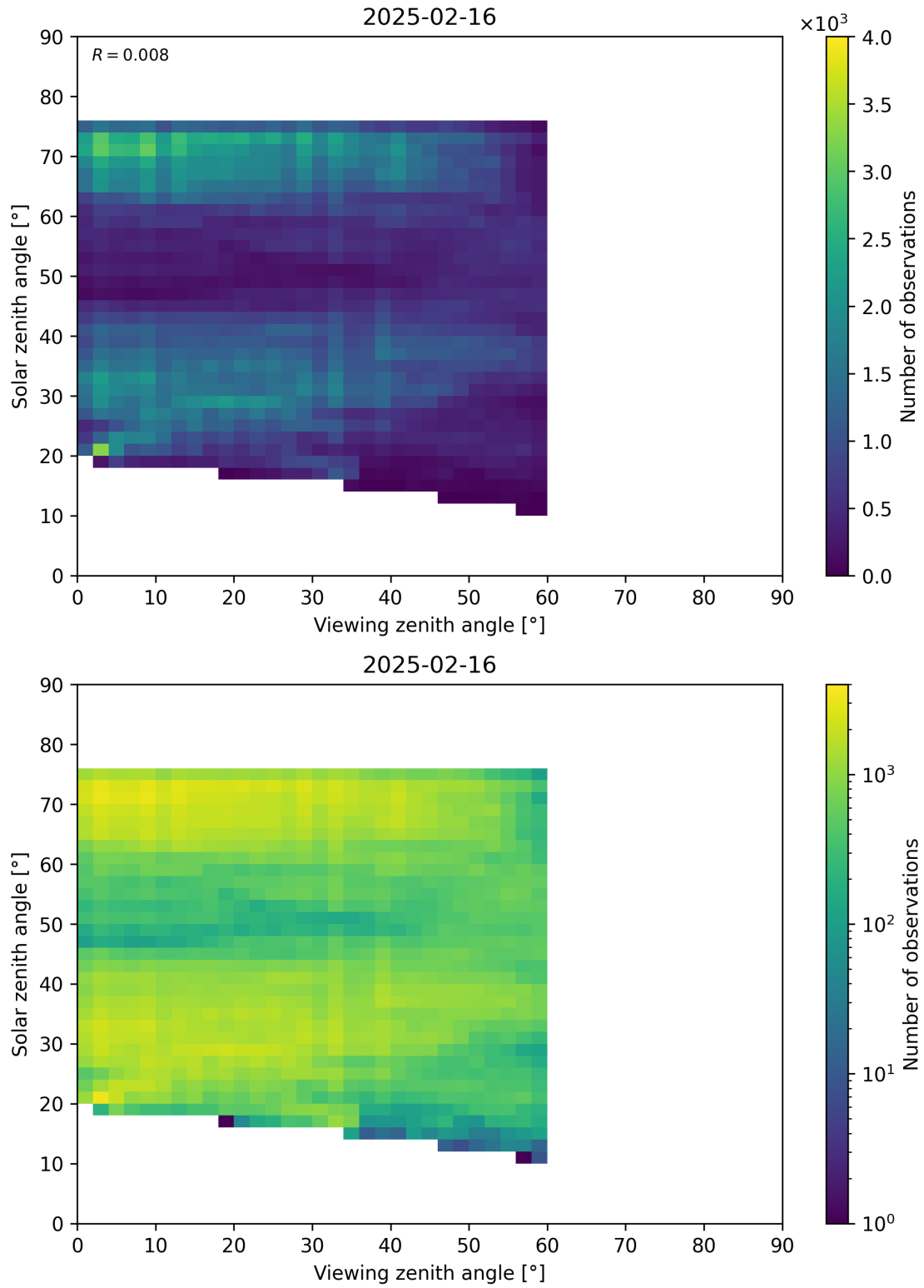
Figure 115: Scatter density plot of “Viewing zenith angle” against “Solar zenith angle” for 2025-02-15 to 2025-02-17.
