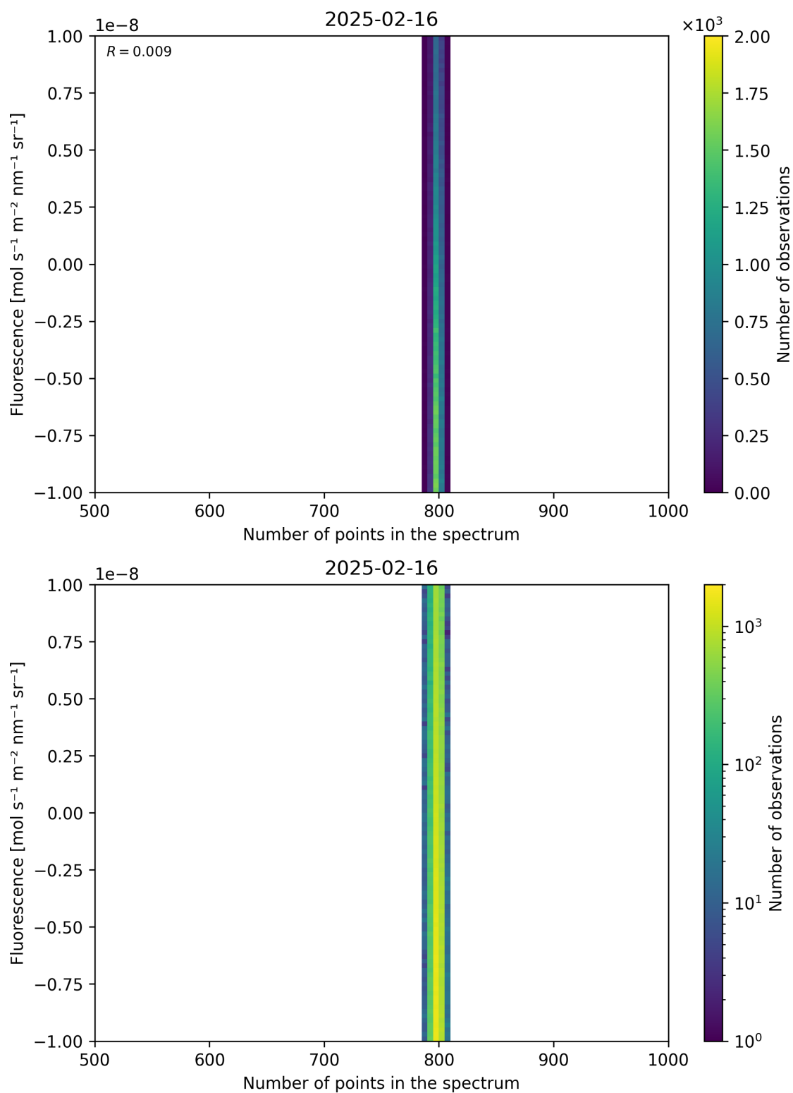
Figure 91: Scatter density plot of “Number of points in the spectrum” against “Fluorescence” for 2025-02-15 to 2025-02-17.
