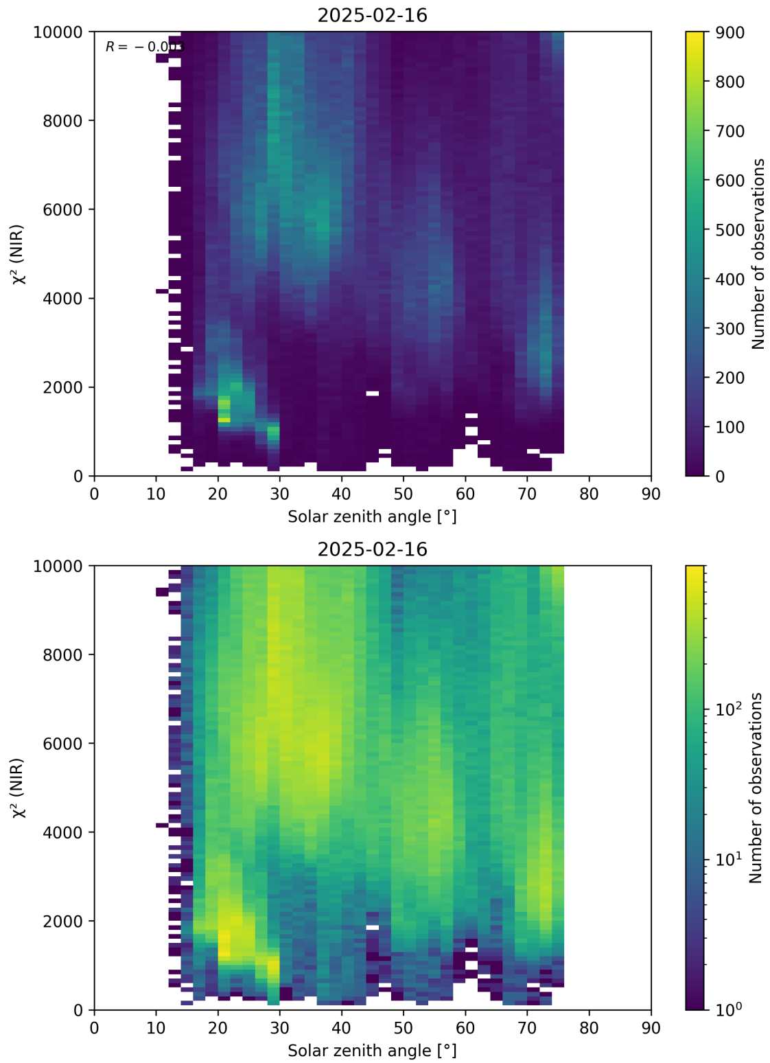
Figure 94: Scatter density plot of “Solar zenith angle” against “ \chi^2 (NIR)” for 2025-02-15 to 2025-02-17.
