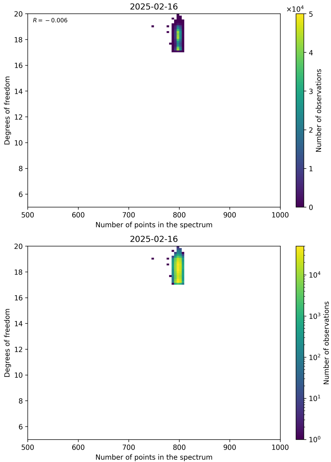
Figure 90: Scatter density plot of “Number of points in the spectrum” against “Degrees of freedom” for 2025-02-15 to 2025-02-17.
