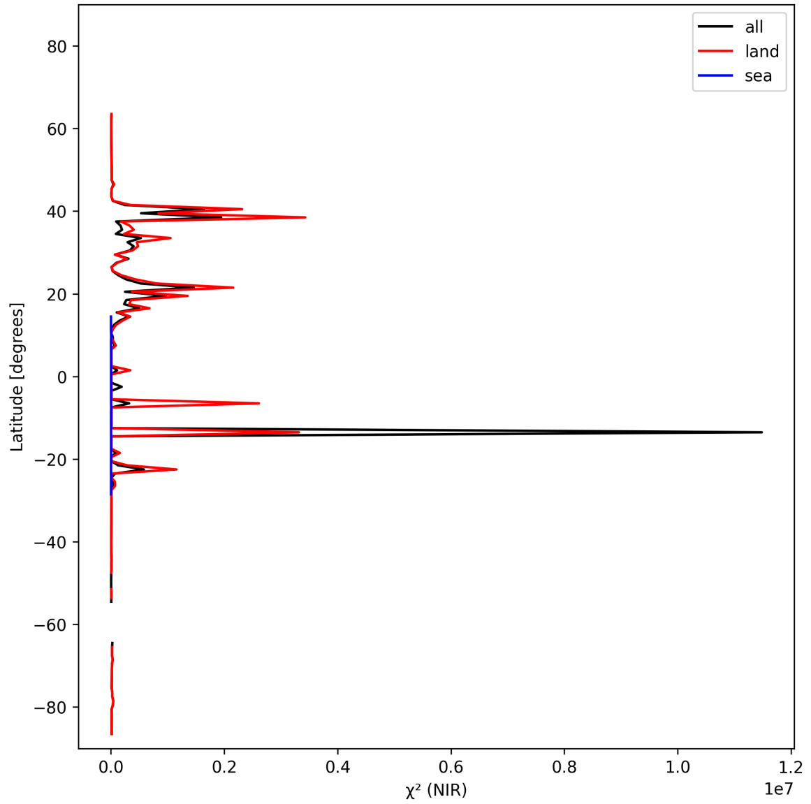
Figure 18: Zonal average of “ \chi^2 (NIR)” for 2025-02-15 to 2025-02-17.
