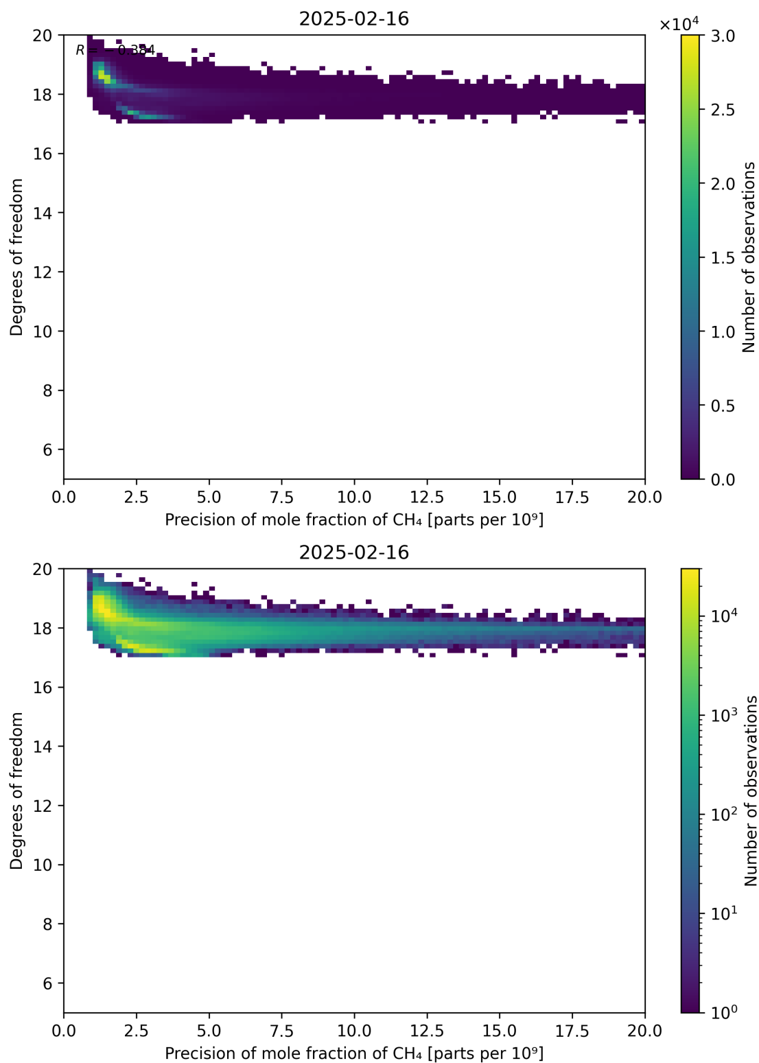
Figure 80: Scatter density plot of “Precision of mole fraction of CH 4 ” against “Degrees of freedom” for 2025-02-15 to 2025-02-17.
