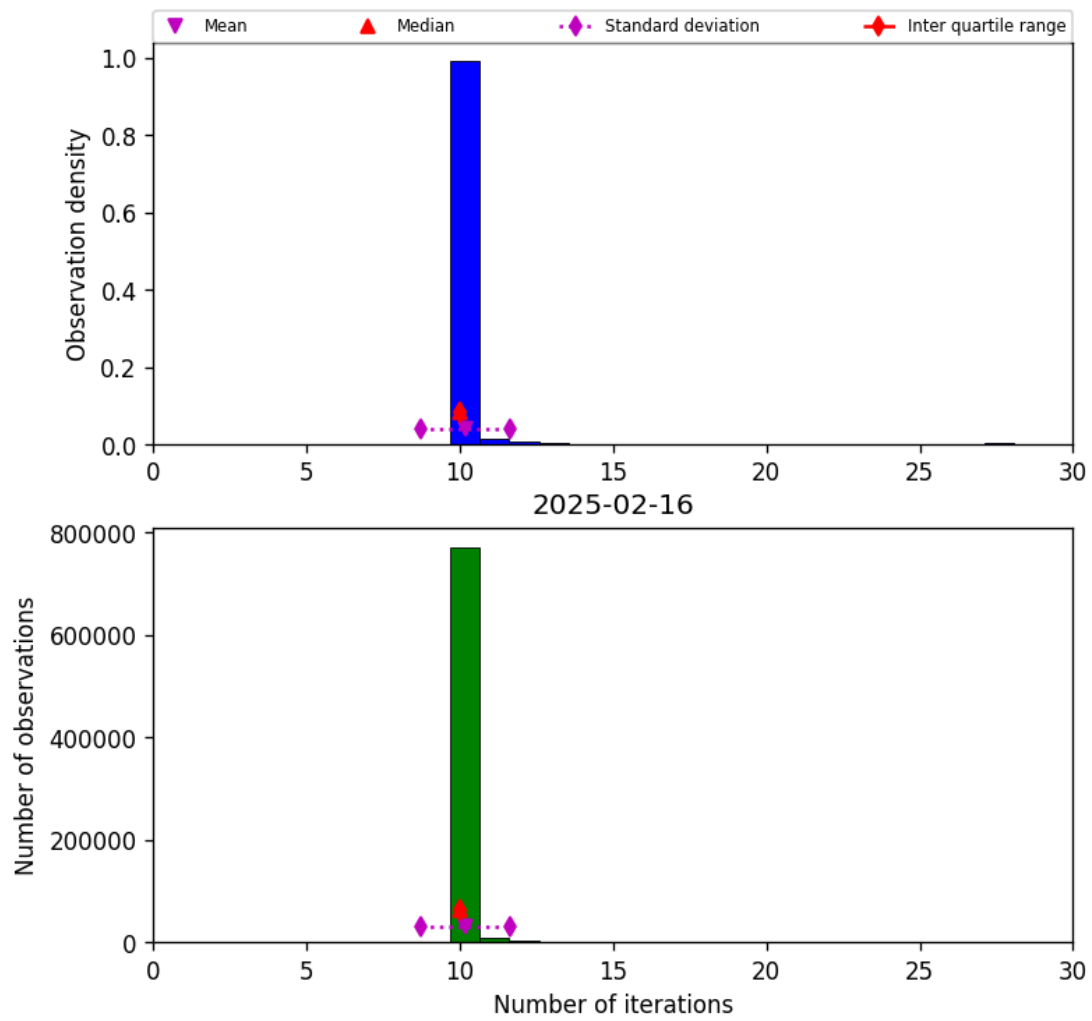
Figure 31: Histogram of “Number of iterations” for 2025-02-15 to 2025-02-17
