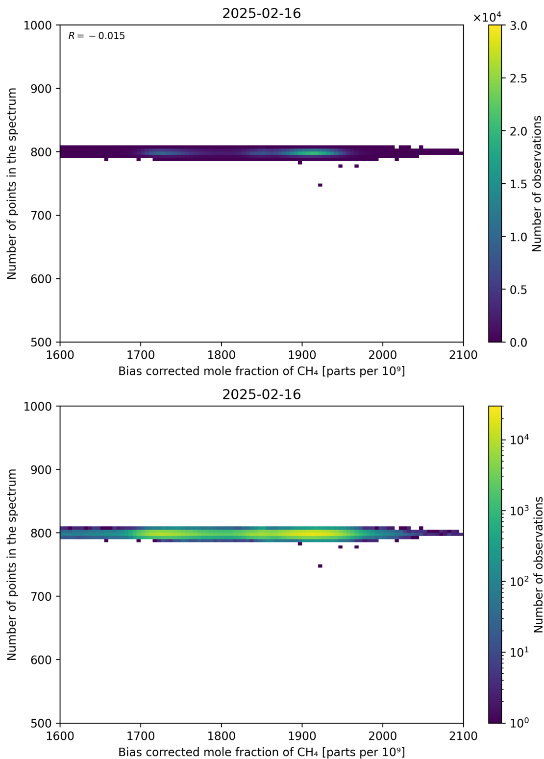
Figure 68: Scatter density plot of “Bias corrected mole fraction of CH 4 ” against “Number of points in the spectrum” for 2025-02-15 to 2025-02-17.
