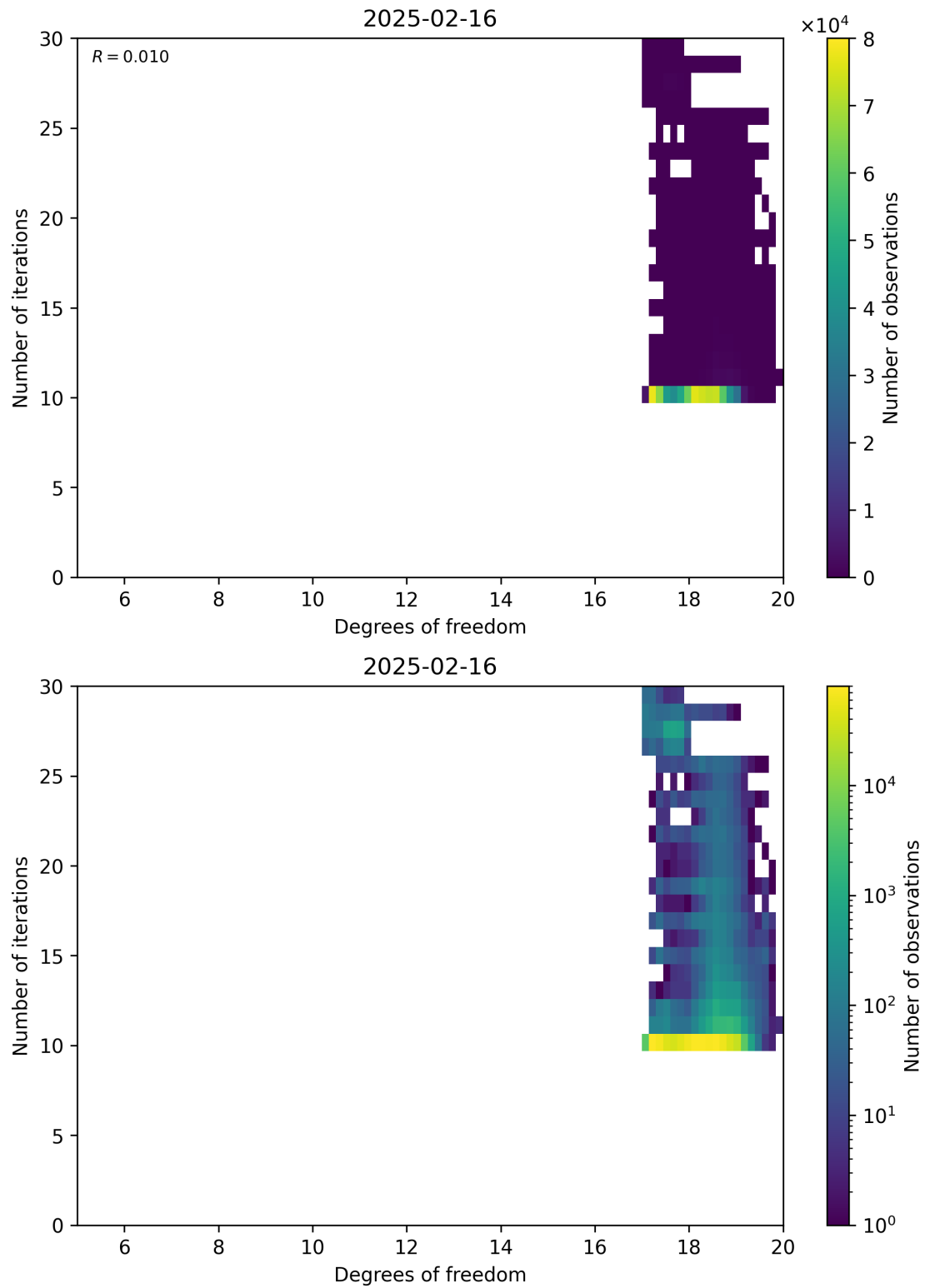
Figure 52: Scatter density plot of “Degrees of freedom” against “Number of iterations” for 2025-02-15 to 2025-02-17.
