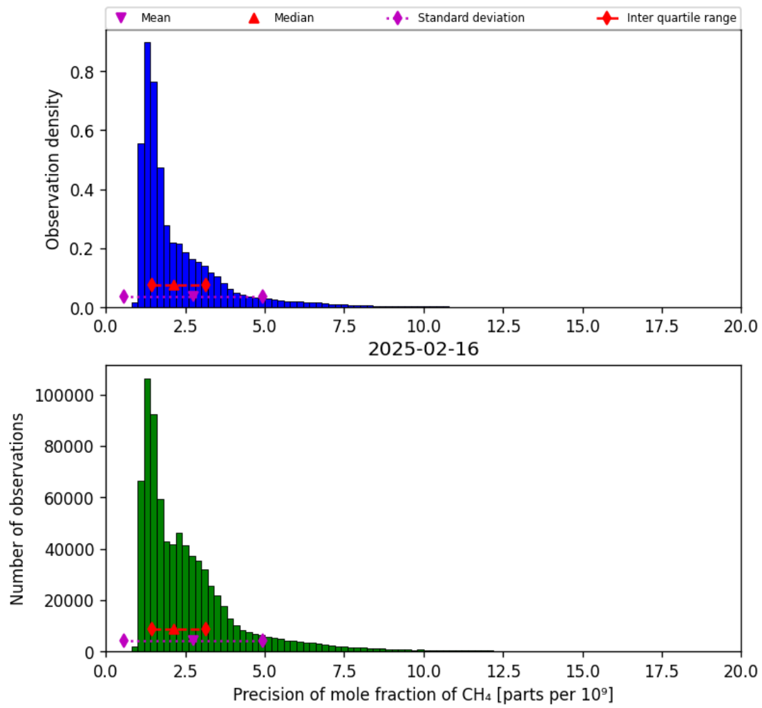
Figure 24: Histogram of “Precision of mole fraction of CH 4 ” for 2025-02-15 to 2025-02-17
