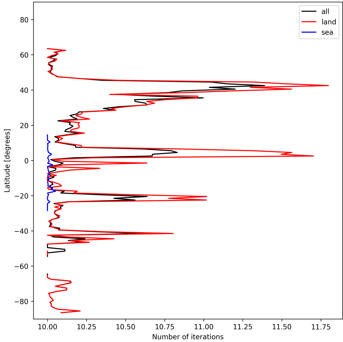
Figure 20: Zonal average of “Number of iterations” for 2025-02-15 to 2025-02-17.
