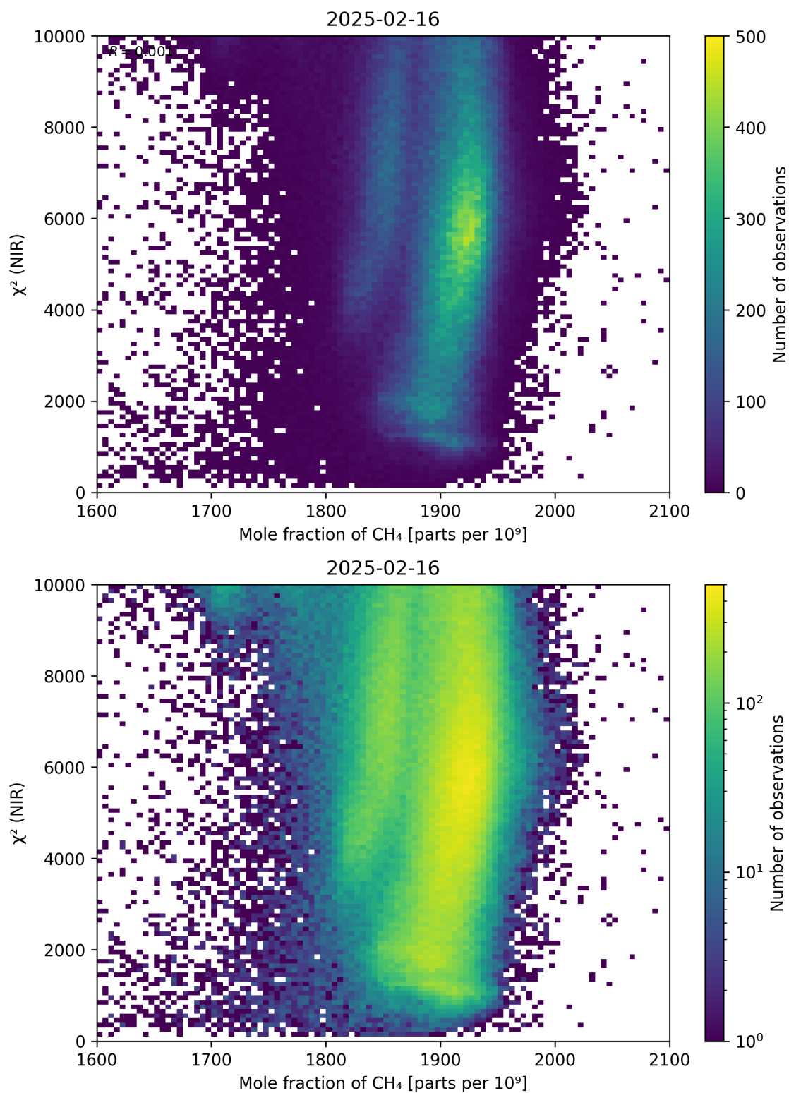
Figure 70: Scatter density plot of “Mole fraction of CH 4 ” against “ \chi^2 (NIR)” for 2025-02-15 to 2025-02-17.
