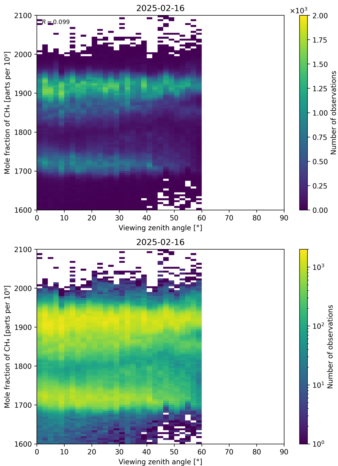
Figure 110: Scatter density plot of “Viewing zenith angle” against “Mole fraction of CH 4 ” for 2025-02-15 to 2025-02-17.
