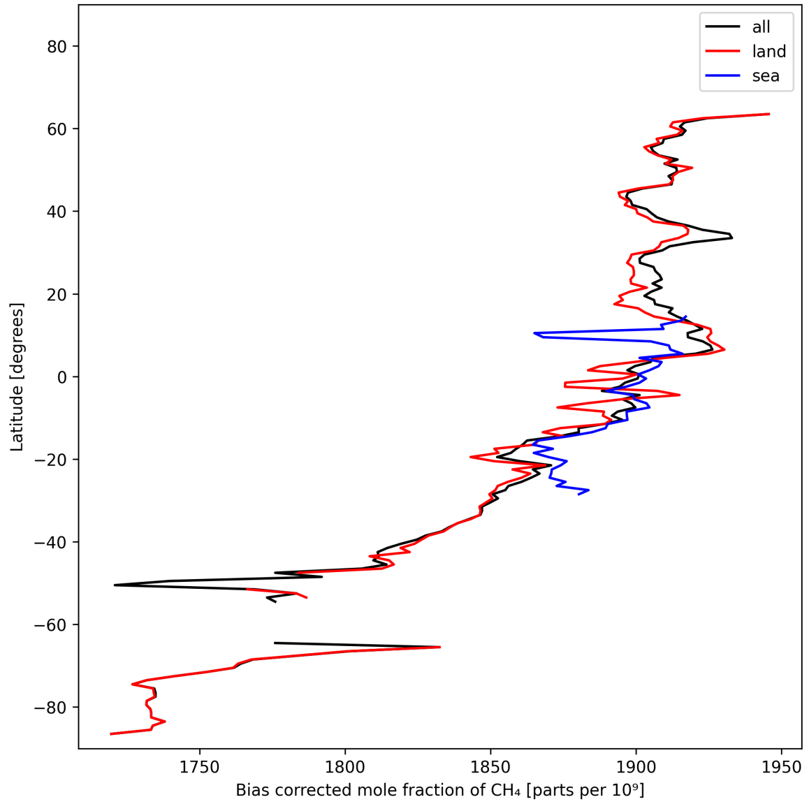
Figure 14: Zonal average of “Bias corrected mole fraction of CH 4 ” for 2025-02-15 to 2025-02-17.
