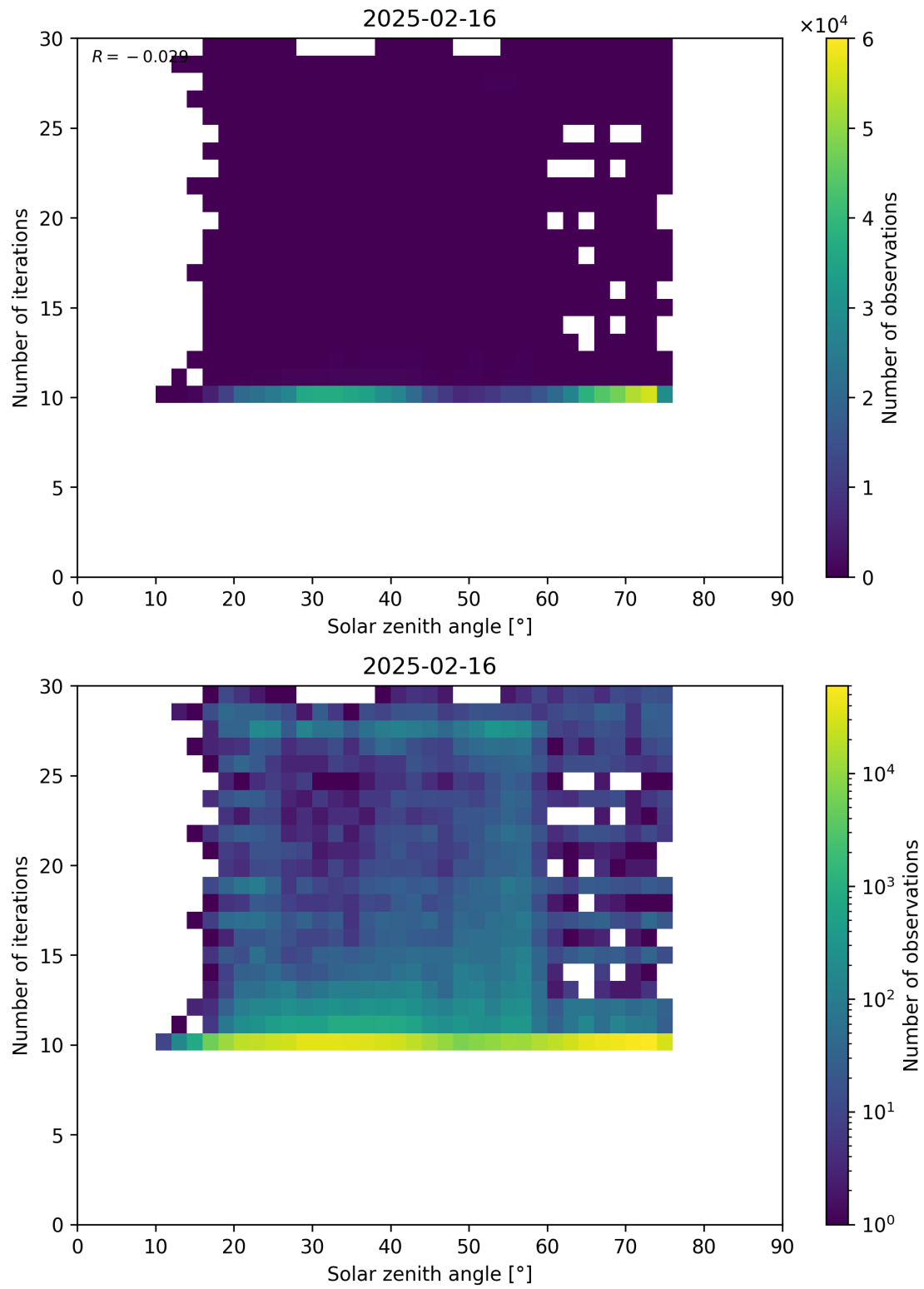
Figure 102: Scatter density plot of “Solar zenith angle” against “Number of iterations” for 2025-02-15 to 2025-02-17.
