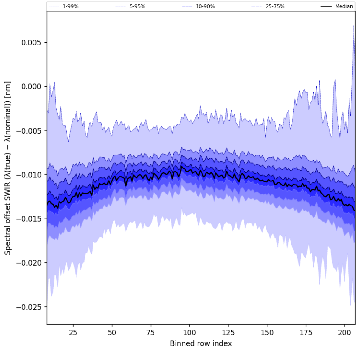
Figure 38: Along track statistics of “Spectral offset SWIR ( \lambda_{\text{true}} - \lambda_{\text{nominal}} )” for 2025-02-15 to 2025-02-17
