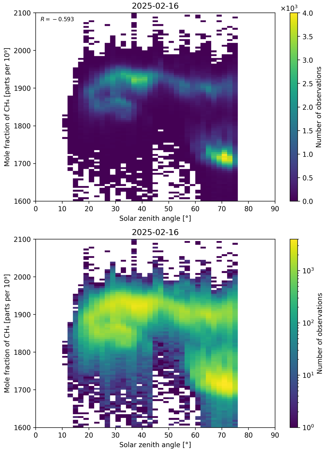
Figure 99: Scatter density plot of “Solar zenith angle” against “Mole fraction of CH 4 ” for 2025-02-15 to 2025-02-17.
