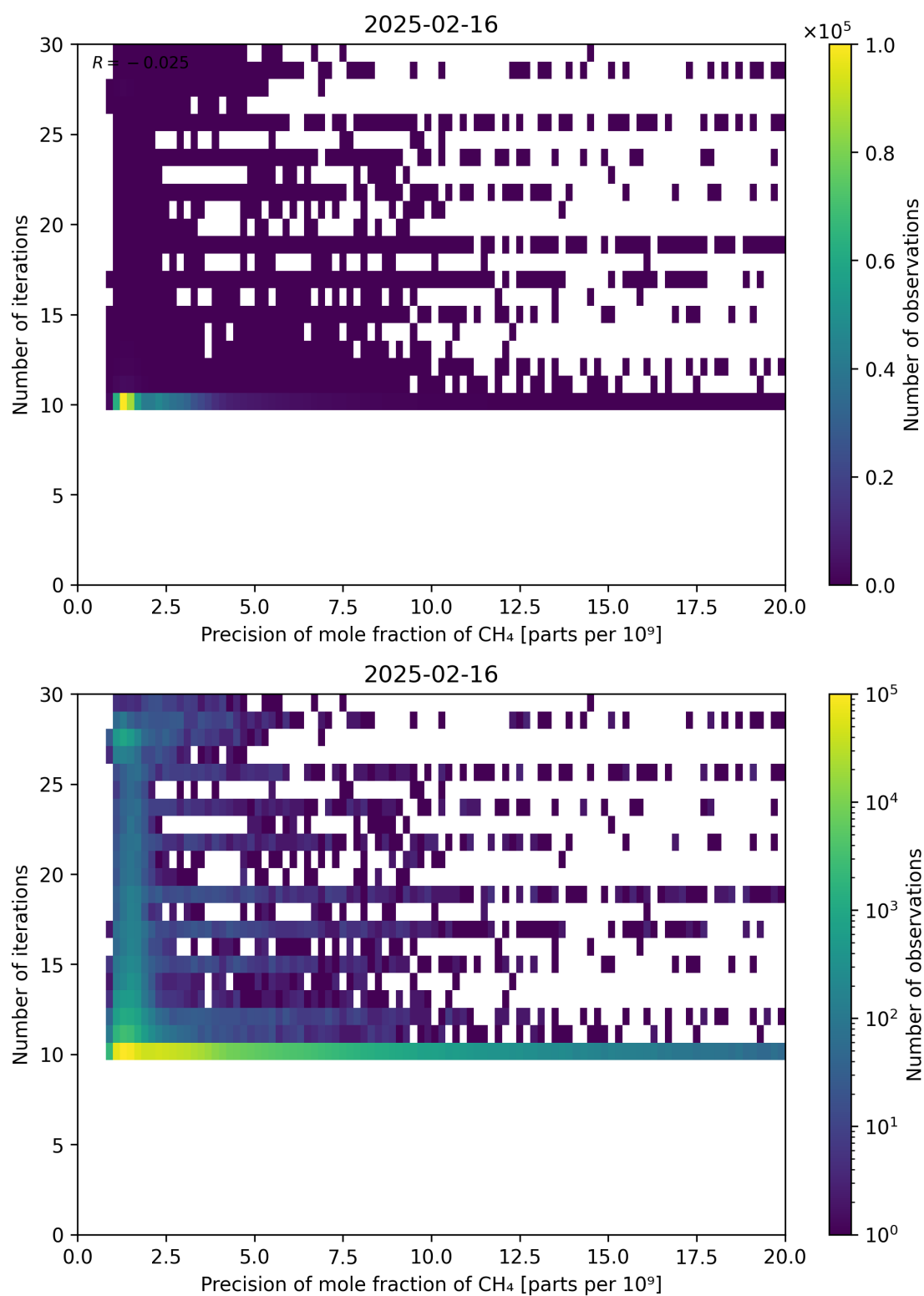
Figure 83: Scatter density plot of “Precision of mole fraction of CH 4 ” against “Number of iterations” for 2025-02-15 to 2025-02-17.
