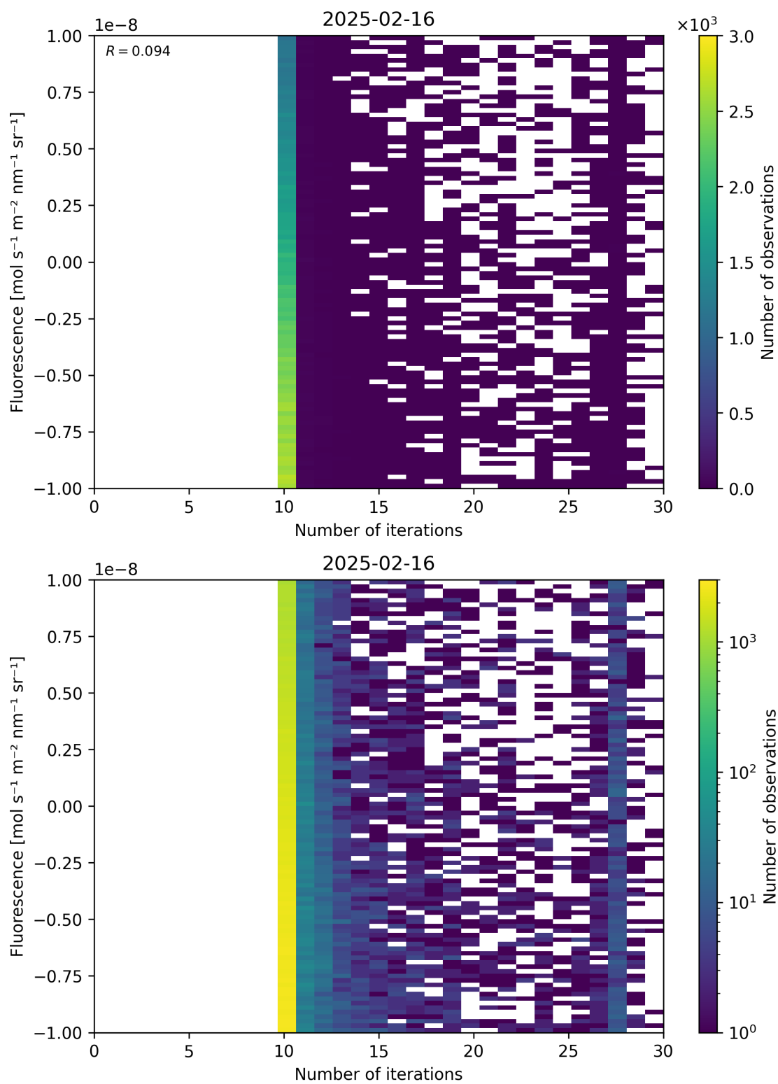
Figure 87: Scatter density plot of “Number of iterations” against “Fluorescence” for 2025-02-15 to 2025-02-17.
