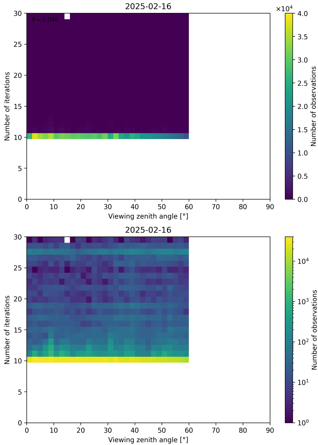
Figure 113: Scatter density plot of “Viewing zenith angle” against “Number of iterations” for 2025-02-15 to 2025-02-17.
