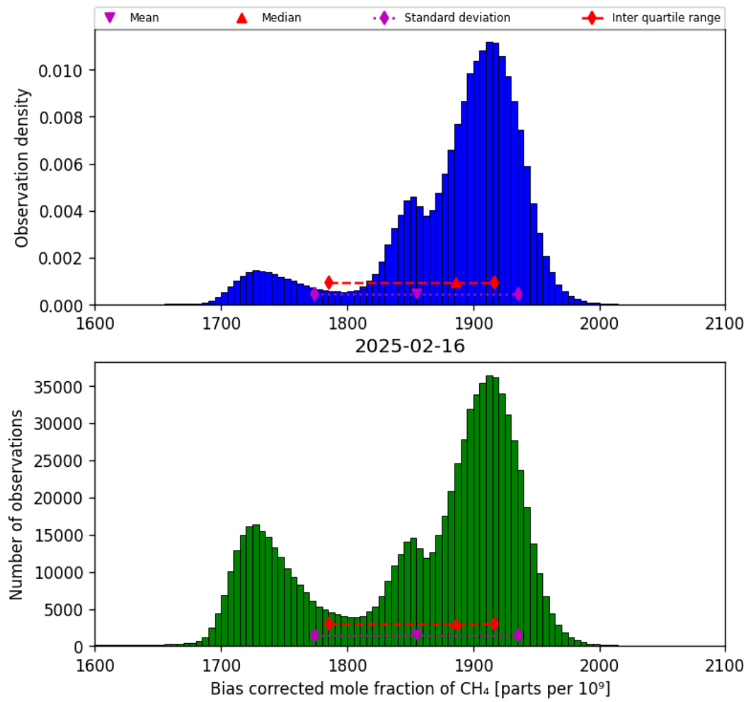
Figure 25: Histogram of “Bias corrected mole fraction of CH 4 ” for 2025-02-15 to 2025-02-17
