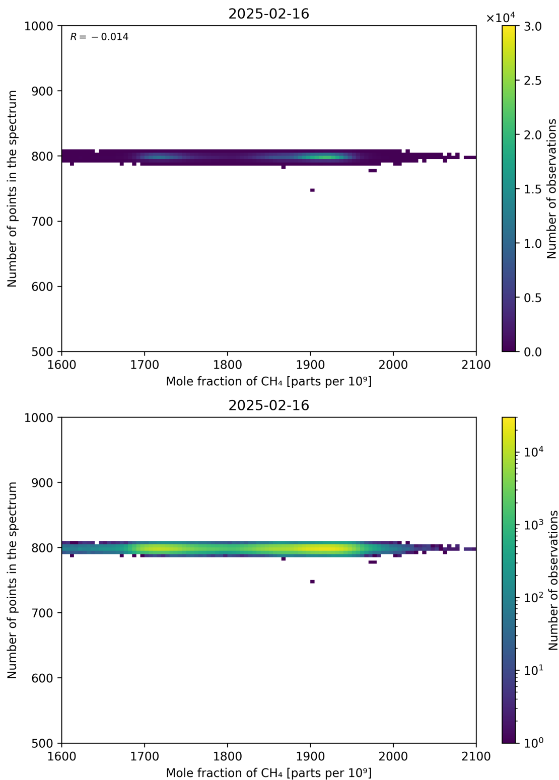
Figure 77: Scatter density plot of “Mole fraction of CH 4 ” against “Number of points in the spectrum” for 2025-02-15 to 2025-02-17.
