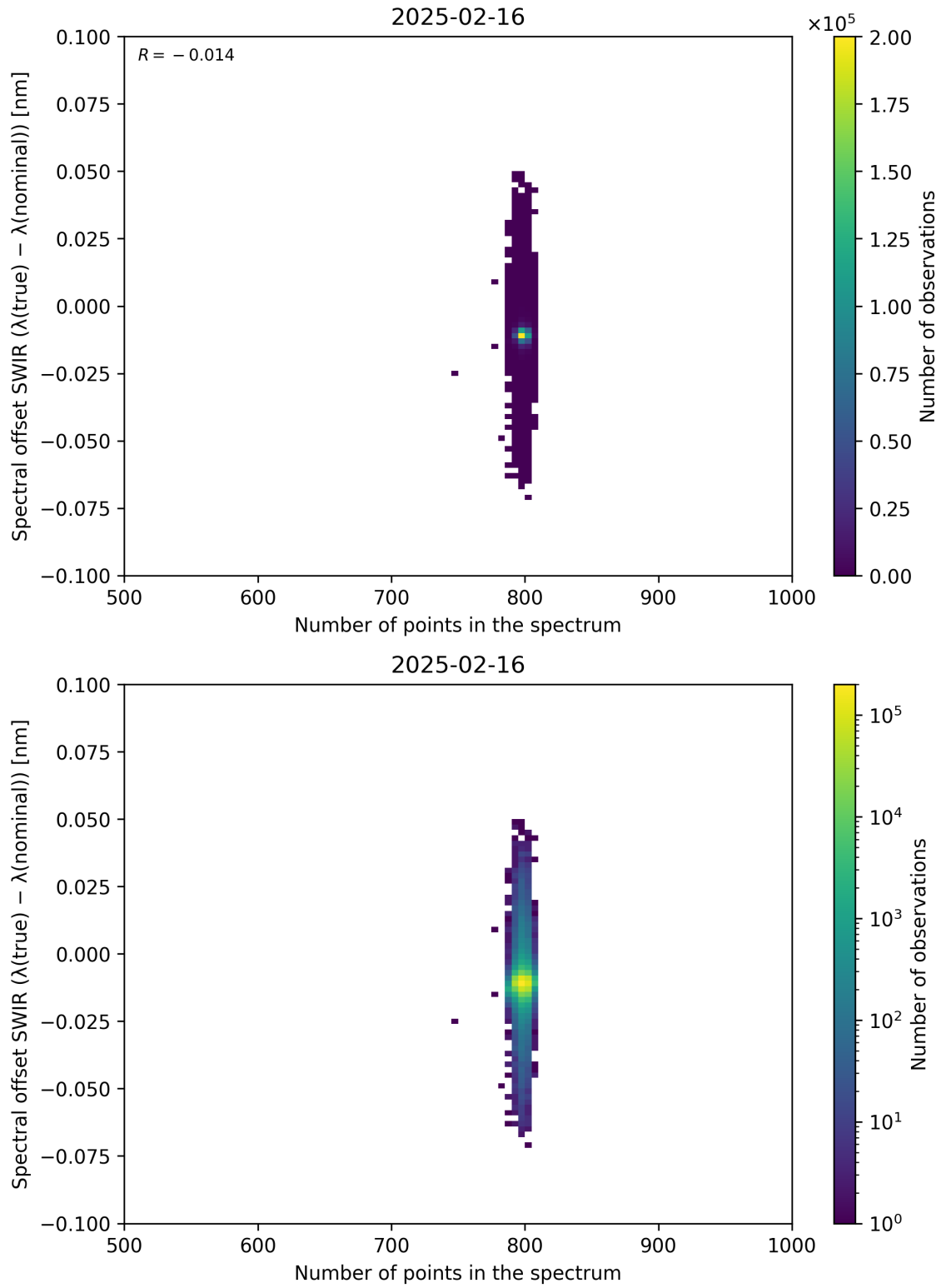
Figure 93: Scatter density plot of “Number of points in the spectrum” against “Spectral offset SWIR ( \lambda_{\text{true}} - \lambda_{\text{nominal}} )” for 2025-02-15 to 2025-02-17.
