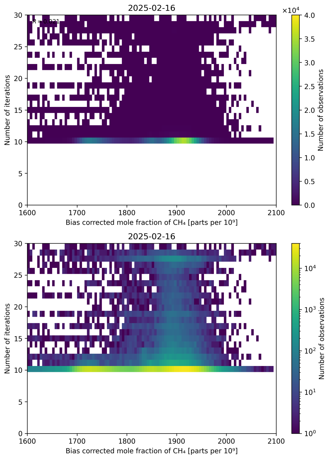
Figure 67: Scatter density plot of “Bias corrected mole fraction of \text{CH}_4 ” against “Number of iterations” for 2025-02-15 to 2025-02-17.
