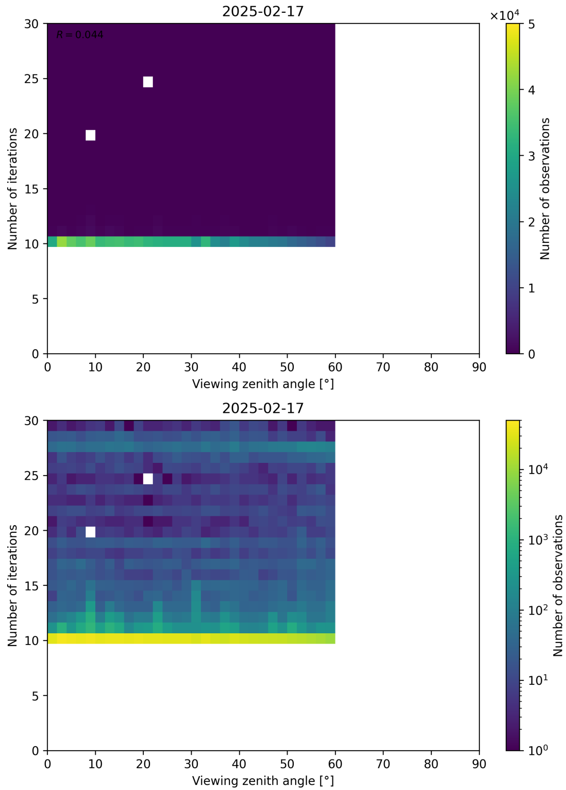
Figure 113: Scatter density plot of “Viewing zenith angle” against “Number of iterations” for 2025-02-16 to 2025-02-18.
