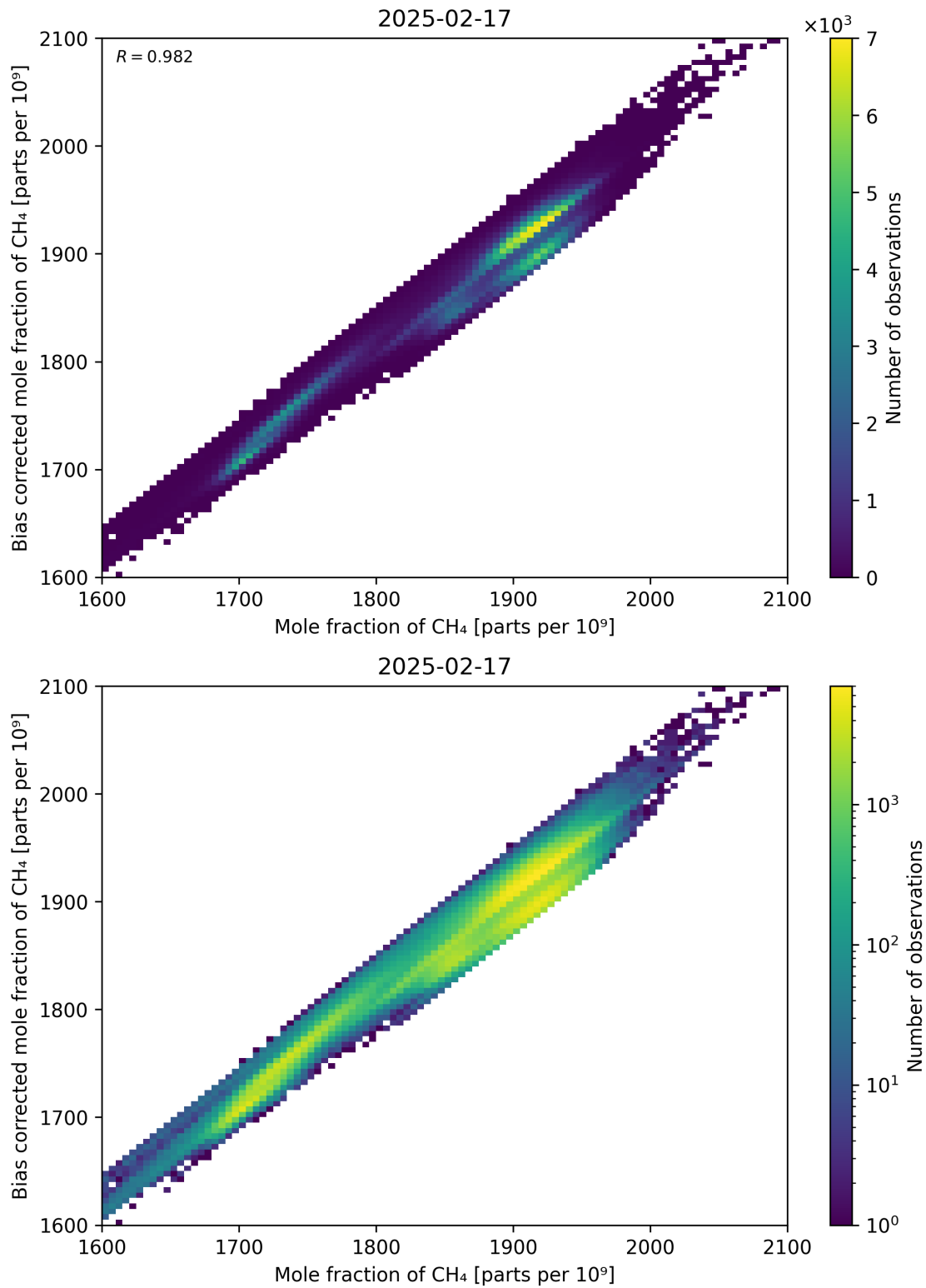
Figure 74: Scatter density plot of “Mole fraction of CH 4 ” against “Bias corrected mole fraction of CH 4 ” for 2025-02-16 to 2025-02-18.
