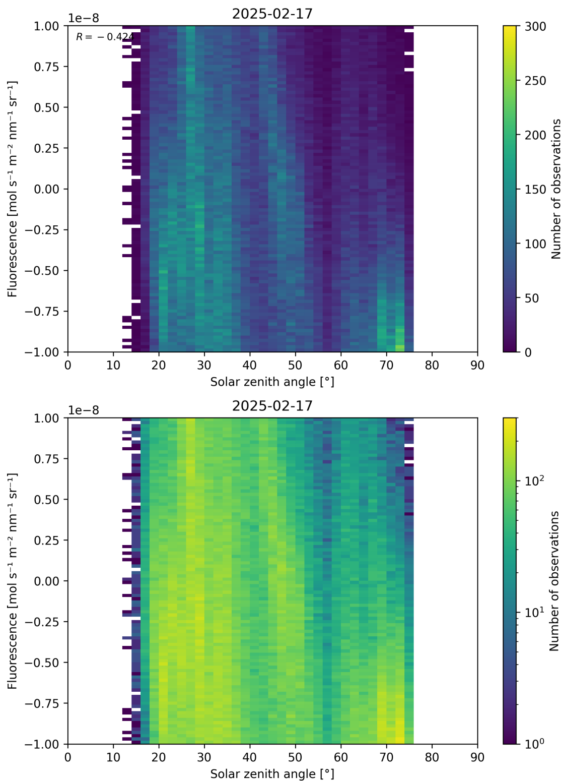
Figure 97: Scatter density plot of “Solar zenith angle” against “Fluorescence” for 2025-02-16 to 2025-02-18.
