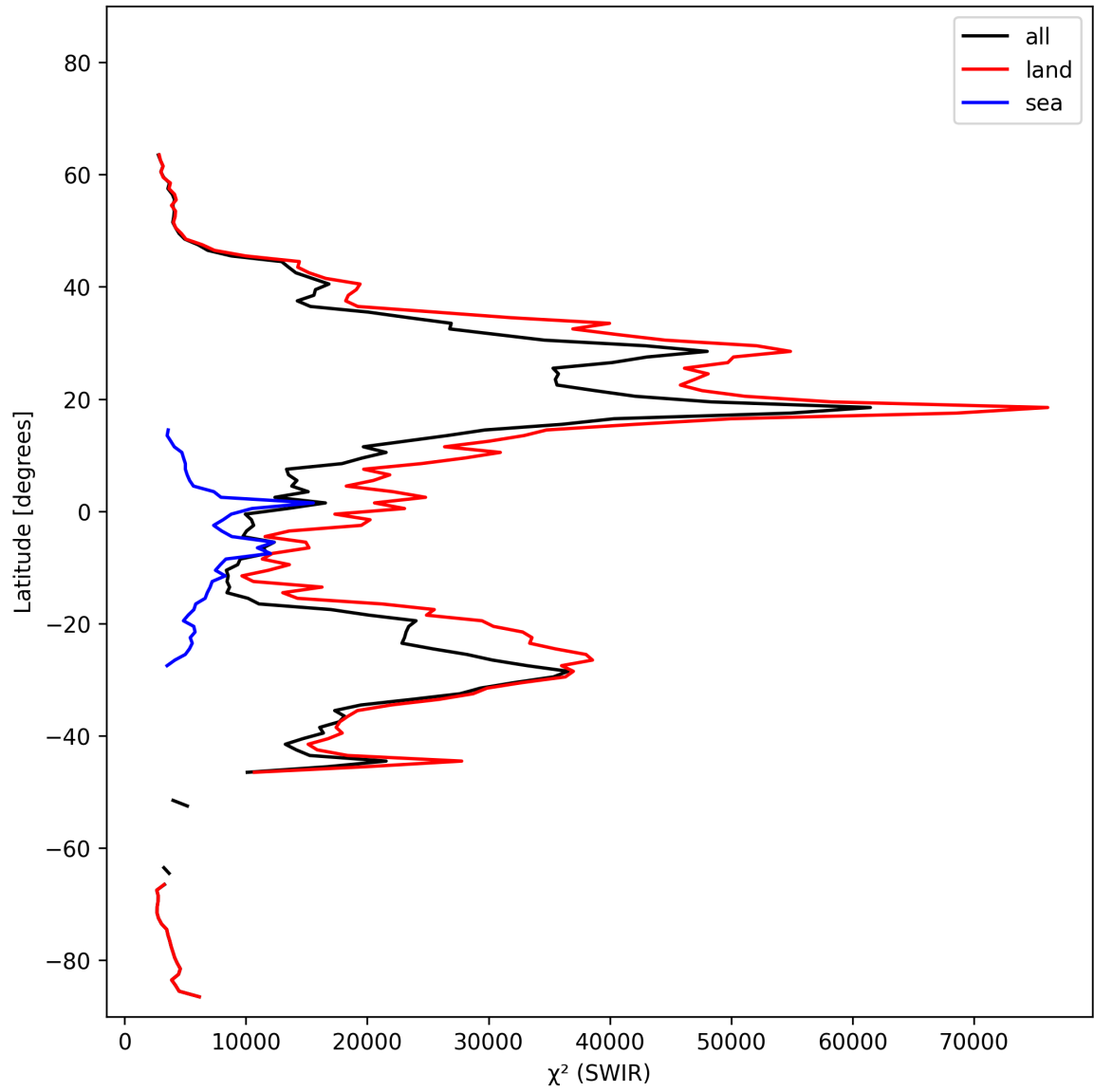
Figure 17: Zonal average of “ \chi^2 (SWIR)” for 2025-02-16 to 2025-02-18.
