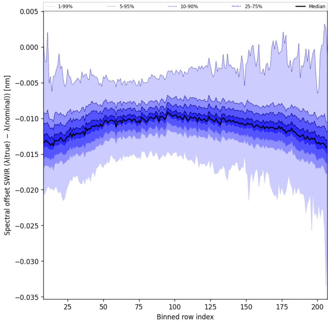
Figure 38: Along track statistics of “Spectral offset SWIR ( \lambda_{\text{true}} - \lambda_{\text{nominal}} )” for 2025-02-16 to 2025-02-18
