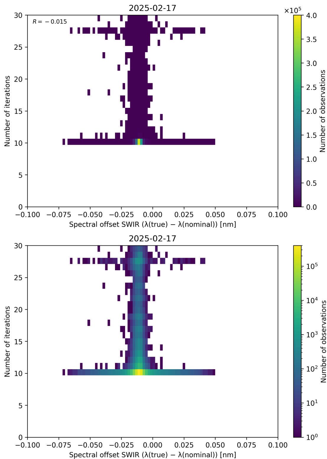
Figure 121: Scatter density plot of “Spectral offset SWIR ( \lambda_{\text{true}} - \lambda_{\text{nominal}} )” against “Number of iterations” for 2025-02-16 to 2025-02-18.
