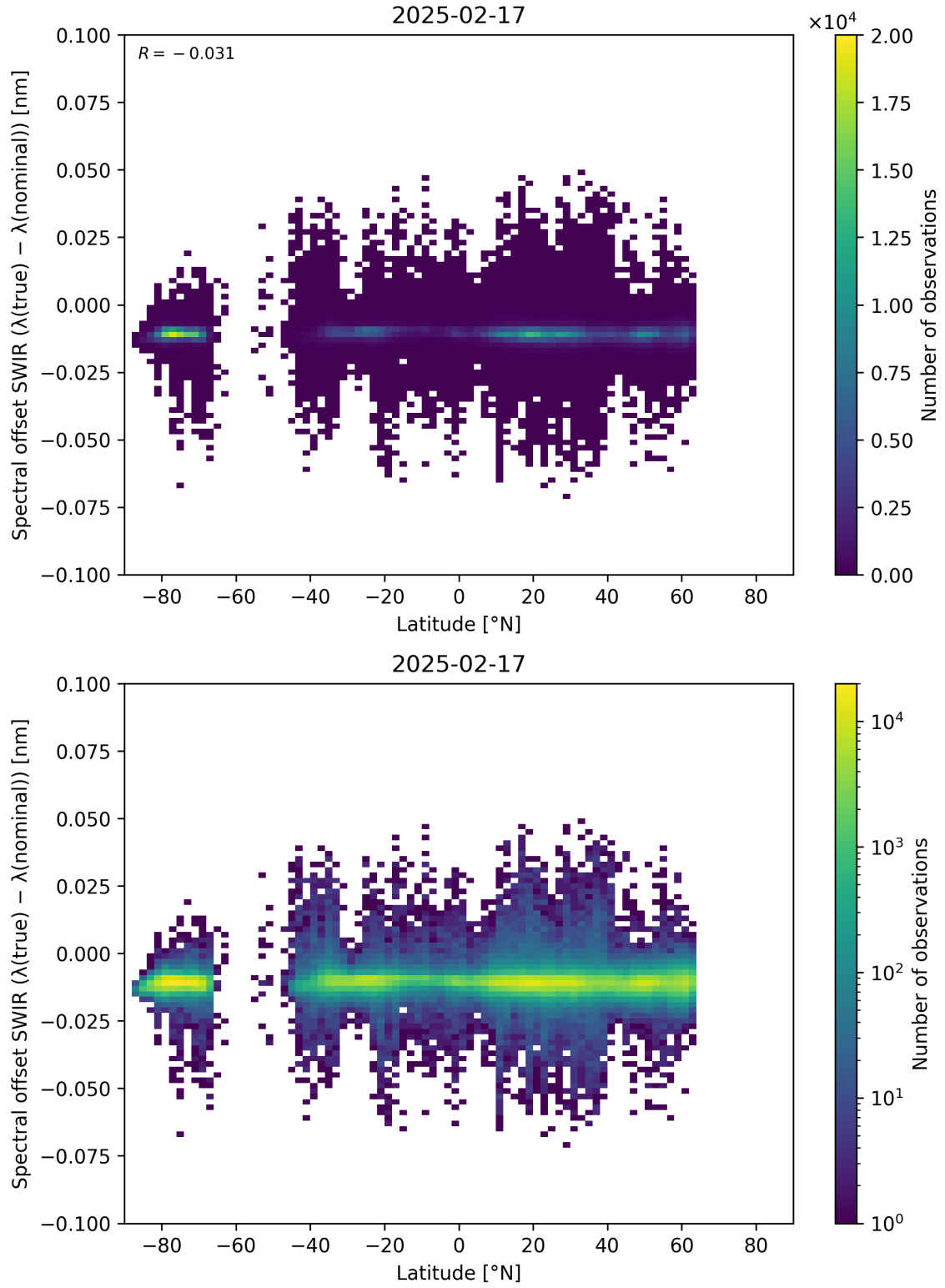
Figure 62: Scatter density plot of “Latitude” against “Spectral offset SWIR ( \lambda_{\text{true}} - \lambda_{\text{nominal}} )” for 2025-02-16 to 2025-02-18.
