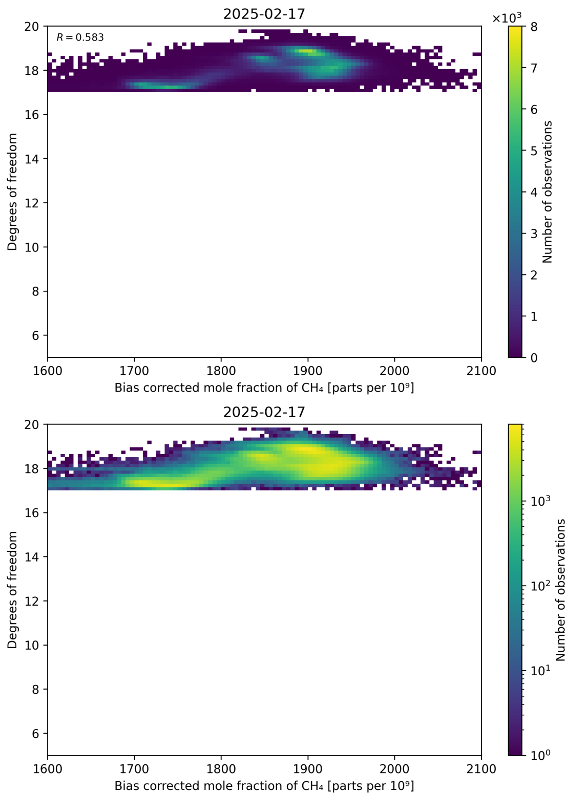
Figure 65: Scatter density plot of “Bias corrected mole fraction of CH 4 ” against “Degrees of freedom” for 2025-02-16 to 2025-02-18.
