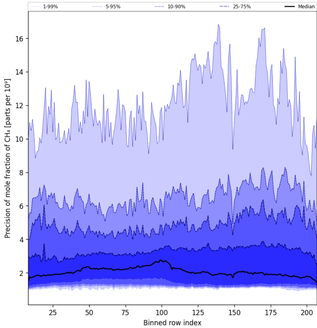
Figure 35: Along track statistics of “Precision of mole fraction of CH 4 ” for 2025-02-16 to 2025-02-18
