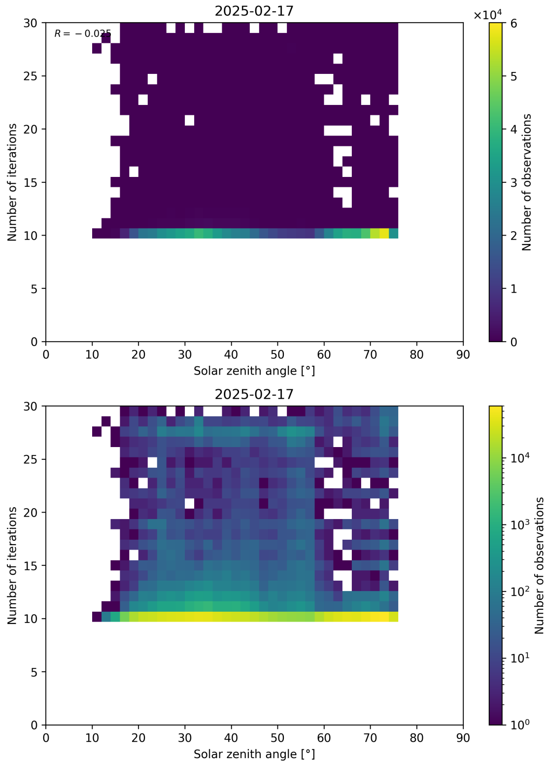
Figure 102: Scatter density plot of “Solar zenith angle” against “Number of iterations” for 2025-02-16 to 2025-02-18.
