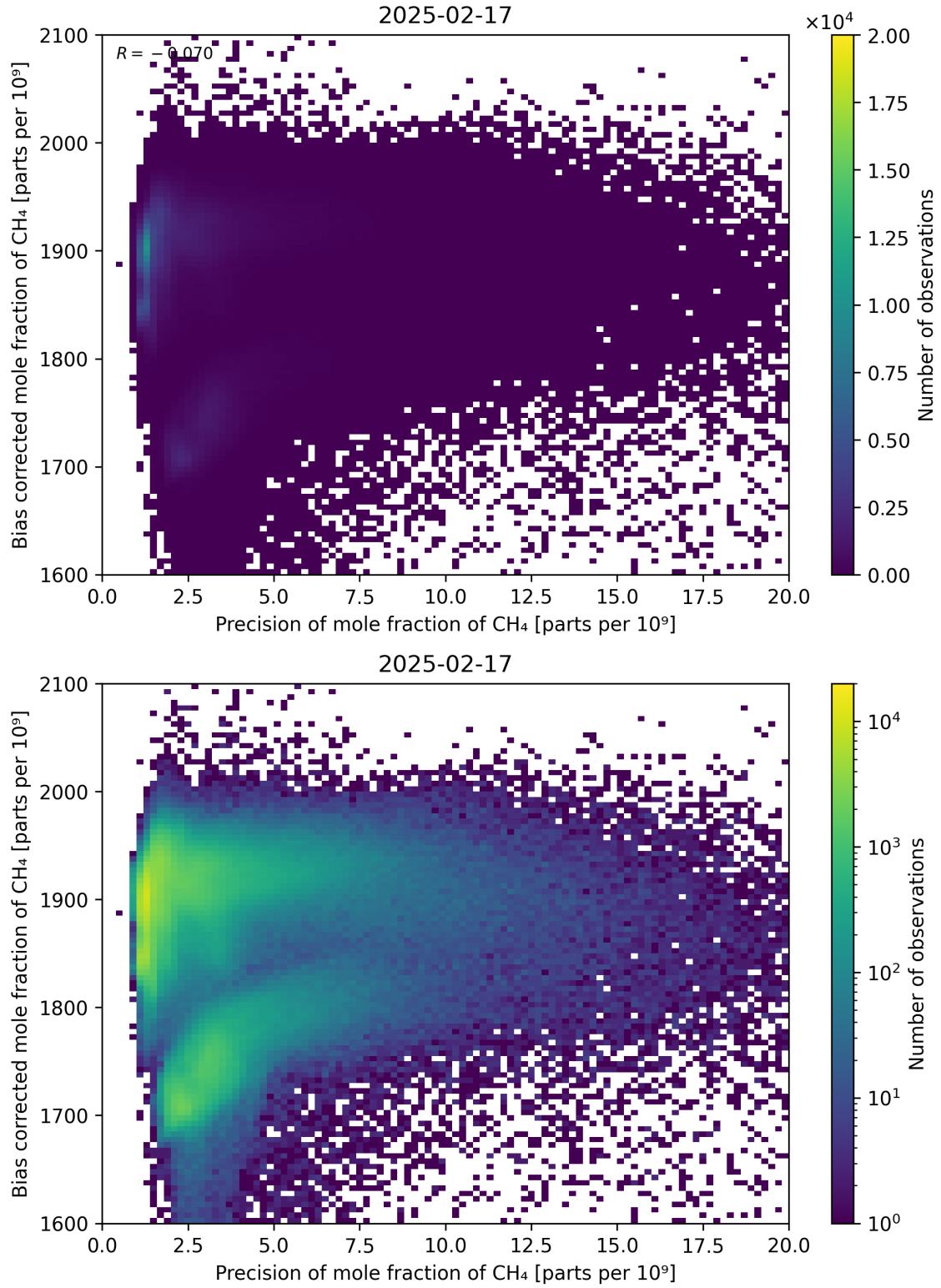
Figure 82: Scatter density plot of “Precision of mole fraction of CH 4 ” against “Bias corrected mole fraction of CH 4 ” for 2025-02-16 to 2025-02-18.
