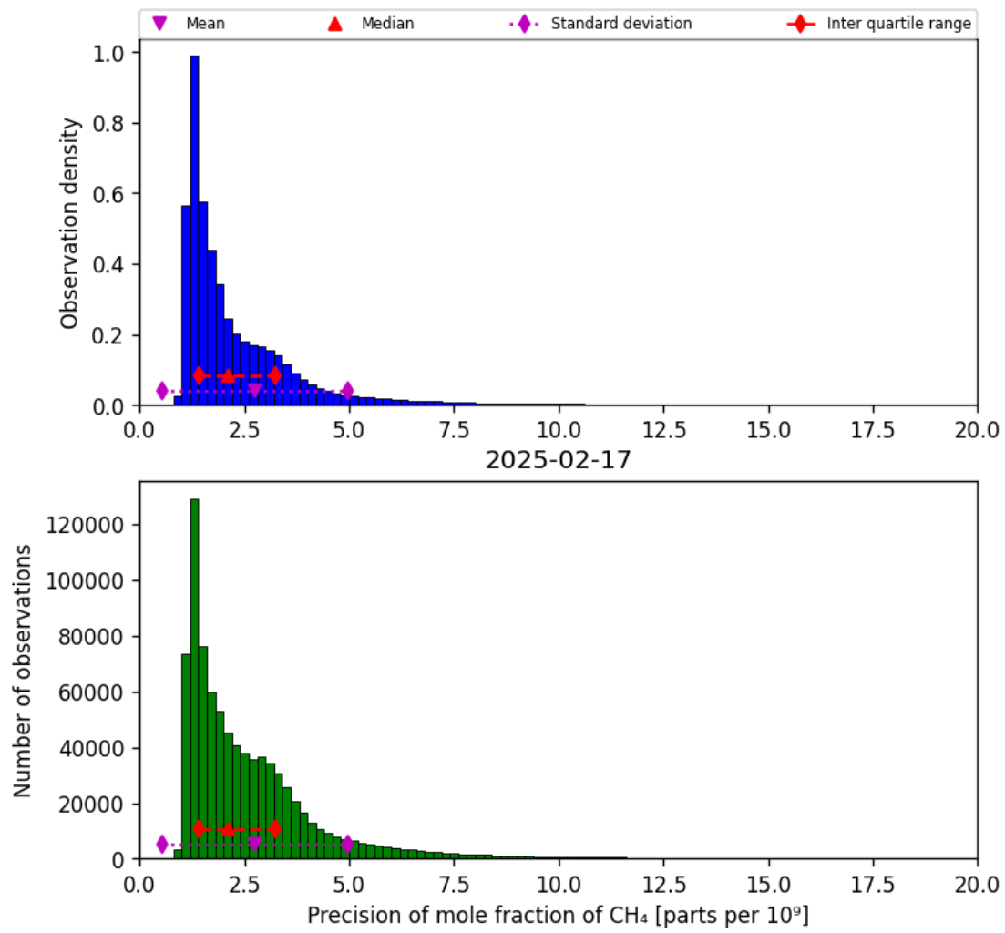
Figure 24: Histogram of “Precision of mole fraction of CH 4 ” for 2025-02-16 to 2025-02-18
