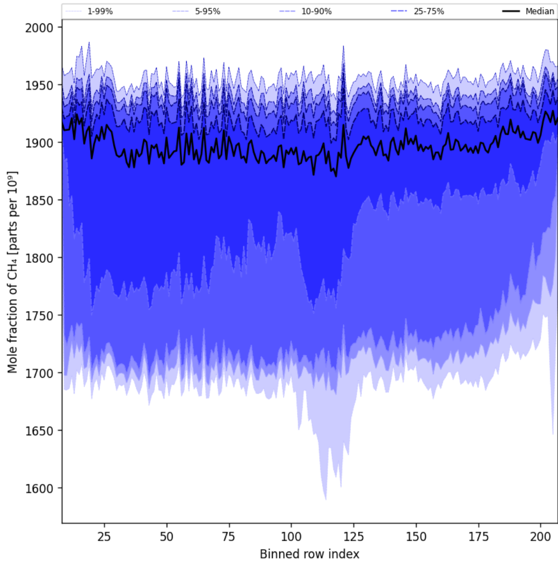
Figure 34: Along track statistics of “Mole fraction of CH 4 ” for 2025-02-16 to 2025-02-18
