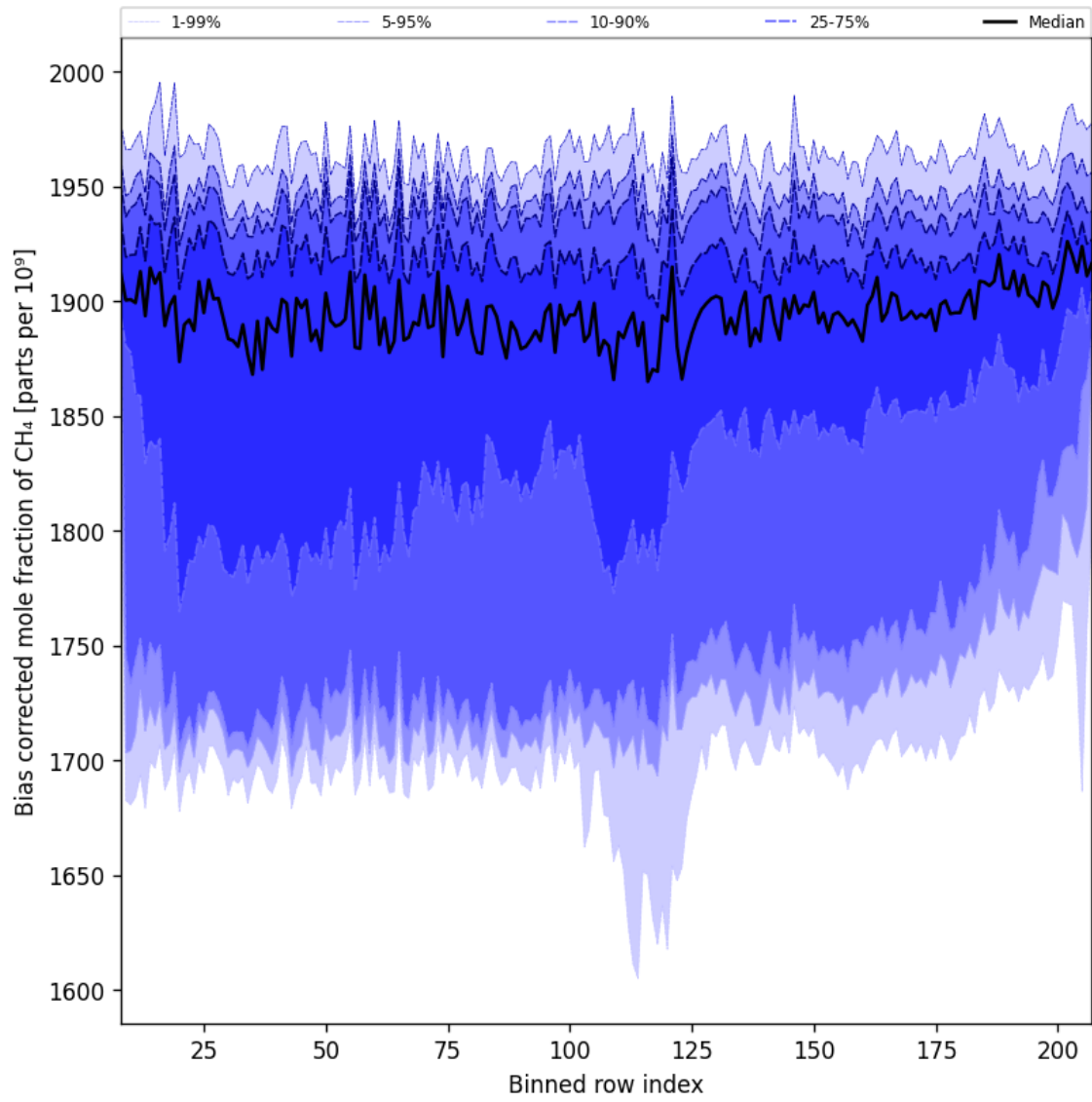
Figure 36: Along track statistics of “Bias corrected mole fraction of CH 4 ” for 2025-02-16 to 2025-02-18
