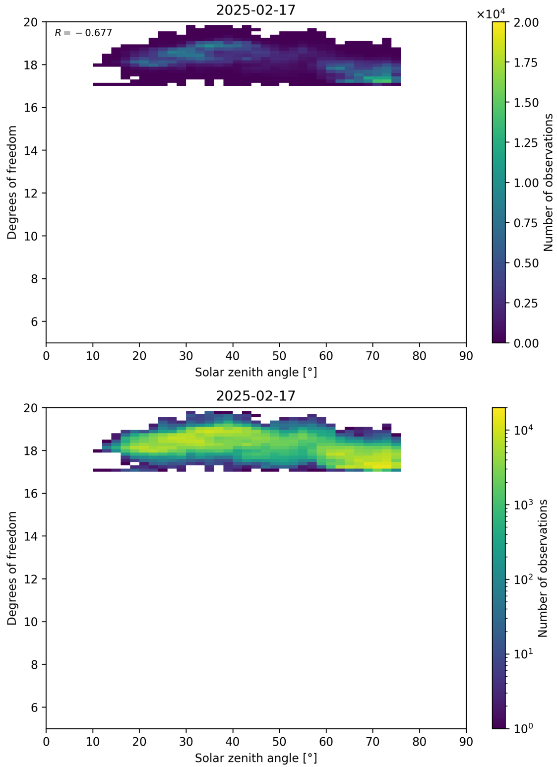
Figure 96: Scatter density plot of “Solar zenith angle” against “Degrees of freedom” for 2025-02-16 to 2025-02-18.
