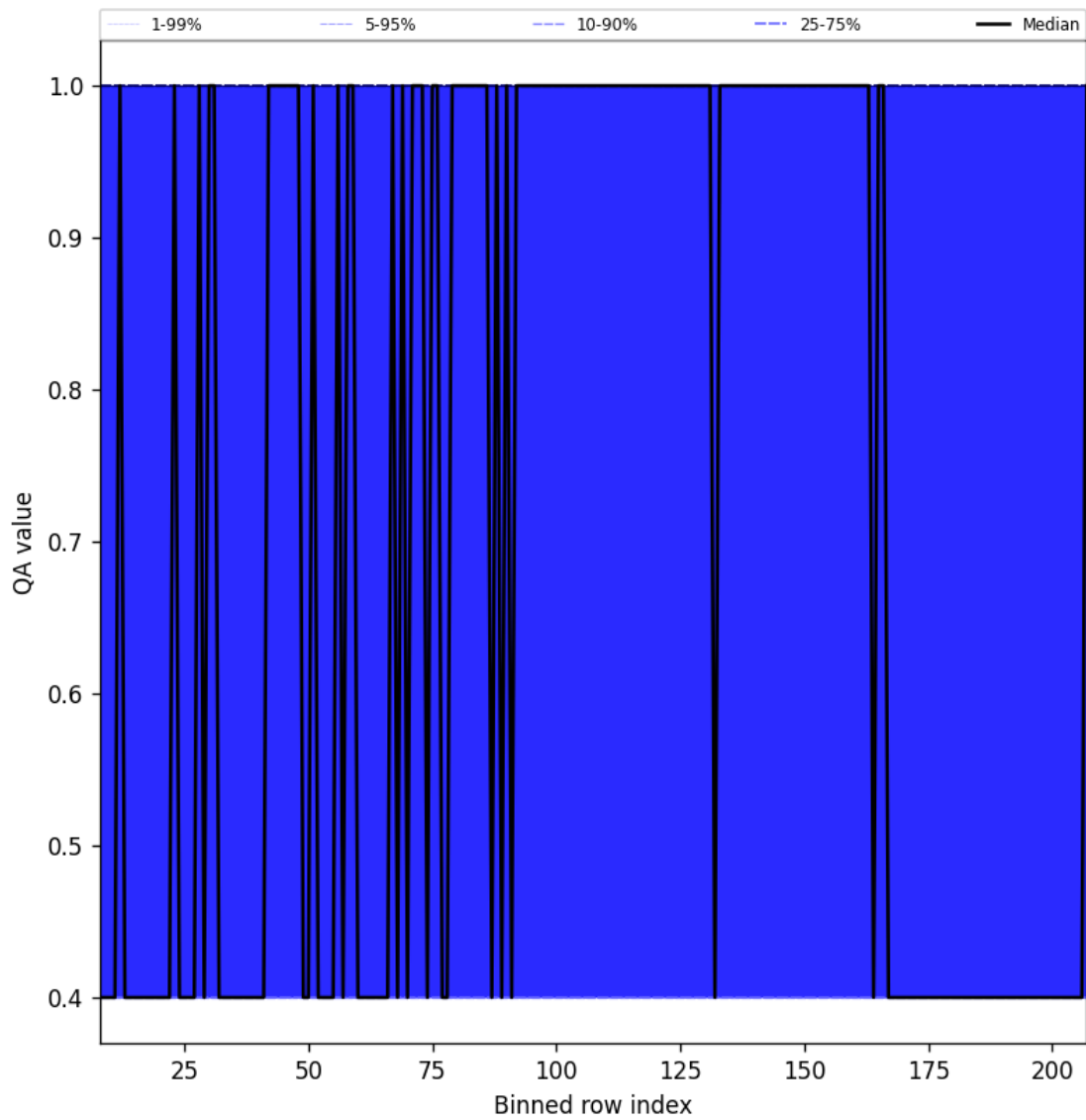
Figure 33: Along track statistics of “QA value” for 2025-02-16 to 2025-02-18
