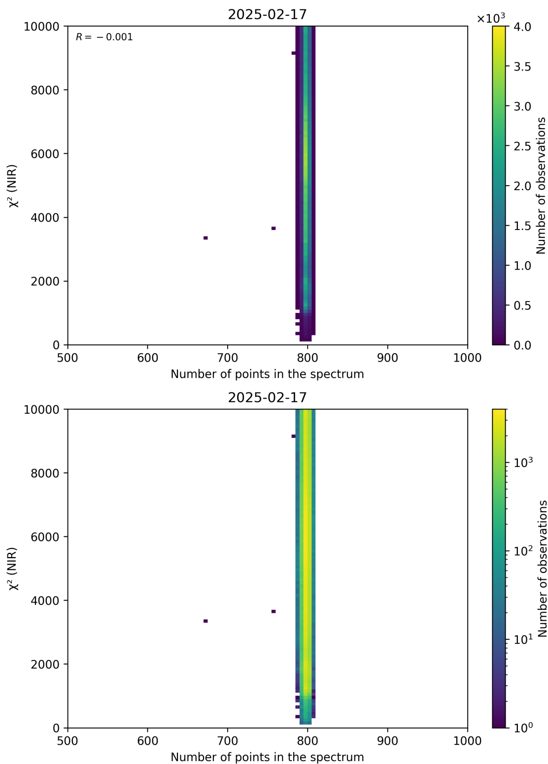
Figure 88: Scatter density plot of “Number of points in the spectrum” against “ \chi^2 (NIR)” for 2025-02-16 to 2025-02-18.
