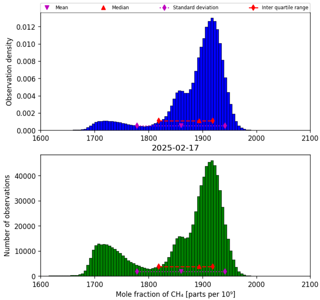
Figure 23: Histogram of “Mole fraction of CH 4 ” for 2025-02-16 to 2025-02-18
