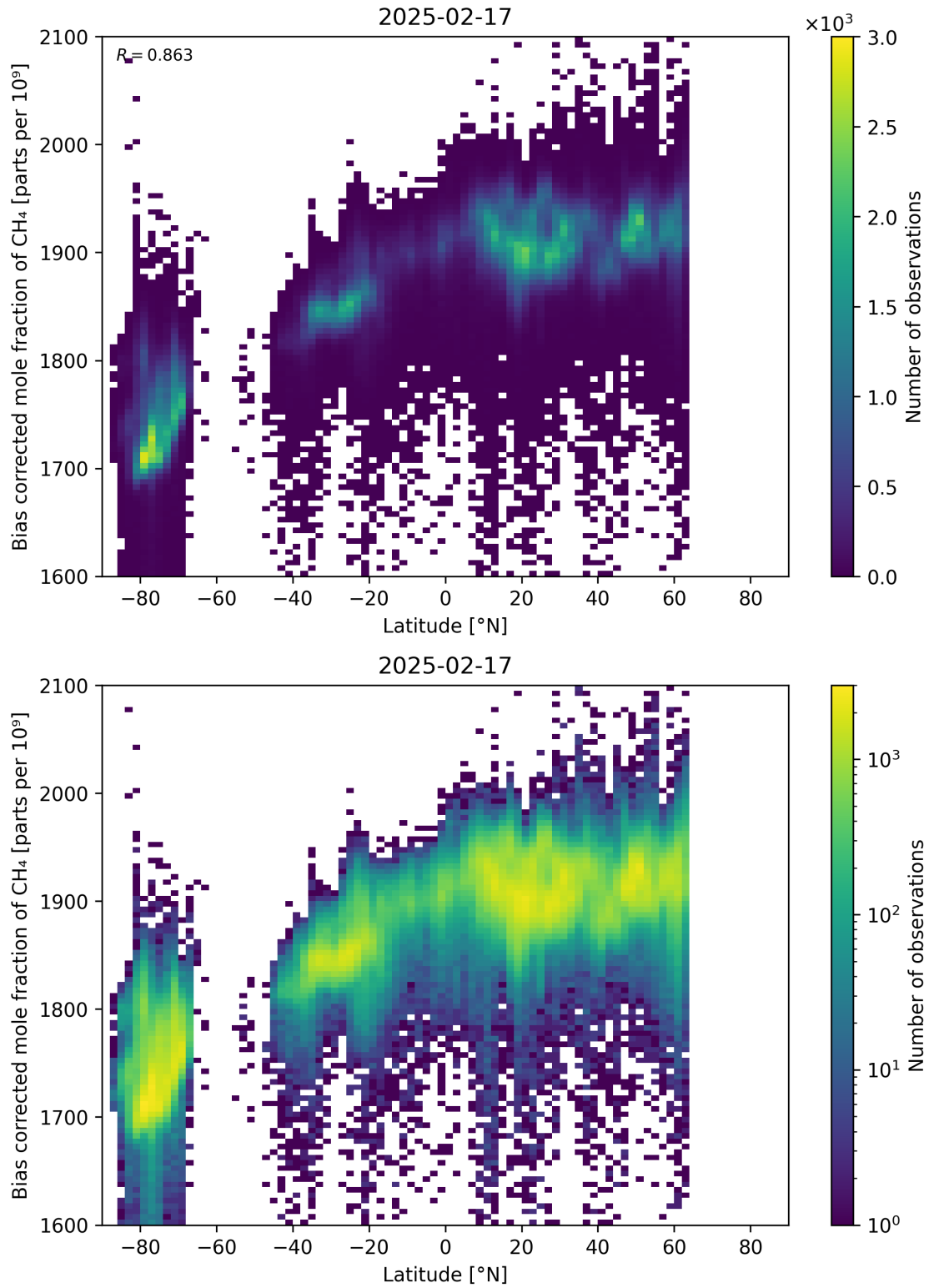
Figure 58: Scatter density plot of “Latitude” against “Bias corrected mole fraction of CH 4 ” for 2025-02-16 to 2025-02-18.
