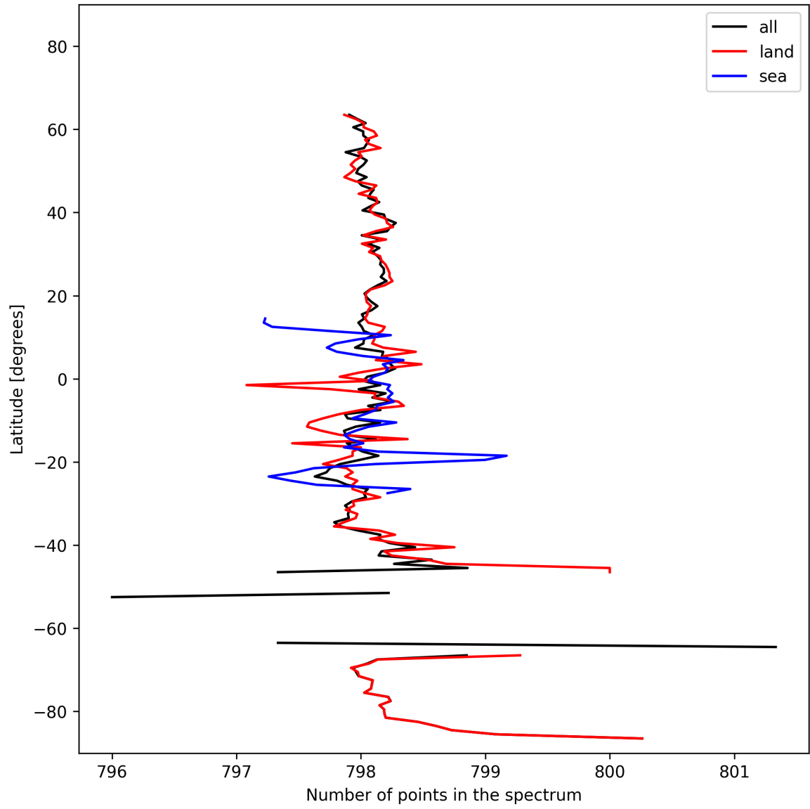
Figure 15: Zonal average of “Number of points in the spectrum” for 2025-02-16 to 2025-02-18.
