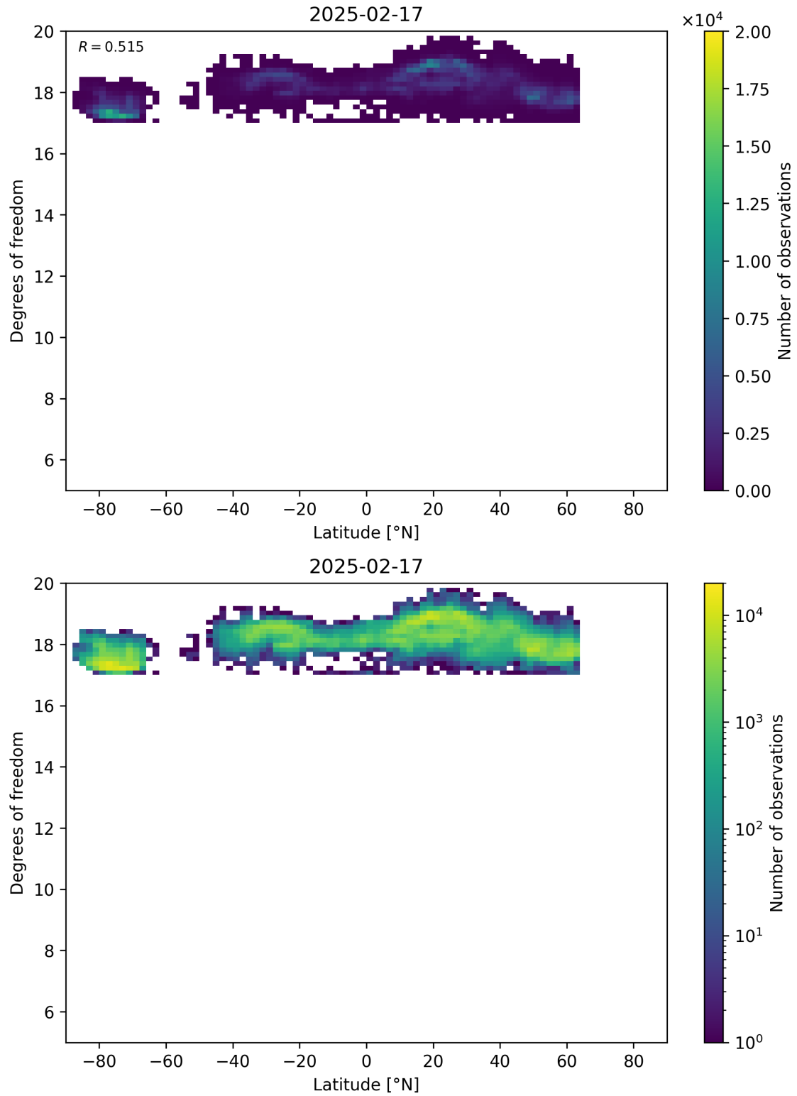
Figure 55: Scatter density plot of “Latitude” against “Degrees of freedom” for 2025-02-16 to 2025-02-18.
