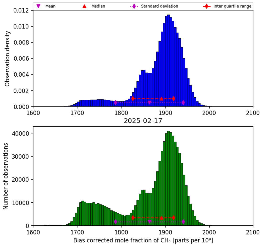
Figure 25: Histogram of “Bias corrected mole fraction of CH 4 ” for 2025-02-16 to 2025-02-18
