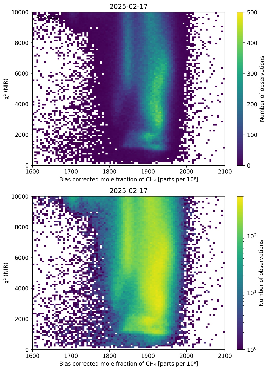
Figure 63: Scatter density plot of “Bias corrected mole fraction of \text{CH}_4 ” against “ \chi^2 (NIR)” for 2025-02-16 to 2025-02-18.
