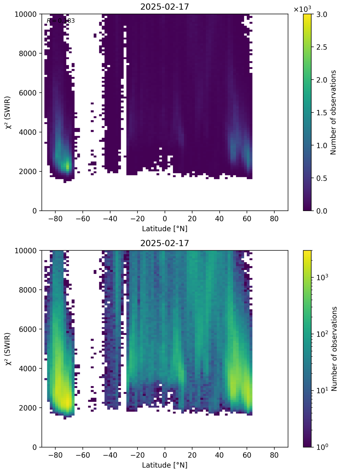
Figure 54: Scatter density plot of “Latitude” against “ \chi^2 (SWIR)” for 2025-02-16 to 2025-02-18.
