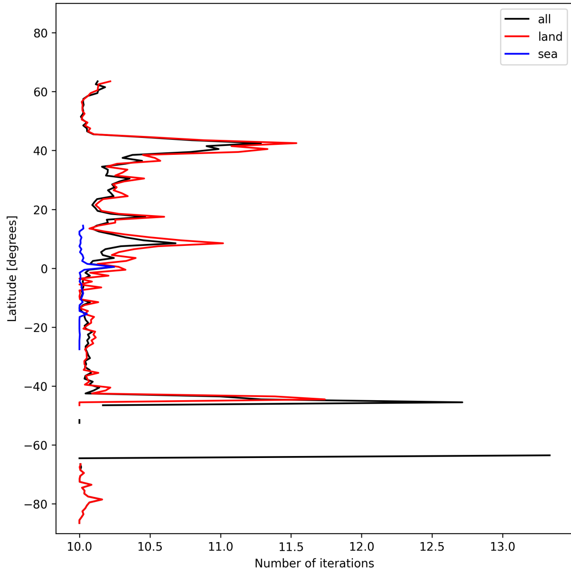
Figure 20: Zonal average of “Number of iterations” for 2025-02-16 to 2025-02-18.
