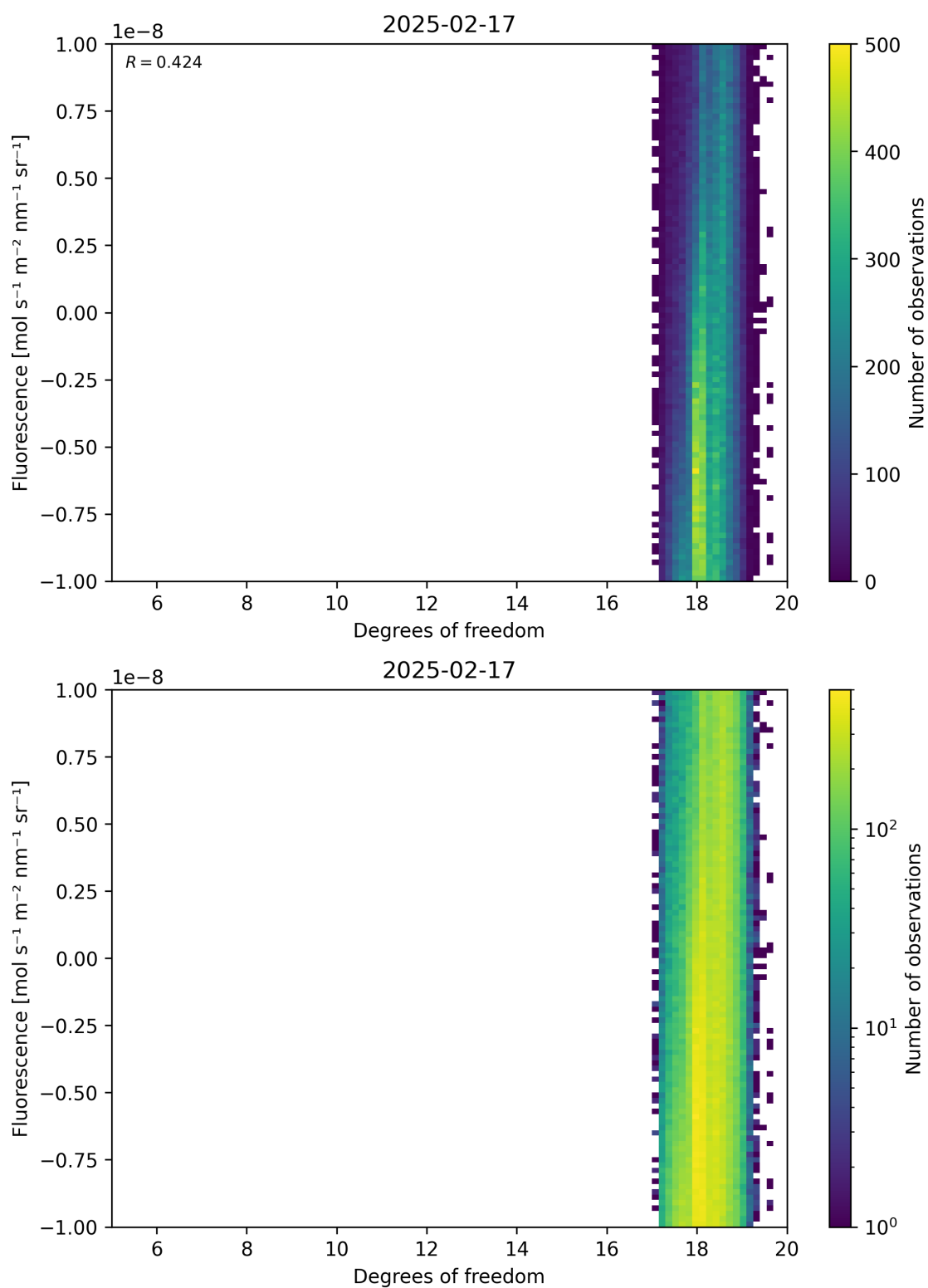
Figure 51: Scatter density plot of “Degrees of freedom” against “Fluorescence” for 2025-02-16 to 2025-02-18.
