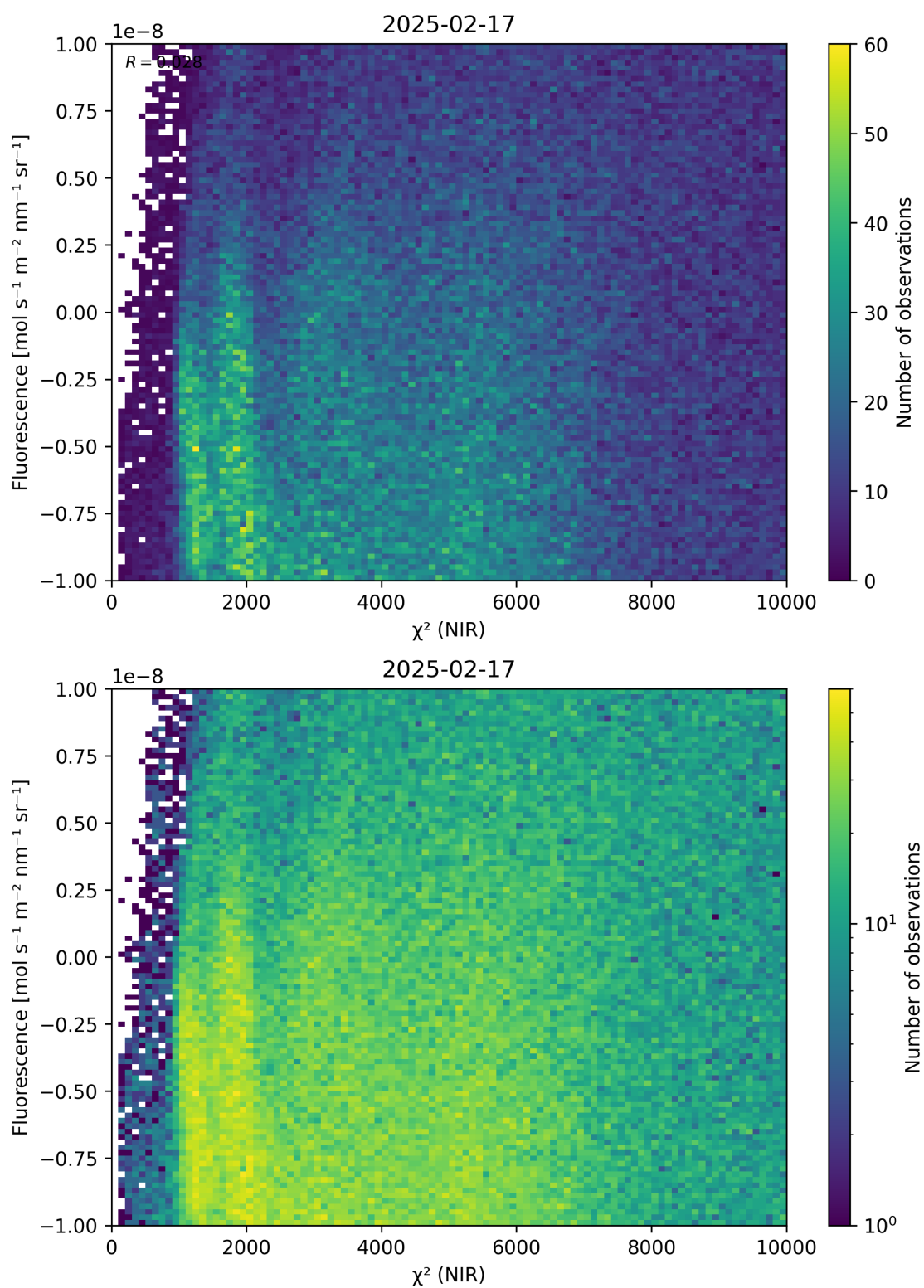
Figure 45: Scatter density plot of “ \chi^2 (NIR)” against “Fluorescence” for 2025-02-16 to 2025-02-18.
