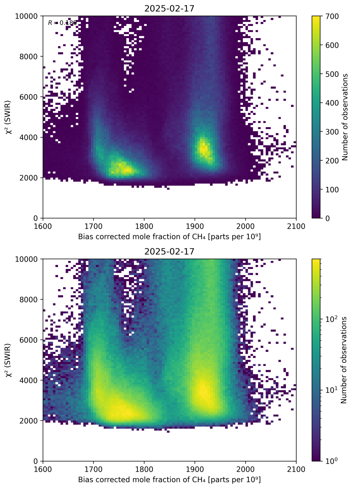
Figure 64: Scatter density plot of “Bias corrected mole fraction of \text{CH}_4 ” against “ \chi^2 (SWIR)” for 2025-02-16 to 2025-02-18.
