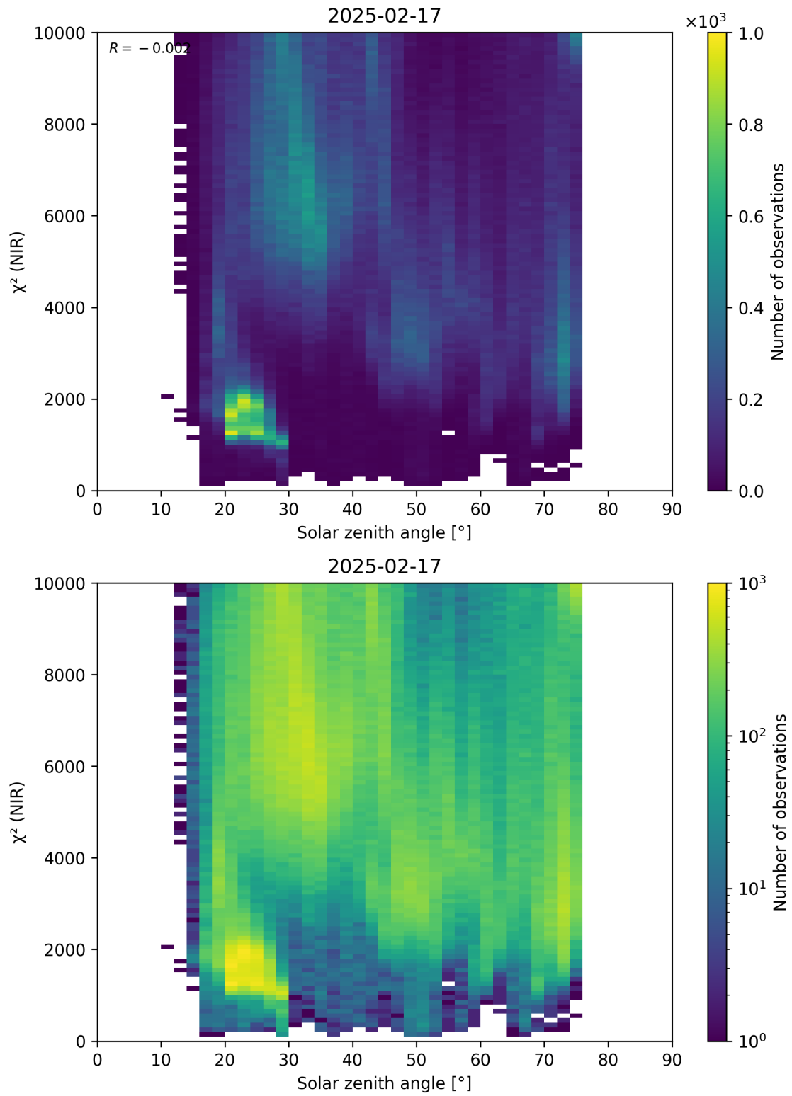
Figure 94: Scatter density plot of “Solar zenith angle” against “ \chi^2 (NIR)” for 2025-02-16 to 2025-02-18.
