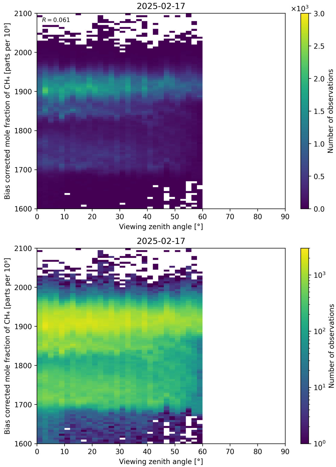
Figure 111: Scatter density plot of “Viewing zenith angle” against “Bias corrected mole fraction of CH 4 ” for 2025-02-16 to 2025-02-18.
