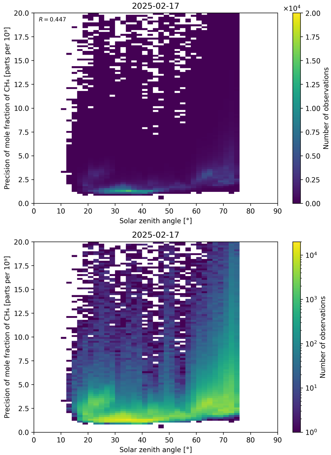
Figure 101: Scatter density plot of “Solar zenith angle” against “Precision of mole fraction of \text{CH}_4 ” for 2025-02-16 to 2025-02-18.
