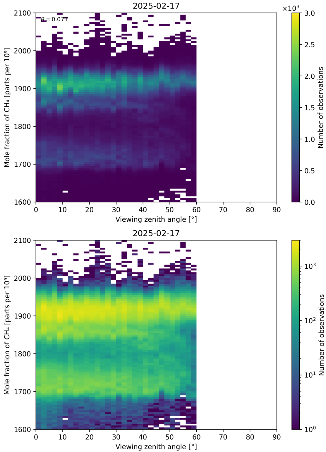
Figure 110: Scatter density plot of “Viewing zenith angle” against “Mole fraction of CH 4 ” for 2025-02-16 to 2025-02-18.
