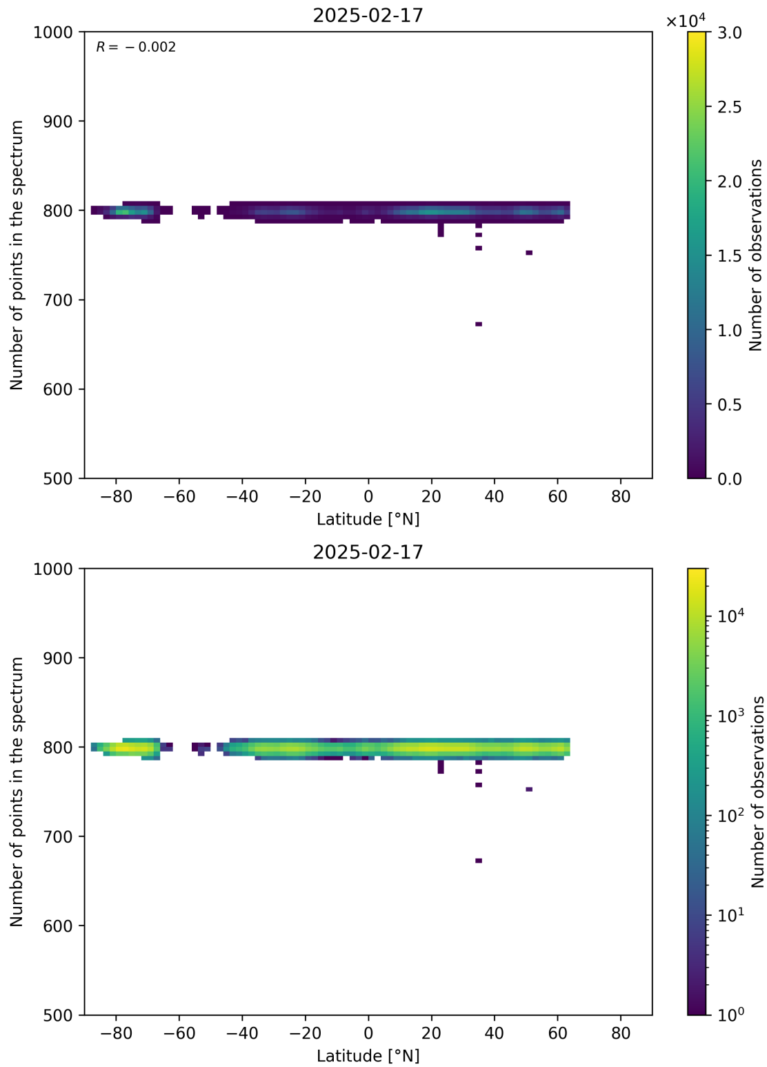
Figure 61: Scatter density plot of “Latitude” against “Number of points in the spectrum” for 2025-02-16 to 2025-02-18.
