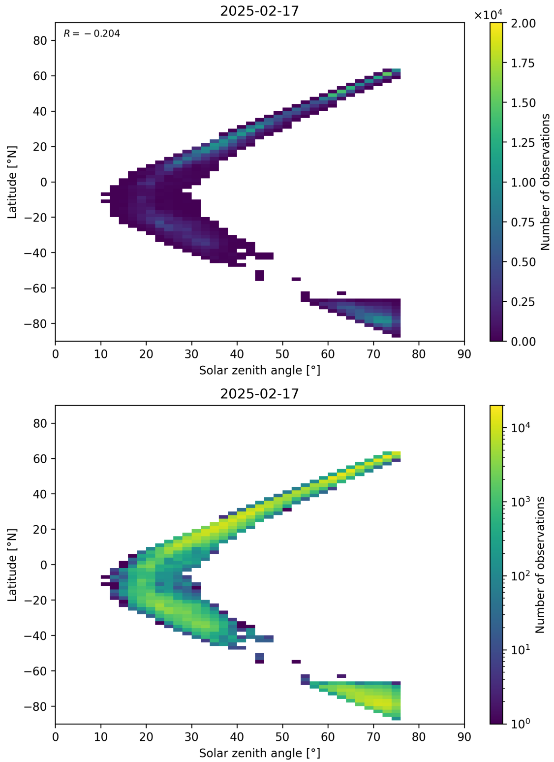
Figure 98: Scatter density plot of “Solar zenith angle” against “Latitude” for 2025-02-16 to 2025-02-18.
