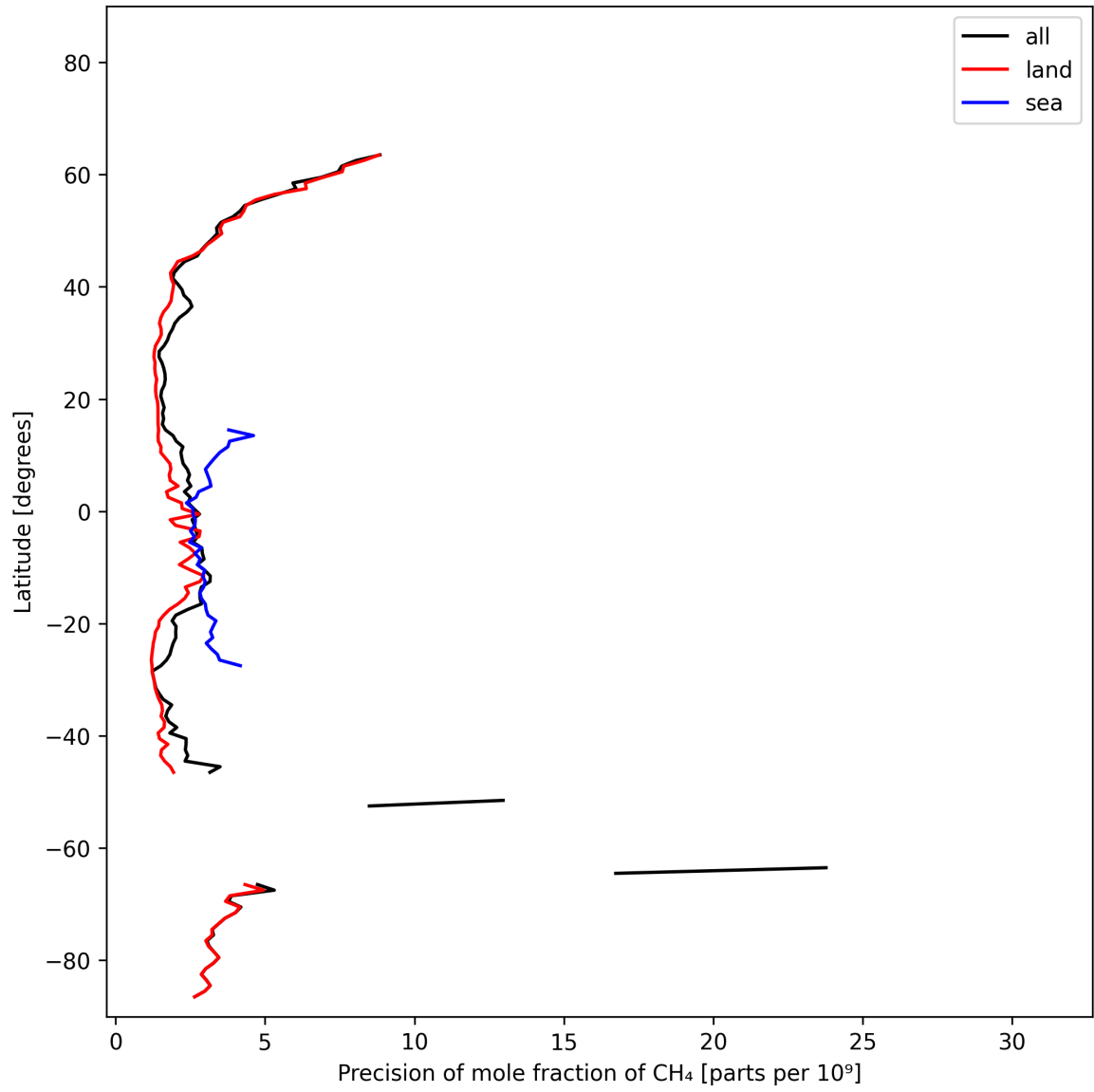
Figure 13: Zonal average of “Precision of mole fraction of CH 4 ” for 2025-02-16 to 2025-02-18.
