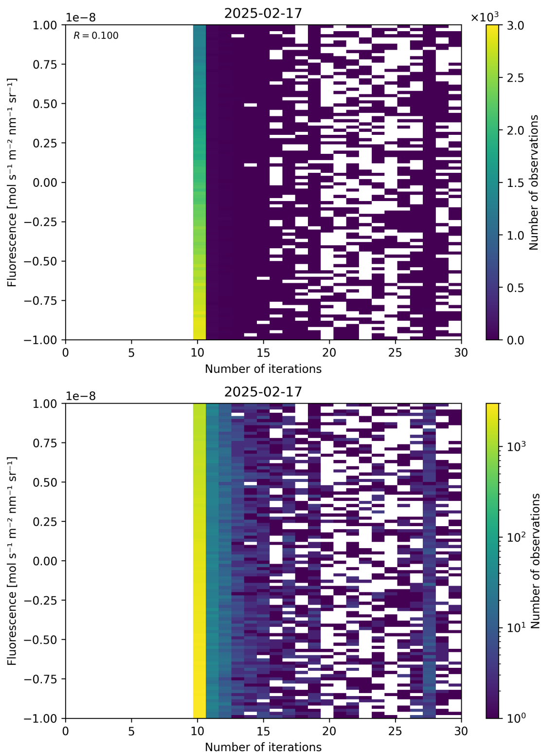
Figure 87: Scatter density plot of “Number of iterations” against “Fluorescence” for 2025-02-16 to 2025-02-18.
