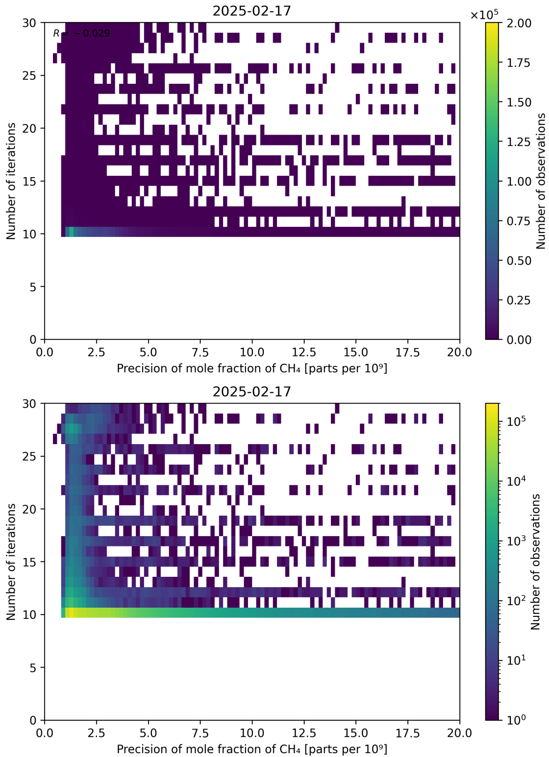
Figure 83: Scatter density plot of “Precision of mole fraction of CH 4 ” against “Number of iterations” for 2025-02-16 to 2025-02-18.
