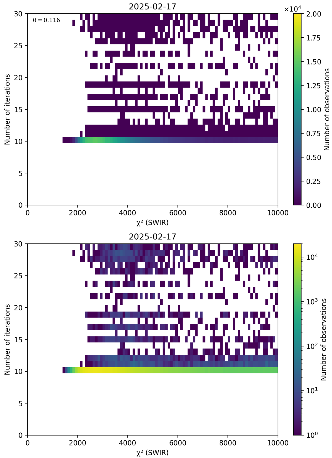
Figure 50: Scatter density plot of “ \chi^2 (SWIR)” against “Number of iterations” for 2025-02-16 to 2025-02-18.
