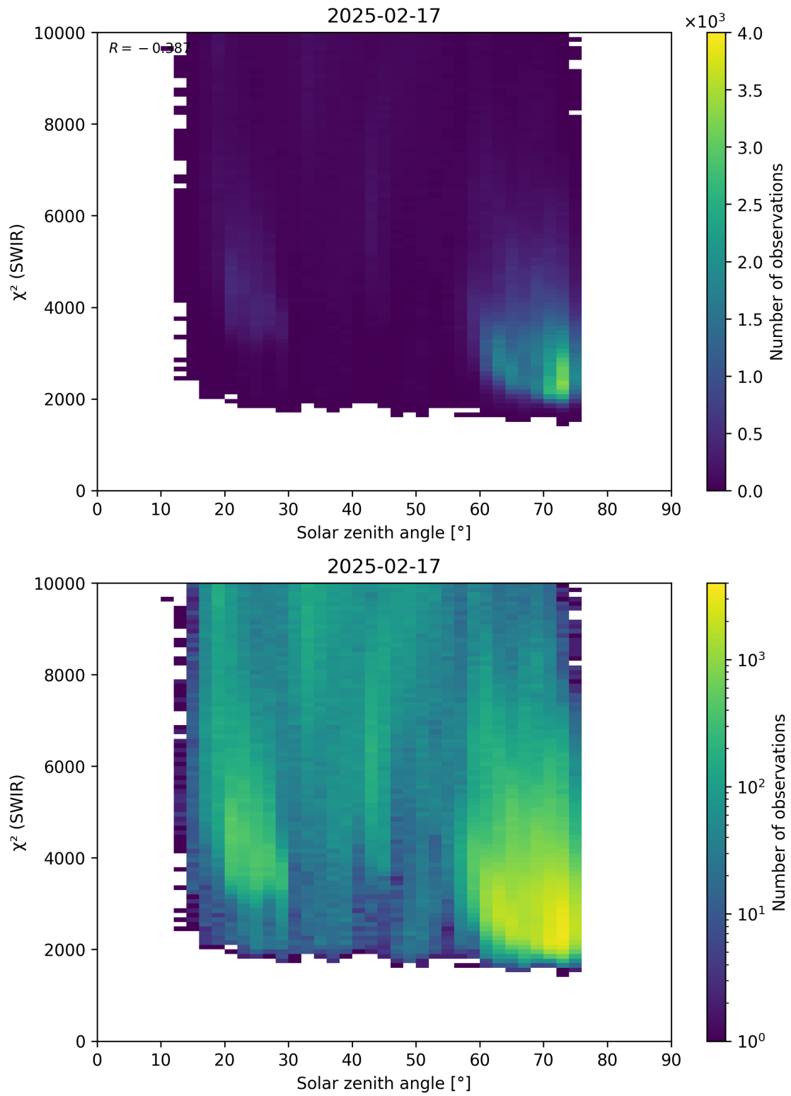
Figure 95: Scatter density plot of “Solar zenith angle” against “ \chi^2 (SWIR)” for 2025-02-16 to 2025-02-18.
