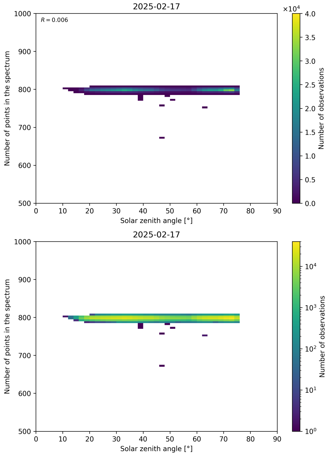
Figure 103: Scatter density plot of “Solar zenith angle” against “Number of points in the spectrum” for 2025-02-16 to 2025-02-18.
