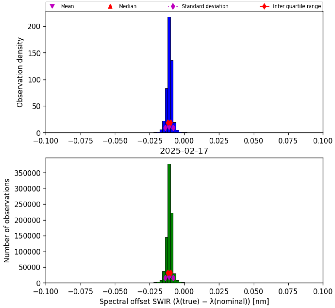
Figure 27: Histogram of “Spectral offset SWIR ( \lambda_{\text{true}} - \lambda_{\text{nominal}} )” for 2025-02-16 to 2025-02-18
