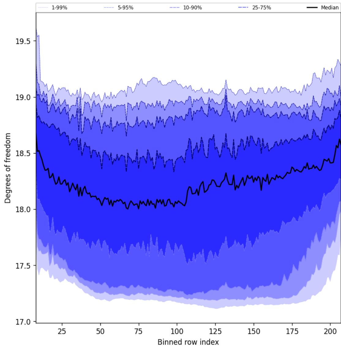
Figure 41: Along track statistics of “Degrees of freedom” for 2025-02-16 to 2025-02-18
