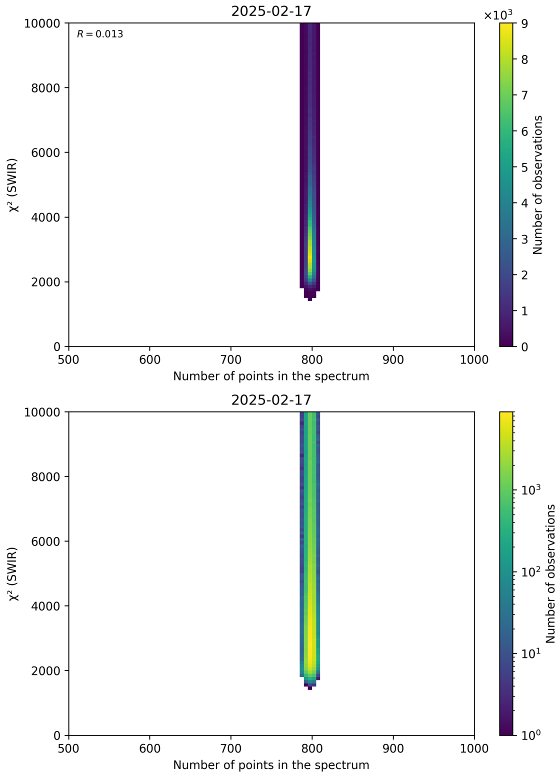
Figure 89: Scatter density plot of “Number of points in the spectrum” against “ \chi^2 (SWIR)” for 2025-02-16 to 2025-02-18.
