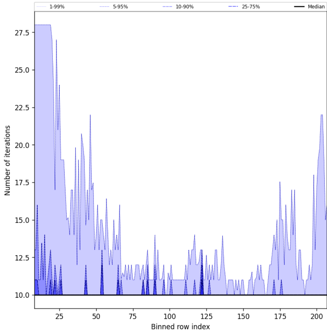
Figure 42: Along track statistics of “Number of iterations” for 2025-02-16 to 2025-02-18
