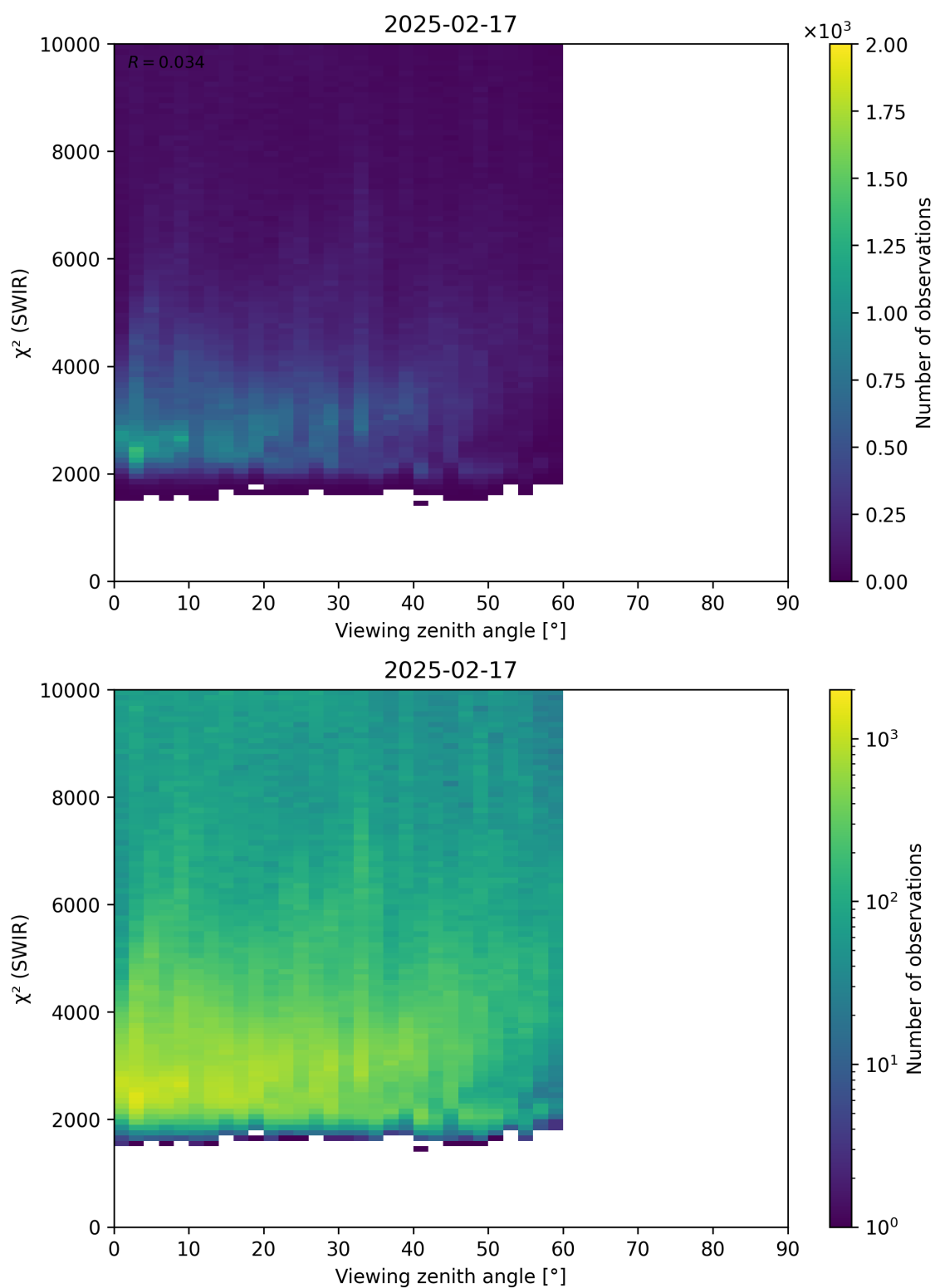
Figure 106: Scatter density plot of “Viewing zenith angle” against “ \chi^2 (SWIR)” for 2025-02-16 to 2025-02-18.
