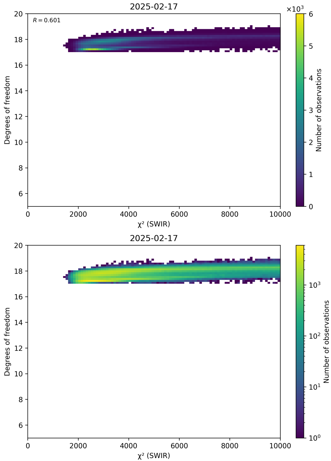
Figure 48: Scatter density plot of “ \chi^2 (SWIR)” against “Degrees of freedom” for 2025-02-16 to 2025-02-18.
