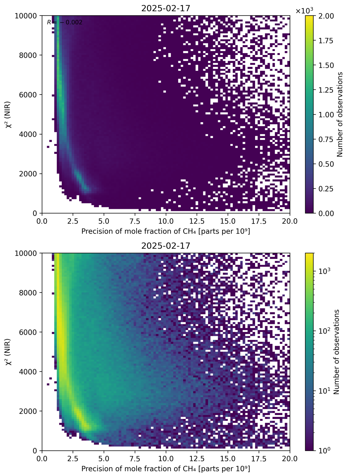
Figure 78: Scatter density plot of “Precision of mole fraction of \text{CH}_4 ” against “ \chi^2 (NIR)” for 2025-02-16 to 2025-02-18.
