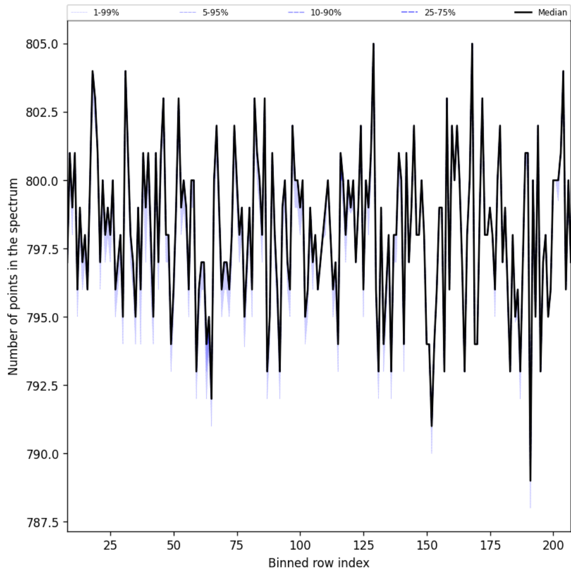
Figure 37: Along track statistics of “Number of points in the spectrum” for 2025-02-16 to 2025-02-18
