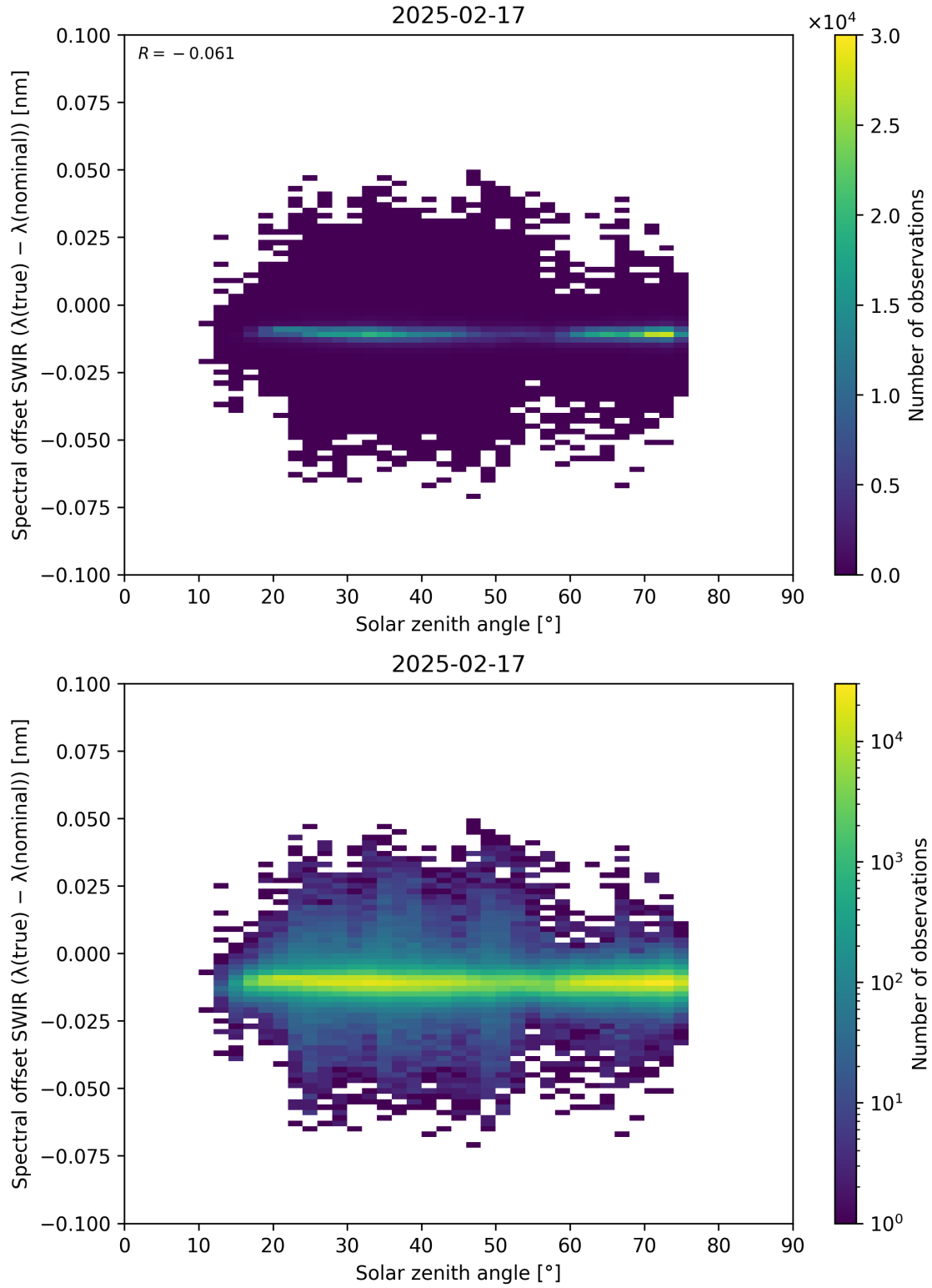
Figure 104: Scatter density plot of “Solar zenith angle” against “Spectral offset SWIR ( \lambda_{\text{true}} - \lambda_{\text{nominal}} )” for 2025-02-16 to 2025-02-18.
