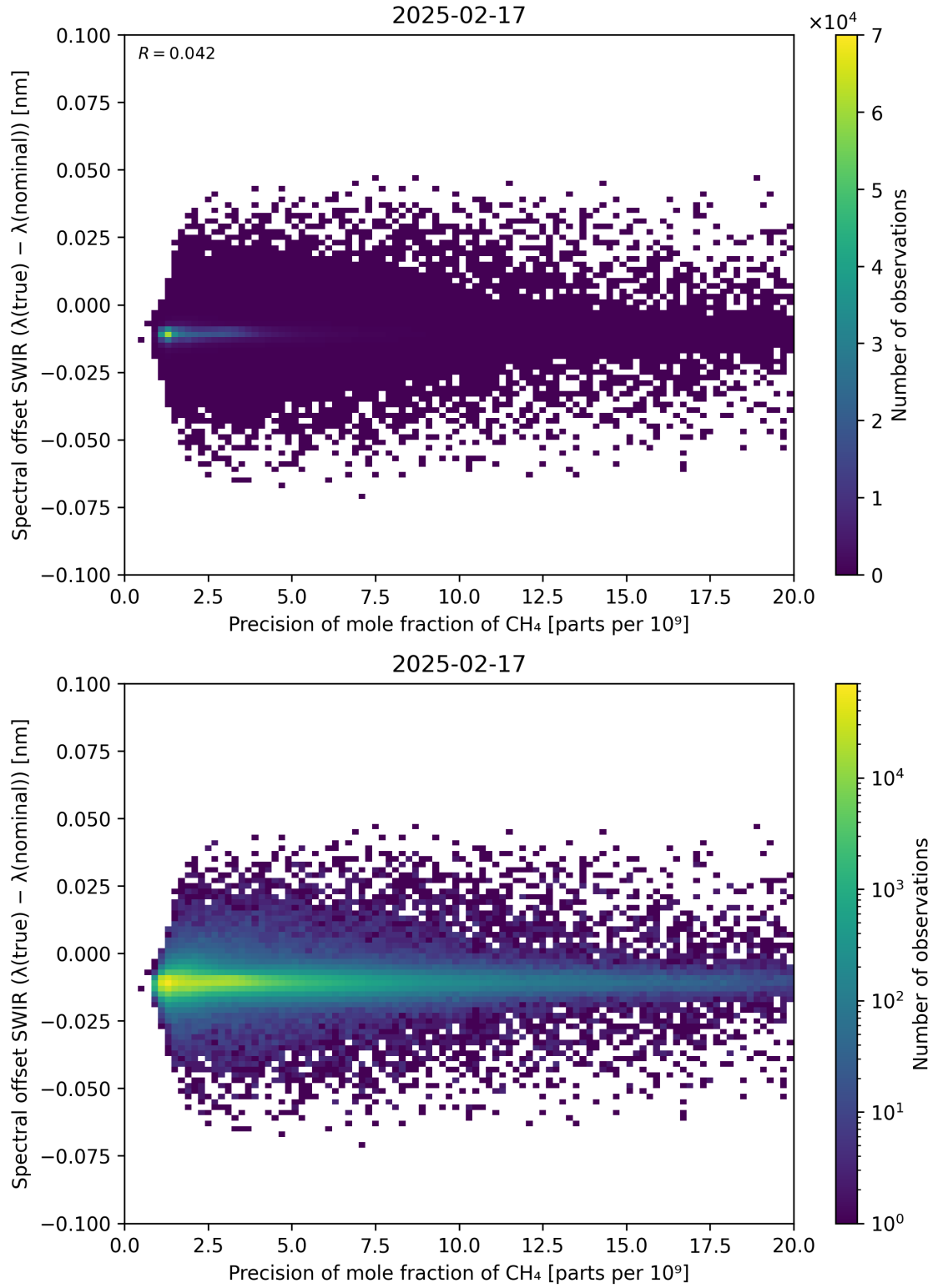
Figure 85: Scatter density plot of “Precision of mole fraction of CH 4 ” against “Spectral offset SWIR ( \lambda_{\text{true}} - \lambda_{\text{nominal}} )” for 2025-02-16 to 2025-02-18.
