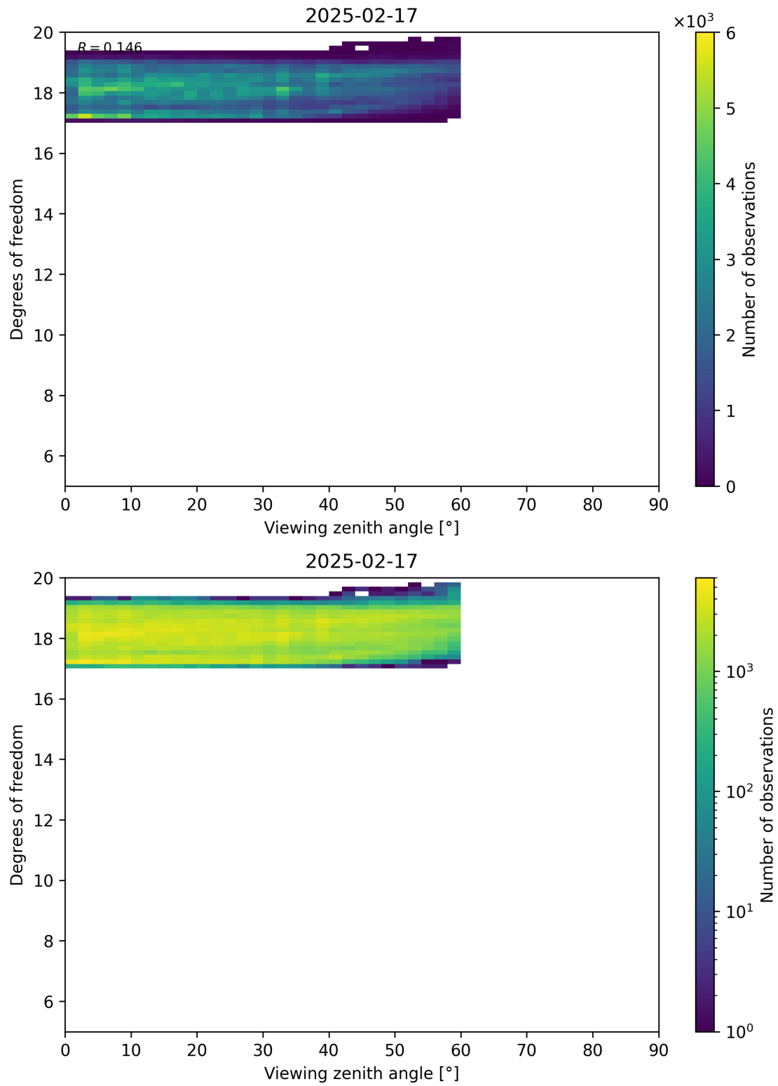
Figure 107: Scatter density plot of “Viewing zenith angle” against “Degrees of freedom” for 2025-02-16 to 2025-02-18.
