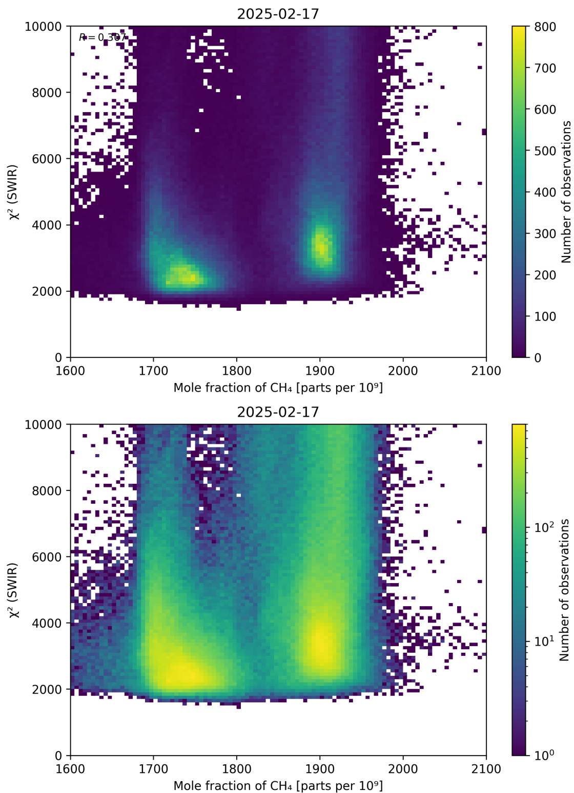
Figure 71: Scatter density plot of “Mole fraction of CH 4 ” against “ \chi^2 (SWIR)” for 2025-02-16 to 2025-02-18.
