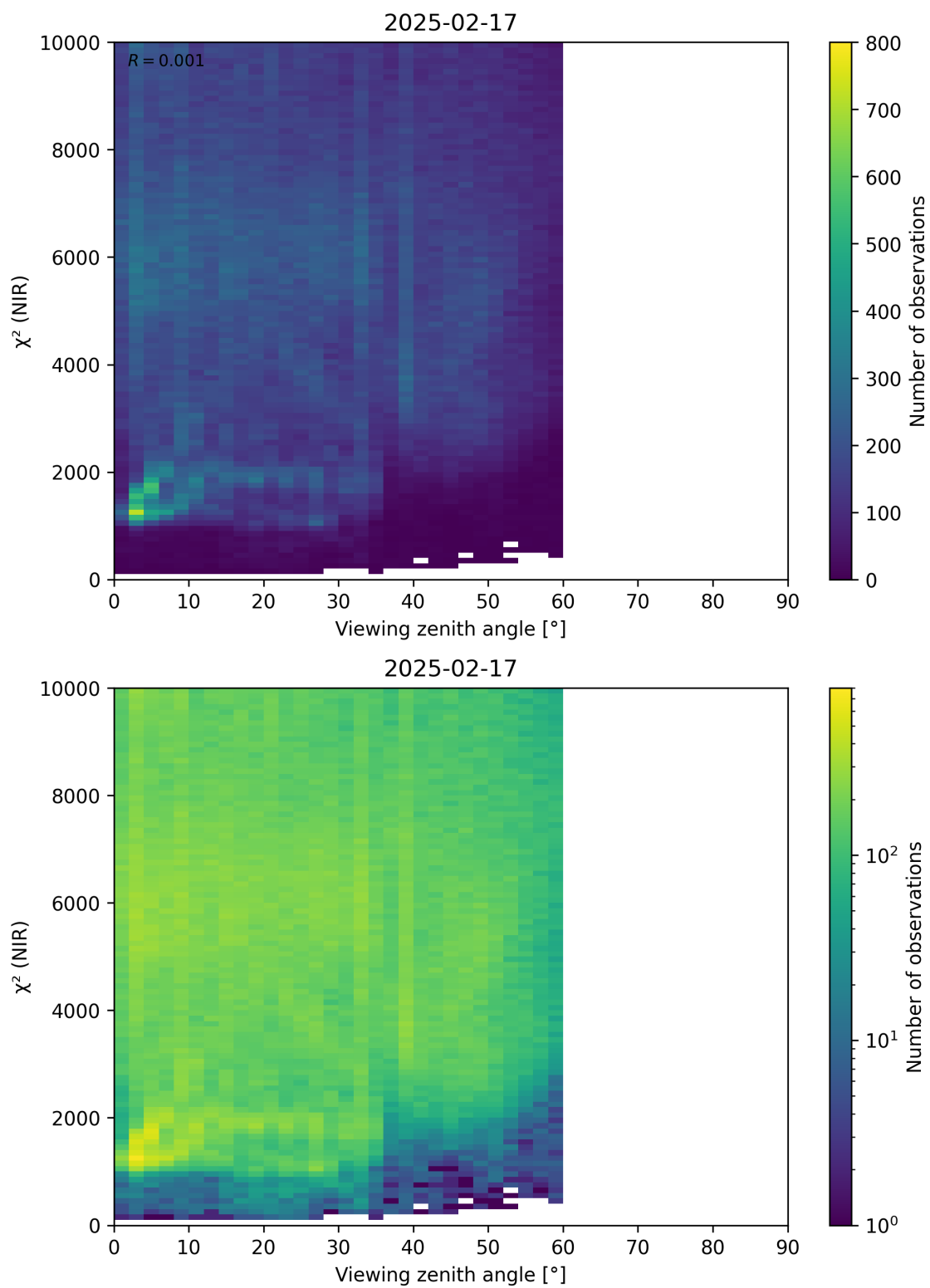
Figure 105: Scatter density plot of “Viewing zenith angle” against “ \chi^2 (NIR)” for 2025-02-16 to 2025-02-18.
