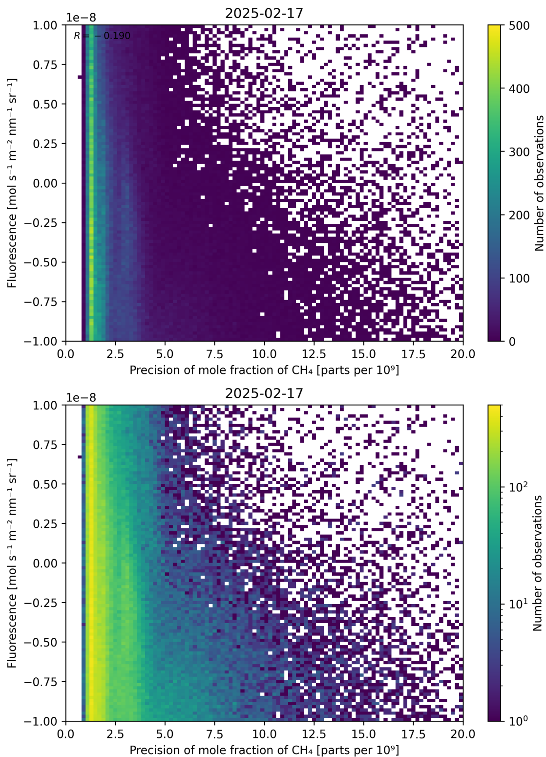
Figure 81: Scatter density plot of “Precision of mole fraction of CH 4 ” against “Fluorescence” for 2025-02-16 to 2025-02-18.
