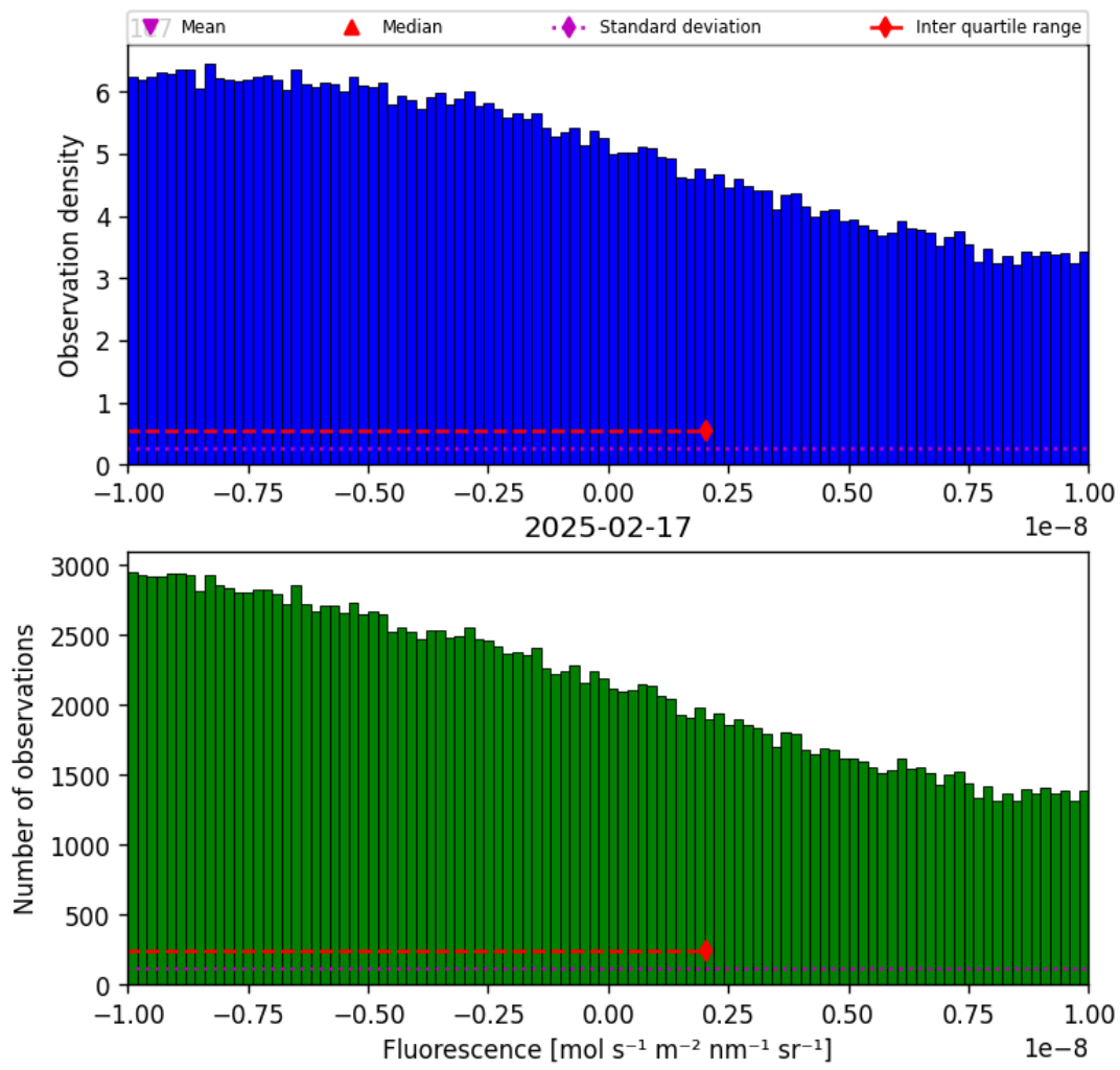
Figure 32: Histogram of “Fluorescence” for 2025-02-16 to 2025-02-18
