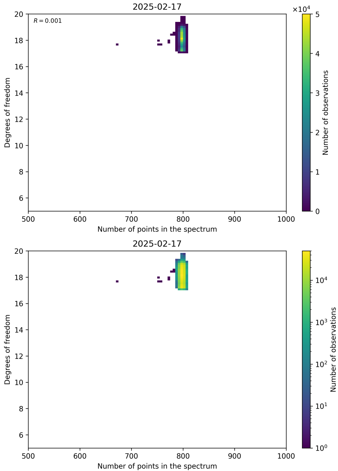
Figure 90: Scatter density plot of “Number of points in the spectrum” against “Degrees of freedom” for 2025-02-16 to 2025-02-18.
