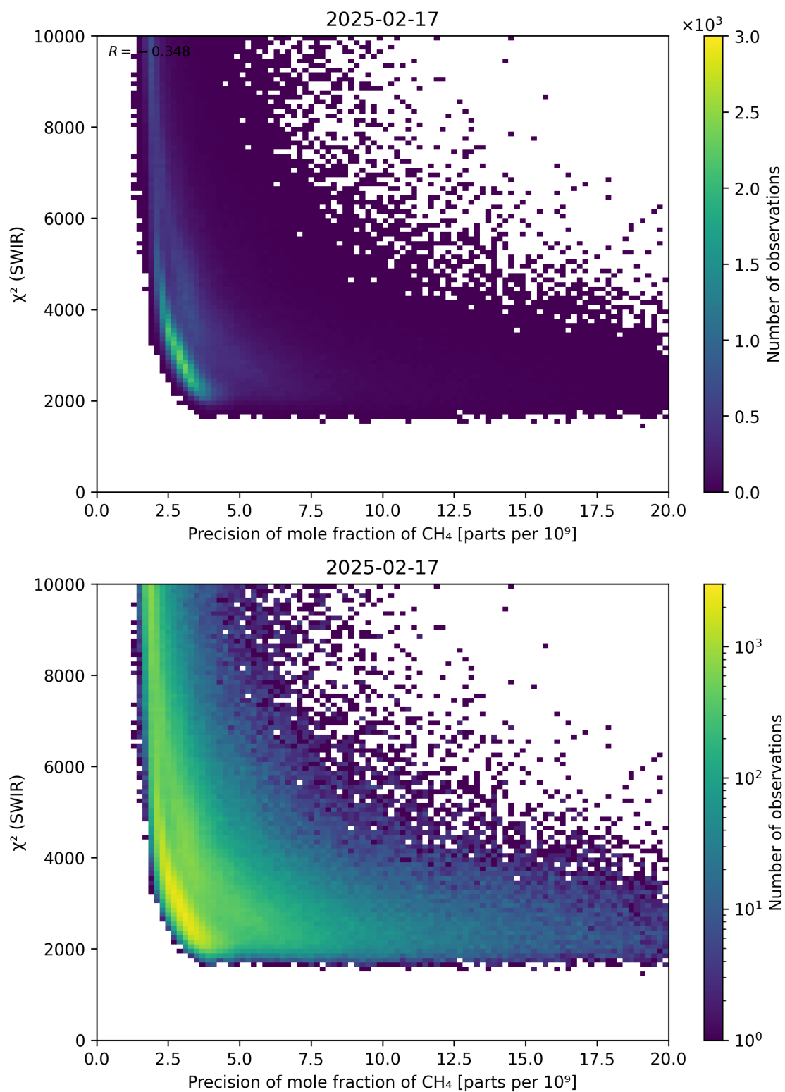
Figure 79: Scatter density plot of “Precision of mole fraction of \text{CH}_4 ” against “ \chi^2 (SWIR)” for 2025-02-16 to 2025-02-18.
