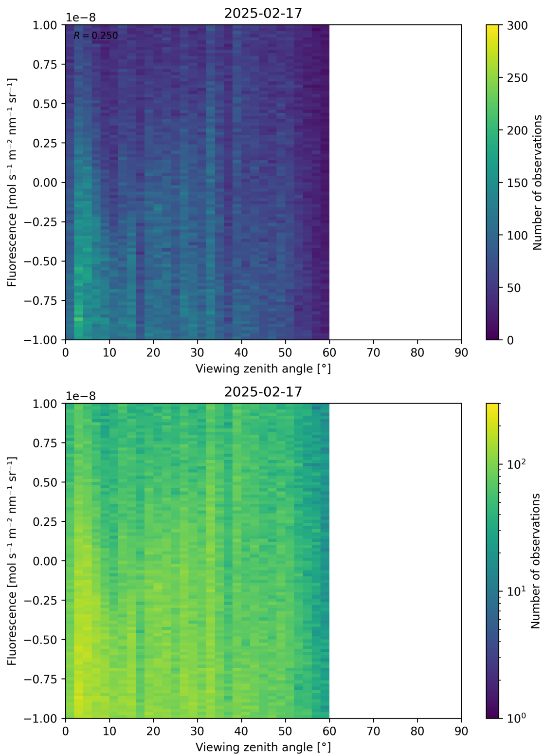
Figure 108: Scatter density plot of “Viewing zenith angle” against “Fluorescence” for 2025-02-16 to 2025-02-18.
