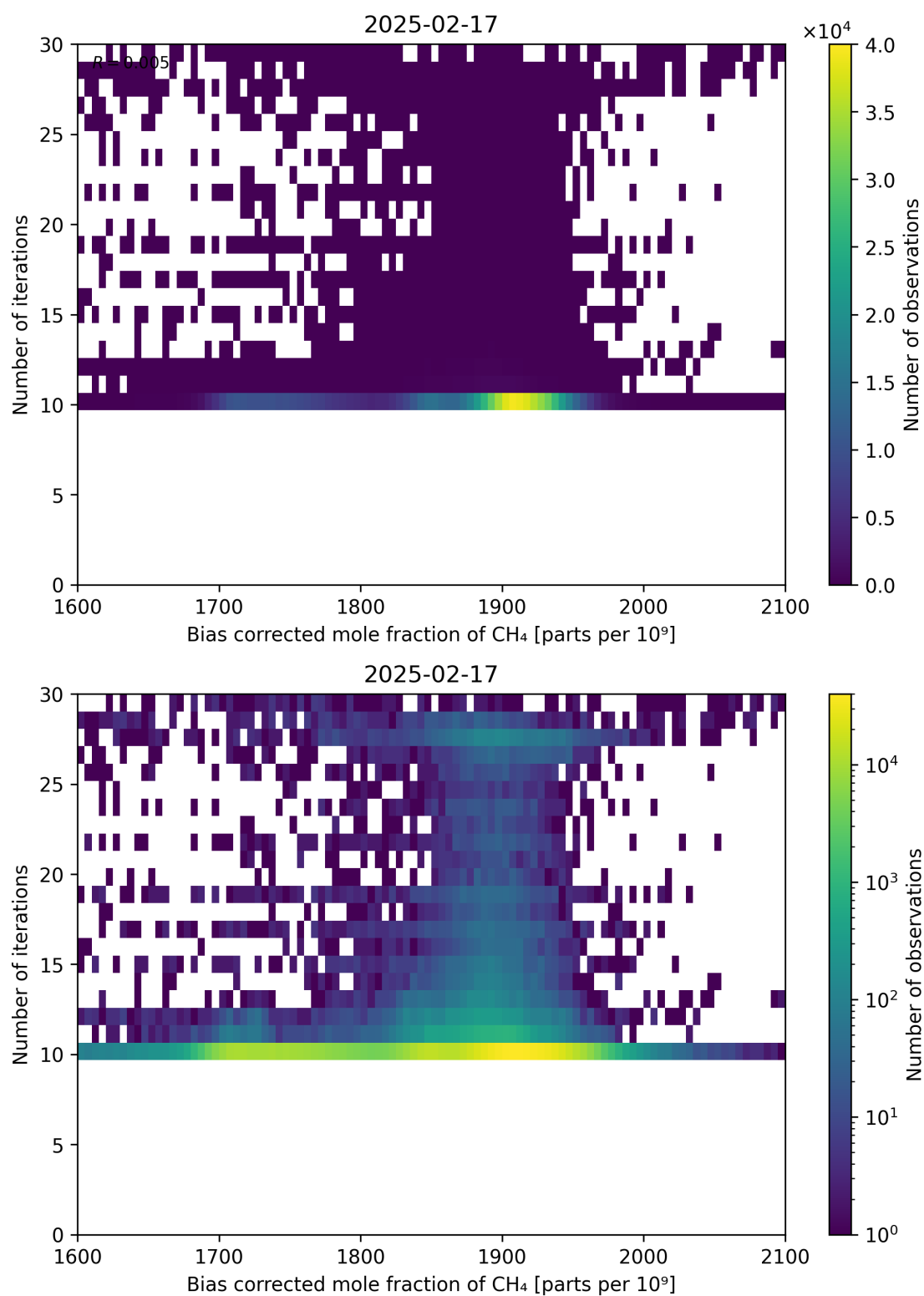
Figure 67: Scatter density plot of “Bias corrected mole fraction of CH 4 ” against “Number of iterations” for 2025-02-16 to 2025-02-18.
