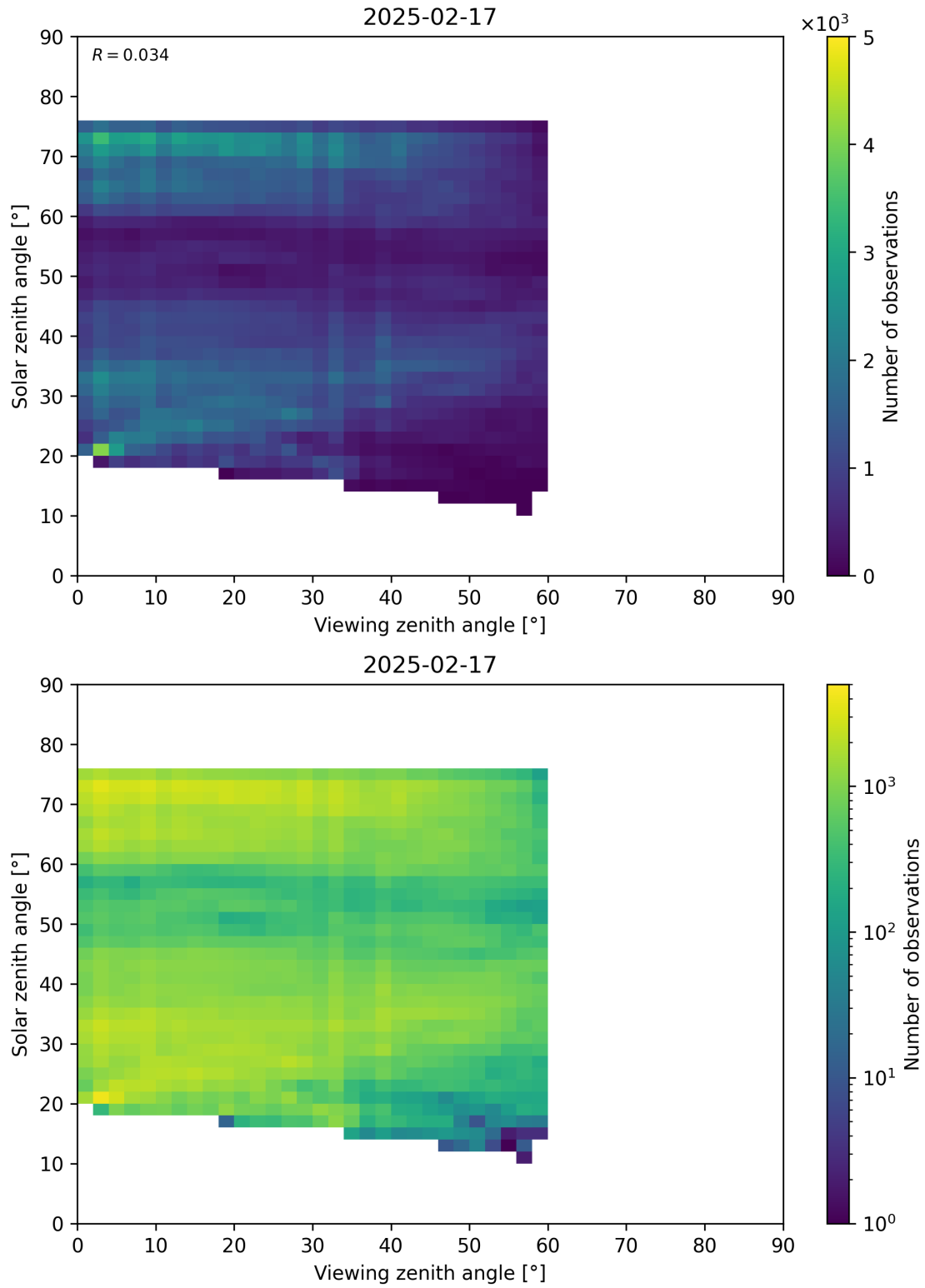
Figure 115: Scatter density plot of “Viewing zenith angle” against “Solar zenith angle” for 2025-02-16 to 2025-02-18.
