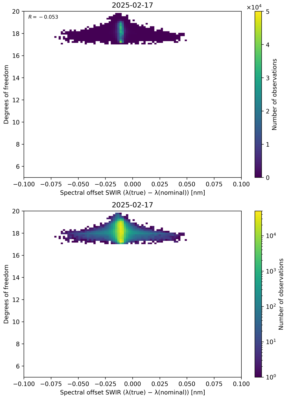
Figure 119: Scatter density plot of “Spectral offset SWIR ( \lambda_{\text{true}} - \lambda_{\text{nominal}} )” against “Degrees of freedom” for 2025-02-16 to 2025-02-18.
