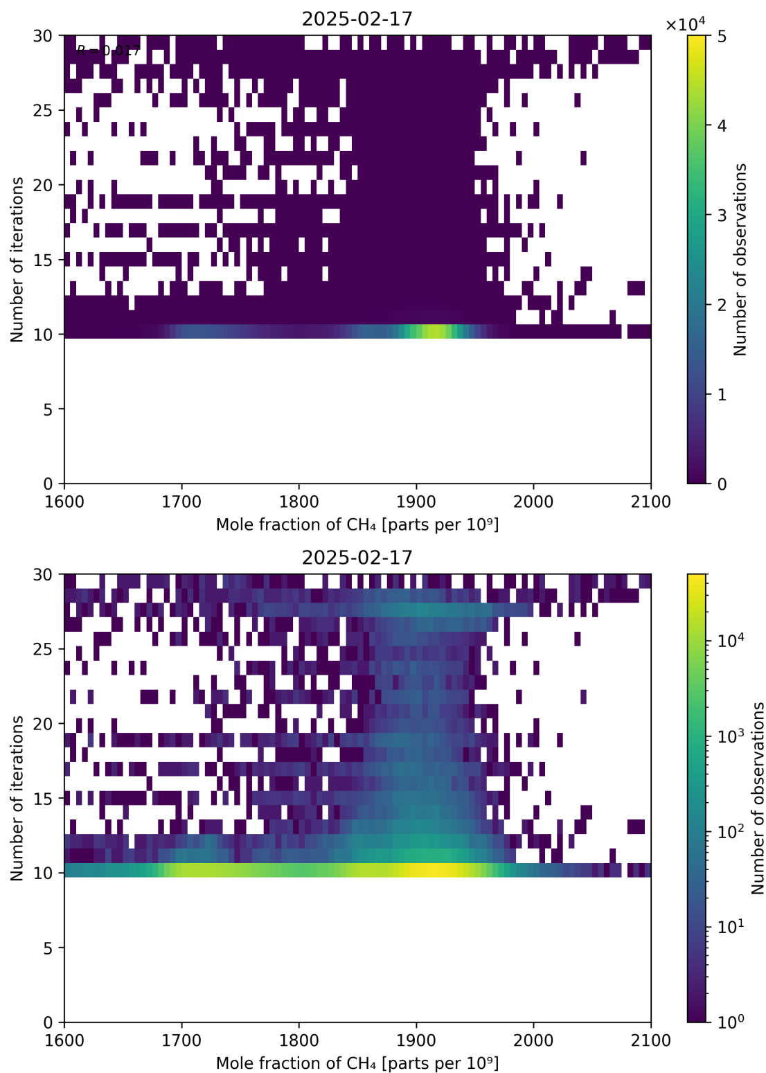
Figure 76: Scatter density plot of “Mole fraction of CH 4 ” against “Number of iterations” for 2025-02-16 to 2025-02-18.
