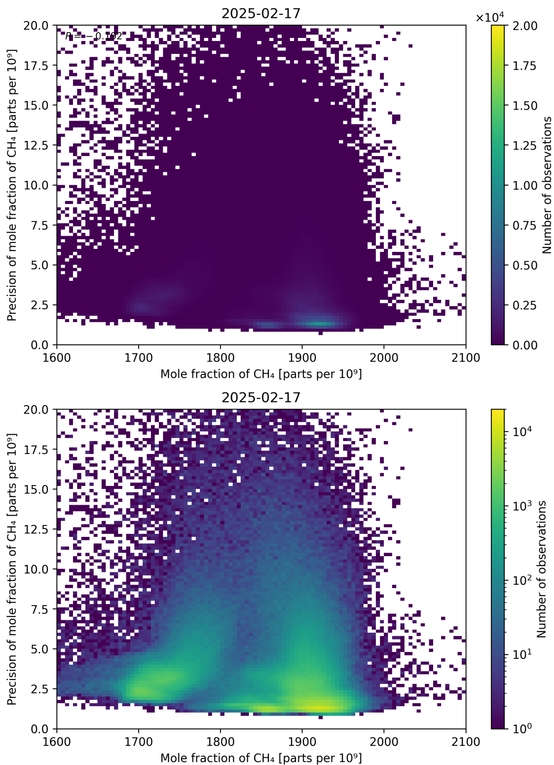
Figure 75: Scatter density plot of “Mole fraction of CH 4 ” against “Precision of mole fraction of CH 4 ” for 2025-02-16 to 2025-02-18.
