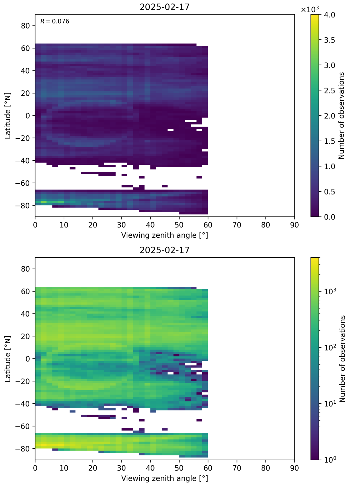
Figure 109: Scatter density plot of “Viewing zenith angle” against “Latitude” for 2025-02-16 to 2025-02-18.
