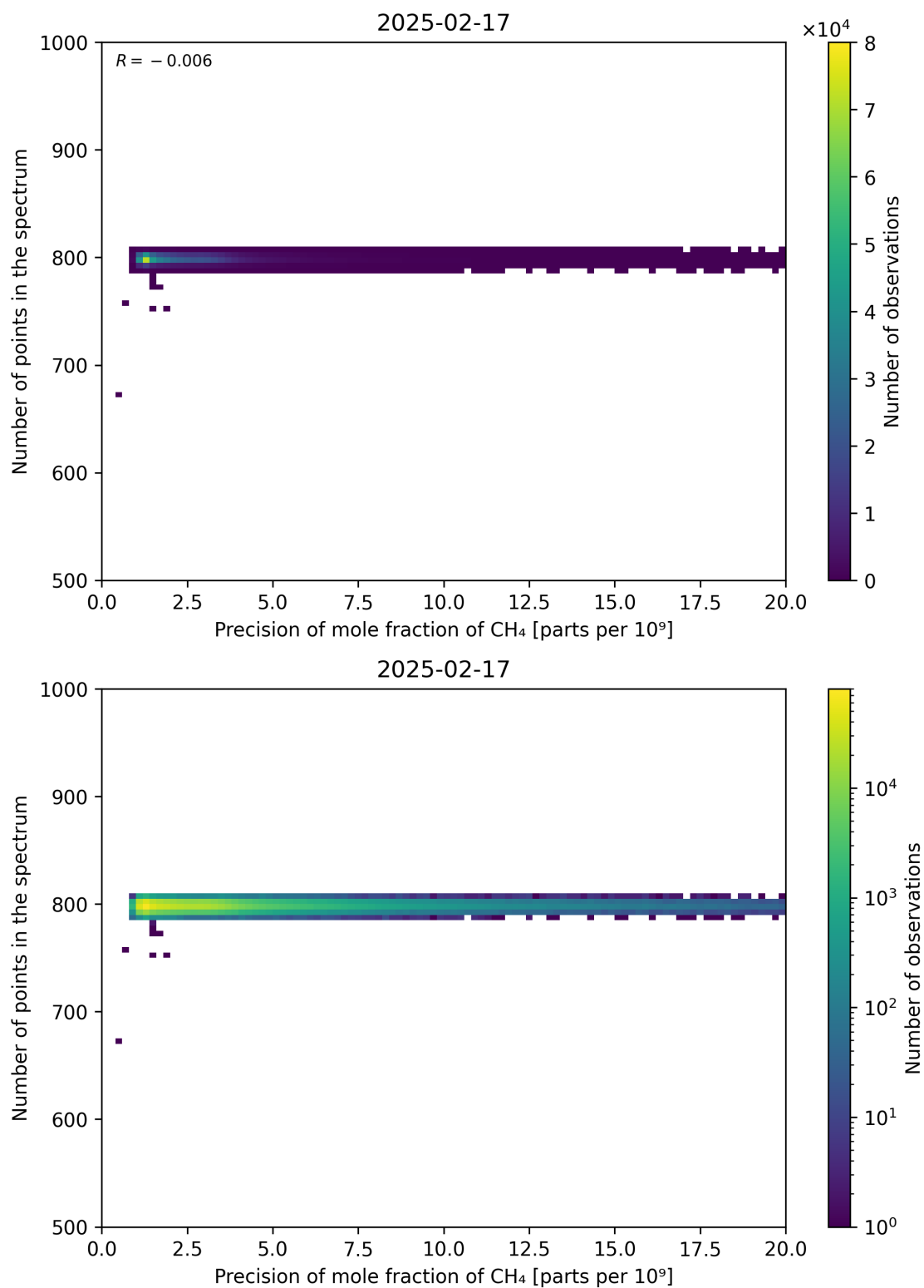
Figure 84: Scatter density plot of “Precision of mole fraction of CH 4 ” against “Number of points in the spectrum” for 2025-02-16 to 2025-02-18.
