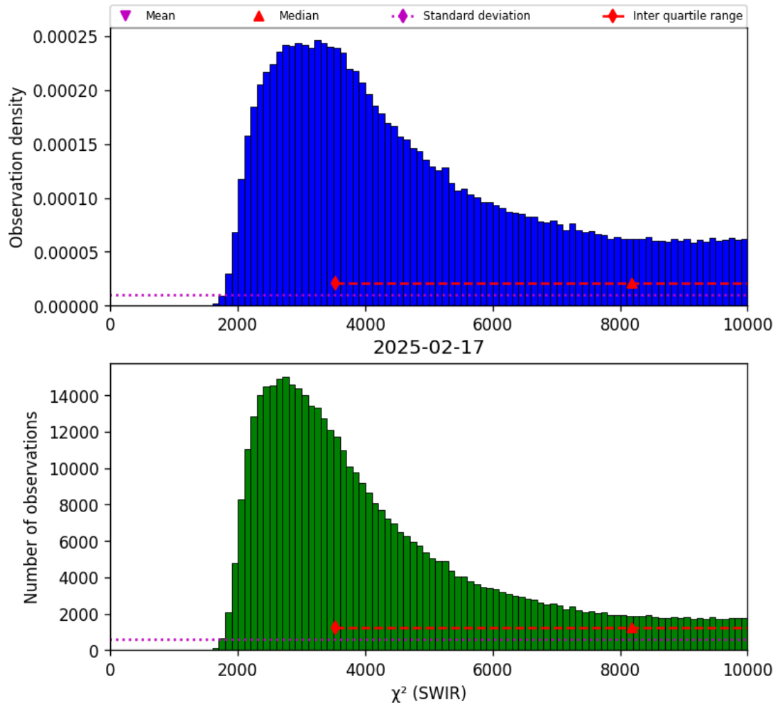
Figure 28: Histogram of " \chi^2 (SWIR)" for 2025-02-16 to 2025-02-18
