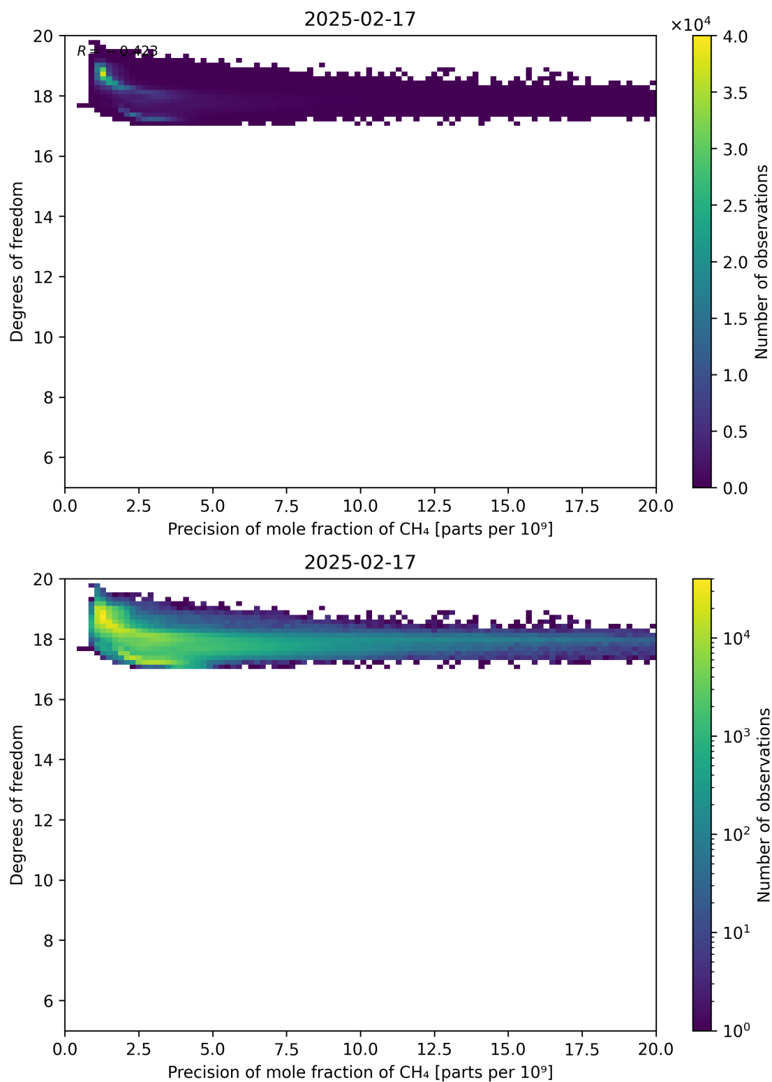
Figure 80: Scatter density plot of “Precision of mole fraction of CH 4 ” against “Degrees of freedom” for 2025-02-16 to 2025-02-18.
