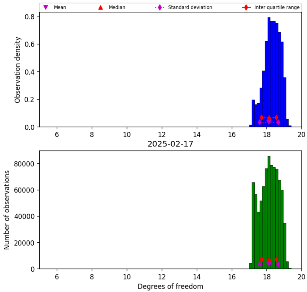
Figure 30: Histogram of “Degrees of freedom” for 2025-02-16 to 2025-02-18
