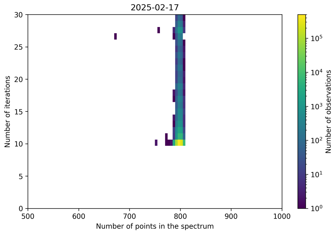
Figure 92: Scatter density plot of “Number of points in the spectrum” against “Number of iterations” for 2025-02-16 to 2025-02-18.
