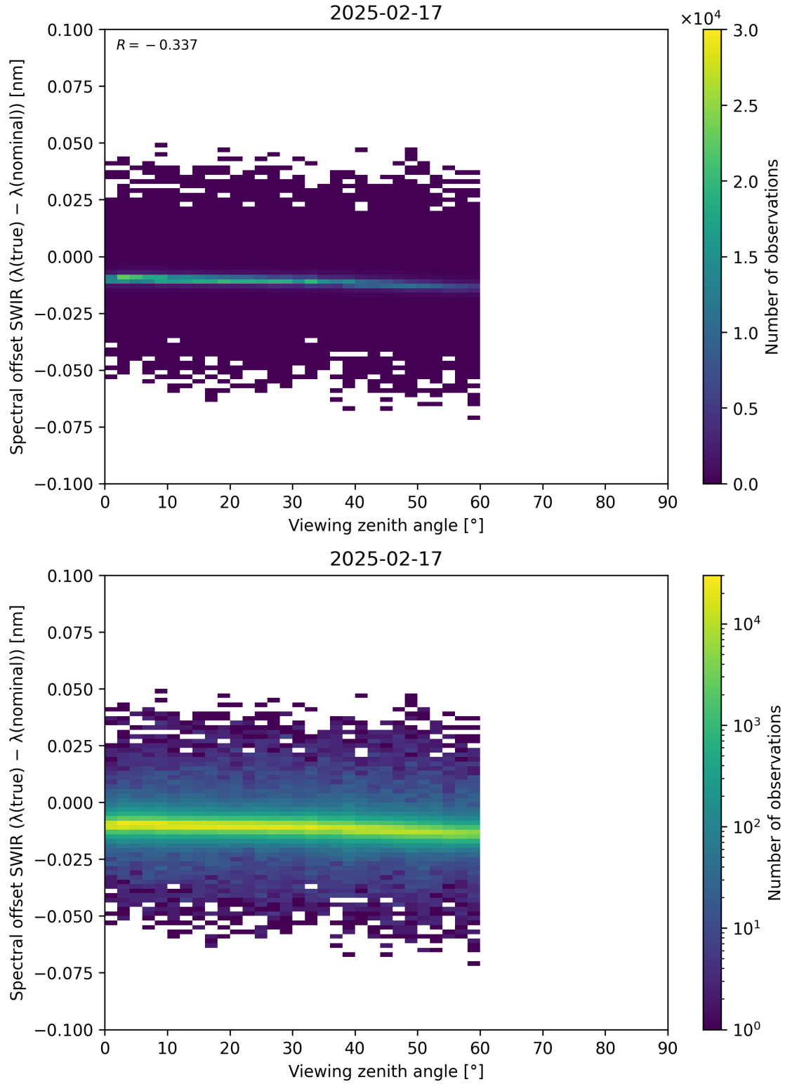
Figure 116: Scatter density plot of “Viewing zenith angle” against “Spectral offset SWIR ( \lambda_{\text{true}} - \lambda_{\text{nominal}} )” for 2025-02-16 to 2025-02-18.
