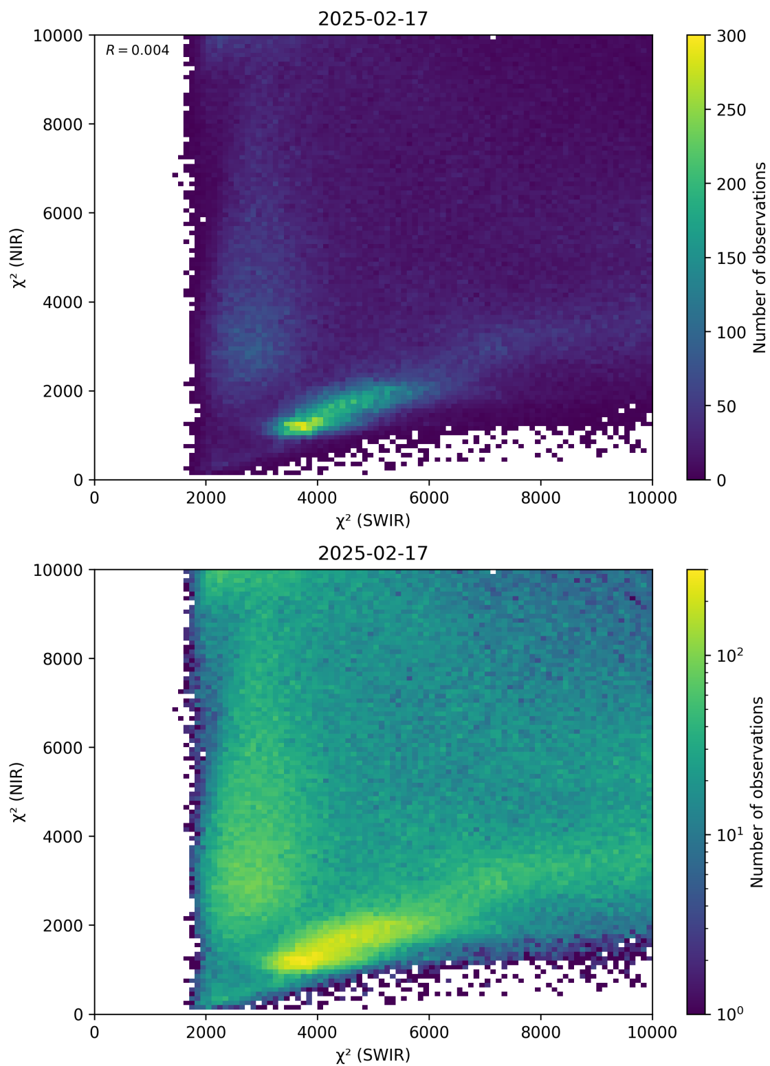
Figure 47: Scatter density plot of “ \chi^2 (SWIR)” against “ \chi^2 (NIR)” for 2025-02-16 to 2025-02-18.
