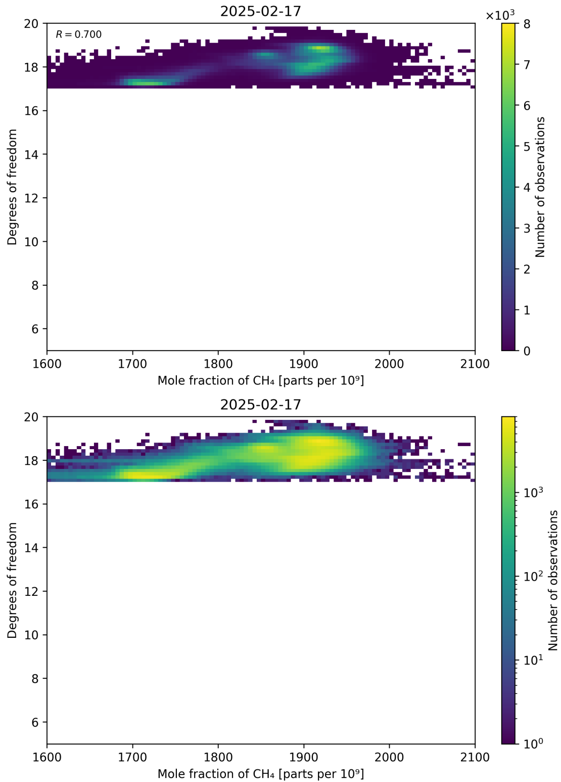
Figure 72: Scatter density plot of “Mole fraction of CH 4 ” against “Degrees of freedom” for 2025-02-16 to 2025-02-18.
