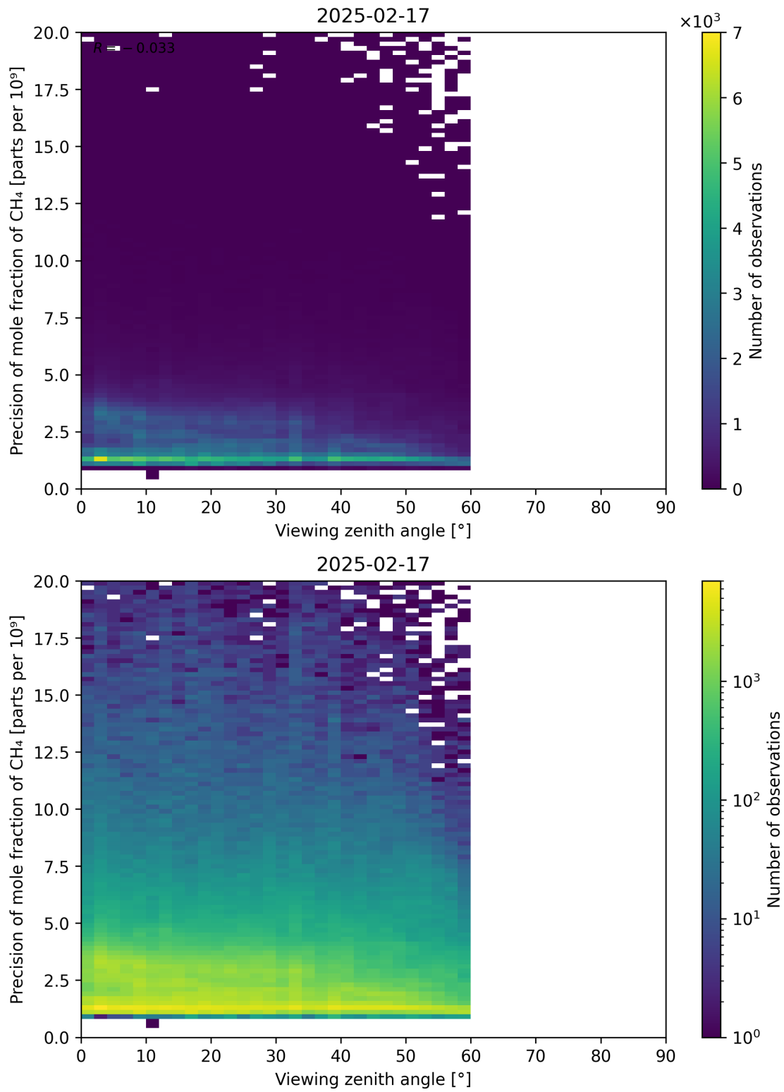
Figure 112: Scatter density plot of “Viewing zenith angle” against “Precision of mole fraction of CH 4 ” for 2025-02-16 to 2025-02-18.
