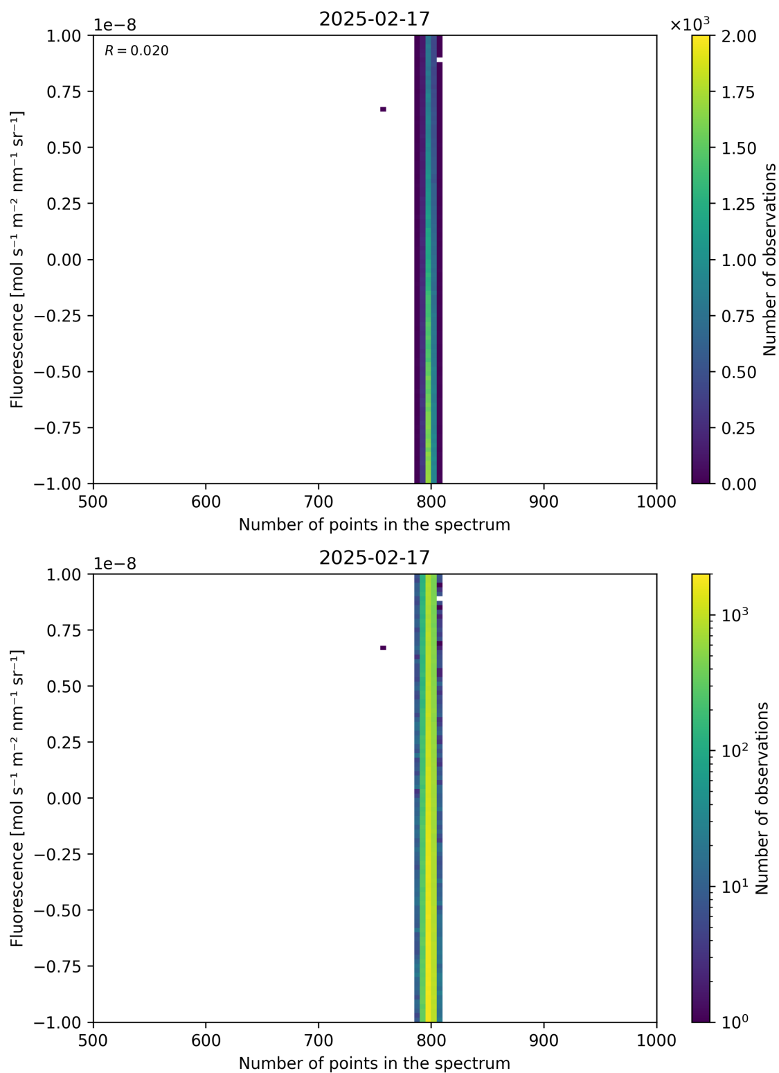
Figure 91: Scatter density plot of “Number of points in the spectrum” against “Fluorescence” for 2025-02-16 to 2025-02-18.
