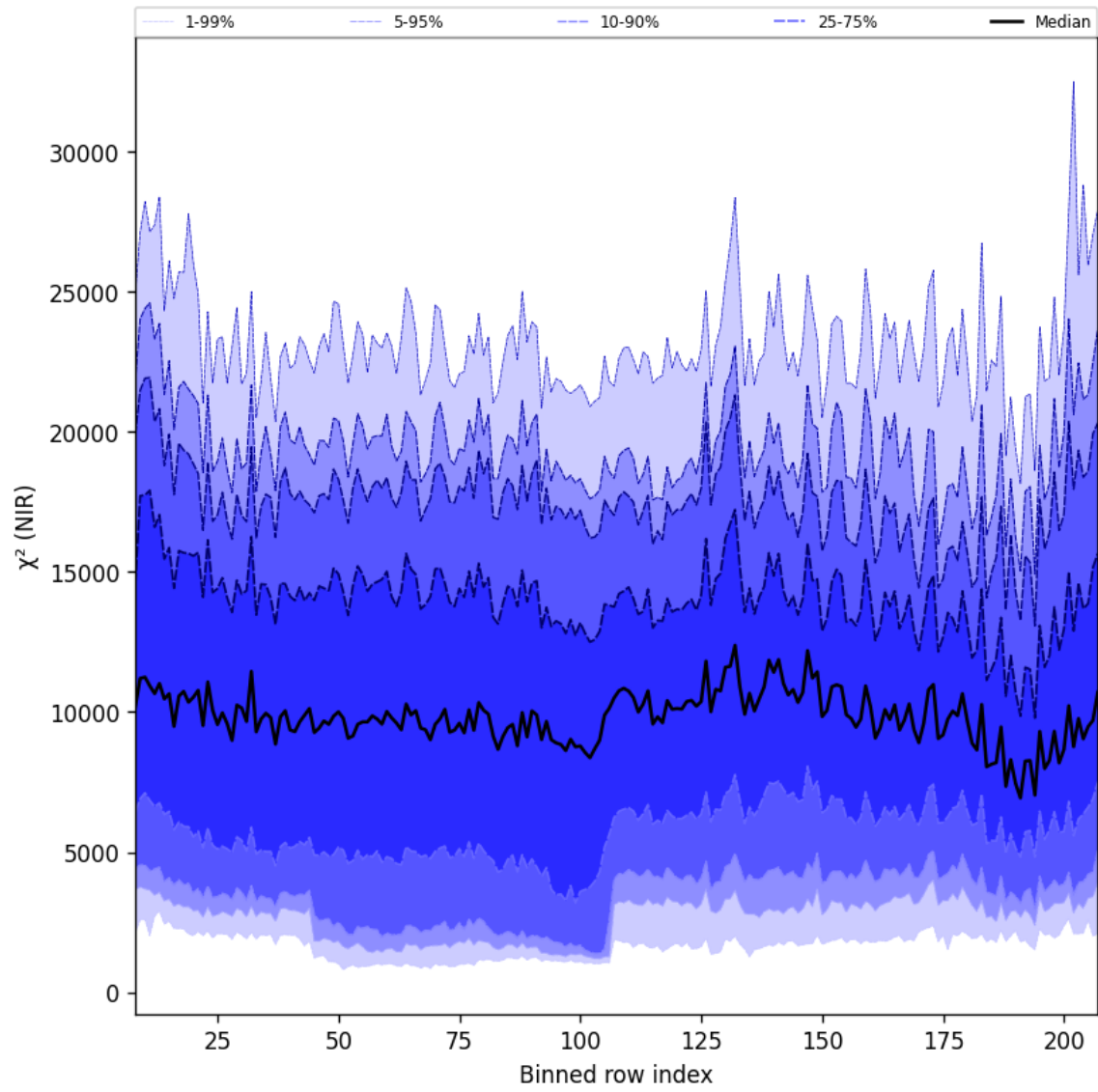
Figure 40: Along track statistics of “ \chi^2 (NIR)” for 2025-02-16 to 2025-02-18
