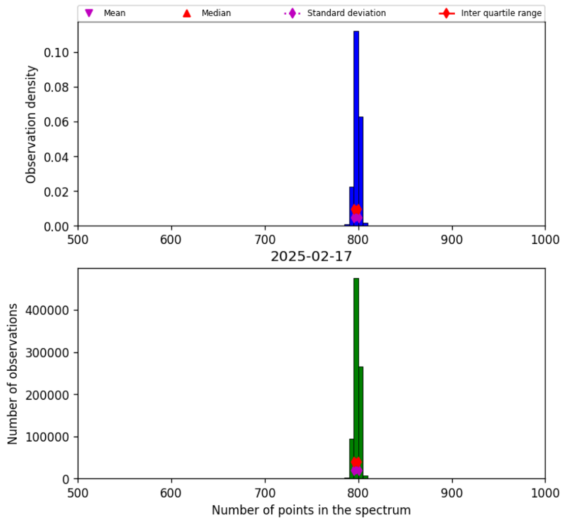
Figure 26: Histogram of “Number of points in the spectrum” for 2025-02-16 to 2025-02-18
