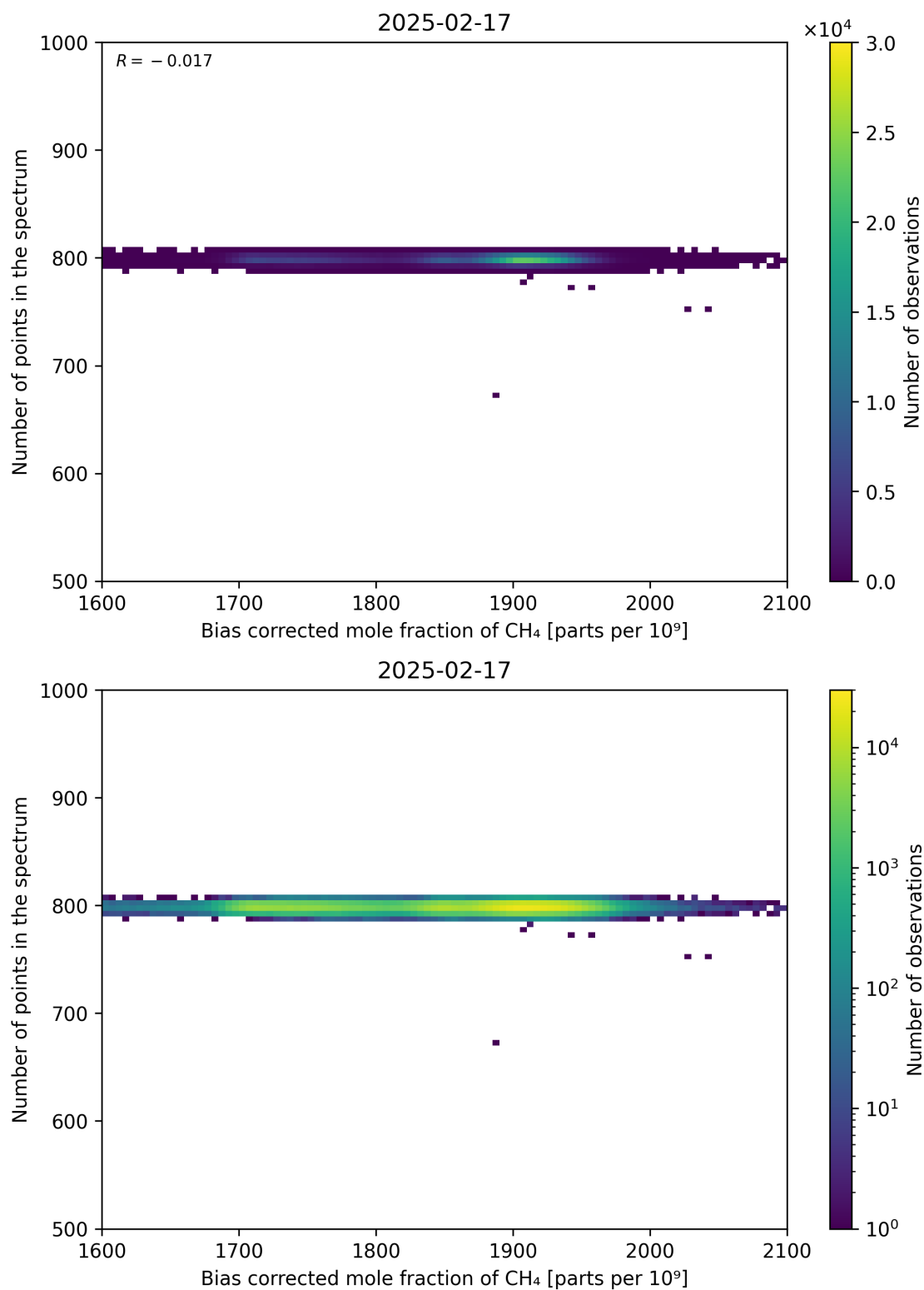
Figure 68: Scatter density plot of “Bias corrected mole fraction of CH 4 ” against “Number of points in the spectrum” for 2025-02-16 to 2025-02-18.
