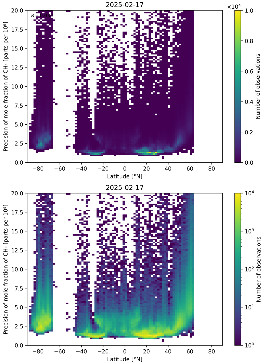
Figure 59: Scatter density plot of “Latitude” against “Precision of mole fraction of CH 4 ” for 2025-02-16 to 2025-02-18.
