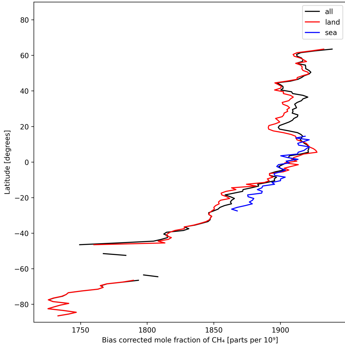
Figure 14: Zonal average of “Bias corrected mole fraction of CH 4 ” for 2025-02-16 to 2025-02-18.
