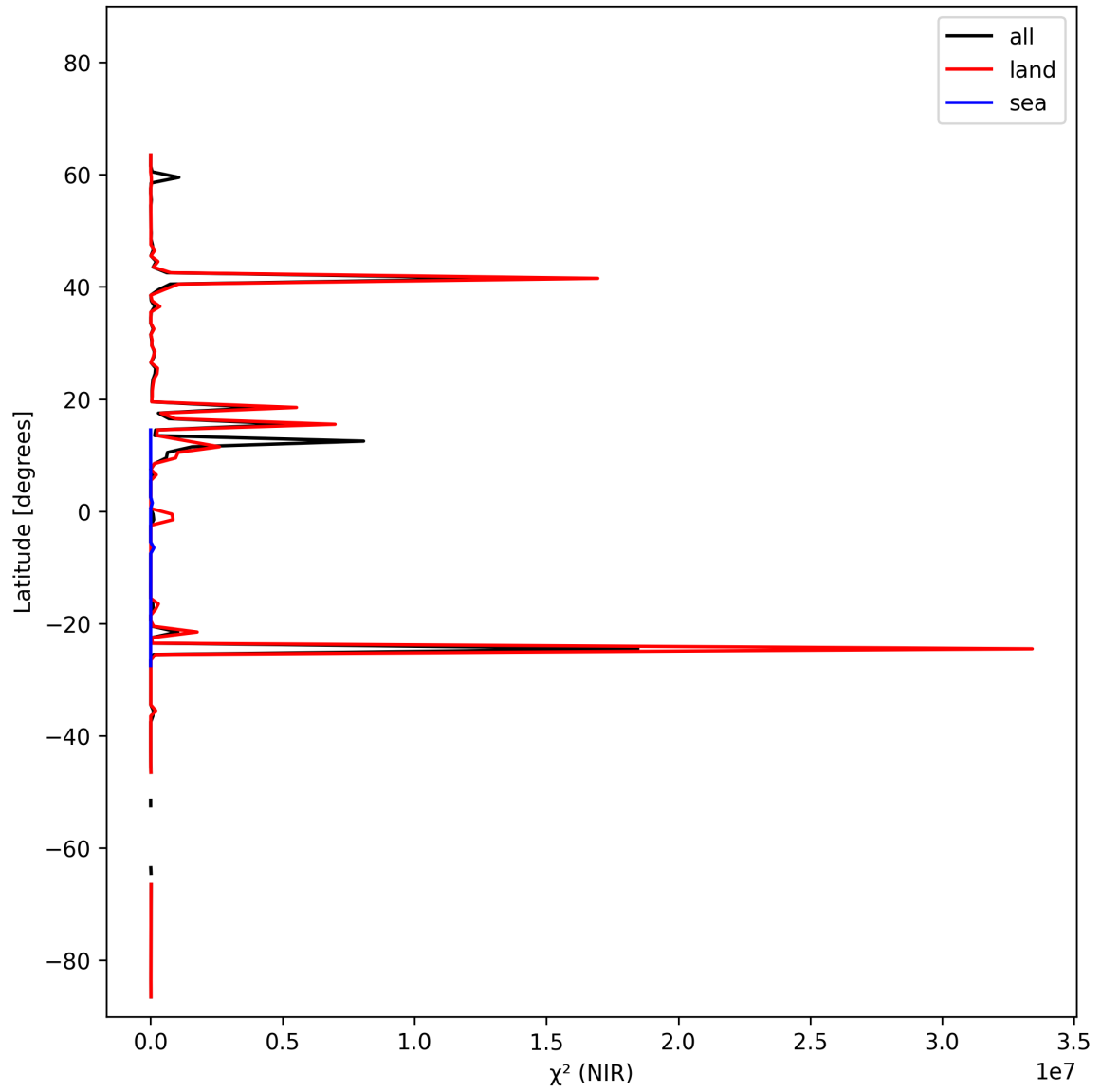
Figure 18: Zonal average of “ \chi^2 (NIR)” for 2025-02-16 to 2025-02-18.
