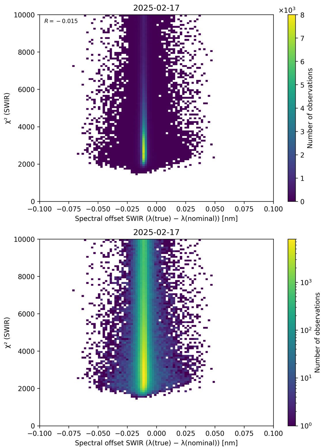
Figure 118: Scatter density plot of “Spectral offset SWIR ( \lambda_{\text{true}} - \lambda_{\text{nominal}} )” against “ \chi^2 (SWIR)” for 2025-02-16 to 2025-02-18.
