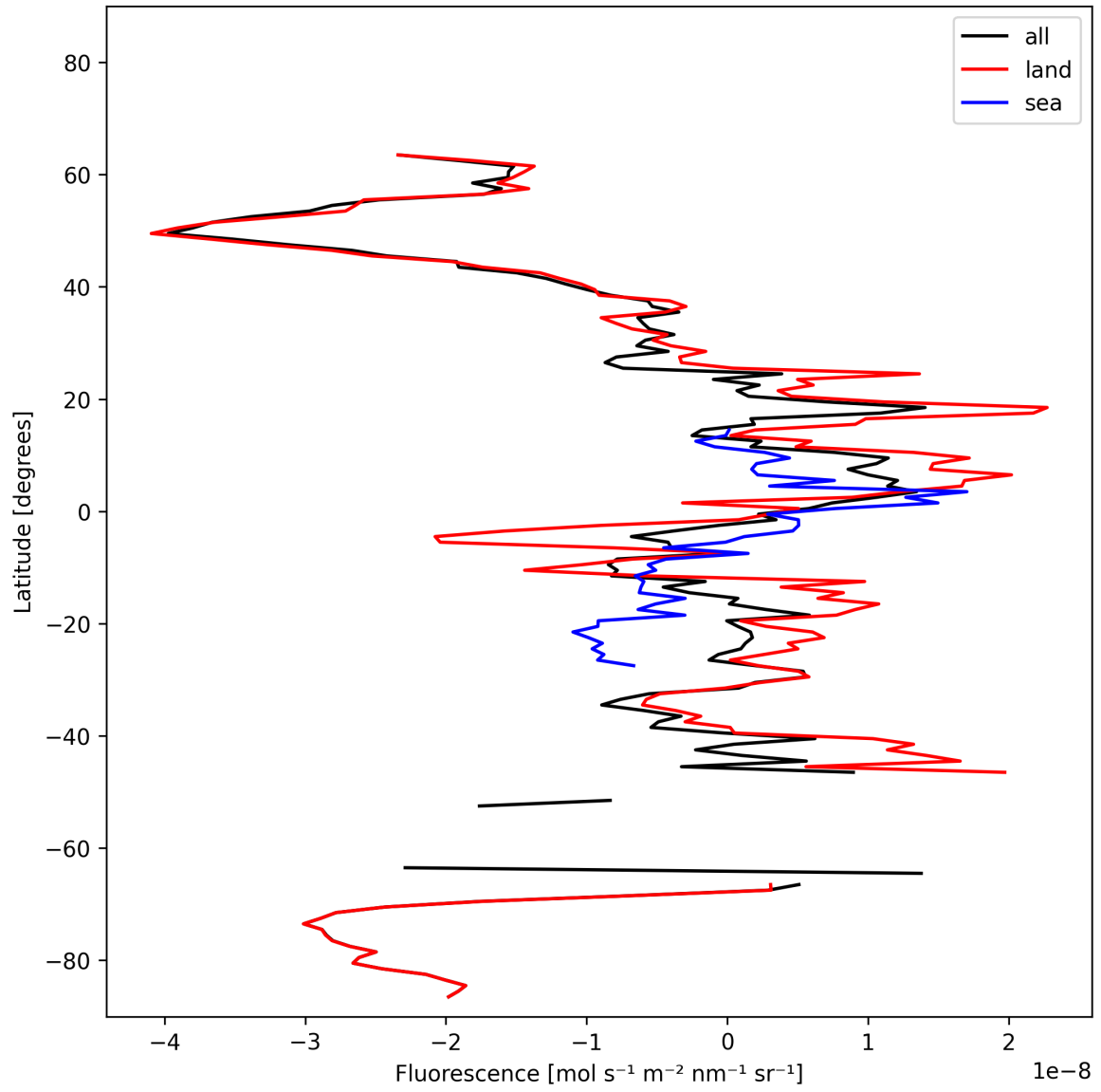
Figure 21: Zonal average of “Fluorescence” for 2025-02-16 to 2025-02-18.
