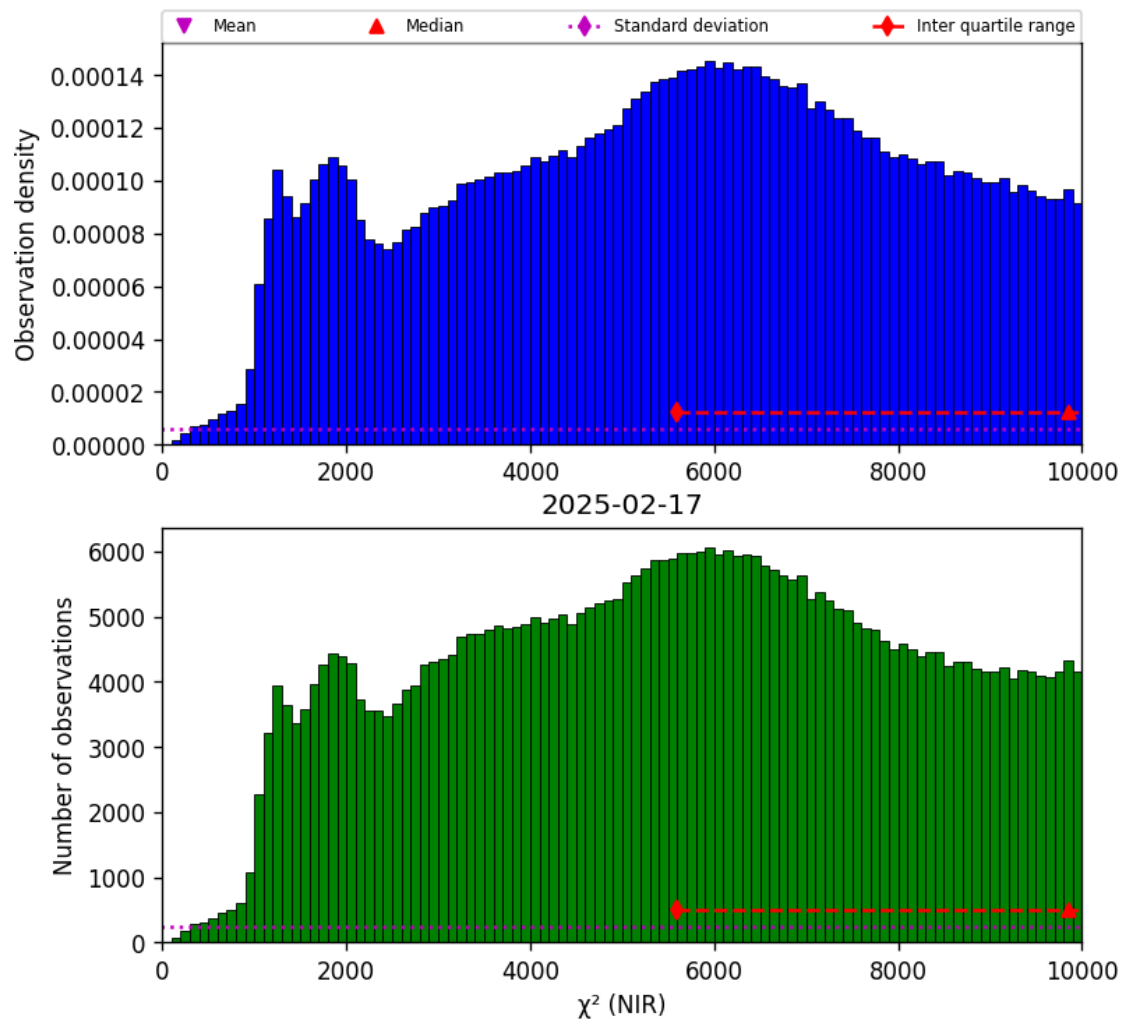
Figure 29: Histogram of “ \chi^2 (NIR)” for 2025-02-16 to 2025-02-18
