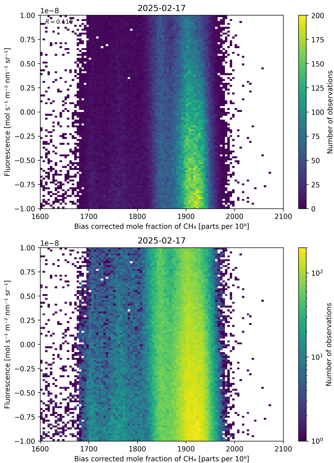
Figure 66: Scatter density plot of “Bias corrected mole fraction of \text{CH}_4 ” against “Fluorescence” for 2025-02-16 to 2025-02-18.
