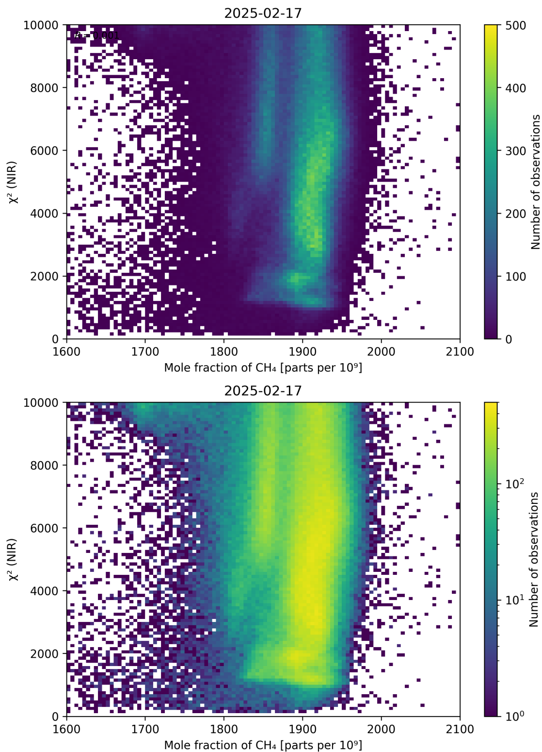
Figure 70: Scatter density plot of “Mole fraction of \text{CH}_4 ” against “ \chi^2 (NIR)” for 2025-02-16 to 2025-02-18.
