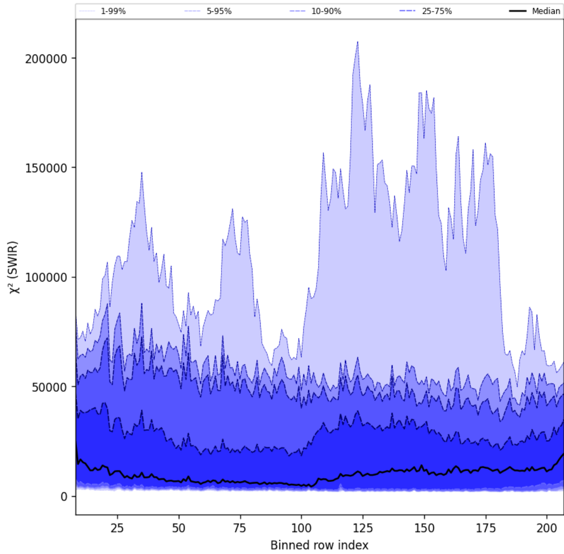
Figure 39: Along track statistics of “ \chi^2 (SWIR)” for 2025-02-16 to 2025-02-18
