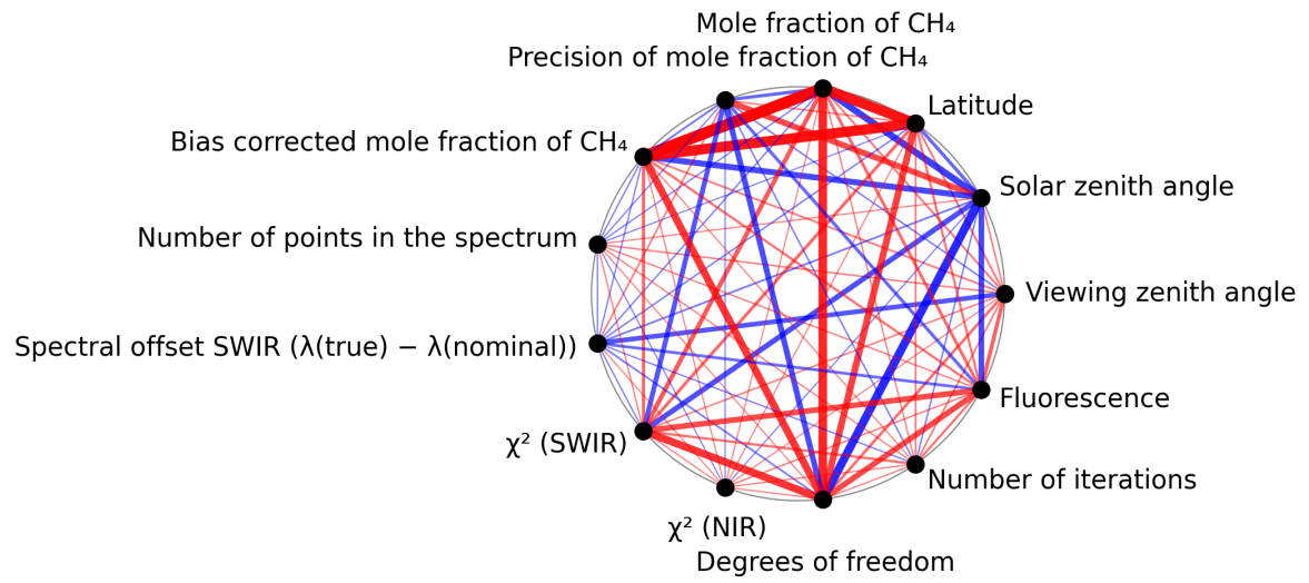
Figure 1: Map of correlation graph for 2025-02-16 to 2025-02-18.
