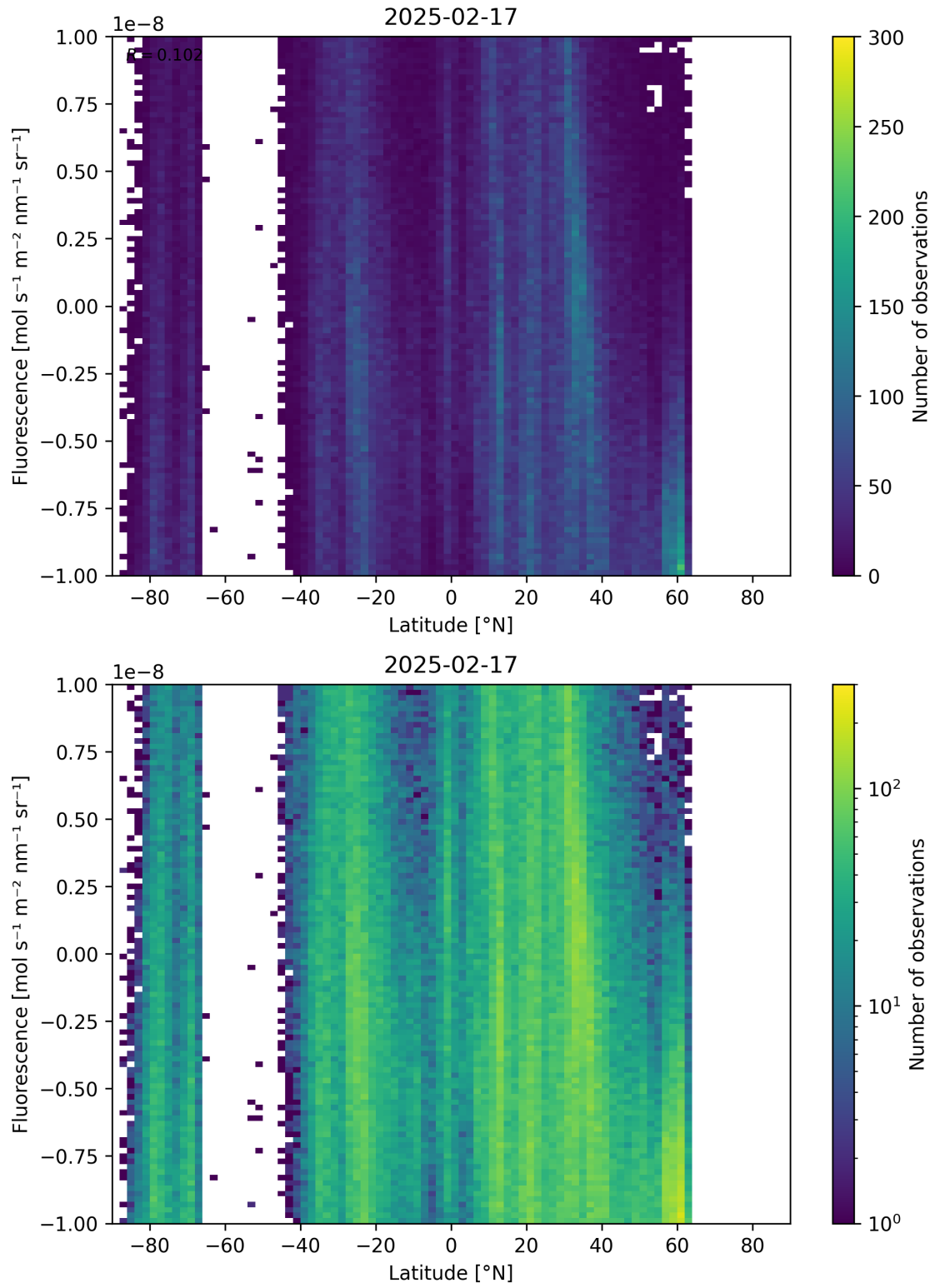
Figure 56: Scatter density plot of “Latitude” against “Fluorescence” for 2025-02-16 to 2025-02-18.
