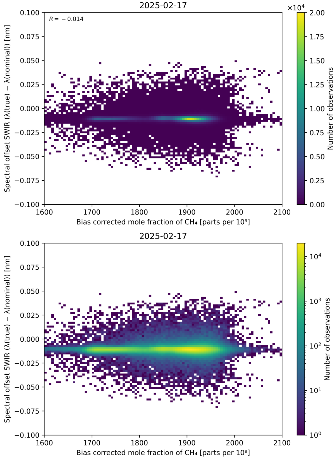
Figure 69: Scatter density plot of “Bias corrected mole fraction of \text{CH}_4 ” against “Spectral offset SWIR ( \lambda_{\text{true}} - \lambda_{\text{nominal}} )” for 2025-02-16 to 2025-02-18.
