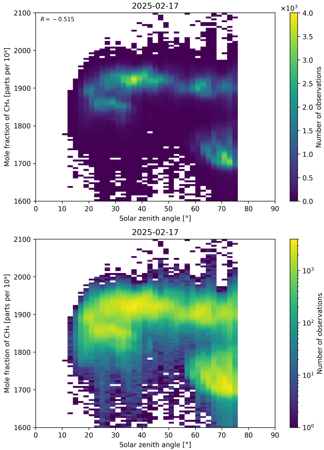
Figure 99: Scatter density plot of “Solar zenith angle” against “Mole fraction of CH 4 ” for 2025-02-16 to 2025-02-18.
