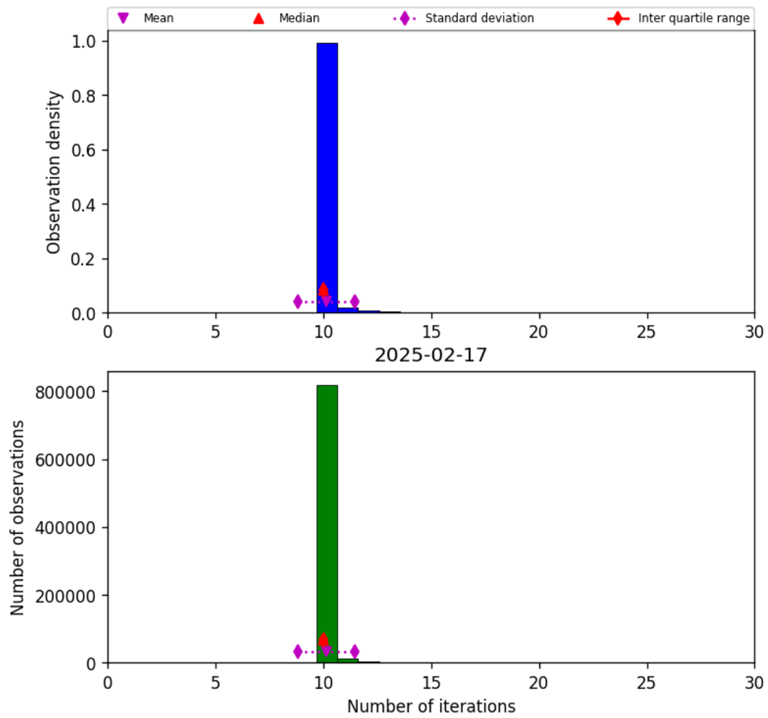
Figure 31: Histogram of “Number of iterations” for 2025-02-16 to 2025-02-18
