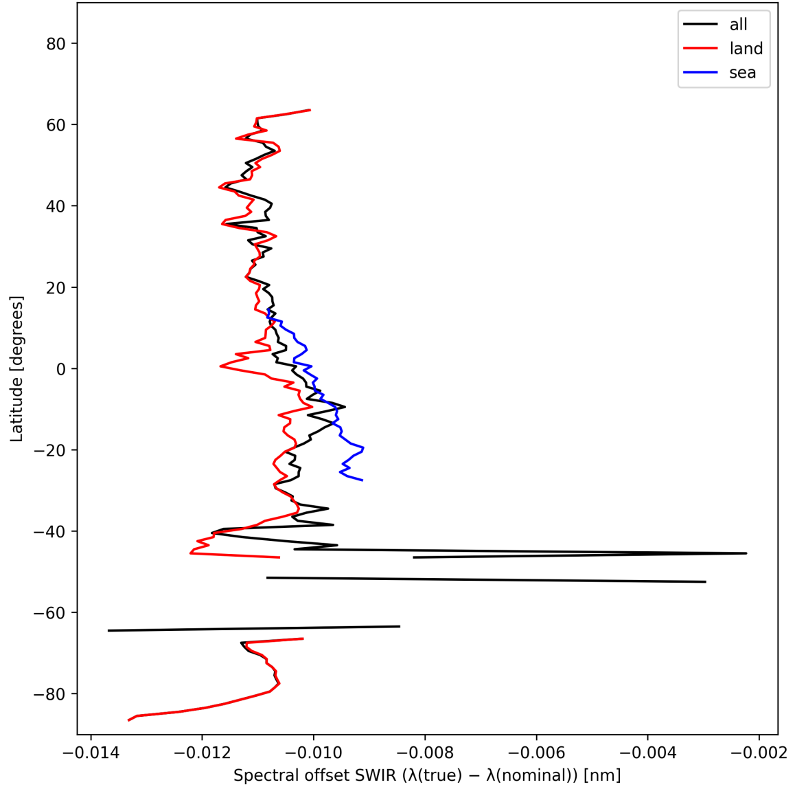
Figure 16: Zonal average of “Spectral offset SWIR ( \lambda_{\text{true}} - \lambda_{\text{nominal}} )” for 2025-02-16 to 2025-02-18.
