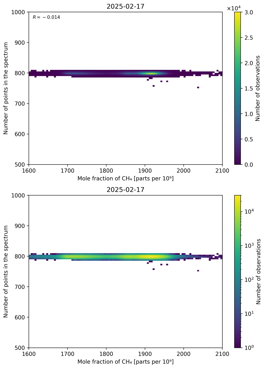
Figure 77: Scatter density plot of “Mole fraction of CH 4 ” against “Number of points in the spectrum” for 2025-02-16 to 2025-02-18.
