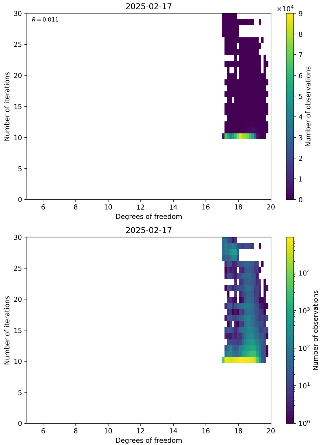
Figure 52: Scatter density plot of “Degrees of freedom” against “Number of iterations” for 2025-02-16 to 2025-02-18.
