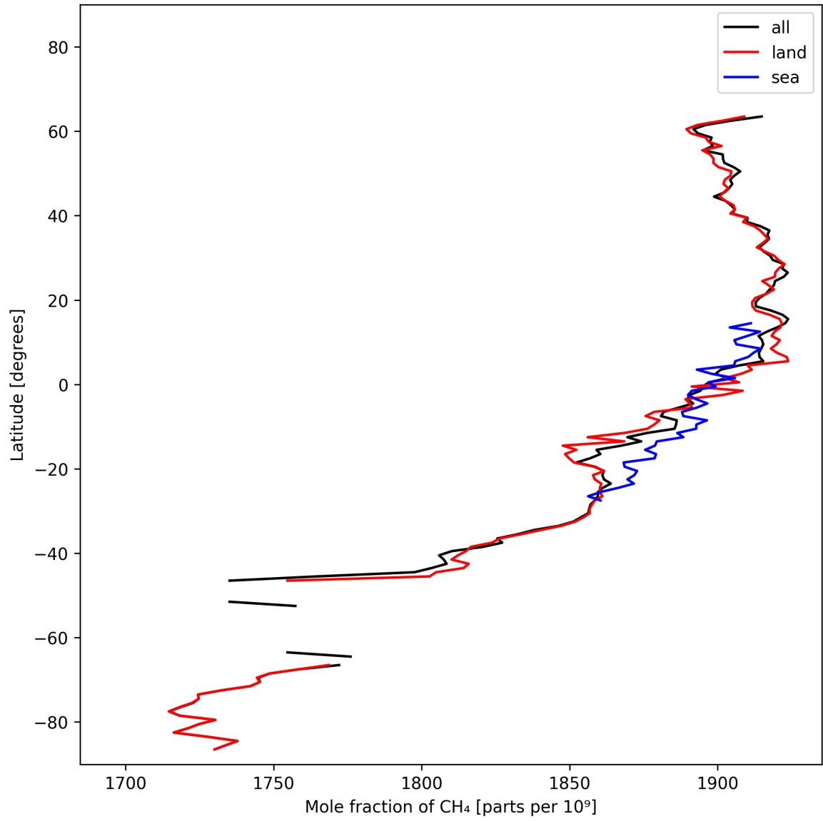
Figure 12: Zonal average of “Mole fraction of CH 4 ” for 2025-02-16 to 2025-02-18.
