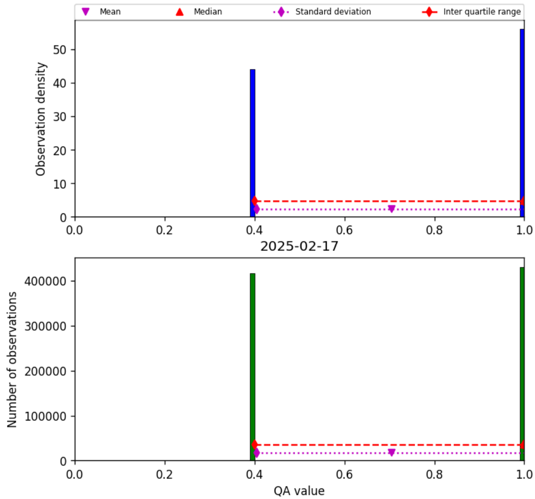
Figure 22: Histogram of “QA value” for 2025-02-16 to 2025-02-18
