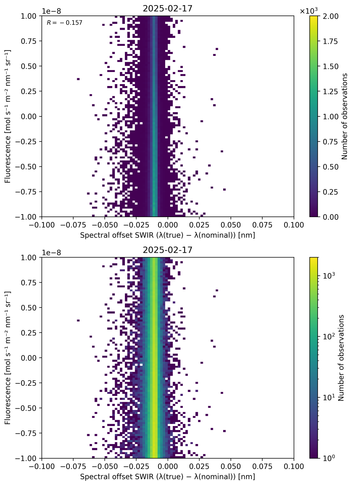
Figure 120: Scatter density plot of “Spectral offset SWIR ( \lambda_{\text{true}} - \lambda_{\text{nominal}} )” against “Fluorescence” for 2025-02-16 to 2025-02-18.
