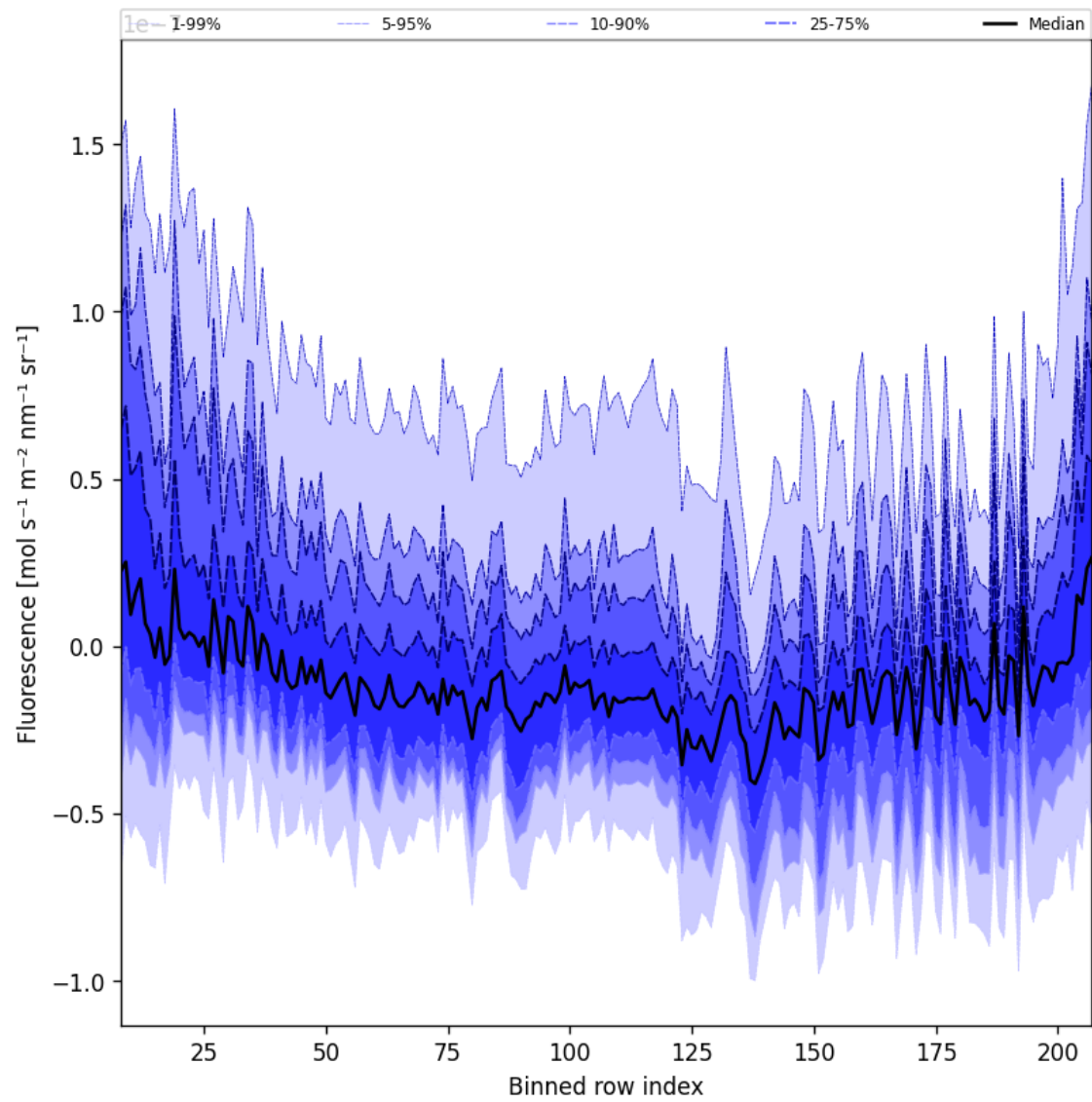
Figure 43: Along track statistics of “Fluorescence” for 2025-02-16 to 2025-02-18
