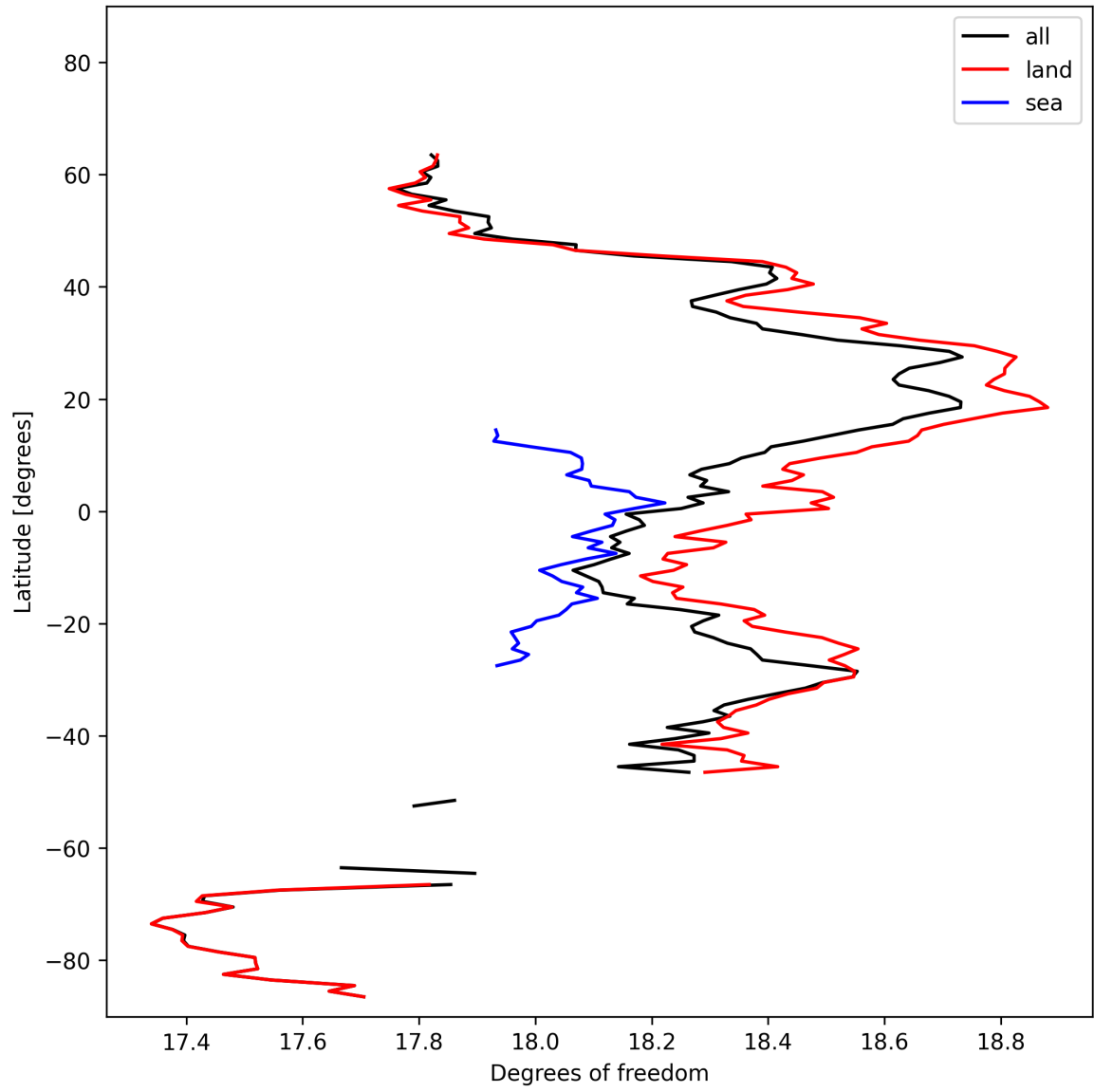
Figure 19: Zonal average of “Degrees of freedom” for 2025-02-16 to 2025-02-18.
