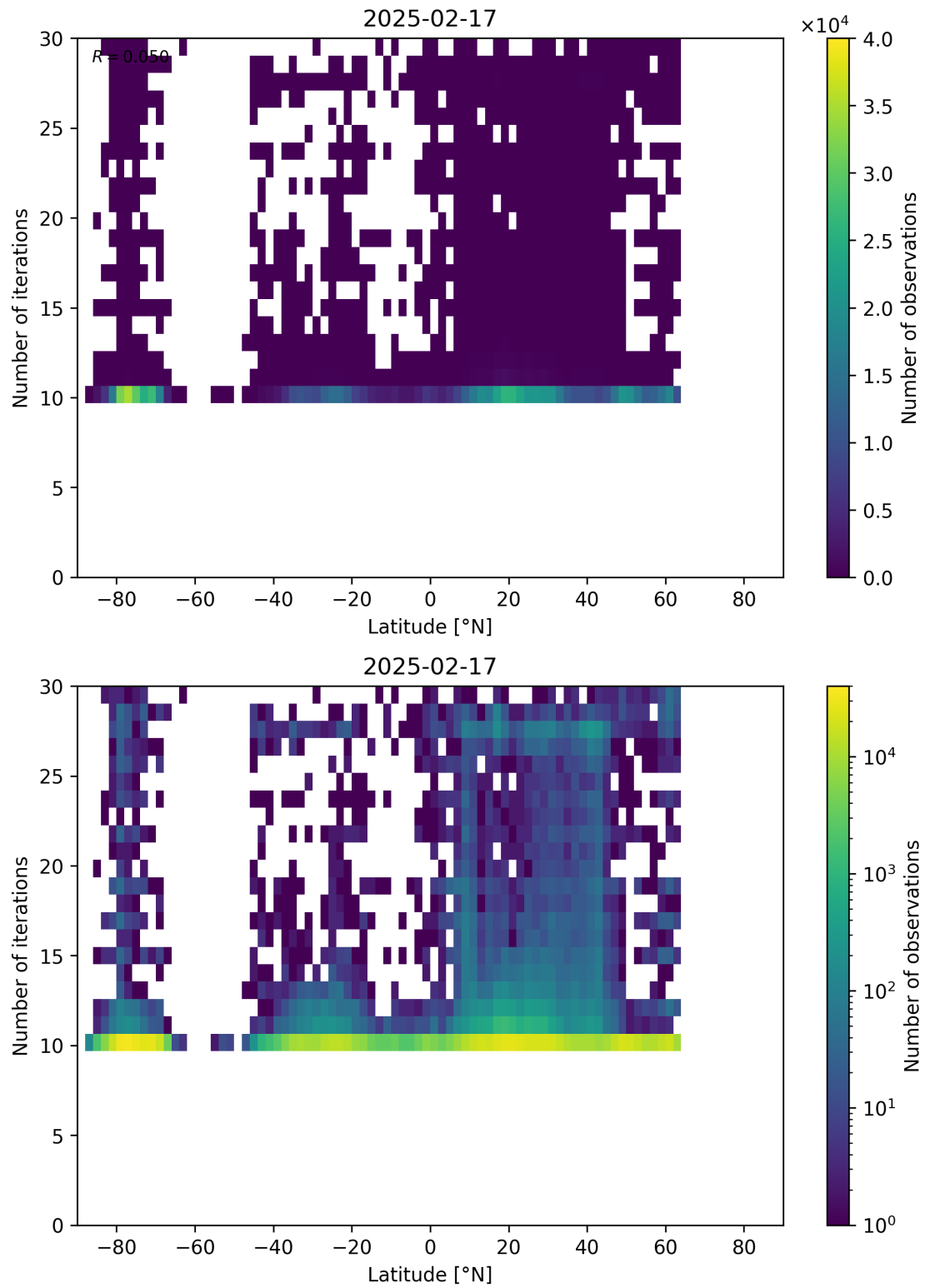
Figure 60: Scatter density plot of “Latitude” against “Number of iterations” for 2025-02-16 to 2025-02-18.
