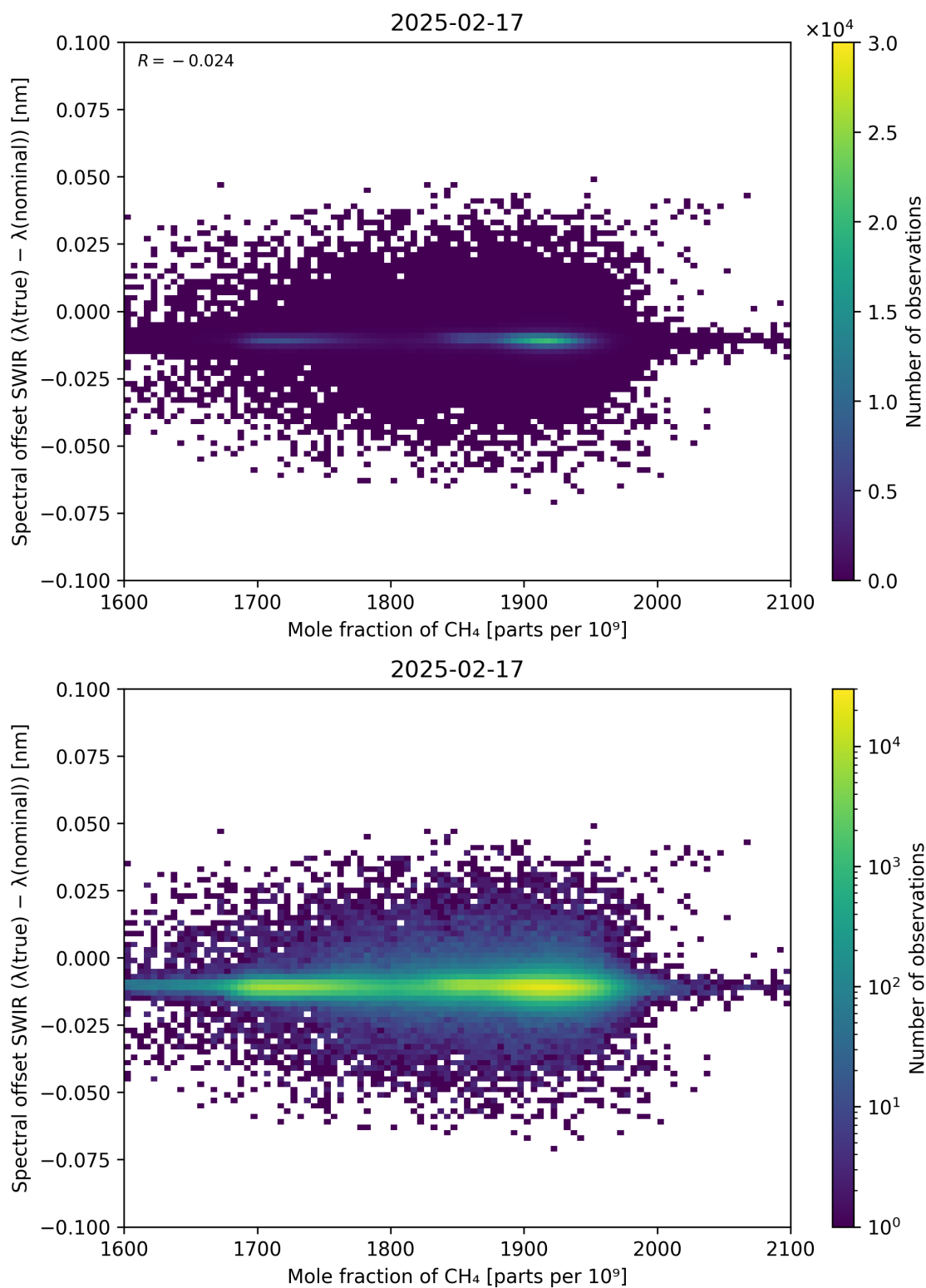
Figure 86: Scatter density plot of “Mole fraction of CH 4 ” against “Spectral offset SWIR ( \lambda_{\text{true}} - \lambda_{\text{nominal}} )” for 2025-02-16 to 2025-02-18.
