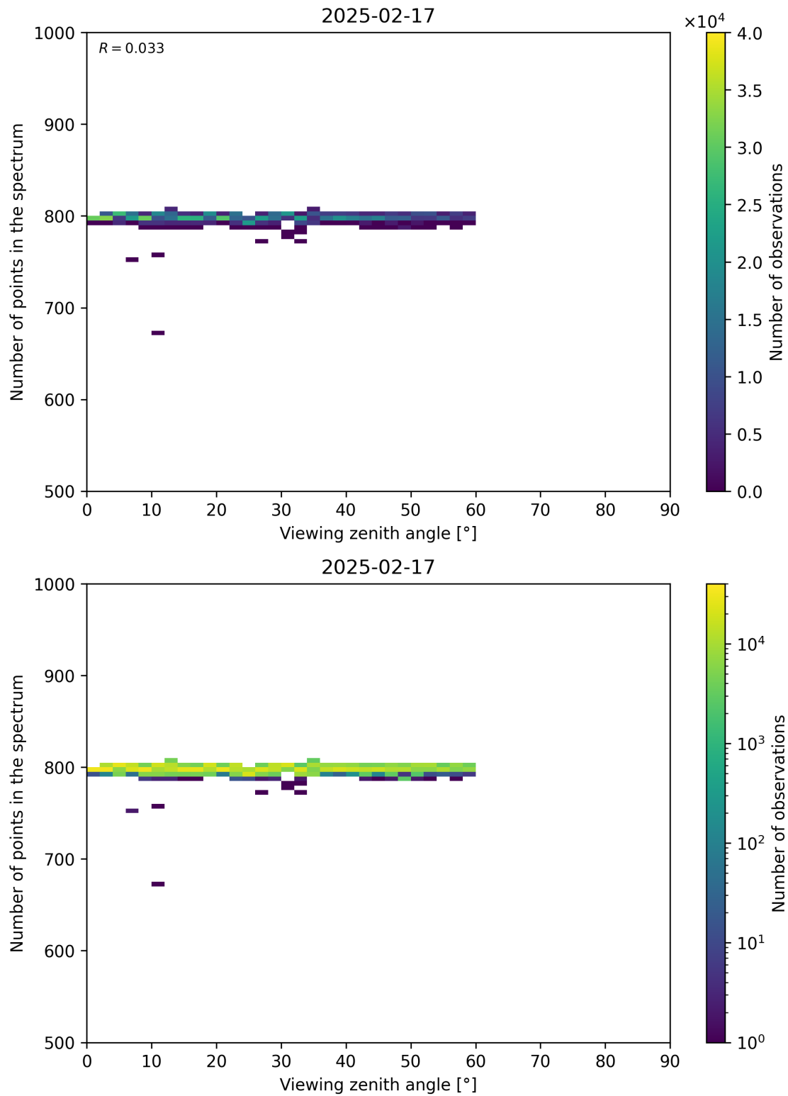
Figure 114: Scatter density plot of “Viewing zenith angle” against “Number of points in the spectrum” for 2025-02-16 to 2025-02-18.
