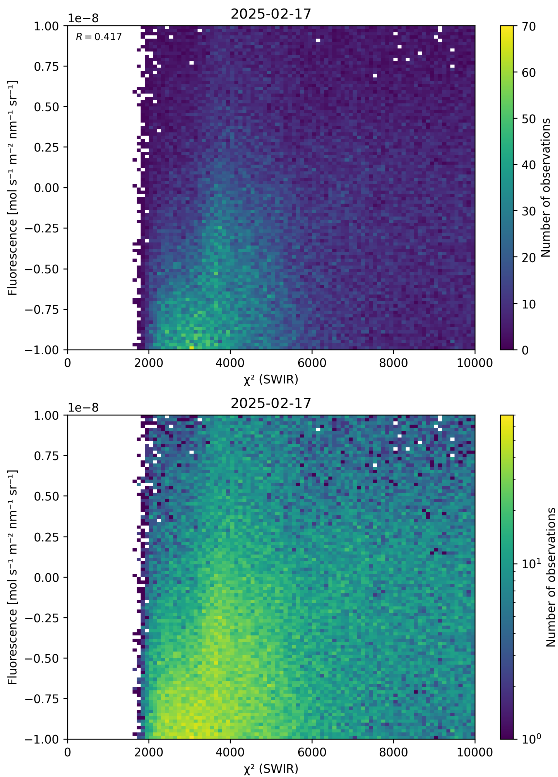
Figure 49: Scatter density plot of “ \chi^2 (SWIR)” against “Fluorescence” for 2025-02-16 to 2025-02-18.
