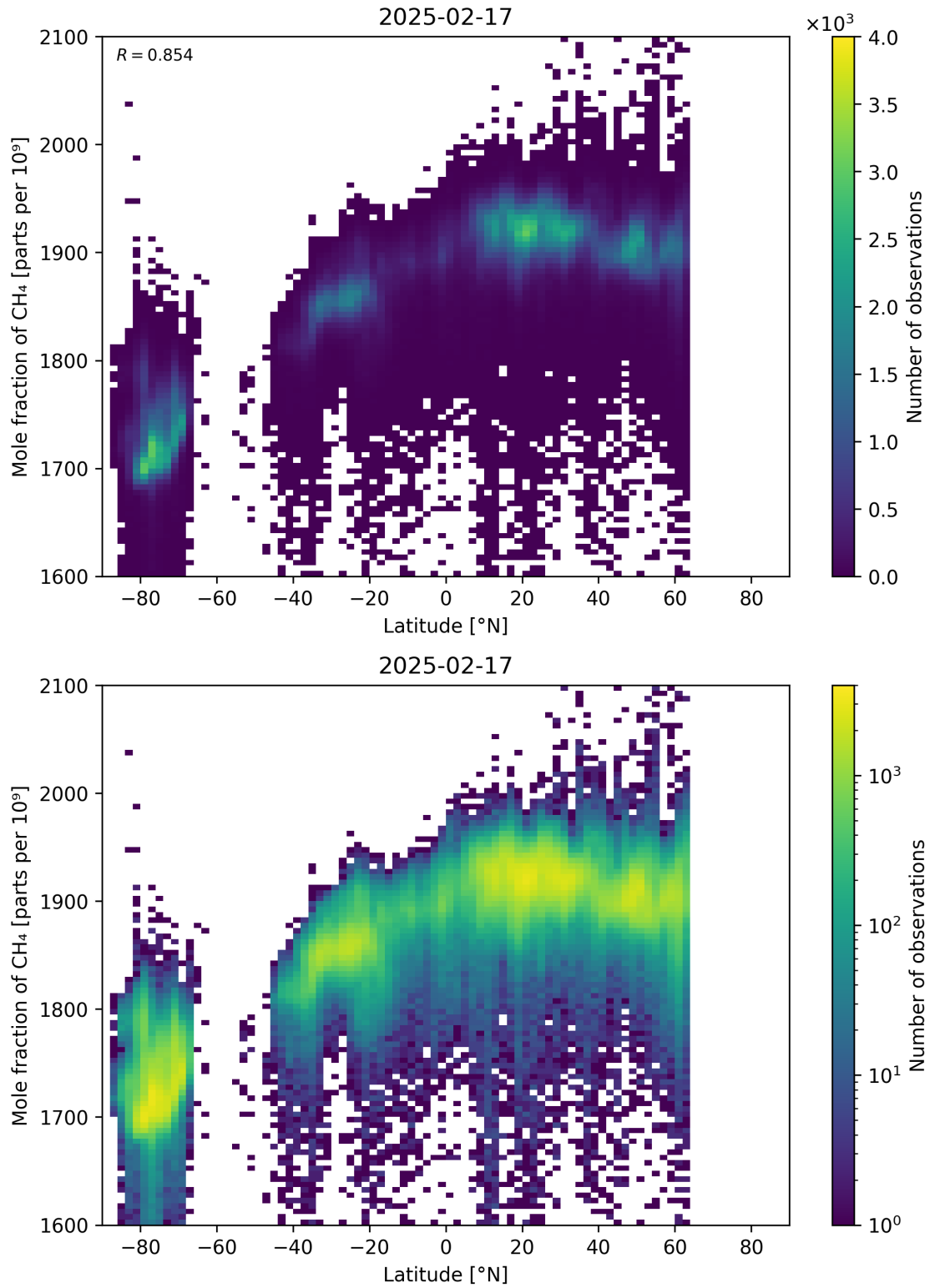
Figure 57: Scatter density plot of “Latitude” against “Mole fraction of CH 4 ” for 2025-02-16 to 2025-02-18.
