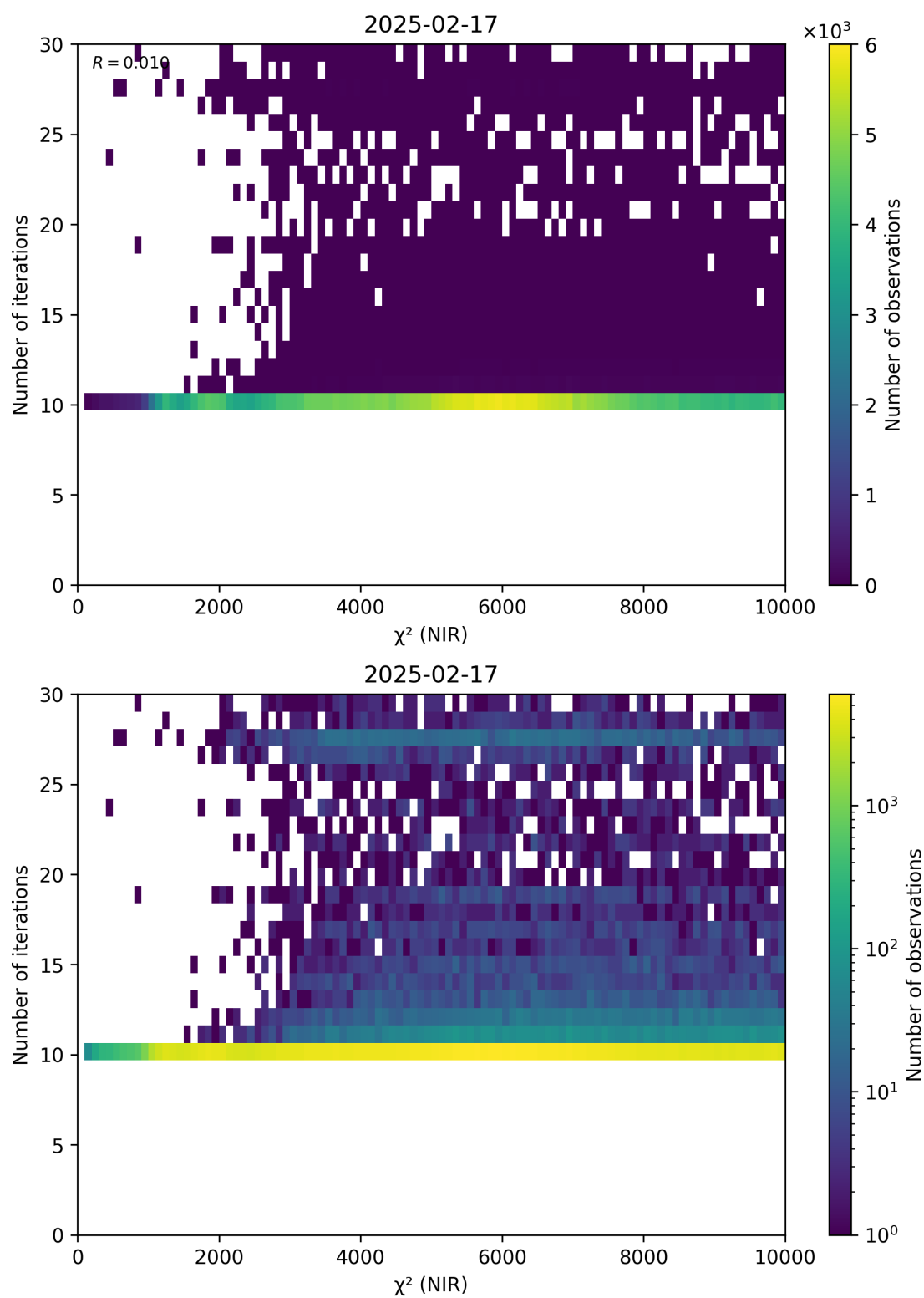
Figure 46: Scatter density plot of “ \chi^2 (NIR)” against “Number of iterations” for 2025-02-16 to 2025-02-18.
