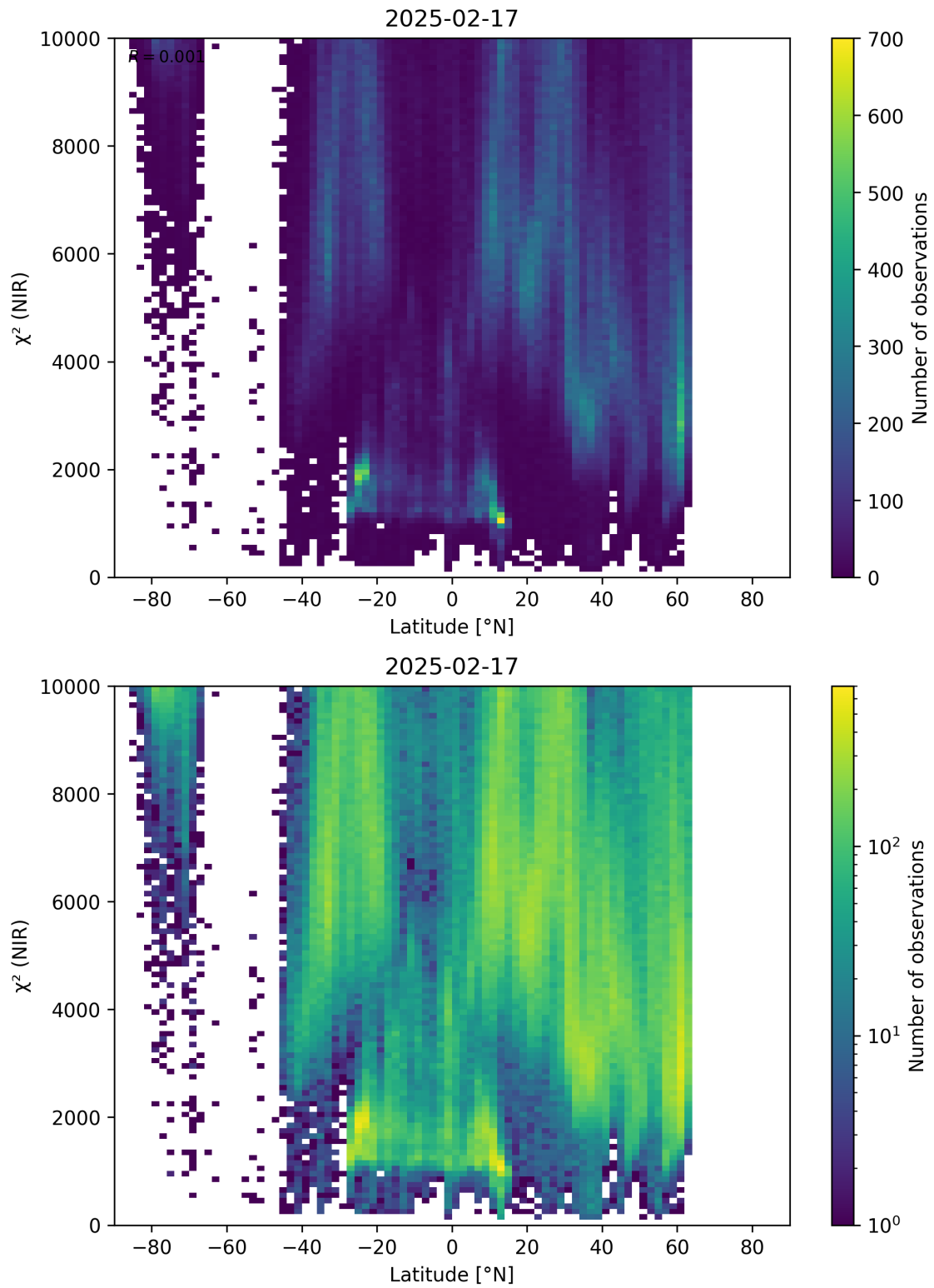
Figure 53: Scatter density plot of “Latitude” against “ \chi^2 (NIR)” for 2025-02-16 to 2025-02-18.
