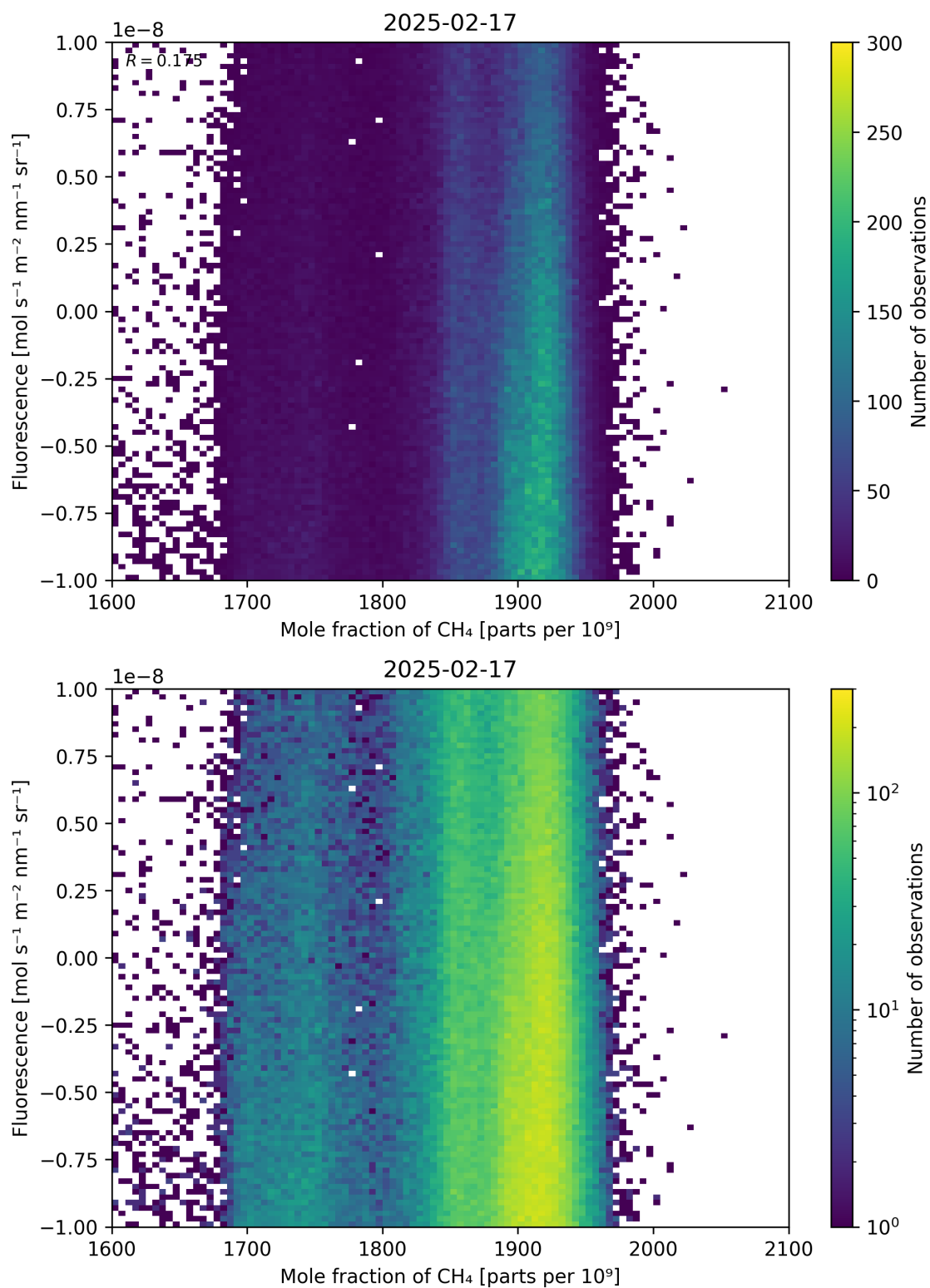
Figure 73: Scatter density plot of “Mole fraction of \text{CH}_4 ” against “Fluorescence” for 2025-02-16 to 2025-02-18.
