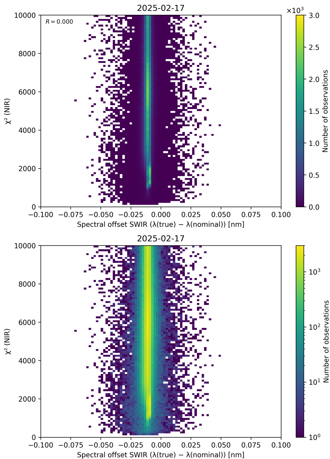
Figure 117: Scatter density plot of “Spectral offset SWIR ( \lambda_{\text{true}} - \lambda_{\text{nominal}} )” against “ \chi^2 (NIR)” for 2025-02-16 to 2025-02-18.
