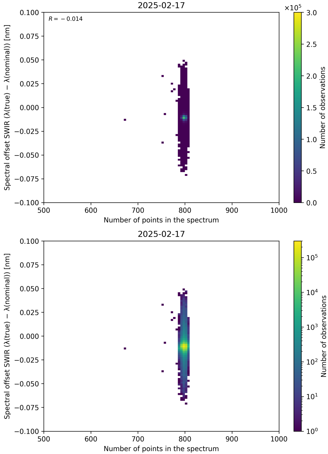
Figure 93: Scatter density plot of “Number of points in the spectrum” against “Spectral offset SWIR ( \lambda_{\text{true}} - \lambda_{\text{nominal}} )” for 2025-02-16 to 2025-02-18.
