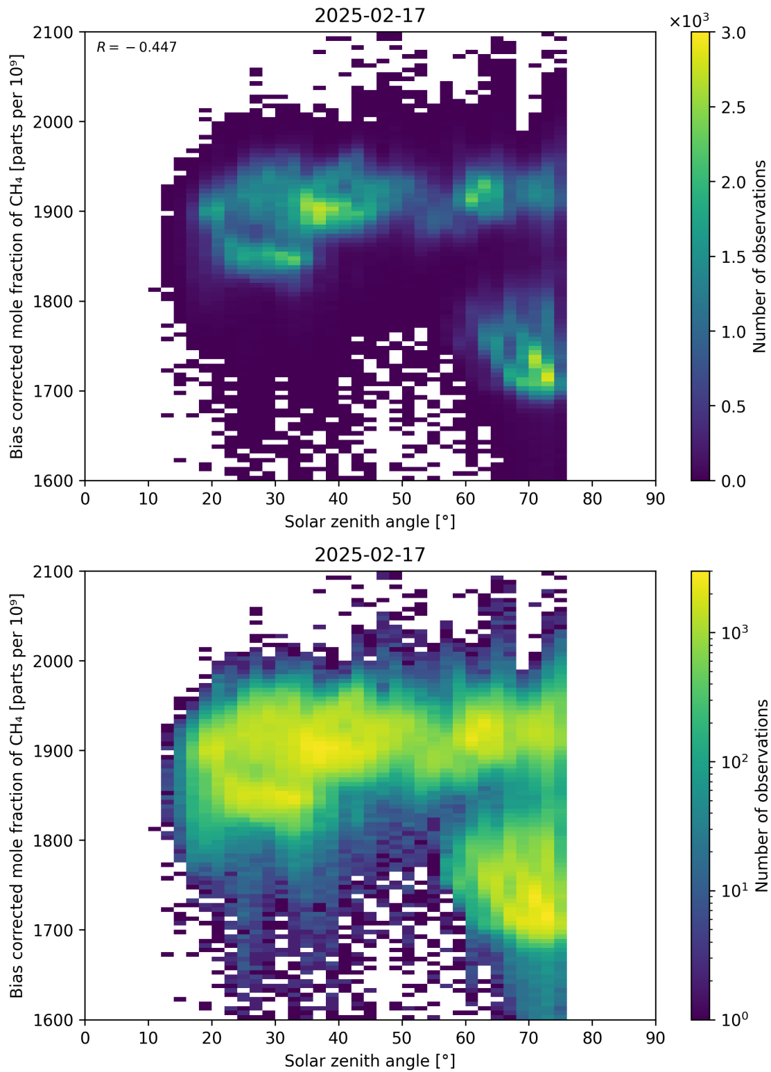
Figure 100: Scatter density plot of “Solar zenith angle” against “Bias corrected mole fraction of \text{CH}_4 ” for 2025-02-16 to 2025-02-18.
