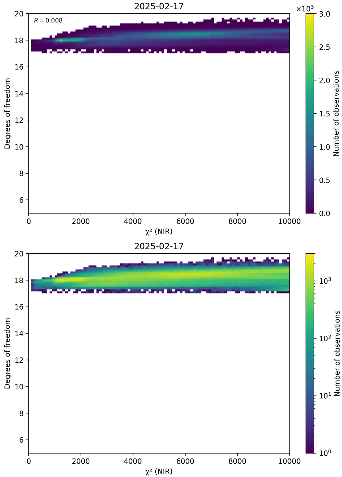
Figure 44: Scatter density plot of “ \chi^2 (NIR)” against “Degrees of freedom” for 2025-02-16 to 2025-02-18.
