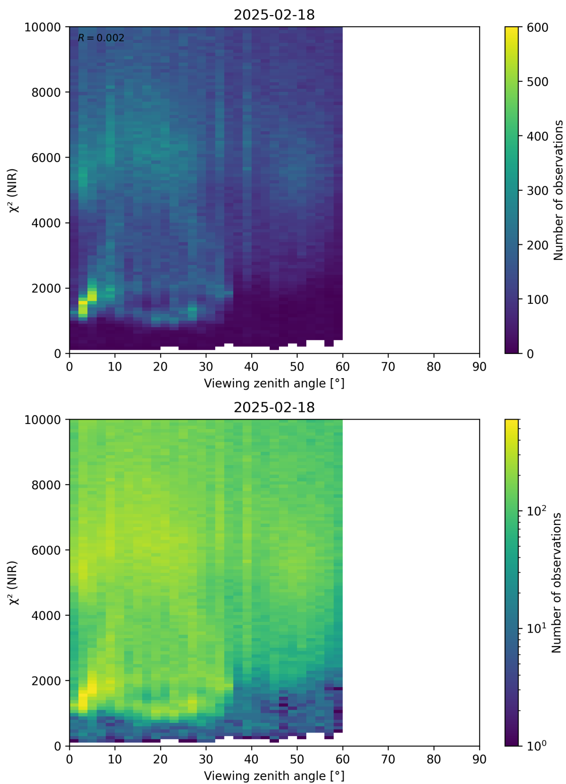
Figure 105: Scatter density plot of “Viewing zenith angle” against “ \chi^2 (NIR)” for 2025-02-18 to 2025-02-19.
