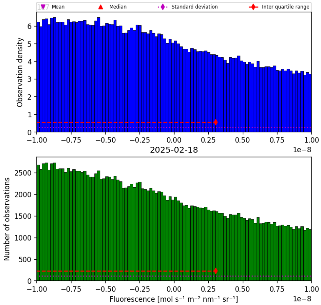
Figure 32: Histogram of “Fluorescence” for 2025-02-18 to 2025-02-19
