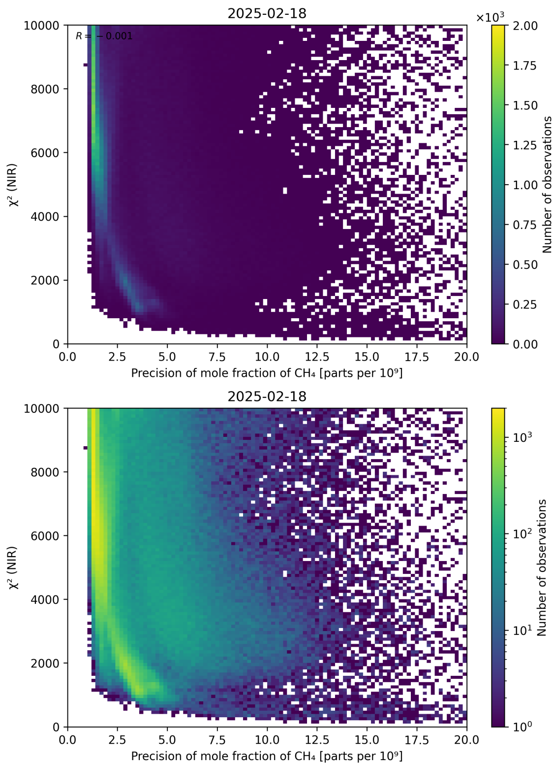
Figure 78: Scatter density plot of “Precision of mole fraction of CH 4 ” against “ \chi^2 (NIR)” for 2025-02-18 to 2025-02-19.
