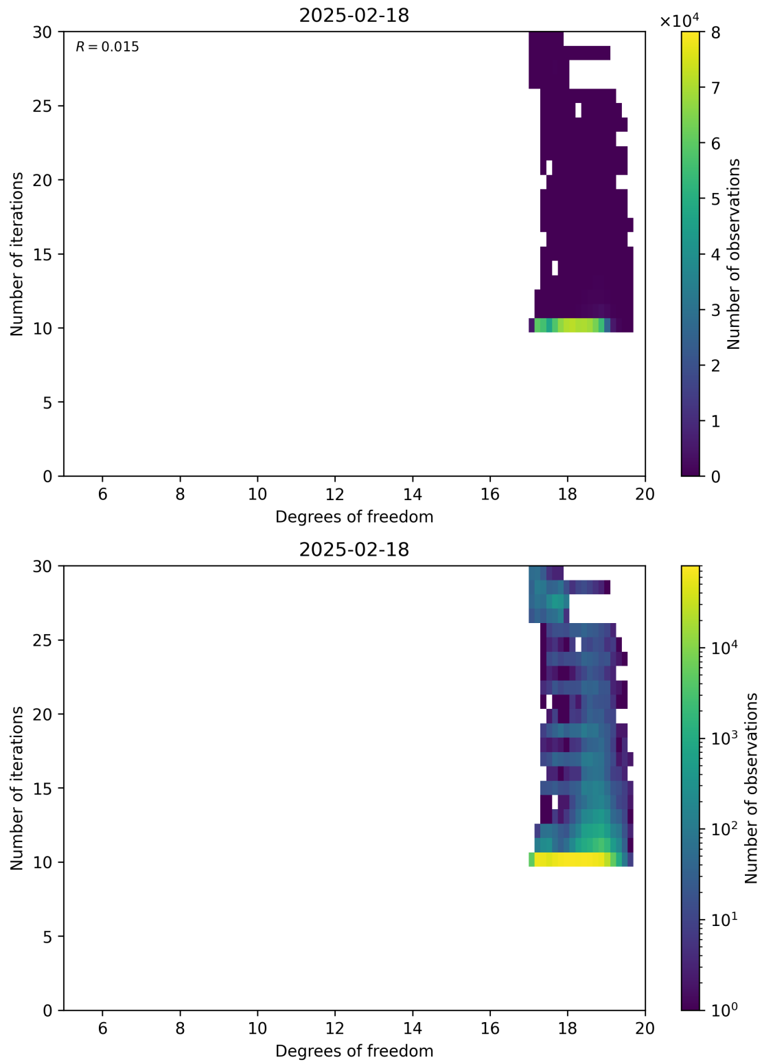
Figure 52: Scatter density plot of “Degrees of freedom” against “Number of iterations” for 2025-02-18 to 2025-02-19.
