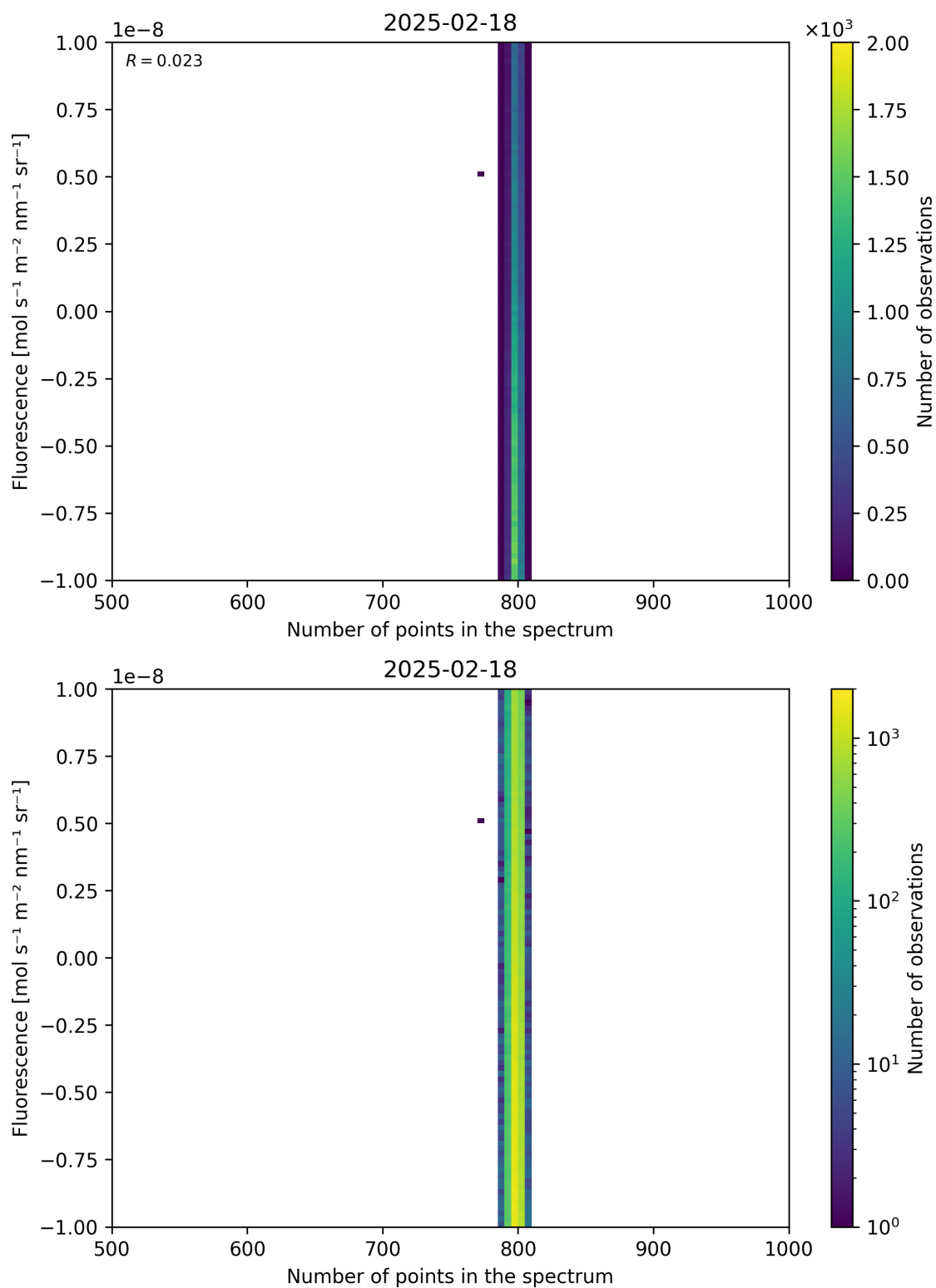
Figure 91: Scatter density plot of “Number of points in the spectrum” against “Fluorescence” for 2025-02-18 to 2025-02-19.
