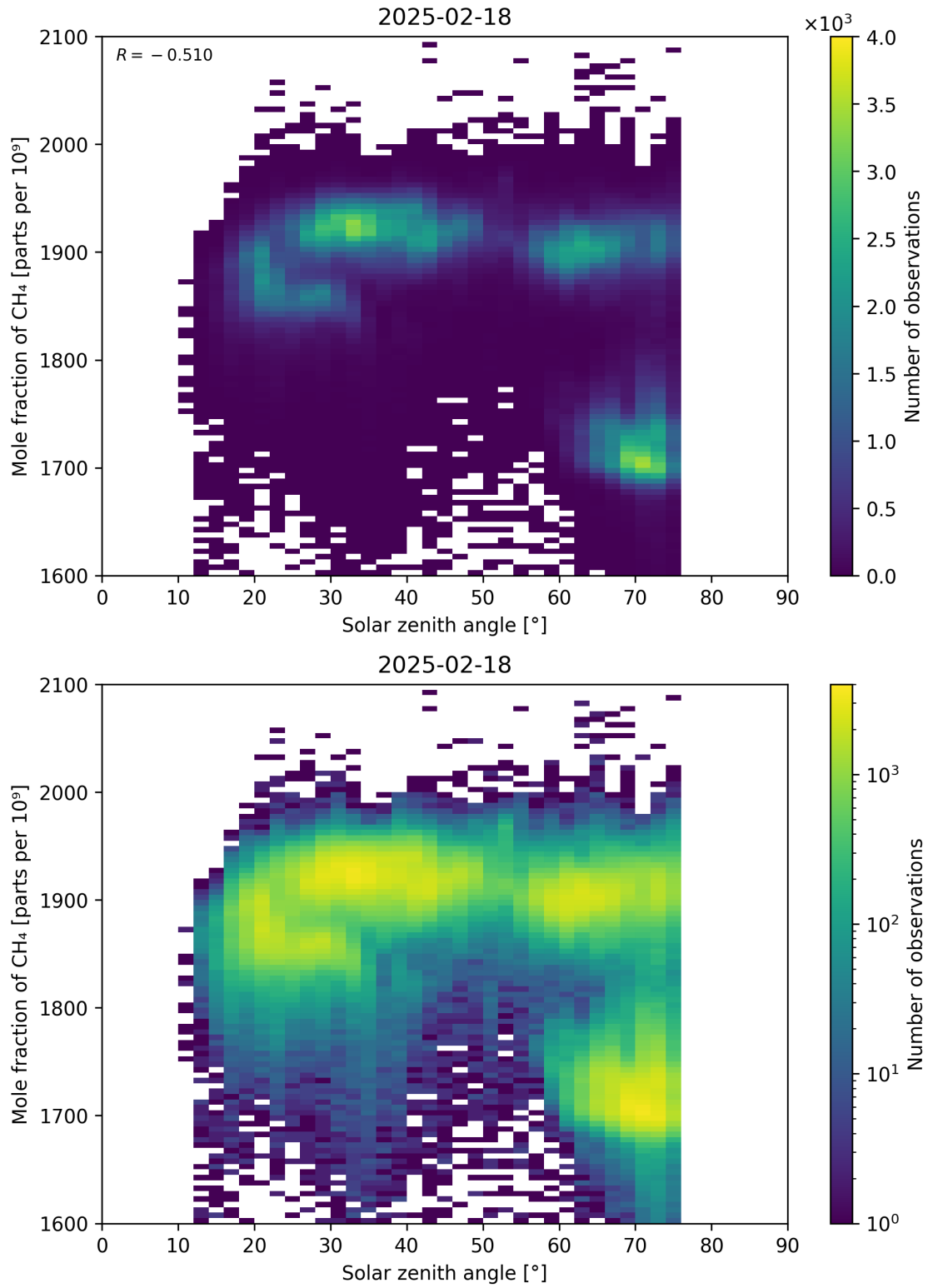
Figure 99: Scatter density plot of “Solar zenith angle” against “Mole fraction of CH 4 ” for 2025-02-18 to 2025-02-19.
