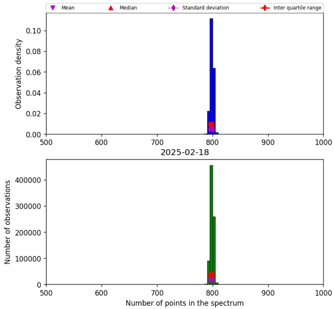
Figure 26: Histogram of “Number of points in the spectrum” for 2025-02-18 to 2025-02-19
