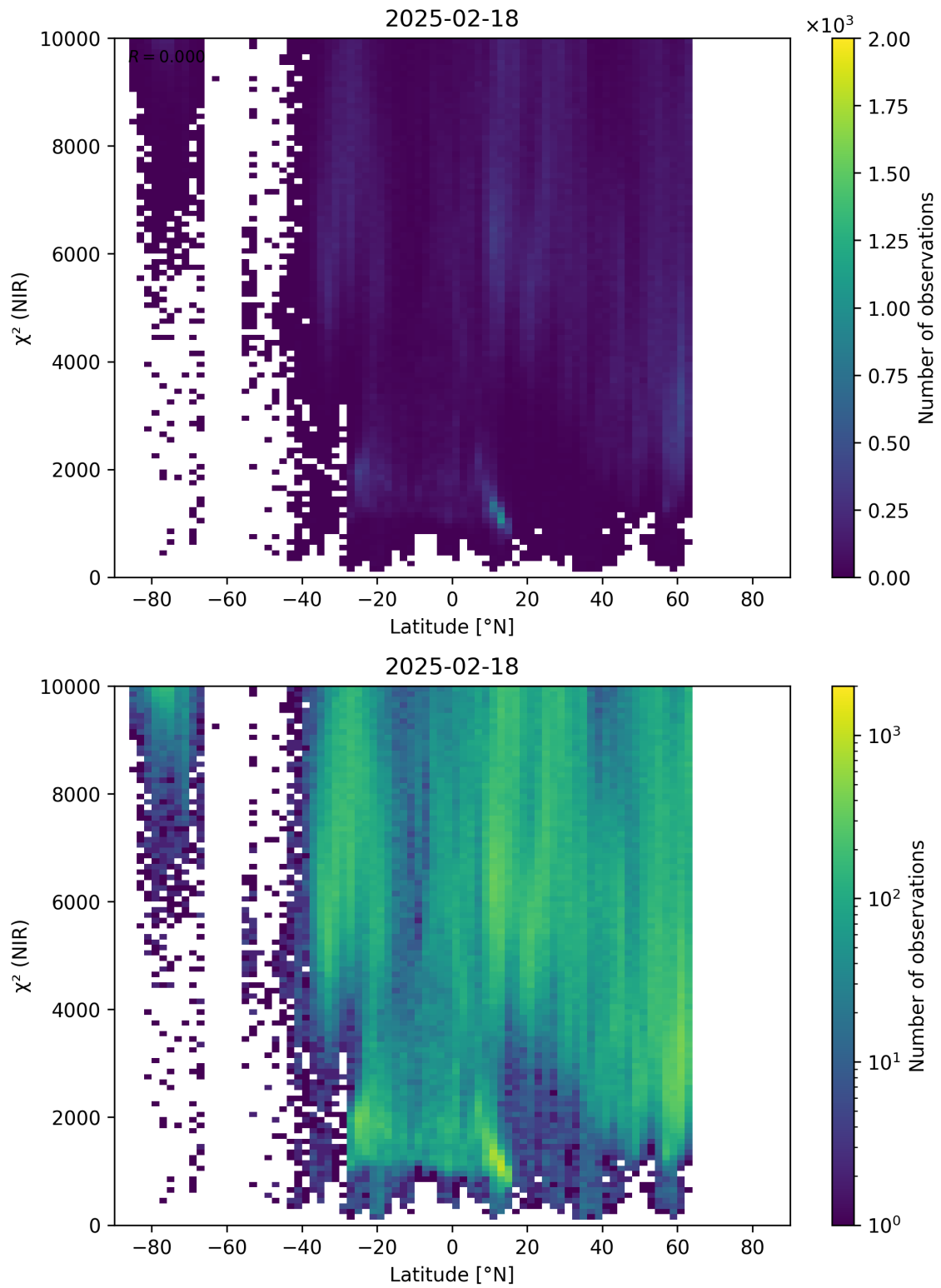
Figure 53: Scatter density plot of “Latitude” against “ \chi^2 (NIR)” for 2025-02-18 to 2025-02-19.
