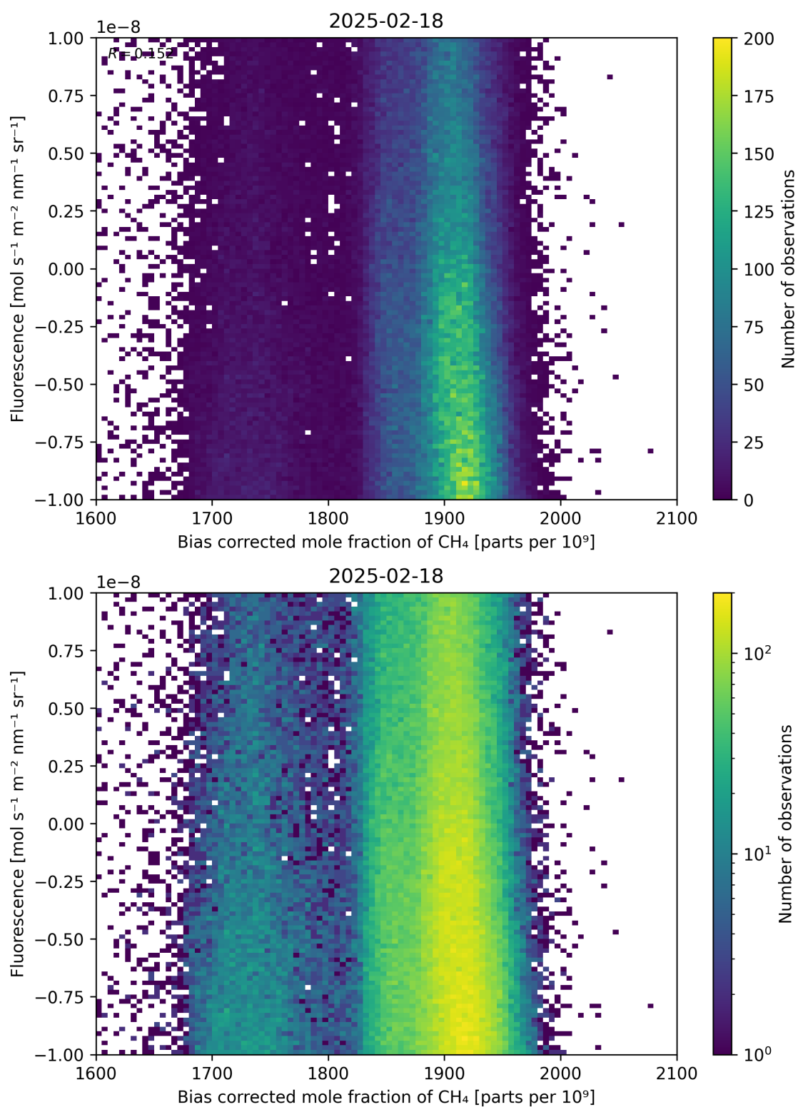
Figure 66: Scatter density plot of “Bias corrected mole fraction of \text{CH}_4 ” against “Fluorescence” for 2025-02-18 to 2025-02-19.
