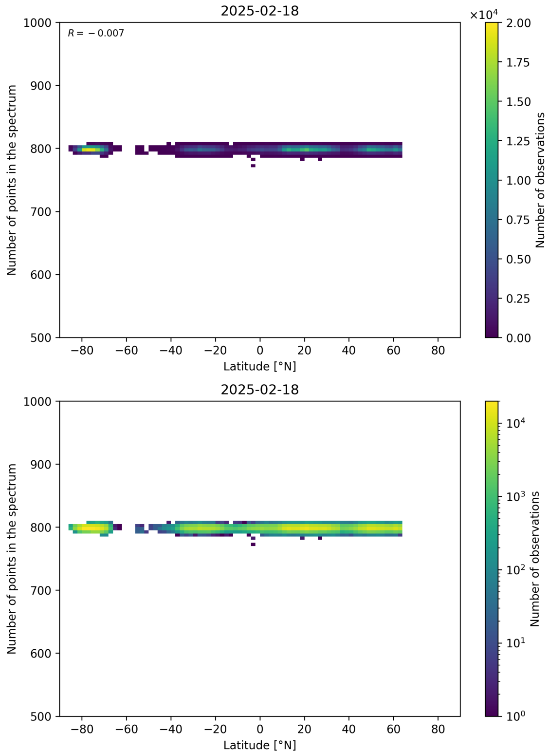
Figure 61: Scatter density plot of “Latitude” against “Number of points in the spectrum” for 2025-02-18 to 2025-02-19.
