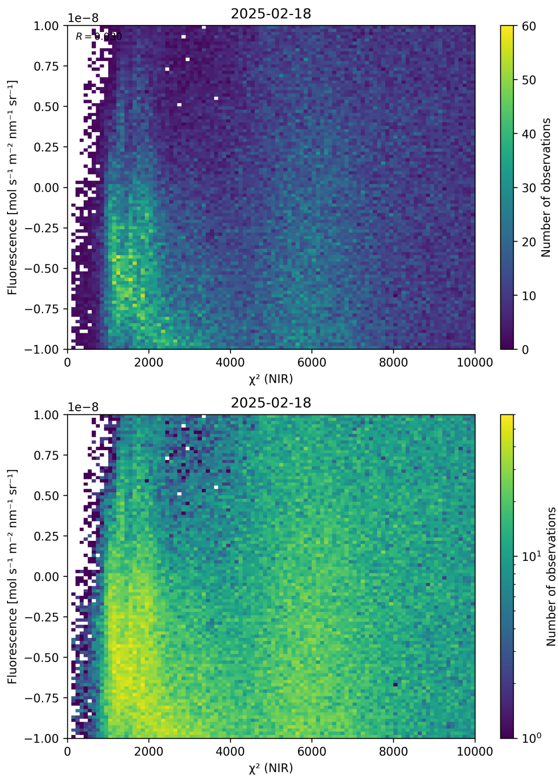
Figure 45: Scatter density plot of “ \chi^2 (NIR)” against “Fluorescence” for 2025-02-18 to 2025-02-19.
