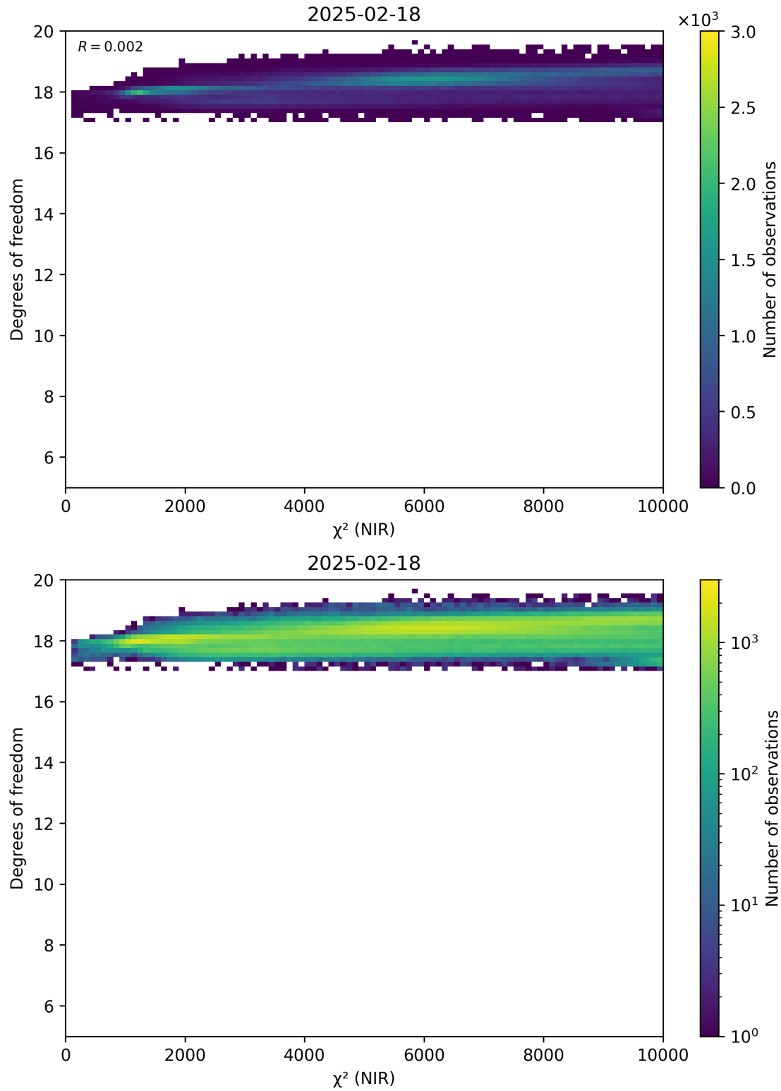
Figure 44: Scatter density plot of “ \chi^2 (NIR)” against “Degrees of freedom” for 2025-02-18 to 2025-02-19.
