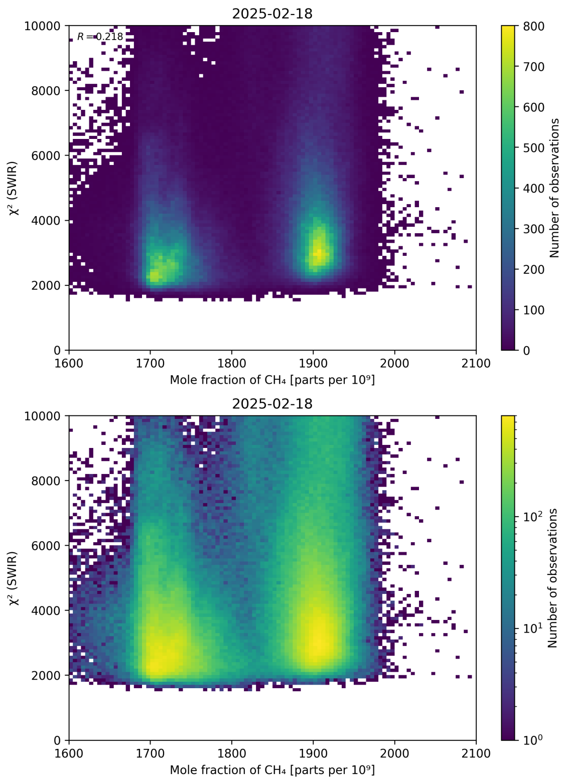
Figure 71: Scatter density plot of “Mole fraction of \text{CH}_4 ” against “ \chi^2 (SWIR)” for 2025-02-18 to 2025-02-19.
