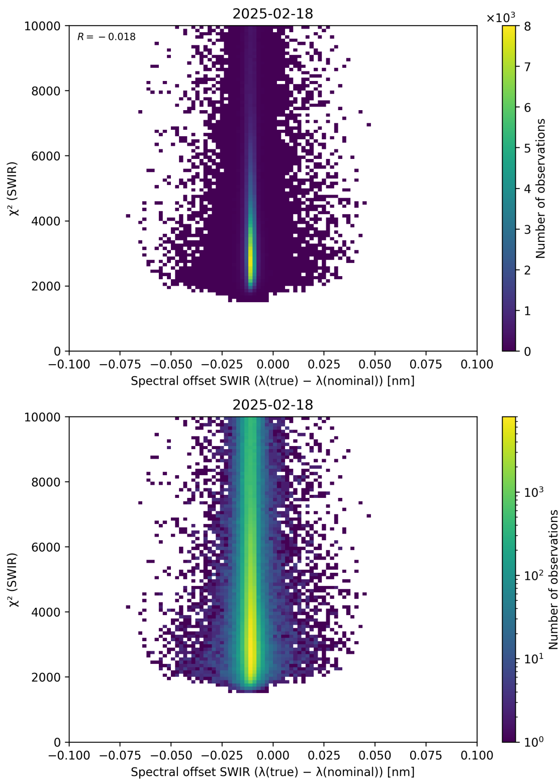
Figure 118: Scatter density plot of “Spectral offset SWIR ( \lambda_{\text{true}} - \lambda_{\text{nominal}} )” against “ \chi^2 (SWIR)” for 2025-02-18 to 2025-02-19.
