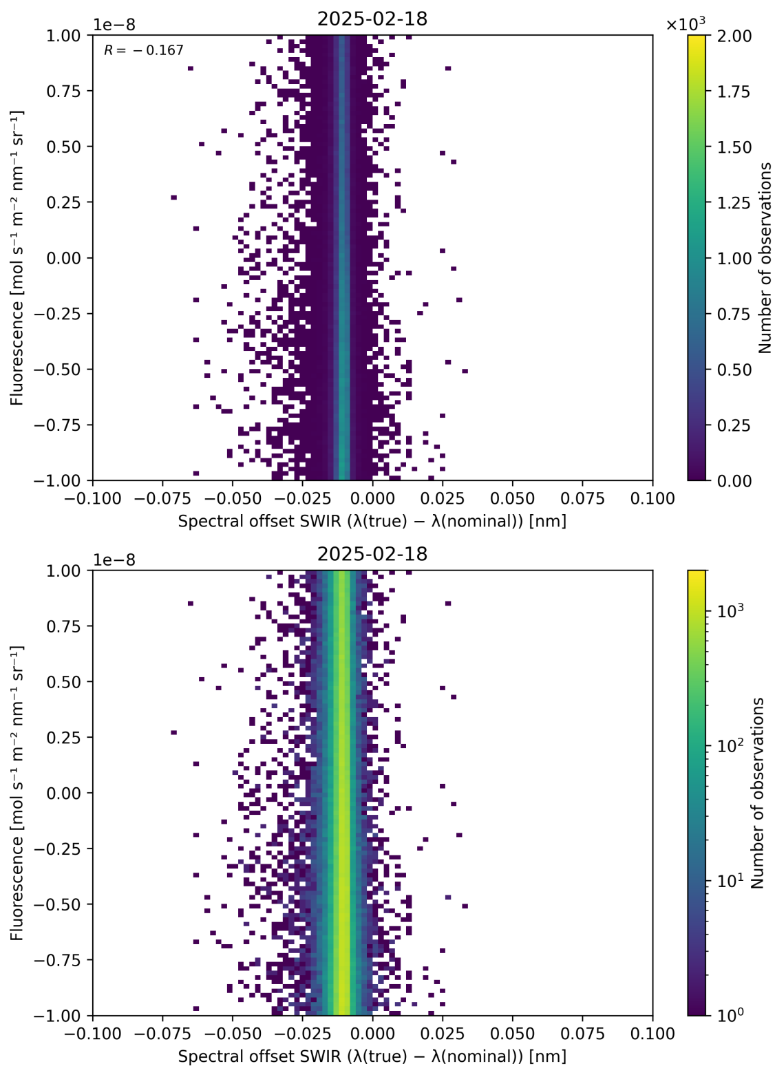
Figure 120: Scatter density plot of “Spectral offset SWIR ( \lambda_{\text{true}} - \lambda_{\text{nominal}} )” against “Fluorescence” for 2025-02-18 to 2025-02-19.
