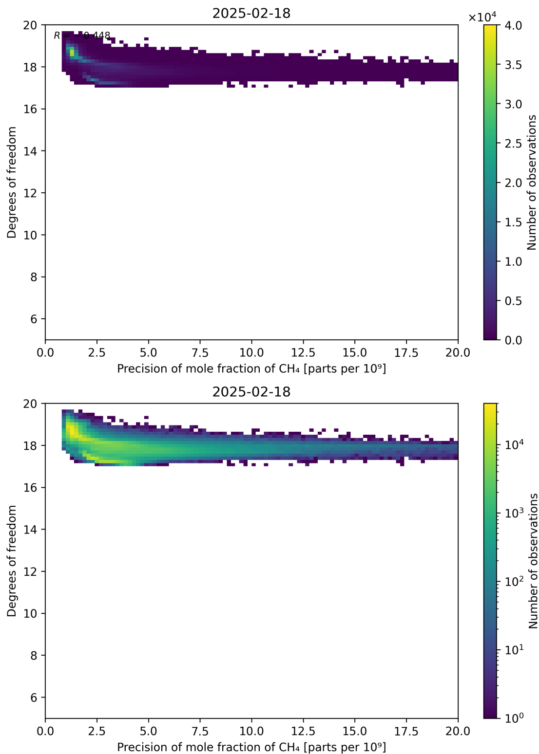
Figure 80: Scatter density plot of “Precision of mole fraction of CH 4 ” against “Degrees of freedom” for 2025-02-18 to 2025-02-19.
