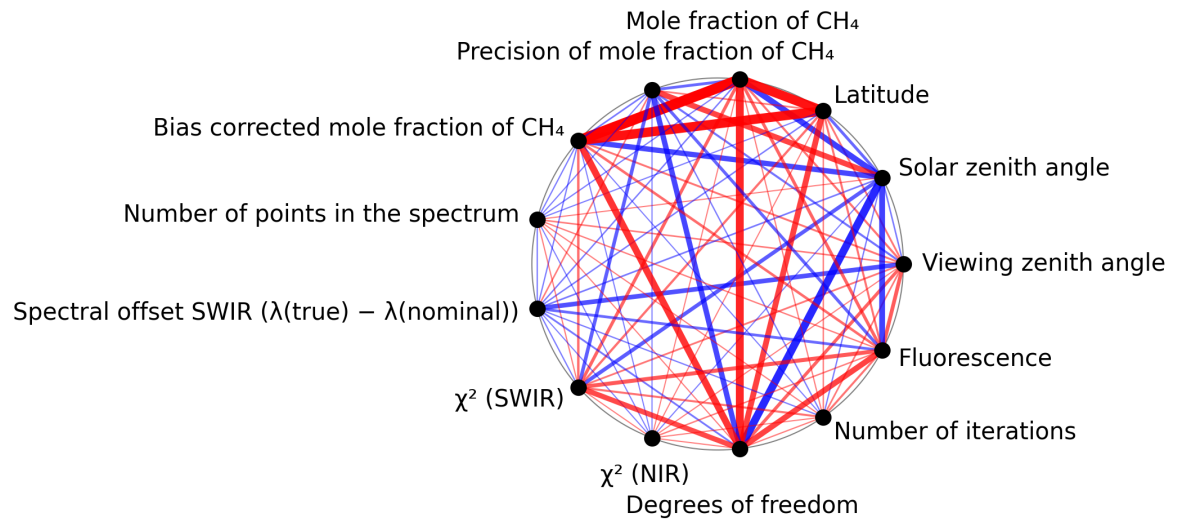
Figure 1: Map of correlation graph for 2025-02-18 to 2025-02-19.
