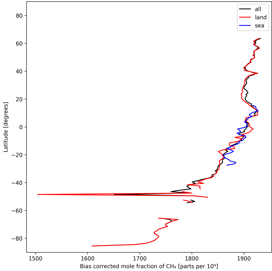
Figure 14: Zonal average of “Bias corrected mole fraction of CH 4 ” for 2025-02-18 to 2025-02-19.
