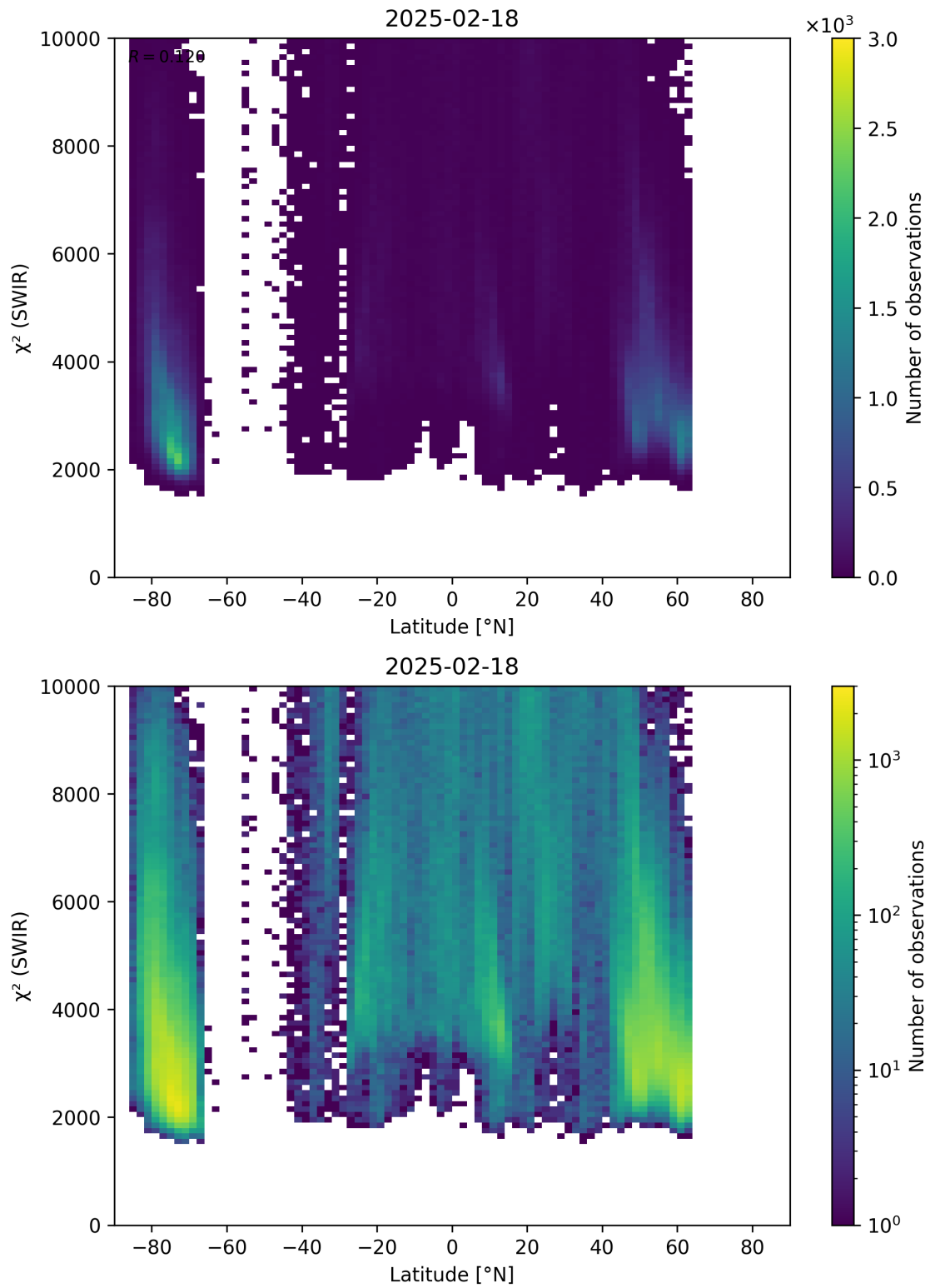
Figure 54: Scatter density plot of “Latitude” against “ \chi^2 (SWIR)” for 2025-02-18 to 2025-02-19.
