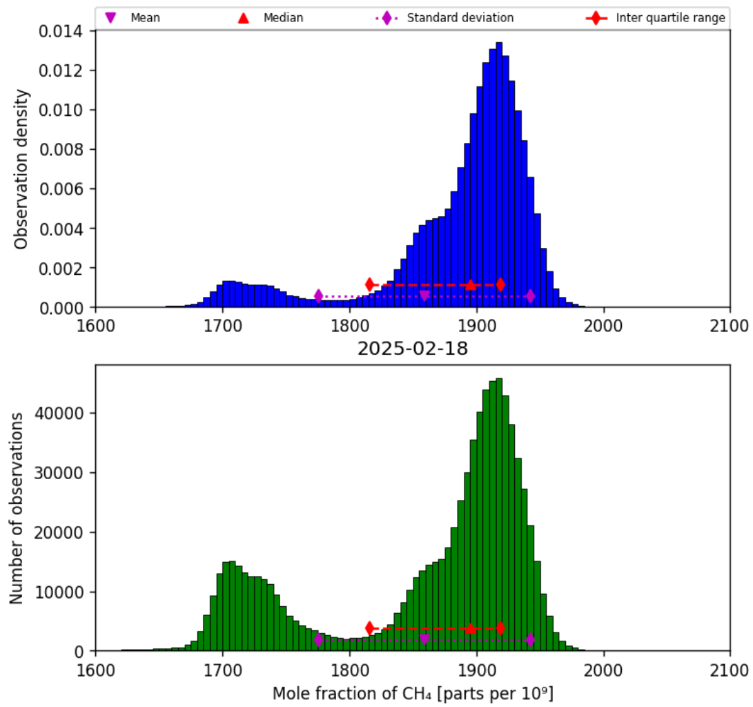
Figure 23: Histogram of “Mole fraction of CH 4 ” for 2025-02-18 to 2025-02-19
