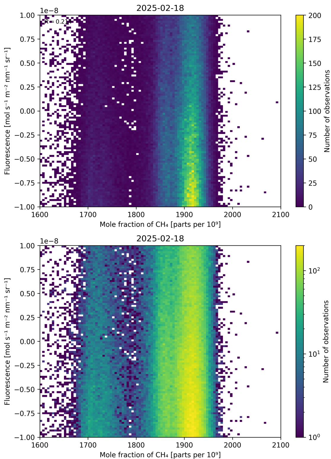
Figure 73: Scatter density plot of “Mole fraction of \text{CH}_4 ” against “Fluorescence” for 2025-02-18 to 2025-02-19.
