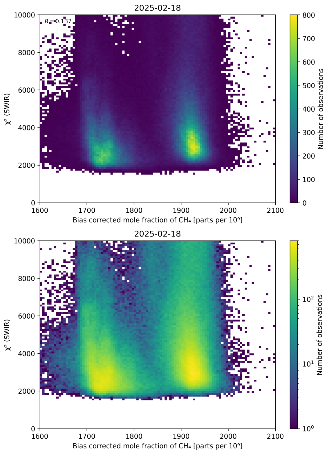
Figure 64: Scatter density plot of “Bias corrected mole fraction of CH 4 ” against “ \chi^2 (SWIR)” for 2025-02-18 to 2025-02-19.
