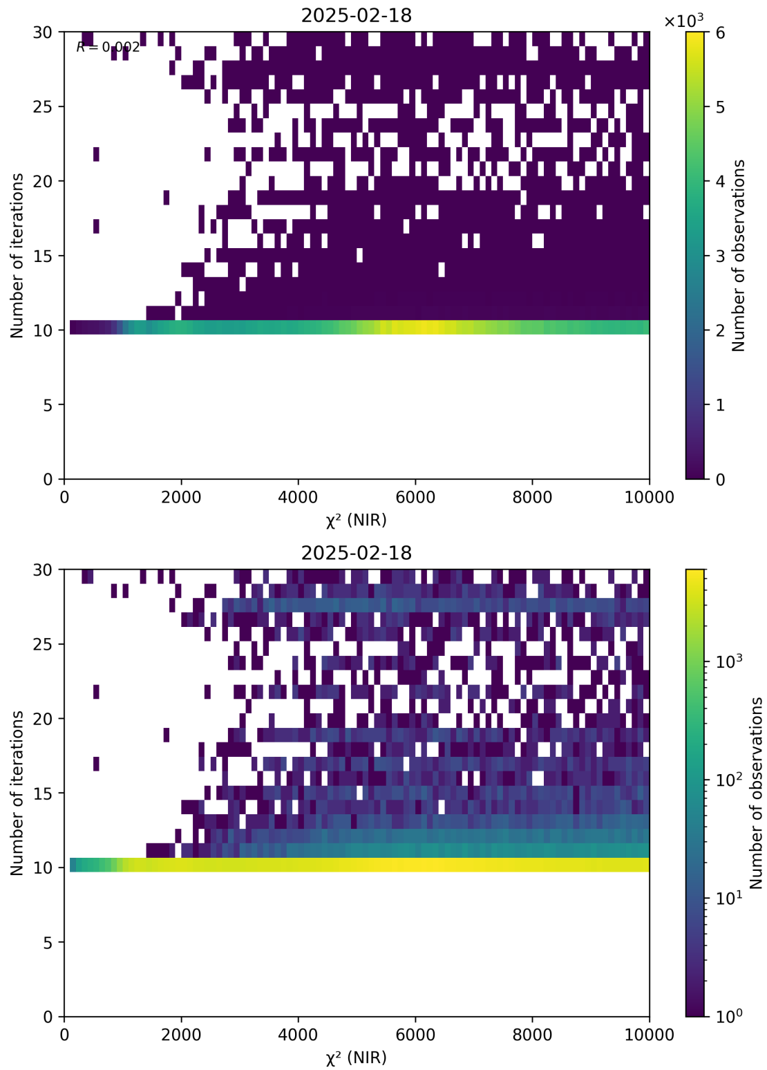
Figure 46: Scatter density plot of “ \chi^2 (NIR)” against “Number of iterations” for 2025-02-18 to 2025-02-19.
