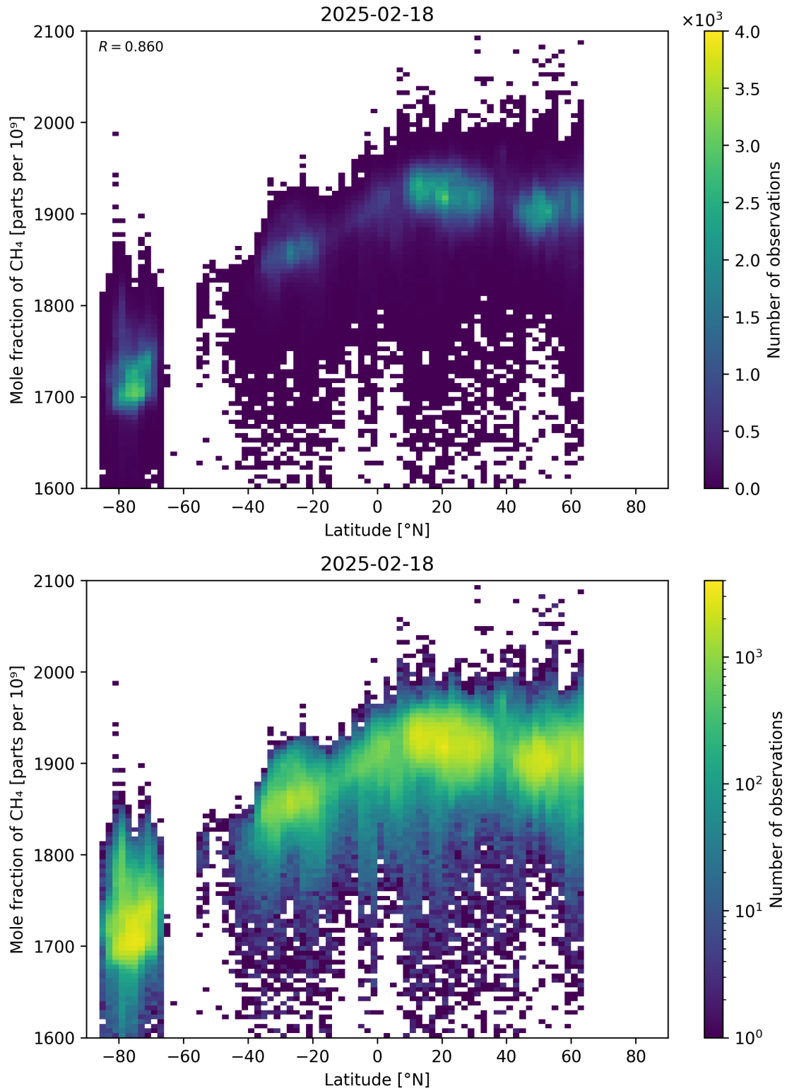
Figure 57: Scatter density plot of “Latitude” against “Mole fraction of CH 4 ” for 2025-02-18 to 2025-02-19.
