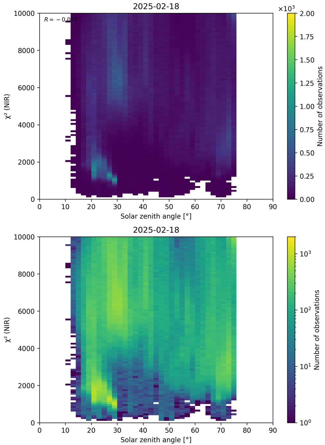
Figure 94: Scatter density plot of “Solar zenith angle” against “ \chi^2 (NIR)” for 2025-02-18 to 2025-02-19.
