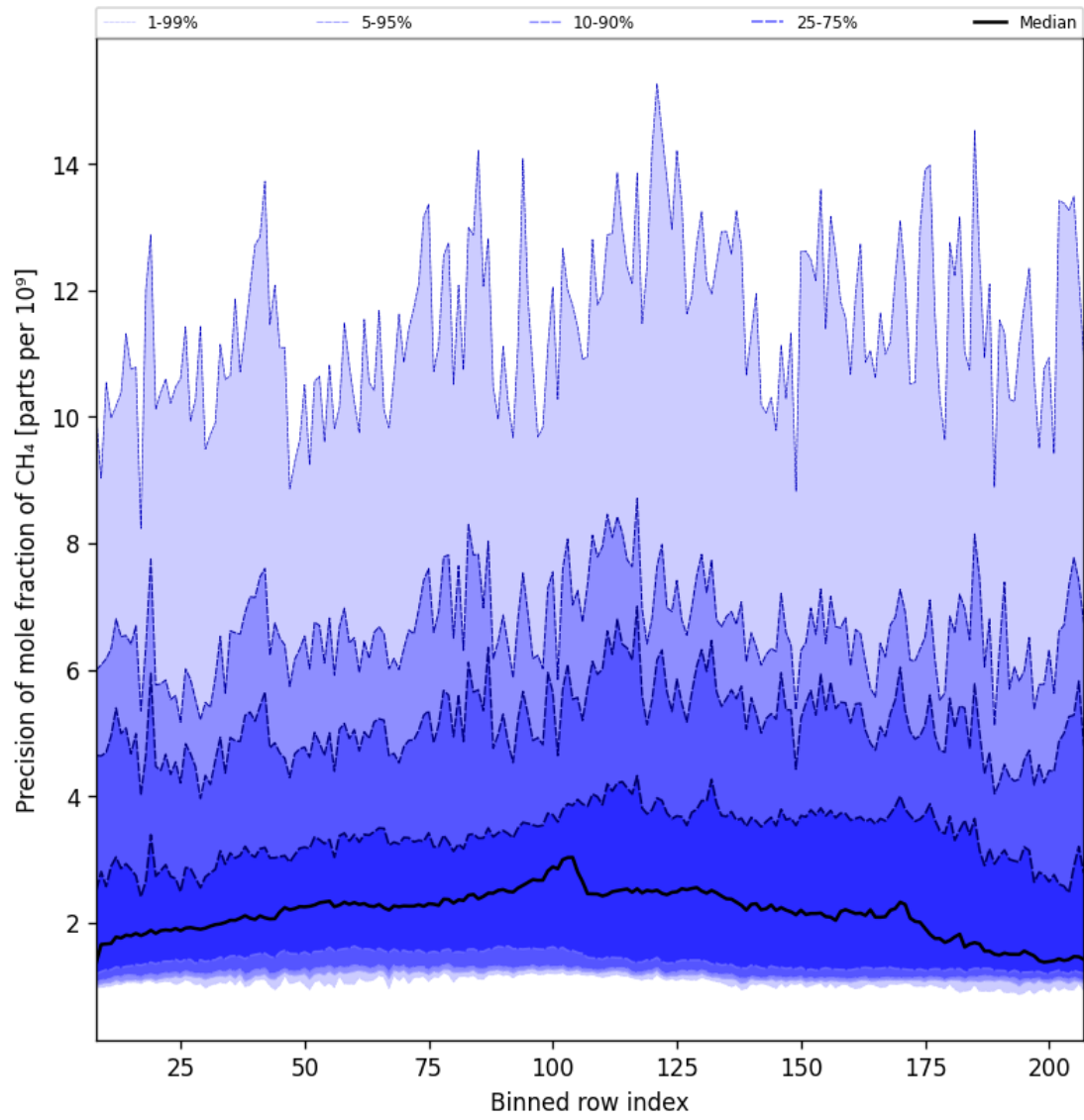
Figure 35: Along track statistics of “Precision of mole fraction of CH 4 ” for 2025-02-18 to 2025-02-19
