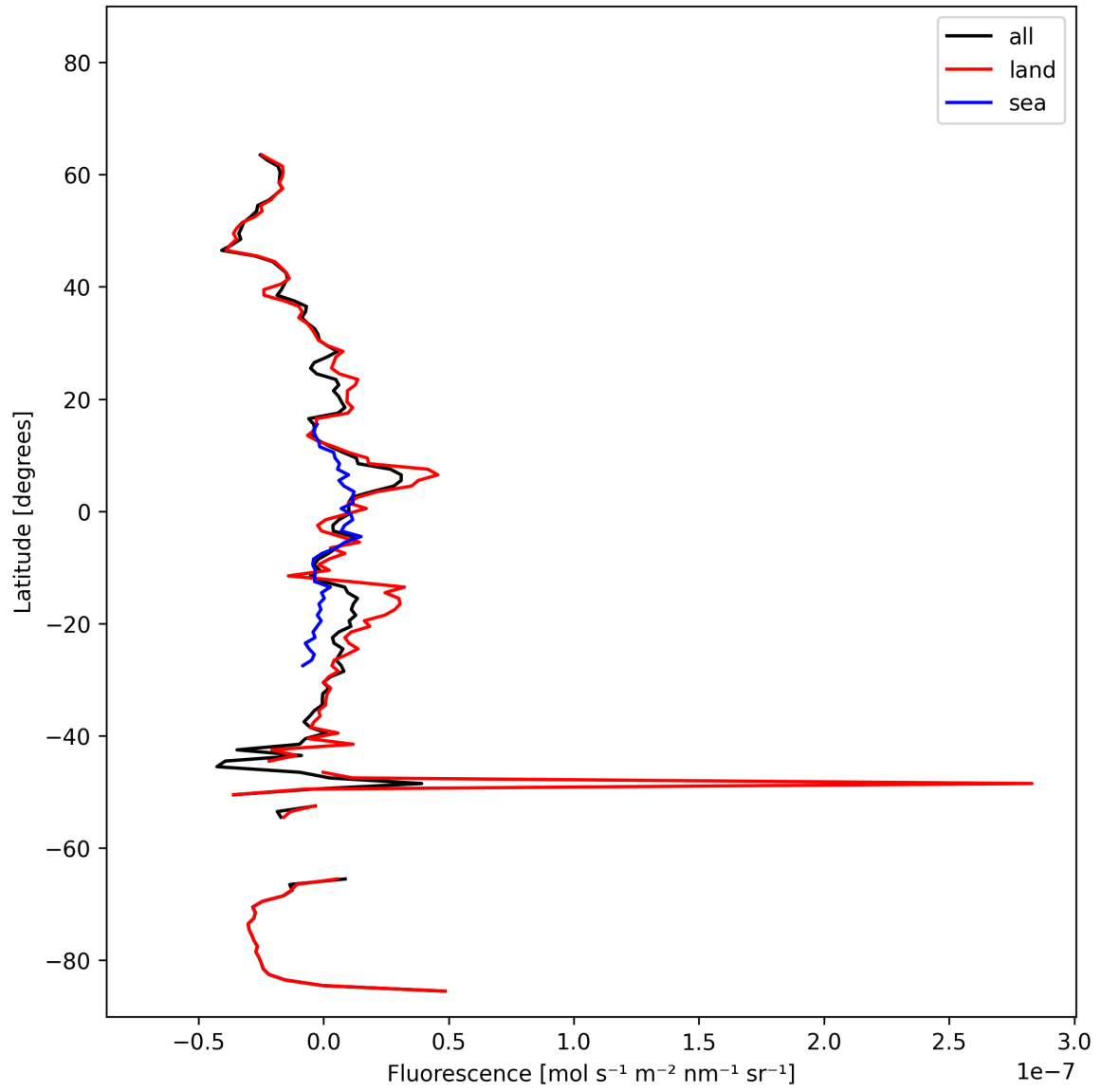
Figure 21: Zonal average of “Fluorescence” for 2025-02-18 to 2025-02-19.
