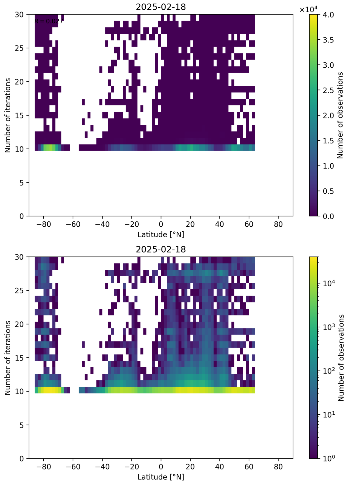
Figure 60: Scatter density plot of “Latitude” against “Number of iterations” for 2025-02-18 to 2025-02-19.
