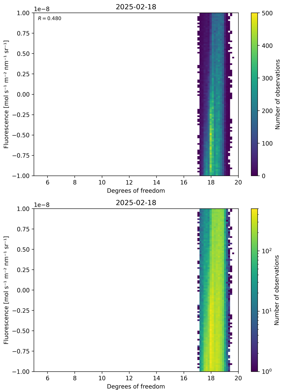
Figure 51: Scatter density plot of “Degrees of freedom” against “Fluorescence” for 2025-02-18 to 2025-02-19.
