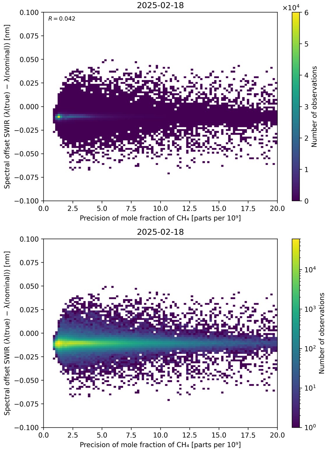
Figure 85: Scatter density plot of “Precision of mole fraction of \text{CH}_4 ” against “Spectral offset SWIR ( \lambda_{\text{true}} - \lambda_{\text{nominal}} )” for 2025-02-18 to 2025-02-19.
