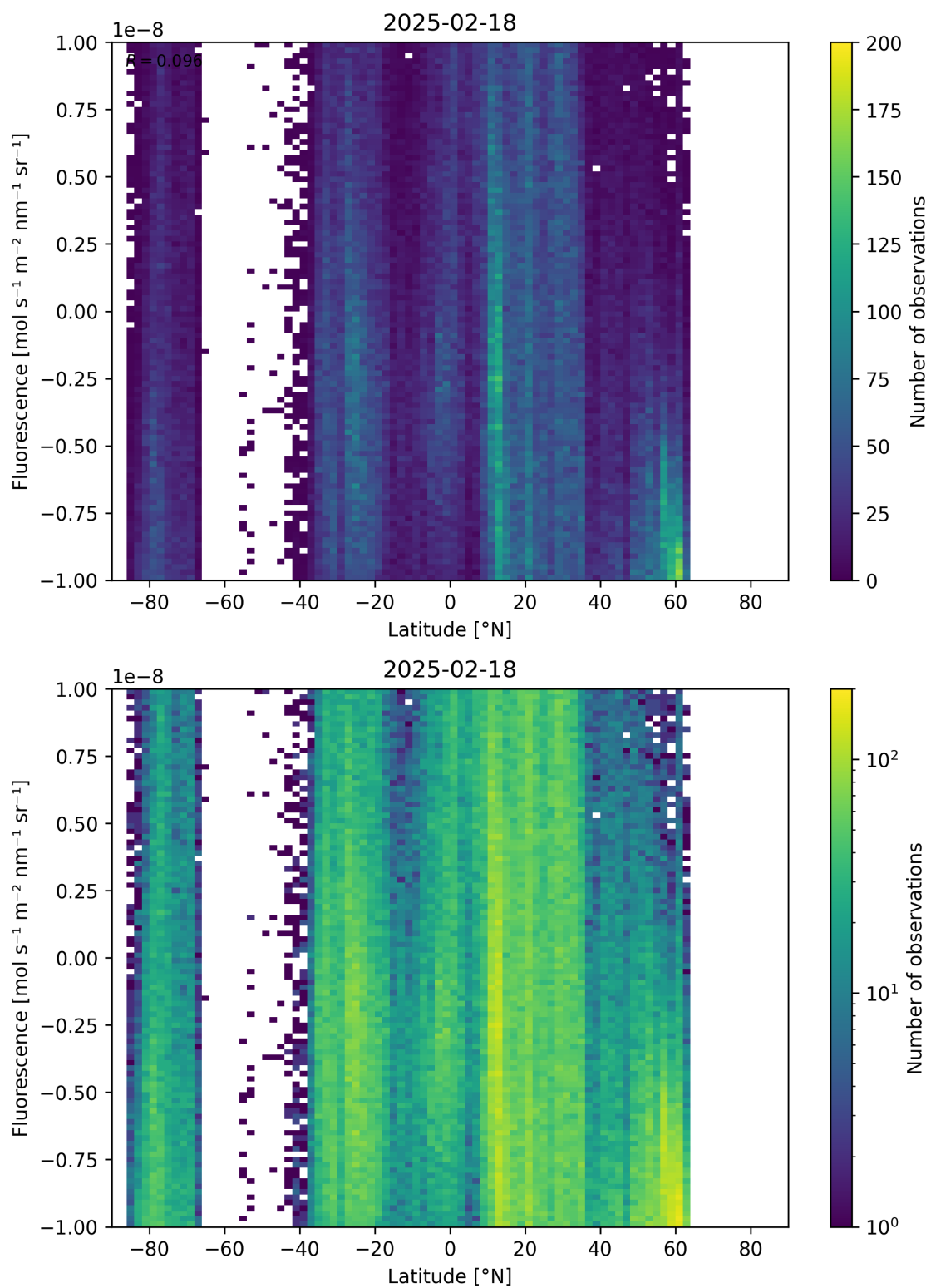
Figure 56: Scatter density plot of “Latitude” against “Fluorescence” for 2025-02-18 to 2025-02-19.
