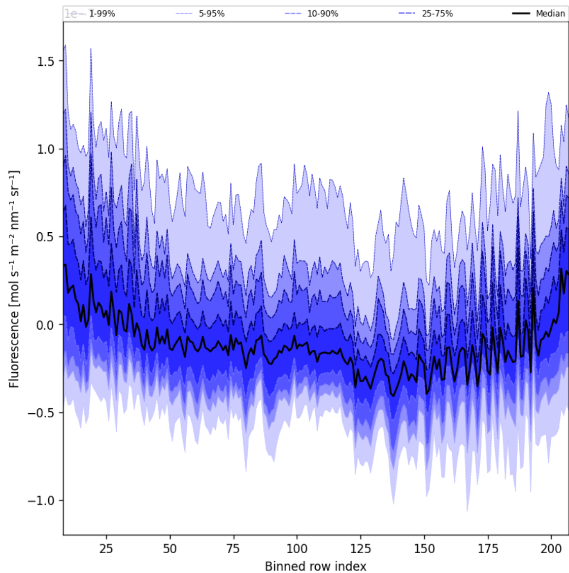
Figure 43: Along track statistics of "Fluorescence" for 2025-02-18 to 2025-02-19
