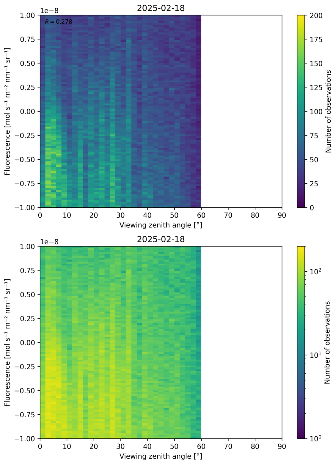
Figure 108: Scatter density plot of “Viewing zenith angle” against “Fluorescence” for 2025-02-18 to 2025-02-19.
