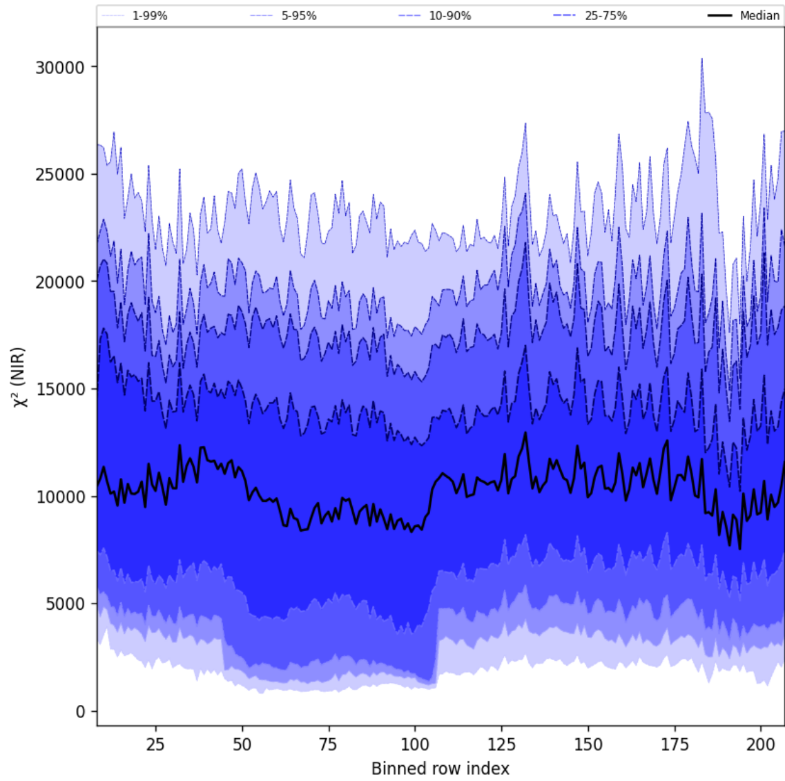
Figure 40: Along track statistics of “ \chi^2 (NIR)” for 2025-02-18 to 2025-02-19
