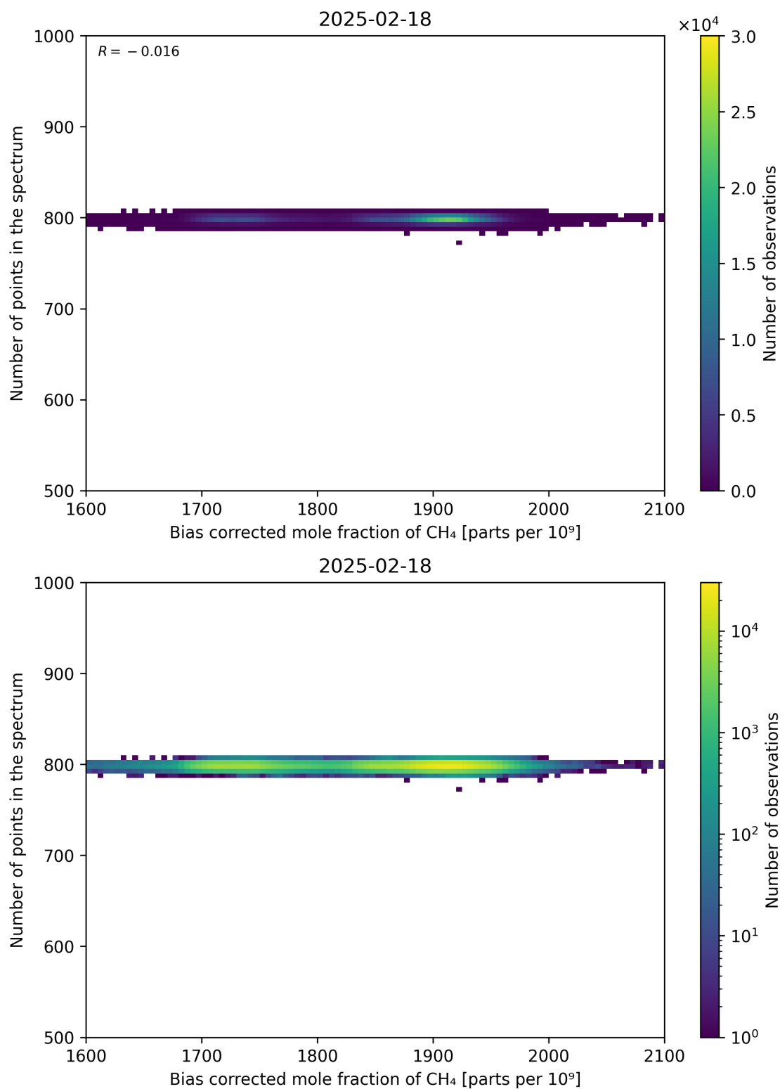
Figure 68: Scatter density plot of “Bias corrected mole fraction of CH 4 ” against “Number of points in the spectrum” for 2025-02-18 to 2025-02-19.
