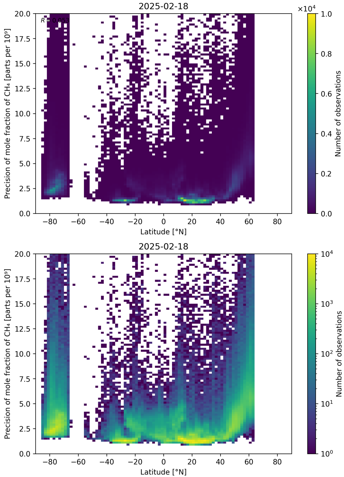
Figure 59: Scatter density plot of “Latitude” against “Precision of mole fraction of CH 4 ” for 2025-02-18 to 2025-02-19.
