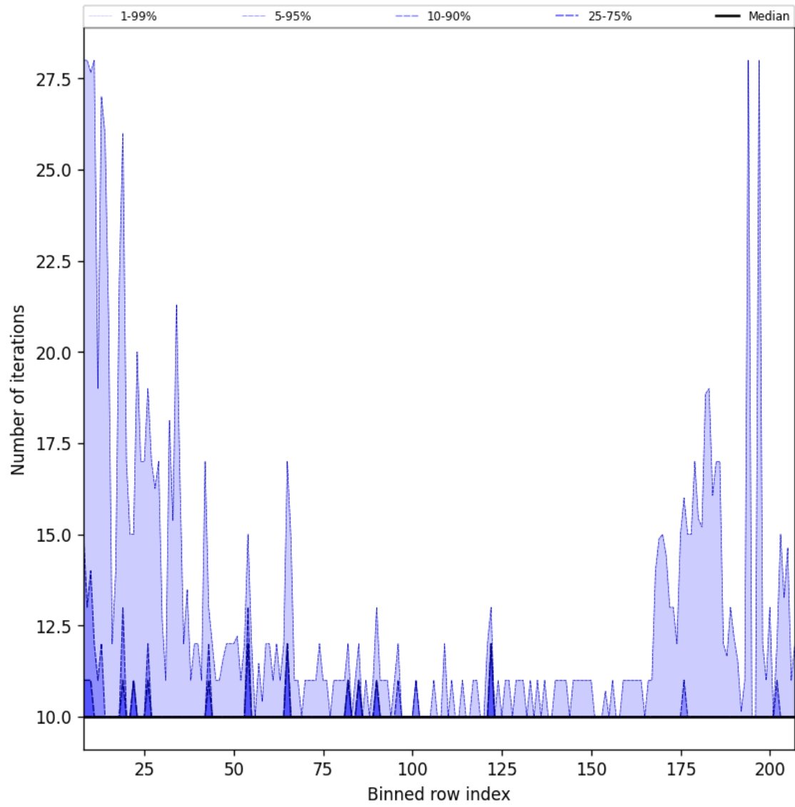
Figure 42: Along track statistics of “Number of iterations” for 2025-02-18 to 2025-02-19
