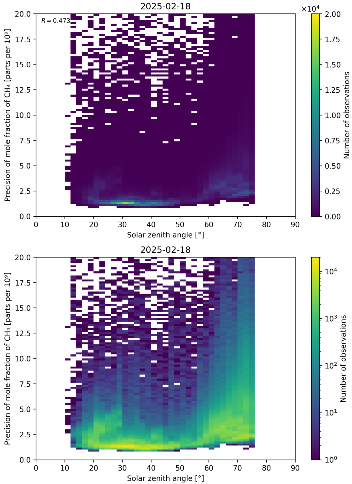
Figure 101: Scatter density plot of “Solar zenith angle” against “Precision of mole fraction of \text{CH}_4 ” for 2025-02-18 to 2025-02-19.
