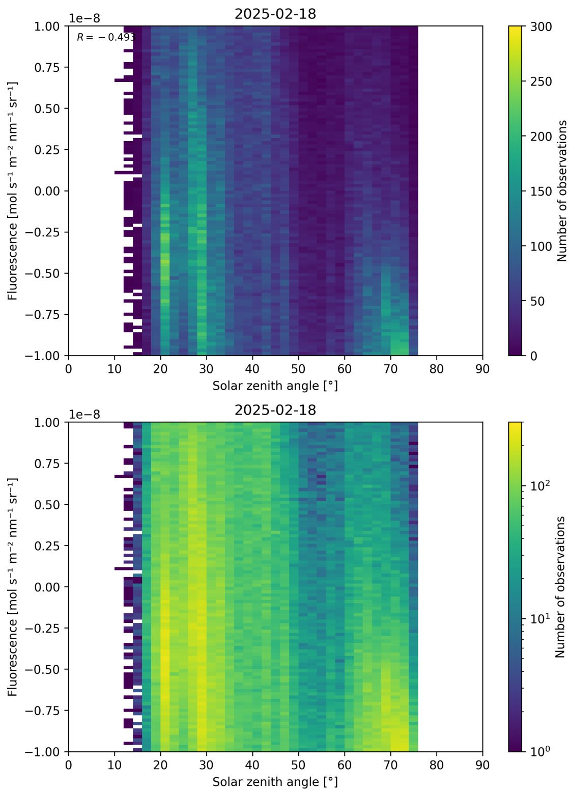
Figure 97: Scatter density plot of “Solar zenith angle” against “Fluorescence” for 2025-02-18 to 2025-02-19.
