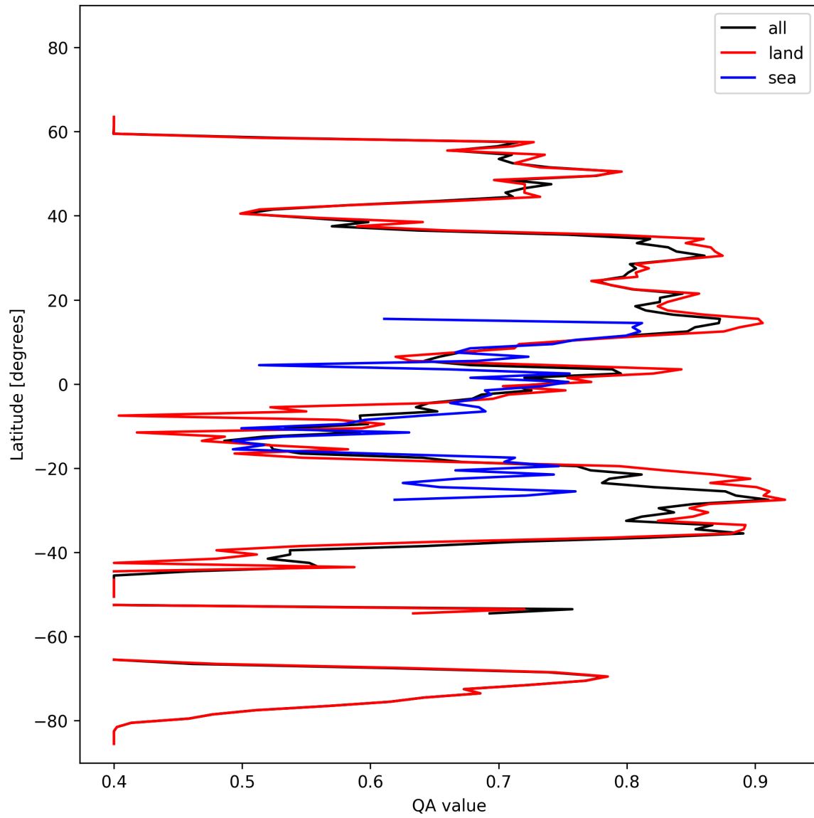
Figure 11: Zonal average of “QA value” for 2025-02-18 to 2025-02-19.
