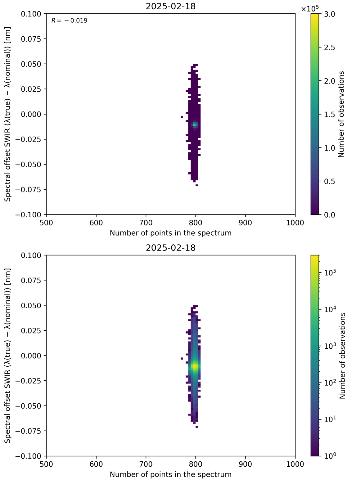
Figure 93: Scatter density plot of “Number of points in the spectrum” against “Spectral offset SWIR ( \lambda_{\text{true}} - \lambda_{\text{nominal}} )” for 2025-02-18 to 2025-02-19.
