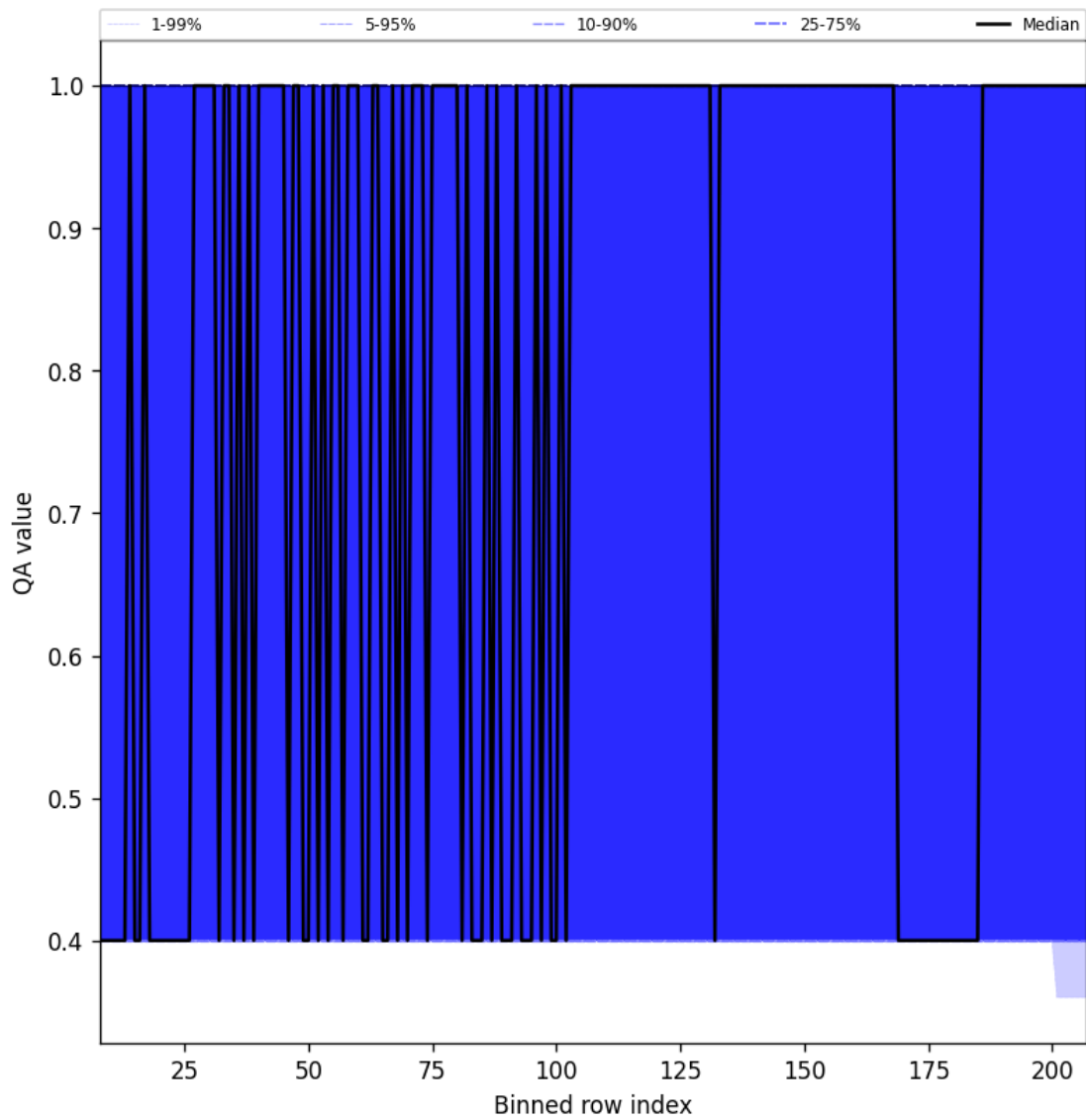
Figure 33: Along track statistics of “QA value” for 2025-02-18 to 2025-02-19
