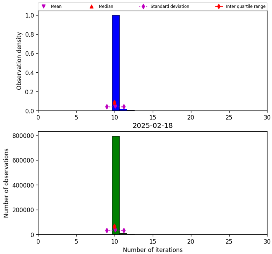
Figure 31: Histogram of “Number of iterations” for 2025-02-18 to 2025-02-19
