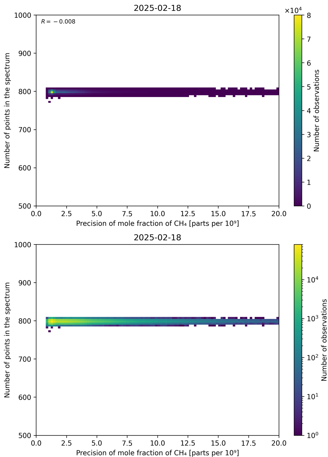
Figure 84: Scatter density plot of “Precision of mole fraction of CH 4 ” against “Number of points in the spectrum” for 2025-02-18 to 2025-02-19.
