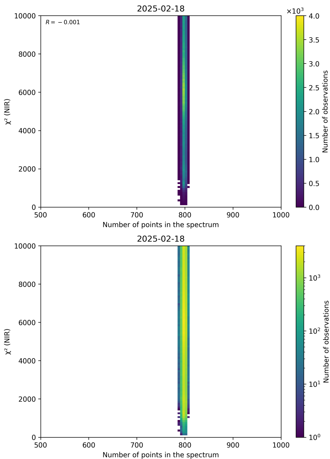
Figure 88: Scatter density plot of “Number of points in the spectrum” against “ \chi^2 (NIR)” for 2025-02-18 to 2025-02-19.
