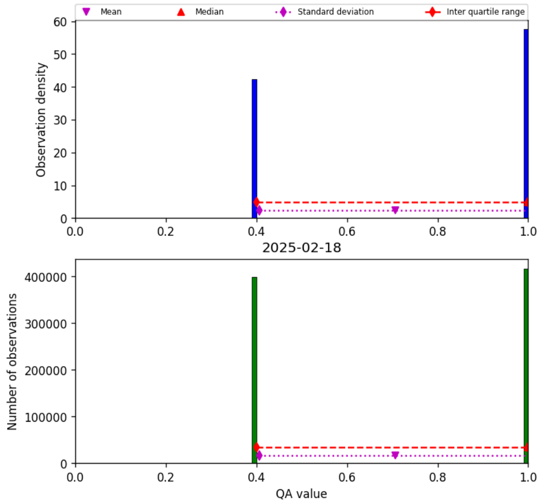
Figure 22: Histogram of “QA value” for 2025-02-18 to 2025-02-19
