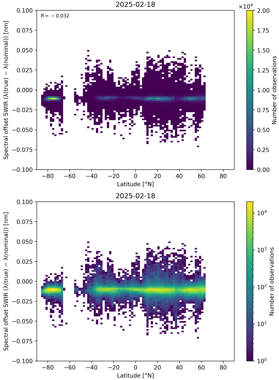
Figure 62: Scatter density plot of “Latitude” against “Spectral offset SWIR ( \lambda_{\text{true}} - \lambda_{\text{nominal}} )” for 2025-02-18 to 2025-02-19.
