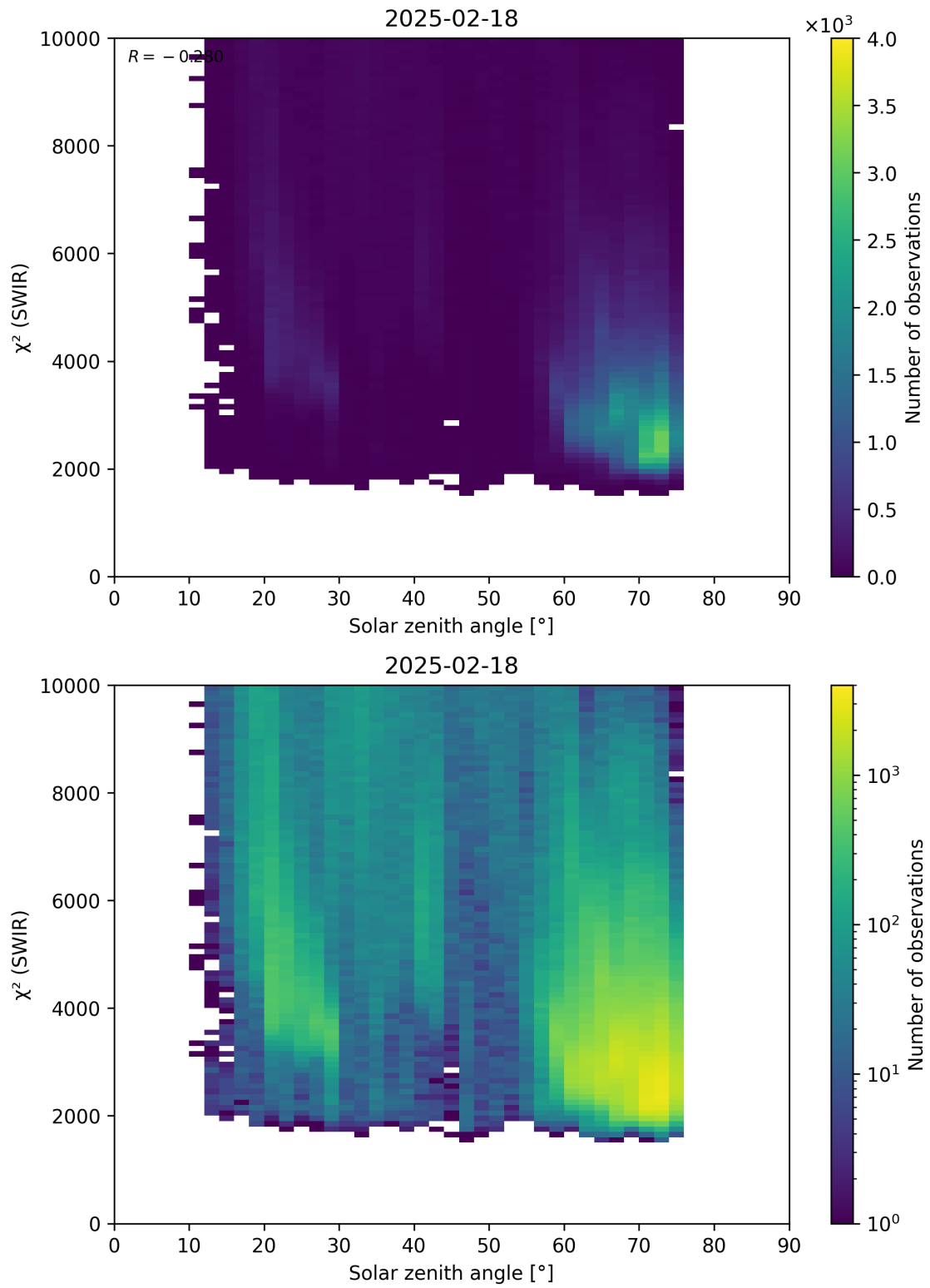
Figure 95: Scatter density plot of “Solar zenith angle” against “ \chi^2 (SWIR)” for 2025-02-18 to 2025-02-19.
