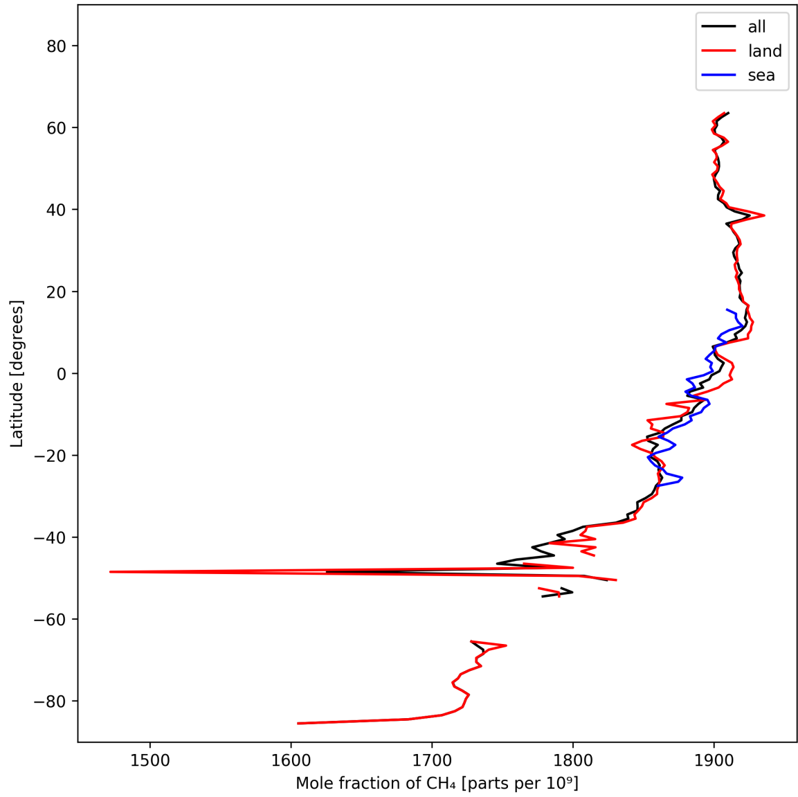
Figure 12: Zonal average of “Mole fraction of CH 4 ” for 2025-02-18 to 2025-02-19.
