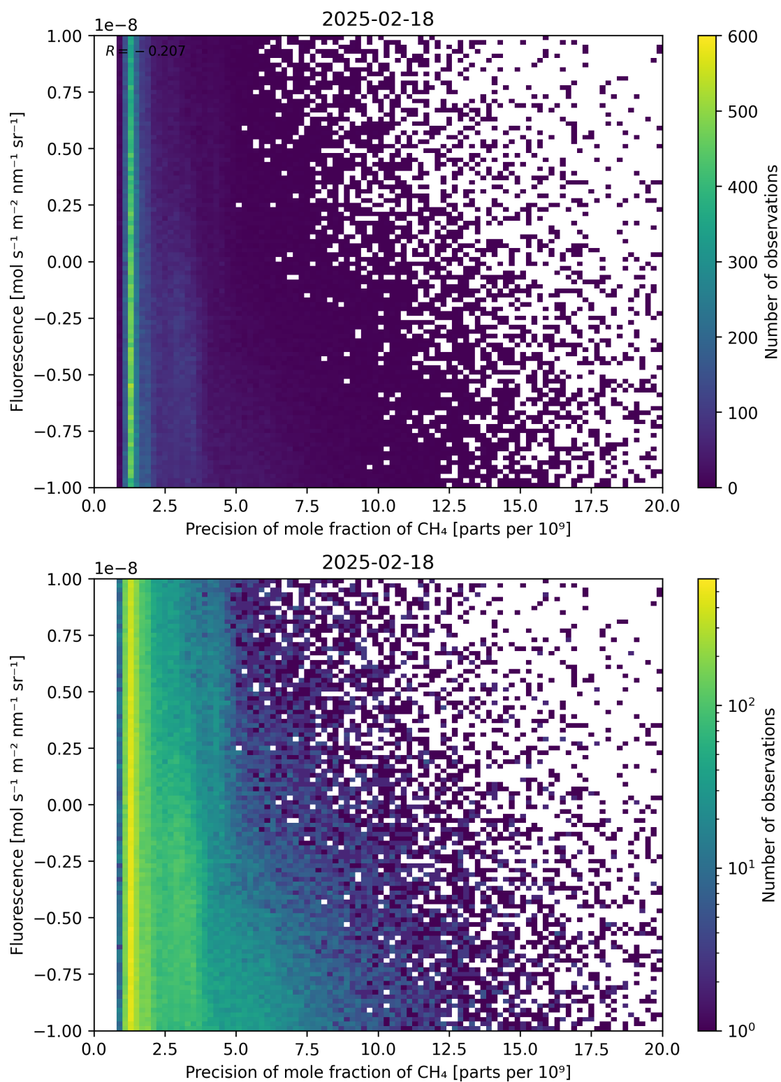
Figure 81: Scatter density plot of “Precision of mole fraction of CH 4 ” against “Fluorescence” for 2025-02-18 to 2025-02-19.
