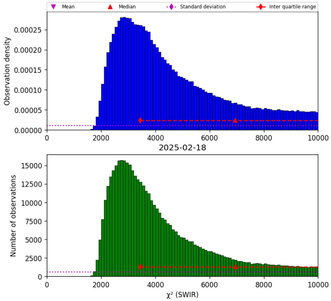
Figure 28: Histogram of “ \chi^2 (SWIR)” for 2025-02-18 to 2025-02-19
