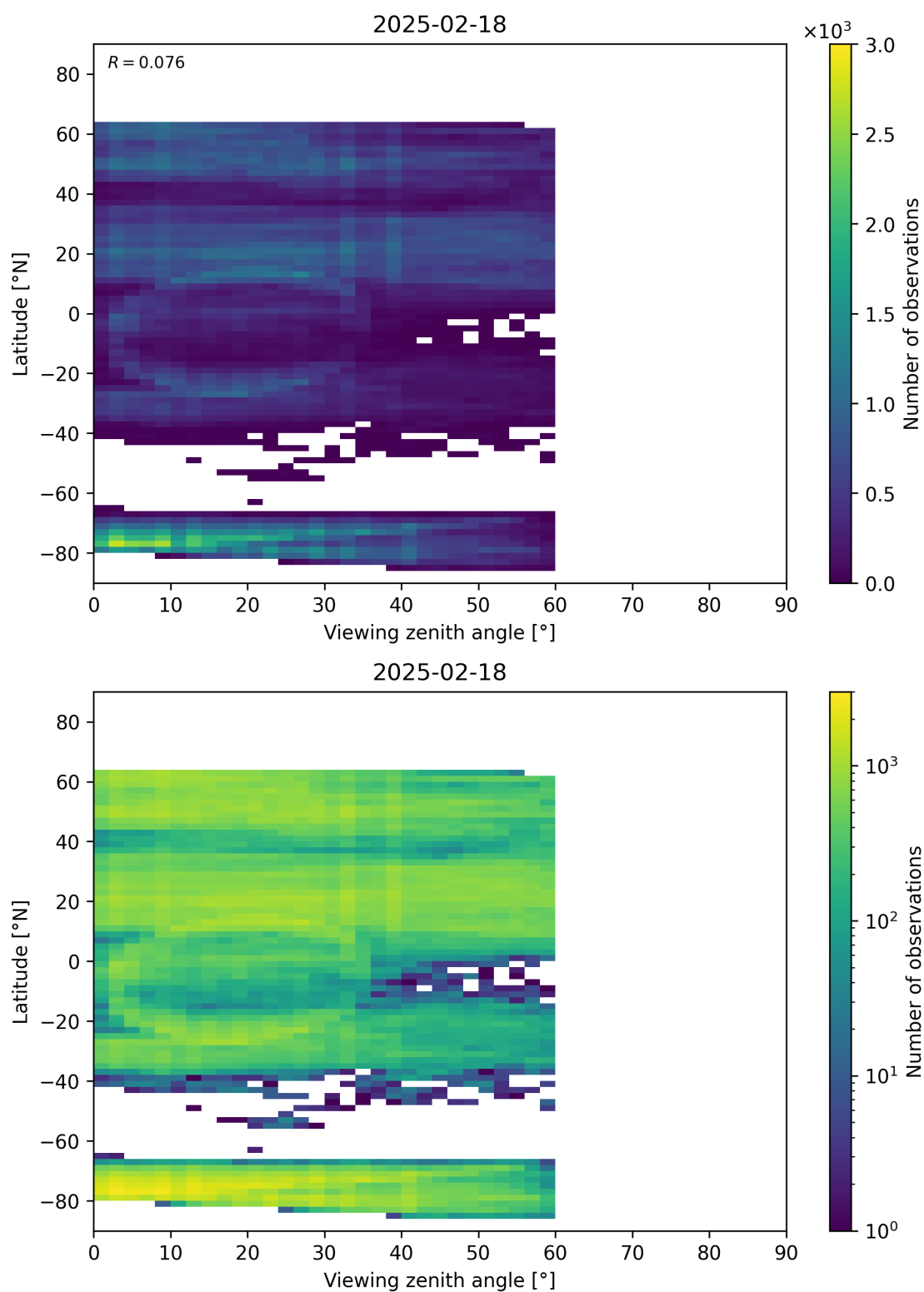
Figure 109: Scatter density plot of “Viewing zenith angle” against “Latitude” for 2025-02-18 to 2025-02-19.
