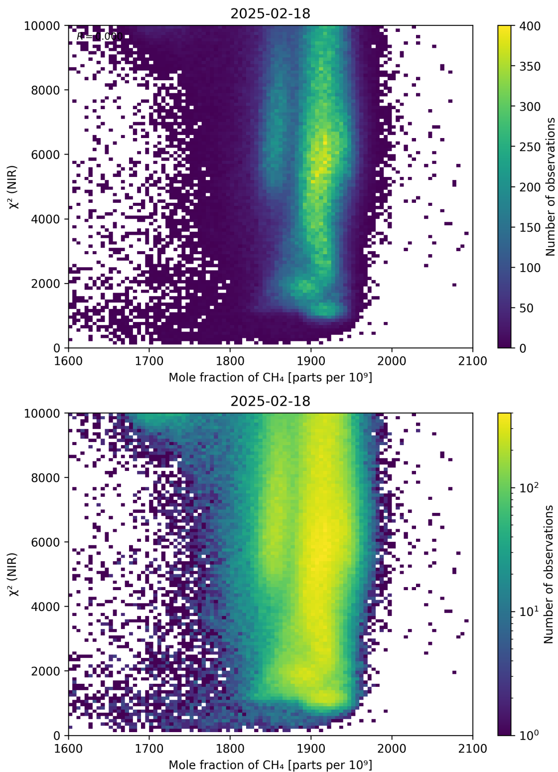
Figure 70: Scatter density plot of “Mole fraction of CH 4 ” against “ \chi^2 (NIR)” for 2025-02-18 to 2025-02-19.
