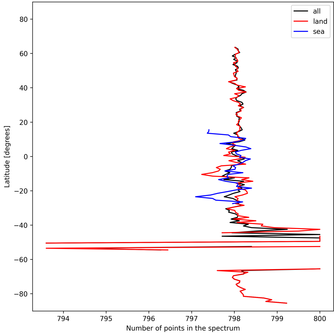
Figure 15: Zonal average of “Number of points in the spectrum” for 2025-02-18 to 2025-02-19.
