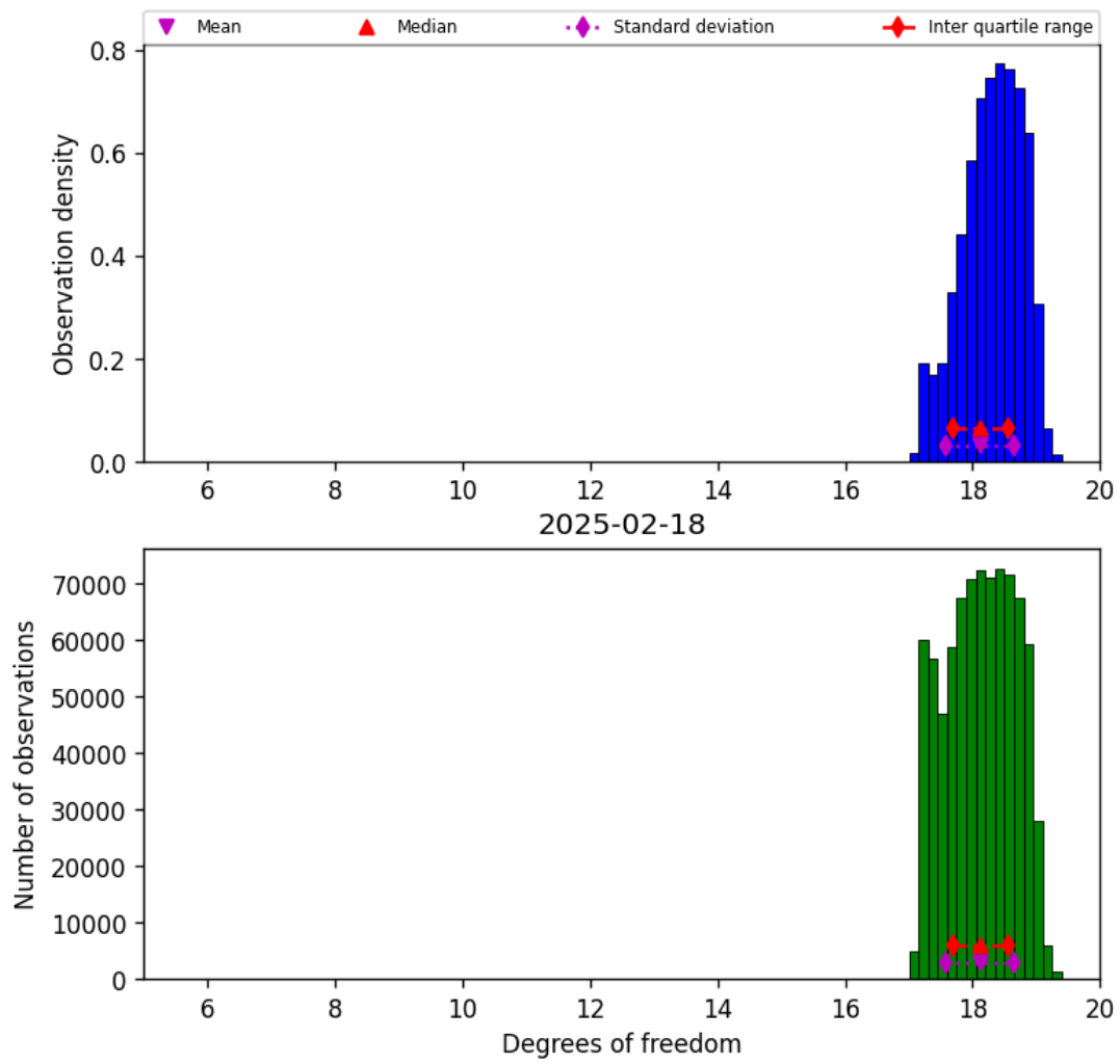
Figure 30: Histogram of “Degrees of freedom” for 2025-02-18 to 2025-02-19
