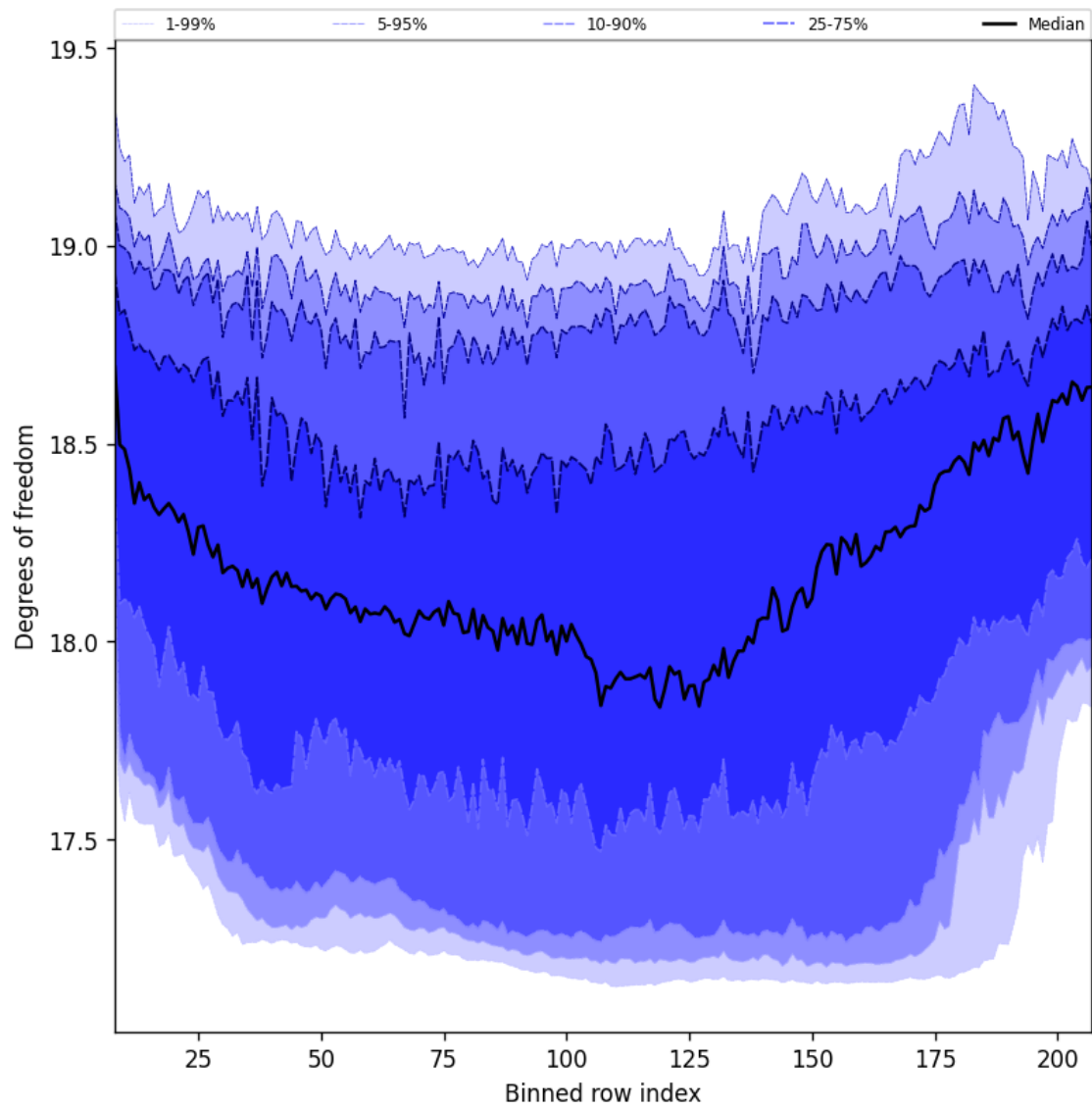
Figure 41: Along track statistics of “Degrees of freedom” for 2025-02-18 to 2025-02-19
