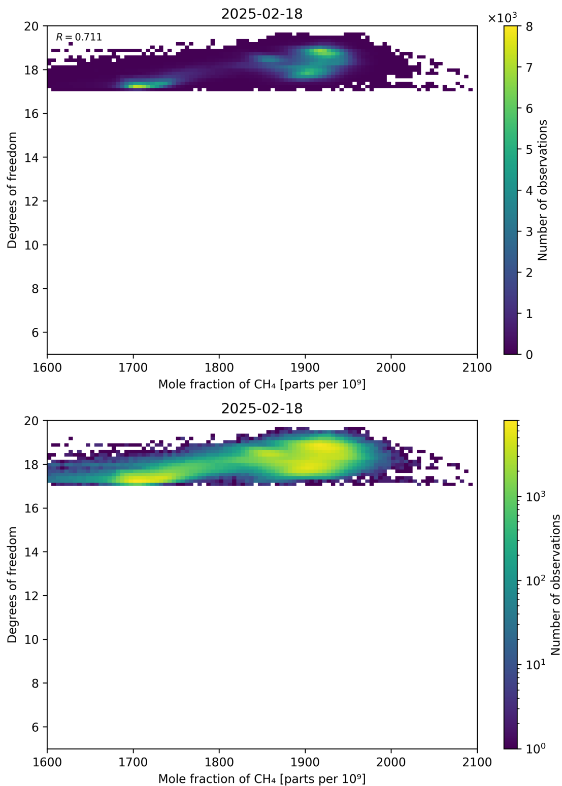
Figure 72: Scatter density plot of “Mole fraction of CH 4 ” against “Degrees of freedom” for 2025-02-18 to 2025-02-19.
