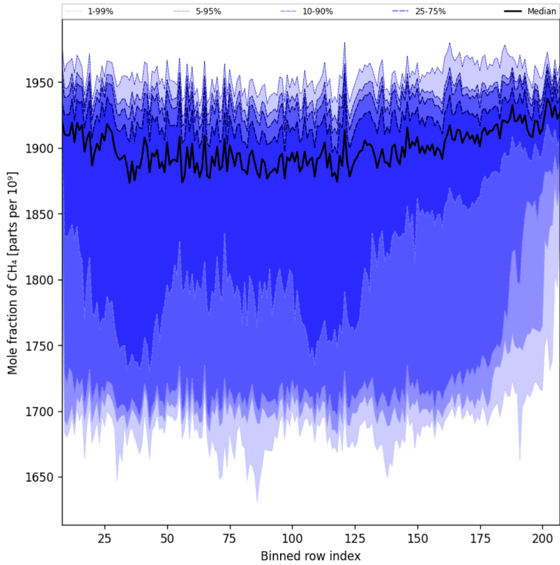
Figure 34: Along track statistics of “Mole fraction of CH 4 ” for 2025-02-18 to 2025-02-19
