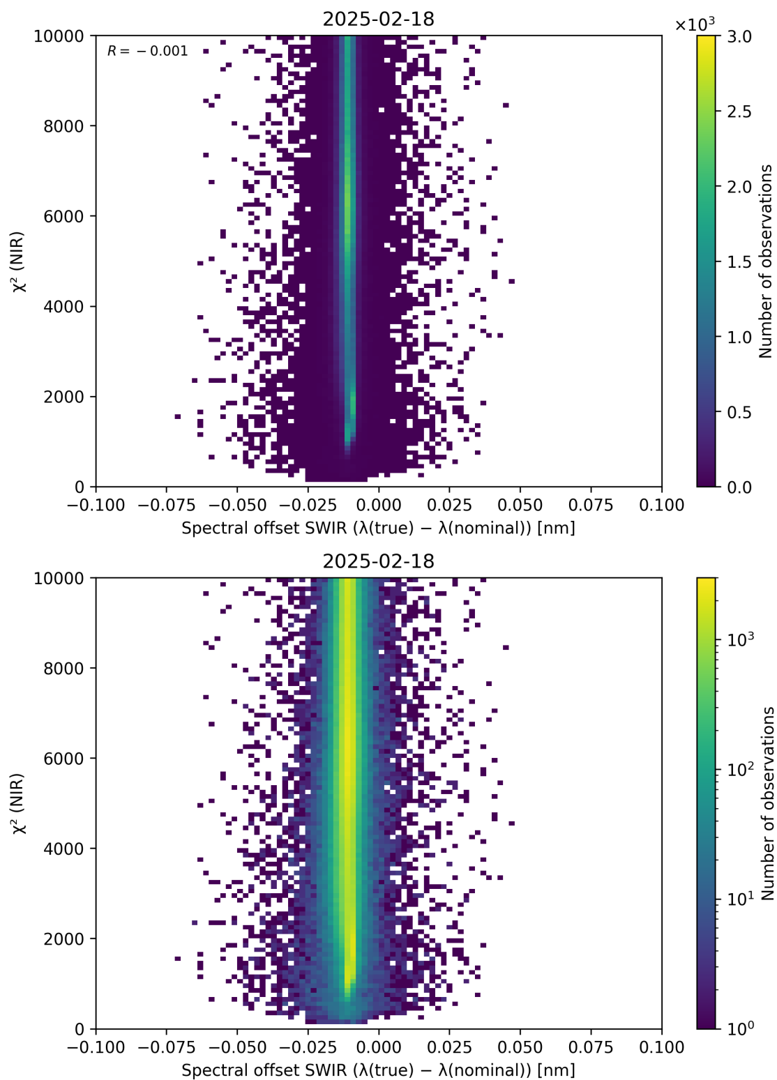
Figure 117: Scatter density plot of “Spectral offset SWIR ( \lambda_{\text{true}} - \lambda_{\text{nominal}} )” against “ \chi^2 (NIR)” for 2025-02-18 to 2025-02-19.
