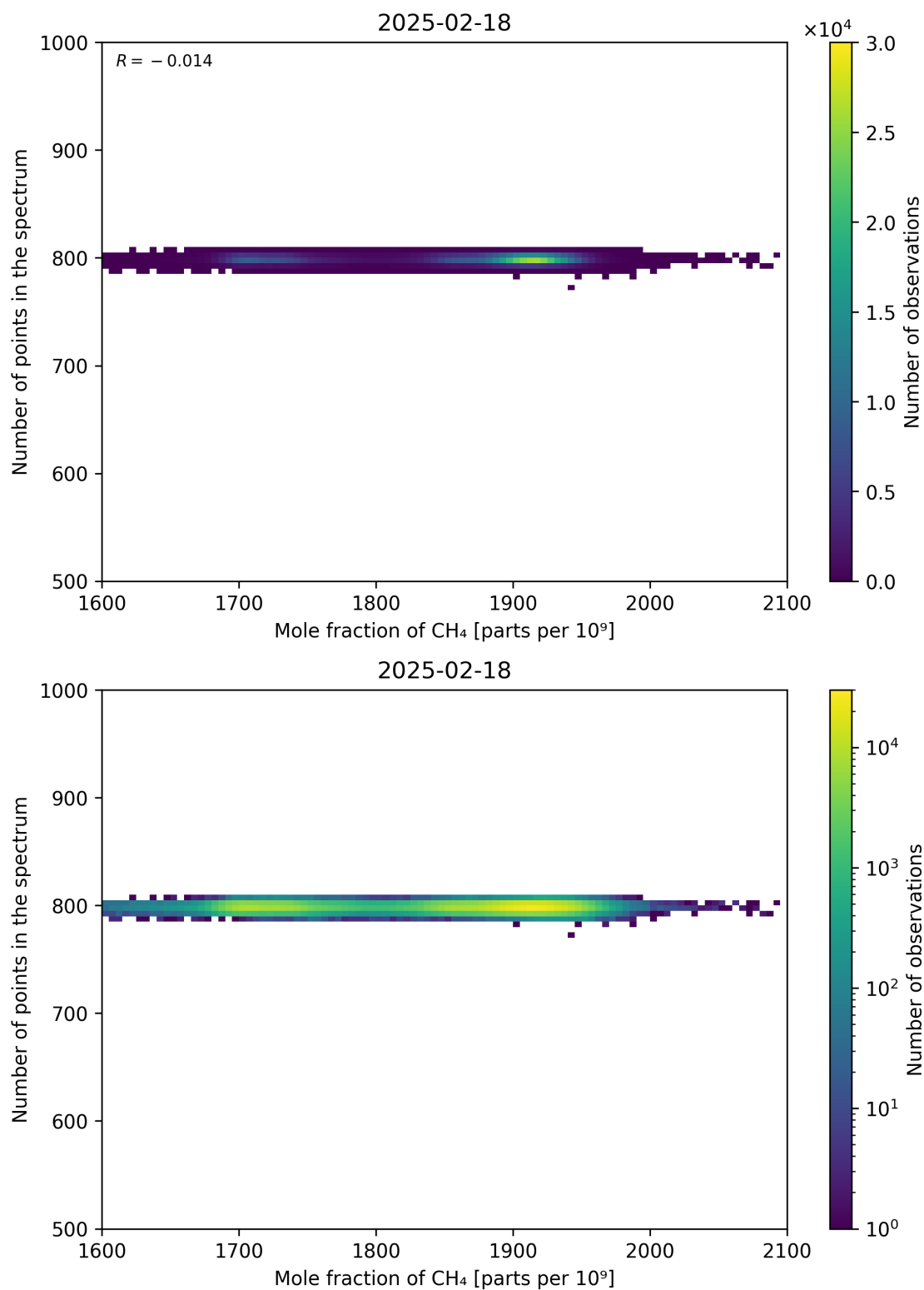
Figure 77: Scatter density plot of “Mole fraction of CH 4 ” against “Number of points in the spectrum” for 2025-02-18 to 2025-02-19.
