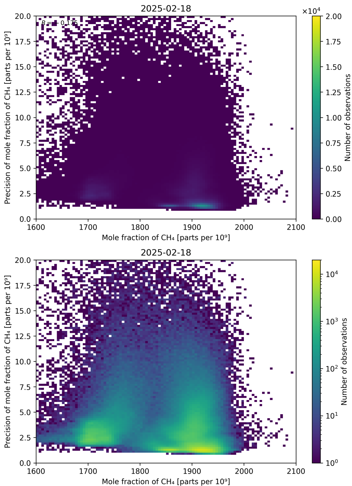
Figure 75: Scatter density plot of “Mole fraction of CH 4 ” against “Precision of mole fraction of CH 4 ” for 2025-02-18 to 2025-02-19.
