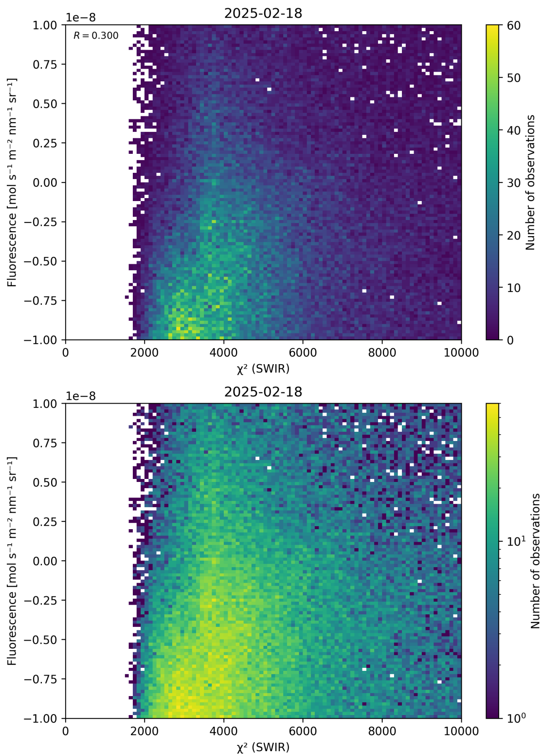
Figure 49: Scatter density plot of “ \chi^2 (SWIR)” against “Fluorescence” for 2025-02-18 to 2025-02-19.
