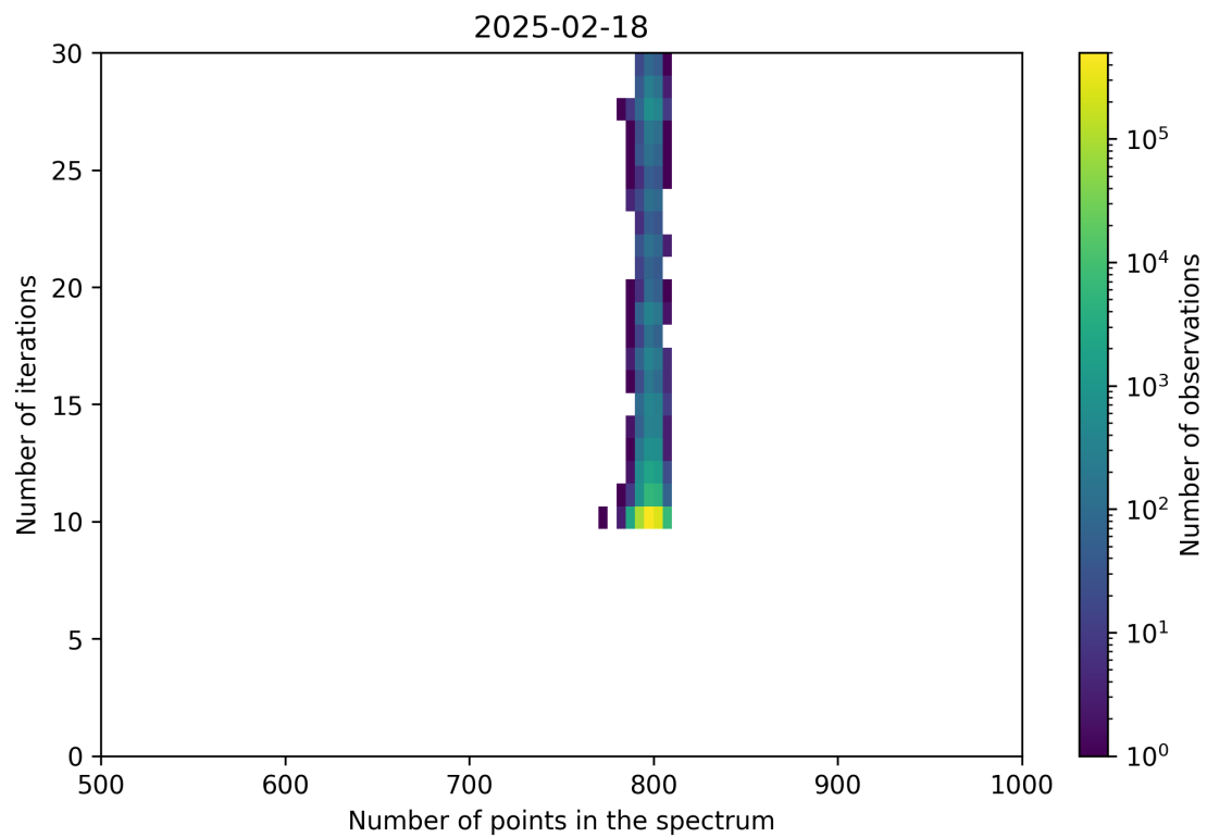
Figure 92: Scatter density plot of “Number of points in the spectrum” against “Number of iterations” for 2025-02-18 to 2025-02-19.
