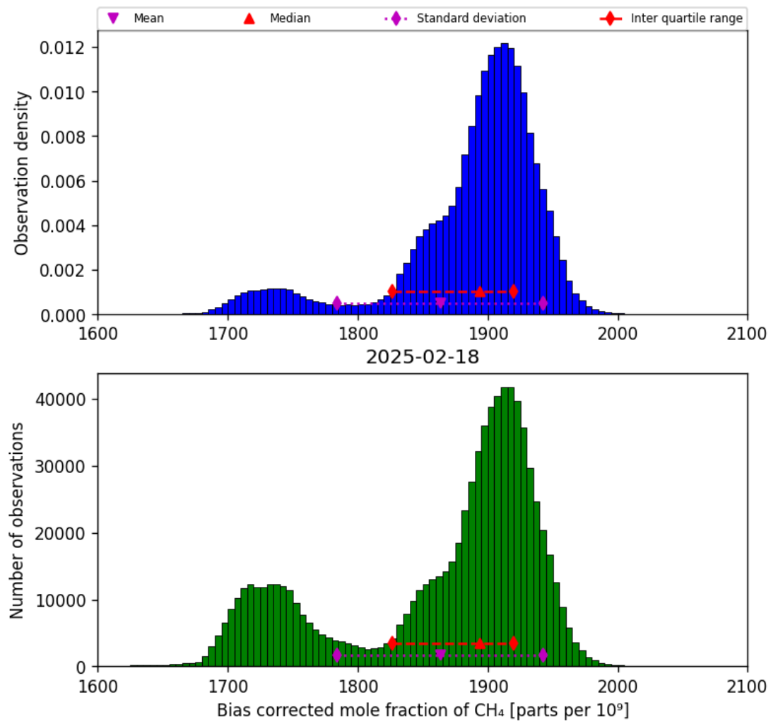
Figure 25: Histogram of “Bias corrected mole fraction of CH 4 ” for 2025-02-18 to 2025-02-19
