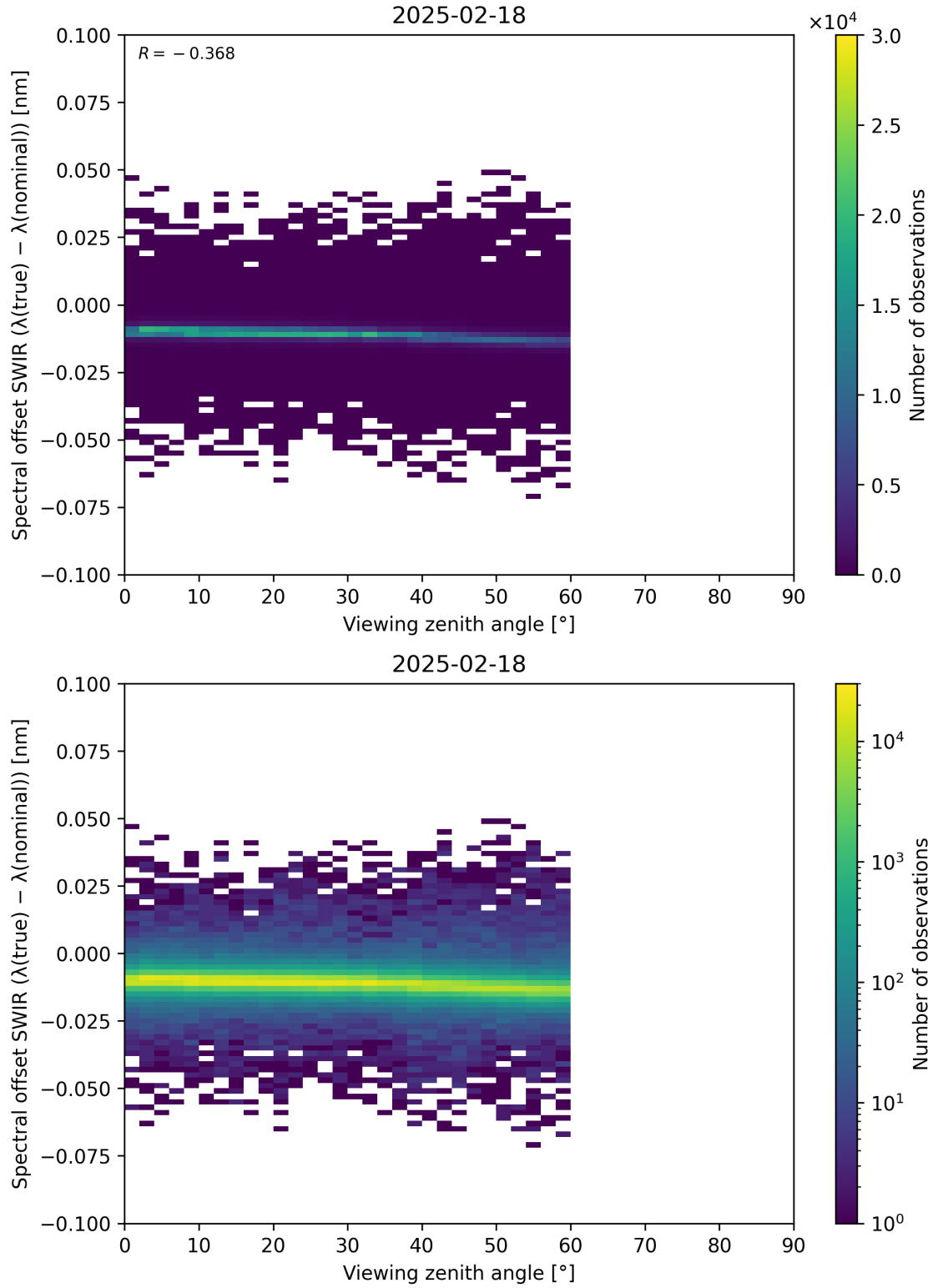
Figure 116: Scatter density plot of “Viewing zenith angle” against “Spectral offset SWIR ( \lambda_{\text{true}} - \lambda_{\text{nominal}} )” for 2025-02-18 to 2025-02-19.
