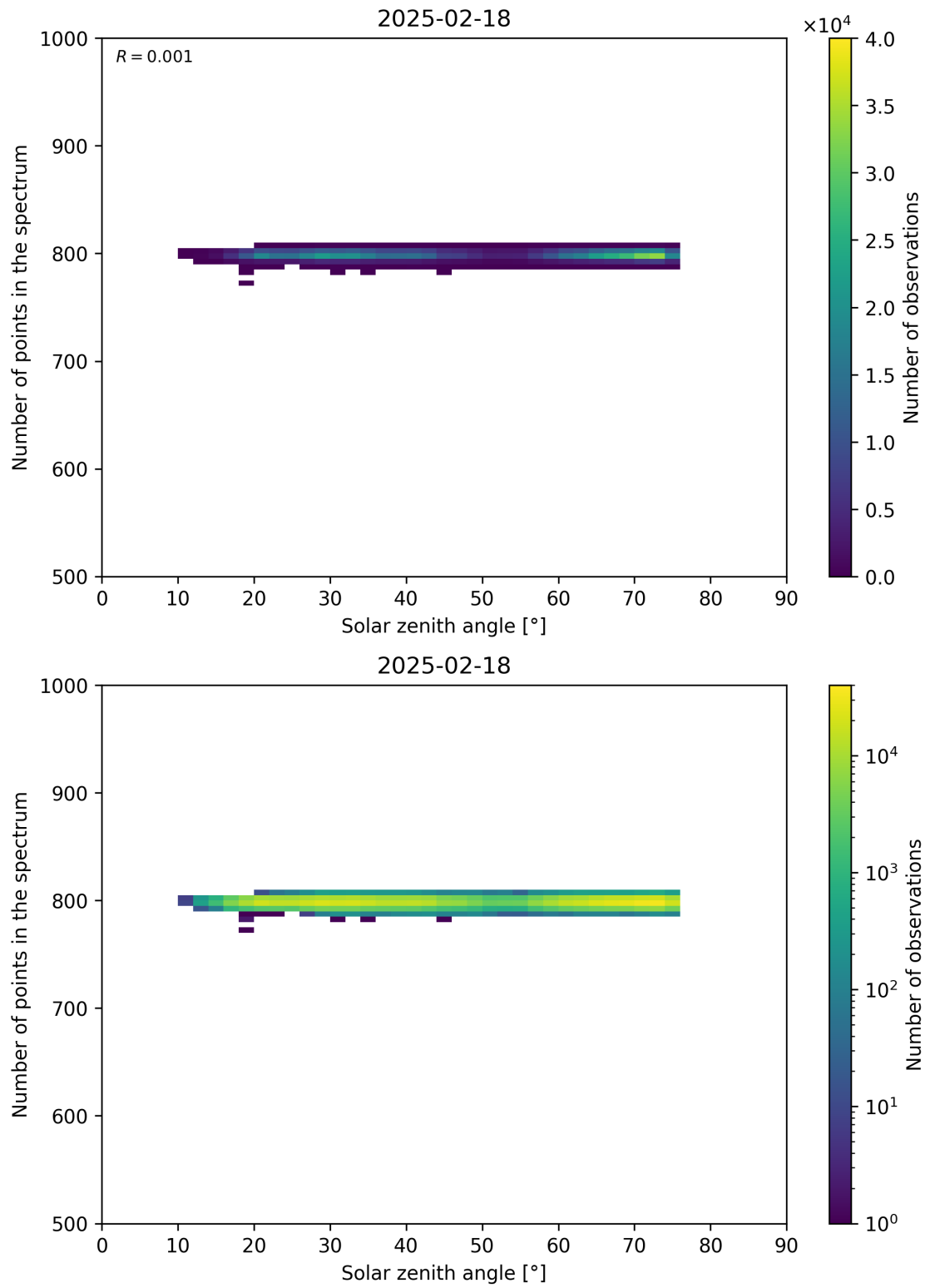
Figure 103: Scatter density plot of “Solar zenith angle” against “Number of points in the spectrum” for 2025-02-18 to 2025-02-19.
