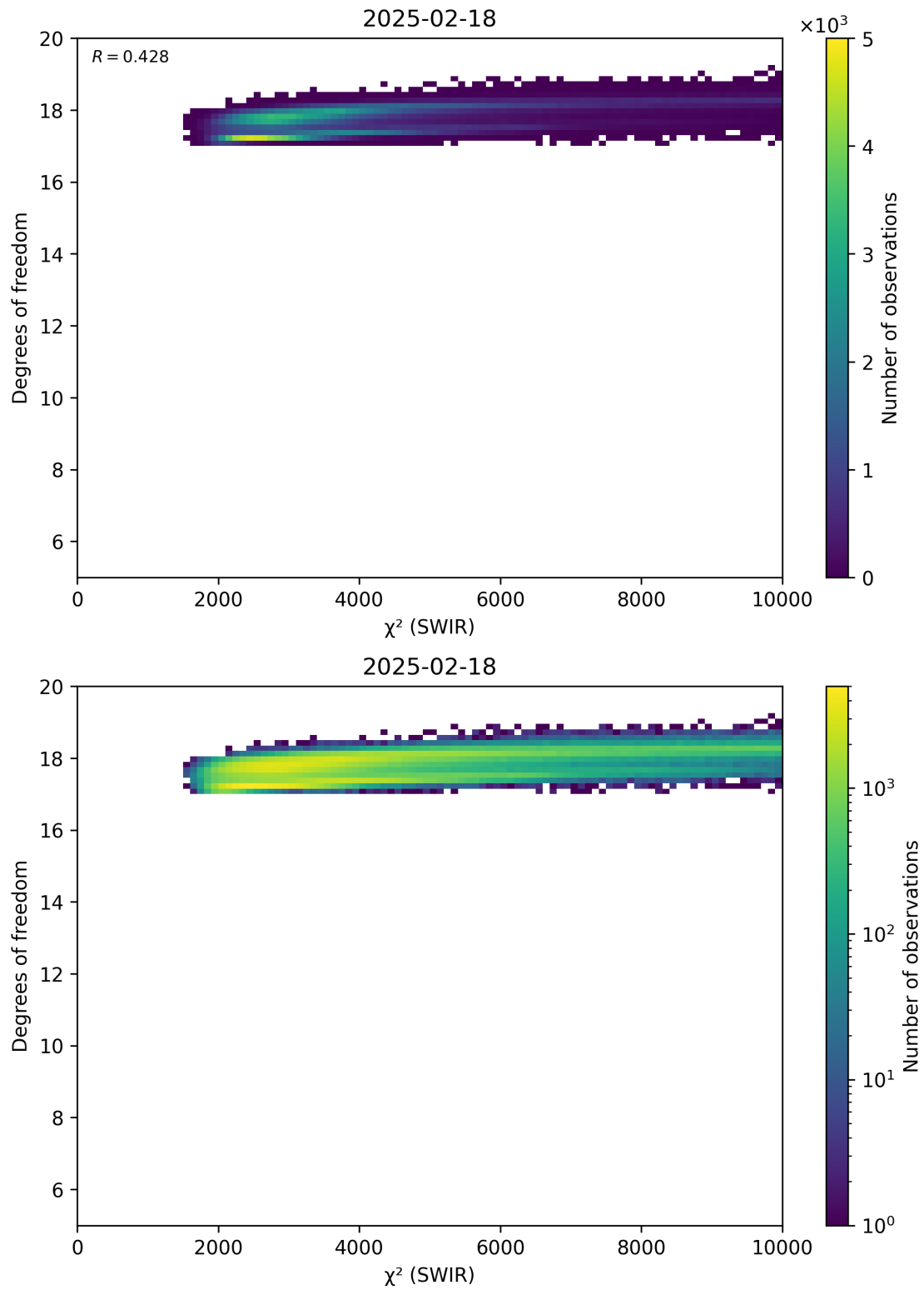
Figure 48: Scatter density plot of “ \chi^2 (SWIR)” against “Degrees of freedom” for 2025-02-18 to 2025-02-19.
