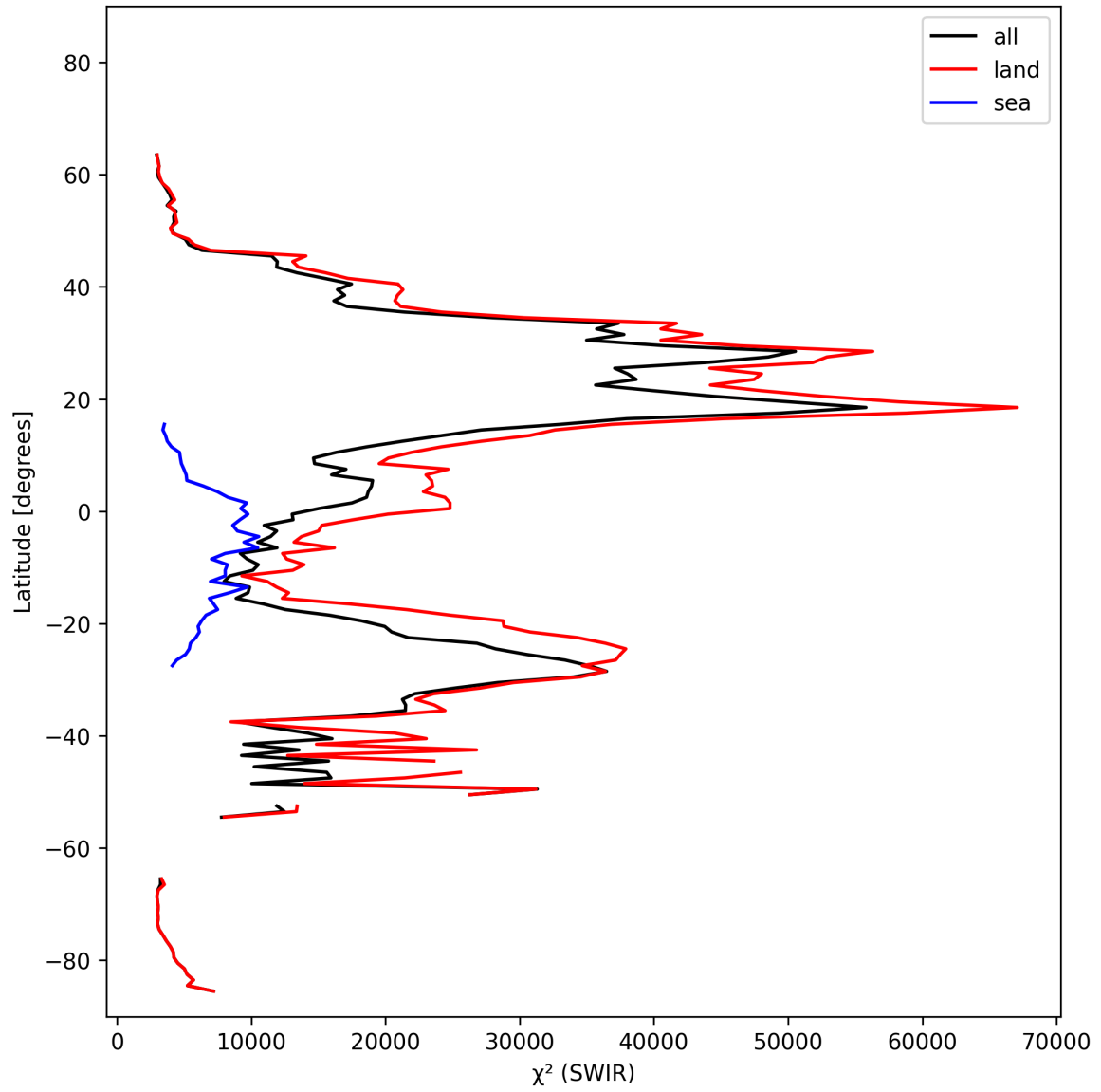
Figure 17: Zonal average of “ \chi^2 (SWIR)” for 2025-02-18 to 2025-02-19.
