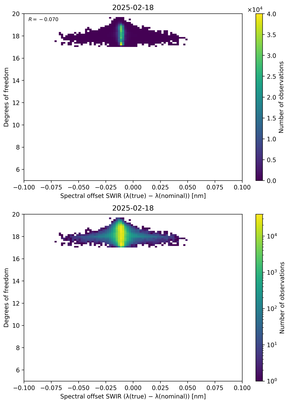
Figure 119: Scatter density plot of “Spectral offset SWIR ( \lambda_{\text{true}} - \lambda_{\text{nominal}} )” against “Degrees of freedom” for 2025-02-18 to 2025-02-19.
