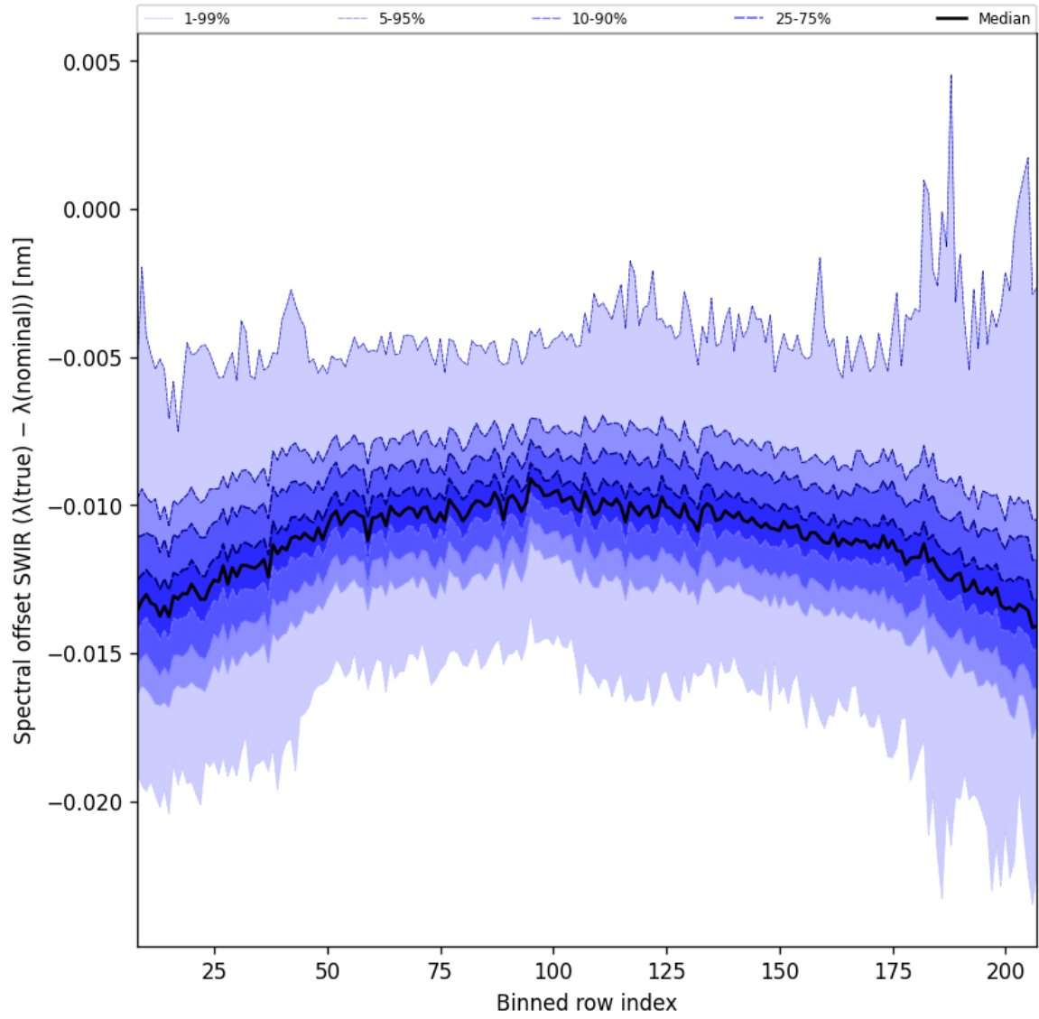
Figure 38: Along track statistics of “Spectral offset SWIR ( \lambda_{\text{true}} - \lambda_{\text{nominal}} )” for 2025-02-18 to 2025-02-19
