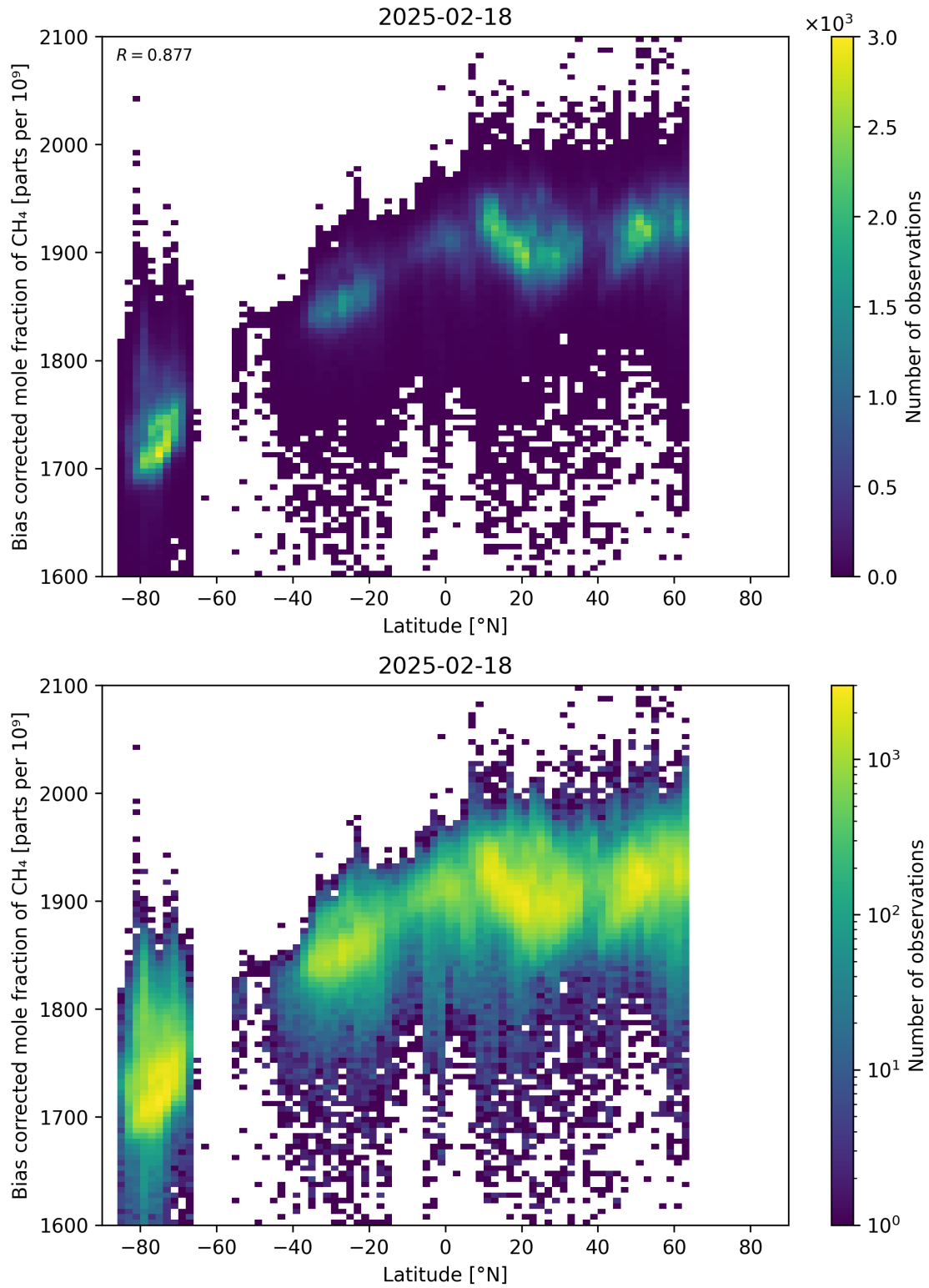
Figure 58: Scatter density plot of “Latitude” against “Bias corrected mole fraction of CH 4 ” for 2025-02-18 to 2025-02-19.
