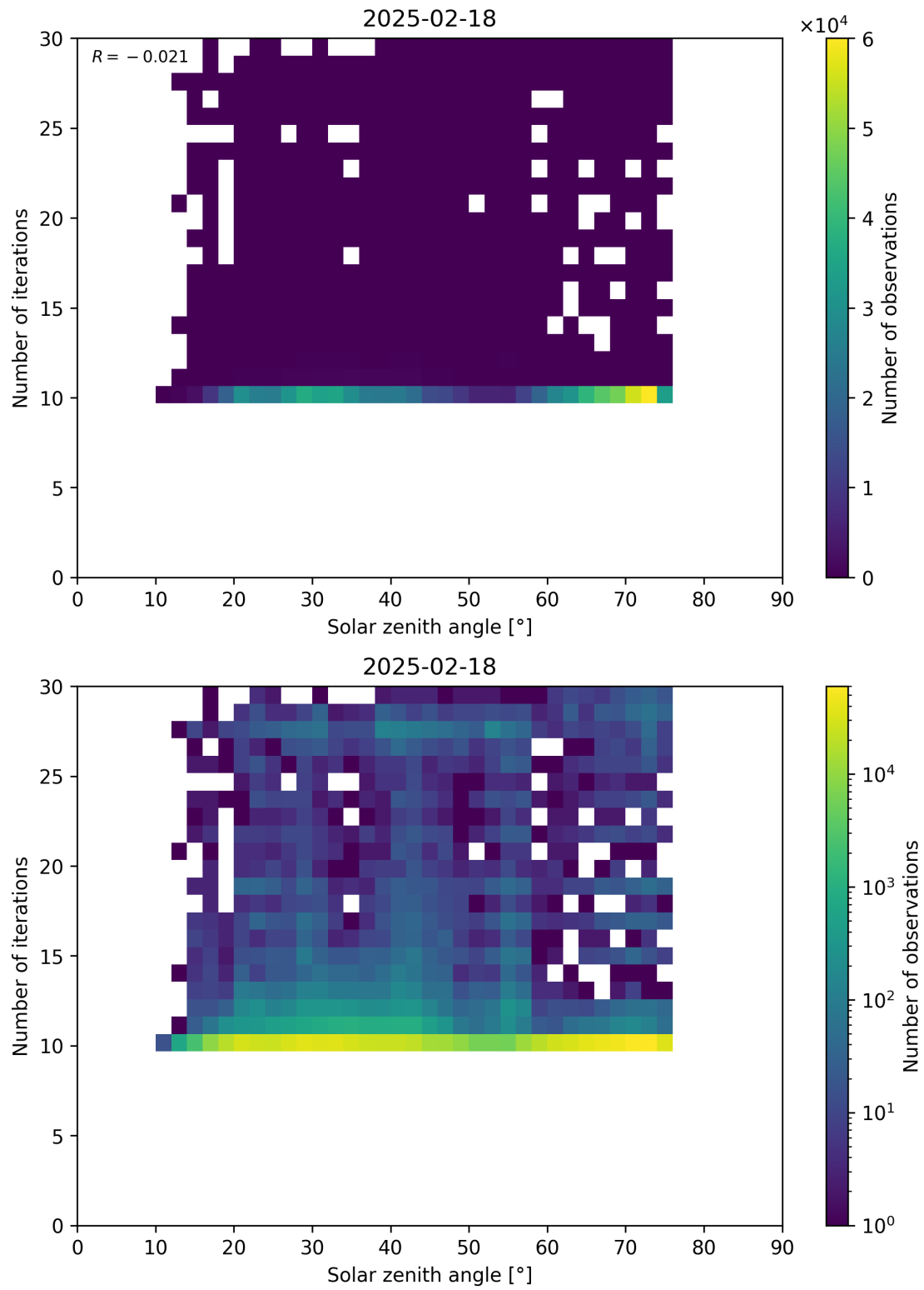
Figure 102: Scatter density plot of “Solar zenith angle” against “Number of iterations” for 2025-02-18 to 2025-02-19.
