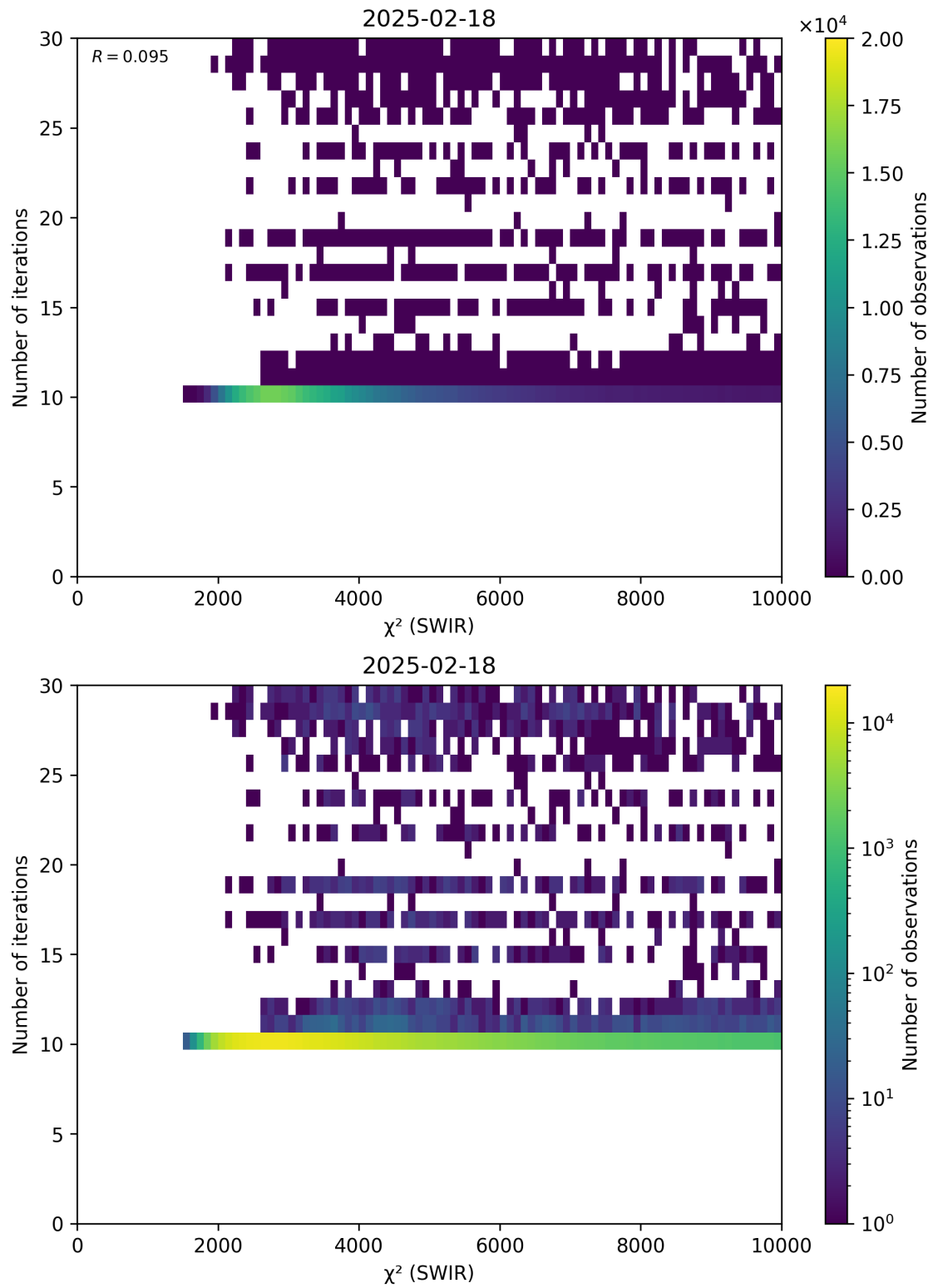
Figure 50: Scatter density plot of “ \chi^2 (SWIR)” against “Number of iterations” for 2025-02-18 to 2025-02-19.
