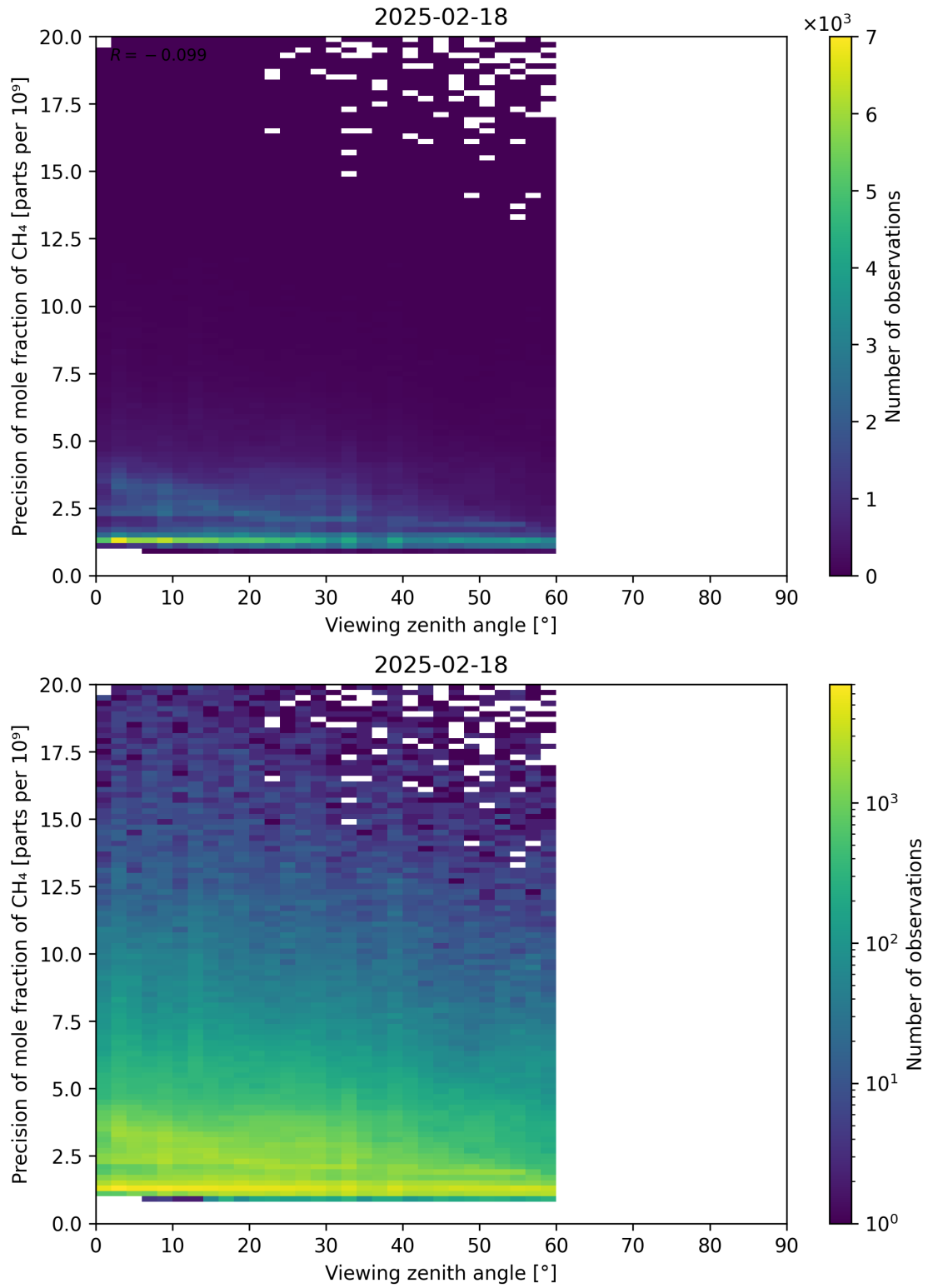
Figure 112: Scatter density plot of “Viewing zenith angle” against “Precision of mole fraction of CH 4 ” for 2025-02-18 to 2025-02-19.
