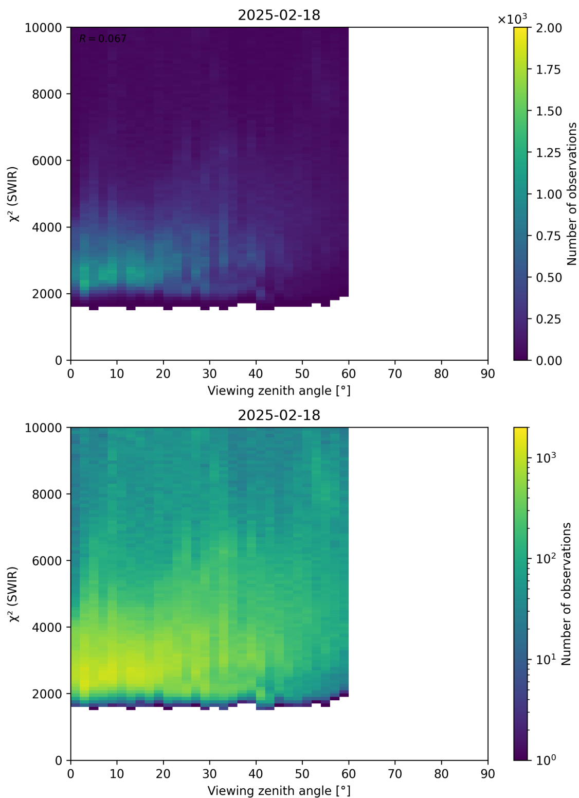
Figure 106: Scatter density plot of “Viewing zenith angle” against “ \chi^2 (SWIR)” for 2025-02-18 to 2025-02-19.
