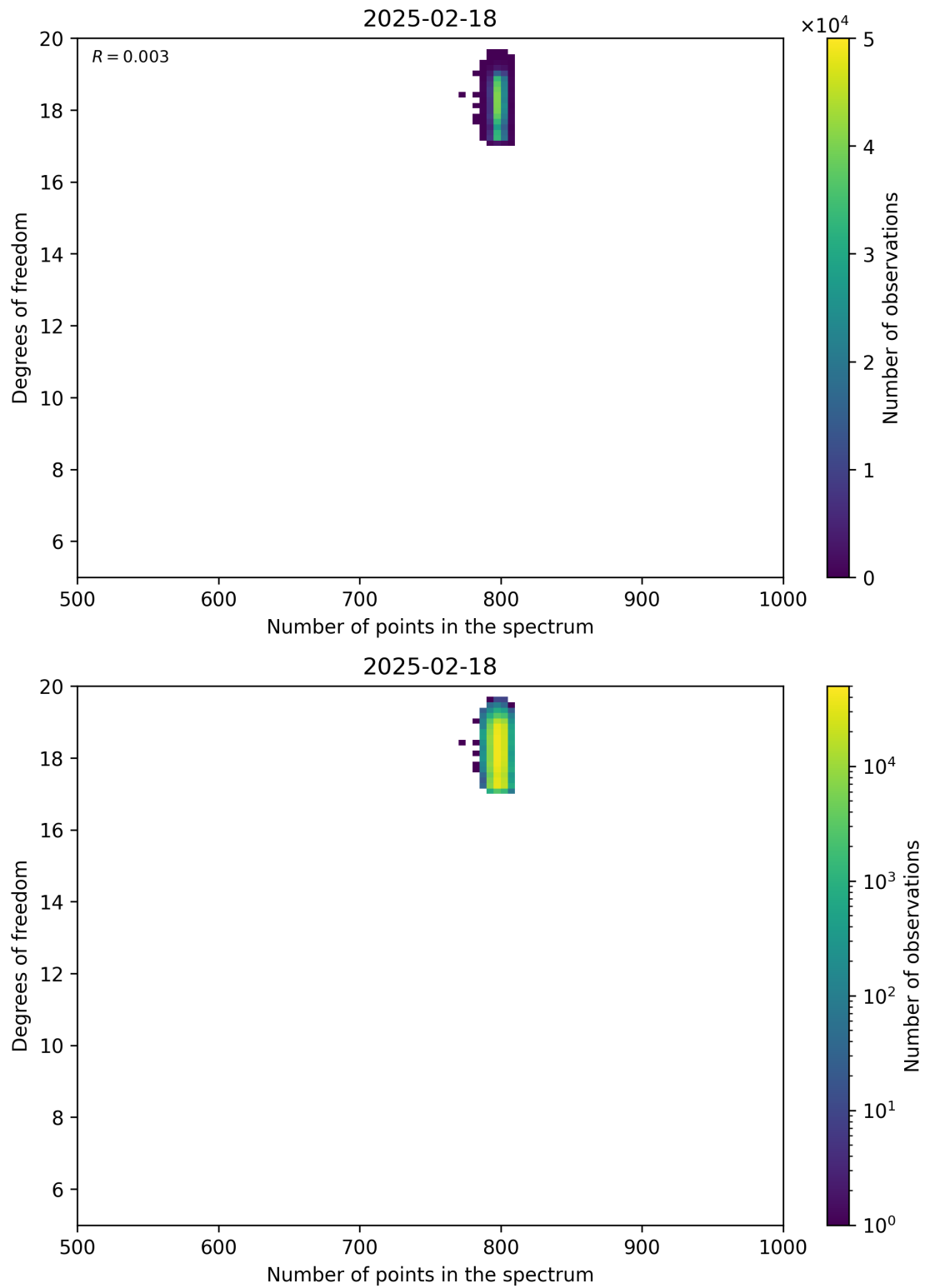
Figure 90: Scatter density plot of “Number of points in the spectrum” against “Degrees of freedom” for 2025-02-18 to 2025-02-19.
