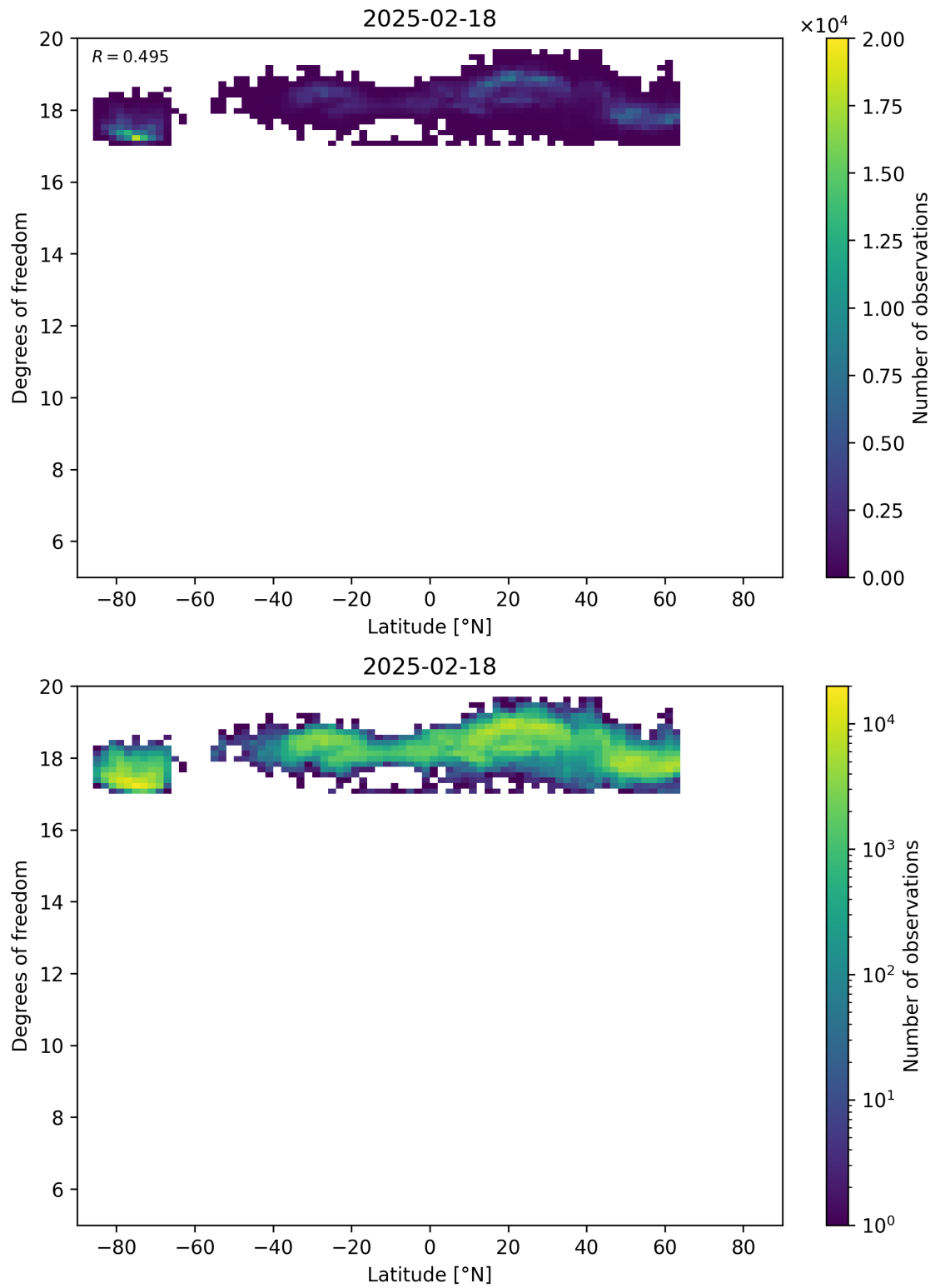
Figure 55: Scatter density plot of “Latitude” against “Degrees of freedom” for 2025-02-18 to 2025-02-19.
