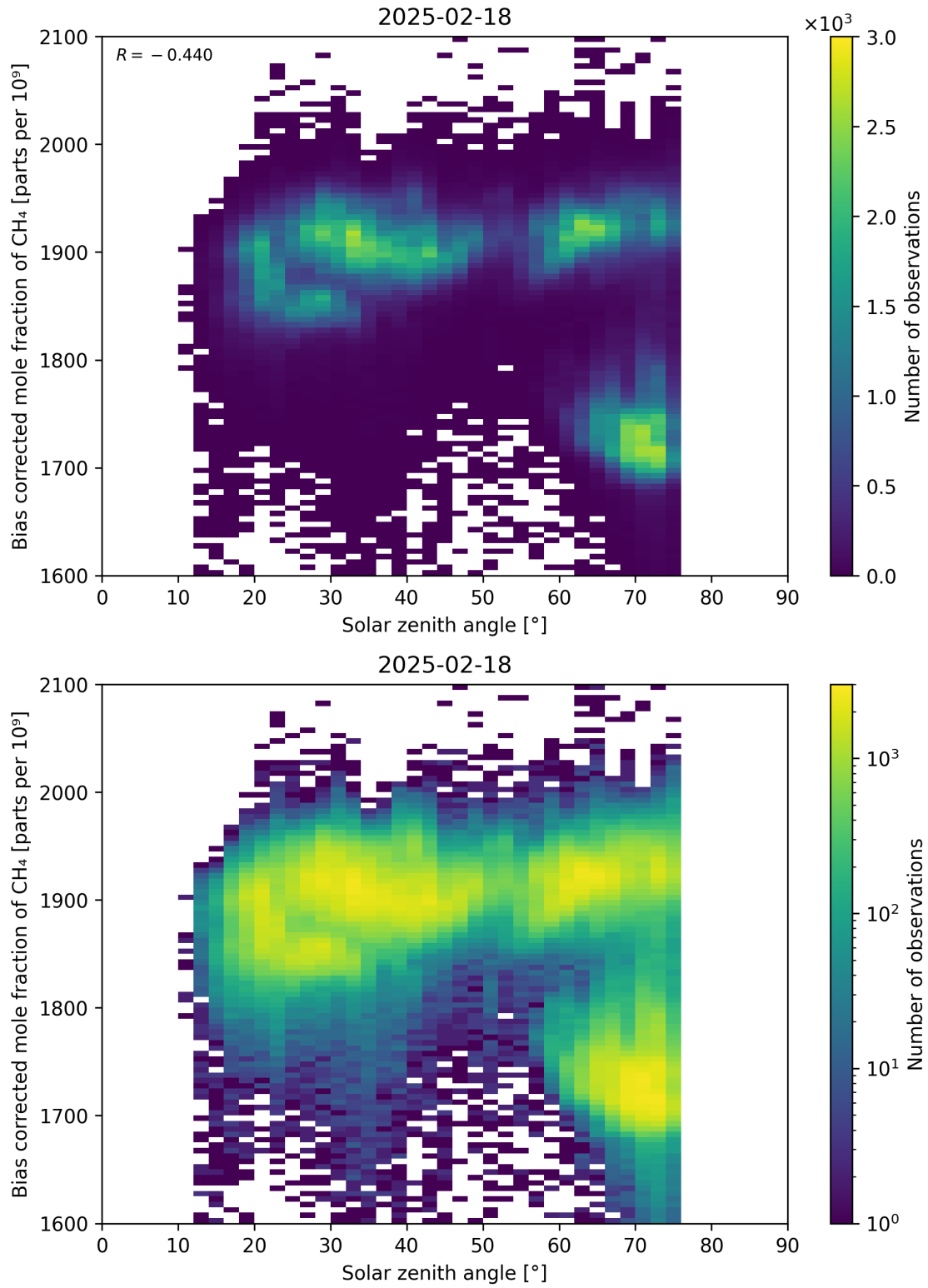
Figure 100: Scatter density plot of “Solar zenith angle” against “Bias corrected mole fraction of CH 4 ” for 2025-02-18 to 2025-02-19.
