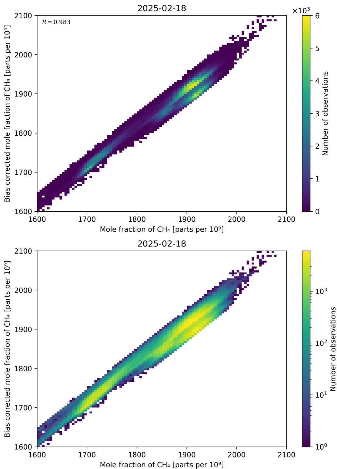
Figure 74: Scatter density plot of “Mole fraction of CH 4 ” against “Bias corrected mole fraction of CH 4 ” for 2025-02-18 to 2025-02-19.
