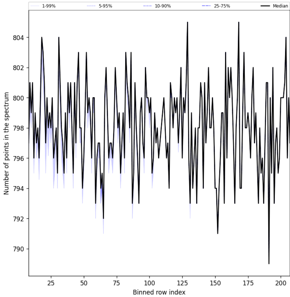
Figure 37: Along track statistics of “Number of points in the spectrum” for 2025-02-18 to 2025-02-19
