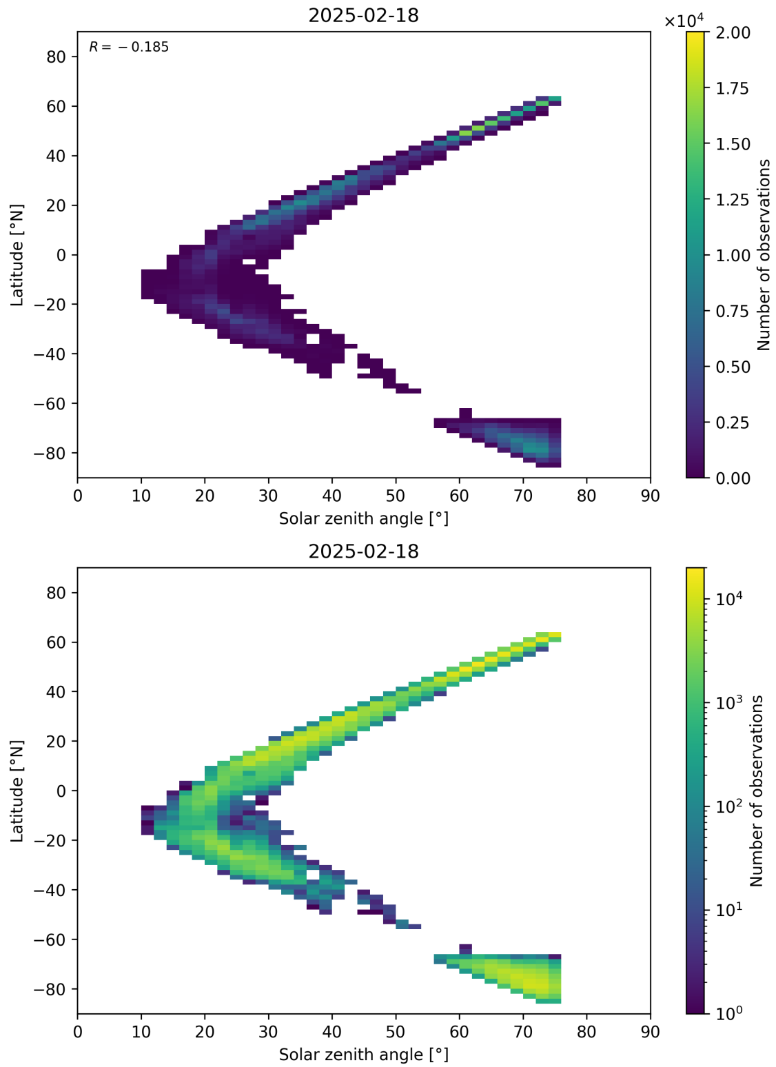
Figure 98: Scatter density plot of “Solar zenith angle” against “Latitude” for 2025-02-18 to 2025-02-19.
