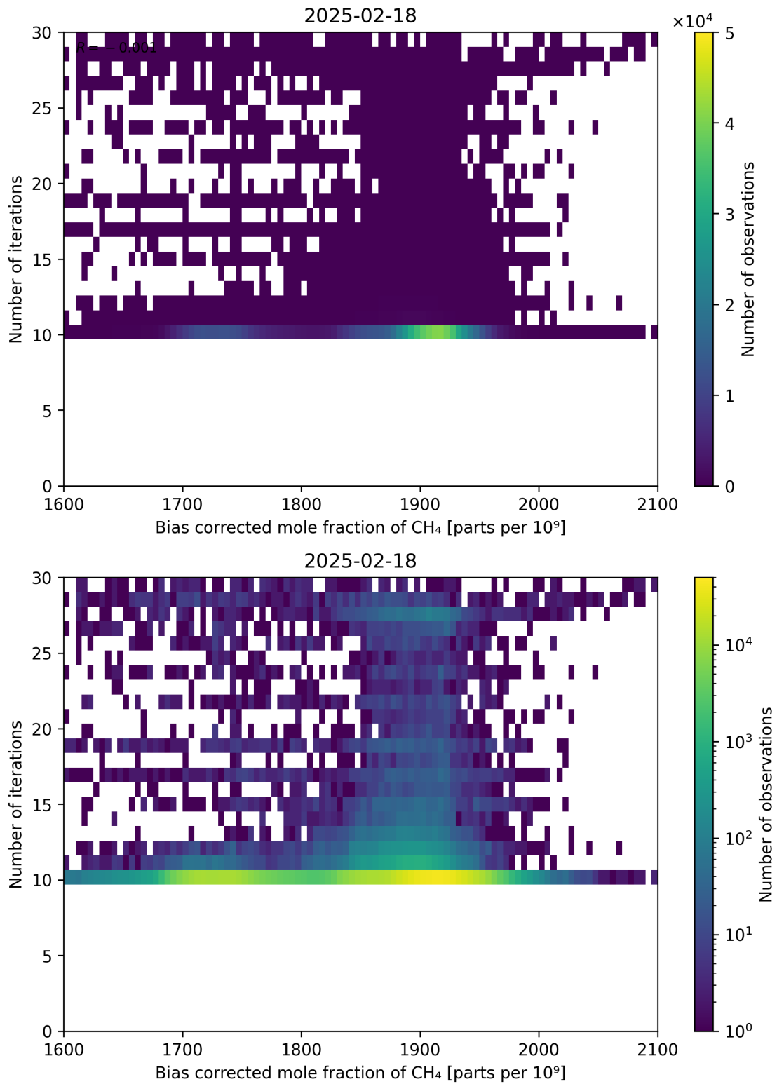
Figure 67: Scatter density plot of “Bias corrected mole fraction of CH 4 ” against “Number of iterations” for 2025-02-18 to 2025-02-19.
