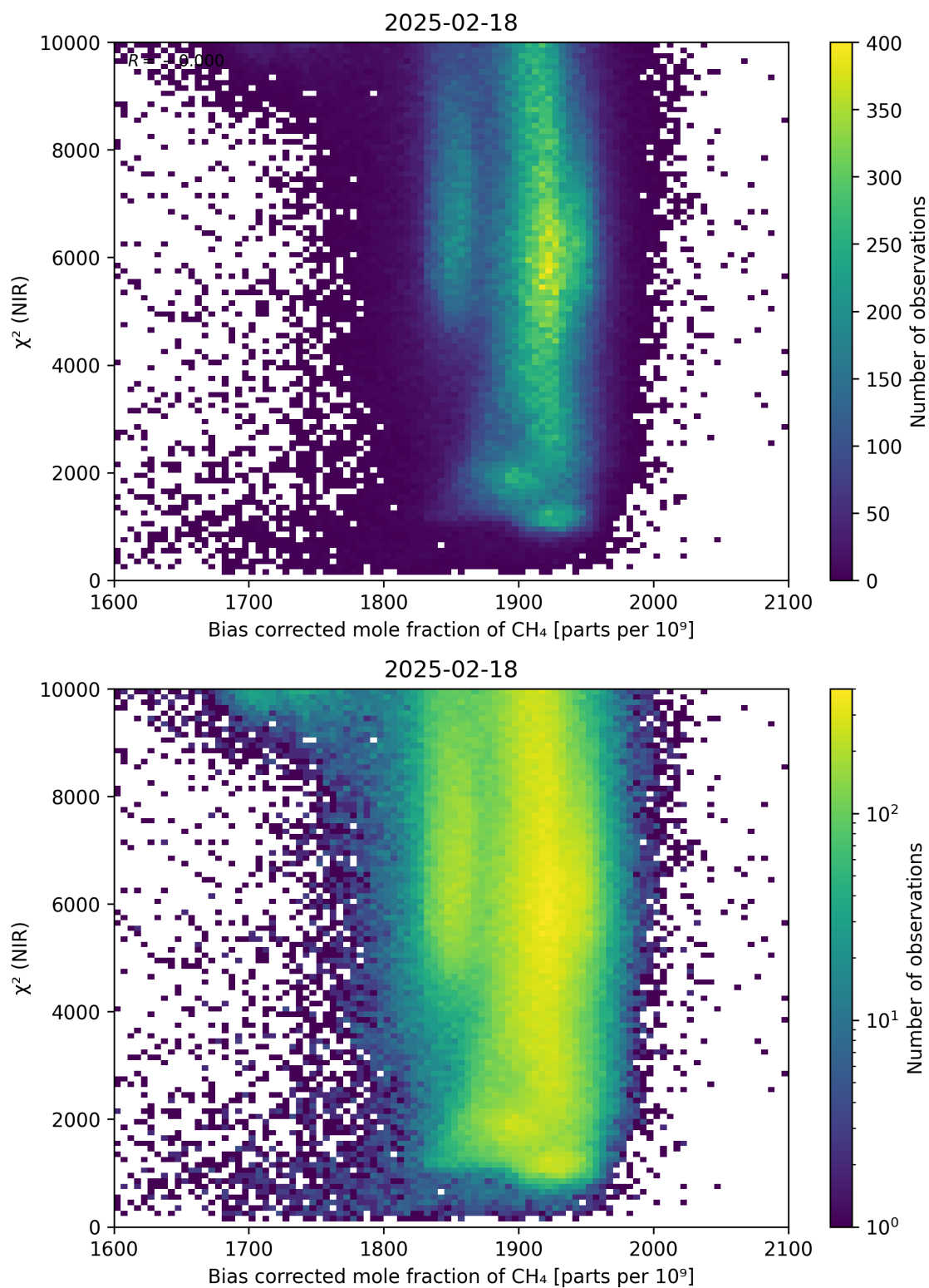
Figure 63: Scatter density plot of “Bias corrected mole fraction of CH 4 ” against “ \chi^2 (NIR)” for 2025-02-18 to 2025-02-19.
