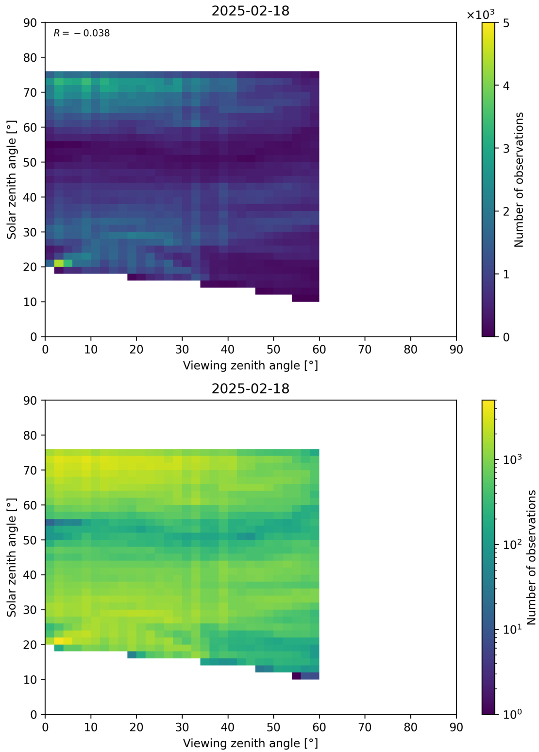
Figure 115: Scatter density plot of “Viewing zenith angle” against “Solar zenith angle” for 2025-02-18 to 2025-02-19.
