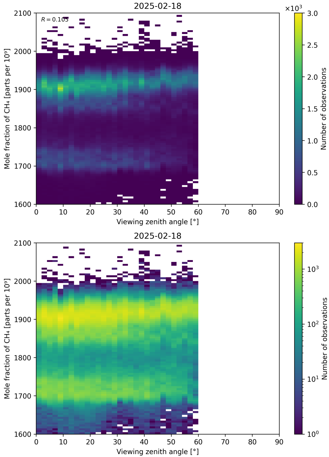
Figure 110: Scatter density plot of “Viewing zenith angle” against “Mole fraction of \text{CH}_4 ” for 2025-02-18 to 2025-02-19.
