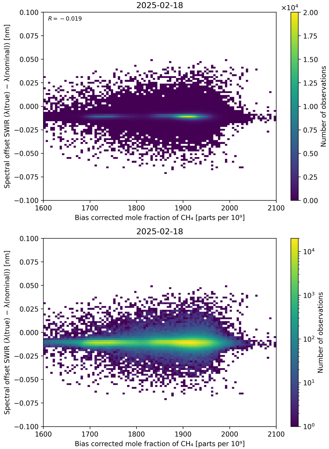
Figure 69: Scatter density plot of “Bias corrected mole fraction of CH 4 ” against “Spectral offset SWIR ( \lambda_{\text{true}} - \lambda_{\text{nominal}} )” for 2025-02-18 to 2025-02-19.
