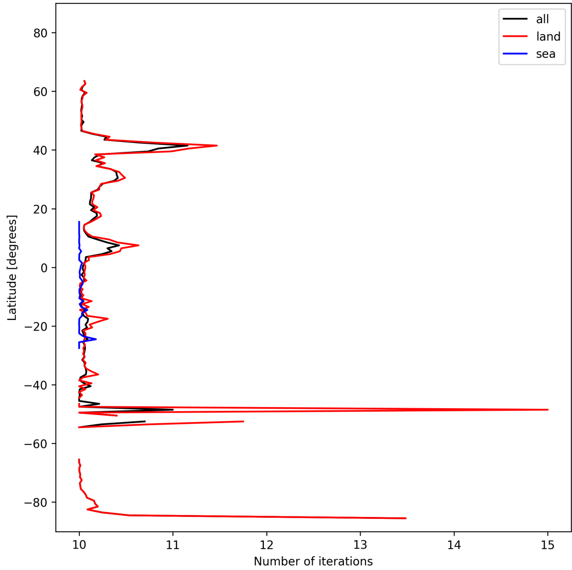
Figure 20: Zonal average of “Number of iterations” for 2025-02-18 to 2025-02-19.
