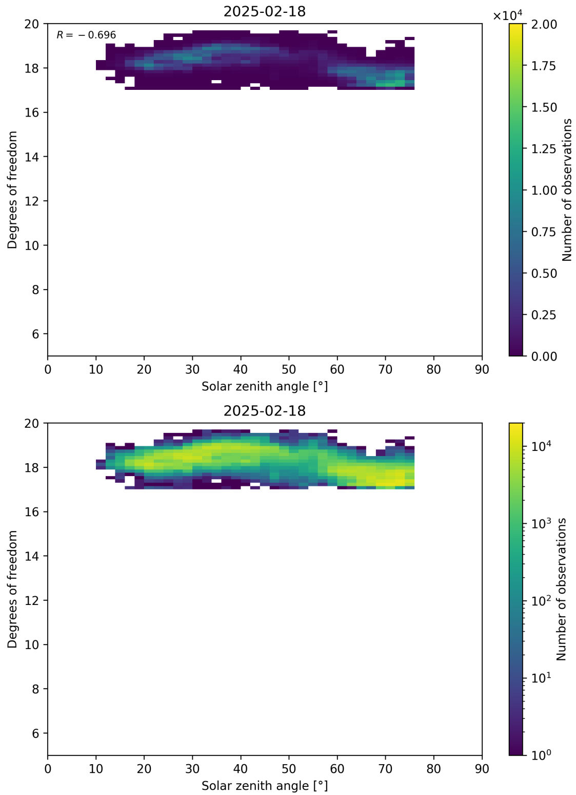
Figure 96: Scatter density plot of “Solar zenith angle” against “Degrees of freedom” for 2025-02-18 to 2025-02-19.
