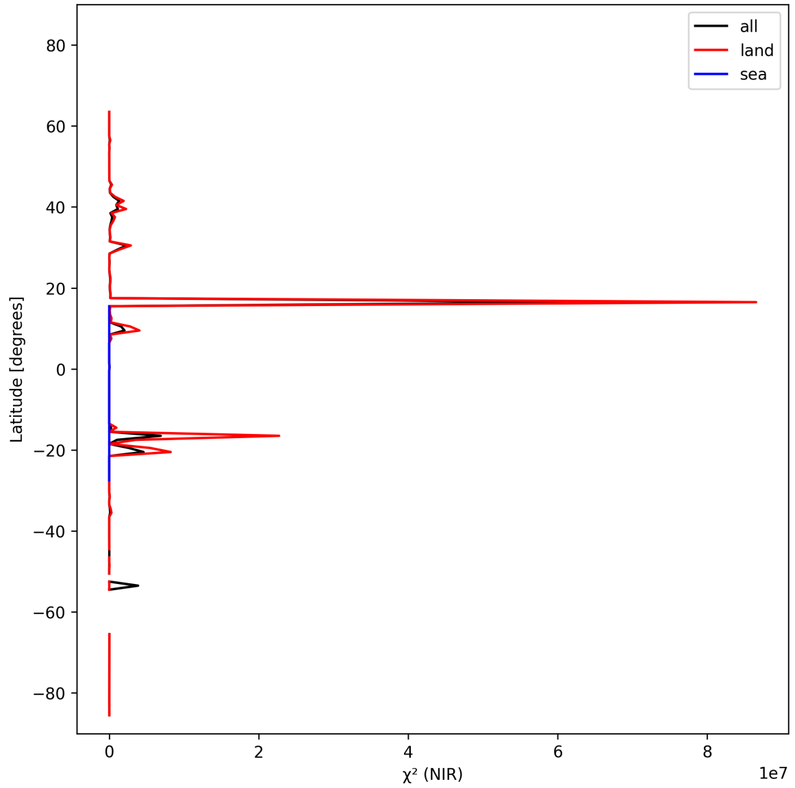
Figure 18: Zonal average of “ \chi^2 (NIR)” for 2025-02-18 to 2025-02-19.
