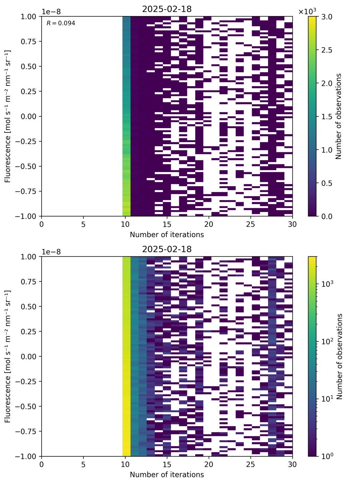
Figure 87: Scatter density plot of “Number of iterations” against “Fluorescence” for 2025-02-18 to 2025-02-19.
