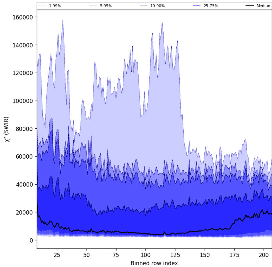
Figure 39: Along track statistics of “ \chi^2 (SWIR)” for 2025-02-18 to 2025-02-19
