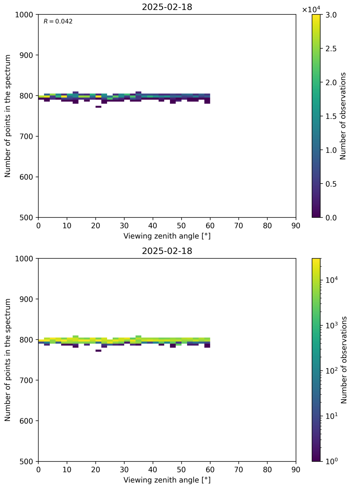
Figure 114: Scatter density plot of “Viewing zenith angle” against “Number of points in the spectrum” for 2025-02-18 to 2025-02-19.
