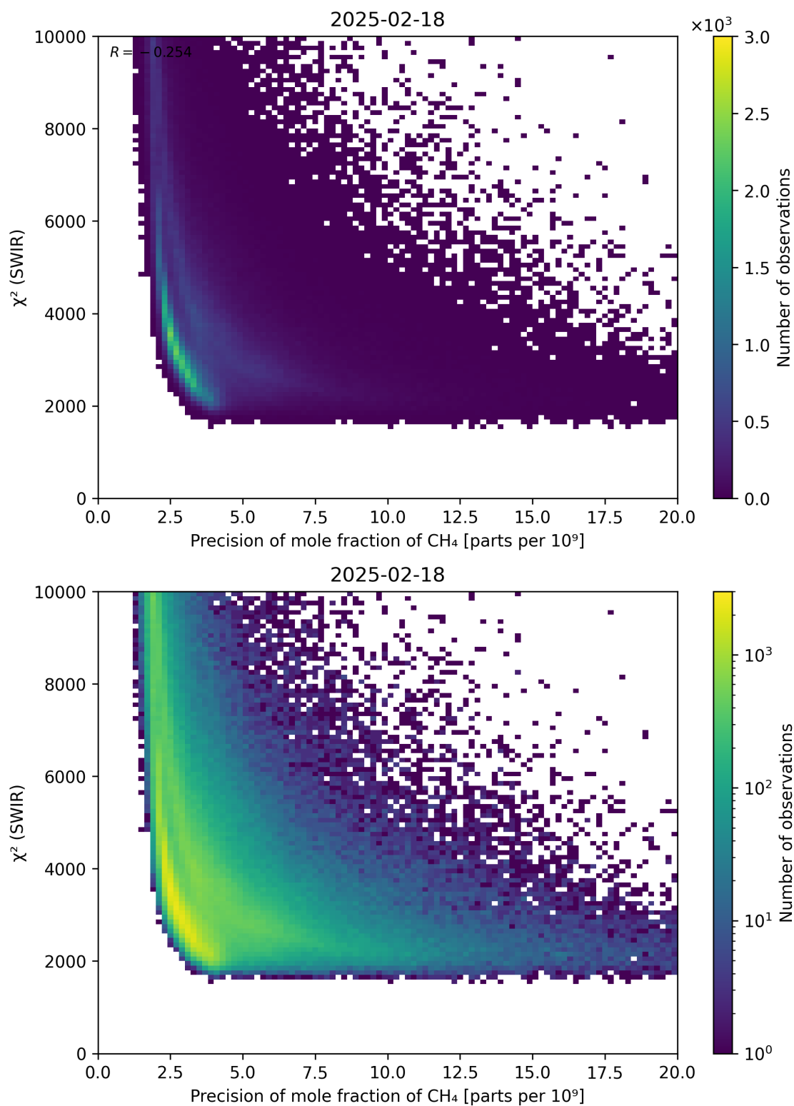
Figure 79: Scatter density plot of “Precision of mole fraction of CH 4 ” against “ \chi^2 (SWIR)” for 2025-02-18 to 2025-02-19.
