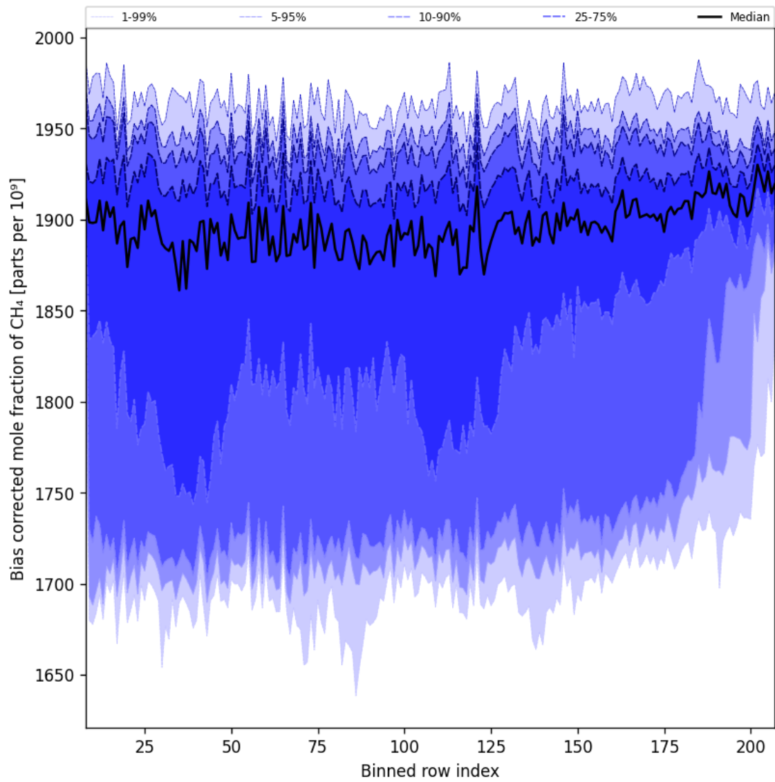
Figure 36: Along track statistics of “Bias corrected mole fraction of CH 4 ” for 2025-02-18 to 2025-02-19
