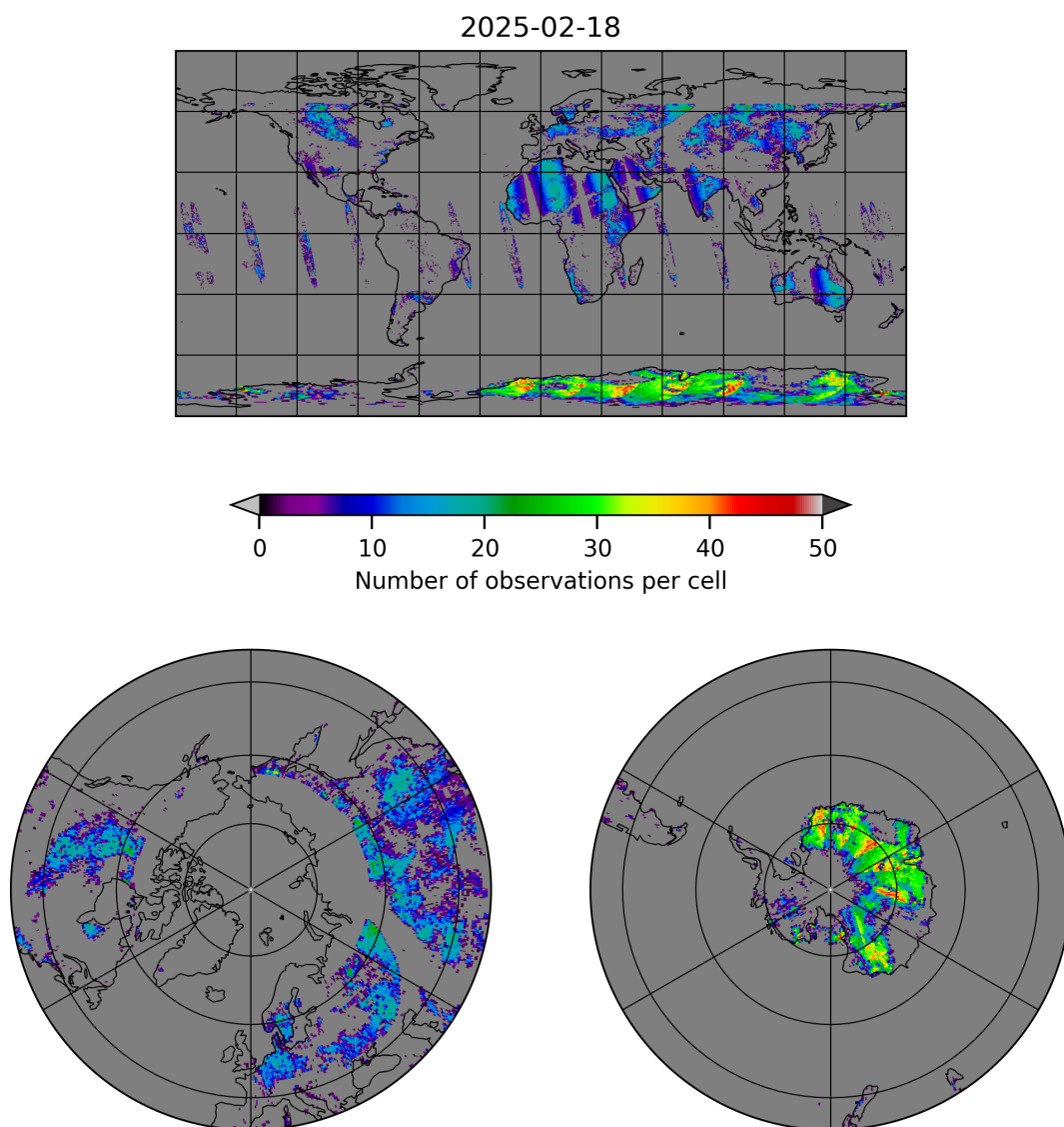
Figure 10: Map of the number of observations for 2025-02-18 to 2025-02-19
