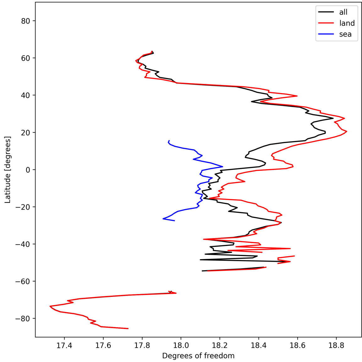
Figure 19: Zonal average of “Degrees of freedom” for 2025-02-18 to 2025-02-19.
