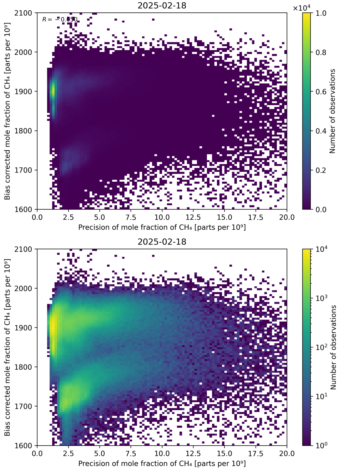
Figure 82: Scatter density plot of “Precision of mole fraction of CH 4 ” against “Bias corrected mole fraction of CH 4 ” for 2025-02-18 to 2025-02-19.
