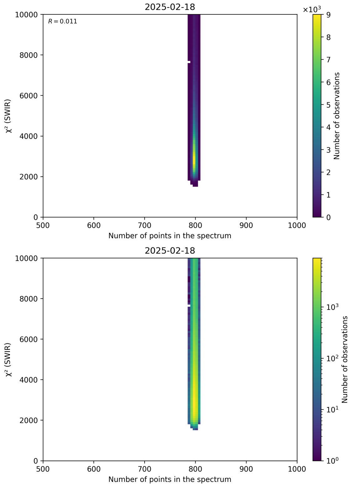
Figure 89: Scatter density plot of “Number of points in the spectrum” against “ \chi^2 (SWIR)” for 2025-02-18 to 2025-02-19.
