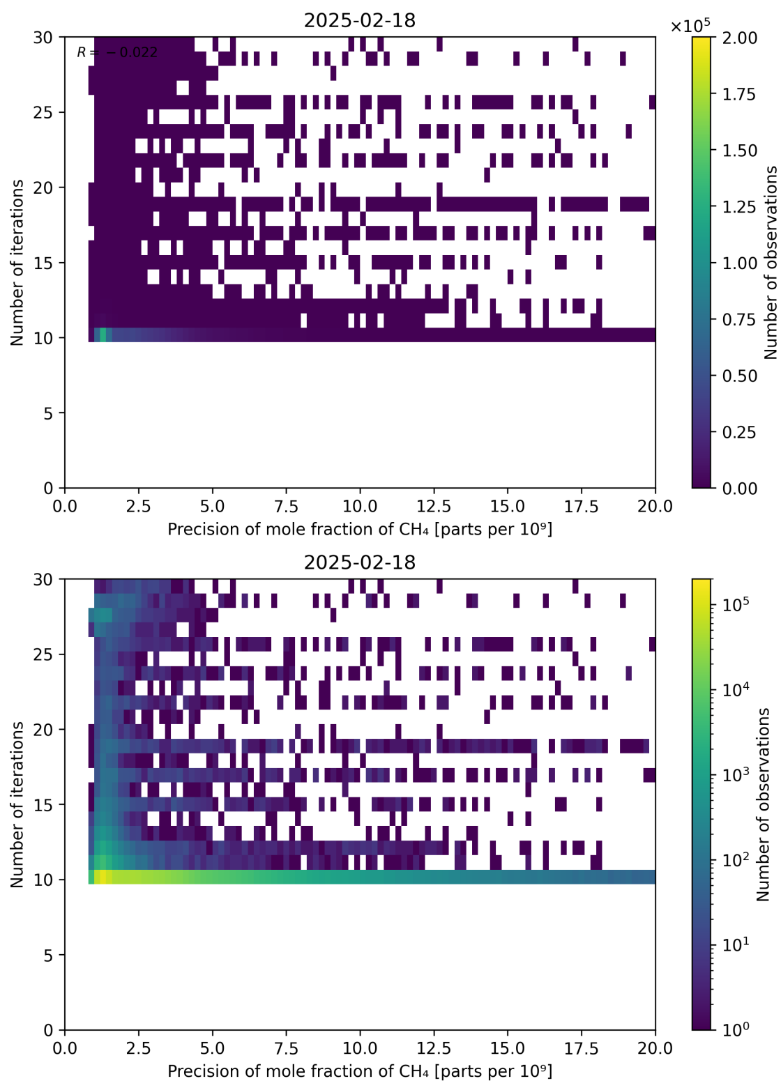
Figure 83: Scatter density plot of “Precision of mole fraction of CH 4 ” against “Number of iterations” for 2025-02-18 to 2025-02-19.
