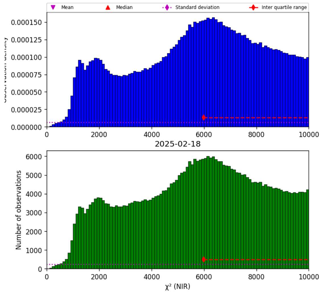
Figure 29: Histogram of “ \chi^2 (NIR)” for 2025-02-18 to 2025-02-19
