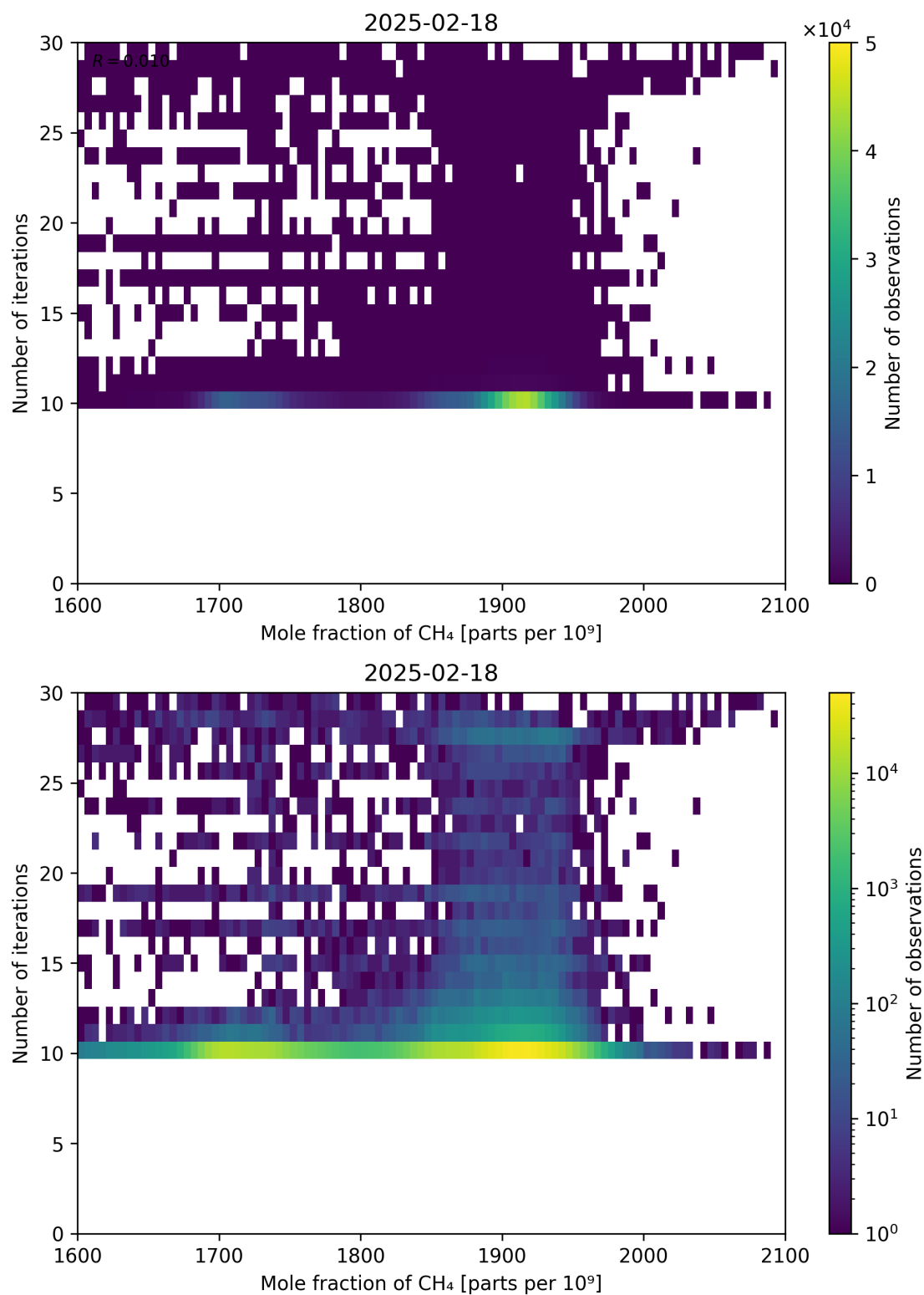
Figure 76: Scatter density plot of “Mole fraction of CH 4 ” against “Number of iterations” for 2025-02-18 to 2025-02-19.
