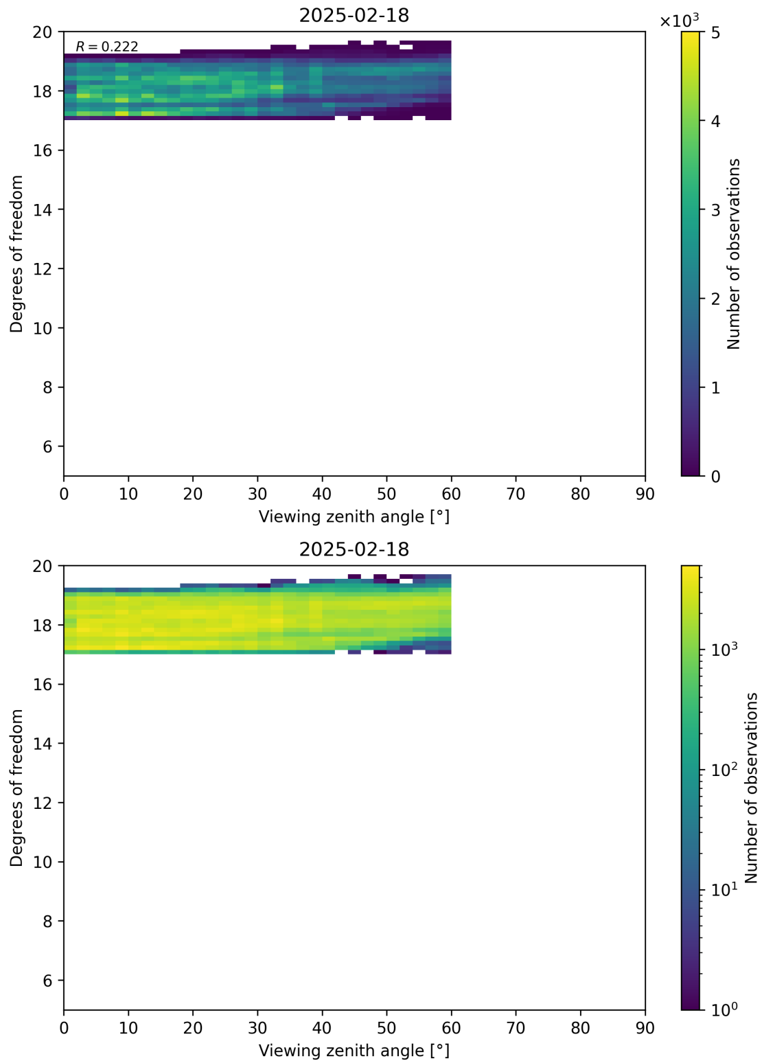
Figure 107: Scatter density plot of “Viewing zenith angle” against “Degrees of freedom” for 2025-02-18 to 2025-02-19.
