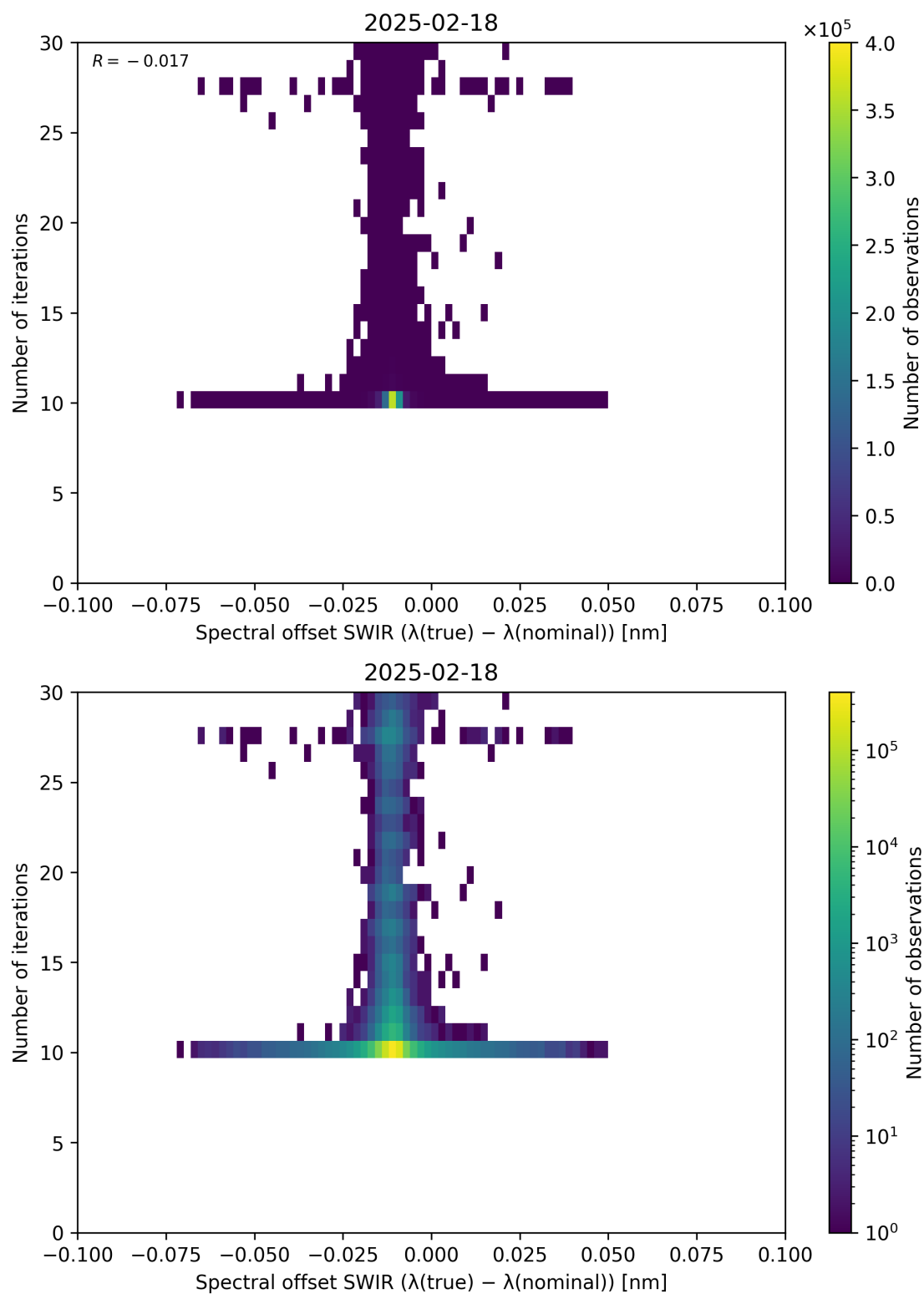
Figure 121: Scatter density plot of “Spectral offset SWIR ( \lambda_{\text{true}} - \lambda_{\text{nominal}} )” against “Number of iterations” for 2025-02-18 to 2025-02-19.
