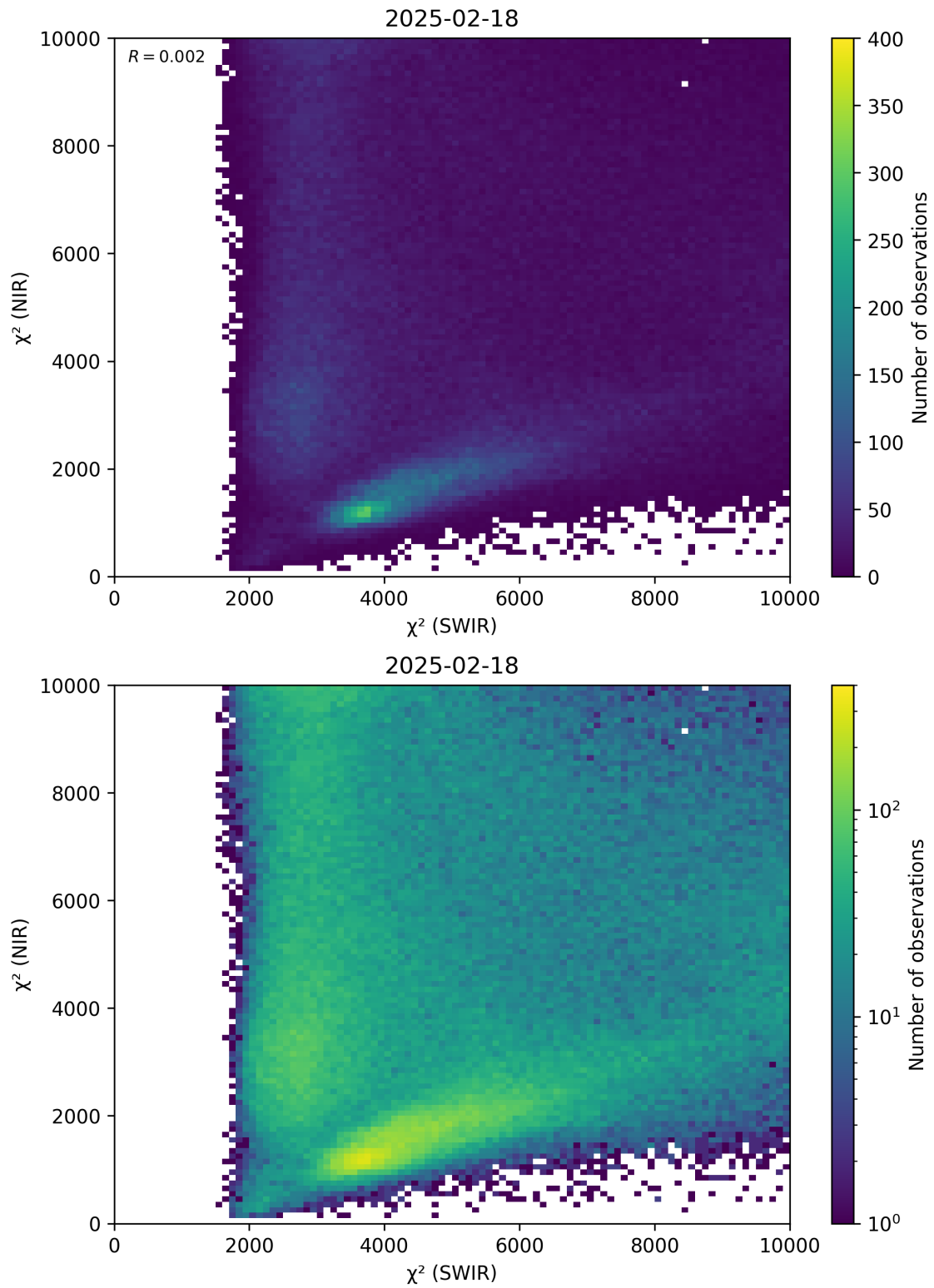
Figure 47: Scatter density plot of “ \chi^2 (SWIR)” against “ \chi^2 (NIR)” for 2025-02-18 to 2025-02-19.
