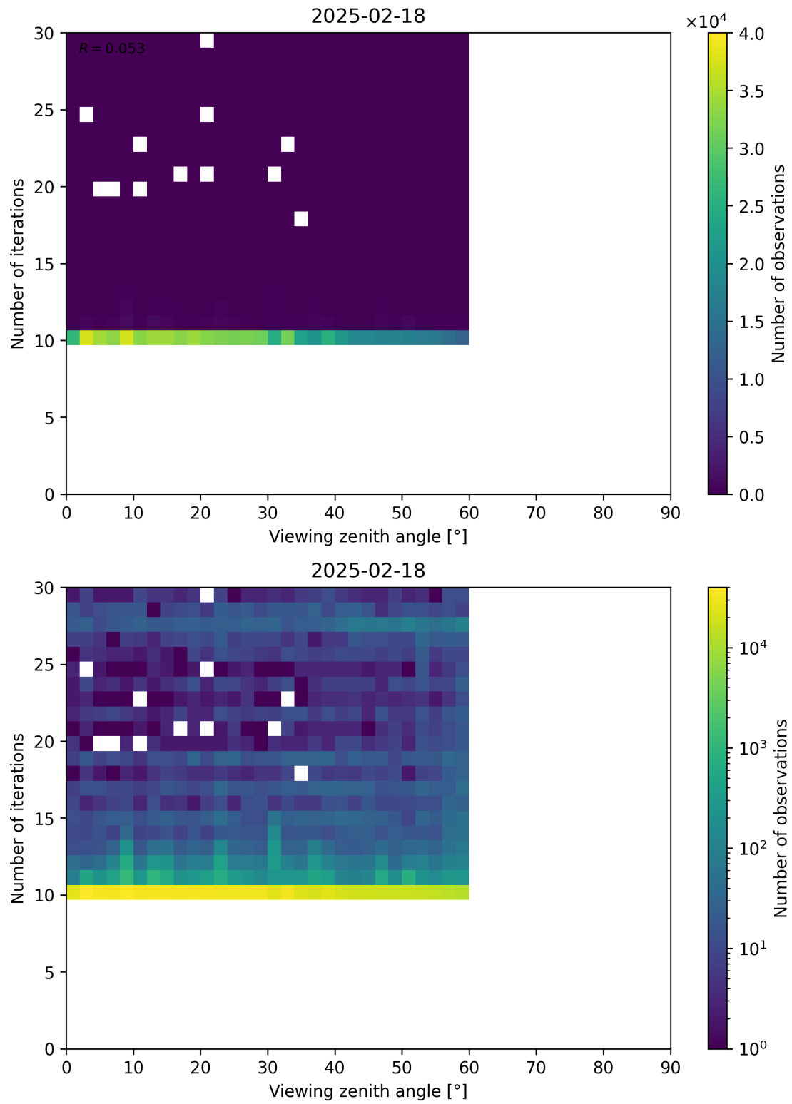
Figure 113: Scatter density plot of “Viewing zenith angle” against “Number of iterations” for 2025-02-18 to 2025-02-19.
