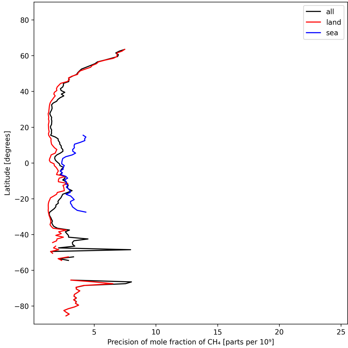
Figure 13: Zonal average of “Precision of mole fraction of CH 4 ” for 2025-02-18 to 2025-02-19.
