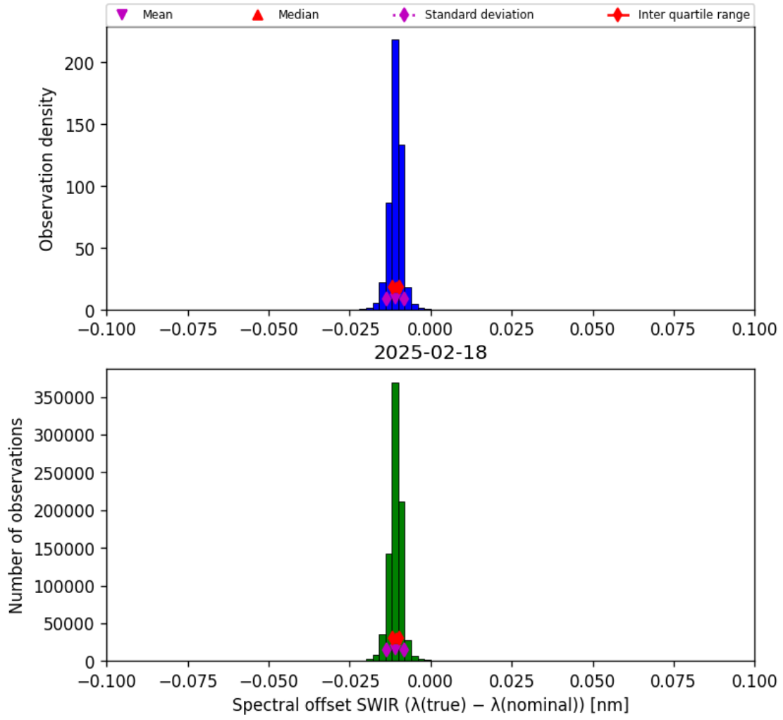
Figure 27: Histogram of “Spectral offset SWIR ( \lambda_{\text{true}} - \lambda_{\text{nominal}} )” for 2025-02-18 to 2025-02-19
