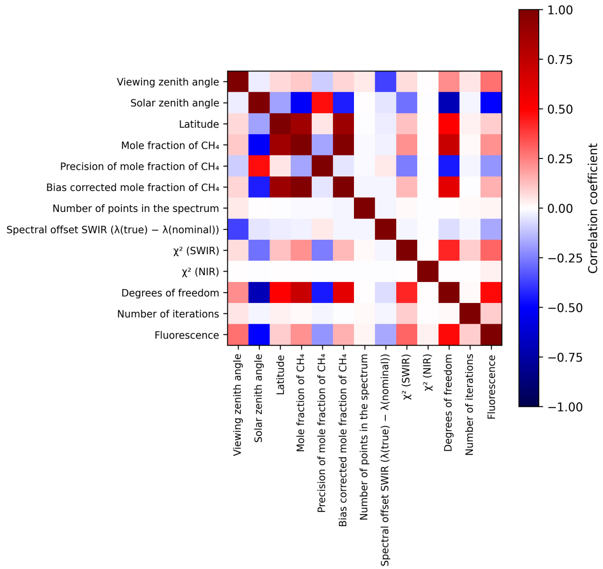
Figure 2: Map of correlation matrix for 2025-02-18 to 2025-02-19.
