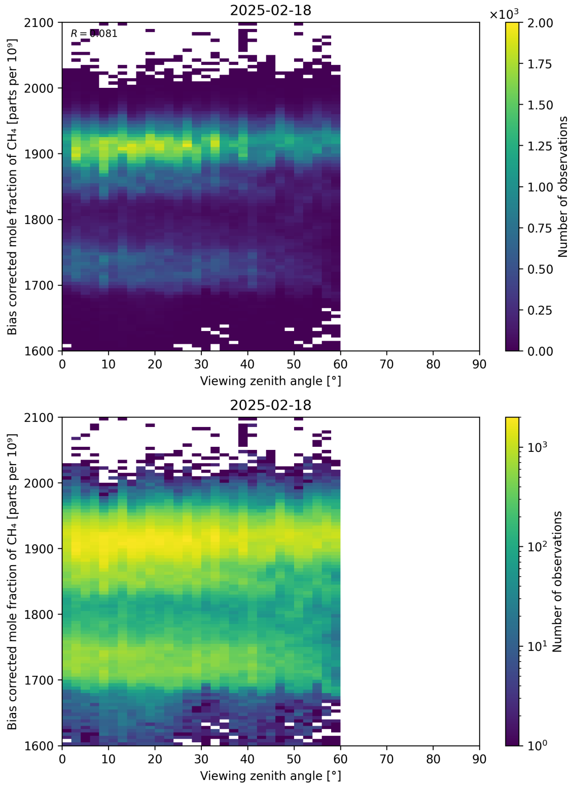
Figure 111: Scatter density plot of “Viewing zenith angle” against “Bias corrected mole fraction of CH 4 ” for 2025-02-18 to 2025-02-19.
