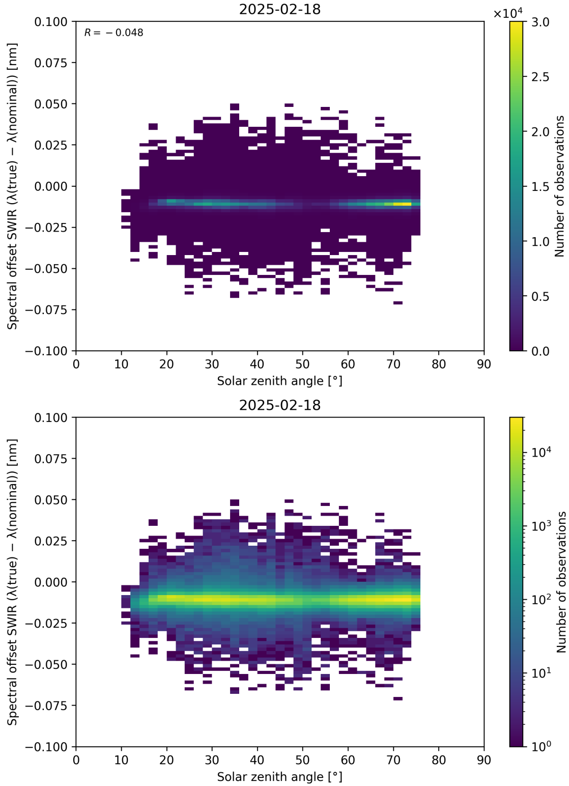
Figure 104: Scatter density plot of “Solar zenith angle” against “Spectral offset SWIR ( \lambda_{\text{true}} - \lambda_{\text{nominal}} )” for 2025-02-18 to 2025-02-19.
