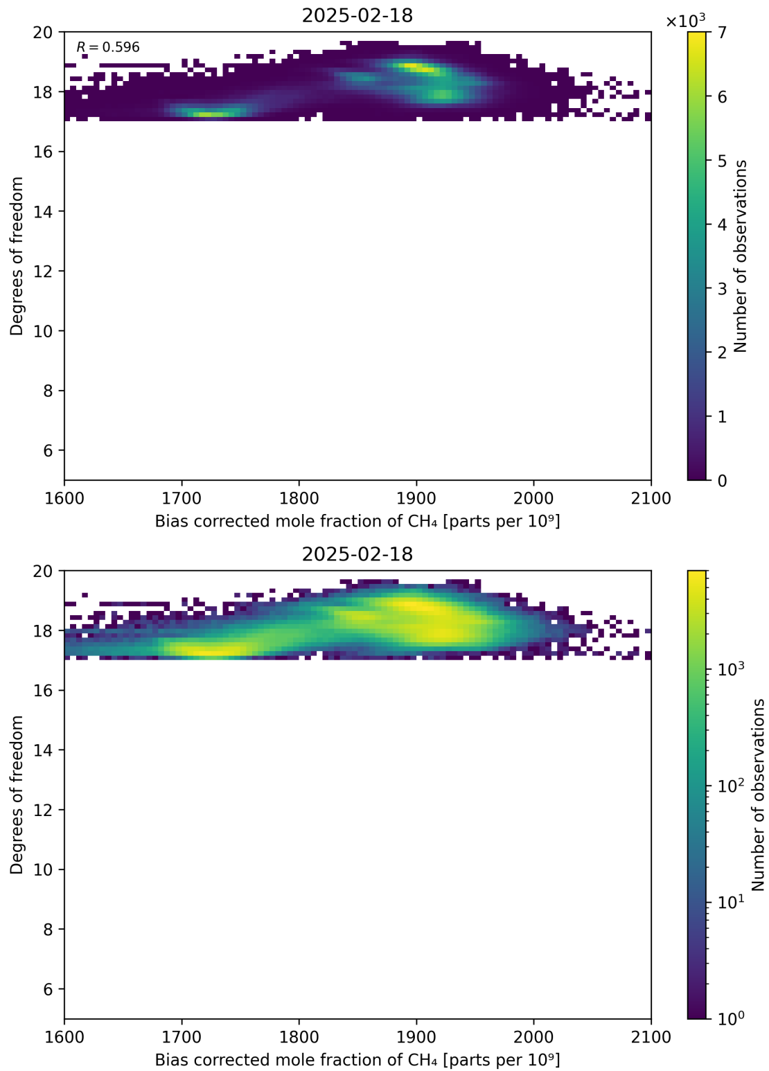
Figure 65: Scatter density plot of “Bias corrected mole fraction of CH 4 ” against “Degrees of freedom” for 2025-02-18 to 2025-02-19.
