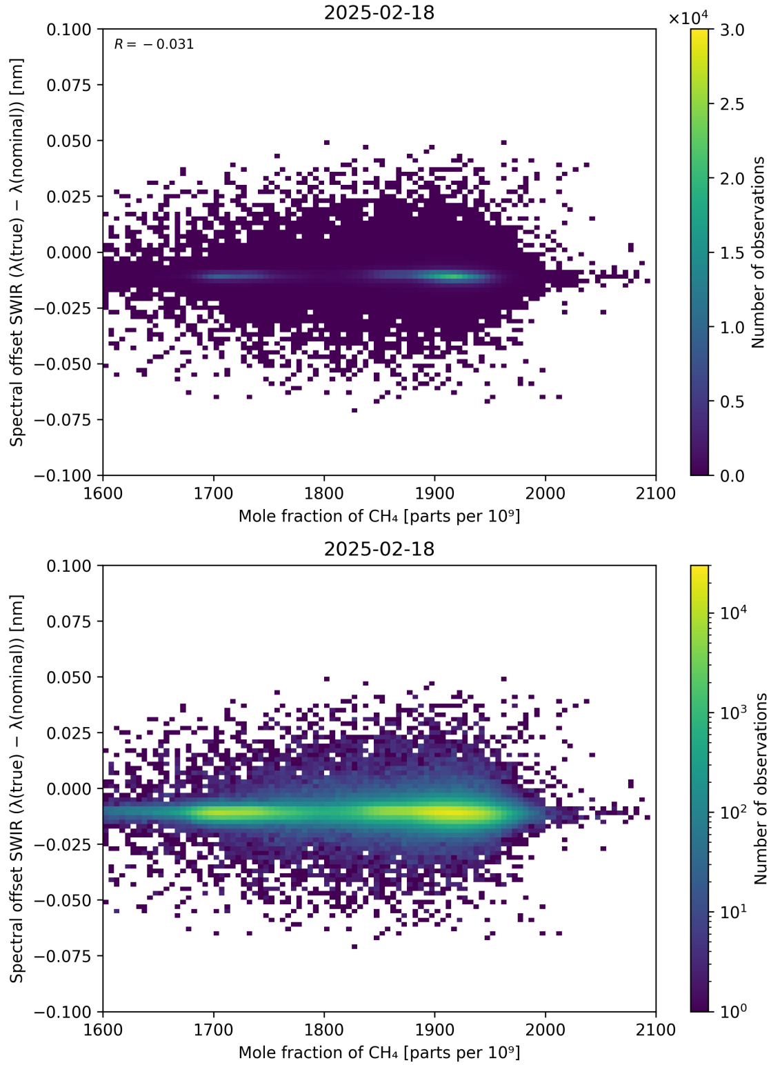
Figure 86: Scatter density plot of “Mole fraction of CH 4 ” against “Spectral offset SWIR ( \lambda_{\text{true}} - \lambda_{\text{nominal}} )” for 2025-02-18 to 2025-02-19.
