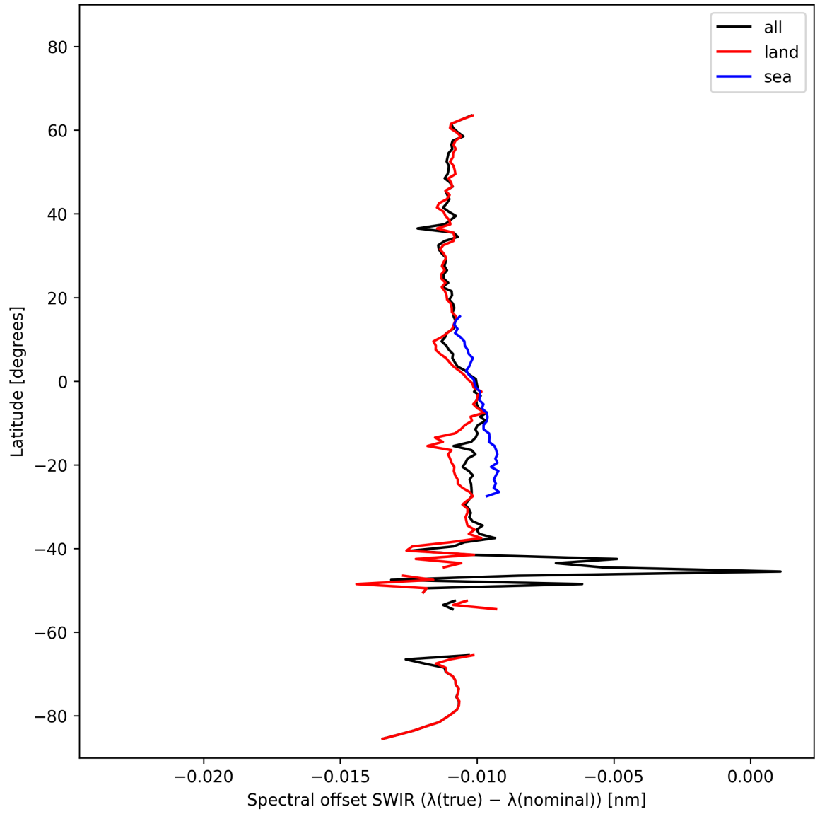
Figure 16: Zonal average of “Spectral offset SWIR ( \lambda_{\text{true}} - \lambda_{\text{nominal}} )” for 2025-02-18 to 2025-02-19.
