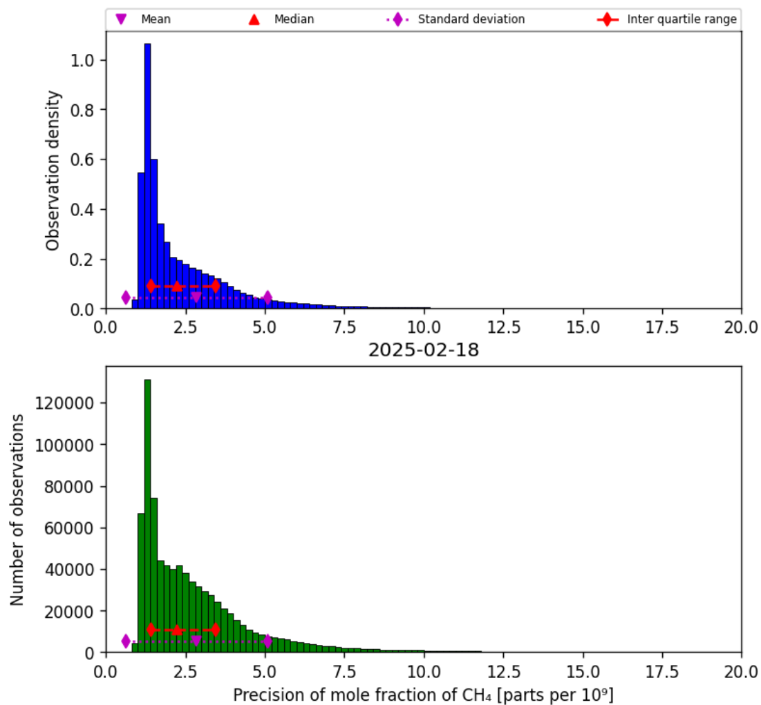
Figure 24: Histogram of “Precision of mole fraction of CH 4 ” for 2025-02-18 to 2025-02-19
