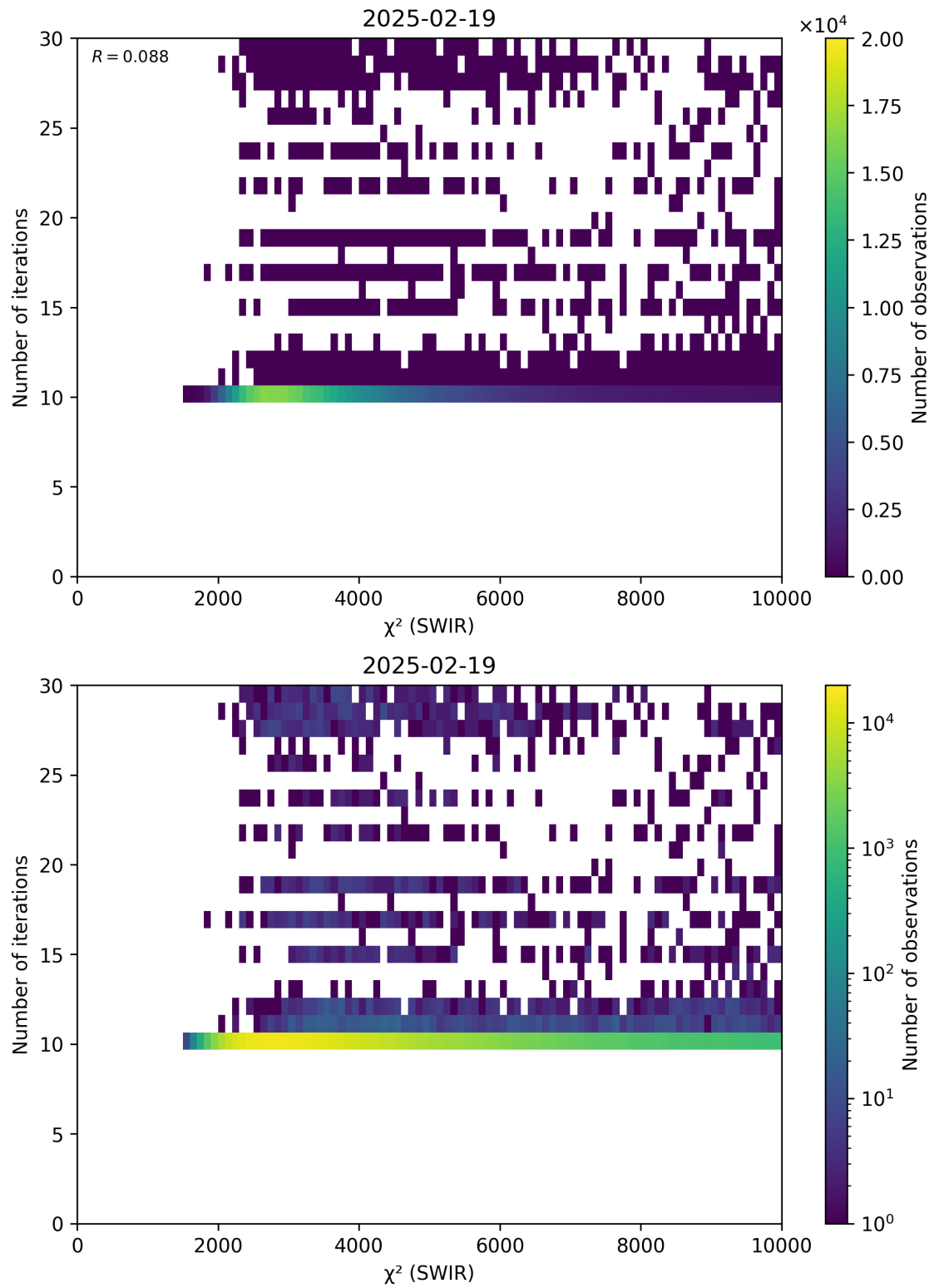
Figure 50: Scatter density plot of “ \chi^2 (SWIR)” against “Number of iterations” for 2025-02-19 to 2025-02-20.
