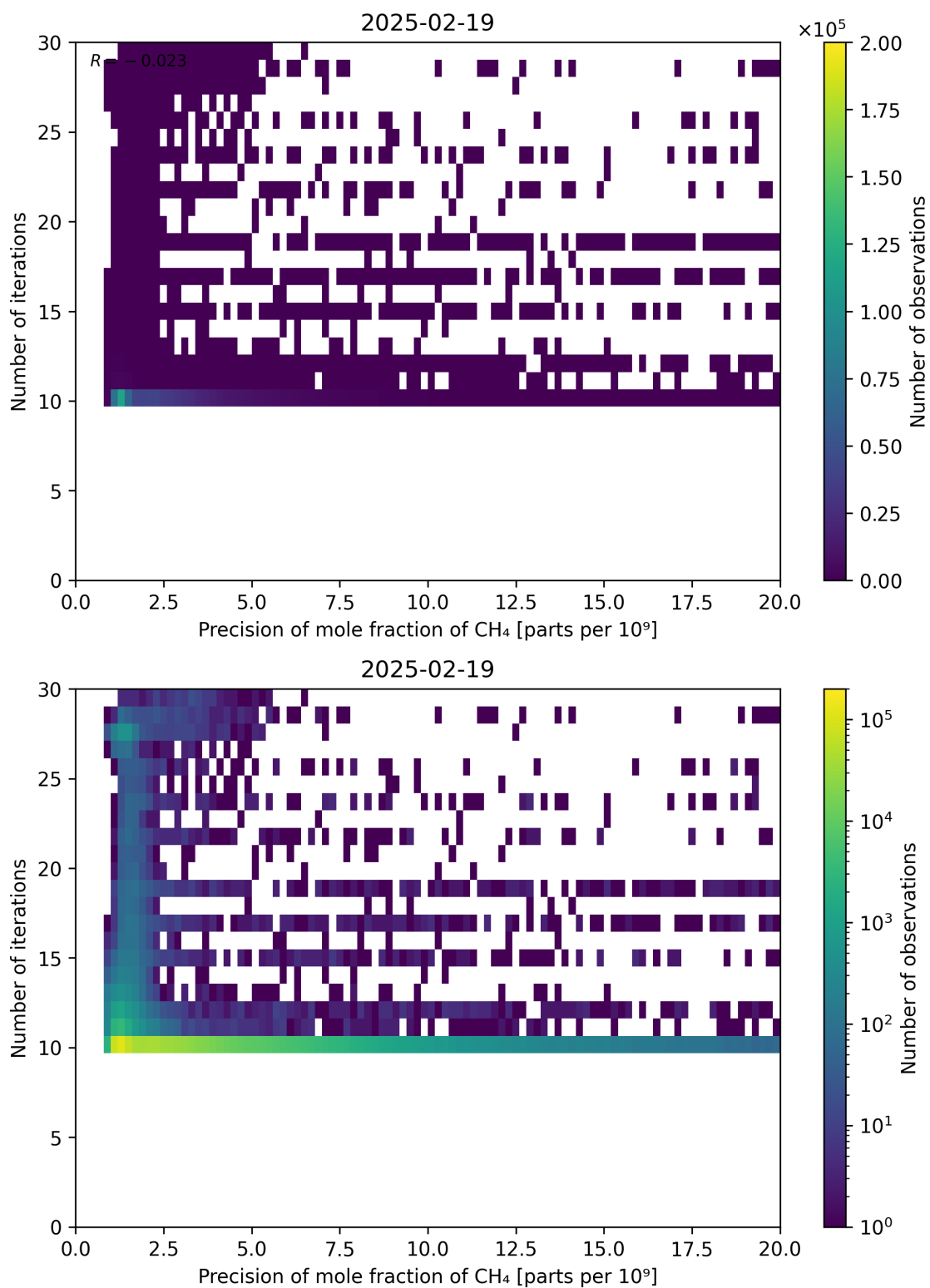
Figure 83: Scatter density plot of “Precision of mole fraction of CH 4 ” against “Number of iterations” for 2025-02-19 to 2025-02-20.
