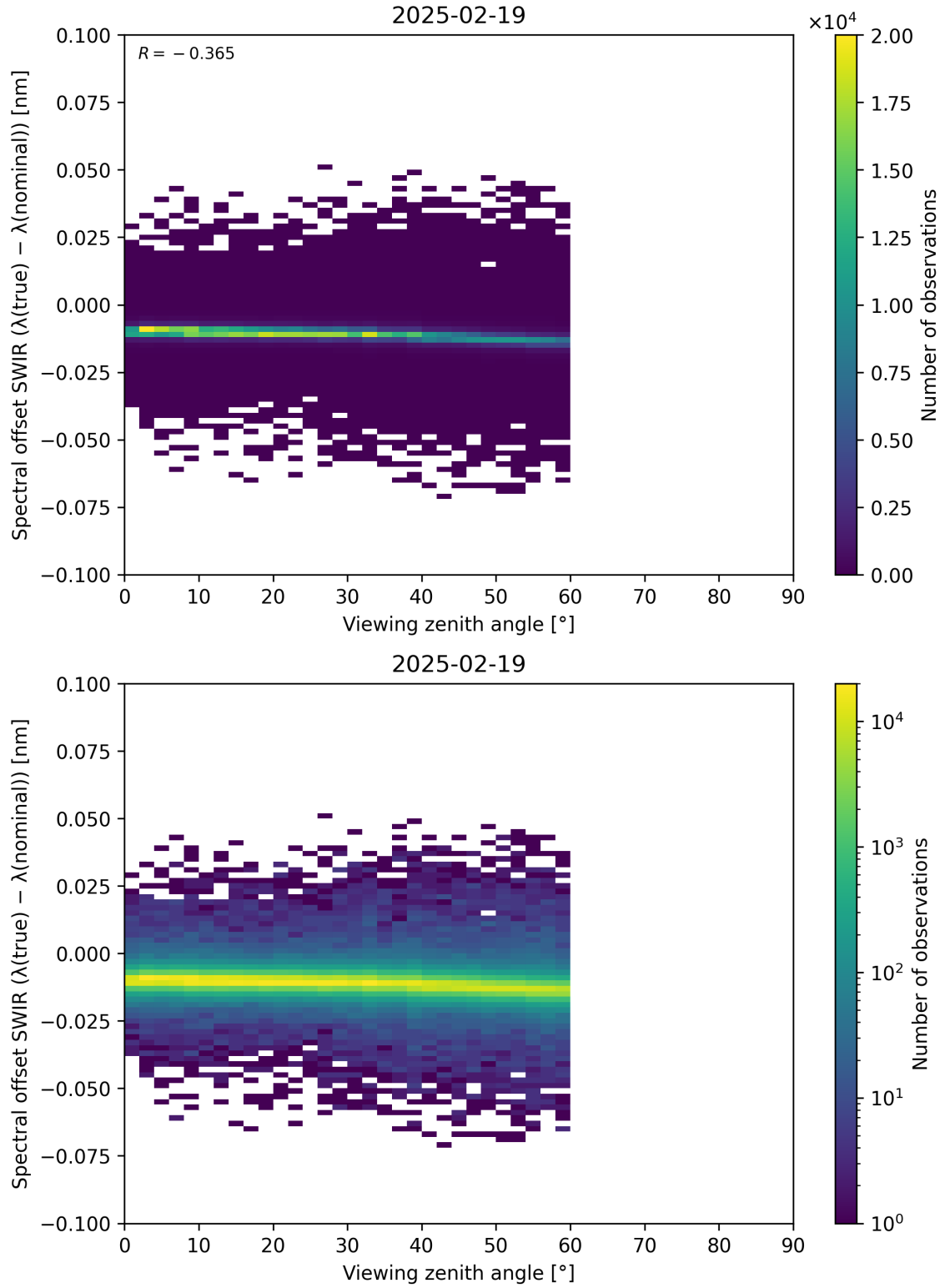
Figure 116: Scatter density plot of “Viewing zenith angle” against “Spectral offset SWIR ( \lambda_{\text{true}} - \lambda_{\text{nominal}} )” for 2025-02-19 to 2025-02-20.
