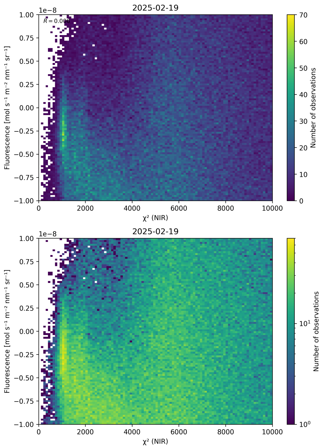
Figure 45: Scatter density plot of “ \chi^2 (NIR)” against “Fluorescence” for 2025-02-19 to 2025-02-20.
