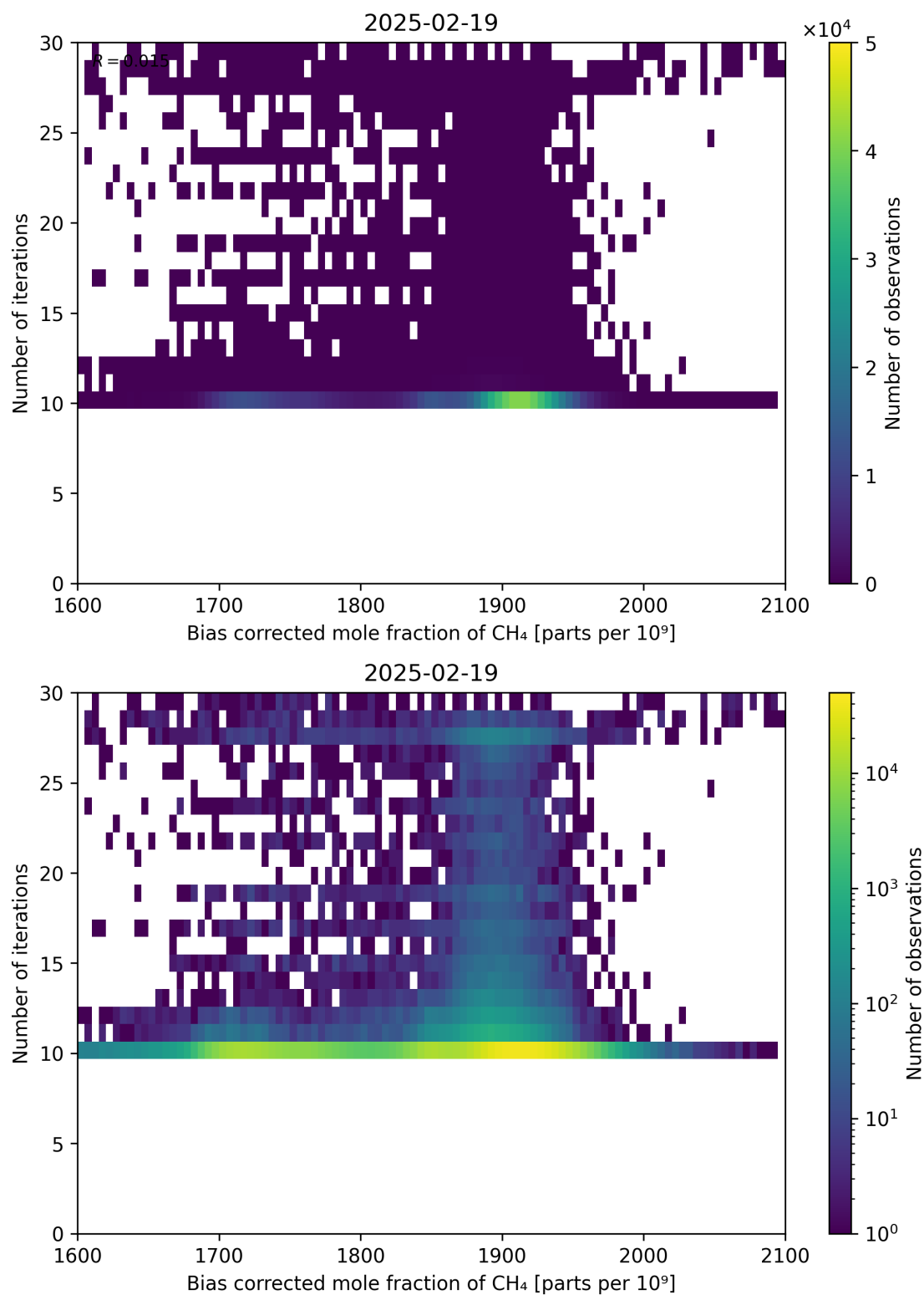
Figure 67: Scatter density plot of “Bias corrected mole fraction of \text{CH}_4 ” against “Number of iterations” for 2025-02-19 to 2025-02-20.
