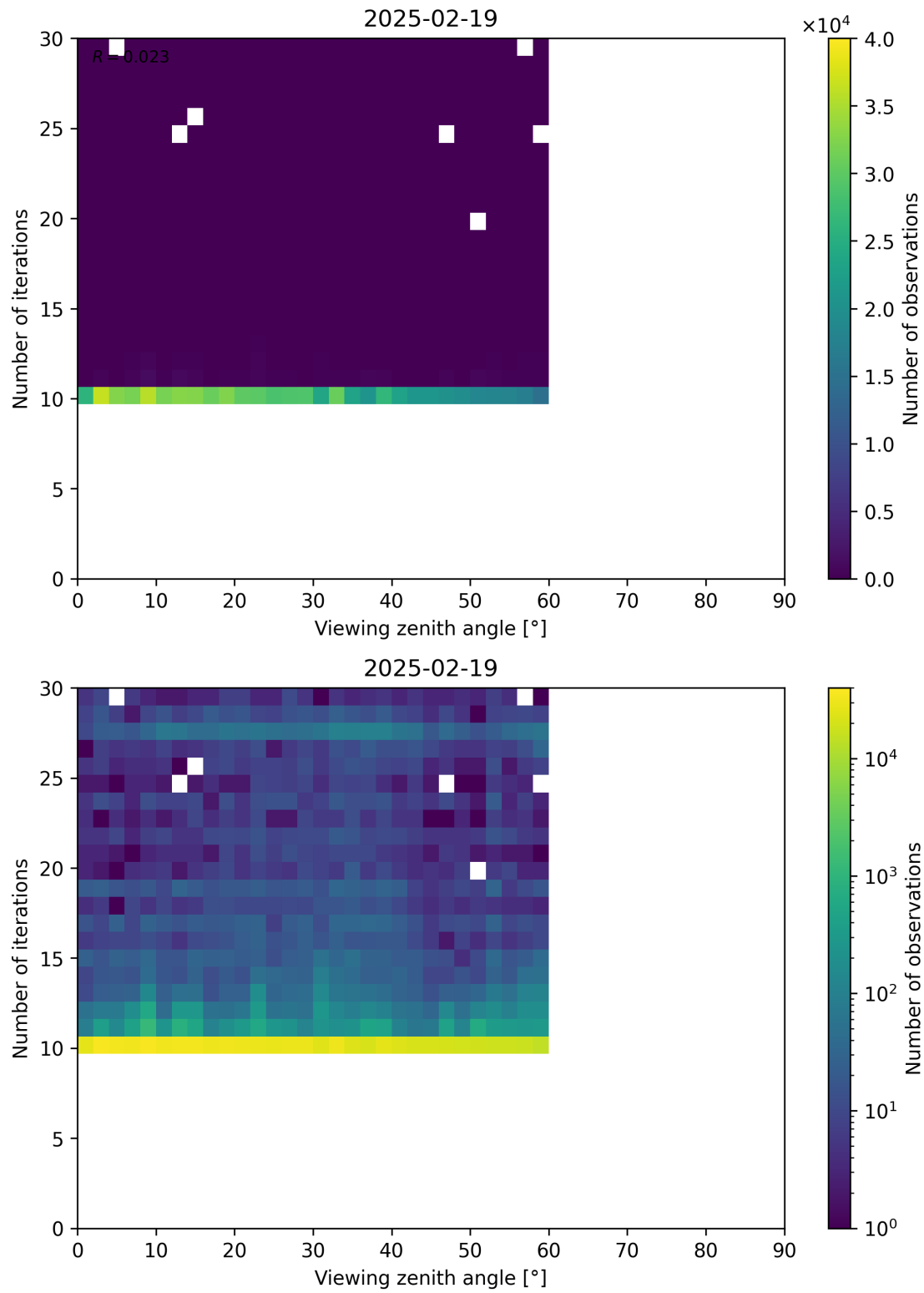
Figure 113: Scatter density plot of “Viewing zenith angle” against “Number of iterations” for 2025-02-19 to 2025-02-20.
