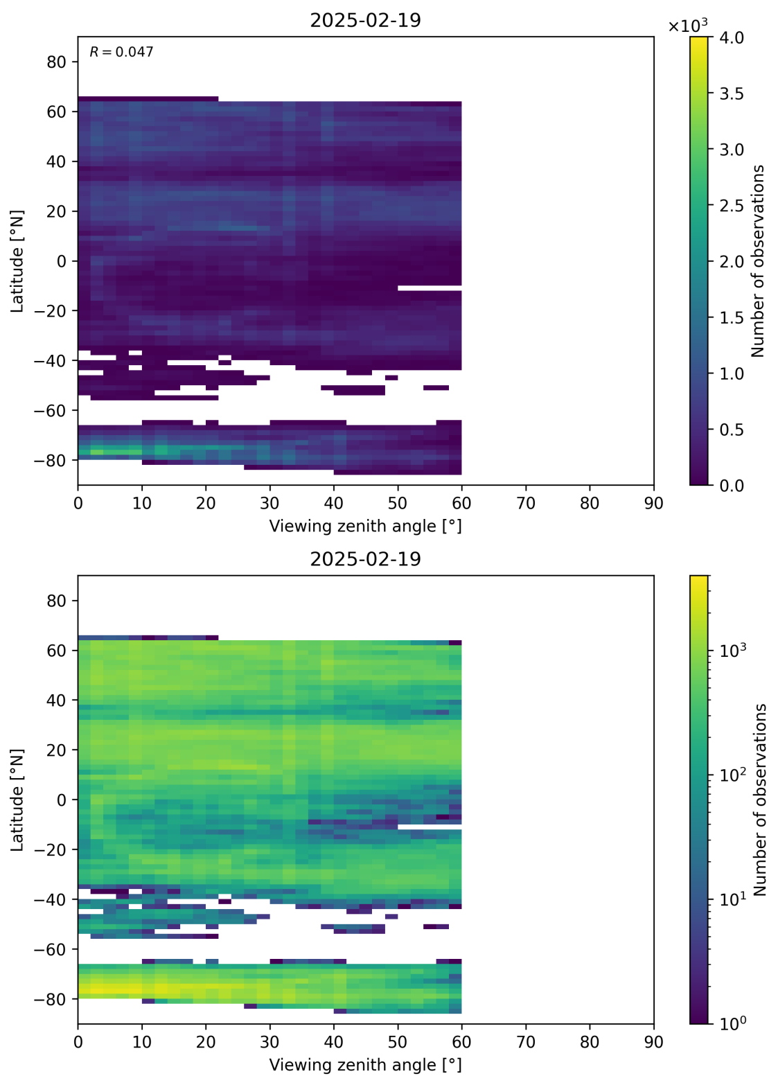
Figure 109: Scatter density plot of “Viewing zenith angle” against “Latitude” for 2025-02-19 to 2025-02-20.
