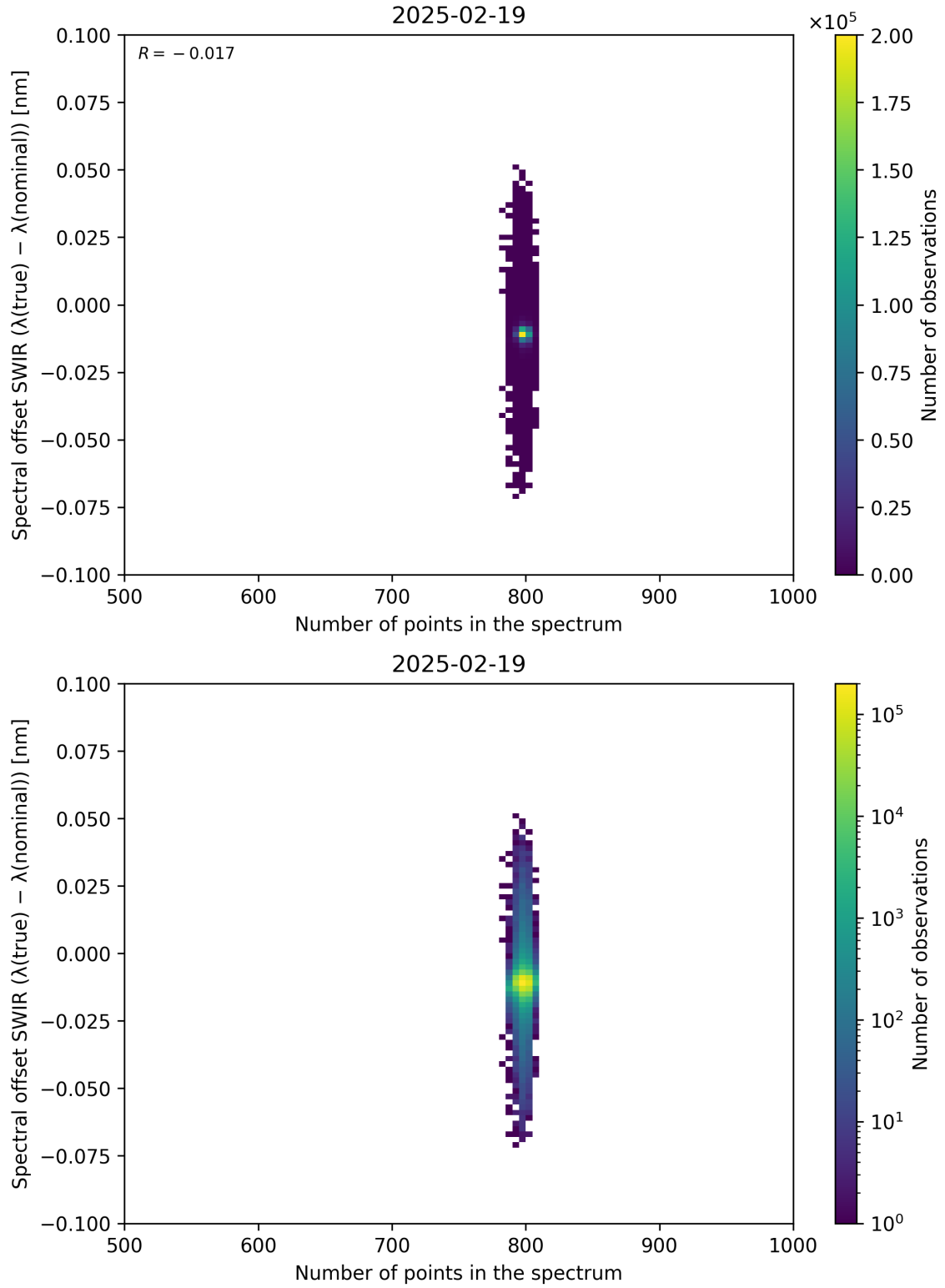
Figure 93: Scatter density plot of “Number of points in the spectrum” against “Spectral offset SWIR ( \lambda_{\text{true}} - \lambda_{\text{nominal}} )” for 2025-02-19 to 2025-02-20.
