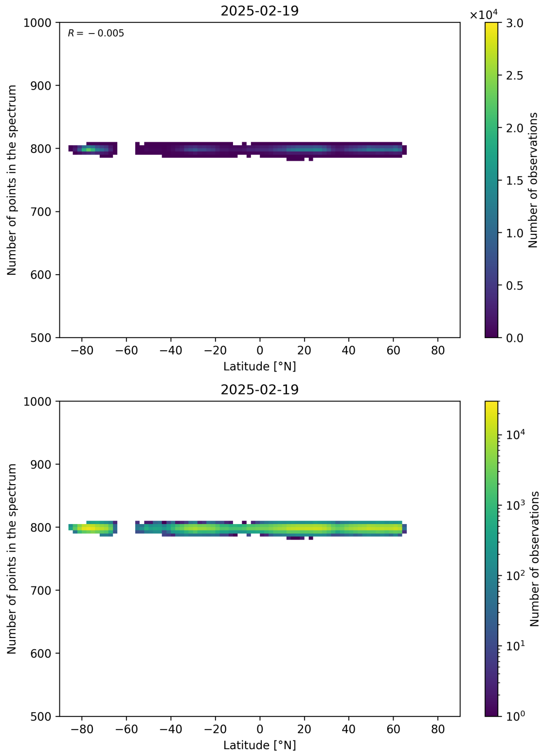
Figure 61: Scatter density plot of “Latitude” against “Number of points in the spectrum” for 2025-02-19 to 2025-02-20.
