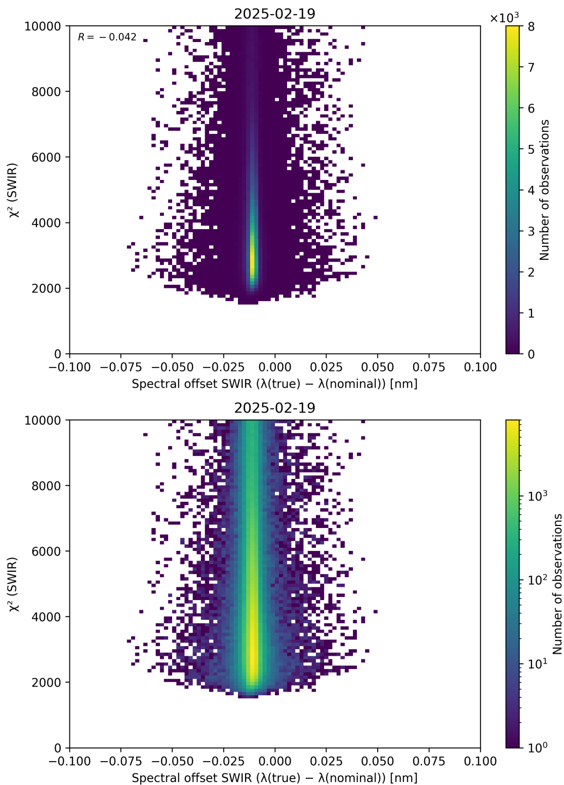
Figure 118: Scatter density plot of “Spectral offset SWIR ( \lambda_{\text{true}} - \lambda_{\text{nominal}} )” against “ \chi^2 (SWIR)” for 2025-02-19 to 2025-02-20.
