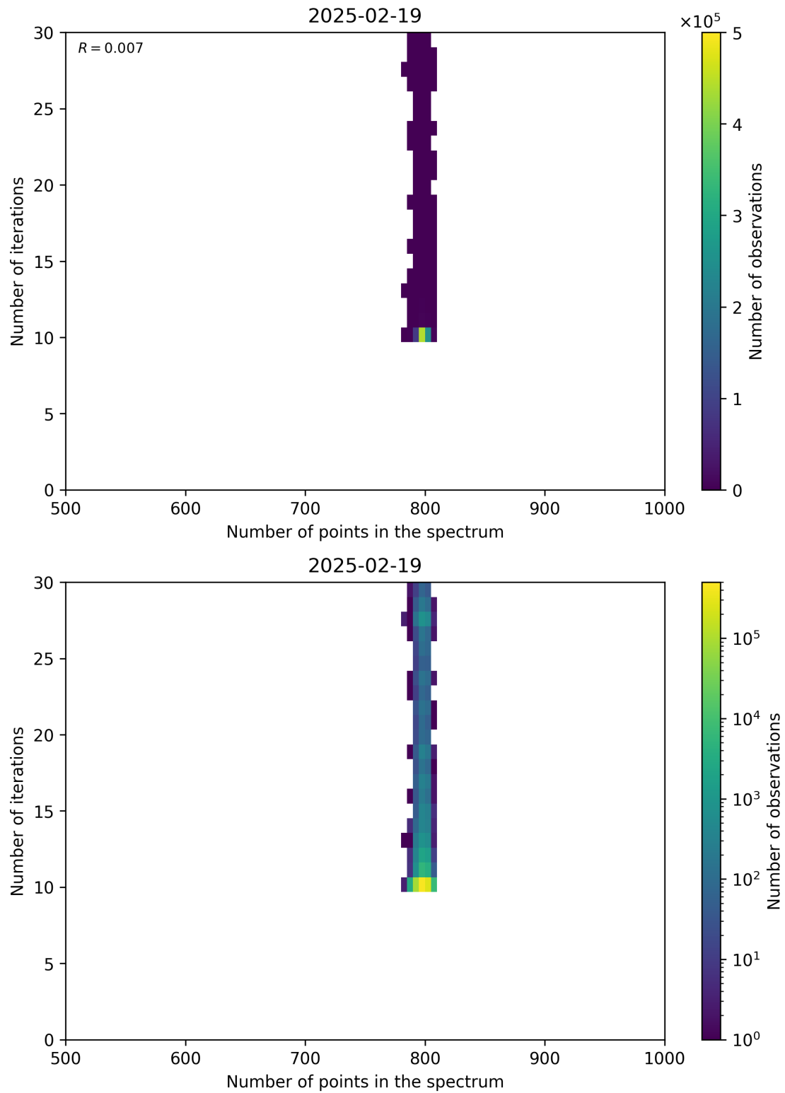
Figure 92: Scatter density plot of “Number of points in the spectrum” against “Number of iterations” for 2025-02-19 to 2025-02-20.
