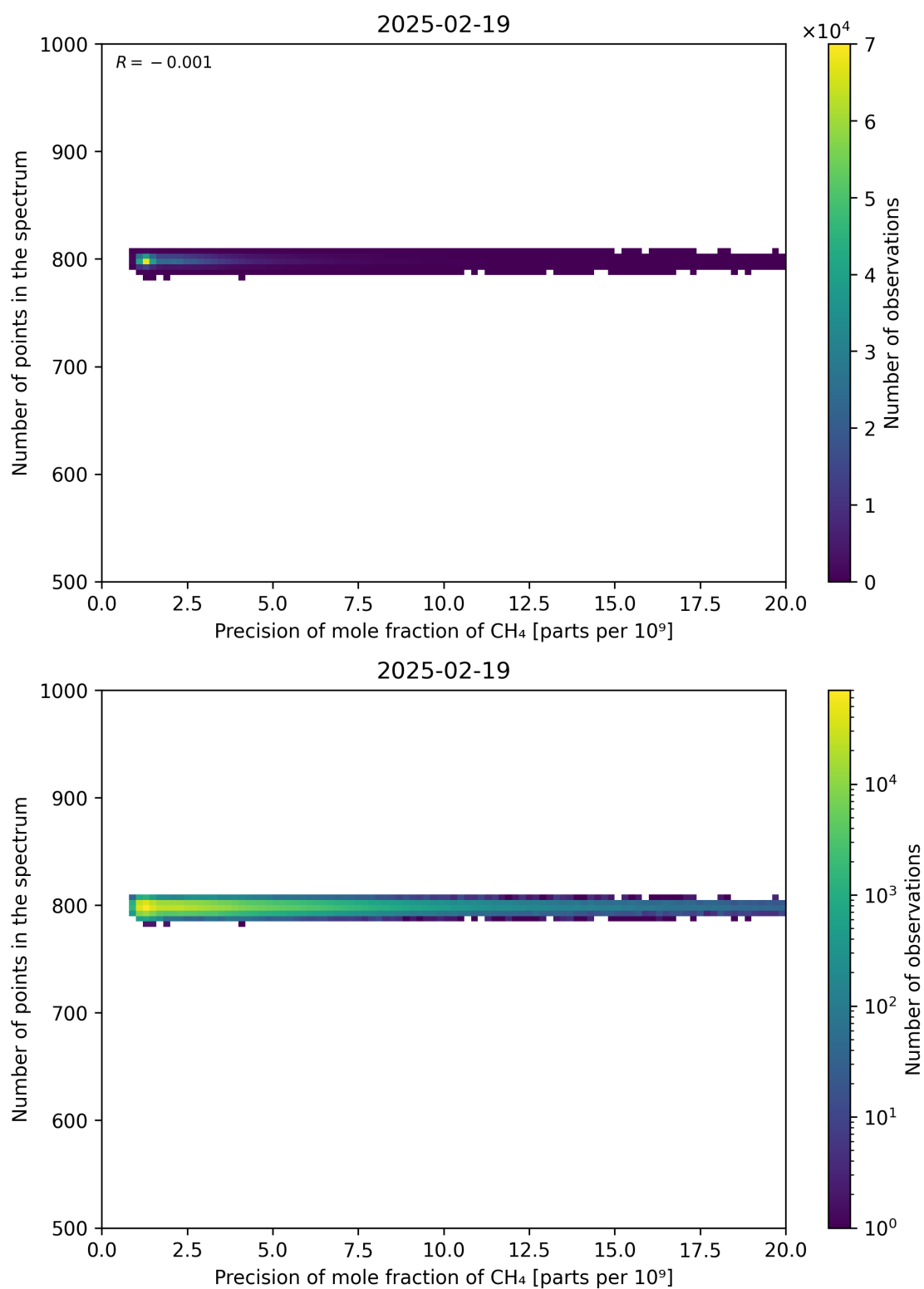
Figure 84: Scatter density plot of “Precision of mole fraction of CH 4 ” against “Number of points in the spectrum” for 2025-02-19 to 2025-02-20.
