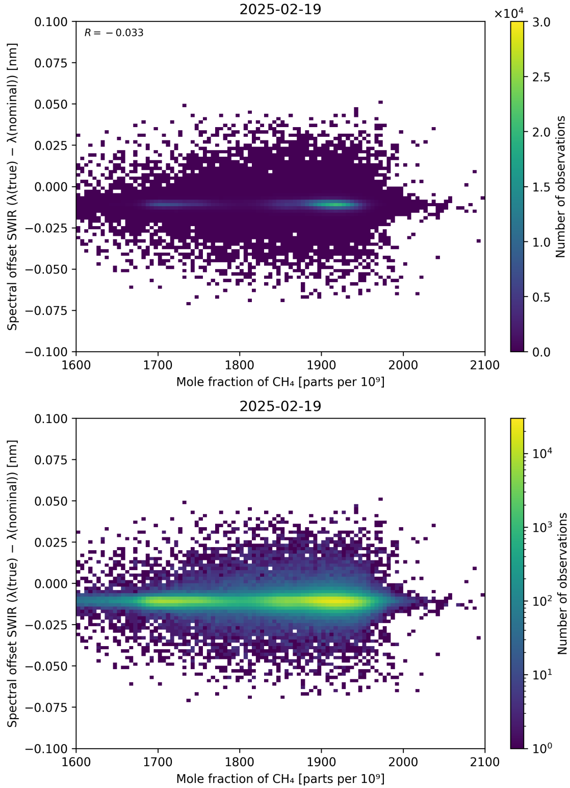
Figure 86: Scatter density plot of “Mole fraction of \text{CH}_4 ” against “Spectral offset SWIR ( \lambda_{\text{true}} - \lambda_{\text{nominal}} )” for 2025-02-19 to 2025-02-20.
