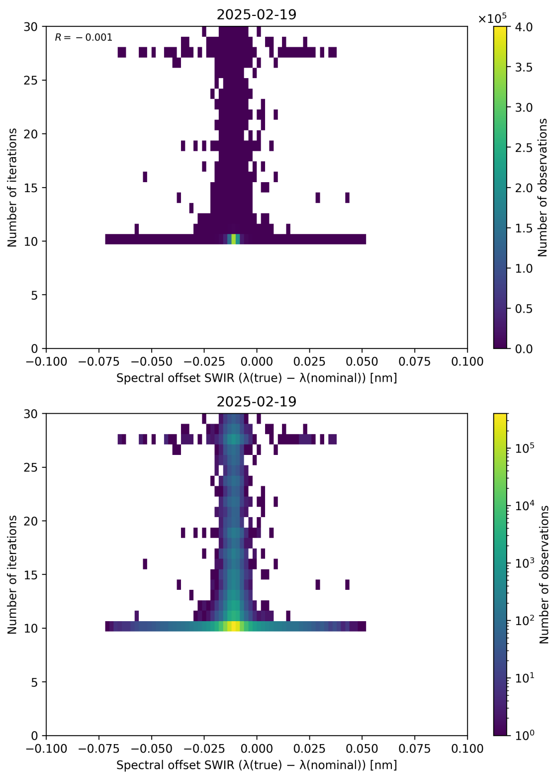
Figure 121: Scatter density plot of “Spectral offset SWIR ( \lambda_{\text{true}} - \lambda_{\text{nominal}} )” against “Number of iterations” for 2025-02-19 to 2025-02-20.
