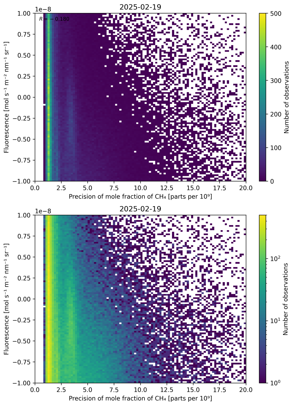
Figure 81: Scatter density plot of “Precision of mole fraction of CH 4 ” against “Fluorescence” for 2025-02-19 to 2025-02-20.
