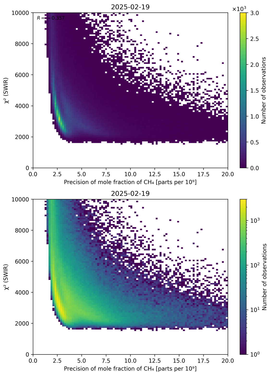
Figure 79: Scatter density plot of “Precision of mole fraction of \text{CH}_4 ” against “ \chi^2 (SWIR)” for 2025-02-19 to 2025-02-20.
