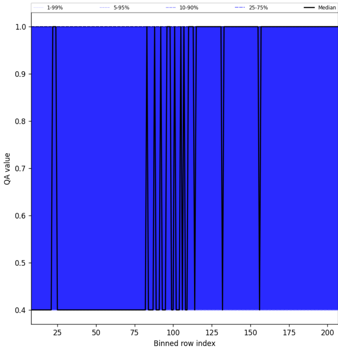
Figure 33: Along track statistics of “QA value” for 2025-02-19 to 2025-02-20
