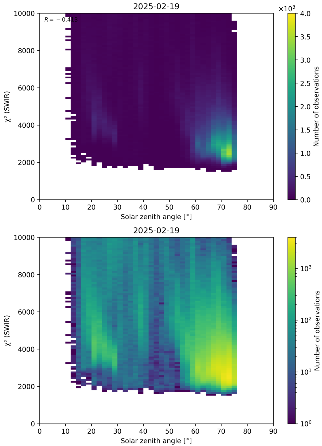
Figure 95: Scatter density plot of “Solar zenith angle” against “ \chi^2 (SWIR)” for 2025-02-19 to 2025-02-20.
