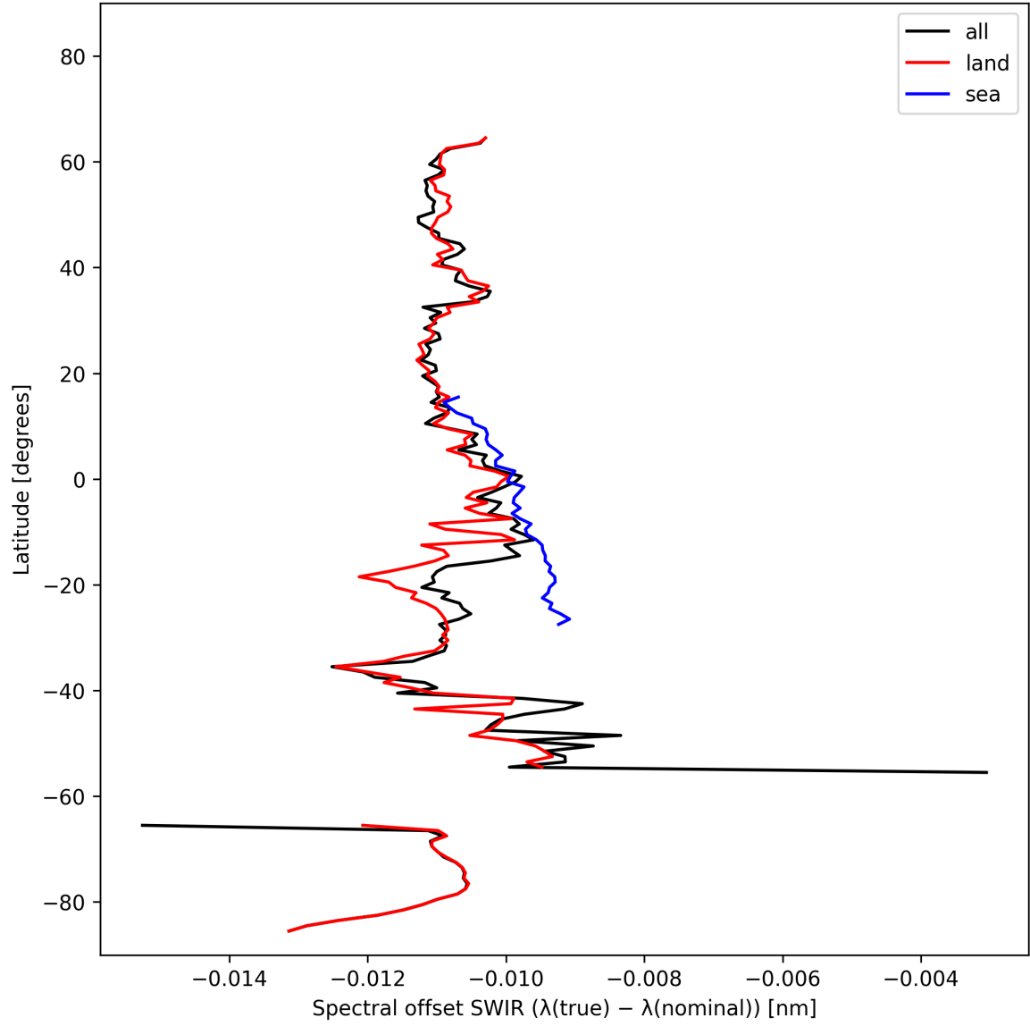
Figure 16: Zonal average of “Spectral offset SWIR ( \lambda_{\text{true}} - \lambda_{\text{nominal}} )” for 2025-02-19 to 2025-02-20.
