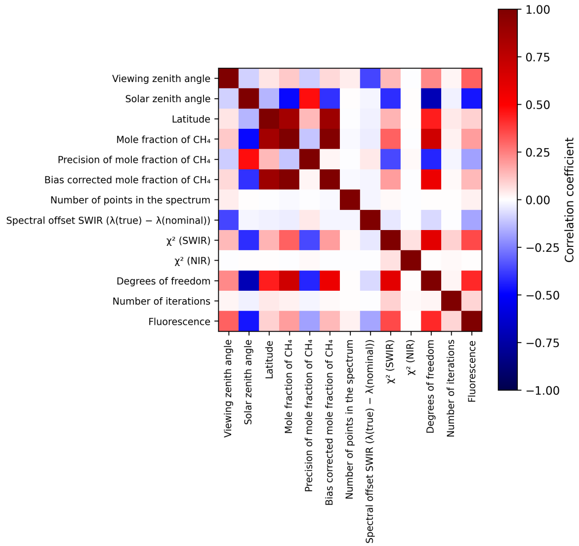
Figure 2: Map of correlation matrix for 2025-02-19 to 2025-02-20.
