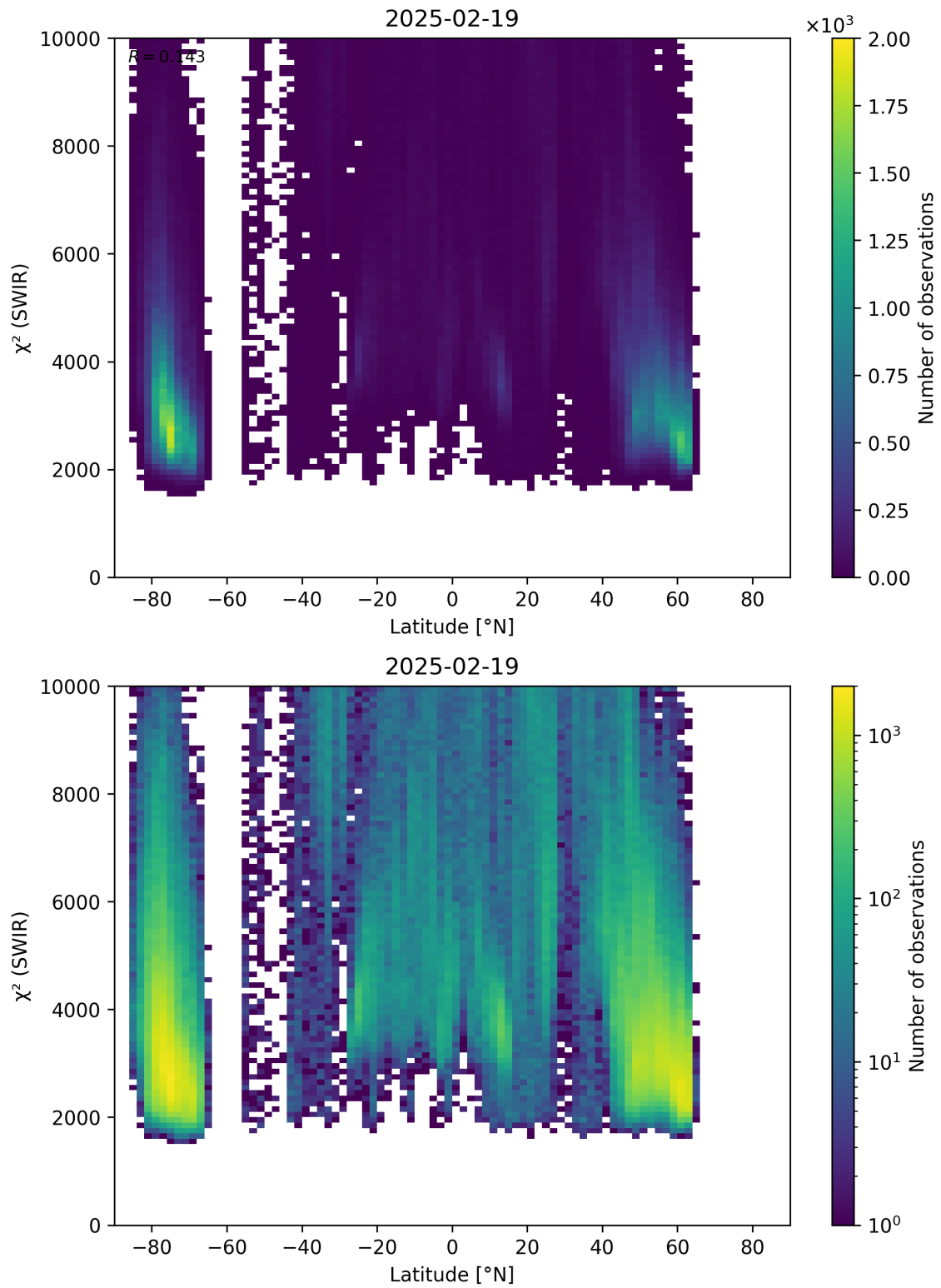
Figure 54: Scatter density plot of “Latitude” against “ \chi^2 (SWIR)” for 2025-02-19 to 2025-02-20.
