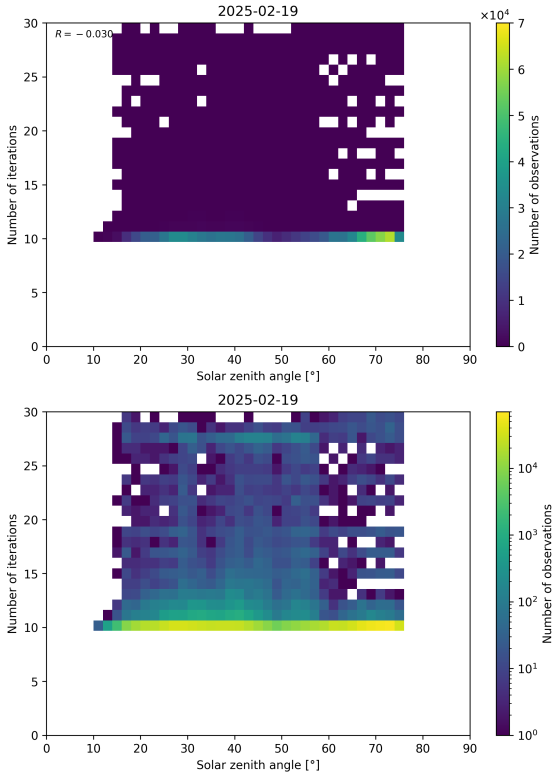
Figure 102: Scatter density plot of “Solar zenith angle” against “Number of iterations” for 2025-02-19 to 2025-02-20.
