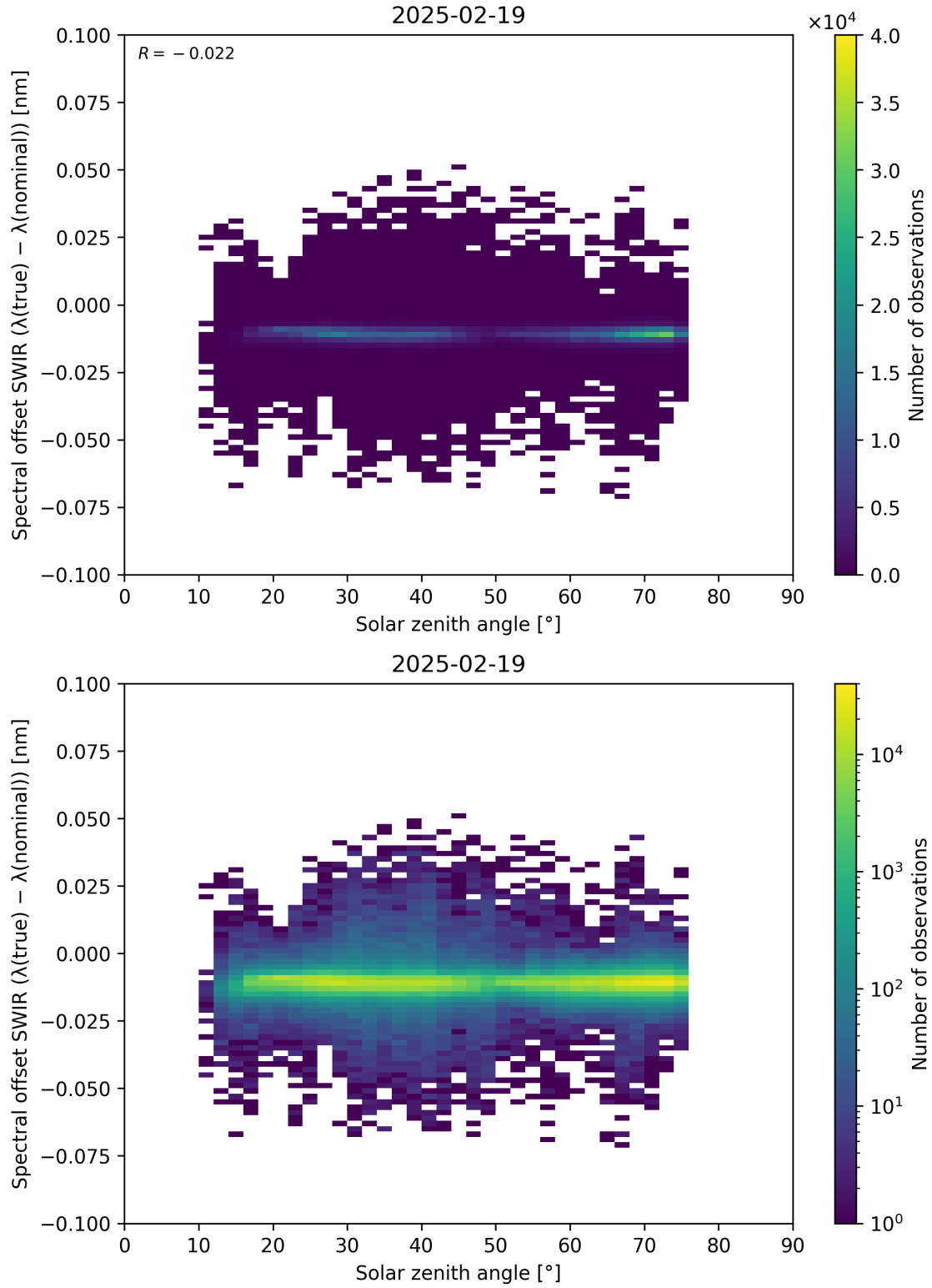
Figure 104: Scatter density plot of “Solar zenith angle” against “Spectral offset SWIR ( \lambda_{\text{true}} - \lambda_{\text{nominal}} )” for 2025-02-19 to 2025-02-20.
