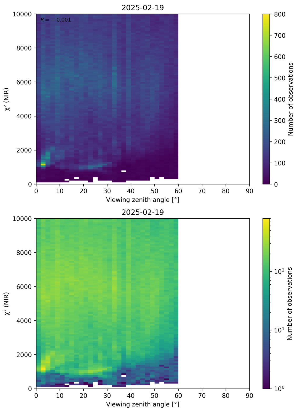
Figure 105: Scatter density plot of “Viewing zenith angle” against “ \chi^2 (NIR)” for 2025-02-19 to 2025-02-20.
