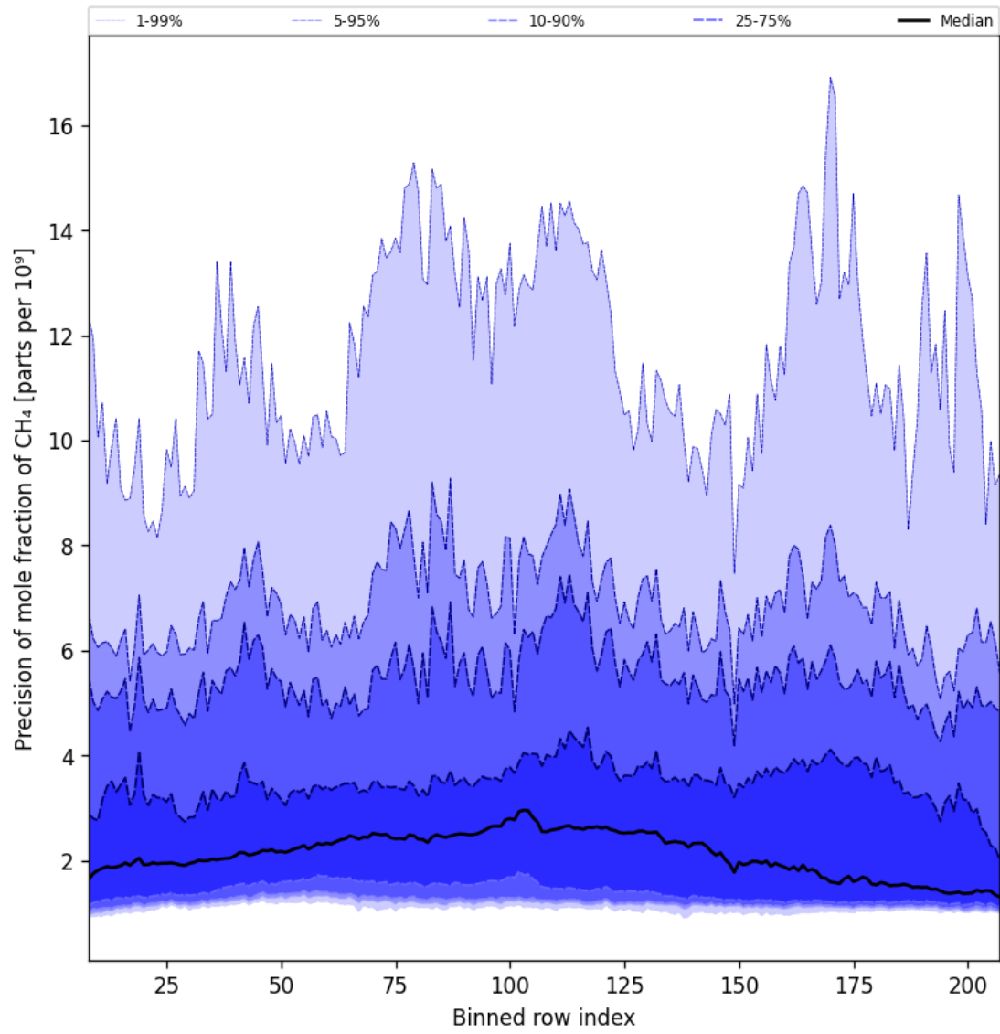
Figure 35: Along track statistics of “Precision of mole fraction of CH 4 ” for 2025-02-19 to 2025-02-20
