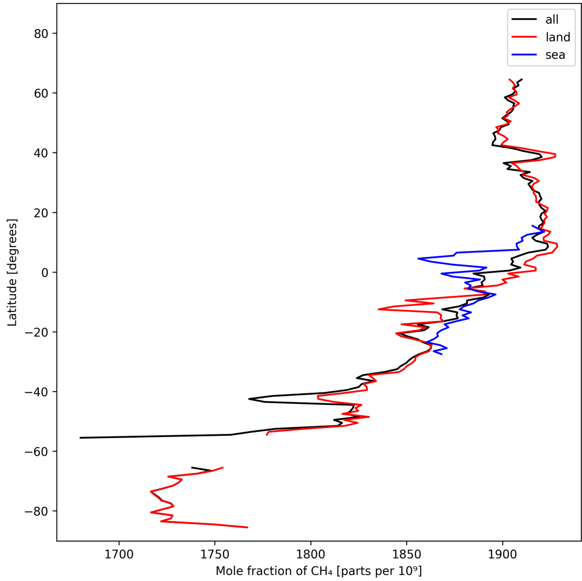
Figure 12: Zonal average of “Mole fraction of \text{CH}_4 ” for 2025-02-19 to 2025-02-20.
