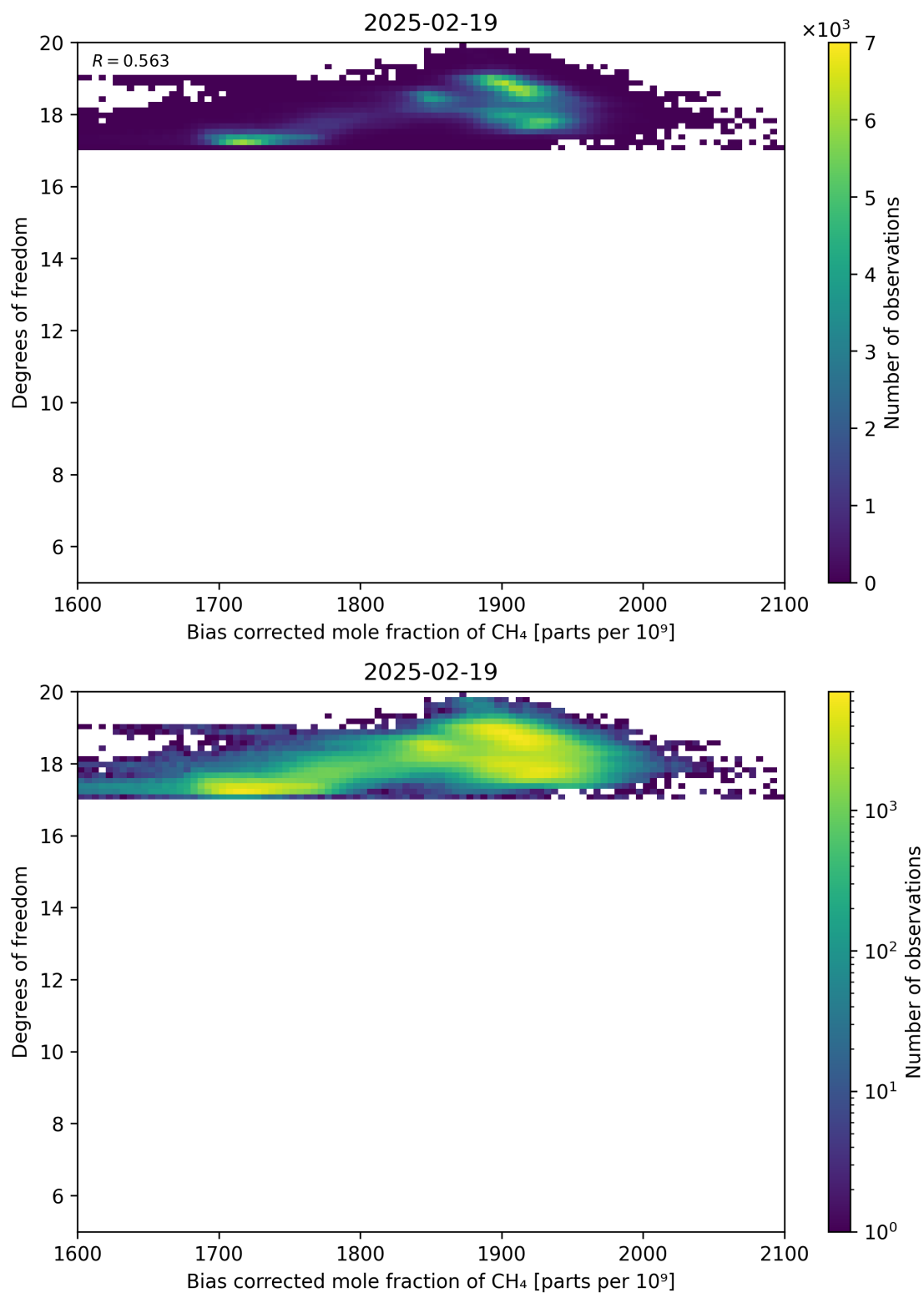
Figure 65: Scatter density plot of “Bias corrected mole fraction of CH 4 ” against “Degrees of freedom” for 2025-02-19 to 2025-02-20.
