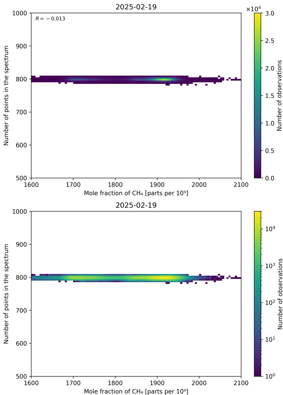
Figure 77: Scatter density plot of “Mole fraction of CH 4 ” against “Number of points in the spectrum” for 2025-02-19 to 2025-02-20.
