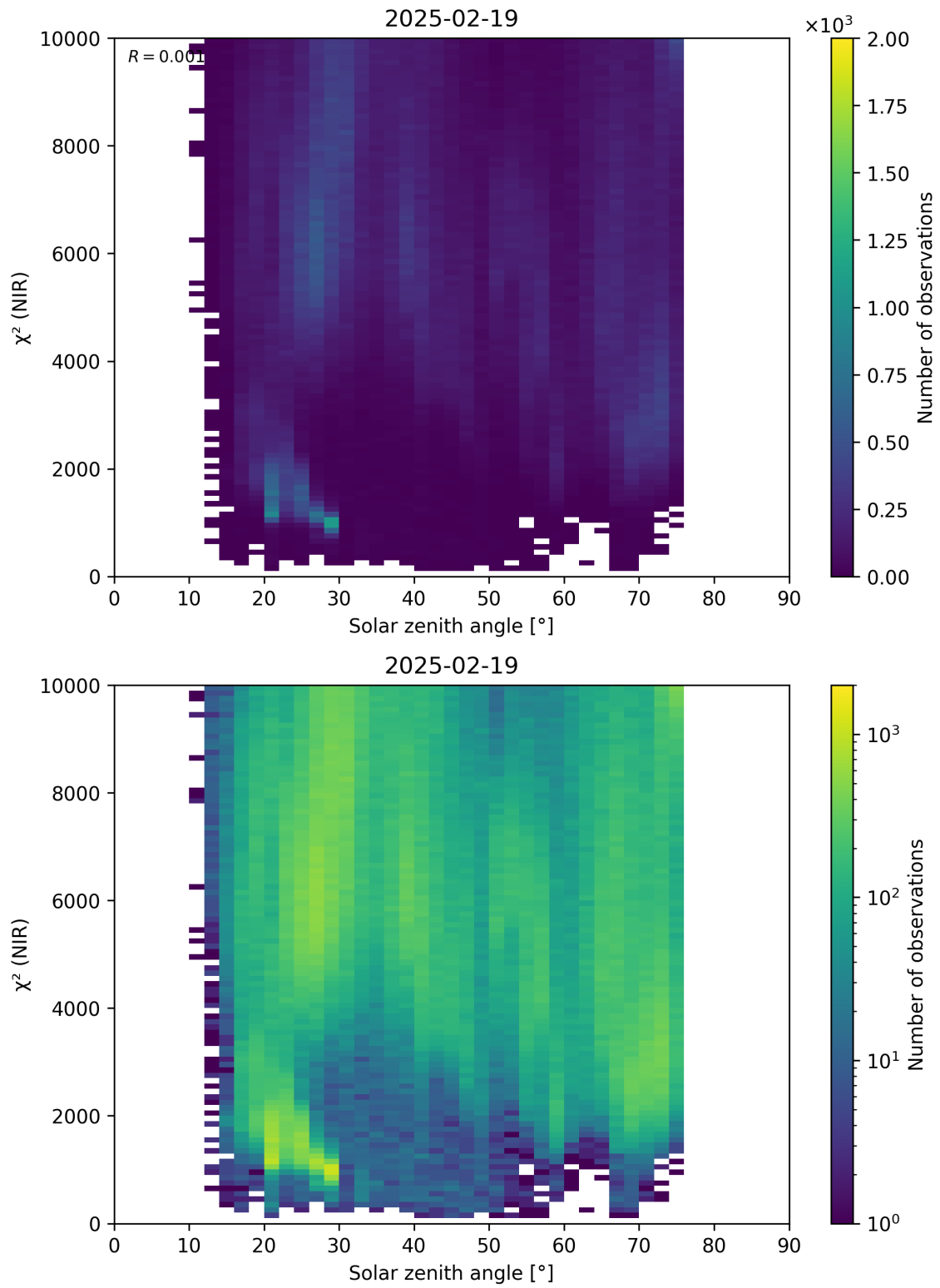
Figure 94: Scatter density plot of “Solar zenith angle” against “ \chi^2 (NIR)” for 2025-02-19 to 2025-02-20.
