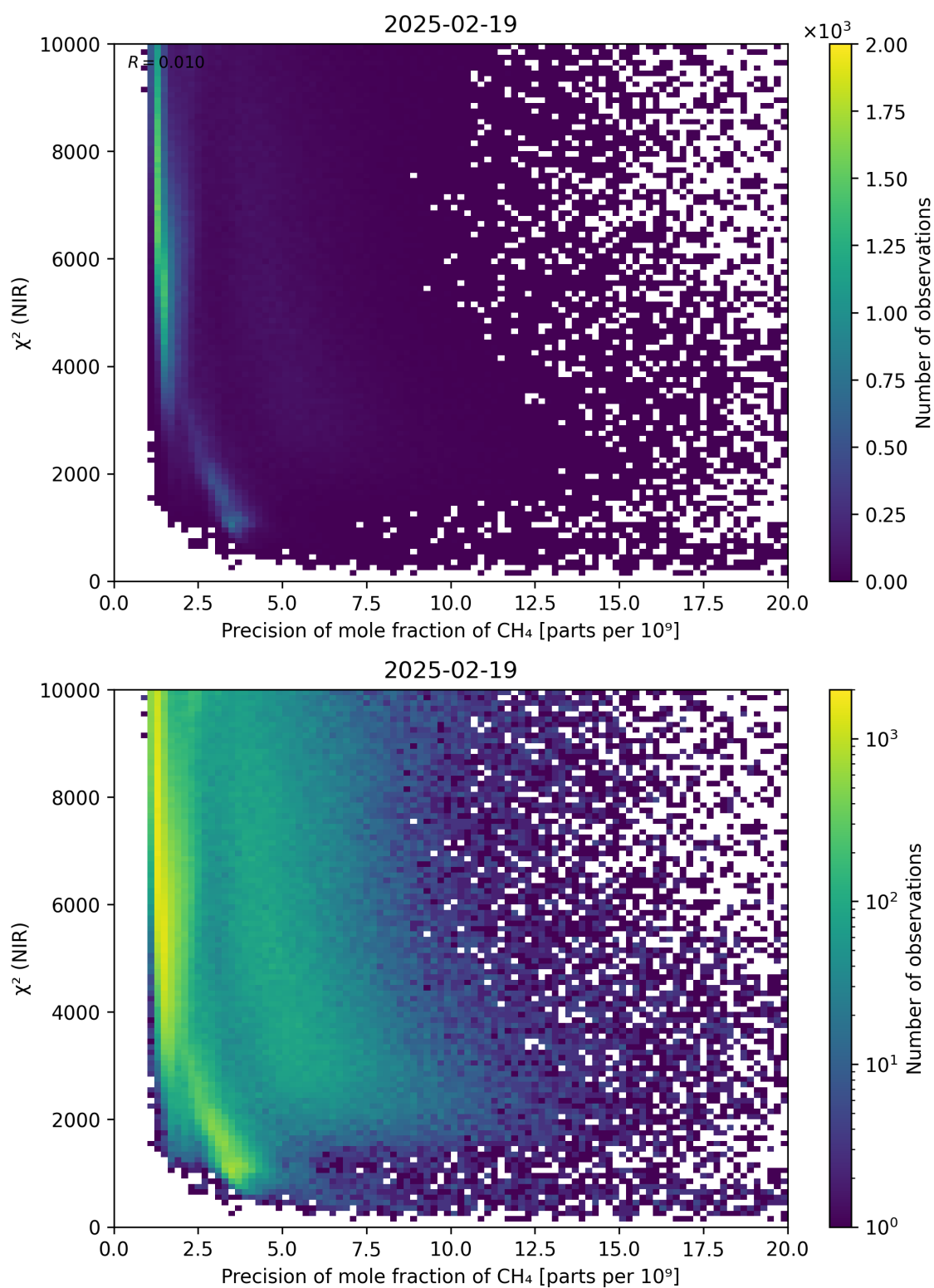
Figure 78: Scatter density plot of “Precision of mole fraction of \text{CH}_4 ” against “ \chi^2 (NIR)” for 2025-02-19 to 2025-02-20.
