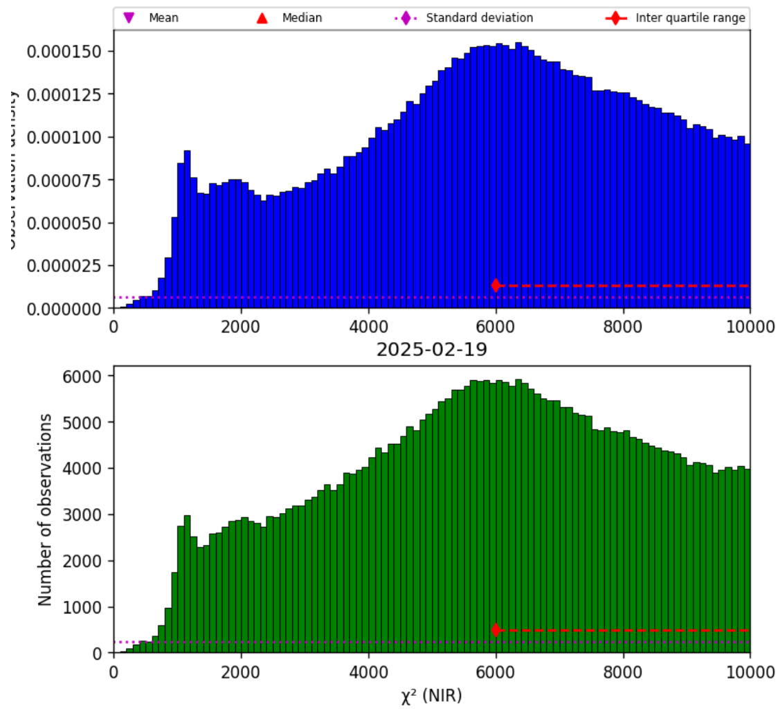
Figure 29: Histogram of “ \chi^2 (NIR)” for 2025-02-19 to 2025-02-20
