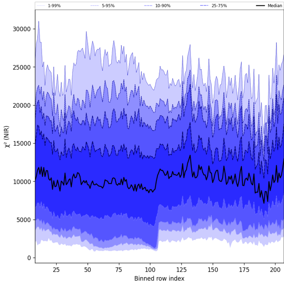
Figure 40: Along track statistics of “ \chi^2 (NIR)” for 2025-02-19 to 2025-02-20
