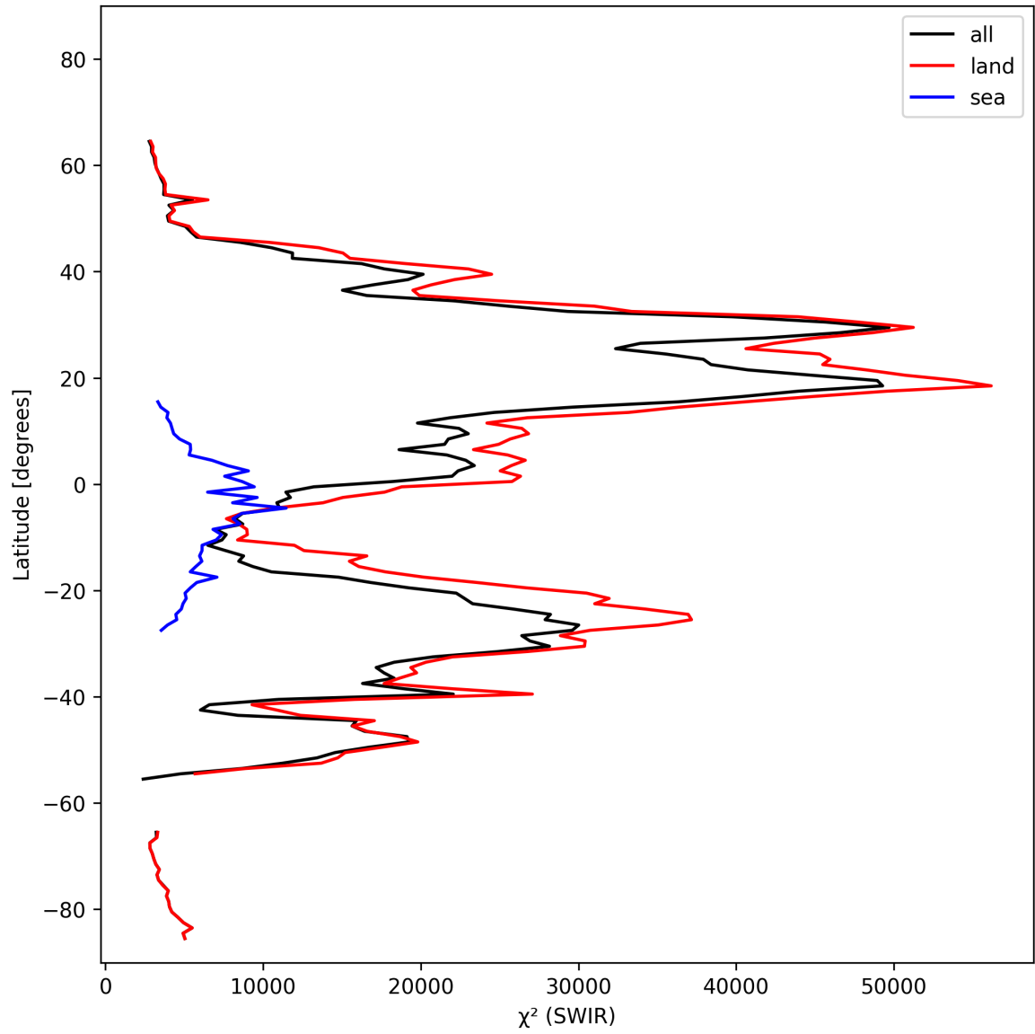
Figure 17: Zonal average of “ \chi^2 (SWIR)” for 2025-02-19 to 2025-02-20.
