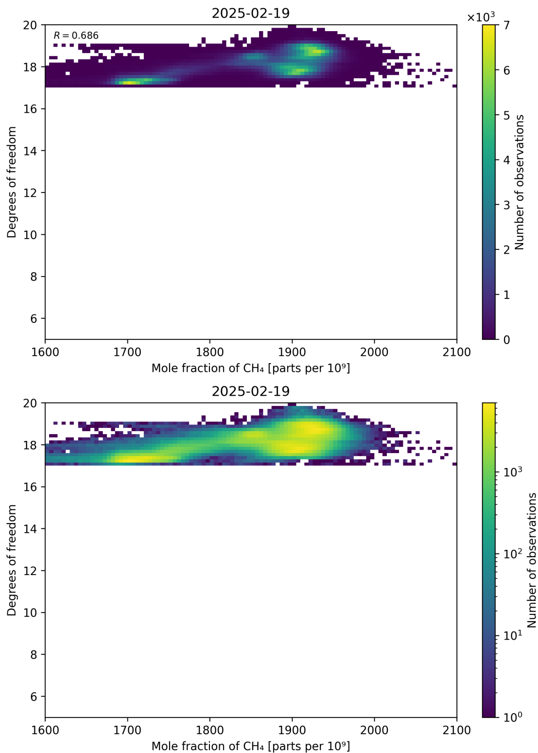
Figure 72: Scatter density plot of “Mole fraction of CH 4 ” against “Degrees of freedom” for 2025-02-19 to 2025-02-20.
