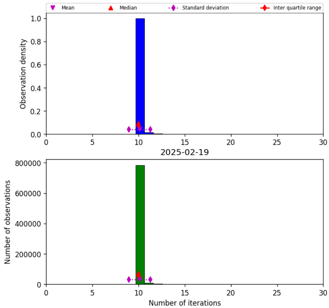
Figure 31: Histogram of “Number of iterations” for 2025-02-19 to 2025-02-20
