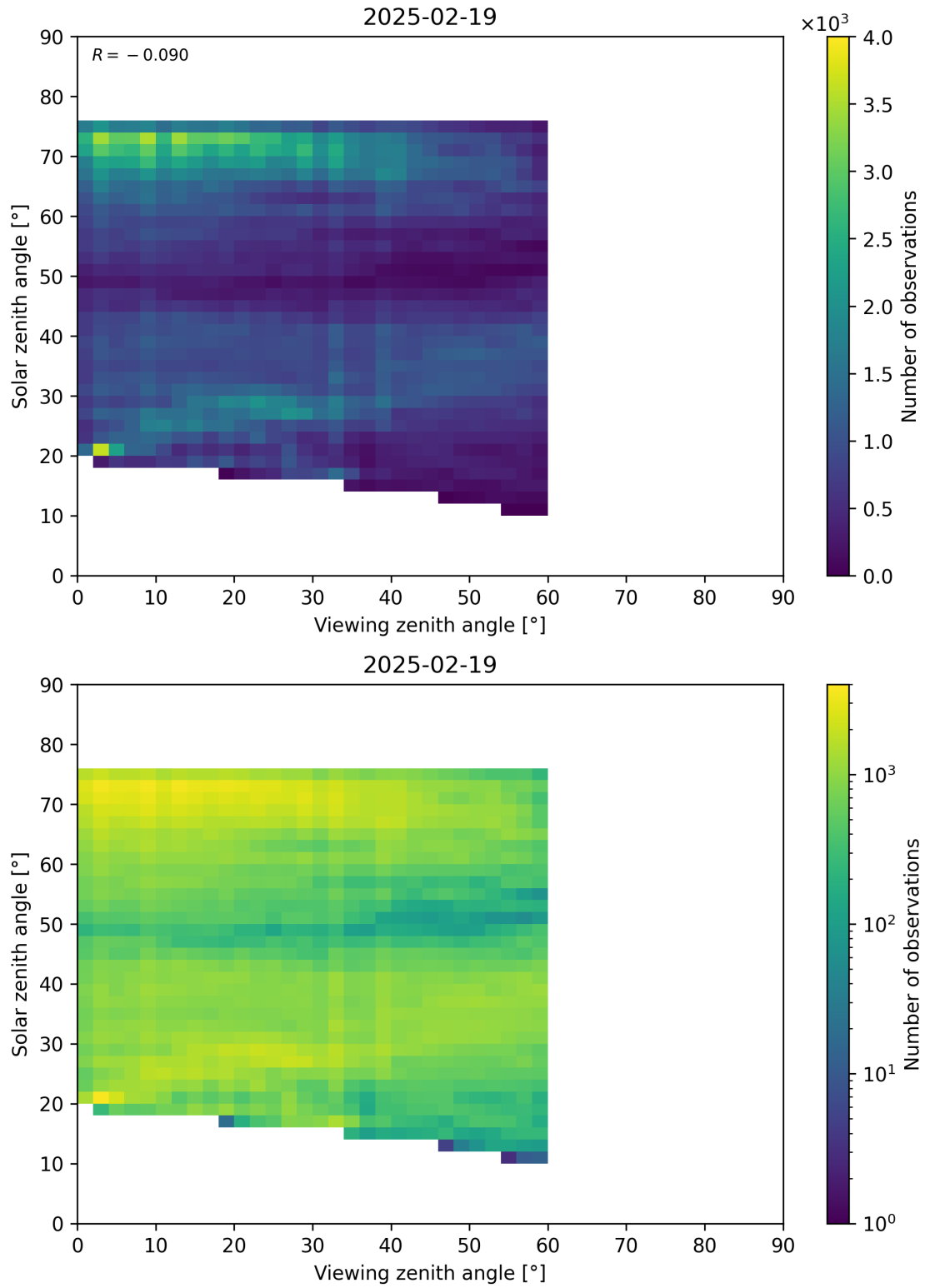
Figure 115: Scatter density plot of “Viewing zenith angle” against “Solar zenith angle” for 2025-02-19 to 2025-02-20.
