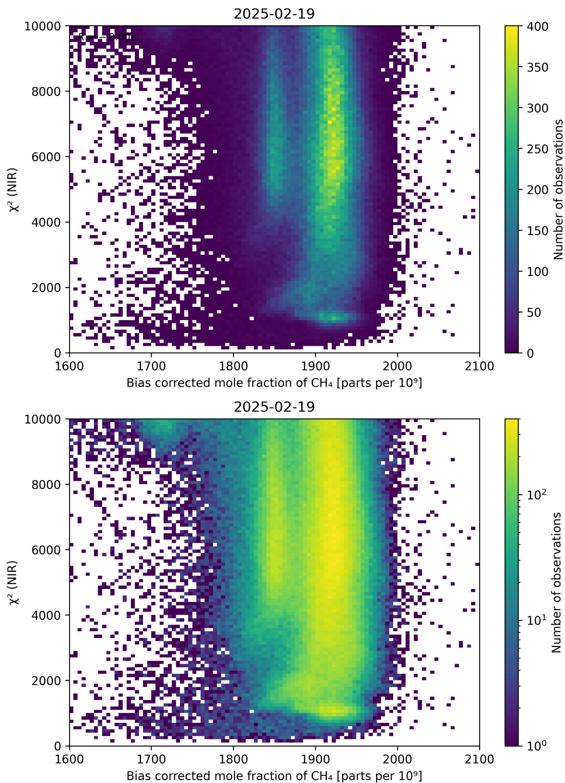
Figure 63: Scatter density plot of “Bias corrected mole fraction of CH 4 ” against “ \chi^2 (NIR)” for 2025-02-19 to 2025-02-20.
