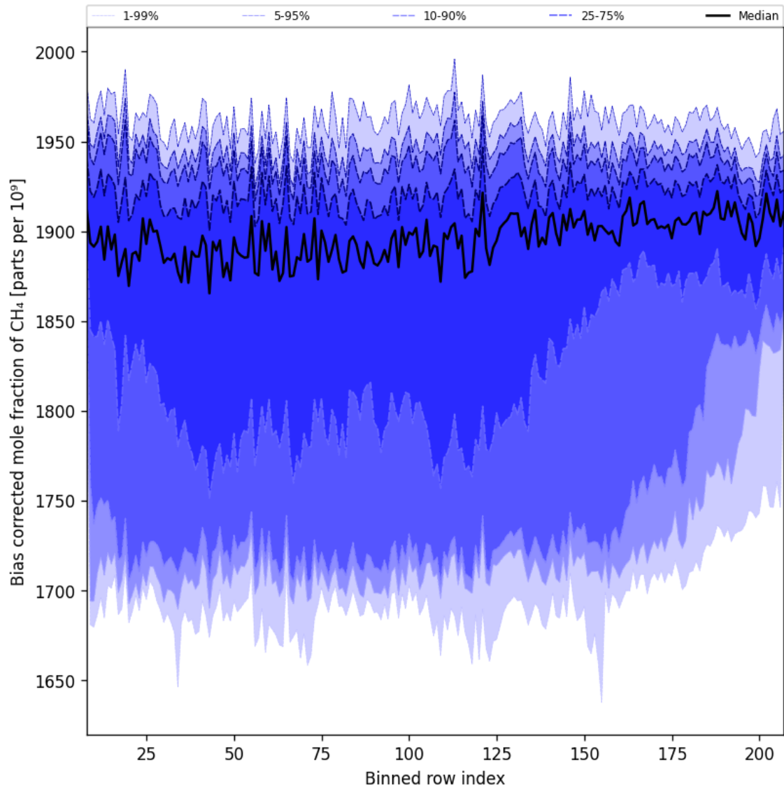
Figure 36: Along track statistics of “Bias corrected mole fraction of CH 4 ” for 2025-02-19 to 2025-02-20
