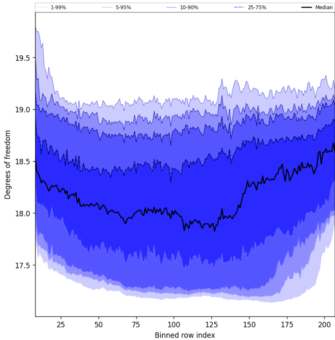
Figure 41: Along track statistics of “Degrees of freedom” for 2025-02-19 to 2025-02-20
