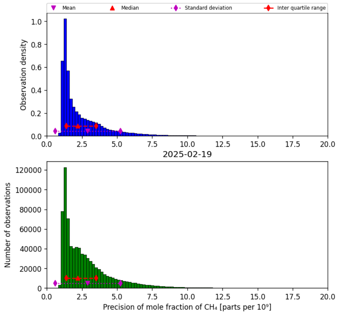
Figure 24: Histogram of “Precision of mole fraction of CH 4 ” for 2025-02-19 to 2025-02-20
