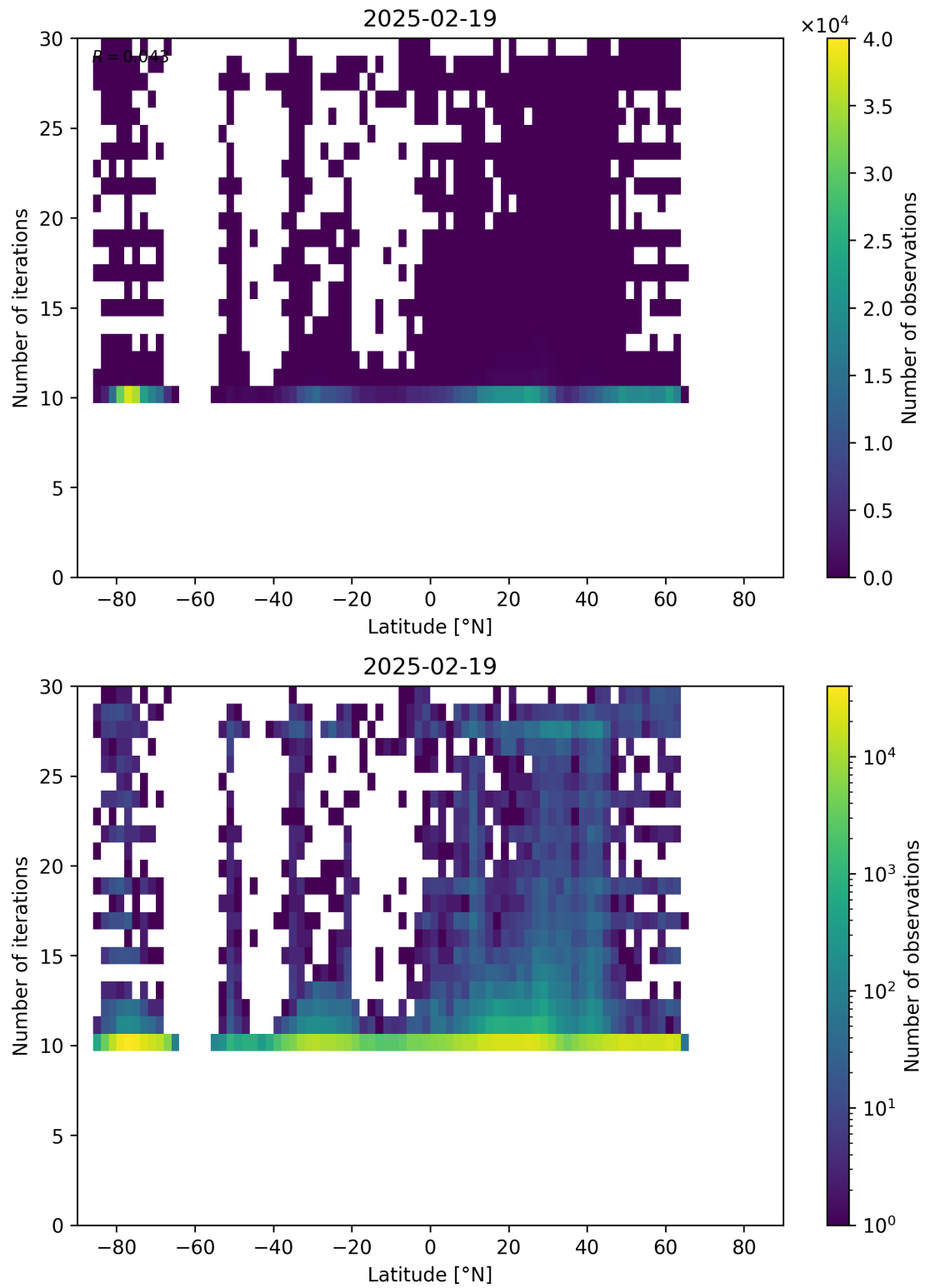
Figure 60: Scatter density plot of “Latitude” against “Number of iterations” for 2025-02-19 to 2025-02-20.
