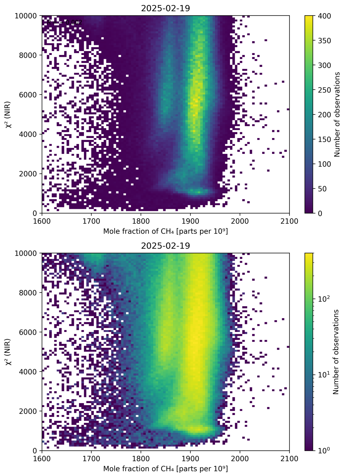
Figure 70: Scatter density plot of “Mole fraction of CH 4 ” against “ \chi^2 (NIR)” for 2025-02-19 to 2025-02-20.
