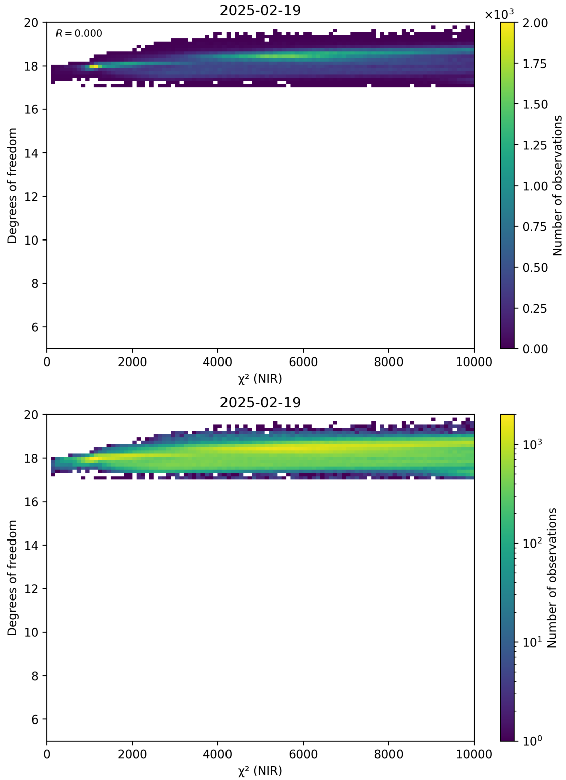
Figure 44: Scatter density plot of “ \chi^2 (NIR)” against “Degrees of freedom” for 2025-02-19 to 2025-02-20.
