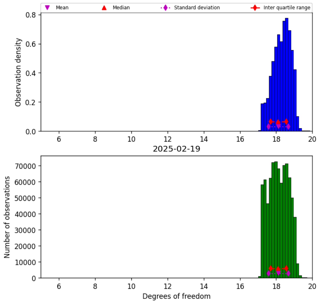
Figure 30: Histogram of “Degrees of freedom” for 2025-02-19 to 2025-02-20
