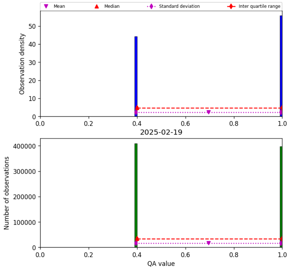
Figure 22: Histogram of “QA value” for 2025-02-19 to 2025-02-20
