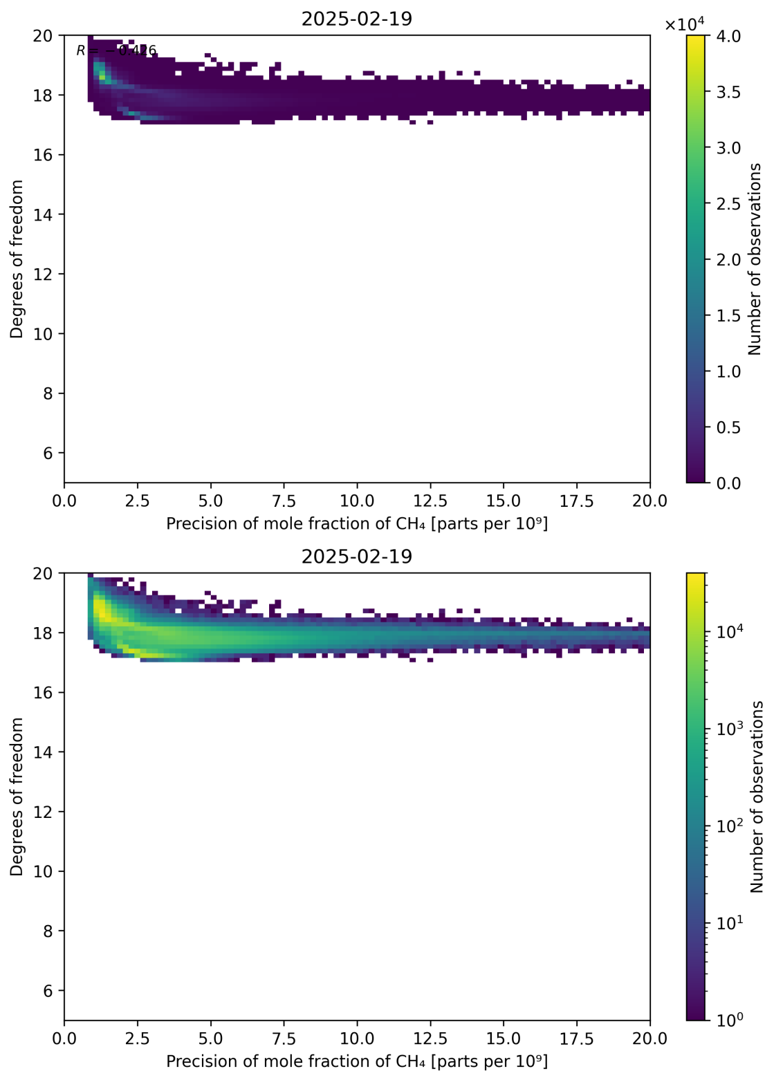
Figure 80: Scatter density plot of “Precision of mole fraction of CH 4 ” against “Degrees of freedom” for 2025-02-19 to 2025-02-20.
