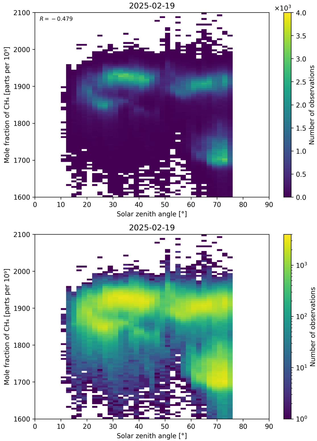
Figure 99: Scatter density plot of “Solar zenith angle” against “Mole fraction of CH 4 ” for 2025-02-19 to 2025-02-20.
