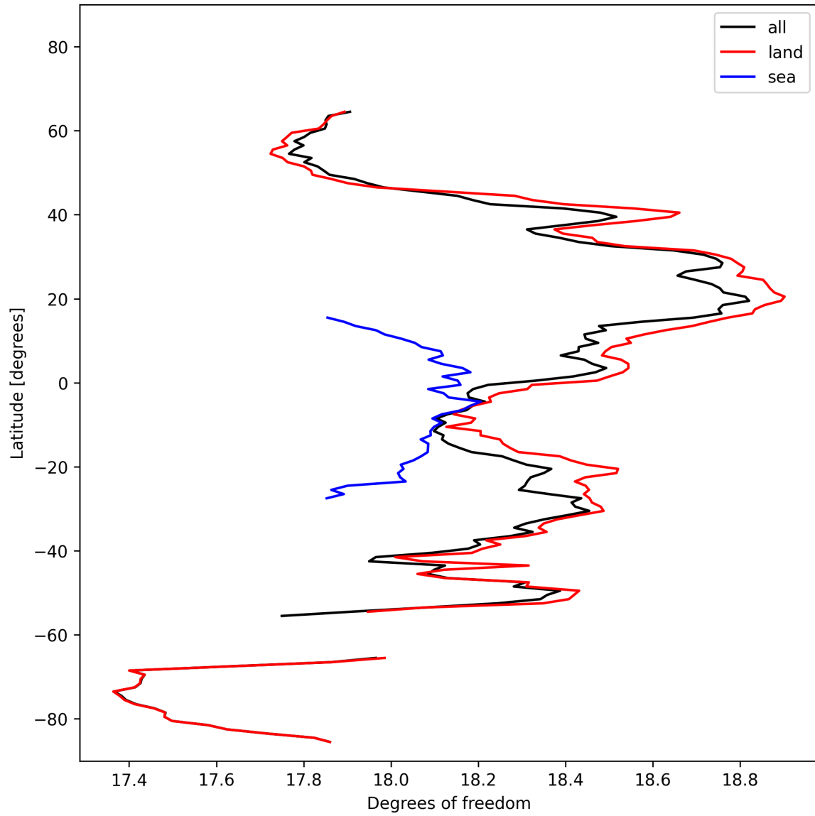
Figure 19: Zonal average of “Degrees of freedom” for 2025-02-19 to 2025-02-20.
