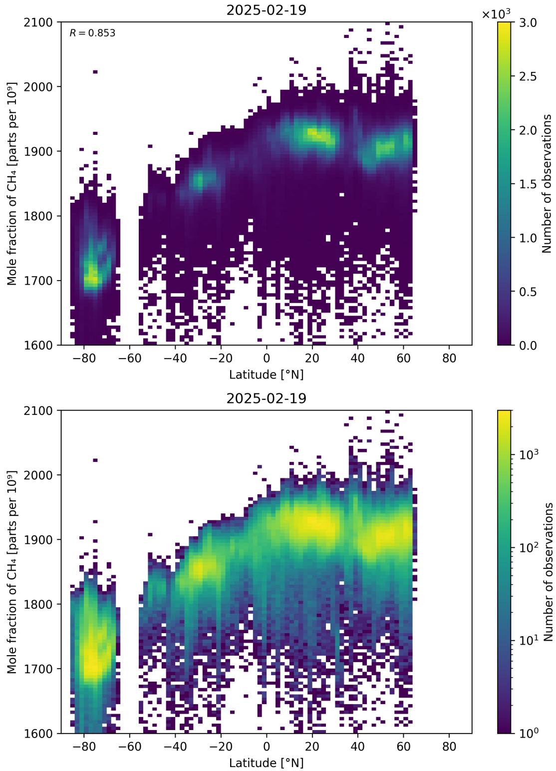
Figure 57: Scatter density plot of “Latitude” against “Mole fraction of CH 4 ” for 2025-02-19 to 2025-02-20.
