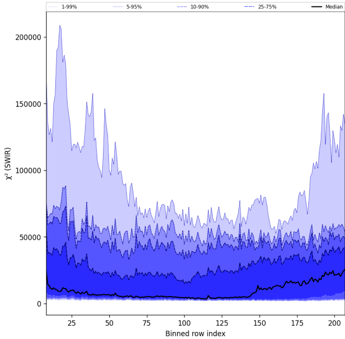
Figure 39: Along track statistics of “ \chi^2 (SWIR)” for 2025-02-19 to 2025-02-20
