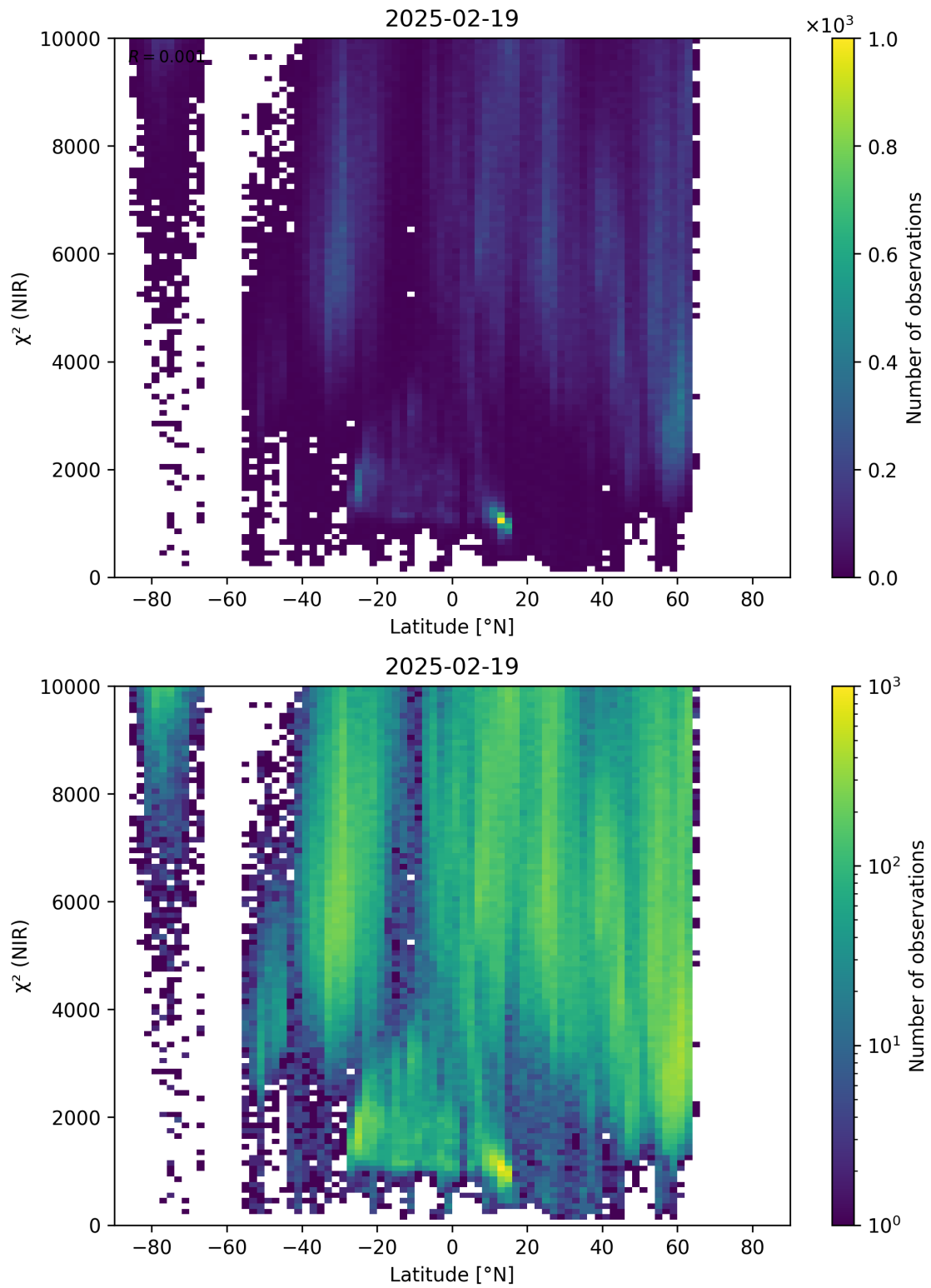
Figure 53: Scatter density plot of “Latitude” against “ \chi^2 (NIR)” for 2025-02-19 to 2025-02-20.
