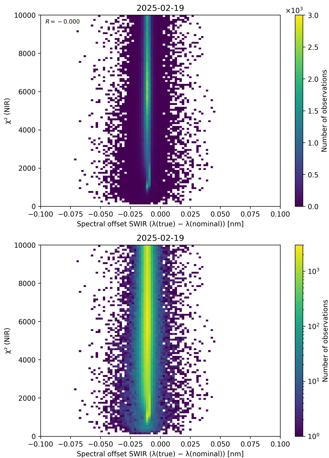
Figure 117: Scatter density plot of “Spectral offset SWIR ( \lambda_{\text{true}} - \lambda_{\text{nominal}} )” against “ \chi^2 (NIR)” for 2025-02-19 to 2025-02-20.
