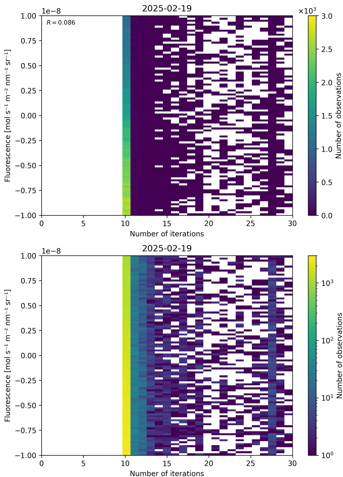
Figure 87: Scatter density plot of “Number of iterations” against “Fluorescence” for 2025-02-19 to 2025-02-20.
