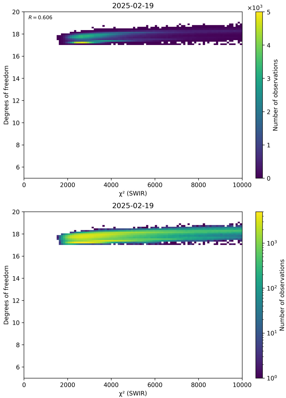
Figure 48: Scatter density plot of “ \chi^2 (SWIR)” against “Degrees of freedom” for 2025-02-19 to 2025-02-20.
