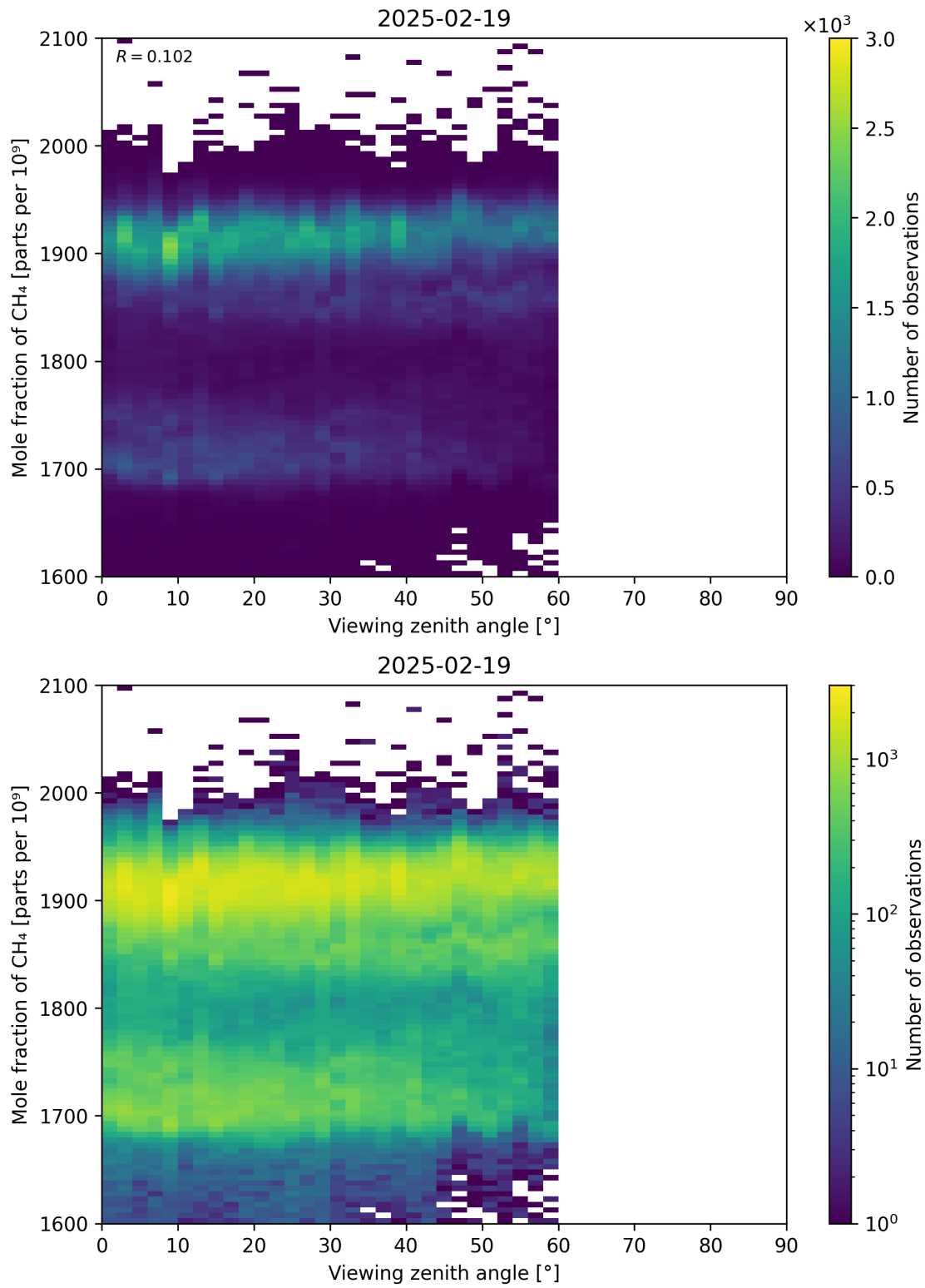
Figure 110: Scatter density plot of “Viewing zenith angle” against “Mole fraction of CH 4 ” for 2025-02-19 to 2025-02-20.
