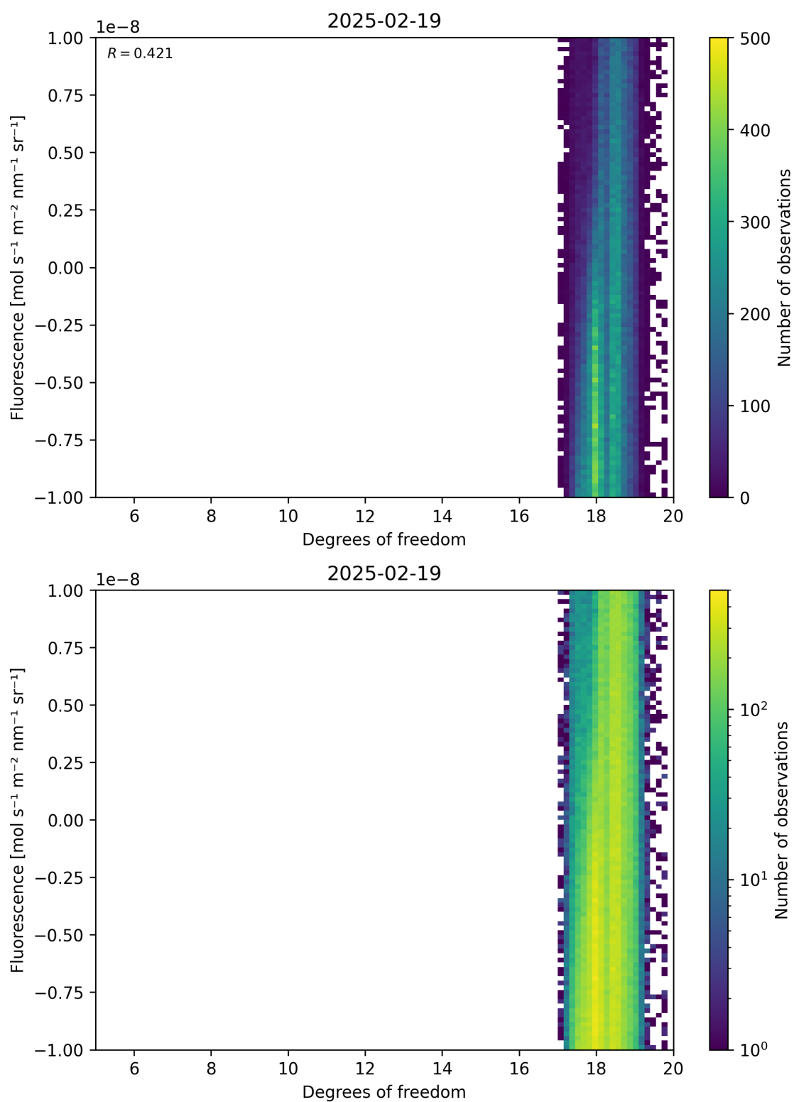
Figure 51: Scatter density plot of “Degrees of freedom” against “Fluorescence” for 2025-02-19 to 2025-02-20.
