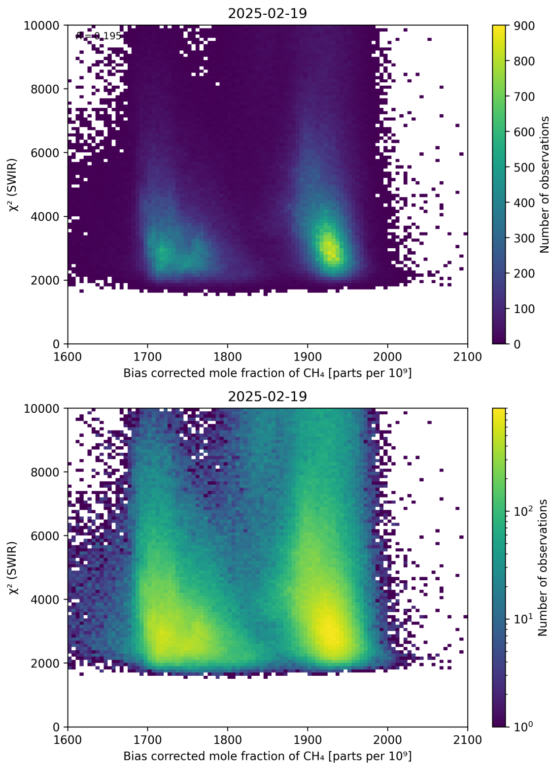
Figure 64: Scatter density plot of “Bias corrected mole fraction of CH 4 ” against “ \chi^2 (SWIR)” for 2025-02-19 to 2025-02-20.
