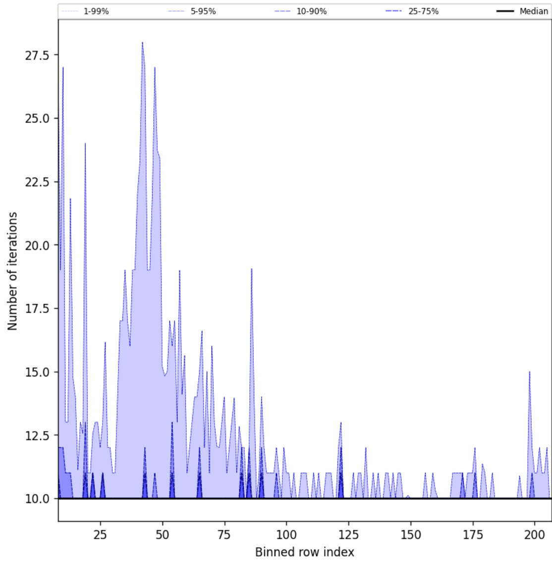
Figure 42: Along track statistics of “Number of iterations” for 2025-02-19 to 2025-02-20
