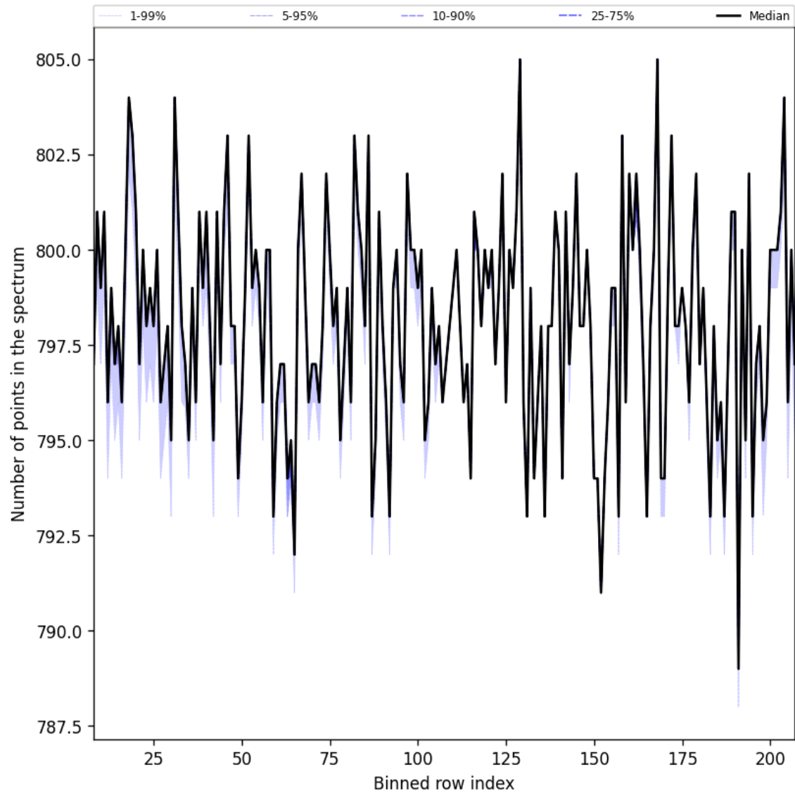
Figure 37: Along track statistics of “Number of points in the spectrum” for 2025-02-19 to 2025-02-20
