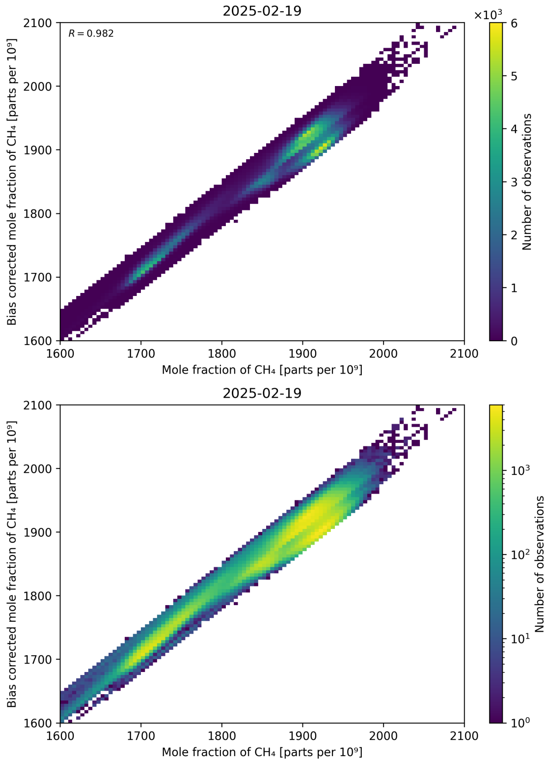
Figure 74: Scatter density plot of “Mole fraction of CH 4 ” against “Bias corrected mole fraction of CH 4 ” for 2025-02-19 to 2025-02-20.
