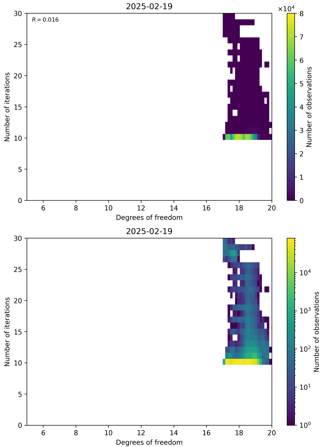
Figure 52: Scatter density plot of “Degrees of freedom” against “Number of iterations” for 2025-02-19 to 2025-02-20.
