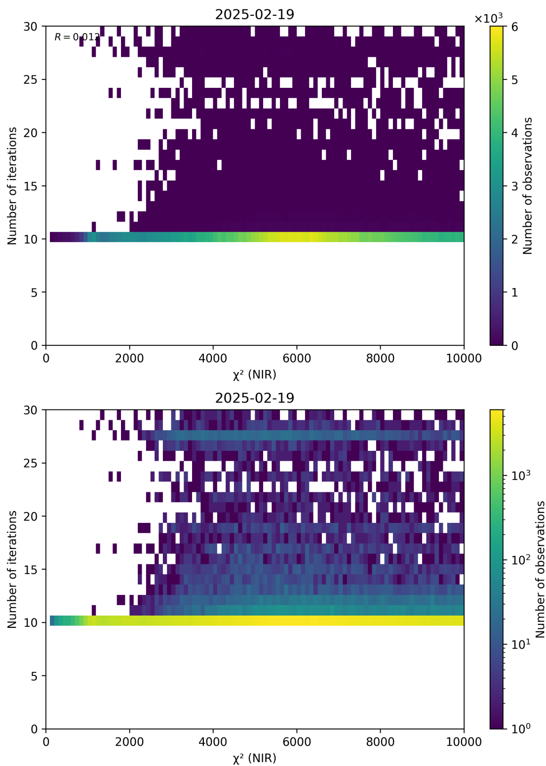
Figure 46: Scatter density plot of “ \chi^2 (NIR)” against “Number of iterations” for 2025-02-19 to 2025-02-20.
