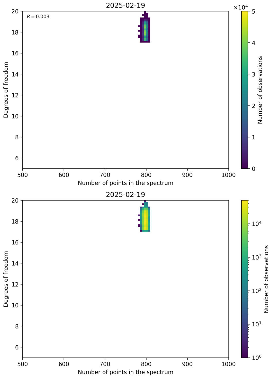
Figure 90: Scatter density plot of “Number of points in the spectrum” against “Degrees of freedom” for 2025-02-19 to 2025-02-20.
