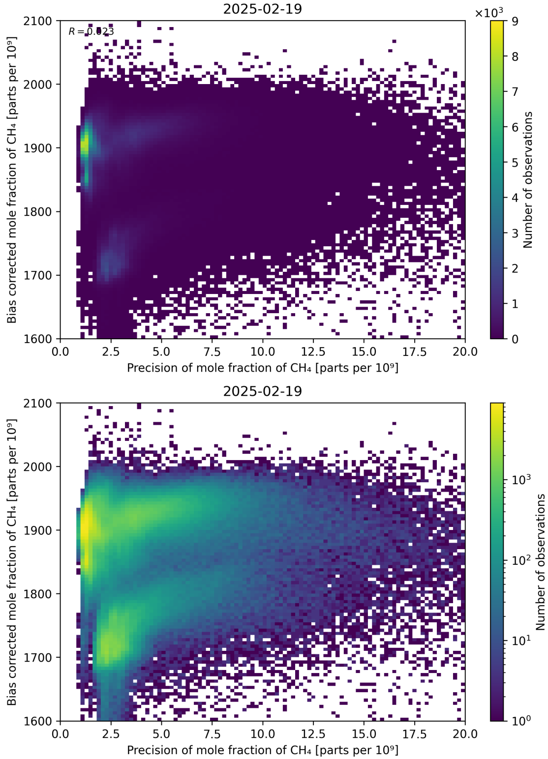
Figure 82: Scatter density plot of “Precision of mole fraction of CH 4 ” against “Bias corrected mole fraction of CH 4 ” for 2025-02-19 to 2025-02-20.
