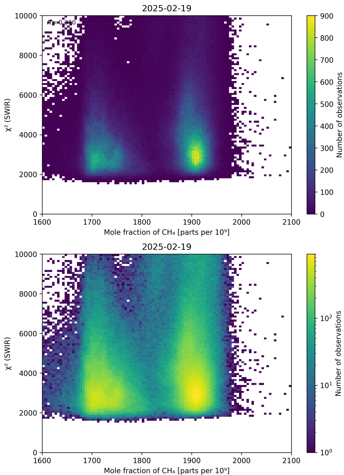
Figure 71: Scatter density plot of “Mole fraction of CH 4 ” against “ \chi^2 (SWIR)” for 2025-02-19 to 2025-02-20.
