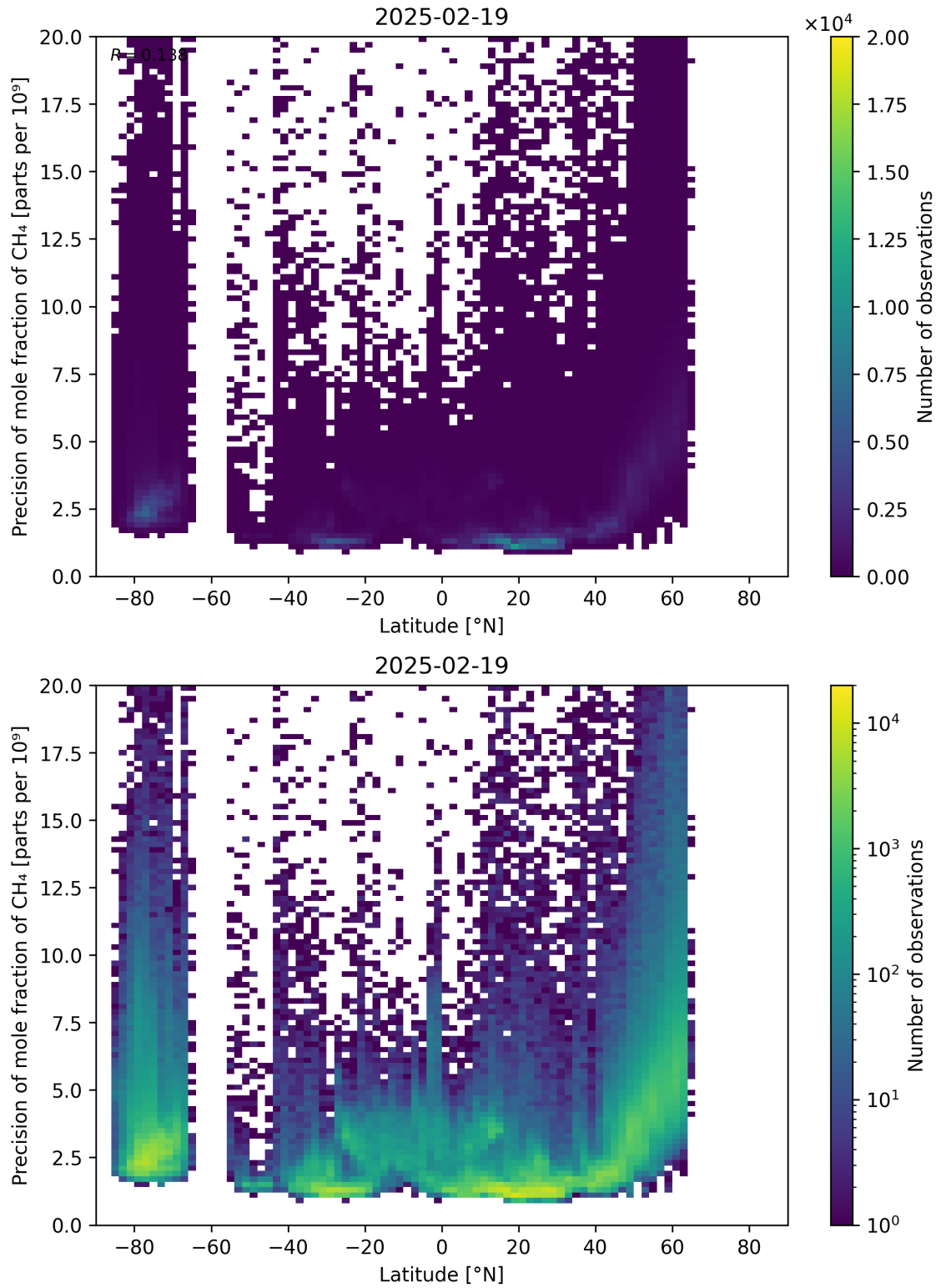
Figure 59: Scatter density plot of “Latitude” against “Precision of mole fraction of CH 4 ” for 2025-02-19 to 2025-02-20.
