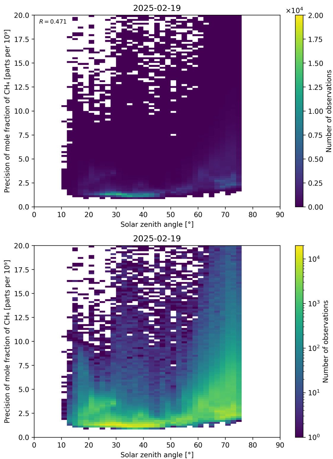
Figure 101: Scatter density plot of “Solar zenith angle” against “Precision of mole fraction of \text{CH}_4 ” for 2025-02-19 to 2025-02-20.
