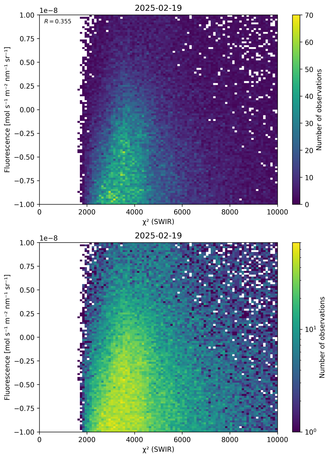
Figure 49: Scatter density plot of “ \chi^2 (SWIR)” against “Fluorescence” for 2025-02-19 to 2025-02-20.
