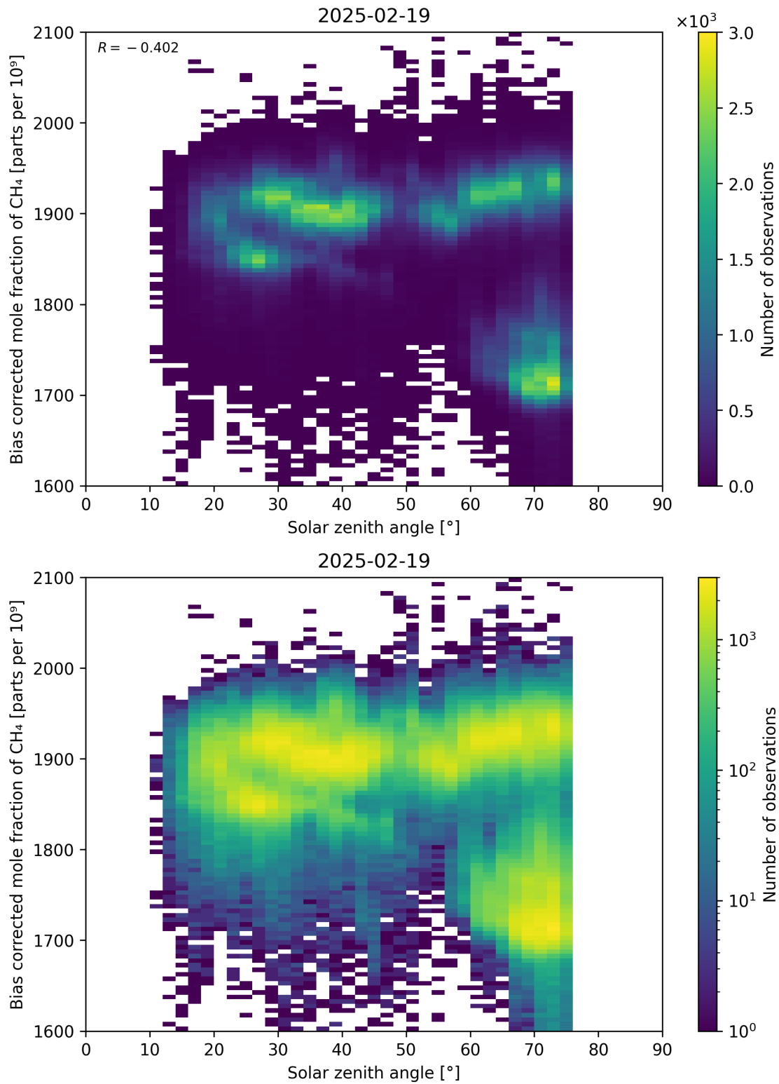
Figure 100: Scatter density plot of “Solar zenith angle” against “Bias corrected mole fraction of CH 4 ” for 2025-02-19 to 2025-02-20.
