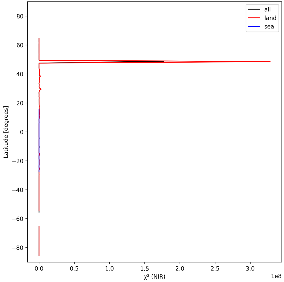
Figure 18: Zonal average of “ \chi^2 (NIR)” for 2025-02-19 to 2025-02-20.
