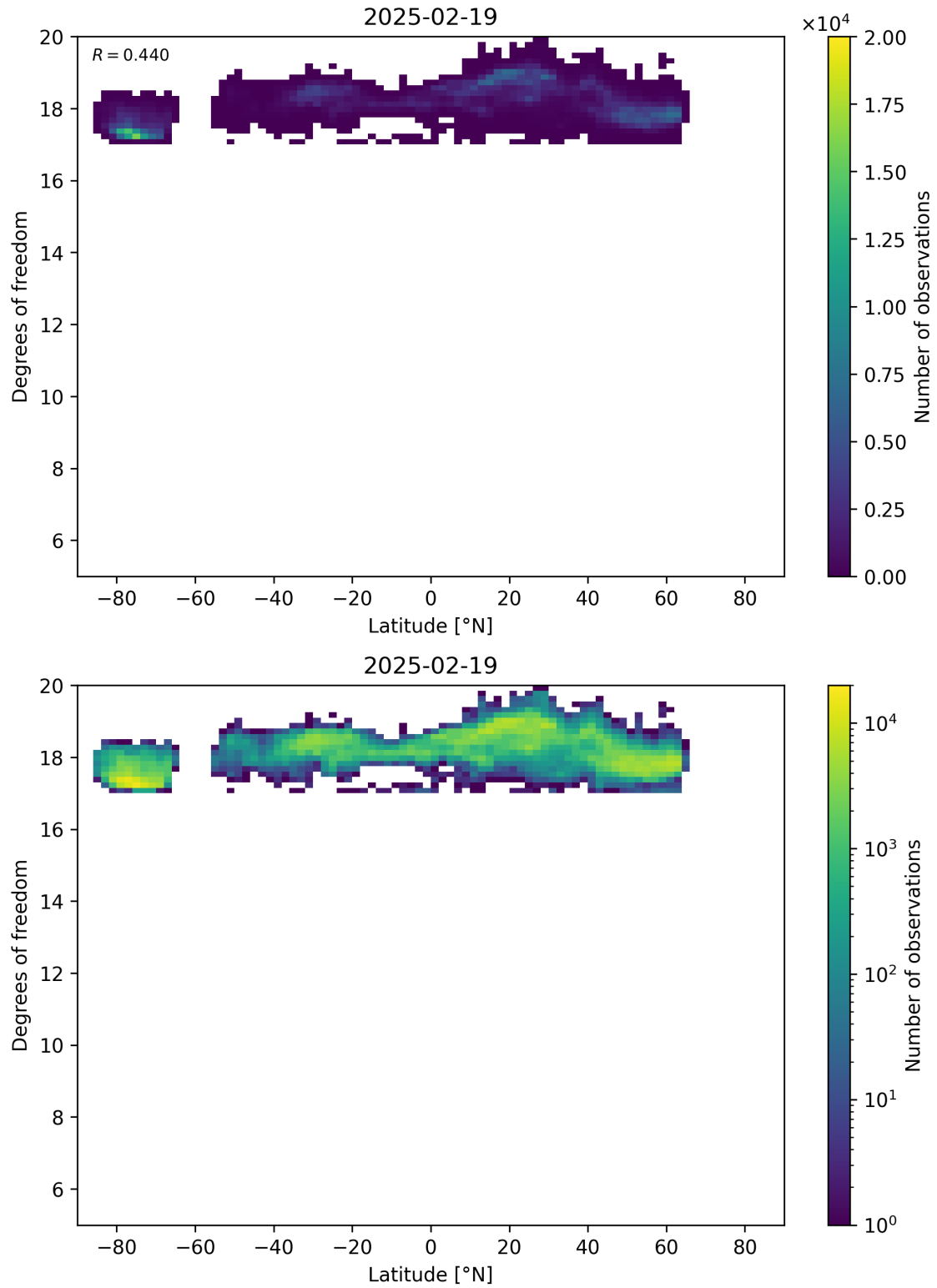
Figure 55: Scatter density plot of “Latitude” against “Degrees of freedom” for 2025-02-19 to 2025-02-20.
