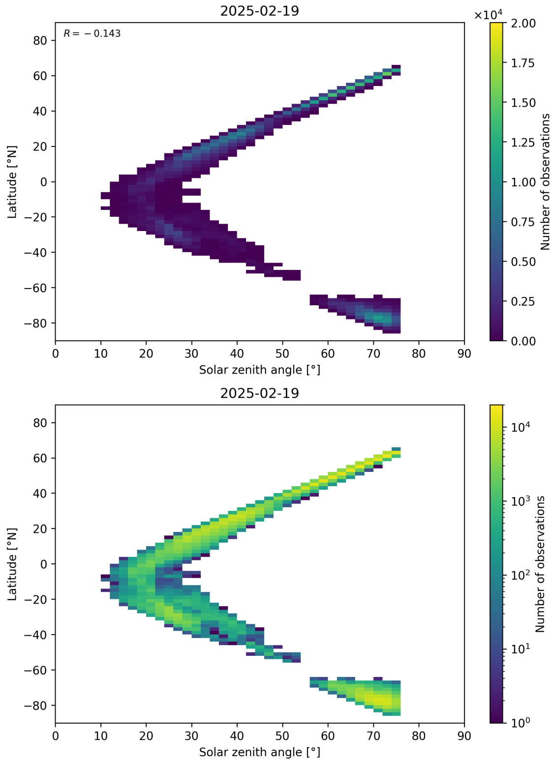
Figure 98: Scatter density plot of “Solar zenith angle” against “Latitude” for 2025-02-19 to 2025-02-20.
