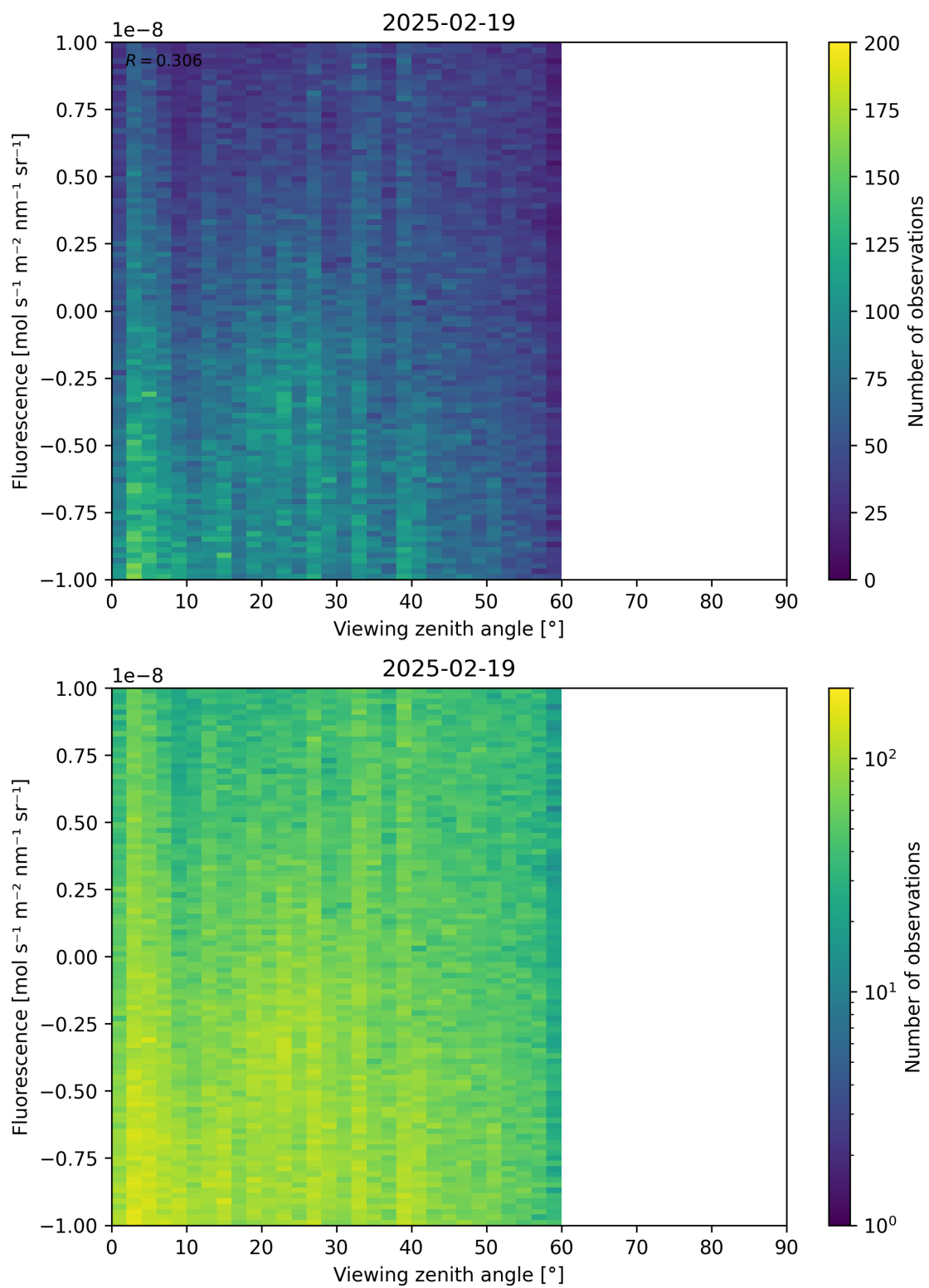
Figure 108: Scatter density plot of “Viewing zenith angle” against “Fluorescence” for 2025-02-19 to 2025-02-20.
