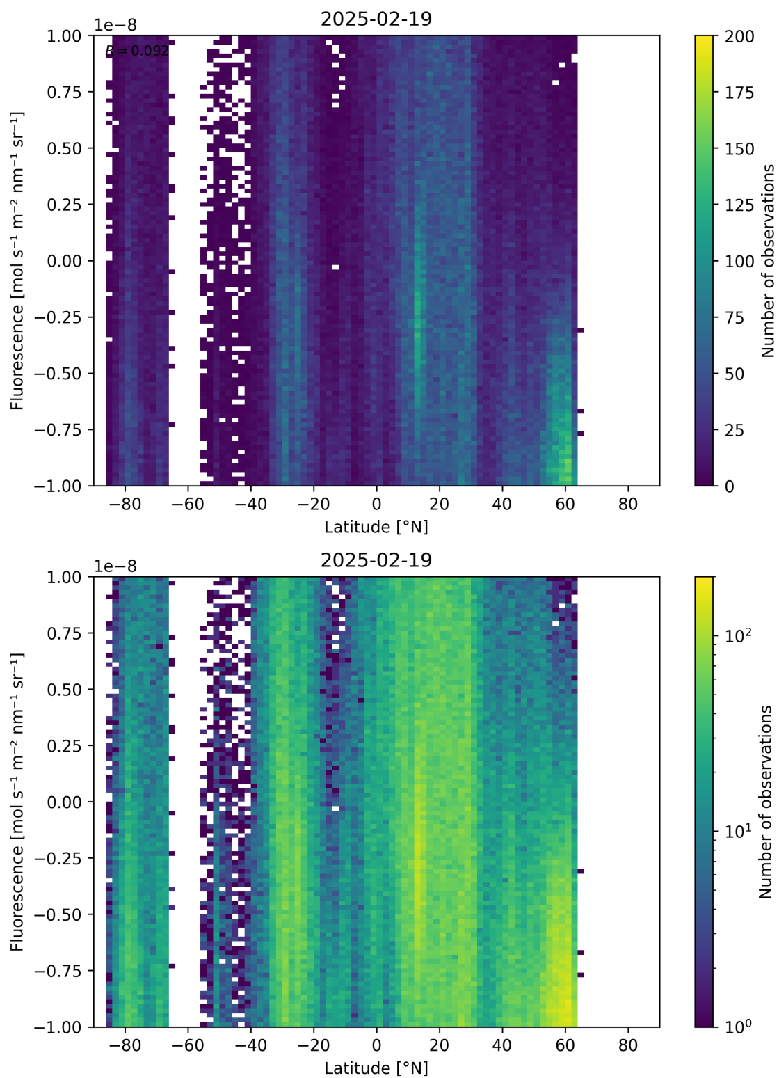
Figure 56: Scatter density plot of “Latitude” against “Fluorescence” for 2025-02-19 to 2025-02-20.
