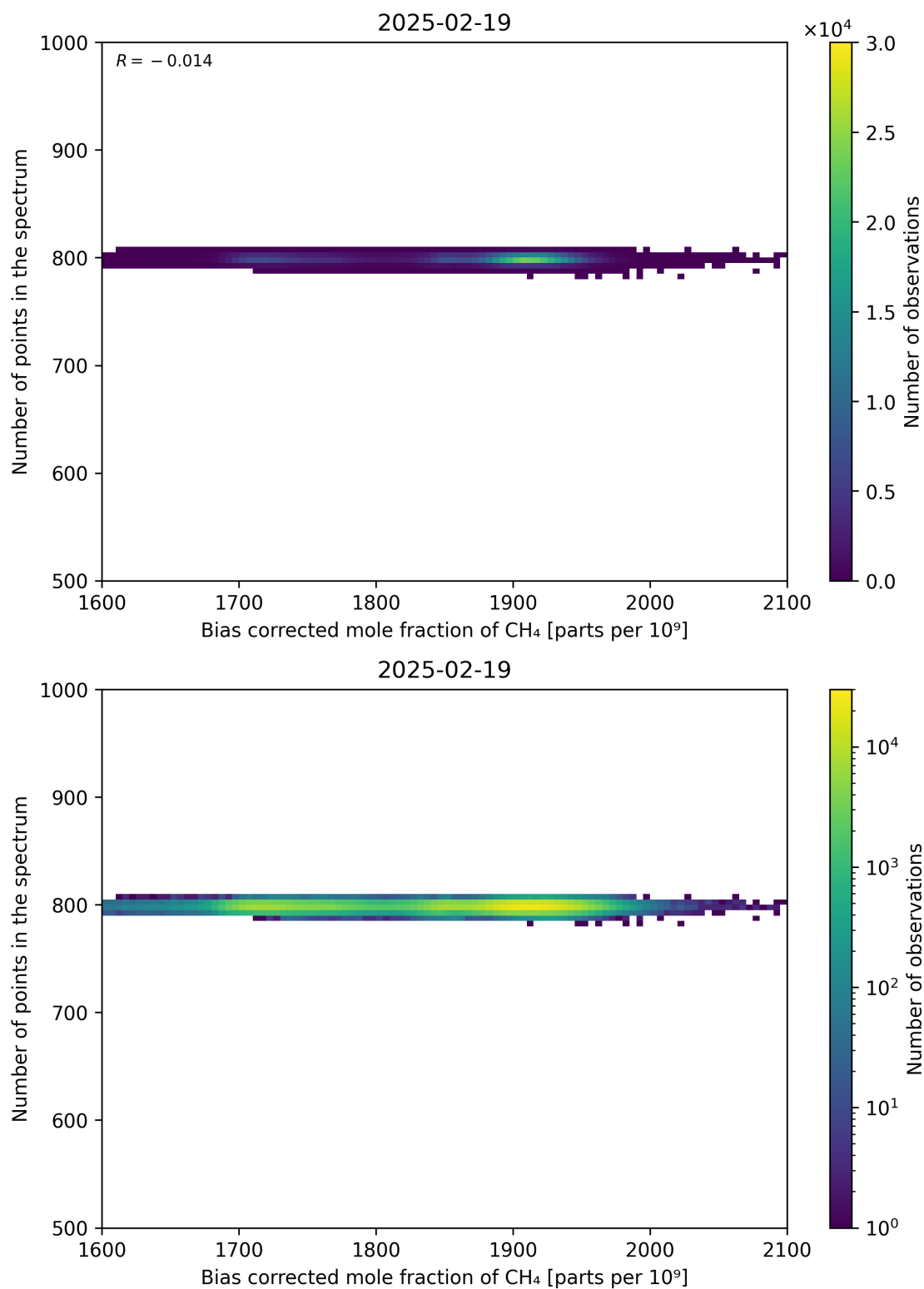
Figure 68: Scatter density plot of “Bias corrected mole fraction of CH 4 ” against “Number of points in the spectrum” for 2025-02-19 to 2025-02-20.
