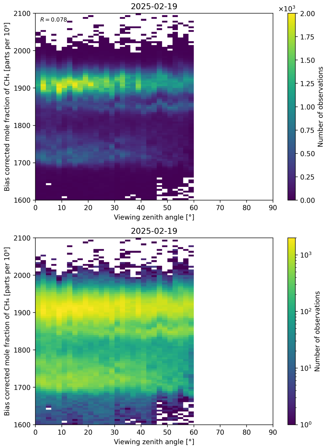
Figure 111: Scatter density plot of “Viewing zenith angle” against “Bias corrected mole fraction of CH 4 ” for 2025-02-19 to 2025-02-20.
