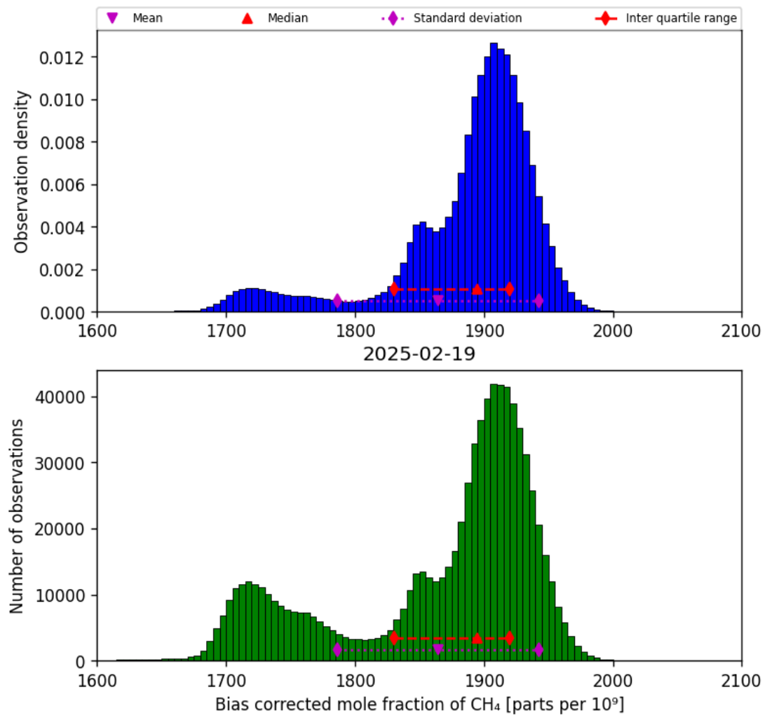
Figure 25: Histogram of “Bias corrected mole fraction of CH 4 ” for 2025-02-19 to 2025-02-20
