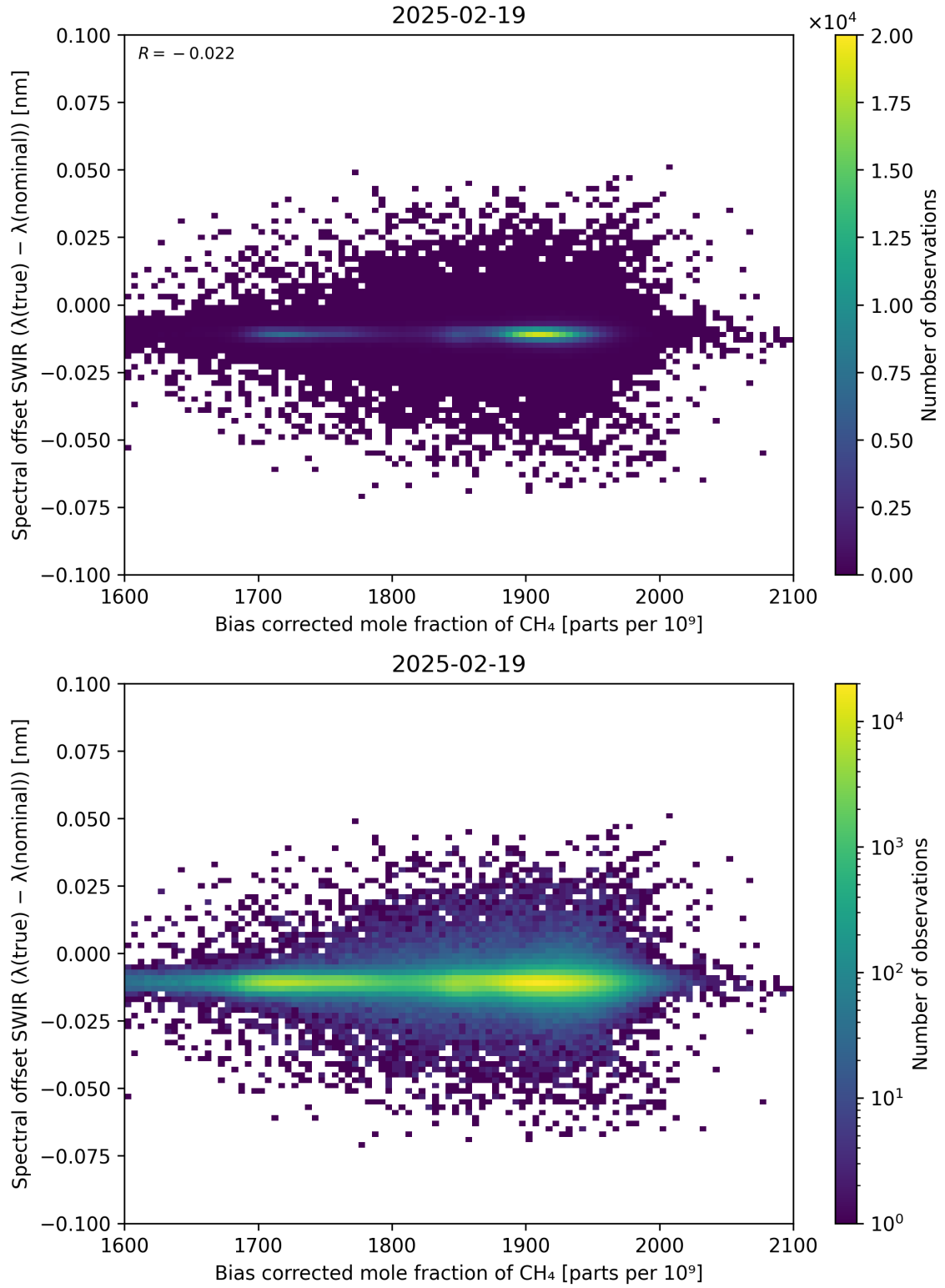
Figure 69: Scatter density plot of “Bias corrected mole fraction of \text{CH}_4 ” against “Spectral offset SWIR ( \lambda_{\text{true}} - \lambda_{\text{nominal}} )” for 2025-02-19 to 2025-02-20.
