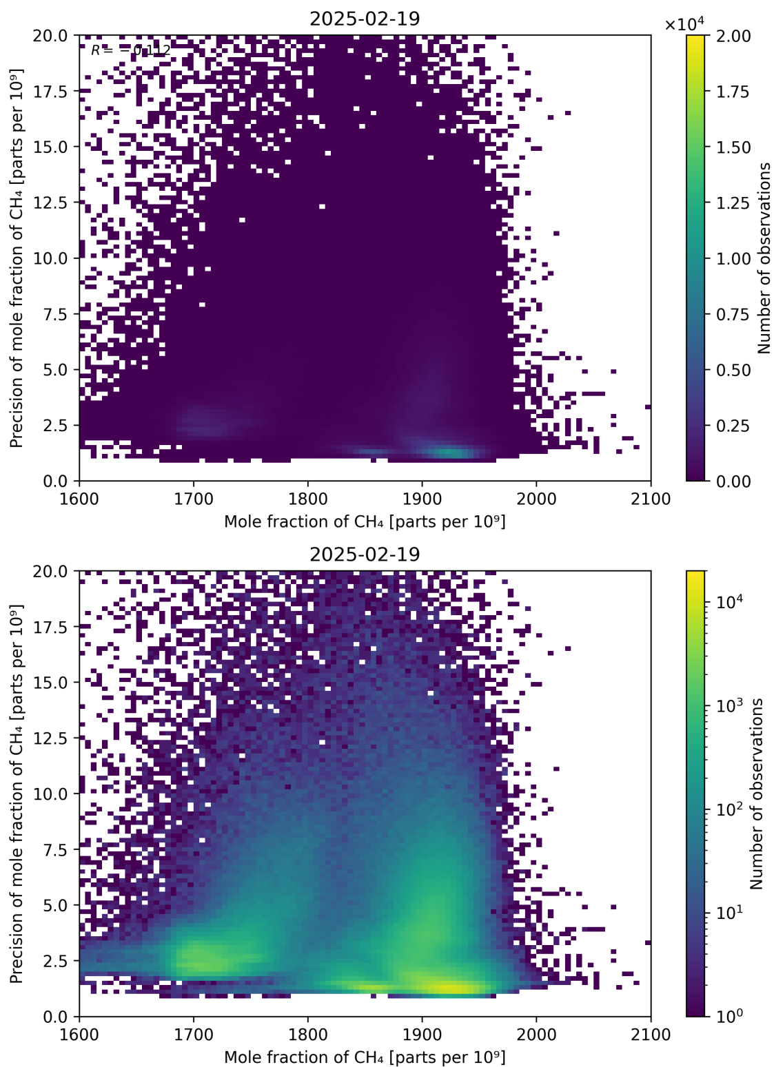
Figure 75: Scatter density plot of “Mole fraction of CH 4 ” against “Precision of mole fraction of CH 4 ” for 2025-02-19 to 2025-02-20.
