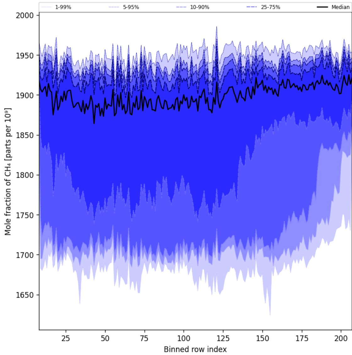
Figure 34: Along track statistics of “Mole fraction of CH 4 ” for 2025-02-19 to 2025-02-20
