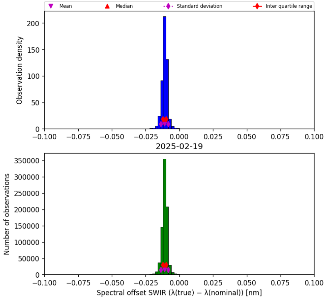
Figure 27: Histogram of “Spectral offset SWIR ( \lambda_{\text{true}} - \lambda_{\text{nominal}} )” for 2025-02-19 to 2025-02-20
