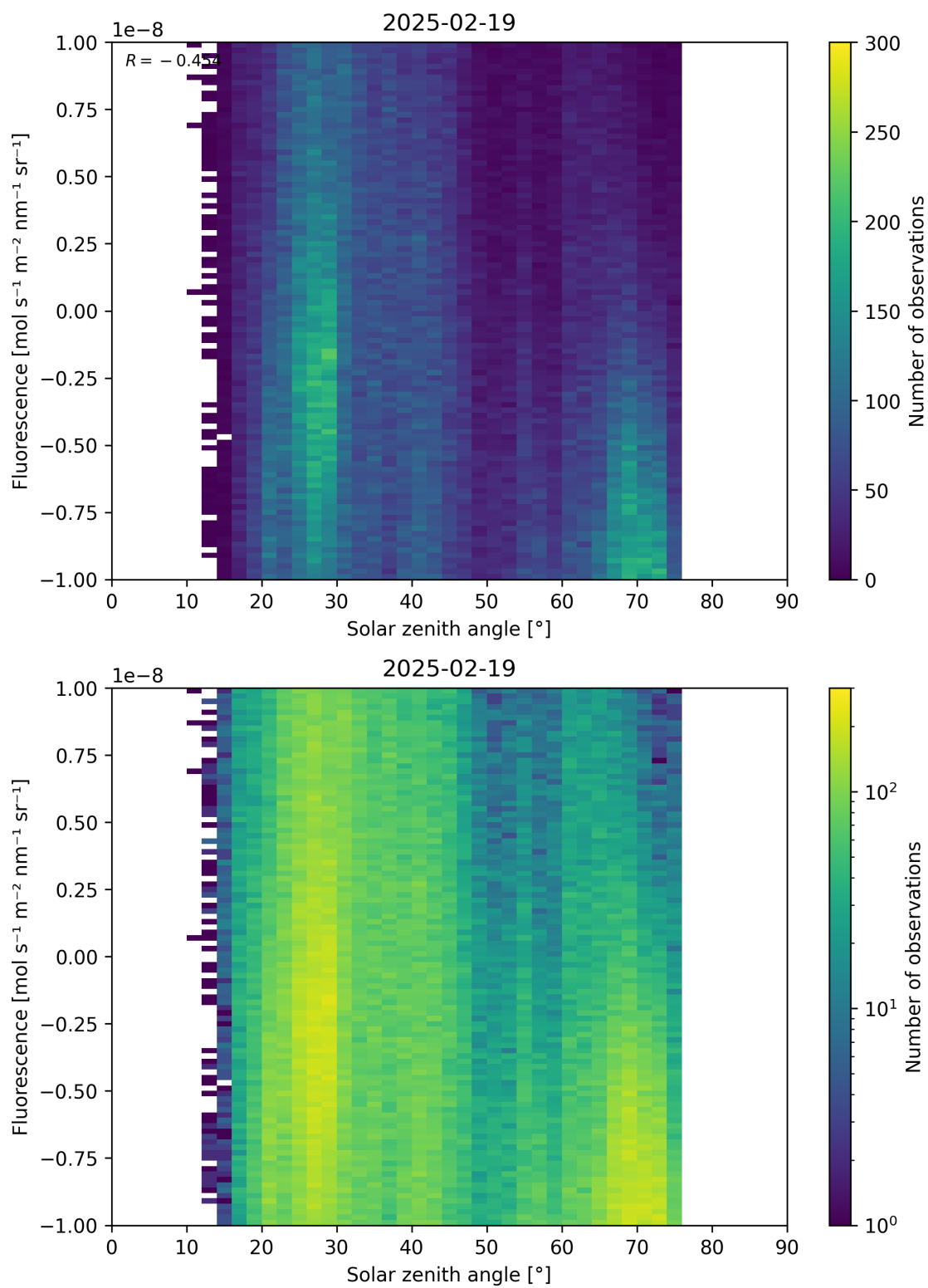
Figure 97: Scatter density plot of “Solar zenith angle” against “Fluorescence” for 2025-02-19 to 2025-02-20.
