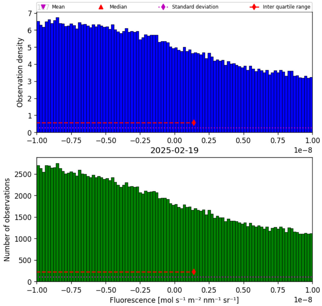
Figure 32: Histogram of “Fluorescence” for 2025-02-19 to 2025-02-20
