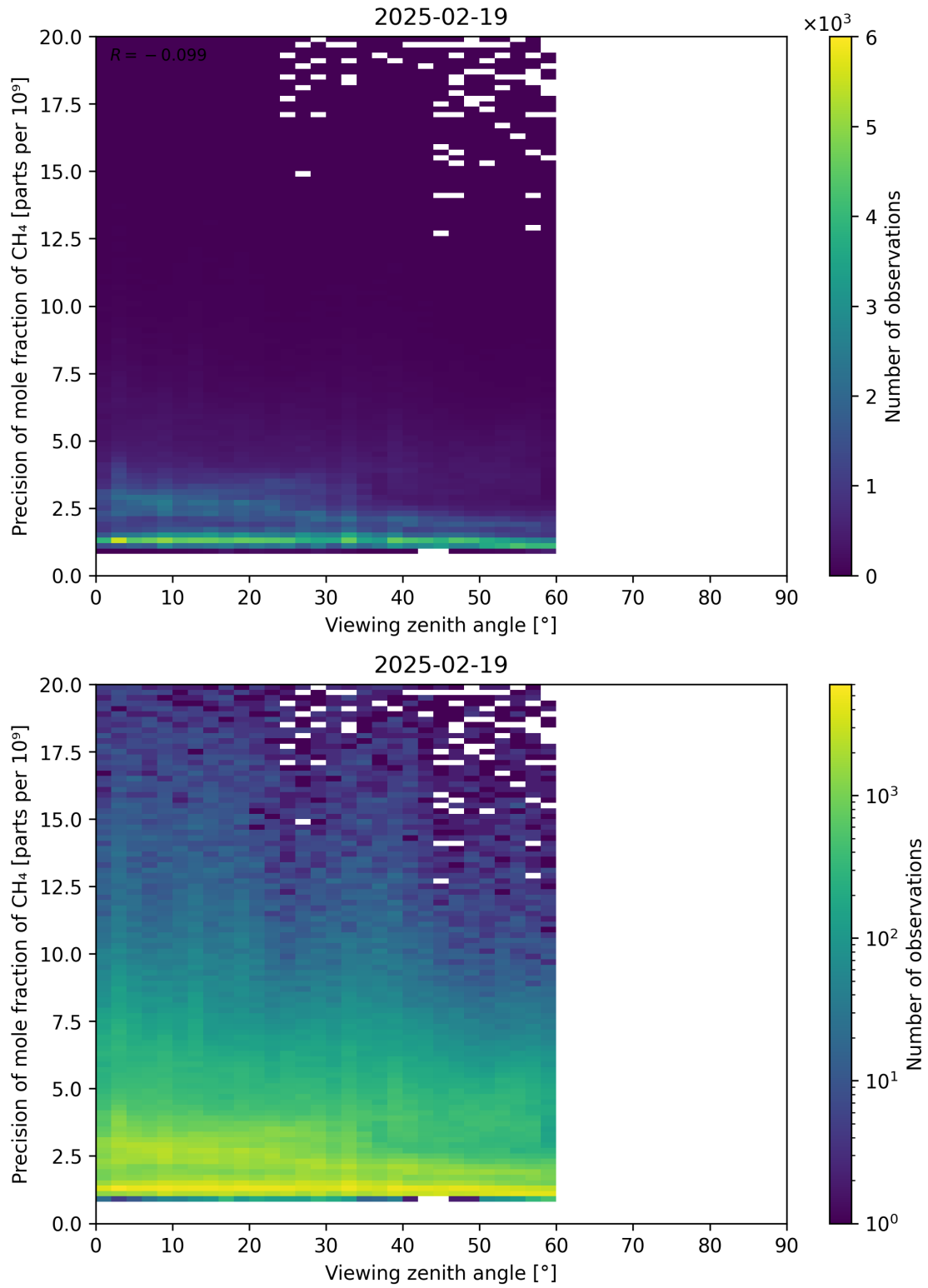
Figure 112: Scatter density plot of “Viewing zenith angle” against “Precision of mole fraction of \text{CH}_4 ” for 2025-02-19 to 2025-02-20.
