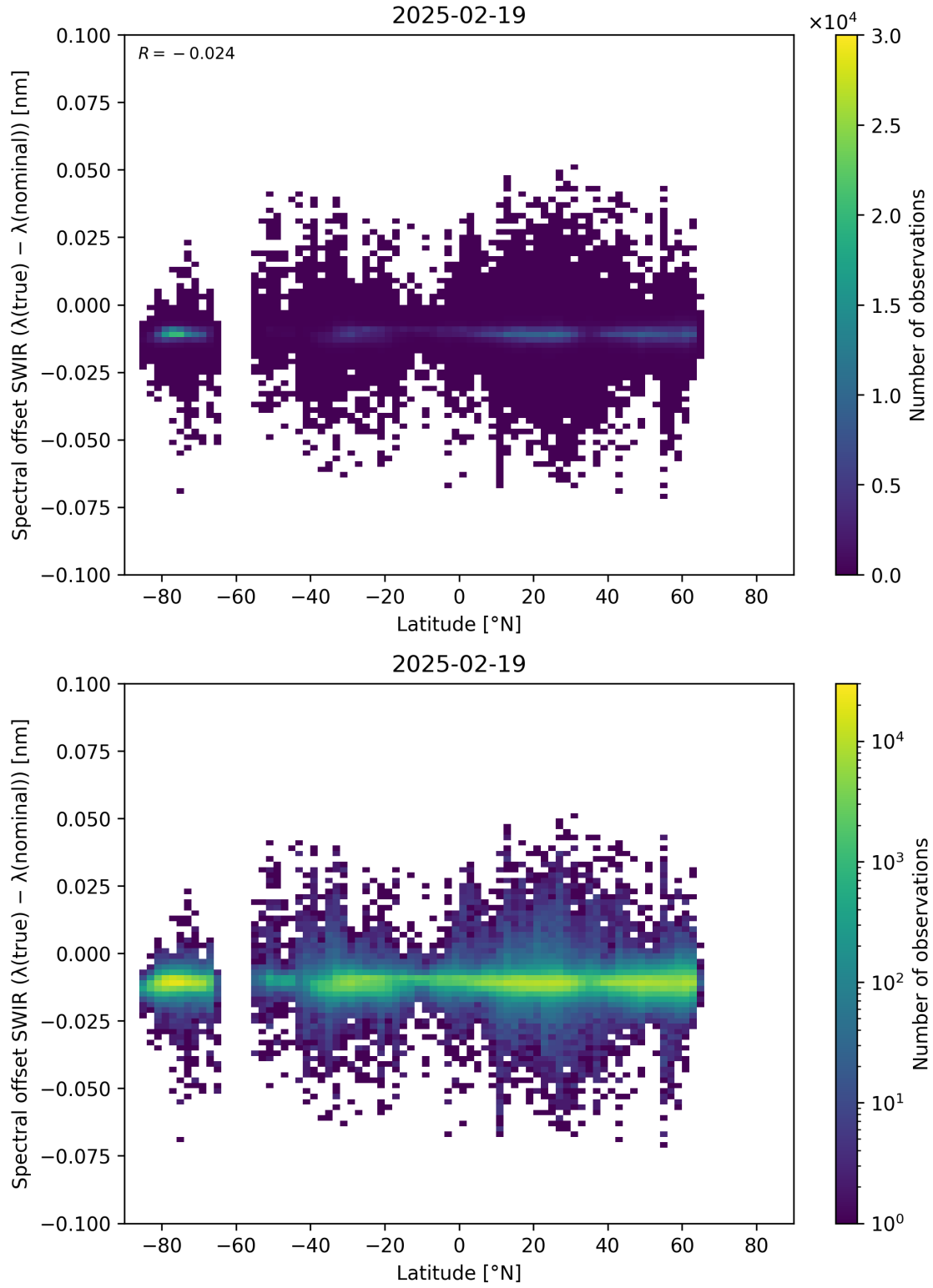
Figure 62: Scatter density plot of “Latitude” against “Spectral offset SWIR ( \lambda_{\text{true}} - \lambda_{\text{nominal}} )” for 2025-02-19 to 2025-02-20.
