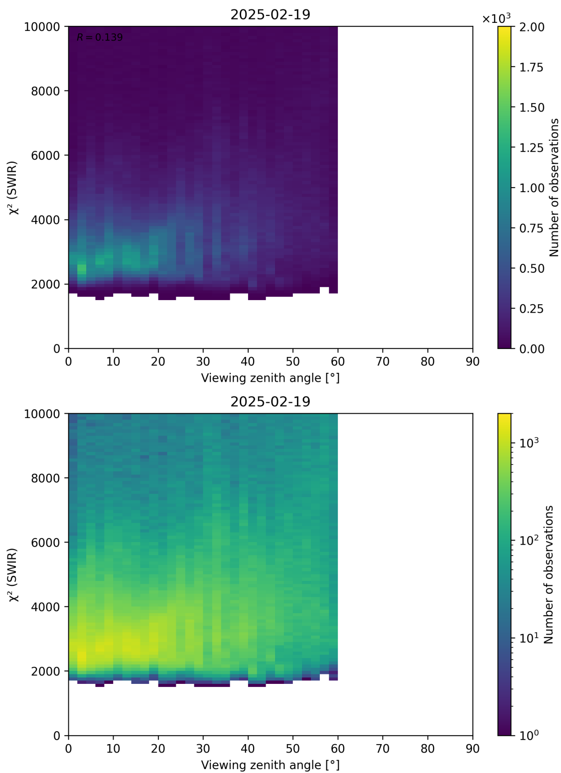
Figure 106: Scatter density plot of “Viewing zenith angle” against “ \chi^2 (SWIR)” for 2025-02-19 to 2025-02-20.
