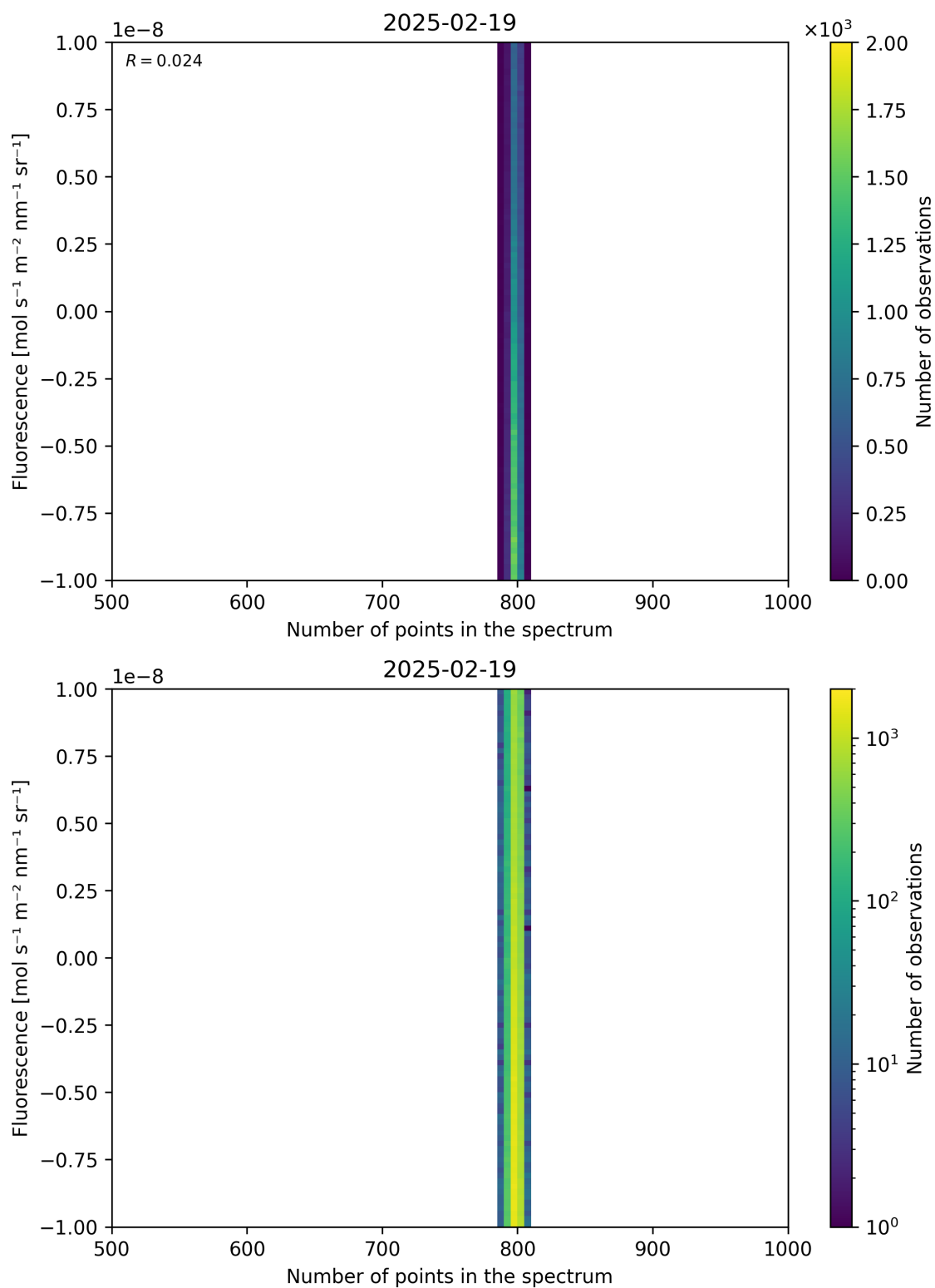
Figure 91: Scatter density plot of “Number of points in the spectrum” against “Fluorescence” for 2025-02-19 to 2025-02-20.
