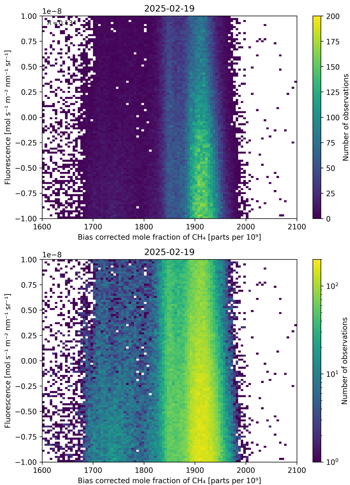
Figure 66: Scatter density plot of “Bias corrected mole fraction of \text{CH}_4 ” against “Fluorescence” for 2025-02-19 to 2025-02-20.
