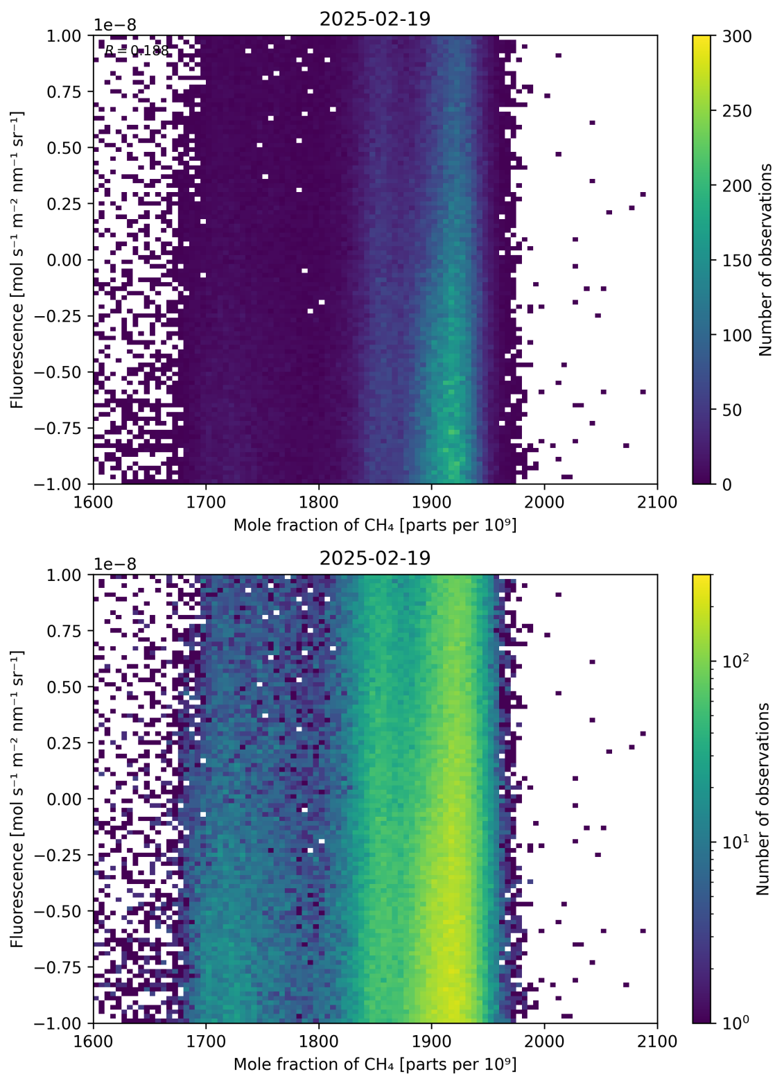
Figure 73: Scatter density plot of “Mole fraction of \text{CH}_4 ” against “Fluorescence” for 2025-02-19 to 2025-02-20.
