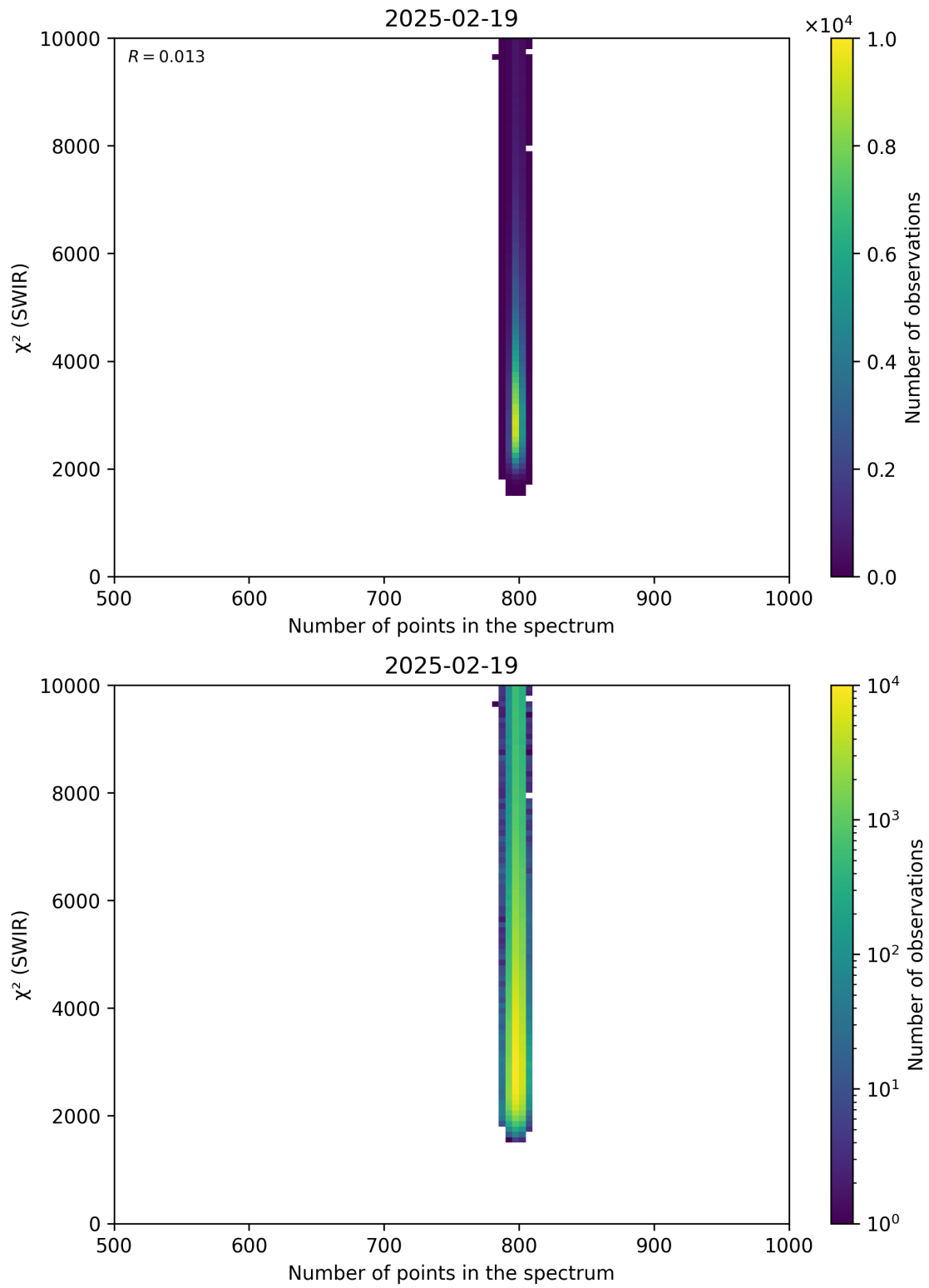
Figure 89: Scatter density plot of “Number of points in the spectrum” against “ \chi^2 (SWIR)” for 2025-02-19 to 2025-02-20.
