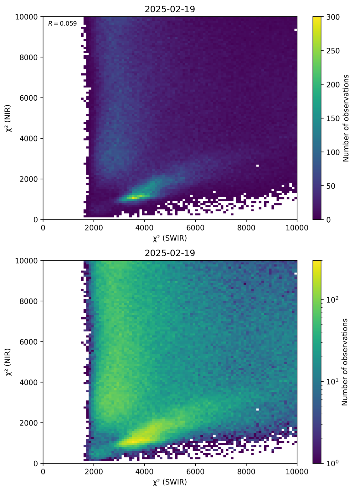
Figure 47: Scatter density plot of “ \chi^2 (SWIR)” against “ \chi^2 (NIR)” for 2025-02-19 to 2025-02-20.
