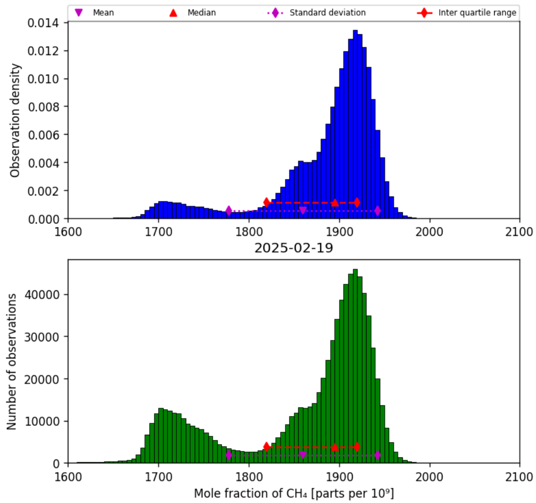
Figure 23: Histogram of “Mole fraction of CH 4 ” for 2025-02-19 to 2025-02-20
