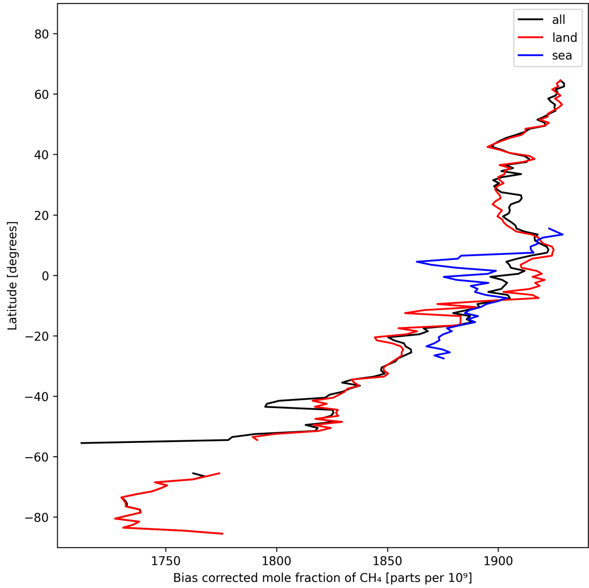
Figure 14: Zonal average of “Bias corrected mole fraction of CH 4 ” for 2025-02-19 to 2025-02-20.
