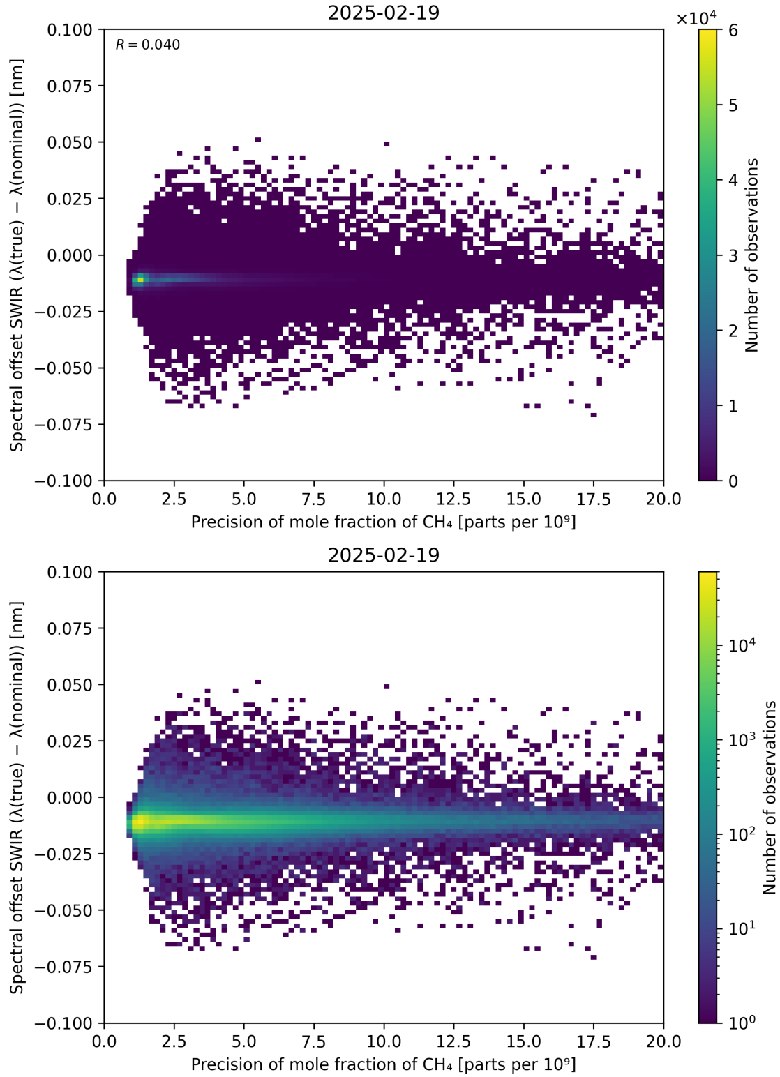
Figure 85: Scatter density plot of “Precision of mole fraction of \text{CH}_4 ” against “Spectral offset SWIR ( \lambda_{\text{true}} - \lambda_{\text{nominal}} )” for 2025-02-19 to 2025-02-20.
