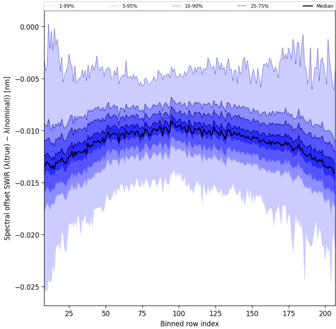
Figure 38: Along track statistics of “Spectral offset SWIR ( \lambda_{\text{true}} - \lambda_{\text{nominal}} )” for 2025-02-19 to 2025-02-20
