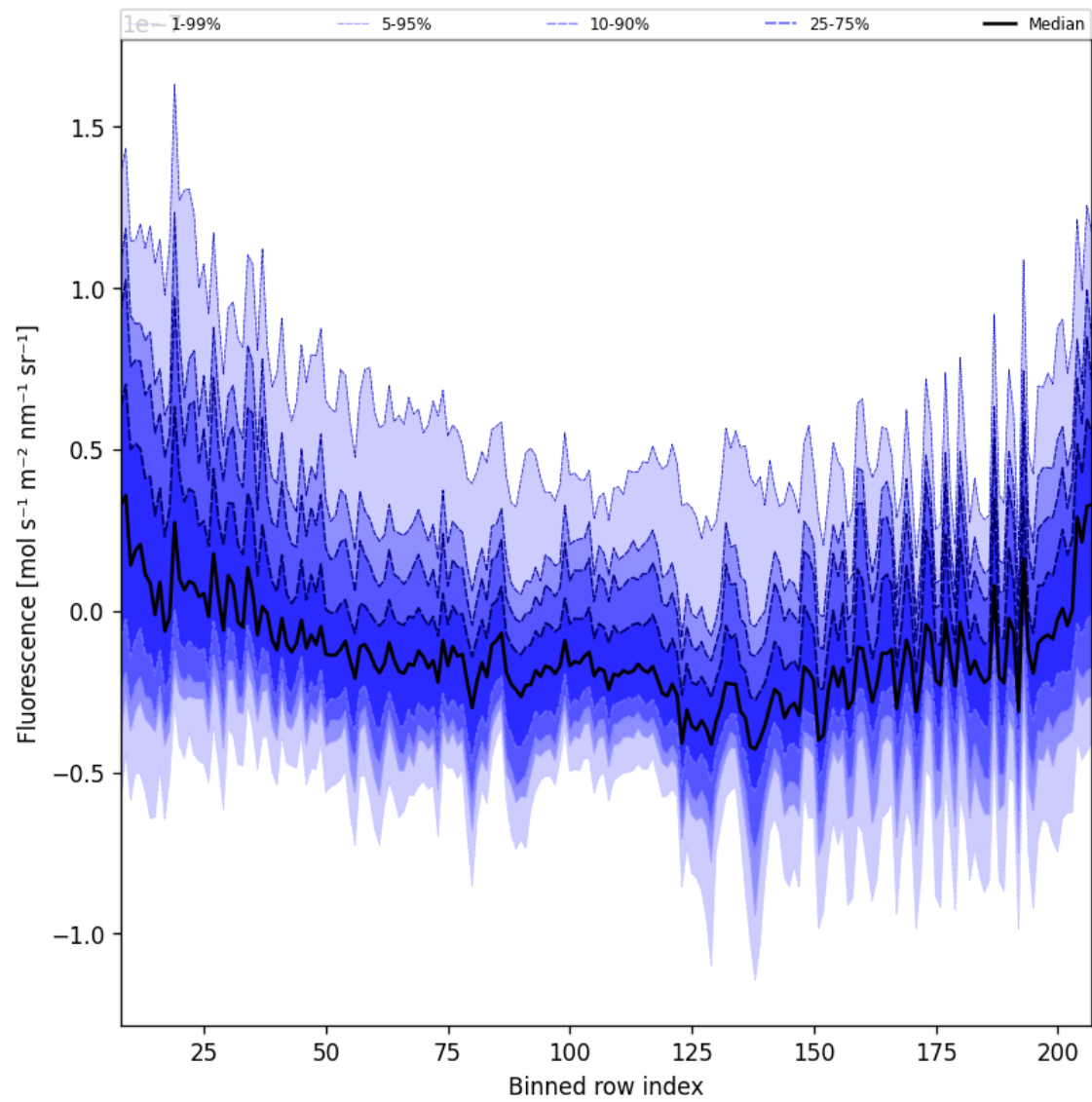
Figure 43: Along track statistics of “Fluorescence” for 2025-02-19 to 2025-02-20
