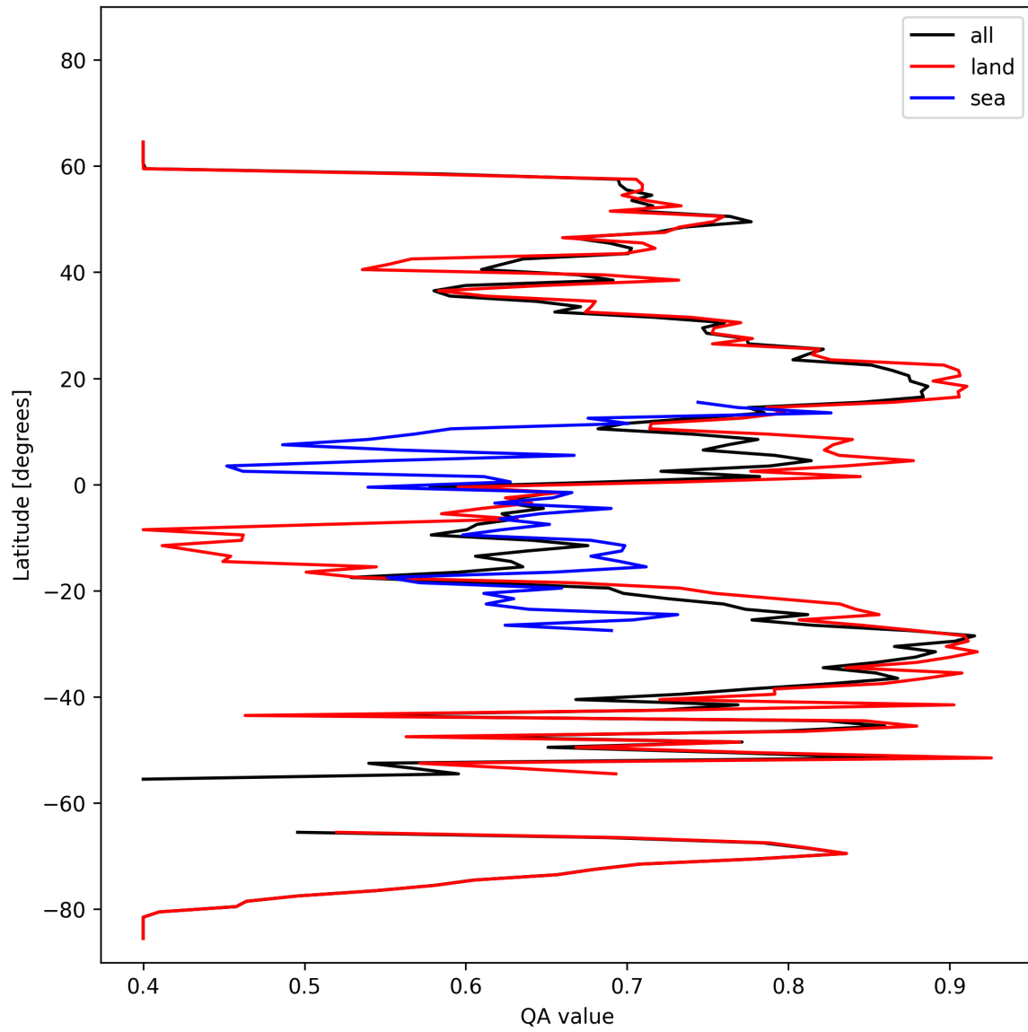
Figure 11: Zonal average of “QA value” for 2025-02-19 to 2025-02-20.
