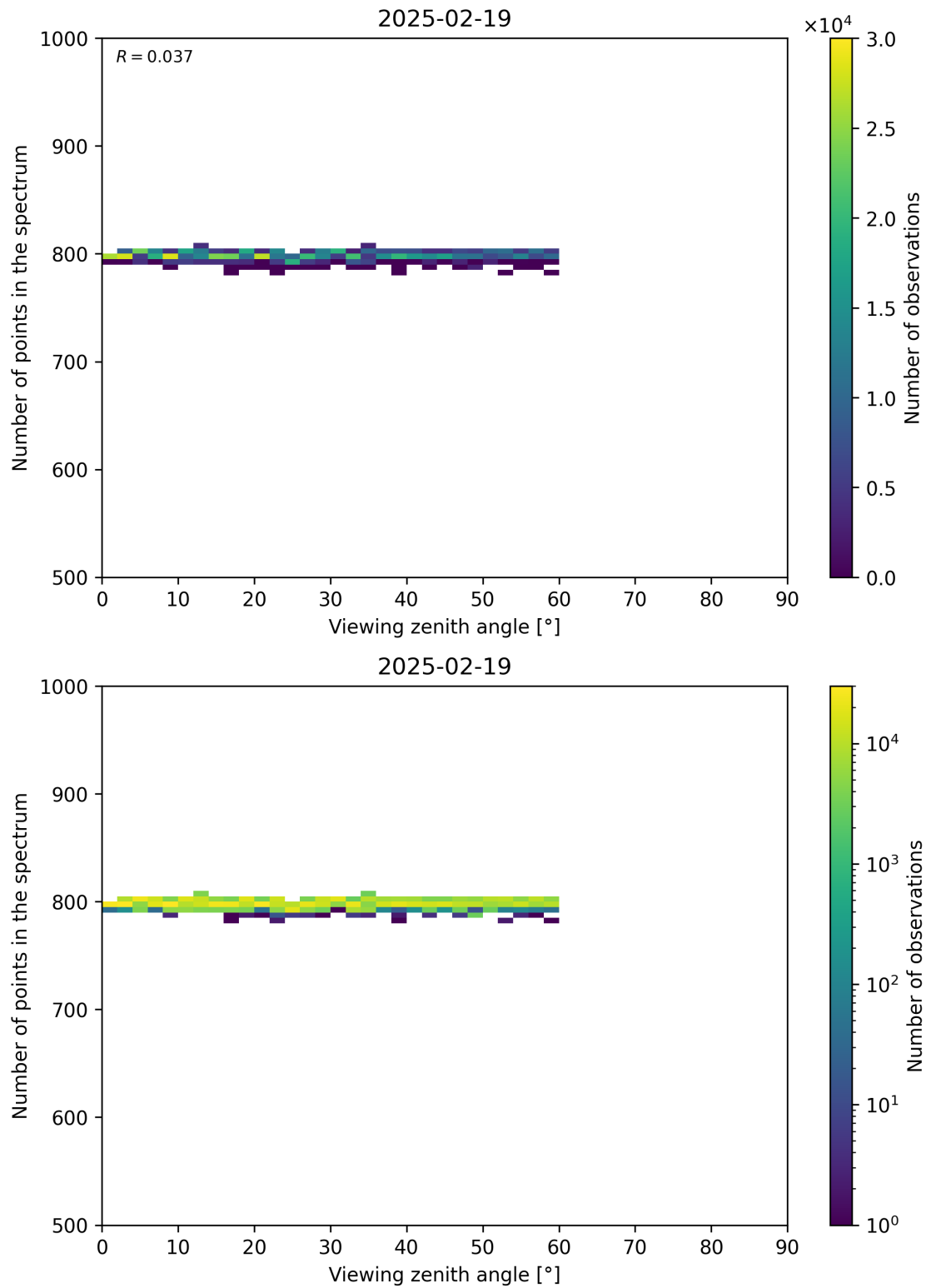
Figure 114: Scatter density plot of “Viewing zenith angle” against “Number of points in the spectrum” for 2025-02-19 to 2025-02-20.
