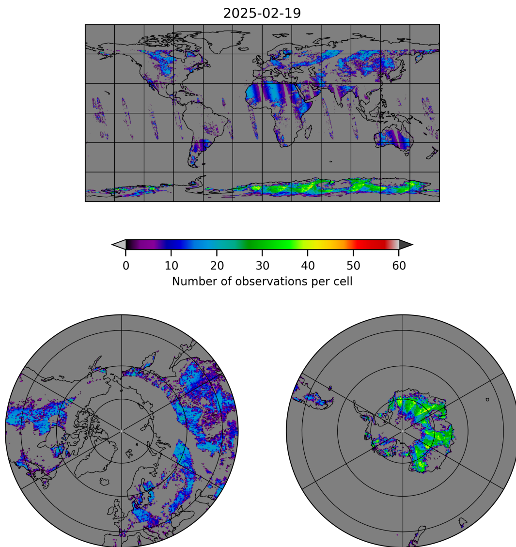
Figure 10: Map of the number of observations for 2025-02-19 to 2025-02-20
