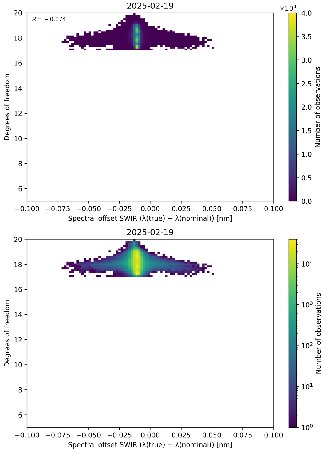
Figure 119: Scatter density plot of “Spectral offset SWIR ( \lambda_{\text{true}} - \lambda_{\text{nominal}} )” against “Degrees of freedom” for 2025-02-19 to 2025-02-20.
