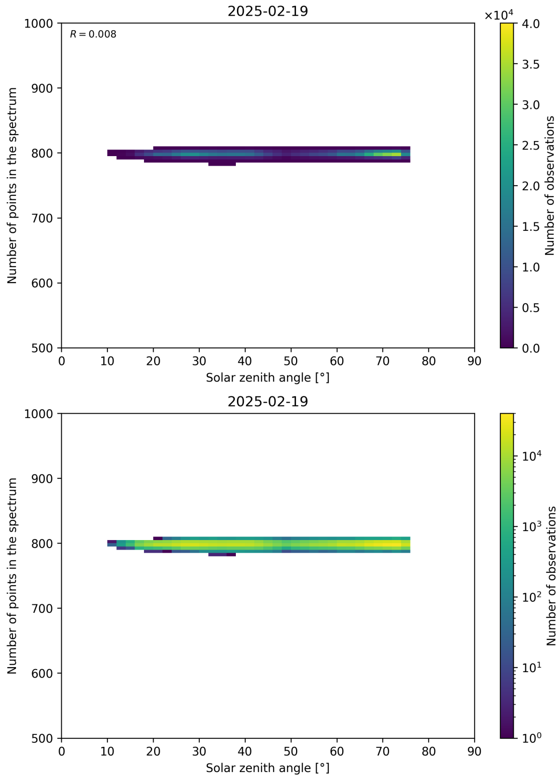
Figure 103: Scatter density plot of “Solar zenith angle” against “Number of points in the spectrum” for 2025-02-19 to 2025-02-20.
