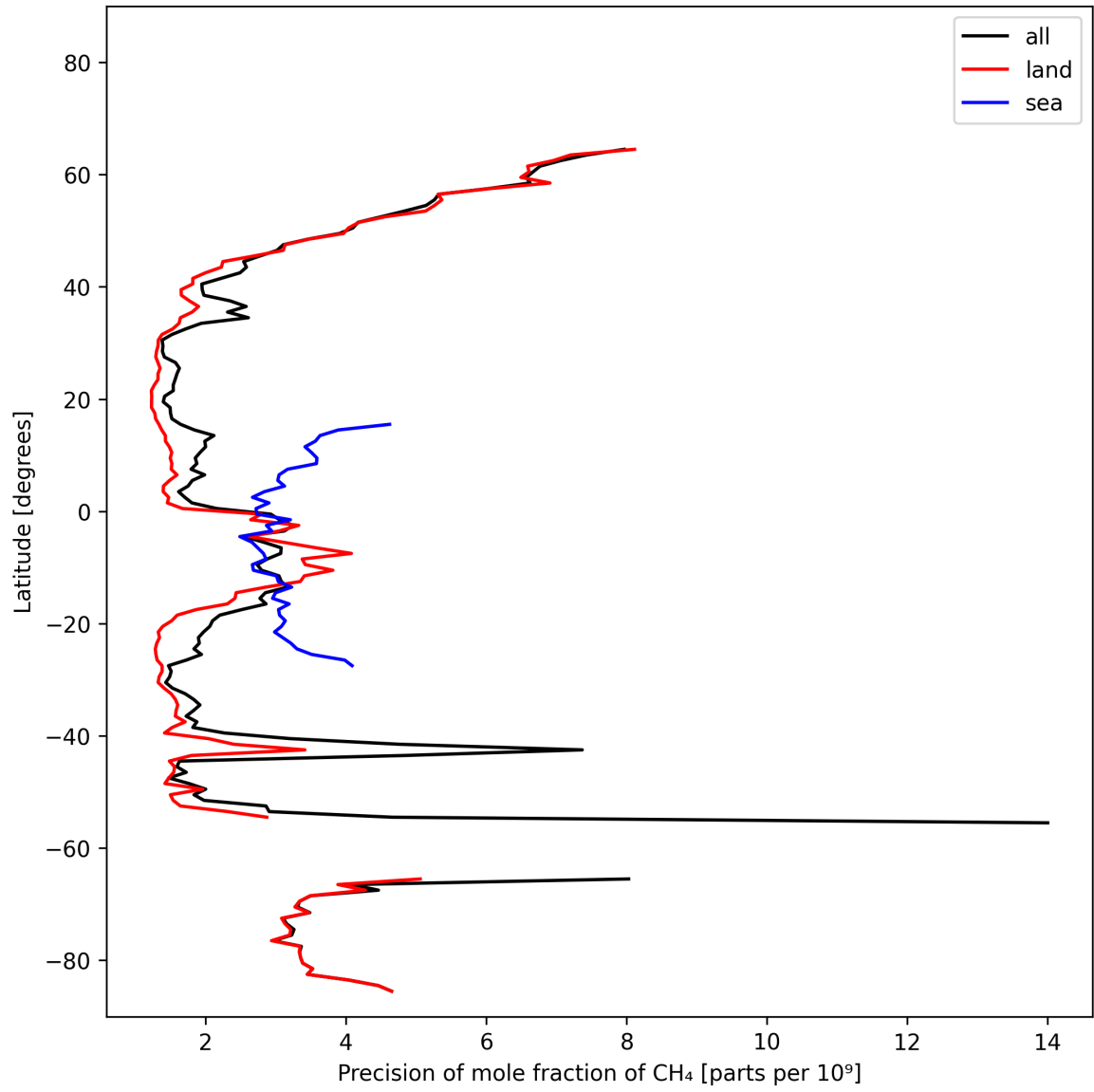
Figure 13: Zonal average of “Precision of mole fraction of CH 4 ” for 2025-02-19 to 2025-02-20.
