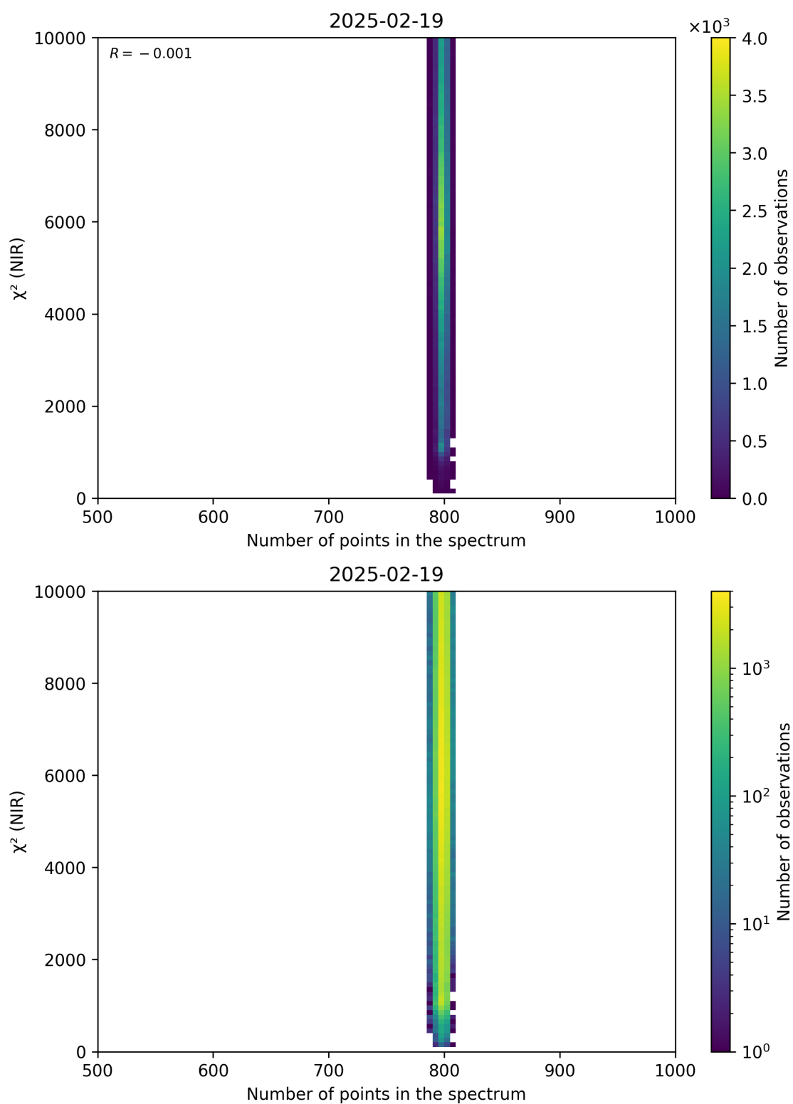
Figure 88: Scatter density plot of “Number of points in the spectrum” against “ \chi^2 (NIR)” for 2025-02-19 to 2025-02-20.
