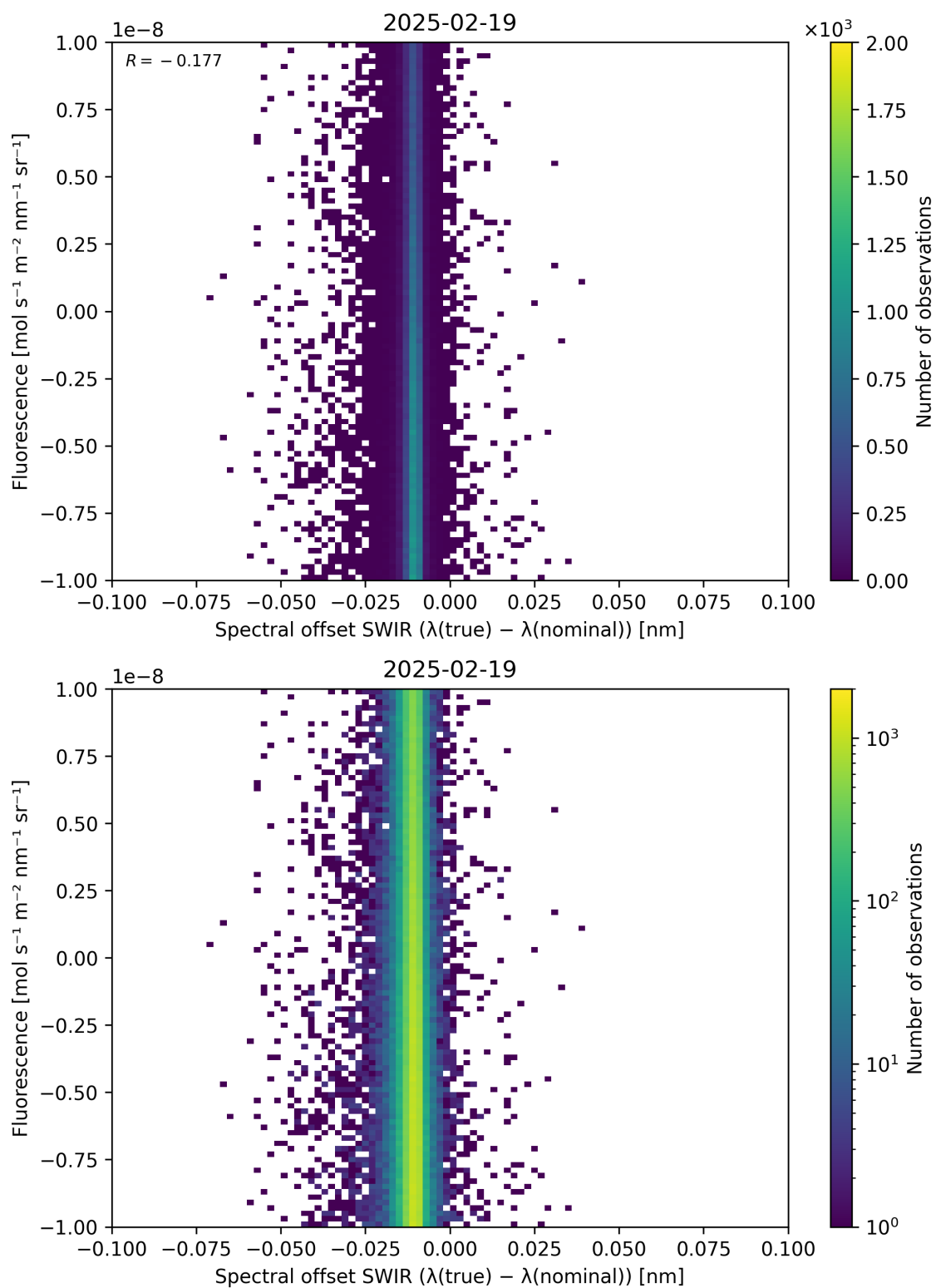
Figure 120: Scatter density plot of “Spectral offset SWIR ( \lambda_{\text{true}} - \lambda_{\text{nominal}} )” against “Fluorescence” for 2025-02-19 to 2025-02-20.
