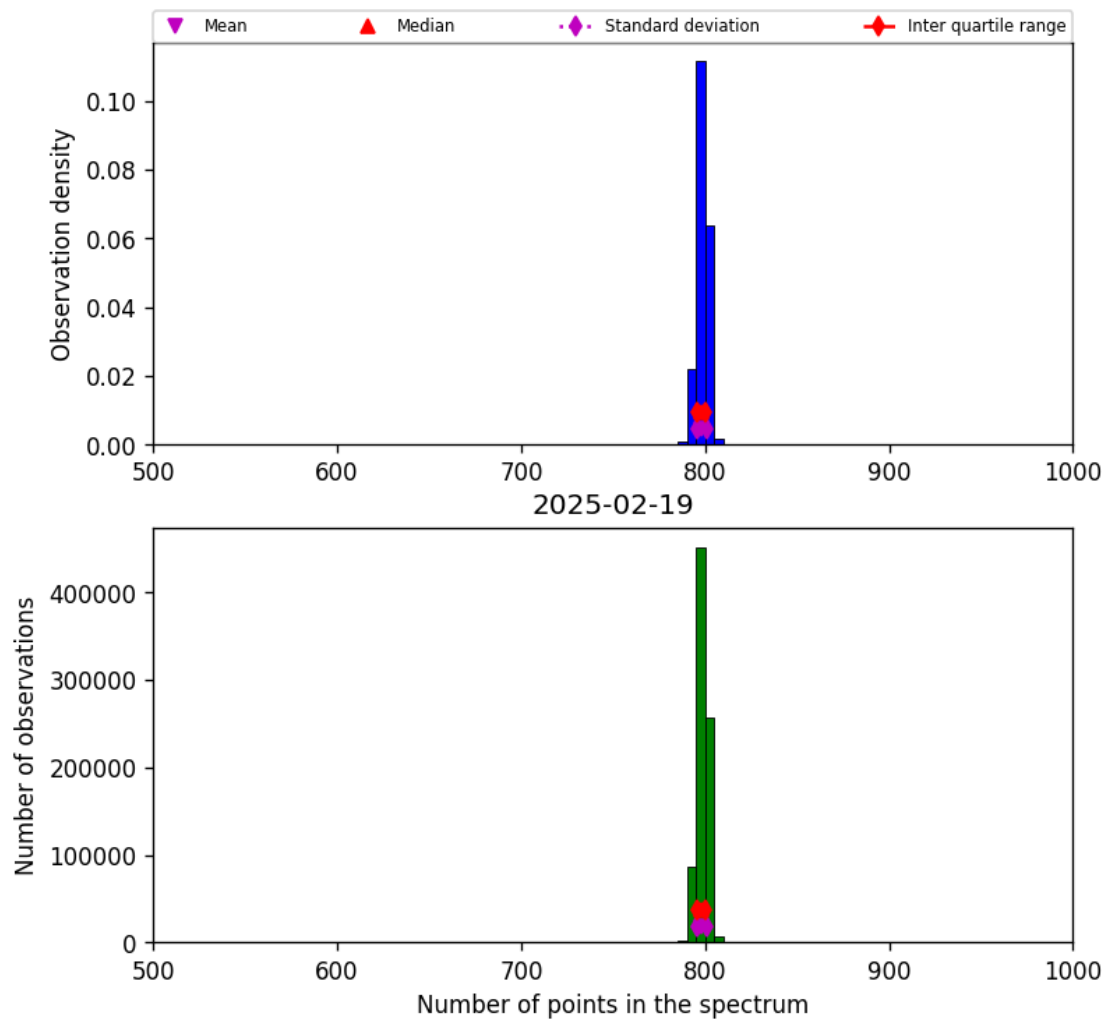
Figure 26: Histogram of “Number of points in the spectrum” for 2025-02-19 to 2025-02-20
