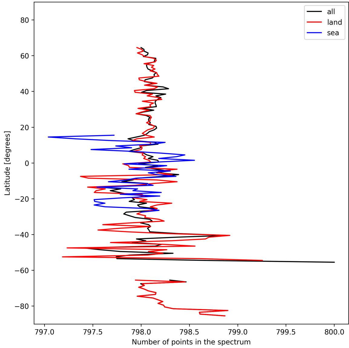
Figure 15: Zonal average of “Number of points in the spectrum” for 2025-02-19 to 2025-02-20.
