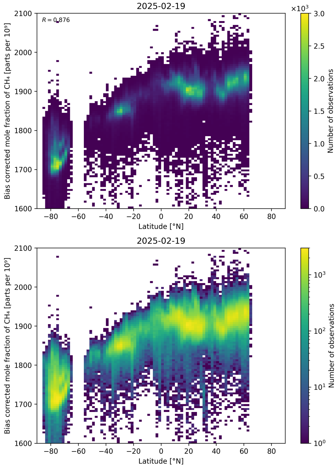
Figure 58: Scatter density plot of “Latitude” against “Bias corrected mole fraction of CH 4 ” for 2025-02-19 to 2025-02-20.
