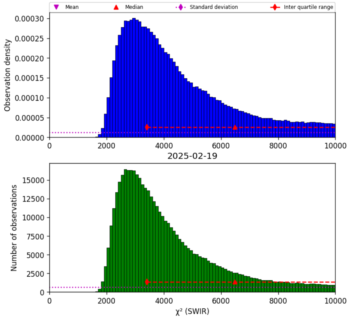
Figure 28: Histogram of “ \chi^2 (SWIR)” for 2025-02-19 to 2025-02-20
