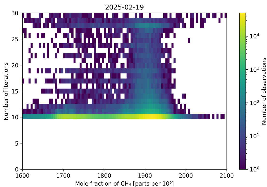
Figure 76: Scatter density plot of “Mole fraction of CH 4 ” against “Number of iterations” for 2025-02-19 to 2025-02-20.
