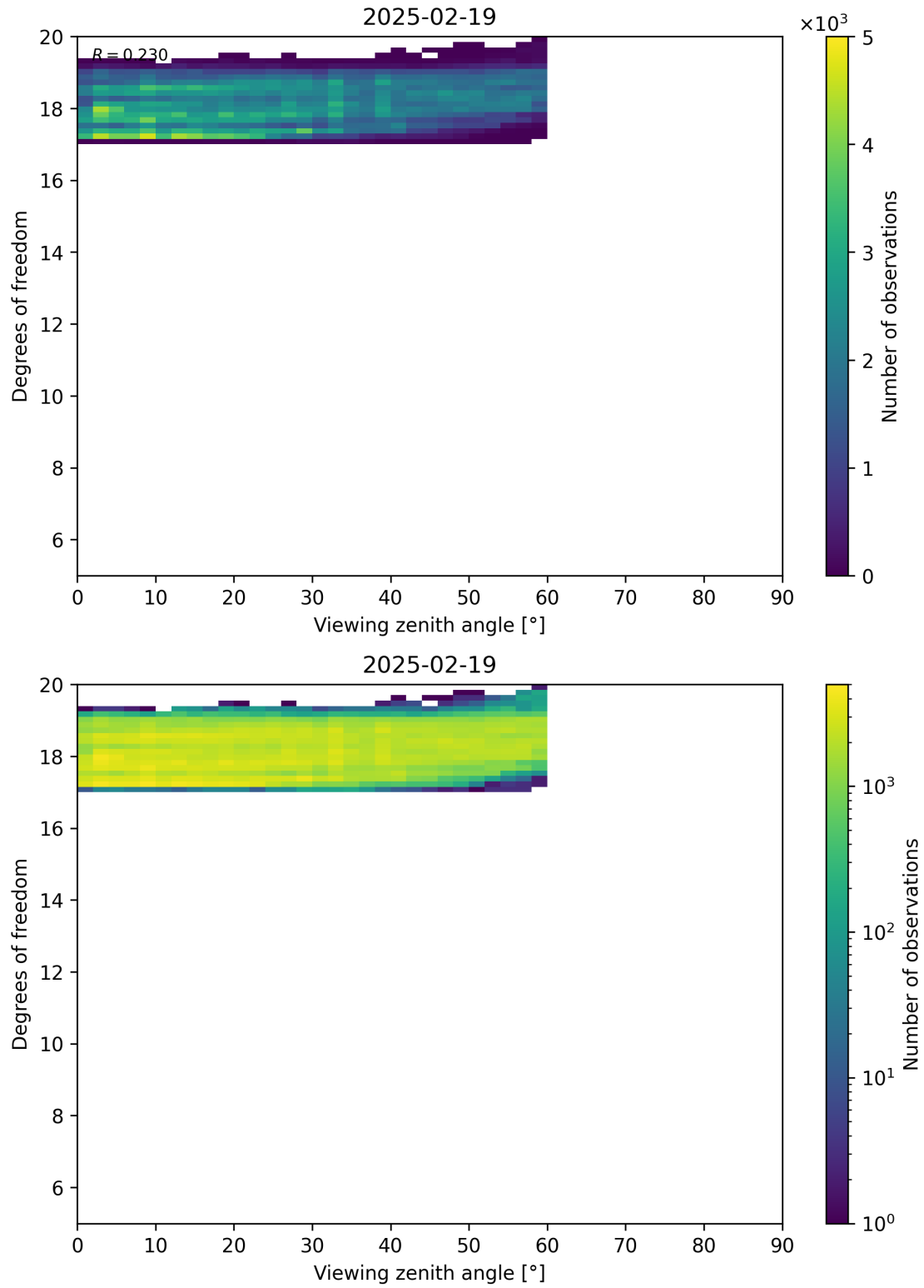
Figure 107: Scatter density plot of “Viewing zenith angle” against “Degrees of freedom” for 2025-02-19 to 2025-02-20.
