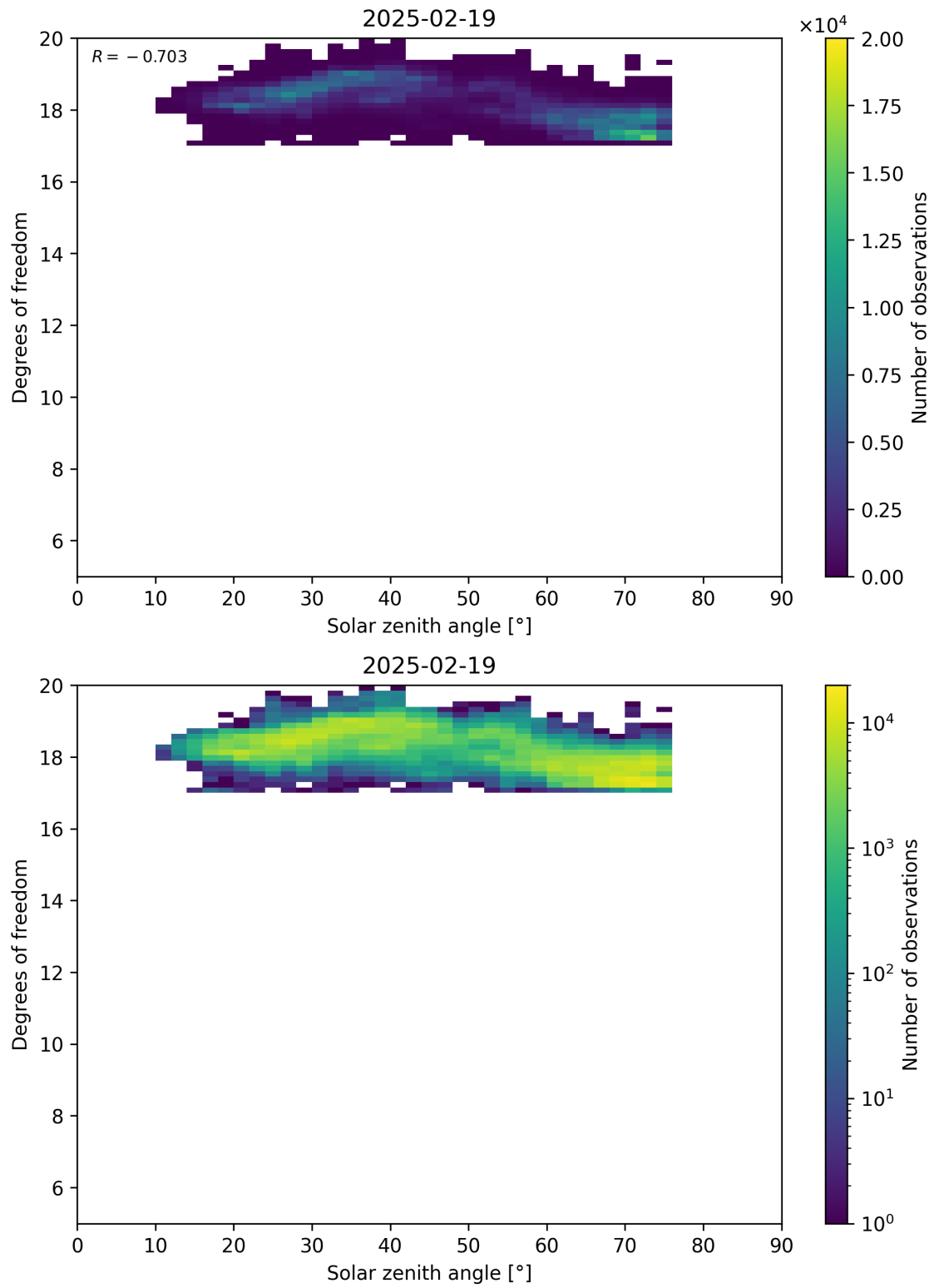
Figure 96: Scatter density plot of “Solar zenith angle” against “Degrees of freedom” for 2025-02-19 to 2025-02-20.
