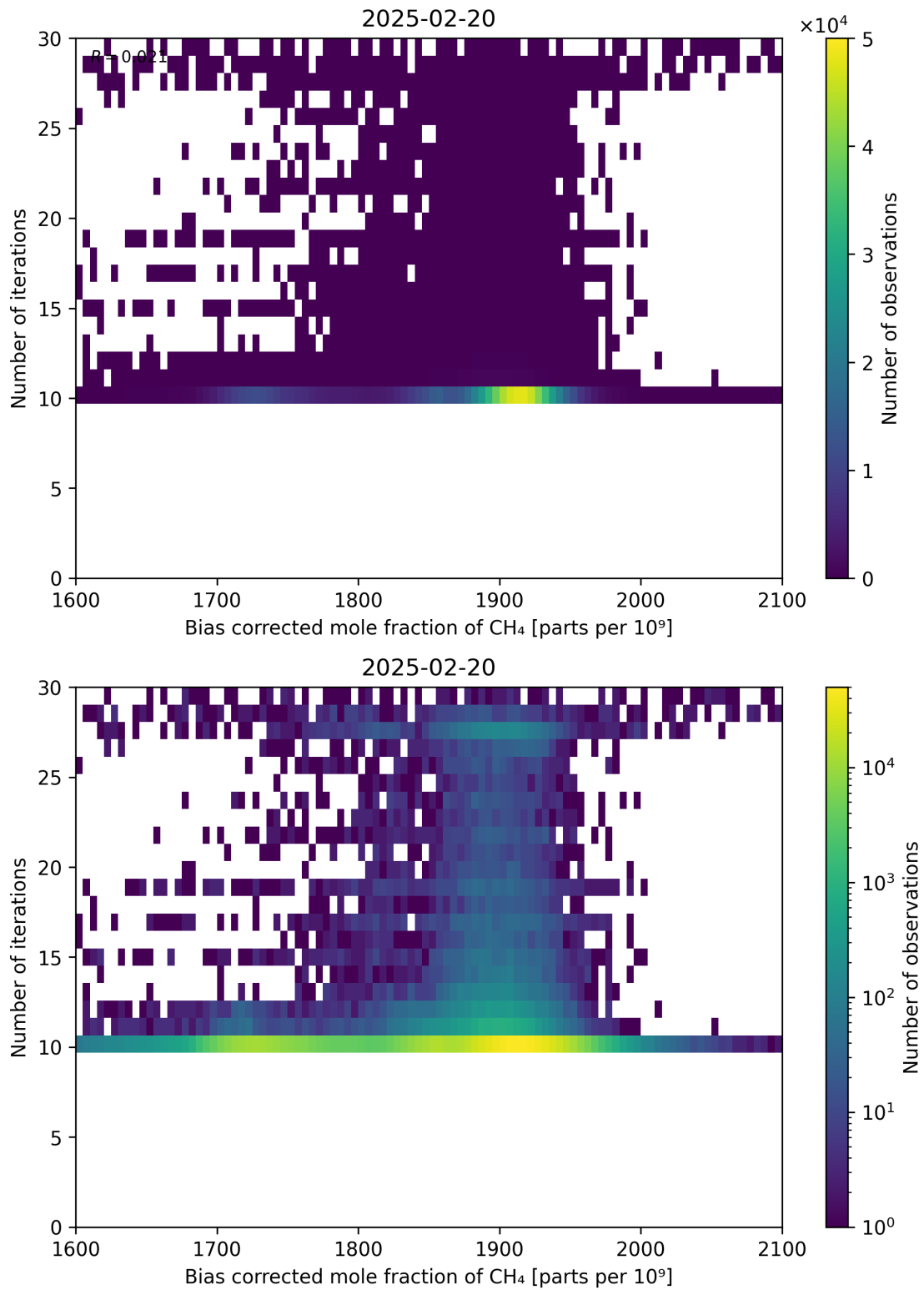
Figure 67: Scatter density plot of “Bias corrected mole fraction of CH 4 ” against “Number of iterations” for 2025-02-19 to 2025-02-21.
