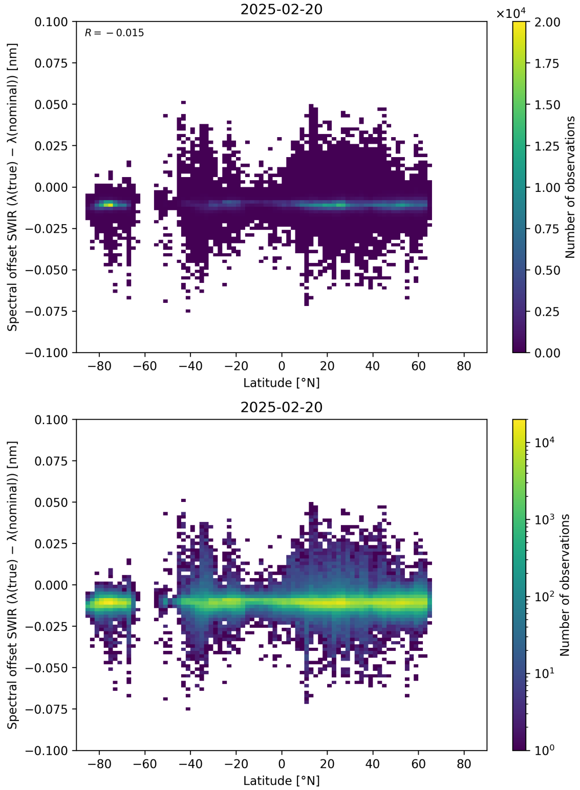
Figure 62: Scatter density plot of “Latitude” against “Spectral offset SWIR ( \lambda_{\text{true}} - \lambda_{\text{nominal}} )” for 2025-02-19 to 2025-02-21.
