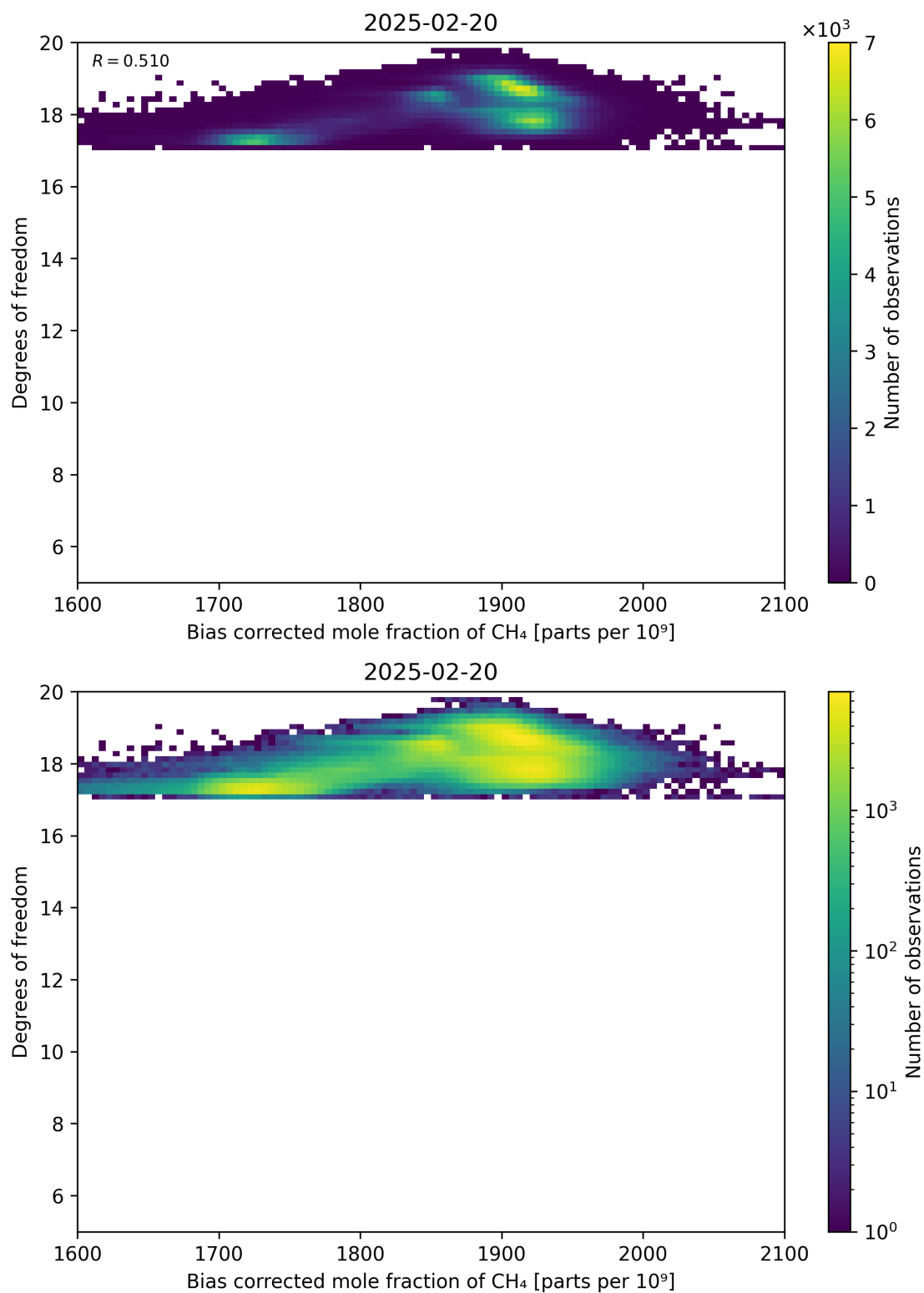
Figure 65: Scatter density plot of “Bias corrected mole fraction of CH 4 ” against “Degrees of freedom” for 2025-02-19 to 2025-02-21.
