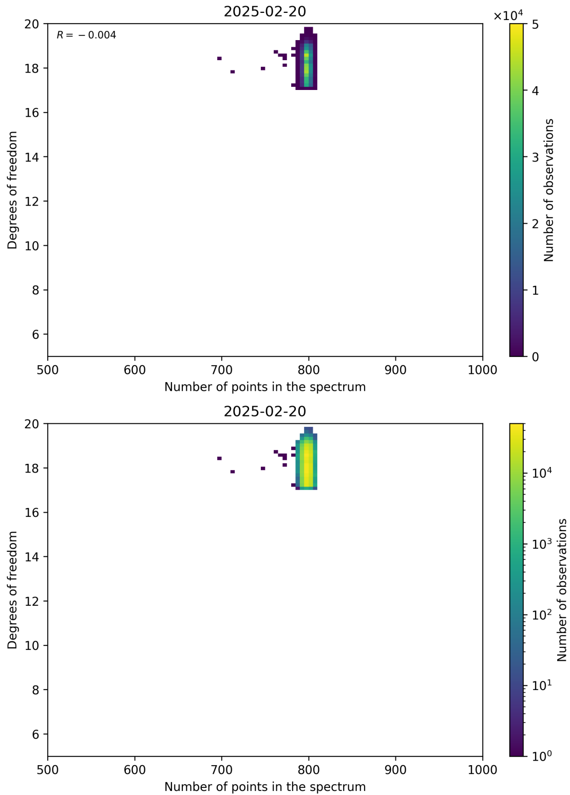
Figure 90: Scatter density plot of “Number of points in the spectrum” against “Degrees of freedom” for 2025-02-19 to 2025-02-21.
