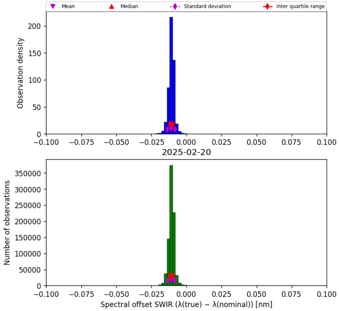
Figure 27: Histogram of “Spectral offset SWIR ( \lambda_{\text{true}} - \lambda_{\text{nominal}} )” for 2025-02-19 to 2025-02-21
