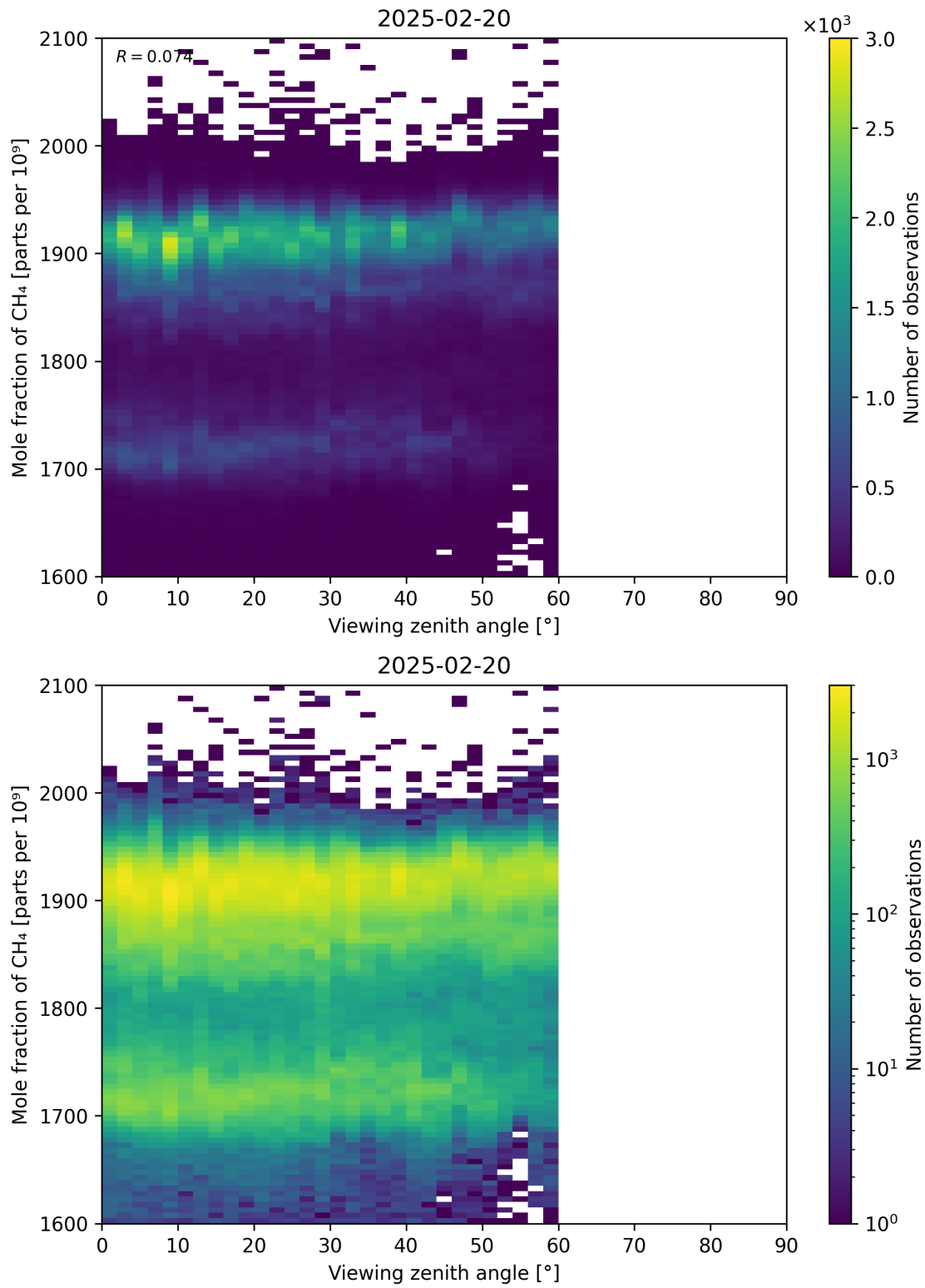
Figure 110: Scatter density plot of “Viewing zenith angle” against “Mole fraction of CH 4 ” for 2025-02-19 to 2025-02-21.
