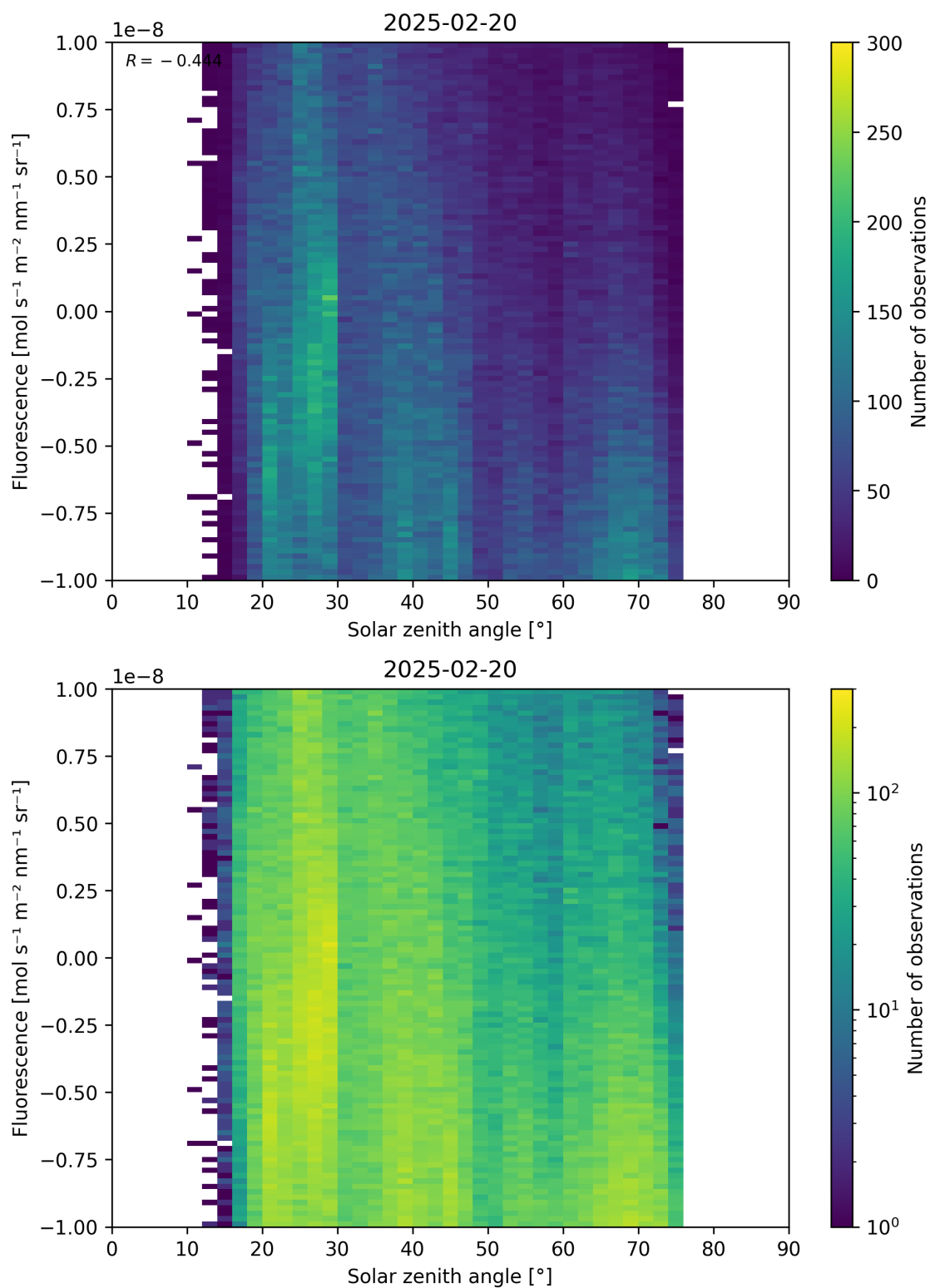
Figure 97: Scatter density plot of “Solar zenith angle” against “Fluorescence” for 2025-02-19 to 2025-02-21.
