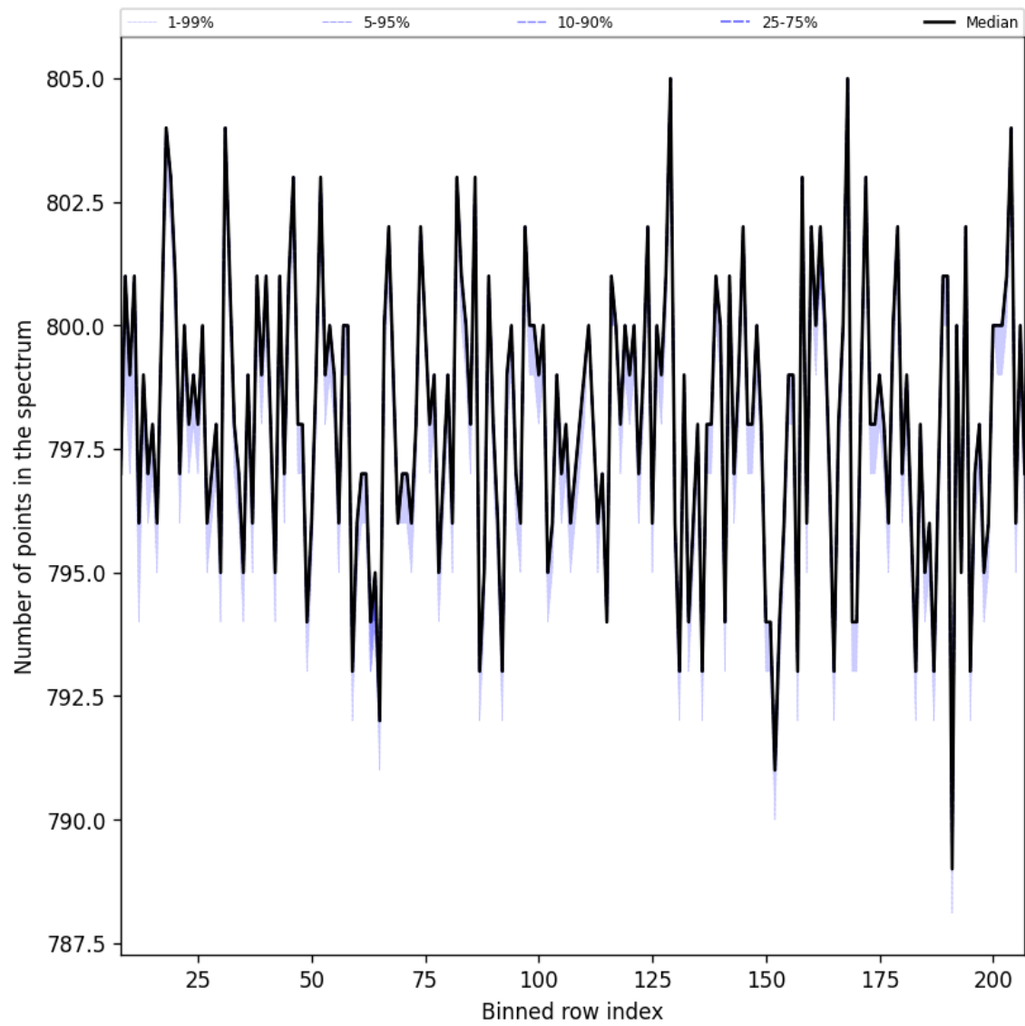
Figure 37: Along track statistics of “Number of points in the spectrum” for 2025-02-19 to 2025-02-21
