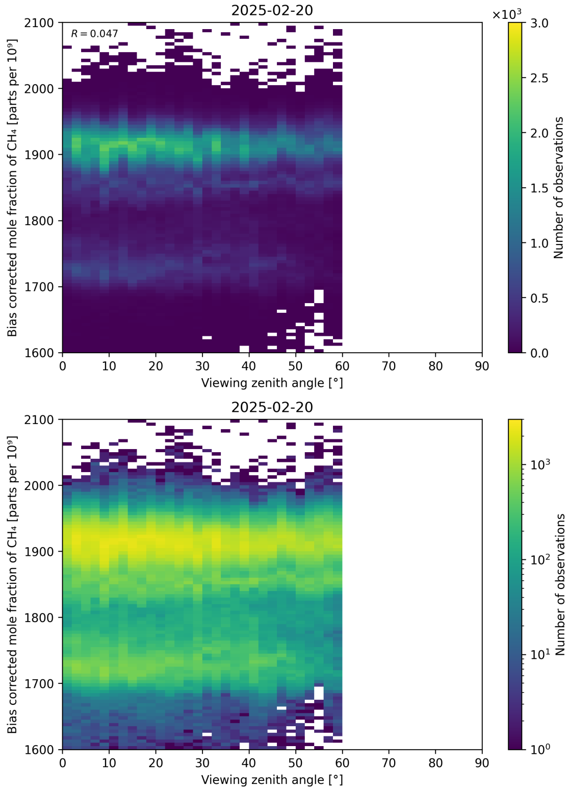
Figure 111: Scatter density plot of “Viewing zenith angle” against “Bias corrected mole fraction of CH 4 ” for 2025-02-19 to 2025-02-21.
