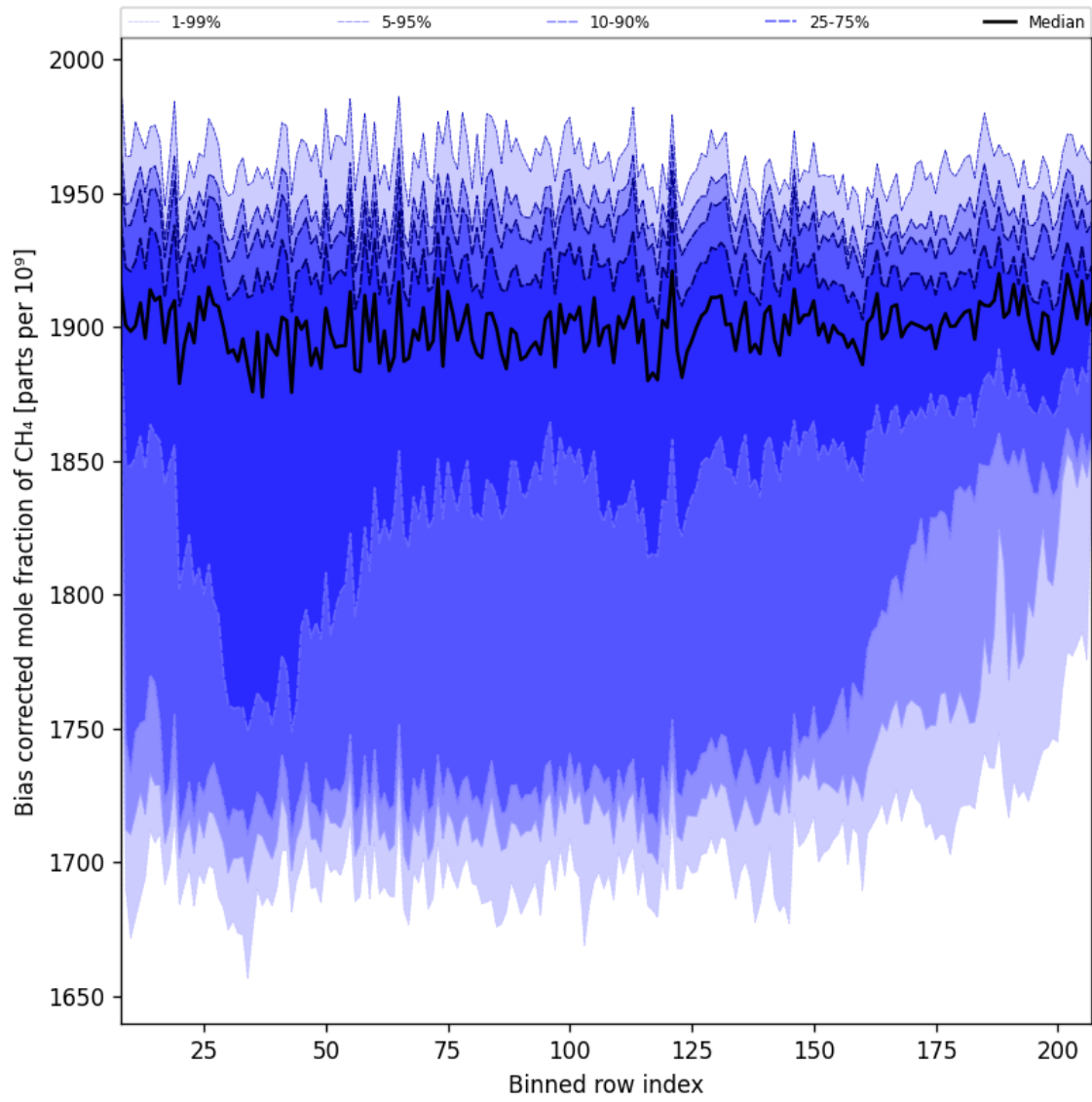
Figure 36: Along track statistics of “Bias corrected mole fraction of CH 4 ” for 2025-02-19 to 2025-02-21
