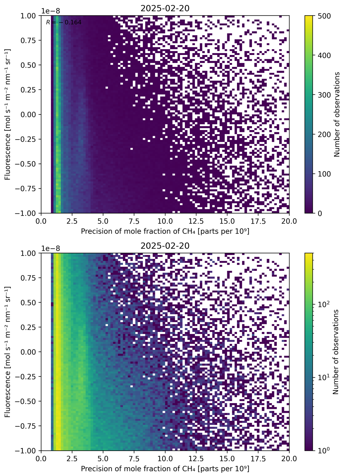
Figure 81: Scatter density plot of “Precision of mole fraction of \text{CH}_4 ” against “Fluorescence” for 2025-02-19 to 2025-02-21.
