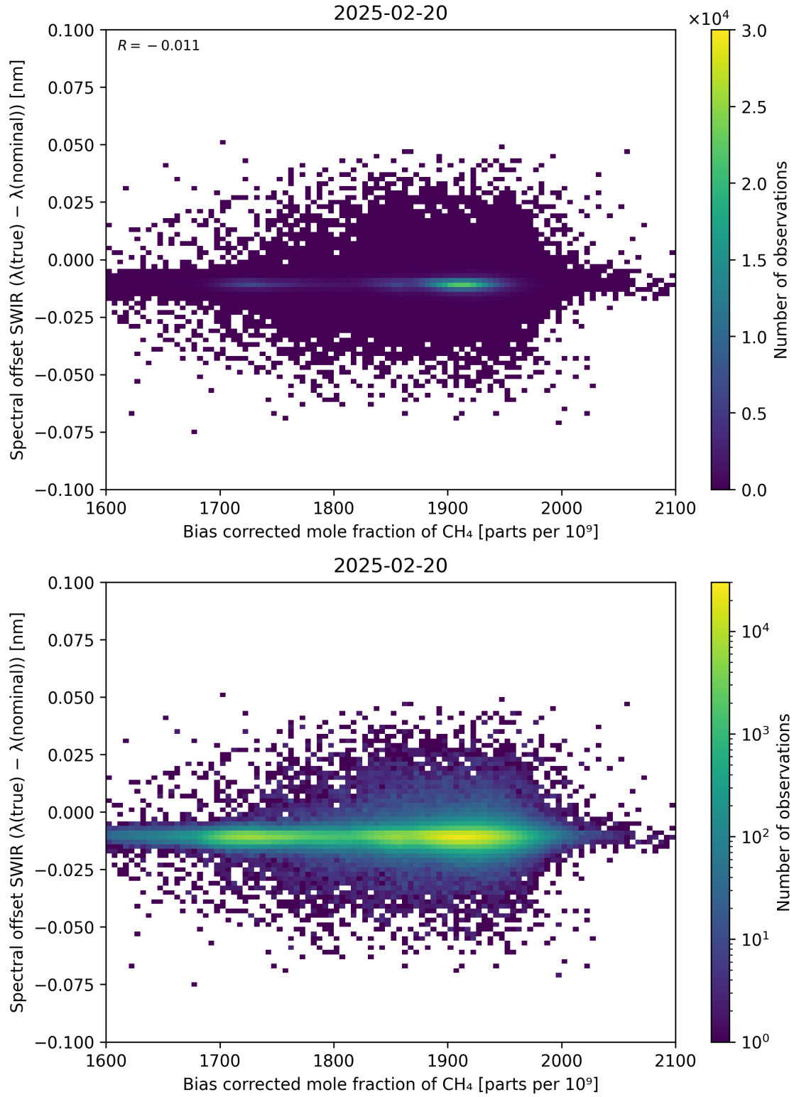
Figure 69: Scatter density plot of “Bias corrected mole fraction of \text{CH}_4 ” against “Spectral offset SWIR ( \lambda_{\text{true}} - \lambda_{\text{nominal}} )” for 2025-02-19 to 2025-02-21.
