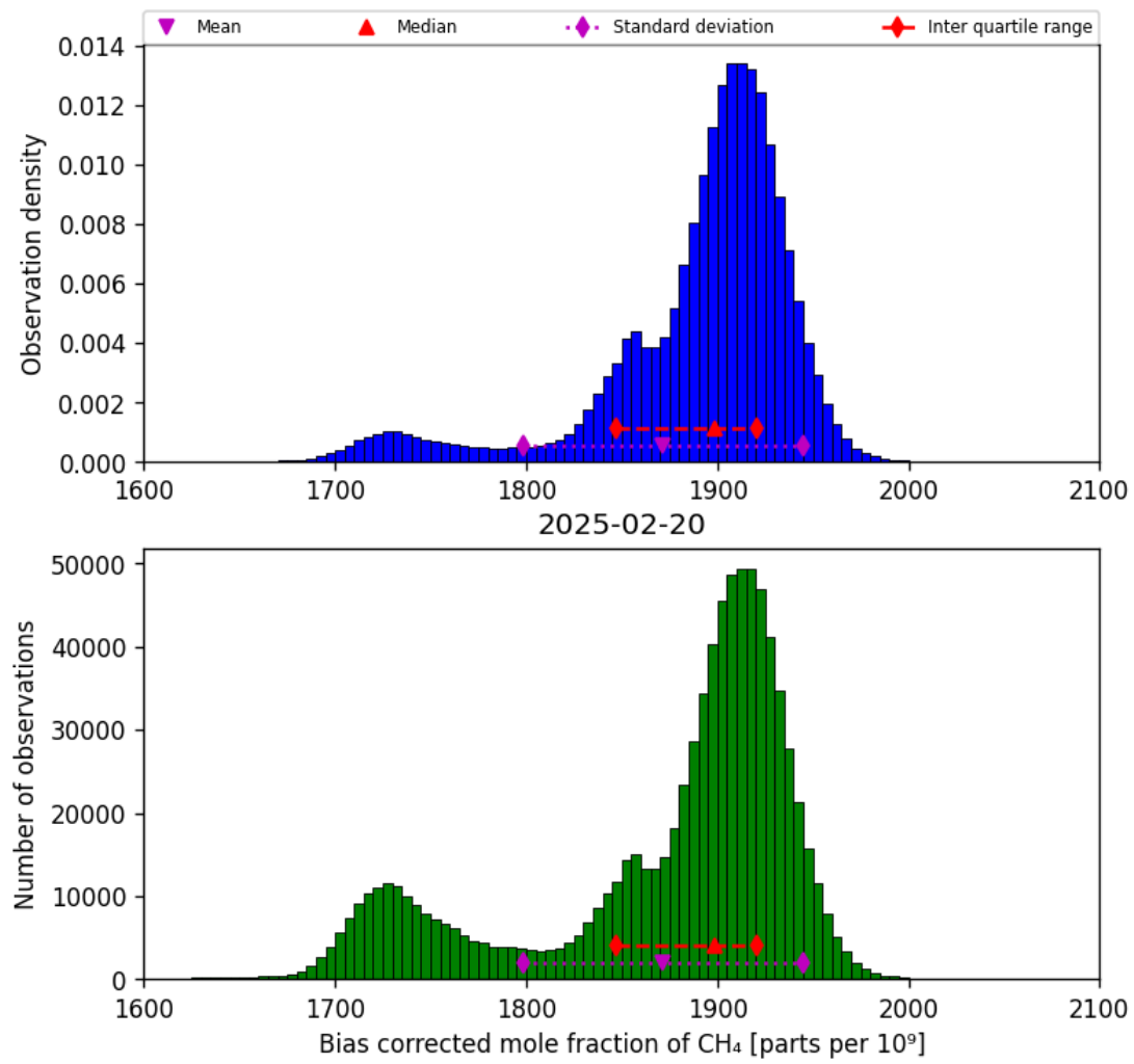
Figure 25: Histogram of “Bias corrected mole fraction of CH 4 ” for 2025-02-19 to 2025-02-21
