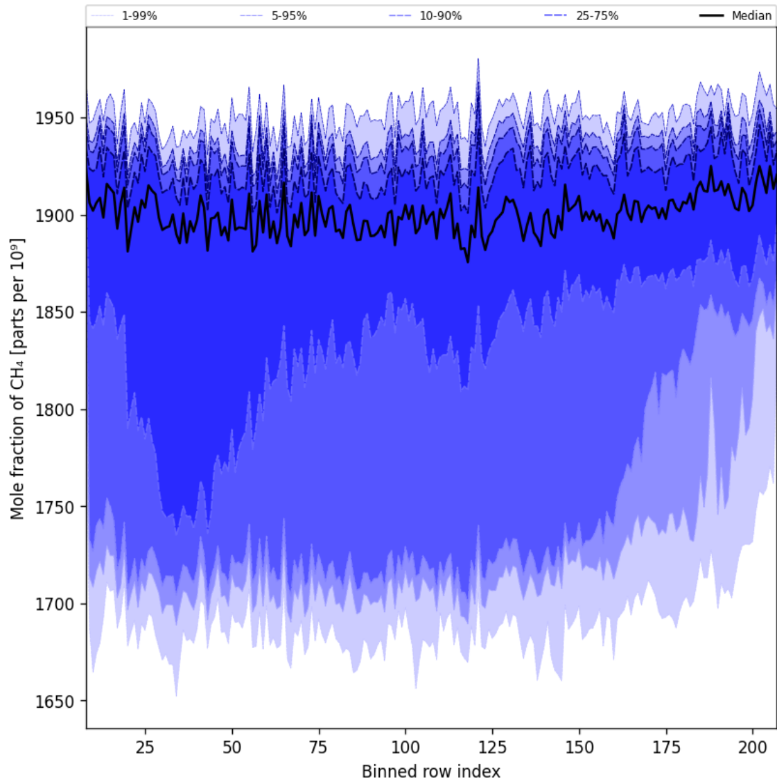
Figure 34: Along track statistics of “Mole fraction of CH 4 ” for 2025-02-19 to 2025-02-21
