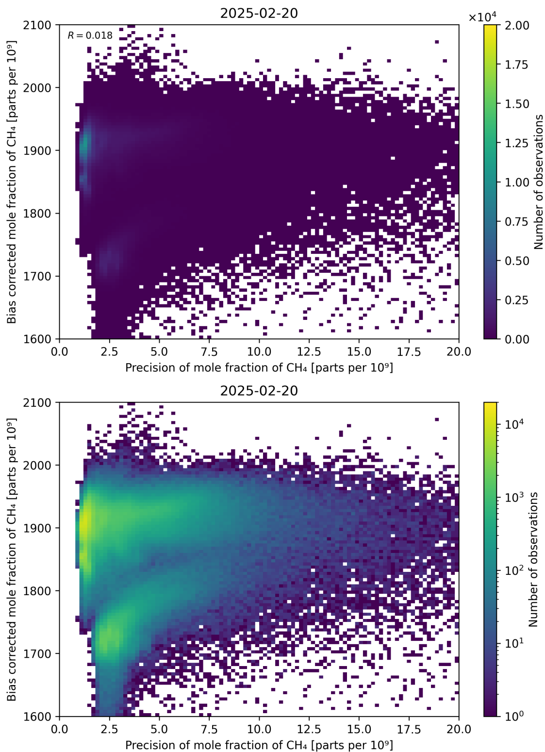
Figure 82: Scatter density plot of “Precision of mole fraction of \text{CH}_4 ” against “Bias corrected mole fraction of \text{CH}_4 ” for 2025-02-19 to 2025-02-21.
