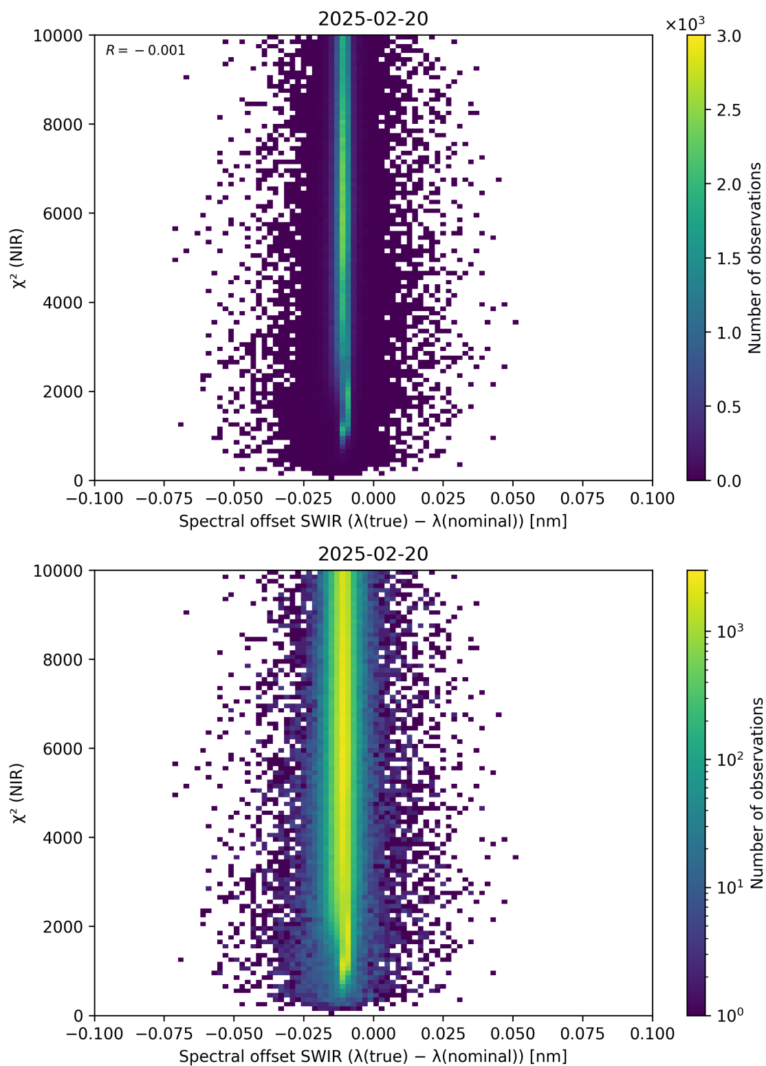
Figure 117: Scatter density plot of “Spectral offset SWIR ( \lambda_{\text{true}} - \lambda_{\text{nominal}} )” against “ \chi^2 (NIR)” for 2025-02-19 to 2025-02-21.
