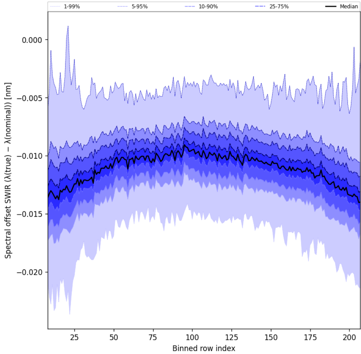
Figure 38: Along track statistics of “Spectral offset SWIR ( \lambda_{\text{true}} - \lambda_{\text{nominal}} )” for 2025-02-19 to 2025-02-21
