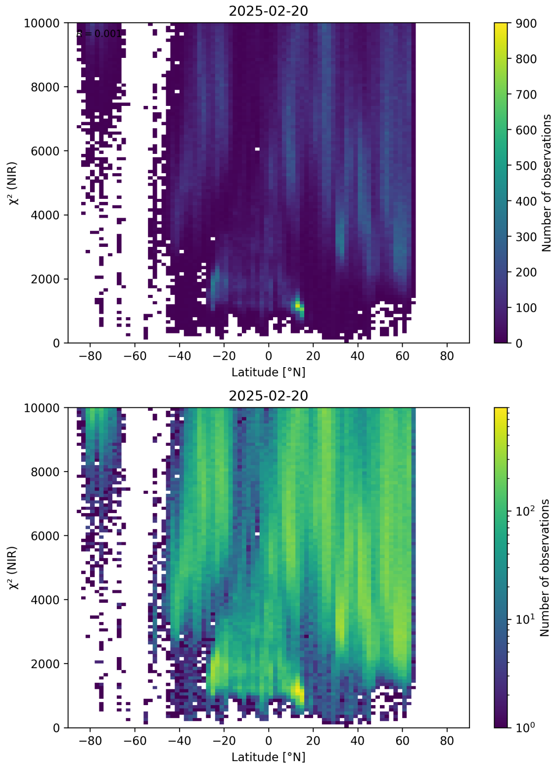
Figure 53: Scatter density plot of “Latitude” against “ \chi^2 (NIR)” for 2025-02-19 to 2025-02-21.
