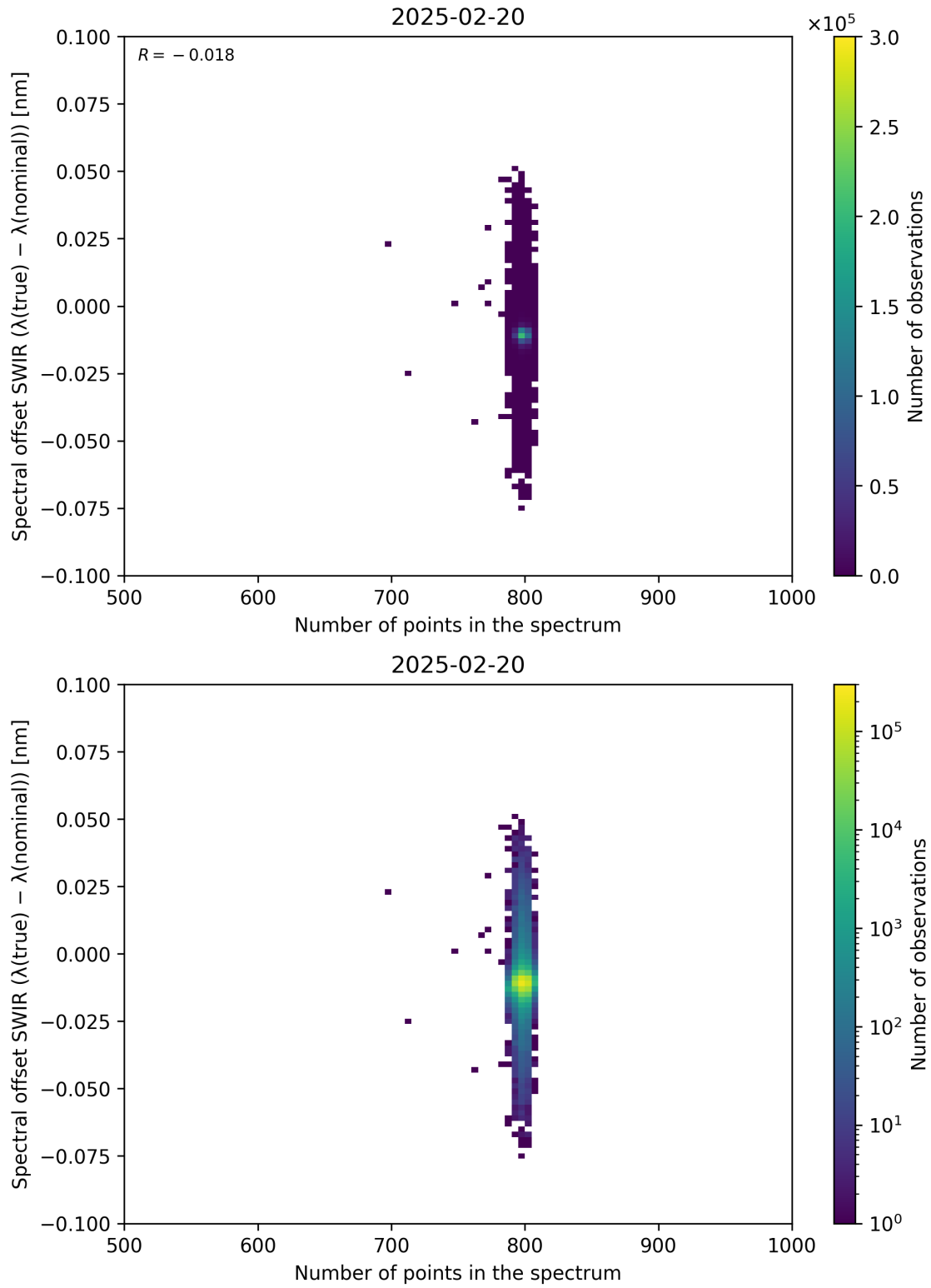
Figure 93: Scatter density plot of “Number of points in the spectrum” against “Spectral offset SWIR ( \lambda_{\text{true}} - \lambda_{\text{nominal}} )” for 2025-02-19 to 2025-02-21.
