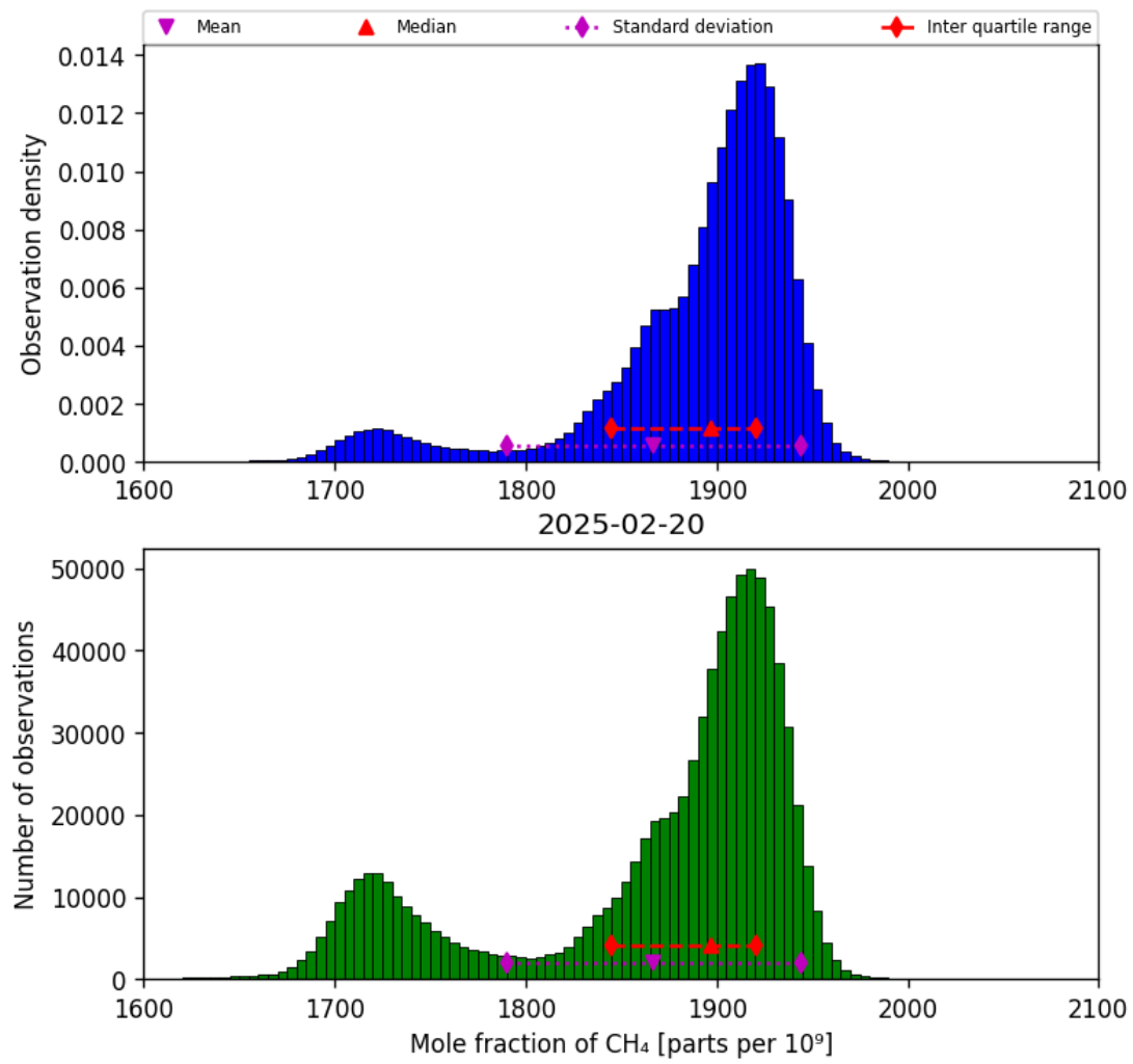
Figure 23: Histogram of “Mole fraction of CH 4 ” for 2025-02-19 to 2025-02-21
