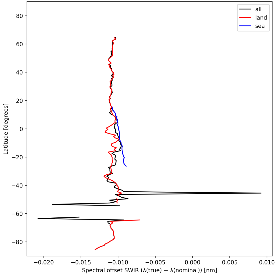
Figure 16: Zonal average of “Spectral offset SWIR ( \lambda_{\text{true}} - \lambda_{\text{nominal}} )” for 2025-02-19 to 2025-02-21.
