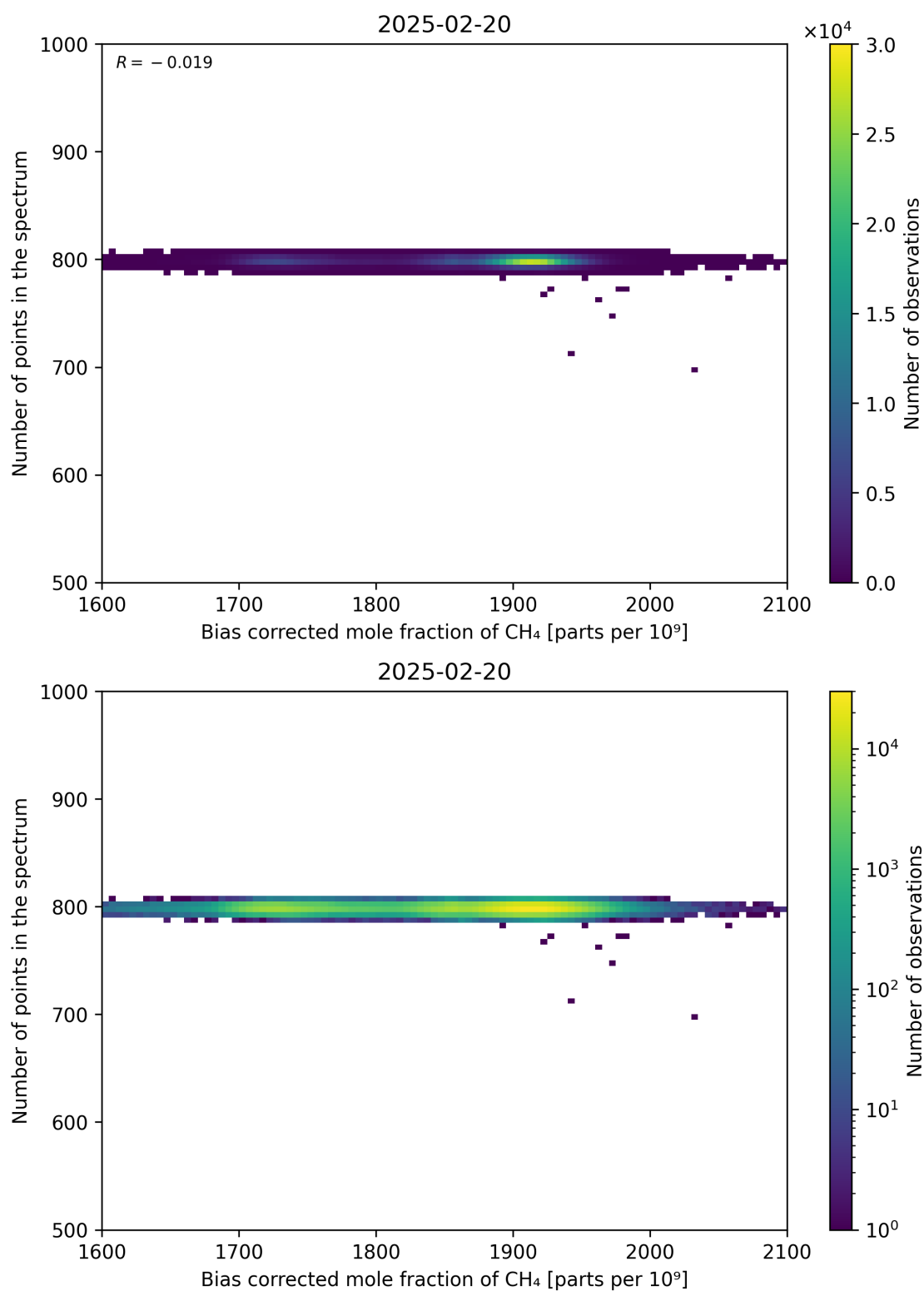
Figure 68: Scatter density plot of “Bias corrected mole fraction of CH 4 ” against “Number of points in the spectrum” for 2025-02-19 to 2025-02-21.
