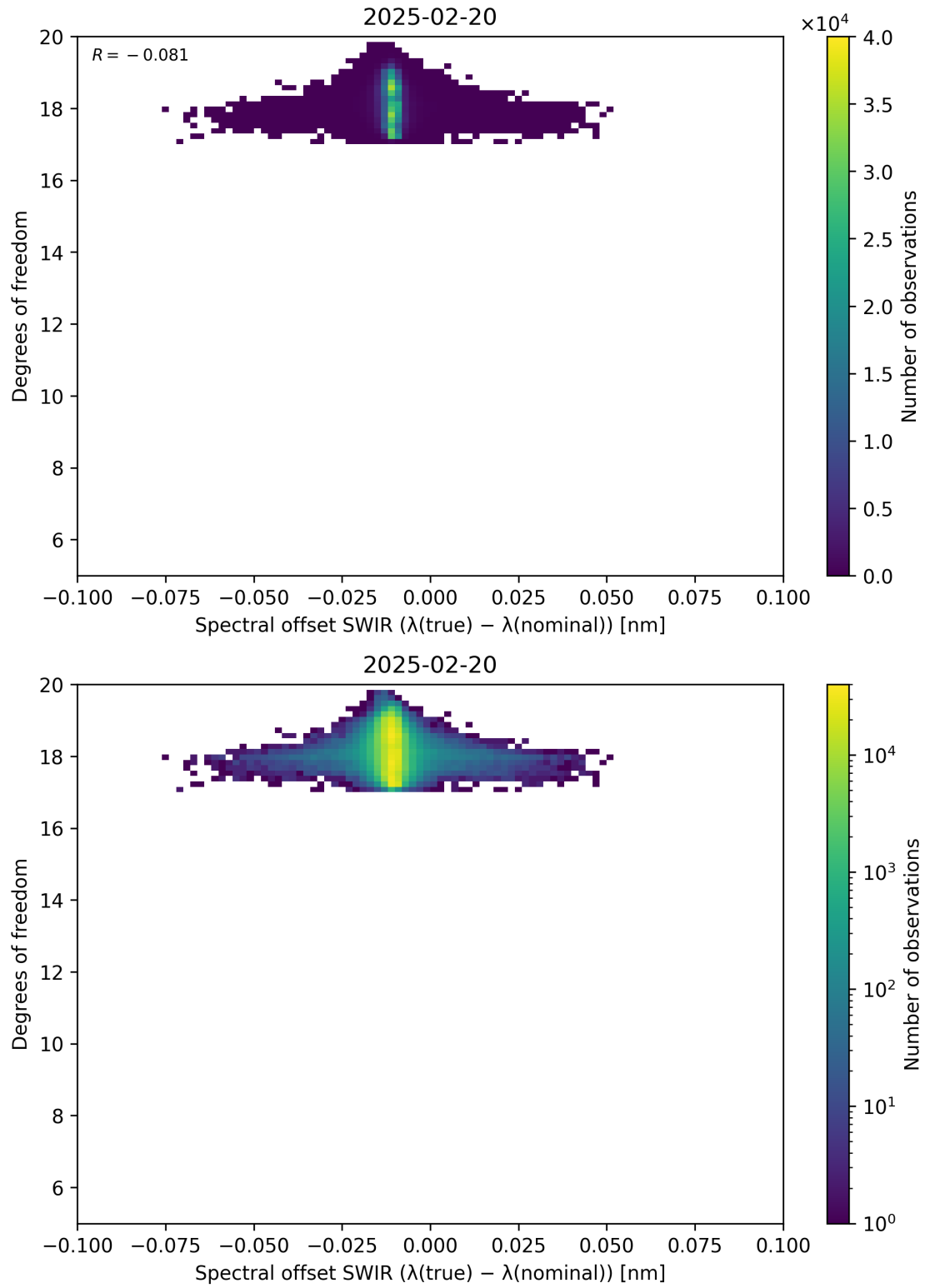
Figure 119: Scatter density plot of “Spectral offset SWIR ( \lambda_{\text{true}} - \lambda_{\text{nominal}} )” against “Degrees of freedom” for 2025-02-19 to 2025-02-21.
