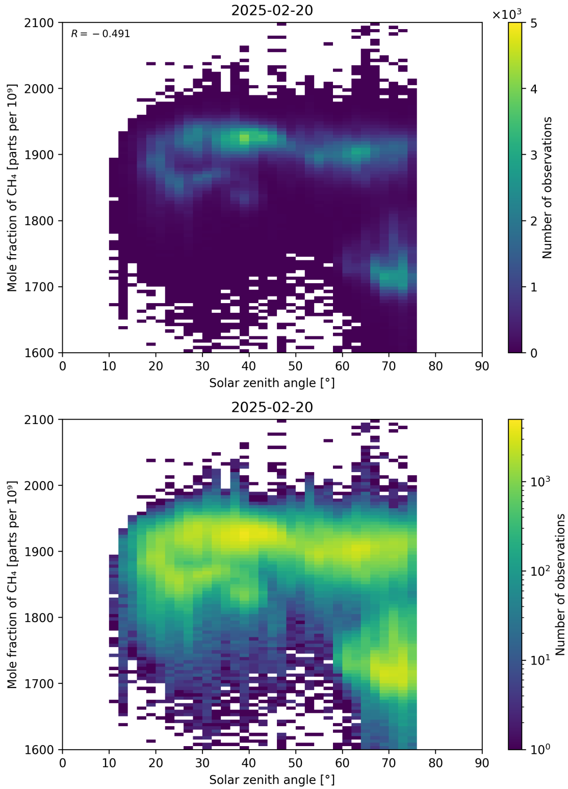
Figure 99: Scatter density plot of “Solar zenith angle” against “Mole fraction of \text{CH}_4 ” for 2025-02-19 to 2025-02-21.
