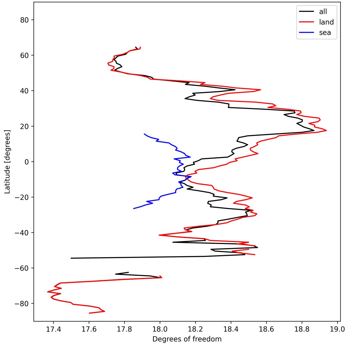
Figure 19: Zonal average of “Degrees of freedom” for 2025-02-19 to 2025-02-21.
