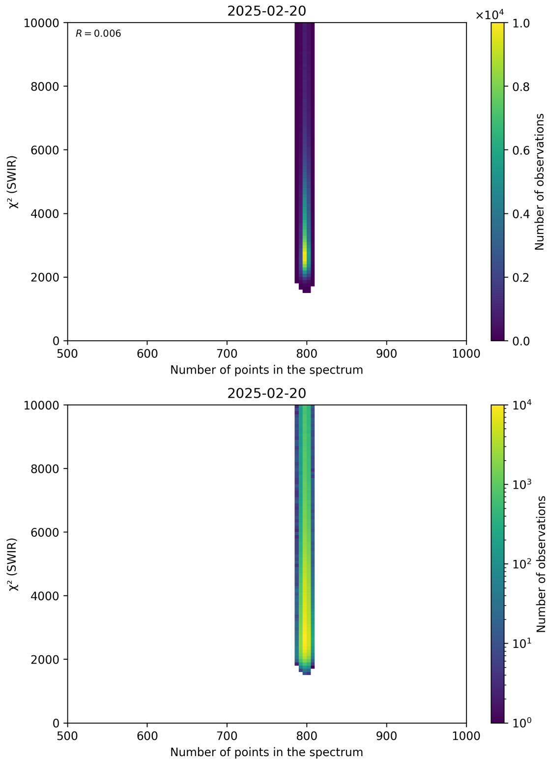
Figure 89: Scatter density plot of “Number of points in the spectrum” against “ \chi^2 (SWIR)” for 2025-02-19 to 2025-02-21.
