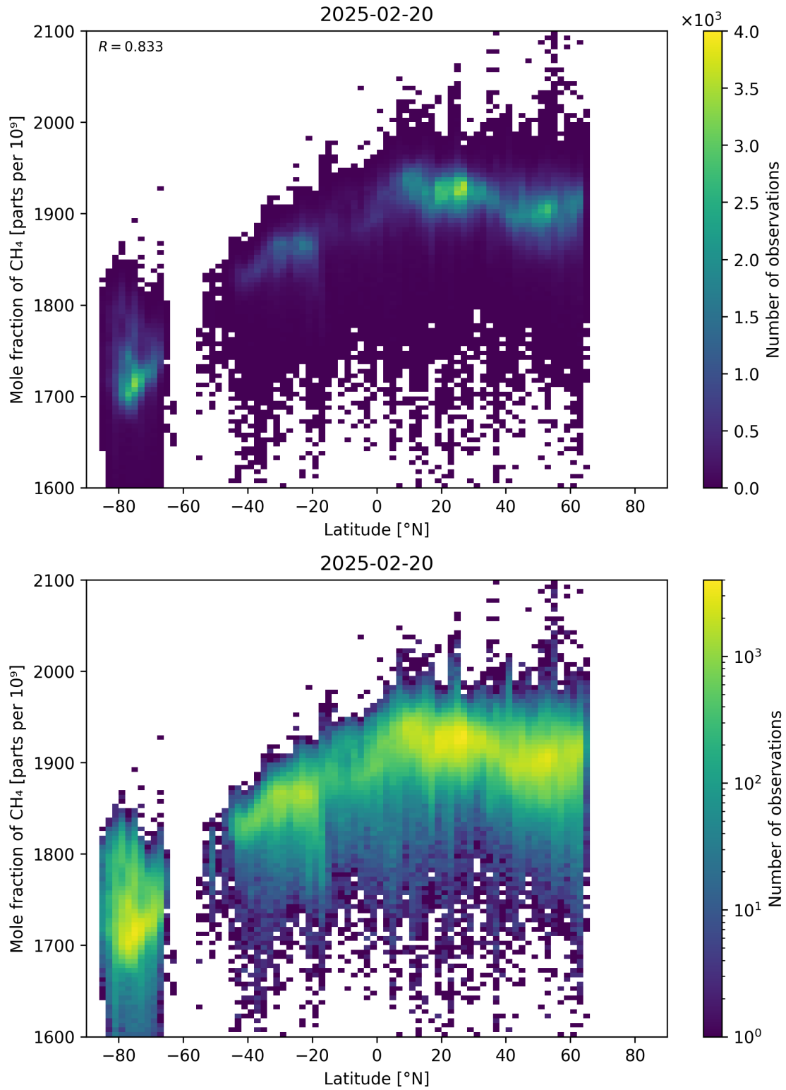
Figure 57: Scatter density plot of “Latitude” against “Mole fraction of CH 4 ” for 2025-02-19 to 2025-02-21.
