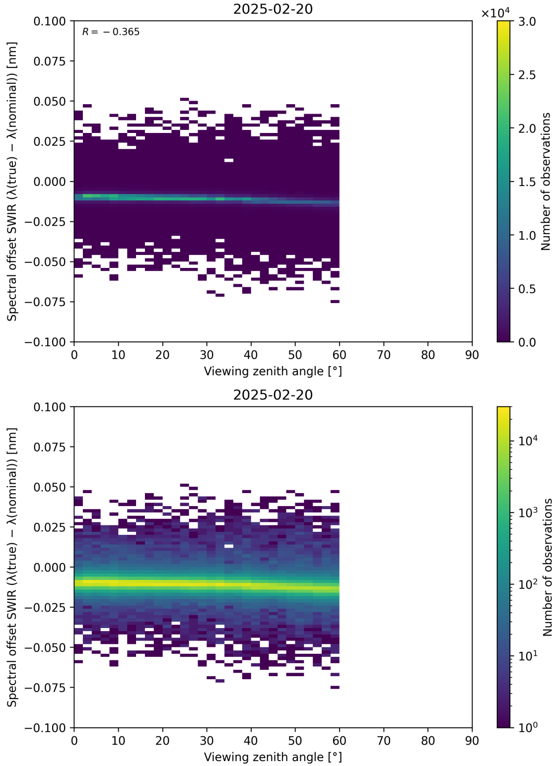
Figure 116: Scatter density plot of “Viewing zenith angle” against “Spectral offset SWIR ( \lambda_{\text{true}} - \lambda_{\text{nominal}} )” for 2025-02-19 to 2025-02-21.
