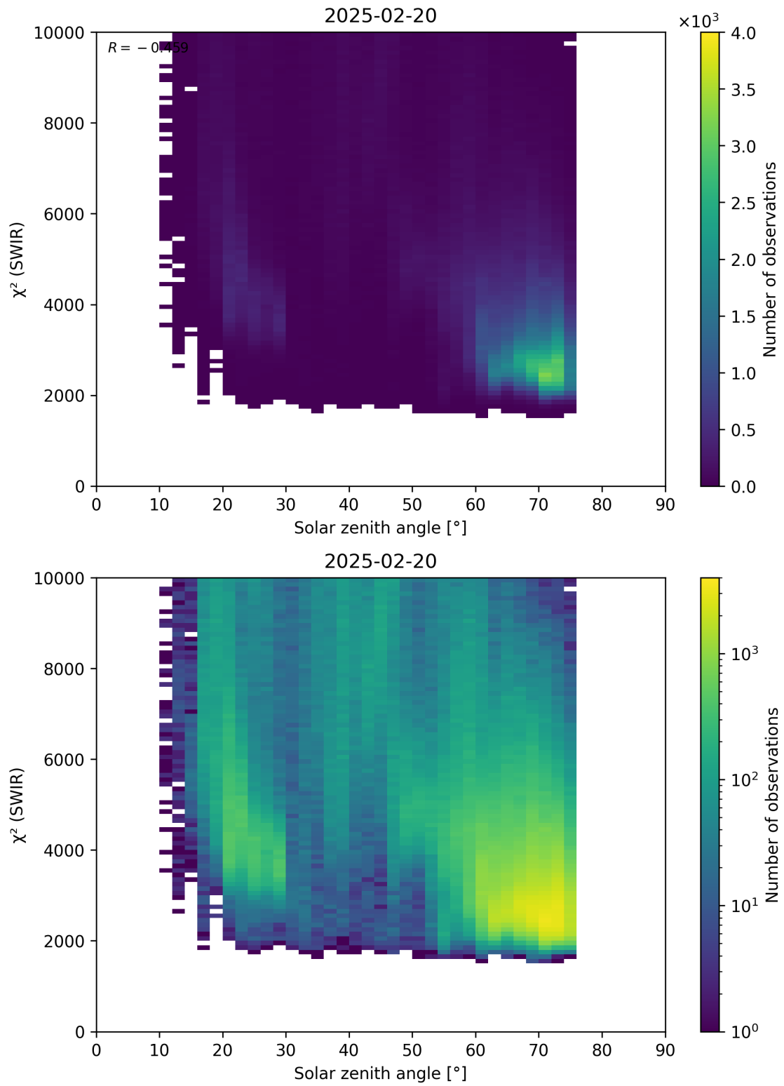
Figure 95: Scatter density plot of “Solar zenith angle” against “ \chi^2 (SWIR)” for 2025-02-19 to 2025-02-21.
