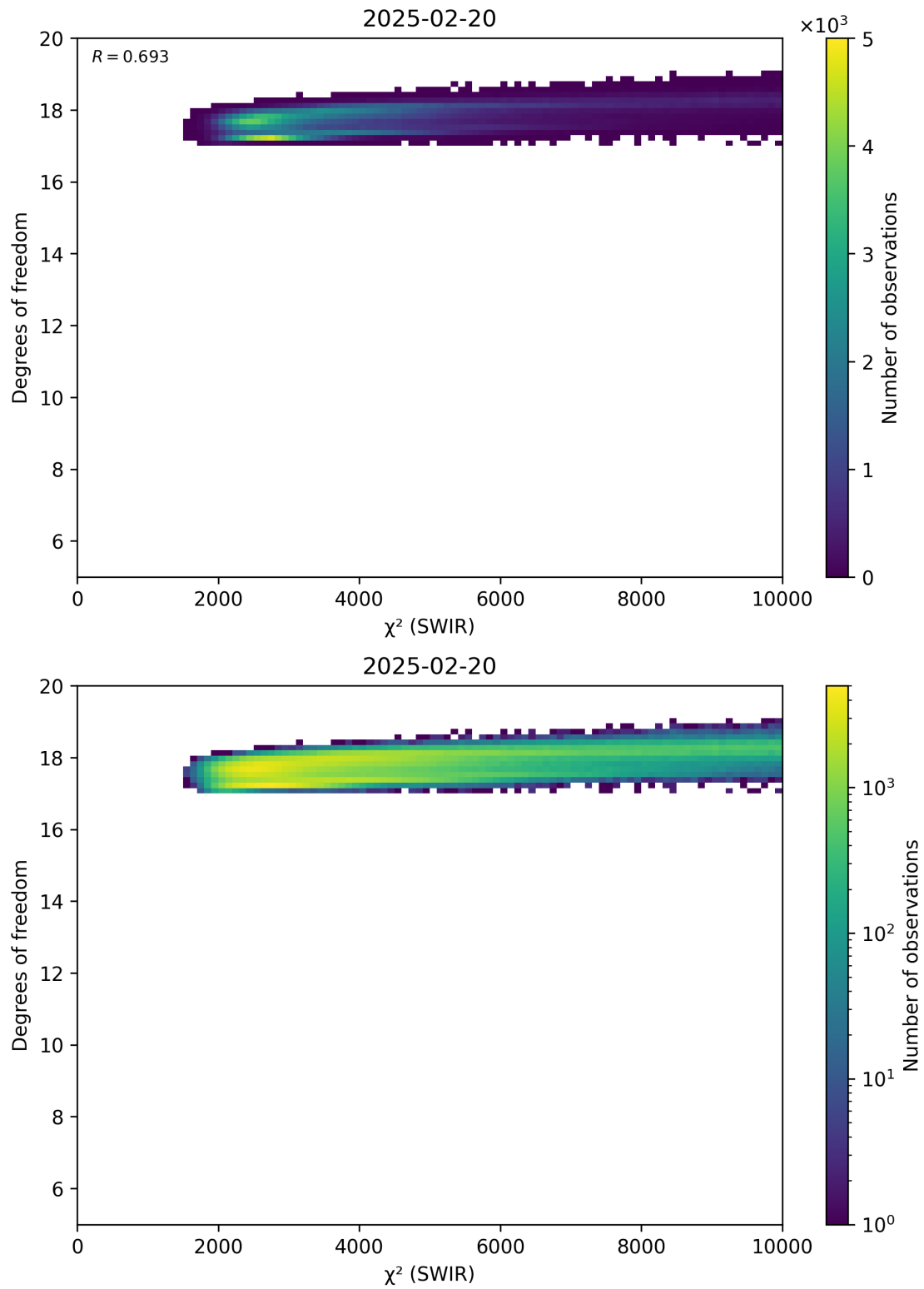
Figure 48: Scatter density plot of “ \chi^2 (SWIR)” against “Degrees of freedom” for 2025-02-19 to 2025-02-21.
