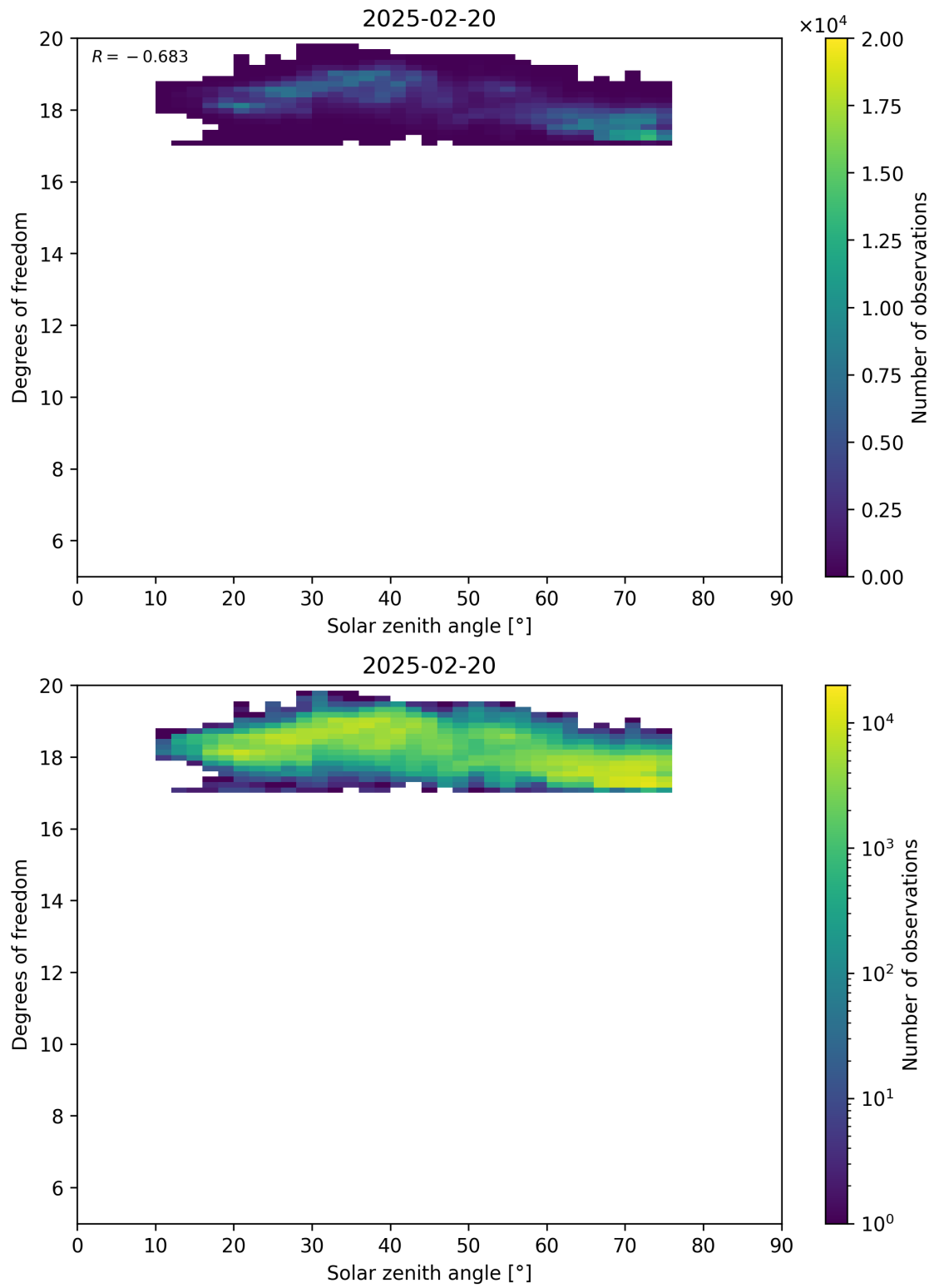
Figure 96: Scatter density plot of “Solar zenith angle” against “Degrees of freedom” for 2025-02-19 to 2025-02-21.
