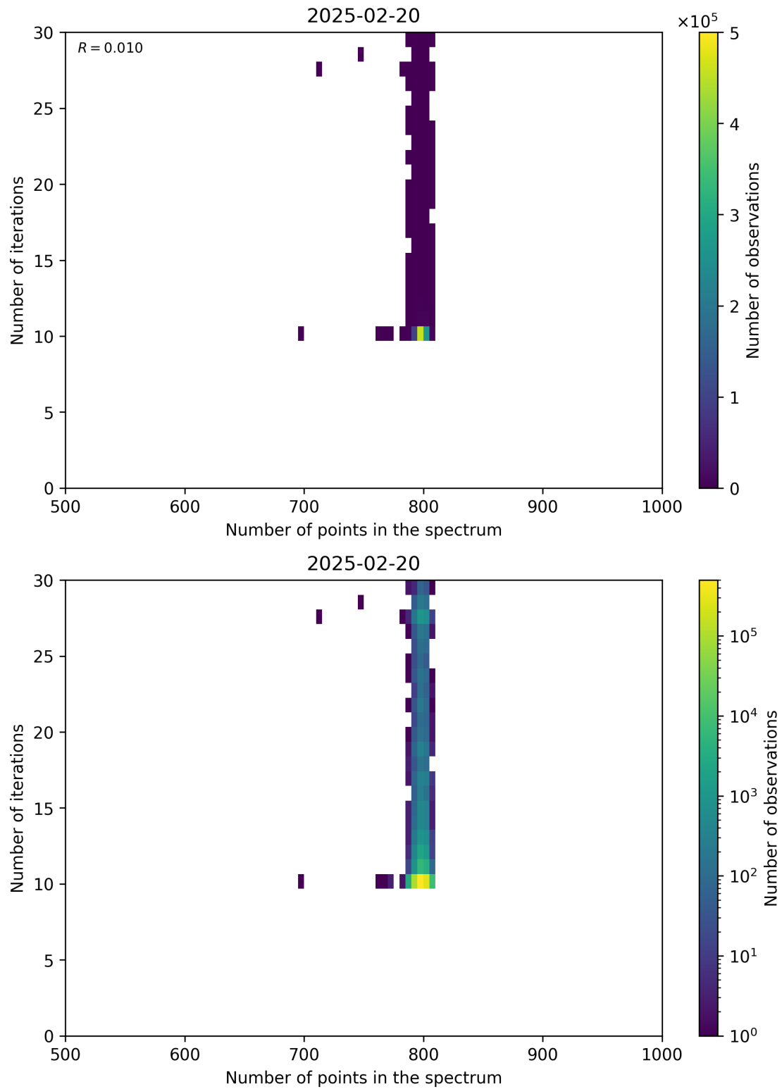
Figure 92: Scatter density plot of “Number of points in the spectrum” against “Number of iterations” for 2025-02-19 to 2025-02-21.
