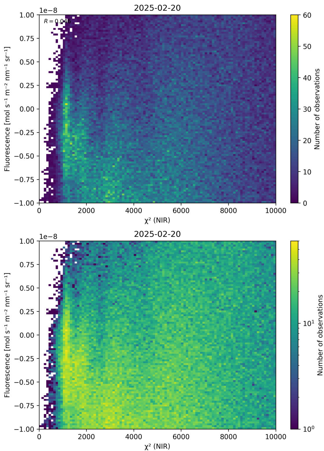
Figure 45: Scatter density plot of “ \chi^2 (NIR)” against “Fluorescence” for 2025-02-19 to 2025-02-21.
