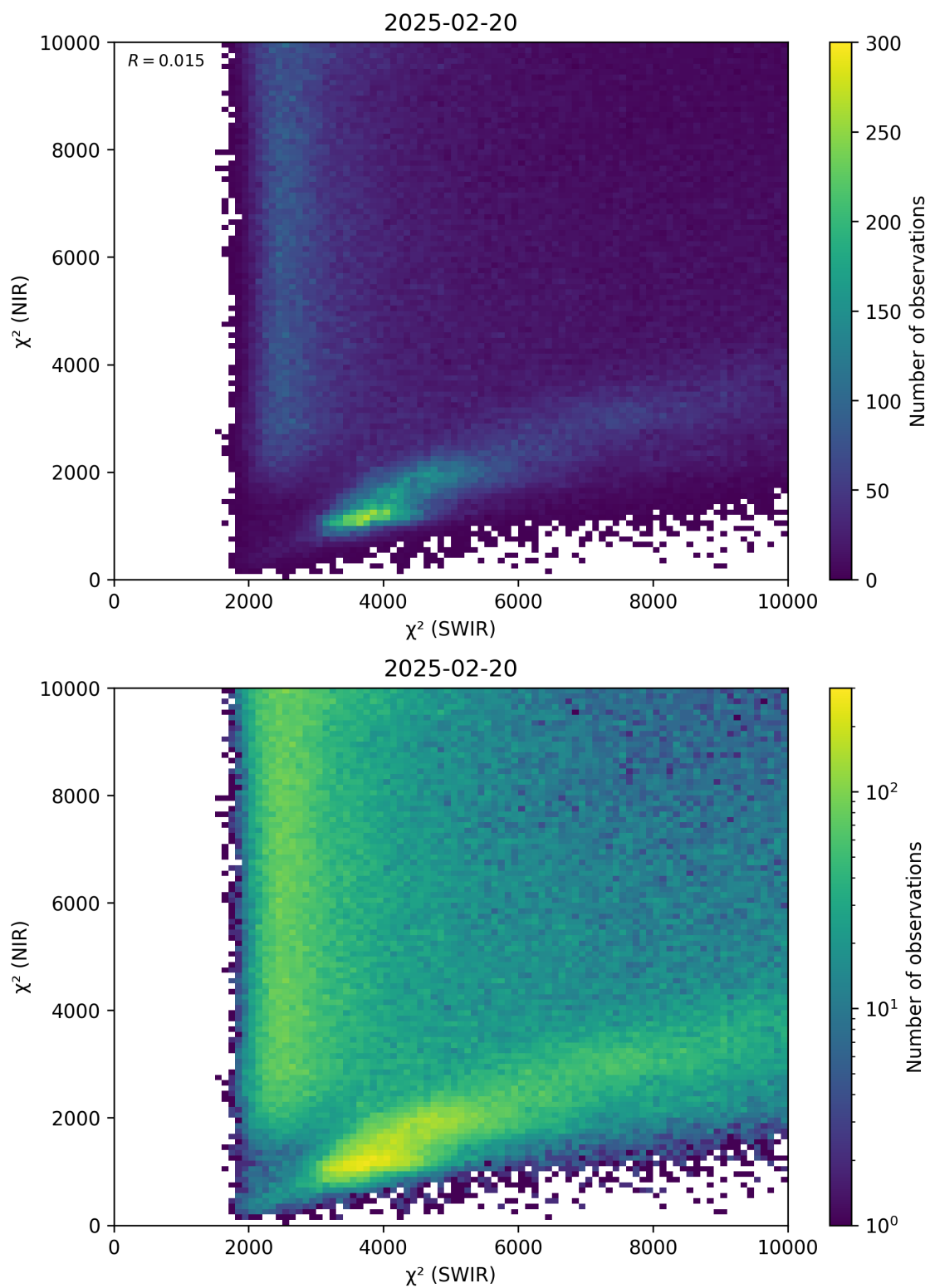
Figure 47: Scatter density plot of “ \chi^2 (SWIR)” against “ \chi^2 (NIR)” for 2025-02-19 to 2025-02-21.
