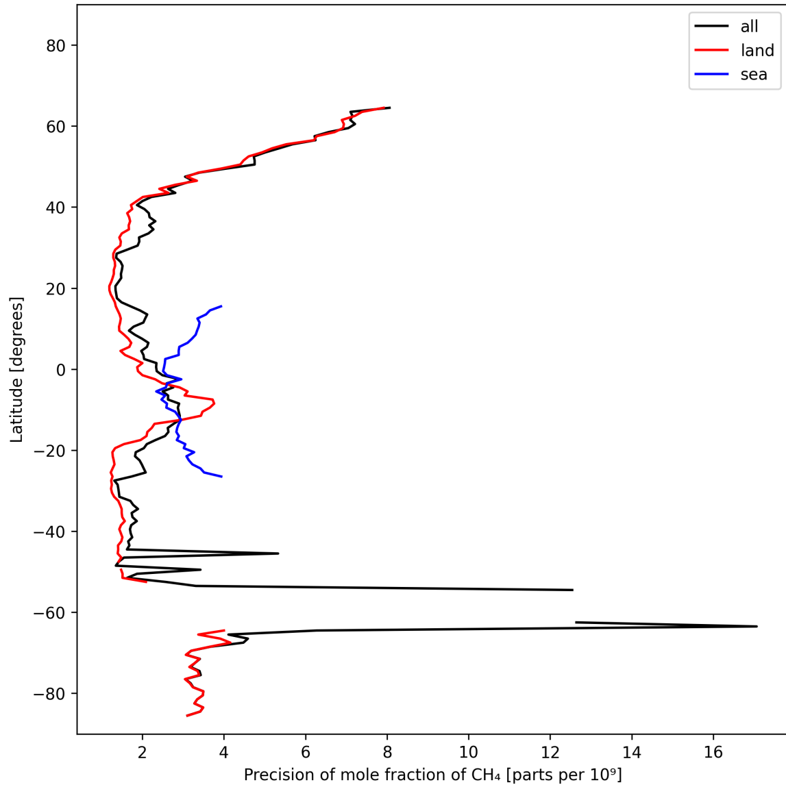
Figure 13: Zonal average of “Precision of mole fraction of CH 4 ” for 2025-02-19 to 2025-02-21.
