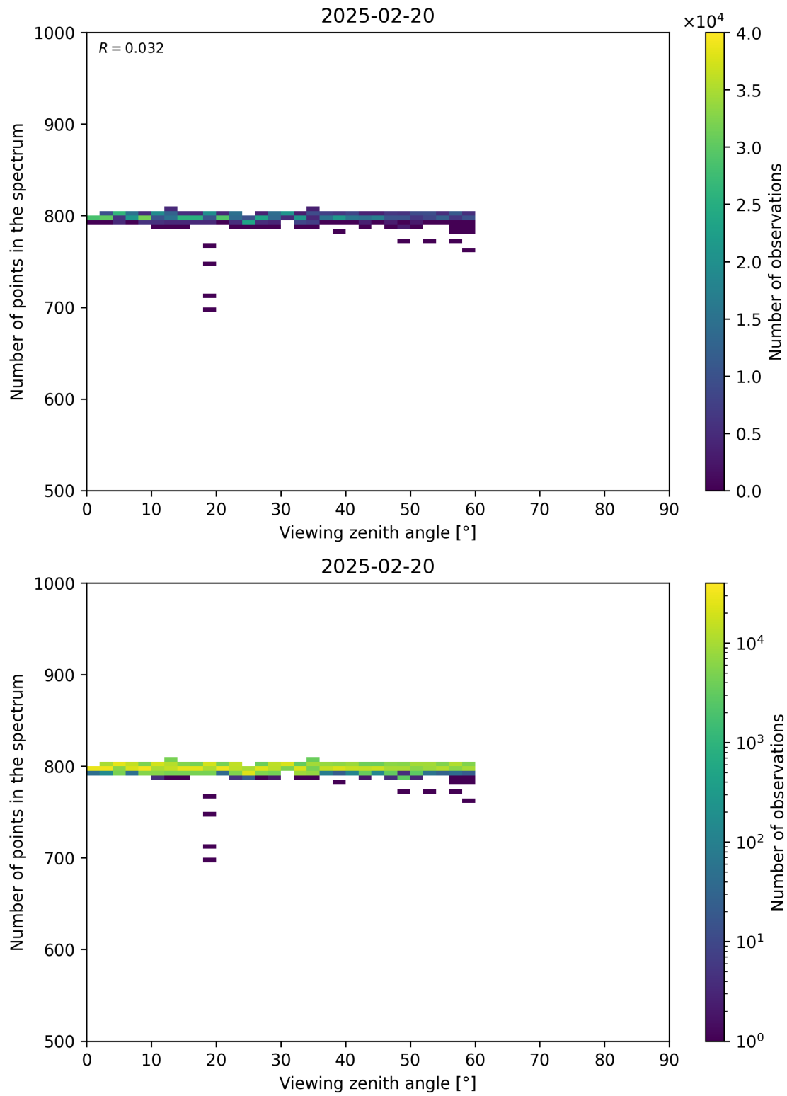
Figure 114: Scatter density plot of “Viewing zenith angle” against “Number of points in the spectrum” for 2025-02-19 to 2025-02-21.
