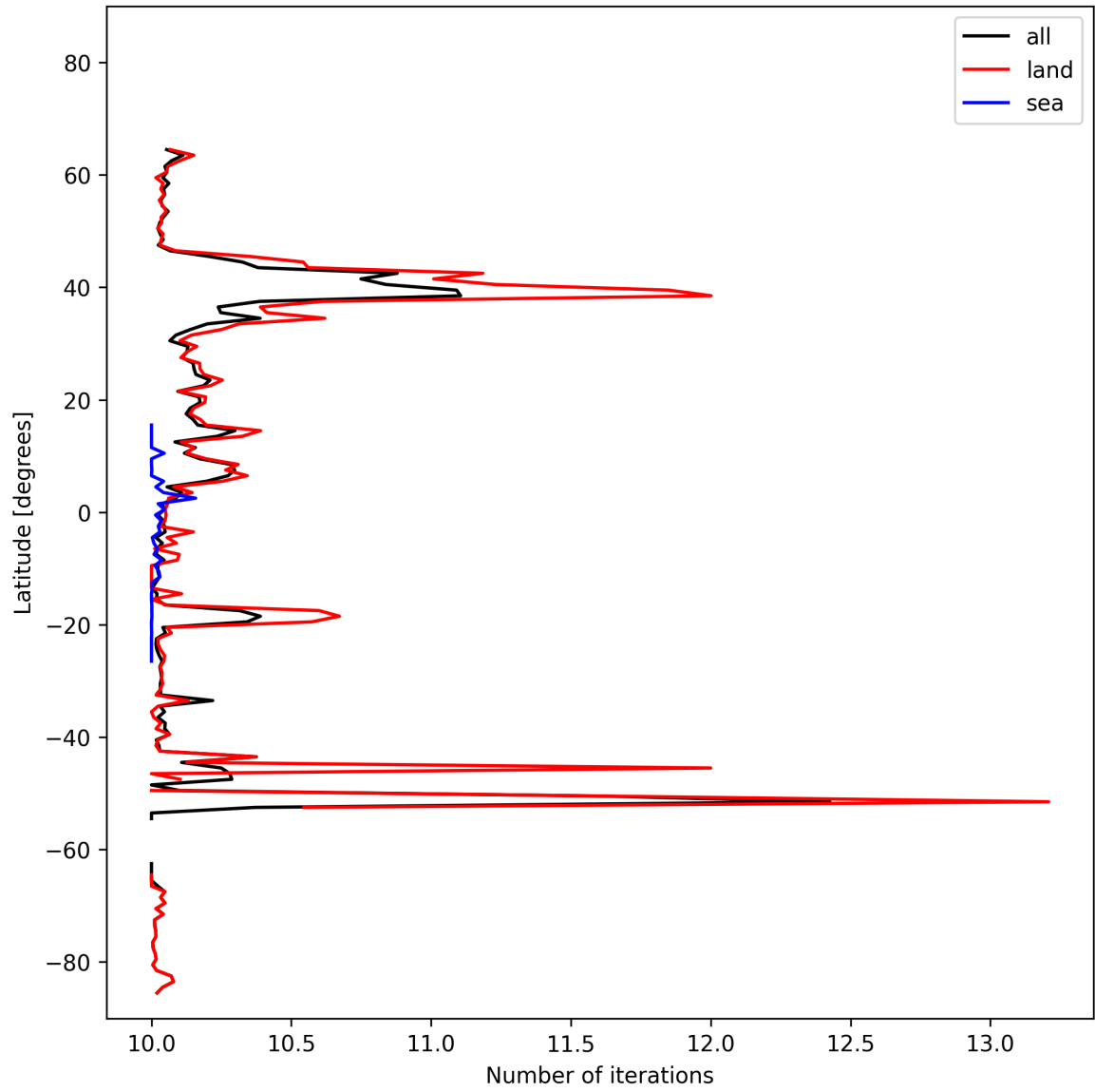
Figure 20: Zonal average of “Number of iterations” for 2025-02-19 to 2025-02-21.
