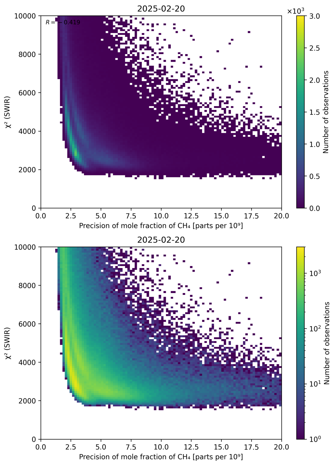
Figure 79: Scatter density plot of “Precision of mole fraction of \text{CH}_4 ” against “ \chi^2 (SWIR)” for 2025-02-19 to 2025-02-21.
