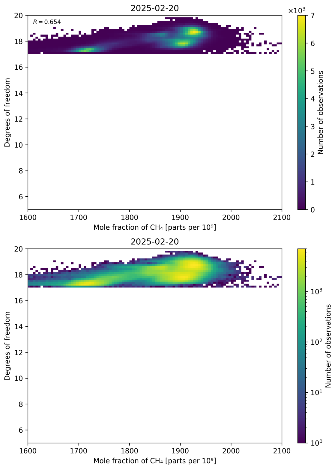
Figure 72: Scatter density plot of “Mole fraction of CH 4 ” against “Degrees of freedom” for 2025-02-19 to 2025-02-21.
