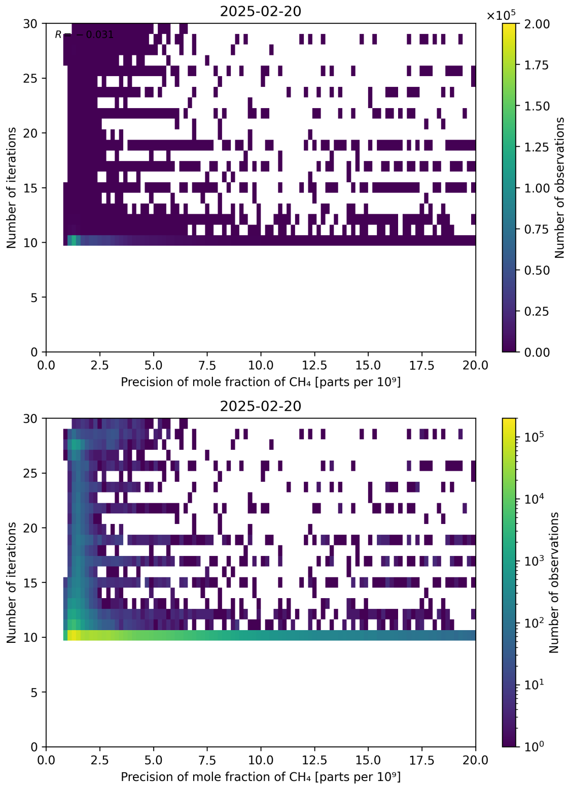
Figure 83: Scatter density plot of “Precision of mole fraction of CH 4 ” against “Number of iterations” for 2025-02-19 to 2025-02-21.
