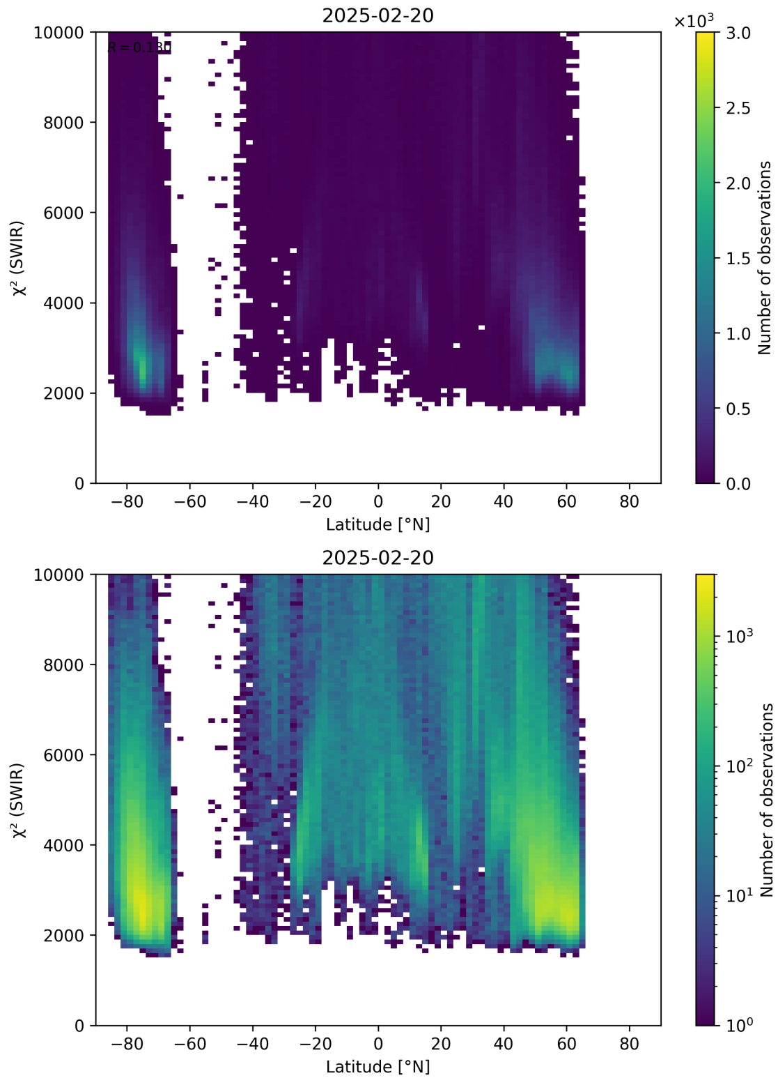
Figure 54: Scatter density plot of “Latitude” against “ \chi^2 (SWIR)” for 2025-02-19 to 2025-02-21.
