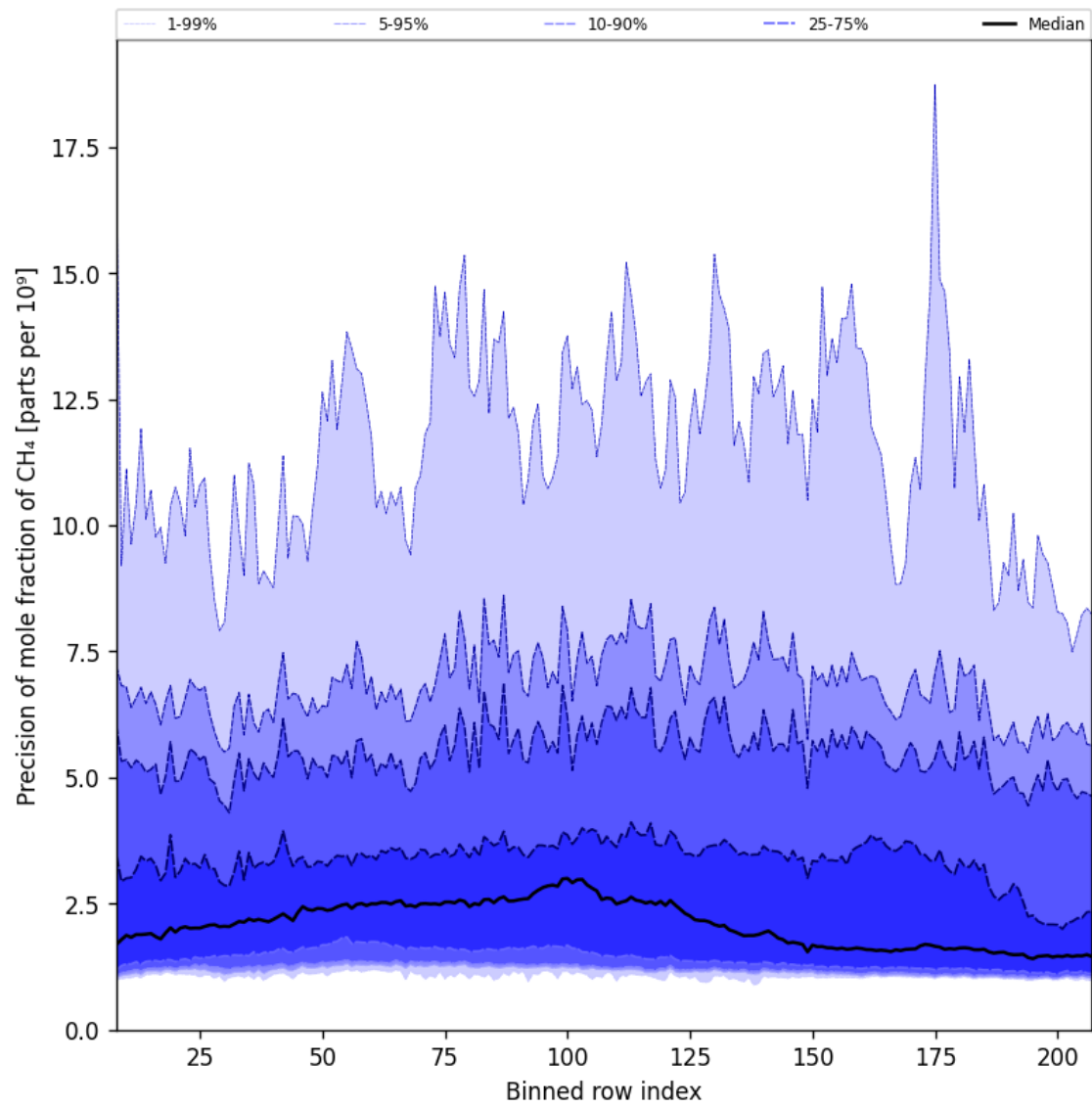
Figure 35: Along track statistics of “Precision of mole fraction of CH 4 ” for 2025-02-19 to 2025-02-21
