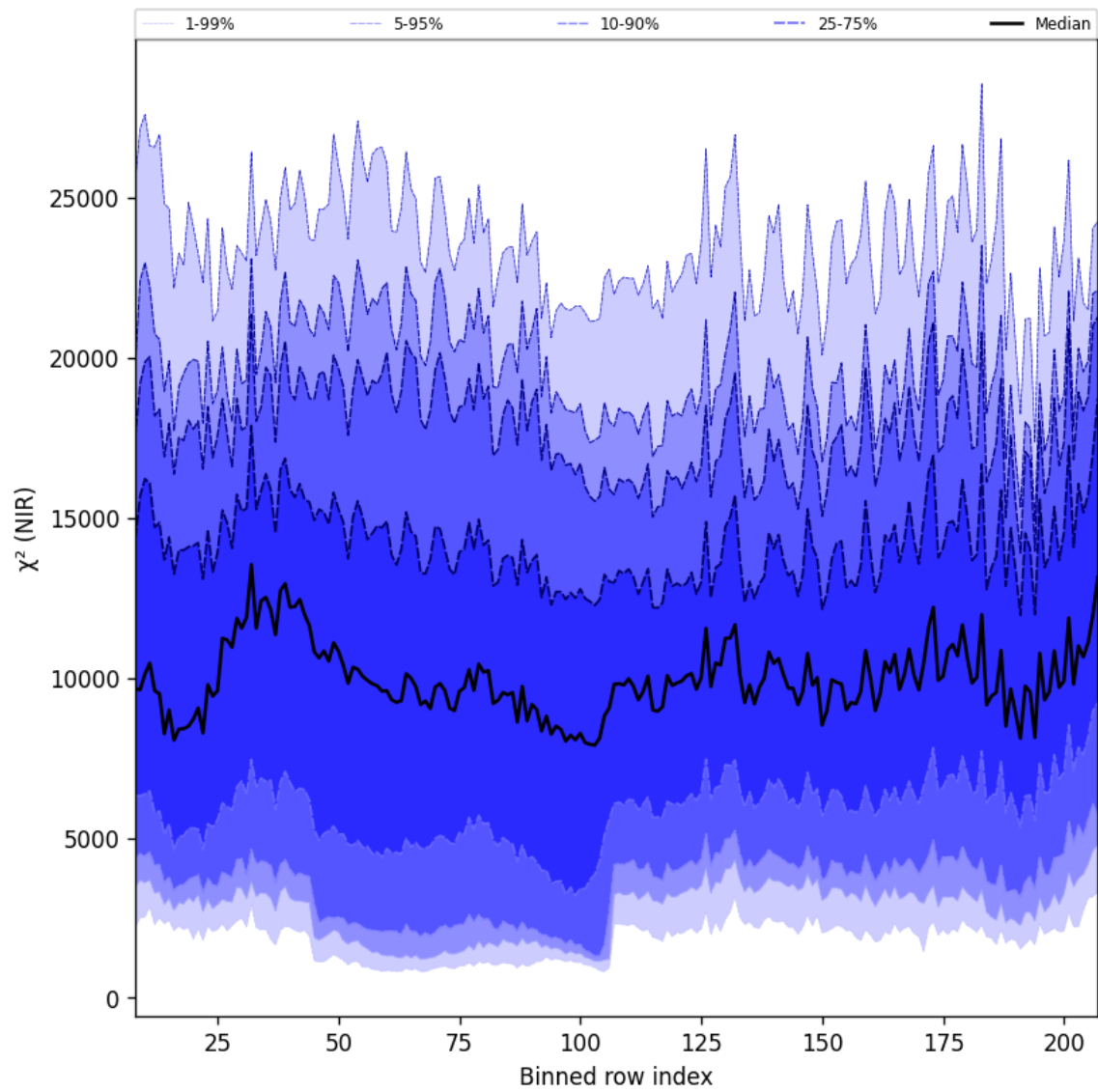
Figure 40: Along track statistics of " \chi^2 (NIR)" for 2025-02-19 to 2025-02-21
