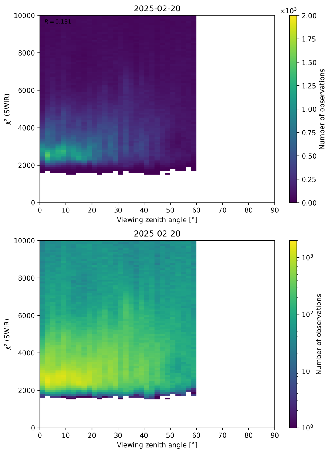
Figure 106: Scatter density plot of “Viewing zenith angle” against “ \chi^2 (SWIR)” for 2025-02-19 to 2025-02-21.
