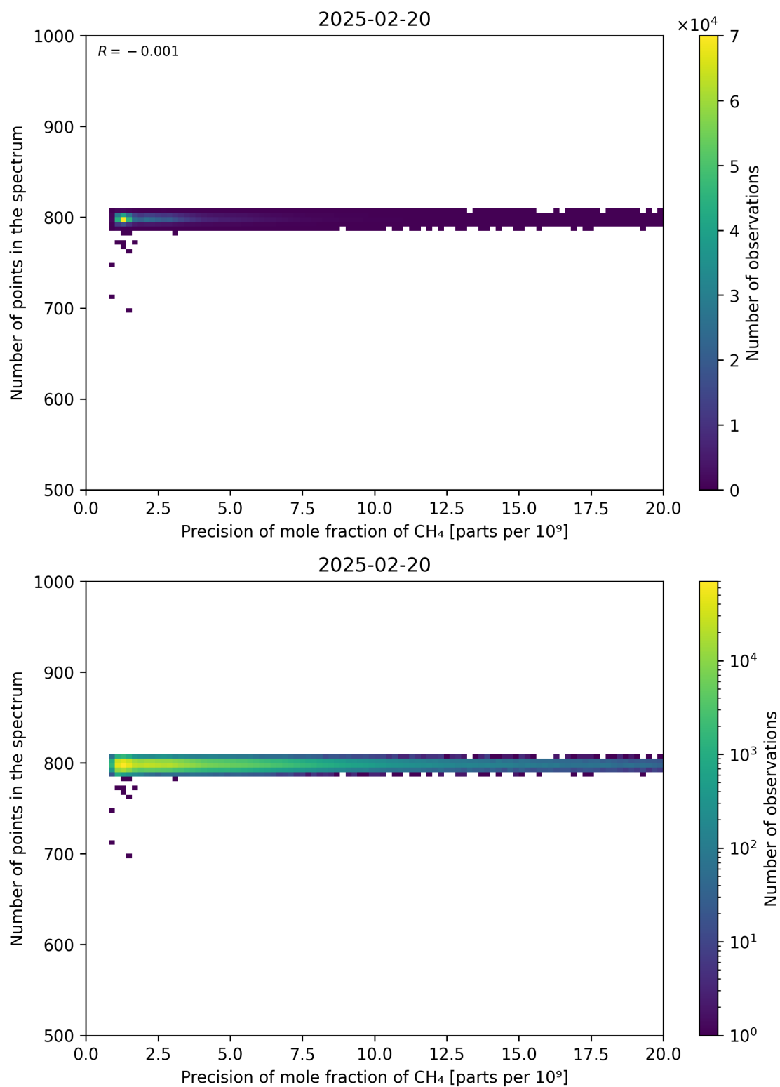
Figure 84: Scatter density plot of “Precision of mole fraction of CH 4 ” against “Number of points in the spectrum” for 2025-02-19 to 2025-02-21.
