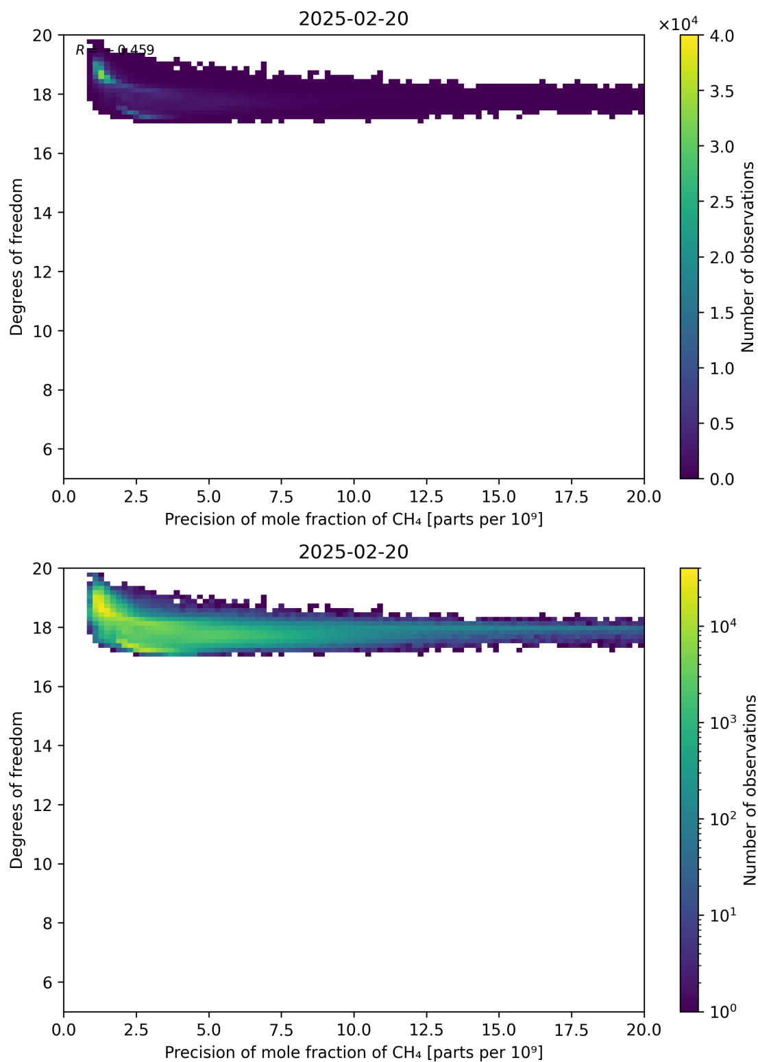
Figure 80: Scatter density plot of “Precision of mole fraction of CH 4 ” against “Degrees of freedom” for 2025-02-19 to 2025-02-21.
