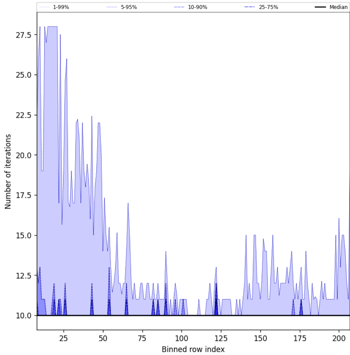
Figure 42: Along track statistics of “Number of iterations” for 2025-02-19 to 2025-02-21
