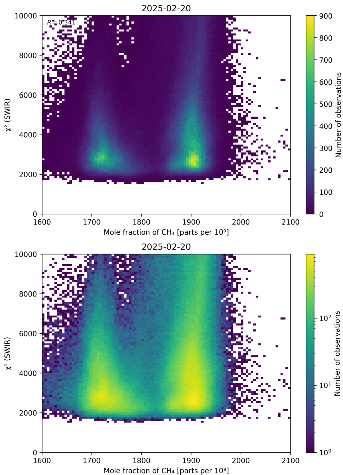
Figure 71: Scatter density plot of “Mole fraction of CH 4 ” against “ \chi^2 (SWIR)” for 2025-02-19 to 2025-02-21.
