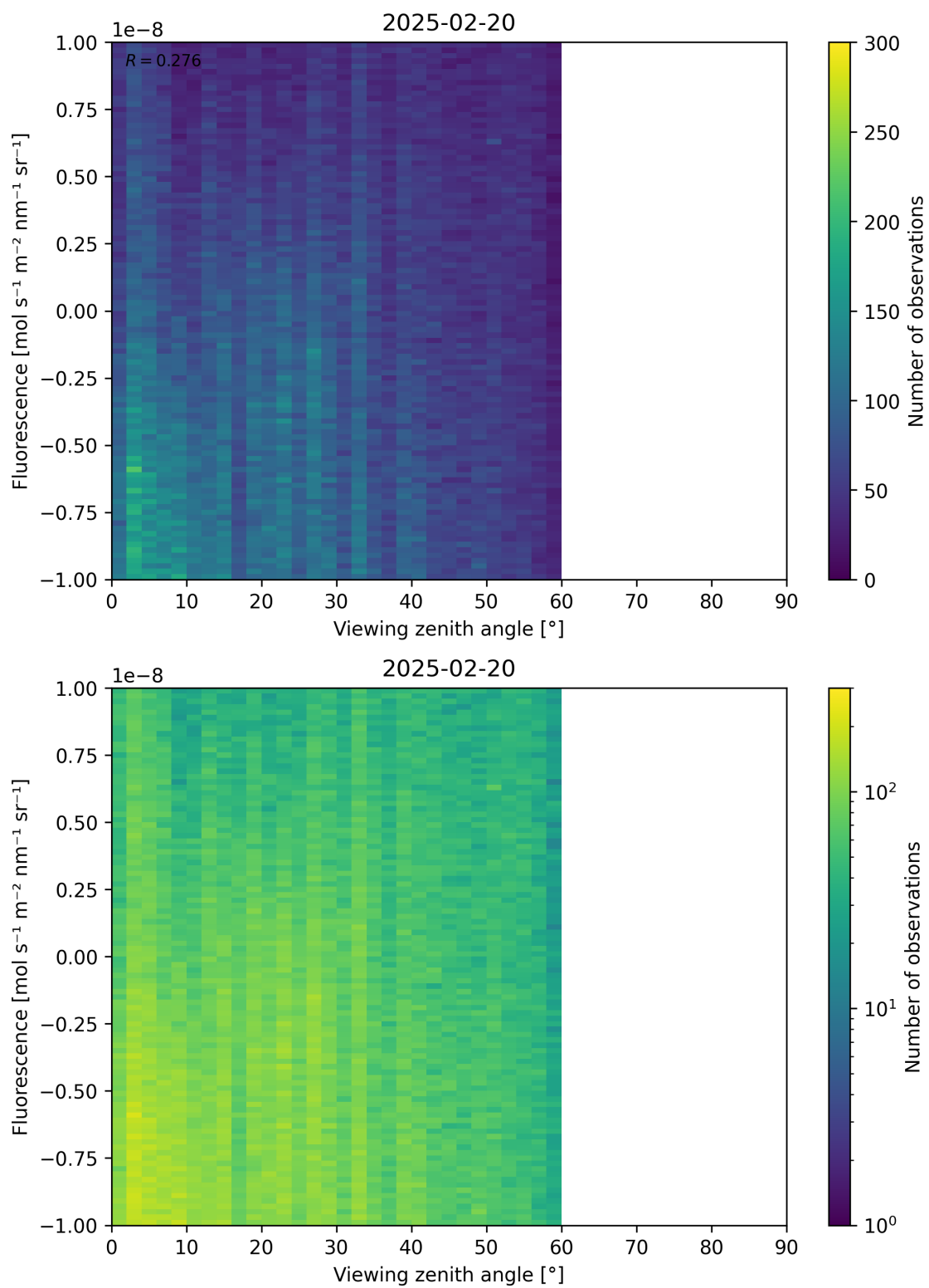
Figure 108: Scatter density plot of “Viewing zenith angle” against “Fluorescence” for 2025-02-19 to 2025-02-21.
