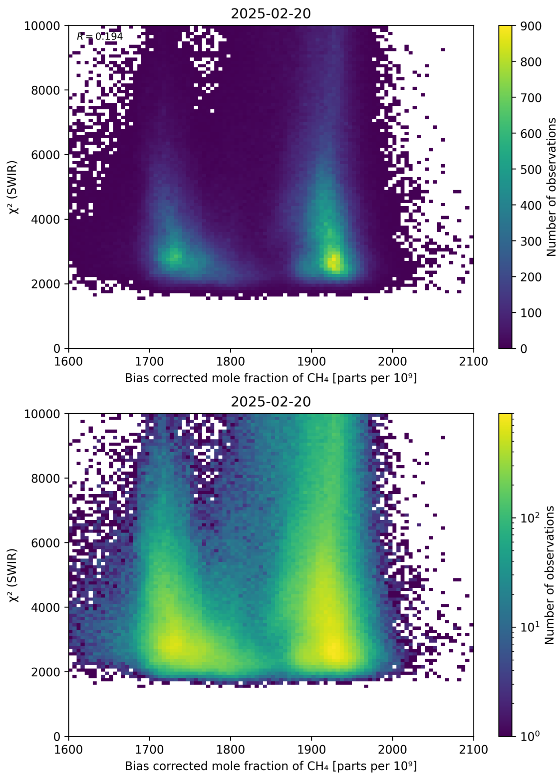
Figure 64: Scatter density plot of “Bias corrected mole fraction of \text{CH}_4 ” against “ \chi^2 (SWIR)” for 2025-02-19 to 2025-02-21.
