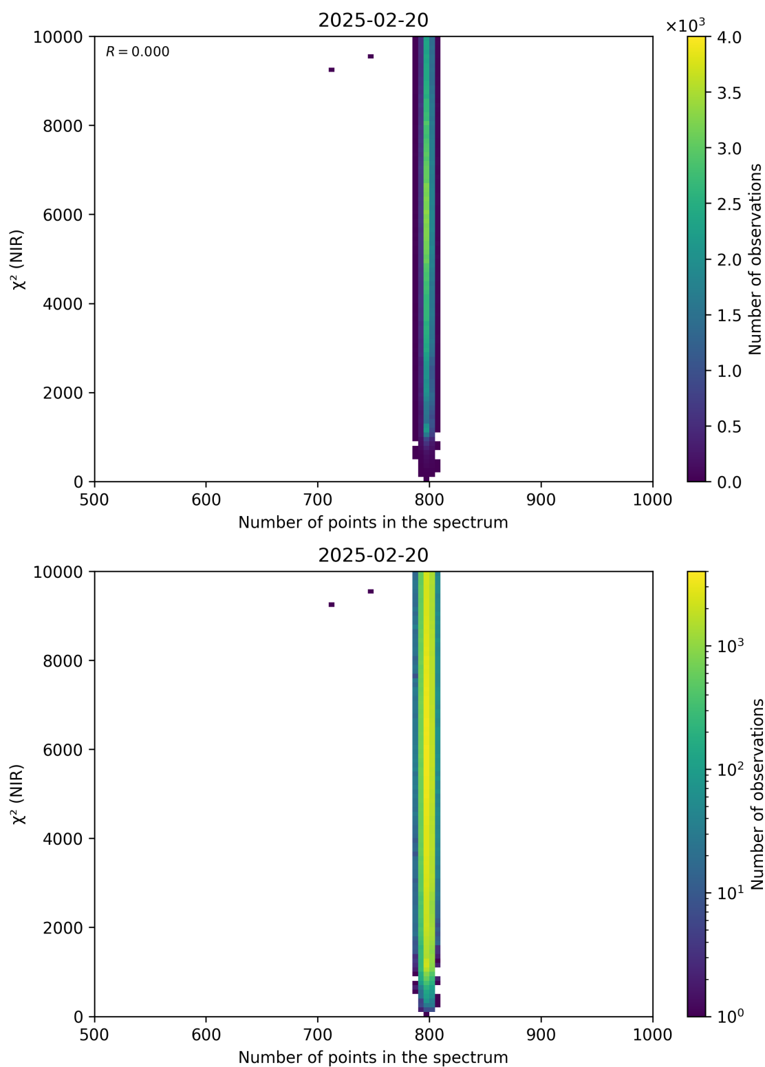
Figure 88: Scatter density plot of “Number of points in the spectrum” against “ \chi^2 (NIR)” for 2025-02-19 to 2025-02-21.
