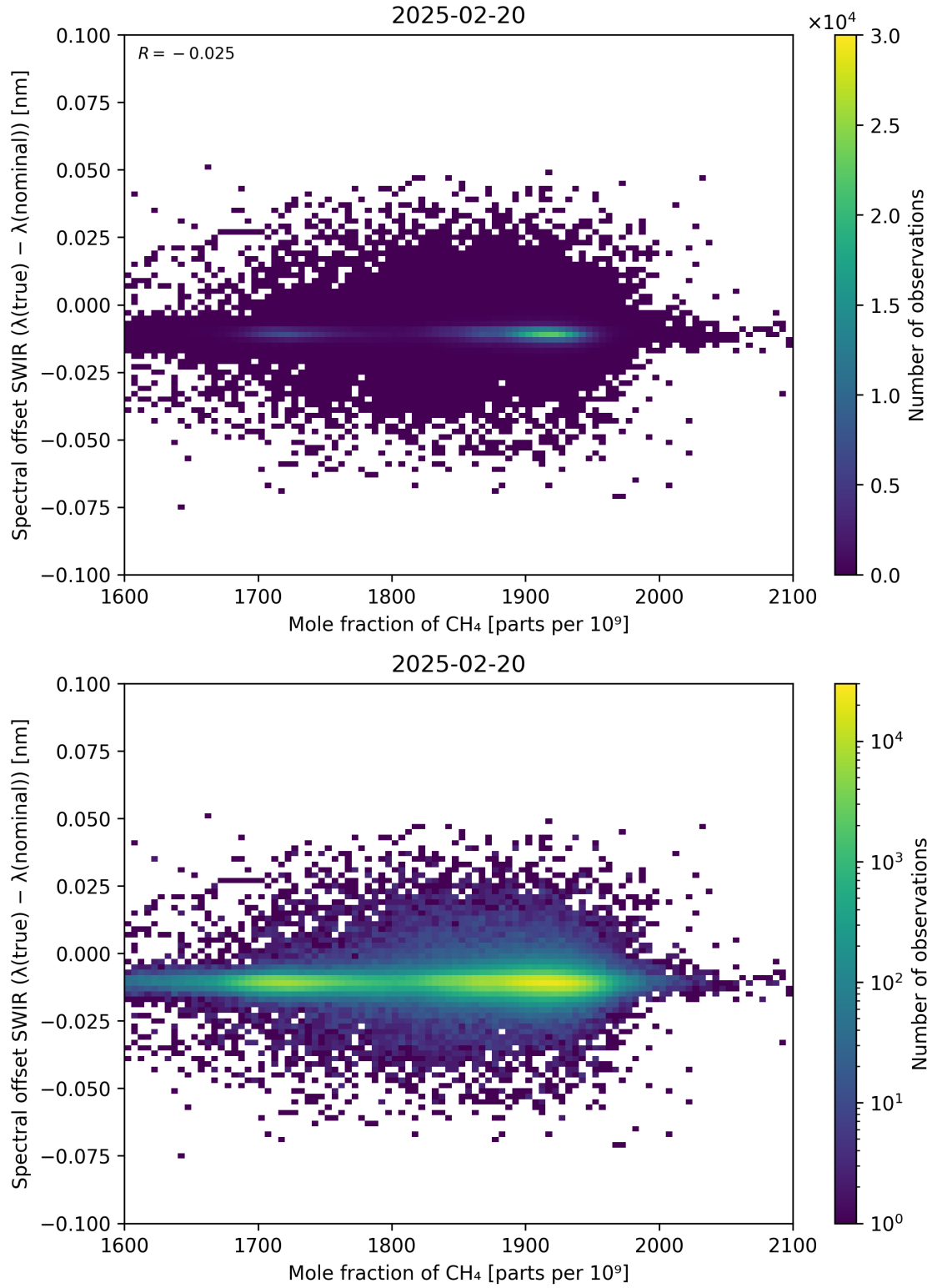
Figure 86: Scatter density plot of “Mole fraction of CH 4 ” against “Spectral offset SWIR ( \lambda_{\text{true}} - \lambda_{\text{nominal}} )” for 2025-02-19 to 2025-02-21.
