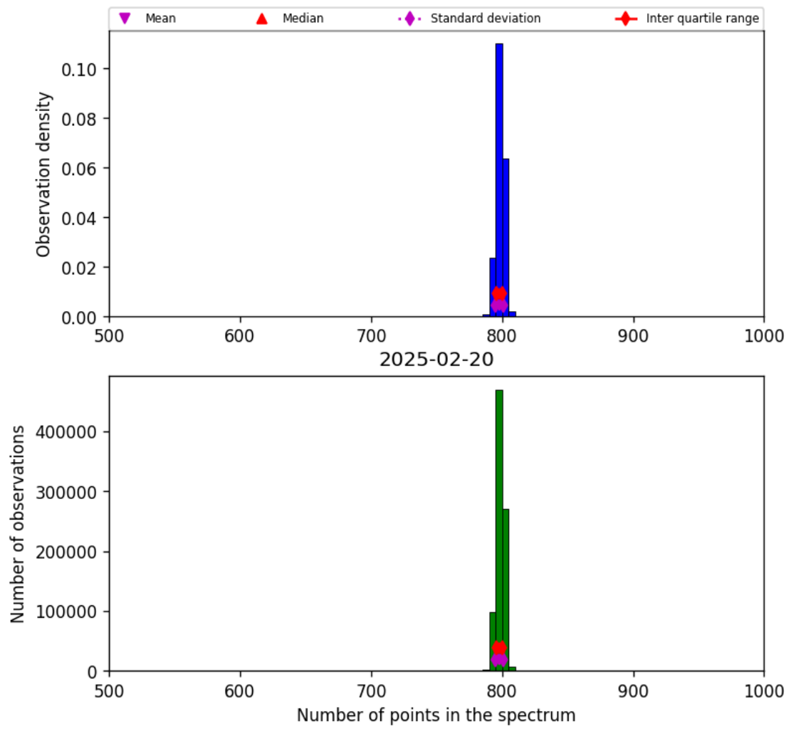
Figure 26: Histogram of “Number of points in the spectrum” for 2025-02-19 to 2025-02-21
