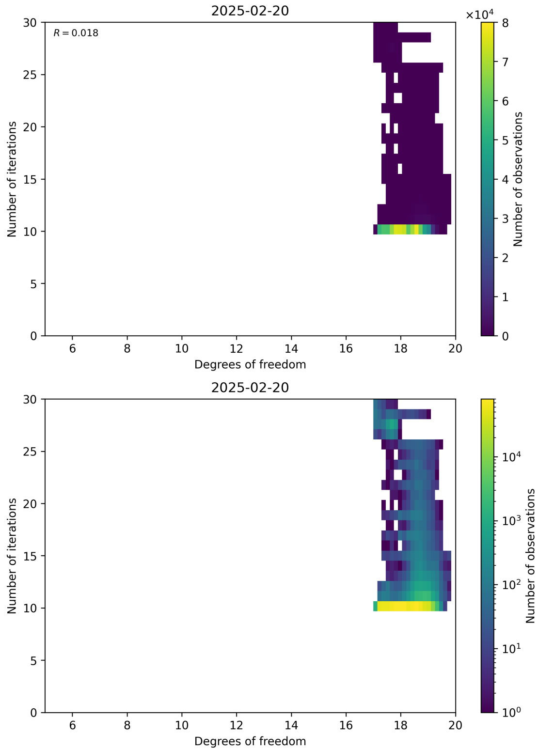
Figure 52: Scatter density plot of “Degrees of freedom” against “Number of iterations” for 2025-02-19 to 2025-02-21.
