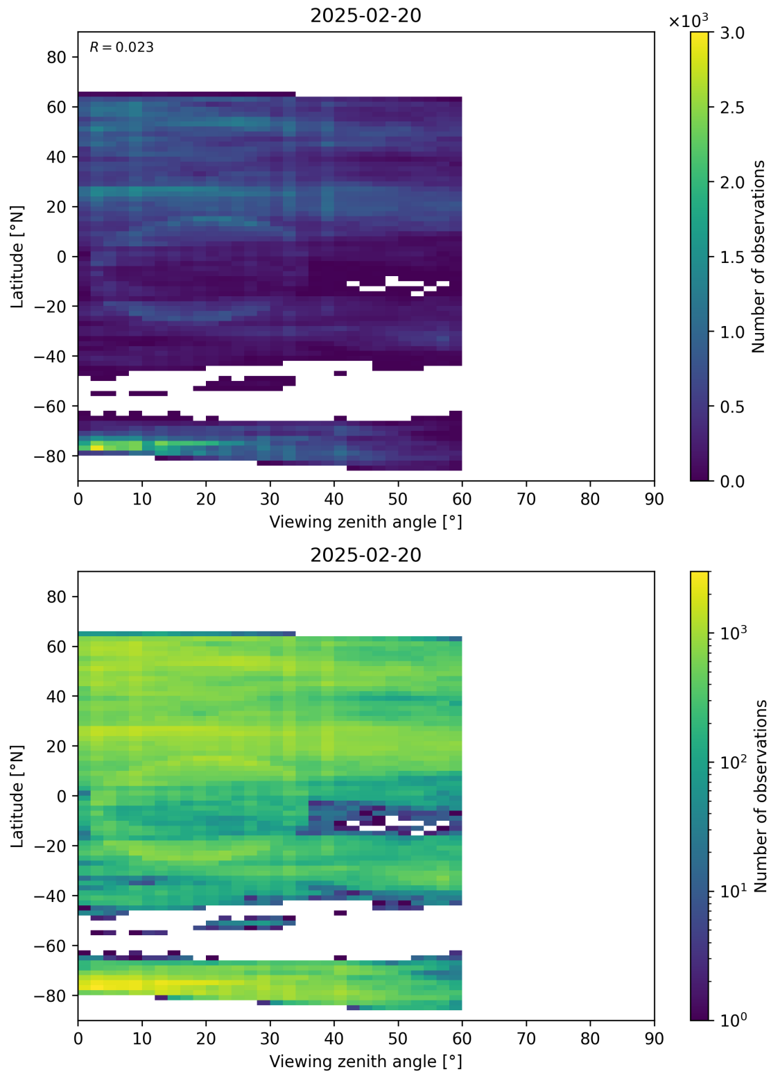
Figure 109: Scatter density plot of “Viewing zenith angle” against “Latitude” for 2025-02-19 to 2025-02-21.
