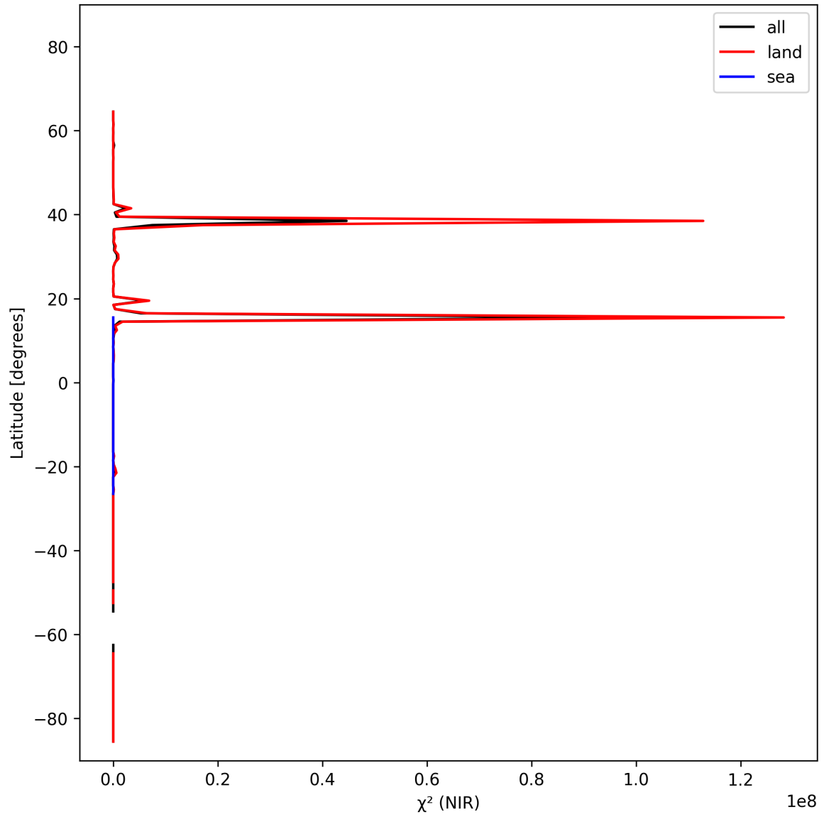
Figure 18: Zonal average of “ \chi^2 (NIR)” for 2025-02-19 to 2025-02-21.
