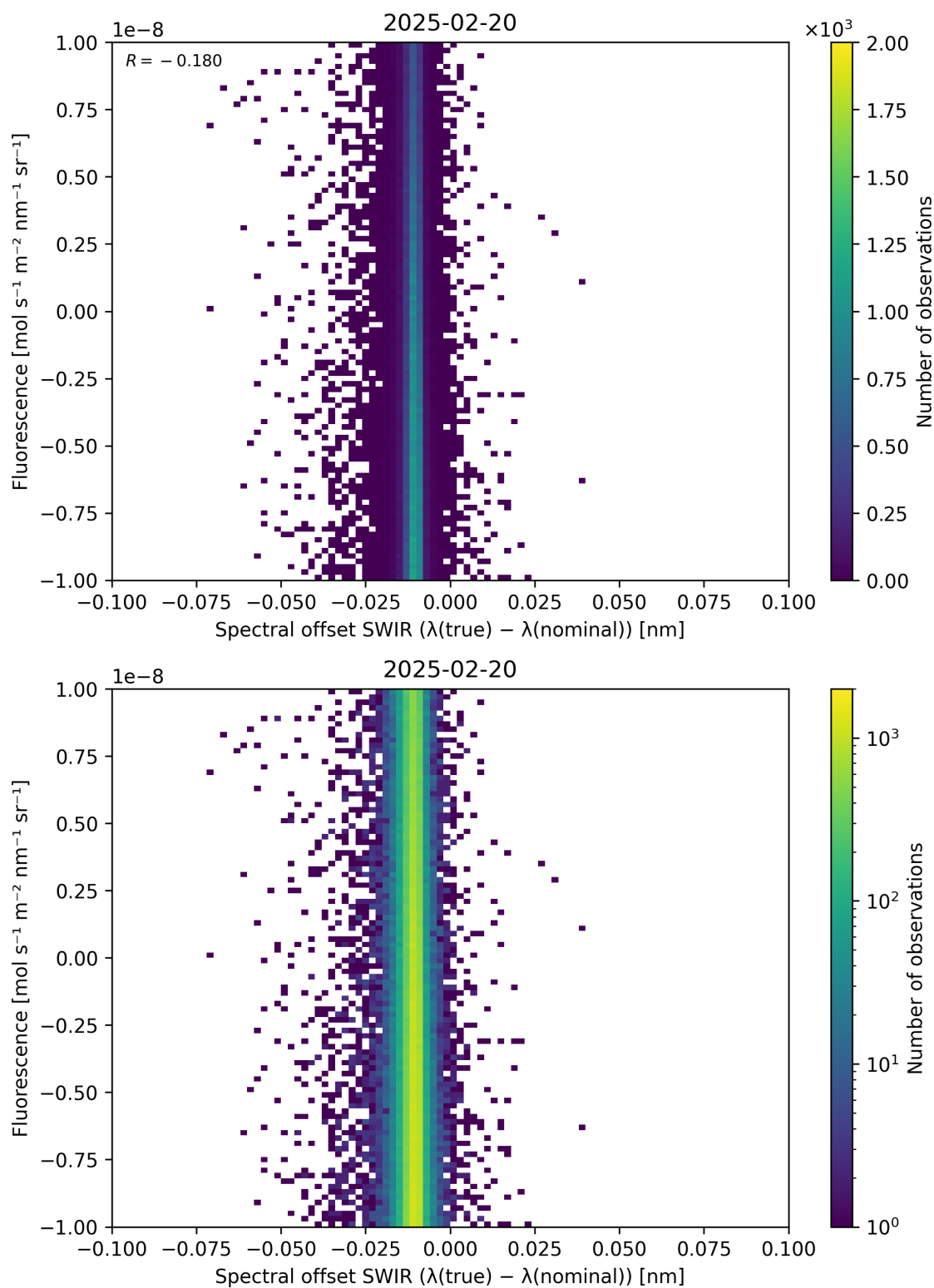
Figure 120: Scatter density plot of “Spectral offset SWIR ( \lambda_{\text{true}} - \lambda_{\text{nominal}} )” against “Fluorescence” for 2025-02-19 to 2025-02-21.
