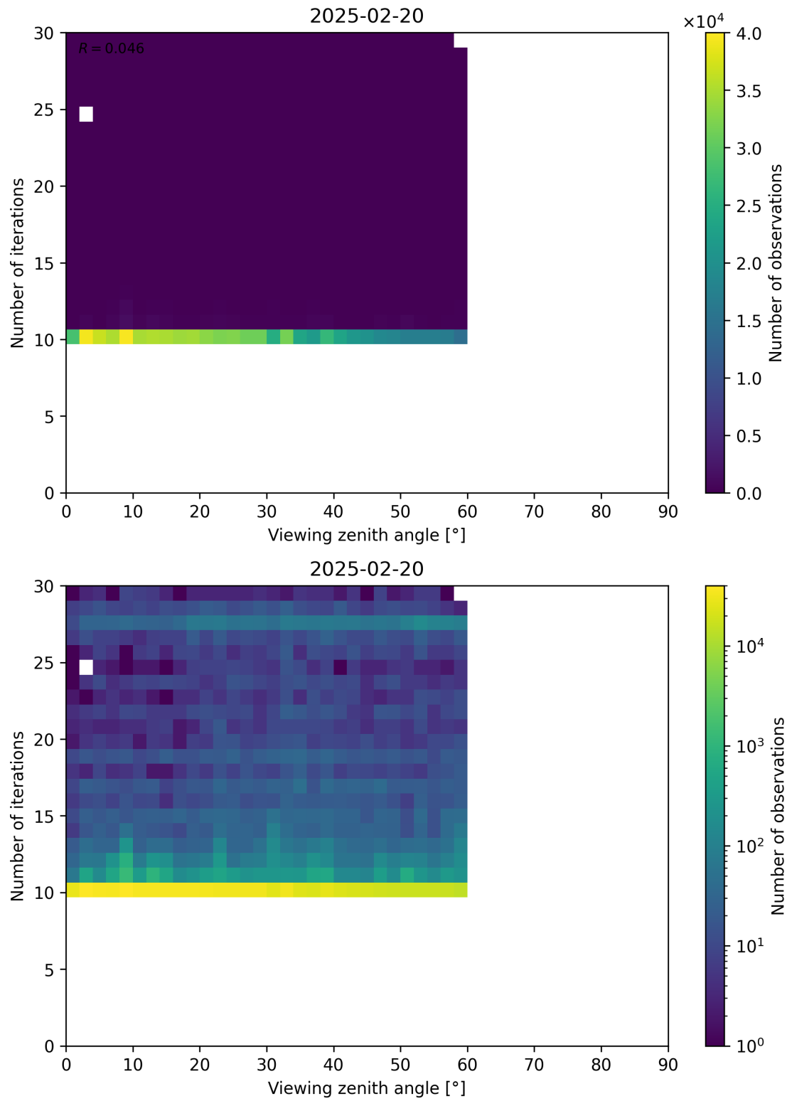
Figure 113: Scatter density plot of “Viewing zenith angle” against “Number of iterations” for 2025-02-19 to 2025-02-21.
