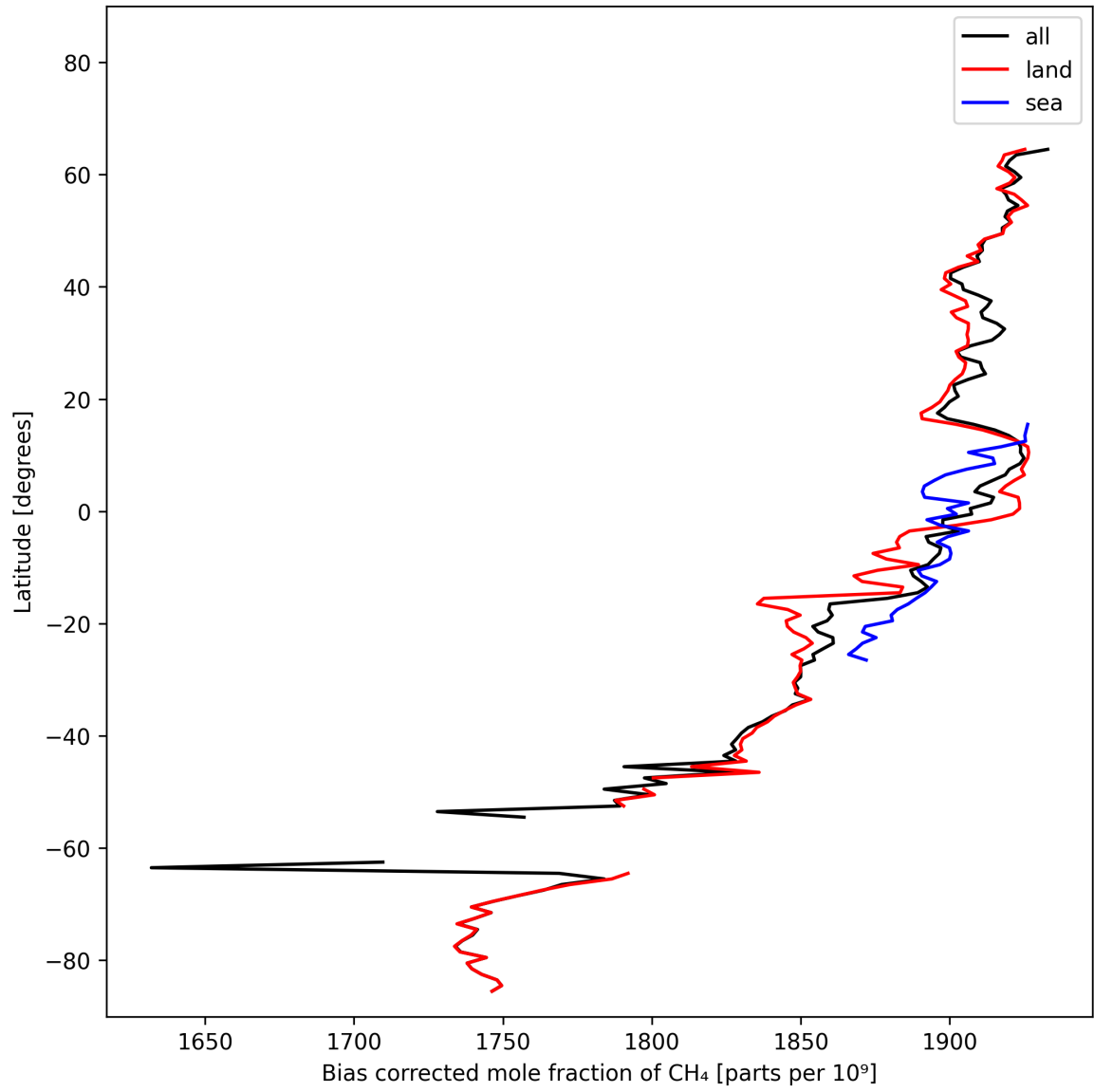
Figure 14: Zonal average of “Bias corrected mole fraction of CH 4 ” for 2025-02-19 to 2025-02-21.
