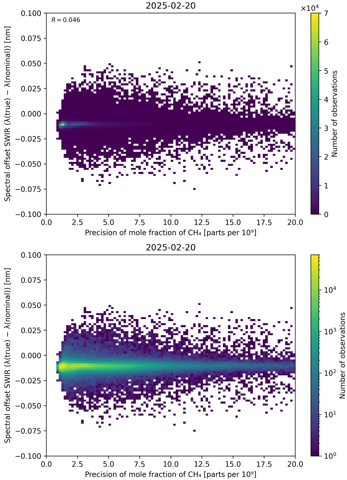
Figure 85: Scatter density plot of “Precision of mole fraction of CH 4 ” against “Spectral offset SWIR ( \lambda_{\text{true}} - \lambda_{\text{nominal}} )” for 2025-02-19 to 2025-02-21.
