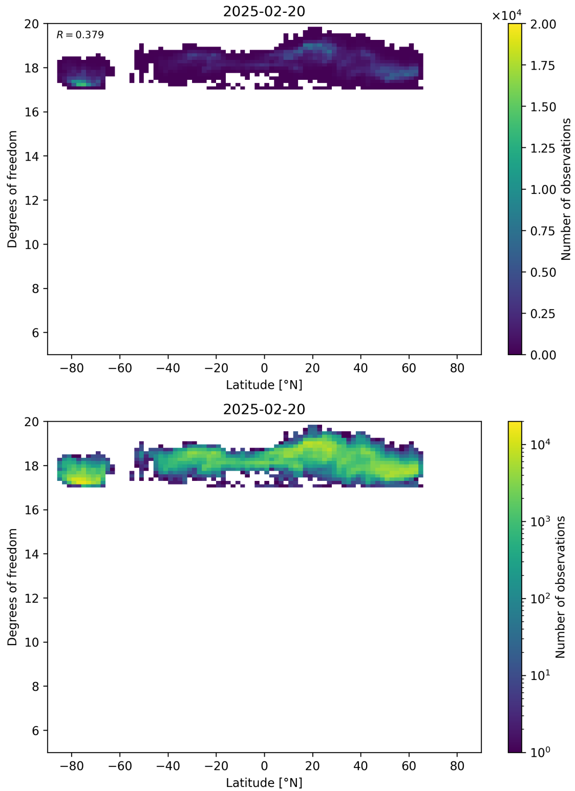
Figure 55: Scatter density plot of “Latitude” against “Degrees of freedom” for 2025-02-19 to 2025-02-21.
