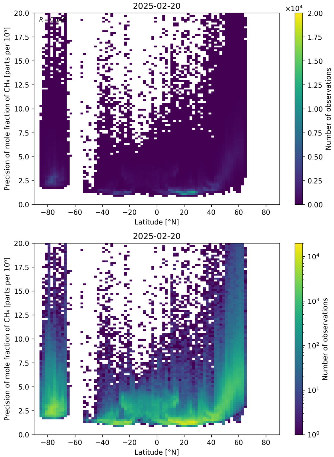
Figure 59: Scatter density plot of “Latitude” against “Precision of mole fraction of CH 4 ” for 2025-02-19 to 2025-02-21.
