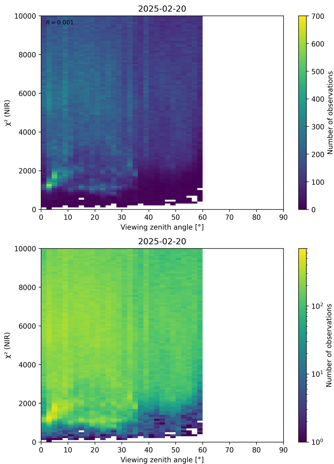
Figure 105: Scatter density plot of “Viewing zenith angle” against “ \chi^2 (NIR)” for 2025-02-19 to 2025-02-21.
