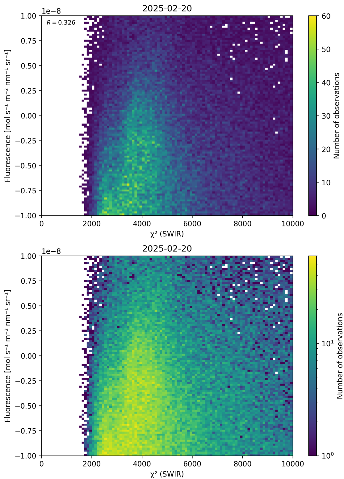
Figure 49: Scatter density plot of “ \chi^2 (SWIR)” against “Fluorescence” for 2025-02-19 to 2025-02-21.
