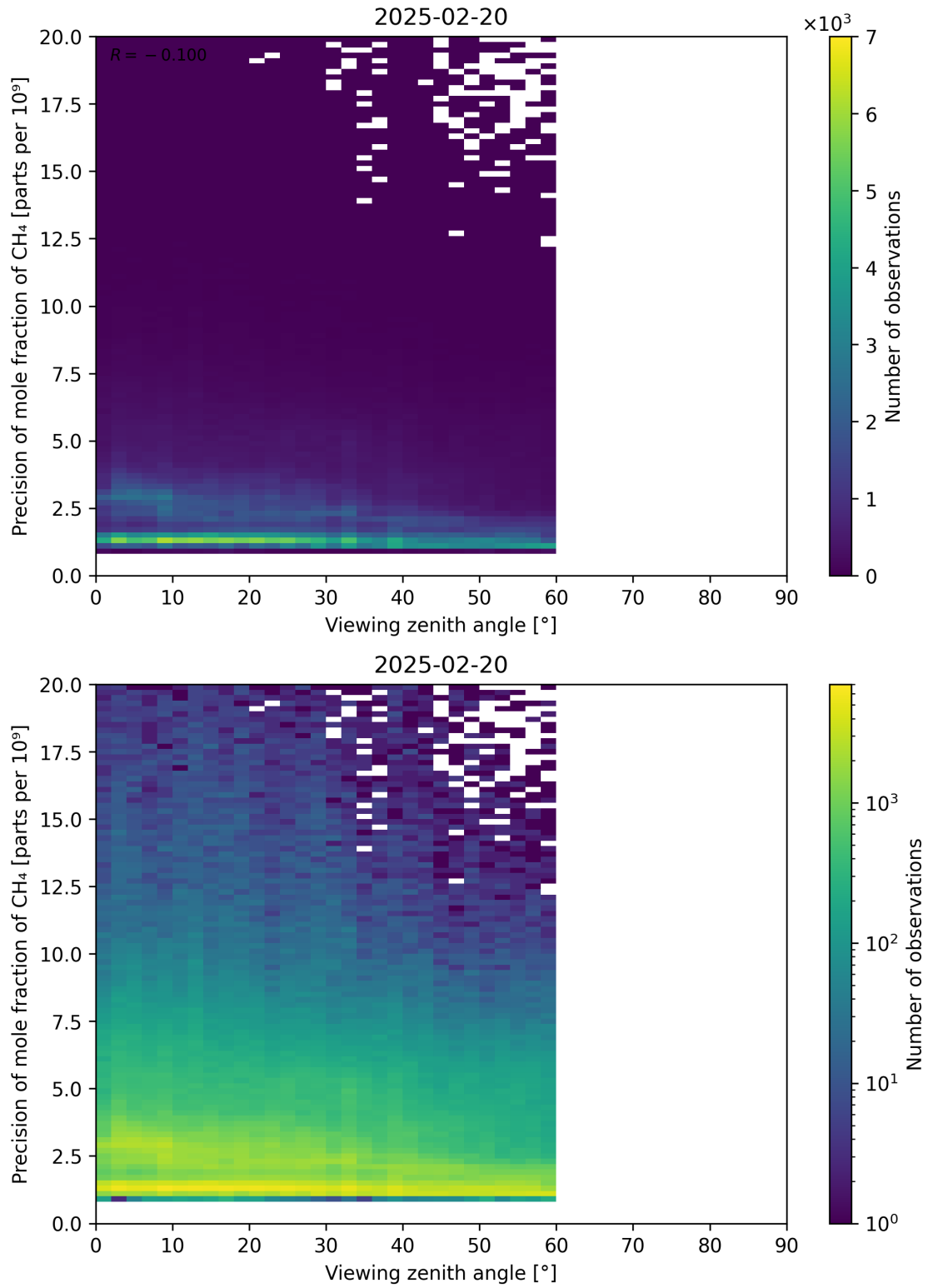
Figure 112: Scatter density plot of “Viewing zenith angle” against “Precision of mole fraction of CH 4 ” for 2025-02-19 to 2025-02-21.
