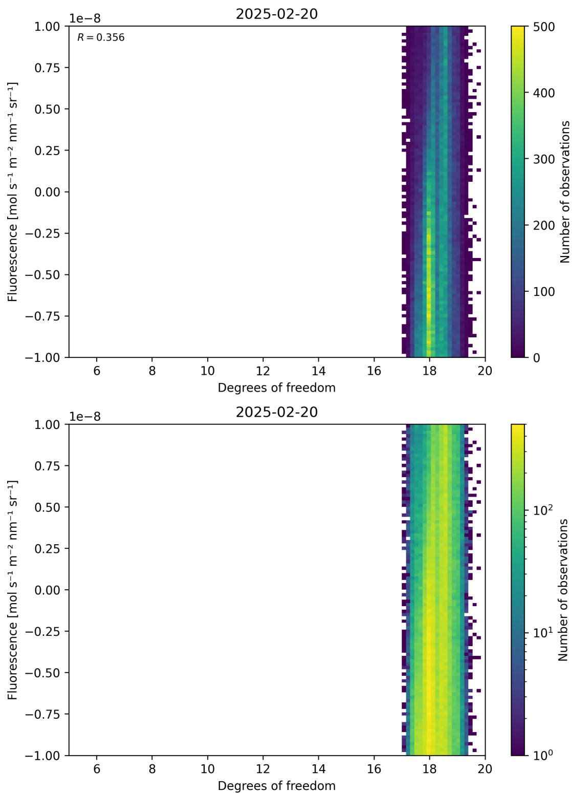
Figure 51: Scatter density plot of “Degrees of freedom” against “Fluorescence” for 2025-02-19 to 2025-02-21.
