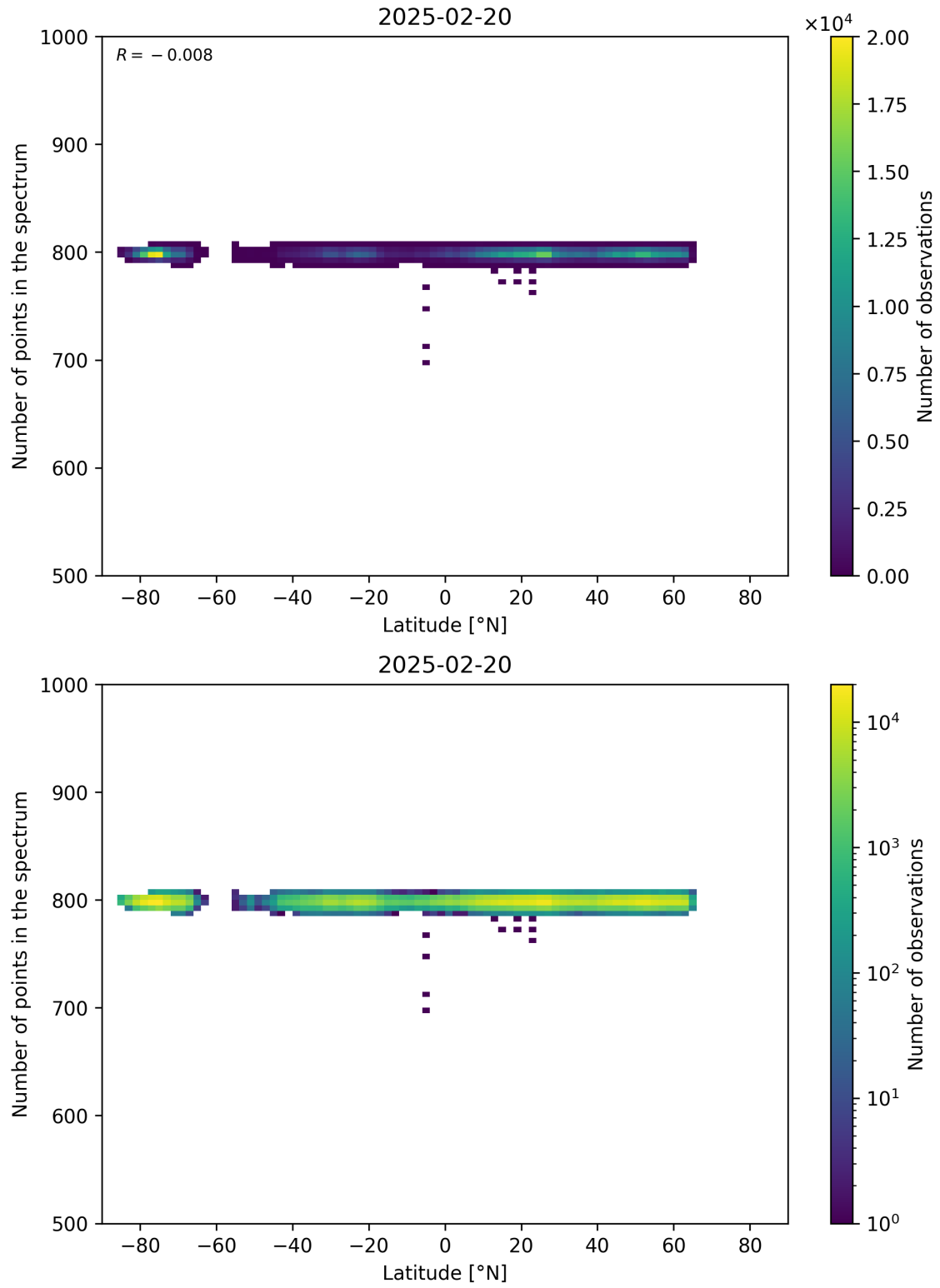
Figure 61: Scatter density plot of “Latitude” against “Number of points in the spectrum” for 2025-02-19 to 2025-02-21.
