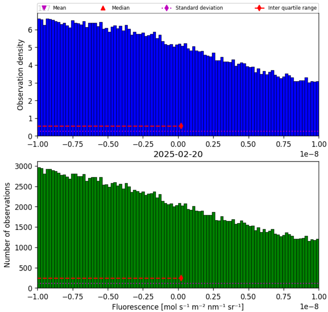
Figure 32: Histogram of “Fluorescence” for 2025-02-19 to 2025-02-21
