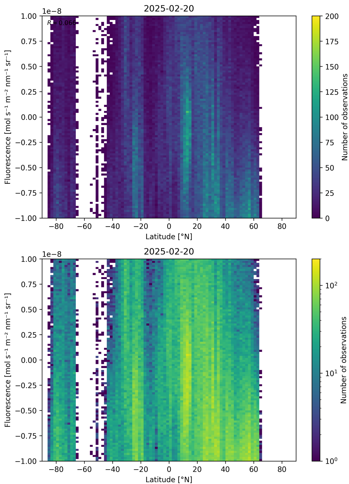
Figure 56: Scatter density plot of “Latitude” against “Fluorescence” for 2025-02-19 to 2025-02-21.
