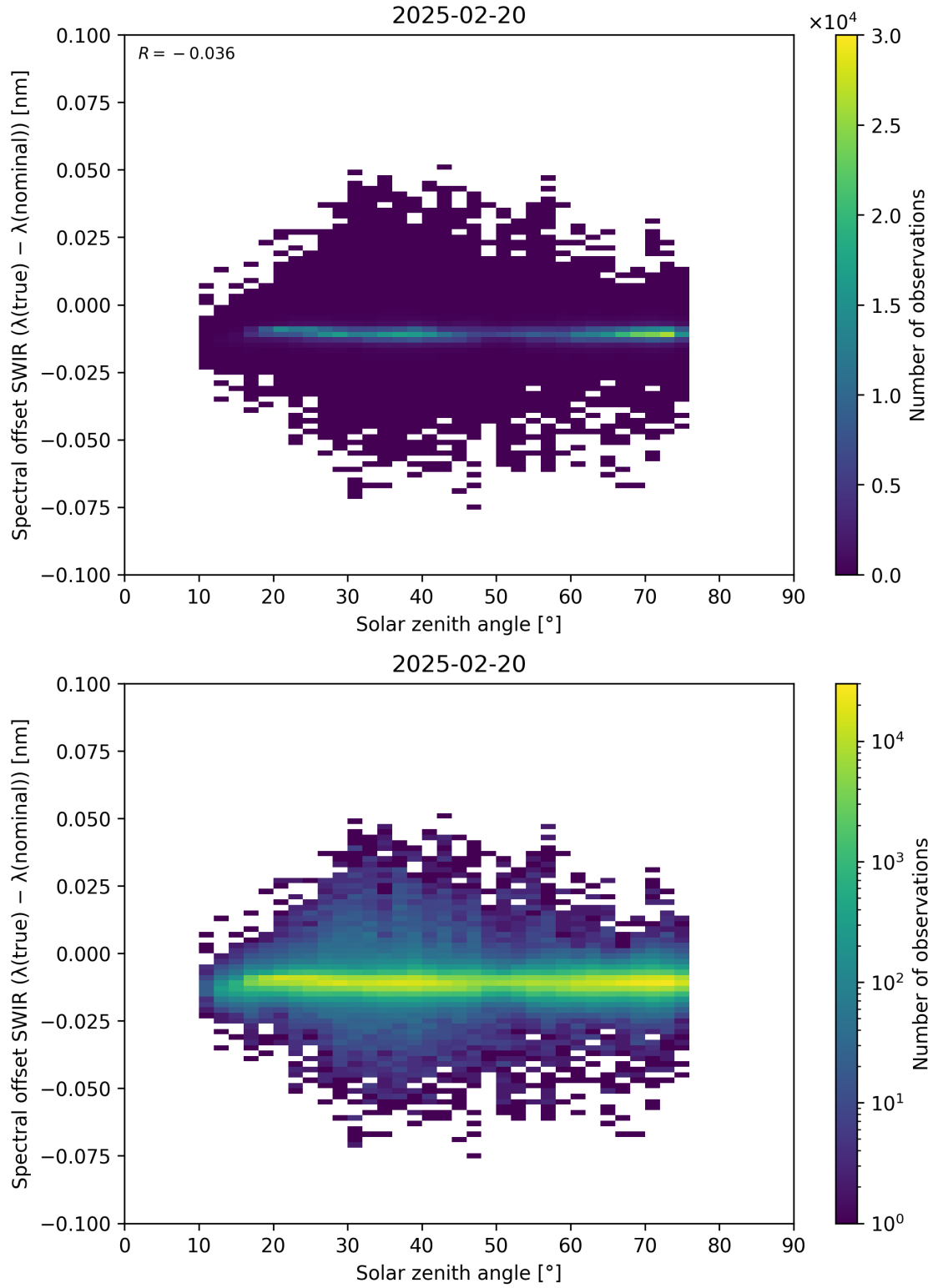
Figure 104: Scatter density plot of “Solar zenith angle” against “Spectral offset SWIR ( \lambda_{\text{true}} - \lambda_{\text{nominal}} )” for 2025-02-19 to 2025-02-21.
