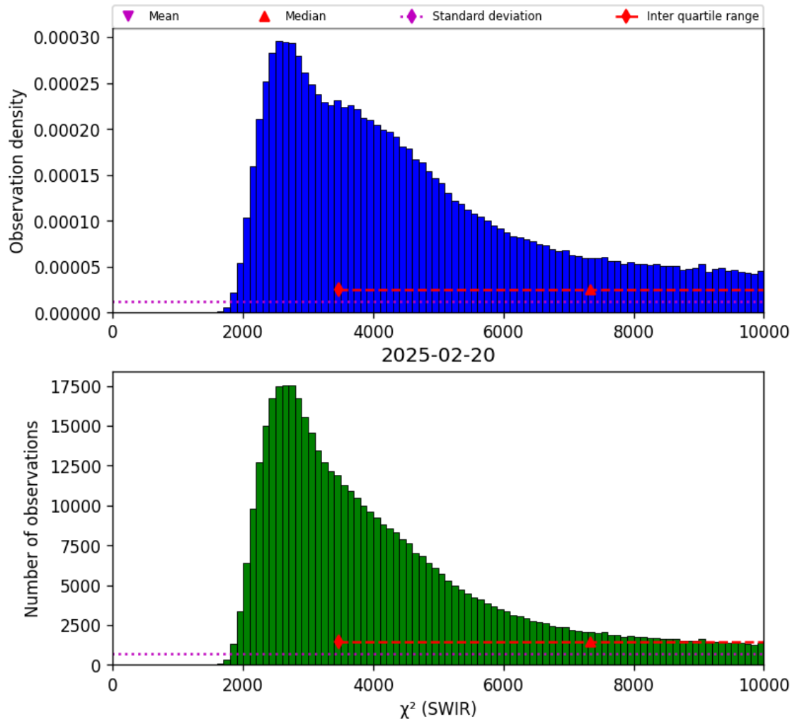
Figure 28: Histogram of “ \chi^2 (SWIR)” for 2025-02-19 to 2025-02-21
