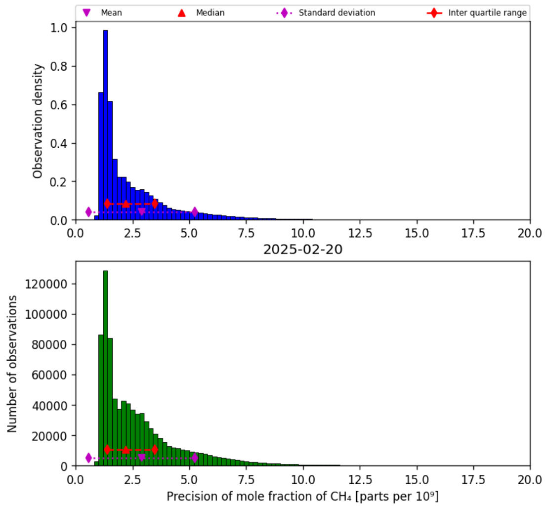
Figure 24: Histogram of “Precision of mole fraction of CH 4 ” for 2025-02-19 to 2025-02-21
