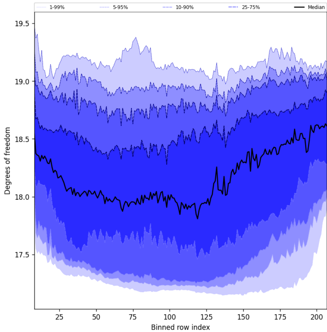
Figure 41: Along track statistics of “Degrees of freedom” for 2025-02-19 to 2025-02-21
