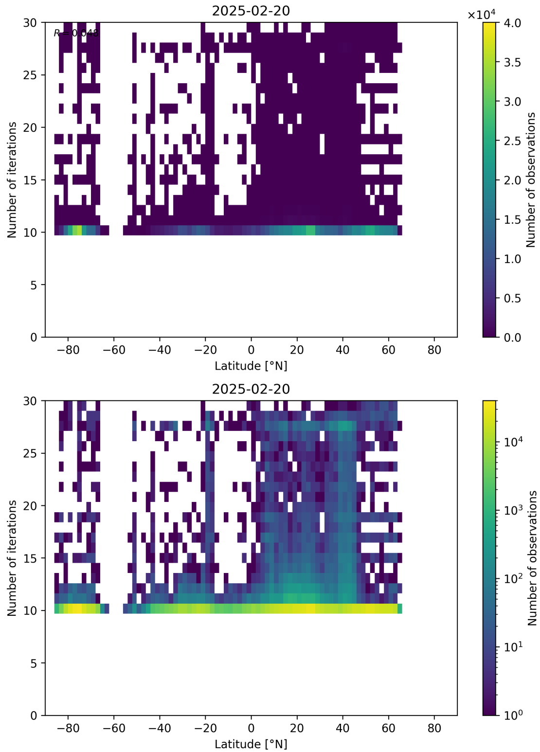
Figure 60: Scatter density plot of “Latitude” against “Number of iterations” for 2025-02-19 to 2025-02-21.
