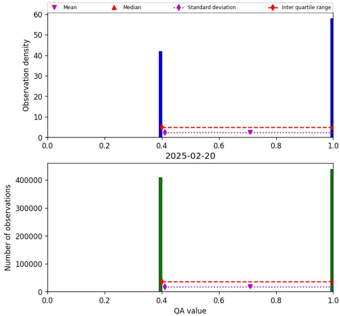
Figure 22: Histogram of “QA value” for 2025-02-19 to 2025-02-21
