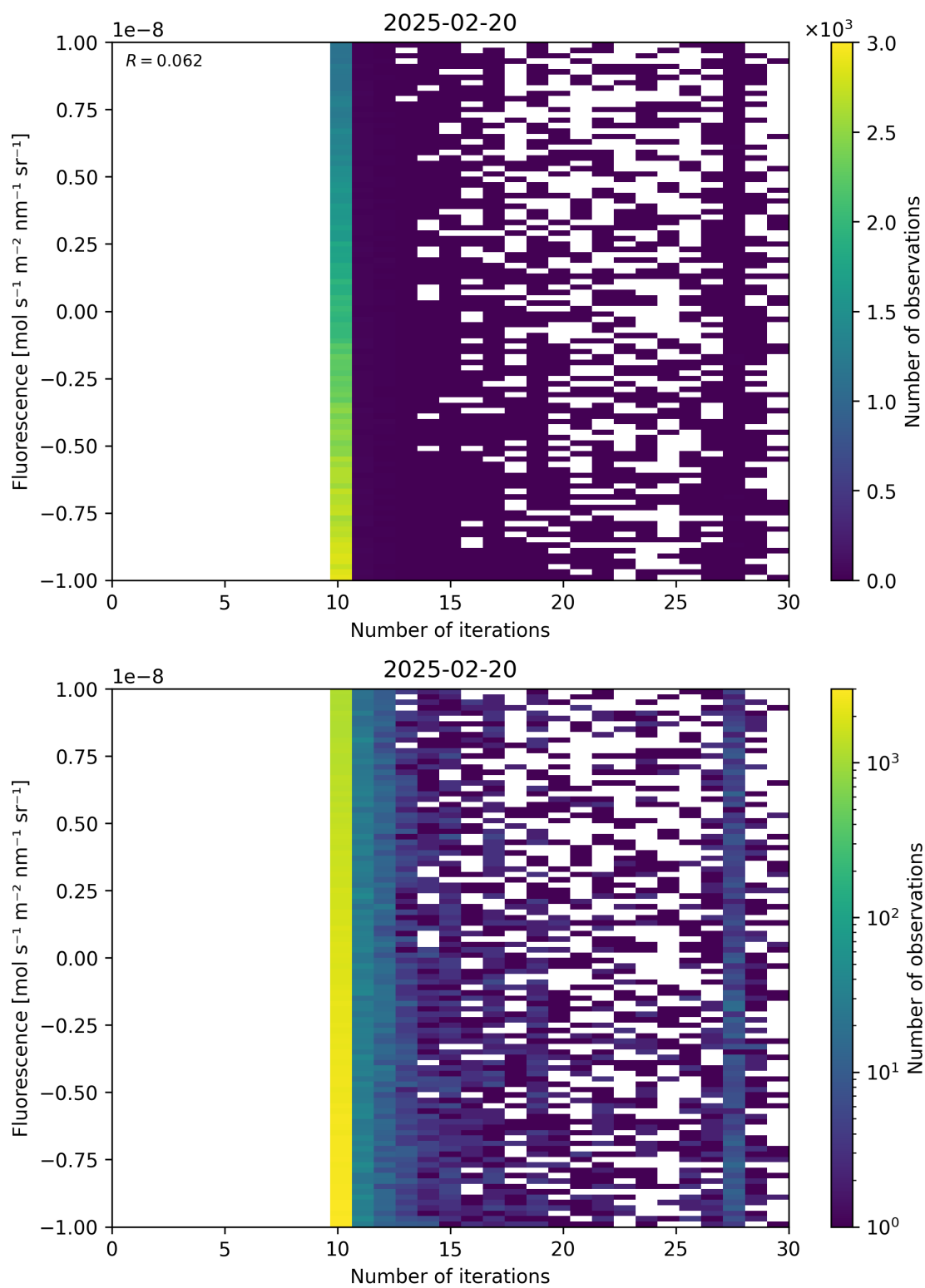
Figure 87: Scatter density plot of “Number of iterations” against “Fluorescence” for 2025-02-19 to 2025-02-21.
