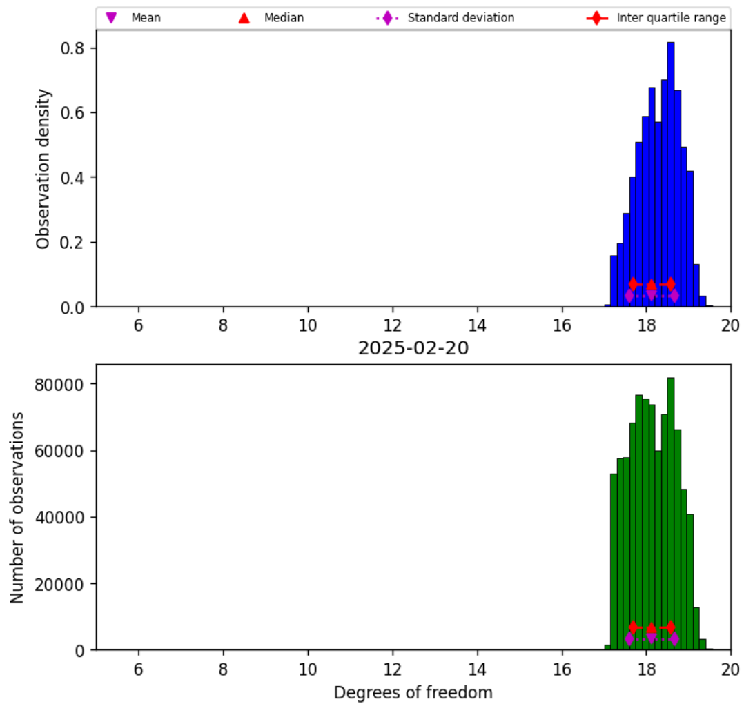
Figure 30: Histogram of “Degrees of freedom” for 2025-02-19 to 2025-02-21
