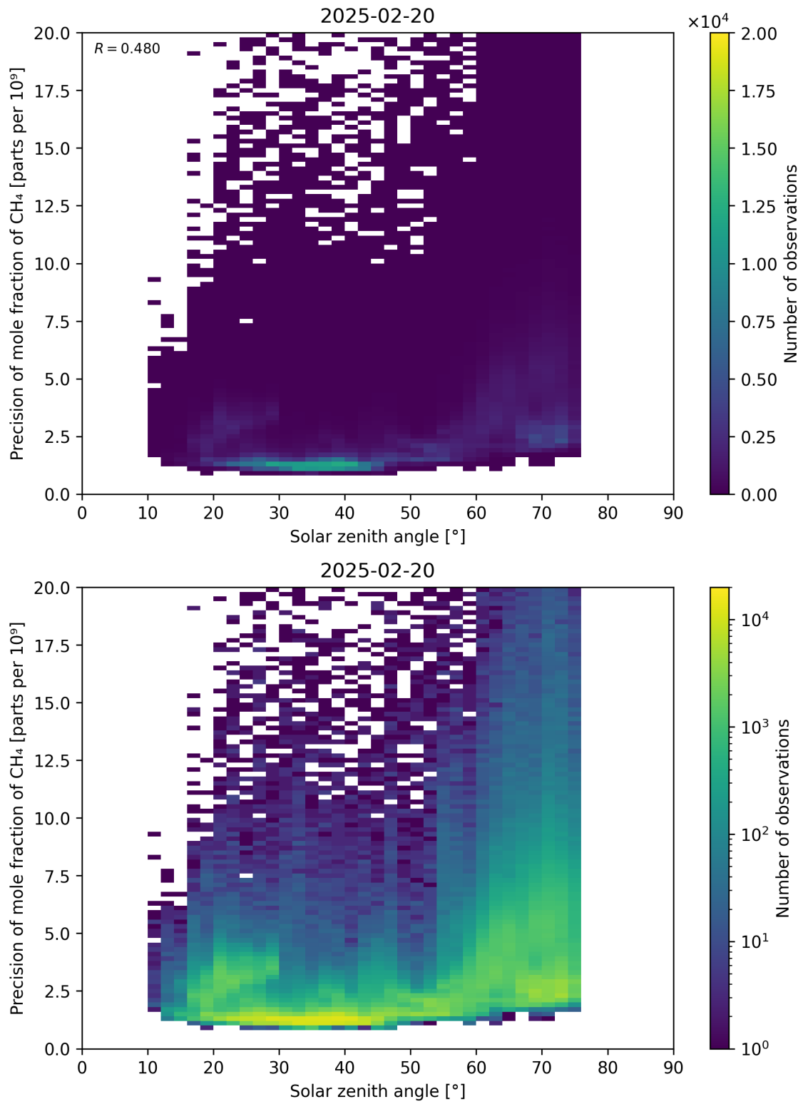
Figure 101: Scatter density plot of “Solar zenith angle” against “Precision of mole fraction of \text{CH}_4 ” for 2025-02-19 to 2025-02-21.
