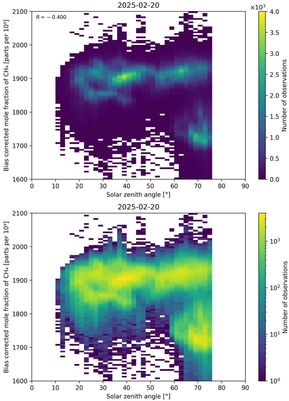
Figure 100: Scatter density plot of “Solar zenith angle” against “Bias corrected mole fraction of CH 4 ” for 2025-02-19 to 2025-02-21.
