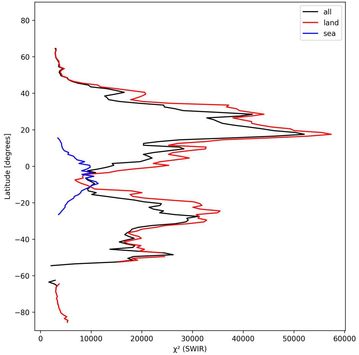
Figure 17: Zonal average of “ \chi^2 (SWIR)” for 2025-02-19 to 2025-02-21.
