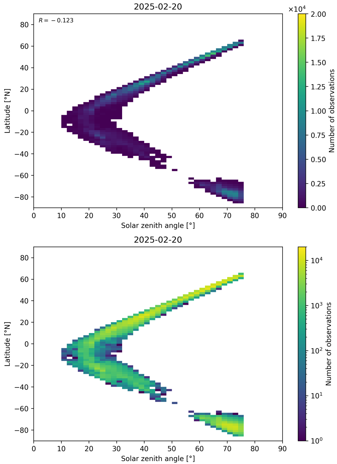
Figure 98: Scatter density plot of “Solar zenith angle” against “Latitude” for 2025-02-19 to 2025-02-21.
