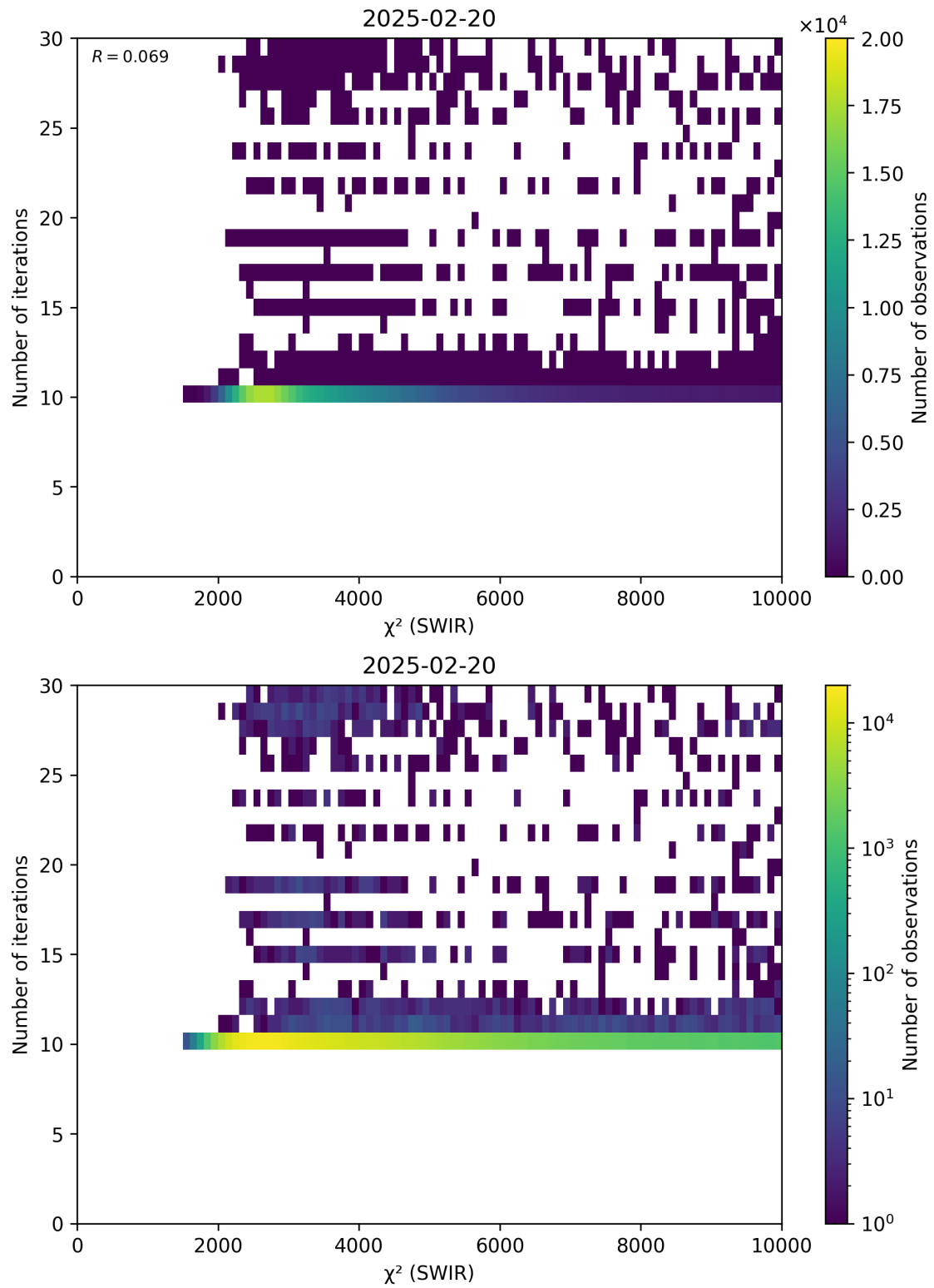
Figure 50: Scatter density plot of “ \chi^2 (SWIR)” against “Number of iterations” for 2025-02-19 to 2025-02-21.
