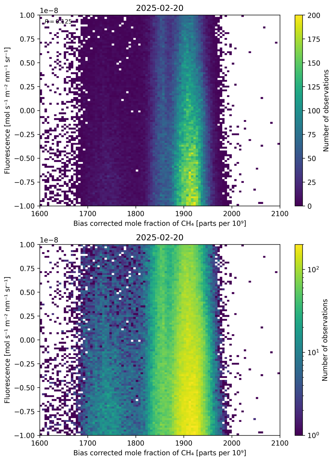
Figure 66: Scatter density plot of “Bias corrected mole fraction of \text{CH}_4 ” against “Fluorescence” for 2025-02-19 to 2025-02-21.
