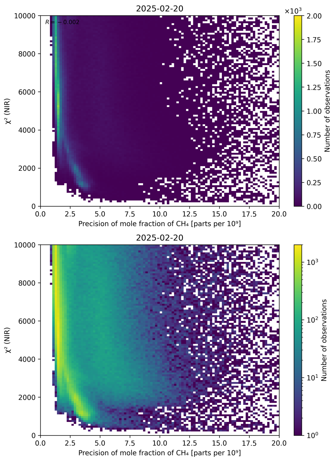
Figure 78: Scatter density plot of “Precision of mole fraction of \text{CH}_4 ” against “ \chi^2 (NIR)” for 2025-02-19 to 2025-02-21.
