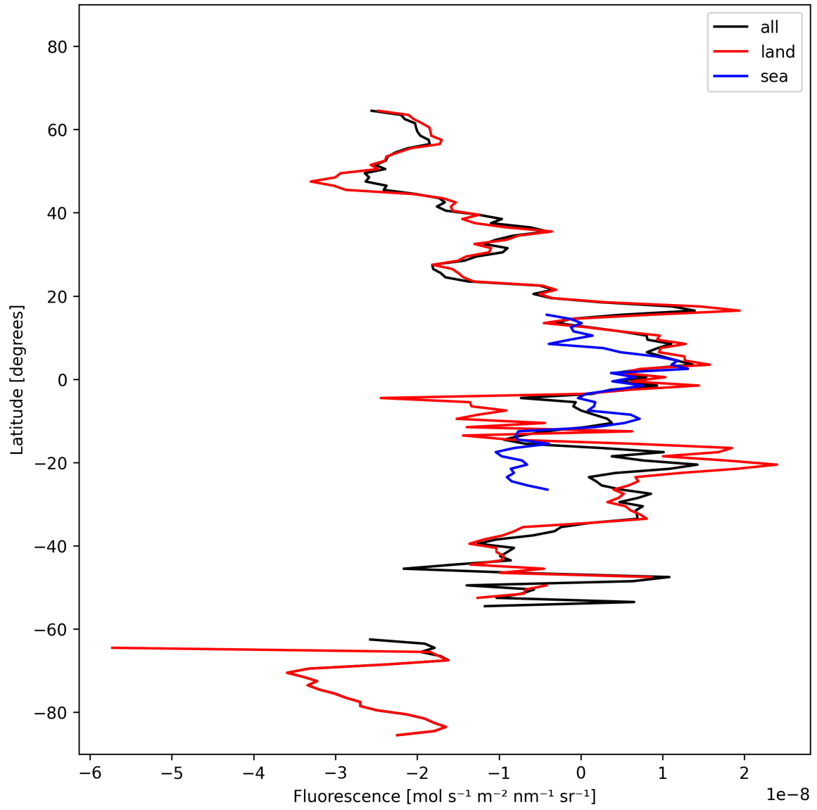
Figure 21: Zonal average of “Fluorescence” for 2025-02-19 to 2025-02-21.
