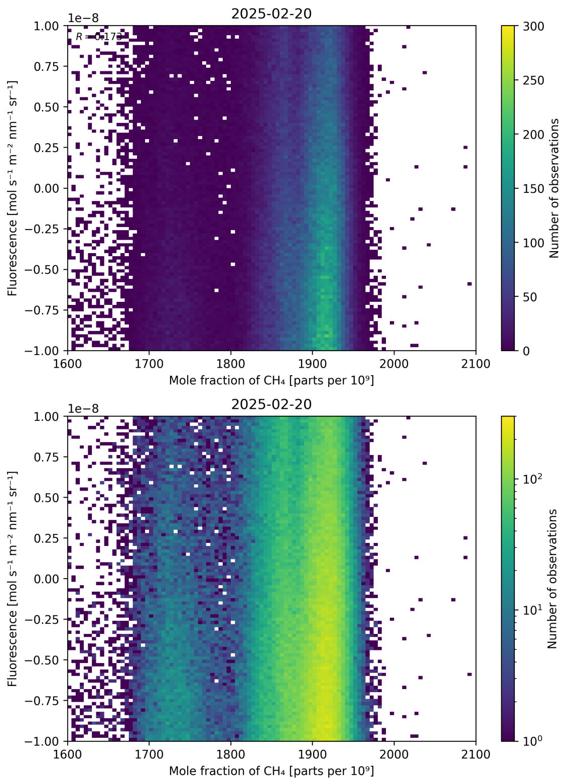
Figure 73: Scatter density plot of “Mole fraction of \text{CH}_4 ” against “Fluorescence” for 2025-02-19 to 2025-02-21.
