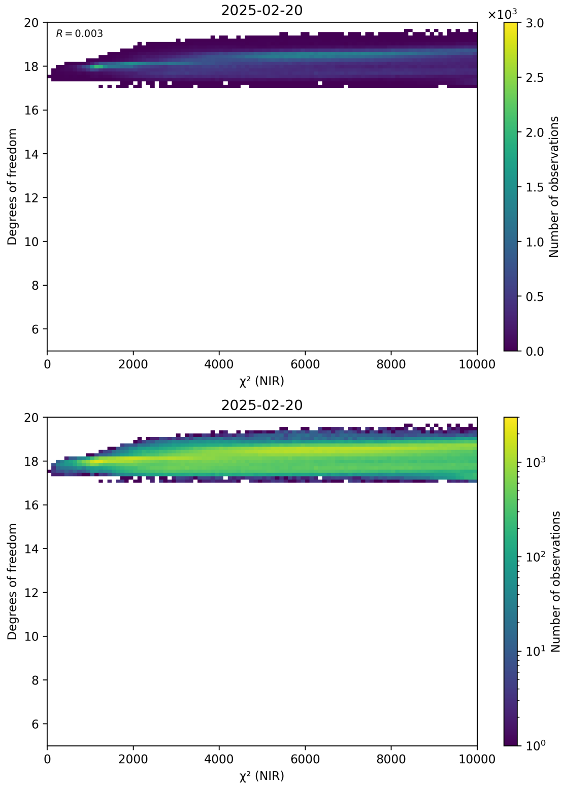
Figure 44: Scatter density plot of “ \chi^2 (NIR)” against “Degrees of freedom” for 2025-02-19 to 2025-02-21.
