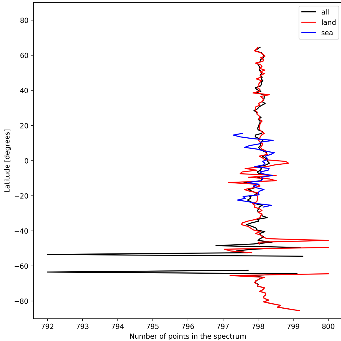
Figure 15: Zonal average of “Number of points in the spectrum” for 2025-02-19 to 2025-02-21.
