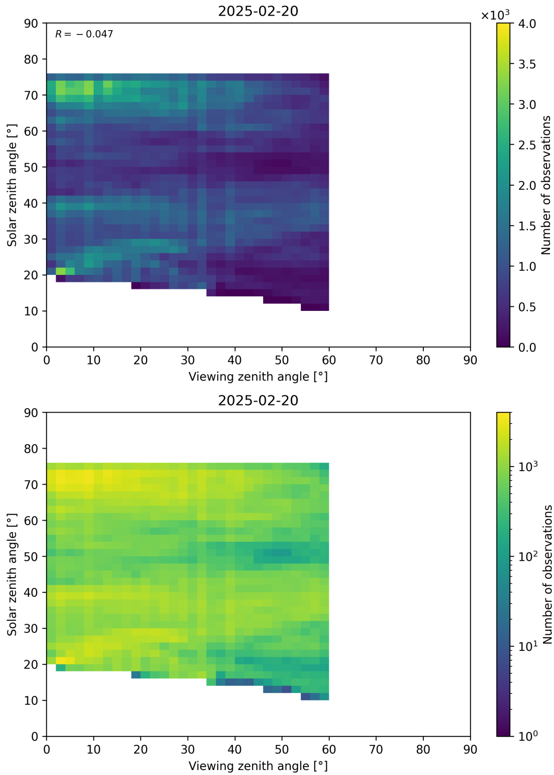
Figure 115: Scatter density plot of “Viewing zenith angle” against “Solar zenith angle” for 2025-02-19 to 2025-02-21.
