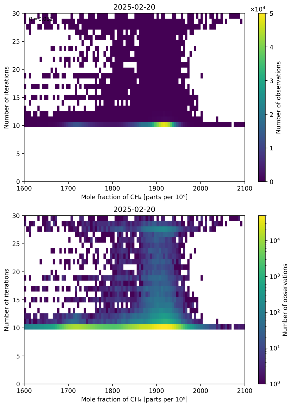
Figure 76: Scatter density plot of “Mole fraction of CH 4 ” against “Number of iterations” for 2025-02-19 to 2025-02-21.
