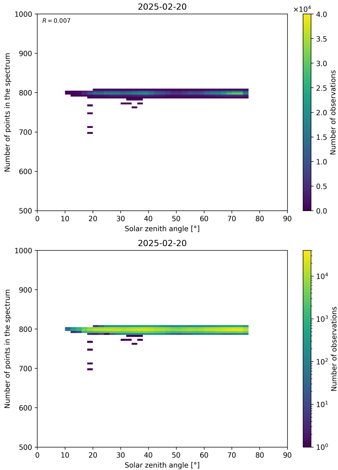
Figure 103: Scatter density plot of “Solar zenith angle” against “Number of points in the spectrum” for 2025-02-19 to 2025-02-21.
