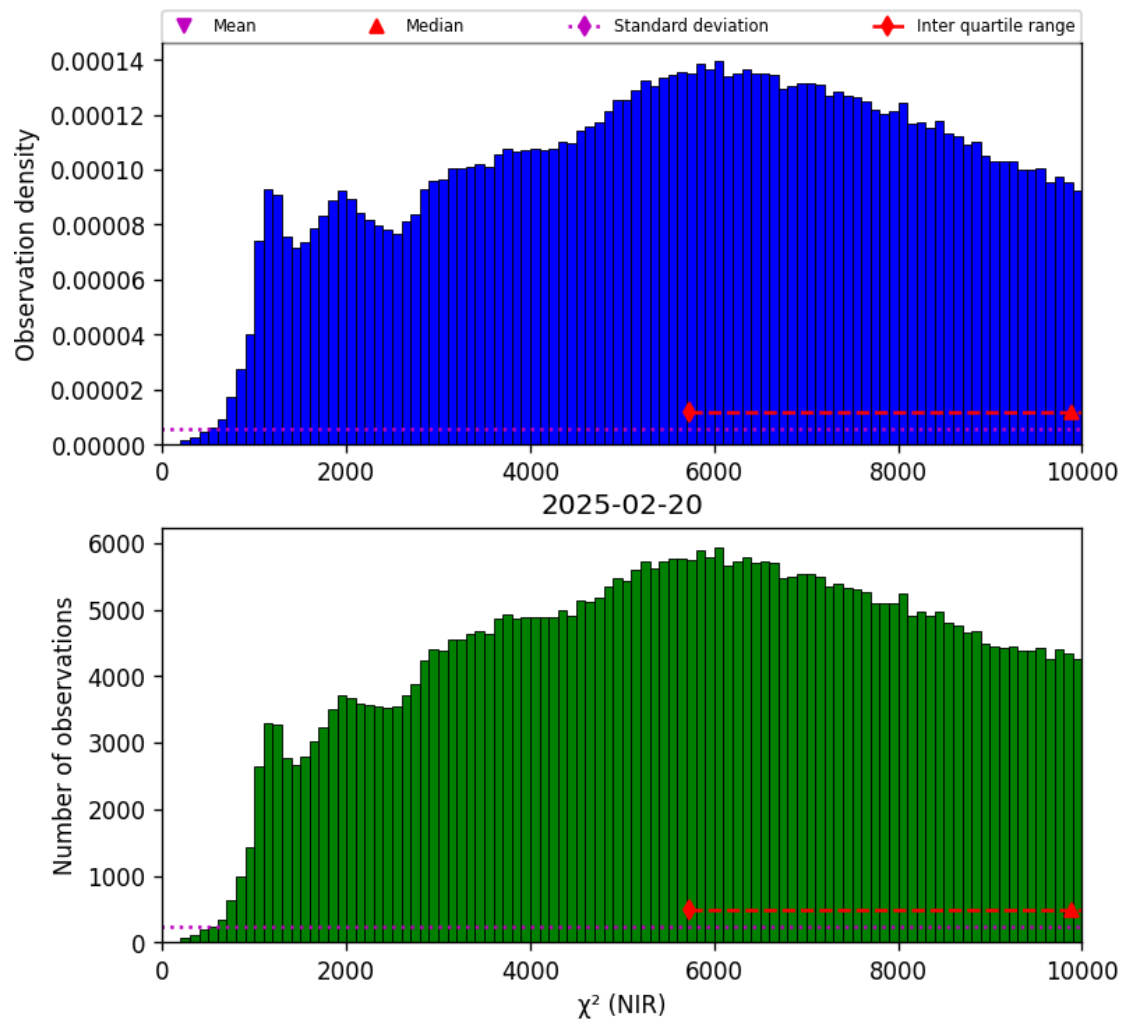
Figure 29: Histogram of “ \chi^2 (NIR)” for 2025-02-19 to 2025-02-21
