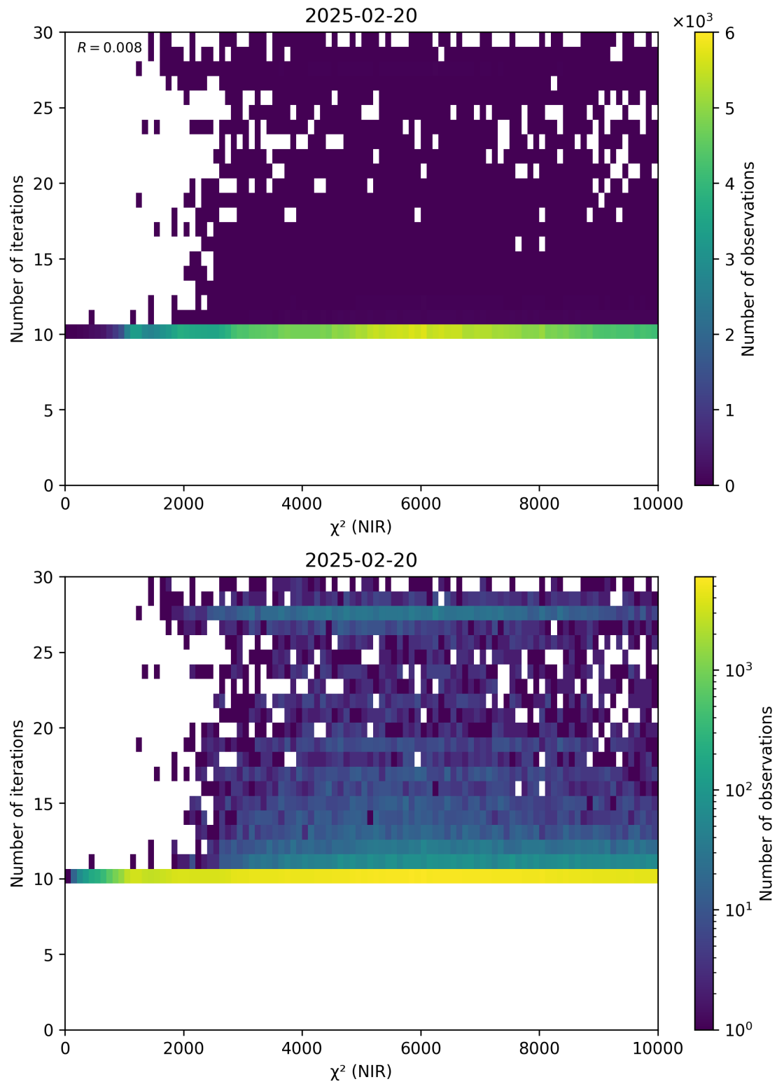
Figure 46: Scatter density plot of “ \chi^2 (NIR)” against “Number of iterations” for 2025-02-19 to 2025-02-21.
