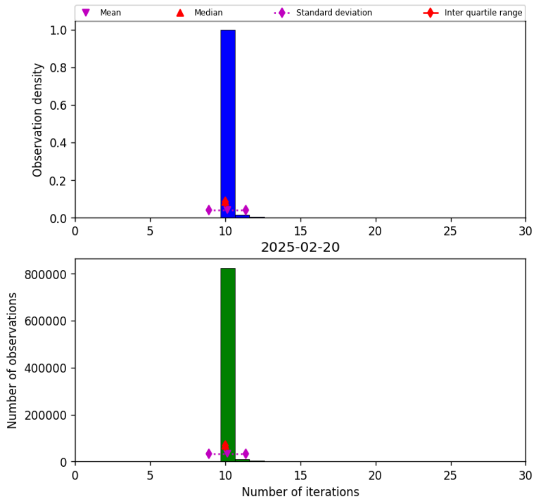
Figure 31: Histogram of “Number of iterations” for 2025-02-19 to 2025-02-21
