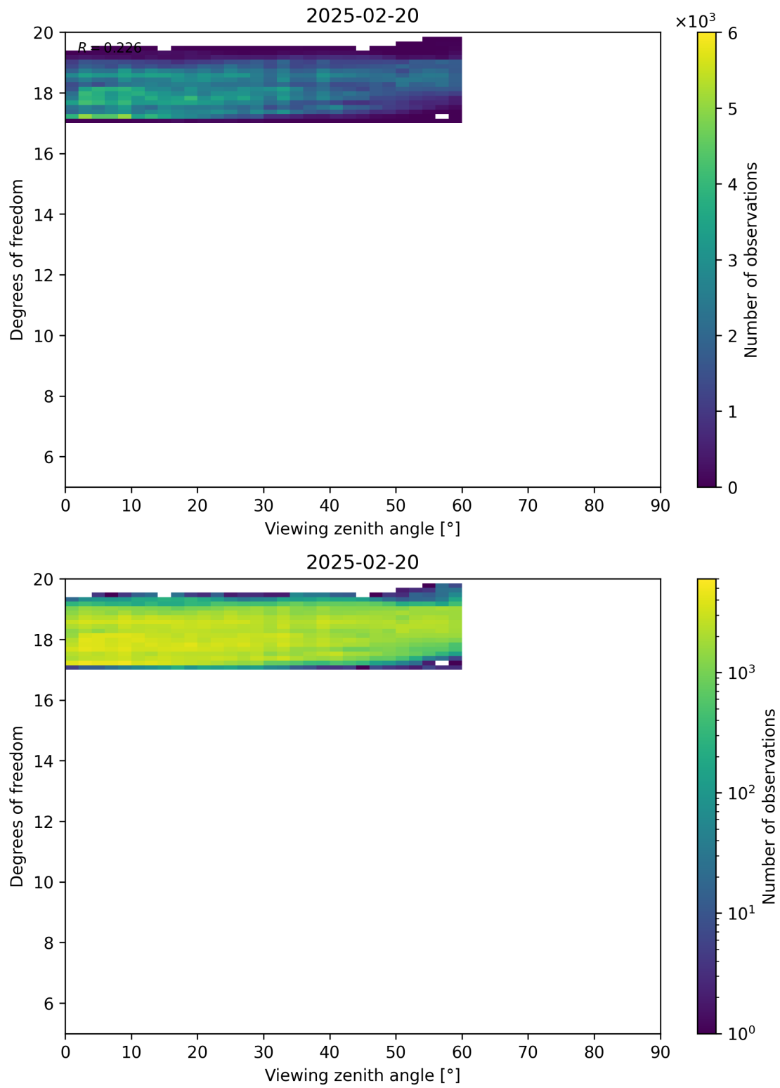
Figure 107: Scatter density plot of “Viewing zenith angle” against “Degrees of freedom” for 2025-02-19 to 2025-02-21.
