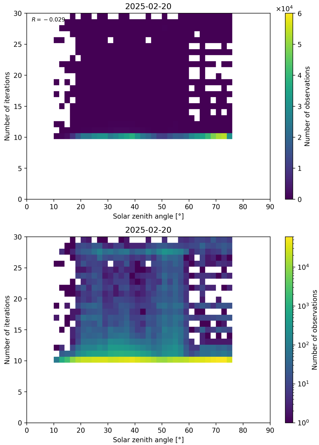
Figure 102: Scatter density plot of “Solar zenith angle” against “Number of iterations” for 2025-02-19 to 2025-02-21.
