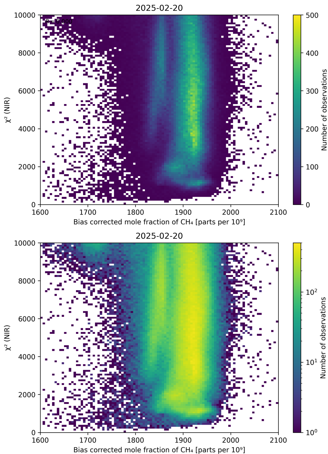
Figure 63: Scatter density plot of “Bias corrected mole fraction of \text{CH}_4 ” against “ \chi^2 (NIR)” for 2025-02-19 to 2025-02-21.
