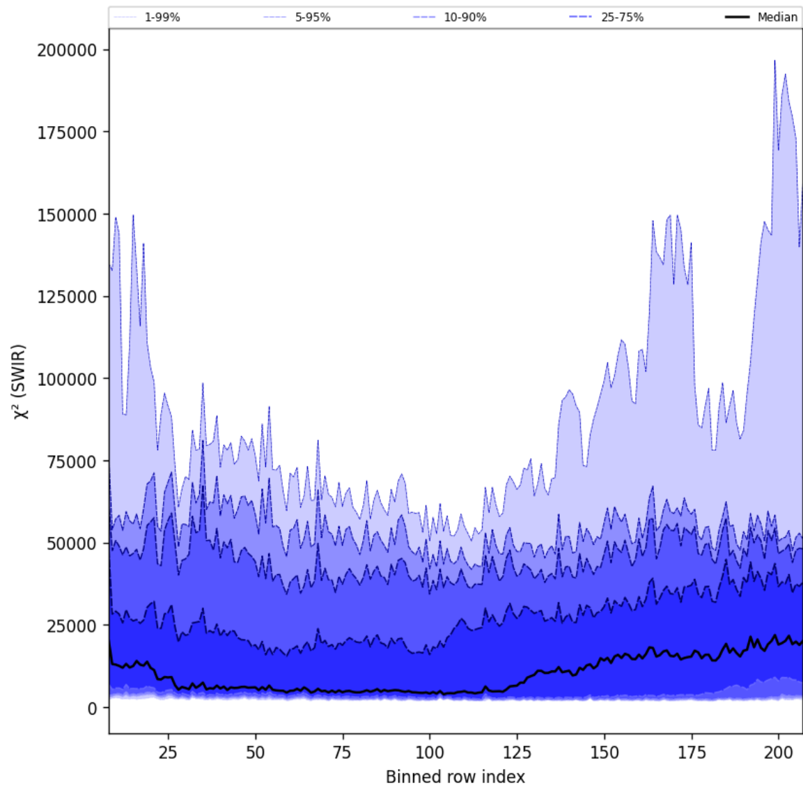
Figure 39: Along track statistics of “ \chi^2 (SWIR)” for 2025-02-19 to 2025-02-21
