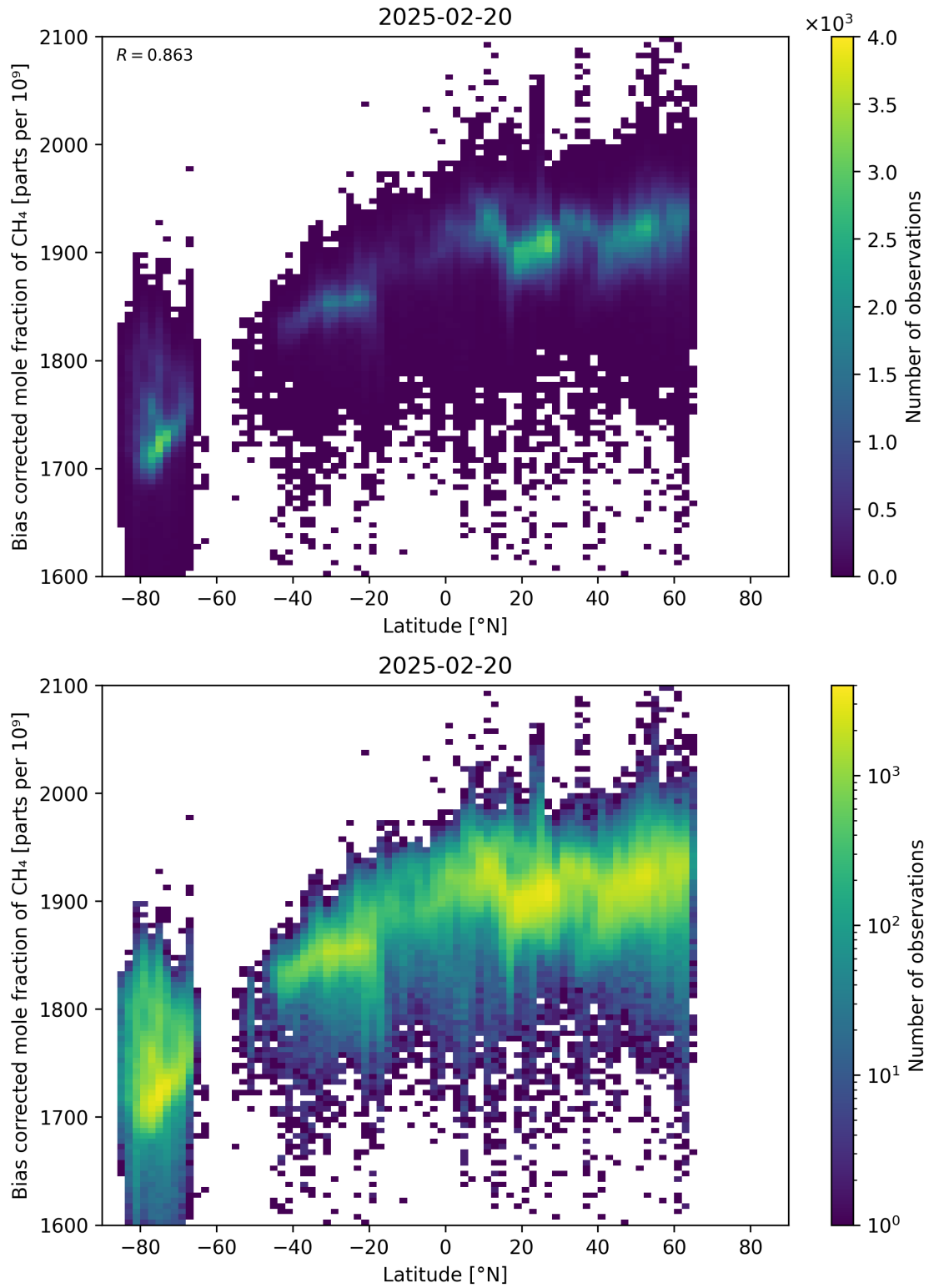
Figure 58: Scatter density plot of “Latitude” against “Bias corrected mole fraction of CH 4 ” for 2025-02-19 to 2025-02-21.
