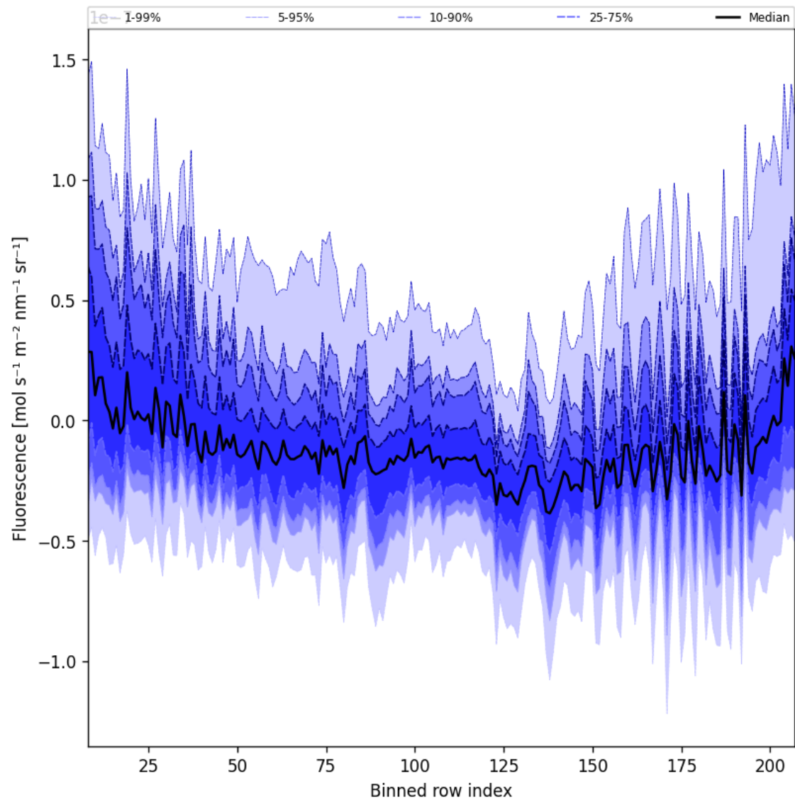
Figure 43: Along track statistics of “Fluorescence” for 2025-02-19 to 2025-02-21
