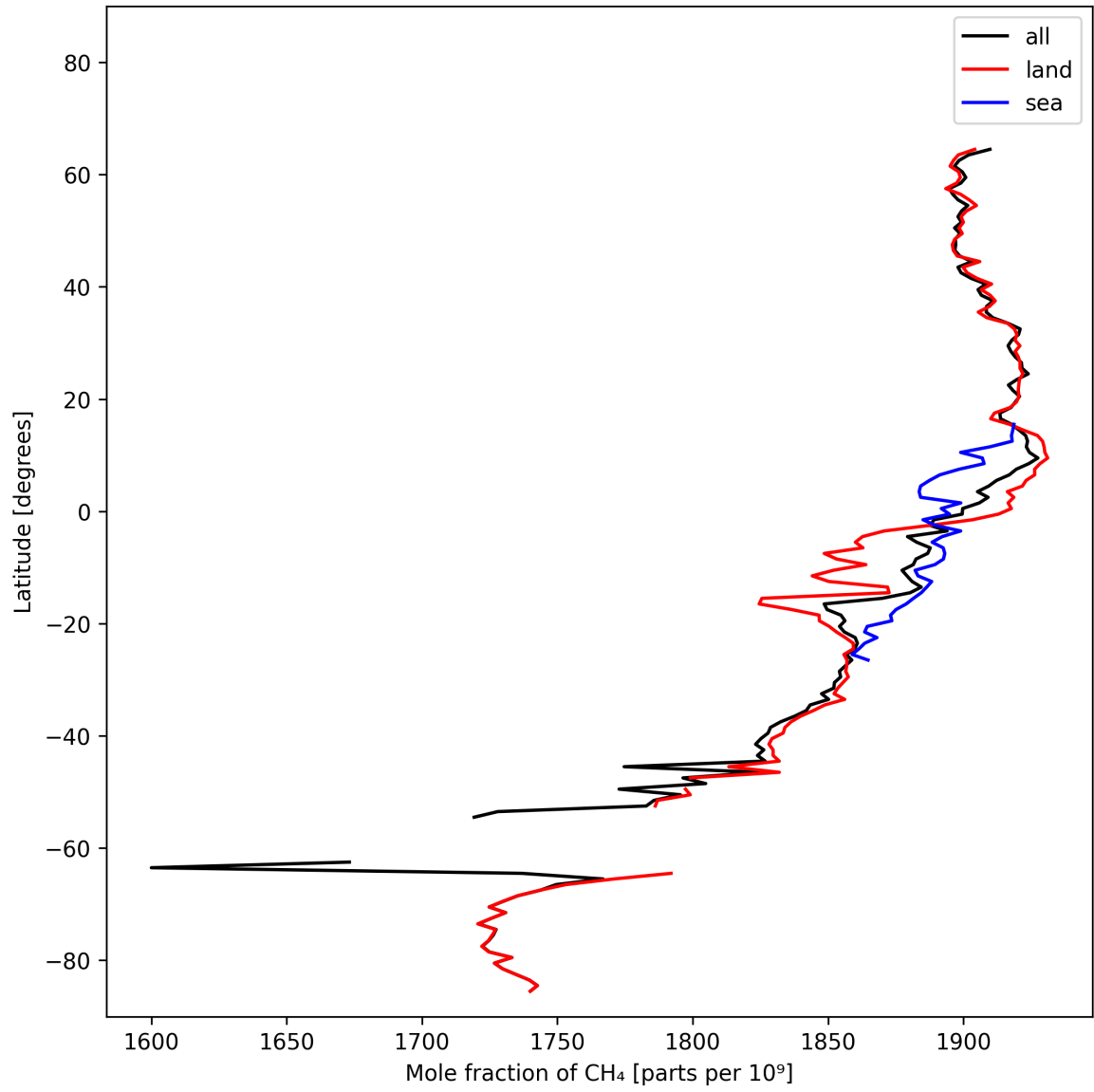
Figure 12: Zonal average of “Mole fraction of CH 4 ” for 2025-02-19 to 2025-02-21.
