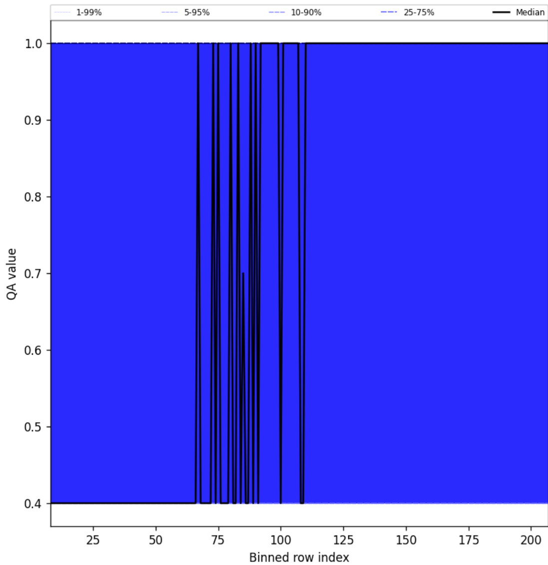
Figure 33: Along track statistics of “QA value” for 2025-02-19 to 2025-02-21
