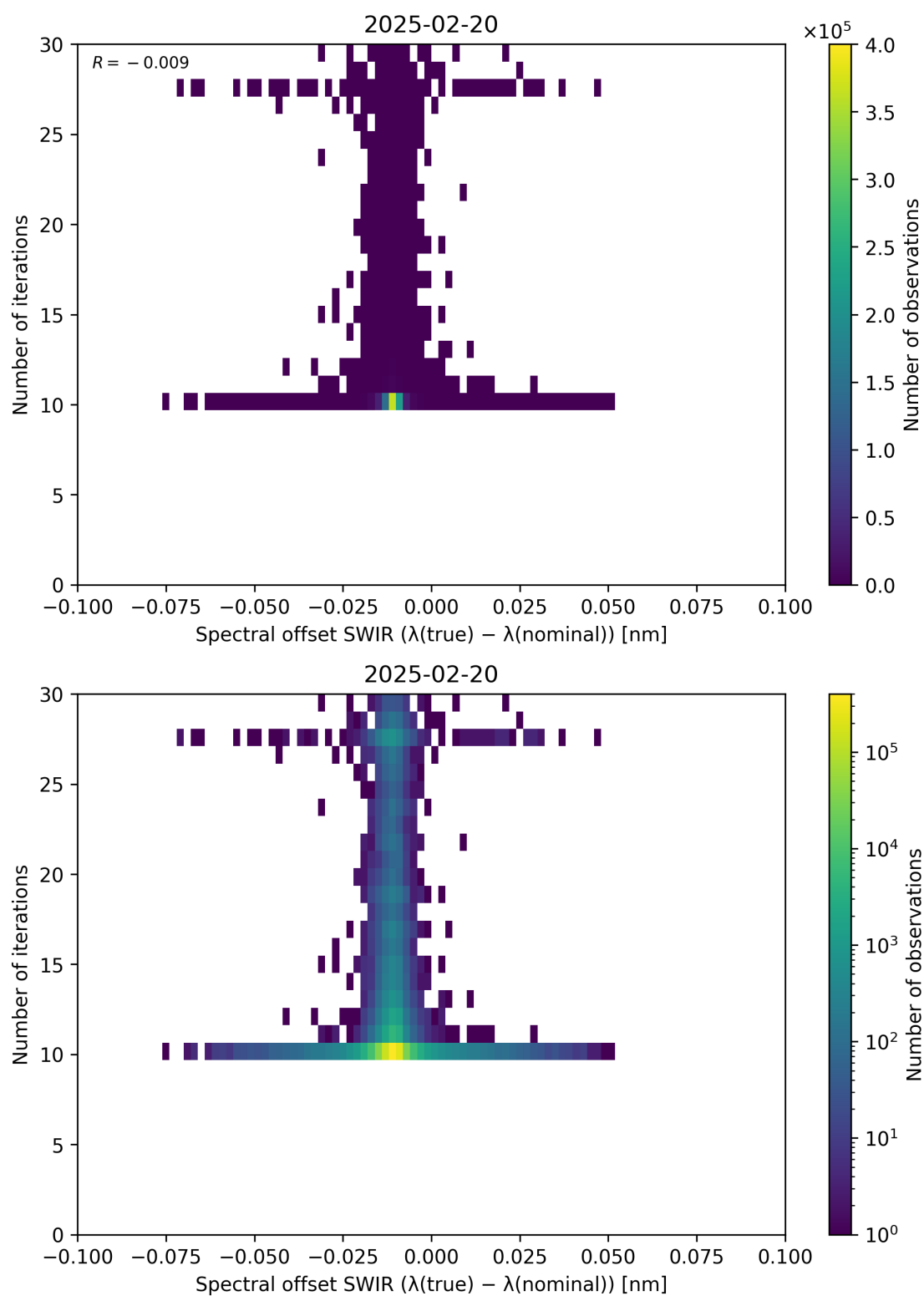
Figure 121: Scatter density plot of “Spectral offset SWIR ( \lambda_{\text{true}} - \lambda_{\text{nominal}} )” against “Number of iterations” for 2025-02-19 to 2025-02-21.
