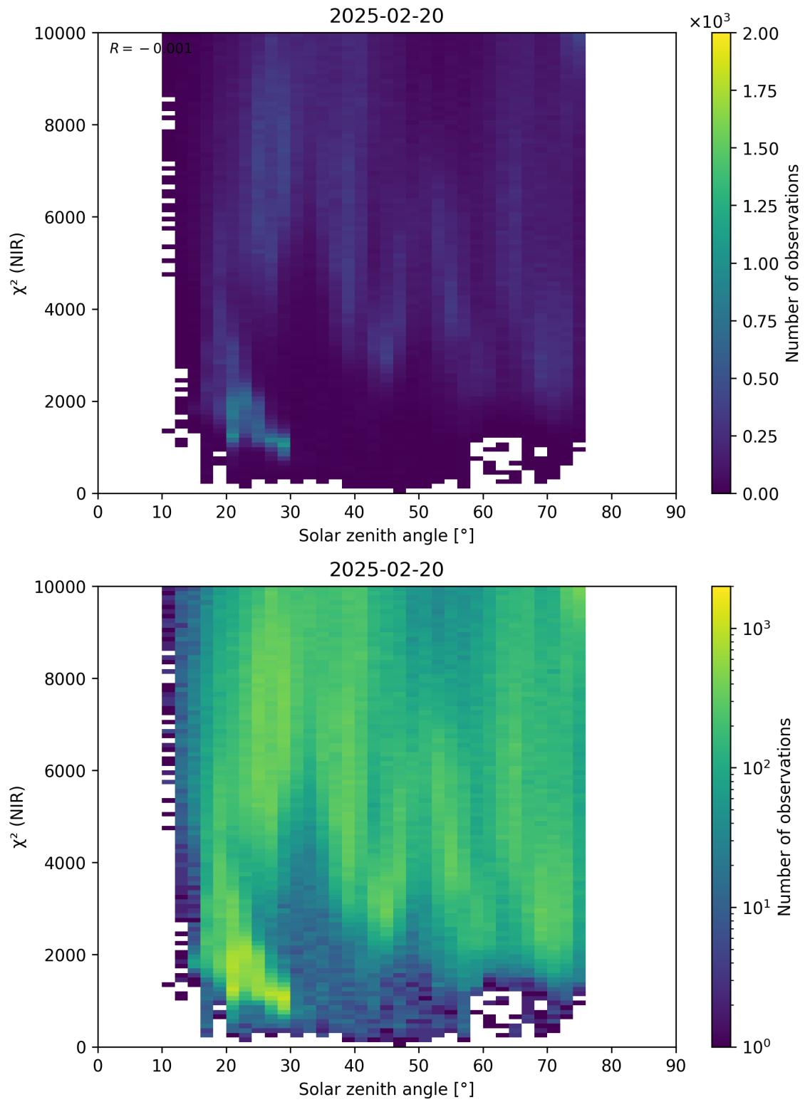
Figure 94: Scatter density plot of “Solar zenith angle” against “ \chi^2 (NIR)” for 2025-02-19 to 2025-02-21.
