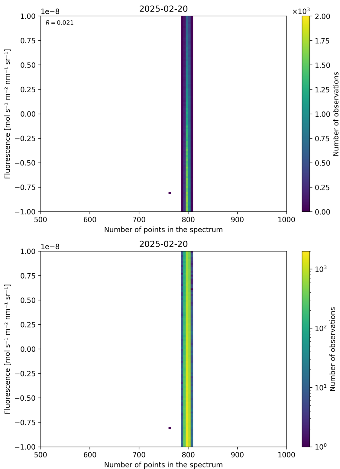
Figure 91: Scatter density plot of “Number of points in the spectrum” against “Fluorescence” for 2025-02-19 to 2025-02-21.
