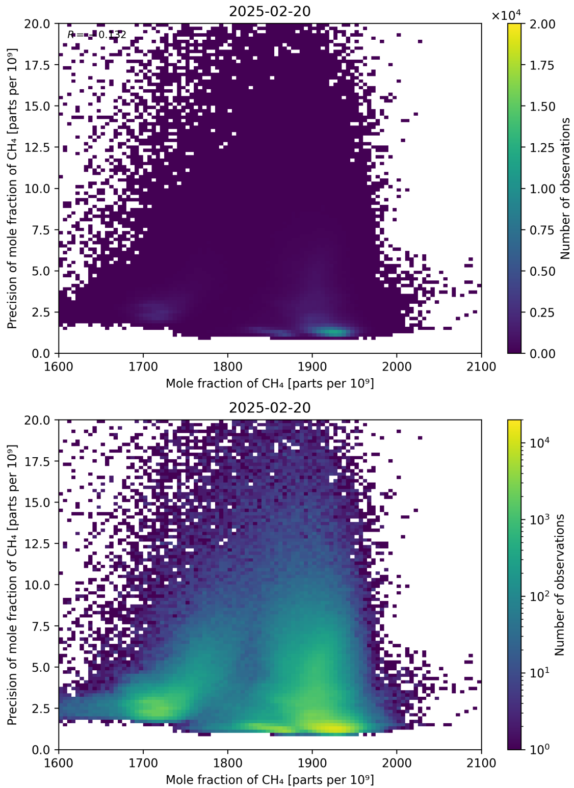
Figure 75: Scatter density plot of “Mole fraction of CH 4 ” against “Precision of mole fraction of CH 4 ” for 2025-02-19 to 2025-02-21.
