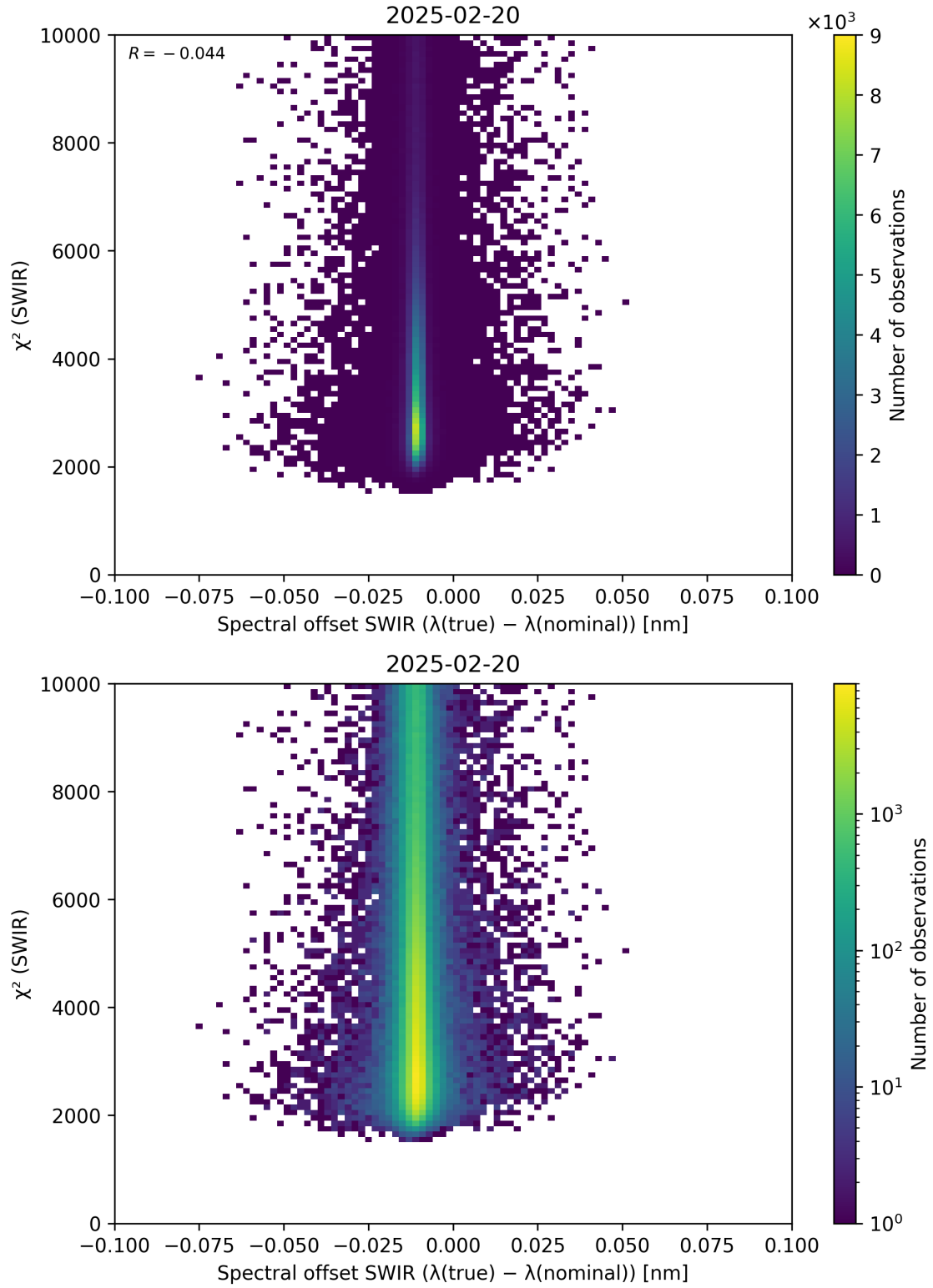
Figure 118: Scatter density plot of “Spectral offset SWIR ( \lambda_{\text{true}} - \lambda_{\text{nominal}} )” against “ \chi^2 (SWIR)” for 2025-02-19 to 2025-02-21.
