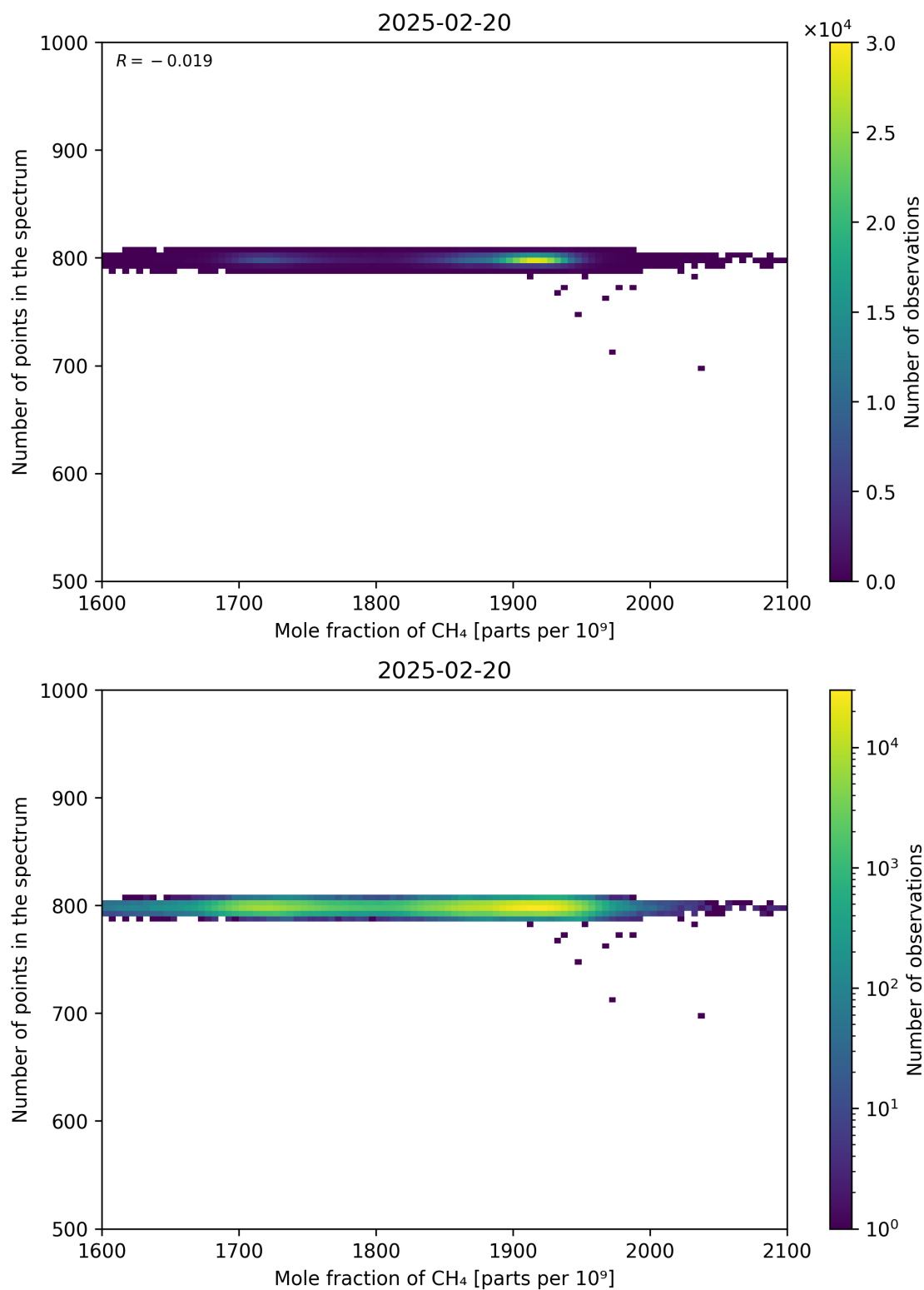
Figure 77: Scatter density plot of “Mole fraction of CH 4 ” against “Number of points in the spectrum” for 2025-02-19 to 2025-02-21.
