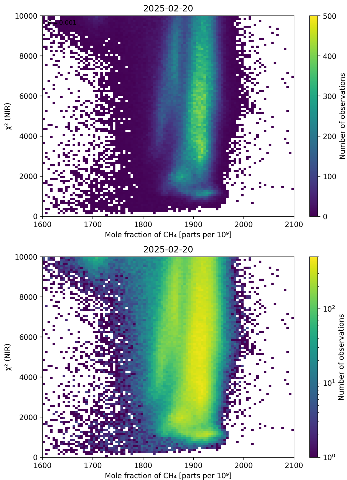
Figure 70: Scatter density plot of “Mole fraction of CH 4 ” against “ \chi^2 (NIR)” for 2025-02-19 to 2025-02-21.
