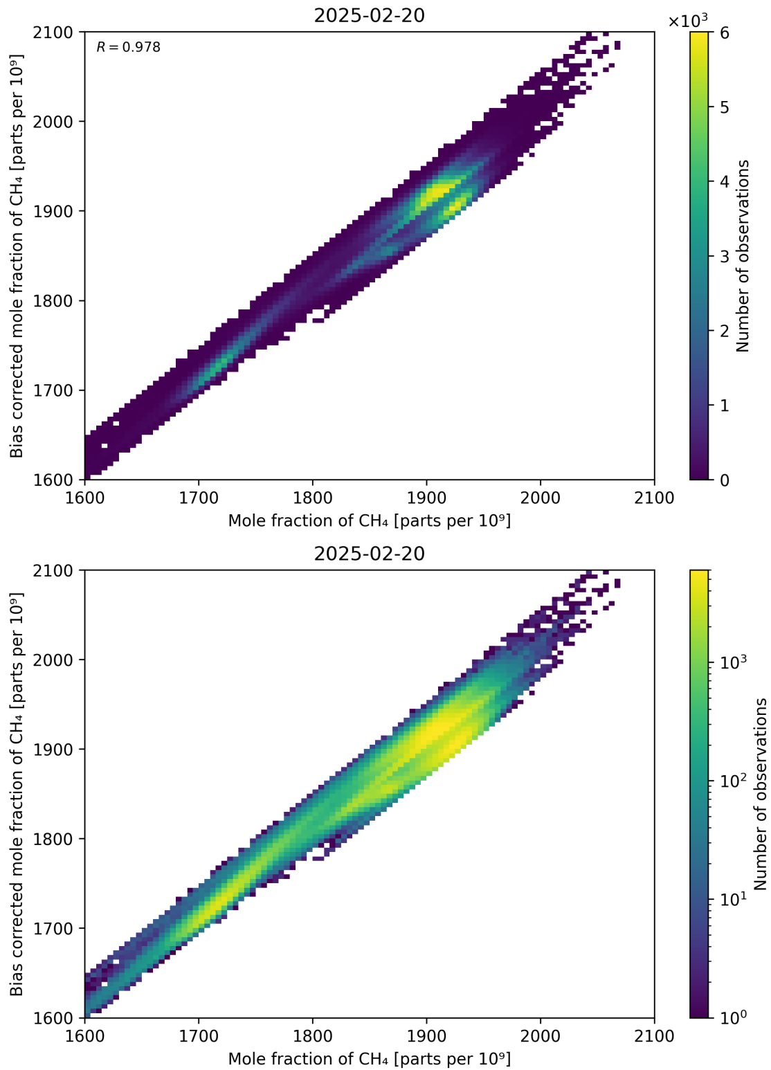
Figure 74: Scatter density plot of “Mole fraction of CH 4 ” against “Bias corrected mole fraction of CH 4 ” for 2025-02-19 to 2025-02-21.
