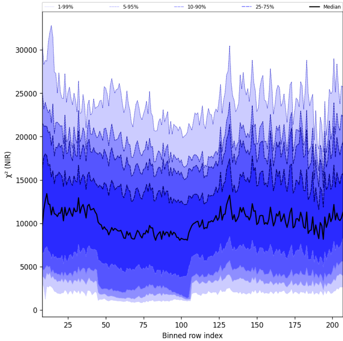
Figure 40: Along track statistics of “ \chi^2 (NIR)” for 2025-02-20 to 2025-02-22
