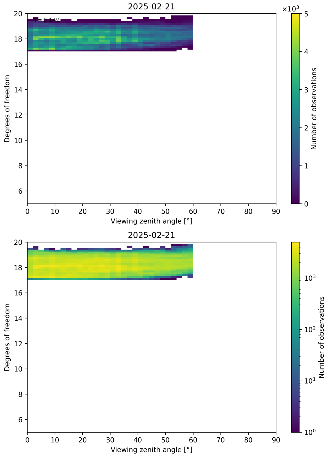
Figure 107: Scatter density plot of “Viewing zenith angle” against “Degrees of freedom” for 2025-02-20 to 2025-02-22.
