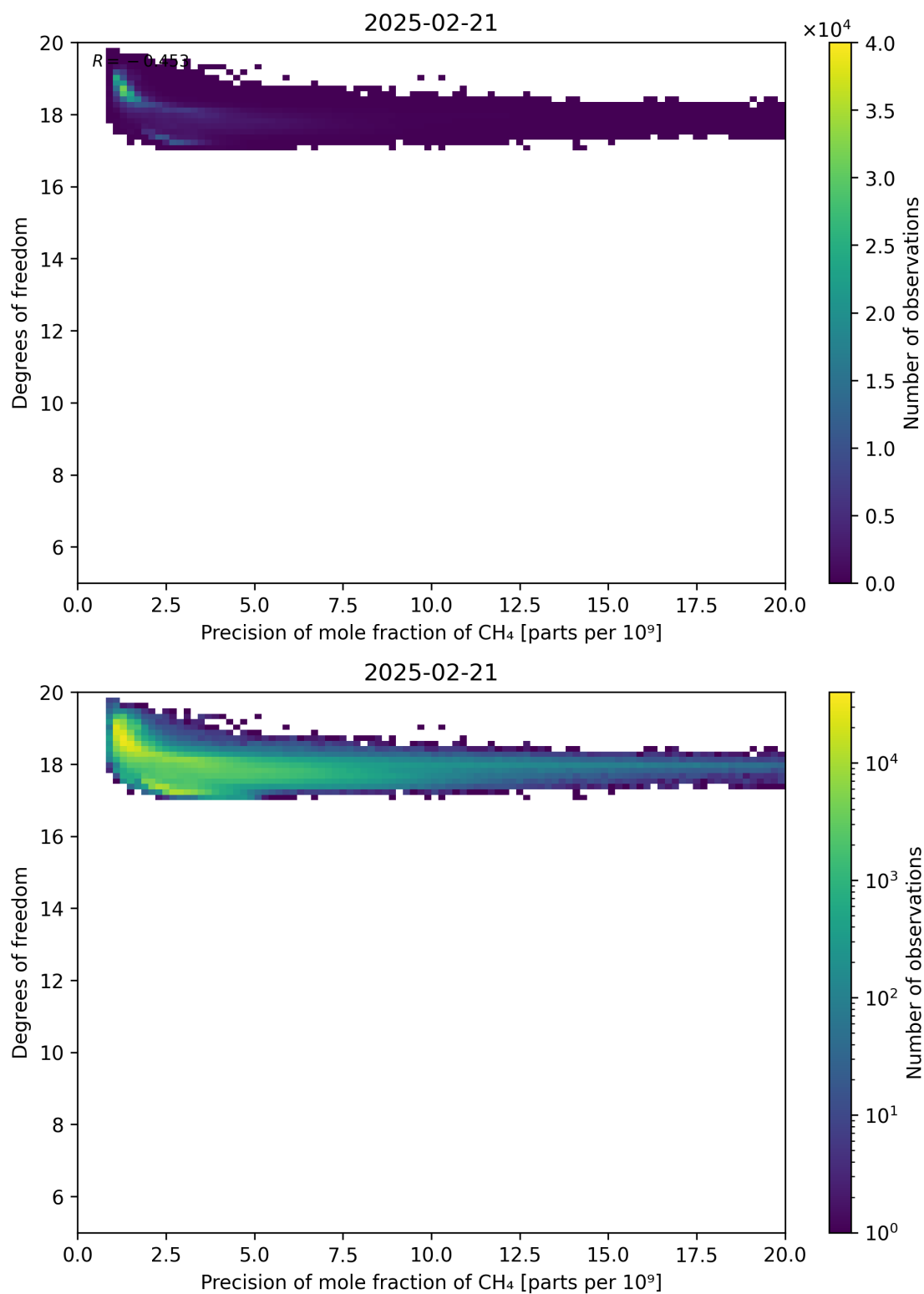
Figure 80: Scatter density plot of “Precision of mole fraction of CH 4 ” against “Degrees of freedom” for 2025-02-20 to 2025-02-22.
