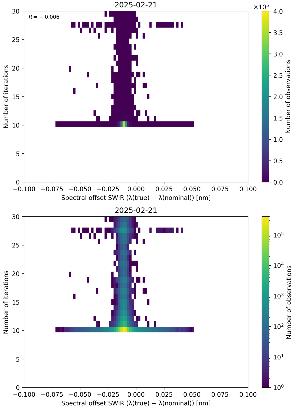
Figure 121: Scatter density plot of “Spectral offset SWIR ( \lambda_{\text{true}} - \lambda_{\text{nominal}} )” against “Number of iterations” for 2025-02-20 to 2025-02-22.
