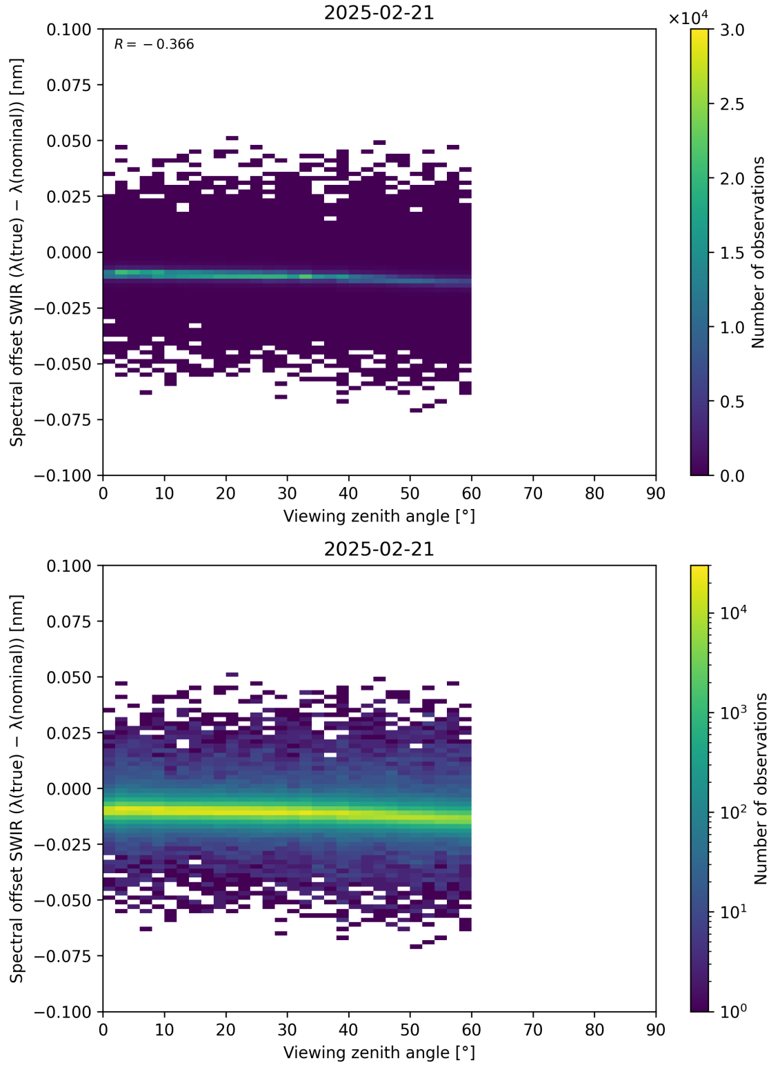
Figure 116: Scatter density plot of “Viewing zenith angle” against “Spectral offset SWIR ( \lambda_{\text{true}} - \lambda_{\text{nominal}} )” for 2025-02-20 to 2025-02-22.
