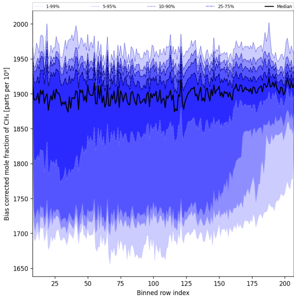
Figure 36: Along track statistics of “Bias corrected mole fraction of CH 4 ” for 2025-02-20 to 2025-02-22
