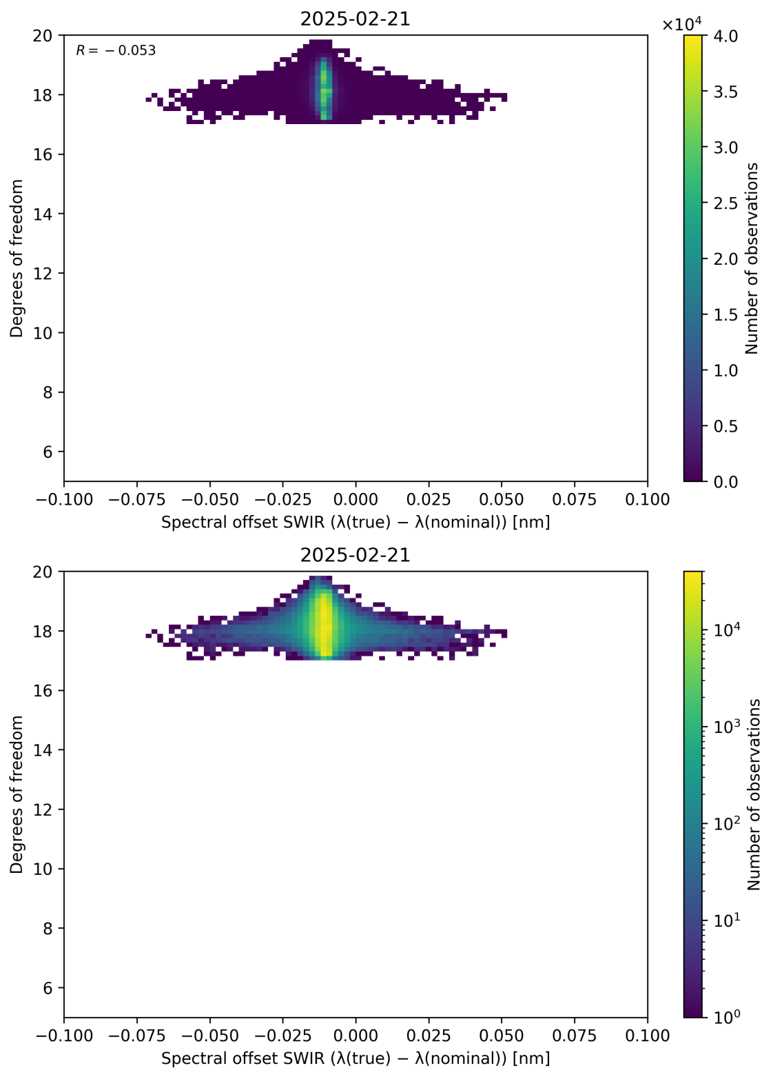
Figure 119: Scatter density plot of “Spectral offset SWIR ( \lambda_{\text{true}} - \lambda_{\text{nominal}} )” against “Degrees of freedom” for 2025-02-20 to 2025-02-22.
