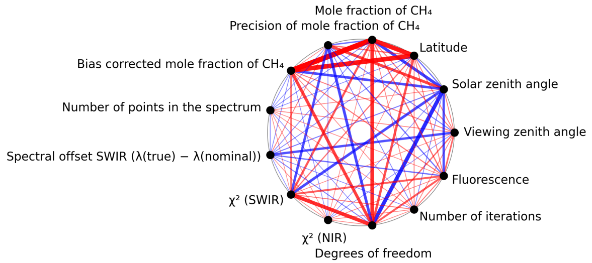
Figure 1: Map of correlation graph for 2025-02-20 to 2025-02-22.
