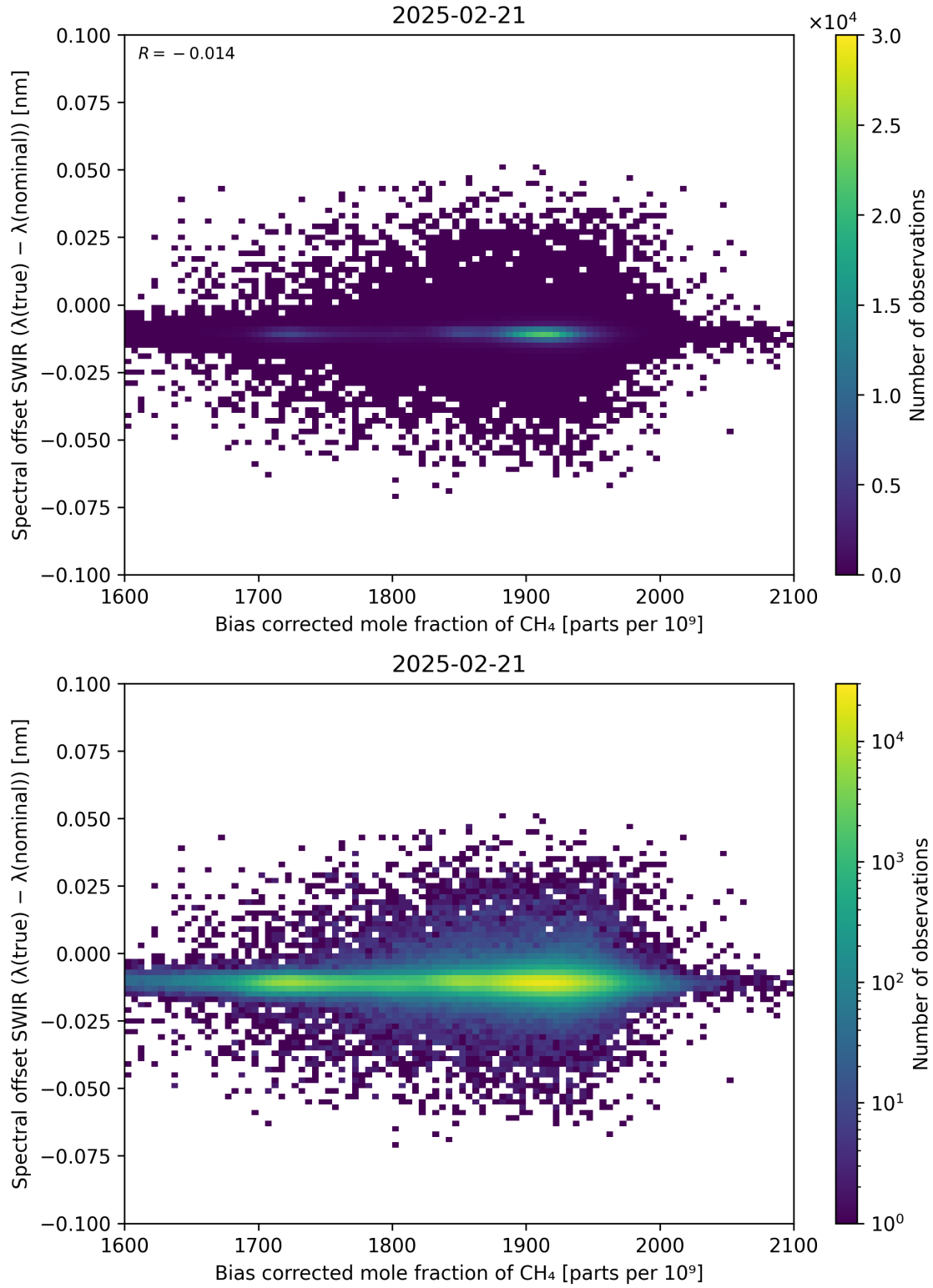
Figure 69: Scatter density plot of “Bias corrected mole fraction of CH 4 ” against “Spectral offset SWIR ( \lambda_{\text{true}} - \lambda_{\text{nominal}} )” for 2025-02-20 to 2025-02-22.
