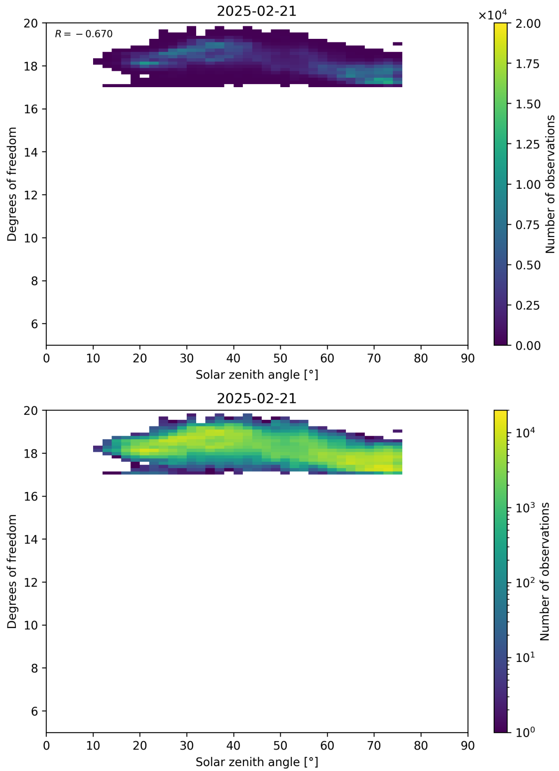
Figure 96: Scatter density plot of “Solar zenith angle” against “Degrees of freedom” for 2025-02-20 to 2025-02-22.
