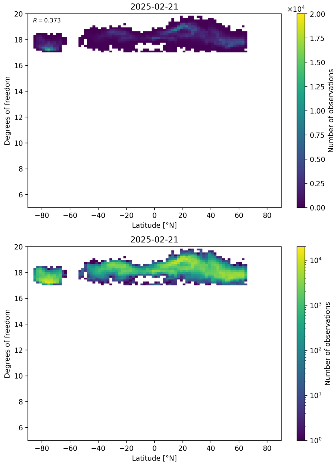
Figure 55: Scatter density plot of “Latitude” against “Degrees of freedom” for 2025-02-20 to 2025-02-22.
