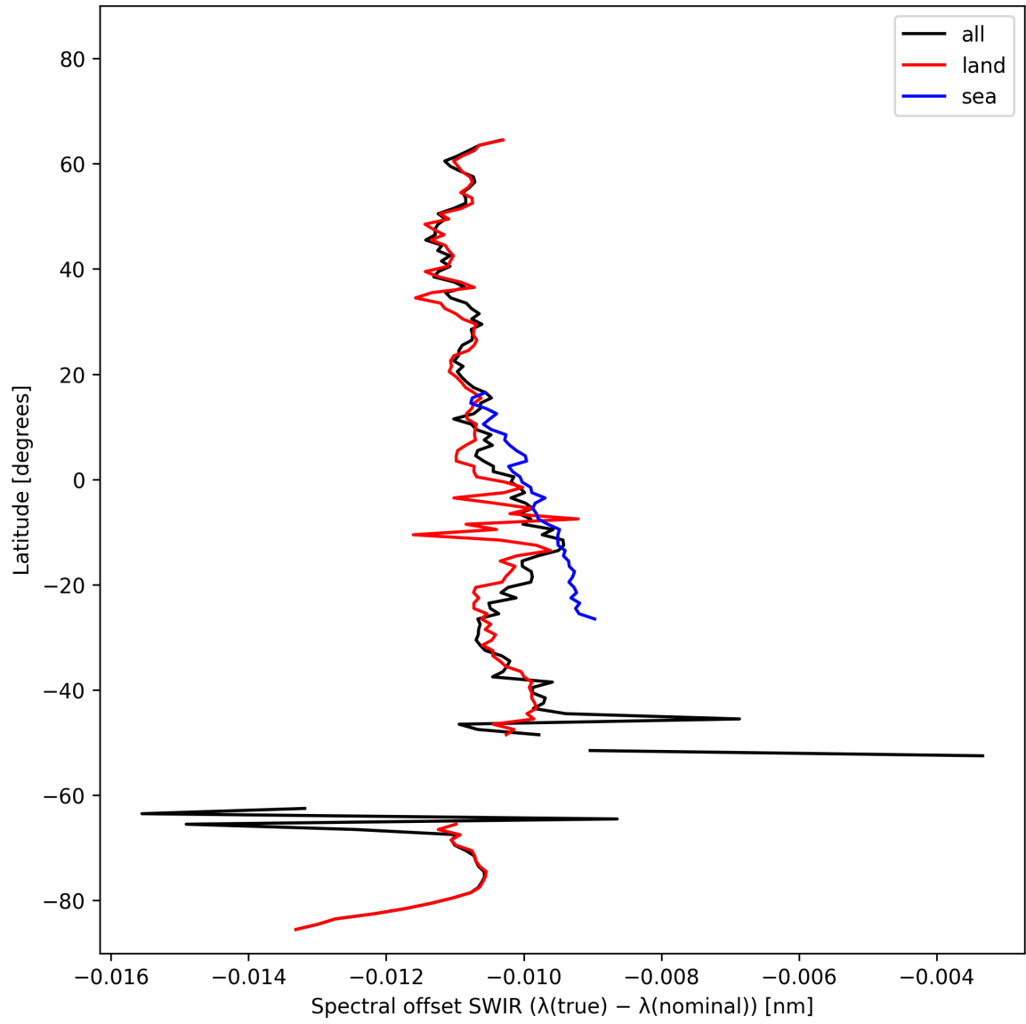
Figure 16: Zonal average of “Spectral offset SWIR ( \lambda_{\text{true}} - \lambda_{\text{nominal}} )” for 2025-02-20 to 2025-02-22.
