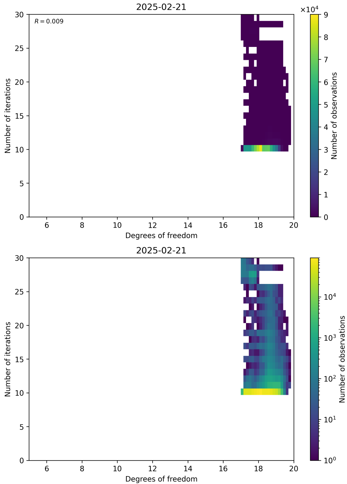
Figure 52: Scatter density plot of “Degrees of freedom” against “Number of iterations” for 2025-02-20 to 2025-02-22.
