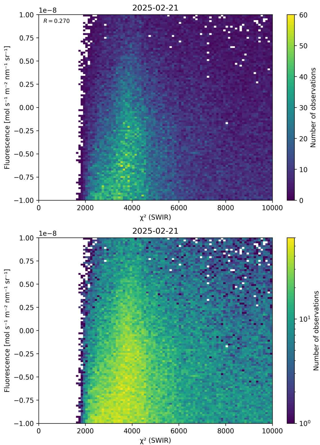
Figure 49: Scatter density plot of “ \chi^2 (SWIR)” against “Fluorescence” for 2025-02-20 to 2025-02-22.
