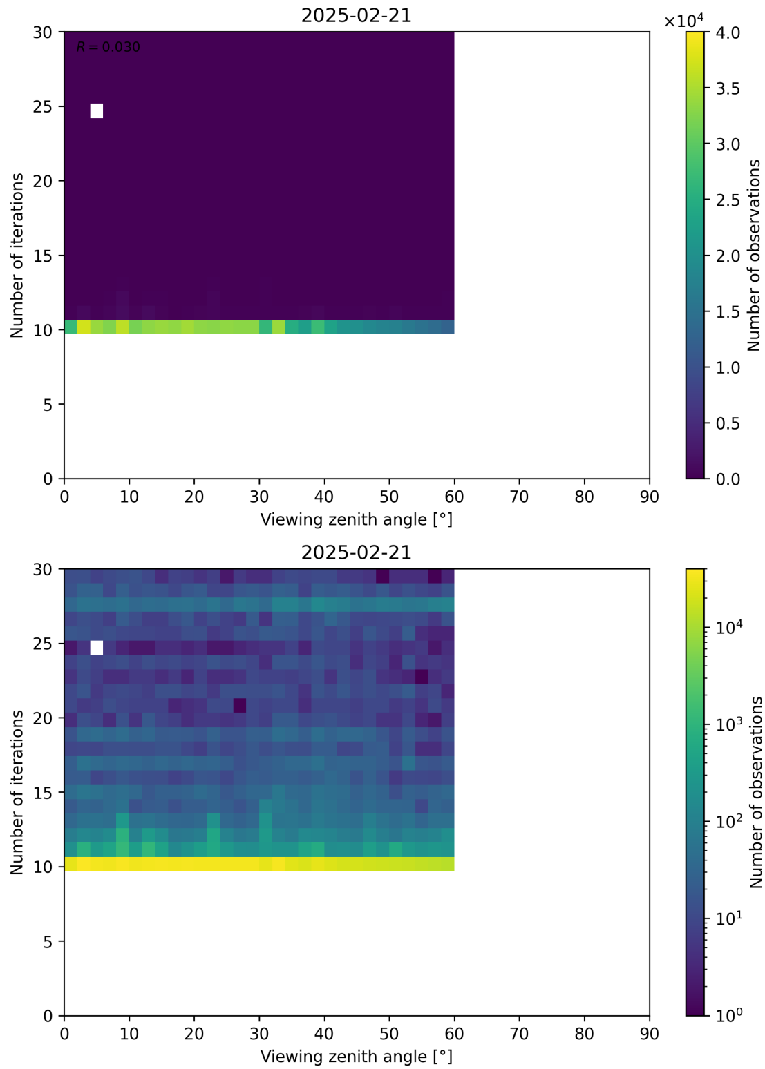
Figure 113: Scatter density plot of “Viewing zenith angle” against “Number of iterations” for 2025-02-20 to 2025-02-22.
