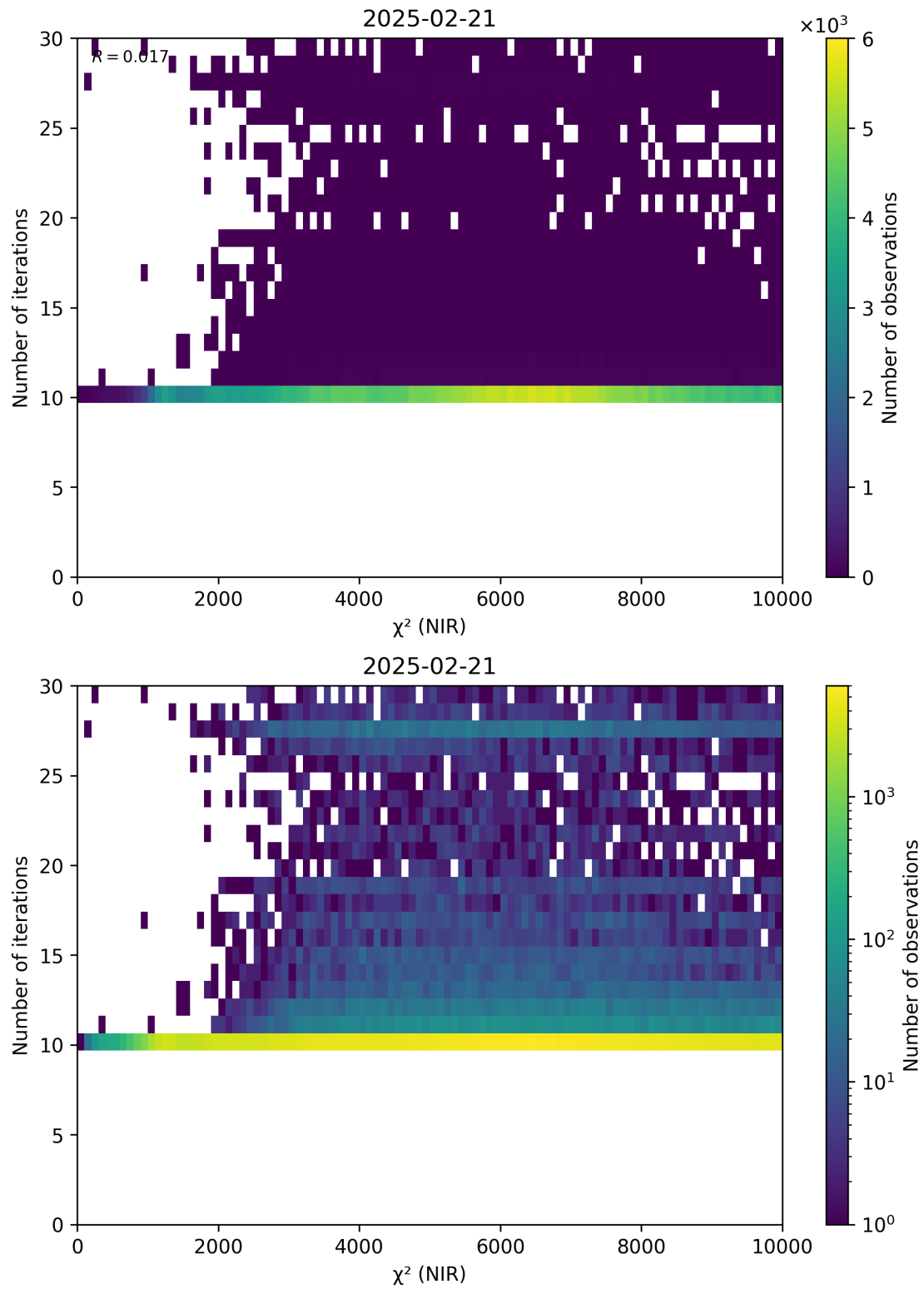
Figure 46: Scatter density plot of “ \chi^2 (NIR)” against “Number of iterations” for 2025-02-20 to 2025-02-22.
