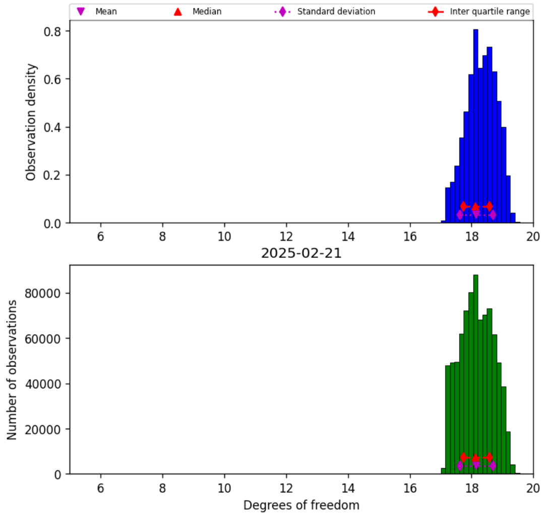
Figure 30: Histogram of “Degrees of freedom” for 2025-02-20 to 2025-02-22
