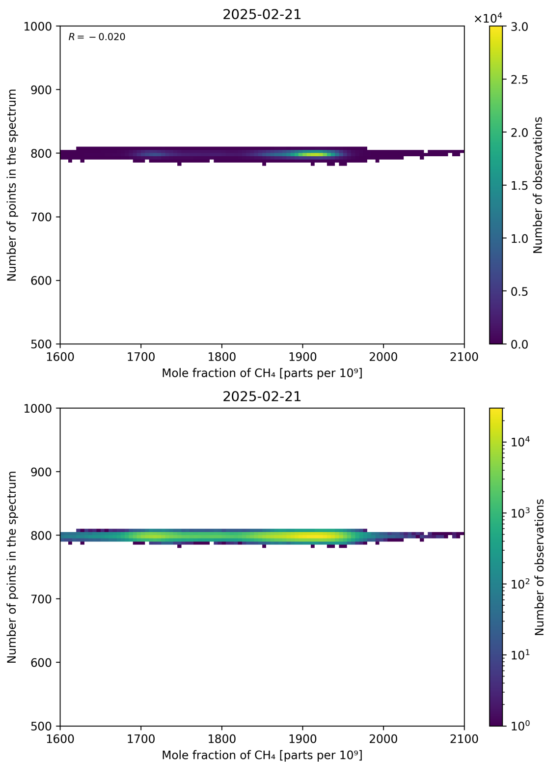
Figure 77: Scatter density plot of “Mole fraction of CH 4 ” against “Number of points in the spectrum” for 2025-02-20 to 2025-02-22.
