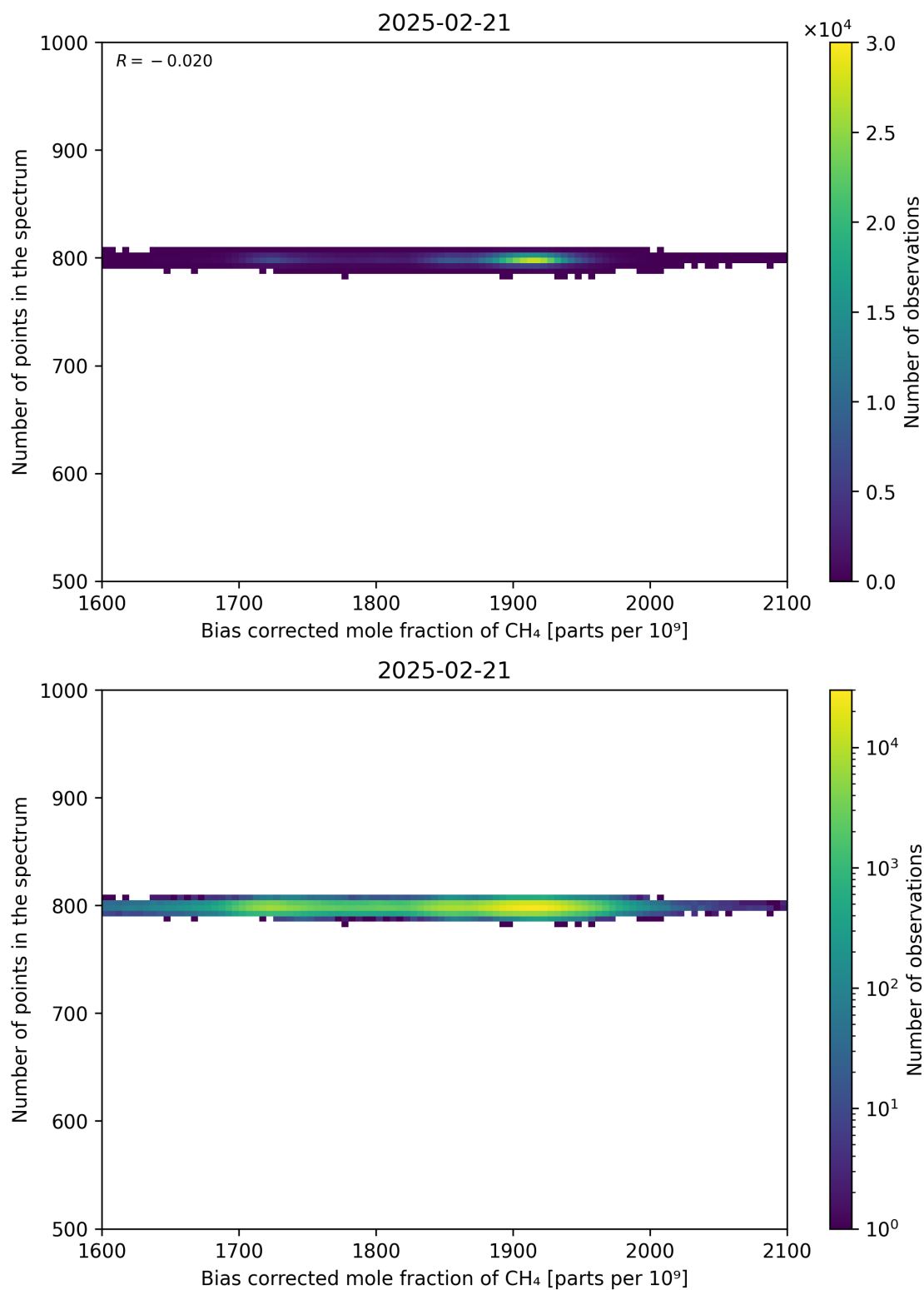
Figure 68: Scatter density plot of “Bias corrected mole fraction of CH 4 ” against “Number of points in the spectrum” for 2025-02-20 to 2025-02-22.
