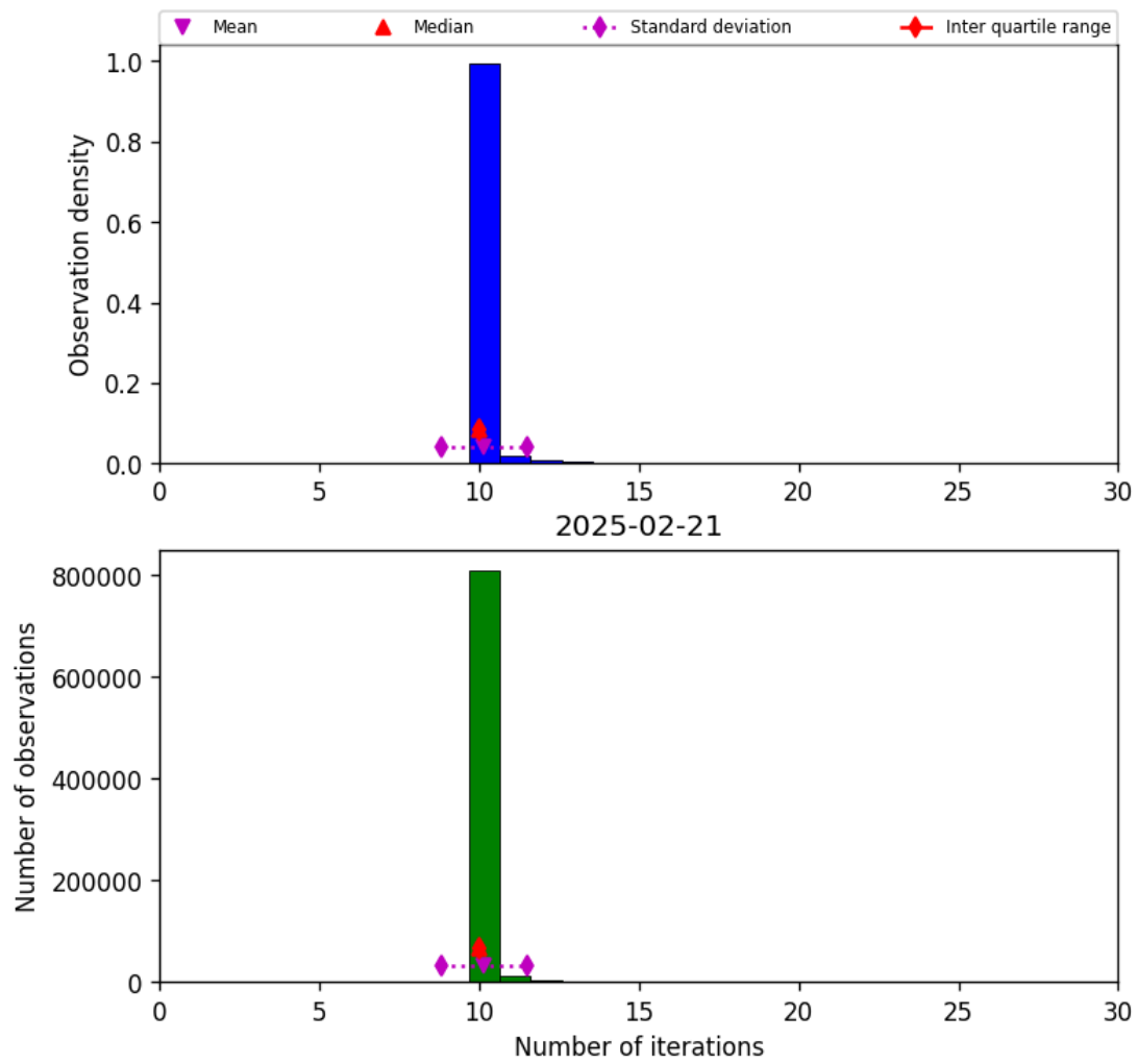
Figure 31: Histogram of “Number of iterations” for 2025-02-20 to 2025-02-22
