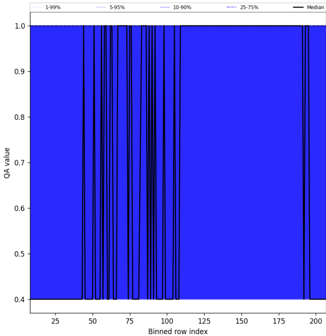
Figure 33: Along track statistics of “QA value” for 2025-02-20 to 2025-02-22
