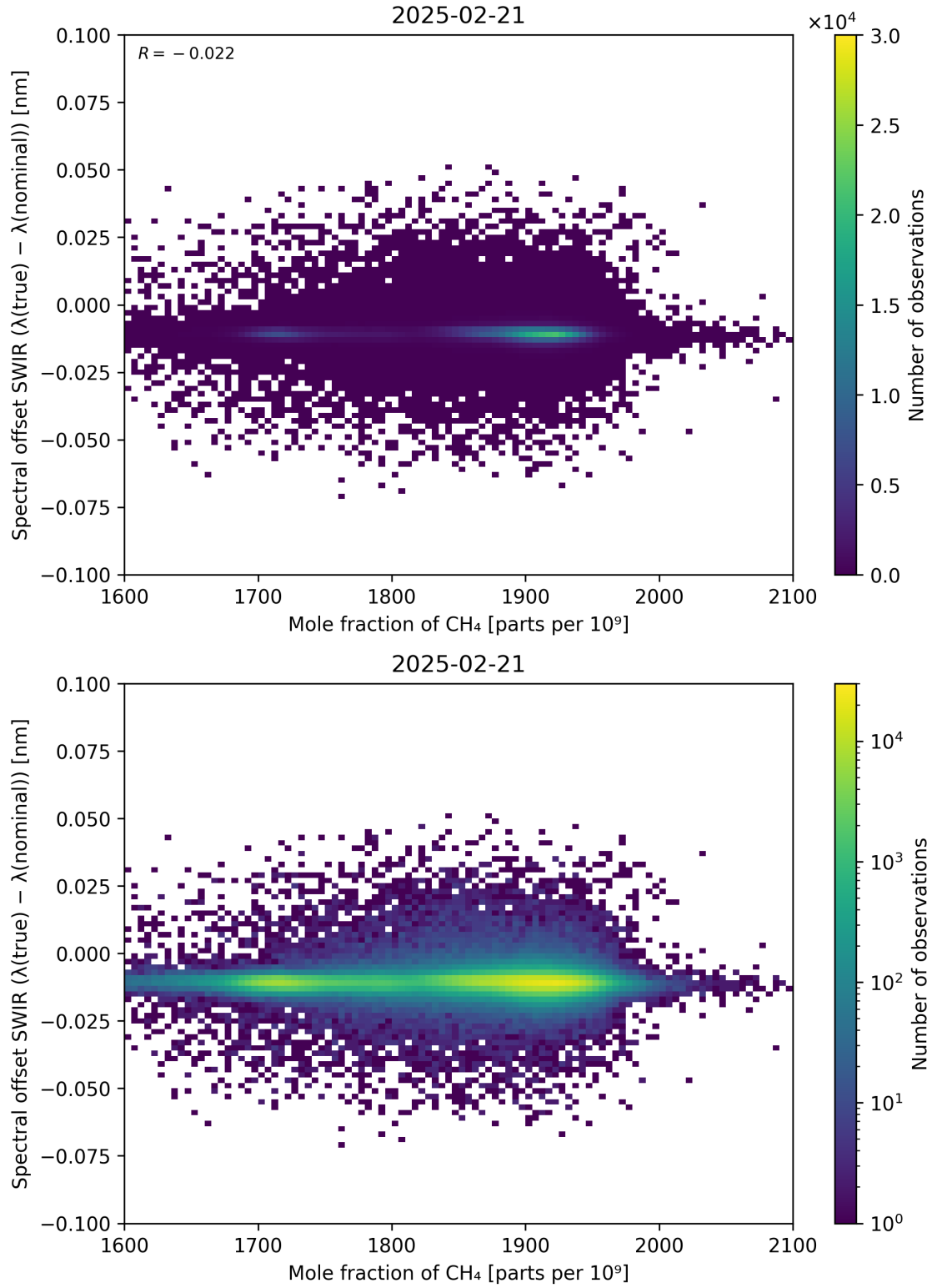
Figure 86: Scatter density plot of “Mole fraction of CH 4 ” against “Spectral offset SWIR ( \lambda_{\text{true}} - \lambda_{\text{nominal}} )” for 2025-02-20 to 2025-02-22.
