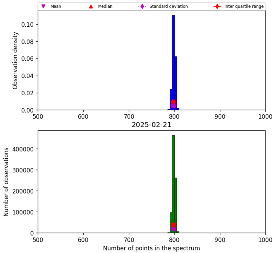
Figure 26: Histogram of “Number of points in the spectrum” for 2025-02-20 to 2025-02-22
