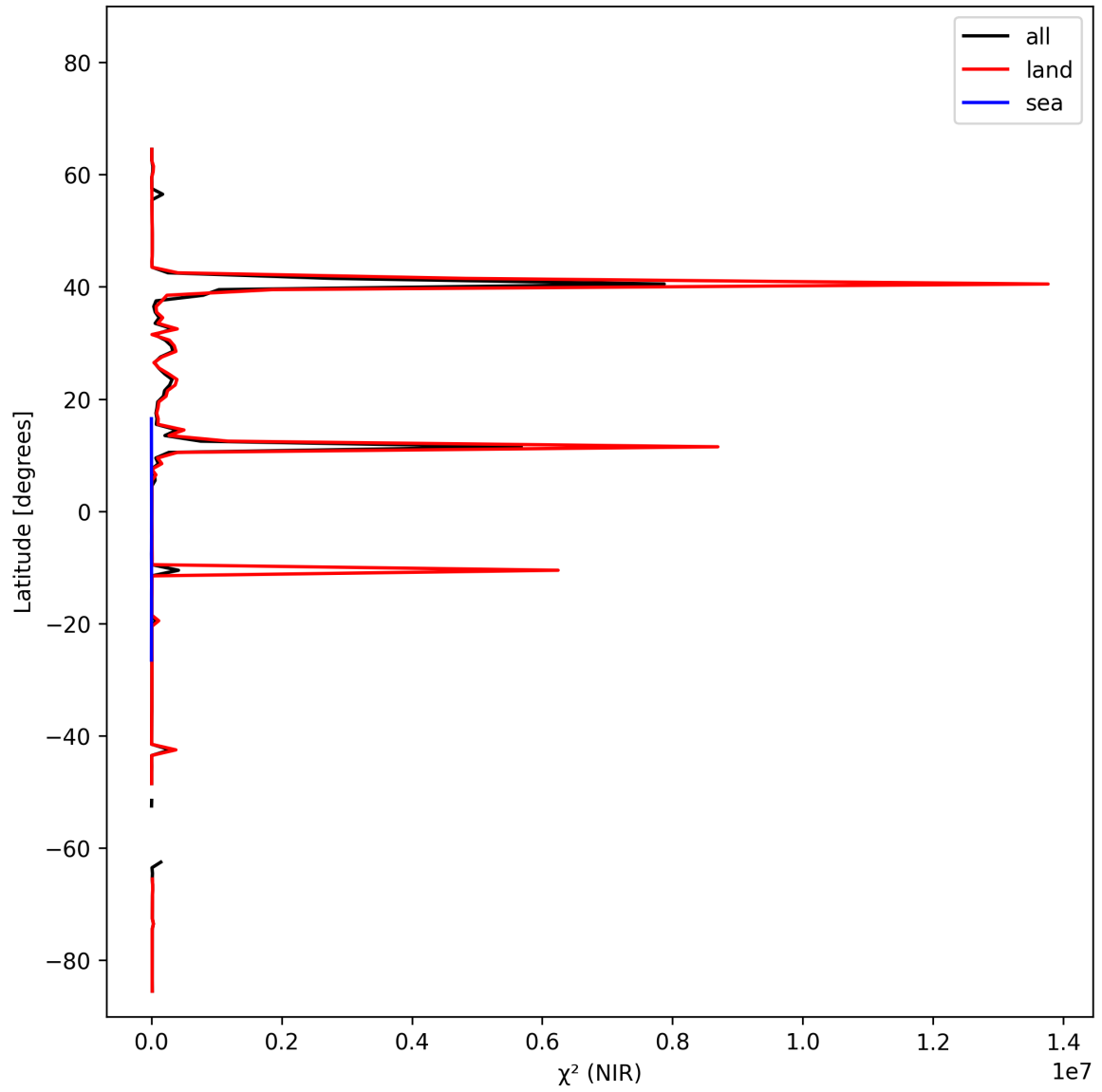
Figure 18: Zonal average of “ \chi^2 (NIR)” for 2025-02-20 to 2025-02-22.
