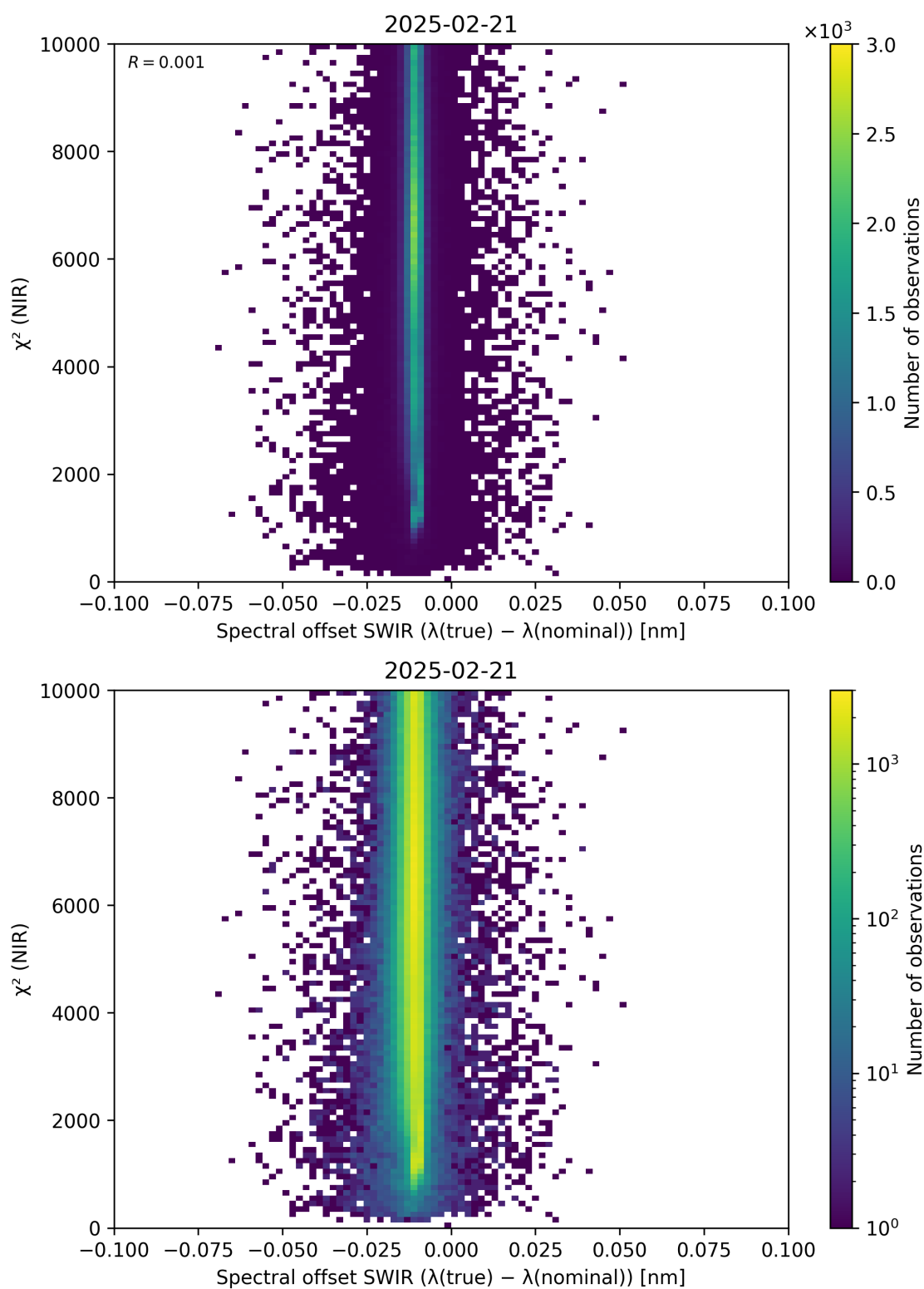
Figure 117: Scatter density plot of “Spectral offset SWIR ( \lambda_{\text{true}} - \lambda_{\text{nominal}} )” against “ \chi^2 (NIR)” for 2025-02-20 to 2025-02-22.
