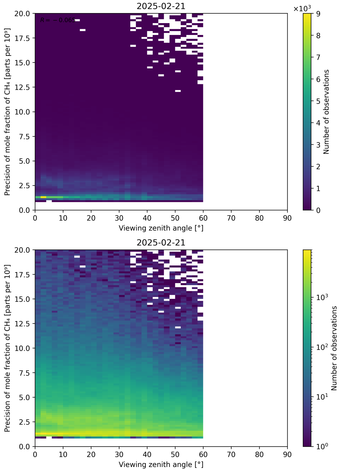
Figure 112: Scatter density plot of “Viewing zenith angle” against “Precision of mole fraction of CH 4 ” for 2025-02-20 to 2025-02-22.
