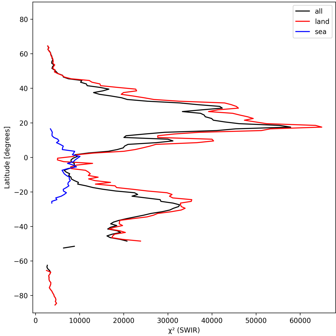
Figure 17: Zonal average of “ \chi^2 (SWIR)” for 2025-02-20 to 2025-02-22.
