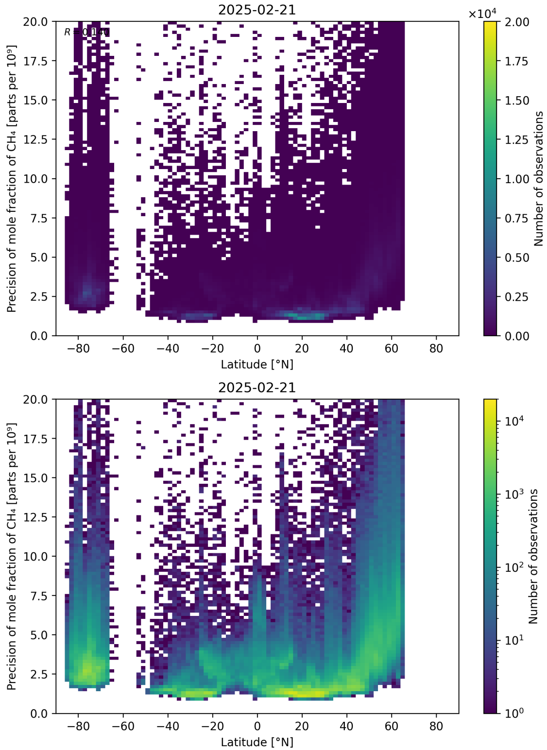
Figure 59: Scatter density plot of “Latitude” against “Precision of mole fraction of CH 4 ” for 2025-02-20 to 2025-02-22.
