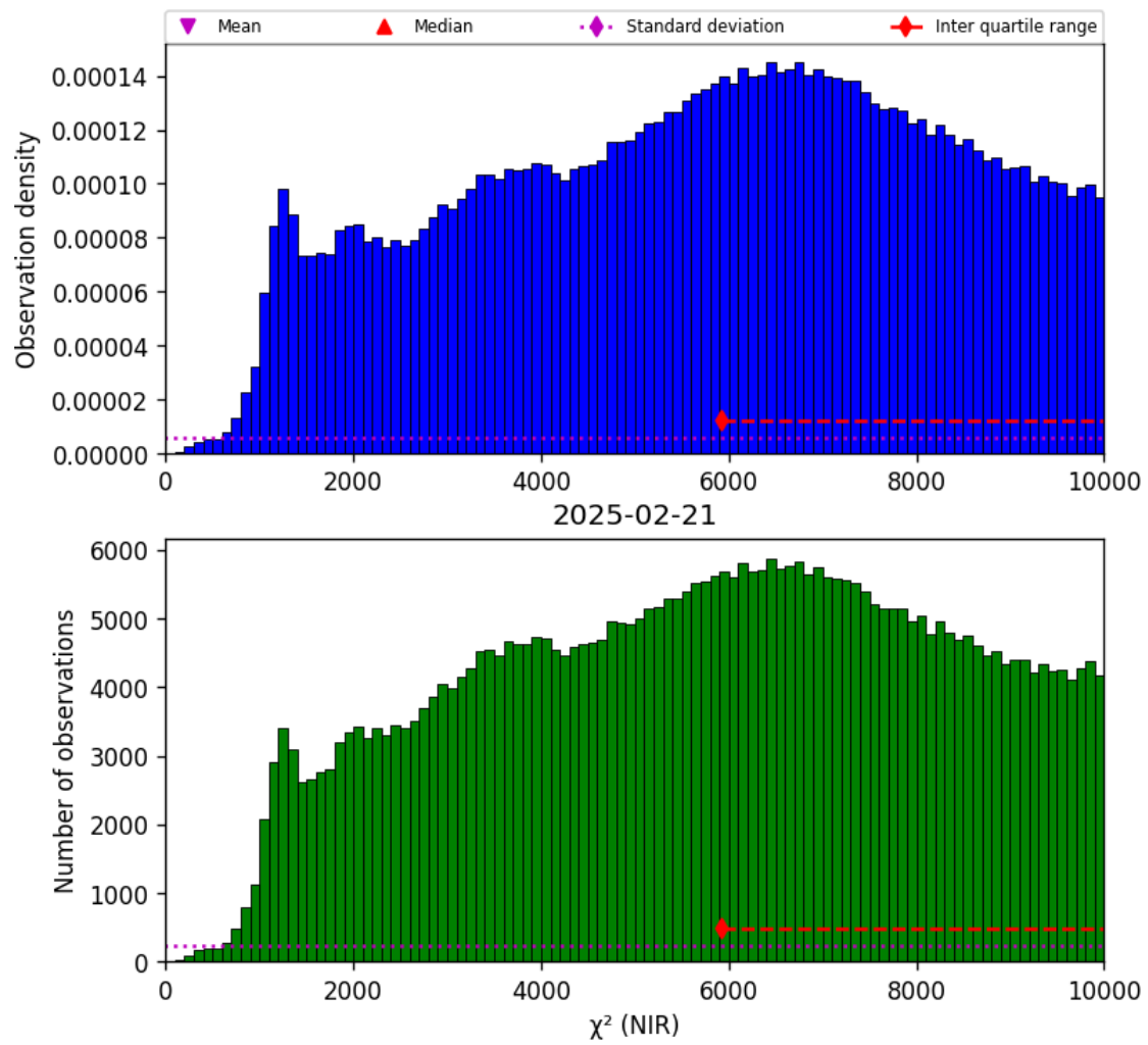
Figure 29: Histogram of “ \chi^2 (NIR)” for 2025-02-20 to 2025-02-22
