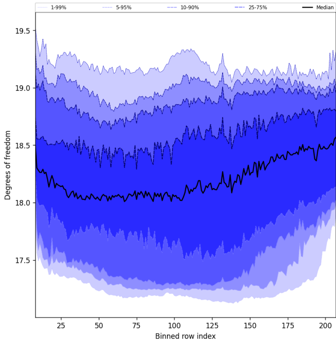
Figure 41: Along track statistics of “Degrees of freedom” for 2025-02-20 to 2025-02-22
