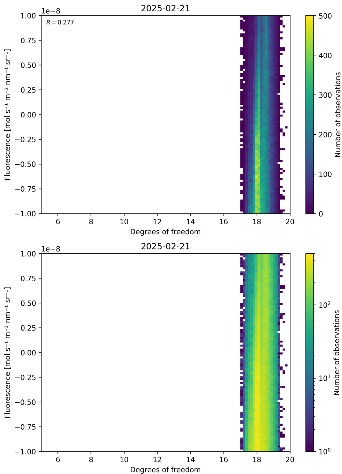
Figure 51: Scatter density plot of “Degrees of freedom” against “Fluorescence” for 2025-02-20 to 2025-02-22.
