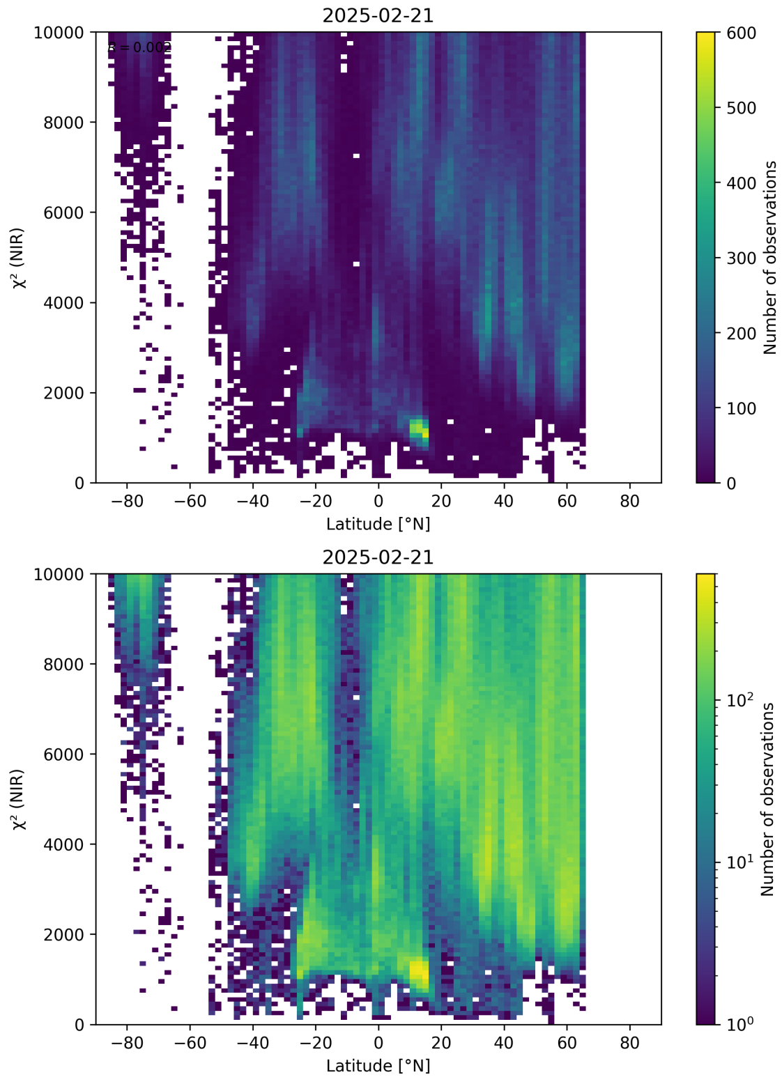
Figure 53: Scatter density plot of “Latitude” against “ \chi^2 (NIR)” for 2025-02-20 to 2025-02-22.
