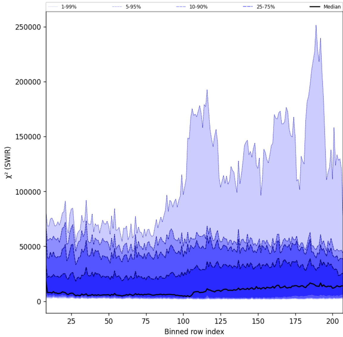
Figure 39: Along track statistics of “ \chi^2 (SWIR)” for 2025-02-20 to 2025-02-22
