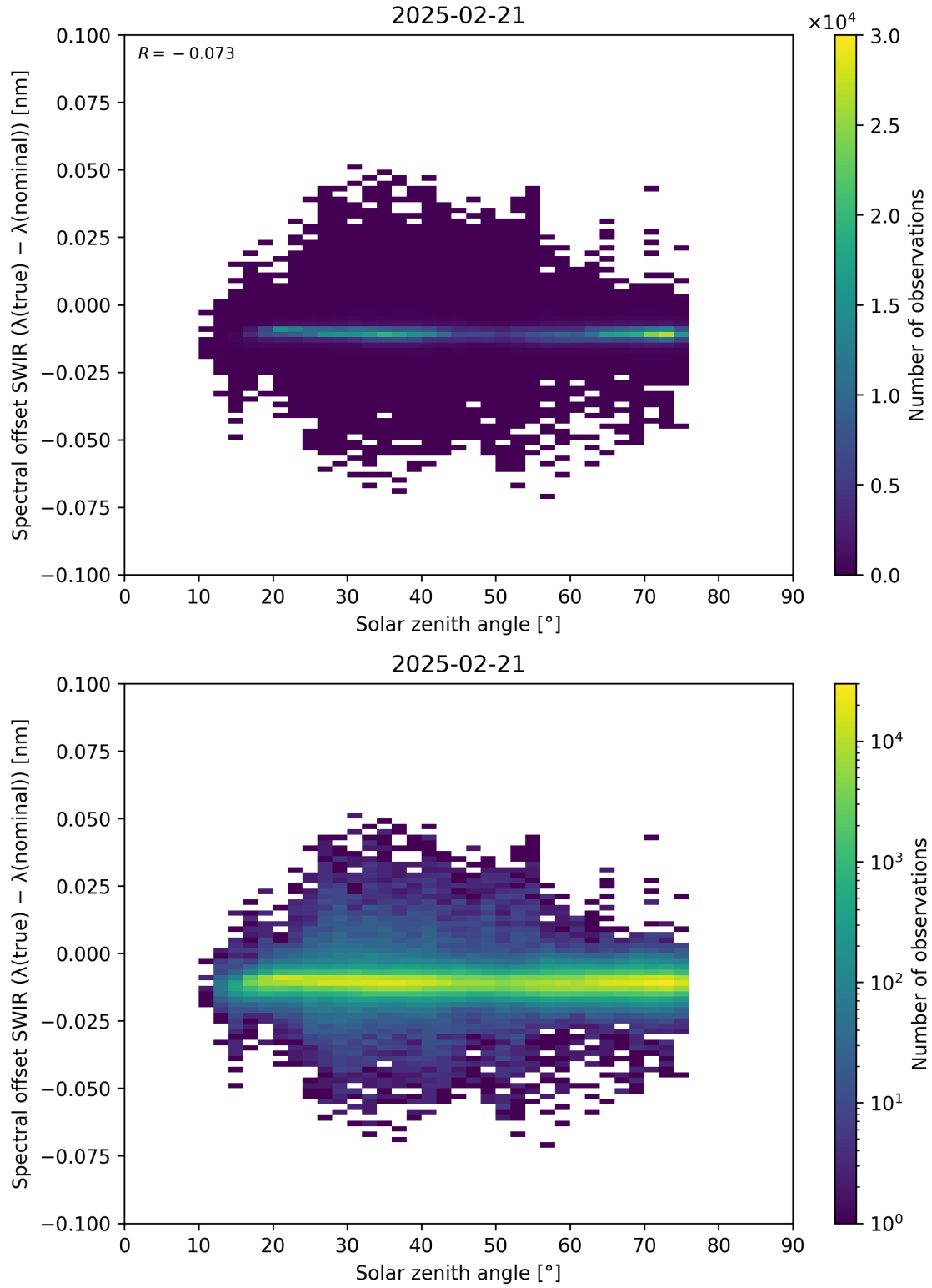
Figure 104: Scatter density plot of “Solar zenith angle” against “Spectral offset SWIR ( \lambda_{\text{true}} - \lambda_{\text{nominal}} )” for 2025-02-20 to 2025-02-22.
