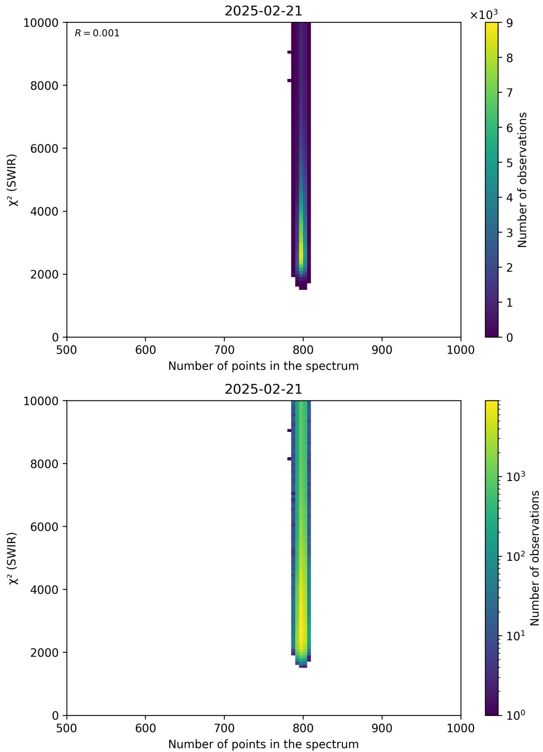
Figure 89: Scatter density plot of “Number of points in the spectrum” against “ \chi^2 (SWIR)” for 2025-02-20 to 2025-02-22.
