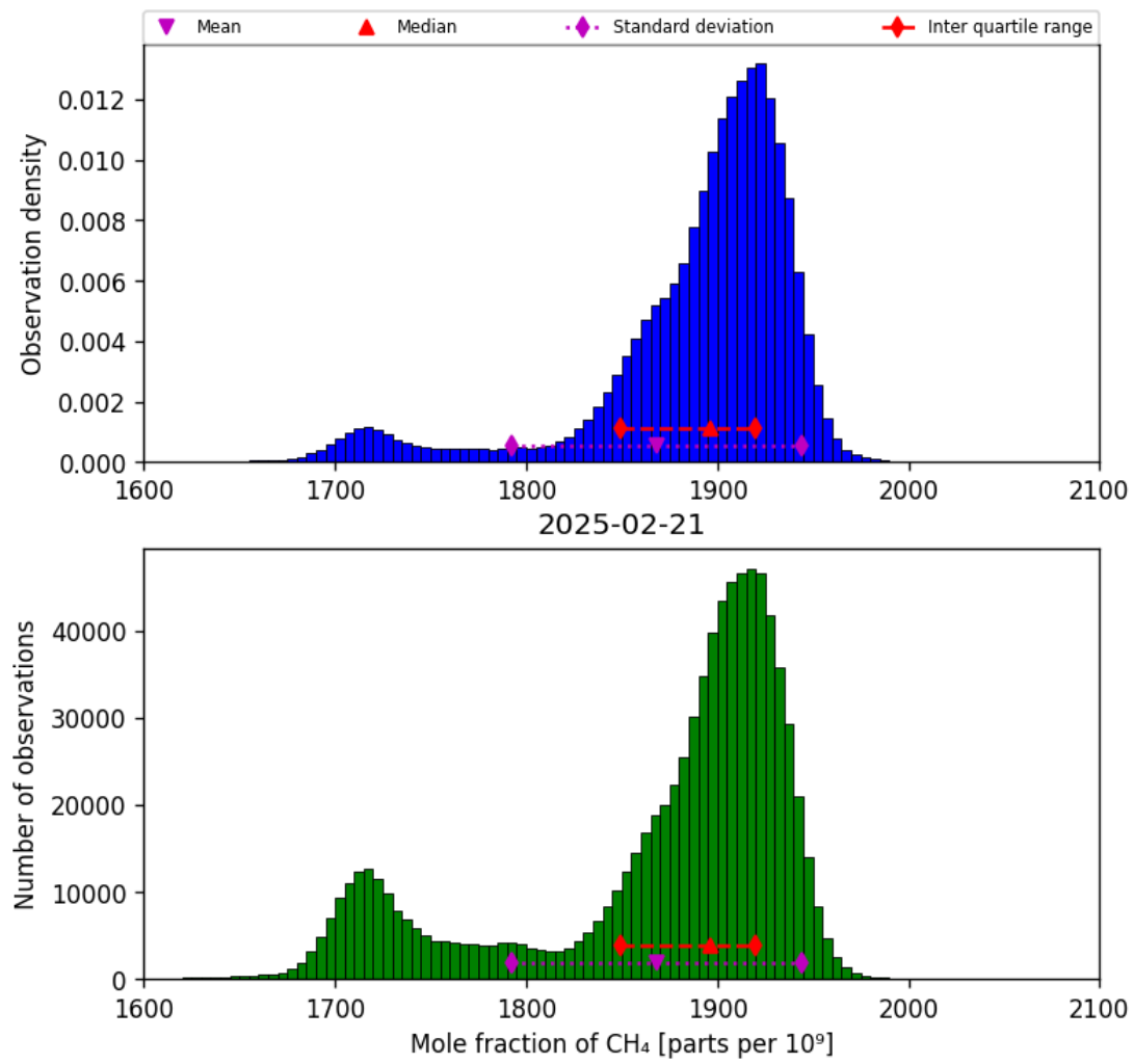
Figure 23: Histogram of “Mole fraction of CH 4 ” for 2025-02-20 to 2025-02-22
