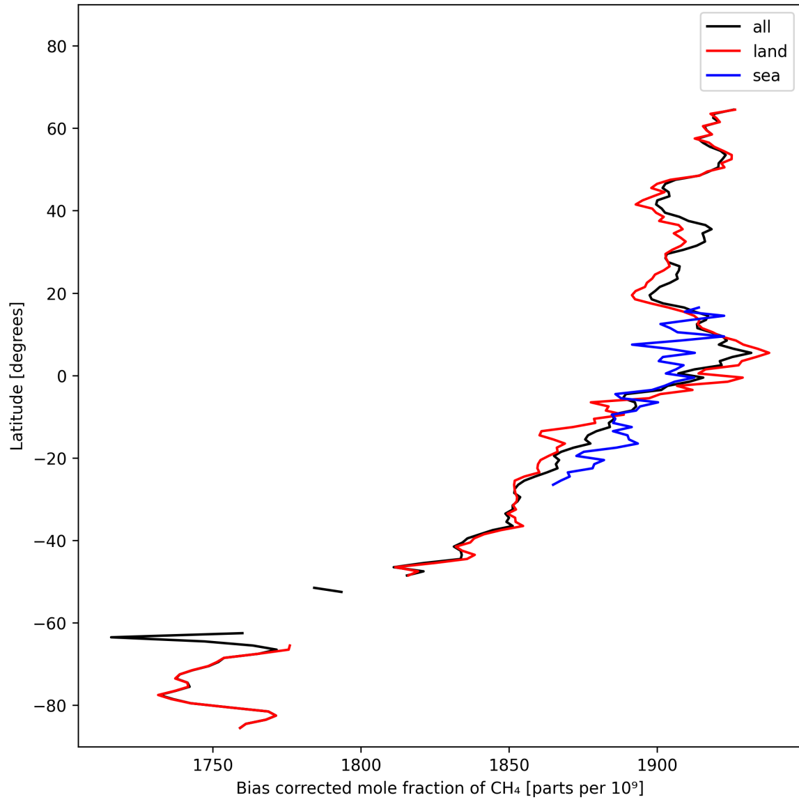
Figure 14: Zonal average of “Bias corrected mole fraction of CH 4 ” for 2025-02-20 to 2025-02-22.
