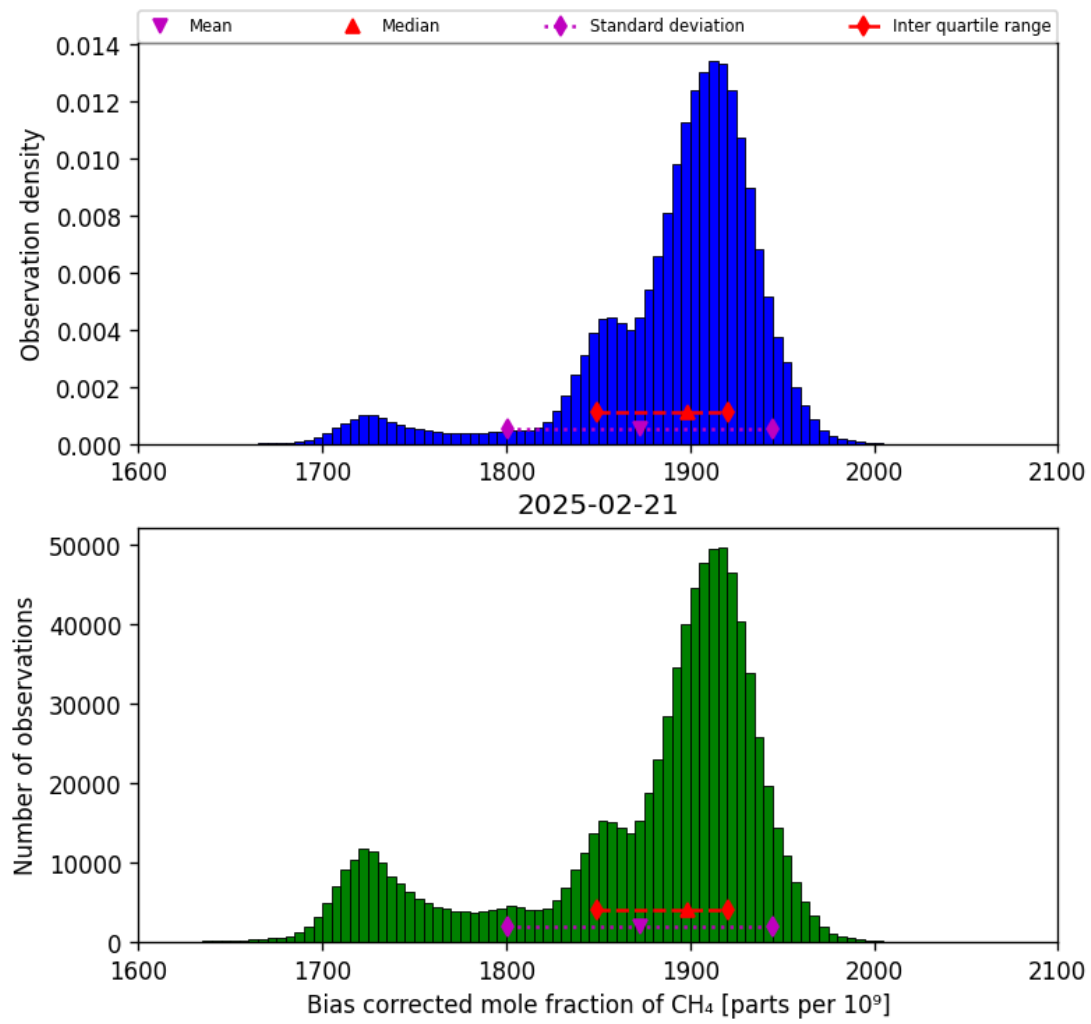
Figure 25: Histogram of “Bias corrected mole fraction of CH 4 ” for 2025-02-20 to 2025-02-22
