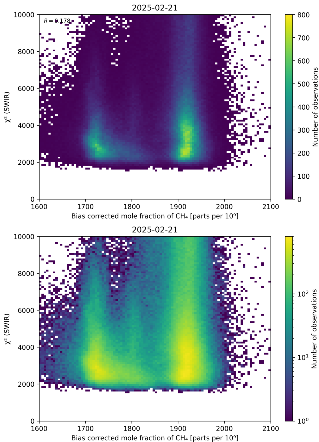
Figure 64: Scatter density plot of “Bias corrected mole fraction of \text{CH}_4 ” against “ \chi^2 (SWIR)” for 2025-02-20 to 2025-02-22.
