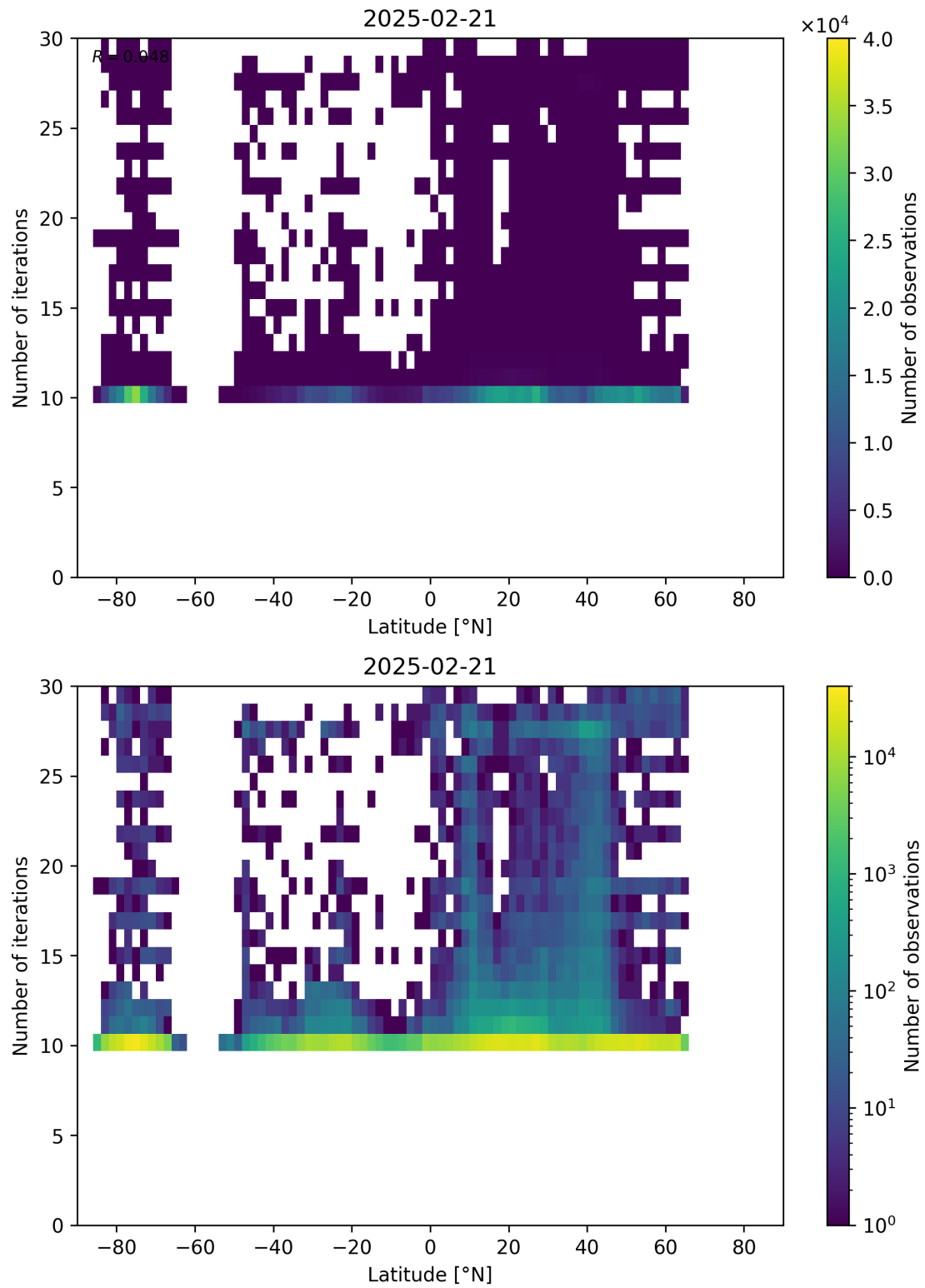
Figure 60: Scatter density plot of “Latitude” against “Number of iterations” for 2025-02-20 to 2025-02-22.
