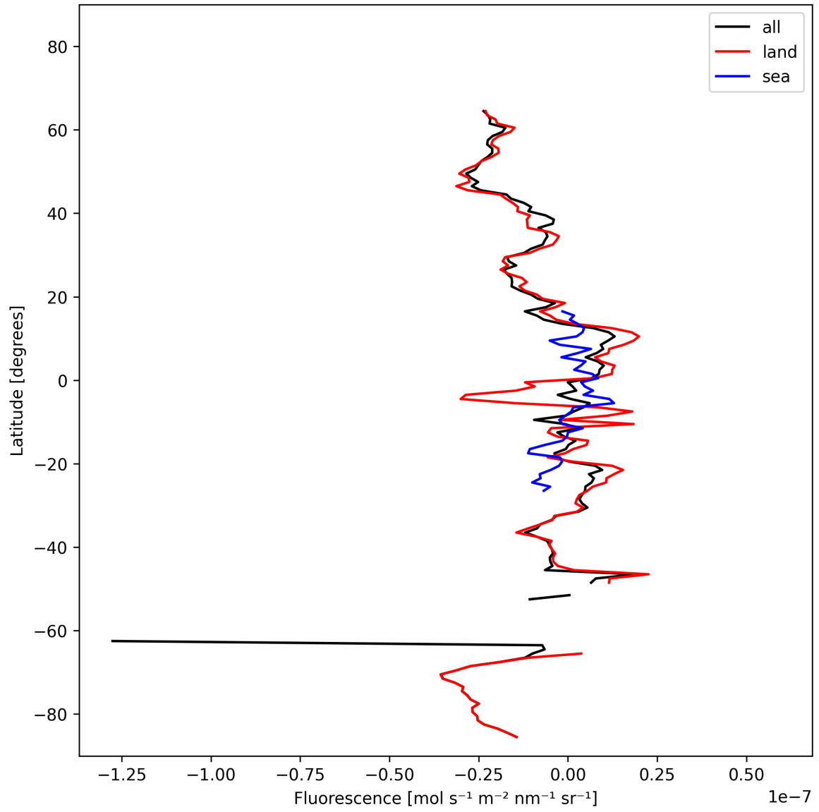
Figure 21: Zonal average of “Fluorescence” for 2025-02-20 to 2025-02-22.
