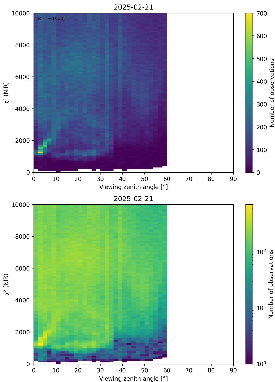
Figure 105: Scatter density plot of “Viewing zenith angle” against “ \chi^2 (NIR)” for 2025-02-20 to 2025-02-22.
