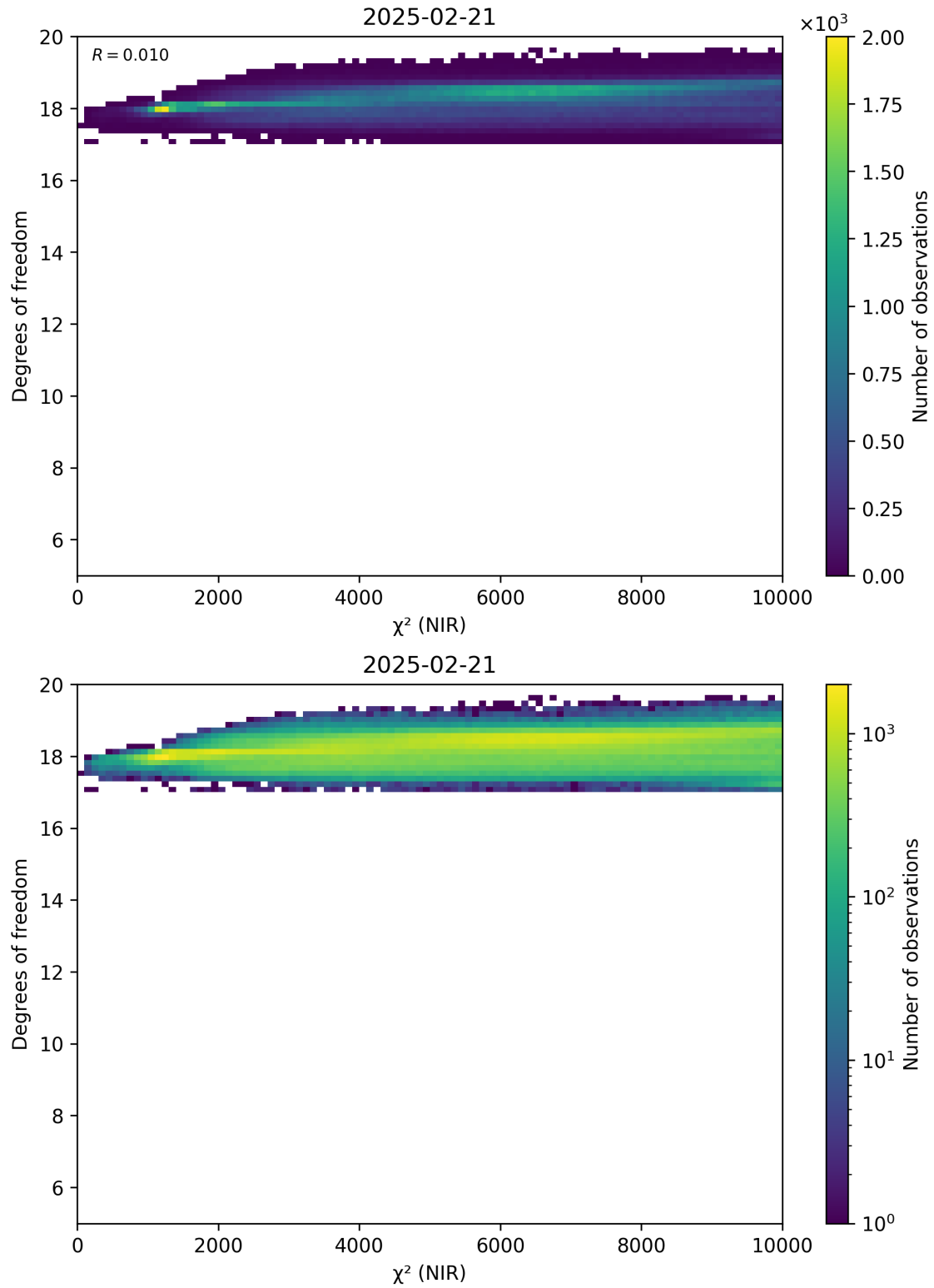
Figure 44: Scatter density plot of “ \chi^2 (NIR)” against “Degrees of freedom” for 2025-02-20 to 2025-02-22.
