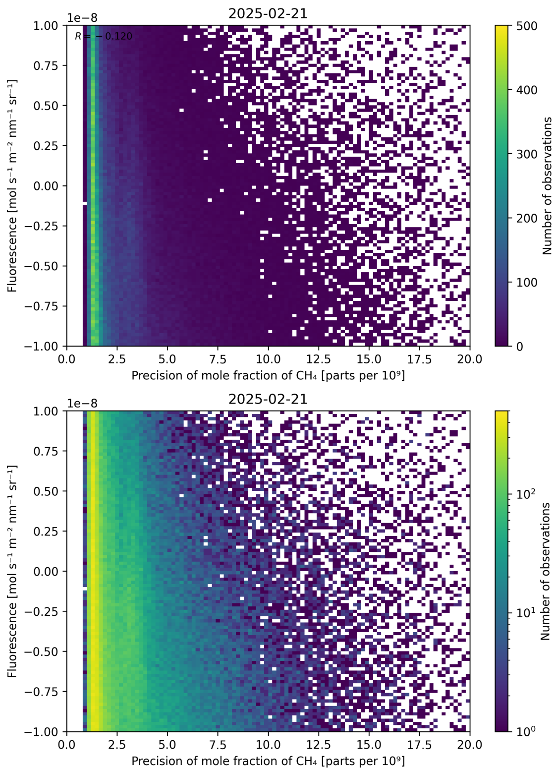
Figure 81: Scatter density plot of “Precision of mole fraction of \text{CH}_4 ” against “Fluorescence” for 2025-02-20 to 2025-02-22.
