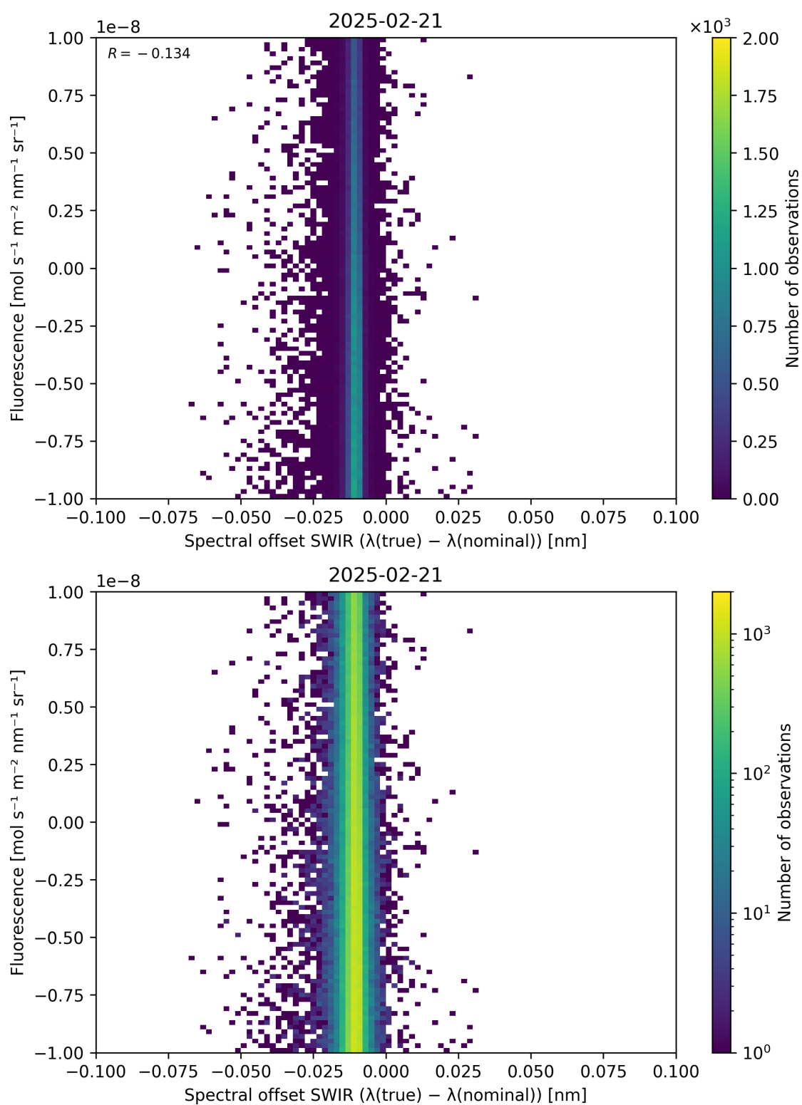
Figure 120: Scatter density plot of “Spectral offset SWIR ( \lambda_{\text{true}} - \lambda_{\text{nominal}} )” against “Fluorescence” for 2025-02-20 to 2025-02-22.
