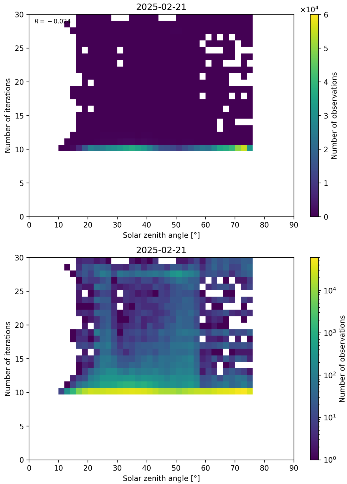
Figure 102: Scatter density plot of “Solar zenith angle” against “Number of iterations” for 2025-02-20 to 2025-02-22.
