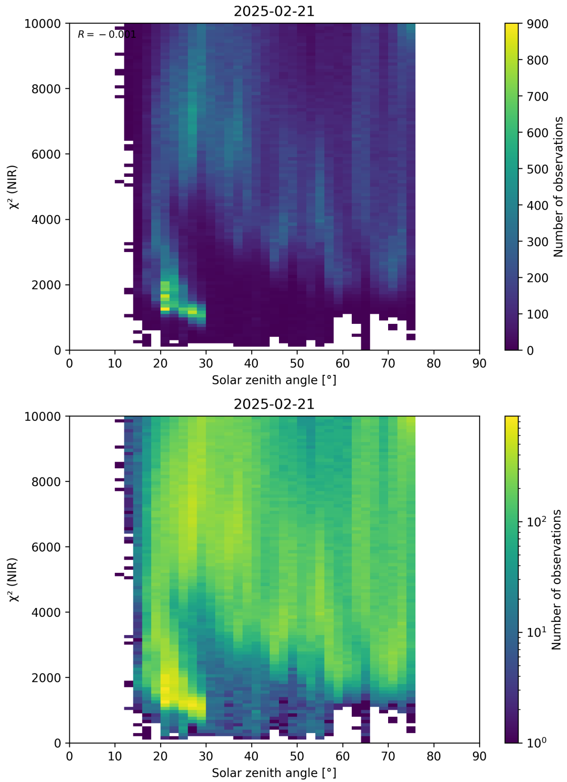
Figure 94: Scatter density plot of “Solar zenith angle” against “ \chi^2 (NIR)” for 2025-02-20 to 2025-02-22.
