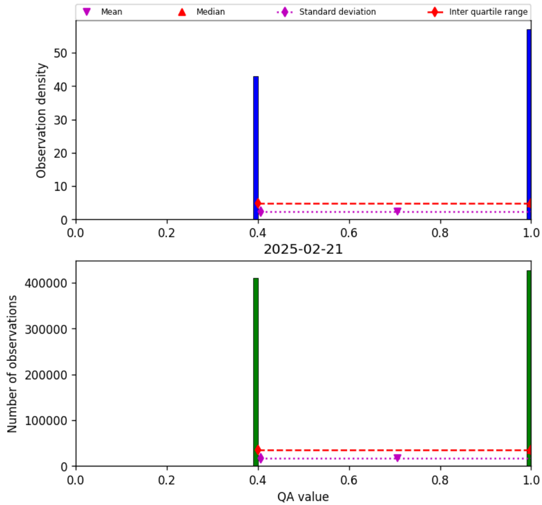
Figure 22: Histogram of “QA value” for 2025-02-20 to 2025-02-22
