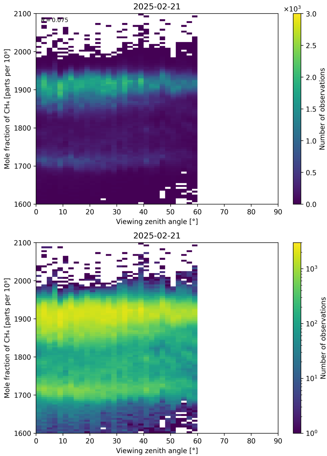
Figure 110: Scatter density plot of “Viewing zenith angle” against “Mole fraction of CH 4 ” for 2025-02-20 to 2025-02-22.
