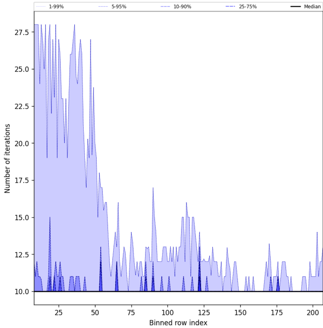
Figure 42: Along track statistics of “Number of iterations” for 2025-02-20 to 2025-02-22
