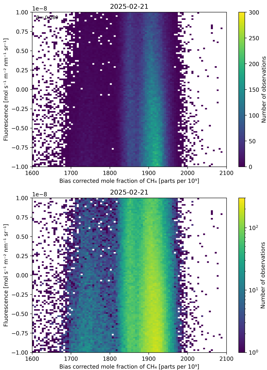
Figure 66: Scatter density plot of “Bias corrected mole fraction of CH 4 ” against “Fluorescence” for 2025-02-20 to 2025-02-22.
