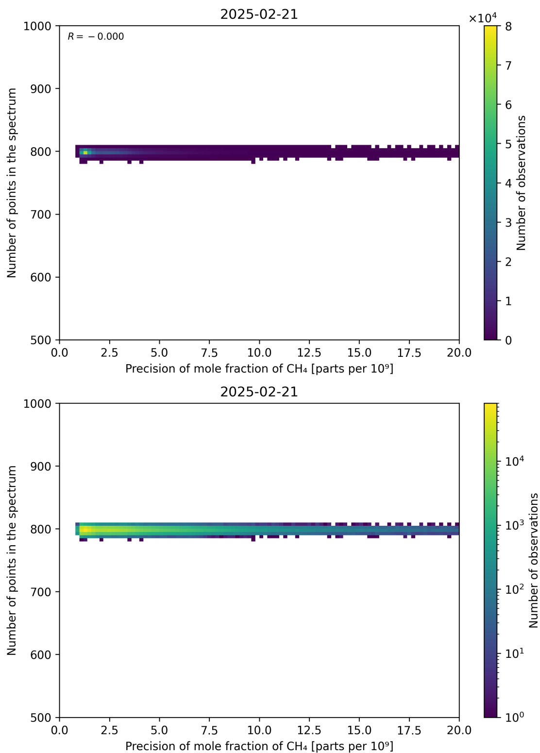
Figure 84: Scatter density plot of “Precision of mole fraction of CH 4 ” against “Number of points in the spectrum” for 2025-02-20 to 2025-02-22.
