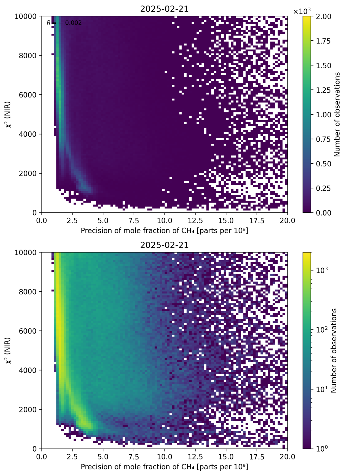
Figure 78: Scatter density plot of “Precision of mole fraction of \text{CH}_4 ” against “ \chi^2 (NIR)” for 2025-02-20 to 2025-02-22.
