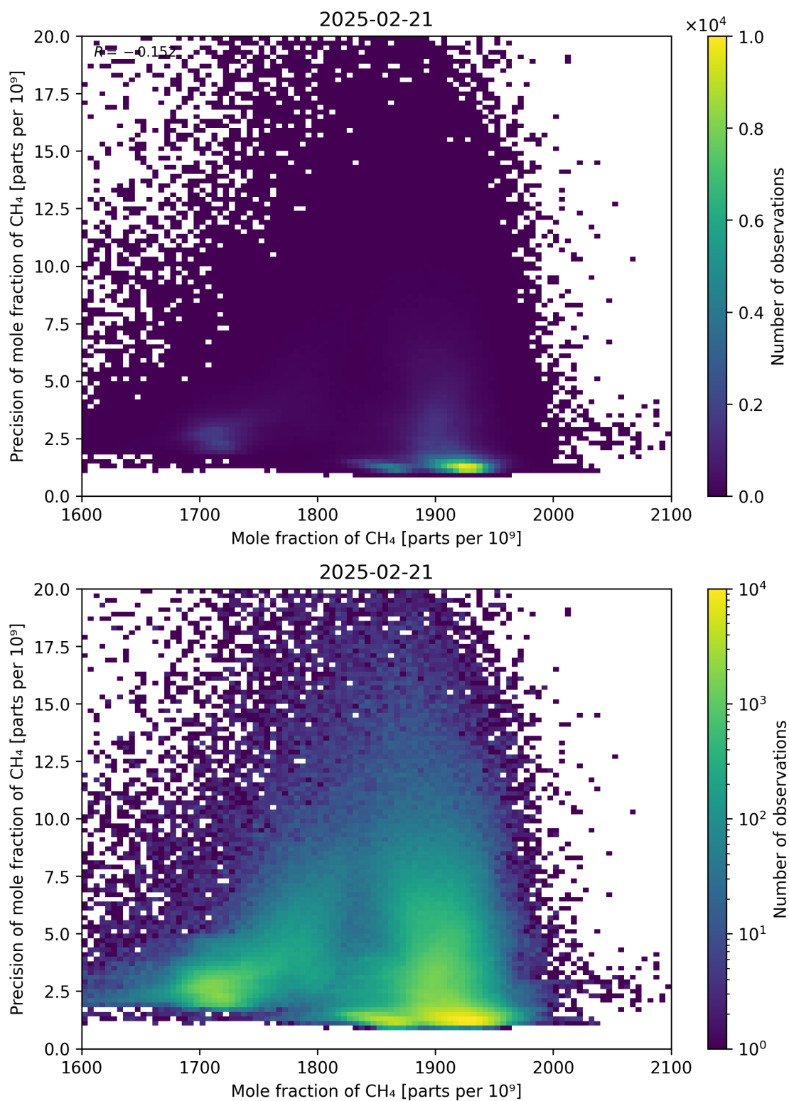
Figure 75: Scatter density plot of “Mole fraction of CH 4 ” against “Precision of mole fraction of CH 4 ” for 2025-02-20 to 2025-02-22.
