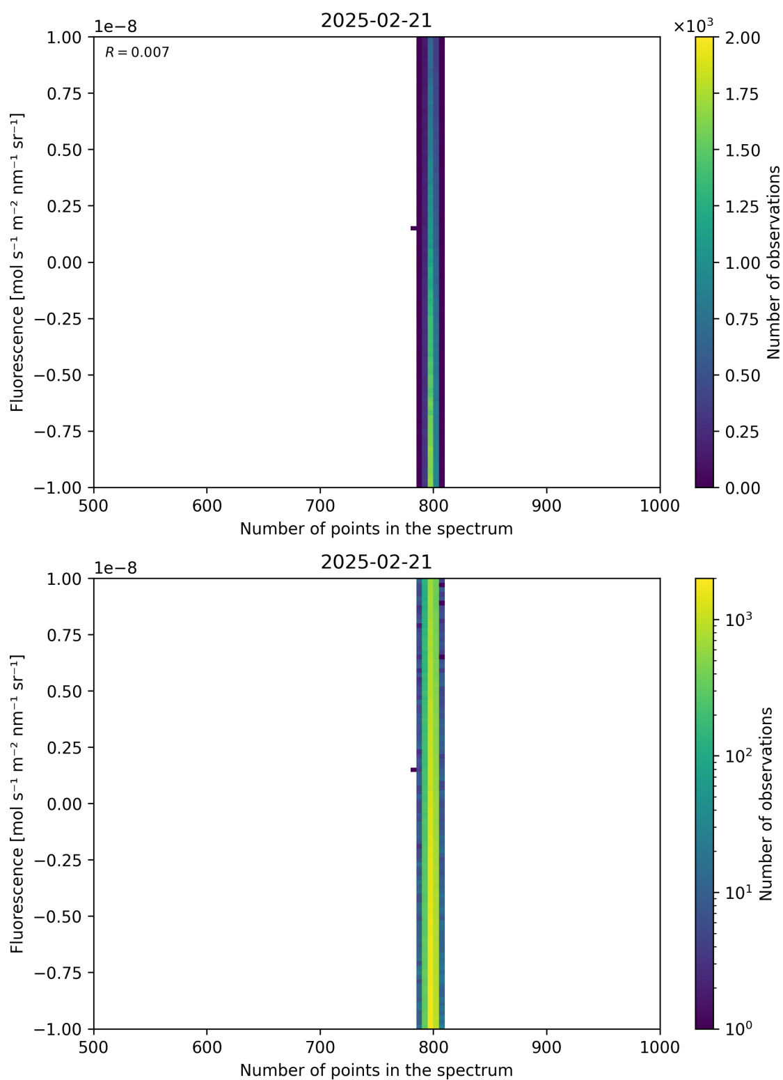
Figure 91: Scatter density plot of “Number of points in the spectrum” against “Fluorescence” for 2025-02-20 to 2025-02-22.
