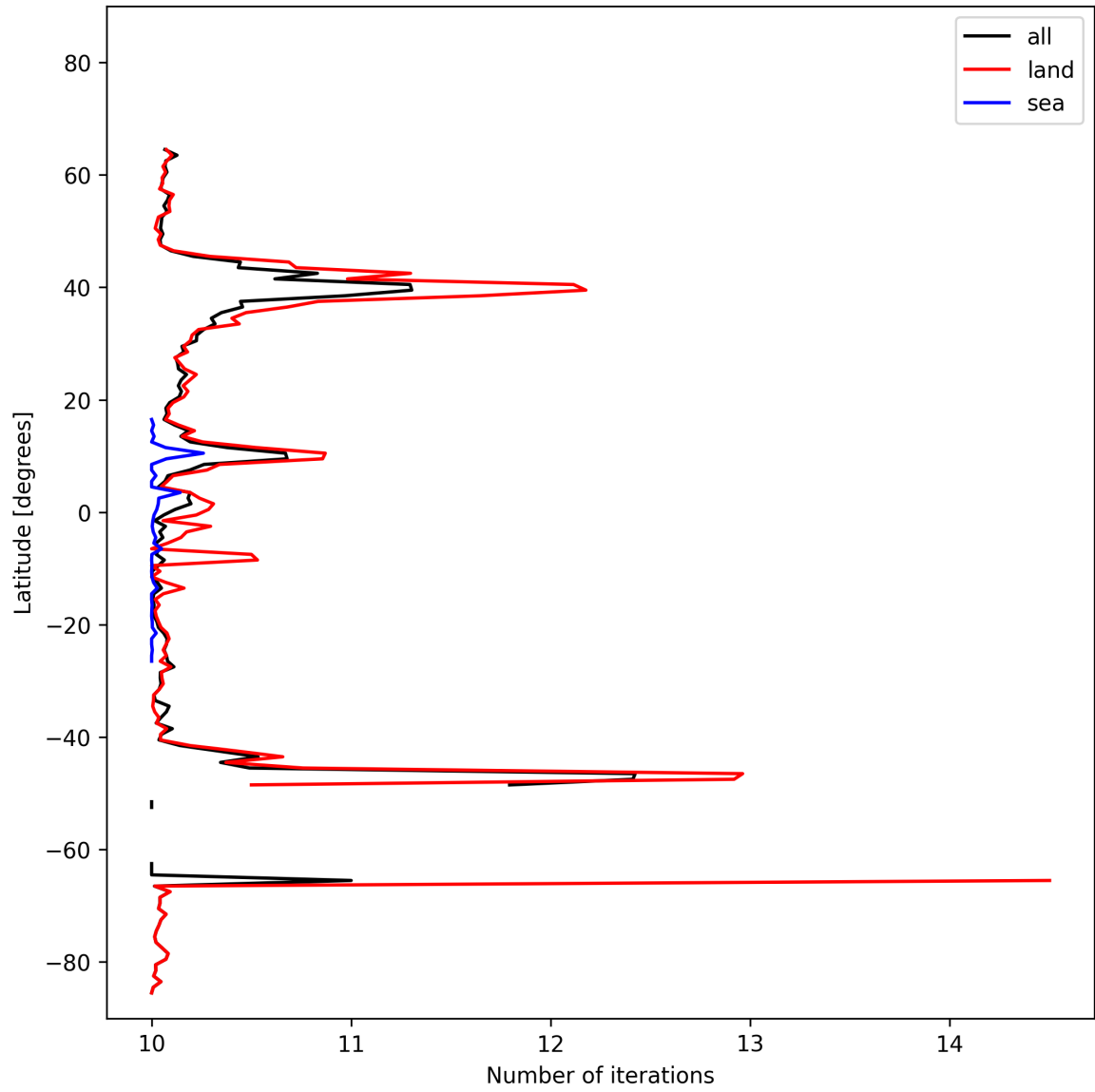
Figure 20: Zonal average of “Number of iterations” for 2025-02-20 to 2025-02-22.
