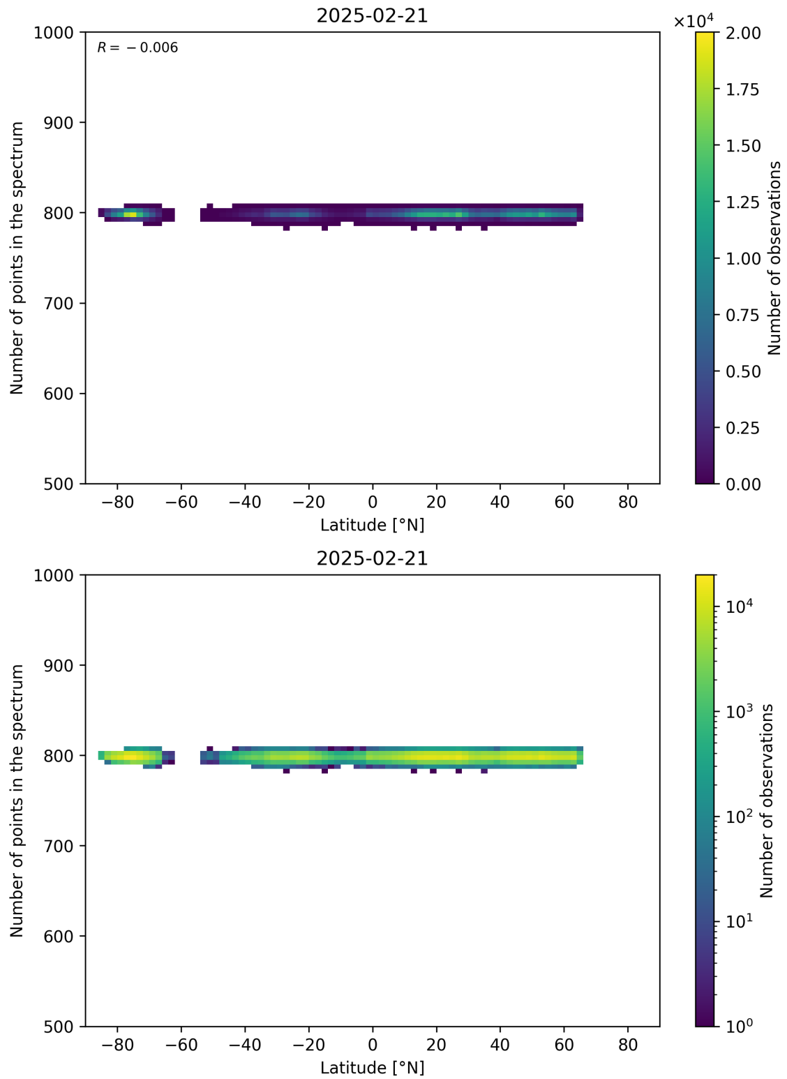
Figure 61: Scatter density plot of “Latitude” against “Number of points in the spectrum” for 2025-02-20 to 2025-02-22.
