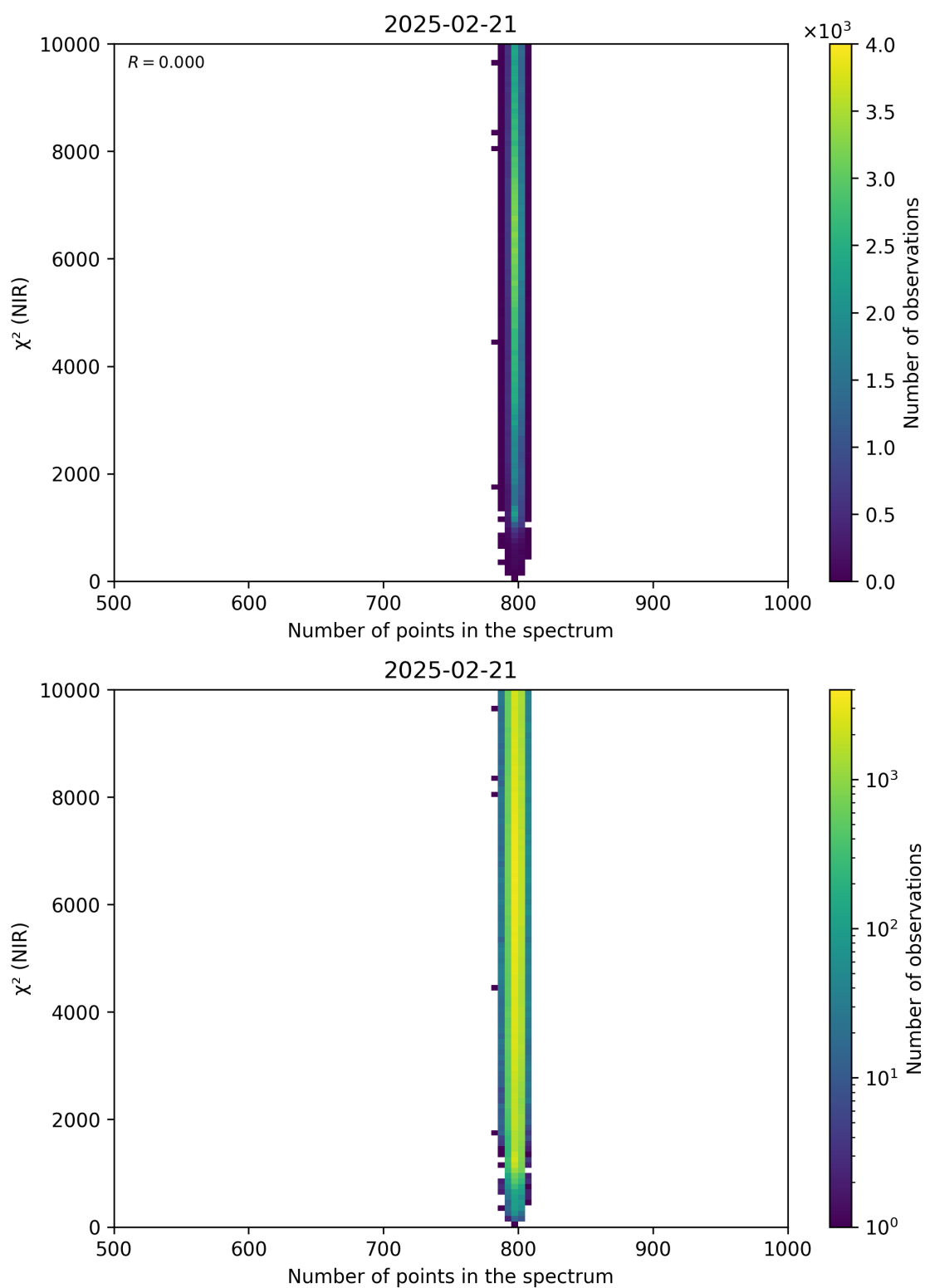
Figure 88: Scatter density plot of “Number of points in the spectrum” against “ \chi^2 (NIR)” for 2025-02-20 to 2025-02-22.
