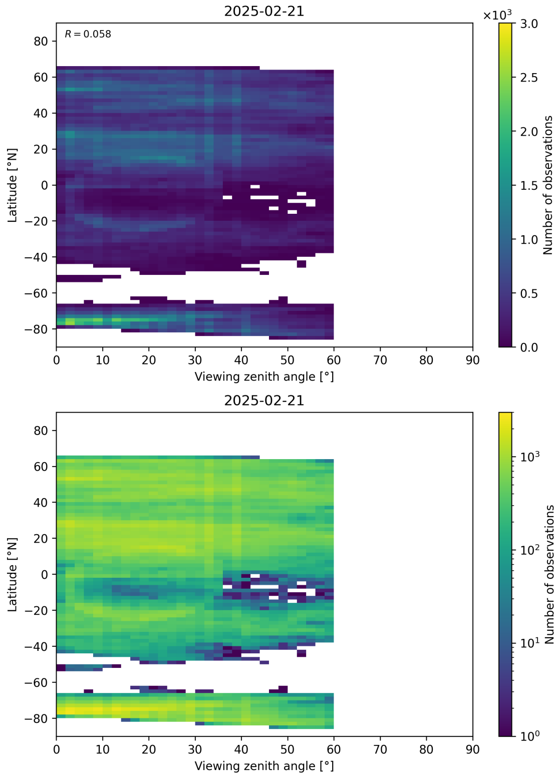
Figure 109: Scatter density plot of “Viewing zenith angle” against “Latitude” for 2025-02-20 to 2025-02-22.
