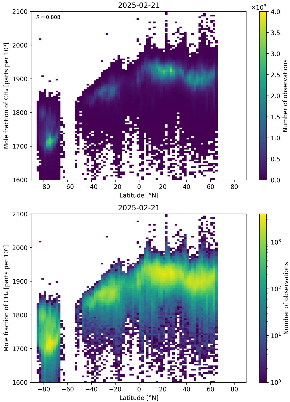
Figure 57: Scatter density plot of “Latitude” against “Mole fraction of CH 4 ” for 2025-02-20 to 2025-02-22.
