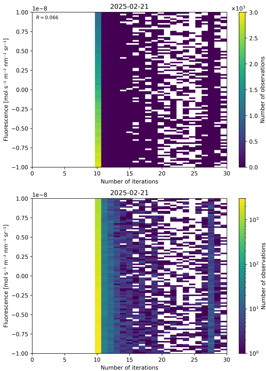
Figure 87: Scatter density plot of “Number of iterations” against “Fluorescence” for 2025-02-20 to 2025-02-22.
