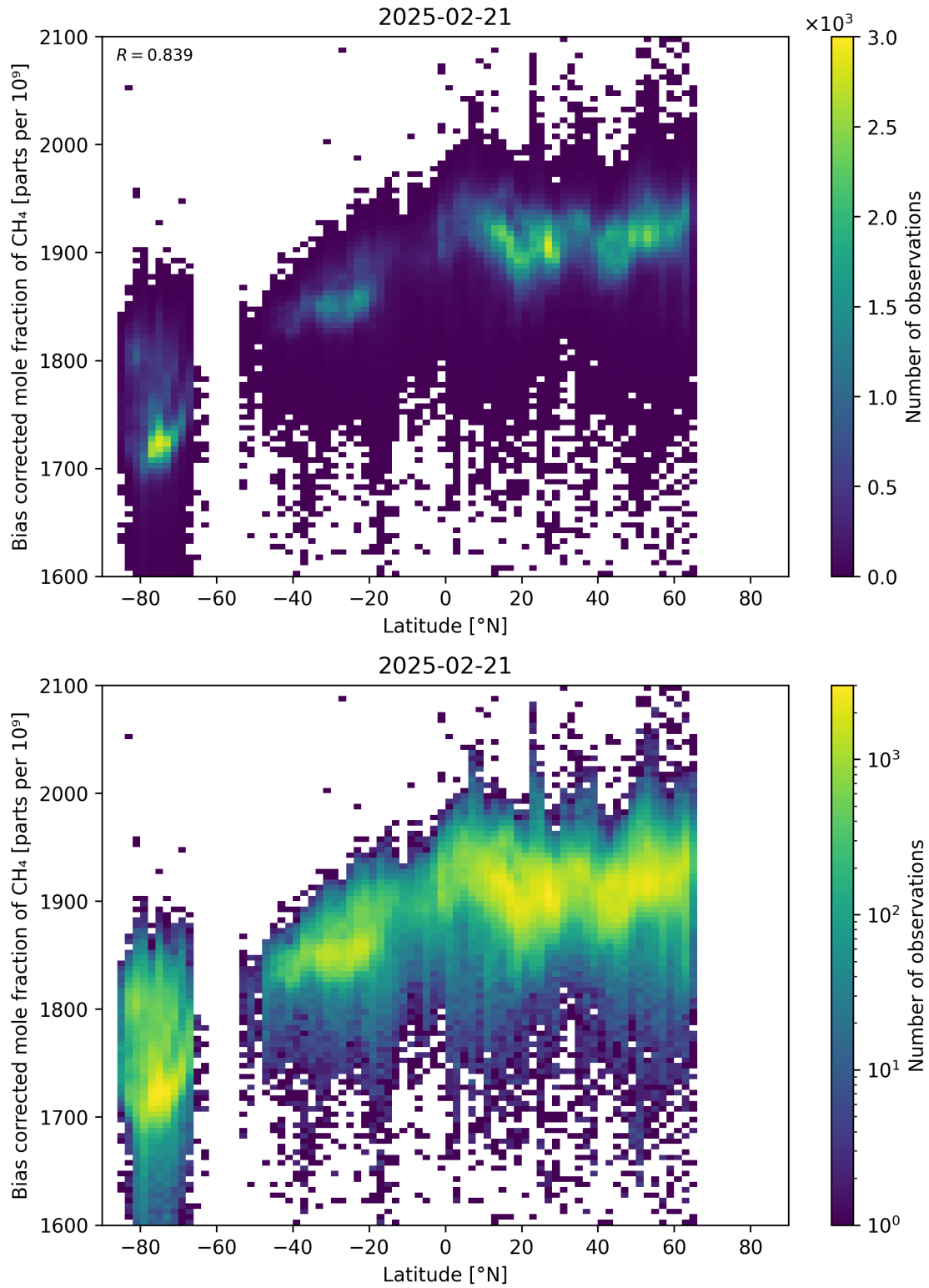
Figure 58: Scatter density plot of “Latitude” against “Bias corrected mole fraction of CH 4 ” for 2025-02-20 to 2025-02-22.
