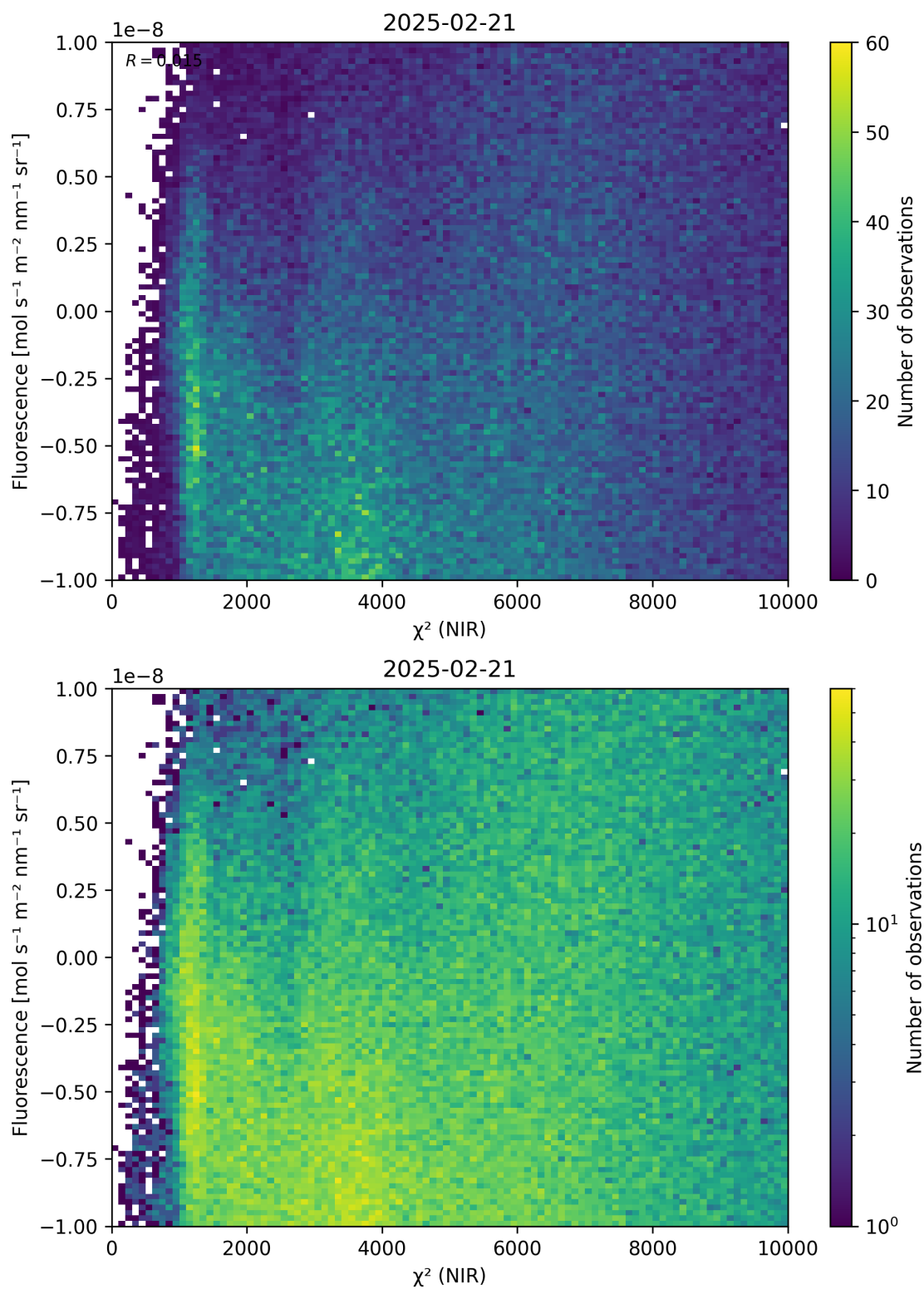
Figure 45: Scatter density plot of “ \chi^2 (NIR)” against “Fluorescence” for 2025-02-20 to 2025-02-22.
