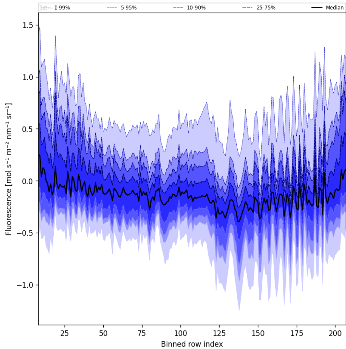
Figure 43: Along track statistics of “Fluorescence” for 2025-02-20 to 2025-02-22
