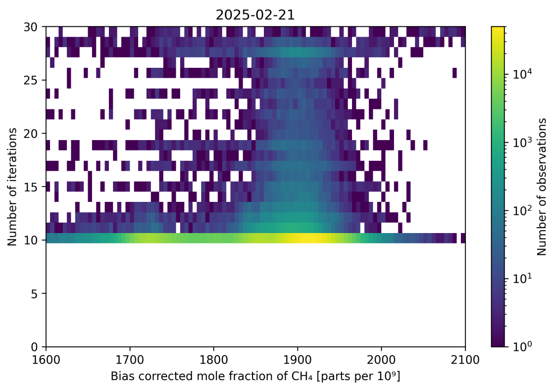
Figure 67: Scatter density plot of “Bias corrected mole fraction of CH 4 ” against “Number of iterations” for 2025-02-20 to 2025-02-22.
