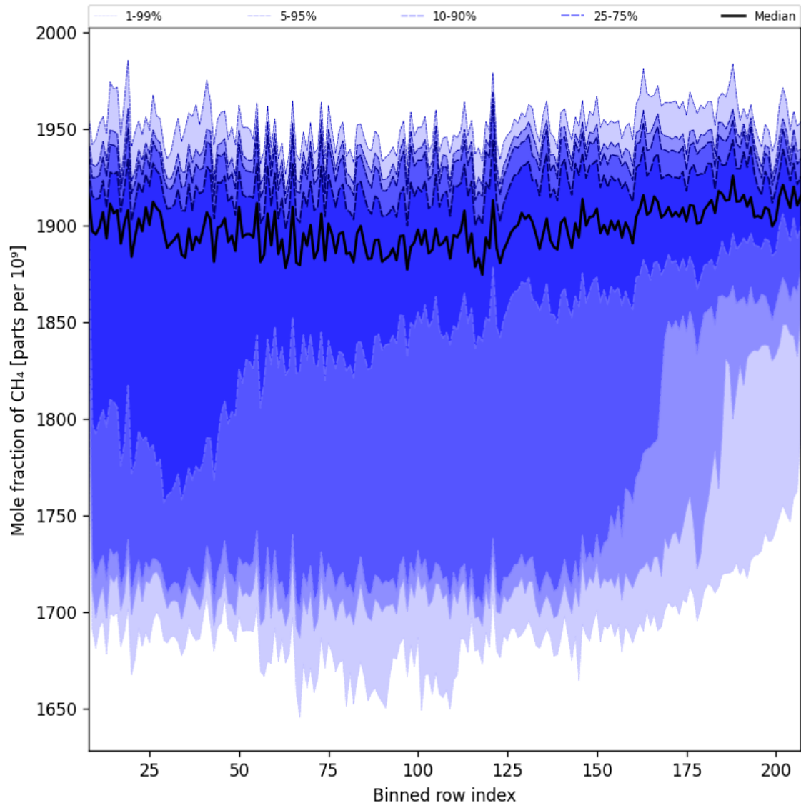
Figure 34: Along track statistics of “Mole fraction of CH 4 ” for 2025-02-20 to 2025-02-22
