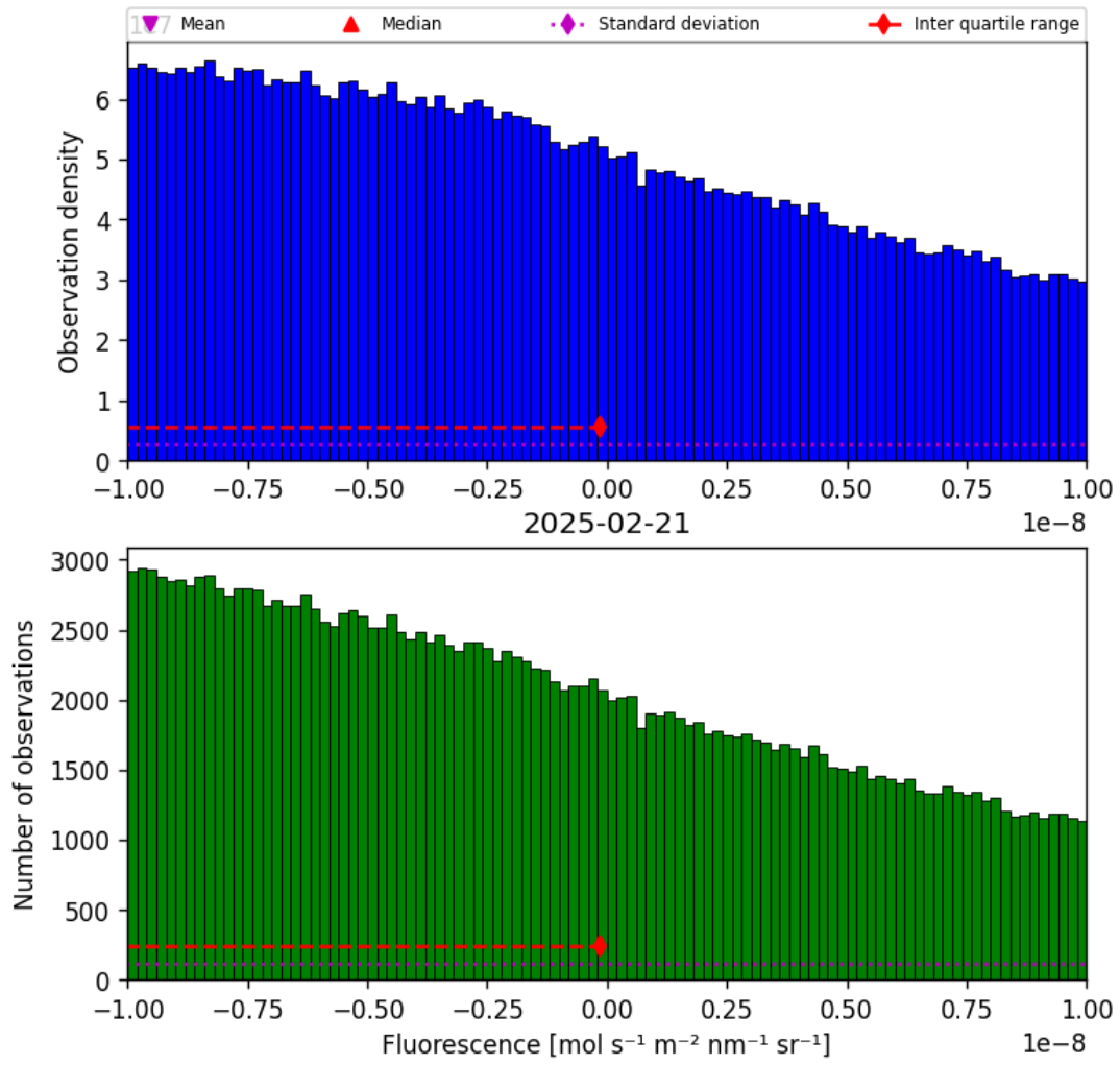
Figure 32: Histogram of “Fluorescence” for 2025-02-20 to 2025-02-22
