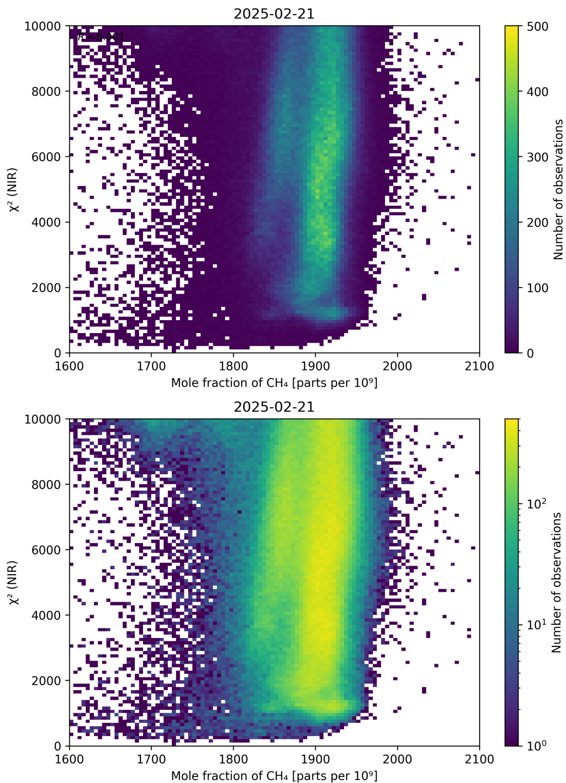
Figure 70: Scatter density plot of “Mole fraction of CH 4 ” against “ \chi^2 (NIR)” for 2025-02-20 to 2025-02-22.
