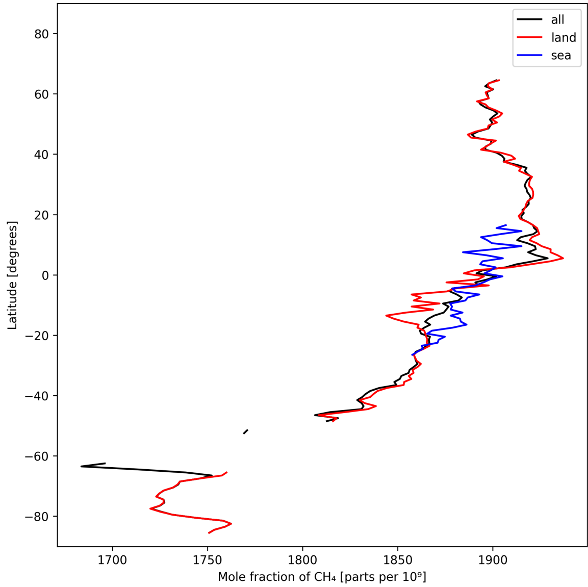
Figure 12: Zonal average of “Mole fraction of CH 4 ” for 2025-02-20 to 2025-02-22.
