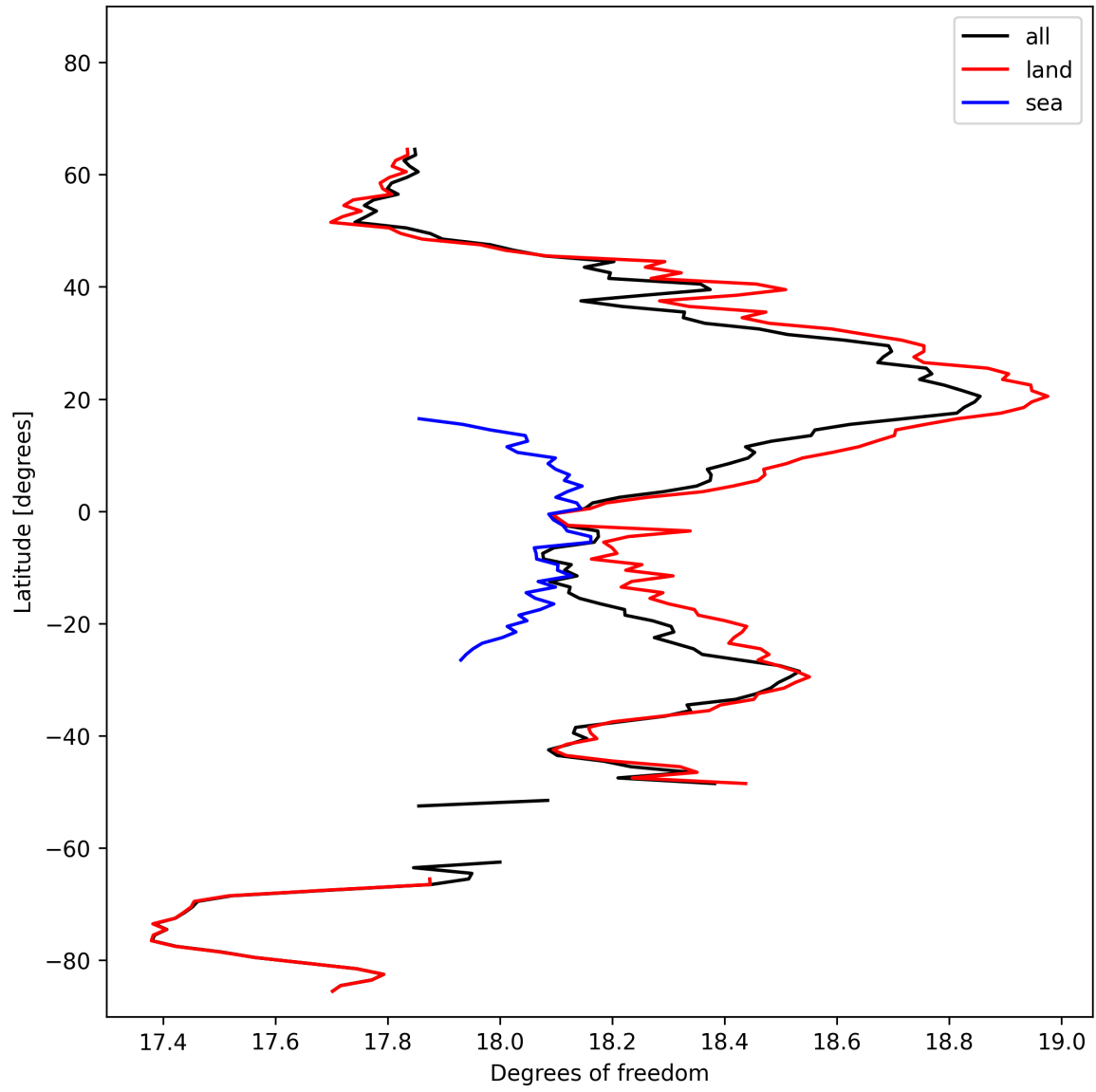
Figure 19: Zonal average of “Degrees of freedom” for 2025-02-20 to 2025-02-22.
