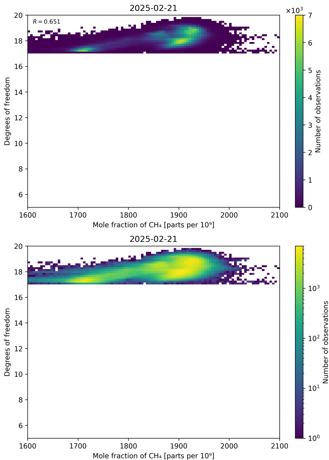
Figure 72: Scatter density plot of “Mole fraction of CH 4 ” against “Degrees of freedom” for 2025-02-20 to 2025-02-22.
