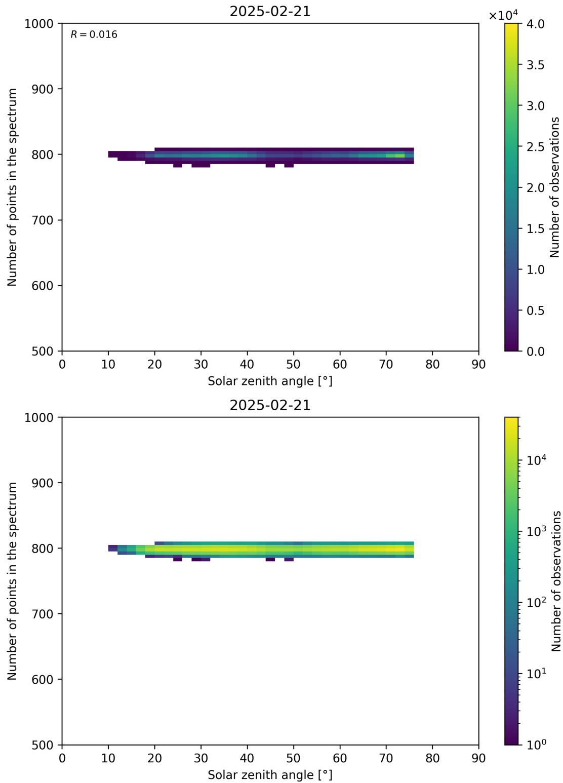
Figure 103: Scatter density plot of “Solar zenith angle” against “Number of points in the spectrum” for 2025-02-20 to 2025-02-22.
