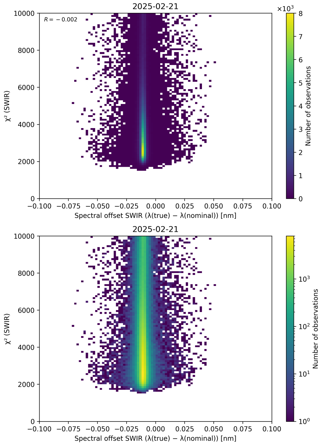
Figure 118: Scatter density plot of “Spectral offset SWIR ( \lambda_{\text{true}} - \lambda_{\text{nominal}} )” against “ \chi^2 (SWIR)” for 2025-02-20 to 2025-02-22.
