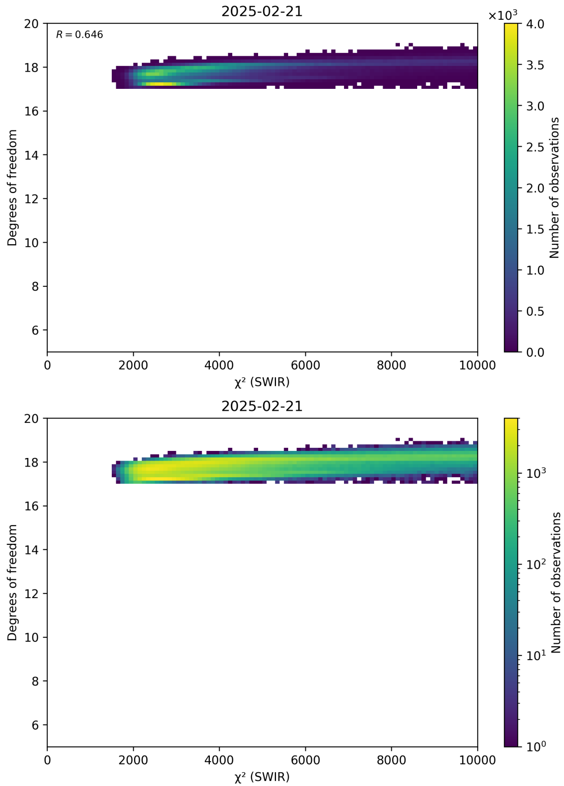
Figure 48: Scatter density plot of “ \chi^2 (SWIR)” against “Degrees of freedom” for 2025-02-20 to 2025-02-22.
