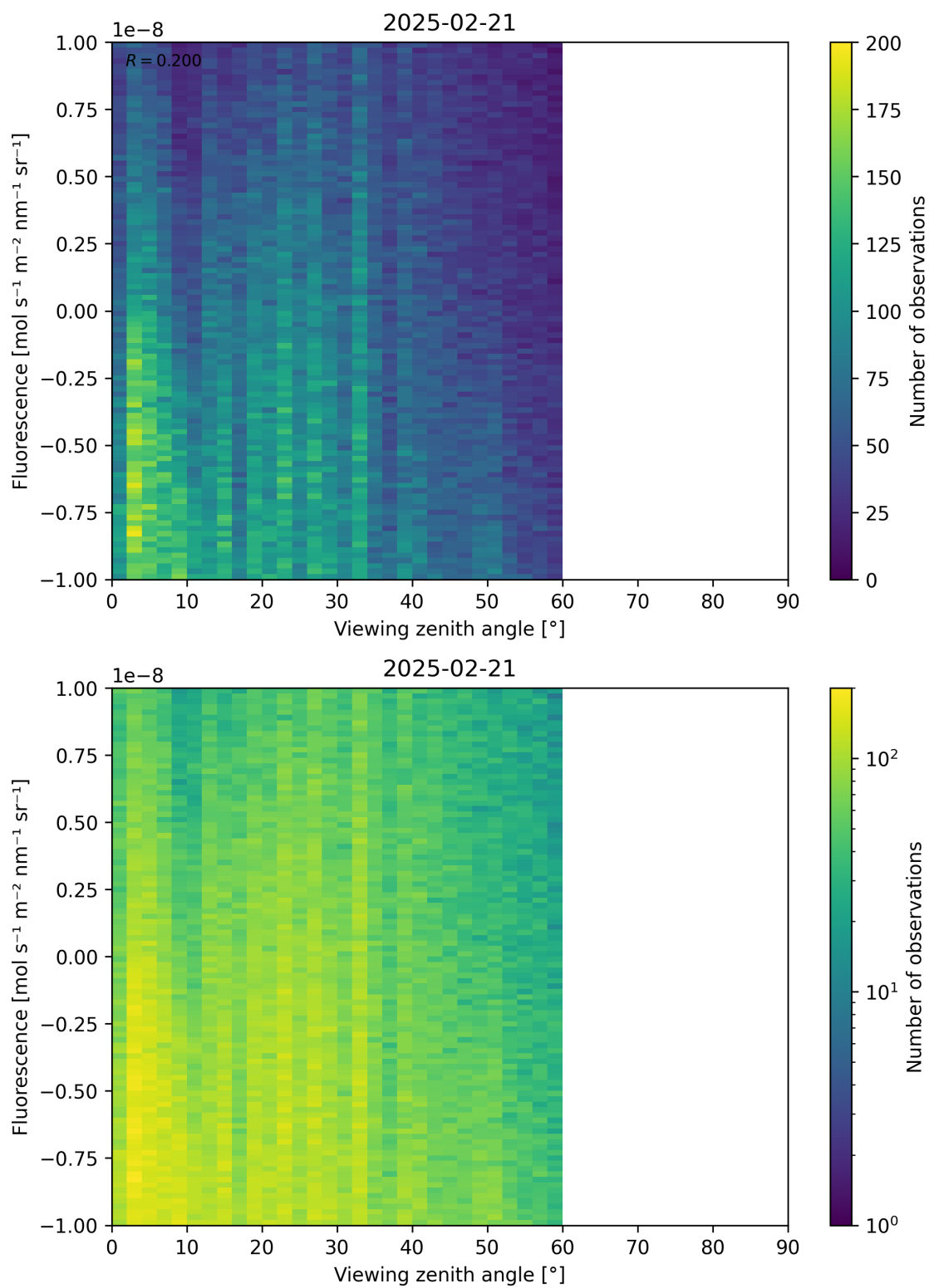
Figure 108: Scatter density plot of “Viewing zenith angle” against “Fluorescence” for 2025-02-20 to 2025-02-22.
