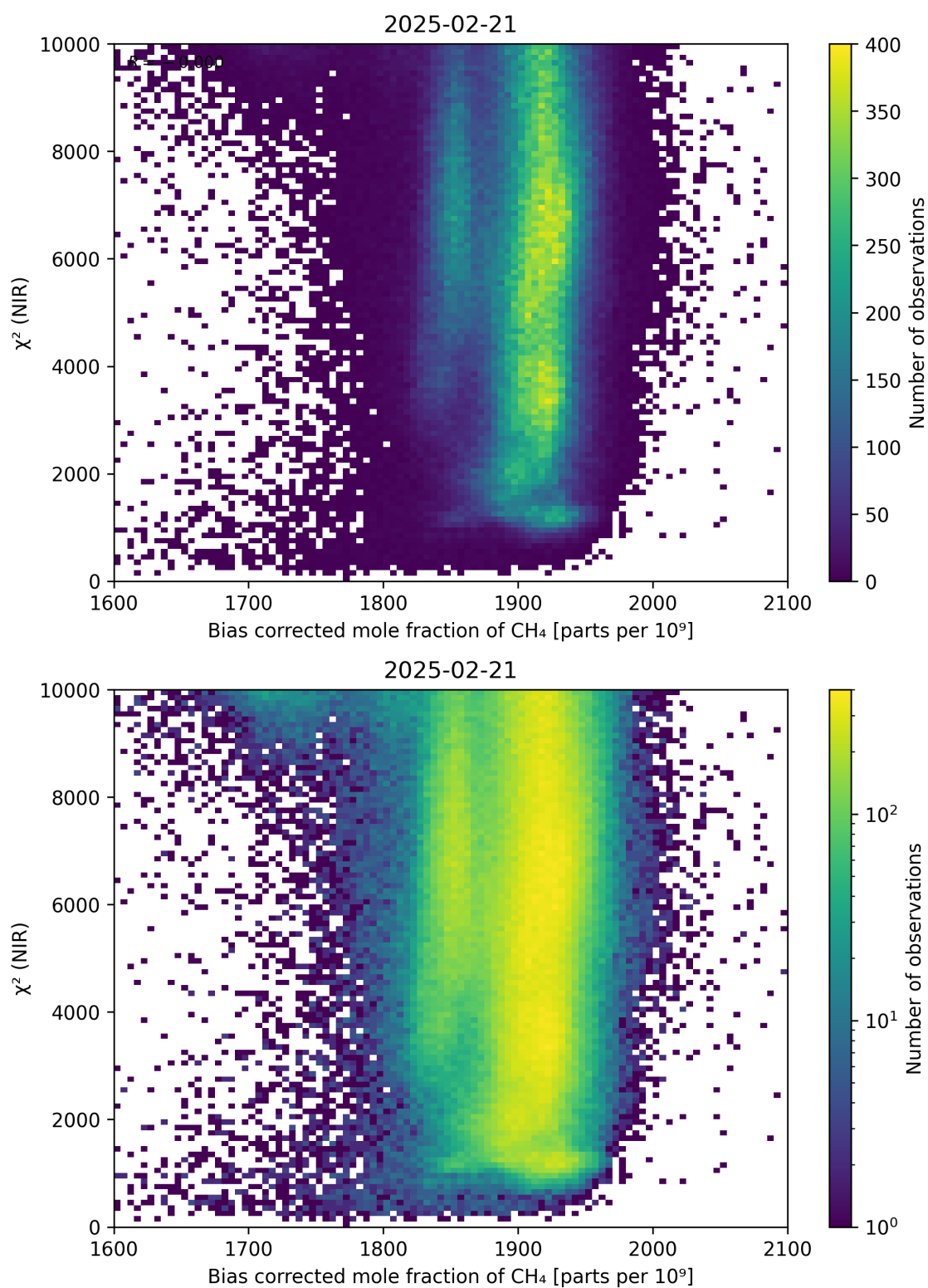
Figure 63: Scatter density plot of “Bias corrected mole fraction of CH 4 ” against “ \chi^2 (NIR)” for 2025-02-20 to 2025-02-22.
