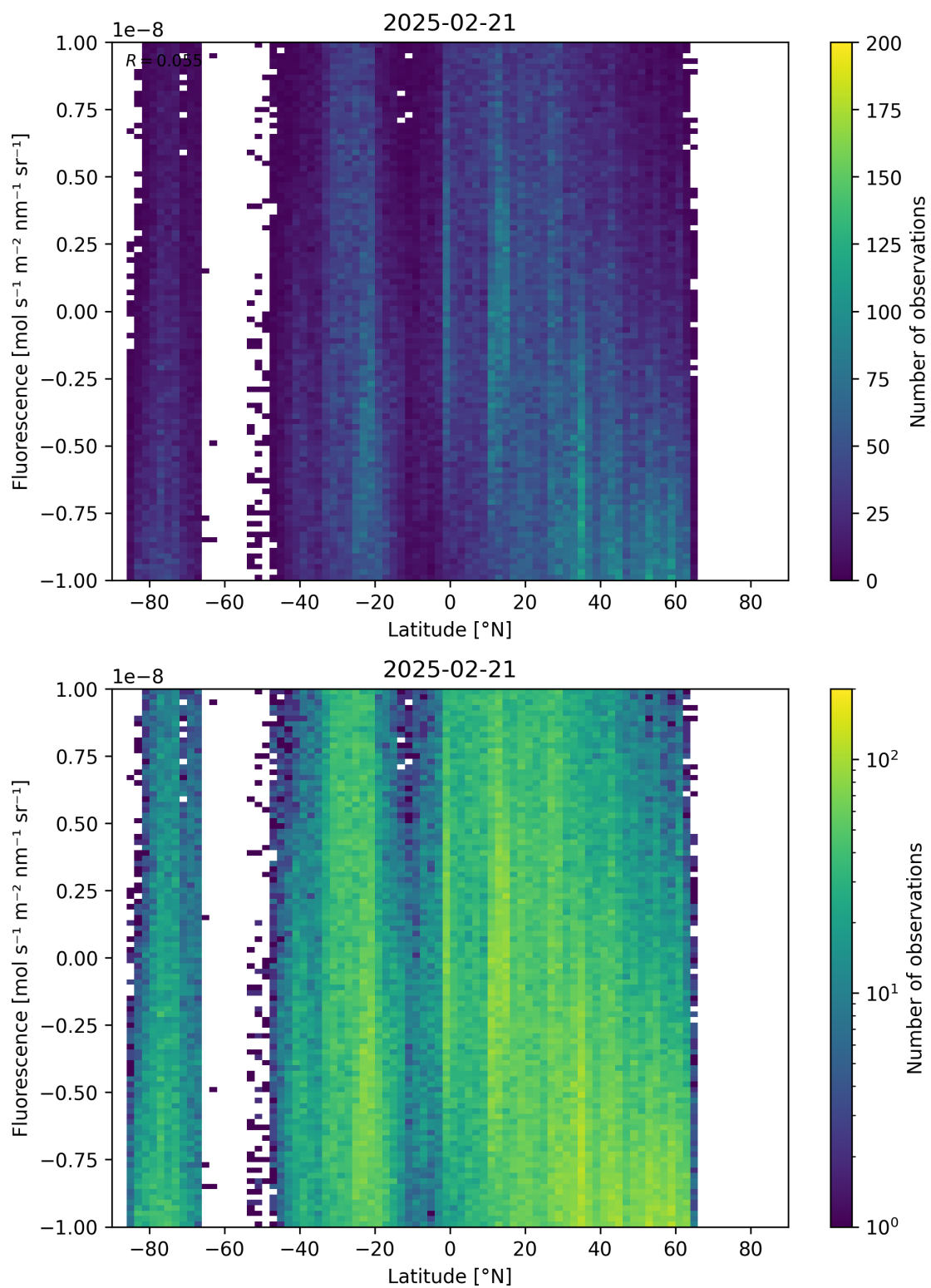
Figure 56: Scatter density plot of “Latitude” against “Fluorescence” for 2025-02-20 to 2025-02-22.
