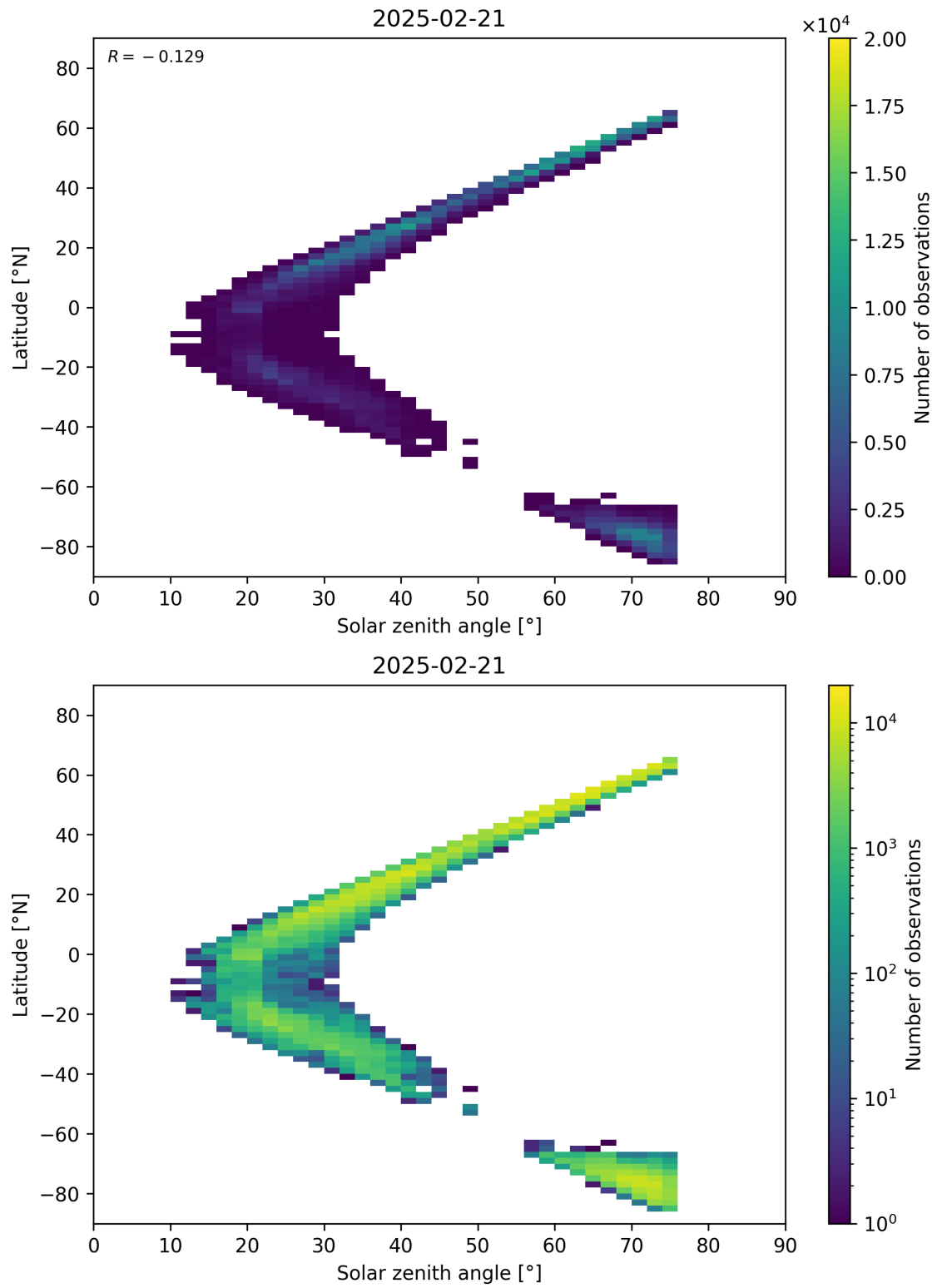
Figure 98: Scatter density plot of “Solar zenith angle” against “Latitude” for 2025-02-20 to 2025-02-22.
