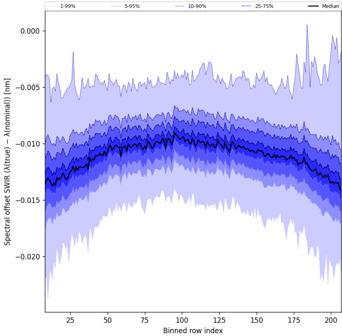
Figure 38: Along track statistics of “Spectral offset SWIR ( \lambda_{\text{true}} - \lambda_{\text{nominal}} )” for 2025-02-20 to 2025-02-22
