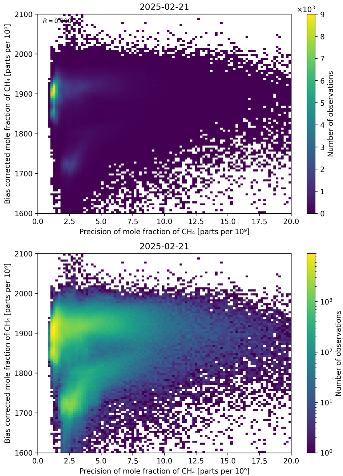
Figure 82: Scatter density plot of “Precision of mole fraction of CH 4 ” against “Bias corrected mole fraction of CH 4 ” for 2025-02-20 to 2025-02-22.
