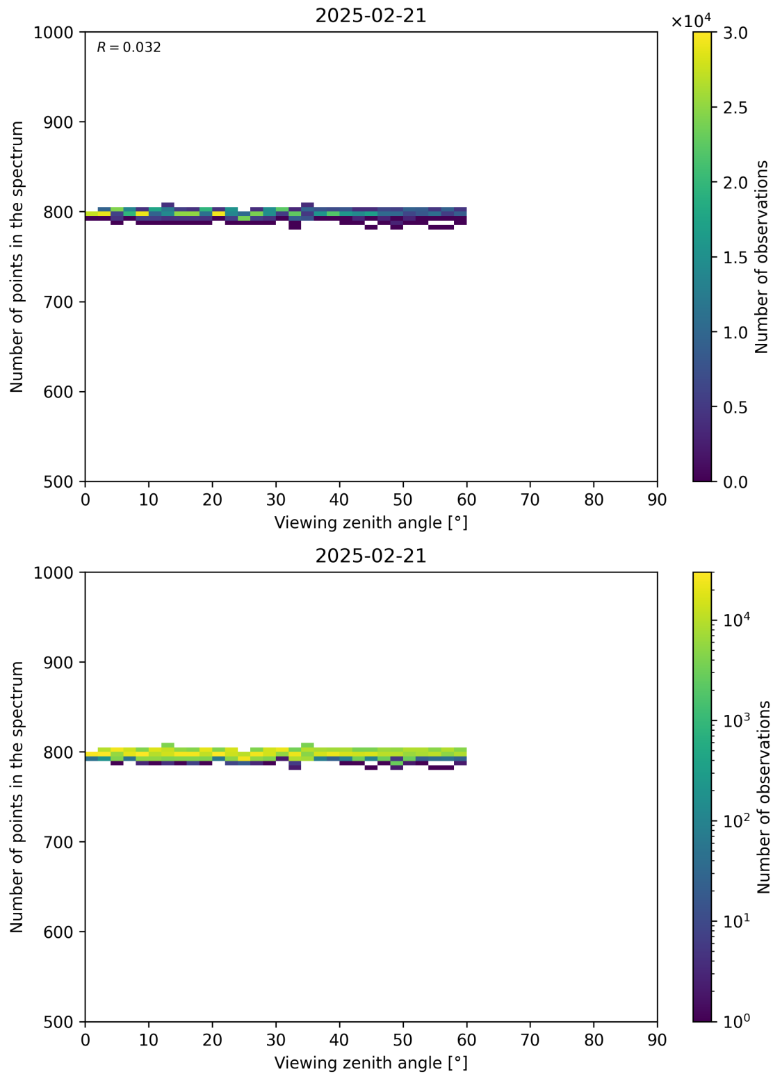
Figure 114: Scatter density plot of “Viewing zenith angle” against “Number of points in the spectrum” for 2025-02-20 to 2025-02-22.
