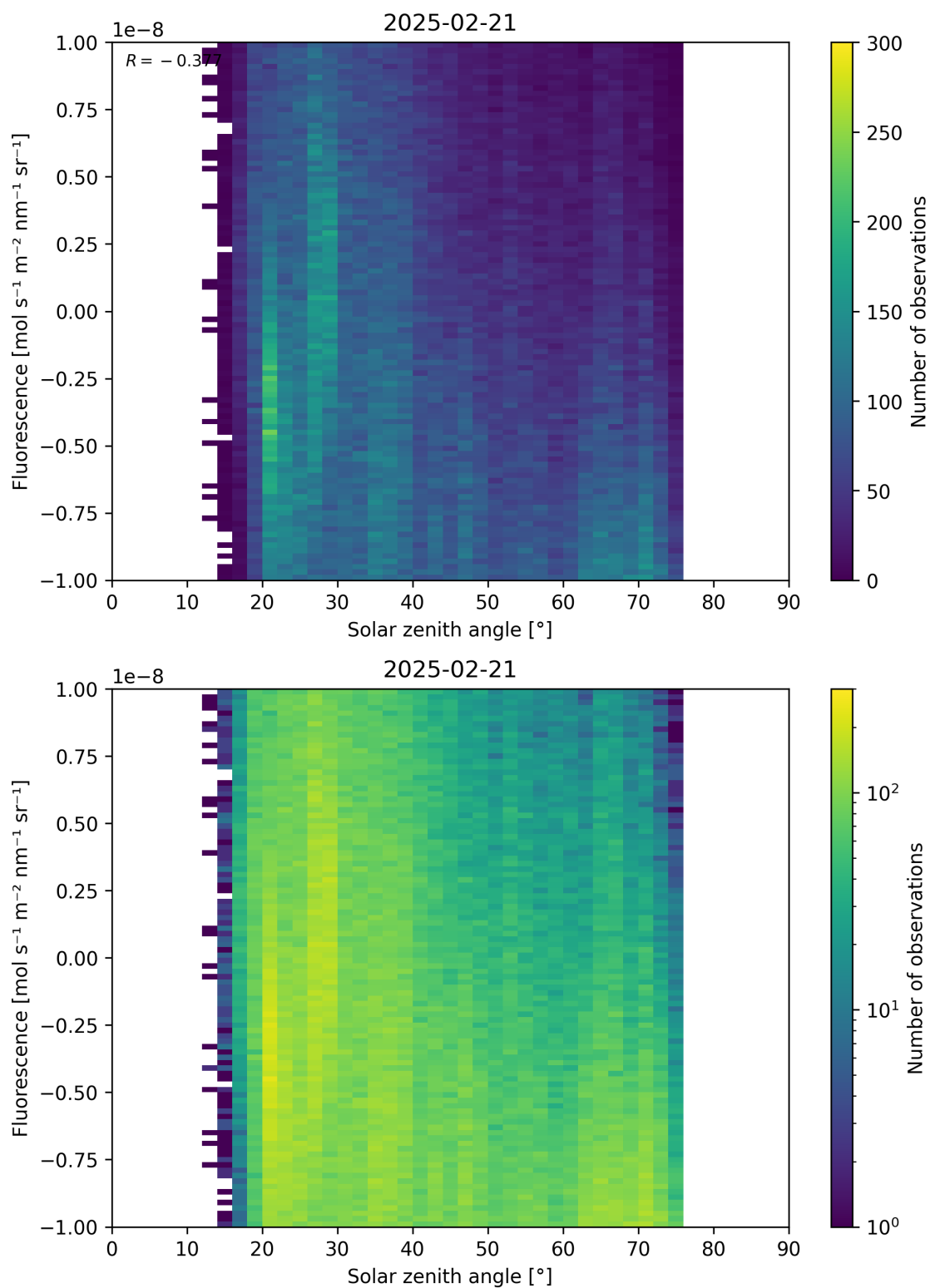
Figure 97: Scatter density plot of “Solar zenith angle” against “Fluorescence” for 2025-02-20 to 2025-02-22.
