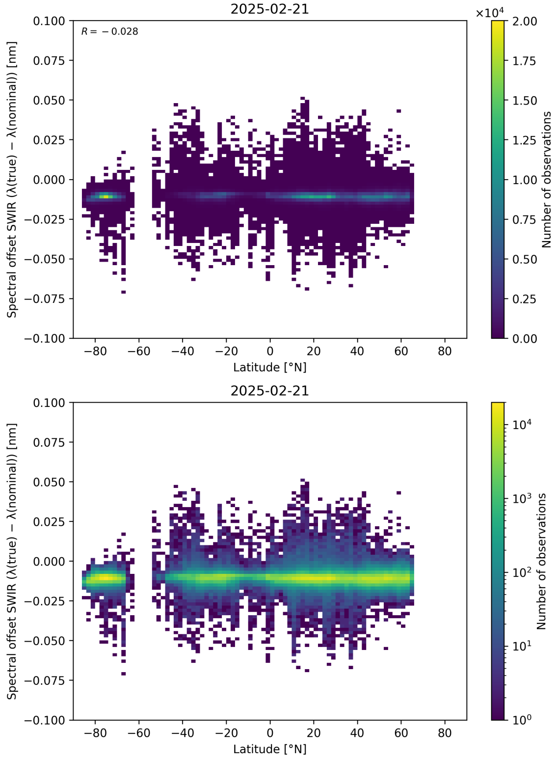
Figure 62: Scatter density plot of “Latitude” against “Spectral offset SWIR ( \lambda_{\text{true}} - \lambda_{\text{nominal}} )” for 2025-02-20 to 2025-02-22.
