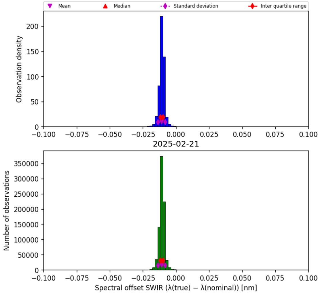
Figure 27: Histogram of “Spectral offset SWIR ( \lambda_{\text{true}} - \lambda_{\text{nominal}} )” for 2025-02-20 to 2025-02-22
