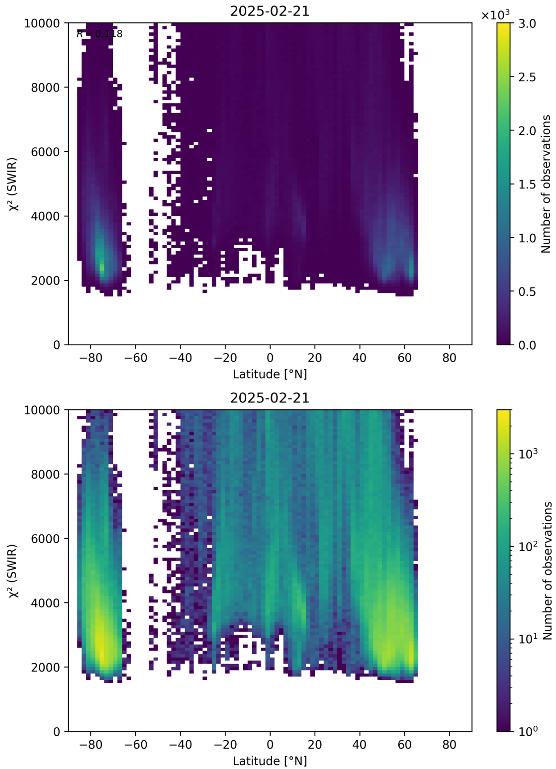
Figure 54: Scatter density plot of “Latitude” against “ \chi^2 (SWIR)” for 2025-02-20 to 2025-02-22.
