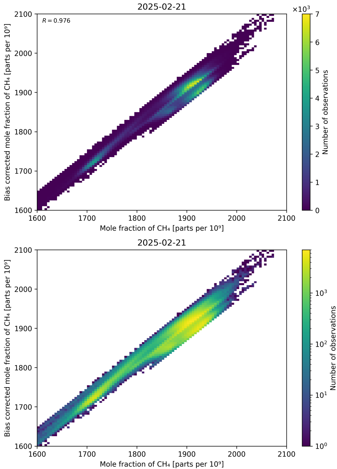
Figure 74: Scatter density plot of “Mole fraction of CH 4 ” against “Bias corrected mole fraction of CH 4 ” for 2025-02-20 to 2025-02-22.
