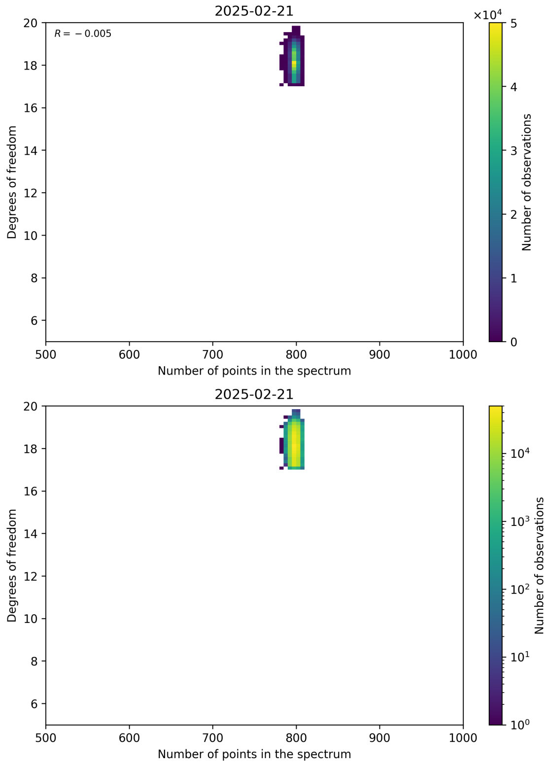
Figure 90: Scatter density plot of “Number of points in the spectrum” against “Degrees of freedom” for 2025-02-20 to 2025-02-22.
