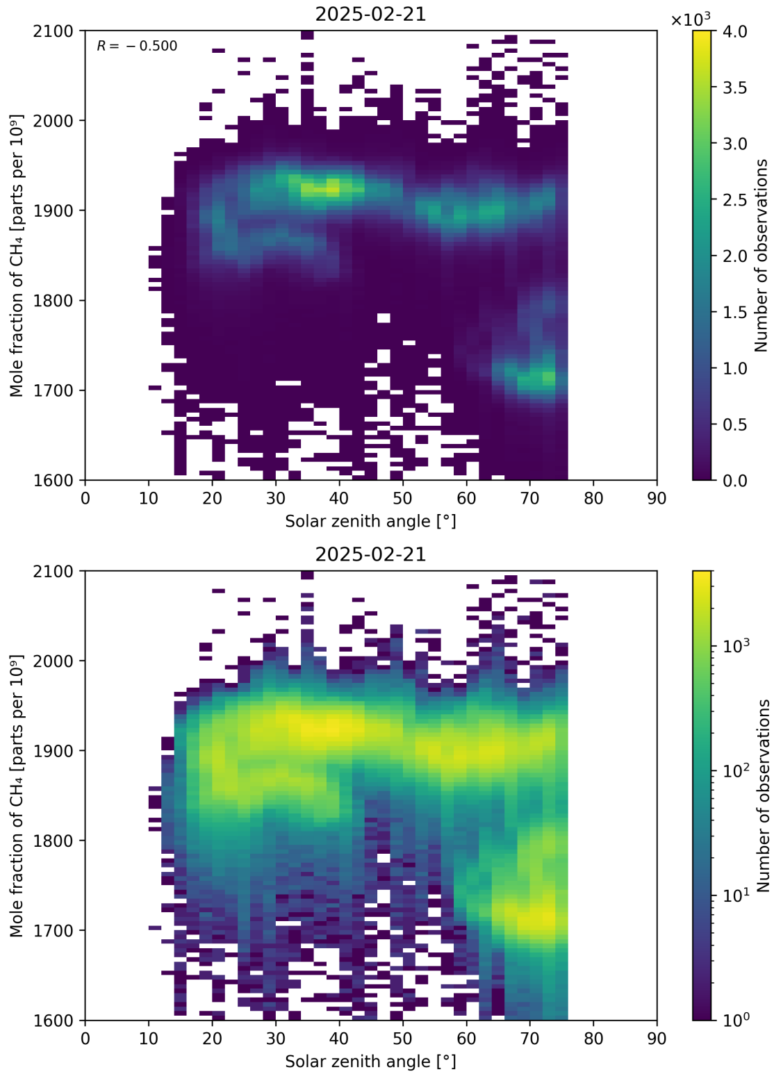
Figure 99: Scatter density plot of “Solar zenith angle” against “Mole fraction of CH 4 ” for 2025-02-20 to 2025-02-22.
