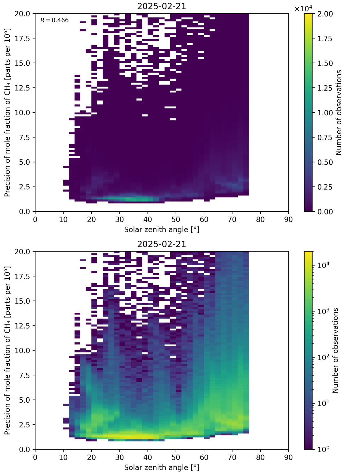
Figure 101: Scatter density plot of “Solar zenith angle” against “Precision of mole fraction of CH 4 ” for 2025-02-20 to 2025-02-22.
