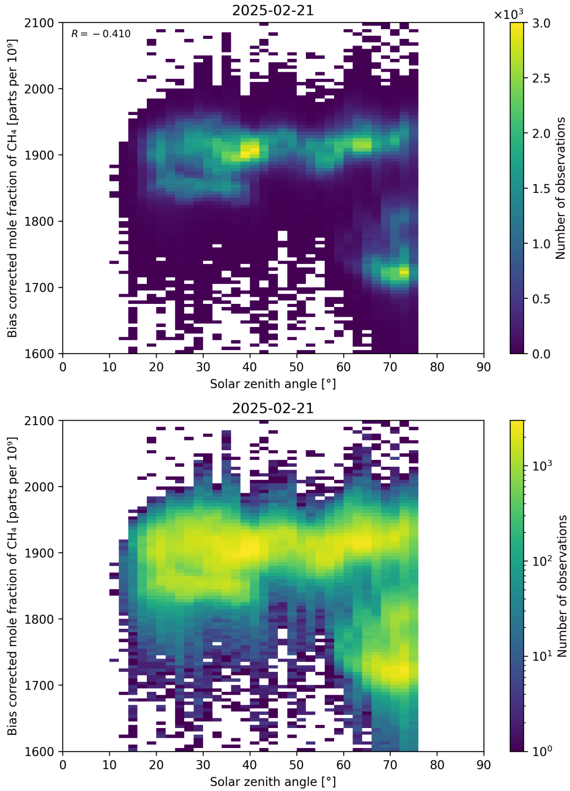
Figure 100: Scatter density plot of “Solar zenith angle” against “Bias corrected mole fraction of \text{CH}_4 ” for 2025-02-20 to 2025-02-22.
