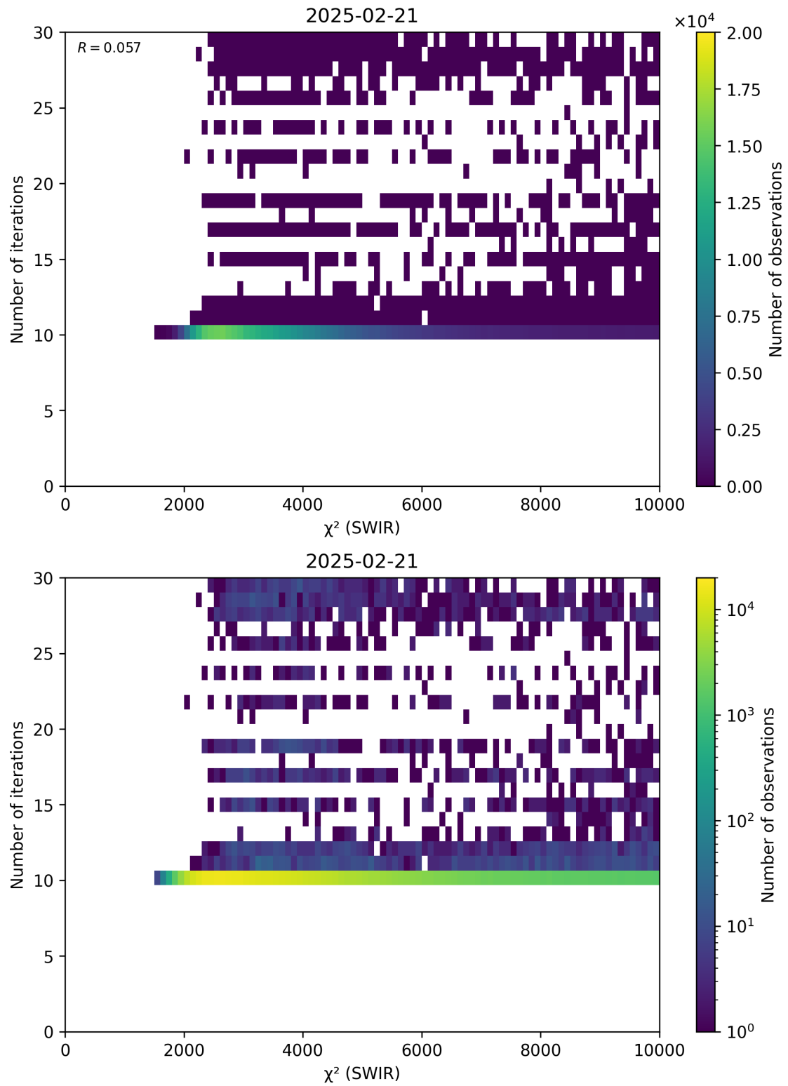
Figure 50: Scatter density plot of “ \chi^2 (SWIR)” against “Number of iterations” for 2025-02-20 to 2025-02-22.
