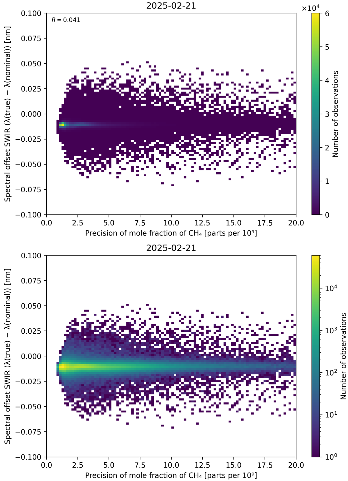
Figure 85: Scatter density plot of “Precision of mole fraction of \text{CH}_4 ” against “Spectral offset SWIR ( \lambda_{\text{true}} - \lambda_{\text{nominal}} )” for 2025-02-20 to 2025-02-22.
