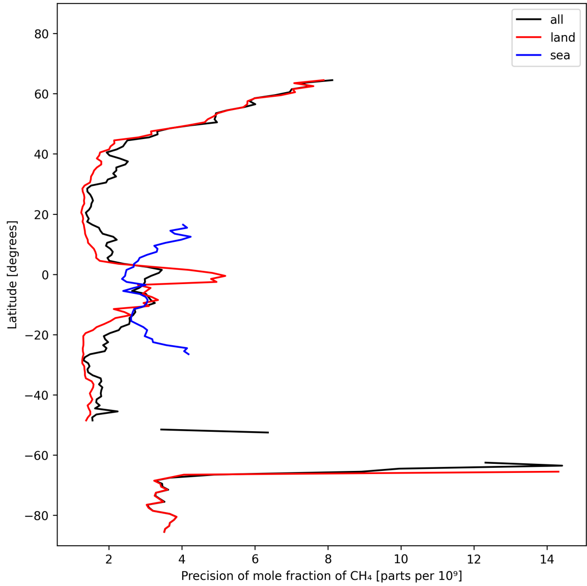
Figure 13: Zonal average of “Precision of mole fraction of CH 4 ” for 2025-02-20 to 2025-02-22.
