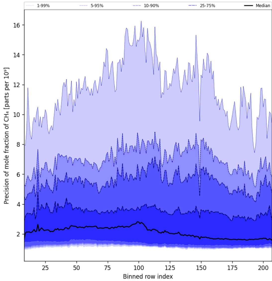
Figure 35: Along track statistics of “Precision of mole fraction of CH 4 ” for 2025-02-20 to 2025-02-22
