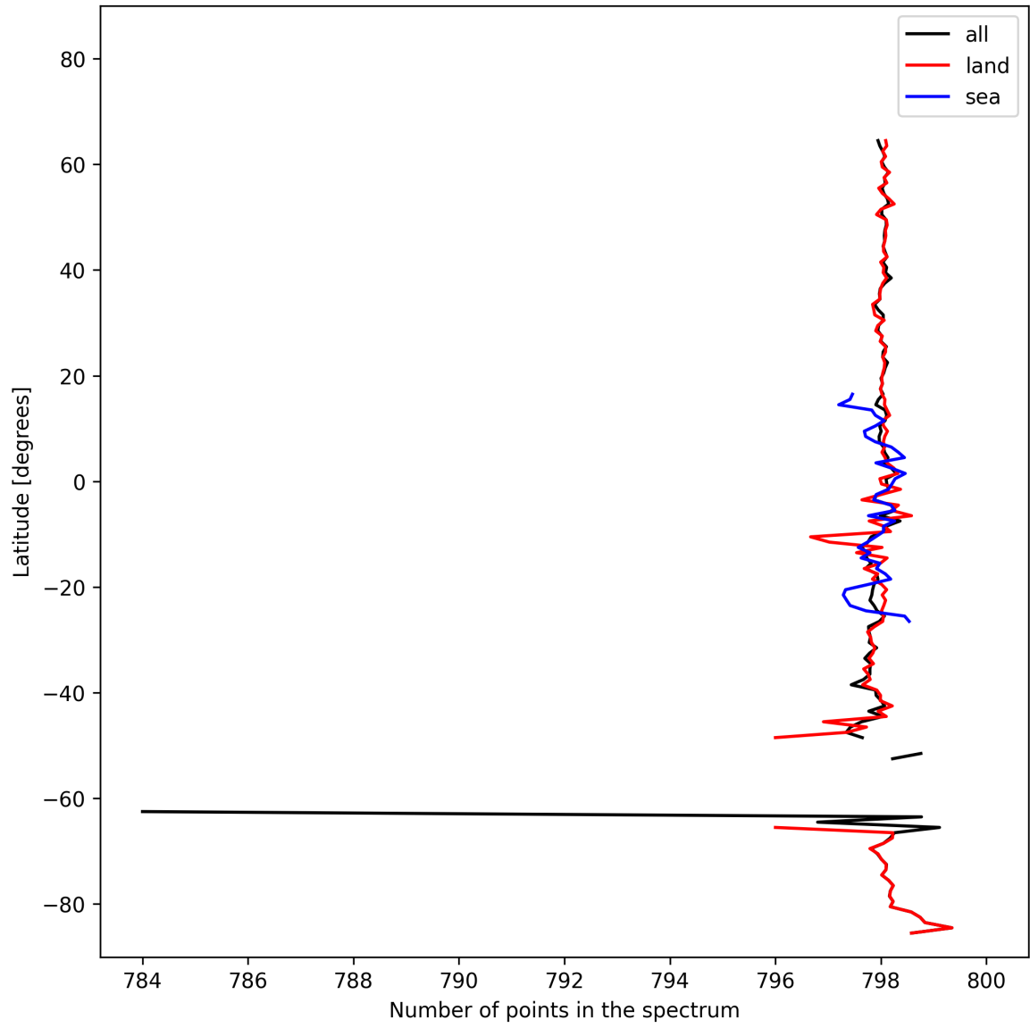
Figure 15: Zonal average of “Number of points in the spectrum” for 2025-02-20 to 2025-02-22.
