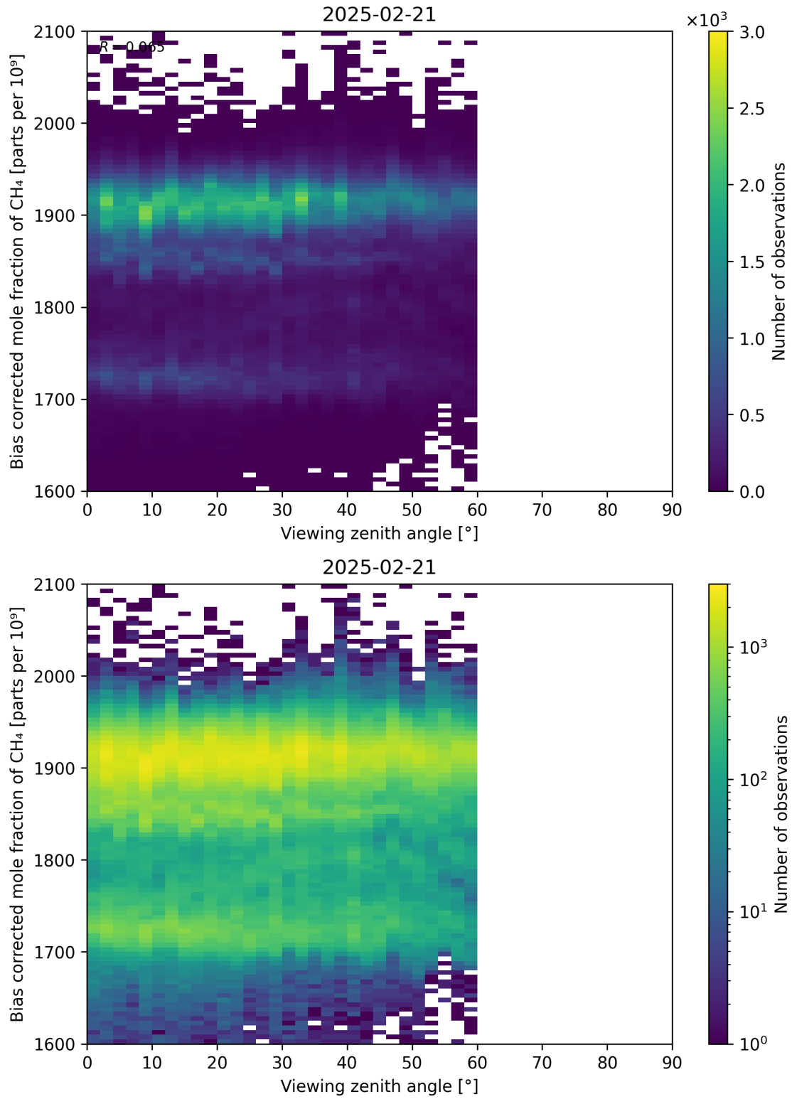
Figure 111: Scatter density plot of “Viewing zenith angle” against “Bias corrected mole fraction of \text{CH}_4 ” for 2025-02-20 to 2025-02-22.
