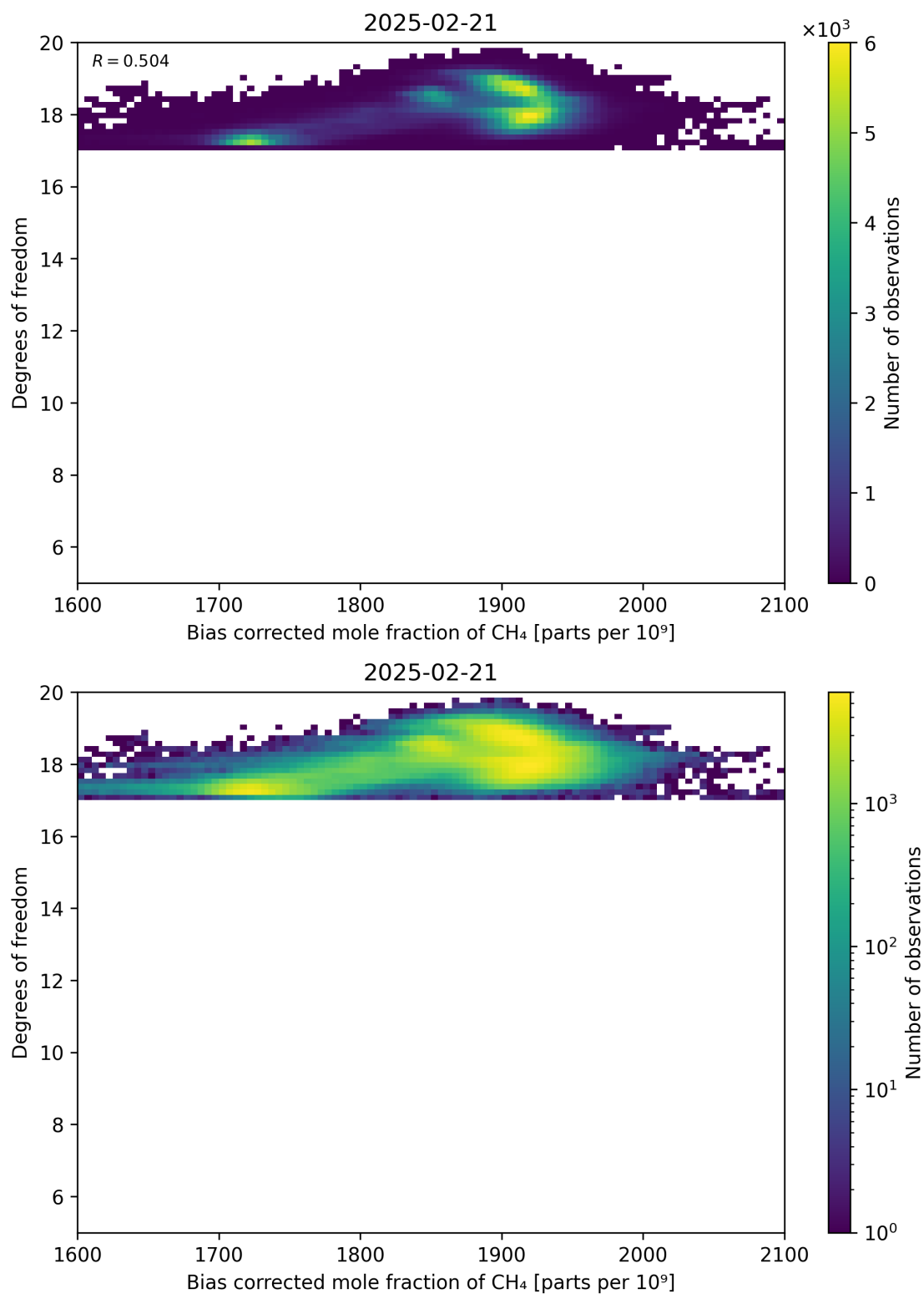
Figure 65: Scatter density plot of “Bias corrected mole fraction of CH 4 ” against “Degrees of freedom” for 2025-02-20 to 2025-02-22.
