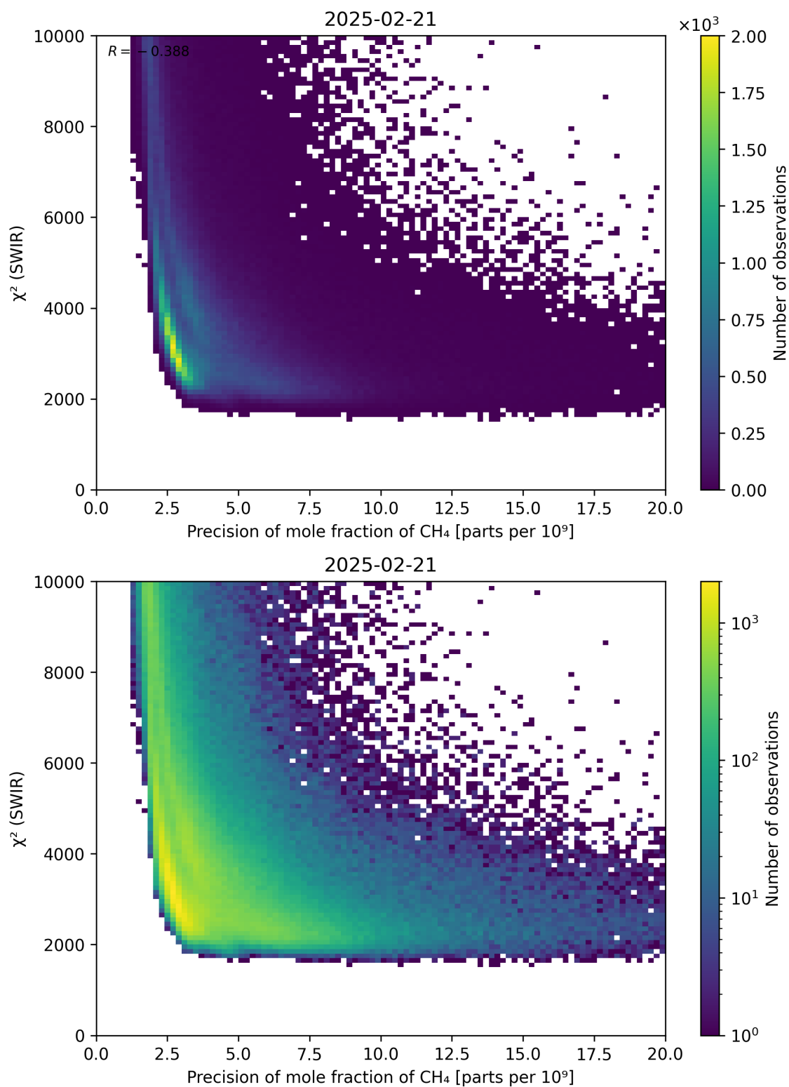
Figure 79: Scatter density plot of “Precision of mole fraction of \text{CH}_4 ” against “ \chi^2 (SWIR)” for 2025-02-20 to 2025-02-22.
