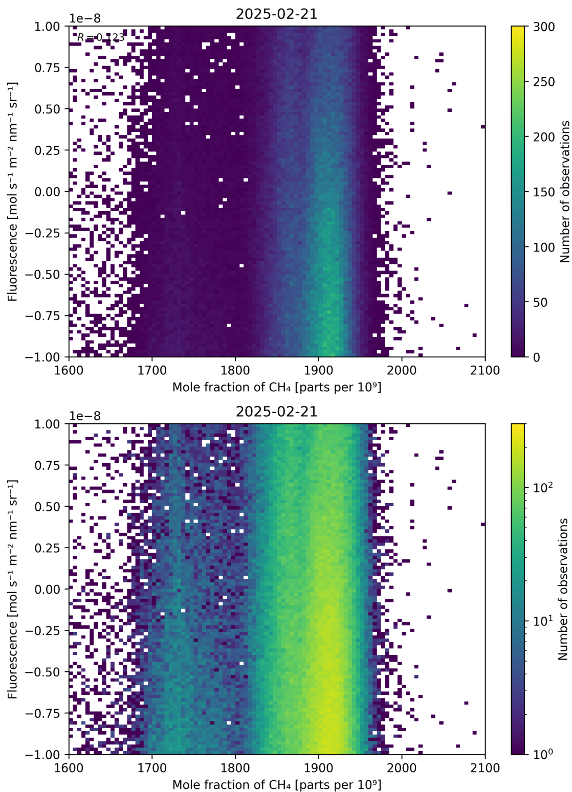
Figure 73: Scatter density plot of “Mole fraction of \text{CH}_4 ” against “Fluorescence” for 2025-02-20 to 2025-02-22.
