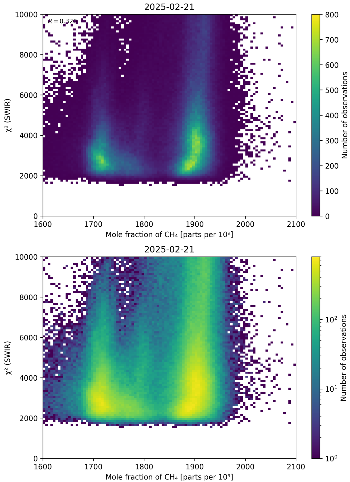
Figure 71: Scatter density plot of “Mole fraction of CH 4 ” against “ \chi^2 (SWIR)” for 2025-02-20 to 2025-02-22.
