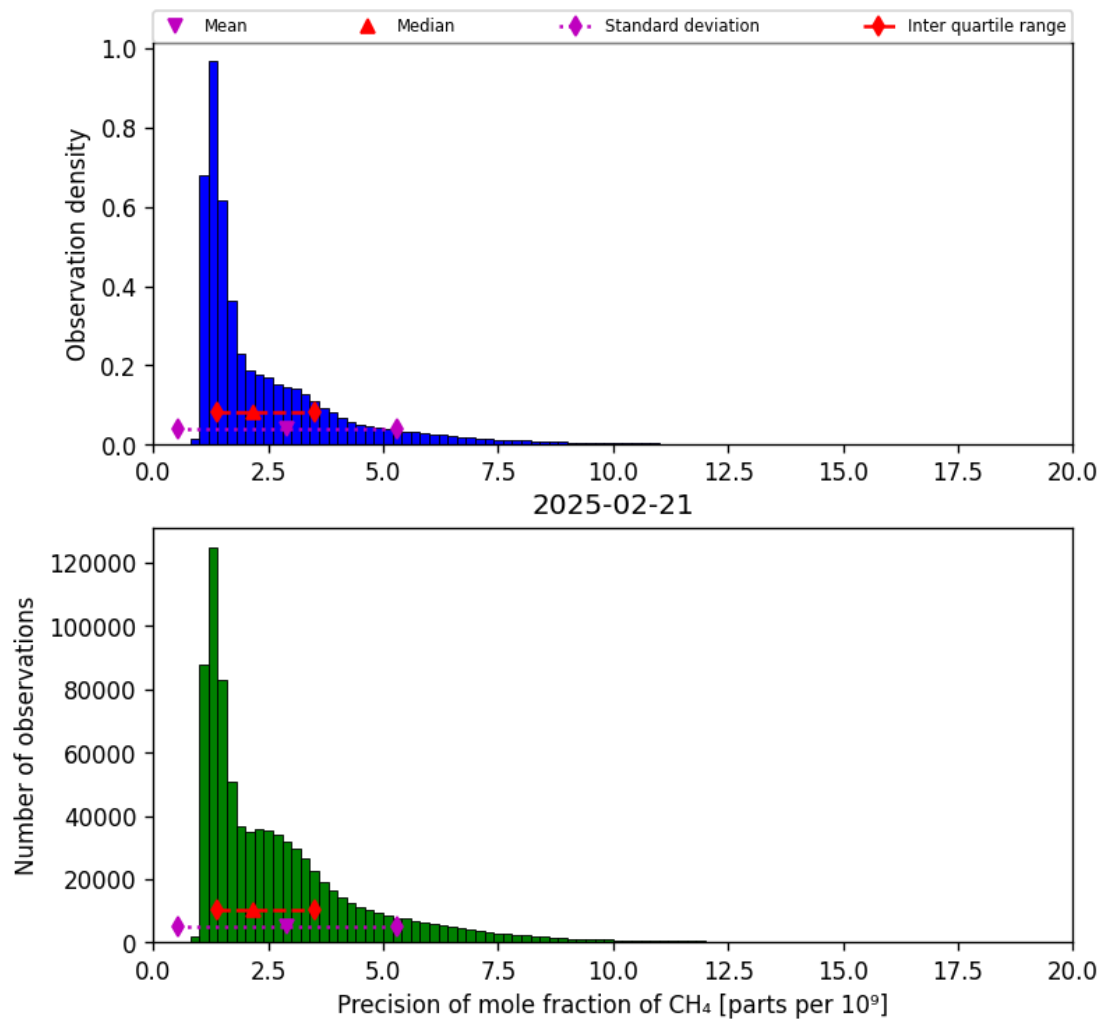
Figure 24: Histogram of “Precision of mole fraction of CH 4 ” for 2025-02-20 to 2025-02-22
