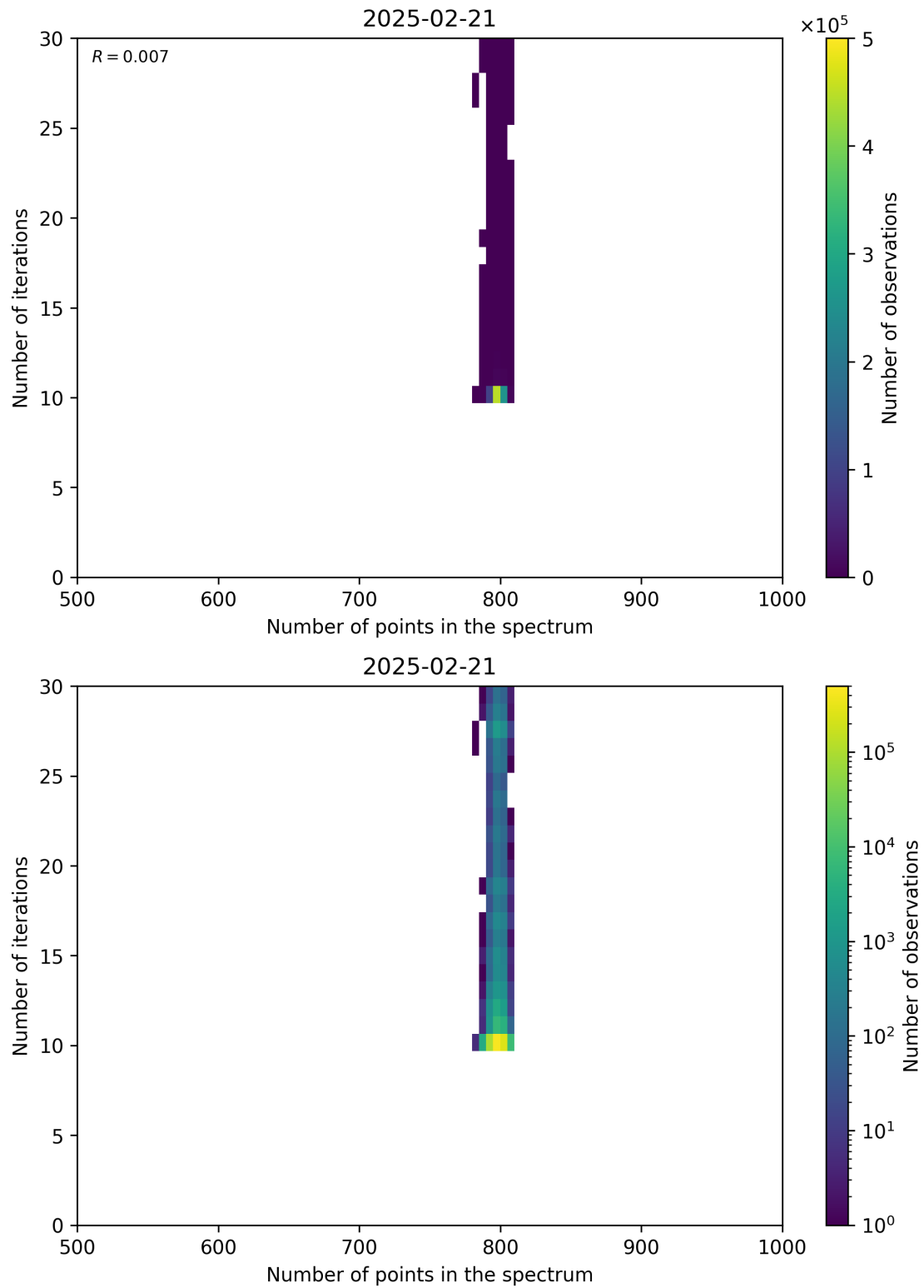
Figure 92: Scatter density plot of “Number of points in the spectrum” against “Number of iterations” for 2025-02-20 to 2025-02-22.
