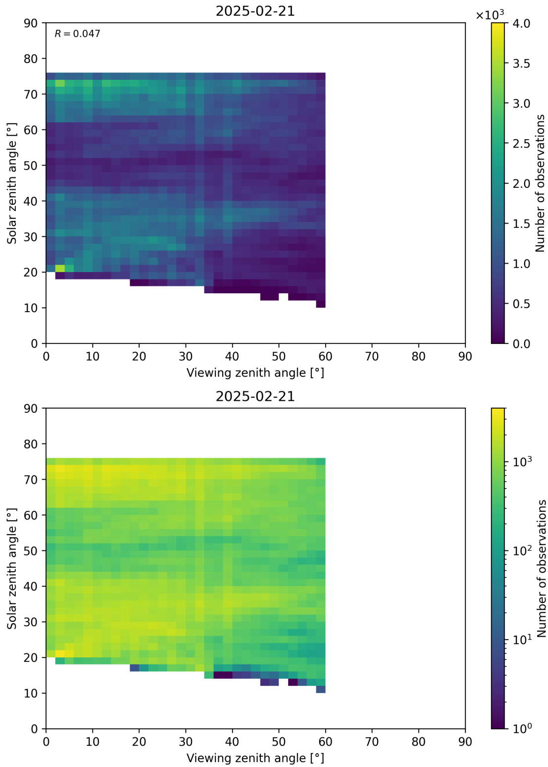
Figure 115: Scatter density plot of “Viewing zenith angle” against “Solar zenith angle” for 2025-02-20 to 2025-02-22.
