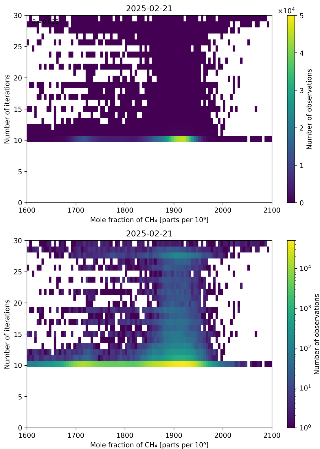
Figure 76: Scatter density plot of “Mole fraction of CH 4 ” against “Number of iterations” for 2025-02-20 to 2025-02-22.
