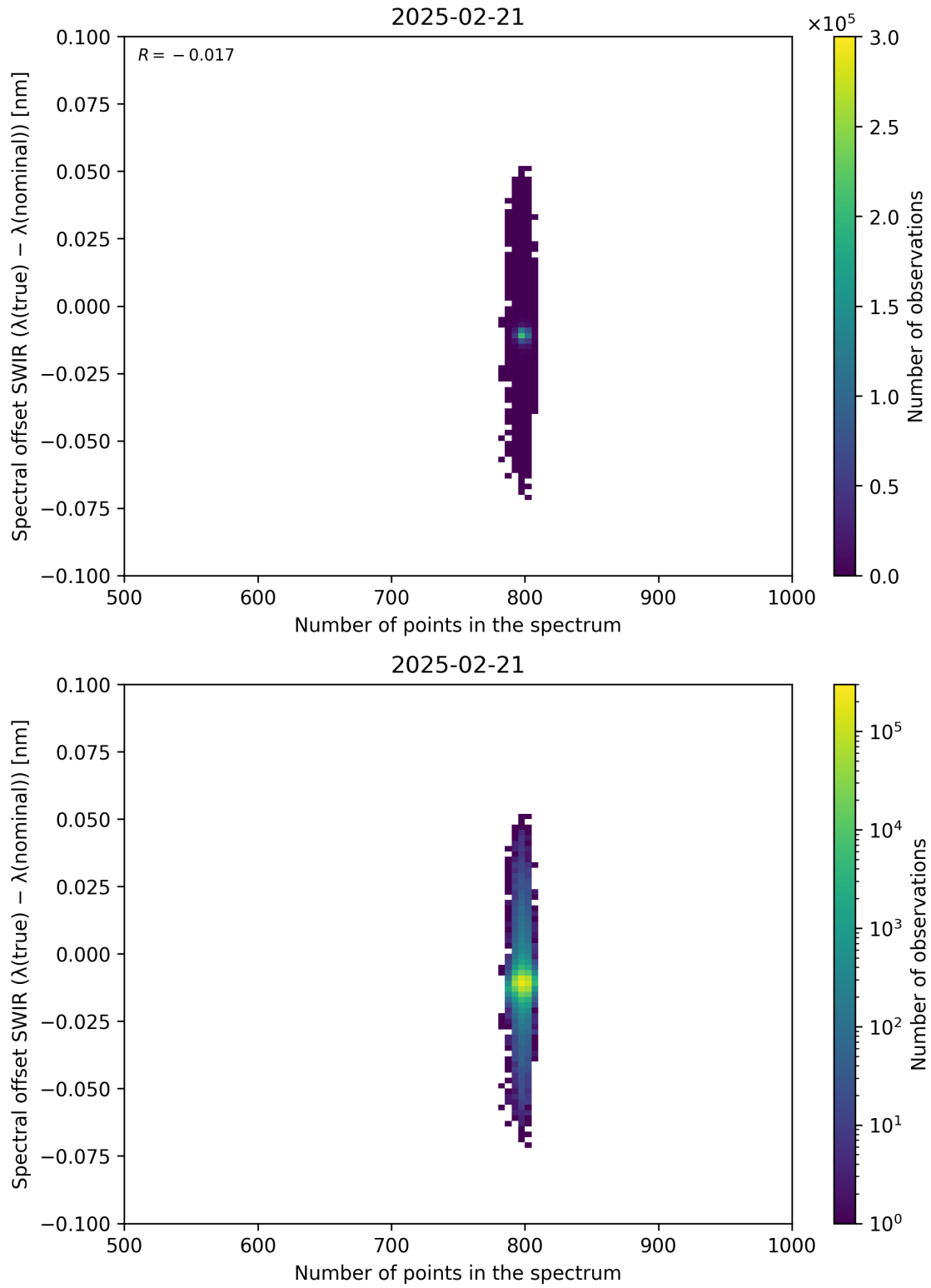
Figure 93: Scatter density plot of “Number of points in the spectrum” against “Spectral offset SWIR ( \lambda_{\text{true}} - \lambda_{\text{nominal}} )” for 2025-02-20 to 2025-02-22.
