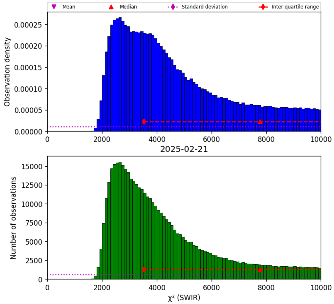
Figure 28: Histogram of “ \chi^2 (SWIR)” for 2025-02-20 to 2025-02-22
