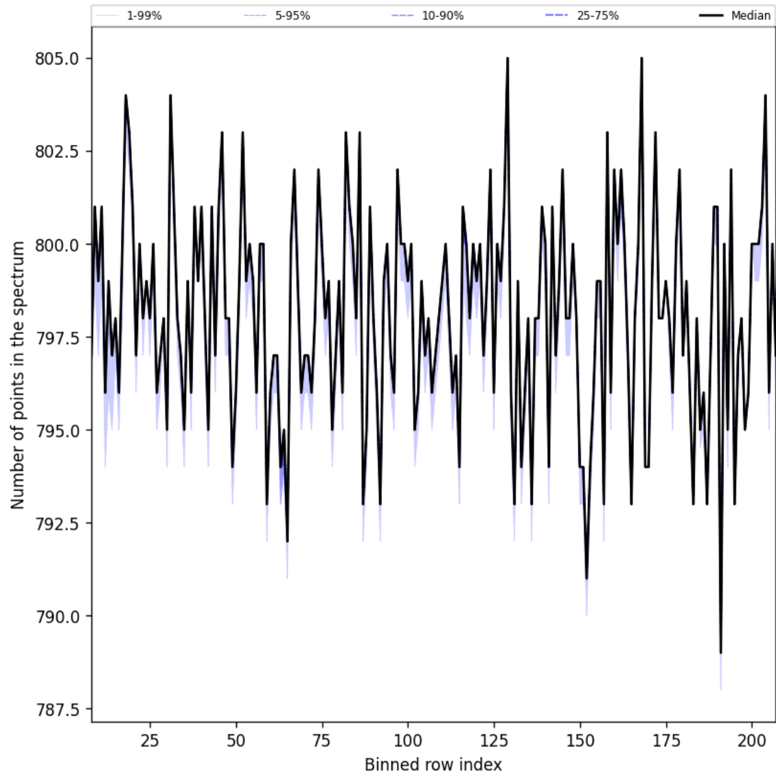
Figure 37: Along track statistics of “Number of points in the spectrum” for 2025-02-20 to 2025-02-22
