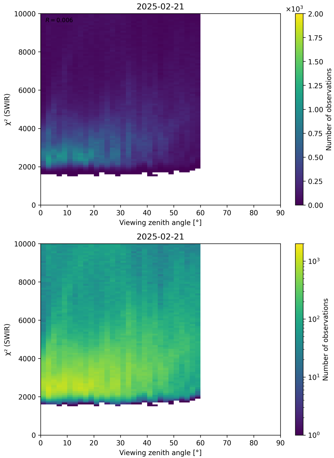
Figure 106: Scatter density plot of “Viewing zenith angle” against “ \chi^2 (SWIR)” for 2025-02-20 to 2025-02-22.
