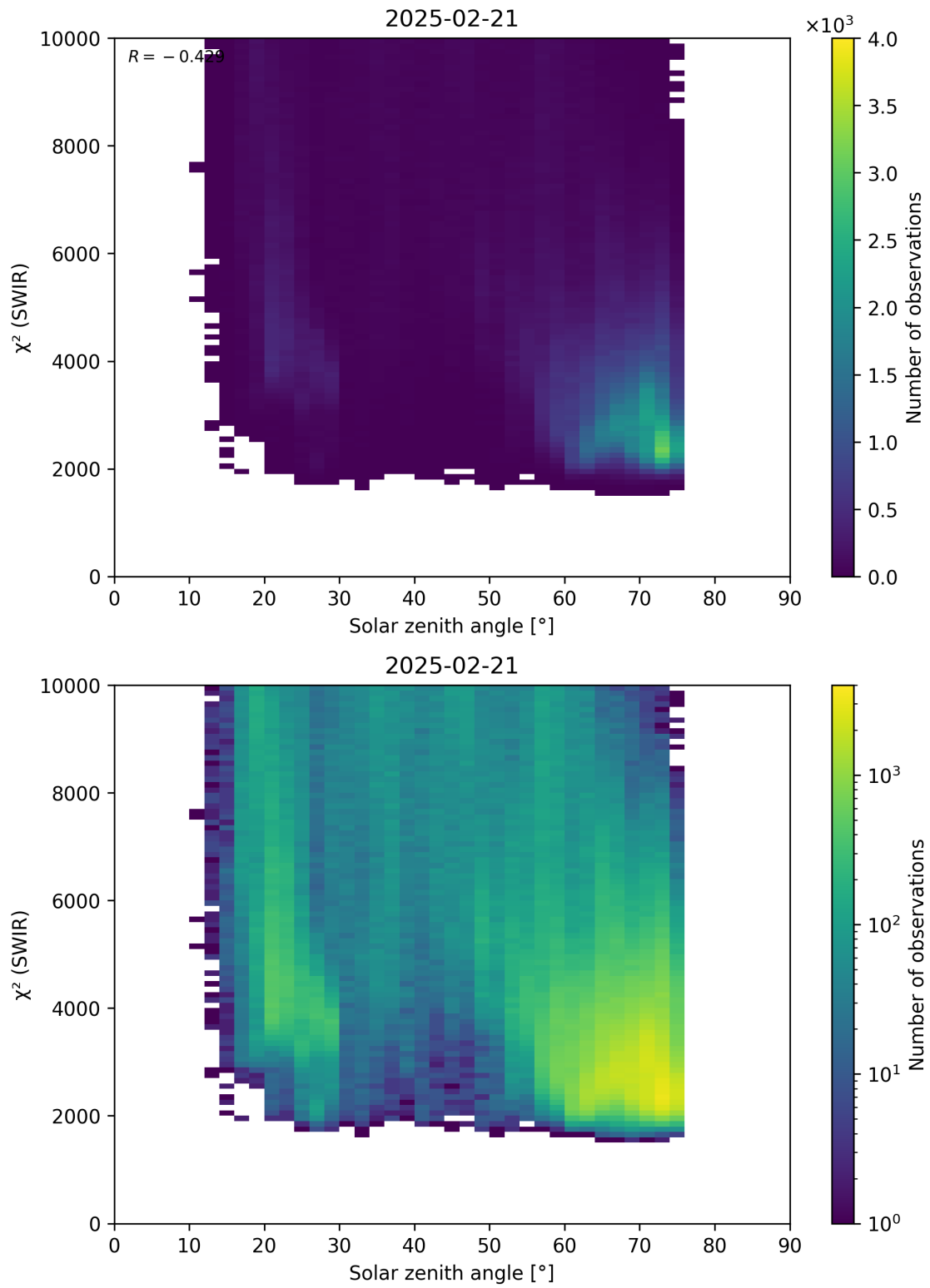
Figure 95: Scatter density plot of “Solar zenith angle” against “ \chi^2 (SWIR)” for 2025-02-20 to 2025-02-22.
