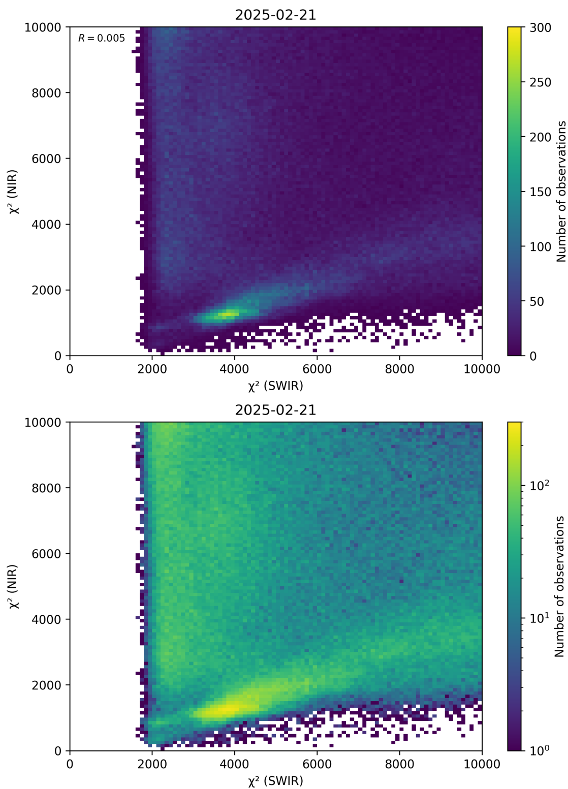
Figure 47: Scatter density plot of “ \chi^2 (SWIR)” against “ \chi^2 (NIR)” for 2025-02-20 to 2025-02-22.
