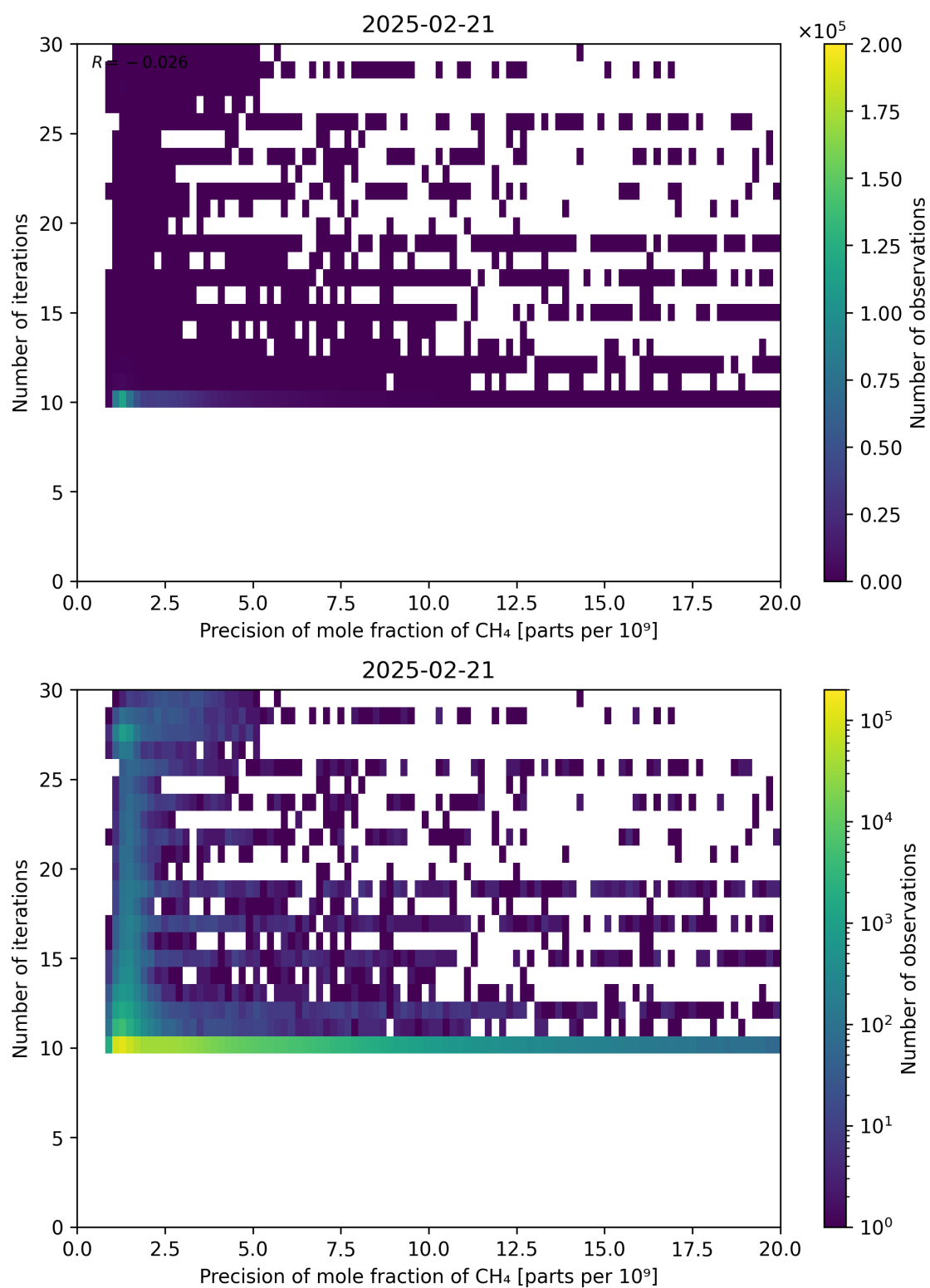
Figure 83: Scatter density plot of “Precision of mole fraction of CH 4 ” against “Number of iterations” for 2025-02-20 to 2025-02-22.
