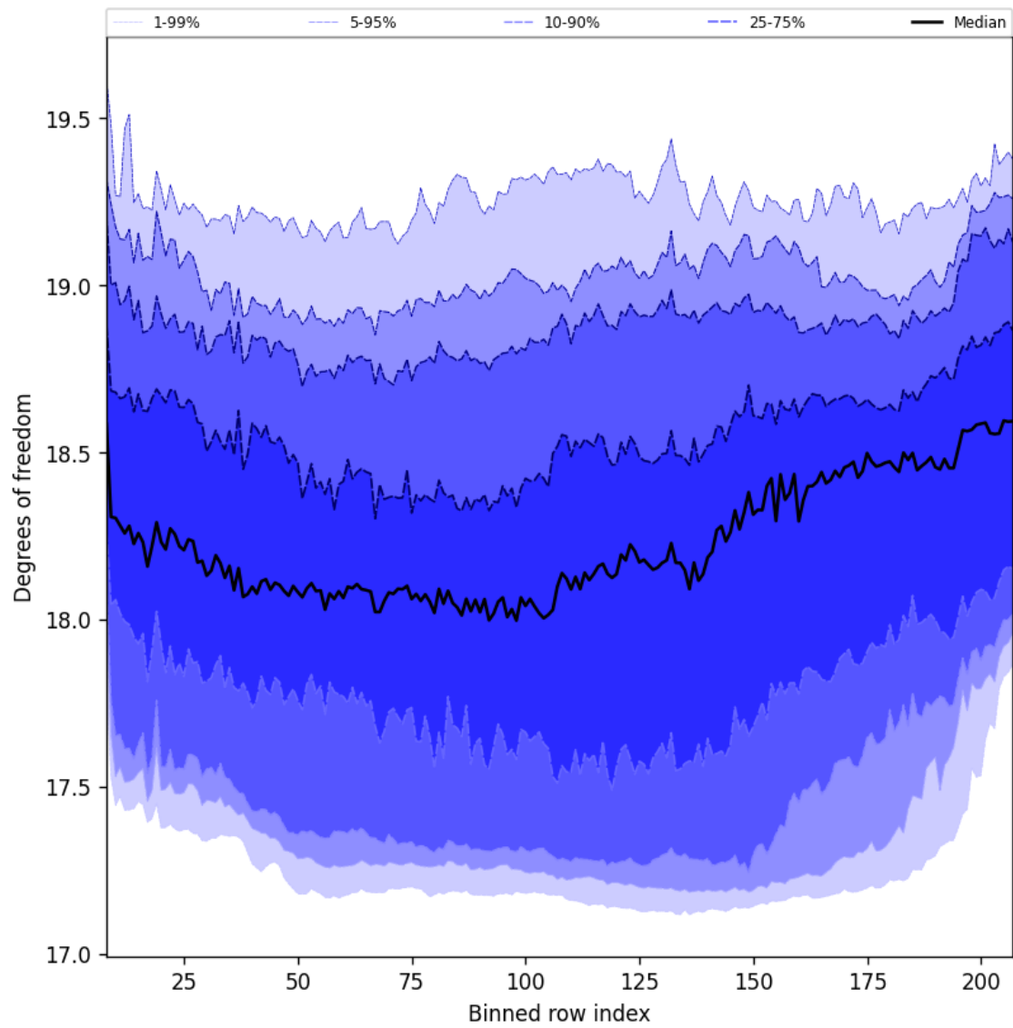
Figure 41: Along track statistics of “Degrees of freedom” for 2025-02-21 to 2025-02-23
