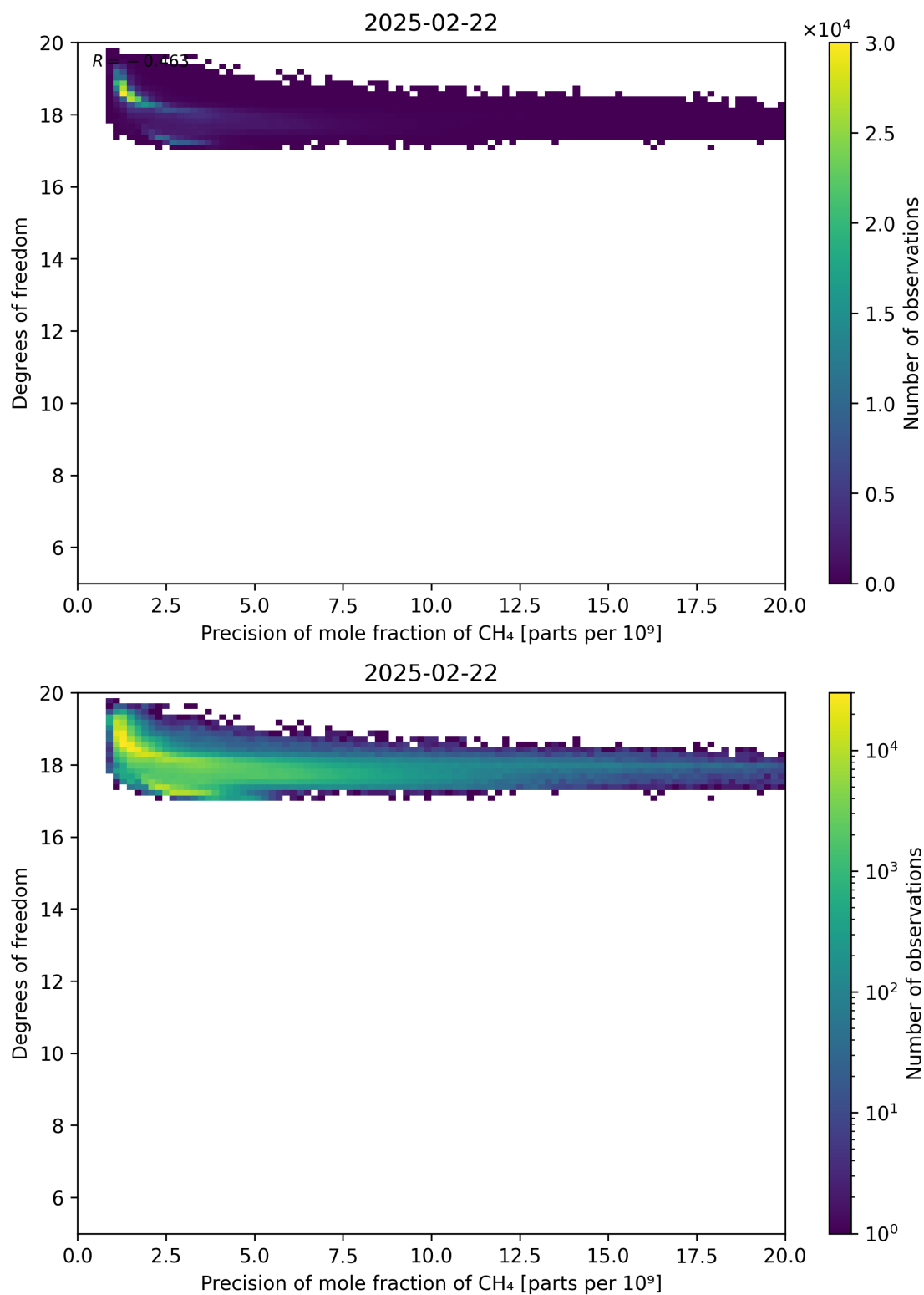
Figure 80: Scatter density plot of “Precision of mole fraction of CH 4 ” against “Degrees of freedom” for 2025-02-21 to 2025-02-23.
