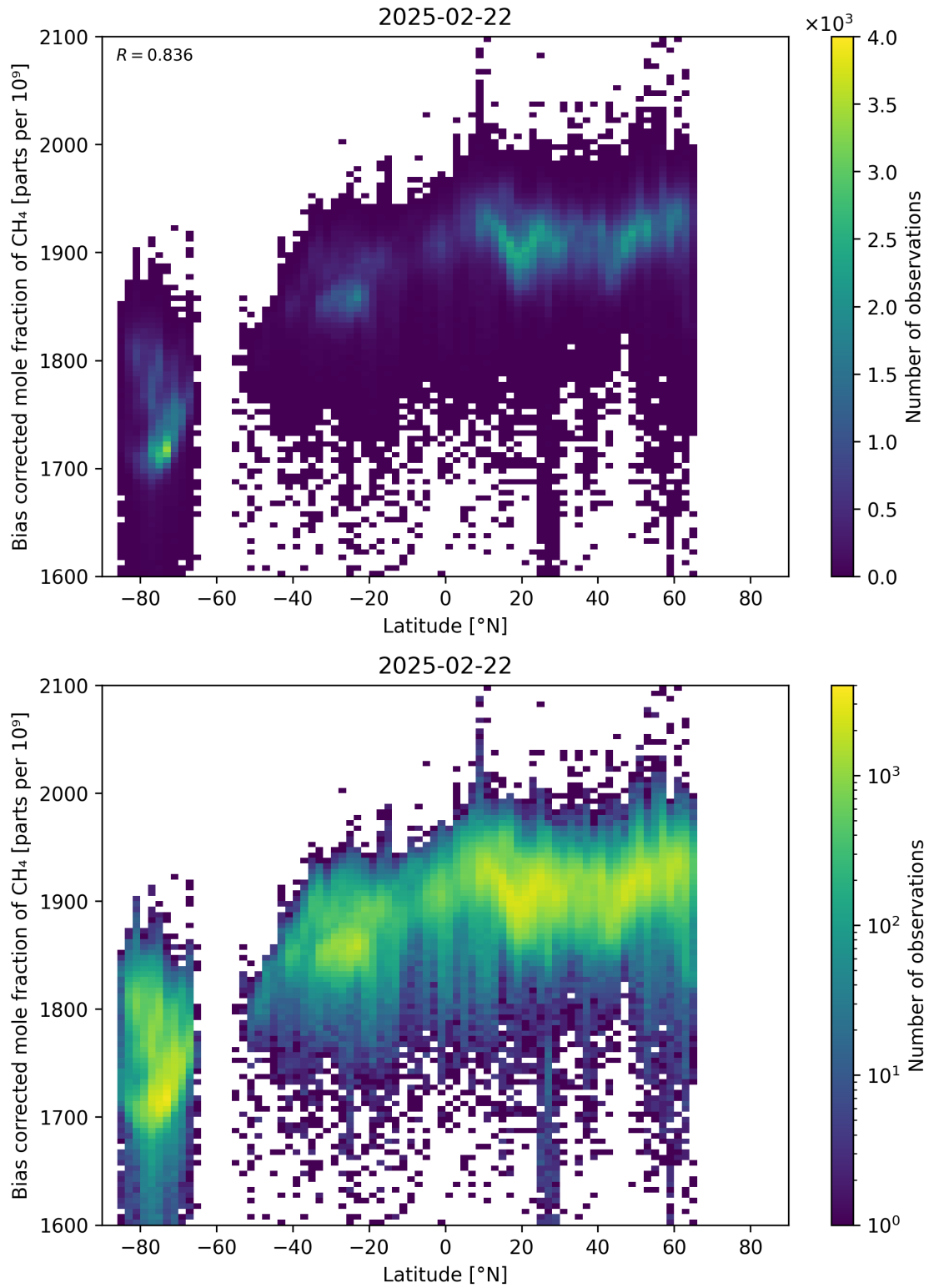
Figure 58: Scatter density plot of “Latitude” against “Bias corrected mole fraction of CH 4 ” for 2025-02-21 to 2025-02-23.
