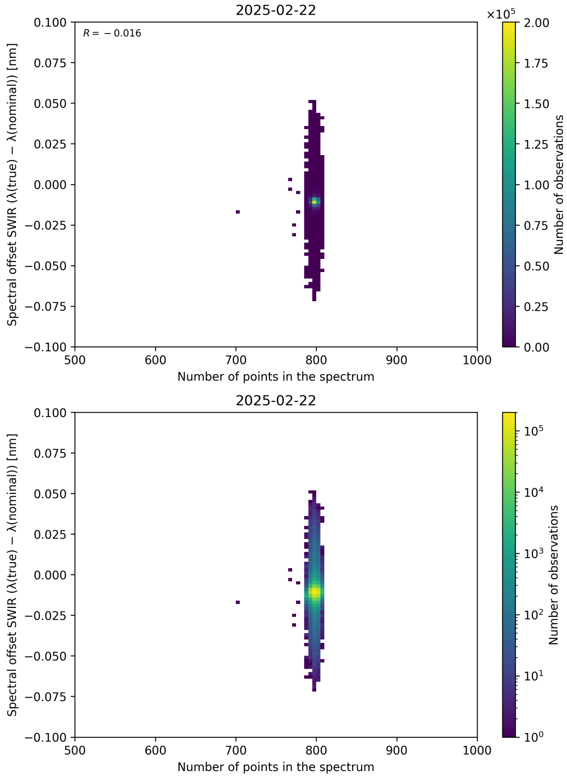
Figure 93: Scatter density plot of “Number of points in the spectrum” against “Spectral offset SWIR ( \lambda_{\text{true}} - \lambda_{\text{nominal}} )” for 2025-02-21 to 2025-02-23.
