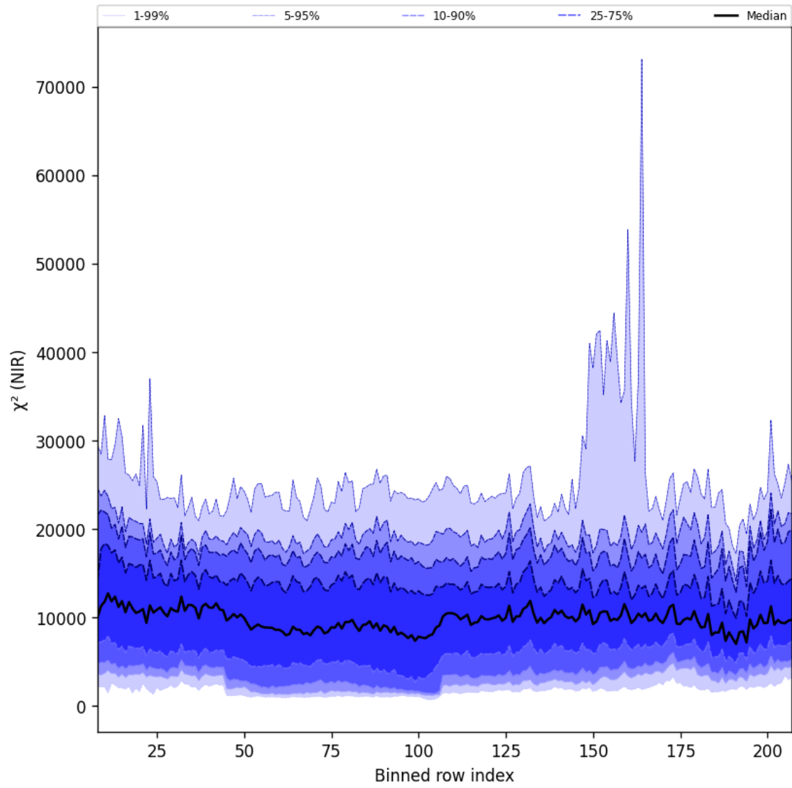
Figure 40: Along track statistics of “ \chi^2 (NIR)” for 2025-02-21 to 2025-02-23
