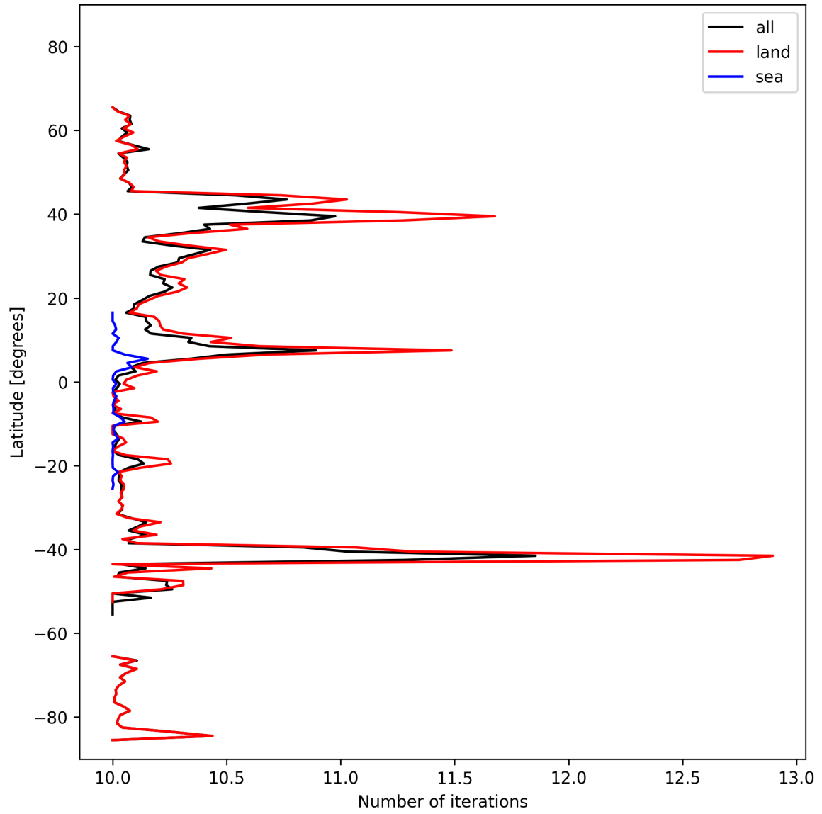
Figure 20: Zonal average of “Number of iterations” for 2025-02-21 to 2025-02-23.
