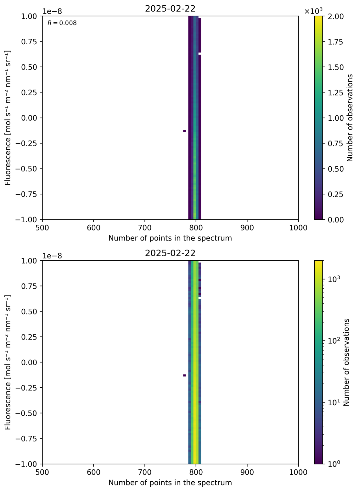
Figure 91: Scatter density plot of “Number of points in the spectrum” against “Fluorescence” for 2025-02-21 to 2025-02-23.
