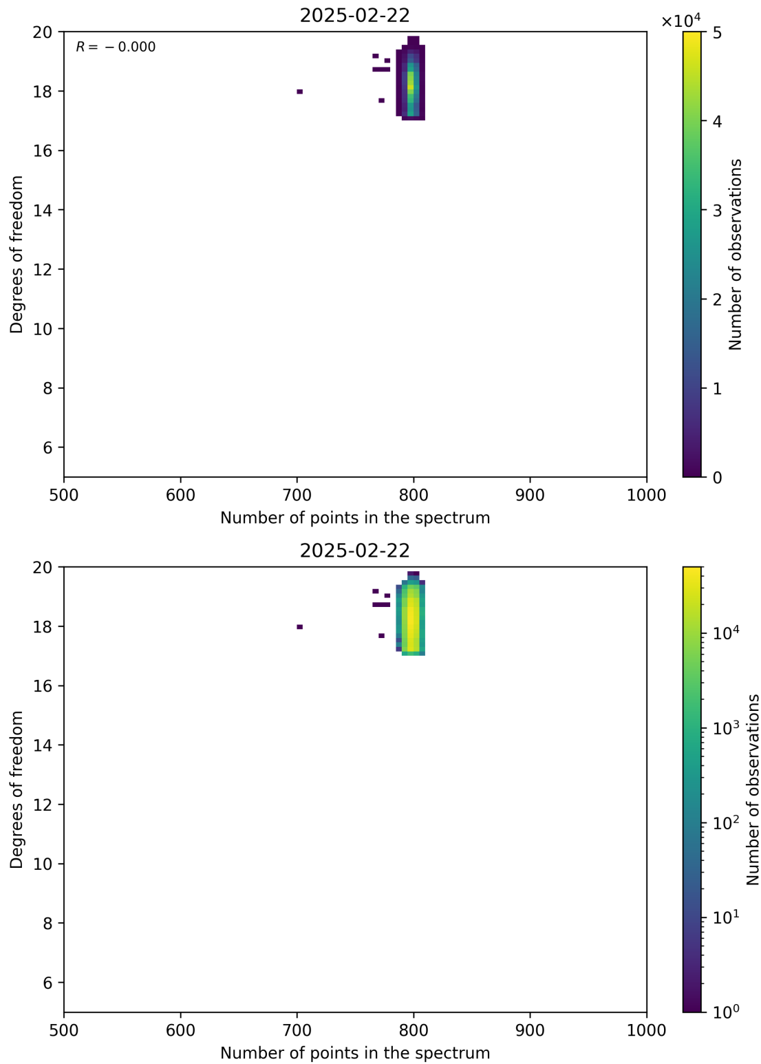
Figure 90: Scatter density plot of “Number of points in the spectrum” against “Degrees of freedom” for 2025-02-21 to 2025-02-23.
