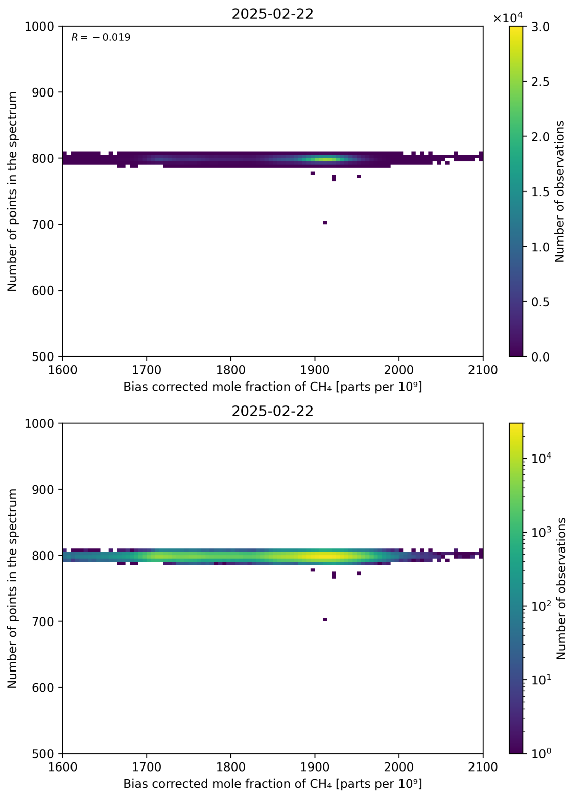
Figure 68: Scatter density plot of “Bias corrected mole fraction of CH 4 ” against “Number of points in the spectrum” for 2025-02-21 to 2025-02-23.
