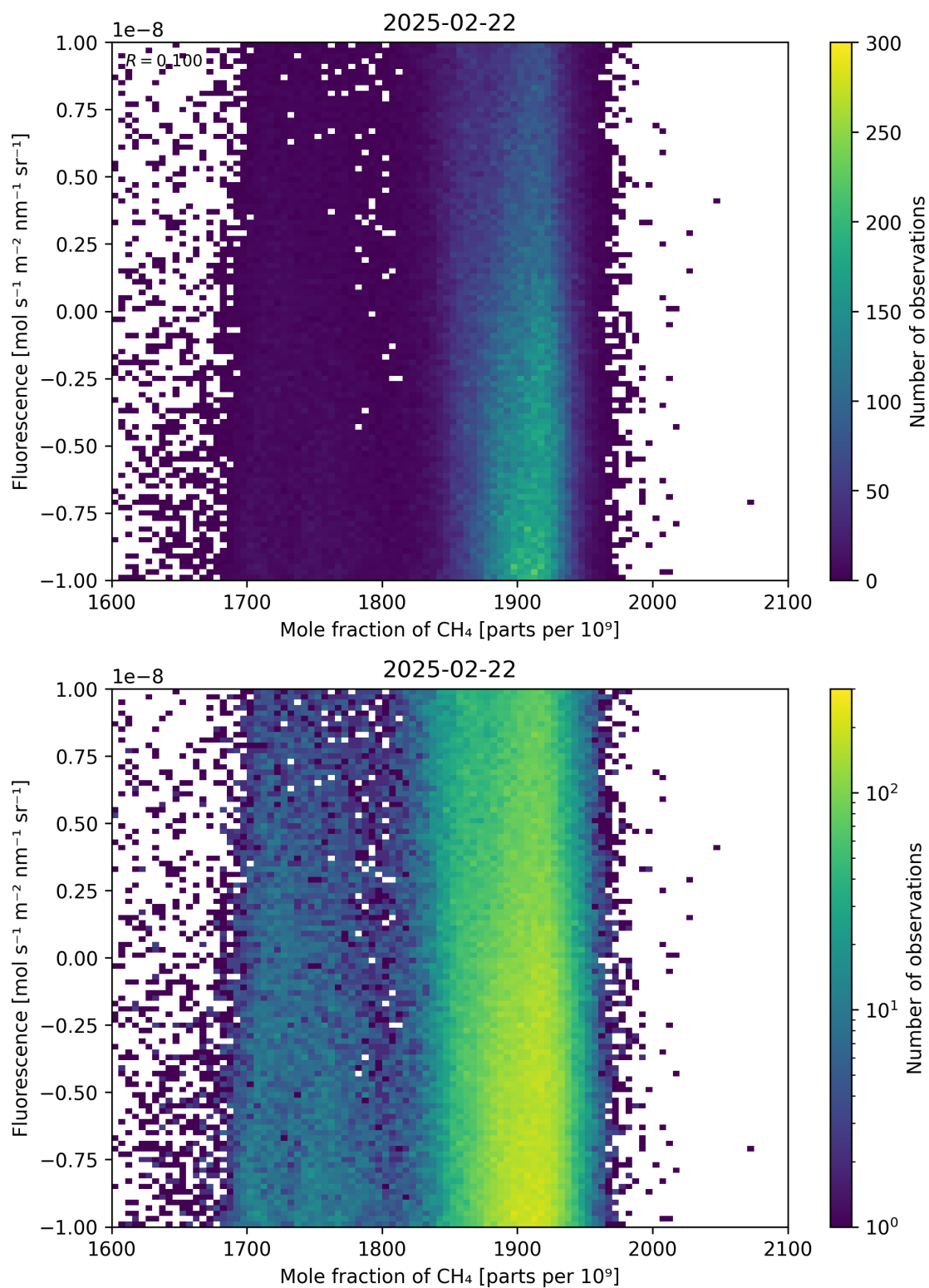
Figure 73: Scatter density plot of “Mole fraction of \text{CH}_4 ” against “Fluorescence” for 2025-02-21 to 2025-02-23.
