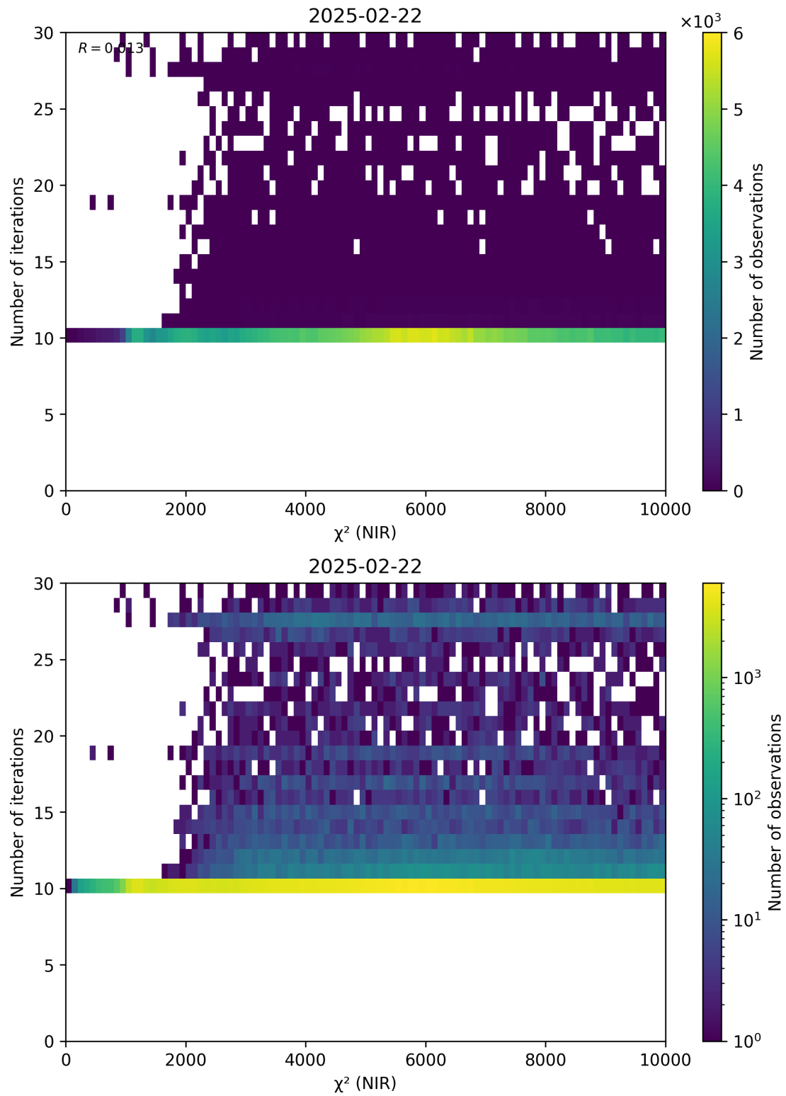
Figure 46: Scatter density plot of “ \chi^2 (NIR)” against “Number of iterations” for 2025-02-21 to 2025-02-23.
