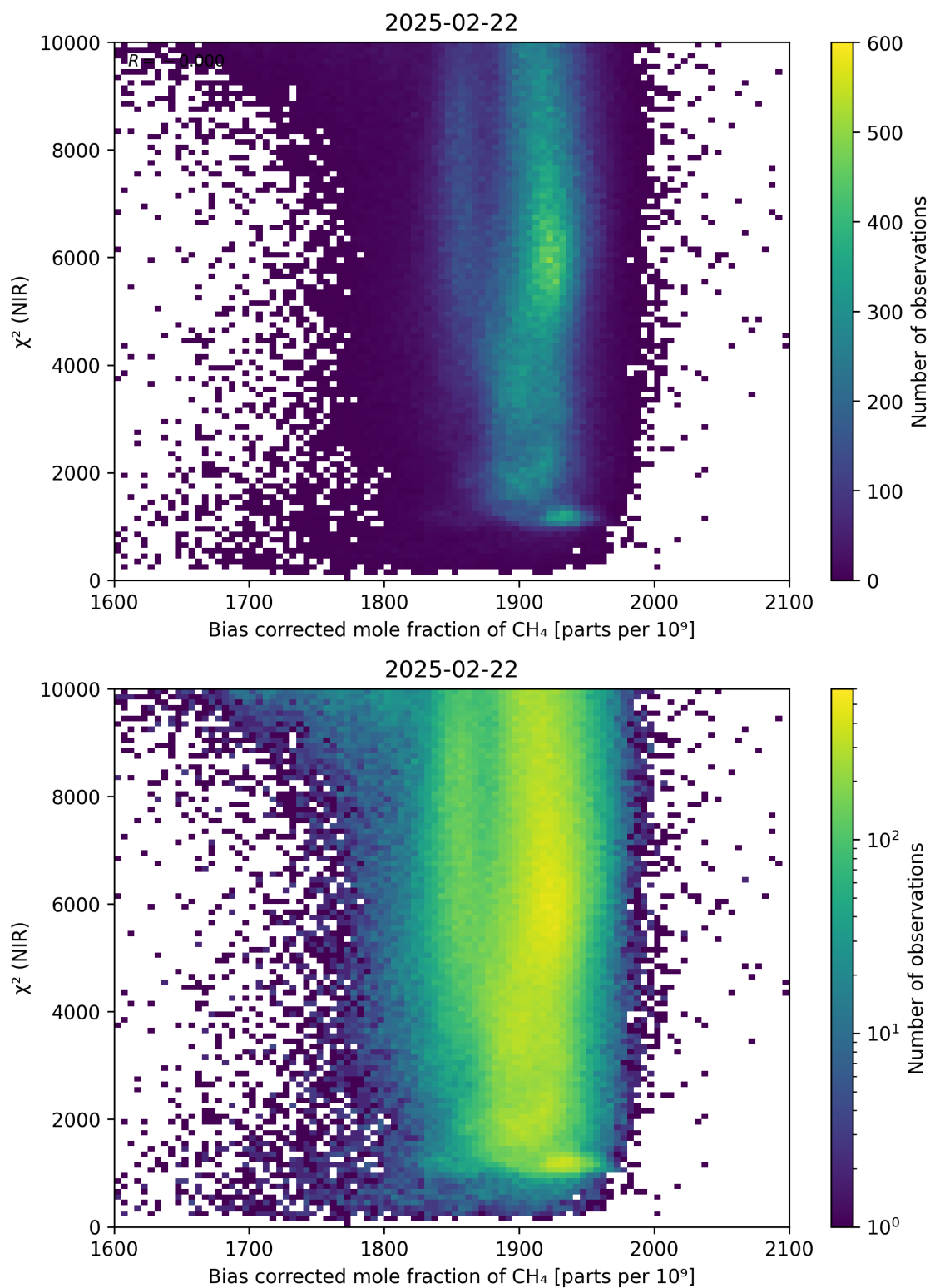
Figure 63: Scatter density plot of “Bias corrected mole fraction of \text{CH}_4 ” against “ \chi^2 (NIR)” for 2025-02-21 to 2025-02-23.
