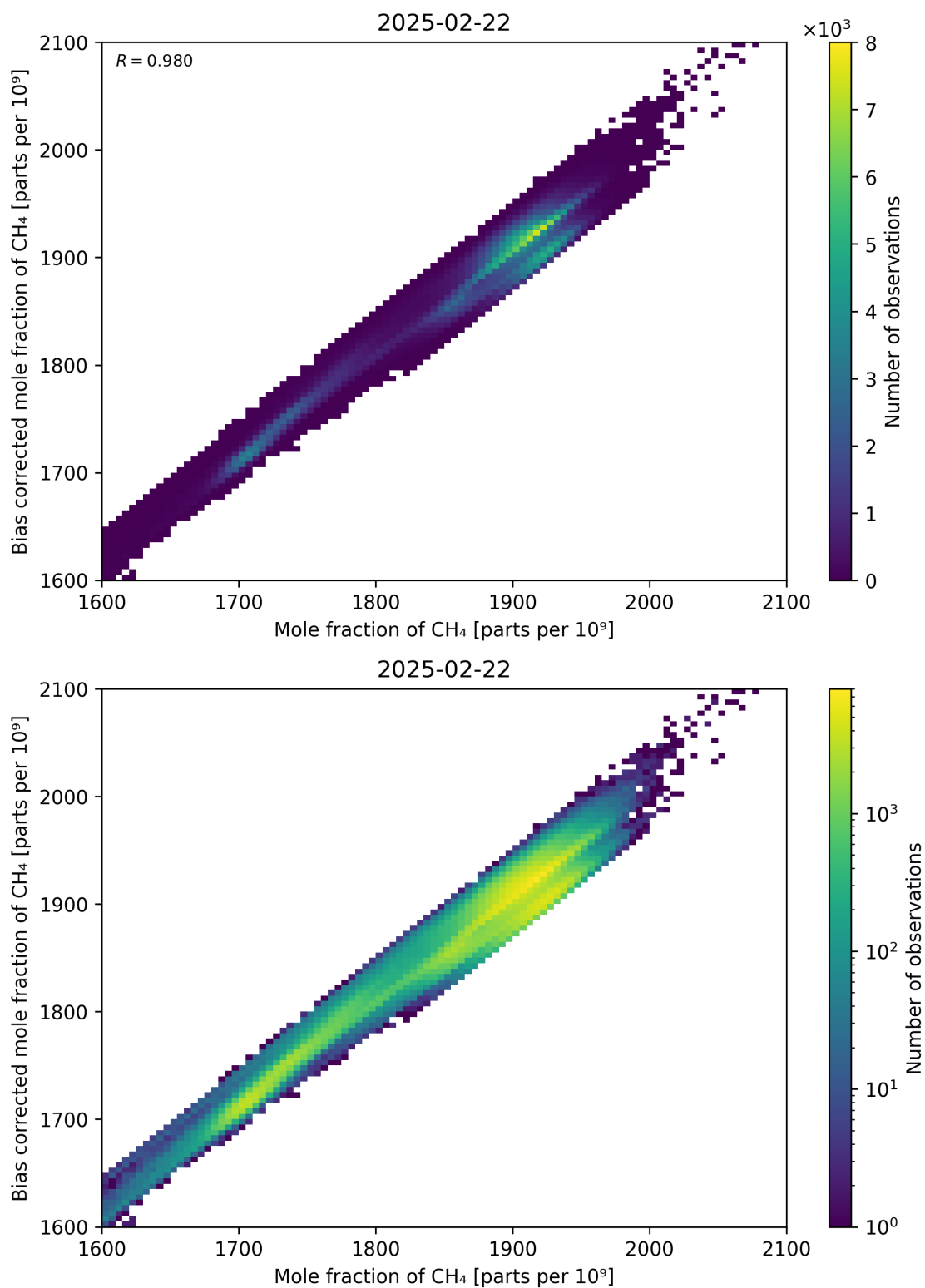
Figure 74: Scatter density plot of “Mole fraction of CH 4 ” against “Bias corrected mole fraction of CH 4 ” for 2025-02-21 to 2025-02-23.
