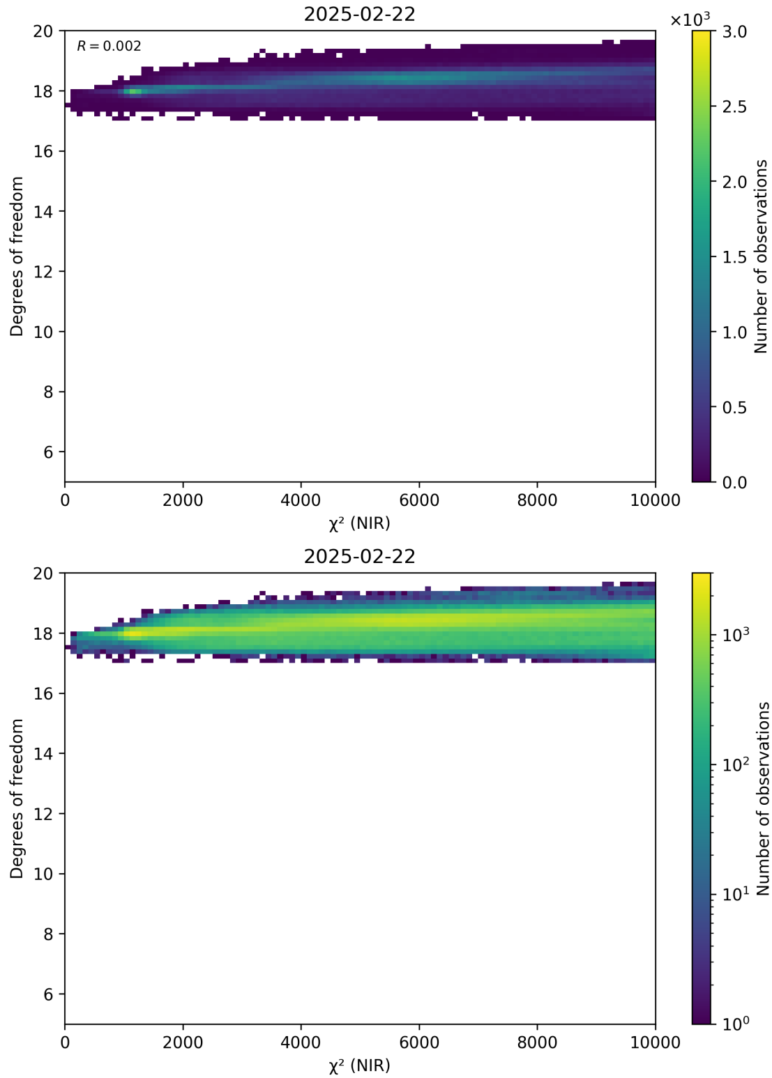
Figure 44: Scatter density plot of “ \chi^2 (NIR)” against “Degrees of freedom” for 2025-02-21 to 2025-02-23.
