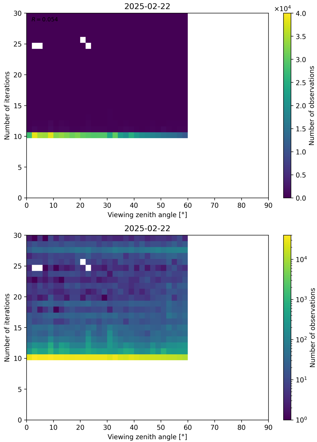
Figure 113: Scatter density plot of “Viewing zenith angle” against “Number of iterations” for 2025-02-21 to 2025-02-23.
