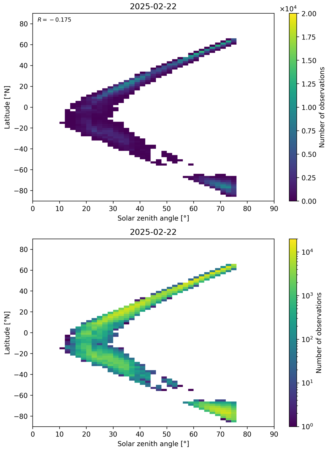
Figure 98: Scatter density plot of “Solar zenith angle” against “Latitude” for 2025-02-21 to 2025-02-23.
