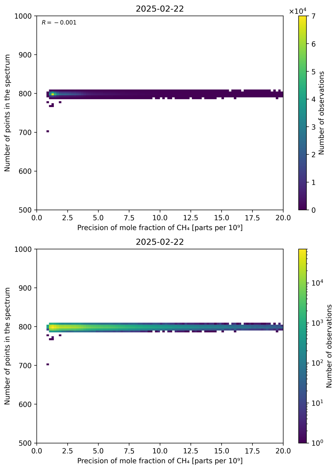
Figure 84: Scatter density plot of “Precision of mole fraction of CH 4 ” against “Number of points in the spectrum” for 2025-02-21 to 2025-02-23.
