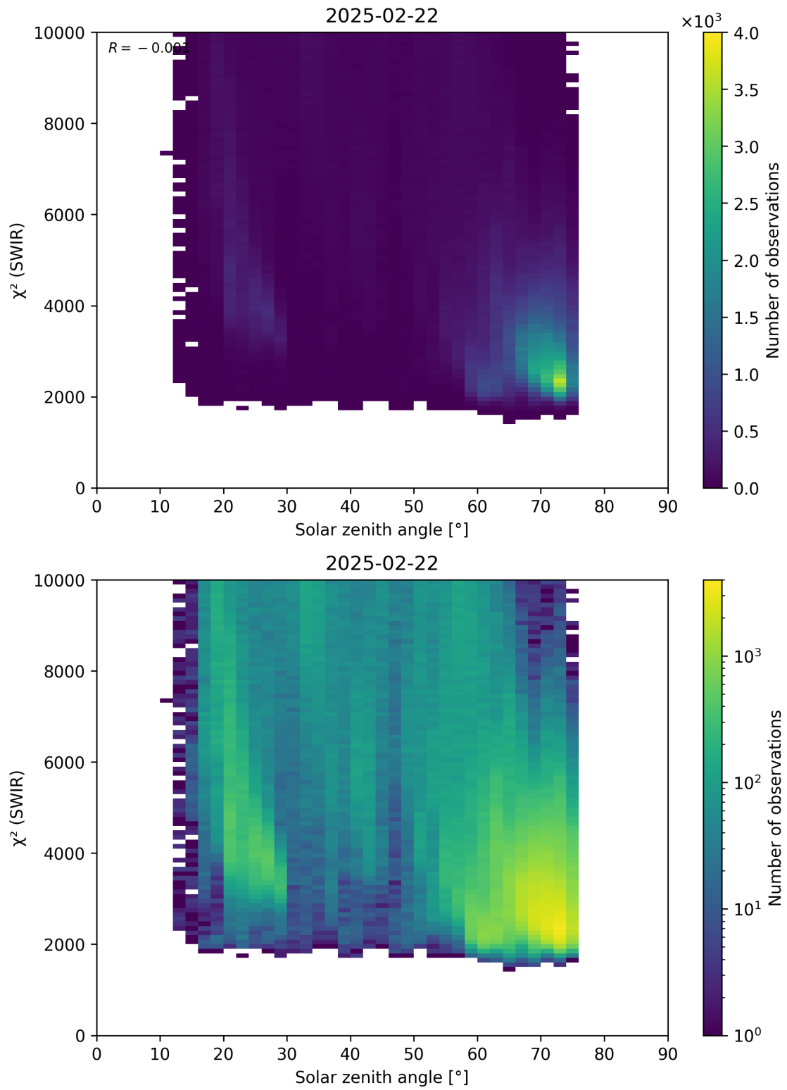
Figure 95: Scatter density plot of “Solar zenith angle” against “ \chi^2 (SWIR)” for 2025-02-21 to 2025-02-23.
