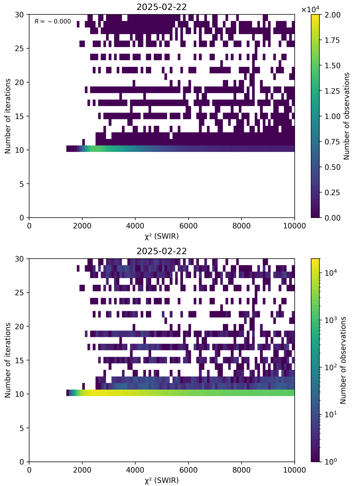
Figure 50: Scatter density plot of “ \chi^2 (SWIR)” against “Number of iterations” for 2025-02-21 to 2025-02-23.
