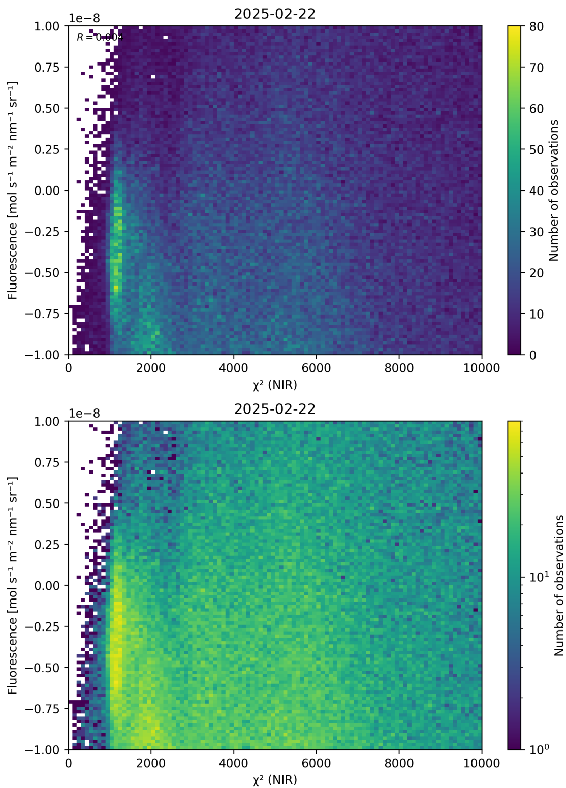
Figure 45: Scatter density plot of “ \chi^2 (NIR)” against “Fluorescence” for 2025-02-21 to 2025-02-23.
