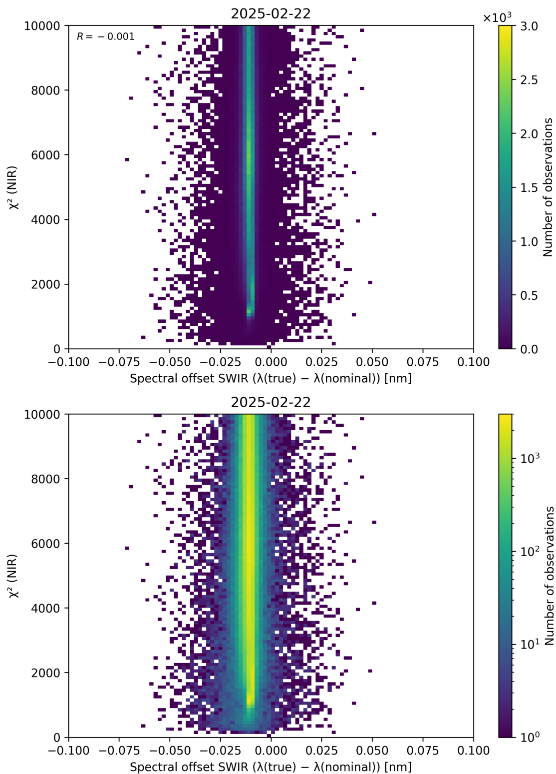
Figure 117: Scatter density plot of “Spectral offset SWIR ( \lambda_{\text{true}} - \lambda_{\text{nominal}} )” against “ \chi^2 (NIR)” for 2025-02-21 to 2025-02-23.
