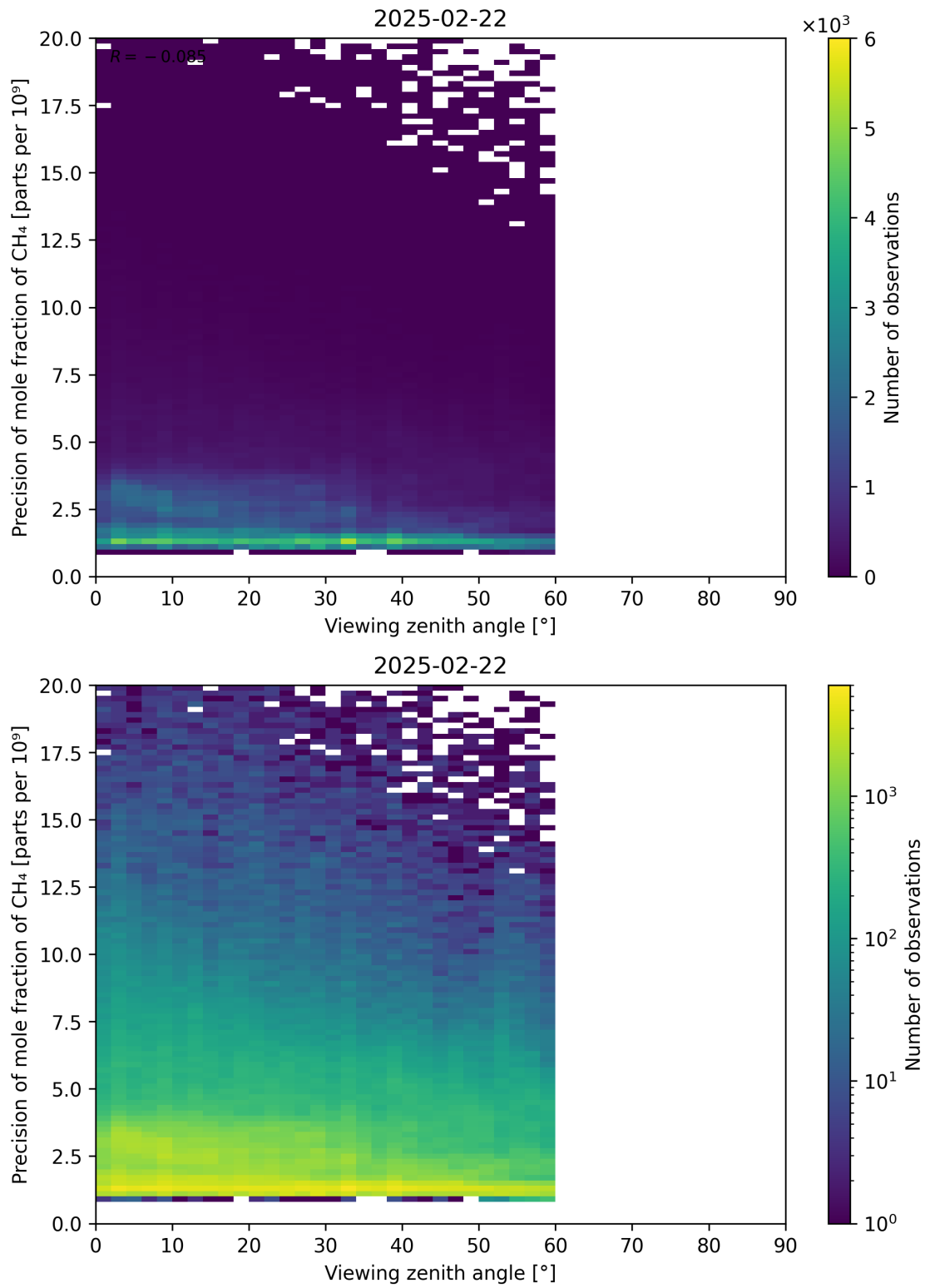
Figure 112: Scatter density plot of “Viewing zenith angle” against “Precision of mole fraction of CH 4 ” for 2025-02-21 to 2025-02-23.
