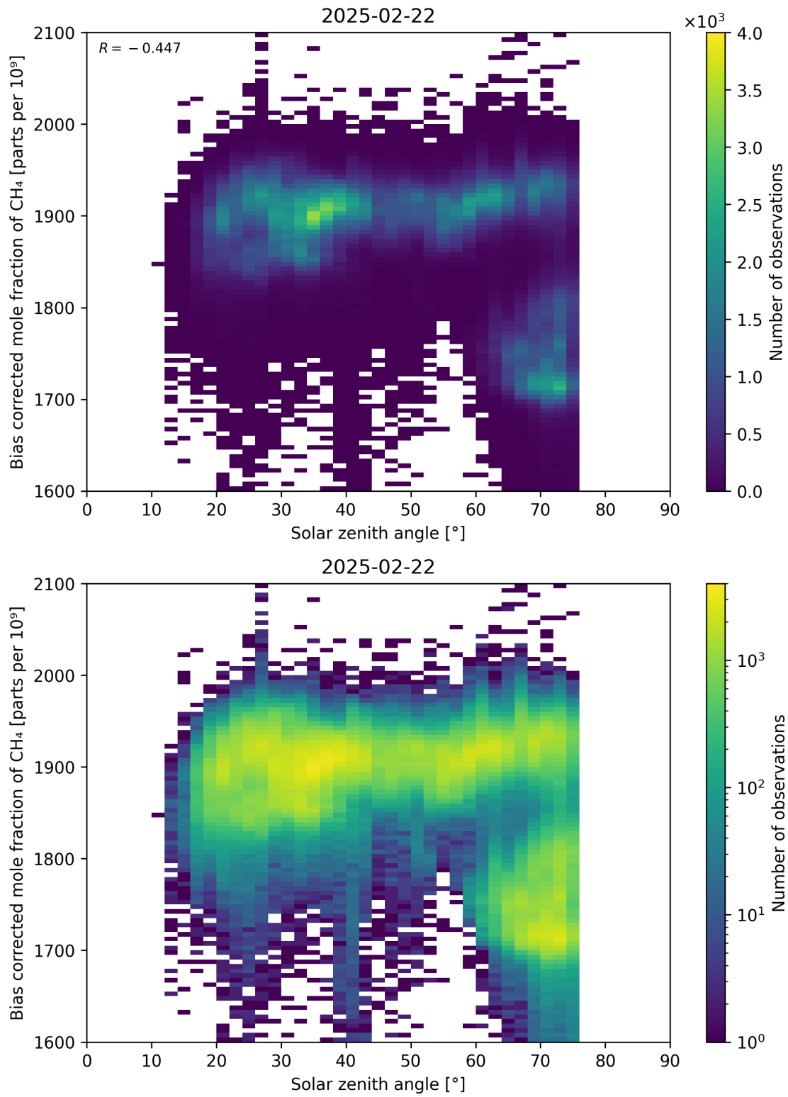
Figure 100: Scatter density plot of “Solar zenith angle” against “Bias corrected mole fraction of CH 4 ” for 2025-02-21 to 2025-02-23.
