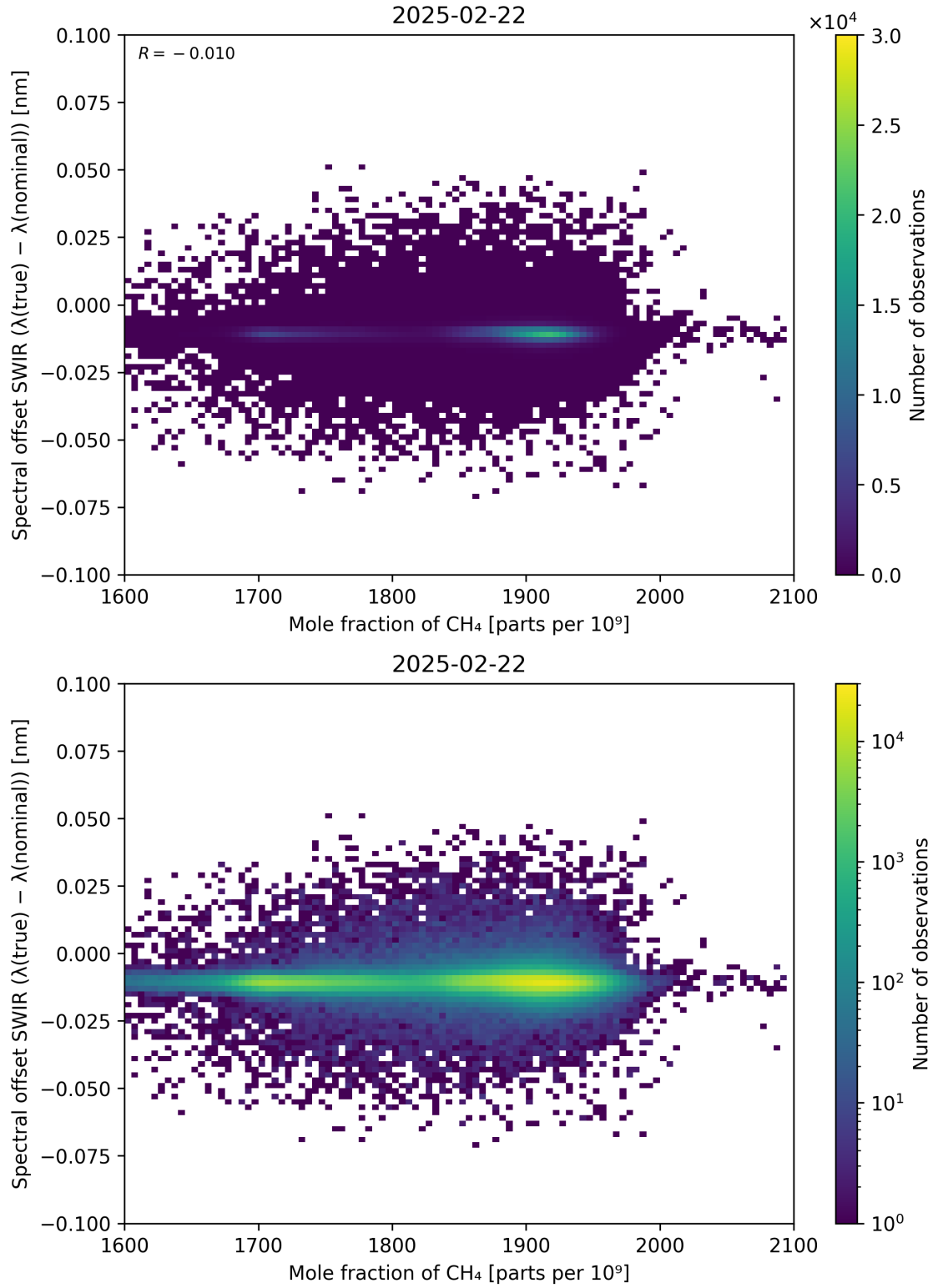
Figure 86: Scatter density plot of “Mole fraction of CH 4 ” against “Spectral offset SWIR ( \lambda_{\text{true}} - \lambda_{\text{nominal}} )” for 2025-02-21 to 2025-02-23.
