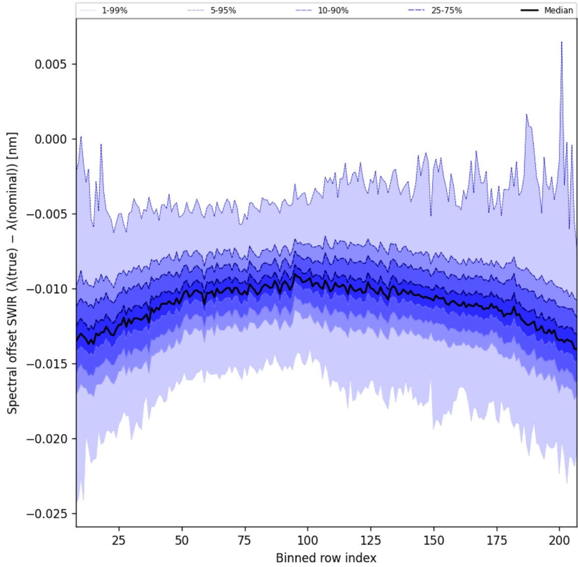
Figure 38: Along track statistics of “Spectral offset SWIR ( \lambda_{\text{true}} - \lambda_{\text{nominal}} )” for 2025-02-21 to 2025-02-23
