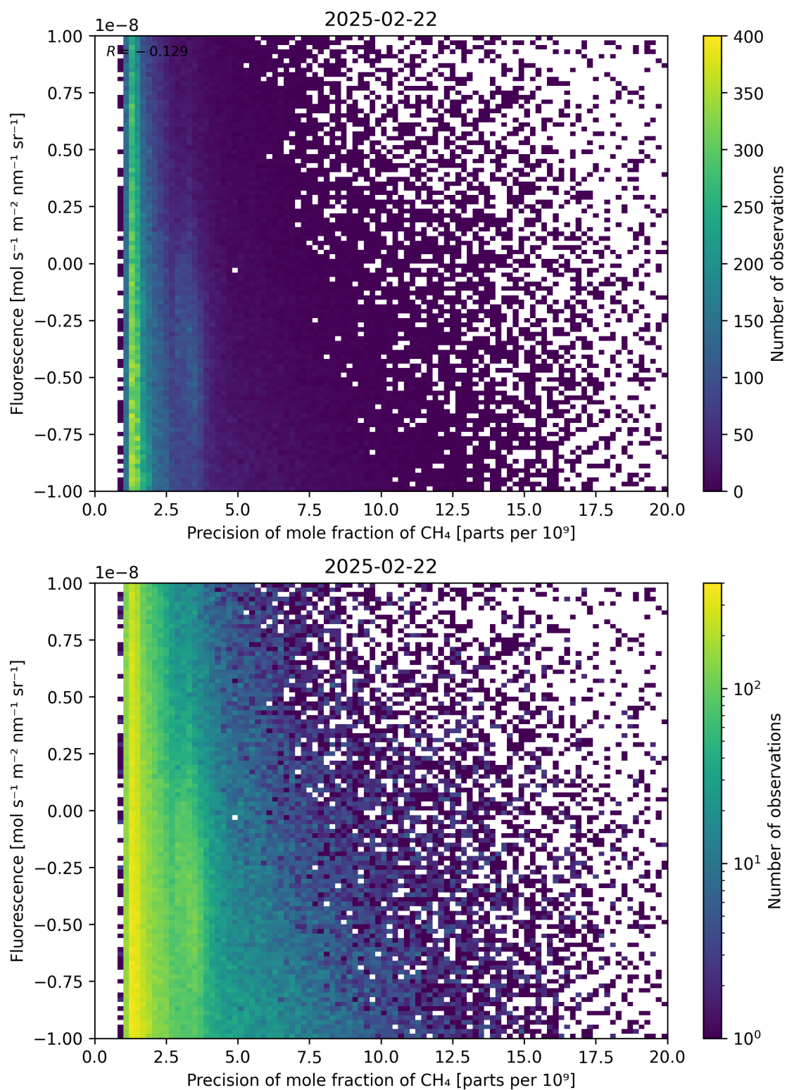
Figure 81: Scatter density plot of “Precision of mole fraction of \text{CH}_4 ” against “Fluorescence” for 2025-02-21 to 2025-02-23.
