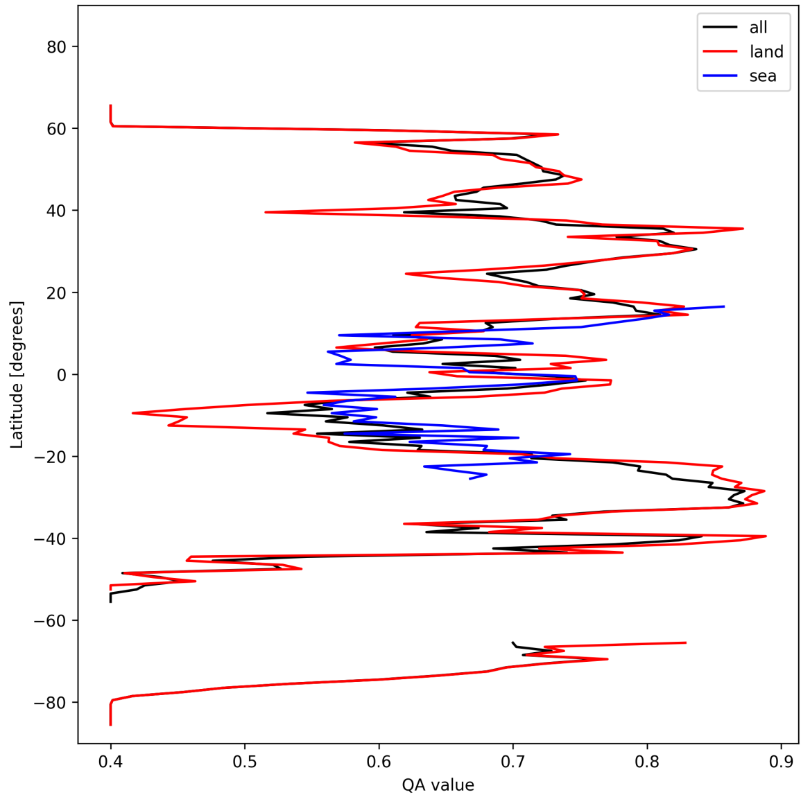
Figure 11: Zonal average of “QA value” for 2025-02-21 to 2025-02-23.
