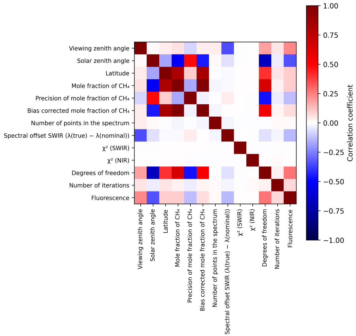
Figure 2: Map of correlation matrix for 2025-02-21 to 2025-02-23.
