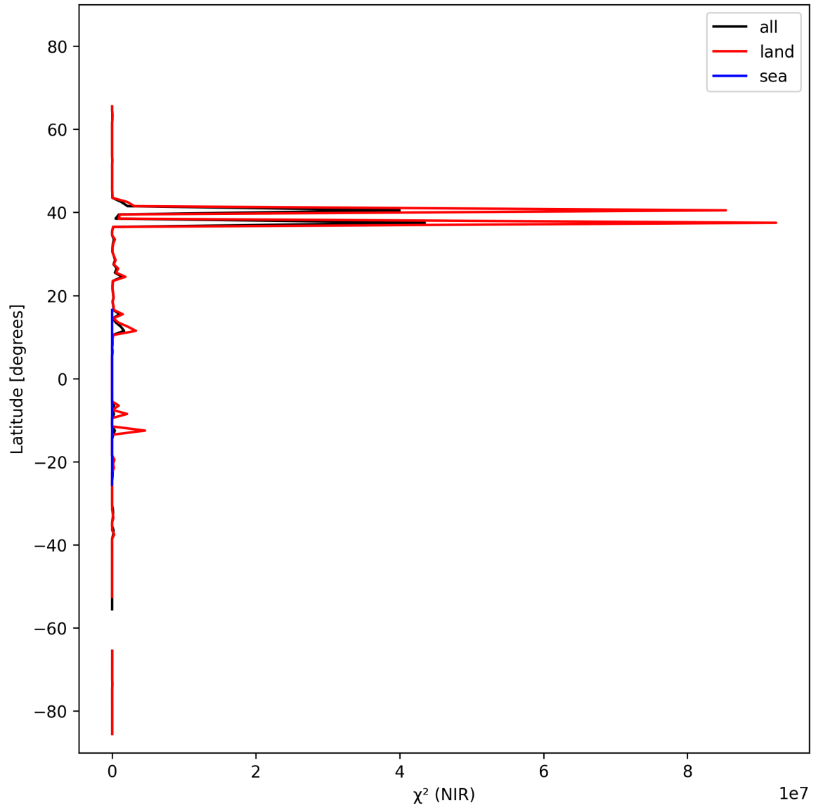
Figure 18: Zonal average of “ \chi^2 (NIR)” for 2025-02-21 to 2025-02-23.
