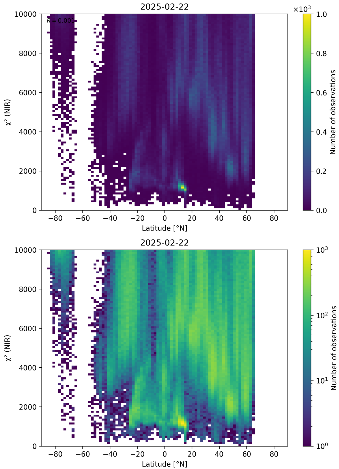
Figure 53: Scatter density plot of “Latitude” against “ \chi^2 (NIR)” for 2025-02-21 to 2025-02-23.
