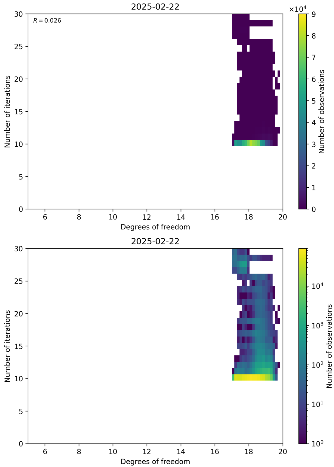
Figure 52: Scatter density plot of “Degrees of freedom” against “Number of iterations” for 2025-02-21 to 2025-02-23.
