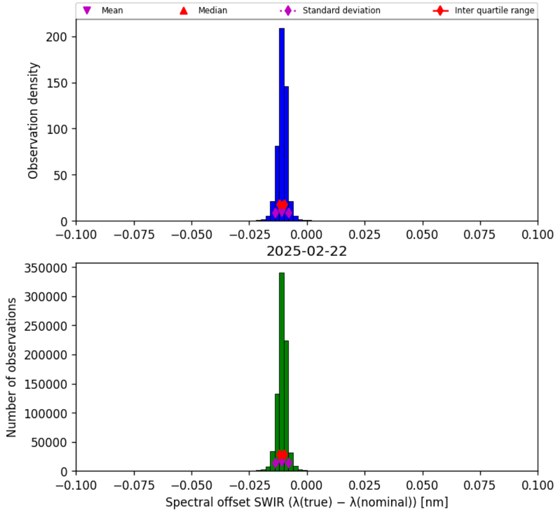
Figure 27: Histogram of “Spectral offset SWIR ( \lambda_{\text{true}} - \lambda_{\text{nominal}} )” for 2025-02-21 to 2025-02-23
