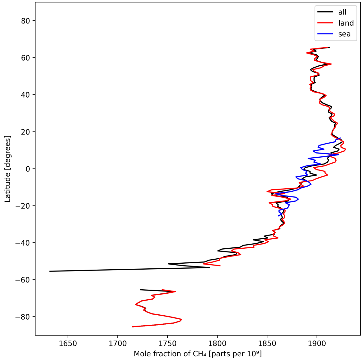
Figure 12: Zonal average of “Mole fraction of \text{CH}_4 ” for 2025-02-21 to 2025-02-23.
