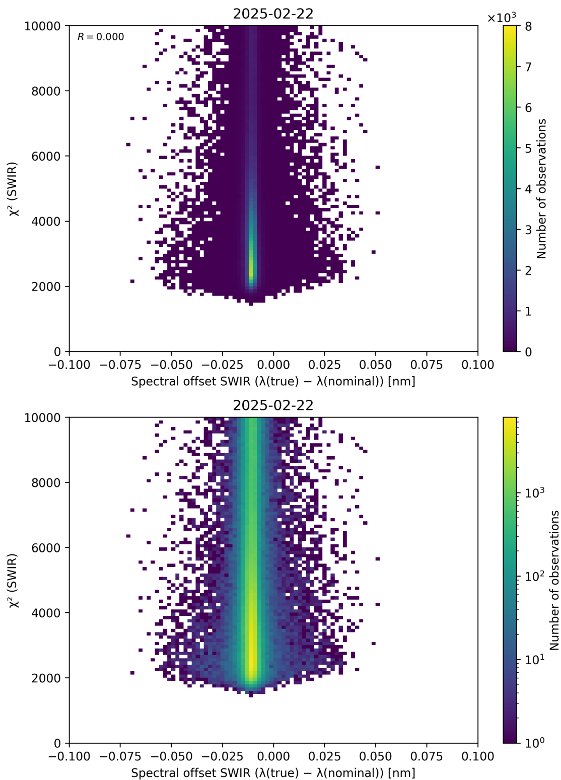
Figure 118: Scatter density plot of “Spectral offset SWIR ( \lambda_{\text{true}} - \lambda_{\text{nominal}} )” against “ \chi^2 (SWIR)” for 2025-02-21 to 2025-02-23.
