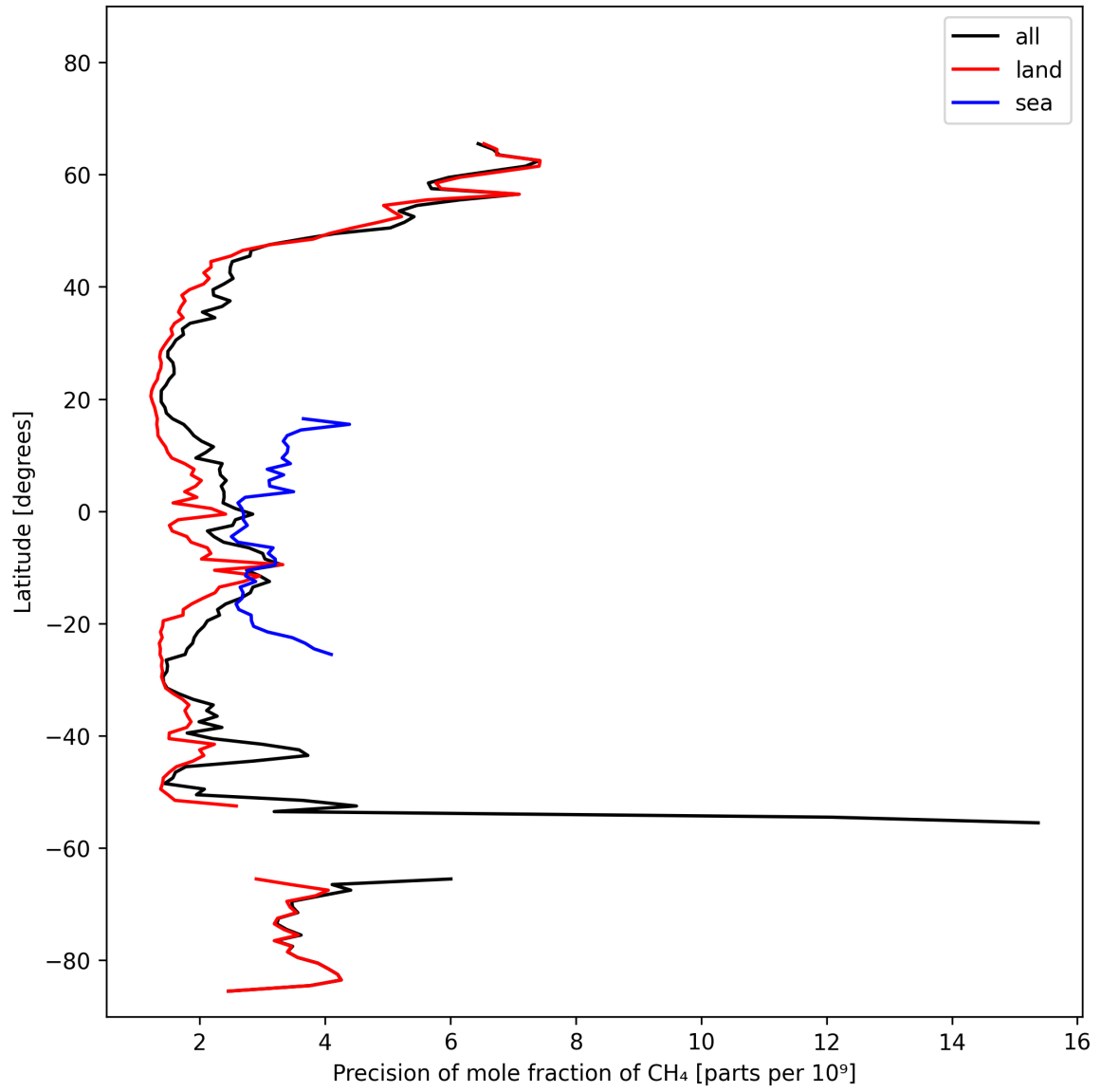
Figure 13: Zonal average of “Precision of mole fraction of CH 4 ” for 2025-02-21 to 2025-02-23.
