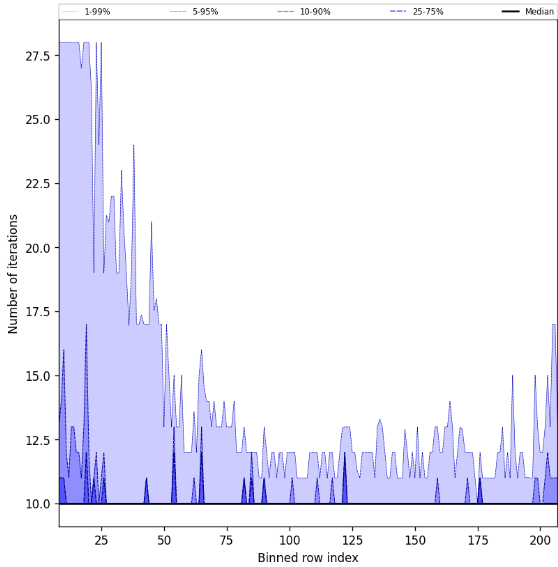
Figure 42: Along track statistics of “Number of iterations” for 2025-02-21 to 2025-02-23
