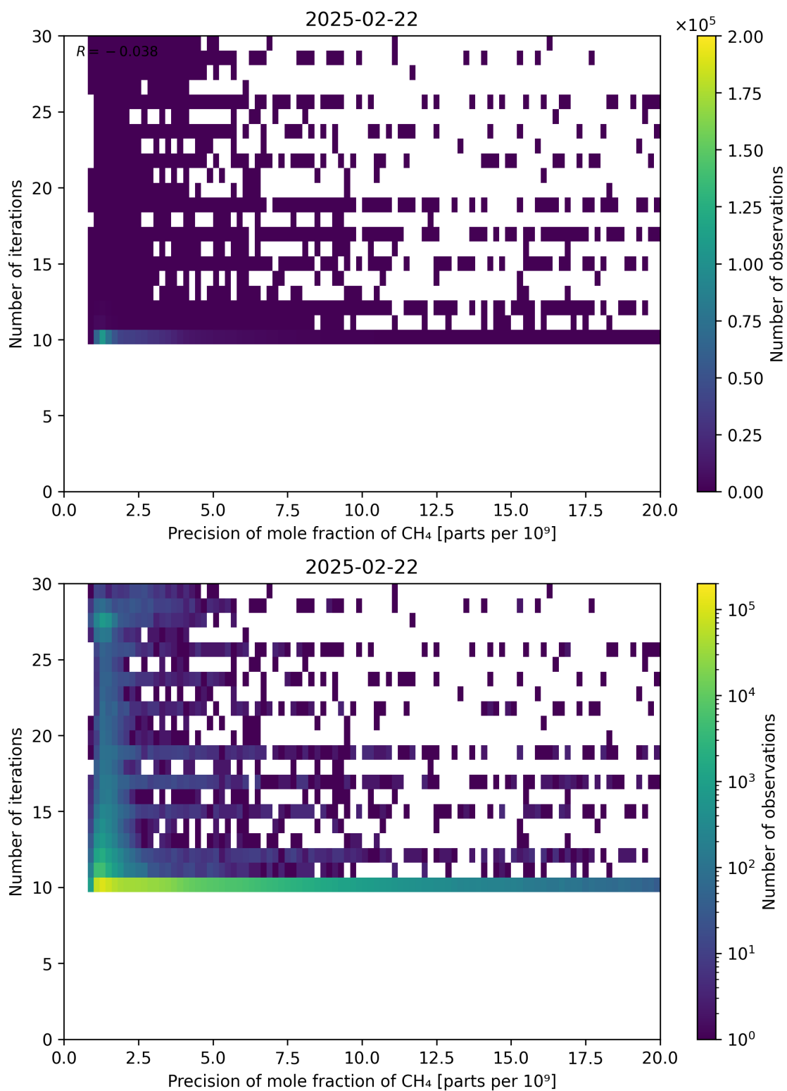
Figure 83: Scatter density plot of “Precision of mole fraction of CH 4 ” against “Number of iterations” for 2025-02-21 to 2025-02-23.
