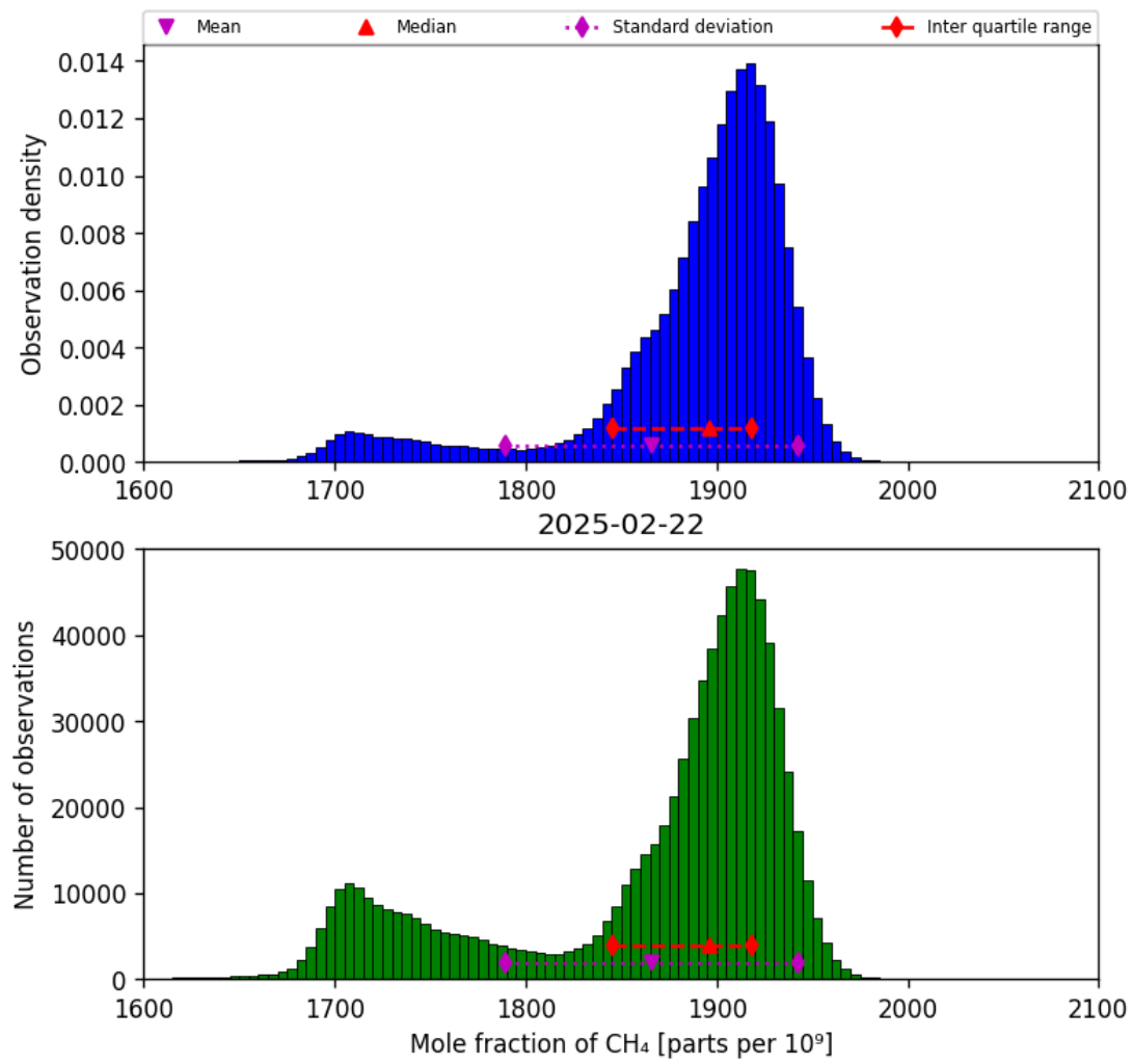
Figure 23: Histogram of “Mole fraction of CH 4 ” for 2025-02-21 to 2025-02-23
