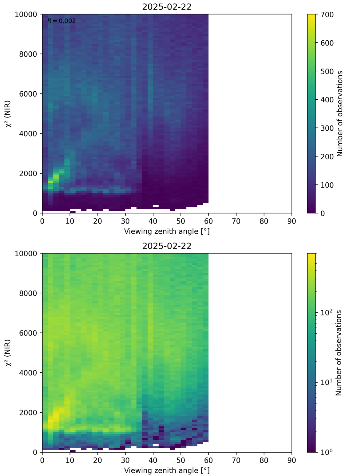
Figure 105: Scatter density plot of “Viewing zenith angle” against “ \chi^2 (NIR)” for 2025-02-21 to 2025-02-23.
