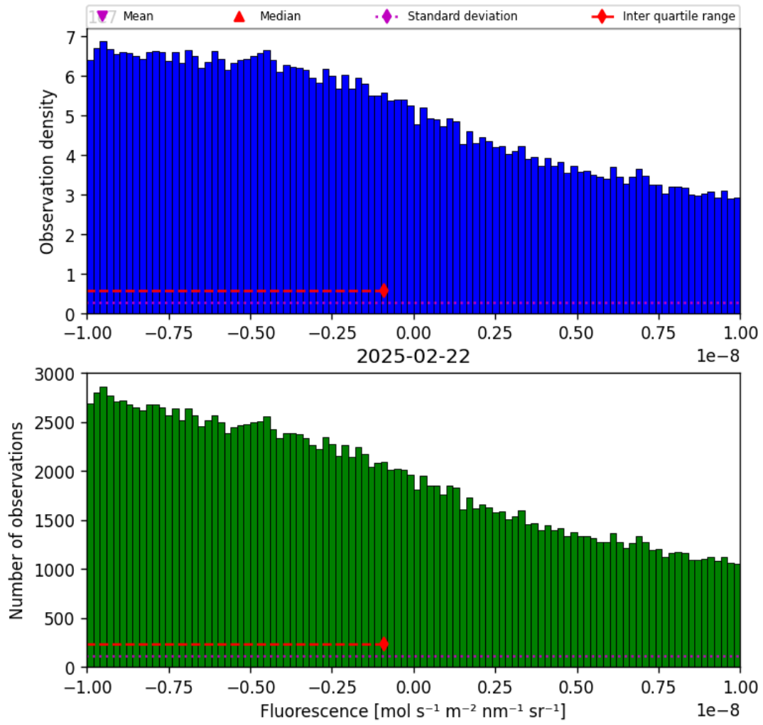
Figure 32: Histogram of “Fluorescence” for 2025-02-21 to 2025-02-23
