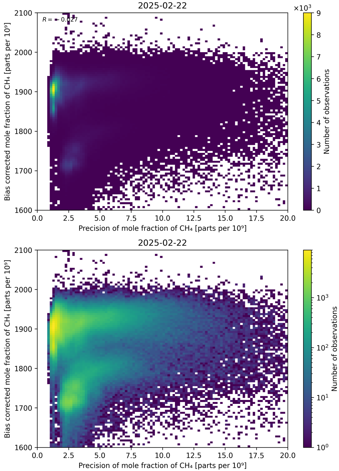
Figure 82: Scatter density plot of “Precision of mole fraction of CH 4 ” against “Bias corrected mole fraction of CH 4 ” for 2025-02-21 to 2025-02-23.
