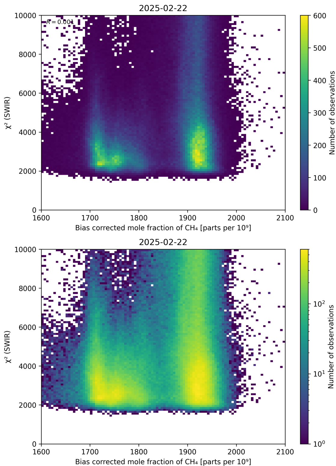
Figure 64: Scatter density plot of “Bias corrected mole fraction of \text{CH}_4 ” against “ \chi^2 (SWIR)” for 2025-02-21 to 2025-02-23.
