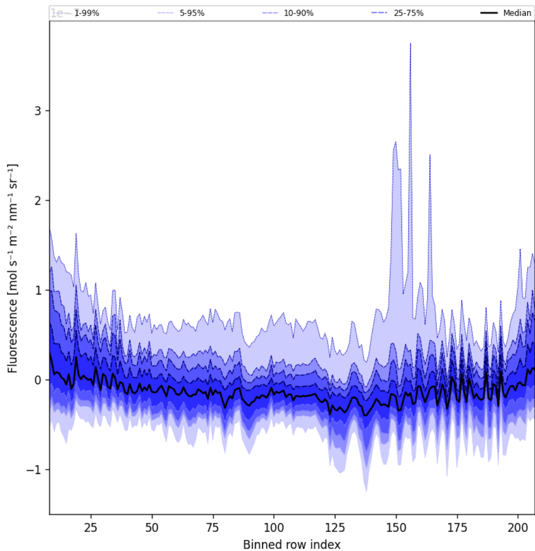
Figure 43: Along track statistics of “Fluorescence” for 2025-02-21 to 2025-02-23
