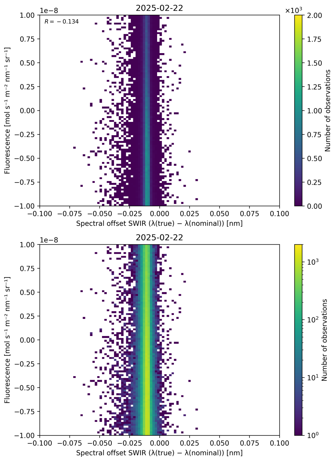
Figure 120: Scatter density plot of “Spectral offset SWIR ( \lambda_{\text{true}} - \lambda_{\text{nominal}} )” against “Fluorescence” for 2025-02-21 to 2025-02-23.
