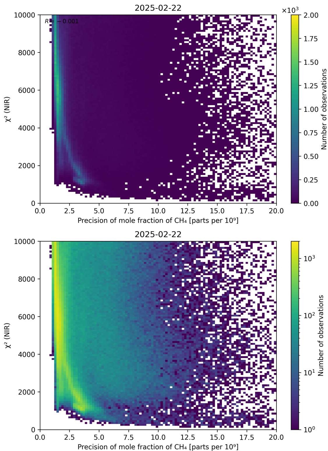
Figure 78: Scatter density plot of “Precision of mole fraction of \text{CH}_4 ” against “ \chi^2 (NIR)” for 2025-02-21 to 2025-02-23.
