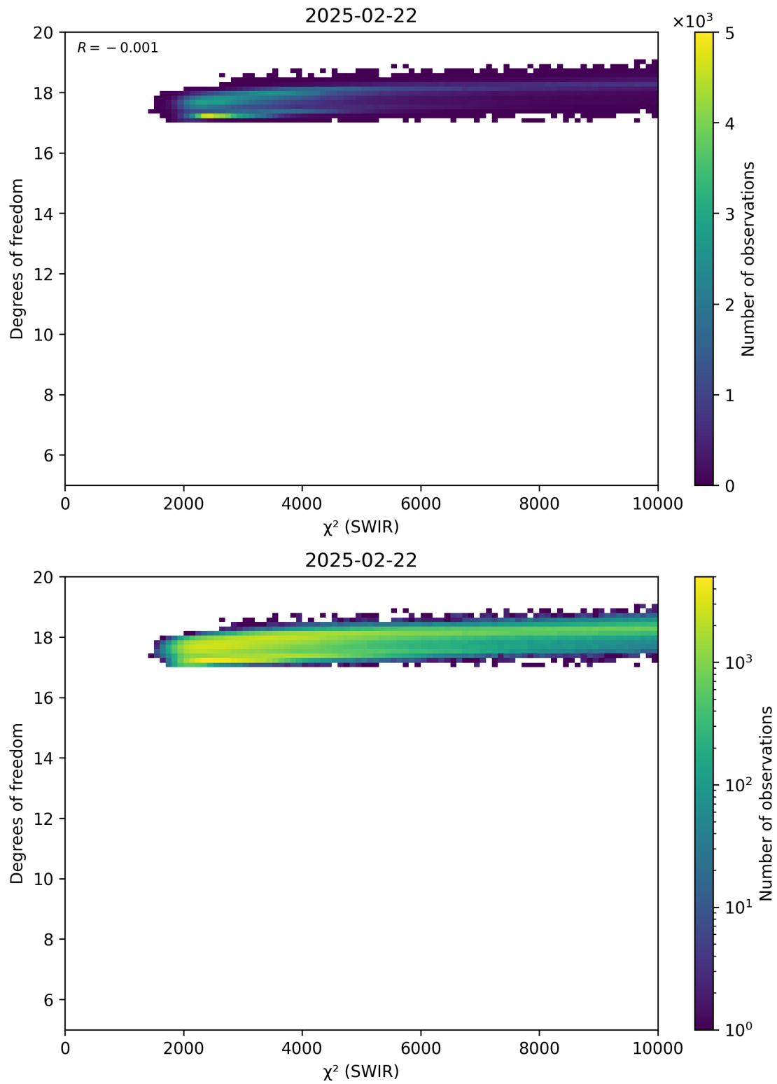
Figure 48: Scatter density plot of “ \chi^2 (SWIR)” against “Degrees of freedom” for 2025-02-21 to 2025-02-23.
