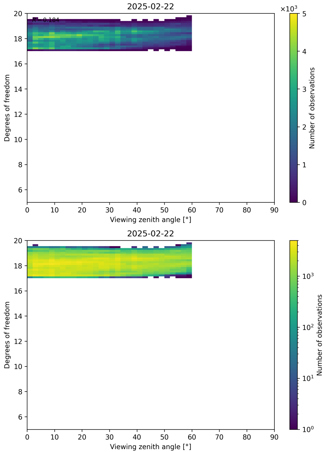
Figure 107: Scatter density plot of “Viewing zenith angle” against “Degrees of freedom” for 2025-02-21 to 2025-02-23.
