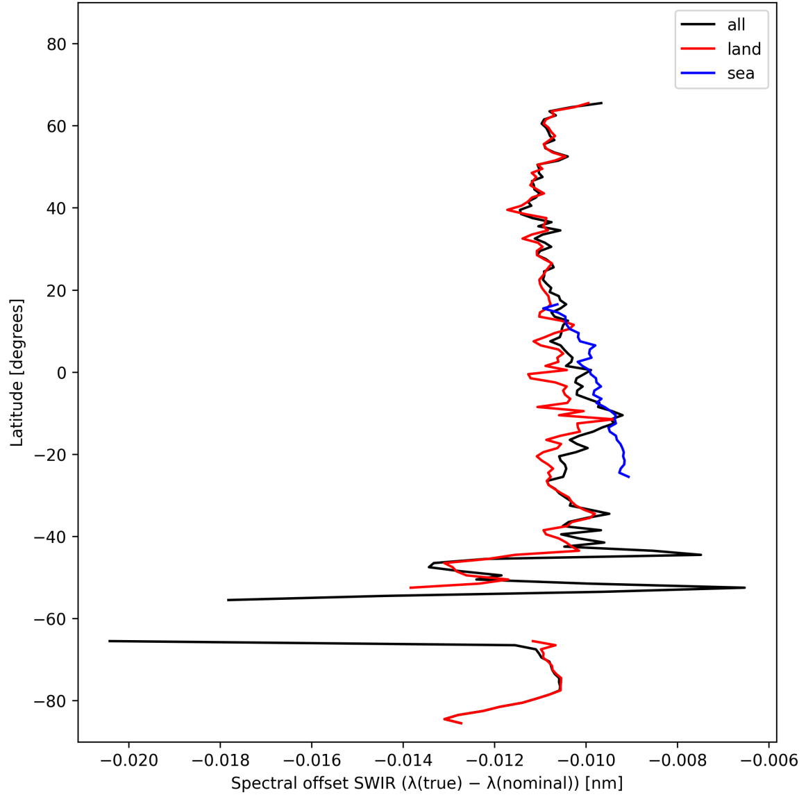
Figure 16: Zonal average of “Spectral offset SWIR ( \lambda_{\text{true}} - \lambda_{\text{nominal}} )” for 2025-02-21 to 2025-02-23.
