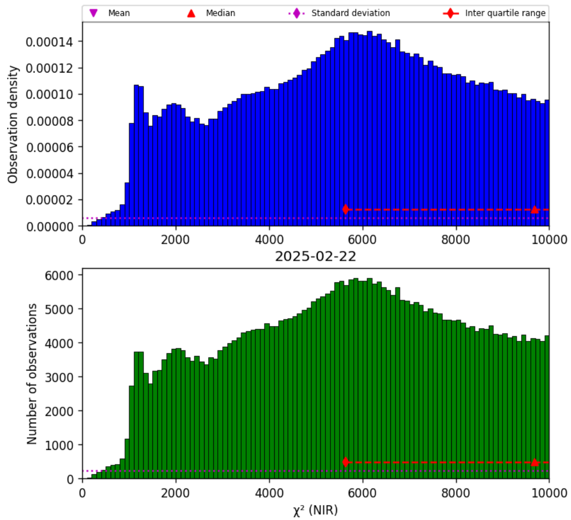
Figure 29: Histogram of " \chi^2 (NIR)" for 2025-02-21 to 2025-02-23
