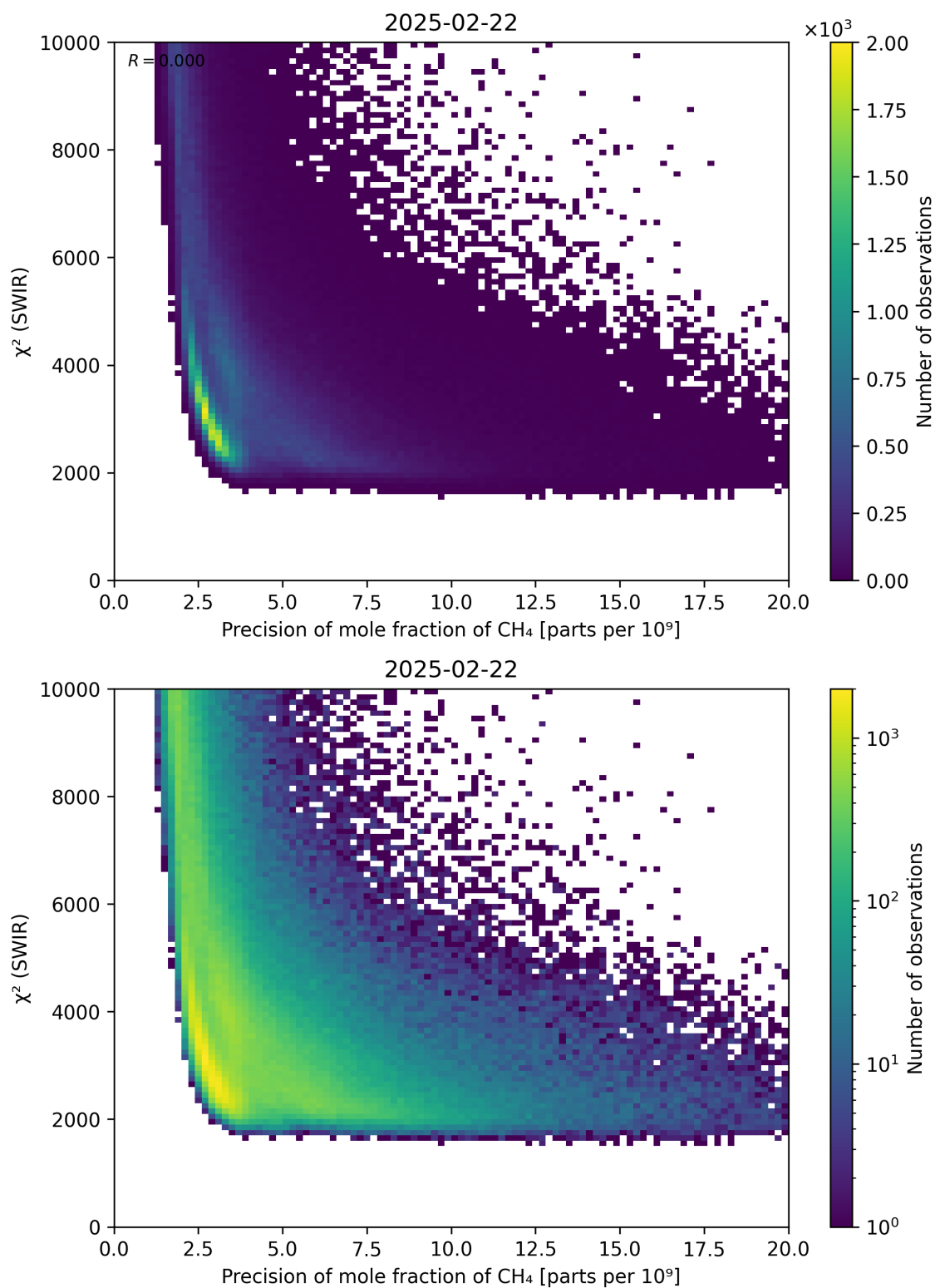
Figure 79: Scatter density plot of “Precision of mole fraction of \text{CH}_4 ” against “ \chi^2 (SWIR)” for 2025-02-21 to 2025-02-23.
