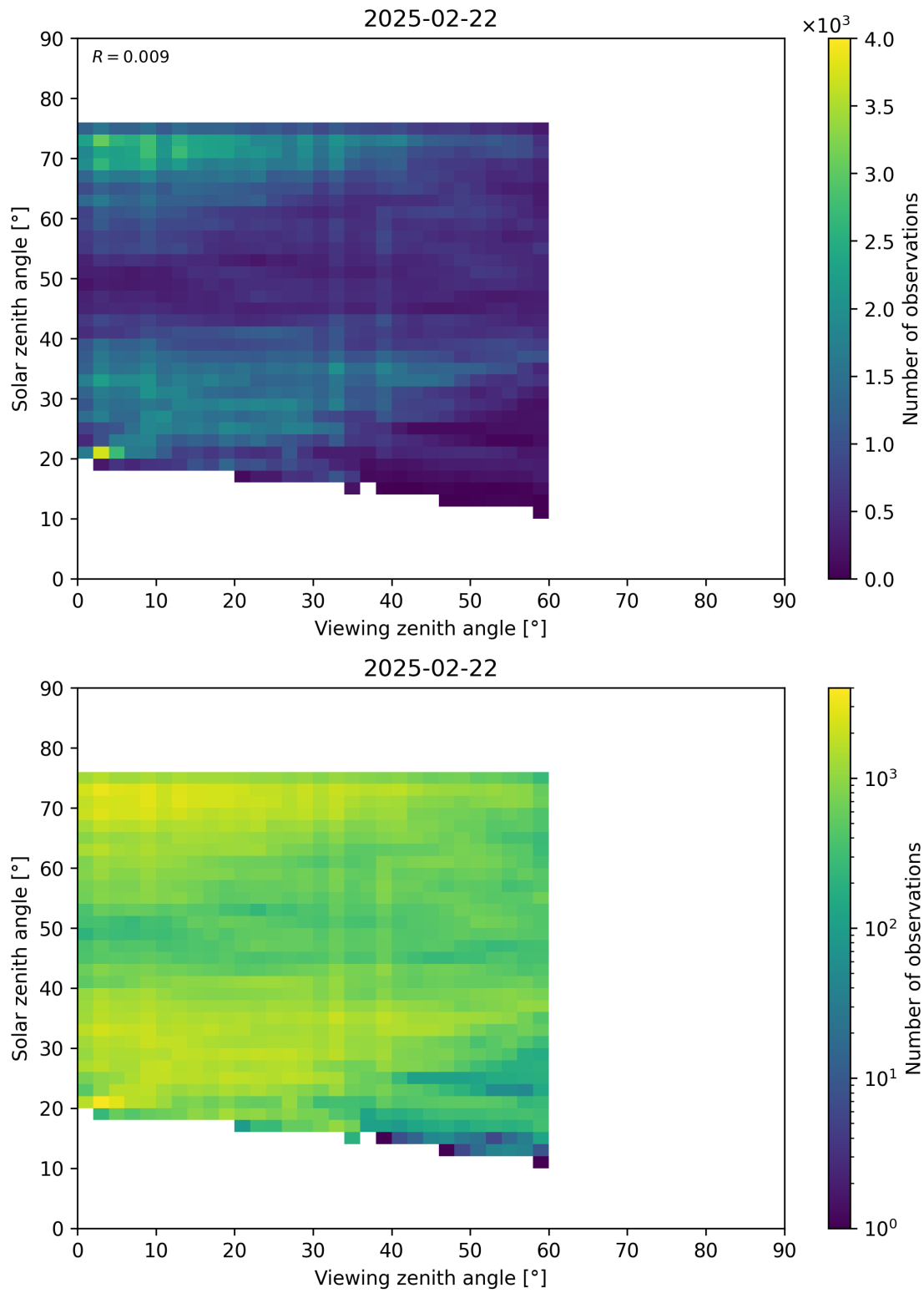
Figure 115: Scatter density plot of “Viewing zenith angle” against “Solar zenith angle” for 2025-02-21 to 2025-02-23.
