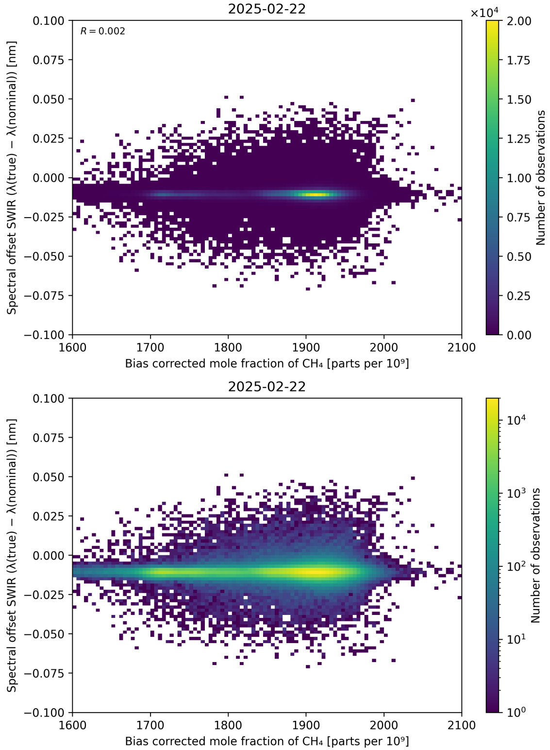
Figure 69: Scatter density plot of “Bias corrected mole fraction of \text{CH}_4 ” against “Spectral offset SWIR ( \lambda_{\text{true}} - \lambda_{\text{nominal}} )” for 2025-02-21 to 2025-02-23.
