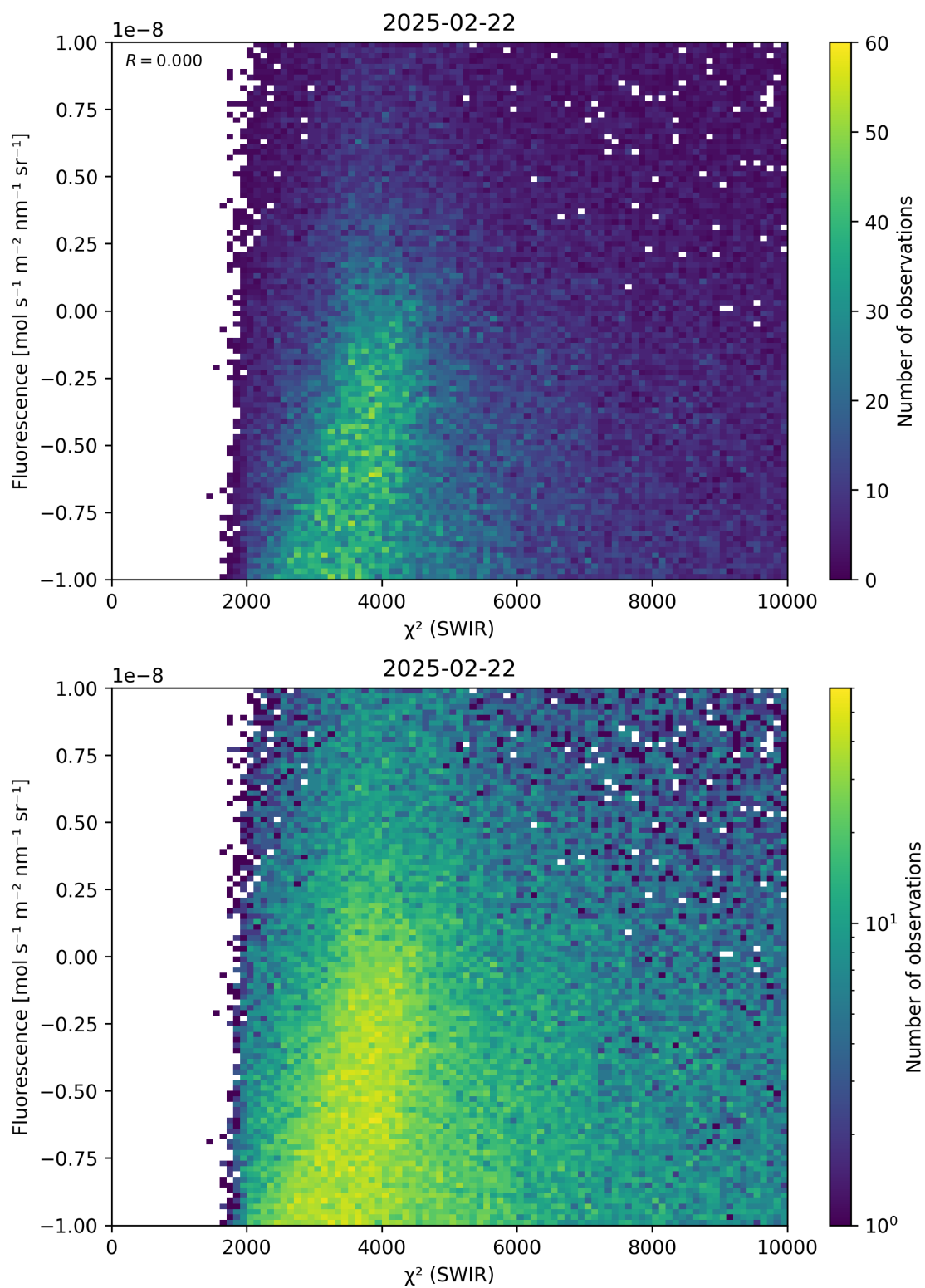
Figure 49: Scatter density plot of “ \chi^2 (SWIR)” against “Fluorescence” for 2025-02-21 to 2025-02-23.
