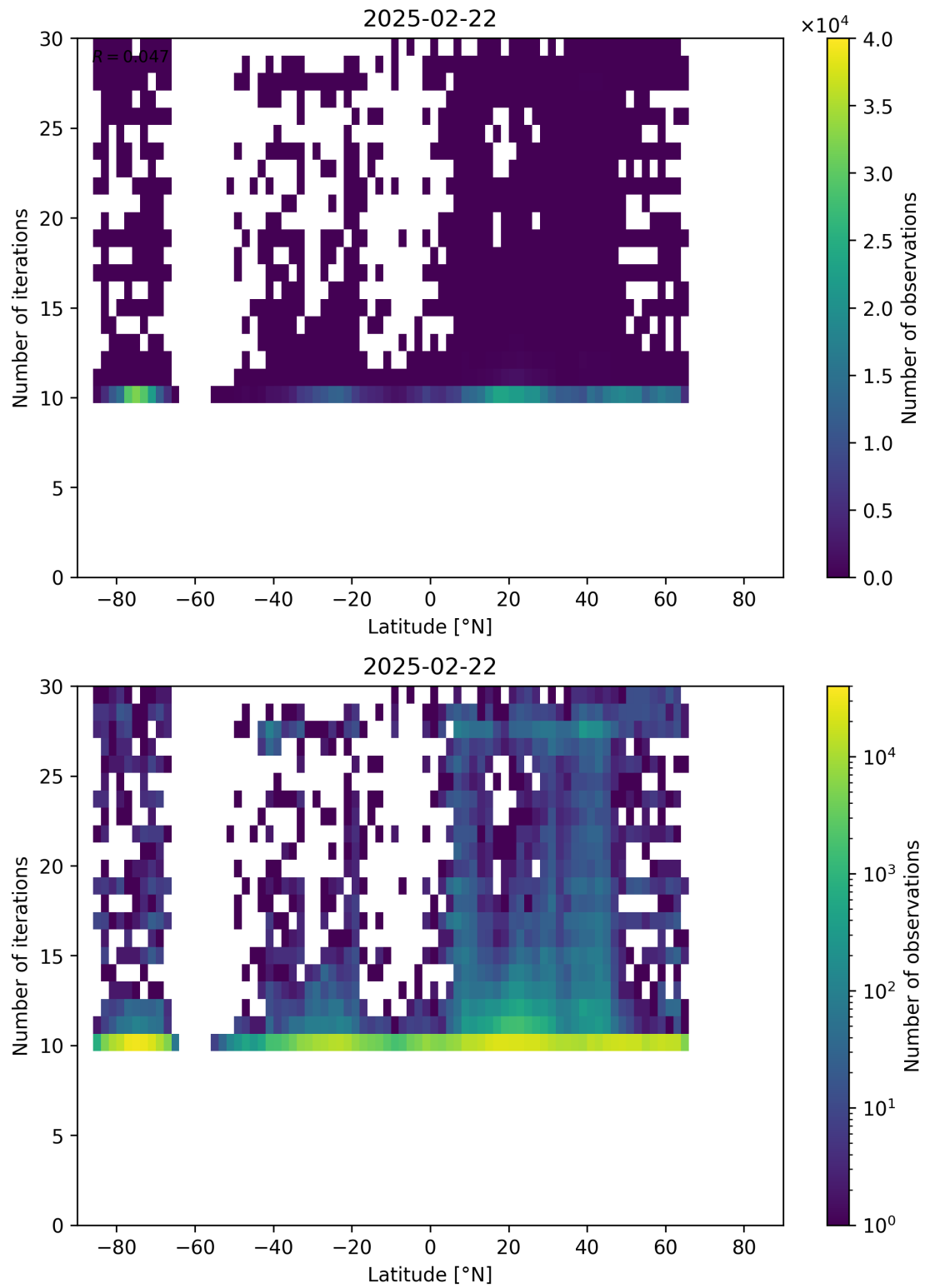
Figure 60: Scatter density plot of “Latitude” against “Number of iterations” for 2025-02-21 to 2025-02-23.
