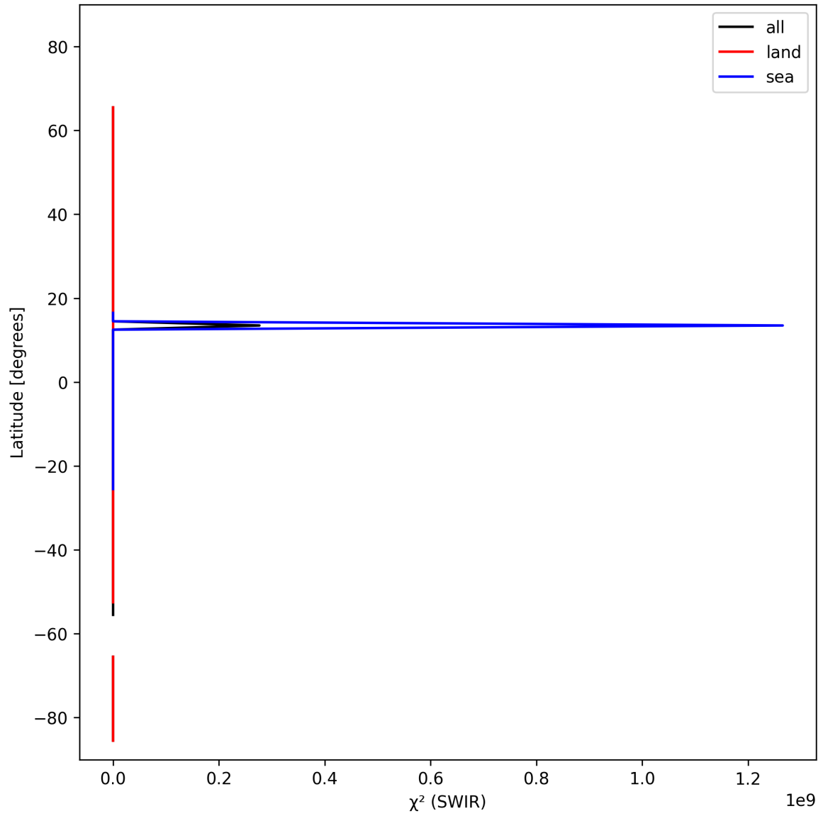
Figure 17: Zonal average of “ \chi^2 (SWIR)” for 2025-02-21 to 2025-02-23.
