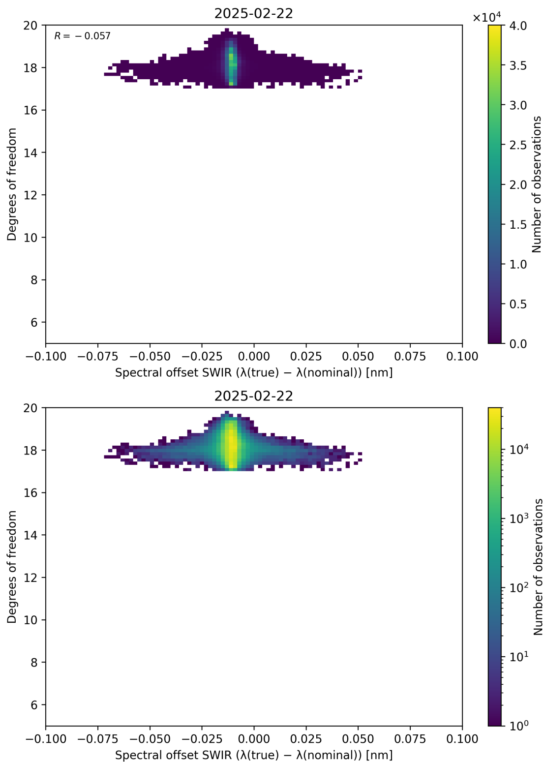
Figure 119: Scatter density plot of “Spectral offset SWIR ( \lambda_{\text{true}} - \lambda_{\text{nominal}} )” against “Degrees of freedom” for 2025-02-21 to 2025-02-23.
