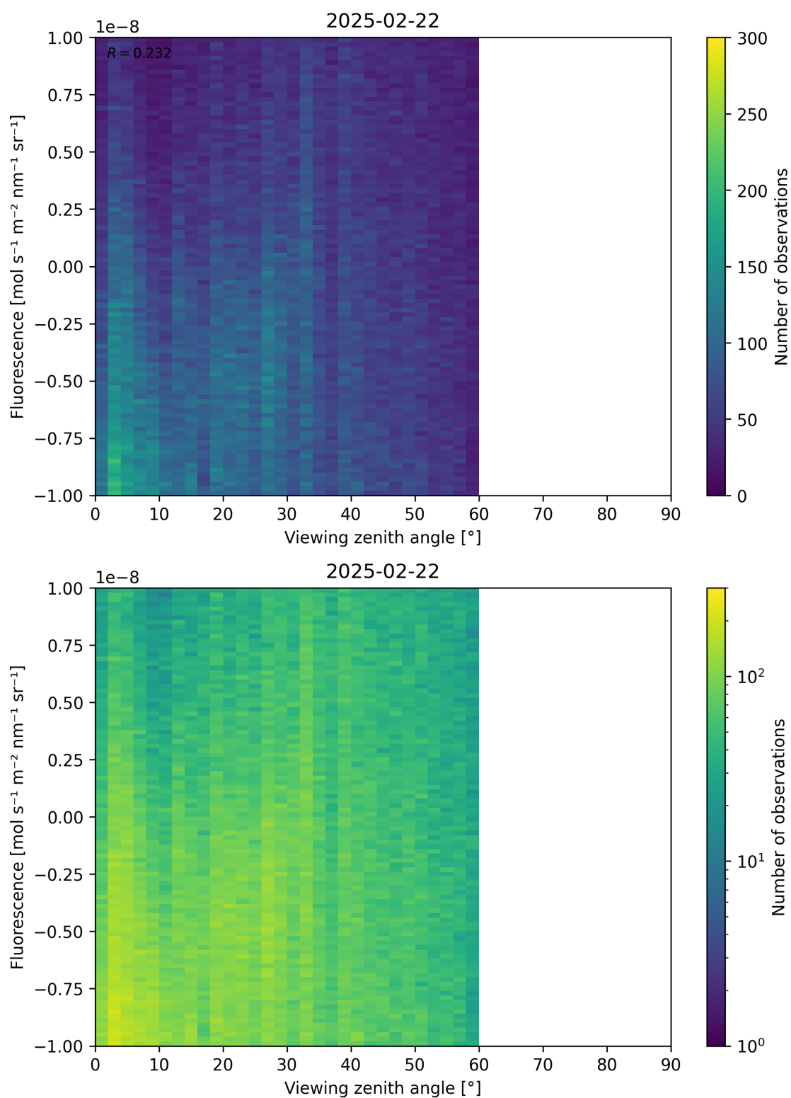
Figure 108: Scatter density plot of “Viewing zenith angle” against “Fluorescence” for 2025-02-21 to 2025-02-23.
