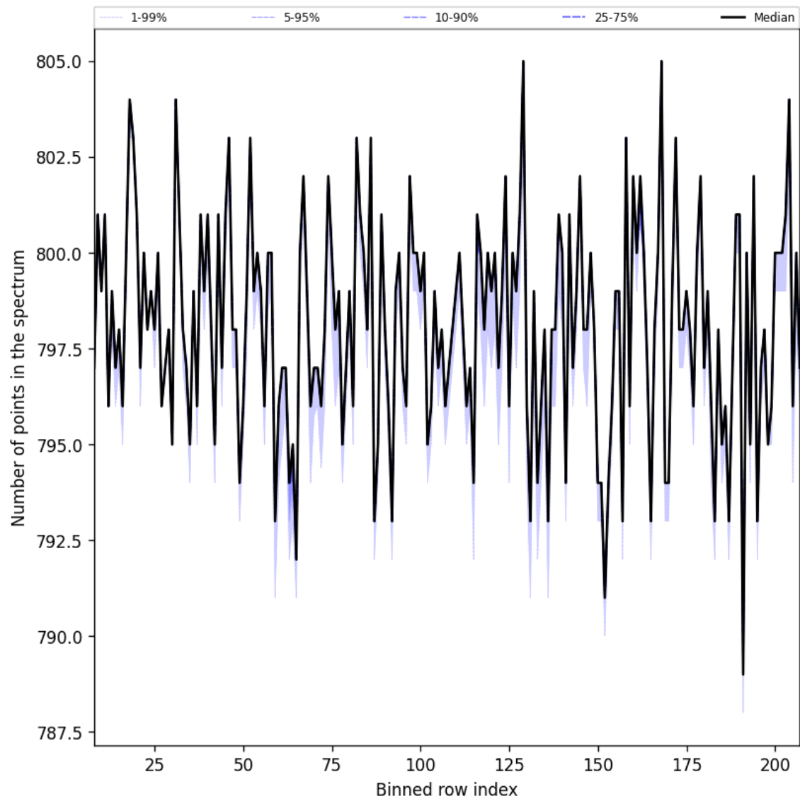
Figure 37: Along track statistics of “Number of points in the spectrum” for 2025-02-21 to 2025-02-23
