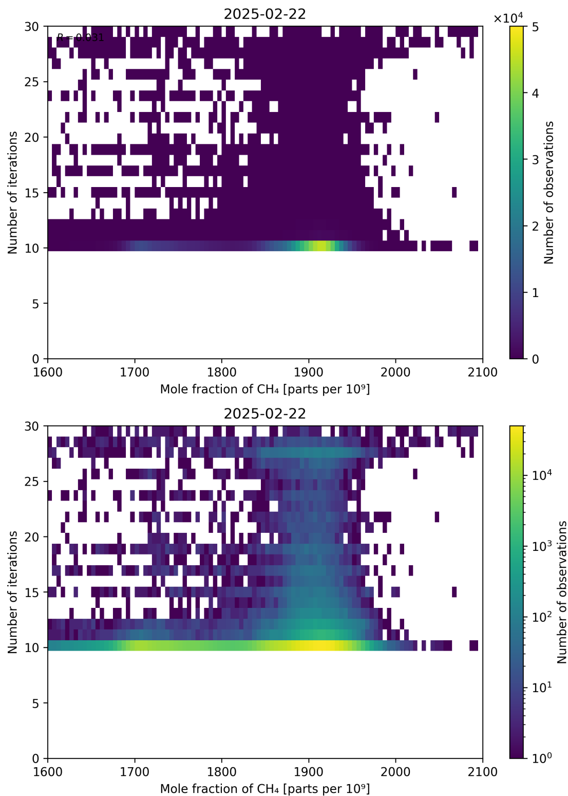
Figure 76: Scatter density plot of “Mole fraction of CH 4 ” against “Number of iterations” for 2025-02-21 to 2025-02-23.
