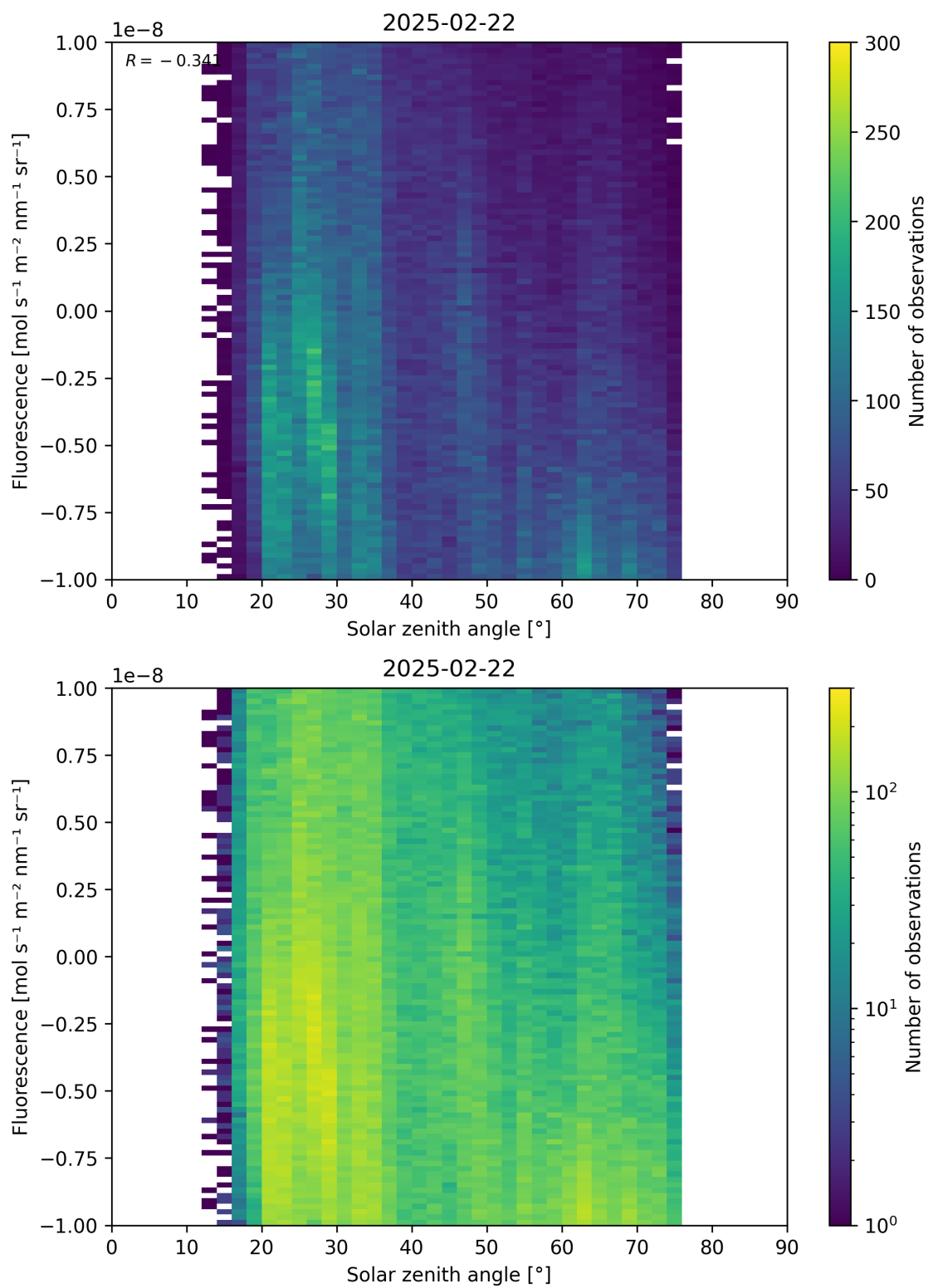
Figure 97: Scatter density plot of “Solar zenith angle” against “Fluorescence” for 2025-02-21 to 2025-02-23.
