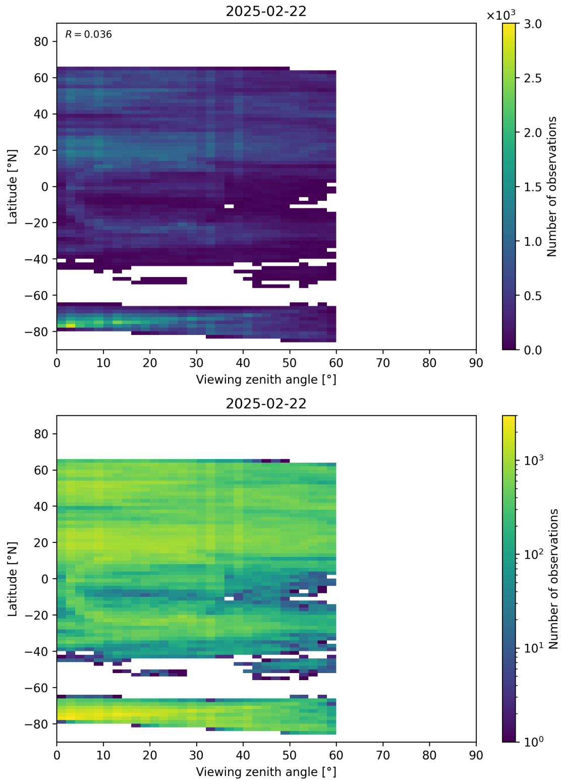
Figure 109: Scatter density plot of “Viewing zenith angle” against “Latitude” for 2025-02-21 to 2025-02-23.
