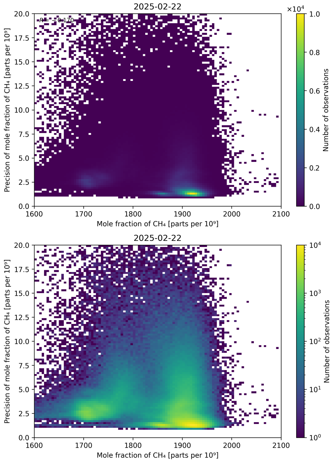
Figure 75: Scatter density plot of “Mole fraction of CH 4 ” against “Precision of mole fraction of CH 4 ” for 2025-02-21 to 2025-02-23.
