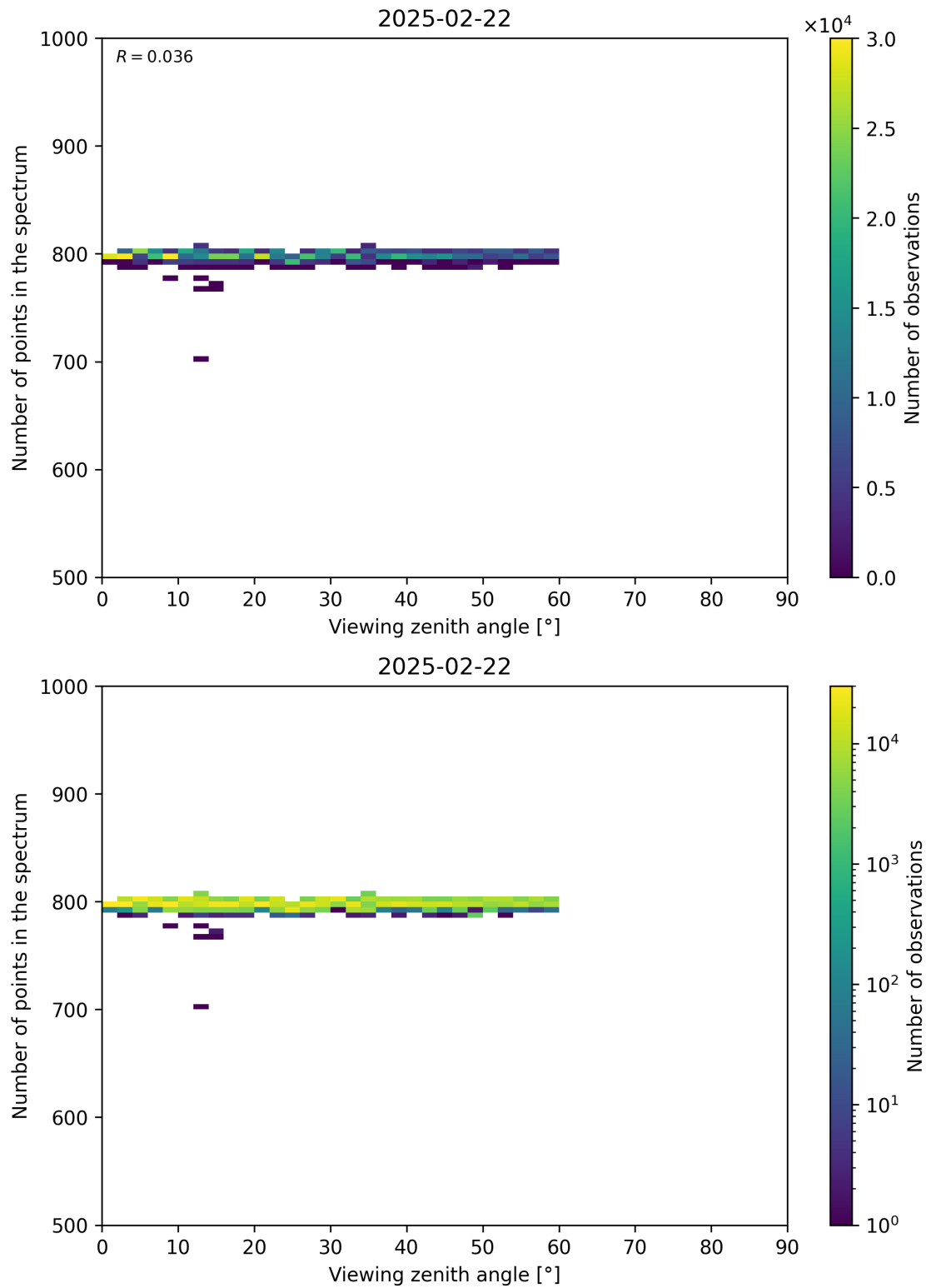
Figure 114: Scatter density plot of “Viewing zenith angle” against “Number of points in the spectrum” for 2025-02-21 to 2025-02-23.
