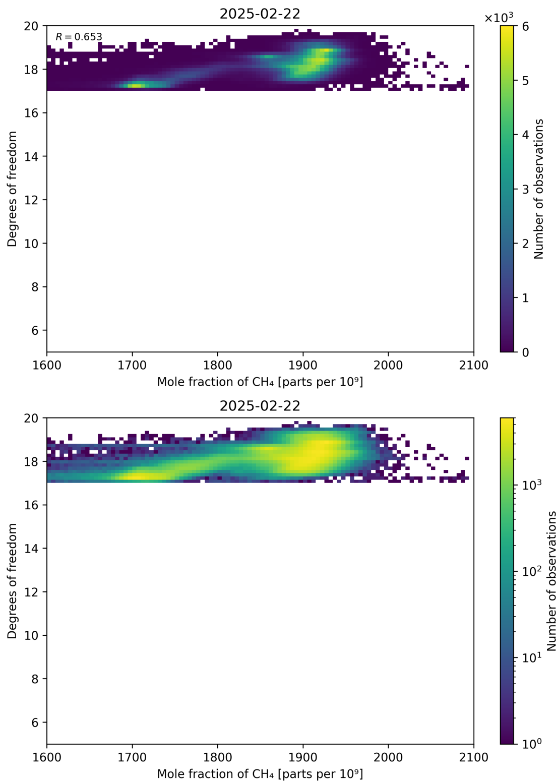
Figure 72: Scatter density plot of “Mole fraction of CH 4 ” against “Degrees of freedom” for 2025-02-21 to 2025-02-23.
