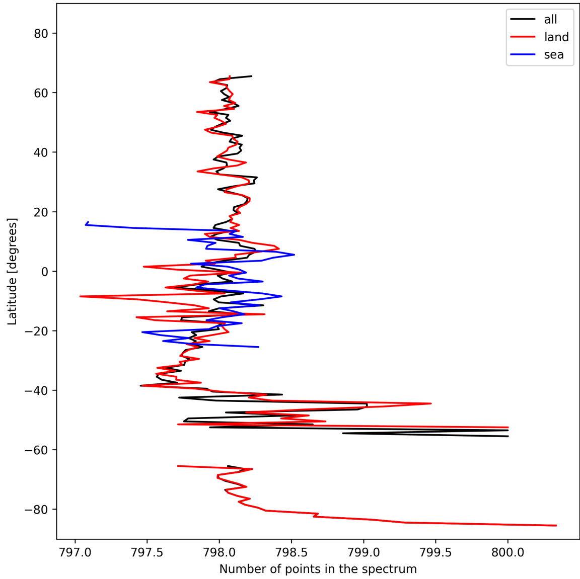
Figure 15: Zonal average of “Number of points in the spectrum” for 2025-02-21 to 2025-02-23.
