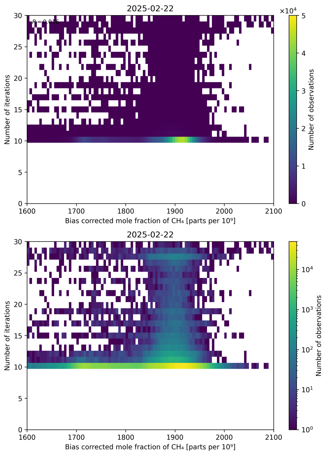
Figure 67: Scatter density plot of “Bias corrected mole fraction of CH 4 ” against “Number of iterations” for 2025-02-21 to 2025-02-23.
