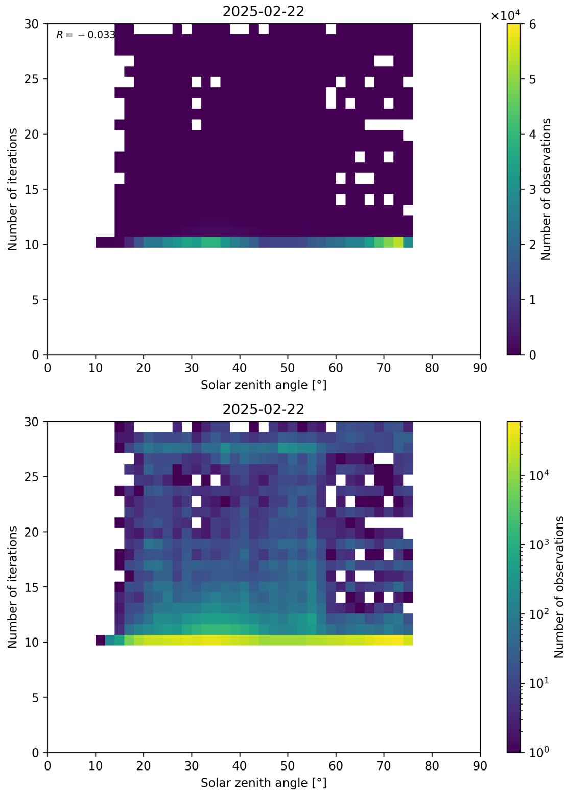
Figure 102: Scatter density plot of “Solar zenith angle” against “Number of iterations” for 2025-02-21 to 2025-02-23.
