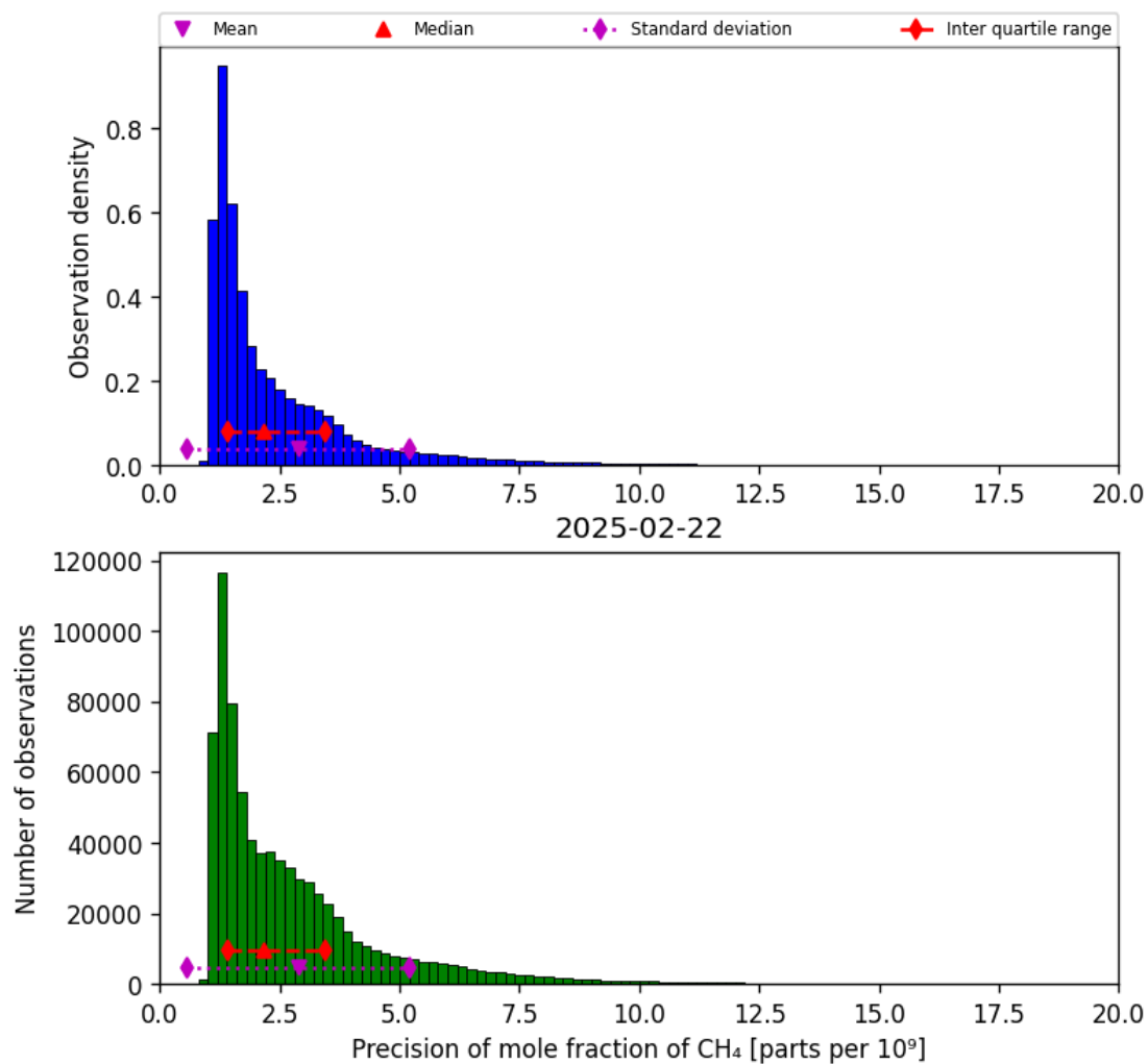
Figure 24: Histogram of “Precision of mole fraction of CH 4 ” for 2025-02-21 to 2025-02-23
