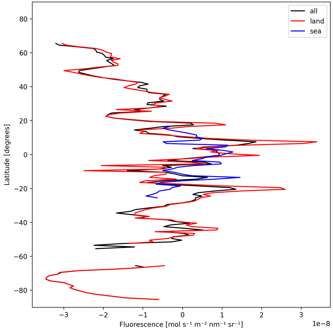
Figure 21: Zonal average of “Fluorescence” for 2025-02-21 to 2025-02-23.
