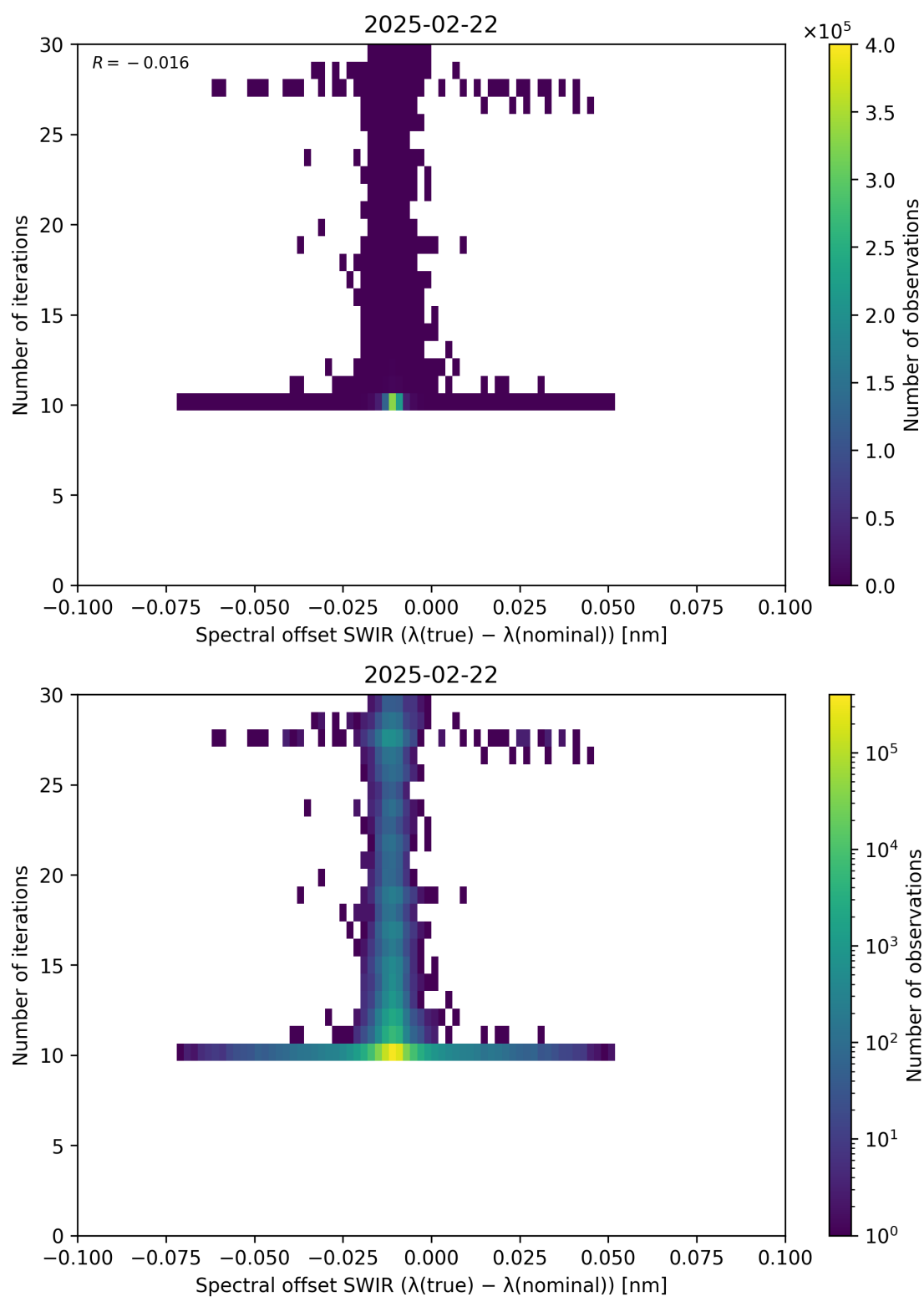
Figure 121: Scatter density plot of “Spectral offset SWIR ( \lambda_{\text{true}} - \lambda_{\text{nominal}} )” against “Number of iterations” for 2025-02-21 to 2025-02-23.
