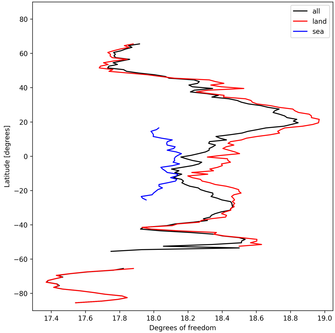
Figure 19: Zonal average of “Degrees of freedom” for 2025-02-21 to 2025-02-23.
