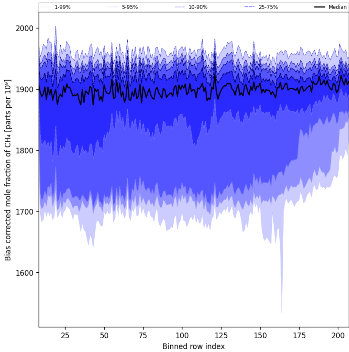
Figure 36: Along track statistics of “Bias corrected mole fraction of CH 4 ” for 2025-02-21 to 2025-02-23
