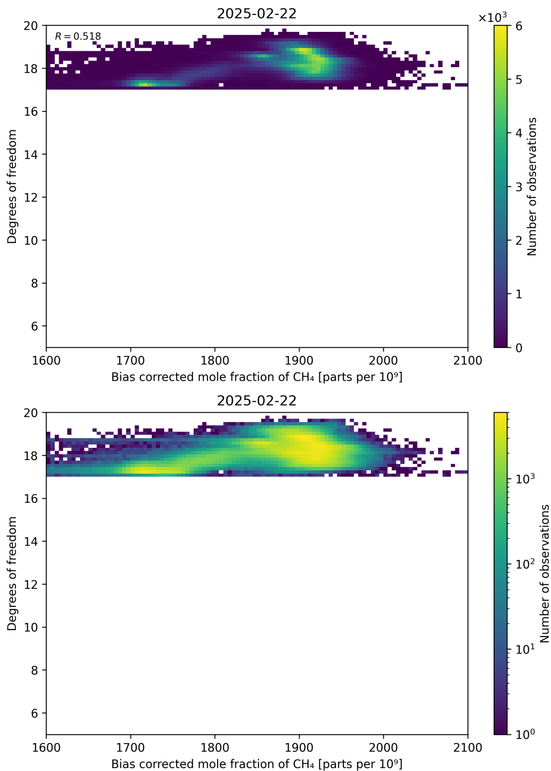
Figure 65: Scatter density plot of “Bias corrected mole fraction of CH 4 ” against “Degrees of freedom” for 2025-02-21 to 2025-02-23.
