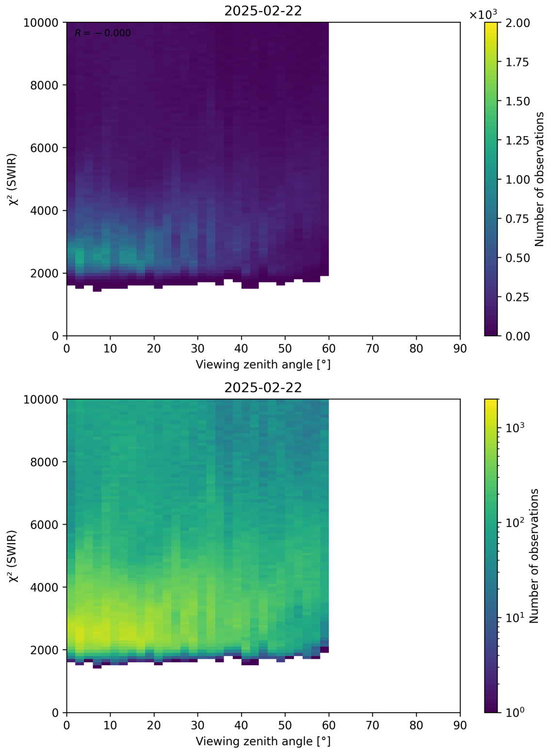
Figure 106: Scatter density plot of “Viewing zenith angle” against “ \chi^2 (SWIR)” for 2025-02-21 to 2025-02-23.
