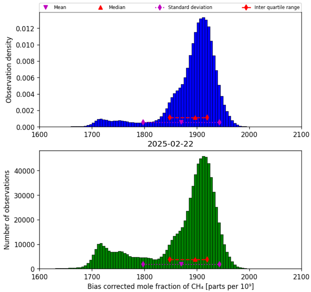
Figure 25: Histogram of “Bias corrected mole fraction of CH 4 ” for 2025-02-21 to 2025-02-23
