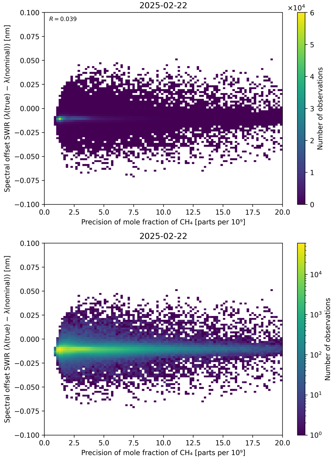
Figure 85: Scatter density plot of “Precision of mole fraction of \text{CH}_4 ” against “Spectral offset SWIR ( \lambda_{\text{true}} - \lambda_{\text{nominal}} )” for 2025-02-21 to 2025-02-23.
