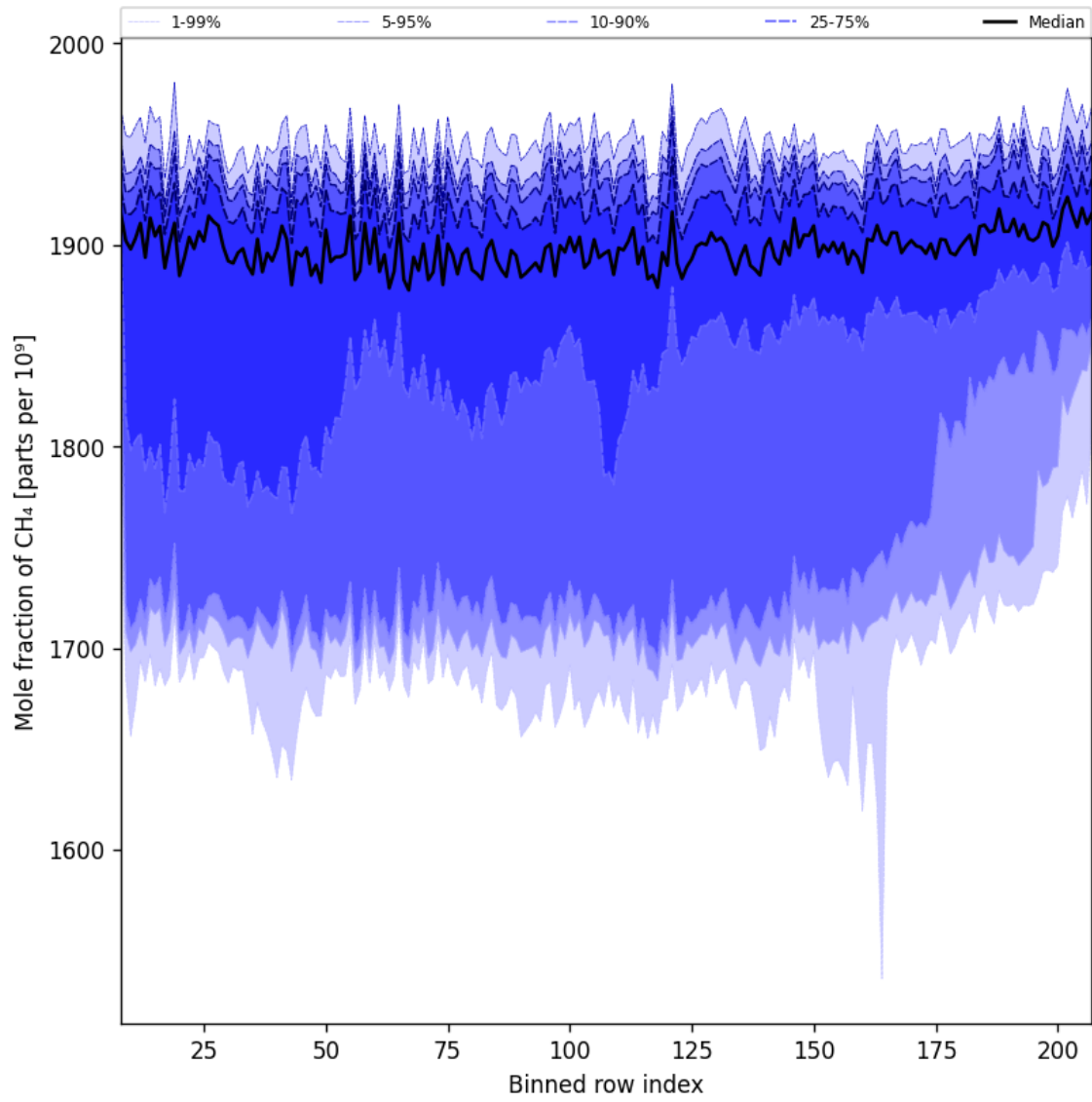
Figure 34: Along track statistics of “Mole fraction of \text{CH}_4 ” for 2025-02-21 to 2025-02-23
