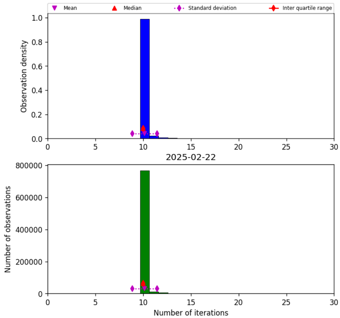
Figure 31: Histogram of “Number of iterations” for 2025-02-21 to 2025-02-23
