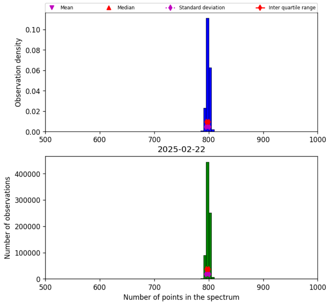
Figure 26: Histogram of “Number of points in the spectrum” for 2025-02-21 to 2025-02-23
