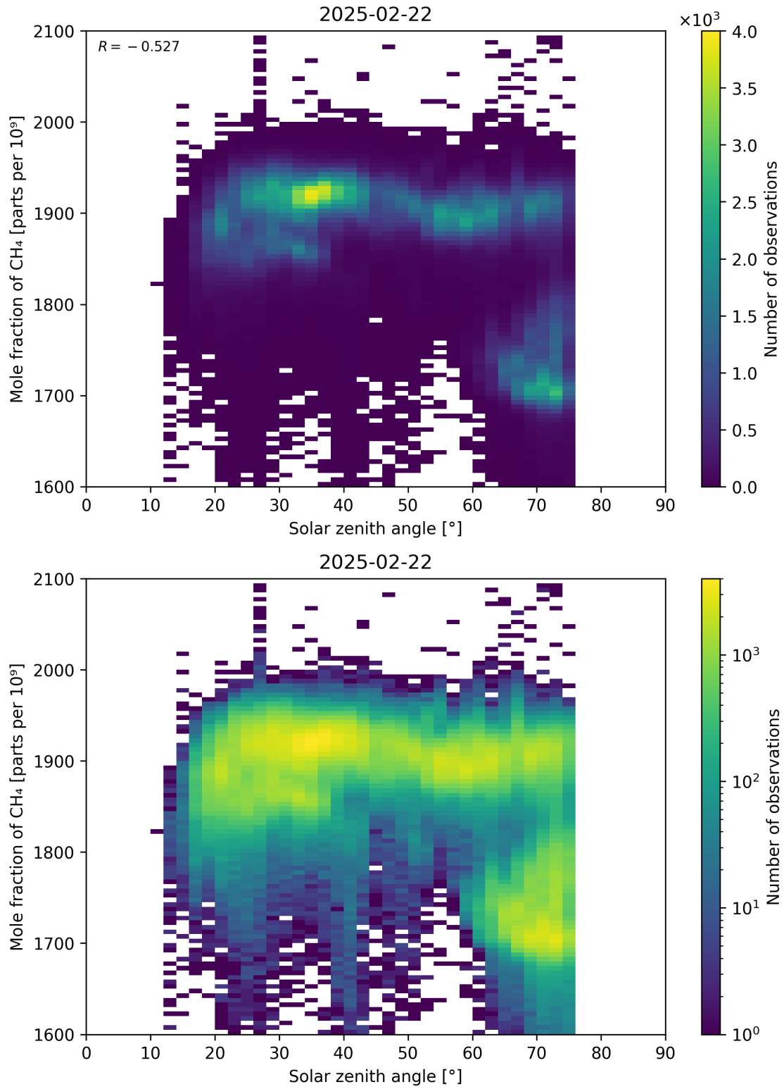
Figure 99: Scatter density plot of “Solar zenith angle” against “Mole fraction of CH 4 ” for 2025-02-21 to 2025-02-23.
