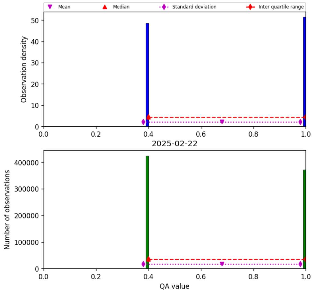
Figure 22: Histogram of “QA value” for 2025-02-21 to 2025-02-23
