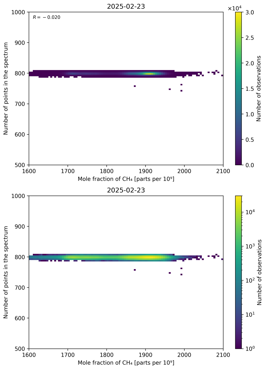
Figure 77: Scatter density plot of “Mole fraction of CH 4 ” against “Number of points in the spectrum” for 2025-02-22 to 2025-02-24.
