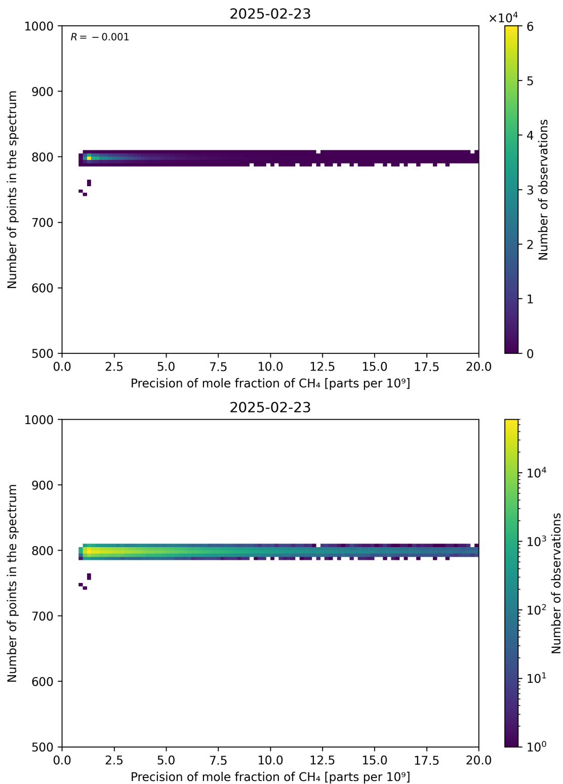
Figure 84: Scatter density plot of “Precision of mole fraction of CH 4 ” against “Number of points in the spectrum” for 2025-02-22 to 2025-02-24.
