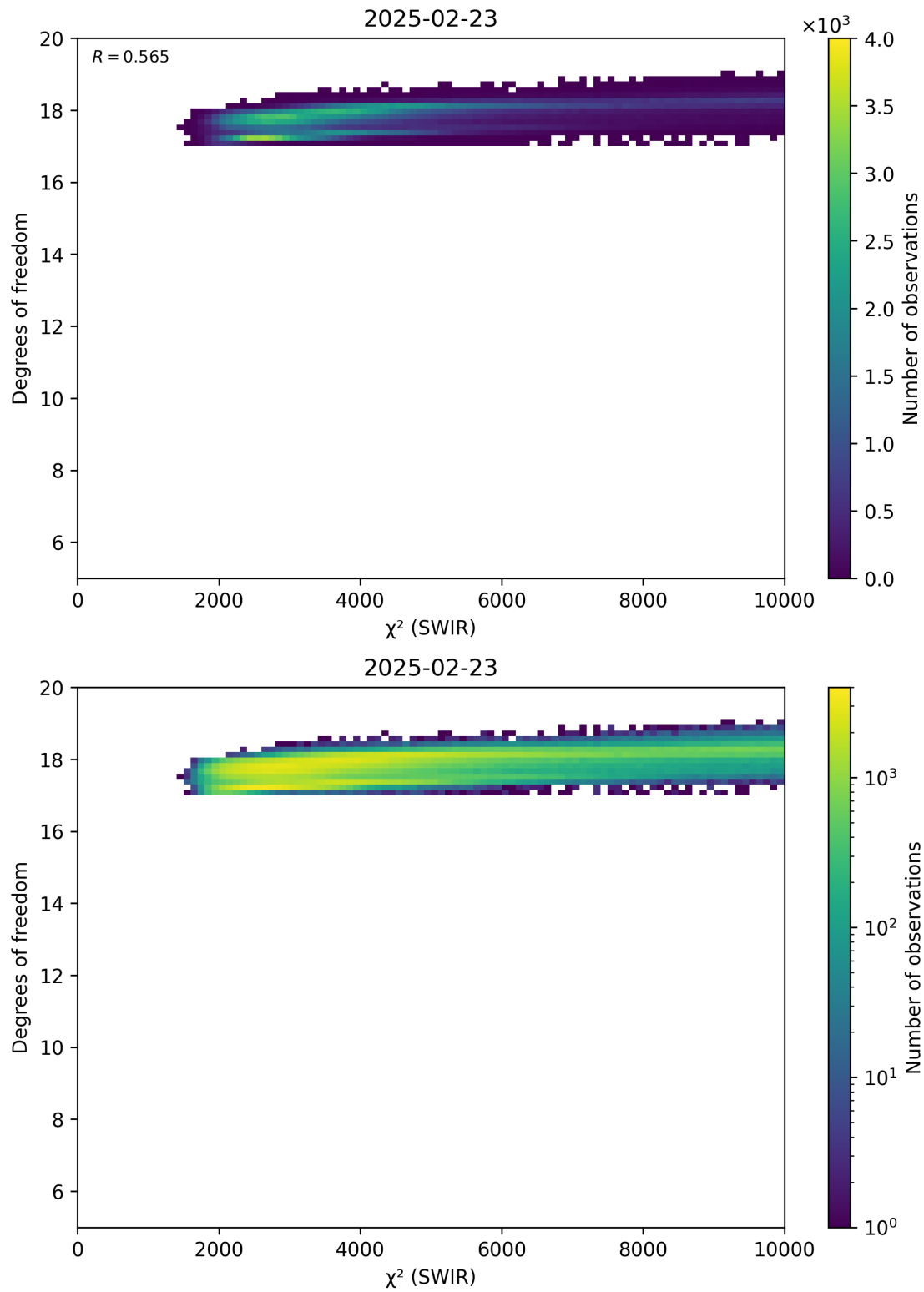
Figure 48: Scatter density plot of “ \chi^2 (SWIR)” against “Degrees of freedom” for 2025-02-22 to 2025-02-24.
