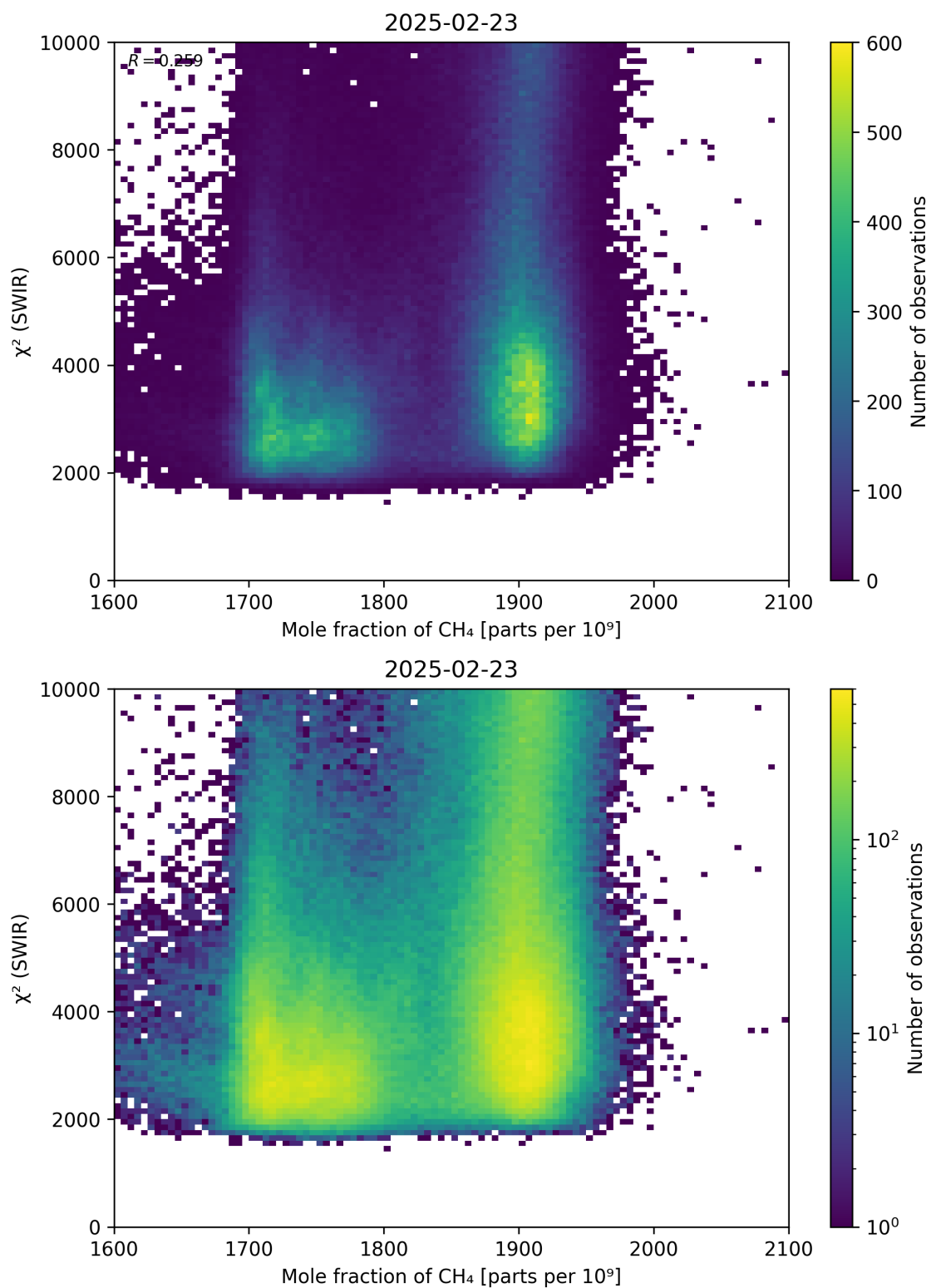
Figure 71: Scatter density plot of “Mole fraction of CH 4 ” against “ \chi^2 (SWIR)” for 2025-02-22 to 2025-02-24.
