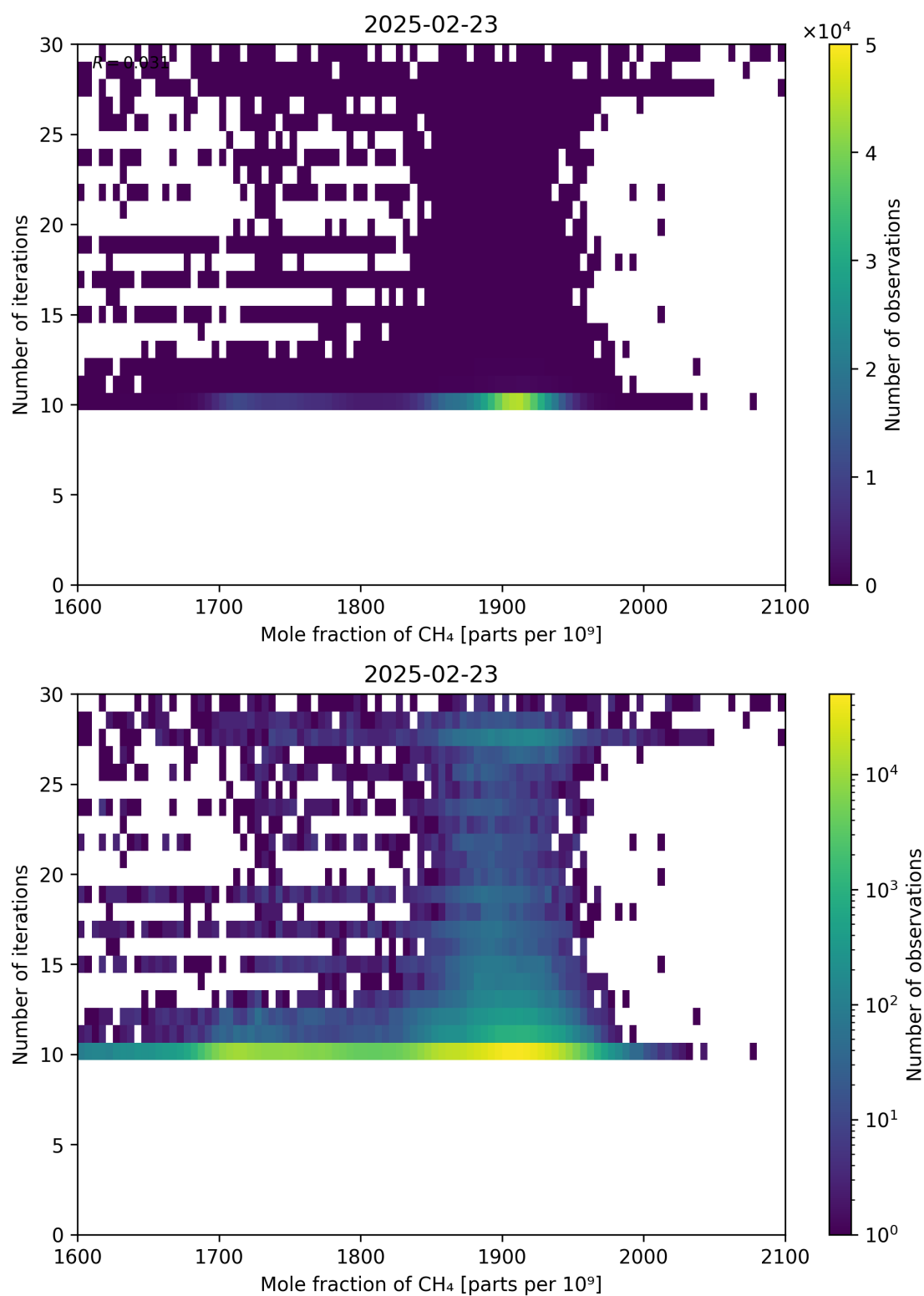
Figure 76: Scatter density plot of “Mole fraction of CH 4 ” against “Number of iterations” for 2025-02-22 to 2025-02-24.
