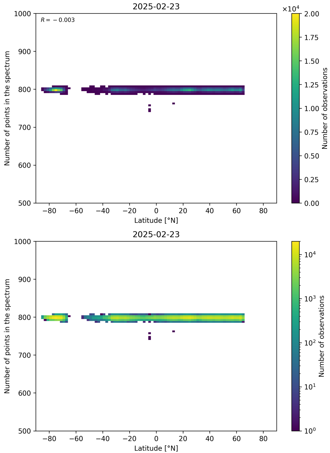
Figure 61: Scatter density plot of “Latitude” against “Number of points in the spectrum” for 2025-02-22 to 2025-02-24.
