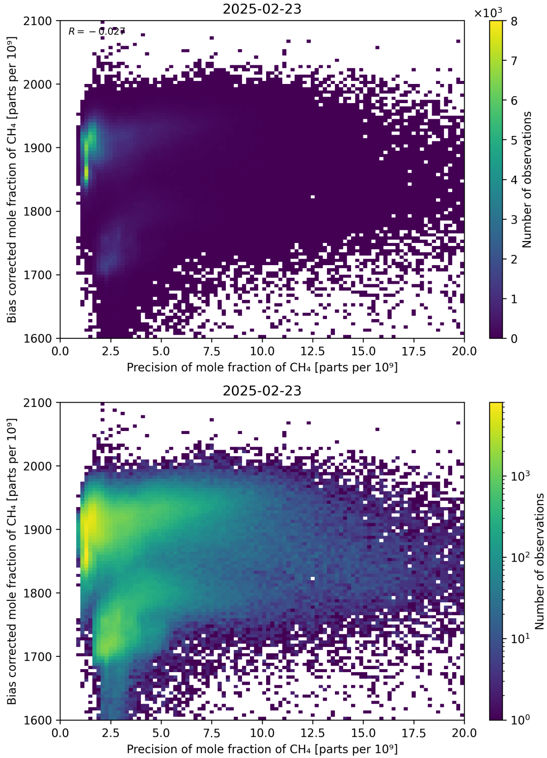
Figure 82: Scatter density plot of “Precision of mole fraction of CH 4 ” against “Bias corrected mole fraction of CH 4 ” for 2025-02-22 to 2025-02-24.
