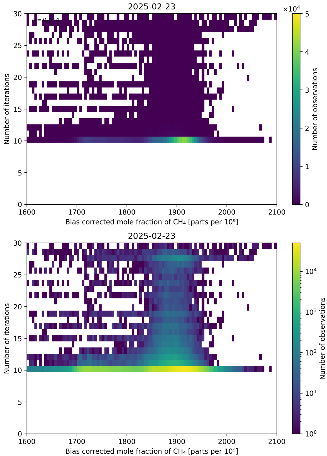
Figure 67: Scatter density plot of “Bias corrected mole fraction of \text{CH}_4 ” against “Number of iterations” for 2025-02-22 to 2025-02-24.
