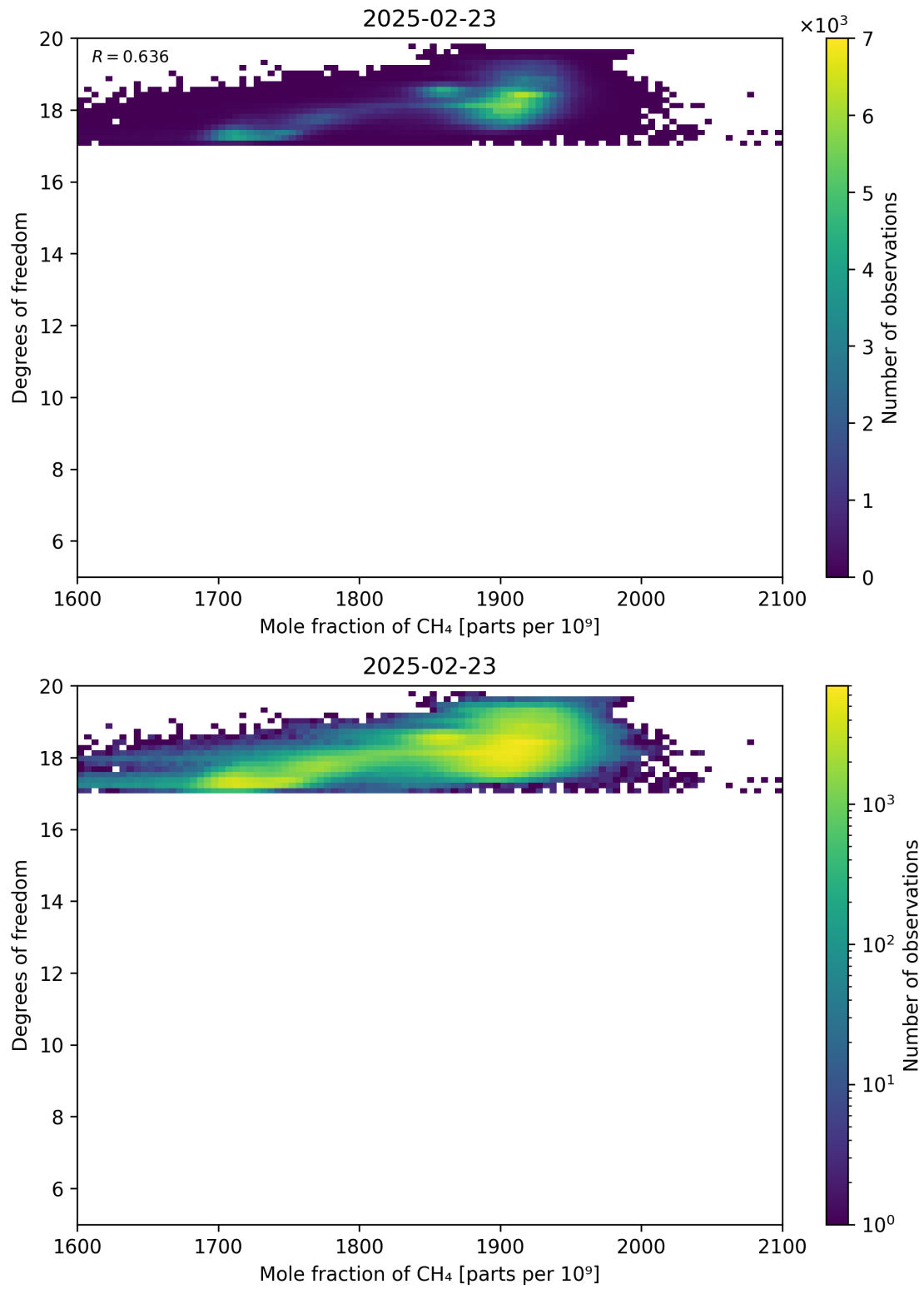
Figure 72: Scatter density plot of “Mole fraction of CH 4 ” against “Degrees of freedom” for 2025-02-22 to 2025-02-24.
