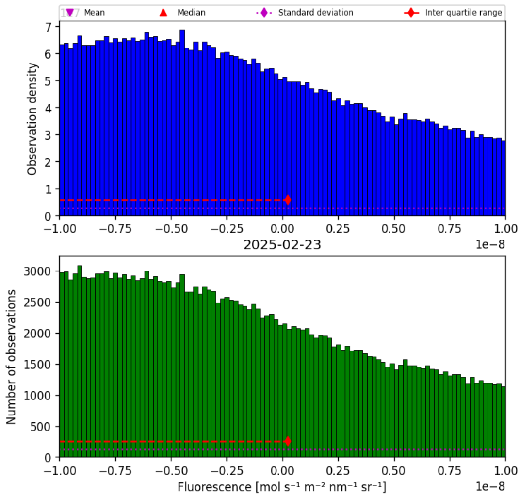
Figure 32: Histogram of “Fluorescence” for 2025-02-22 to 2025-02-24
