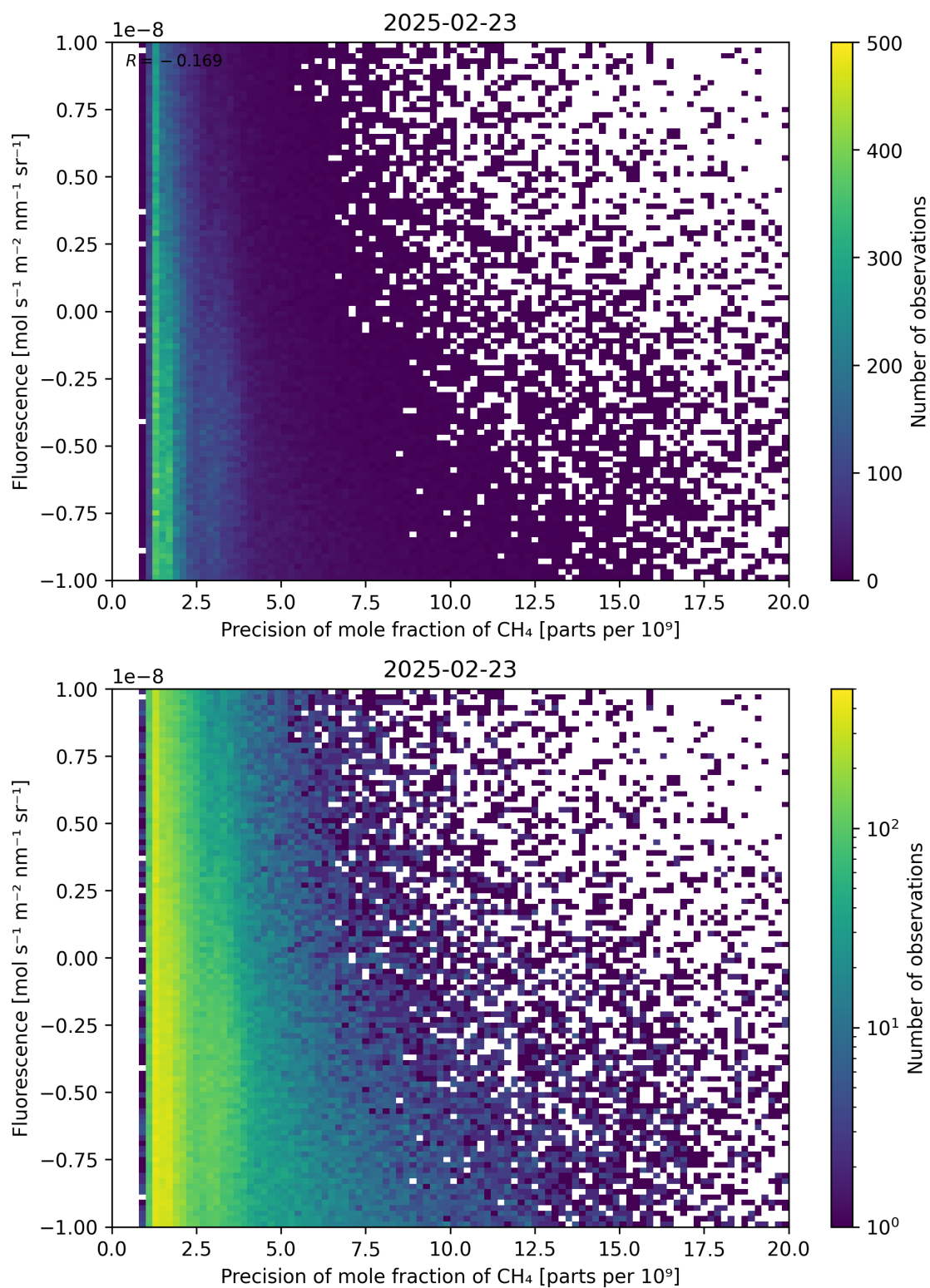
Figure 81: Scatter density plot of “Precision of mole fraction of \text{CH}_4 ” against “Fluorescence” for 2025-02-22 to 2025-02-24.
