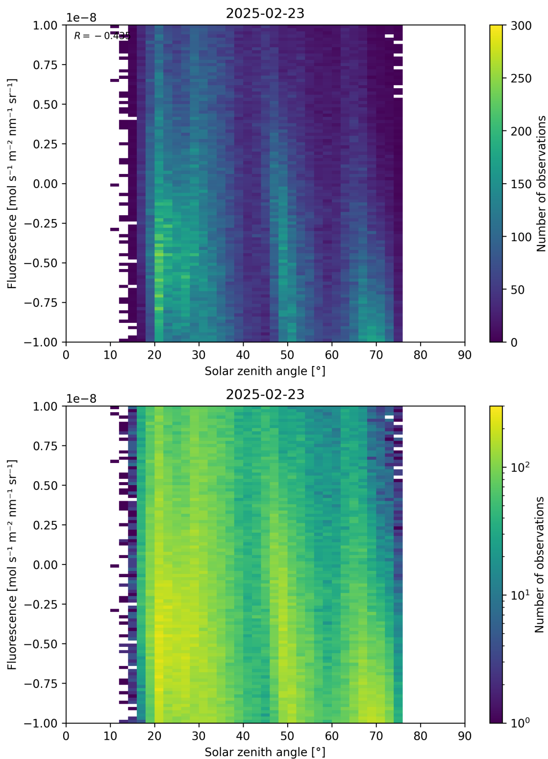
Figure 97: Scatter density plot of “Solar zenith angle” against “Fluorescence” for 2025-02-22 to 2025-02-24.
