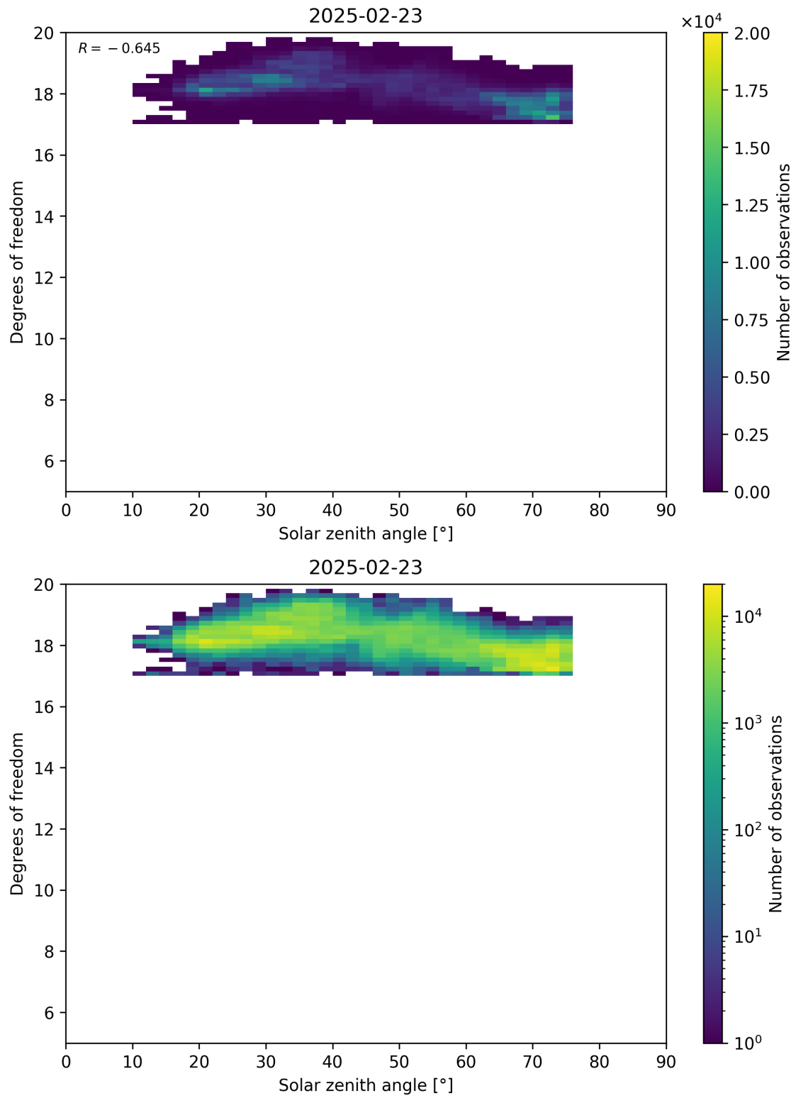
Figure 96: Scatter density plot of “Solar zenith angle” against “Degrees of freedom” for 2025-02-22 to 2025-02-24.
