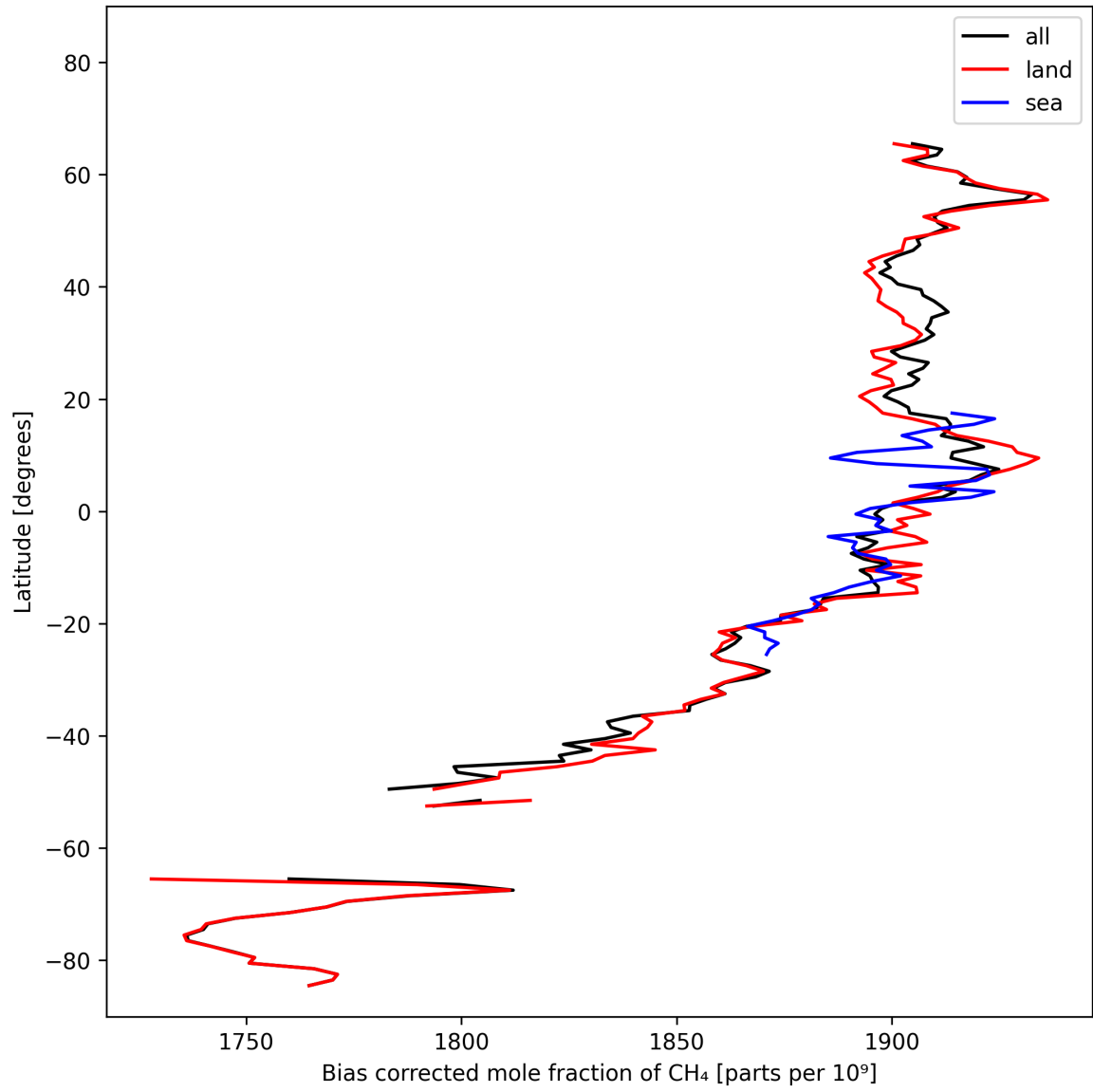
Figure 14: Zonal average of “Bias corrected mole fraction of CH 4 ” for 2025-02-22 to 2025-02-24.
