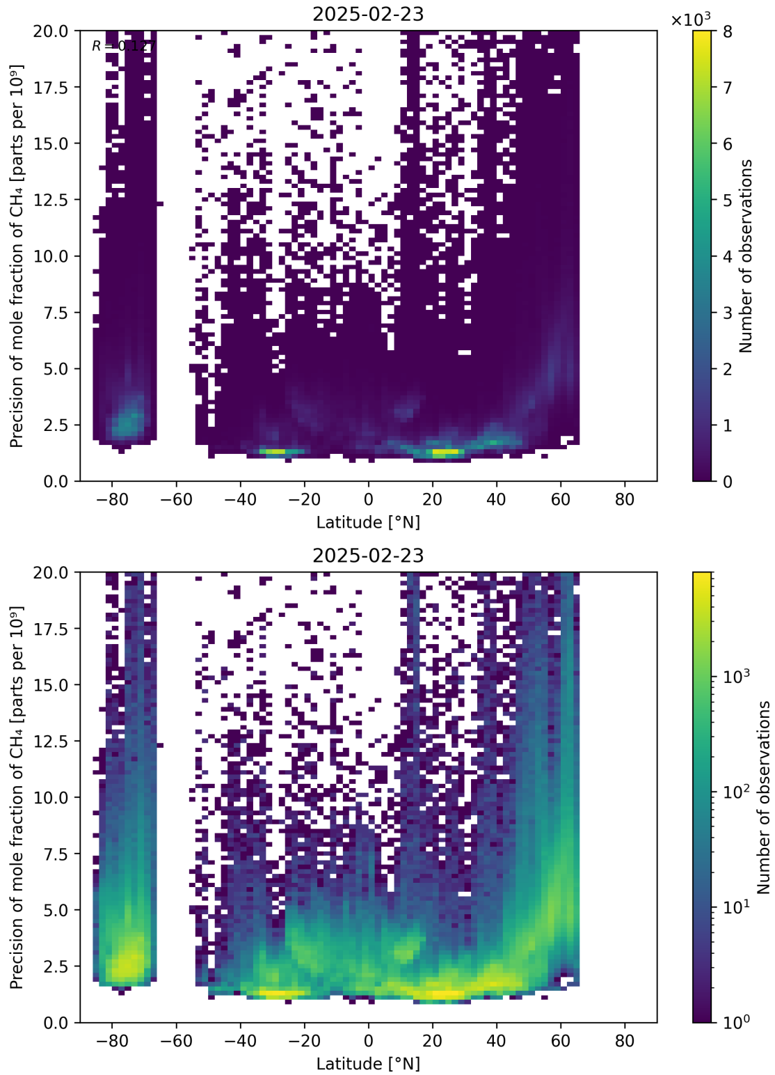
Figure 59: Scatter density plot of “Latitude” against “Precision of mole fraction of CH 4 ” for 2025-02-22 to 2025-02-24.
