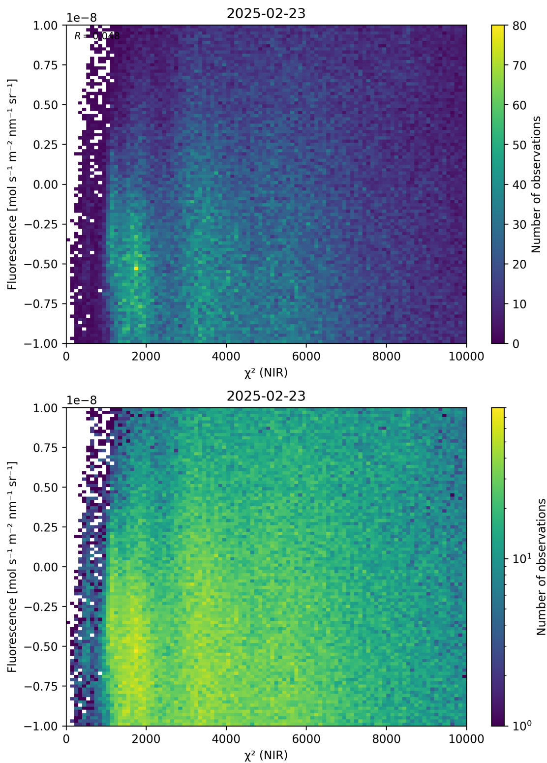
Figure 45: Scatter density plot of “ \chi^2 (NIR)” against “Fluorescence” for 2025-02-22 to 2025-02-24.
