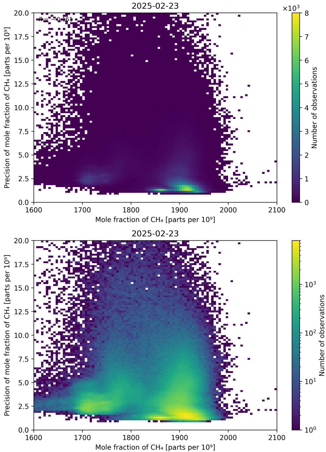
Figure 75: Scatter density plot of “Mole fraction of CH 4 ” against “Precision of mole fraction of CH 4 ” for 2025-02-22 to 2025-02-24.
