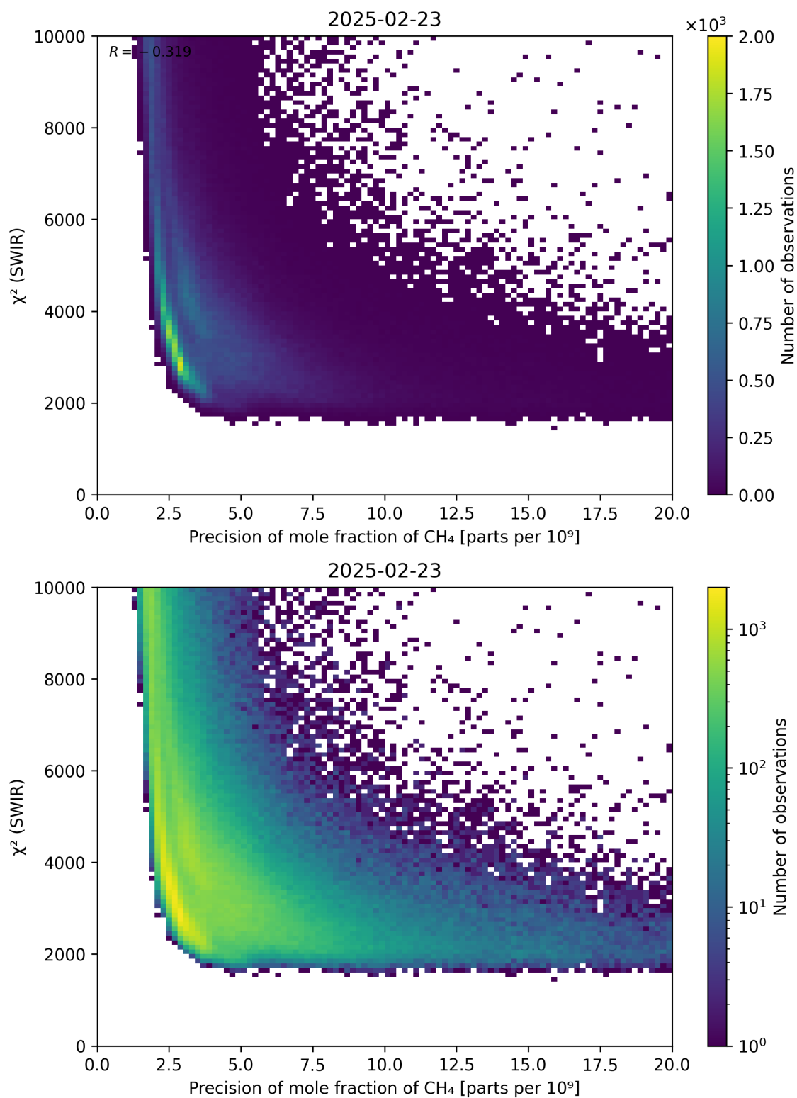
Figure 79: Scatter density plot of “Precision of mole fraction of \text{CH}_4 ” against “ \chi^2 (SWIR)” for 2025-02-22 to 2025-02-24.
