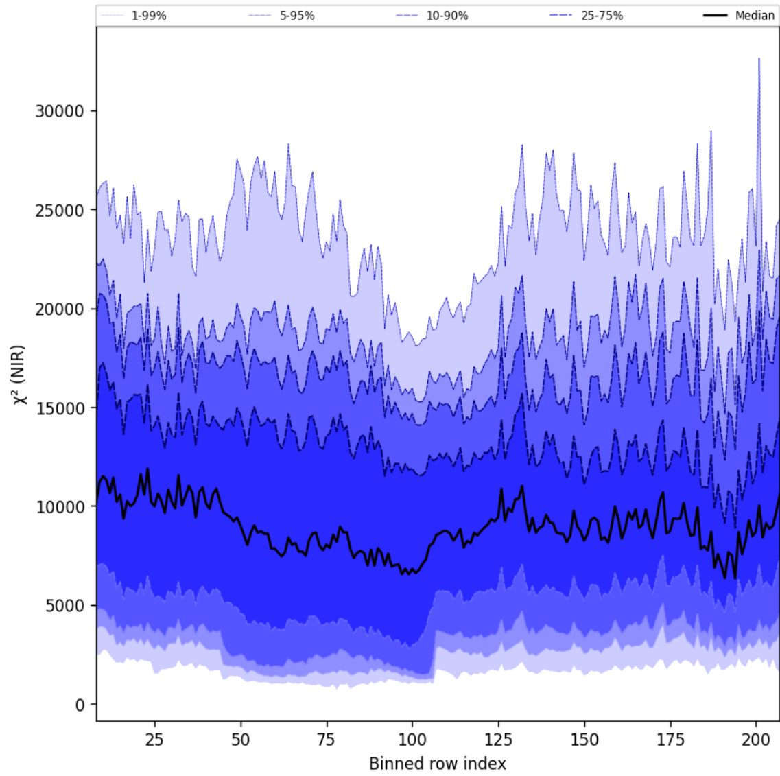
Figure 40: Along track statistics of “ \chi^2 (NIR)” for 2025-02-22 to 2025-02-24
