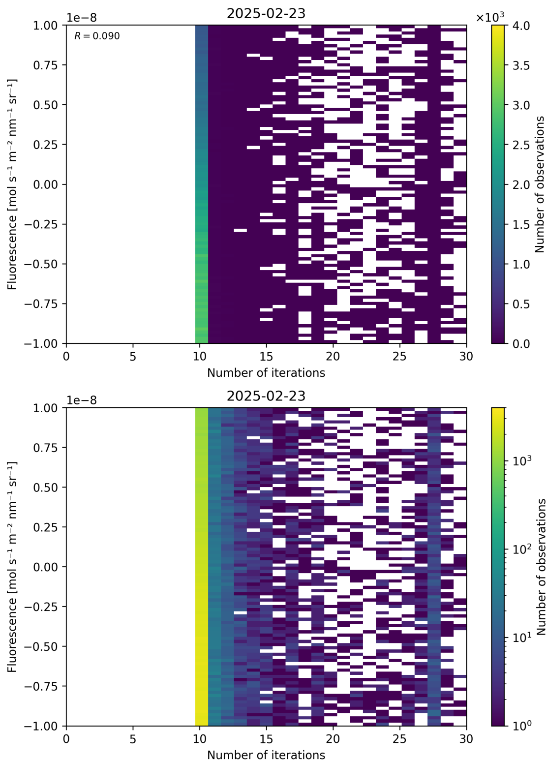
Figure 87: Scatter density plot of “Number of iterations” against “Fluorescence” for 2025-02-22 to 2025-02-24.
