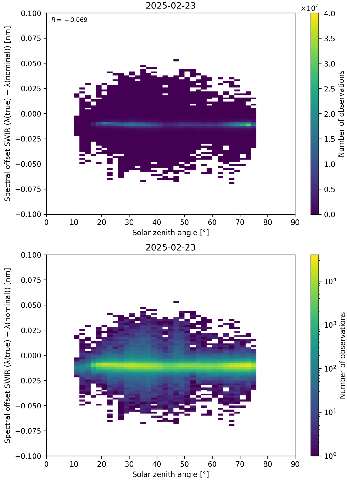
Figure 104: Scatter density plot of “Solar zenith angle” against “Spectral offset SWIR ( \lambda_{\text{true}} - \lambda_{\text{nominal}} )” for 2025-02-22 to 2025-02-24.
