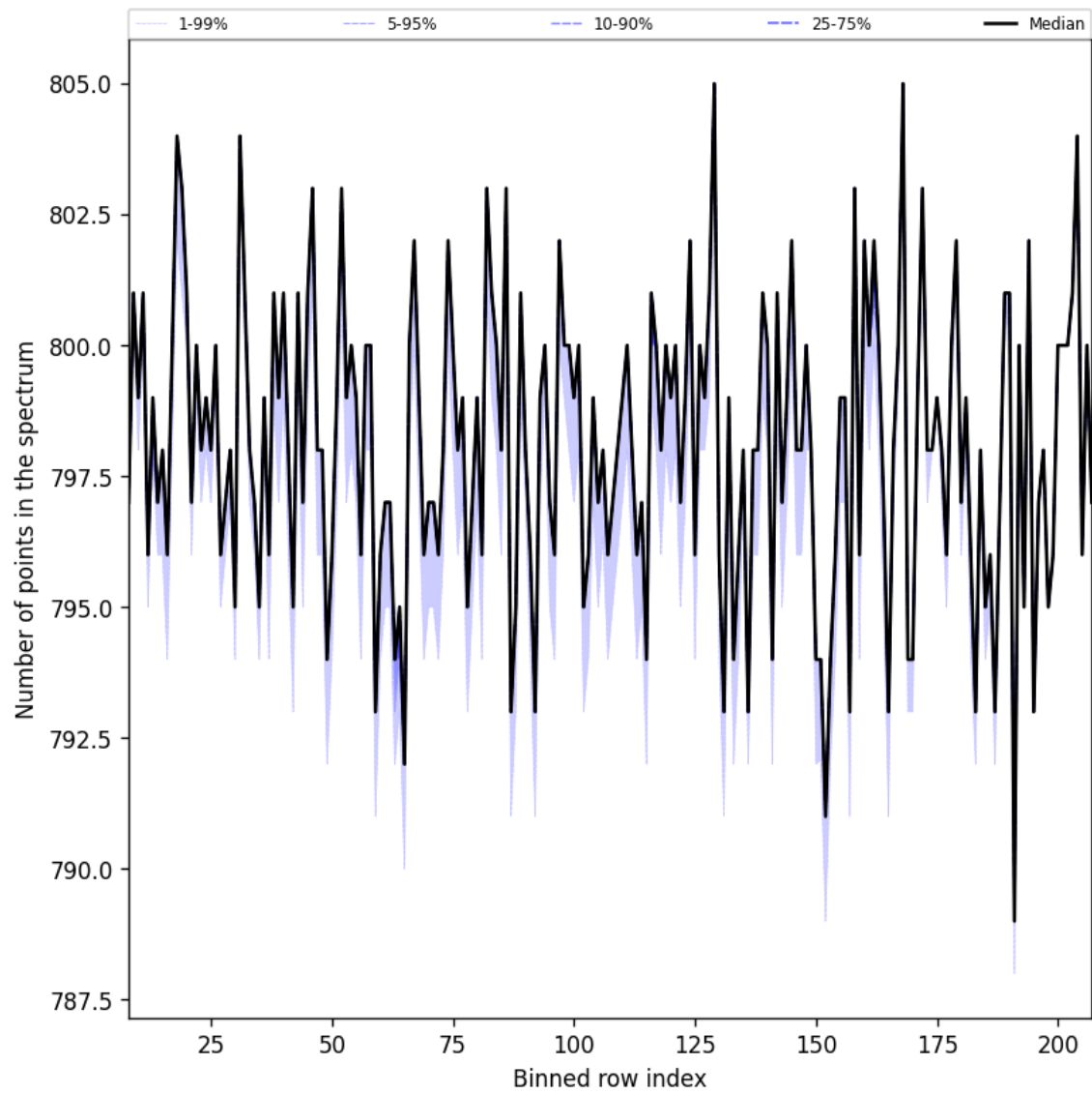
Figure 37: Along track statistics of “Number of points in the spectrum” for 2025-02-22 to 2025-02-24
