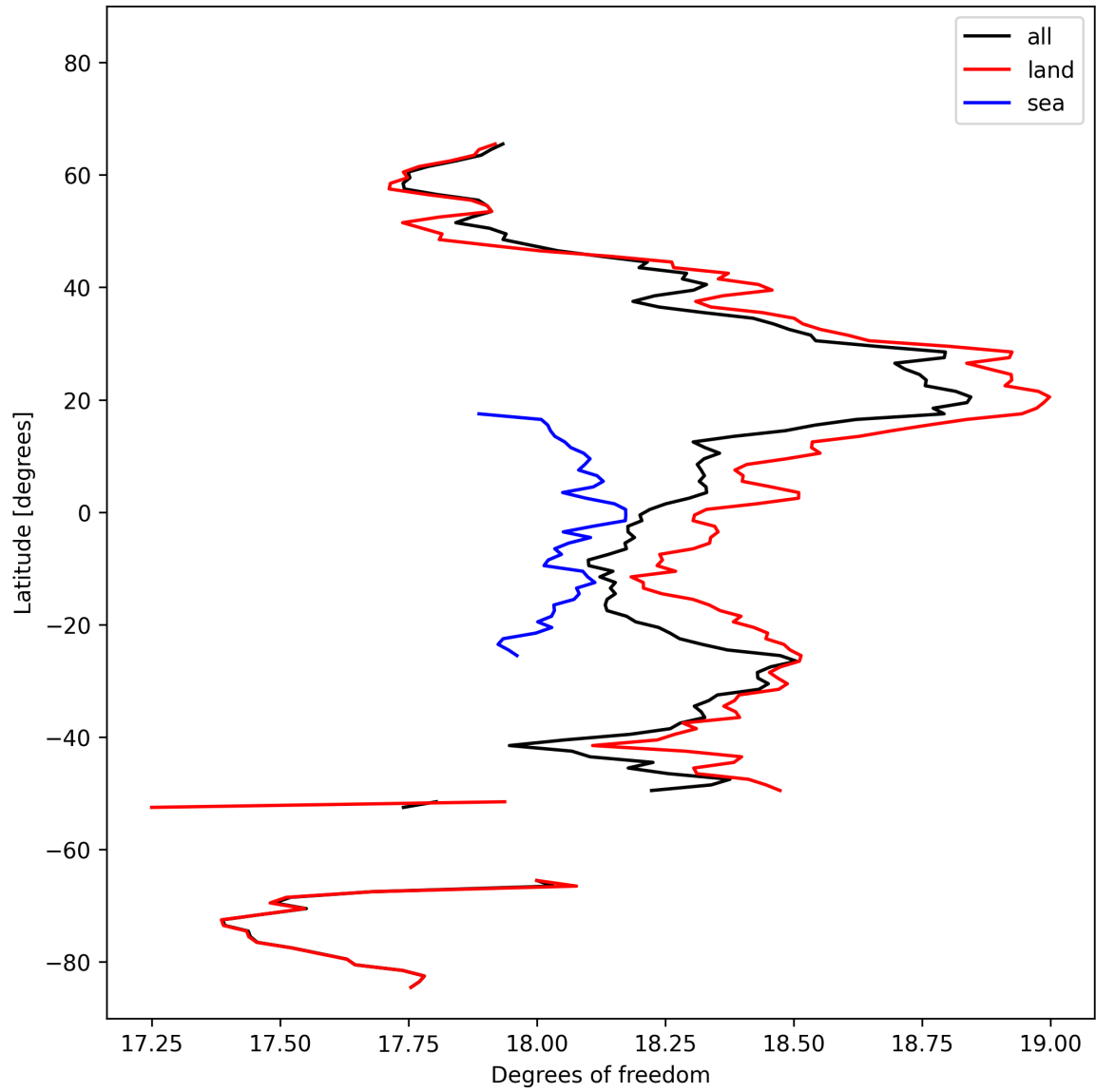
Figure 19: Zonal average of “Degrees of freedom” for 2025-02-22 to 2025-02-24.
