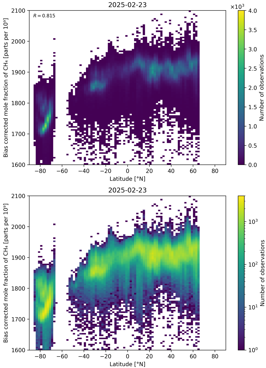
Figure 58: Scatter density plot of “Latitude” against “Bias corrected mole fraction of CH 4 ” for 2025-02-22 to 2025-02-24.
