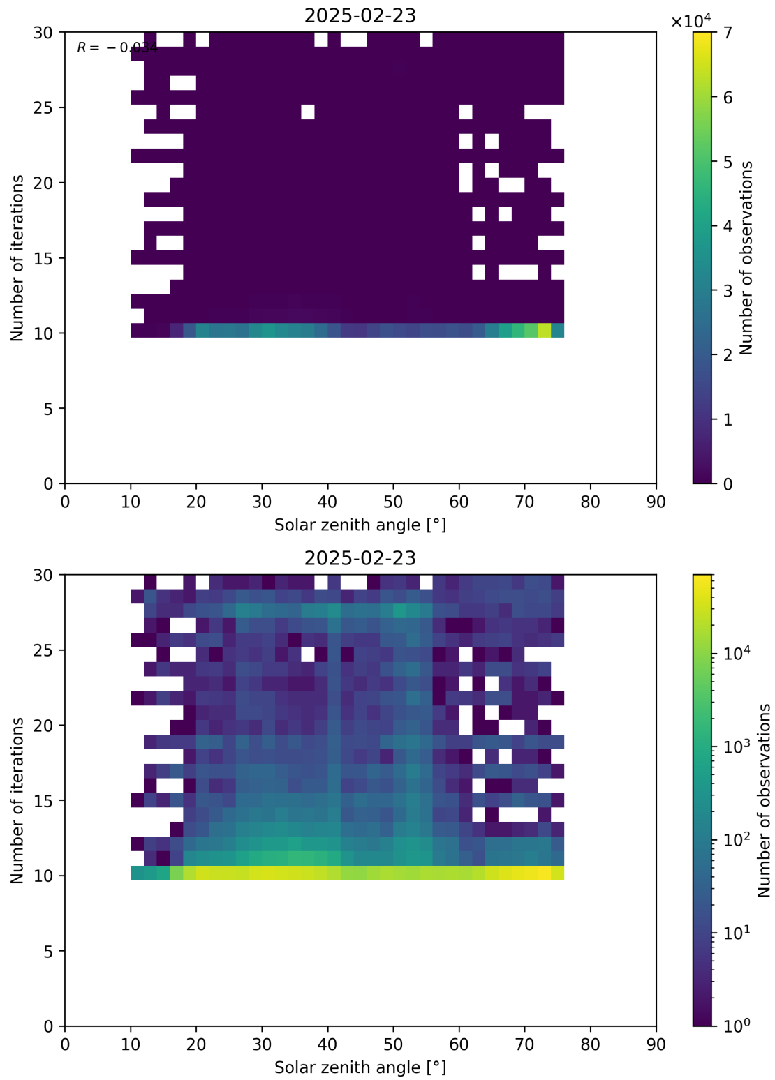
Figure 102: Scatter density plot of “Solar zenith angle” against “Number of iterations” for 2025-02-22 to 2025-02-24.
