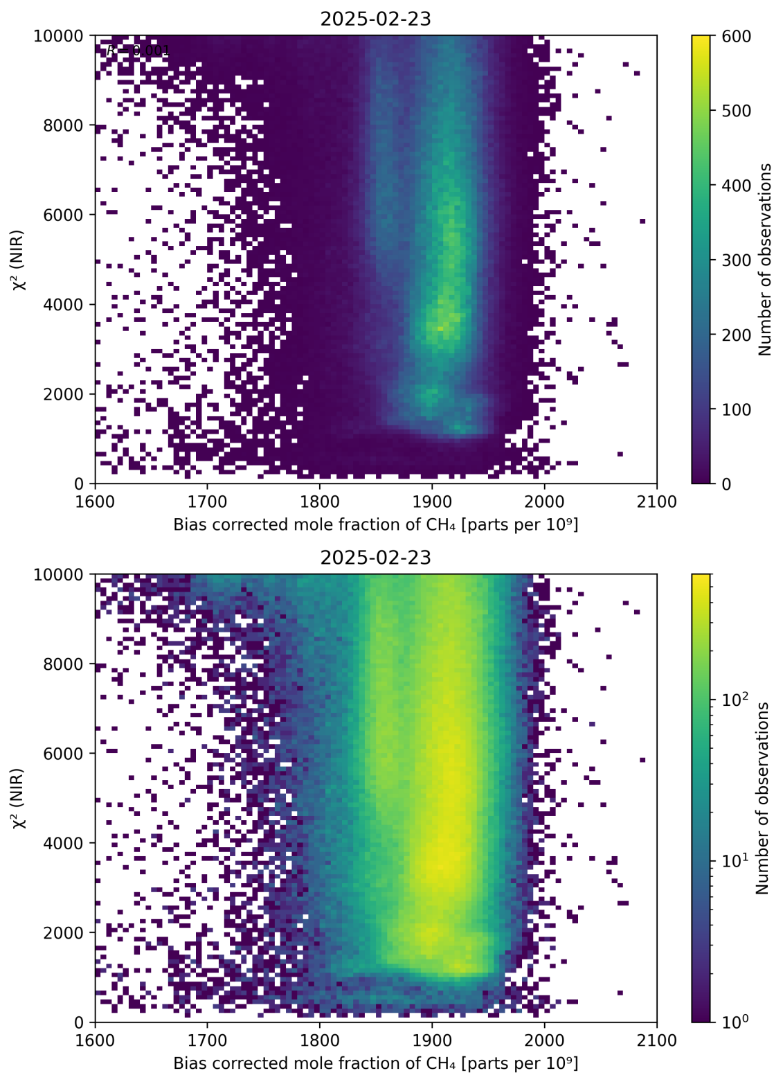
Figure 63: Scatter density plot of “Bias corrected mole fraction of \text{CH}_4 ” against “ \chi^2 (NIR)” for 2025-02-22 to 2025-02-24.
