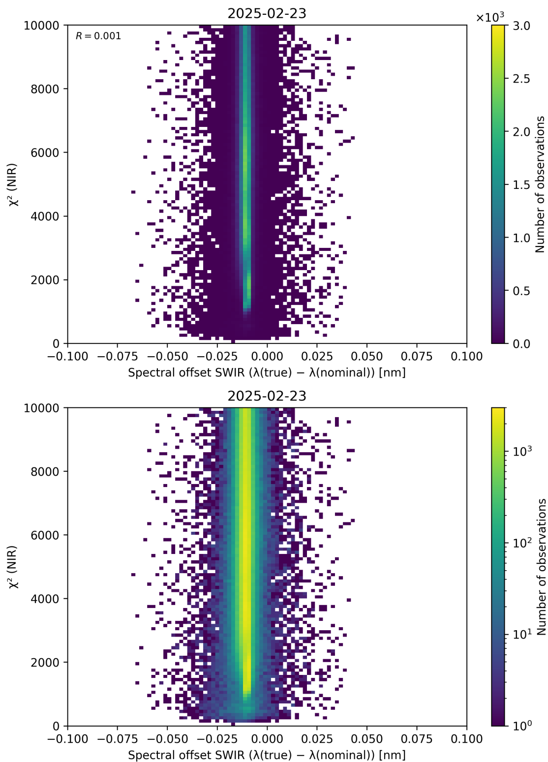
Figure 117: Scatter density plot of “Spectral offset SWIR ( \lambda_{\text{true}} - \lambda_{\text{nominal}} )” against “ \chi^2 (NIR)” for 2025-02-22 to 2025-02-24.
