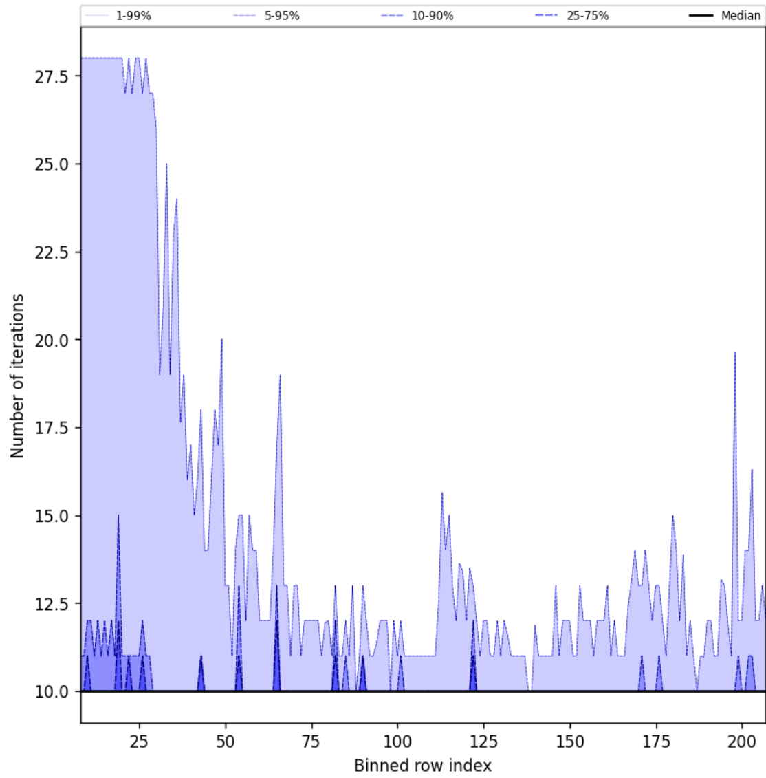
Figure 42: Along track statistics of “Number of iterations” for 2025-02-22 to 2025-02-24
