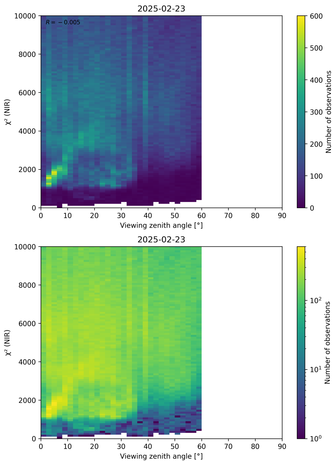
Figure 105: Scatter density plot of “Viewing zenith angle” against “ \chi^2 (NIR)” for 2025-02-22 to 2025-02-24.
