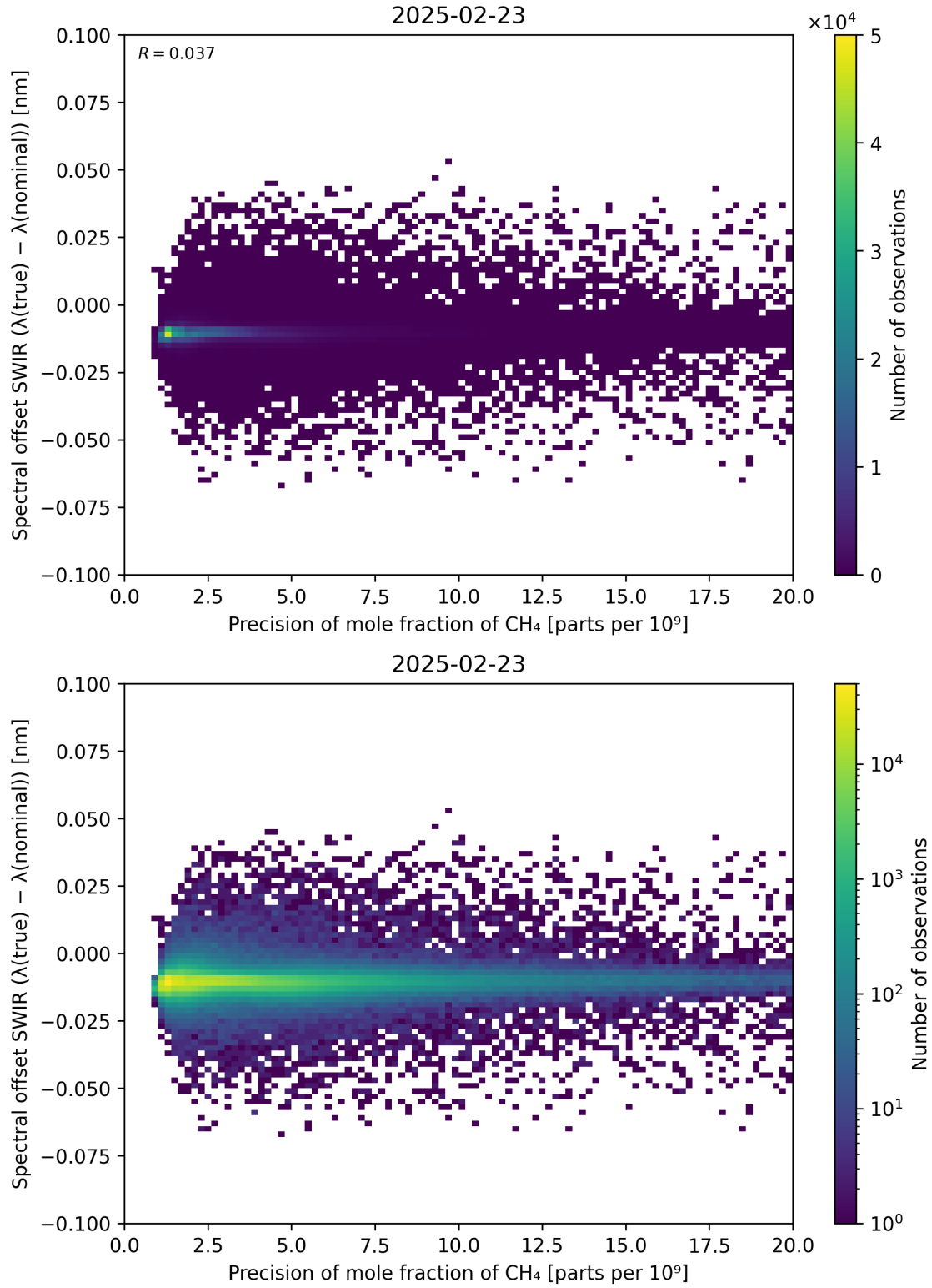
Figure 85: Scatter density plot of “Precision of mole fraction of \text{CH}_4 ” against “Spectral offset SWIR ( \lambda_{\text{true}} - \lambda_{\text{nominal}} )” for 2025-02-22 to 2025-02-24.
