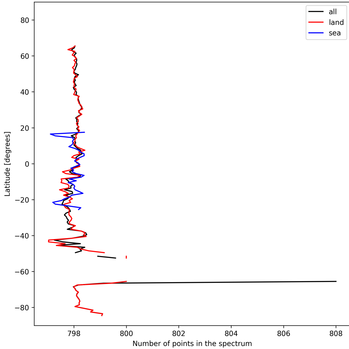
Figure 15: Zonal average of “Number of points in the spectrum” for 2025-02-22 to 2025-02-24.
