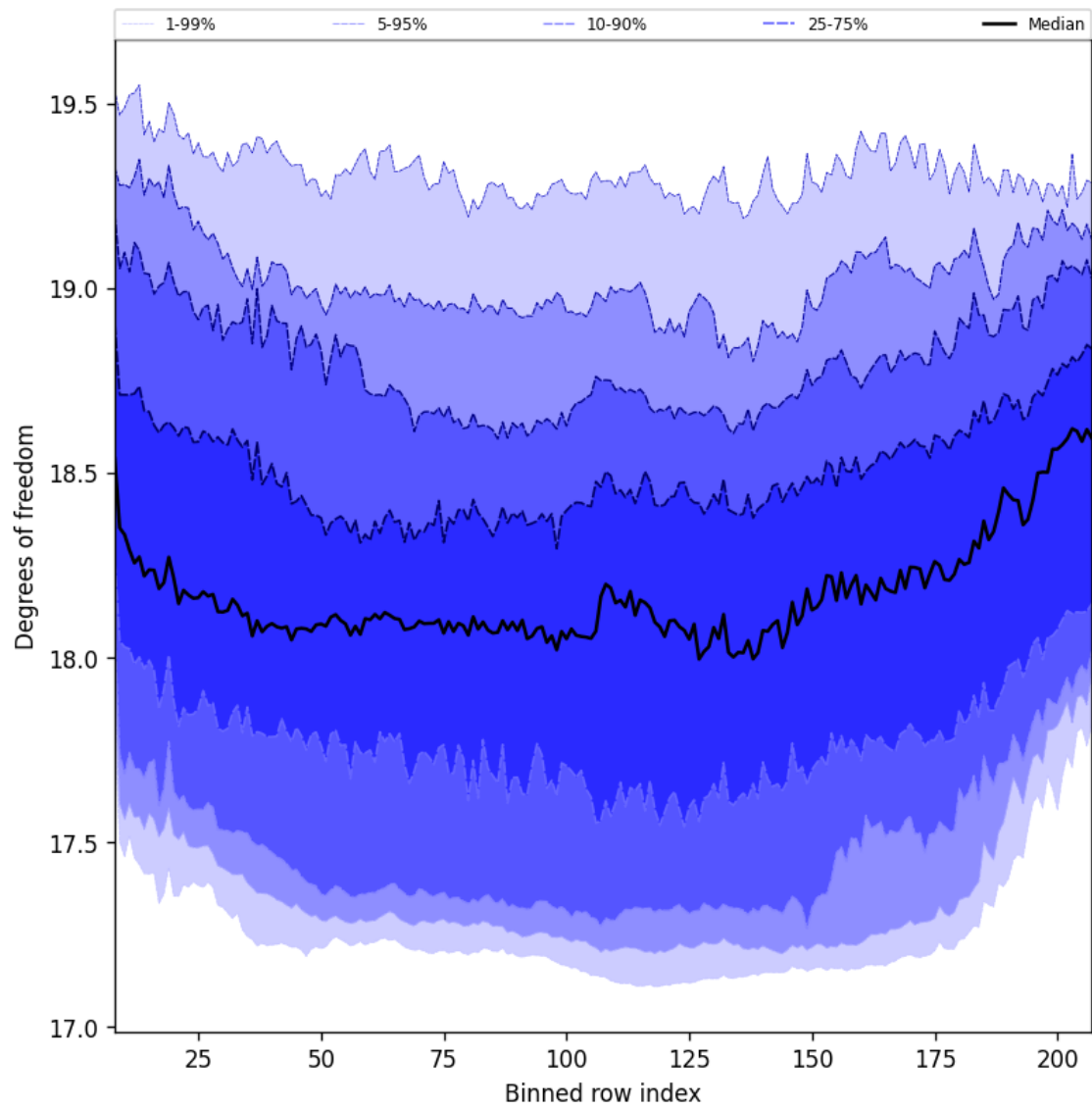
Figure 41: Along track statistics of “Degrees of freedom” for 2025-02-22 to 2025-02-24
