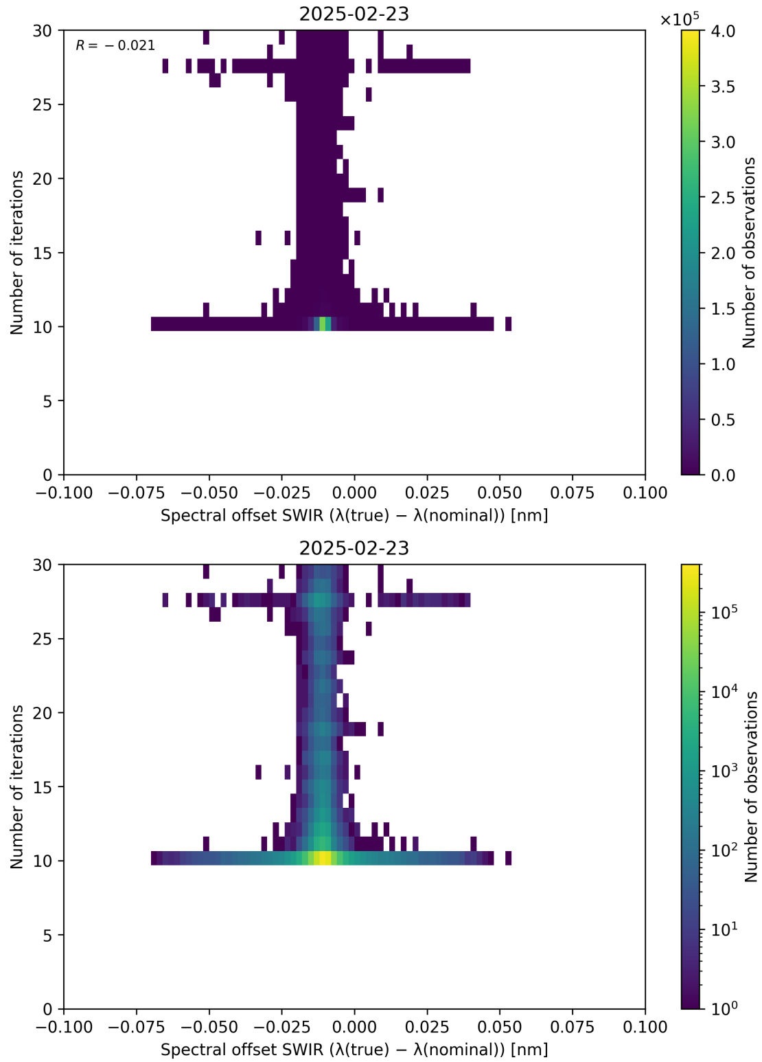
Figure 121: Scatter density plot of “Spectral offset SWIR ( \lambda_{\text{true}} - \lambda_{\text{nominal}} )” against “Number of iterations” for 2025-02-22 to 2025-02-24.
