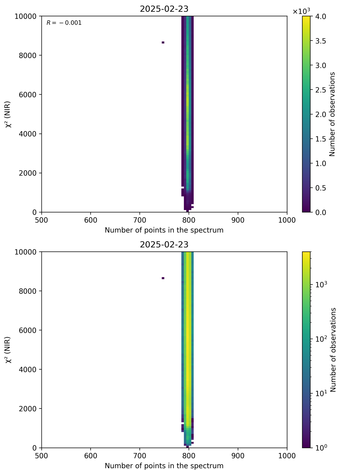
Figure 88: Scatter density plot of “Number of points in the spectrum” against “ \chi^2 (NIR)” for 2025-02-22 to 2025-02-24.
