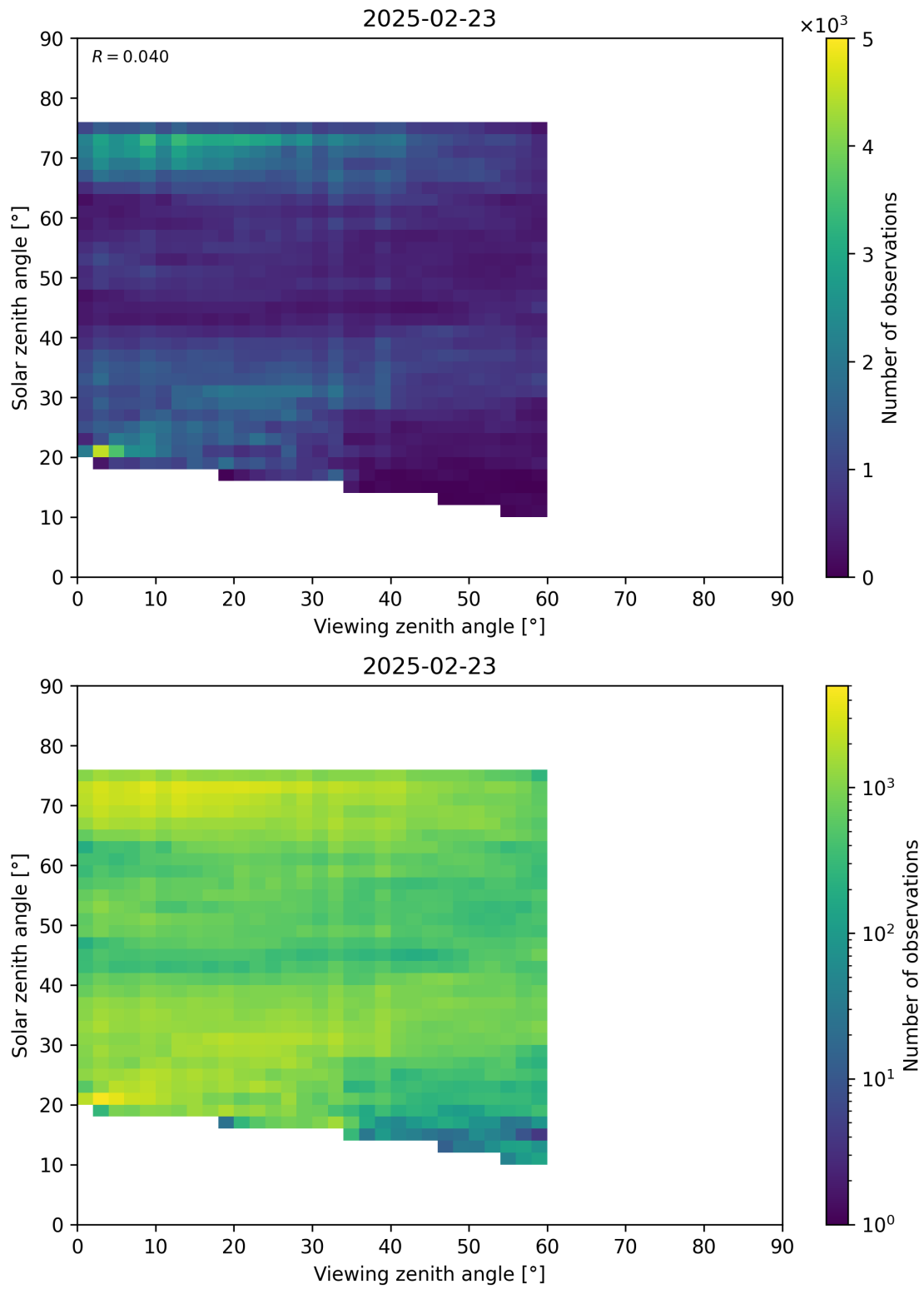
Figure 115: Scatter density plot of “Viewing zenith angle” against “Solar zenith angle” for 2025-02-22 to 2025-02-24.
