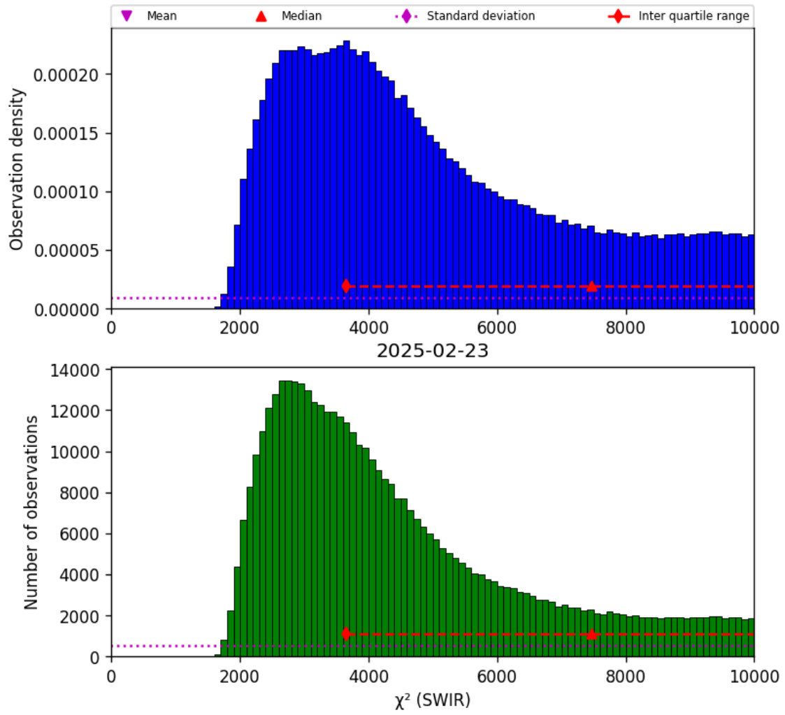
Figure 28: Histogram of “ \chi^2 (SWIR)” for 2025-02-22 to 2025-02-24
