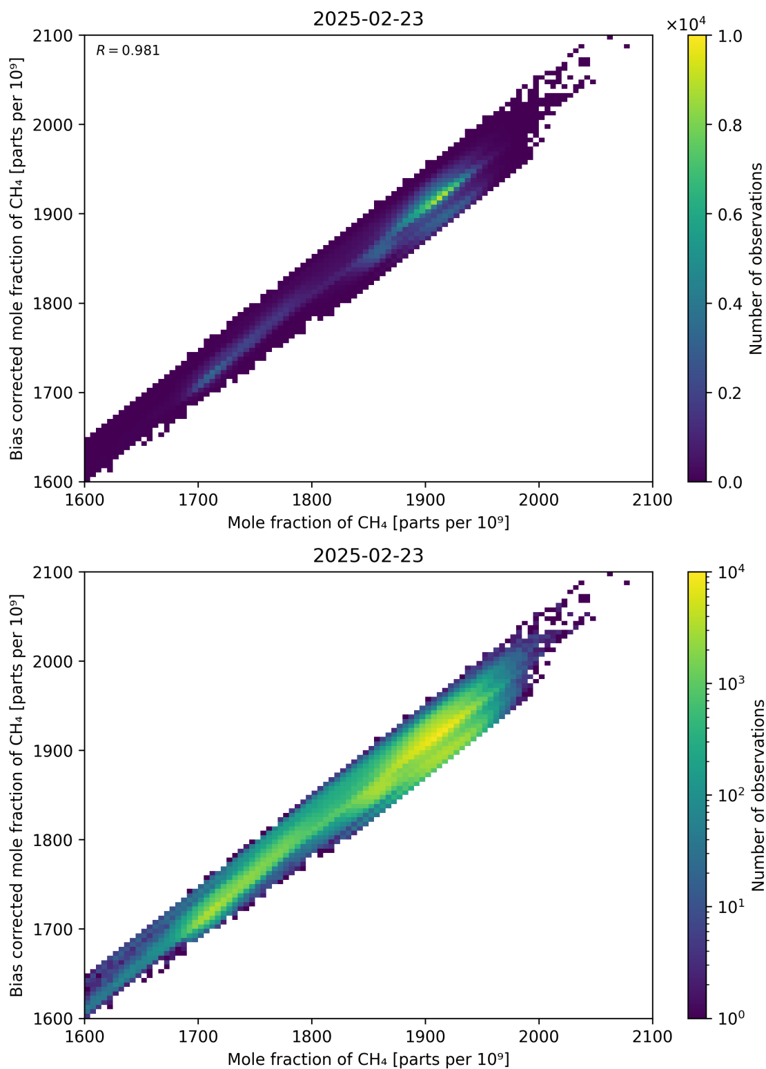
Figure 74: Scatter density plot of “Mole fraction of \text{CH}_4 ” against “Bias corrected mole fraction of \text{CH}_4 ” for 2025-02-22 to 2025-02-24.
