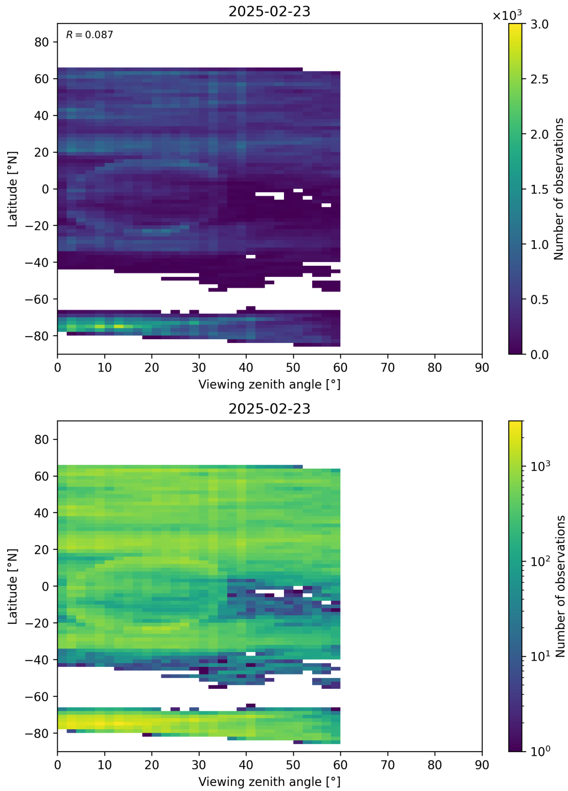
Figure 109: Scatter density plot of “Viewing zenith angle” against “Latitude” for 2025-02-22 to 2025-02-24.
