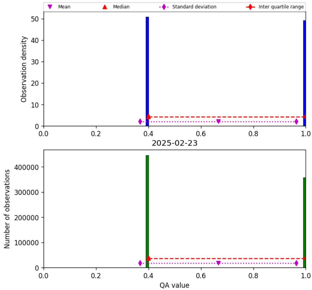
Figure 22: Histogram of “QA value” for 2025-02-22 to 2025-02-24
