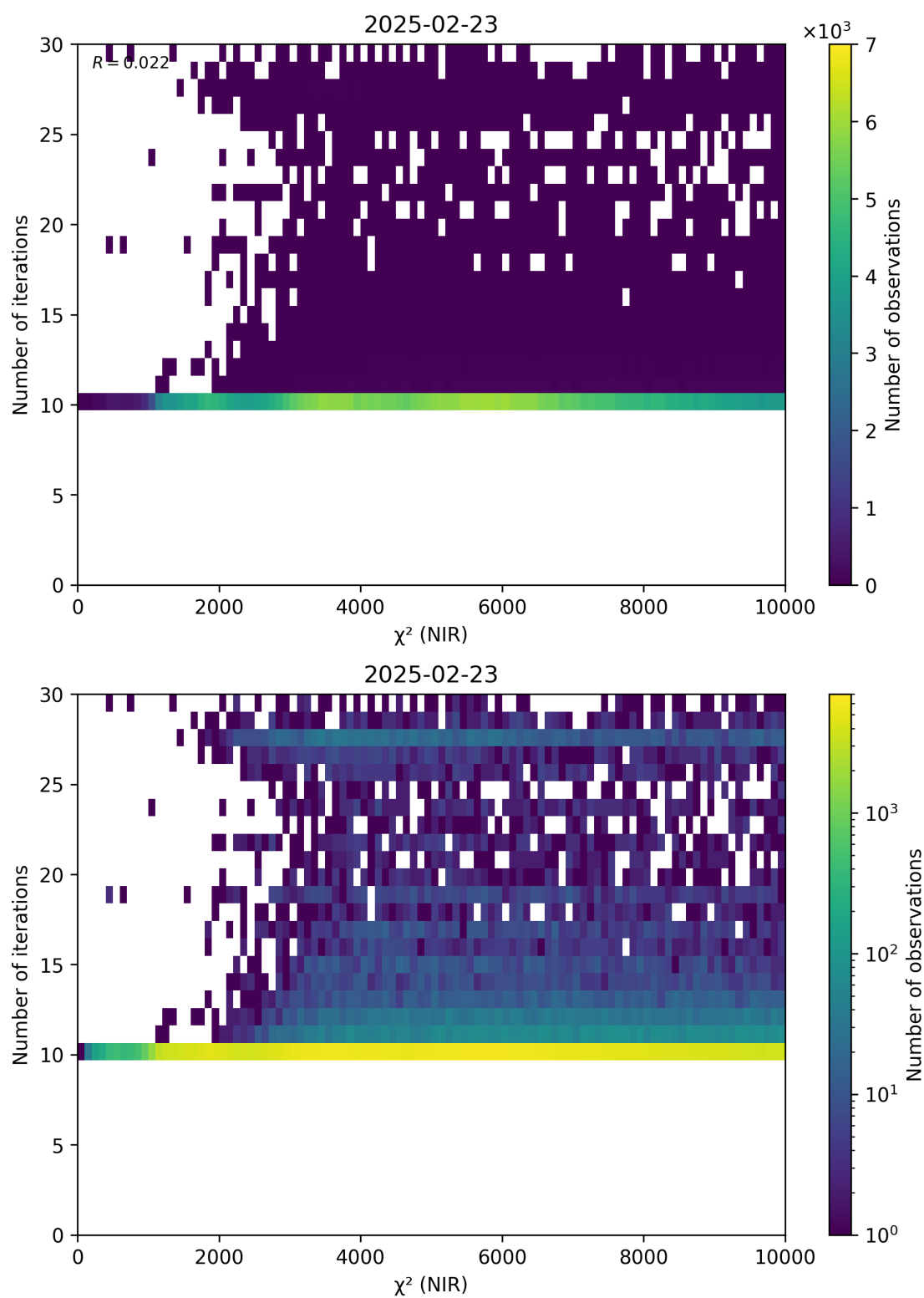
Figure 46: Scatter density plot of “ \chi^2 (NIR)” against “Number of iterations” for 2025-02-22 to 2025-02-24.
