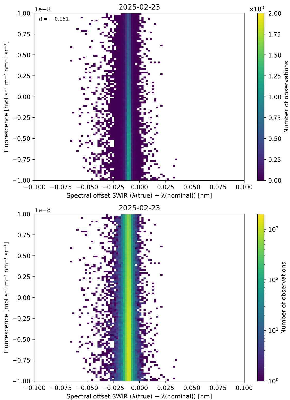
Figure 120: Scatter density plot of “Spectral offset SWIR ( \lambda_{\text{true}} - \lambda_{\text{nominal}} )” against “Fluorescence” for 2025-02-22 to 2025-02-24.
