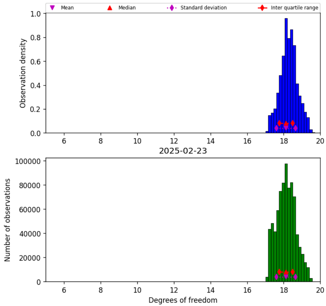
Figure 30: Histogram of “Degrees of freedom” for 2025-02-22 to 2025-02-24
