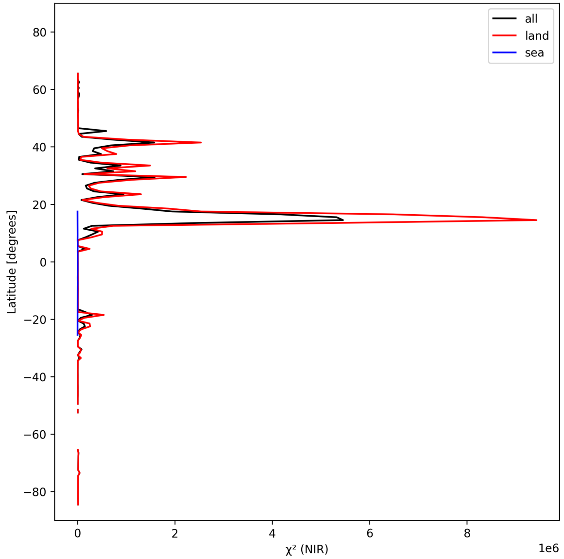
Figure 18: Zonal average of “ \chi^2 (NIR)” for 2025-02-22 to 2025-02-24.
