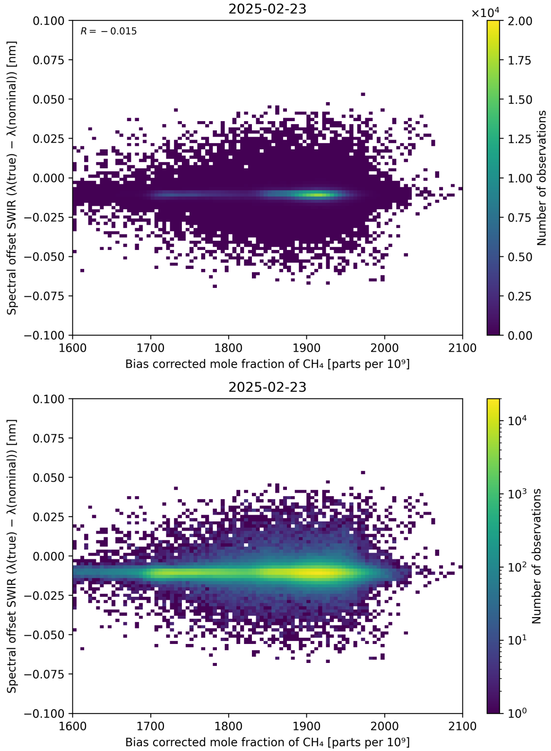
Figure 69: Scatter density plot of “Bias corrected mole fraction of \text{CH}_4 ” against “Spectral offset SWIR ( \lambda_{\text{true}} - \lambda_{\text{nominal}} )” for 2025-02-22 to 2025-02-24.
