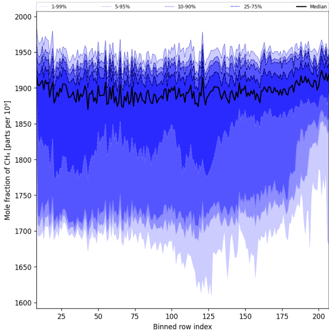
Figure 34: Along track statistics of “Mole fraction of CH 4 ” for 2025-02-22 to 2025-02-24
