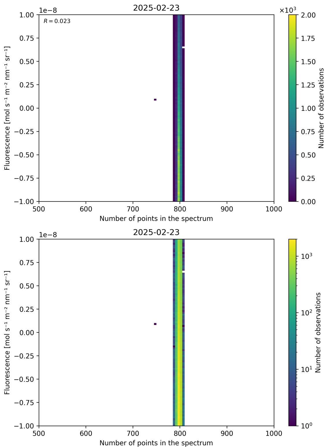
Figure 91: Scatter density plot of “Number of points in the spectrum” against “Fluorescence” for 2025-02-22 to 2025-02-24.
