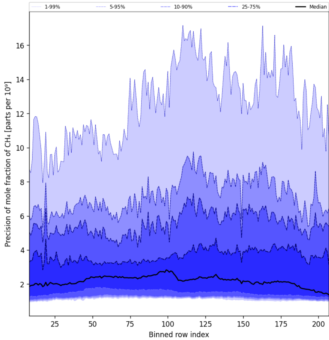
Figure 35: Along track statistics of “Precision of mole fraction of CH 4 ” for 2025-02-22 to 2025-02-24
