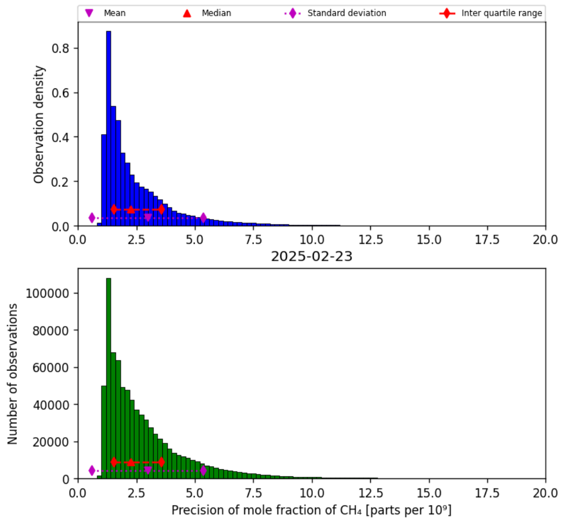
Figure 24: Histogram of “Precision of mole fraction of CH 4 ” for 2025-02-22 to 2025-02-24
