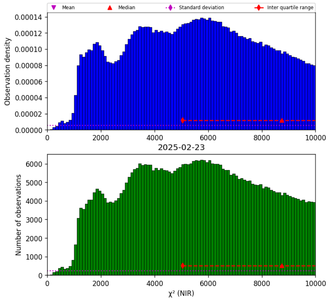
Figure 29: Histogram of " \chi^2 (NIR)" for 2025-02-22 to 2025-02-24
