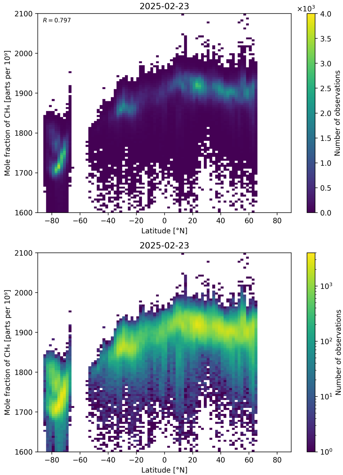
Figure 57: Scatter density plot of “Latitude” against “Mole fraction of CH 4 ” for 2025-02-22 to 2025-02-24.
