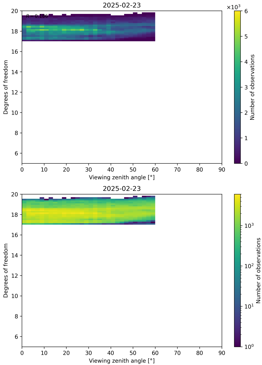
Figure 107: Scatter density plot of “Viewing zenith angle” against “Degrees of freedom” for 2025-02-22 to 2025-02-24.
