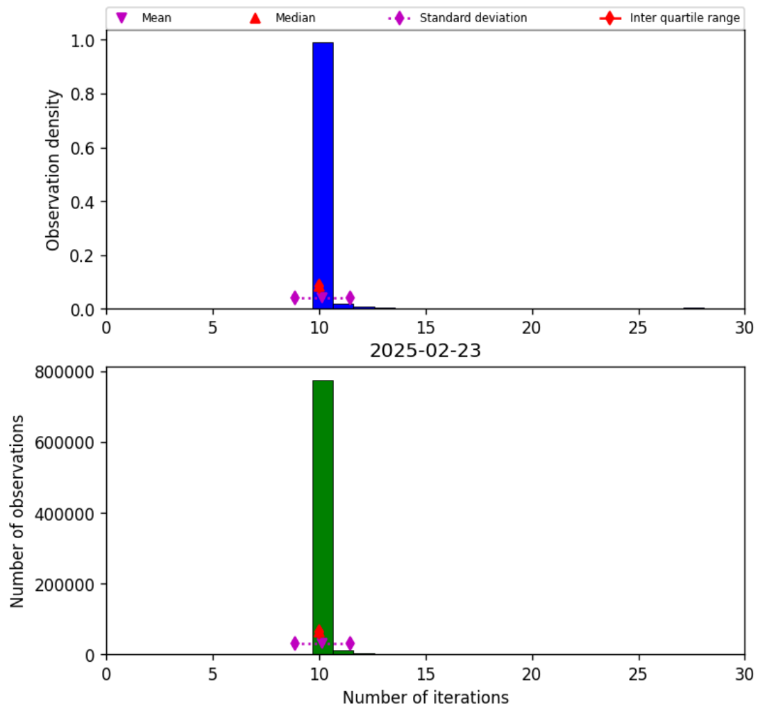
Figure 31: Histogram of “Number of iterations” for 2025-02-22 to 2025-02-24
