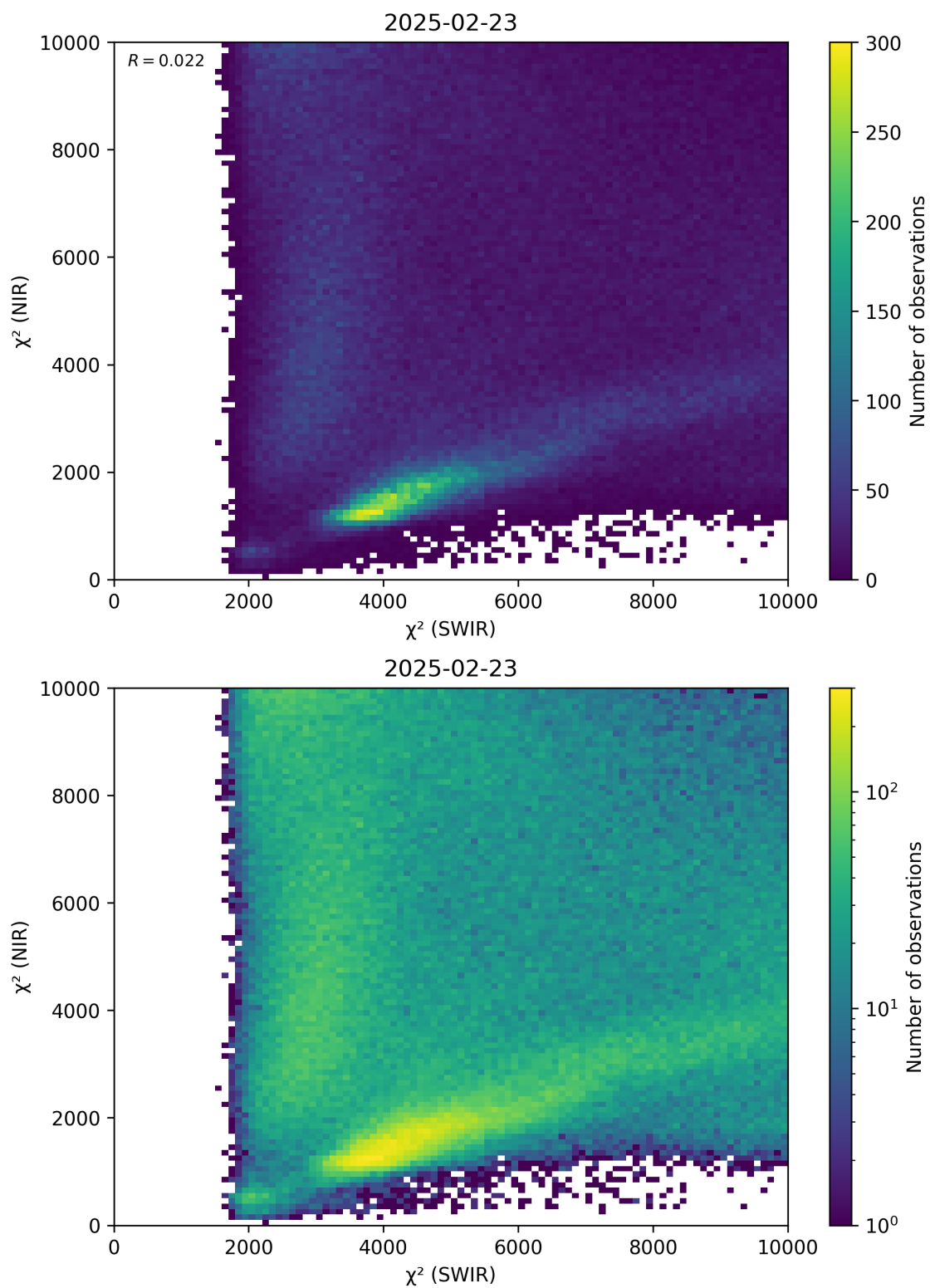
Figure 47: Scatter density plot of “ \chi^2 (SWIR)” against “ \chi^2 (NIR)” for 2025-02-22 to 2025-02-24.
