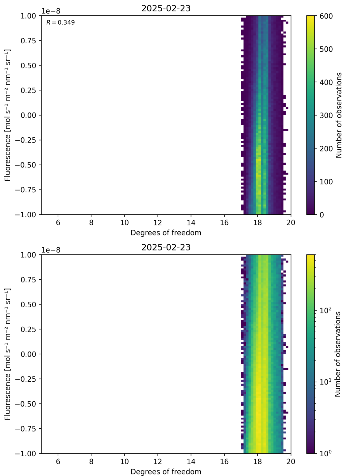
Figure 51: Scatter density plot of “Degrees of freedom” against “Fluorescence” for 2025-02-22 to 2025-02-24.
