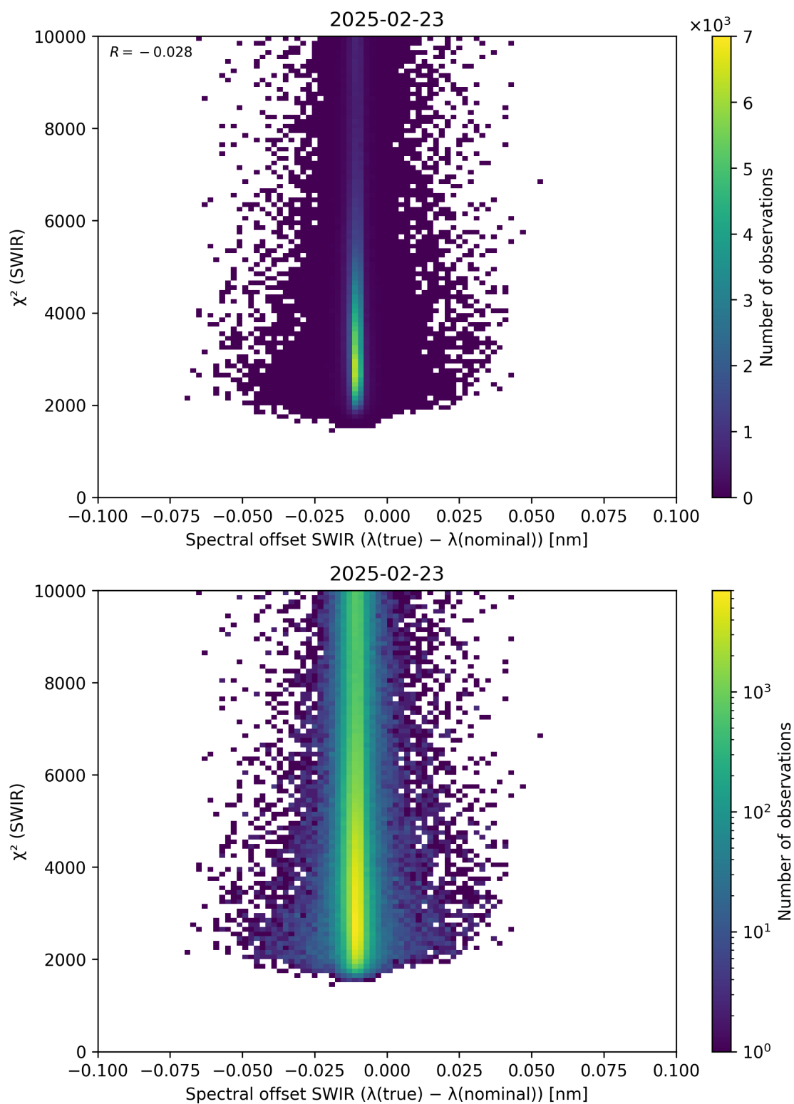
Figure 118: Scatter density plot of “Spectral offset SWIR ( \lambda_{\text{true}} - \lambda_{\text{nominal}} )” against “ \chi^2 (SWIR)” for 2025-02-22 to 2025-02-24.
