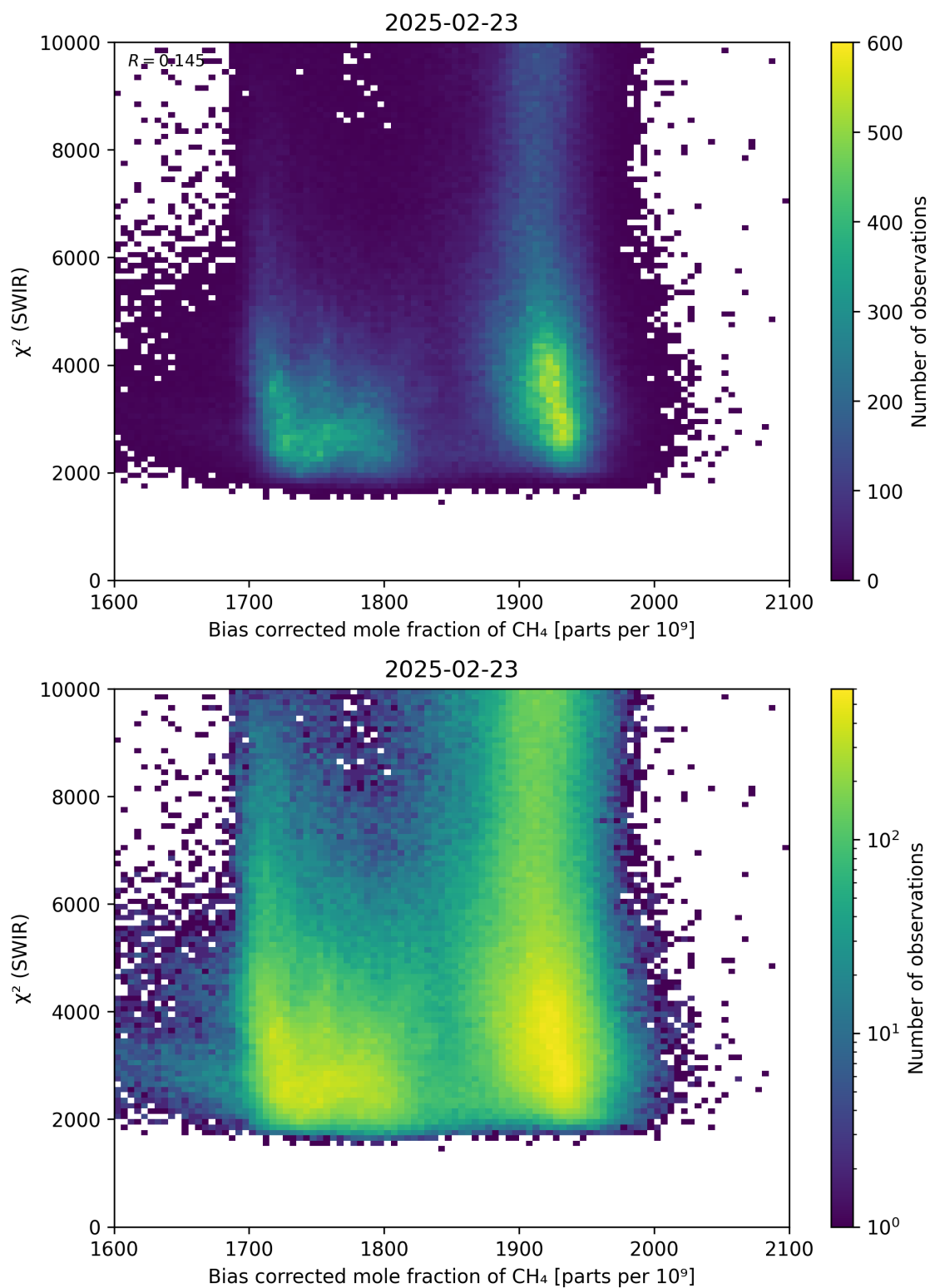
Figure 64: Scatter density plot of “Bias corrected mole fraction of CH 4 ” against “ \chi^2 (SWIR)” for 2025-02-22 to 2025-02-24.
