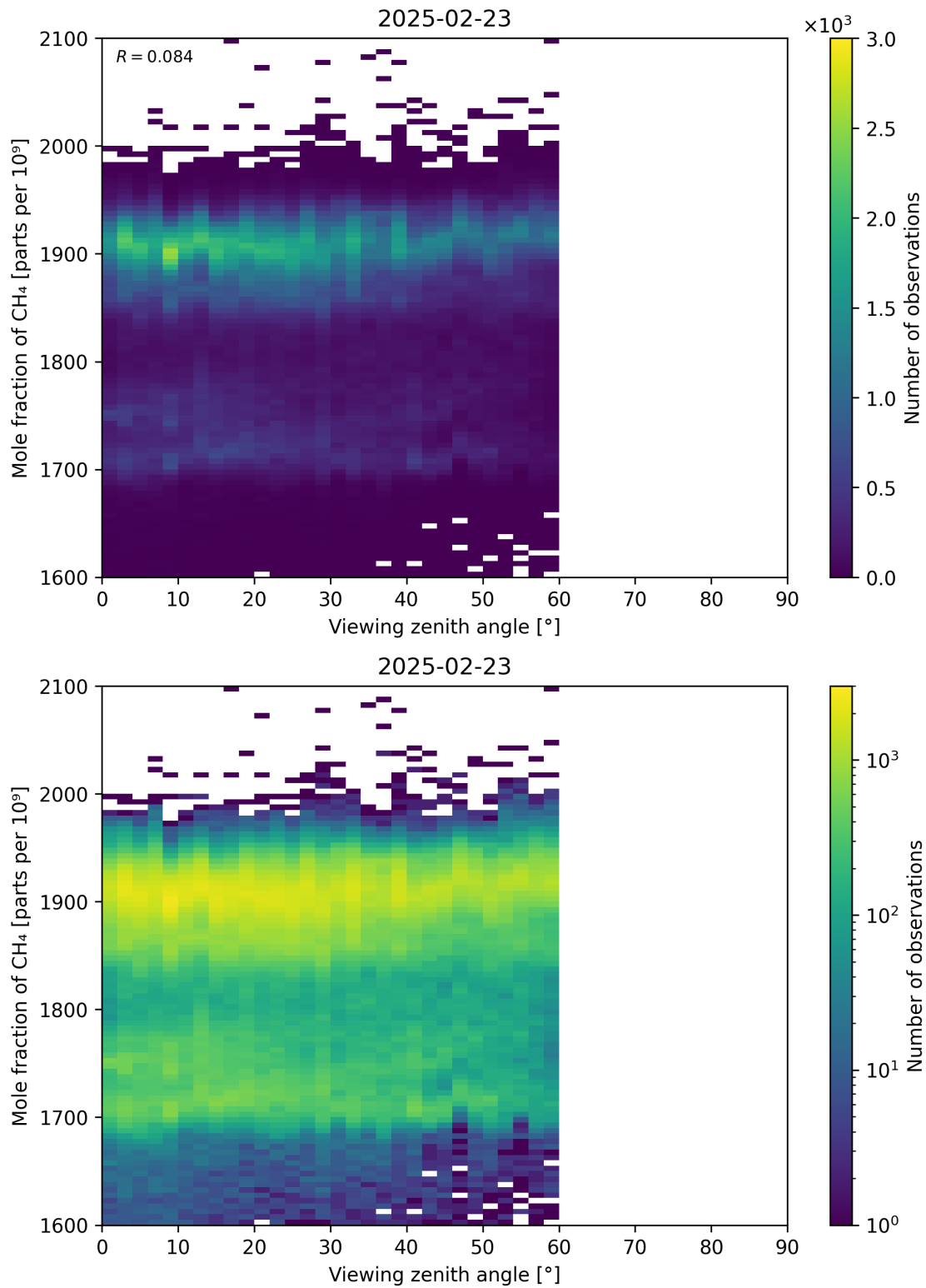
Figure 110: Scatter density plot of “Viewing zenith angle” against “Mole fraction of CH 4 ” for 2025-02-22 to 2025-02-24.
