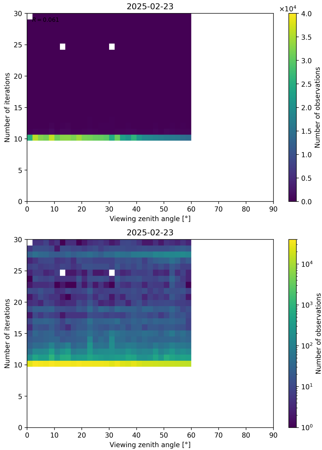
Figure 113: Scatter density plot of “Viewing zenith angle” against “Number of iterations” for 2025-02-22 to 2025-02-24.
