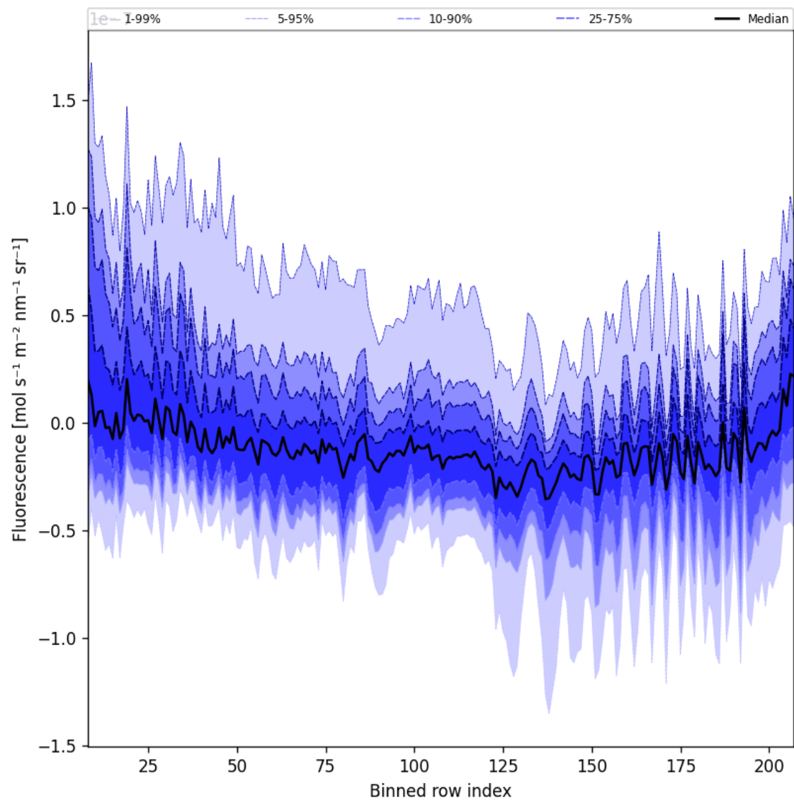
Figure 43: Along track statistics of “Fluorescence” for 2025-02-22 to 2025-02-24
