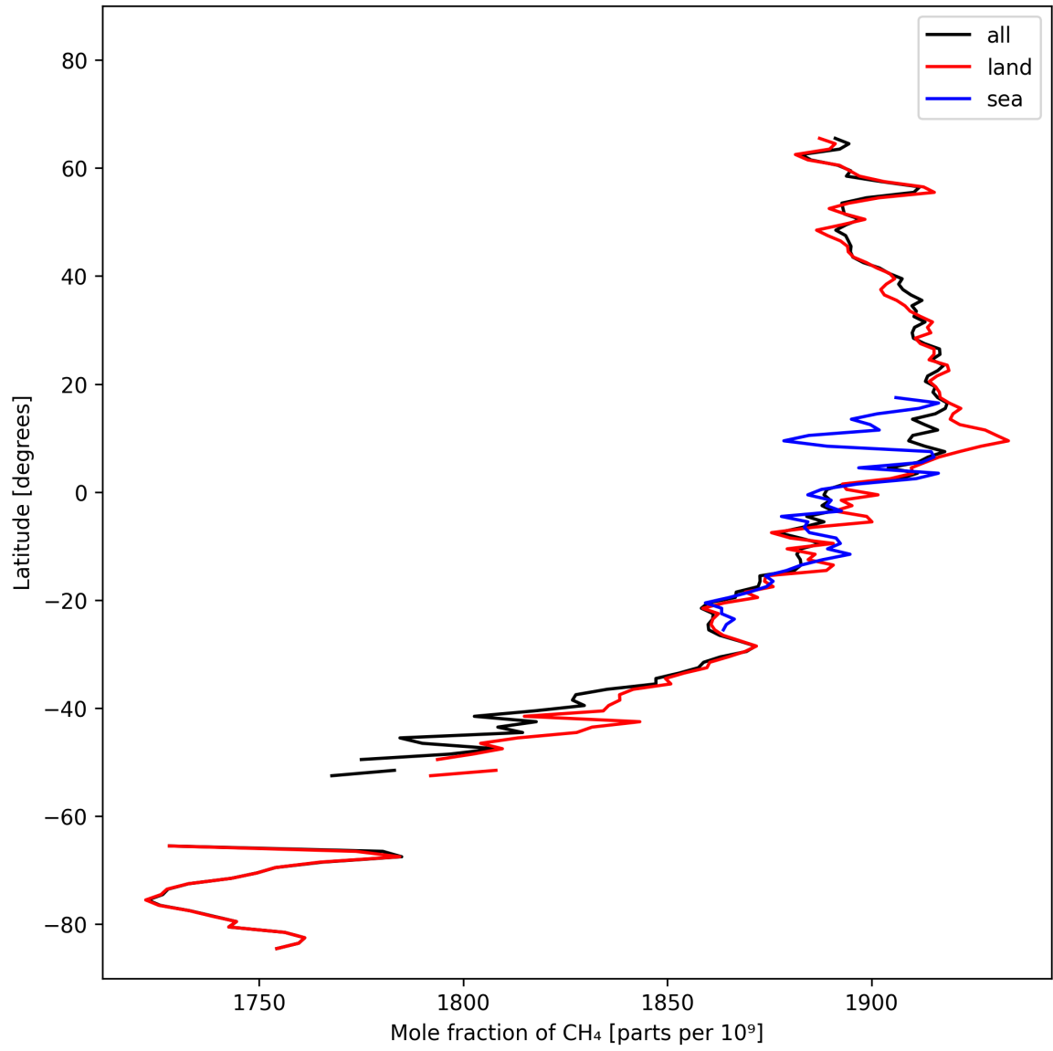
Figure 12: Zonal average of “Mole fraction of CH 4 ” for 2025-02-22 to 2025-02-24.
