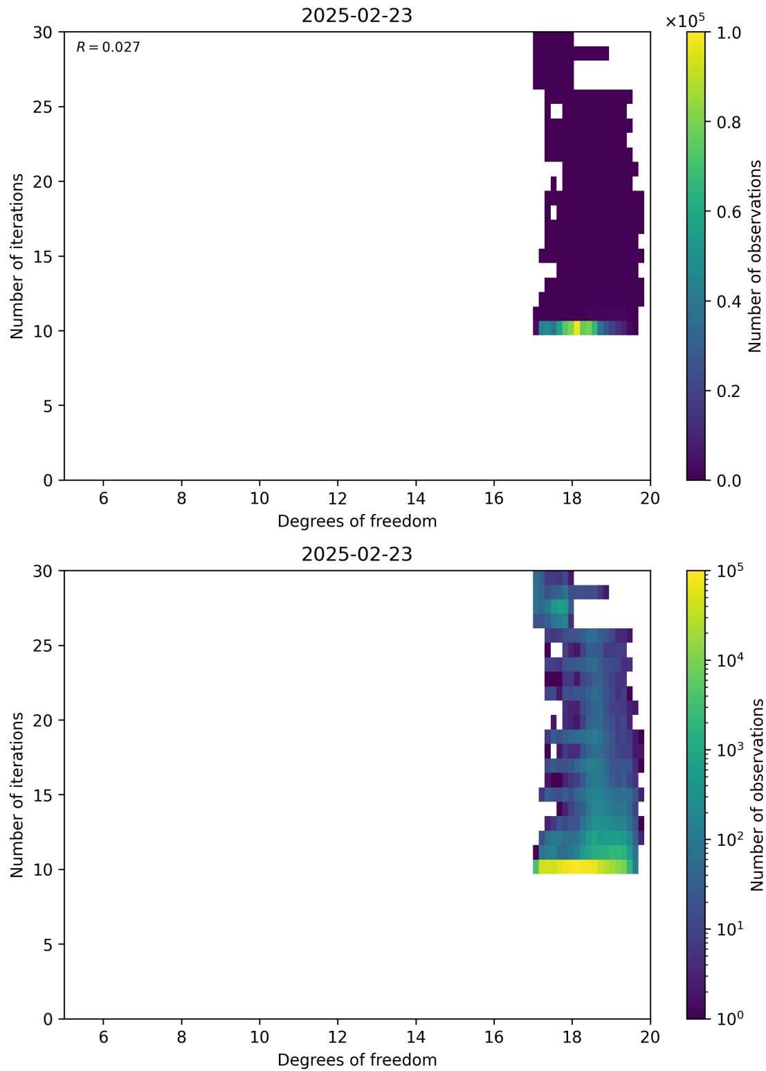
Figure 52: Scatter density plot of “Degrees of freedom” against “Number of iterations” for 2025-02-22 to 2025-02-24.
