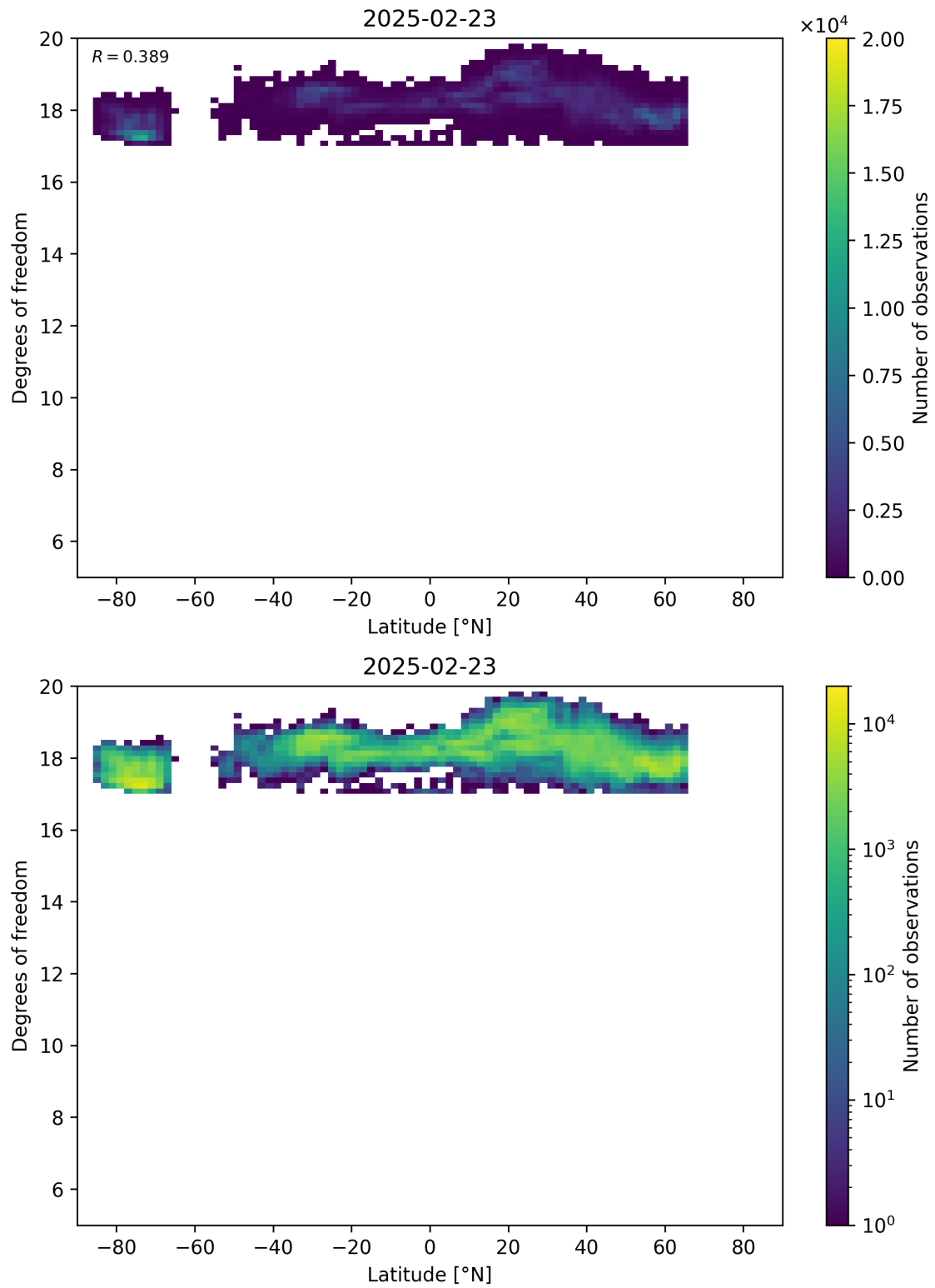
Figure 55: Scatter density plot of “Latitude” against “Degrees of freedom” for 2025-02-22 to 2025-02-24.
