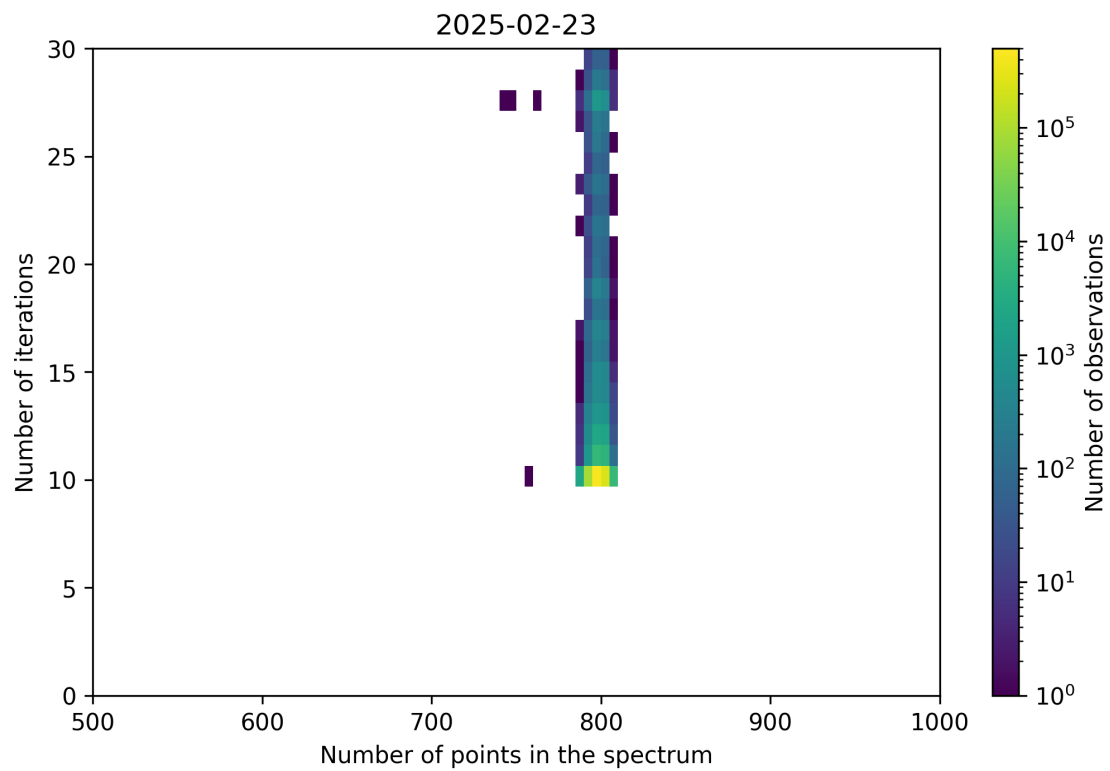
Figure 92: Scatter density plot of “Number of points in the spectrum” against “Number of iterations” for 2025-02-22 to 2025-02-24.
