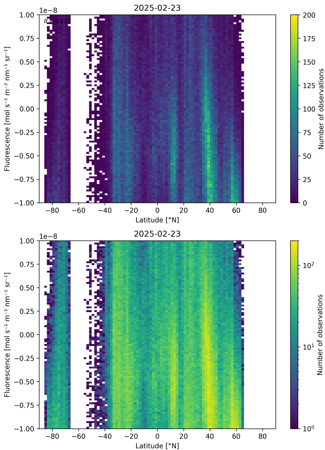
Figure 56: Scatter density plot of “Latitude” against “Fluorescence” for 2025-02-22 to 2025-02-24.
