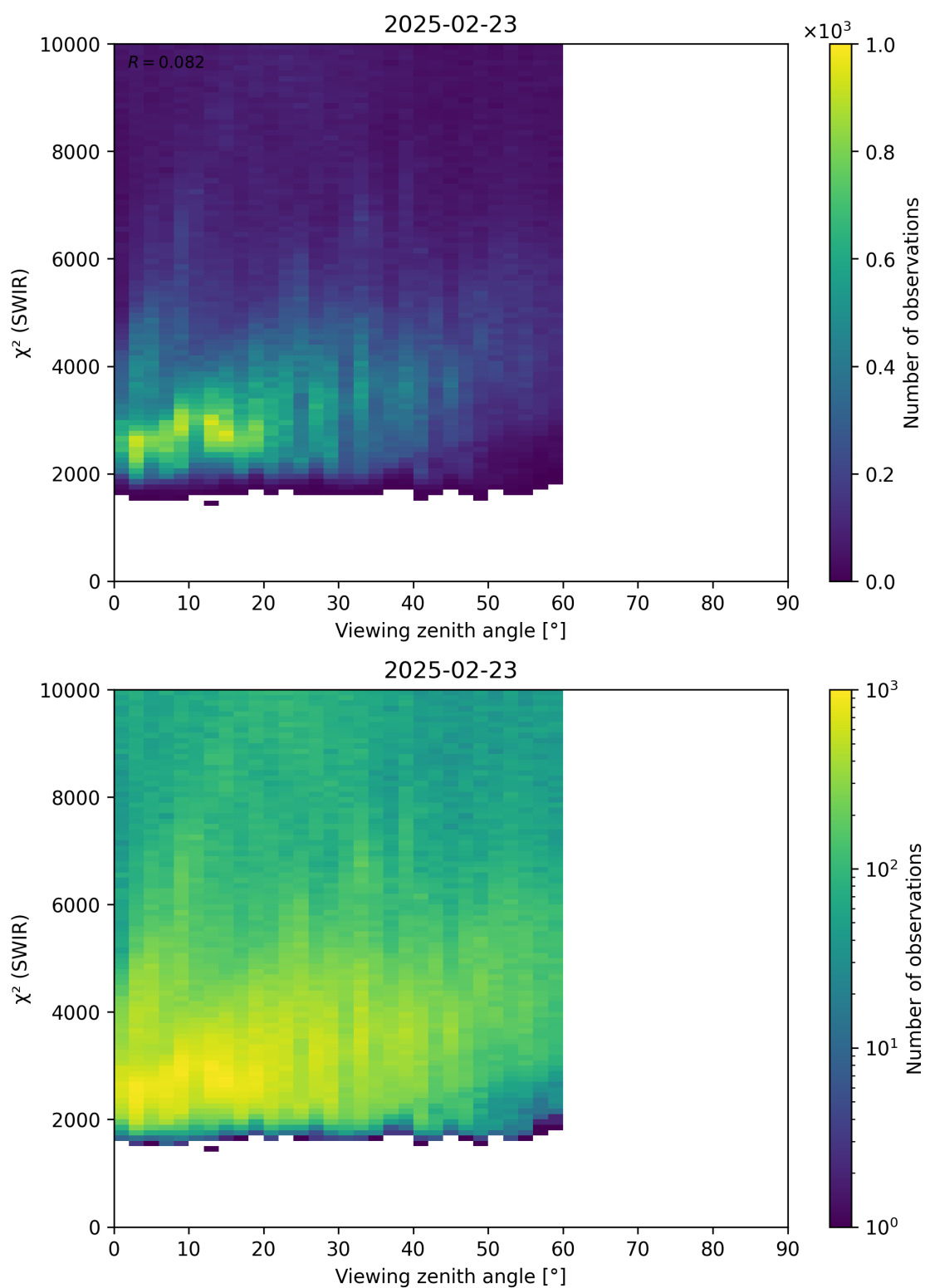
Figure 106: Scatter density plot of “Viewing zenith angle” against “ \chi^2 (SWIR)” for 2025-02-22 to 2025-02-24.
