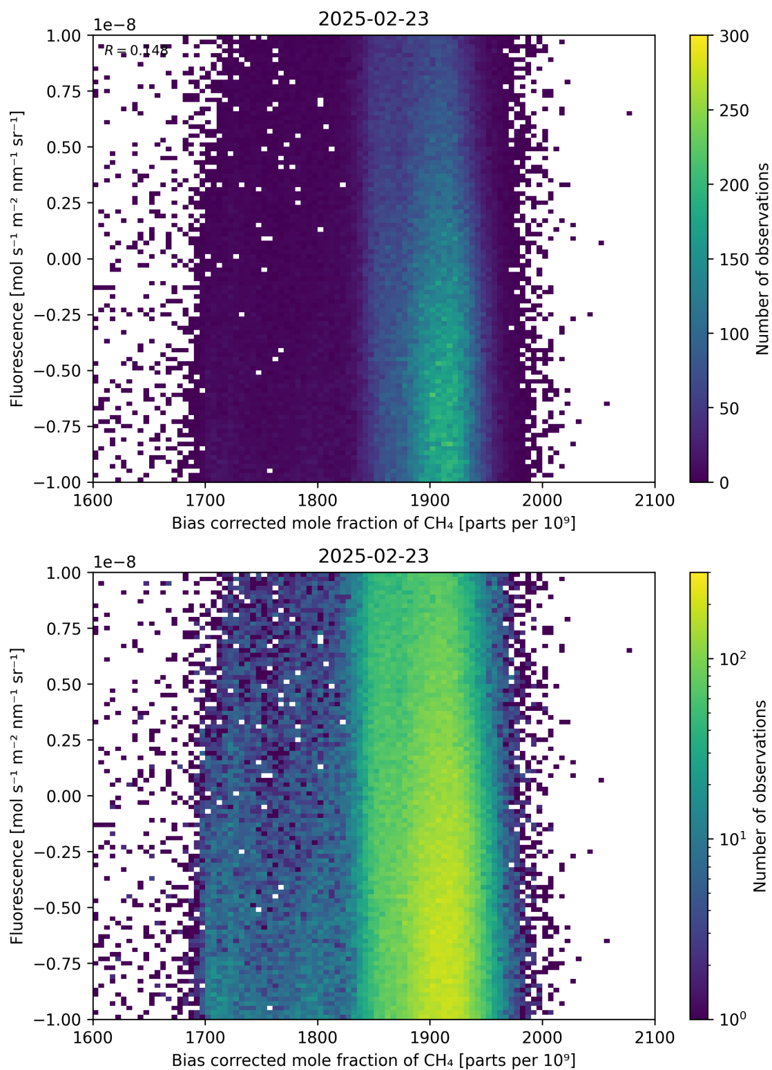
Figure 66: Scatter density plot of “Bias corrected mole fraction of \text{CH}_4 ” against “Fluorescence” for 2025-02-22 to 2025-02-24.
