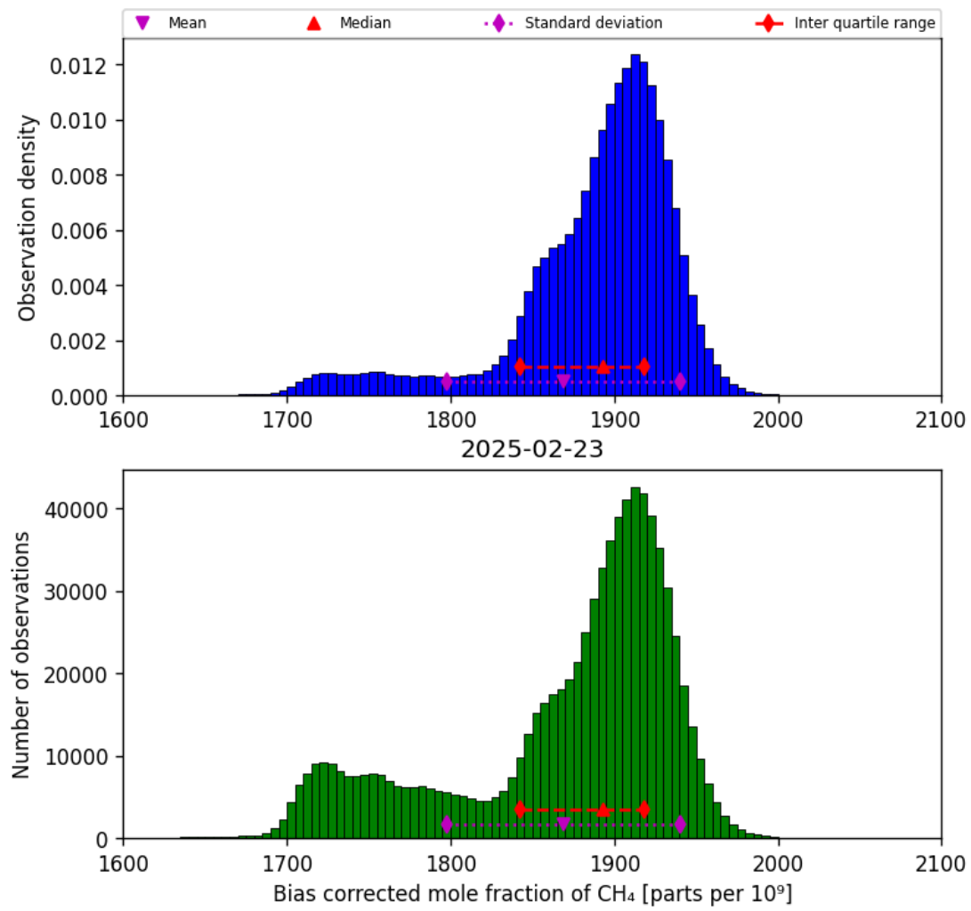
Figure 25: Histogram of “Bias corrected mole fraction of CH 4 ” for 2025-02-22 to 2025-02-24
