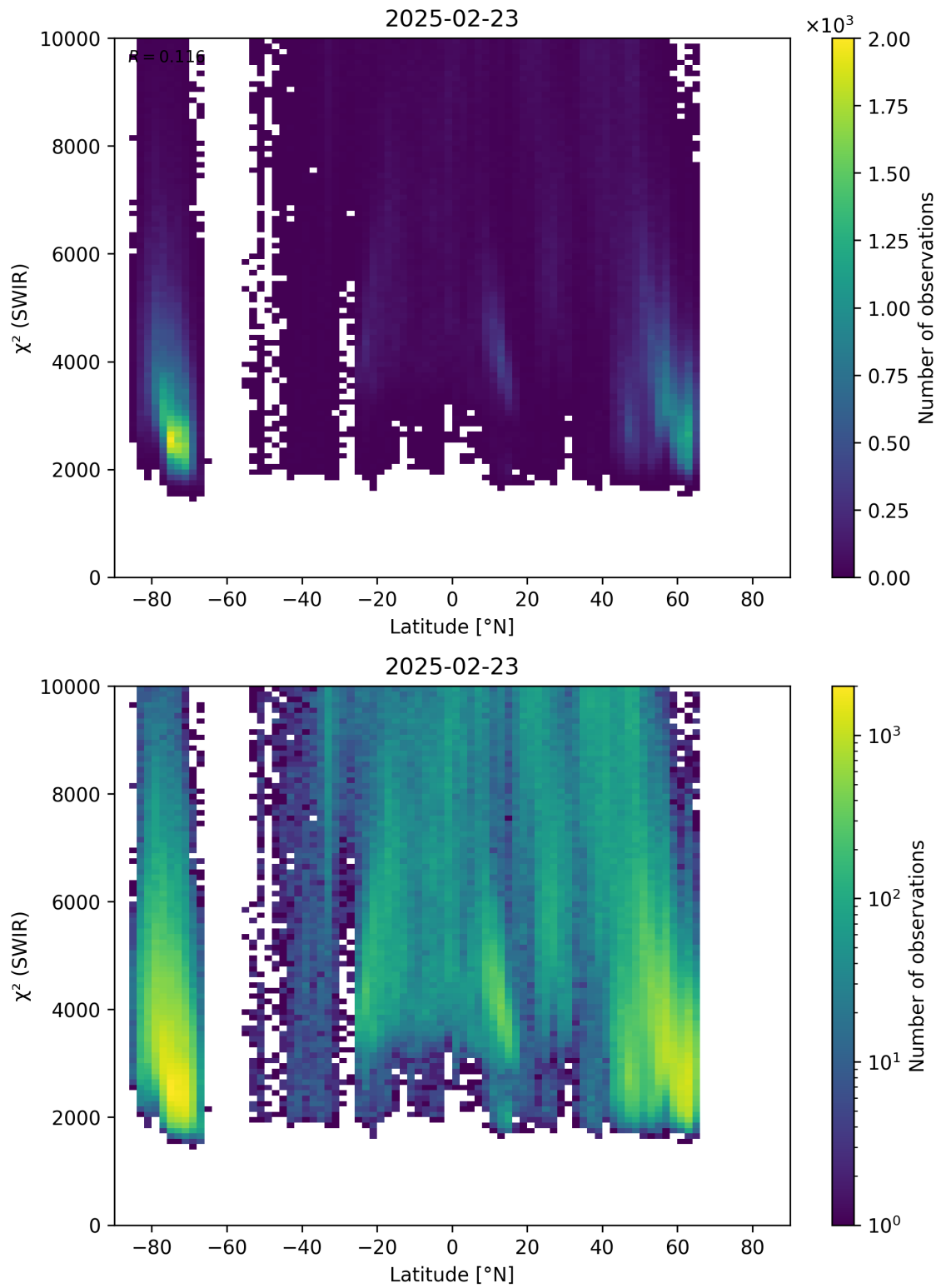
Figure 54: Scatter density plot of “Latitude” against “ \chi^2 (SWIR)” for 2025-02-22 to 2025-02-24.
