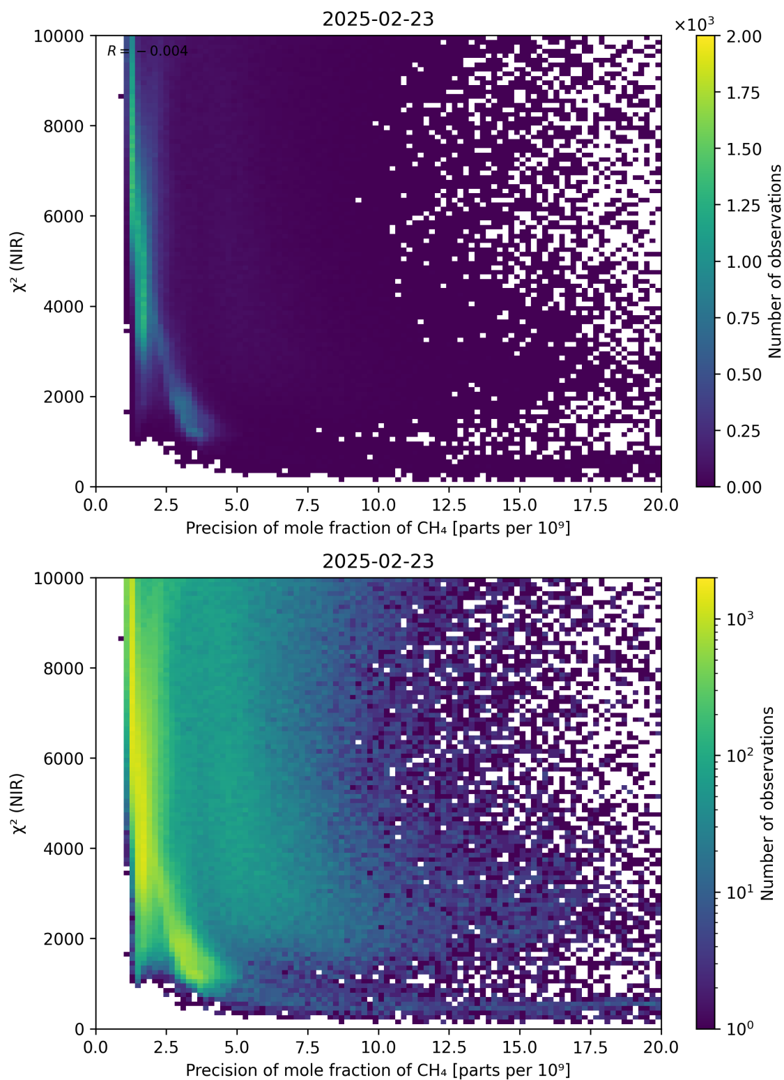
Figure 78: Scatter density plot of “Precision of mole fraction of CH 4 ” against “ \chi^2 (NIR)” for 2025-02-22 to 2025-02-24.
