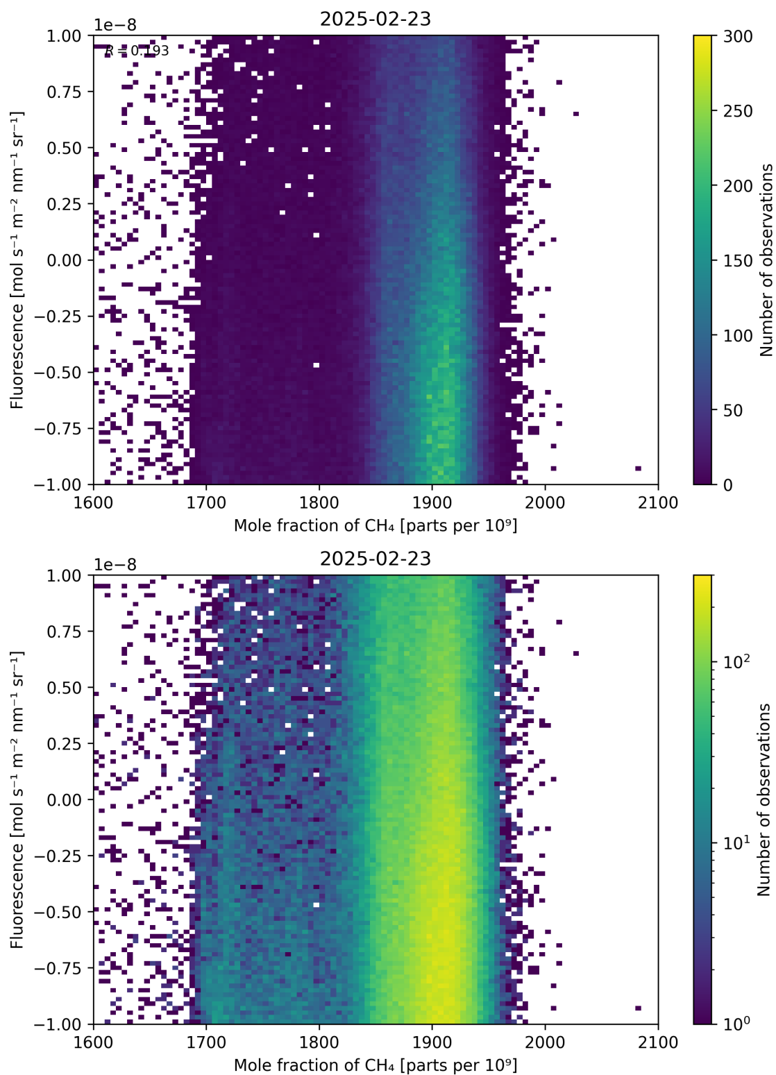
Figure 73: Scatter density plot of “Mole fraction of \text{CH}_4 ” against “Fluorescence” for 2025-02-22 to 2025-02-24.
