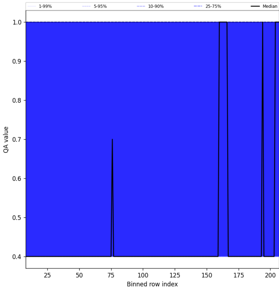
Figure 33: Along track statistics of “QA value” for 2025-02-22 to 2025-02-24
