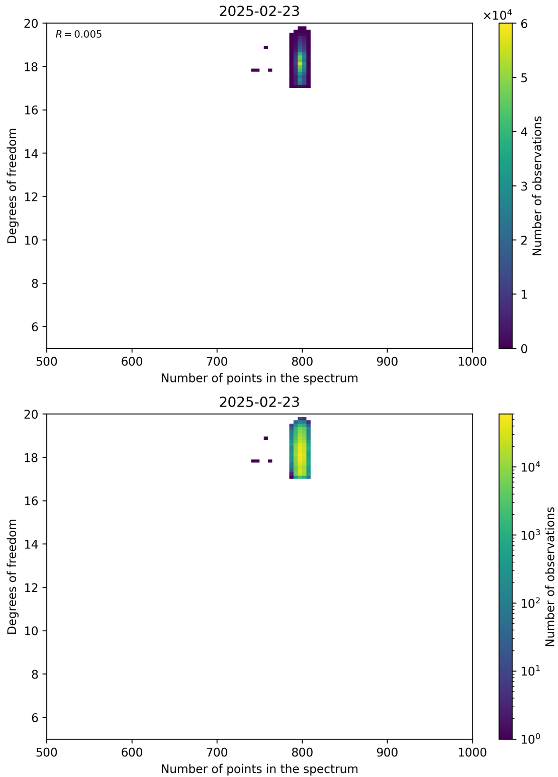
Figure 90: Scatter density plot of “Number of points in the spectrum” against “Degrees of freedom” for 2025-02-22 to 2025-02-24.
