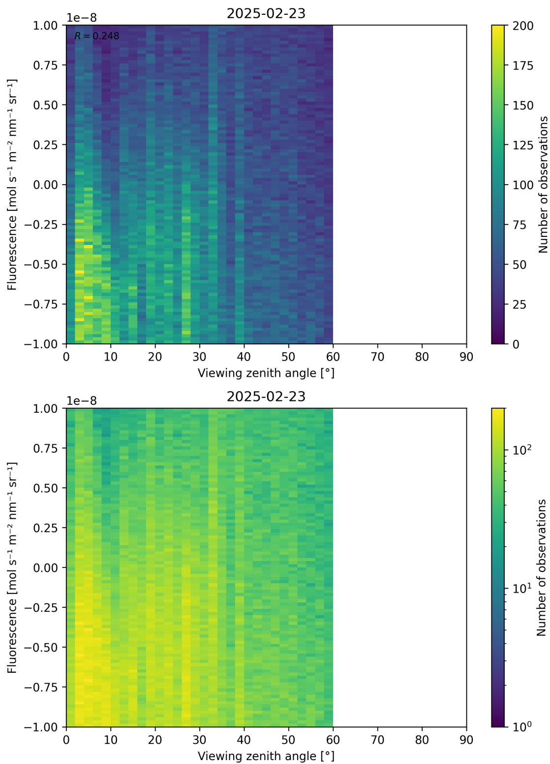
Figure 108: Scatter density plot of “Viewing zenith angle” against “Fluorescence” for 2025-02-22 to 2025-02-24.
