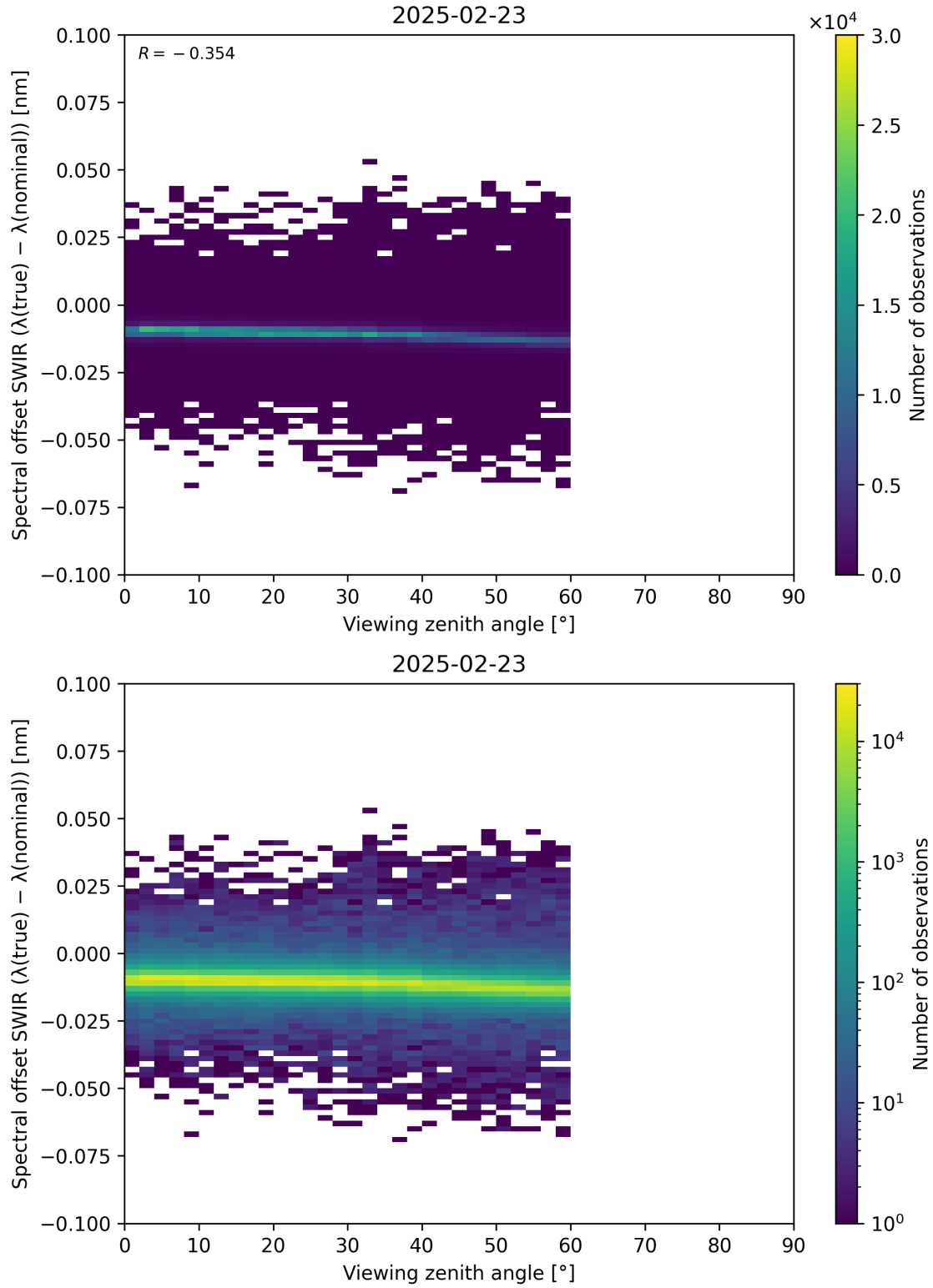
Figure 116: Scatter density plot of “Viewing zenith angle” against “Spectral offset SWIR ( \lambda_{\text{true}} - \lambda_{\text{nominal}} )” for 2025-02-22 to 2025-02-24.
