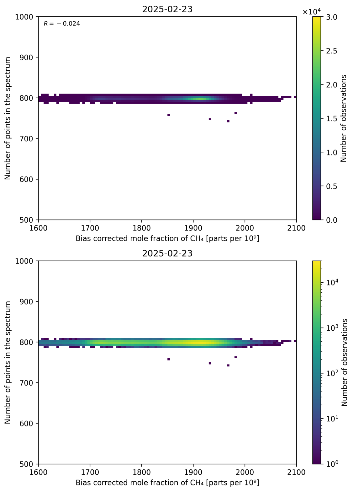
Figure 68: Scatter density plot of “Bias corrected mole fraction of CH 4 ” against “Number of points in the spectrum” for 2025-02-22 to 2025-02-24.
