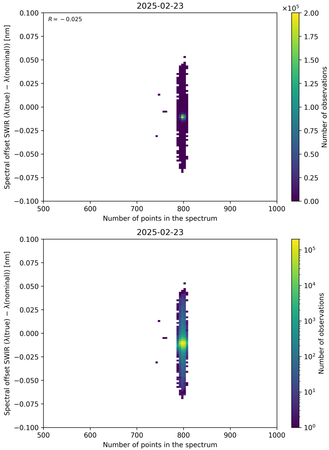
Figure 93: Scatter density plot of “Number of points in the spectrum” against “Spectral offset SWIR ( \lambda_{\text{true}} - \lambda_{\text{nominal}} )” for 2025-02-22 to 2025-02-24.
