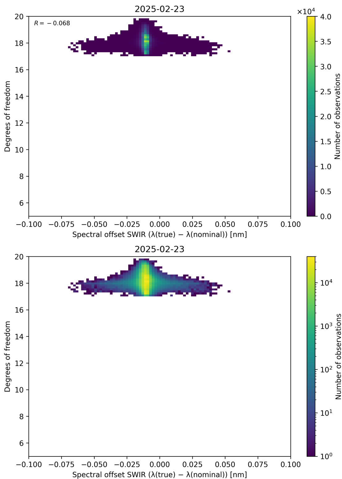
Figure 119: Scatter density plot of “Spectral offset SWIR ( \lambda_{\text{true}} - \lambda_{\text{nominal}} )” against “Degrees of freedom” for 2025-02-22 to 2025-02-24.
