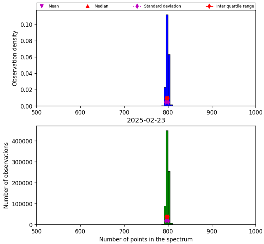
Figure 26: Histogram of “Number of points in the spectrum” for 2025-02-22 to 2025-02-24
