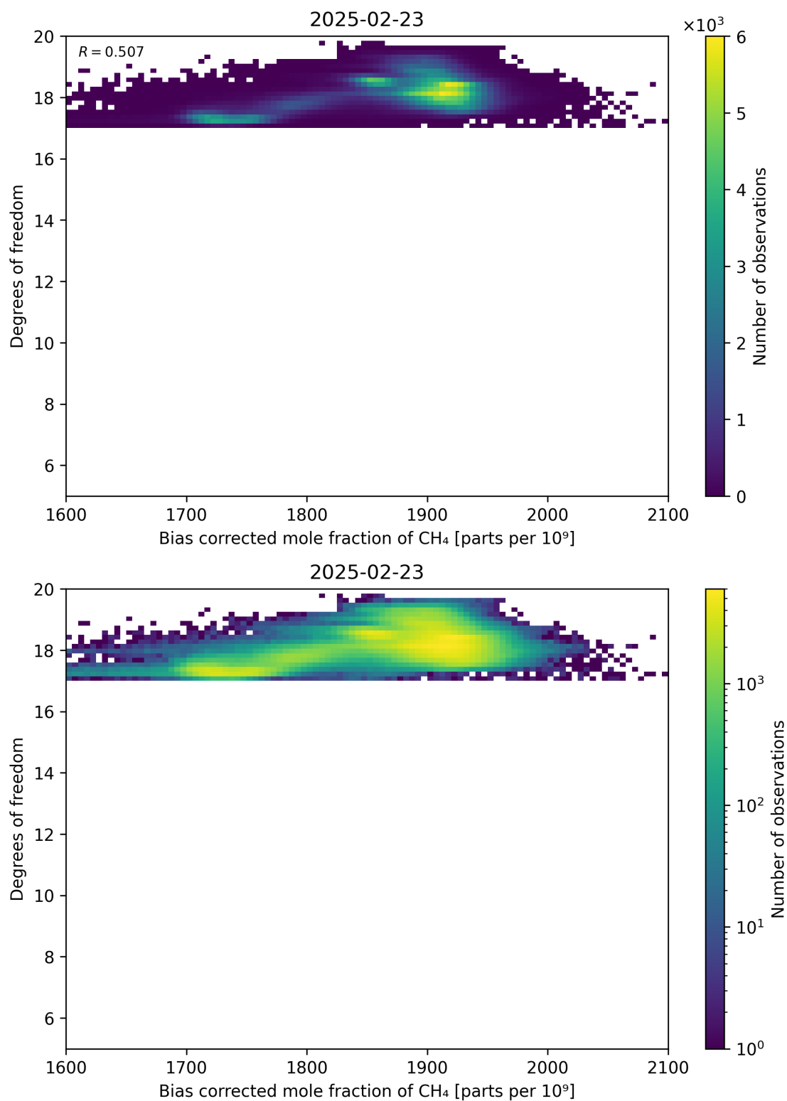
Figure 65: Scatter density plot of “Bias corrected mole fraction of CH 4 ” against “Degrees of freedom” for 2025-02-22 to 2025-02-24.
