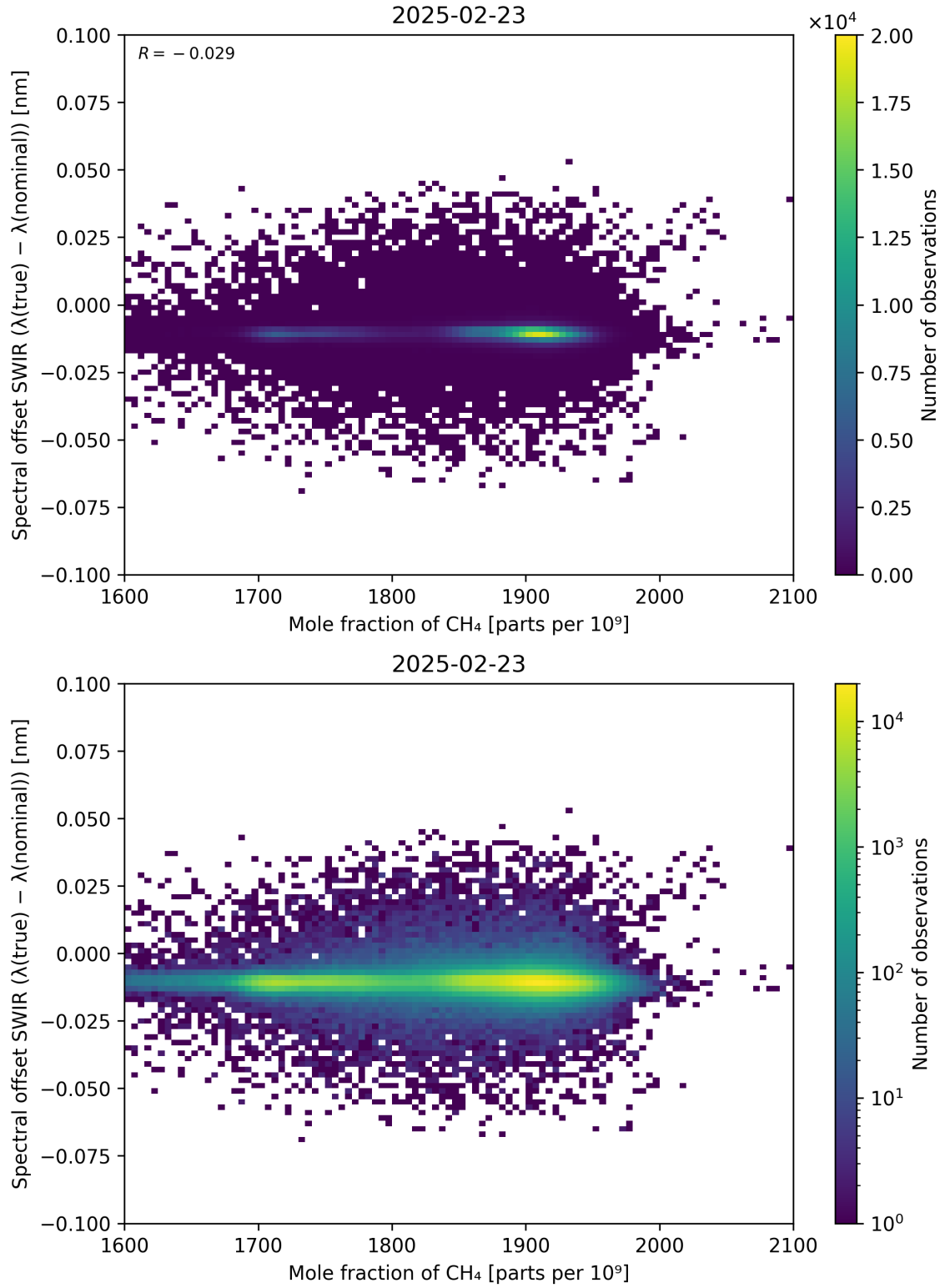
Figure 86: Scatter density plot of “Mole fraction of CH 4 ” against “Spectral offset SWIR ( \lambda_{\text{true}} - \lambda_{\text{nominal}} )” for 2025-02-22 to 2025-02-24.
