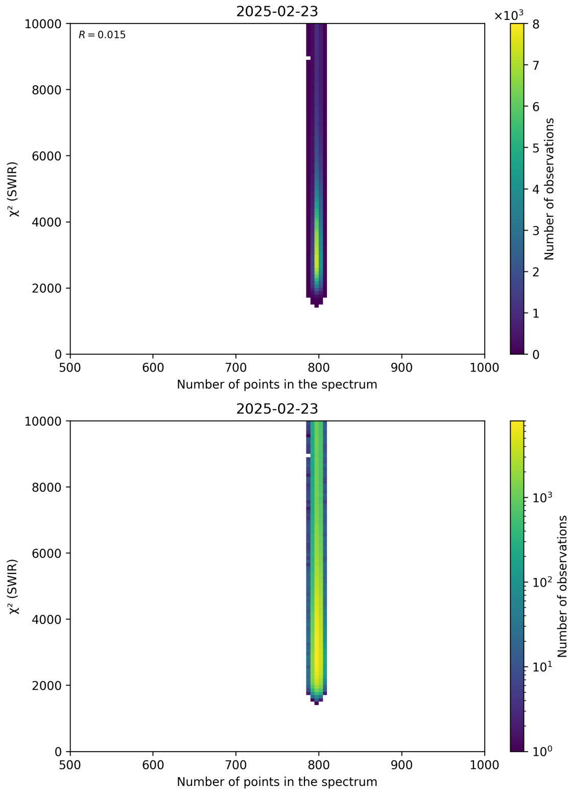
Figure 89: Scatter density plot of “Number of points in the spectrum” against “ \chi^2 (SWIR)” for 2025-02-22 to 2025-02-24.
