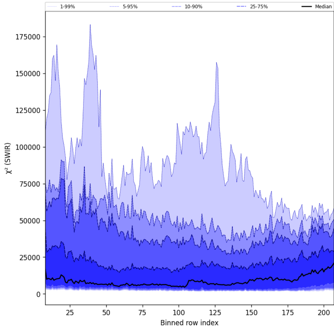
Figure 39: Along track statistics of “ \chi^2 (SWIR)” for 2025-02-22 to 2025-02-24
