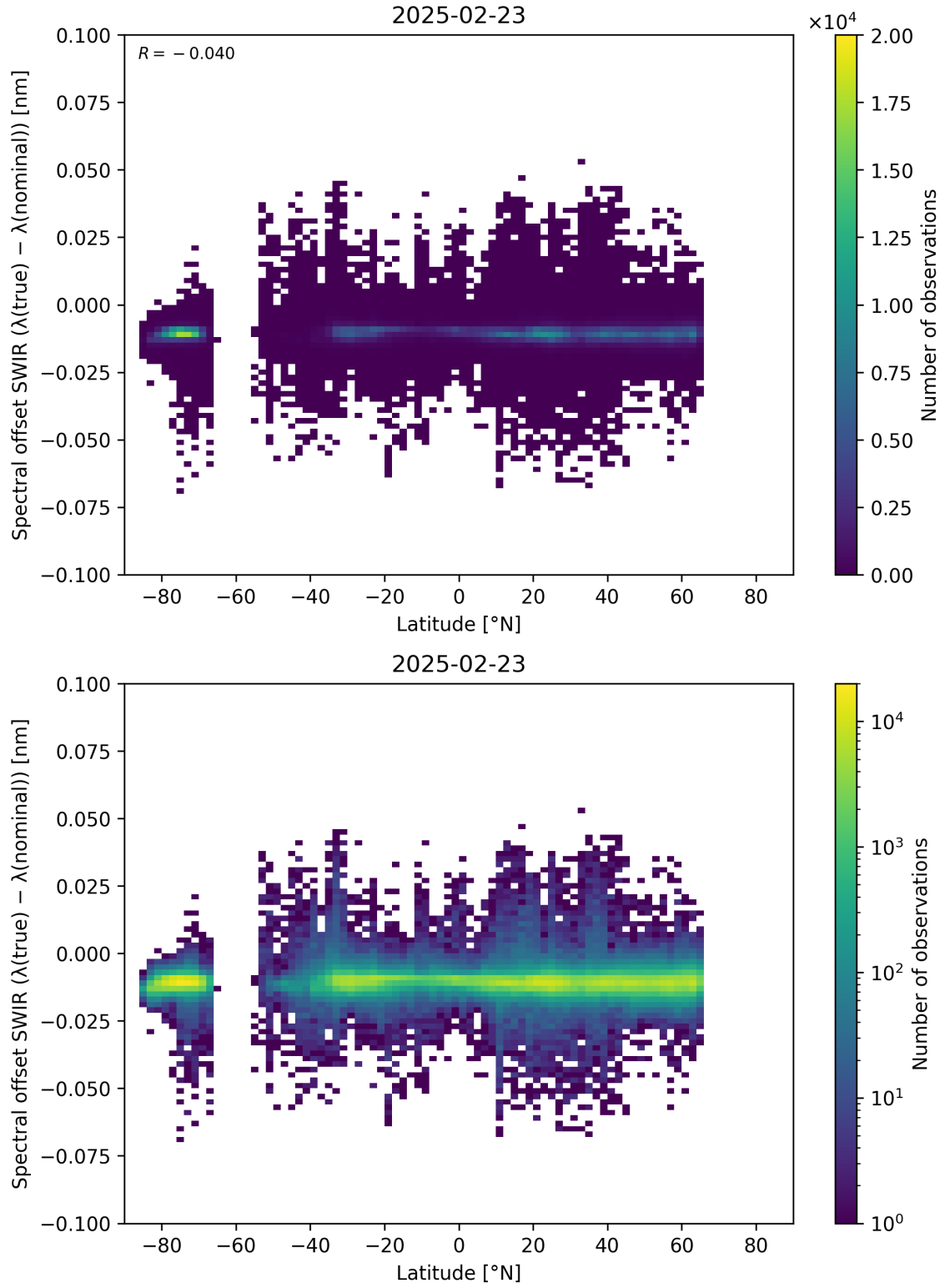
Figure 62: Scatter density plot of “Latitude” against “Spectral offset SWIR ( \lambda_{\text{true}} - \lambda_{\text{nominal}} )” for 2025-02-22 to 2025-02-24.
