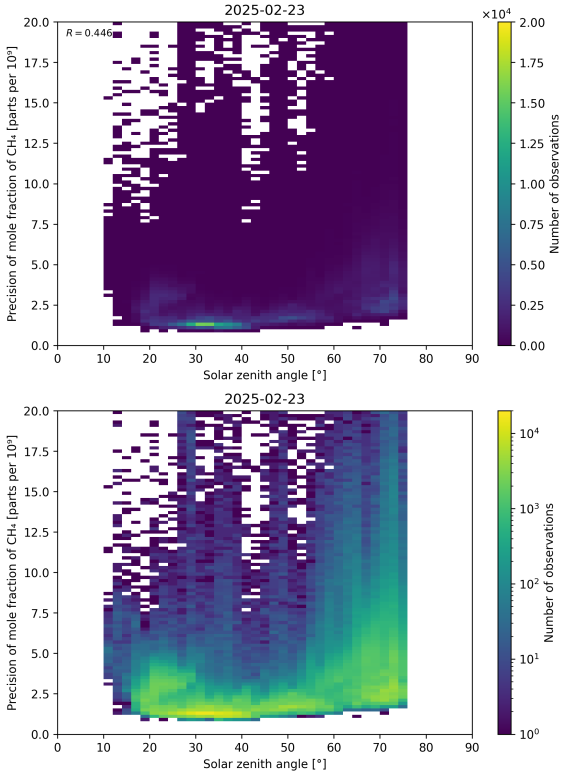
Figure 101: Scatter density plot of “Solar zenith angle” against “Precision of mole fraction of CH 4 ” for 2025-02-22 to 2025-02-24.
