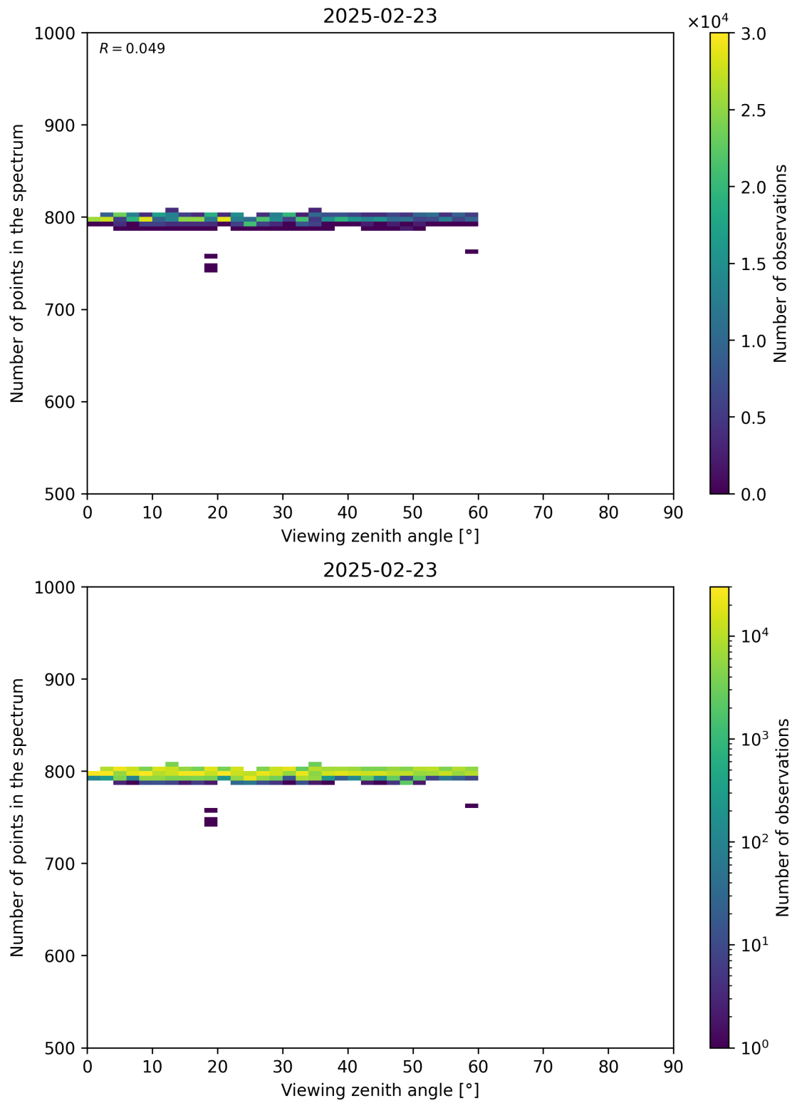
Figure 114: Scatter density plot of “Viewing zenith angle” against “Number of points in the spectrum” for 2025-02-22 to 2025-02-24.
