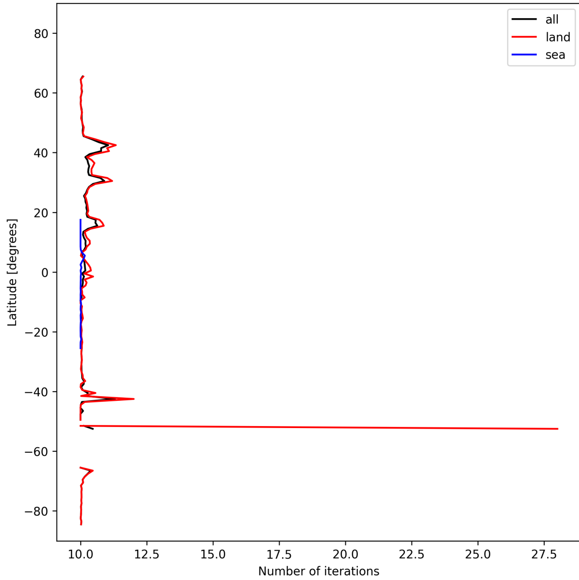
Figure 20: Zonal average of “Number of iterations” for 2025-02-22 to 2025-02-24.
