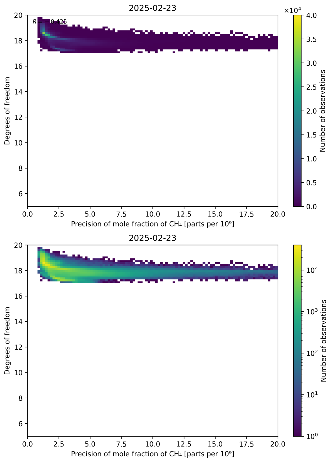
Figure 80: Scatter density plot of “Precision of mole fraction of CH 4 ” against “Degrees of freedom” for 2025-02-22 to 2025-02-24.
