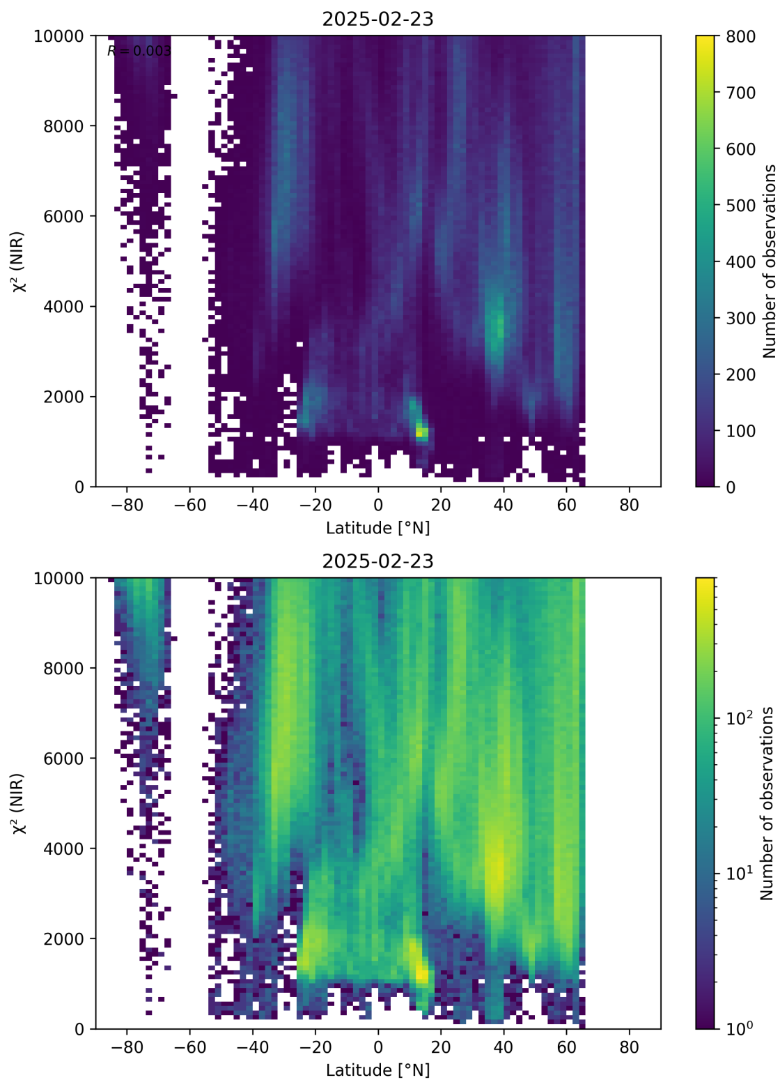
Figure 53: Scatter density plot of “Latitude” against “ \chi^2 (NIR)” for 2025-02-22 to 2025-02-24.
