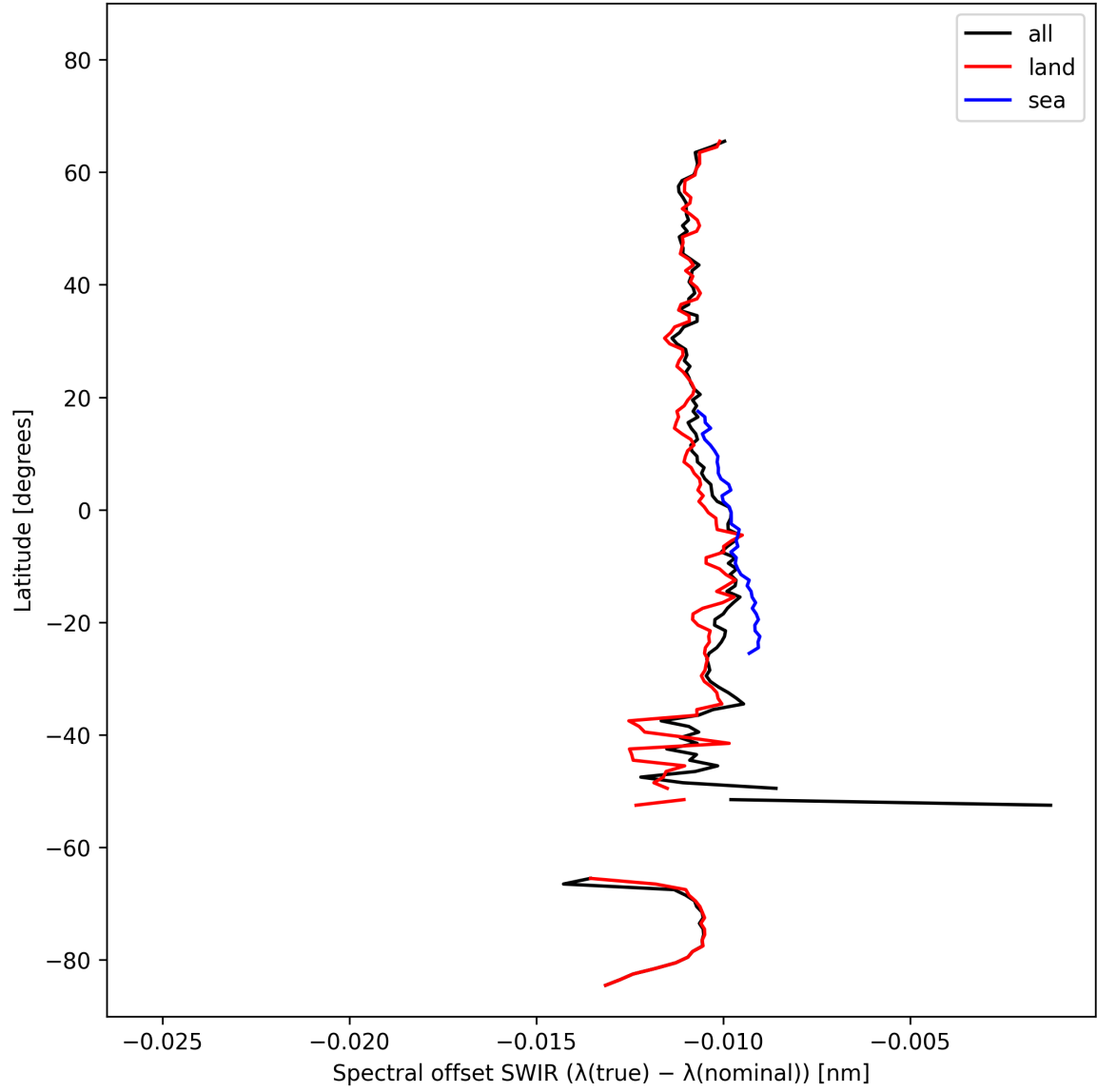
Figure 16: Zonal average of “Spectral offset SWIR ( \lambda_{\text{true}} - \lambda_{\text{nominal}} )” for 2025-02-22 to 2025-02-24.
