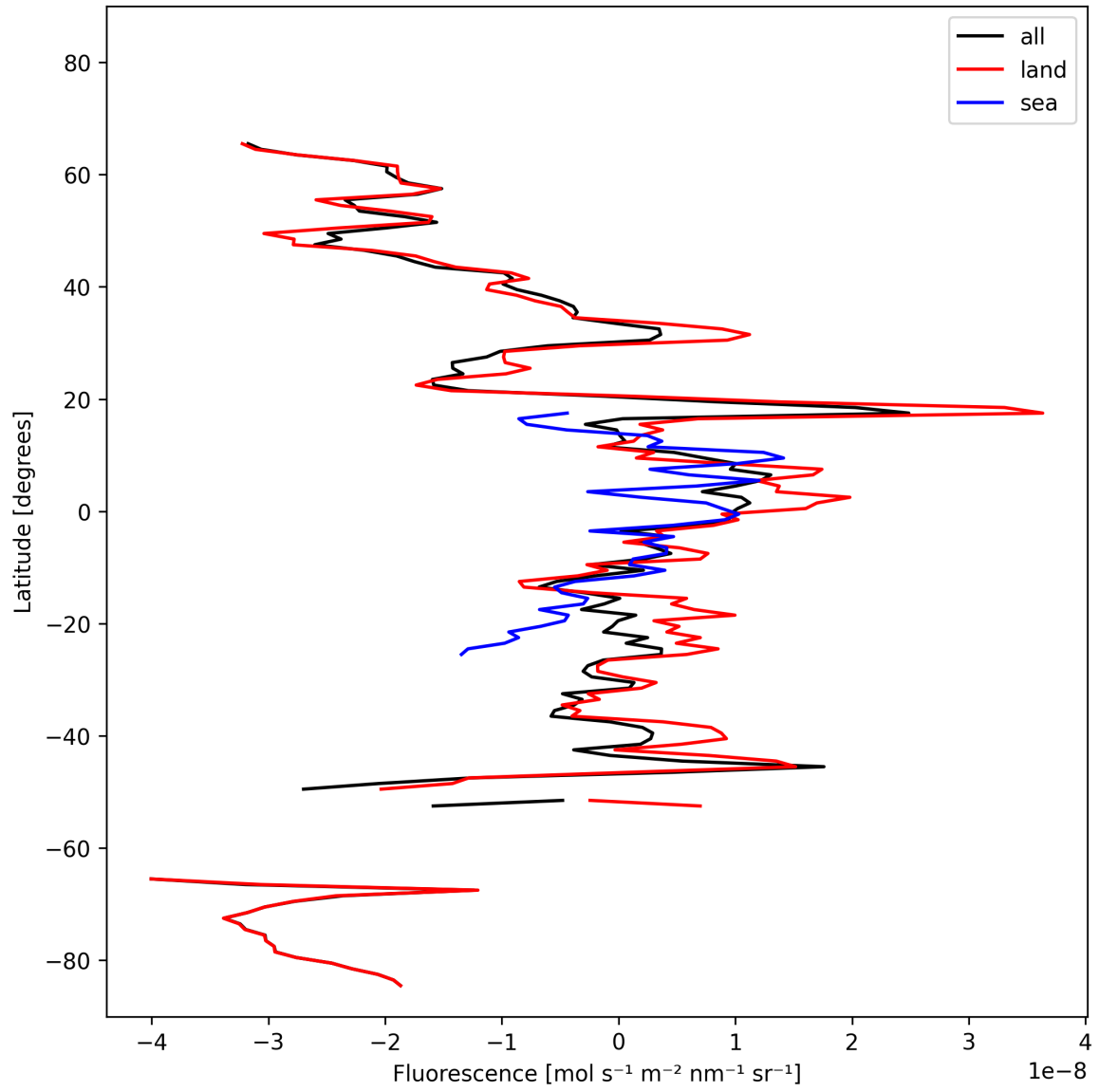
Figure 21: Zonal average of “Fluorescence” for 2025-02-22 to 2025-02-24.
