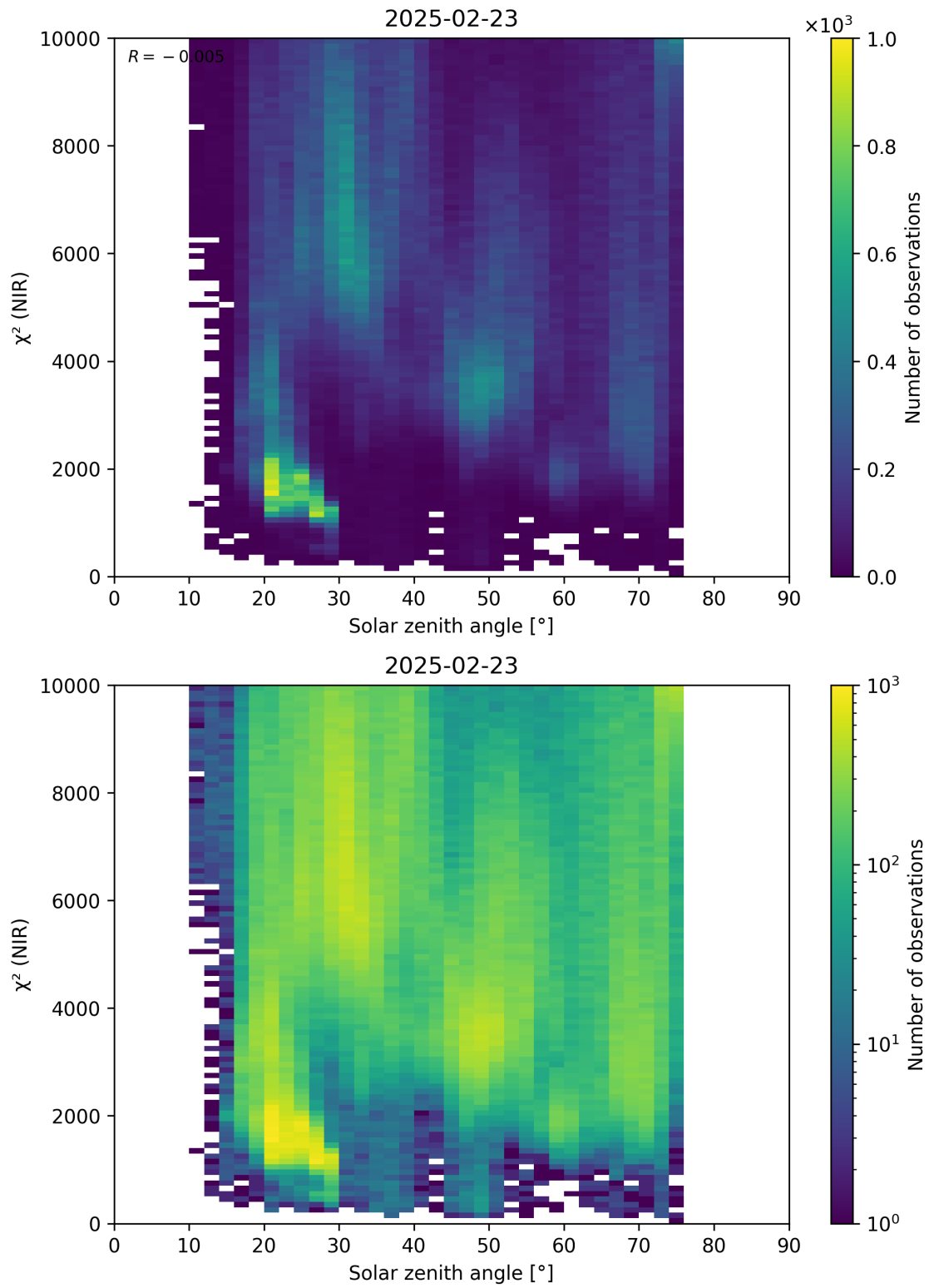
Figure 94: Scatter density plot of “Solar zenith angle” against “ \chi^2 (NIR)” for 2025-02-22 to 2025-02-24.
