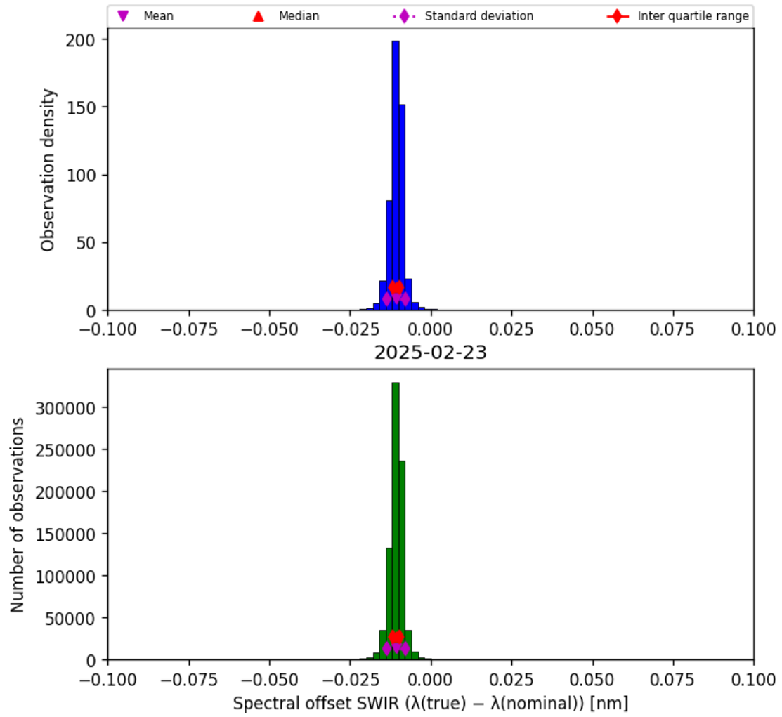
Figure 27: Histogram of “Spectral offset SWIR ( \lambda_{\text{true}} - \lambda_{\text{nominal}} )” for 2025-02-22 to 2025-02-24
