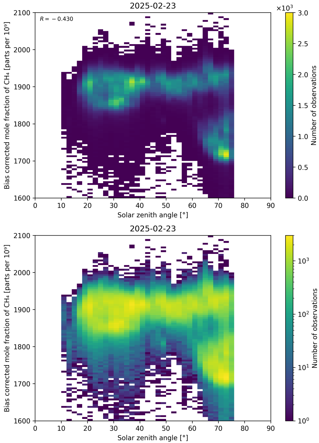
Figure 100: Scatter density plot of “Solar zenith angle” against “Bias corrected mole fraction of \text{CH}_4 ” for 2025-02-22 to 2025-02-24.
