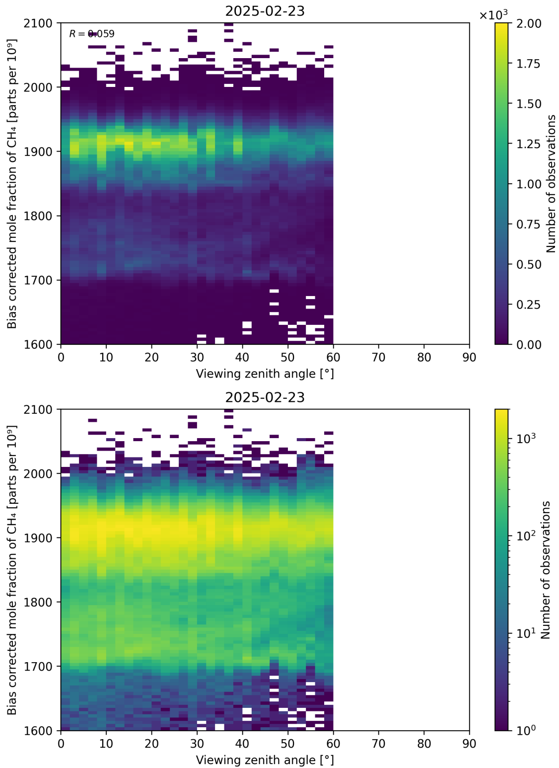
Figure 111: Scatter density plot of “Viewing zenith angle” against “Bias corrected mole fraction of CH 4 ” for 2025-02-22 to 2025-02-24.
