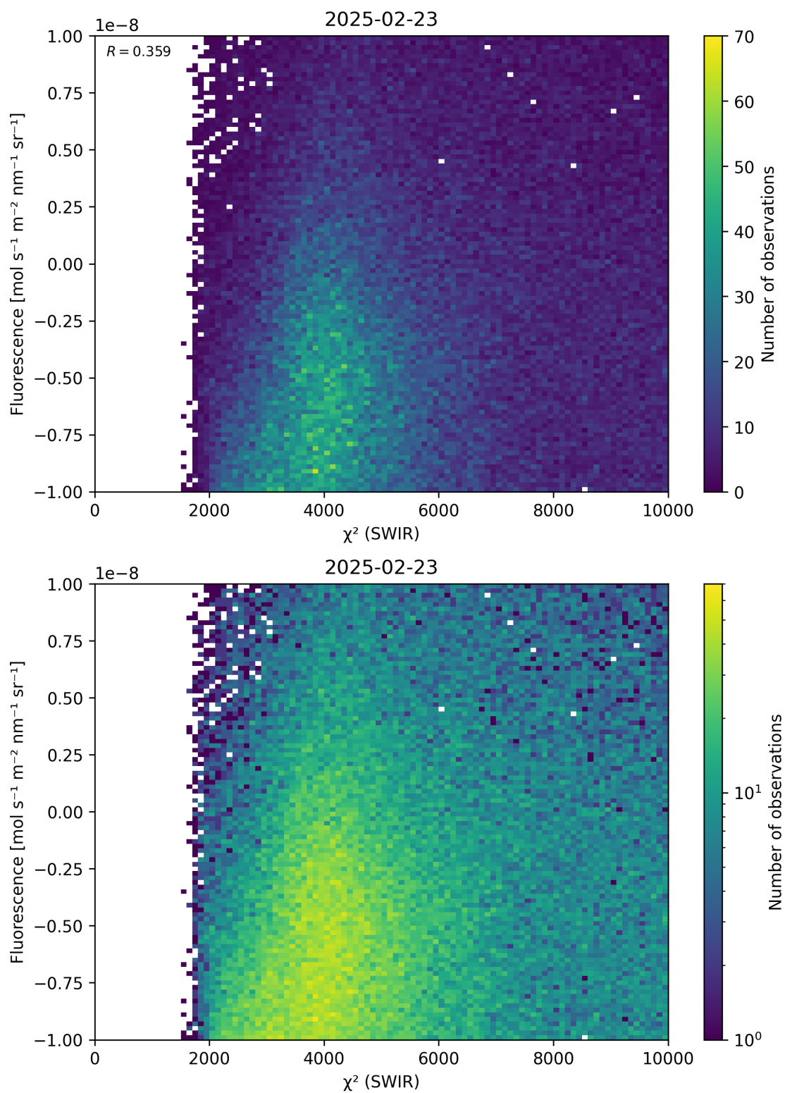
Figure 49: Scatter density plot of “ \chi^2 (SWIR)” against “Fluorescence” for 2025-02-22 to 2025-02-24.
