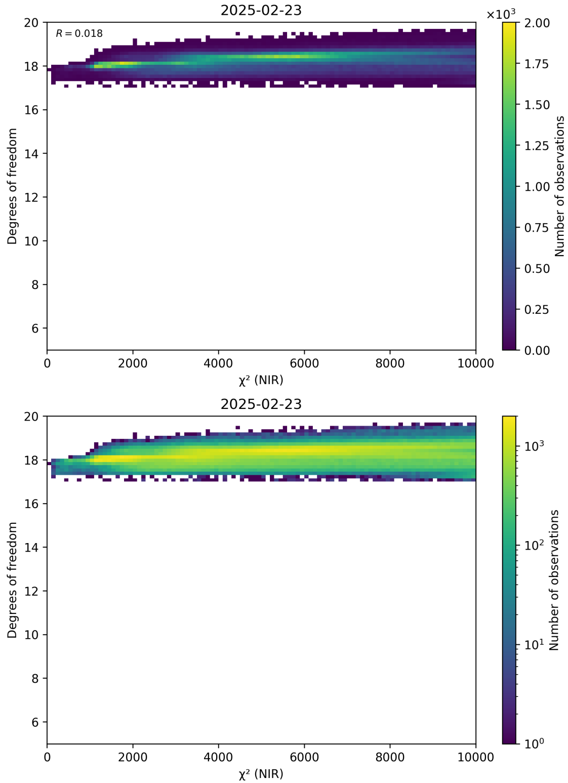
Figure 44: Scatter density plot of “ \chi^2 (NIR)” against “Degrees of freedom” for 2025-02-22 to 2025-02-24.
