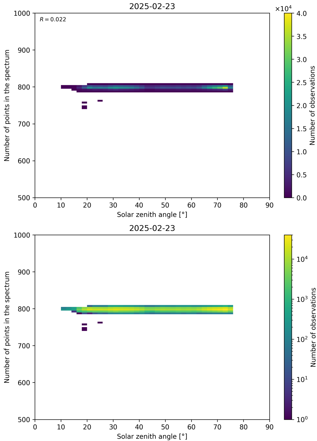
Figure 103: Scatter density plot of “Solar zenith angle” against “Number of points in the spectrum” for 2025-02-22 to 2025-02-24.
