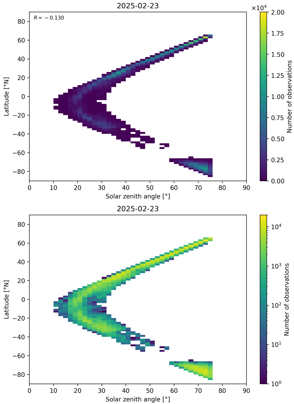
Figure 98: Scatter density plot of “Solar zenith angle” against “Latitude” for 2025-02-22 to 2025-02-24.
