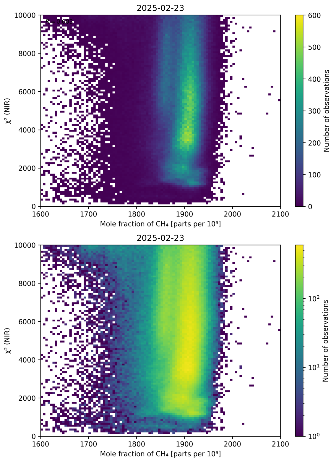
Figure 70: Scatter density plot of “Mole fraction of \text{CH}_4 ” against “ \chi^2 (NIR)” for 2025-02-22 to 2025-02-24.
