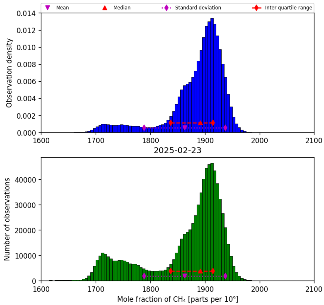
Figure 23: Histogram of “Mole fraction of CH 4 ” for 2025-02-22 to 2025-02-24
