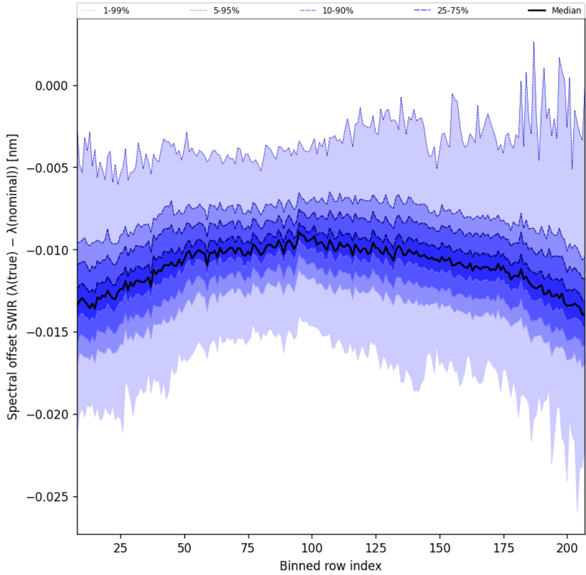
Figure 38: Along track statistics of “Spectral offset SWIR ( \lambda_{\text{true}} - \lambda_{\text{nominal}} )” for 2025-02-22 to 2025-02-24
