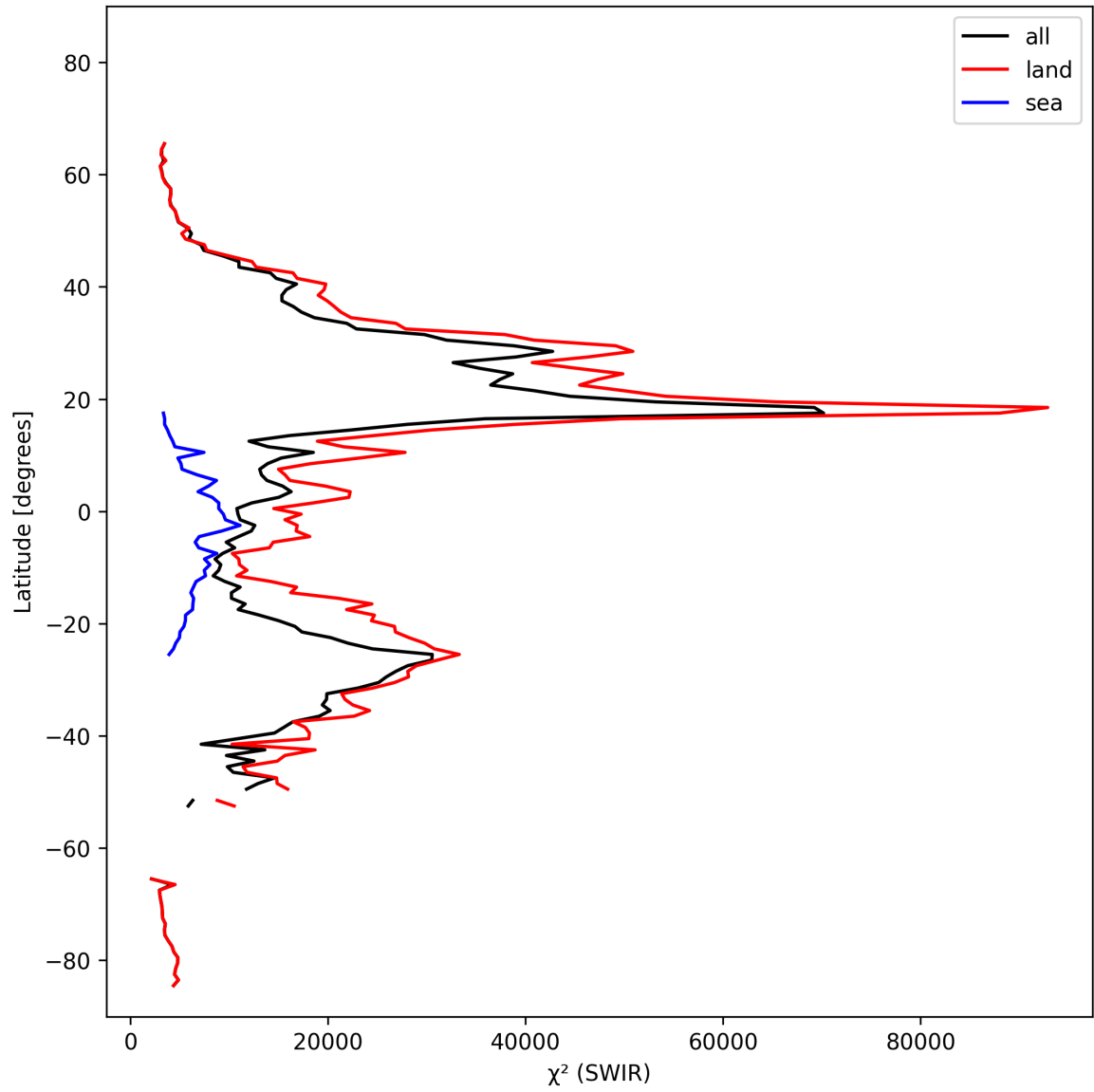
Figure 17: Zonal average of “ \chi^2 (SWIR)” for 2025-02-22 to 2025-02-24.
