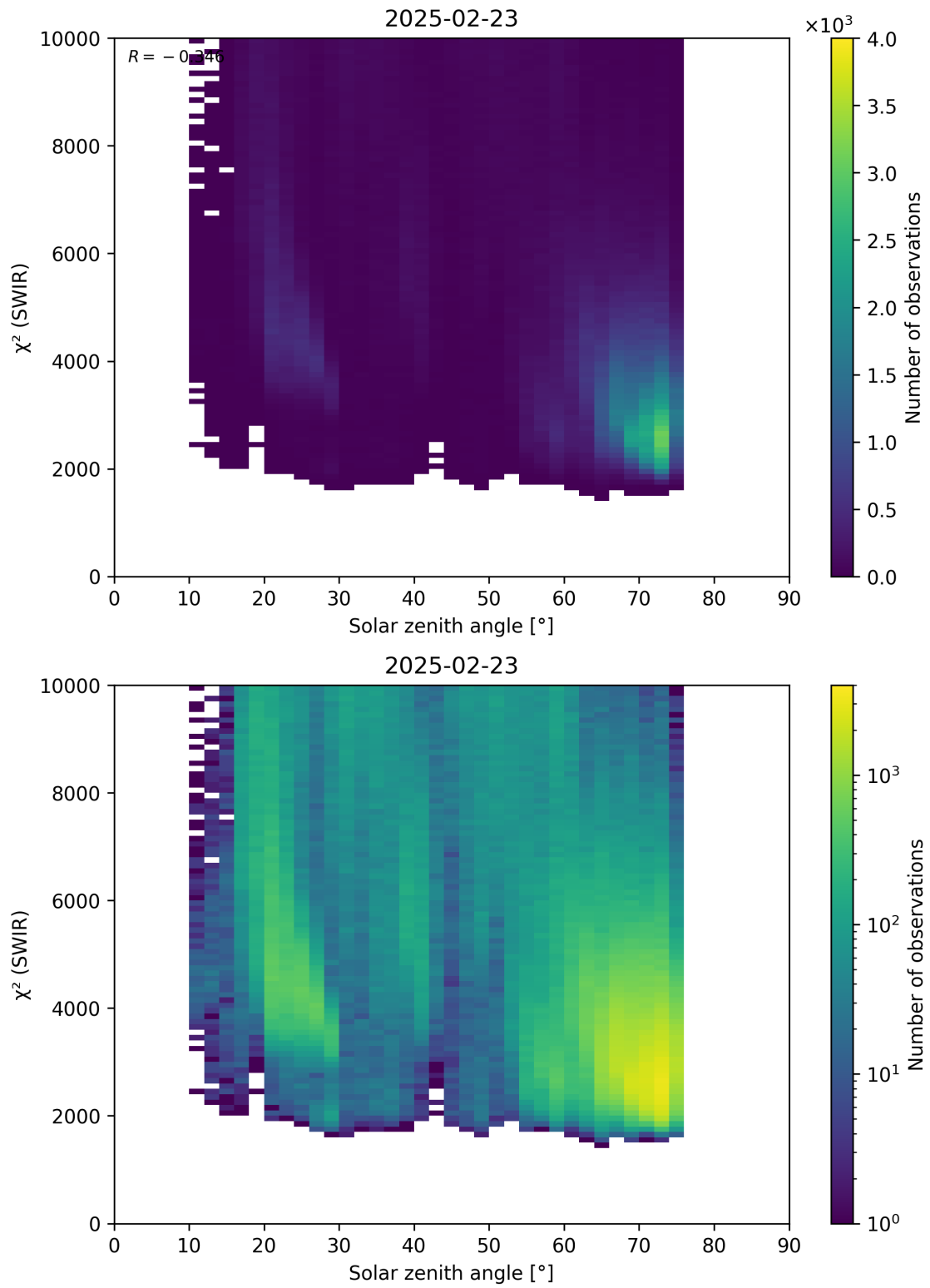
Figure 95: Scatter density plot of “Solar zenith angle” against “ \chi^2 (SWIR)” for 2025-02-22 to 2025-02-24.
