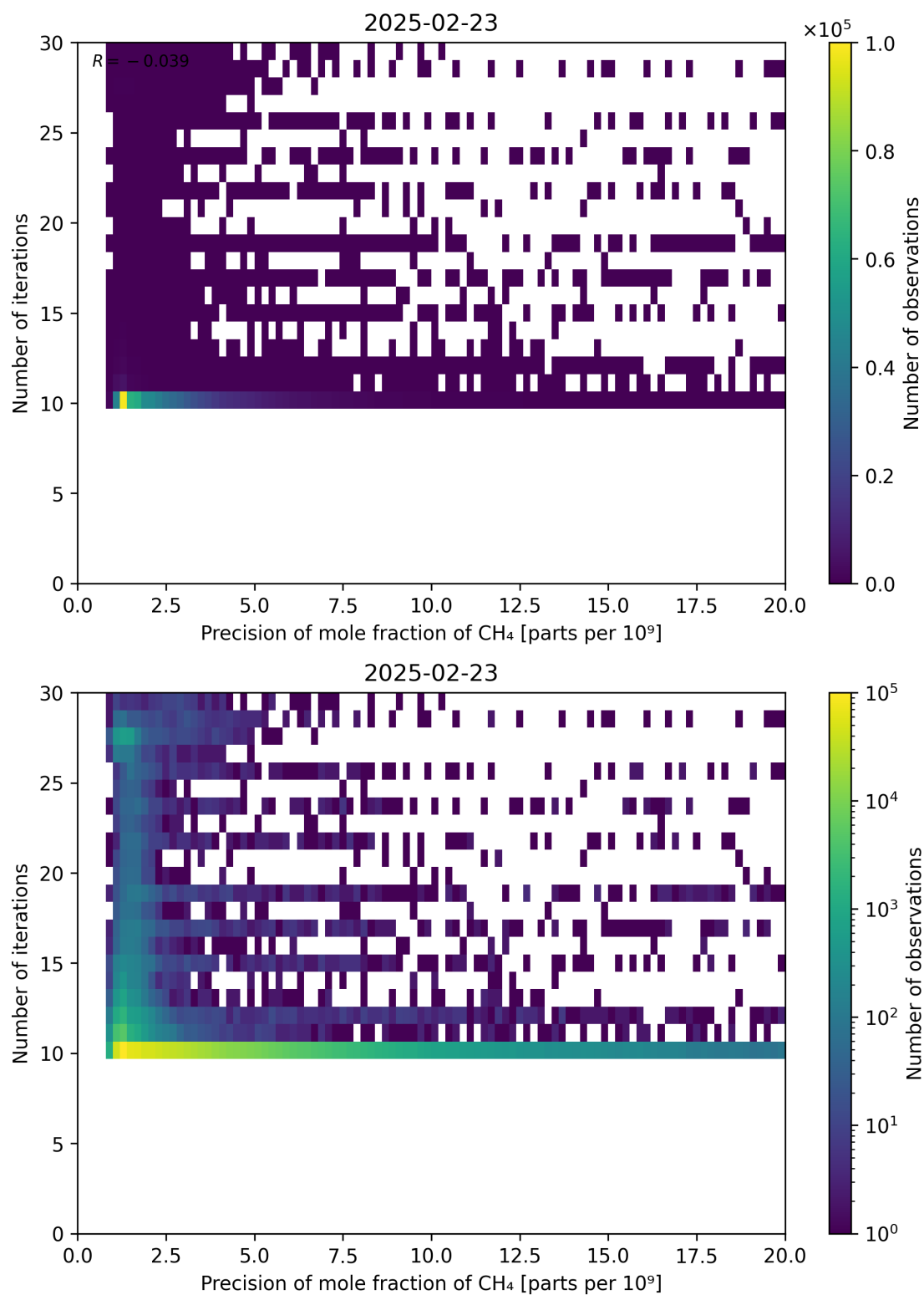
Figure 83: Scatter density plot of “Precision of mole fraction of CH 4 ” against “Number of iterations” for 2025-02-22 to 2025-02-24.
