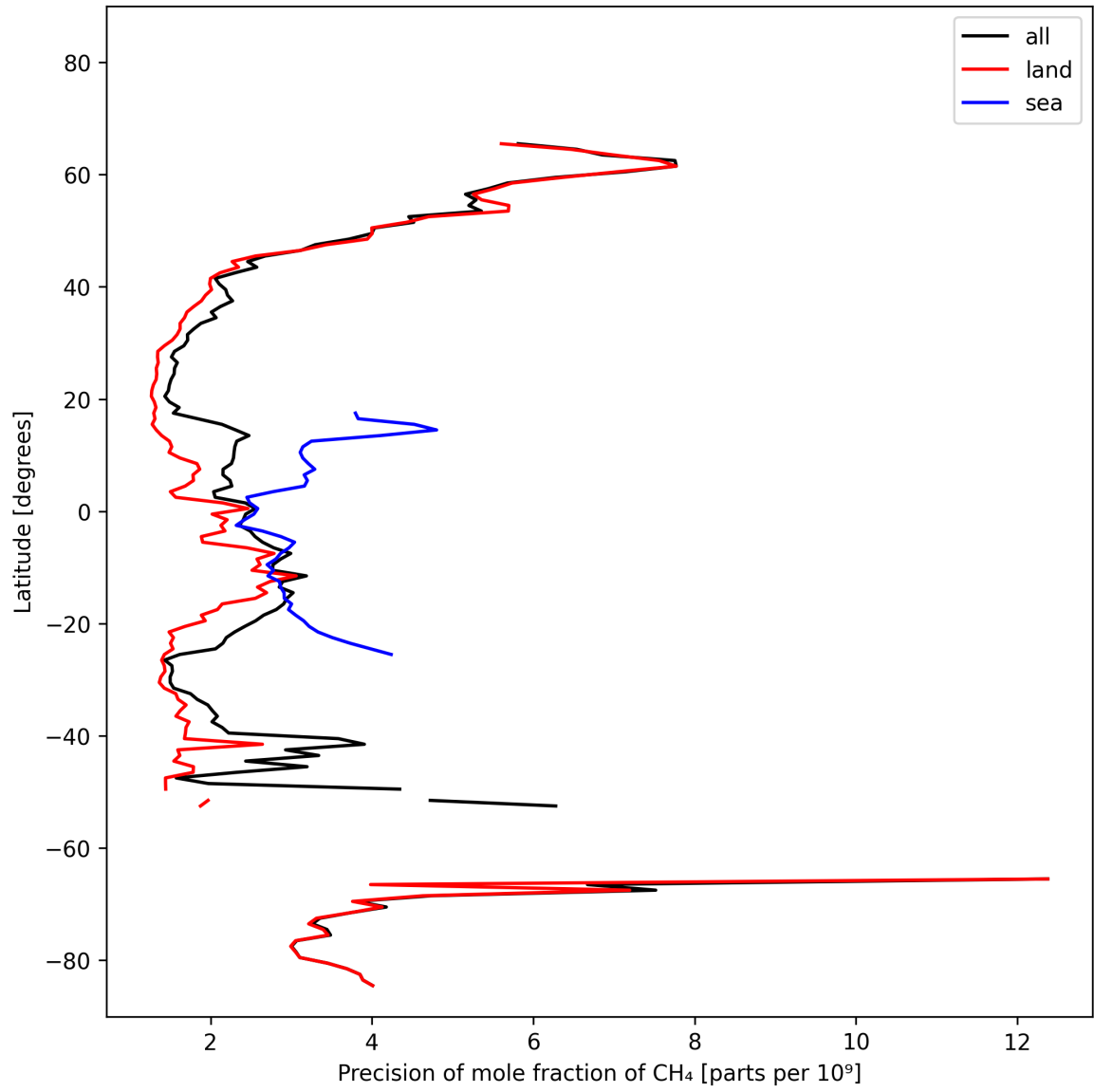
Figure 13: Zonal average of “Precision of mole fraction of CH 4 ” for 2025-02-22 to 2025-02-24.
