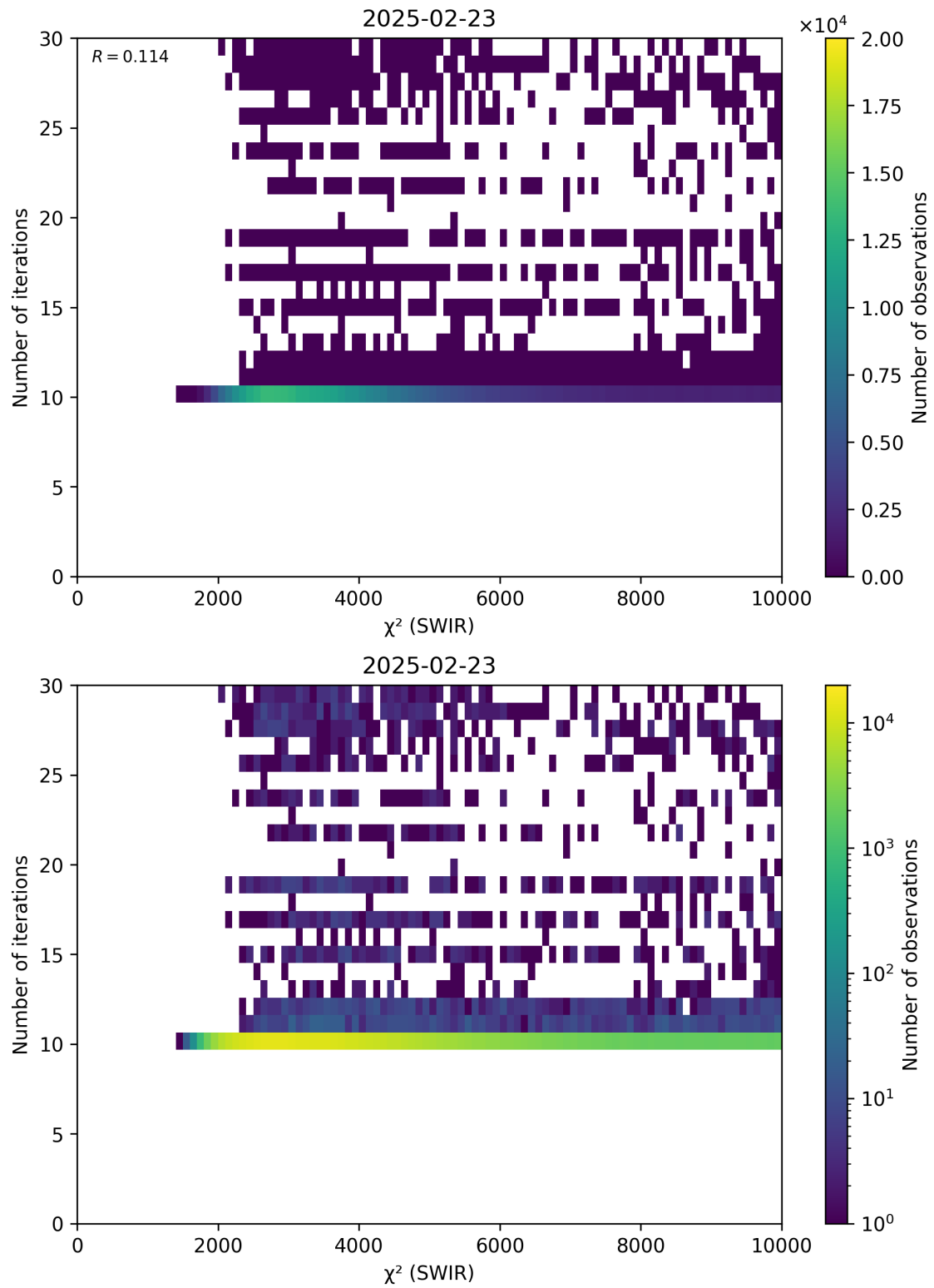
Figure 50: Scatter density plot of “ \chi^2 (SWIR)” against “Number of iterations” for 2025-02-22 to 2025-02-24.
