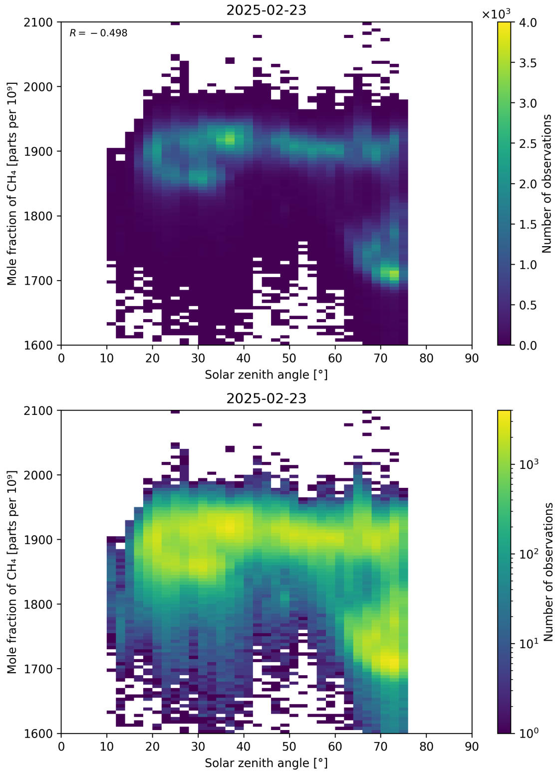
Figure 99: Scatter density plot of “Solar zenith angle” against “Mole fraction of CH 4 ” for 2025-02-22 to 2025-02-24.
