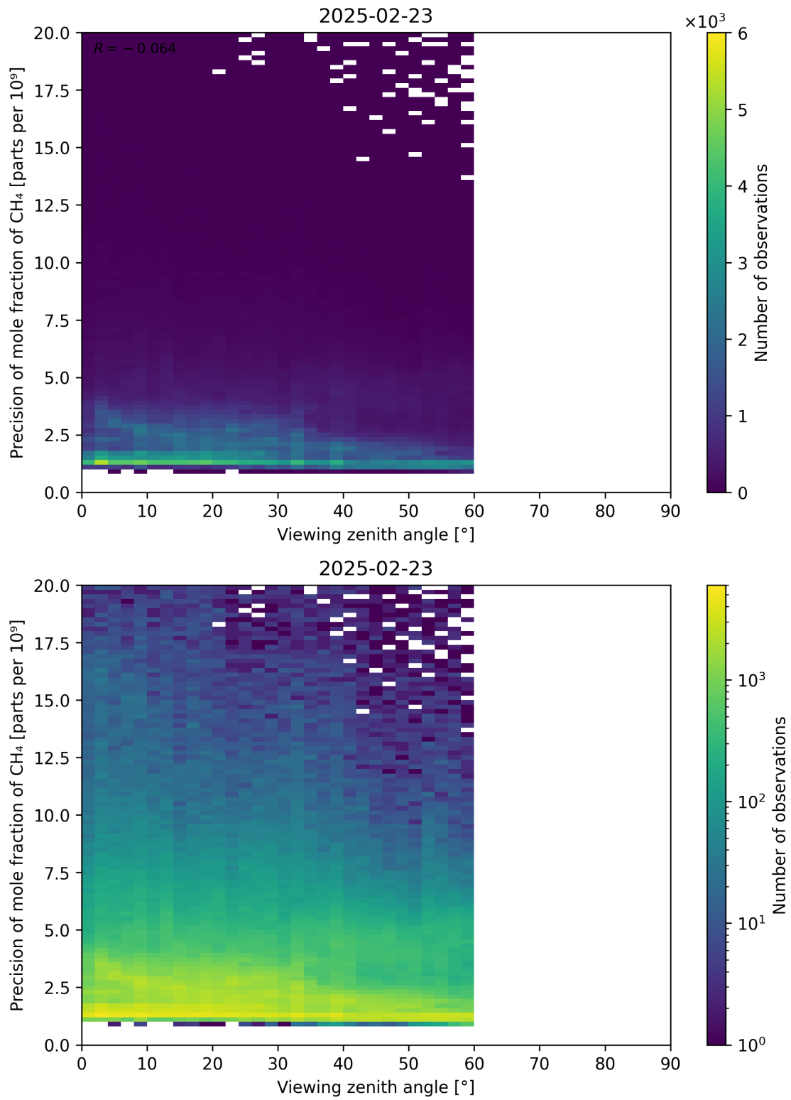
Figure 112: Scatter density plot of “Viewing zenith angle” against “Precision of mole fraction of CH 4 ” for 2025-02-22 to 2025-02-24.
