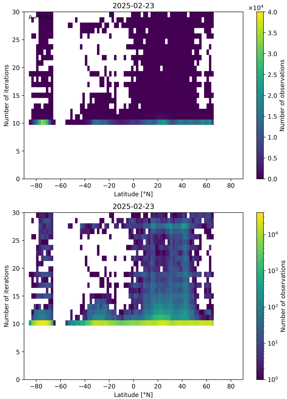
Figure 60: Scatter density plot of “Latitude” against “Number of iterations” for 2025-02-22 to 2025-02-24.
