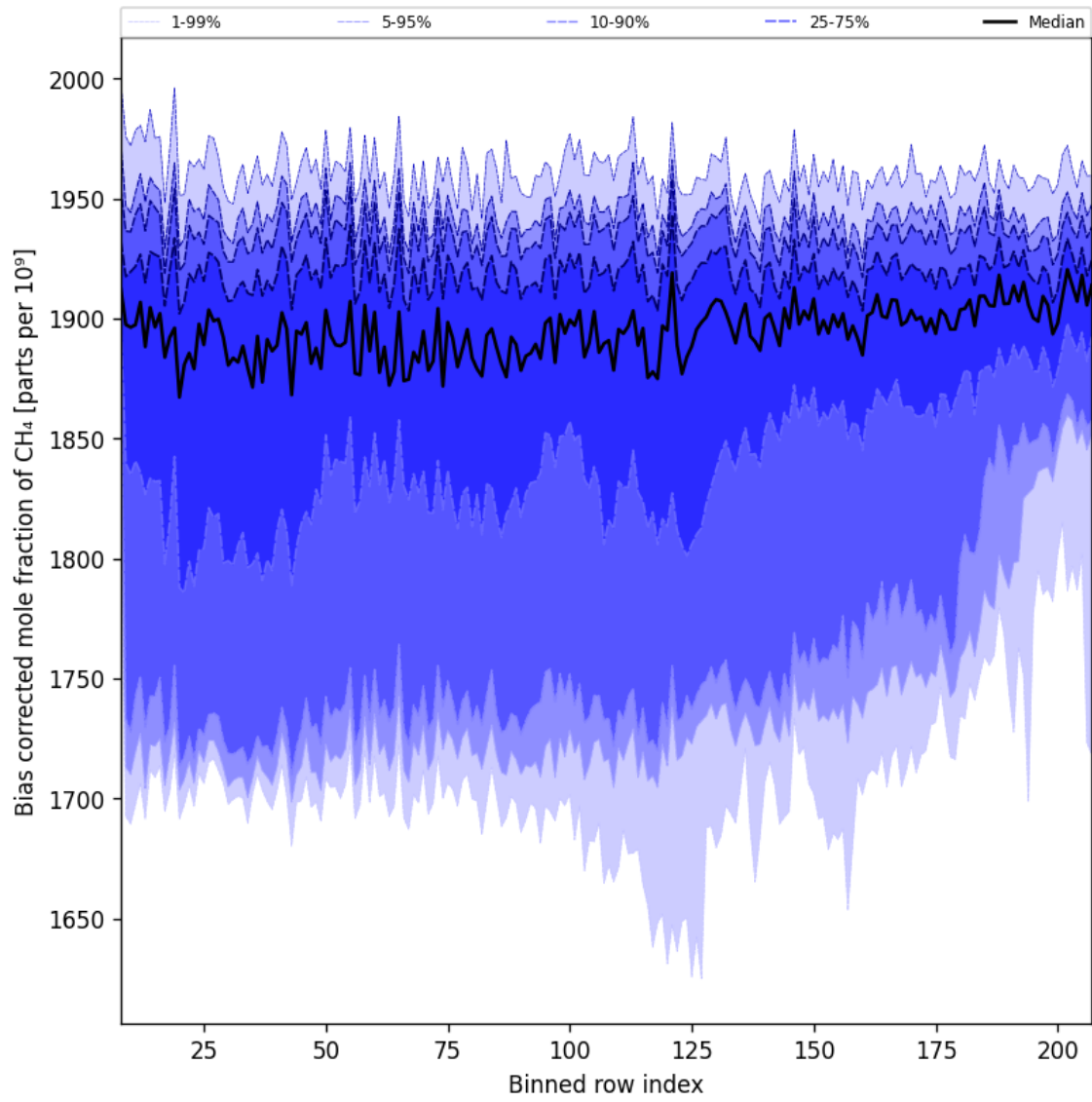
Figure 36: Along track statistics of “Bias corrected mole fraction of CH 4 ” for 2025-02-22 to 2025-02-24
