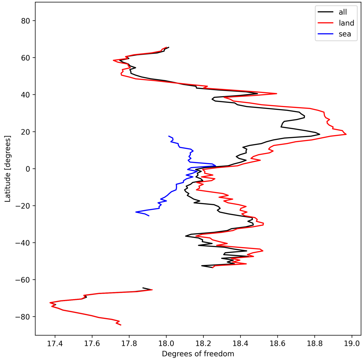
Figure 19: Zonal average of “Degrees of freedom” for 2025-02-24 to 2025-02-25.
