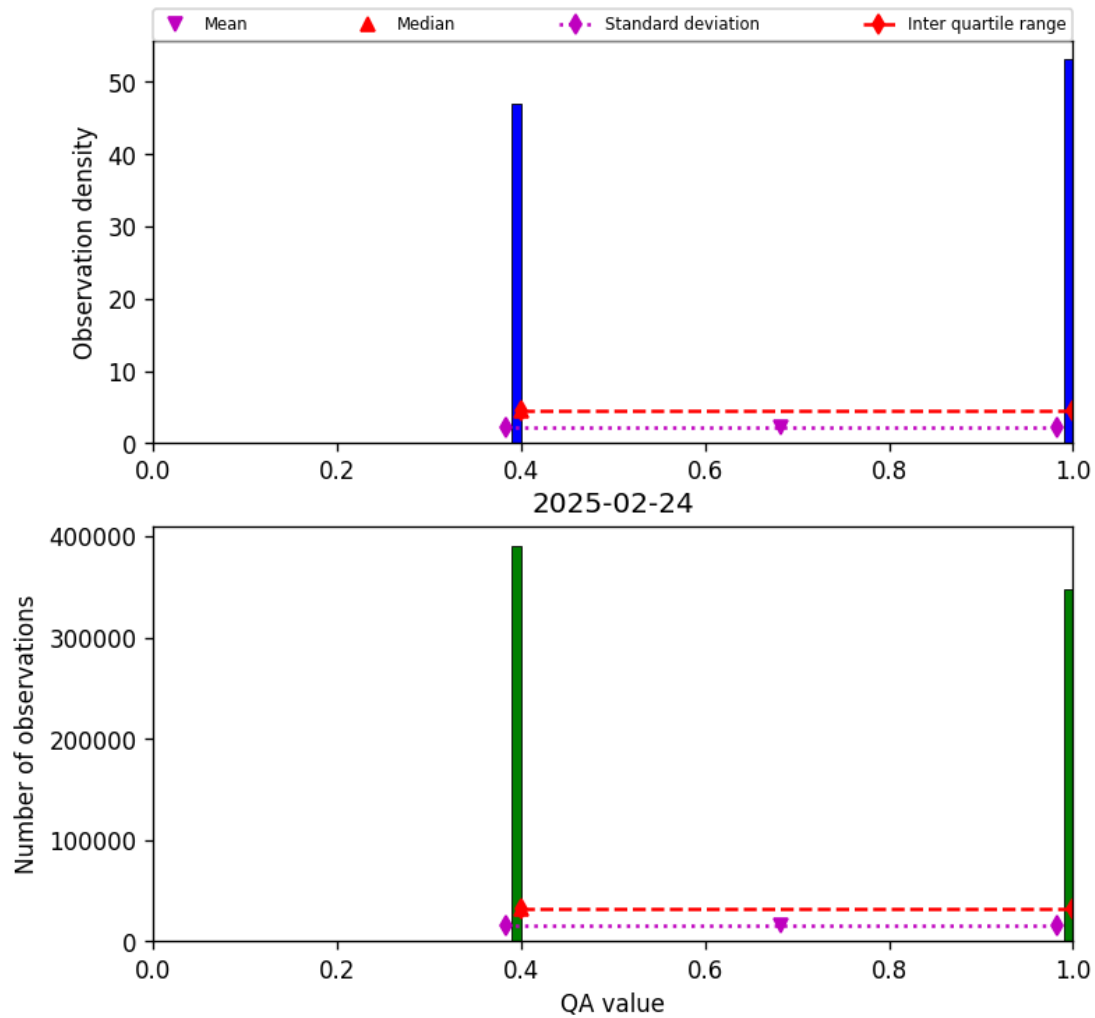
Figure 22: Histogram of “QA value” for 2025-02-24 to 2025-02-25
