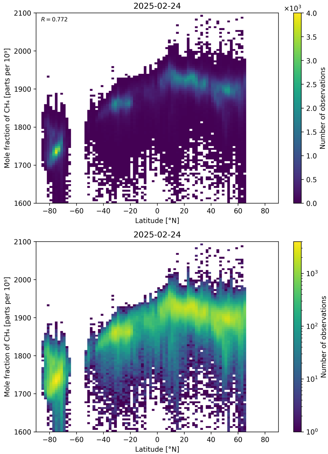
Figure 57: Scatter density plot of “Latitude” against “Mole fraction of CH 4 ” for 2025-02-24 to 2025-02-25.
