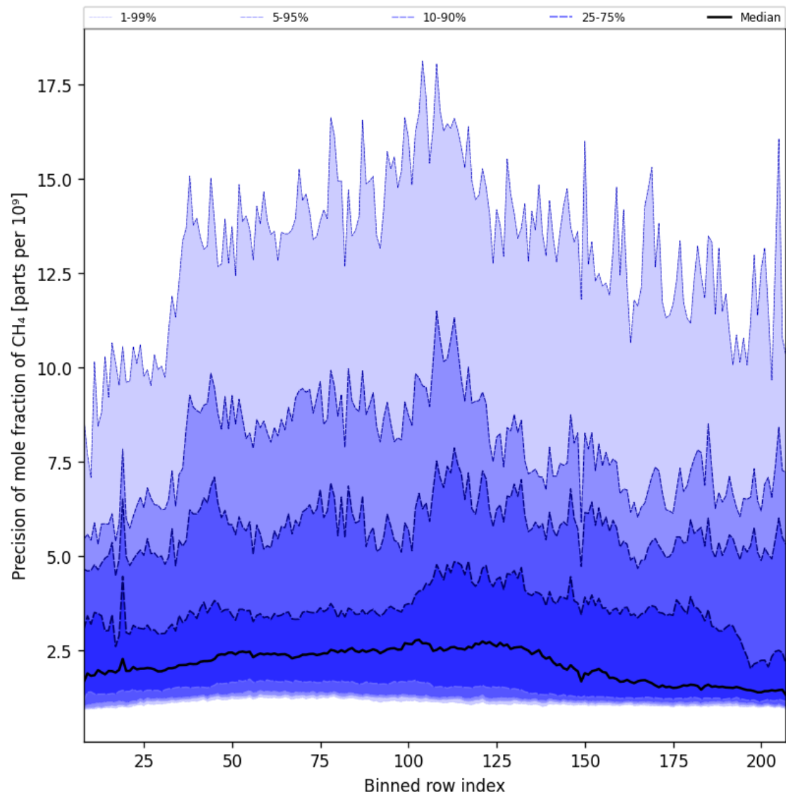
Figure 35: Along track statistics of "Precision of mole fraction of CH 4 " for 2025-02-24 to 2025-02-25
