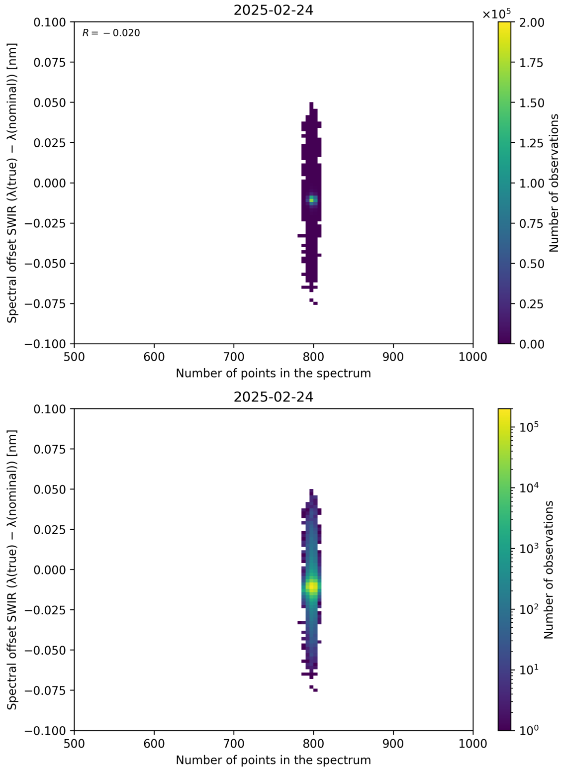
Figure 93: Scatter density plot of “Number of points in the spectrum” against “Spectral offset SWIR ( \lambda_{\text{true}} - \lambda_{\text{nominal}} )” for 2025-02-24 to 2025-02-25.
