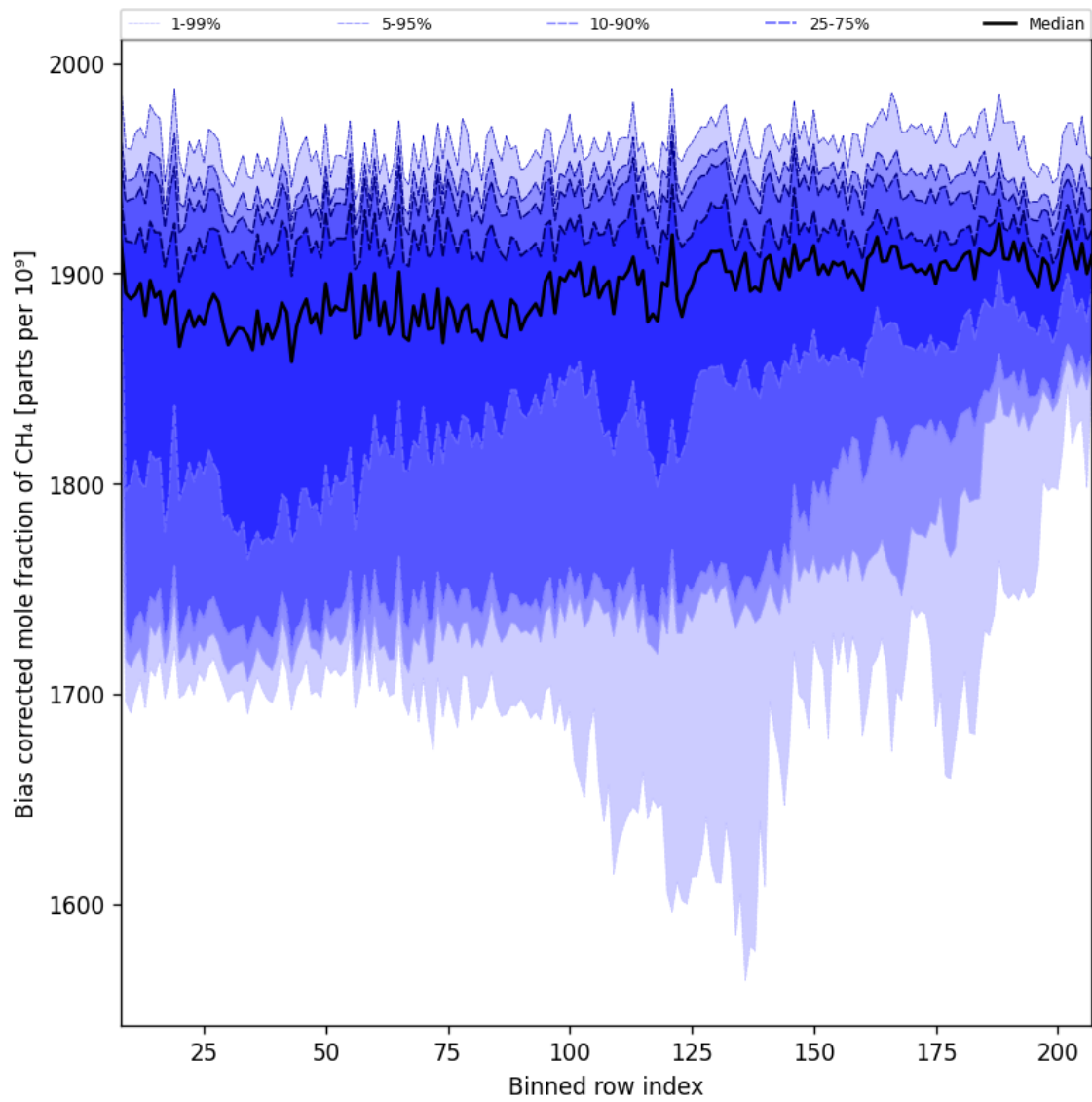
Figure 36: Along track statistics of “Bias corrected mole fraction of CH 4 ” for 2025-02-24 to 2025-02-25
