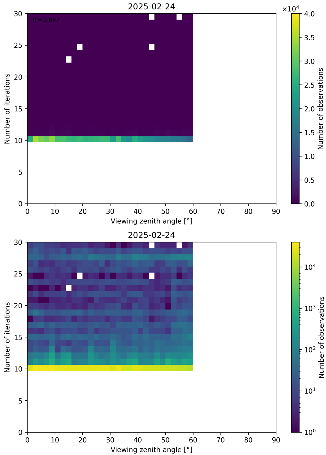
Figure 113: Scatter density plot of “Viewing zenith angle” against “Number of iterations” for 2025-02-24 to 2025-02-25.
