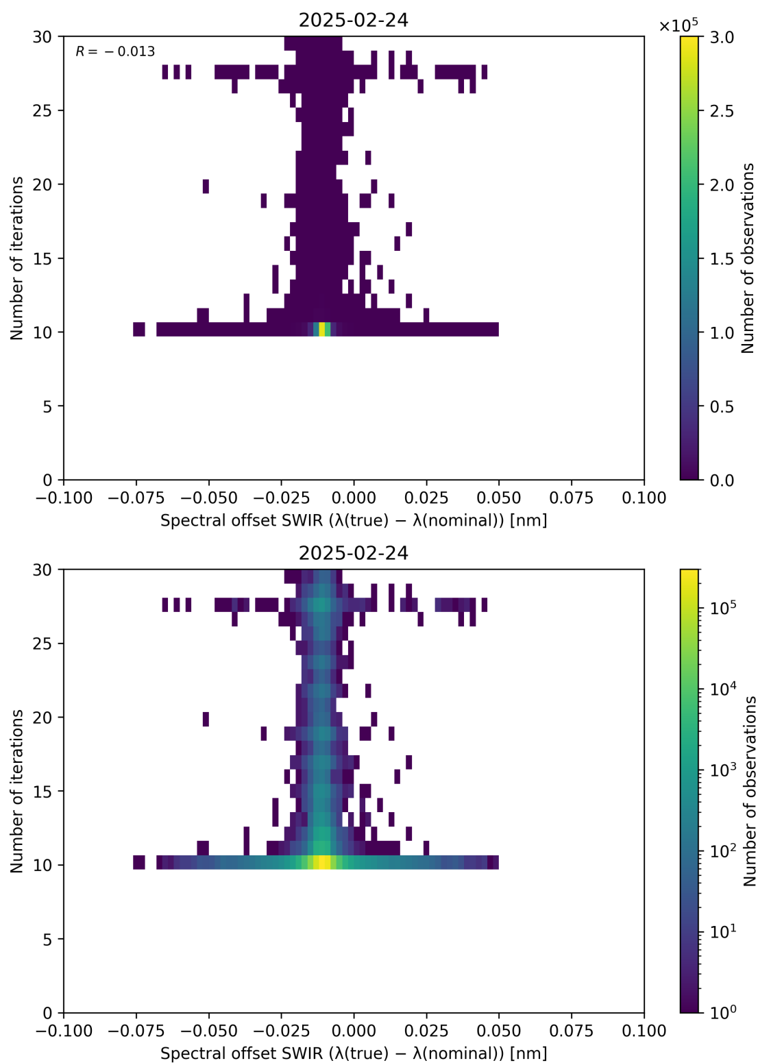
Figure 121: Scatter density plot of “Spectral offset SWIR ( \lambda_{\text{true}} - \lambda_{\text{nominal}} )” against “Number of iterations” for 2025-02-24 to 2025-02-25.
