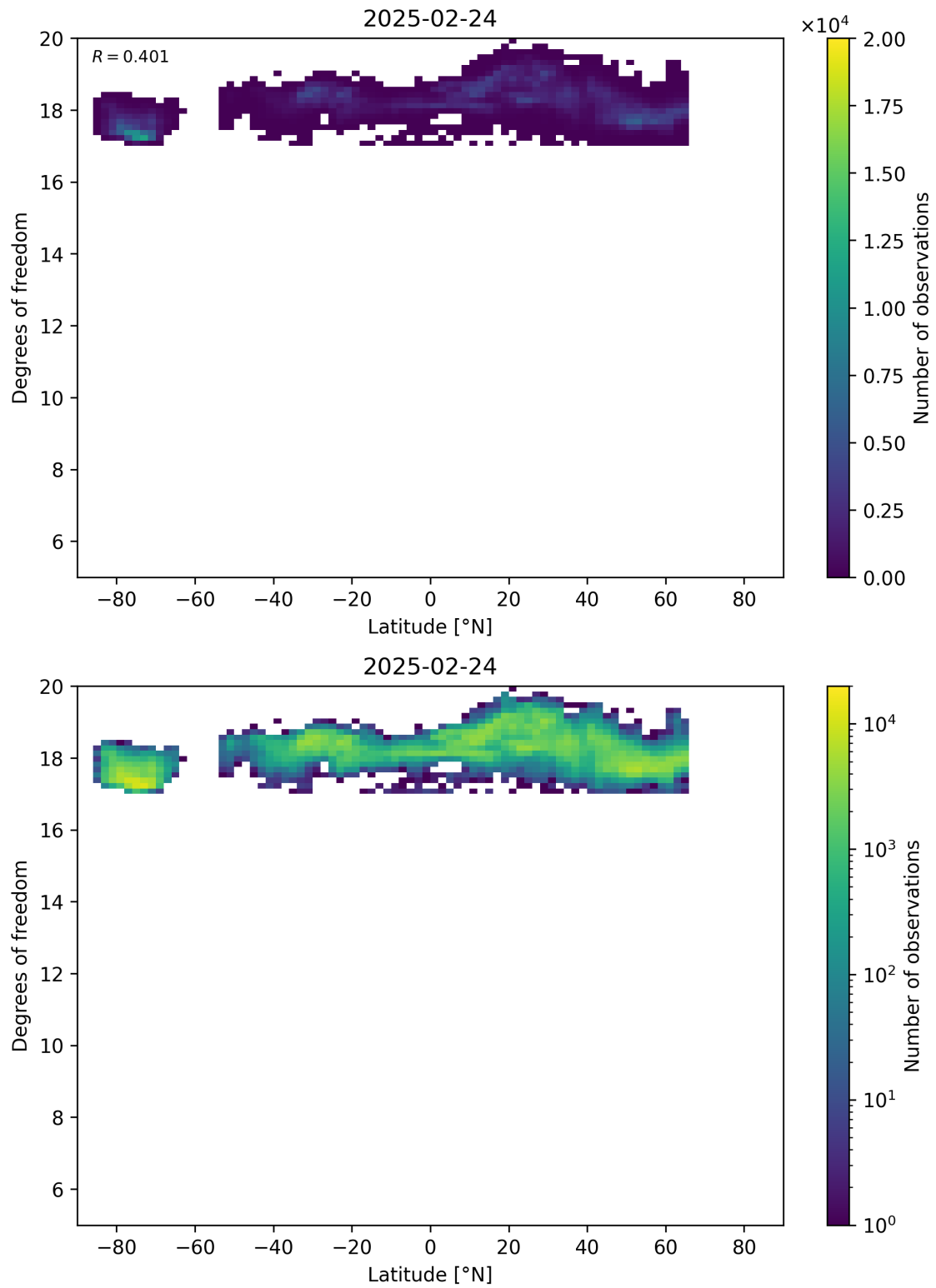
Figure 55: Scatter density plot of “Latitude” against “Degrees of freedom” for 2025-02-24 to 2025-02-25.
