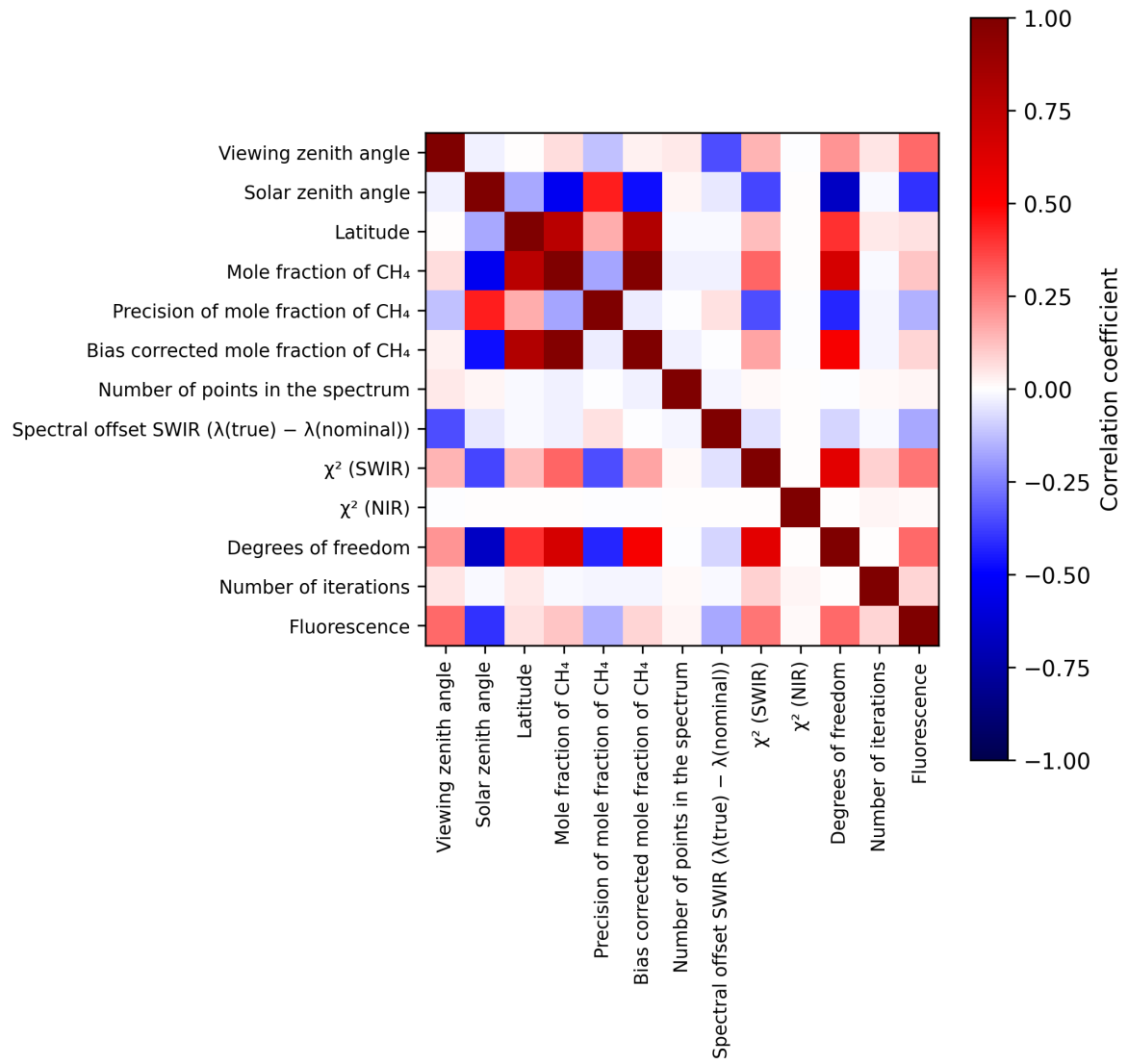
Figure 2: Map of correlation matrix for 2025-02-24 to 2025-02-25.
