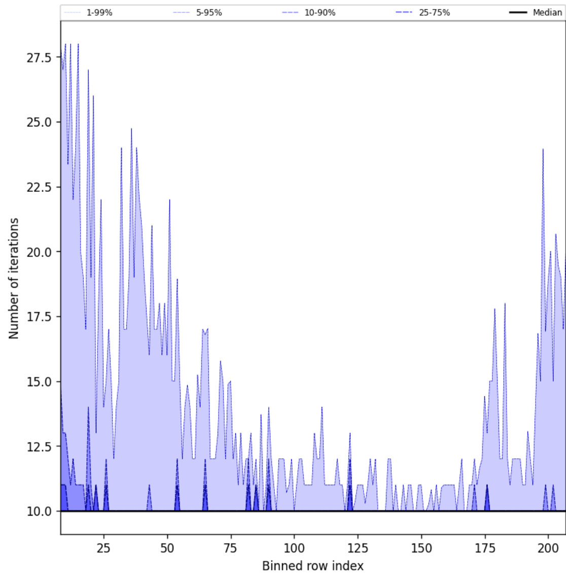
Figure 42: Along track statistics of “Number of iterations” for 2025-02-24 to 2025-02-25
