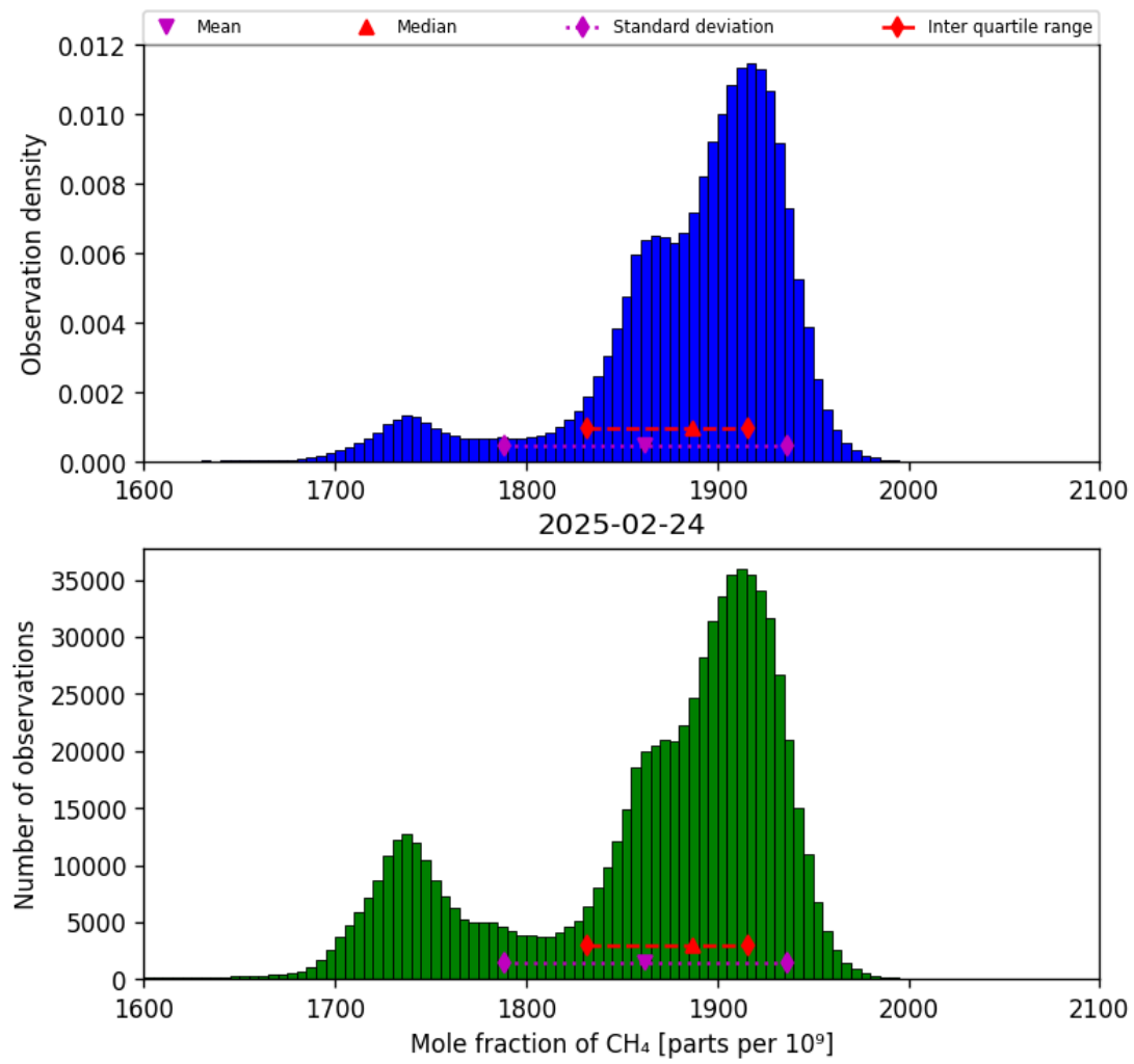
Figure 23: Histogram of “Mole fraction of CH 4 ” for 2025-02-24 to 2025-02-25
