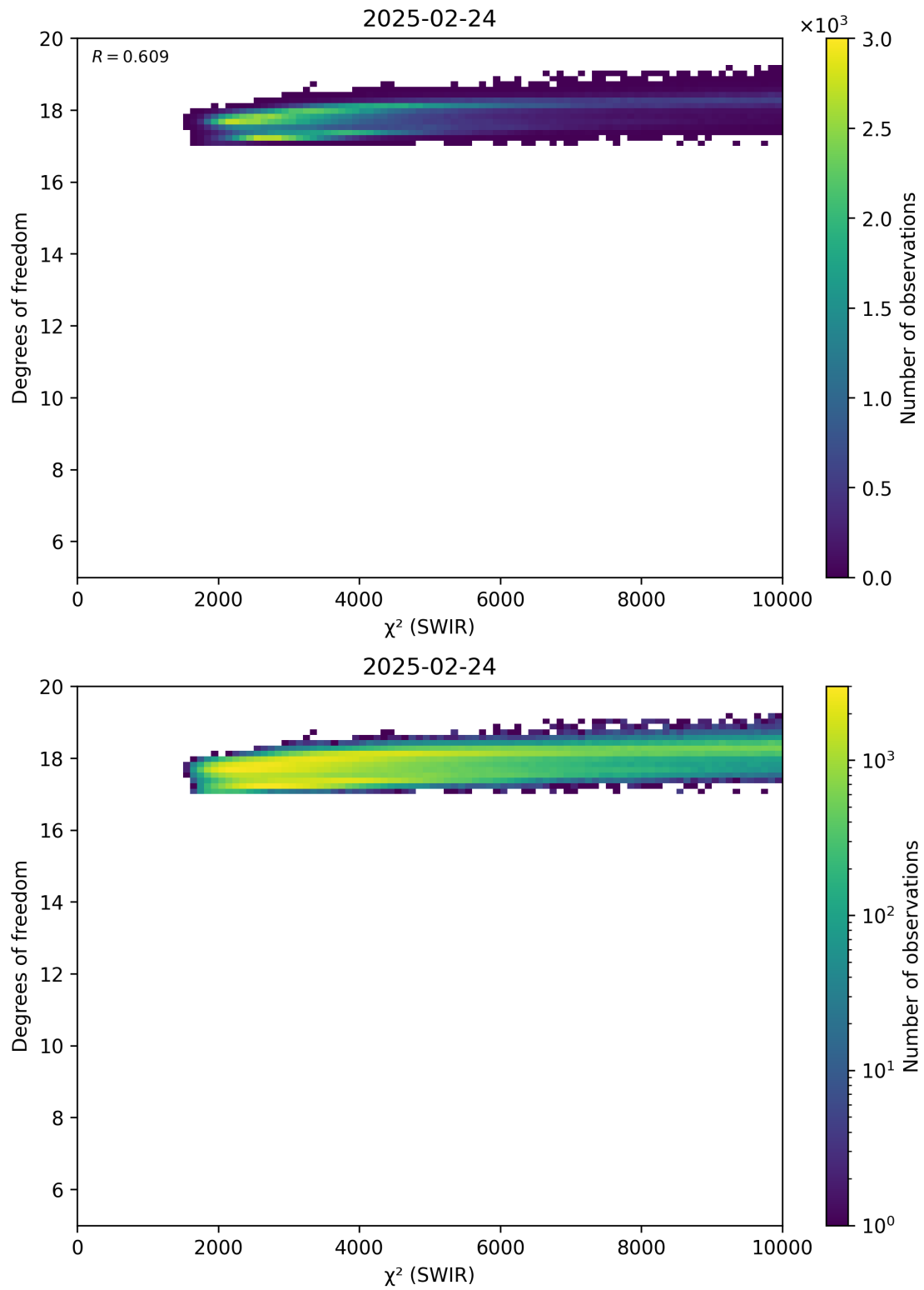
Figure 48: Scatter density plot of “ \chi^2 (SWIR)” against “Degrees of freedom” for 2025-02-24 to 2025-02-25.
