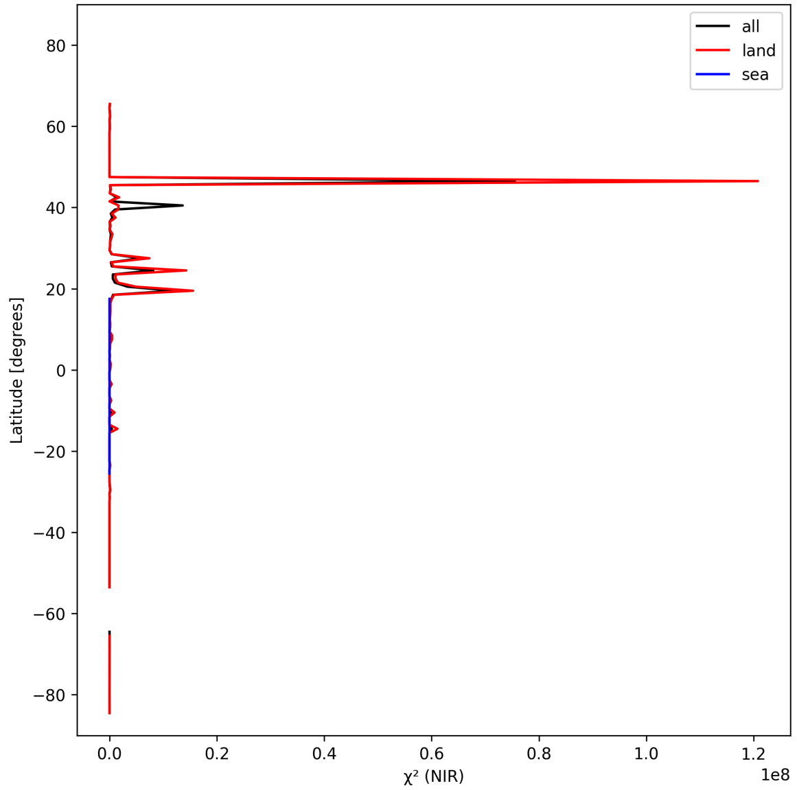
Figure 18: Zonal average of “ \chi^2 (NIR)” for 2025-02-24 to 2025-02-25.
