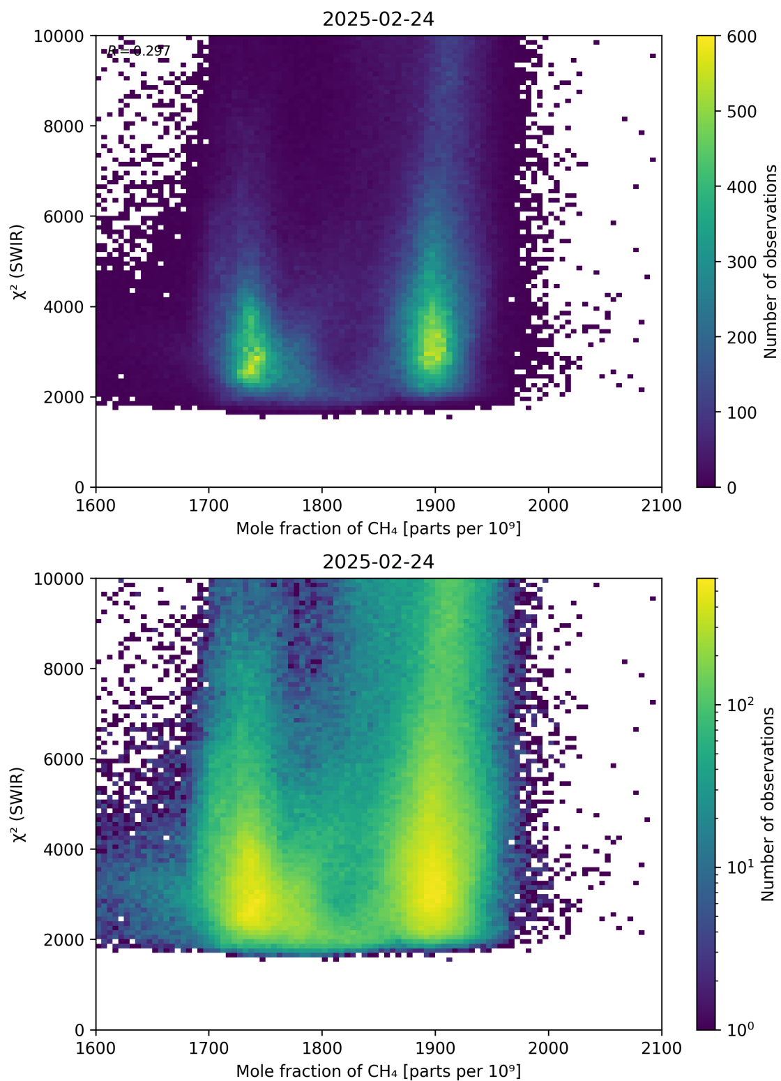
Figure 71: Scatter density plot of “Mole fraction of CH 4 ” against “ \chi^2 (SWIR)” for 2025-02-24 to 2025-02-25.
