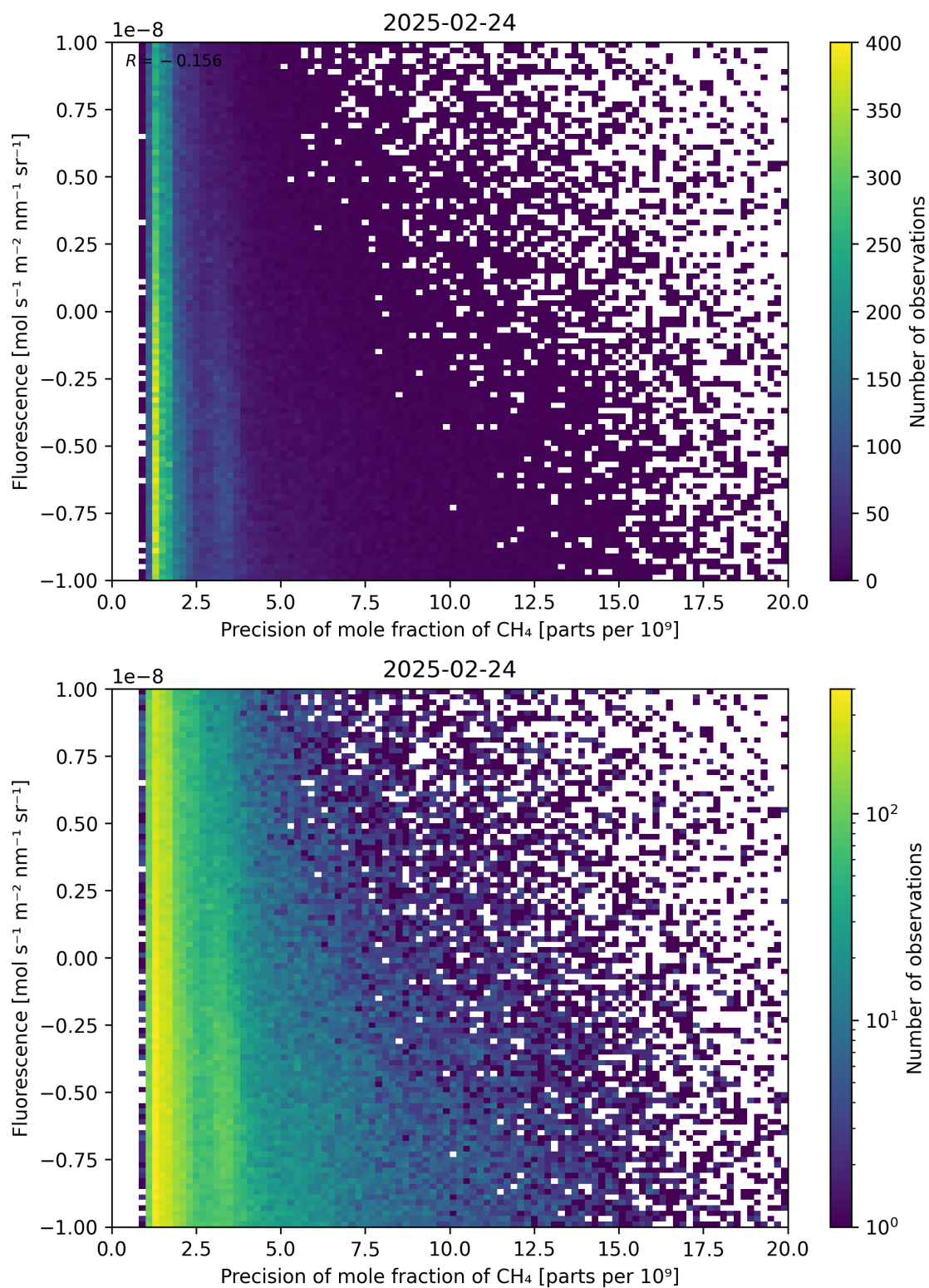
Figure 81: Scatter density plot of “Precision of mole fraction of CH 4 ” against “Fluorescence” for 2025-02-24 to 2025-02-25.
