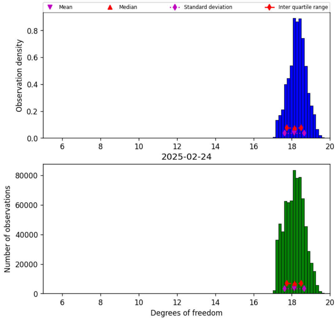
Figure 30: Histogram of “Degrees of freedom” for 2025-02-24 to 2025-02-25
