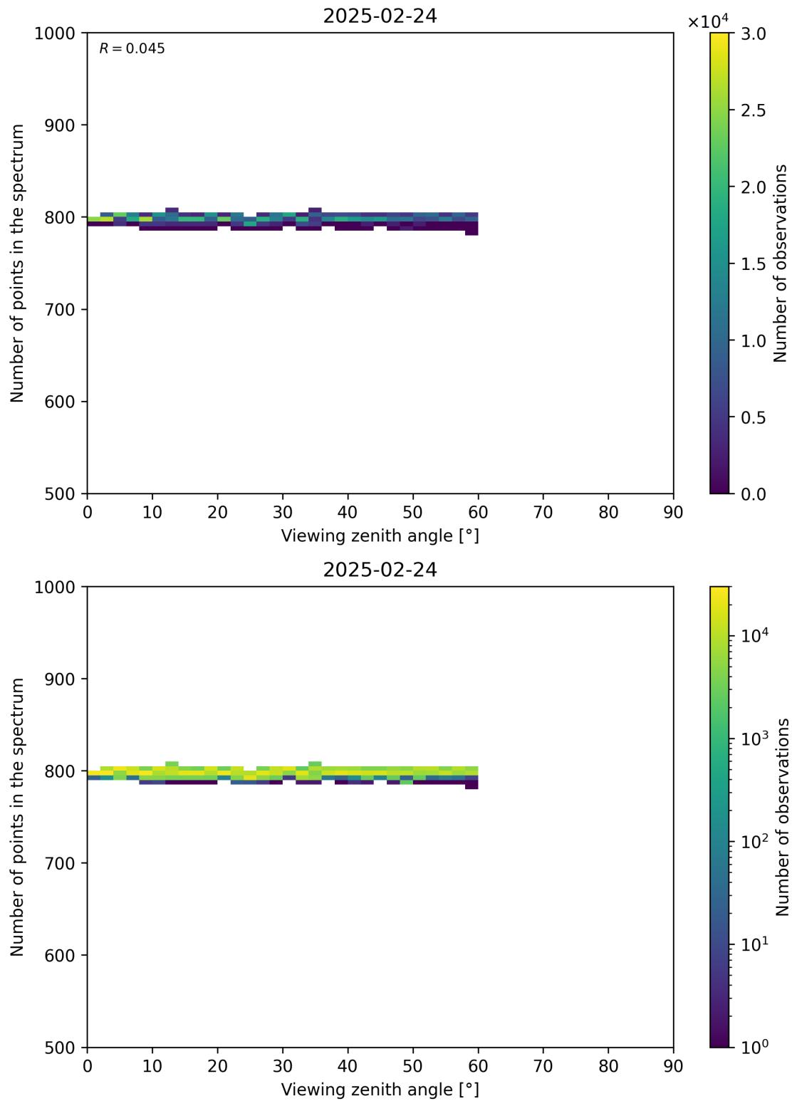
Figure 114: Scatter density plot of “Viewing zenith angle” against “Number of points in the spectrum” for 2025-02-24 to 2025-02-25.
