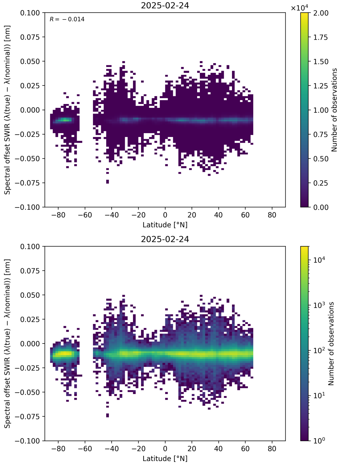
Figure 62: Scatter density plot of “Latitude” against “Spectral offset SWIR ( \lambda_{\text{true}} - \lambda_{\text{nominal}} )” for 2025-02-24 to 2025-02-25.
