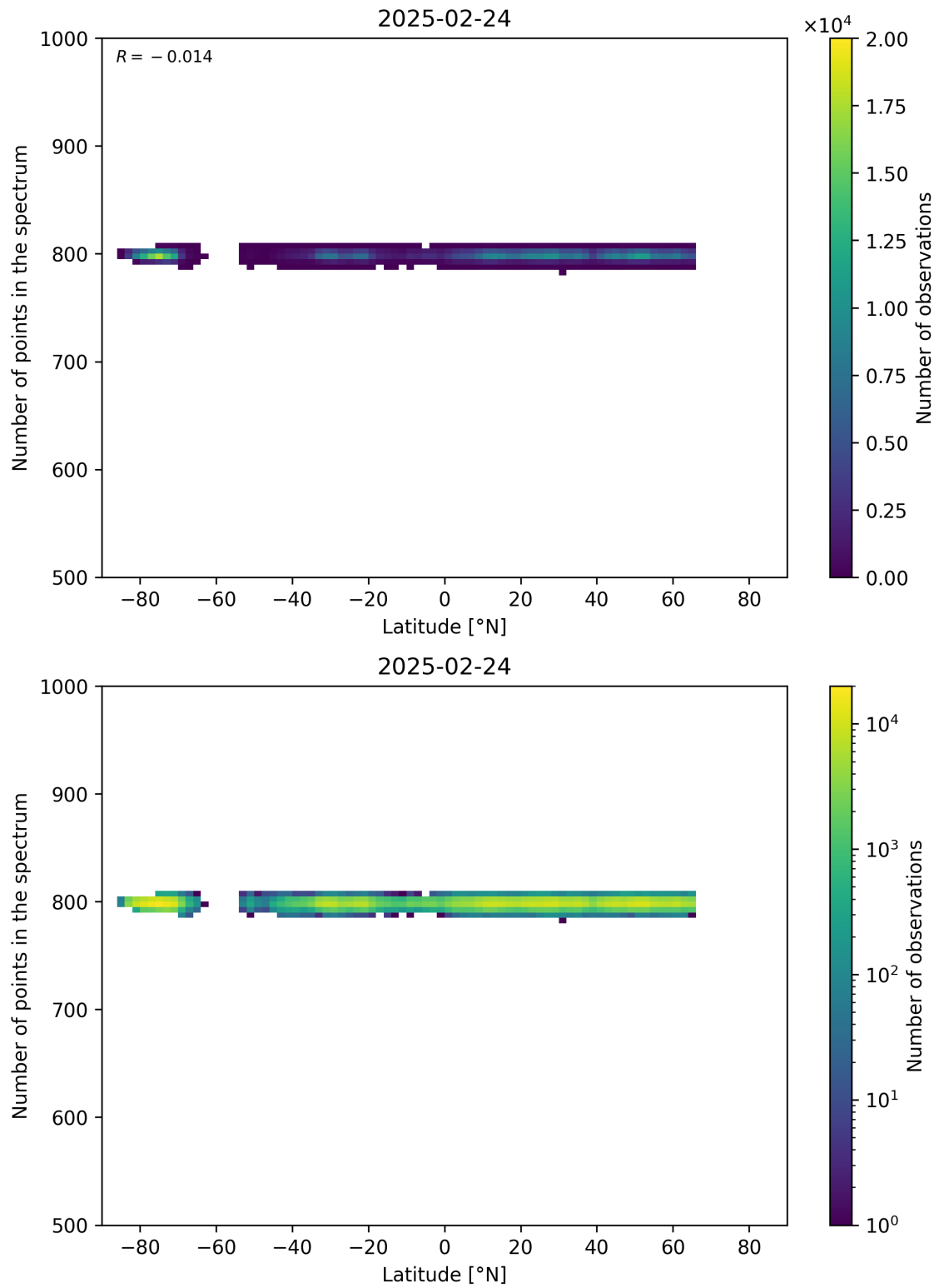
Figure 61: Scatter density plot of “Latitude” against “Number of points in the spectrum” for 2025-02-24 to 2025-02-25.
