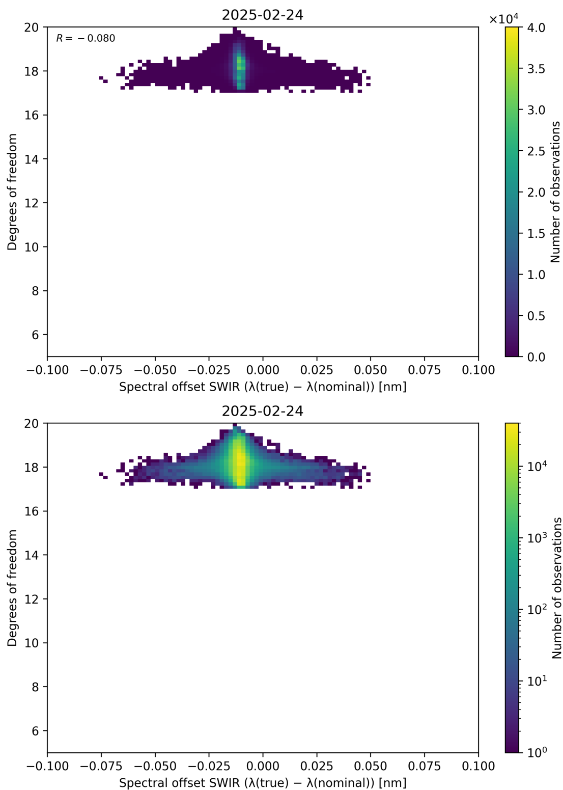
Figure 119: Scatter density plot of “Spectral offset SWIR ( \lambda_{\text{true}} - \lambda_{\text{nominal}} )” against “Degrees of freedom” for 2025-02-24 to 2025-02-25.
