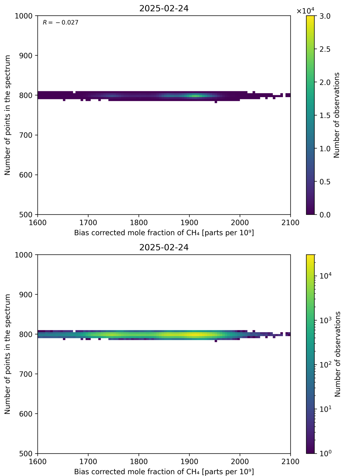
Figure 68: Scatter density plot of “Bias corrected mole fraction of CH 4 ” against “Number of points in the spectrum” for 2025-02-24 to 2025-02-25.
