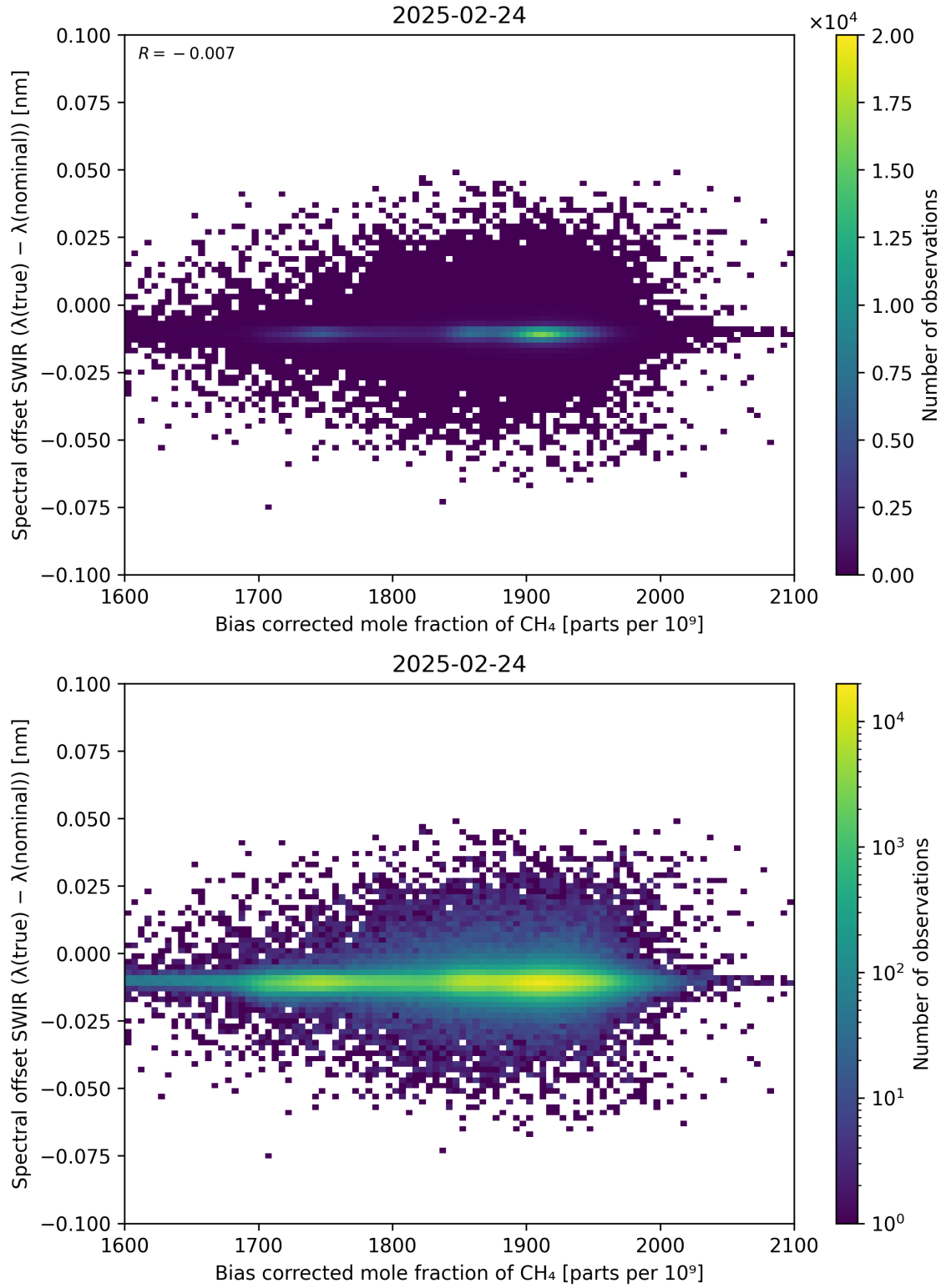
Figure 69: Scatter density plot of “Bias corrected mole fraction of \text{CH}_4 ” against “Spectral offset SWIR ( \lambda_{\text{true}} - \lambda_{\text{nominal}} )” for 2025-02-24 to 2025-02-25.
