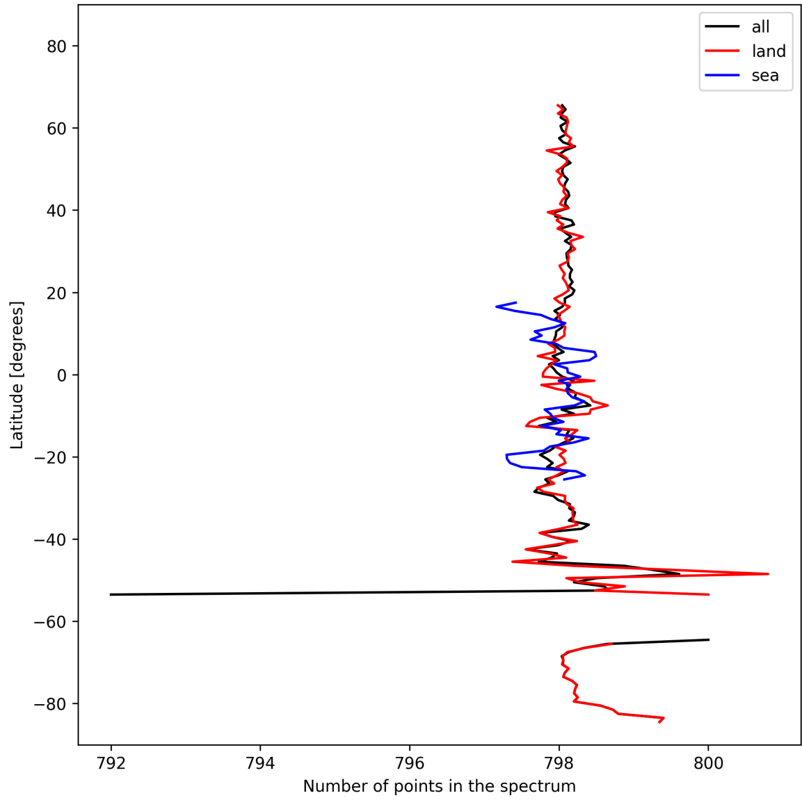
Figure 15: Zonal average of “Number of points in the spectrum” for 2025-02-24 to 2025-02-25.
