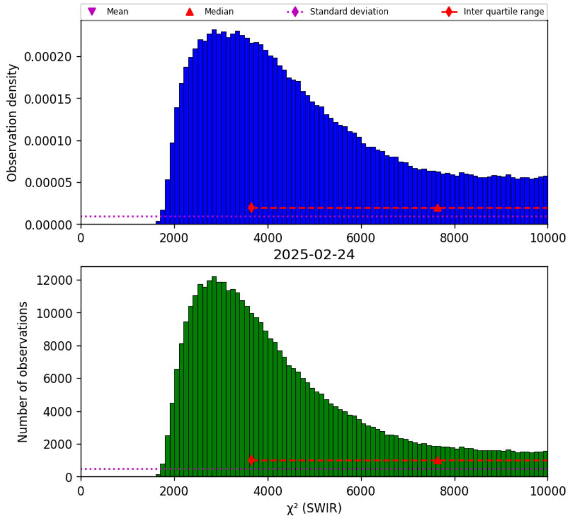
Figure 28: Histogram of “ \chi^2 (SWIR)” for 2025-02-24 to 2025-02-25
