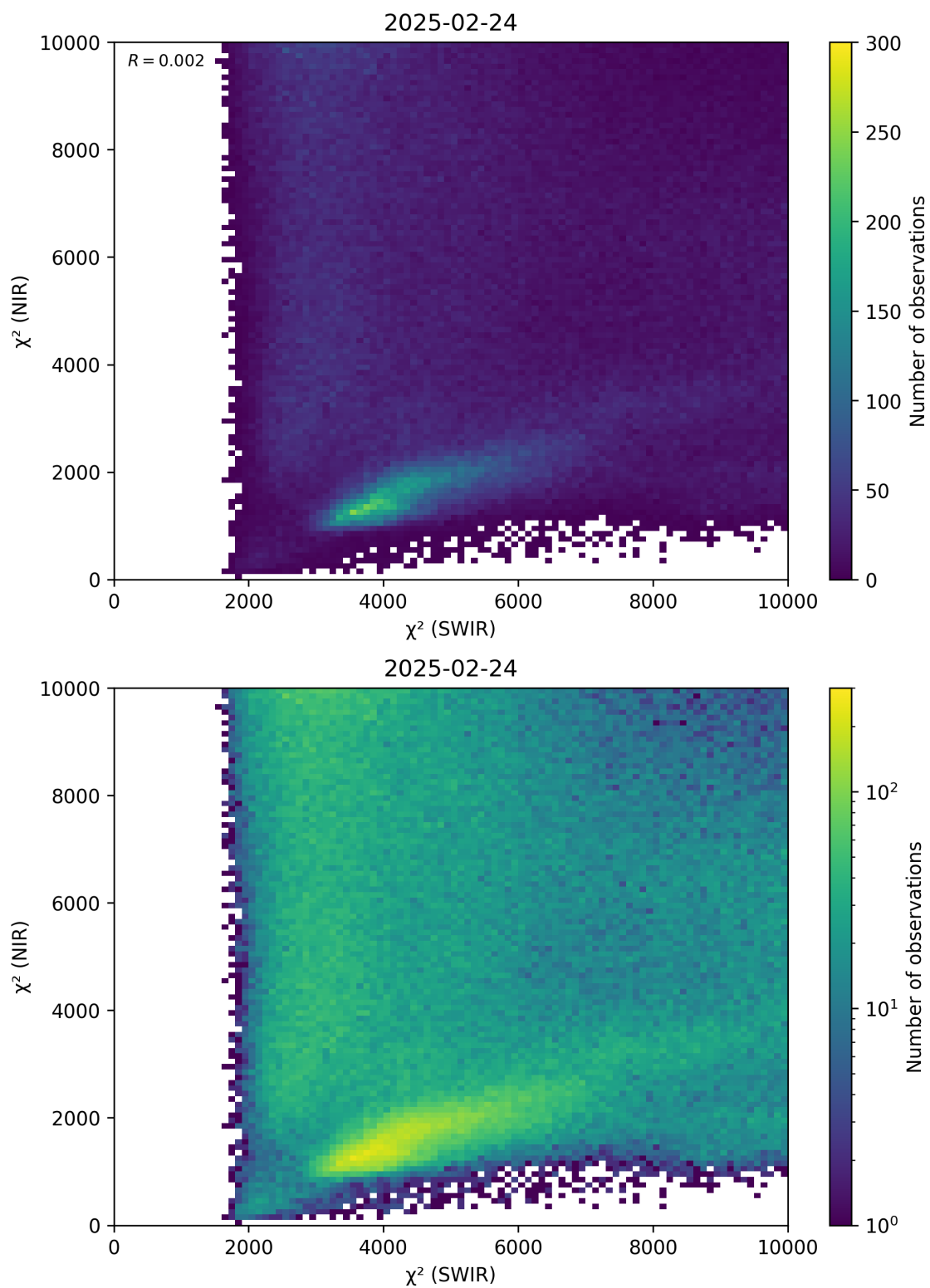
Figure 47: Scatter density plot of “ \chi^2 (SWIR)” against “ \chi^2 (NIR)” for 2025-02-24 to 2025-02-25.
