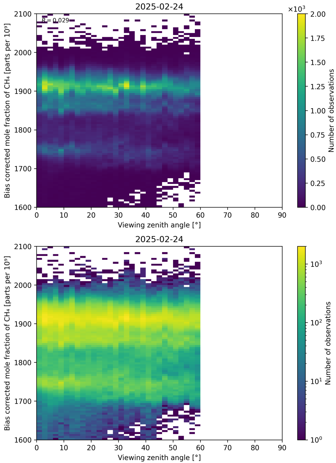
Figure 111: Scatter density plot of “Viewing zenith angle” against “Bias corrected mole fraction of CH 4 ” for 2025-02-24 to 2025-02-25.
