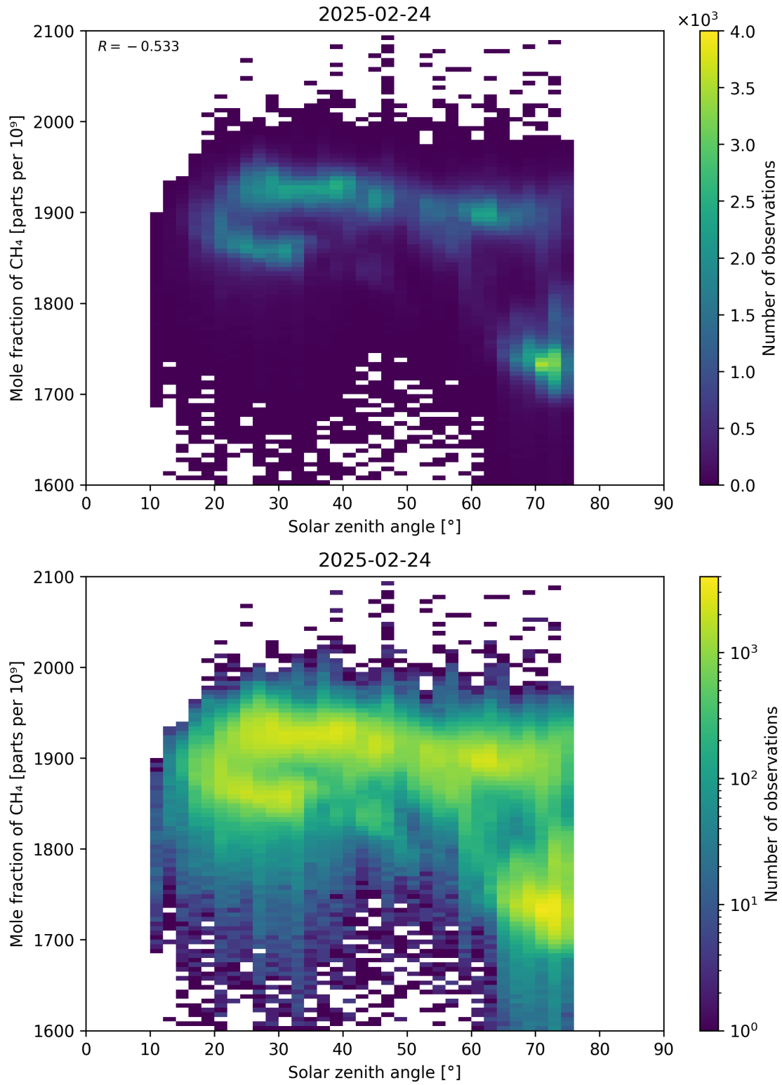
Figure 99: Scatter density plot of “Solar zenith angle” against “Mole fraction of CH 4 ” for 2025-02-24 to 2025-02-25.
