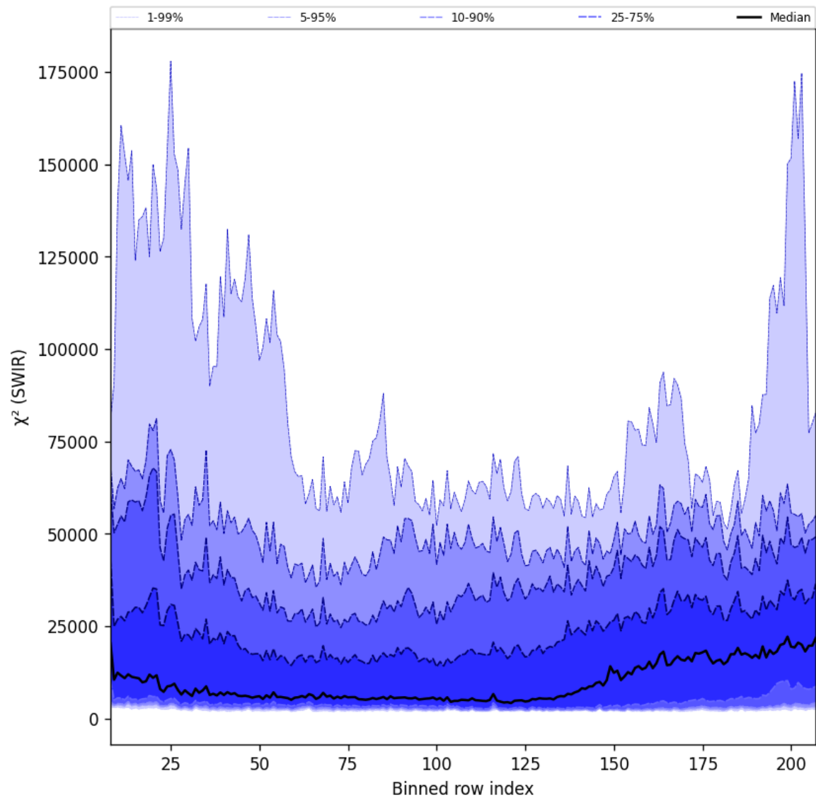
Figure 39: Along track statistics of “ \chi^2 (SWIR)” for 2025-02-24 to 2025-02-25
