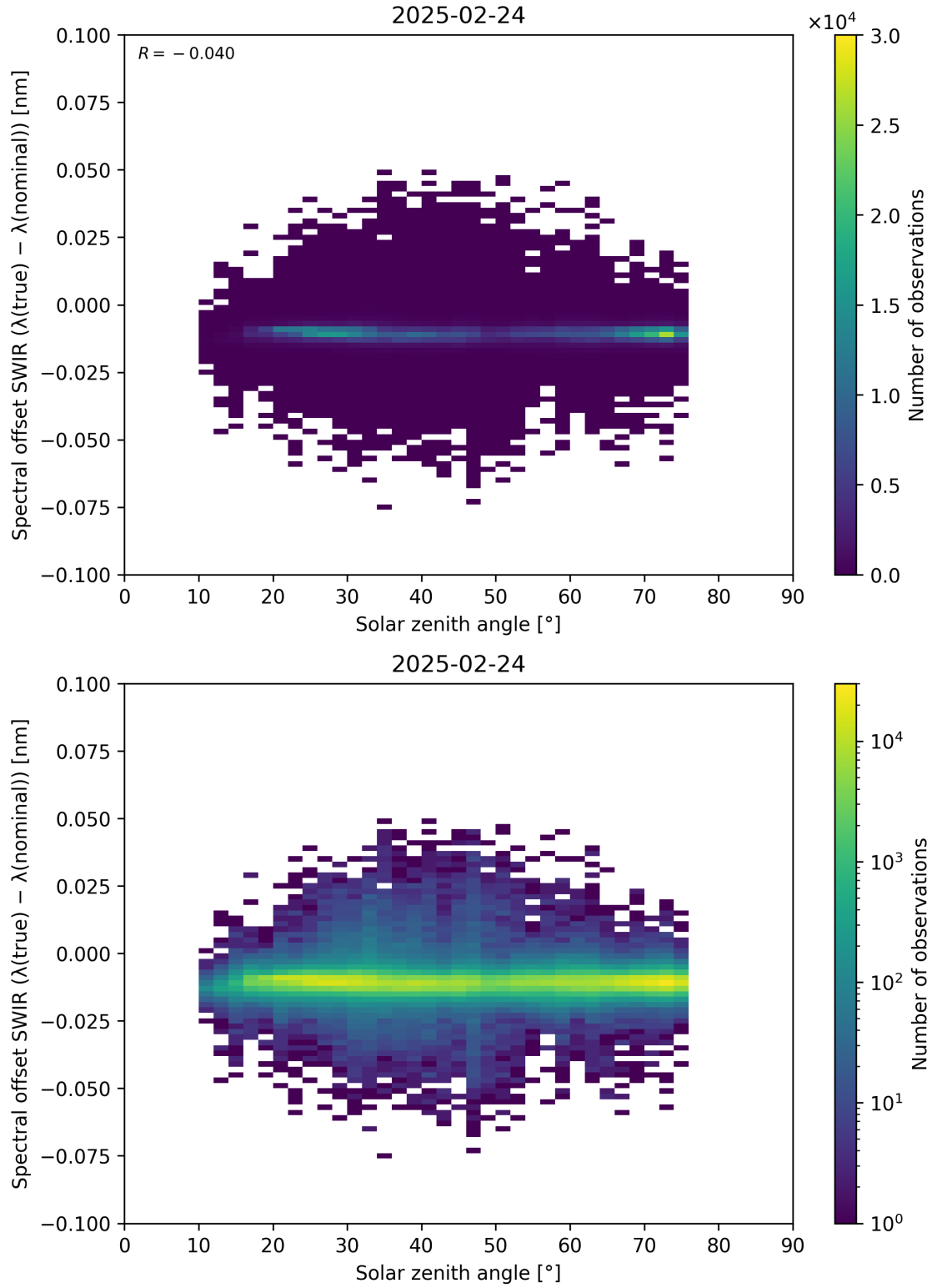
Figure 104: Scatter density plot of “Solar zenith angle” against “Spectral offset SWIR ( \lambda_{\text{true}} - \lambda_{\text{nominal}} )” for 2025-02-24 to 2025-02-25.
