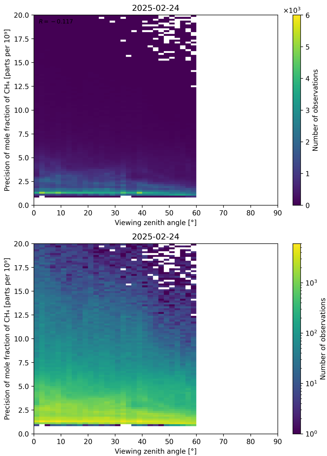
Figure 112: Scatter density plot of “Viewing zenith angle” against “Precision of mole fraction of CH 4 ” for 2025-02-24 to 2025-02-25.
