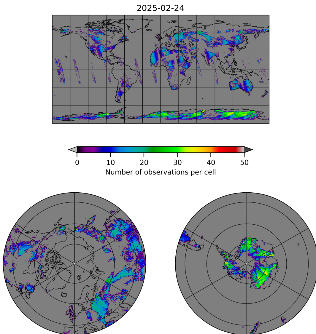
Figure 10: Map of the number of observations for 2025-02-24 to 2025-02-25
