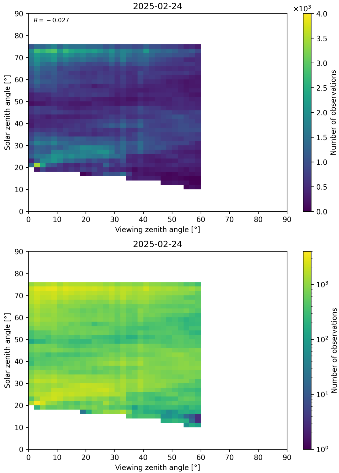
Figure 115: Scatter density plot of “Viewing zenith angle” against “Solar zenith angle” for 2025-02-24 to 2025-02-25.
