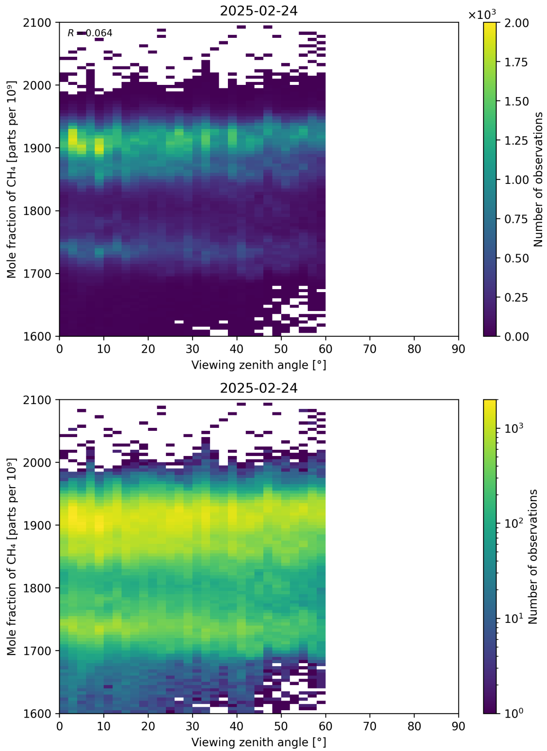
Figure 110: Scatter density plot of “Viewing zenith angle” against “Mole fraction of CH 4 ” for 2025-02-24 to 2025-02-25.
