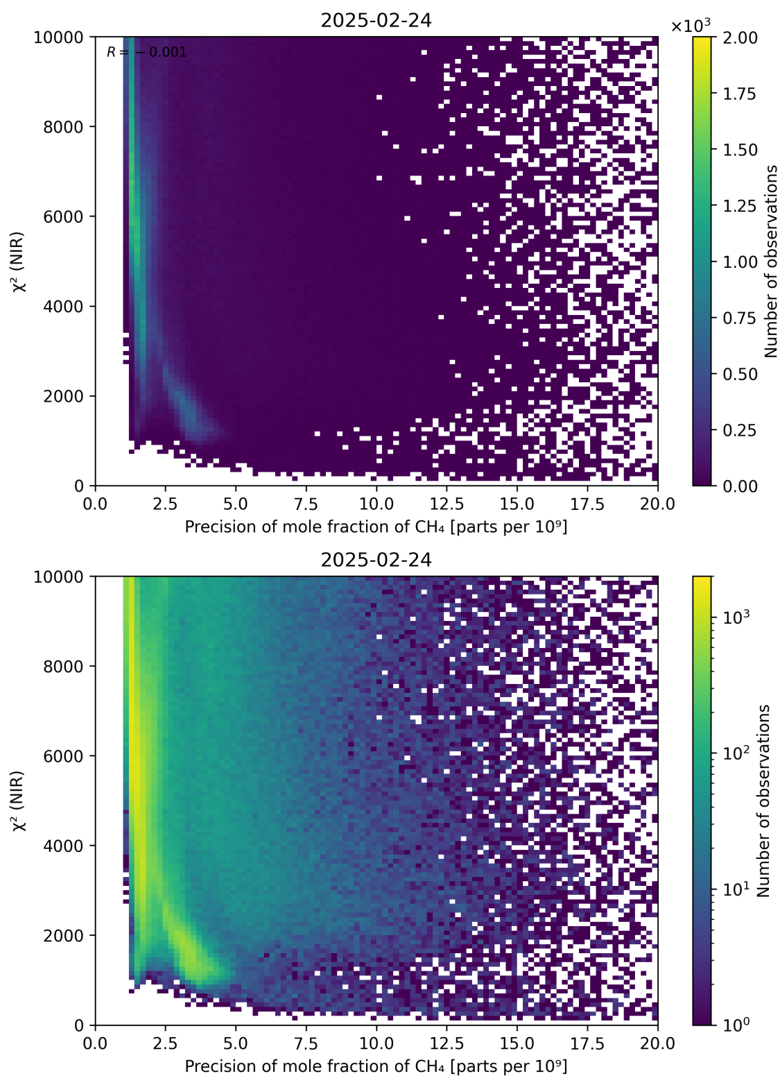
Figure 78: Scatter density plot of “Precision of mole fraction of \text{CH}_4 ” against “ \chi^2 (NIR)” for 2025-02-24 to 2025-02-25.
