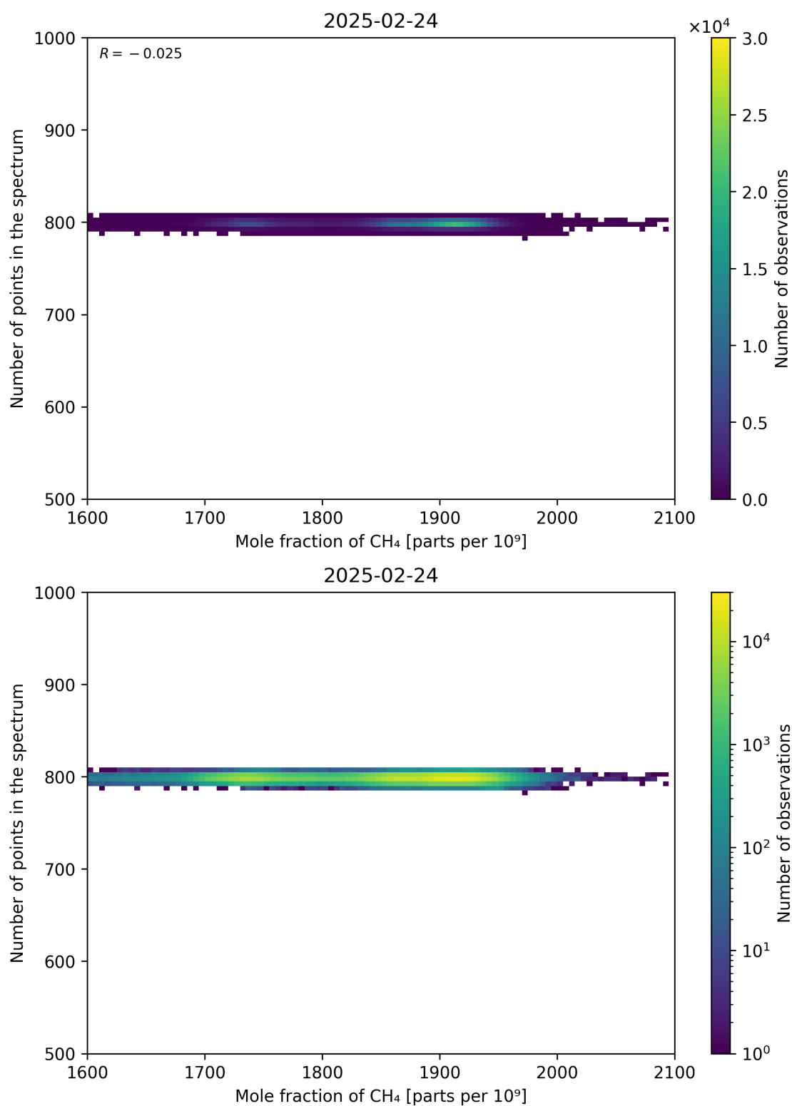
Figure 77: Scatter density plot of “Mole fraction of CH 4 ” against “Number of points in the spectrum” for 2025-02-24 to 2025-02-25.
