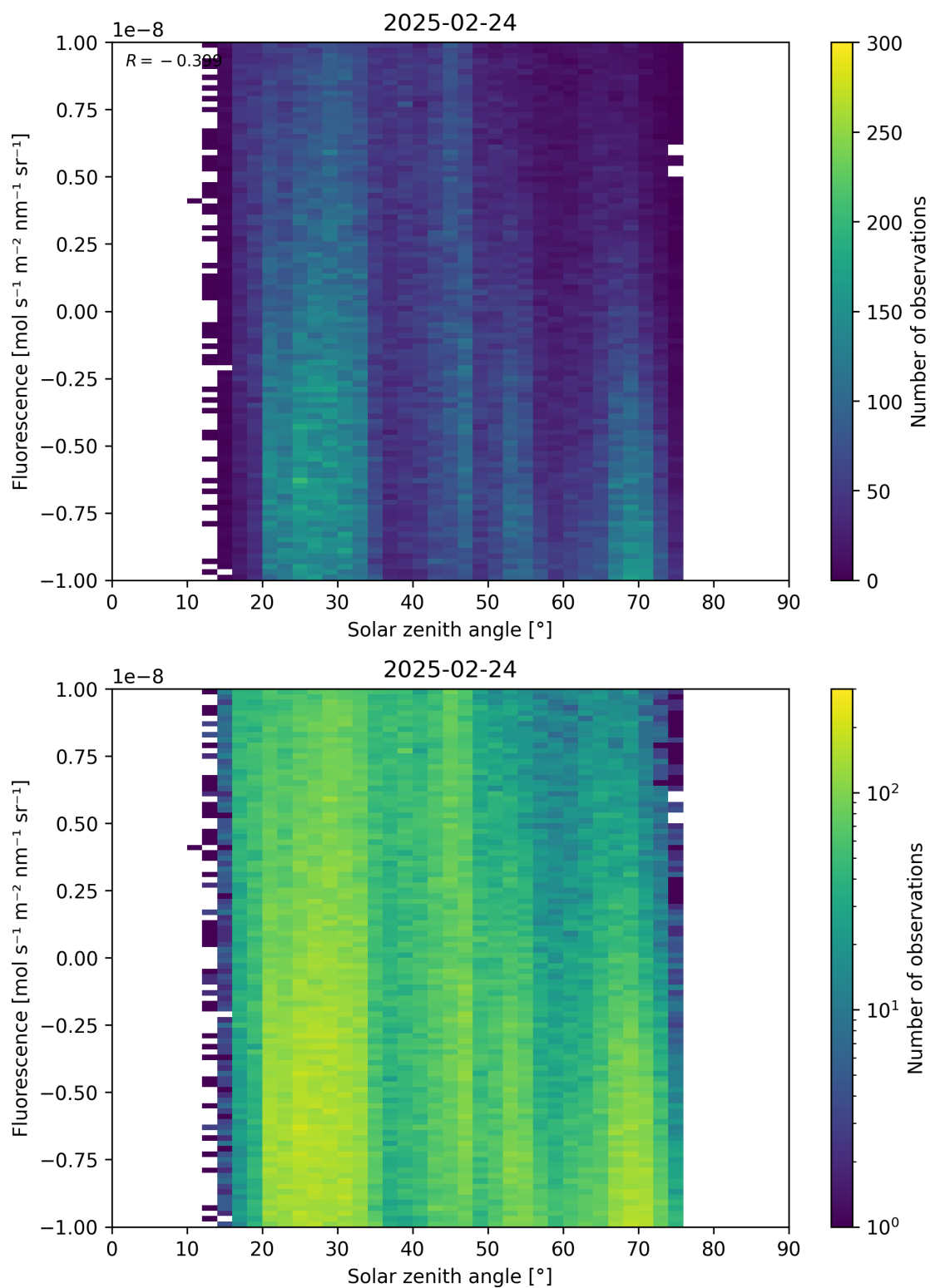
Figure 97: Scatter density plot of “Solar zenith angle” against “Fluorescence” for 2025-02-24 to 2025-02-25.
