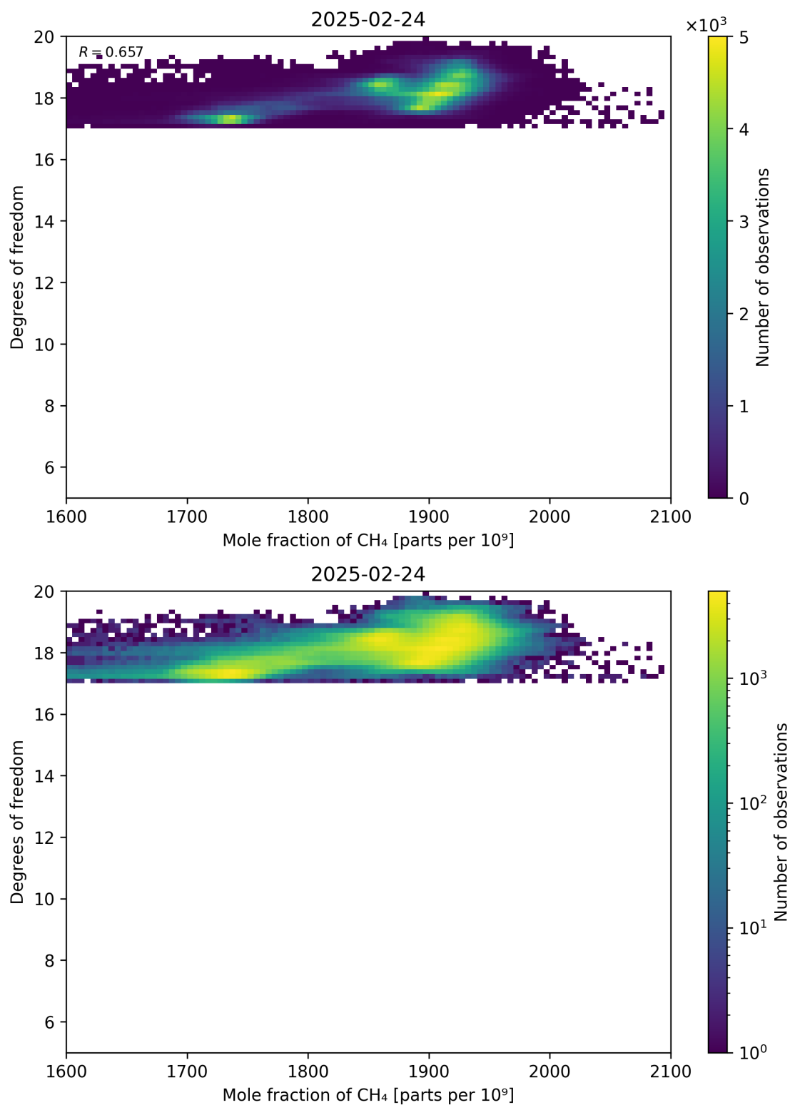
Figure 72: Scatter density plot of “Mole fraction of CH 4 ” against “Degrees of freedom” for 2025-02-24 to 2025-02-25.
