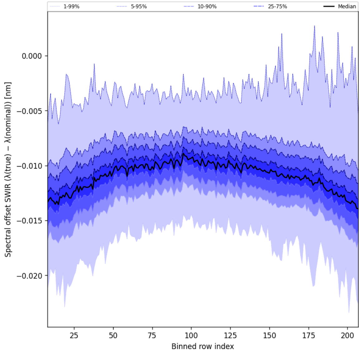
Figure 38: Along track statistics of “Spectral offset SWIR ( \lambda_{\text{true}} - \lambda_{\text{nominal}} )” for 2025-02-24 to 2025-02-25
