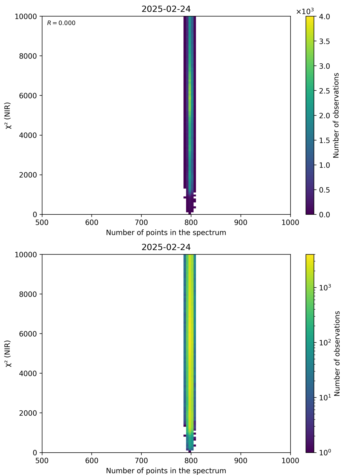
Figure 88: Scatter density plot of “Number of points in the spectrum” against “ \chi^2 (NIR)” for 2025-02-24 to 2025-02-25.
