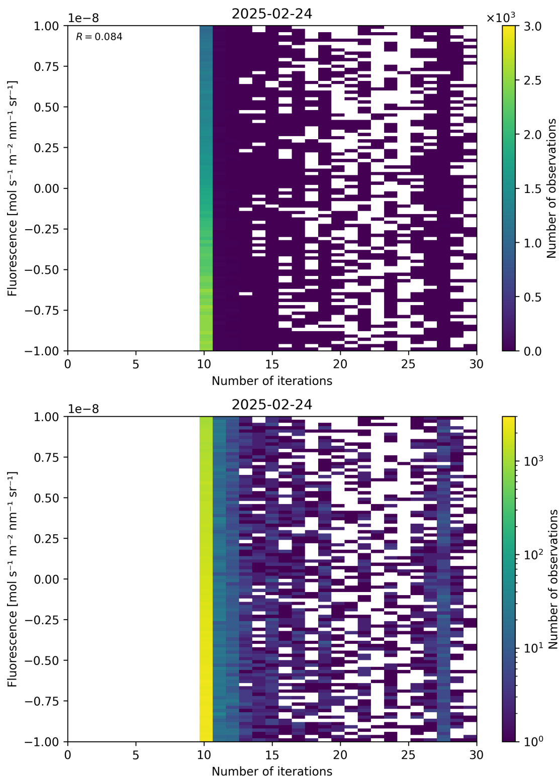
Figure 87: Scatter density plot of “Number of iterations” against “Fluorescence” for 2025-02-24 to 2025-02-25.
