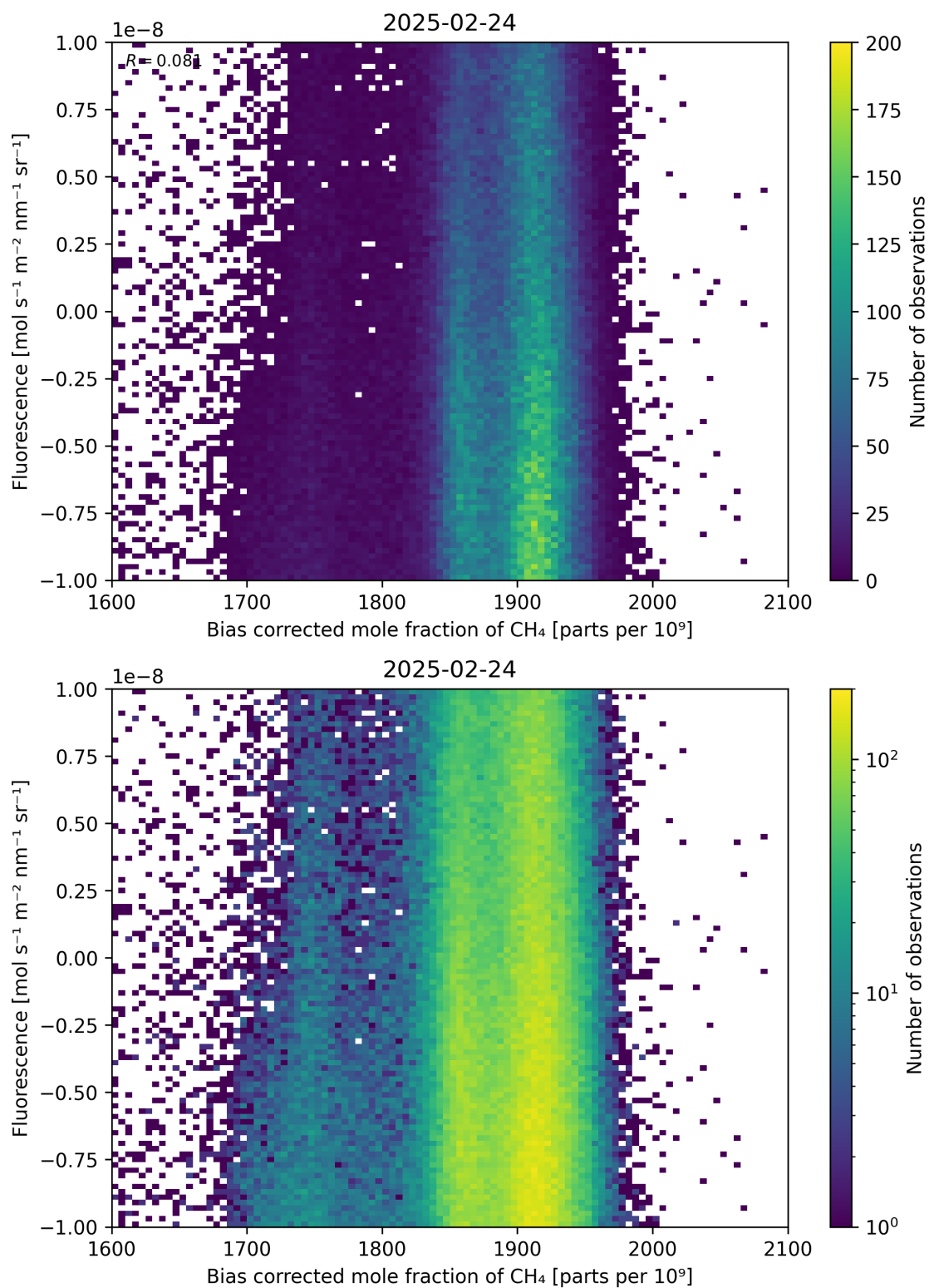
Figure 66: Scatter density plot of “Bias corrected mole fraction of \text{CH}_4 ” against “Fluorescence” for 2025-02-24 to 2025-02-25.
