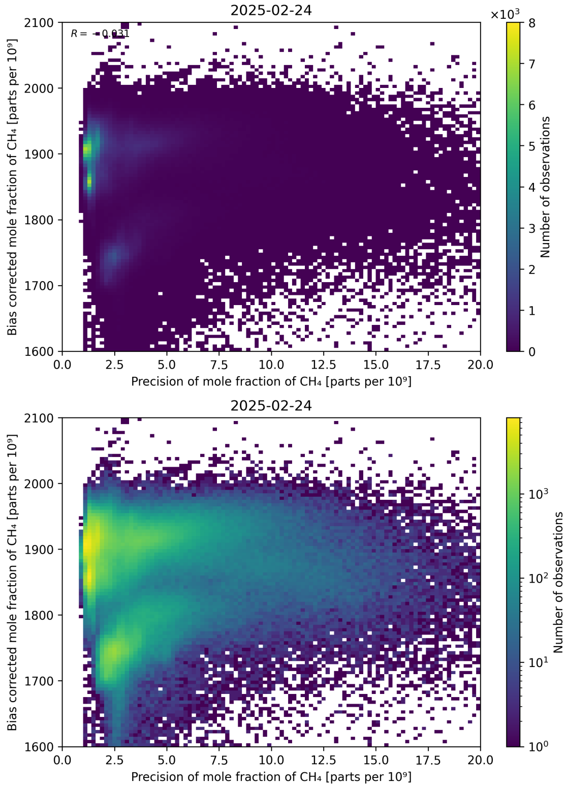
Figure 82: Scatter density plot of “Precision of mole fraction of CH 4 ” against “Bias corrected mole fraction of CH 4 ” for 2025-02-24 to 2025-02-25.
