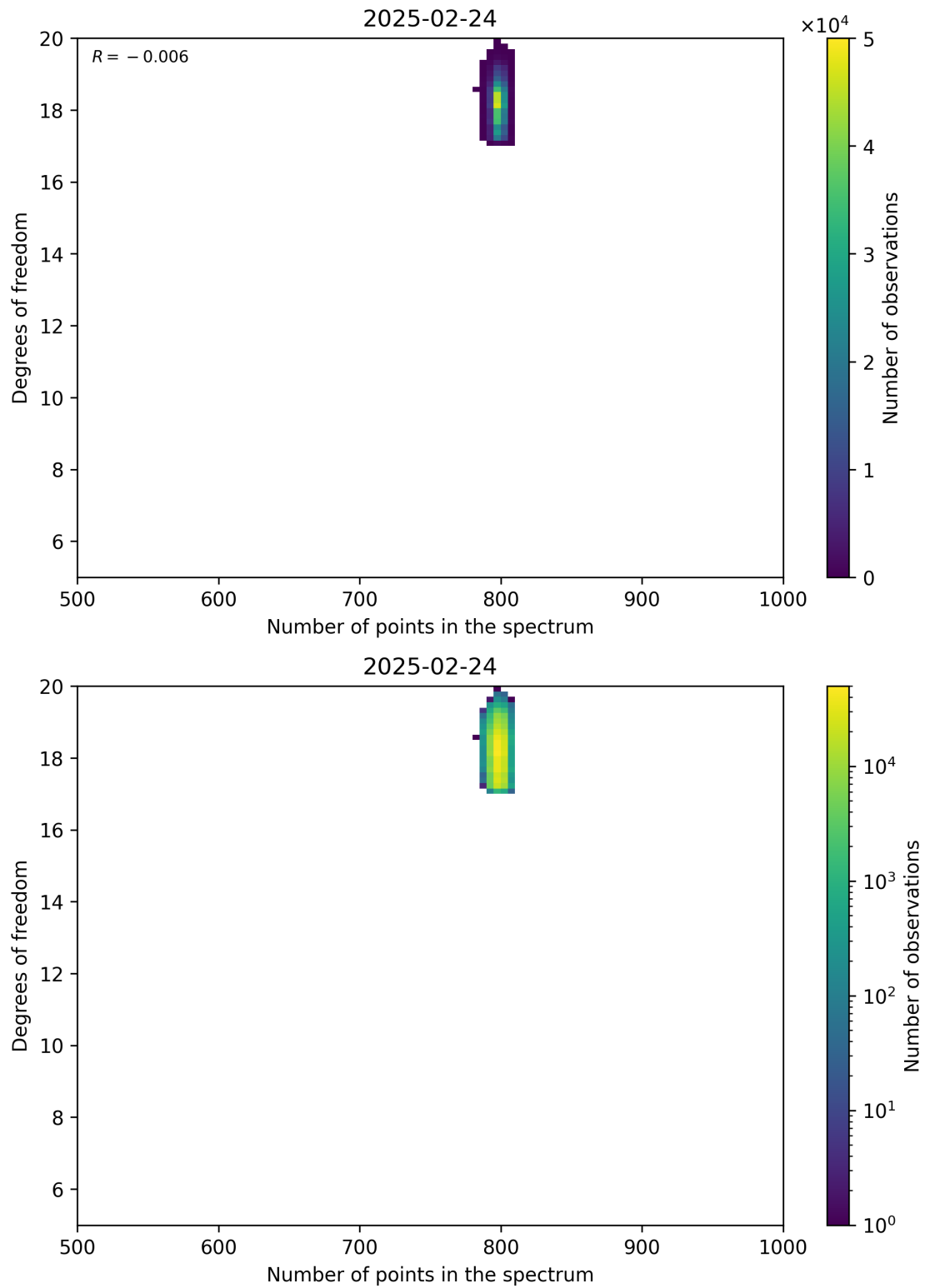
Figure 90: Scatter density plot of “Number of points in the spectrum” against “Degrees of freedom” for 2025-02-24 to 2025-02-25.
