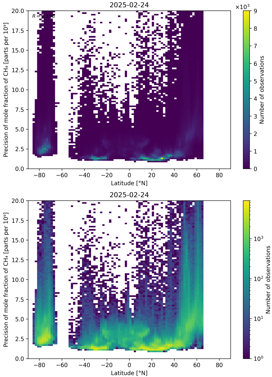
Figure 59: Scatter density plot of “Latitude” against “Precision of mole fraction of CH 4 ” for 2025-02-24 to 2025-02-25.
