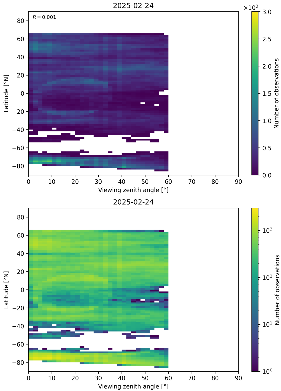
Figure 109: Scatter density plot of “Viewing zenith angle” against “Latitude” for 2025-02-24 to 2025-02-25.
