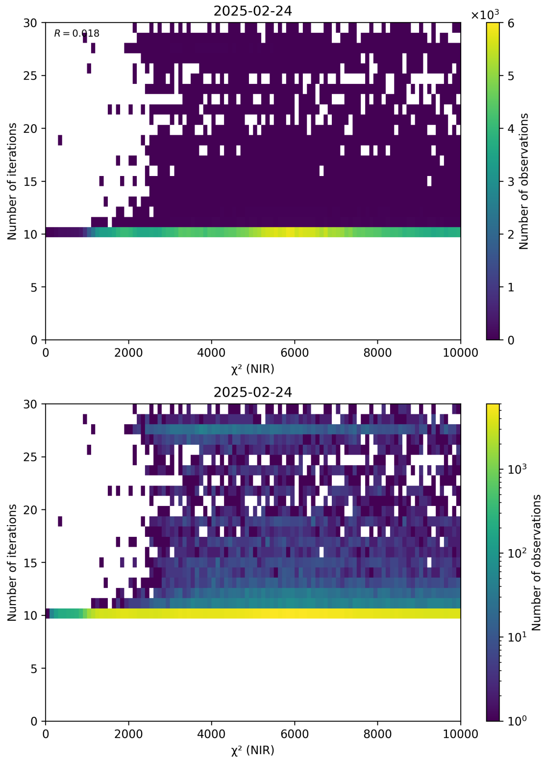
Figure 46: Scatter density plot of “ \chi^2 (NIR)” against “Number of iterations” for 2025-02-24 to 2025-02-25.
