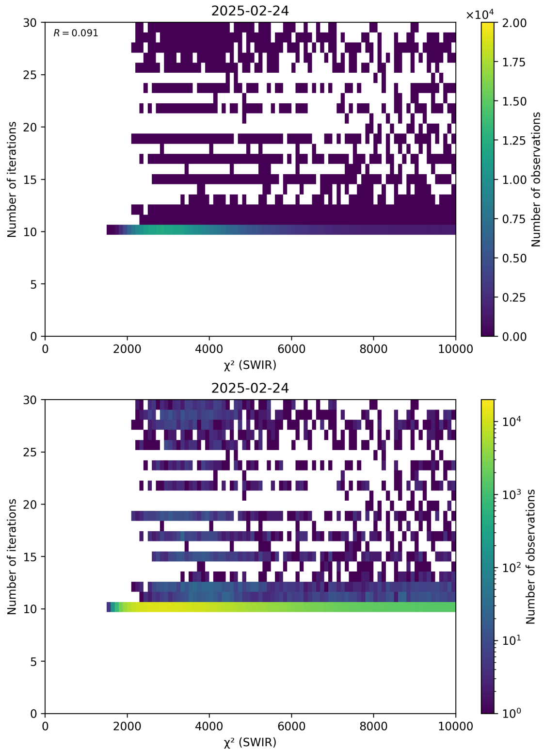
Figure 50: Scatter density plot of “ \chi^2 (SWIR)” against “Number of iterations” for 2025-02-24 to 2025-02-25.
