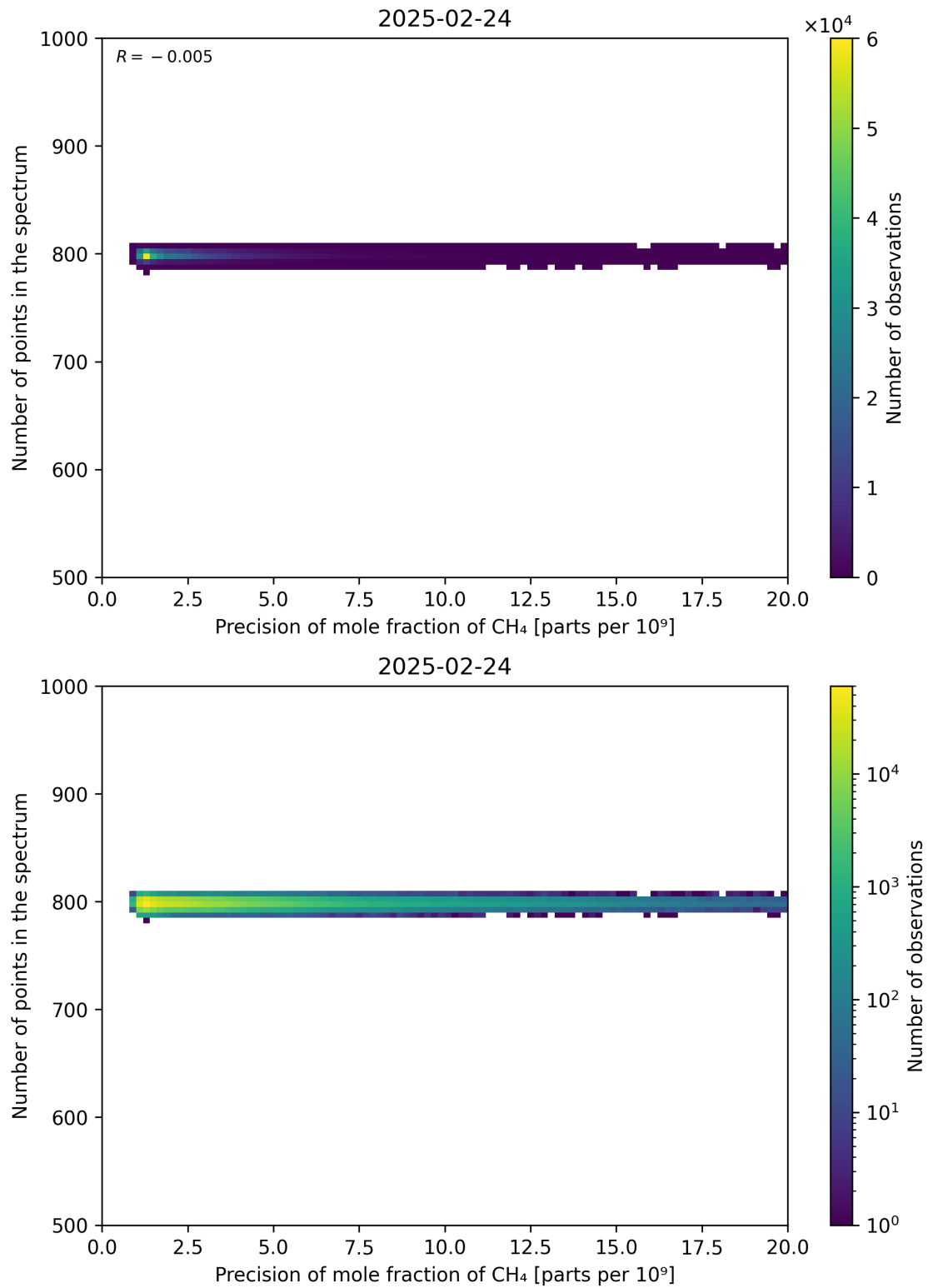
Figure 84: Scatter density plot of “Precision of mole fraction of CH 4 ” against “Number of points in the spectrum” for 2025-02-24 to 2025-02-25.
