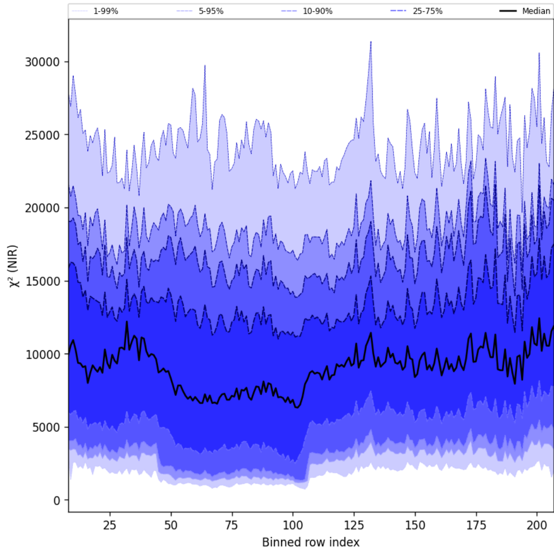
Figure 40: Along track statistics of “ \chi^2 (NIR)” for 2025-02-24 to 2025-02-26
