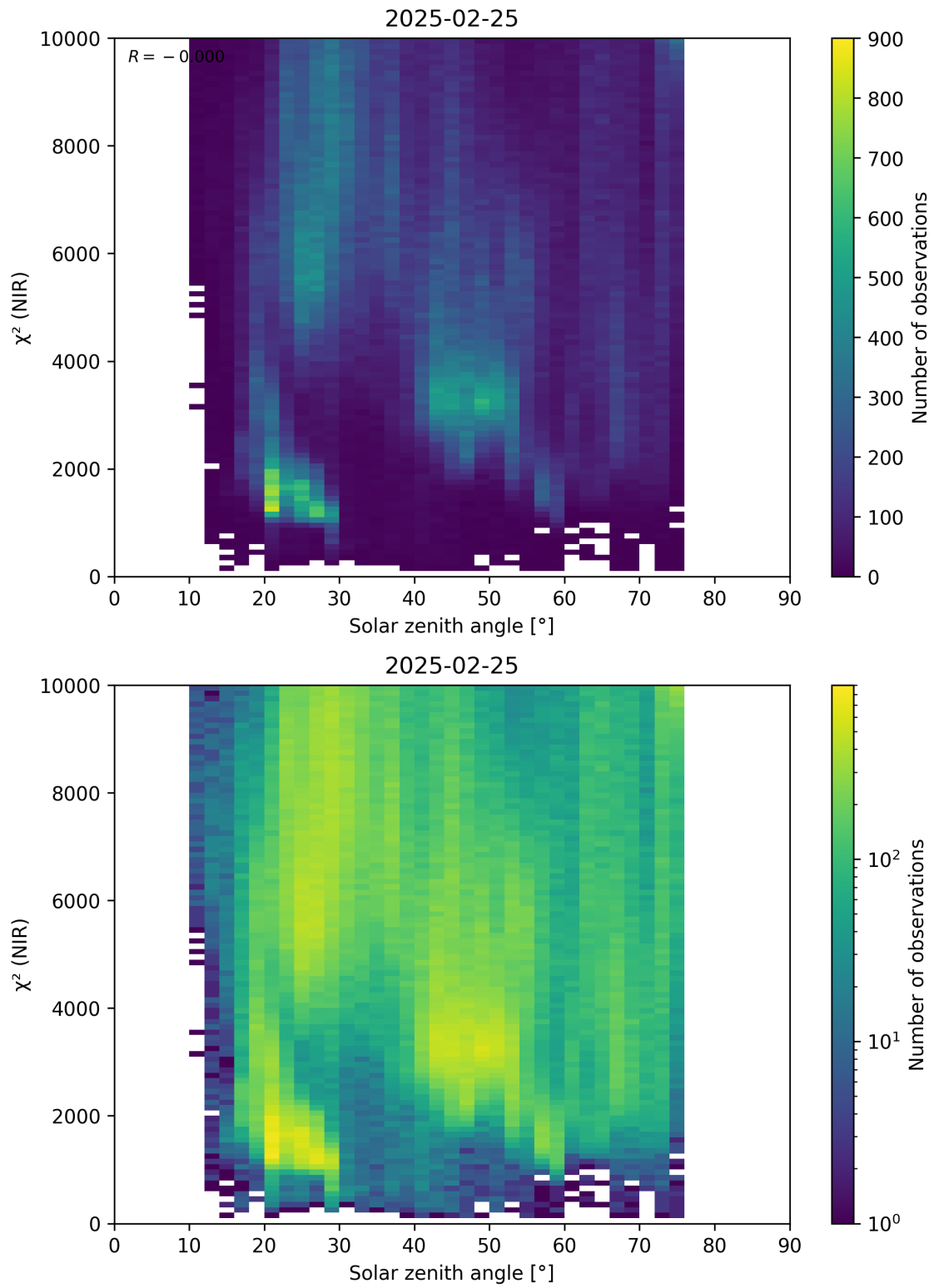
Figure 94: Scatter density plot of “Solar zenith angle” against “ \chi^2 (NIR)” for 2025-02-24 to 2025-02-26.
