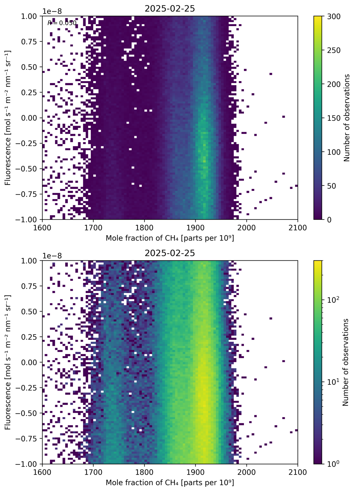
Figure 73: Scatter density plot of “Mole fraction of \text{CH}_4 ” against “Fluorescence” for 2025-02-24 to 2025-02-26.
