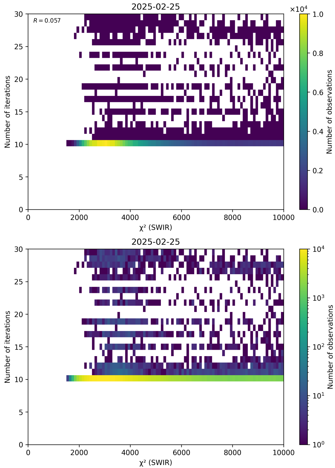
Figure 50: Scatter density plot of “ \chi^2 (SWIR)” against “Number of iterations” for 2025-02-24 to 2025-02-26.
