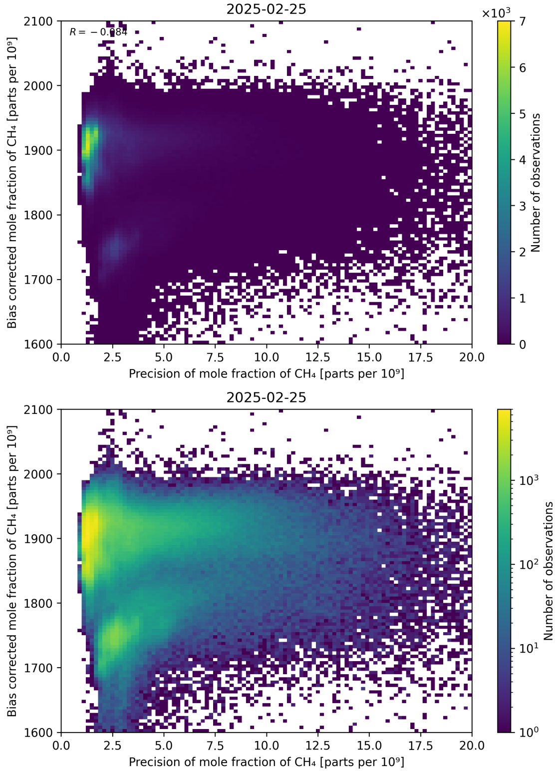
Figure 82: Scatter density plot of “Precision of mole fraction of CH 4 ” against “Bias corrected mole fraction of CH 4 ” for 2025-02-24 to 2025-02-26.
