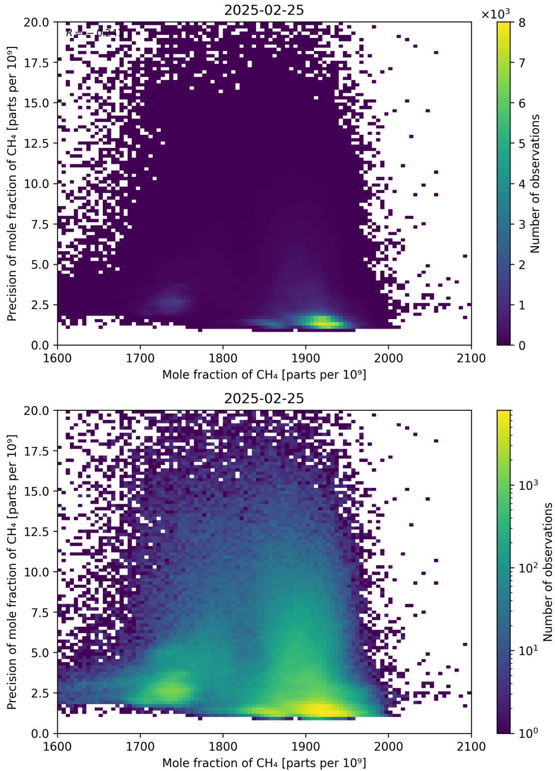
Figure 75: Scatter density plot of “Mole fraction of CH 4 ” against “Precision of mole fraction of CH 4 ” for 2025-02-24 to 2025-02-26.
