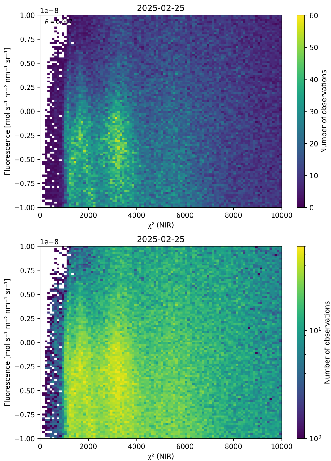
Figure 45: Scatter density plot of “ \chi^2 (NIR)” against “Fluorescence” for 2025-02-24 to 2025-02-26.
