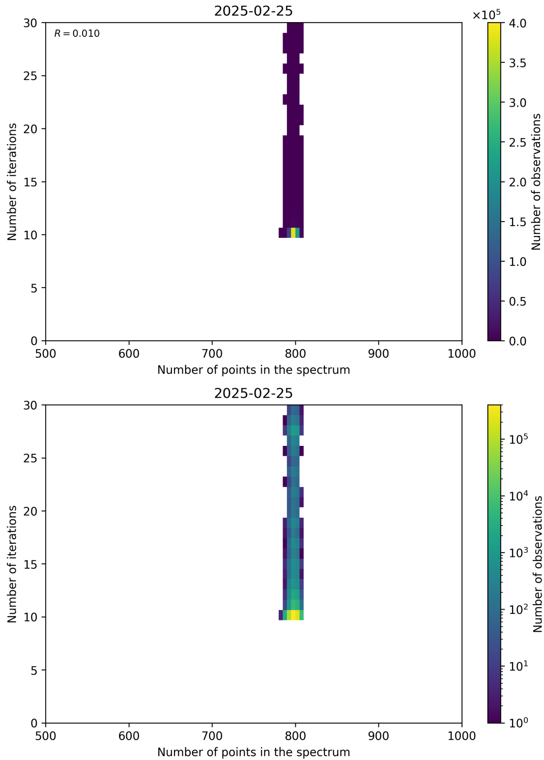
Figure 92: Scatter density plot of “Number of points in the spectrum” against “Number of iterations” for 2025-02-24 to 2025-02-26.
