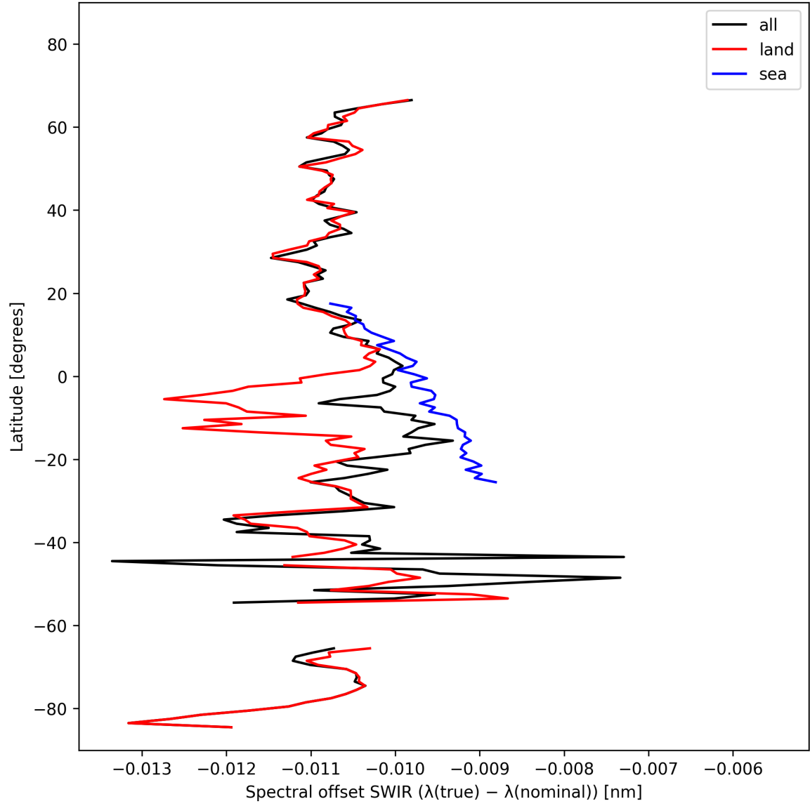
Figure 16: Zonal average of “Spectral offset SWIR ( \lambda_{\text{true}} - \lambda_{\text{nominal}} )” for 2025-02-24 to 2025-02-26.
