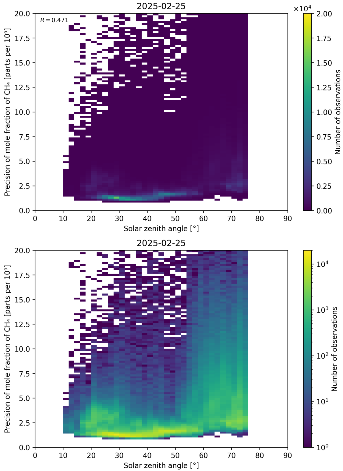
Figure 101: Scatter density plot of “Solar zenith angle” against “Precision of mole fraction of \text{CH}_4 ” for 2025-02-24 to 2025-02-26.
