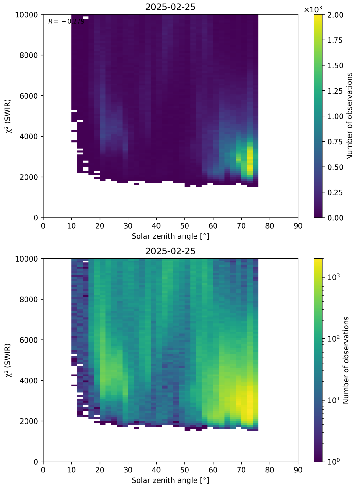
Figure 95: Scatter density plot of “Solar zenith angle” against “ \chi^2 (SWIR)” for 2025-02-24 to 2025-02-26.
