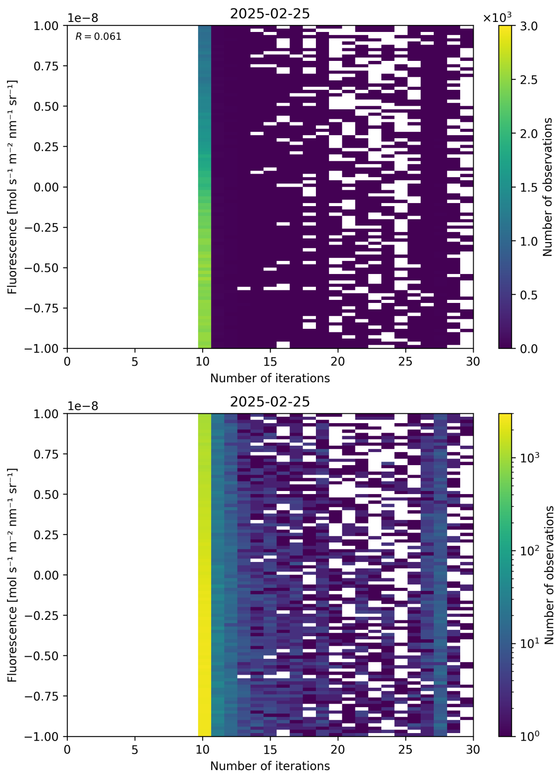
Figure 87: Scatter density plot of “Number of iterations” against “Fluorescence” for 2025-02-24 to 2025-02-26.
