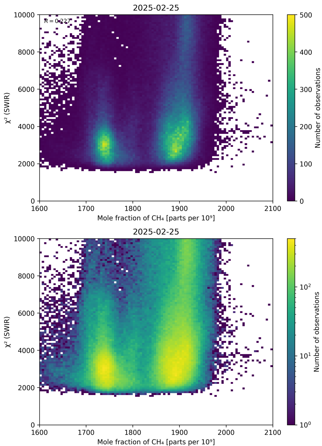
Figure 71: Scatter density plot of “Mole fraction of \text{CH}_4 ” against “ \chi^2 (SWIR)” for 2025-02-24 to 2025-02-26.
