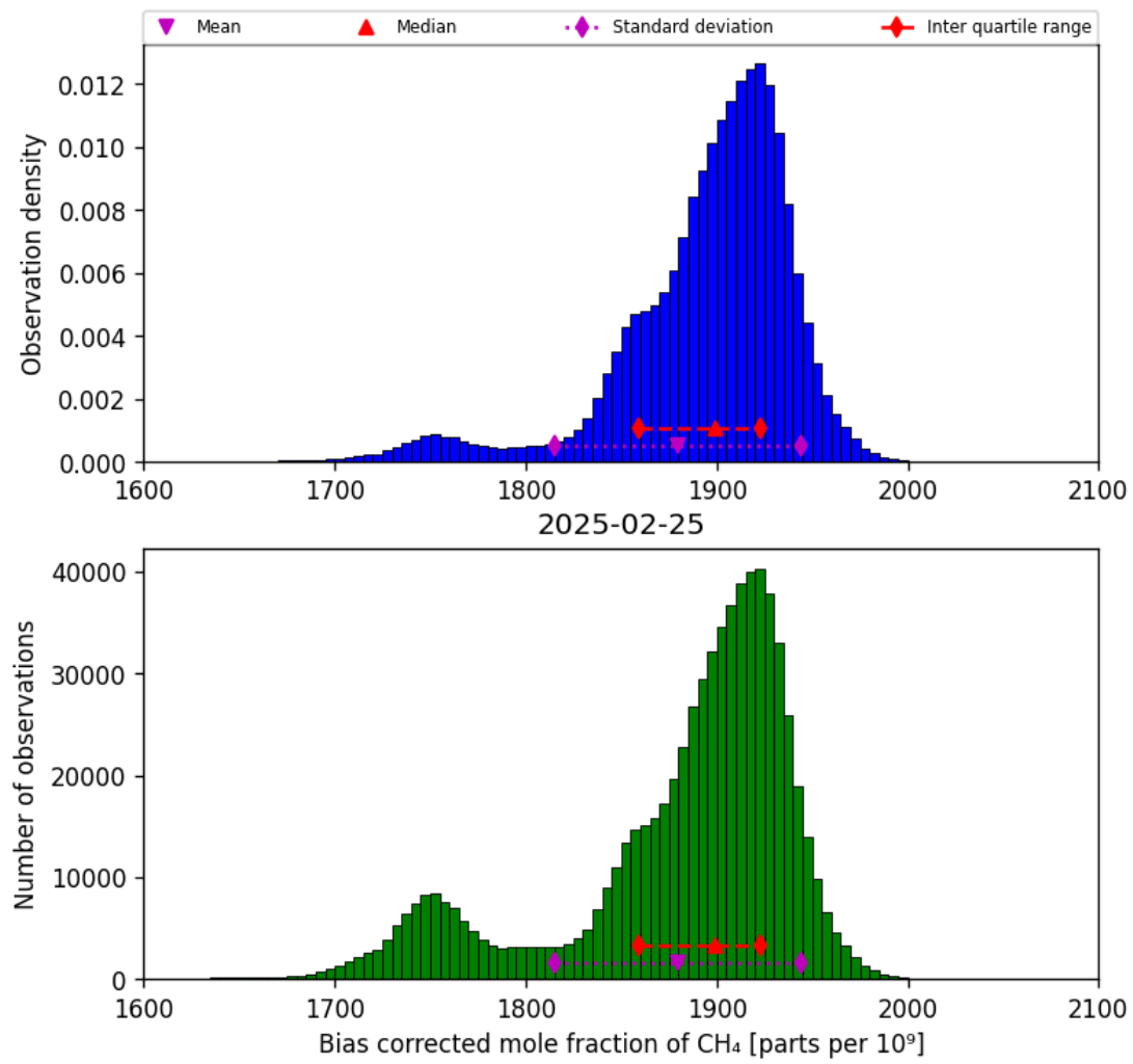
Figure 25: Histogram of “Bias corrected mole fraction of CH 4 ” for 2025-02-24 to 2025-02-26
