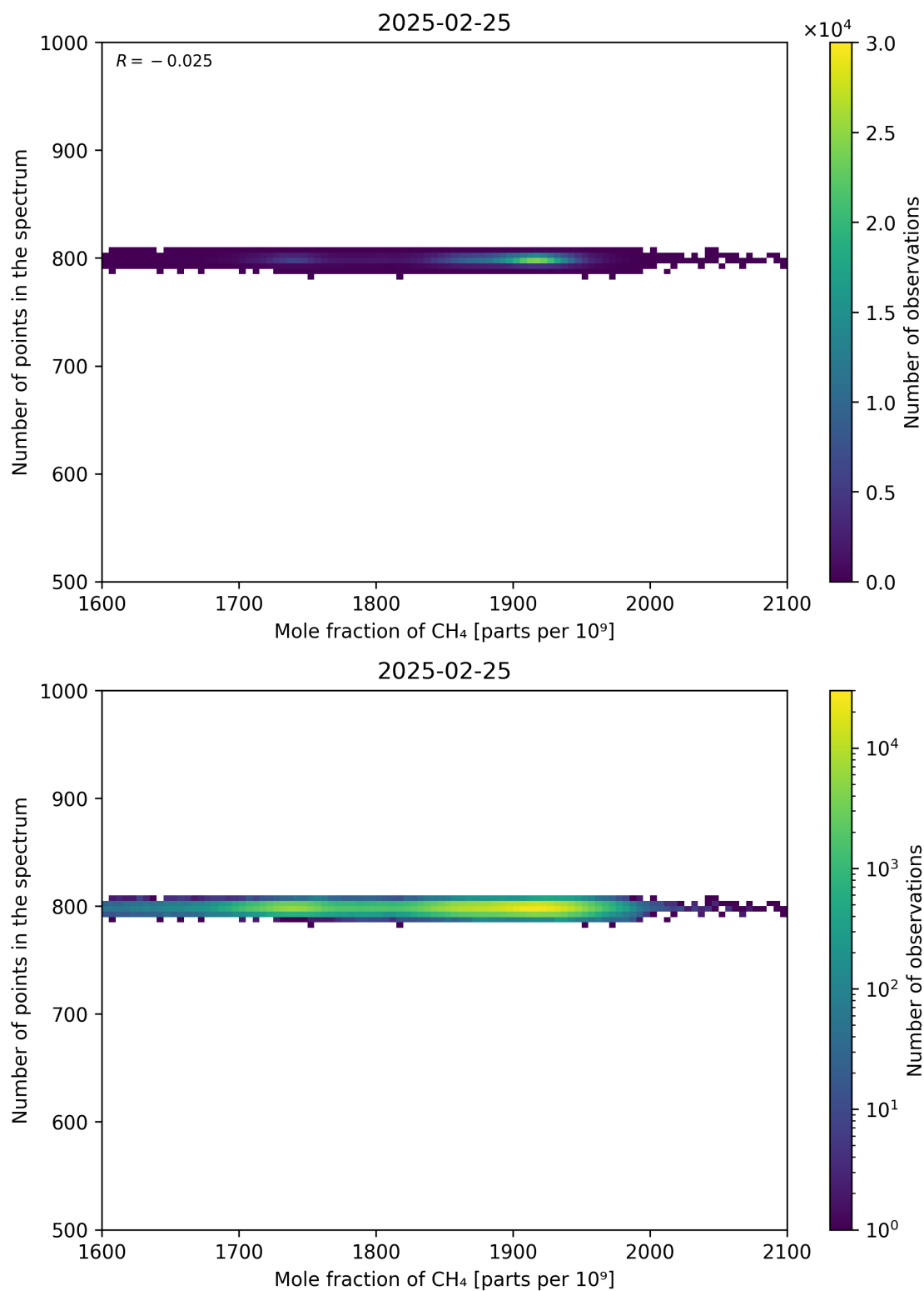
Figure 77: Scatter density plot of “Mole fraction of CH 4 ” against “Number of points in the spectrum” for 2025-02-24 to 2025-02-26.
