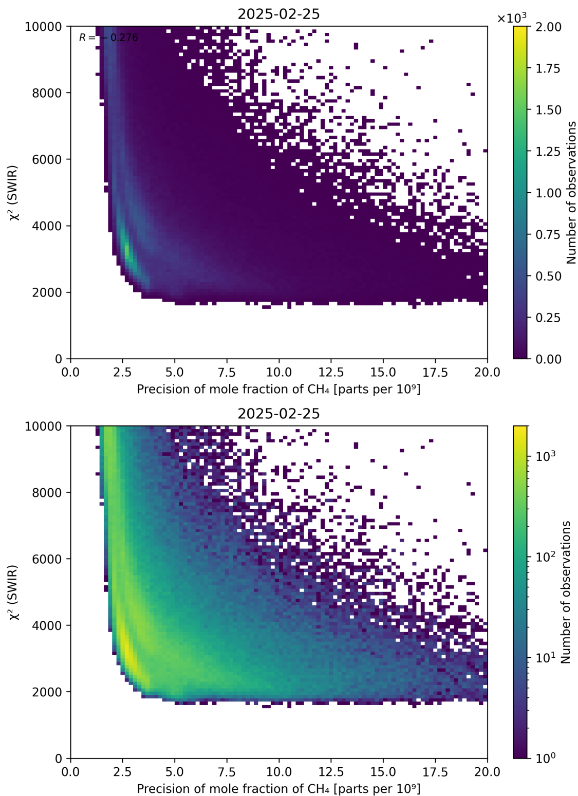
Figure 79: Scatter density plot of “Precision of mole fraction of CH 4 ” against “ \chi^2 (SWIR)” for 2025-02-24 to 2025-02-26.
