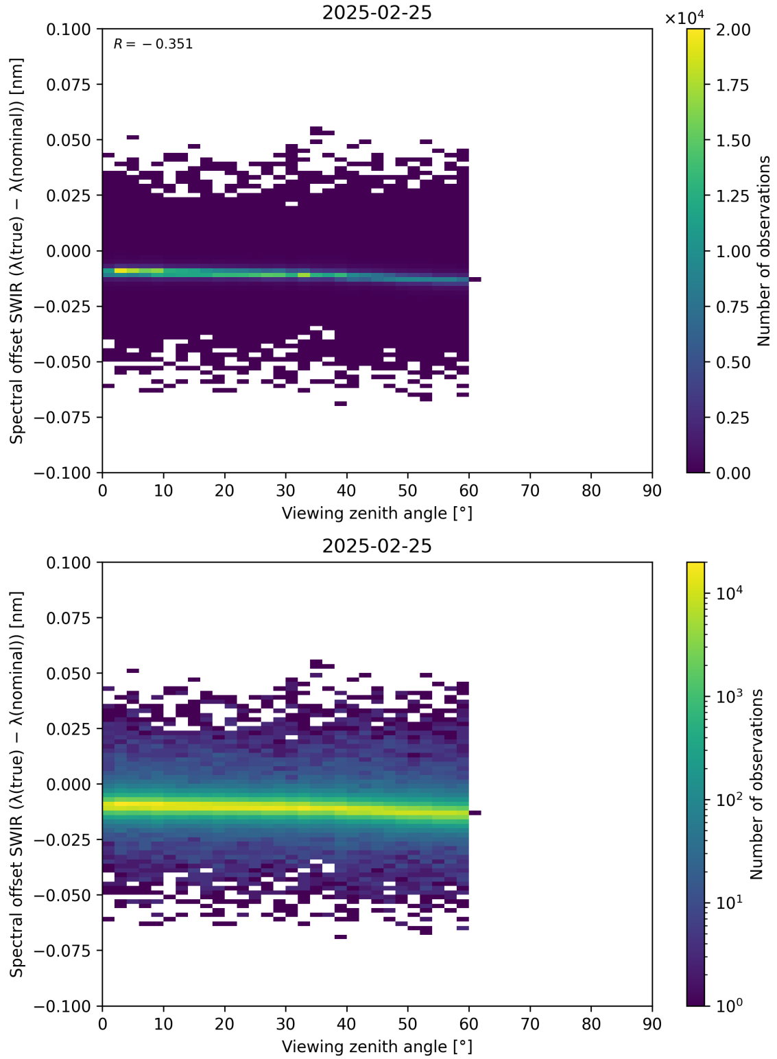
Figure 116: Scatter density plot of “Viewing zenith angle” against “Spectral offset SWIR ( \lambda_{\text{true}} - \lambda_{\text{nominal}} )” for 2025-02-24 to 2025-02-26.
