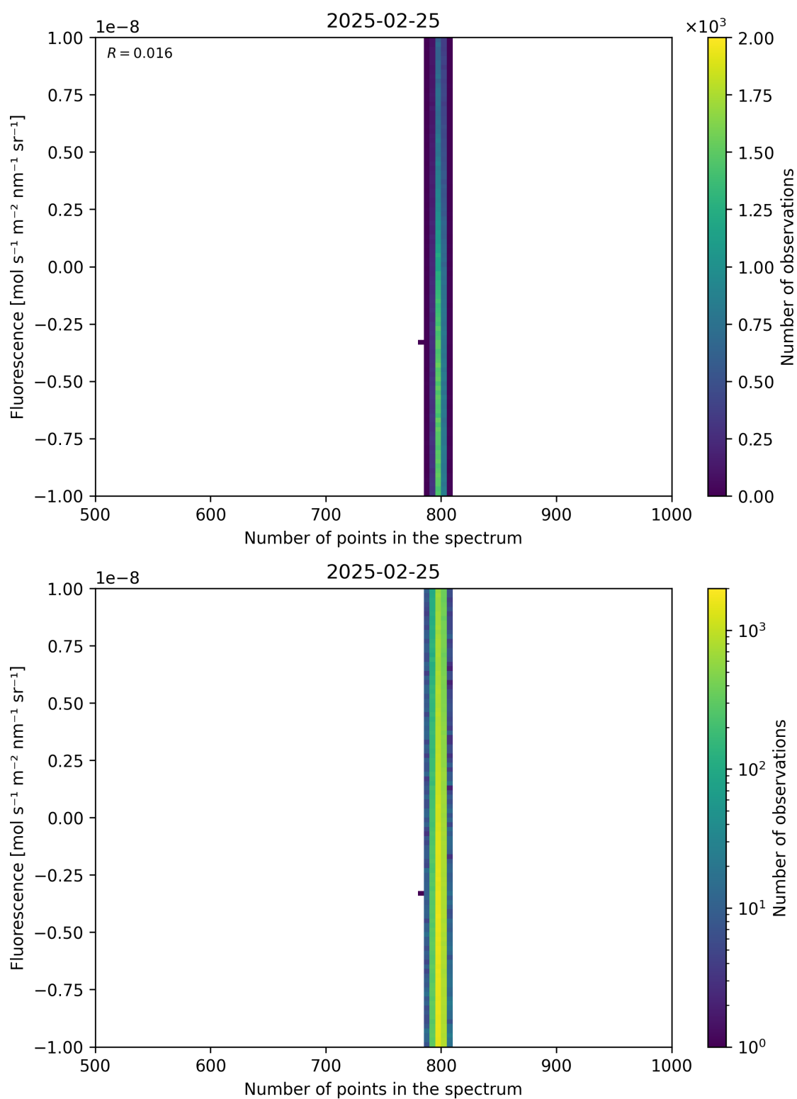
Figure 91: Scatter density plot of “Number of points in the spectrum” against “Fluorescence” for 2025-02-24 to 2025-02-26.
