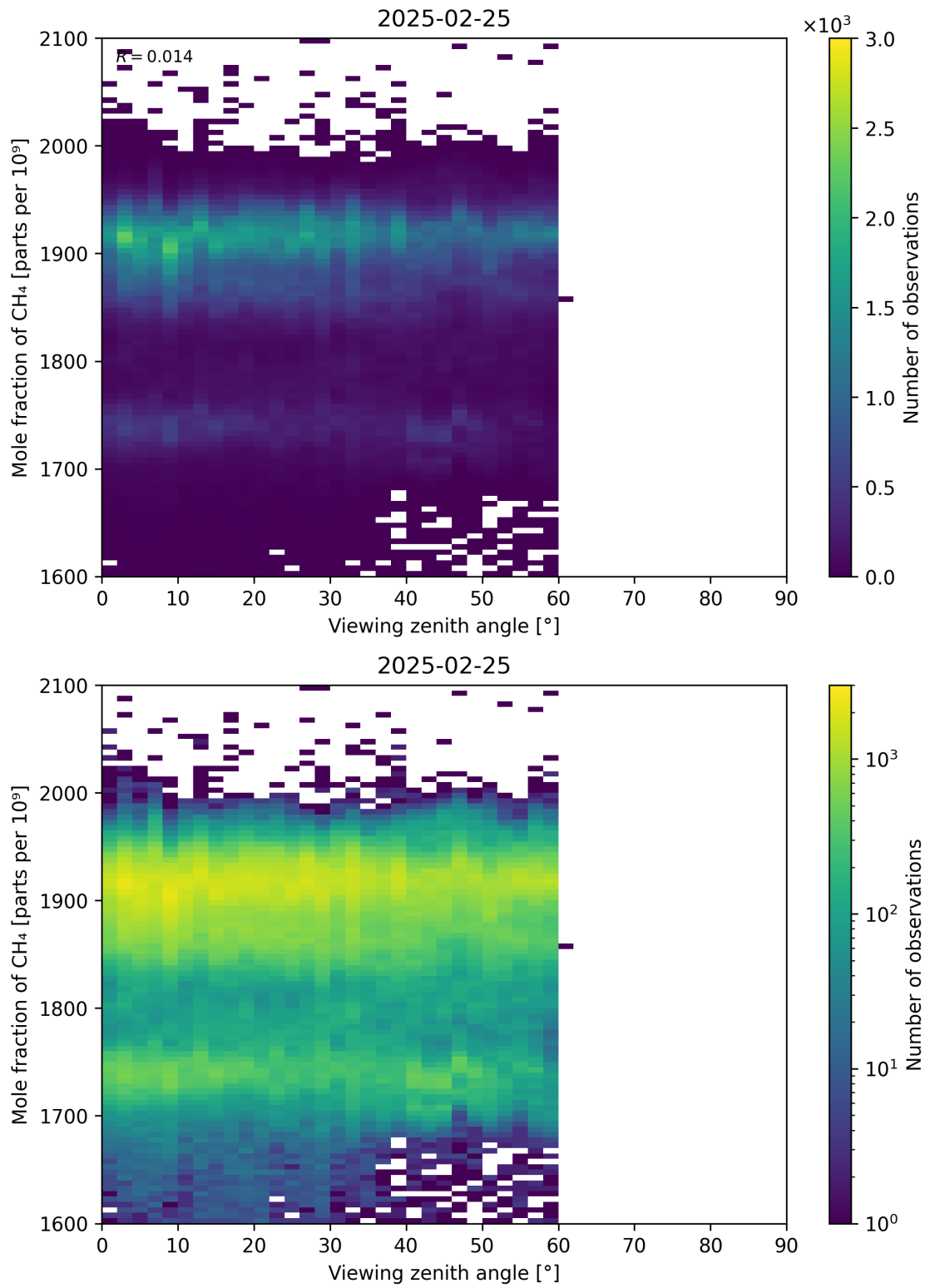
Figure 110: Scatter density plot of “Viewing zenith angle” against “Mole fraction of CH 4 ” for 2025-02-24 to 2025-02-26.
