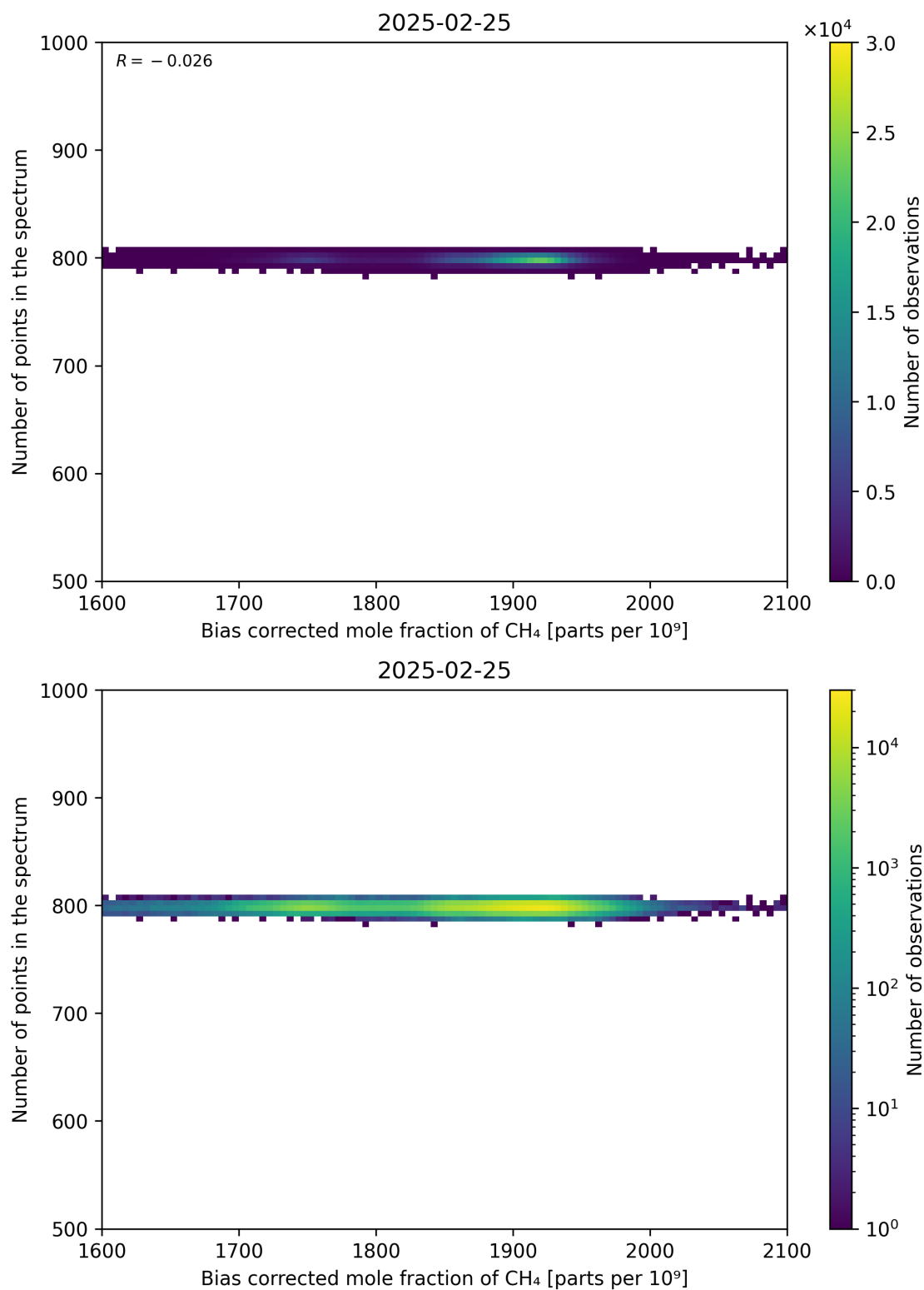
Figure 68: Scatter density plot of “Bias corrected mole fraction of CH 4 ” against “Number of points in the spectrum” for 2025-02-24 to 2025-02-26.
