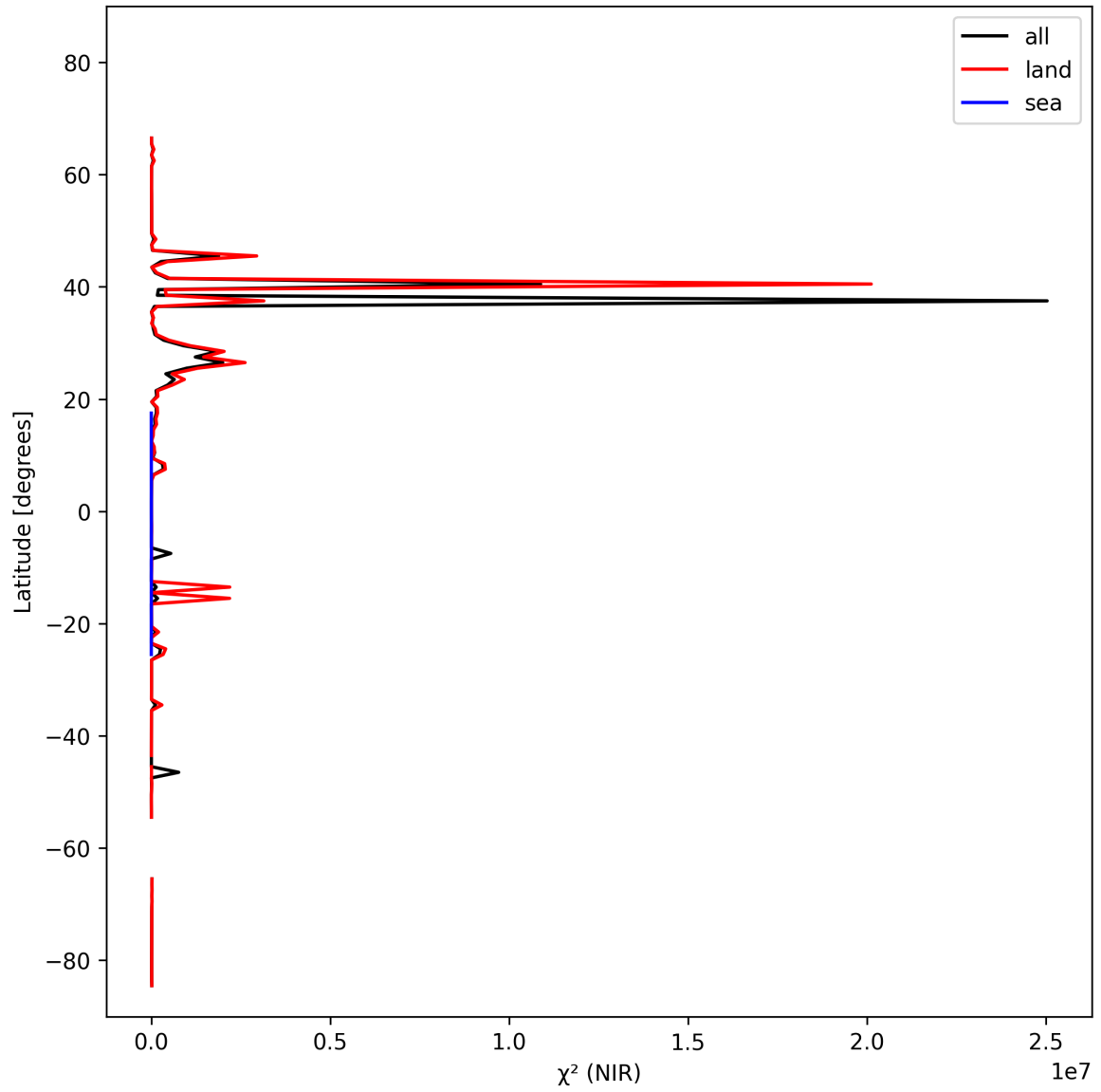
Figure 18: Zonal average of “ \chi^2 (NIR)” for 2025-02-24 to 2025-02-26.
