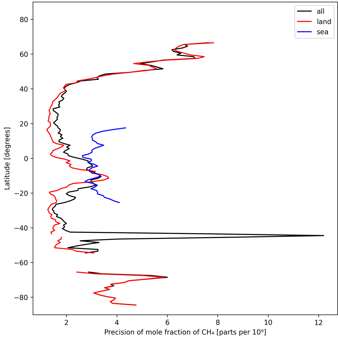
Figure 13: Zonal average of “Precision of mole fraction of CH 4 ” for 2025-02-24 to 2025-02-26.
