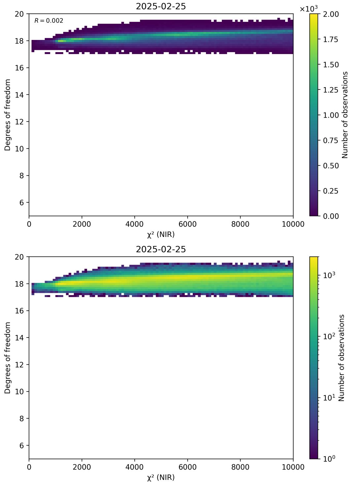
Figure 44: Scatter density plot of “ \chi^2 (NIR)” against “Degrees of freedom” for 2025-02-24 to 2025-02-26.
