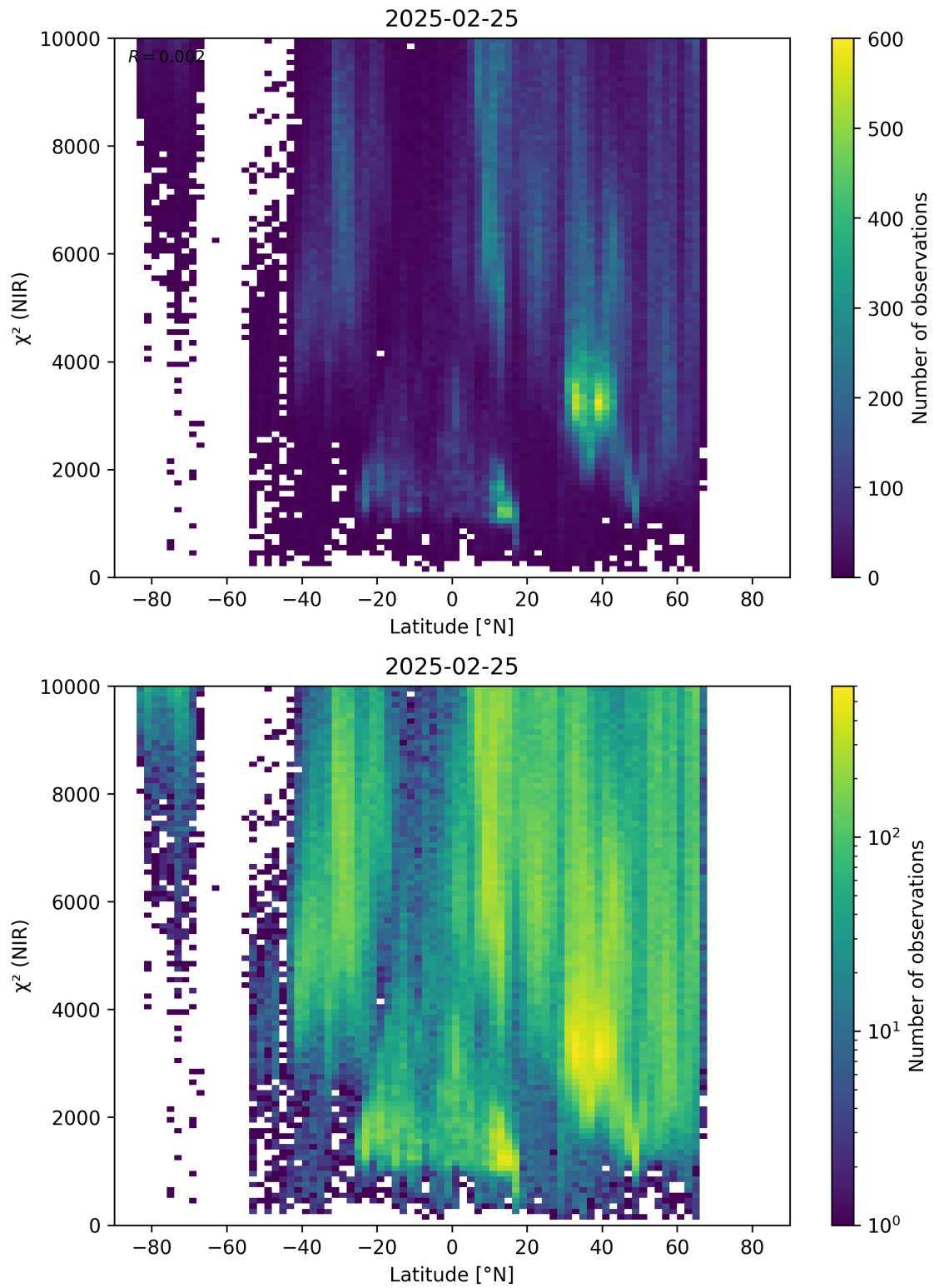
Figure 53: Scatter density plot of “Latitude” against “ \chi^2 (NIR)” for 2025-02-24 to 2025-02-26.
