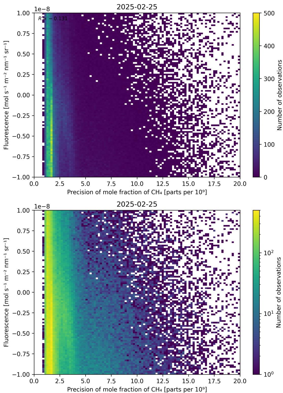
Figure 81: Scatter density plot of “Precision of mole fraction of \text{CH}_4 ” against “Fluorescence” for 2025-02-24 to 2025-02-26.
