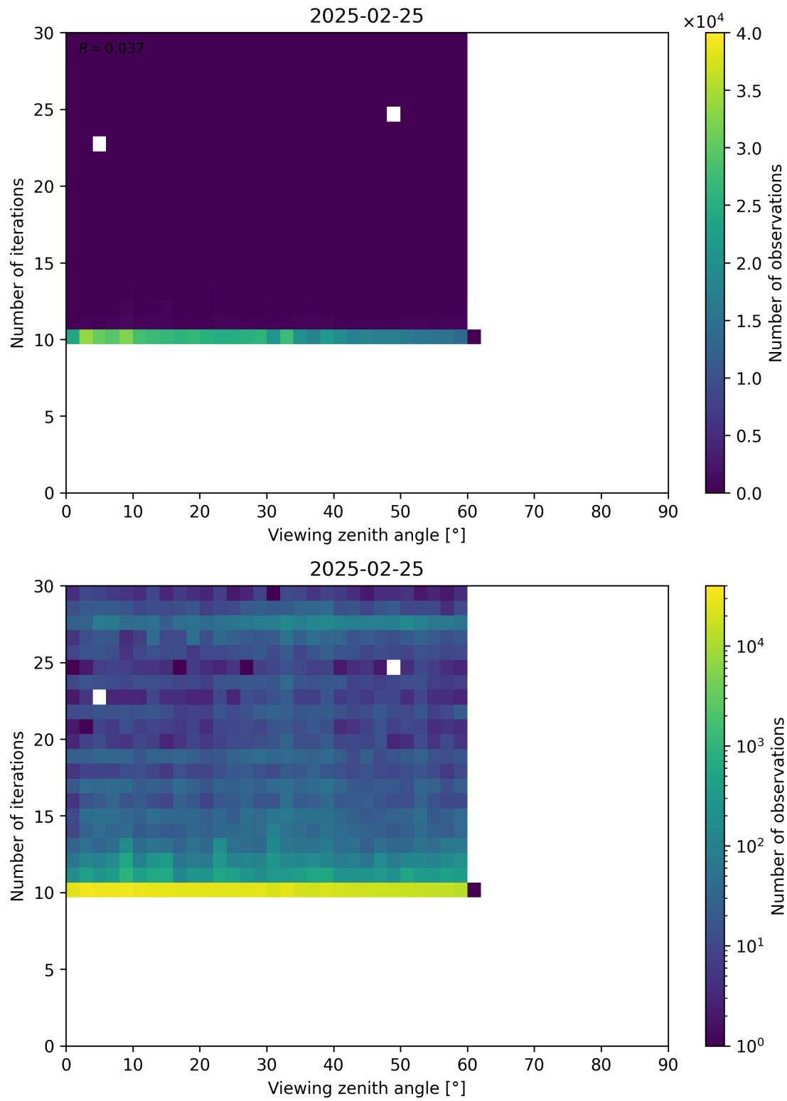
Figure 113: Scatter density plot of “Viewing zenith angle” against “Number of iterations” for 2025-02-24 to 2025-02-26.
