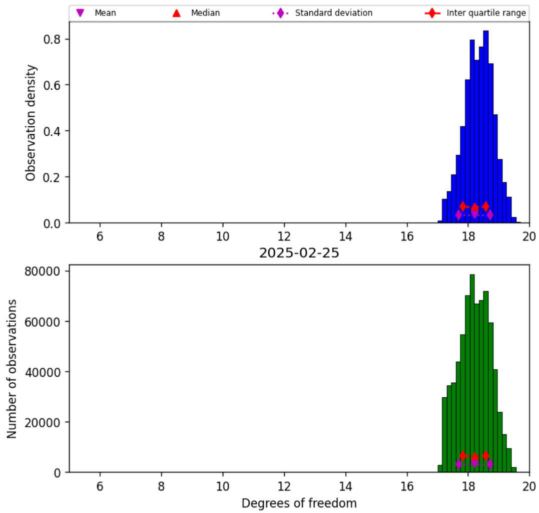
Figure 30: Histogram of “Degrees of freedom” for 2025-02-24 to 2025-02-26
