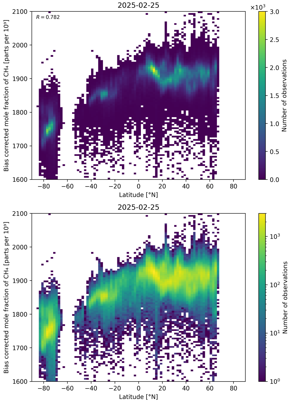
Figure 58: Scatter density plot of “Latitude” against “Bias corrected mole fraction of \text{CH}_4 ” for 2025-02-24 to 2025-02-26.
