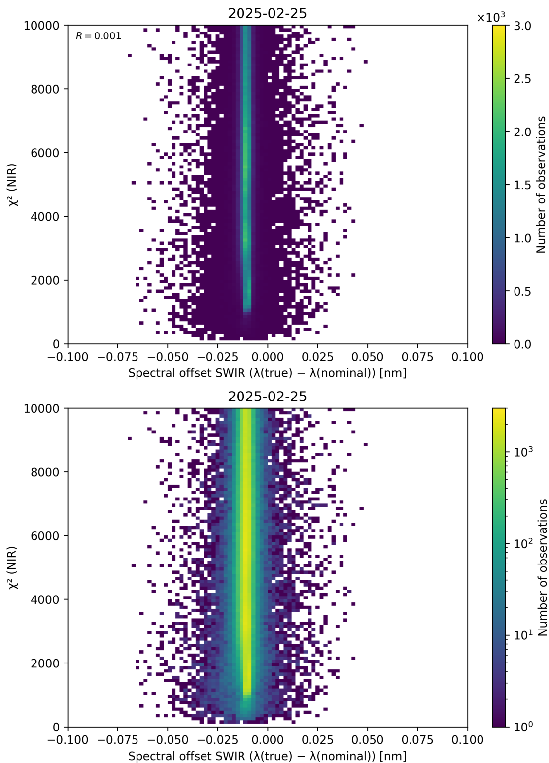
Figure 117: Scatter density plot of “Spectral offset SWIR ( \lambda_{\text{true}} - \lambda_{\text{nominal}} )” against “ \chi^2 (NIR)” for 2025-02-24 to 2025-02-26.
