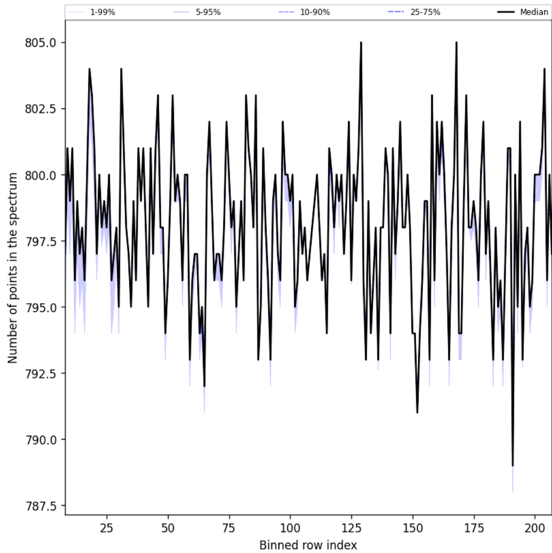
Figure 37: Along track statistics of “Number of points in the spectrum” for 2025-02-24 to 2025-02-26
