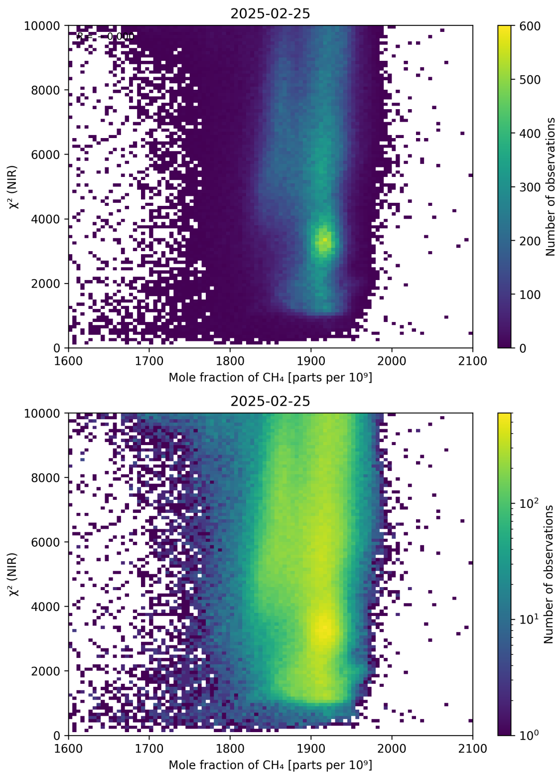
Figure 70: Scatter density plot of “Mole fraction of \text{CH}_4 ” against “ \chi^2 (NIR)” for 2025-02-24 to 2025-02-26.
