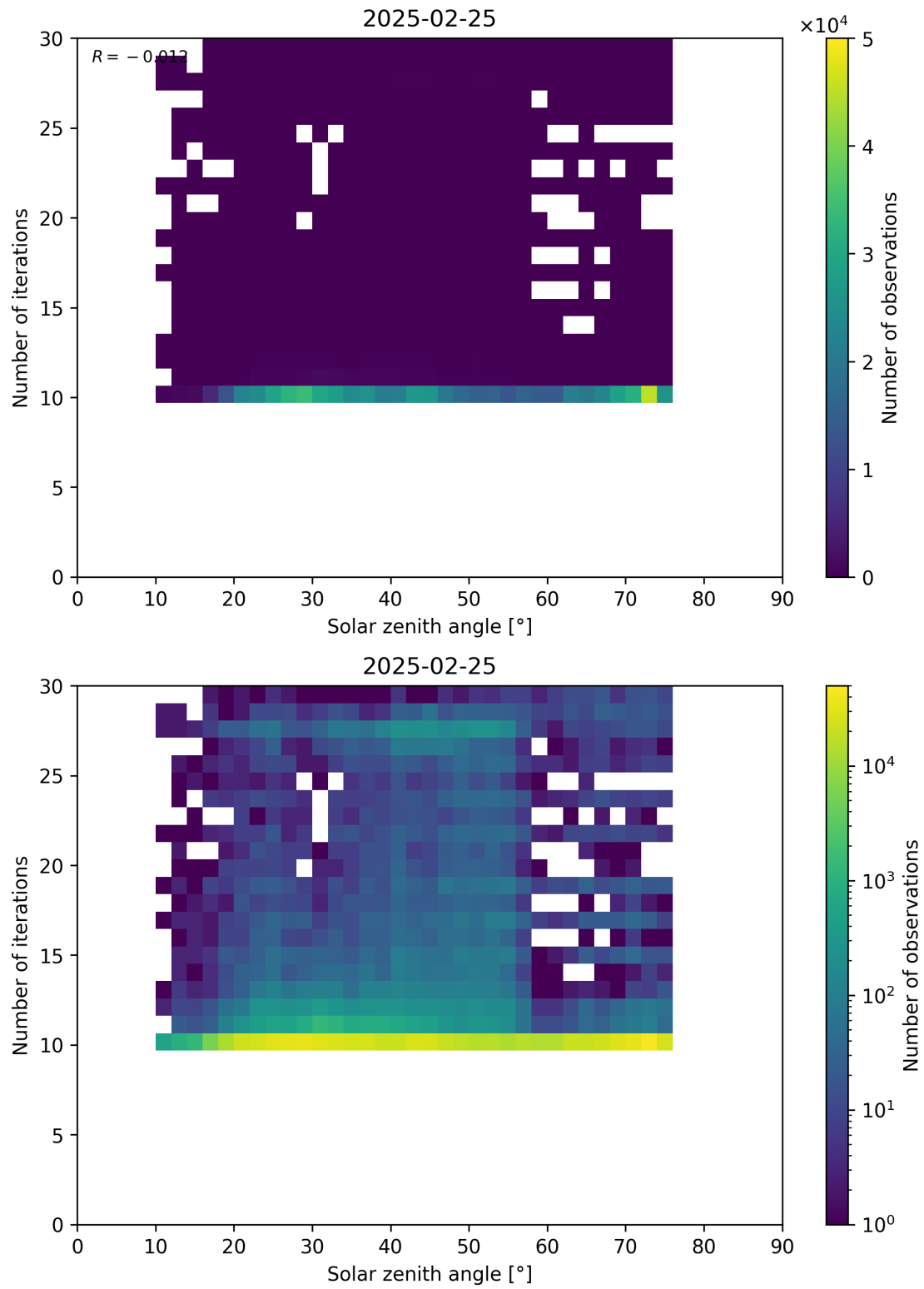
Figure 102: Scatter density plot of “Solar zenith angle” against “Number of iterations” for 2025-02-24 to 2025-02-26.
