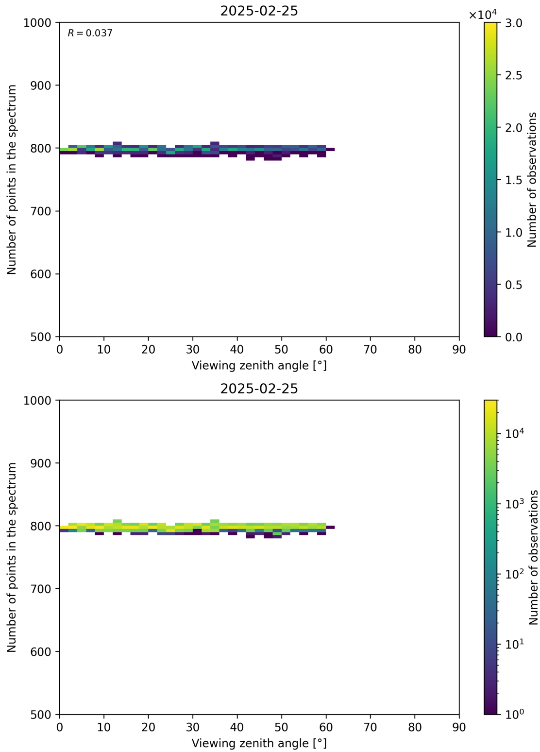
Figure 114: Scatter density plot of “Viewing zenith angle” against “Number of points in the spectrum” for 2025-02-24 to 2025-02-26.
