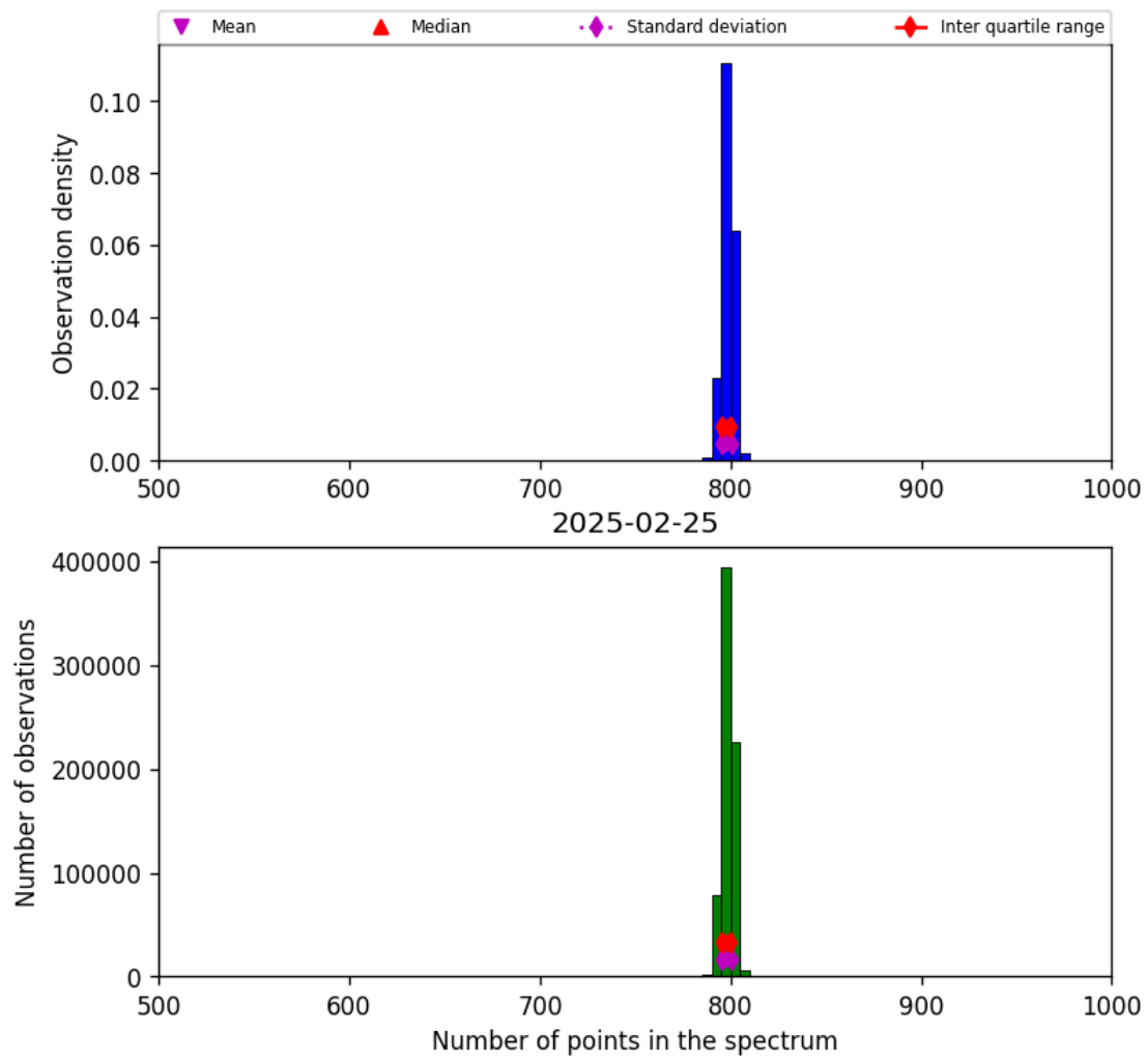
Figure 26: Histogram of “Number of points in the spectrum” for 2025-02-24 to 2025-02-26
