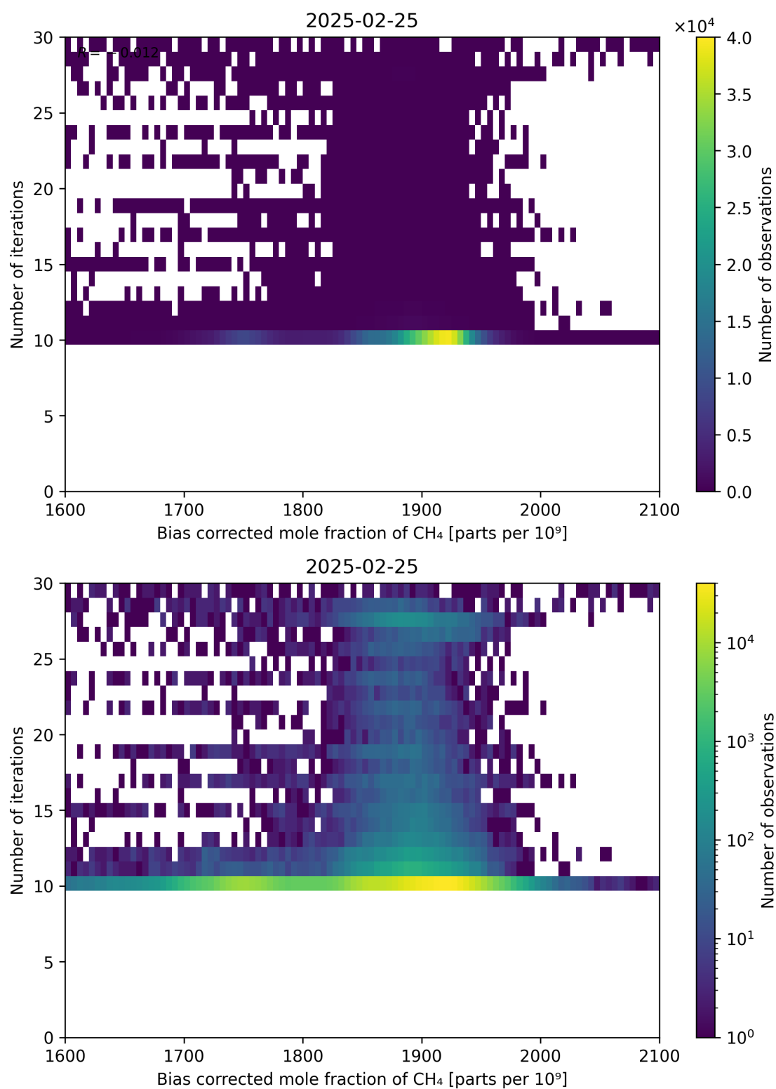
Figure 67: Scatter density plot of “Bias corrected mole fraction of \text{CH}_4 ” against “Number of iterations” for 2025-02-24 to 2025-02-26.
