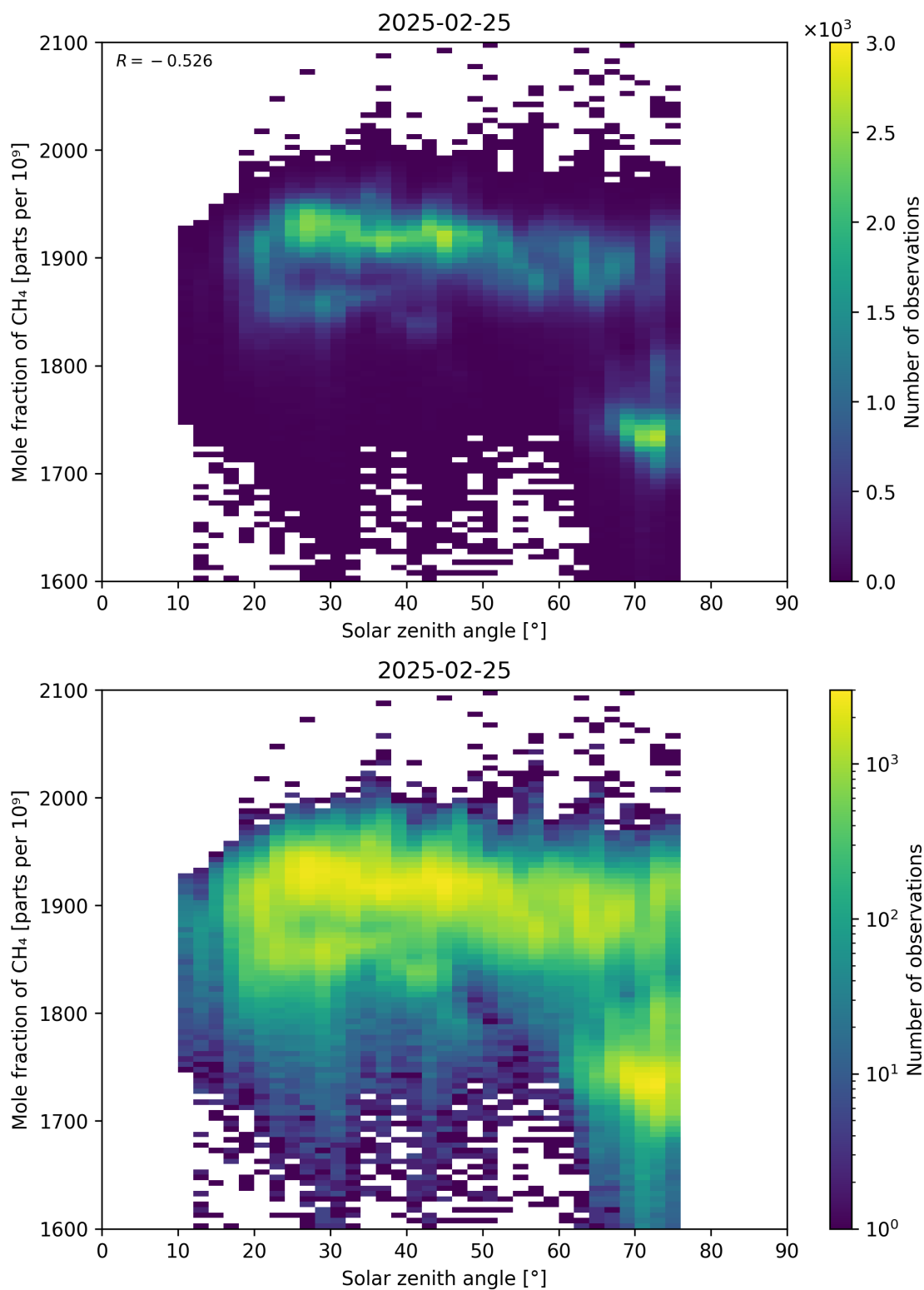
Figure 99: Scatter density plot of “Solar zenith angle” against “Mole fraction of CH 4 ” for 2025-02-24 to 2025-02-26.
