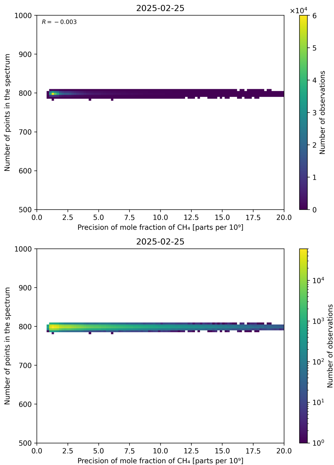
Figure 84: Scatter density plot of “Precision of mole fraction of CH 4 ” against “Number of points in the spectrum” for 2025-02-24 to 2025-02-26.
