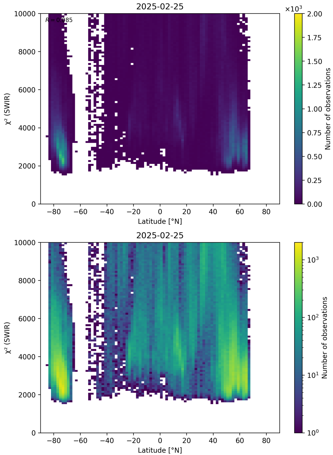
Figure 54: Scatter density plot of “Latitude” against “ \chi^2 (SWIR)” for 2025-02-24 to 2025-02-26.
