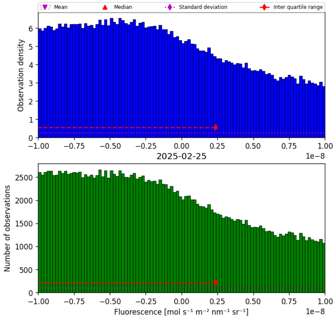
Figure 32: Histogram of “Fluorescence” for 2025-02-24 to 2025-02-26
