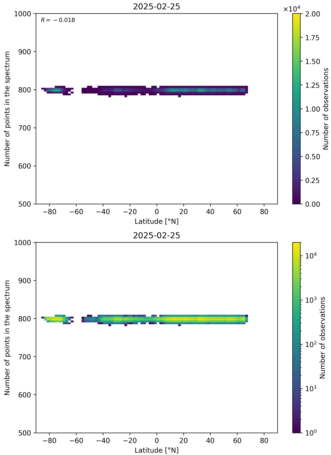
Figure 61: Scatter density plot of “Latitude” against “Number of points in the spectrum” for 2025-02-24 to 2025-02-26.
