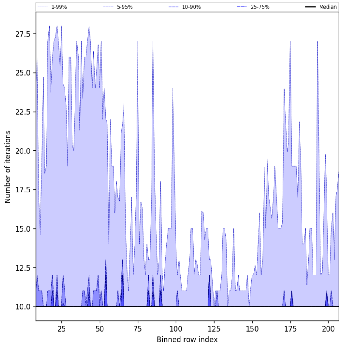
Figure 42: Along track statistics of “Number of iterations” for 2025-02-24 to 2025-02-26
