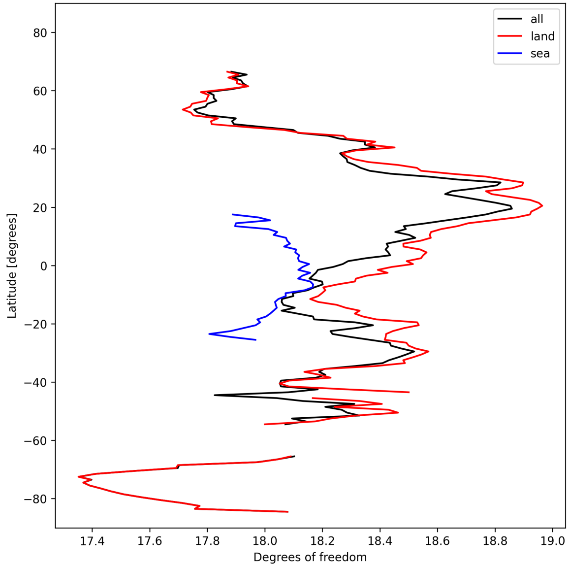
Figure 19: Zonal average of “Degrees of freedom” for 2025-02-24 to 2025-02-26.
