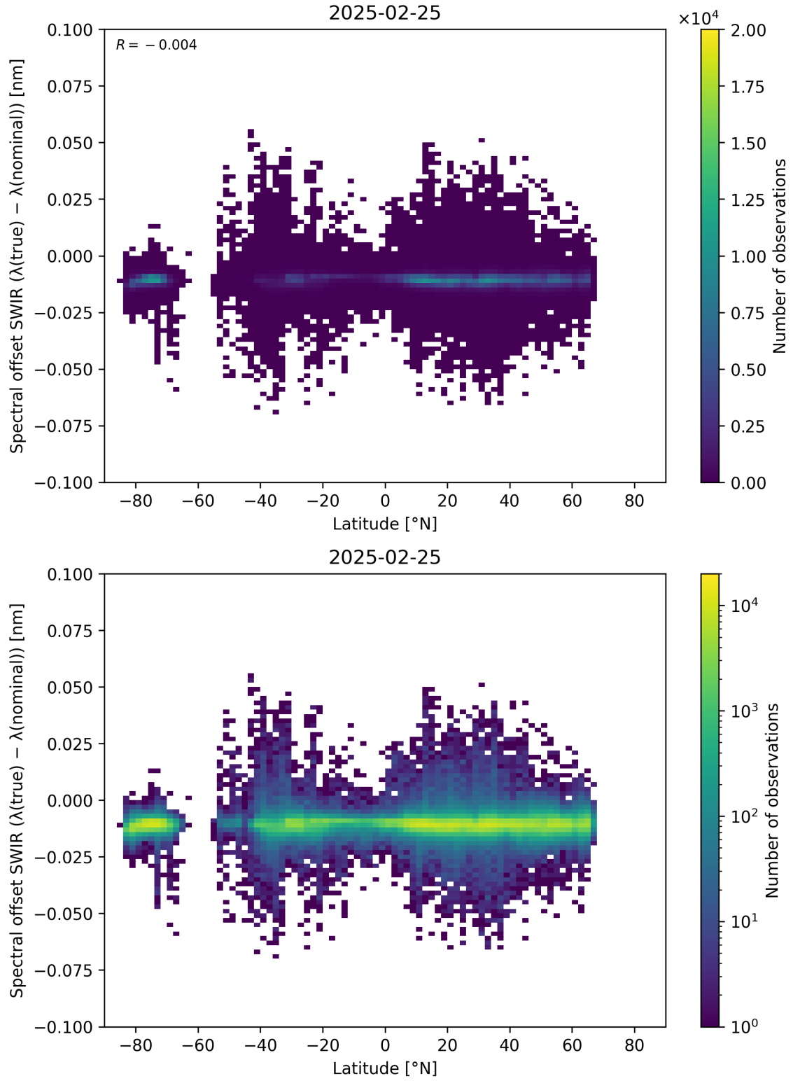
Figure 62: Scatter density plot of “Latitude” against “Spectral offset SWIR ( \lambda_{\text{true}} - \lambda_{\text{nominal}} )” for 2025-02-24 to 2025-02-26.
