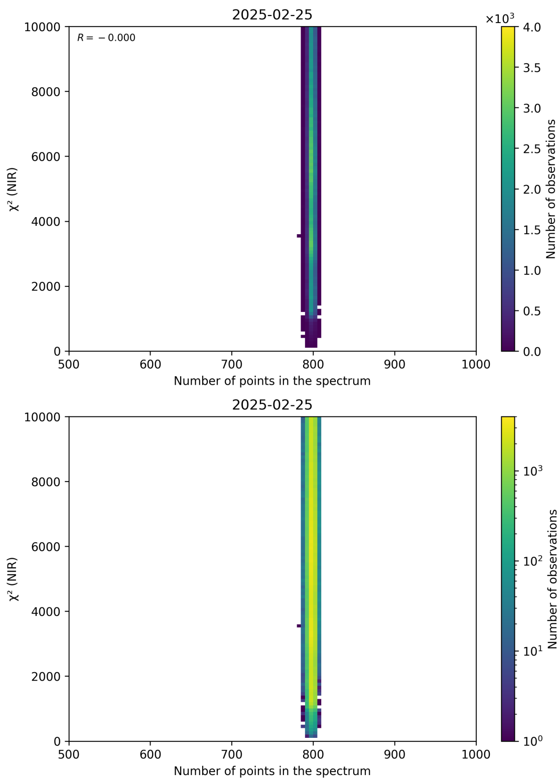
Figure 88: Scatter density plot of “Number of points in the spectrum” against “ \chi^2 (NIR)” for 2025-02-24 to 2025-02-26.
