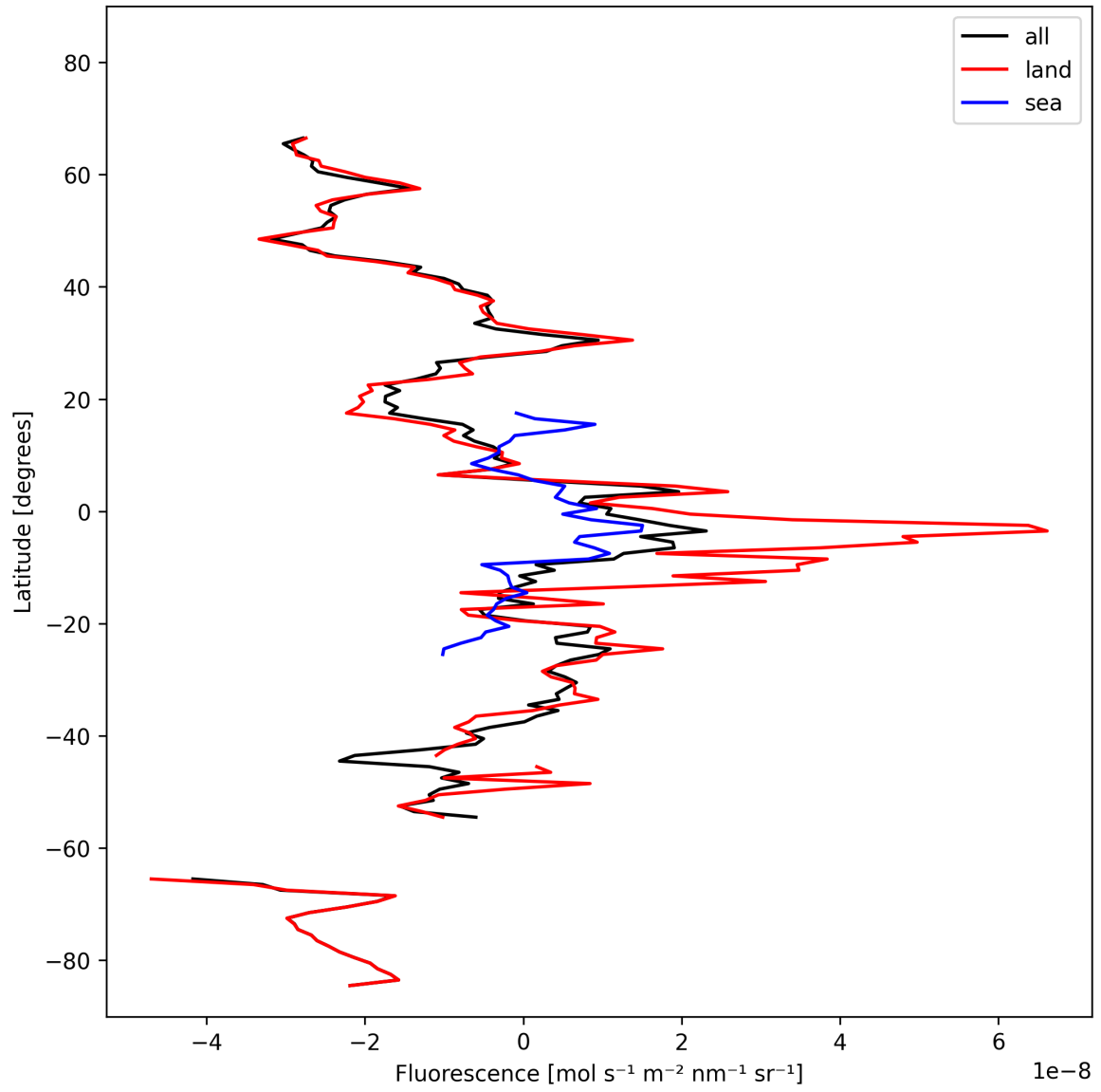
Figure 21: Zonal average of “Fluorescence” for 2025-02-24 to 2025-02-26.
