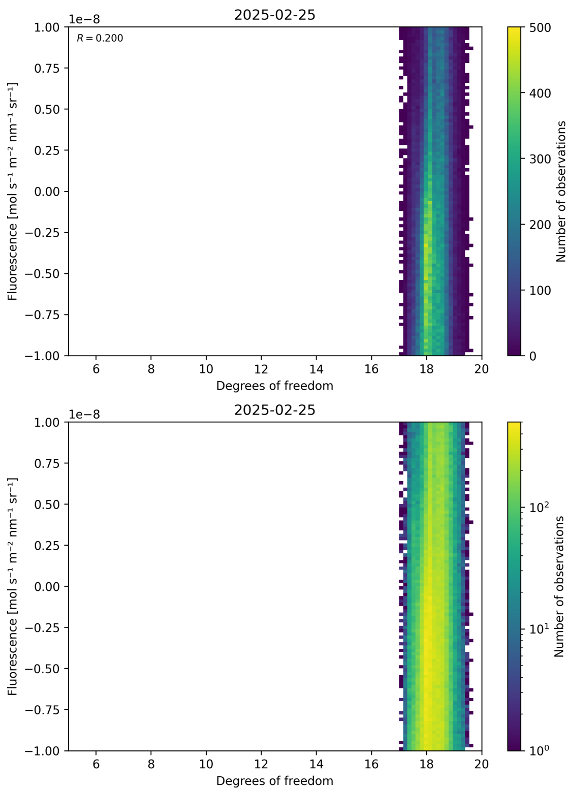
Figure 51: Scatter density plot of “Degrees of freedom” against “Fluorescence” for 2025-02-24 to 2025-02-26.
