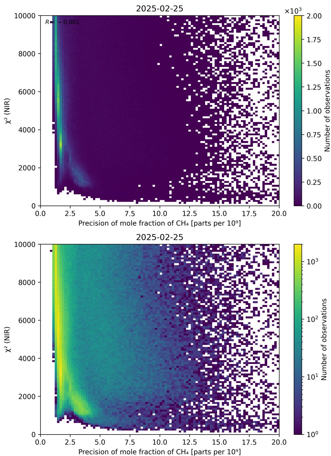
Figure 78: Scatter density plot of “Precision of mole fraction of CH 4 ” against “ \chi^2 (NIR)” for 2025-02-24 to 2025-02-26.
