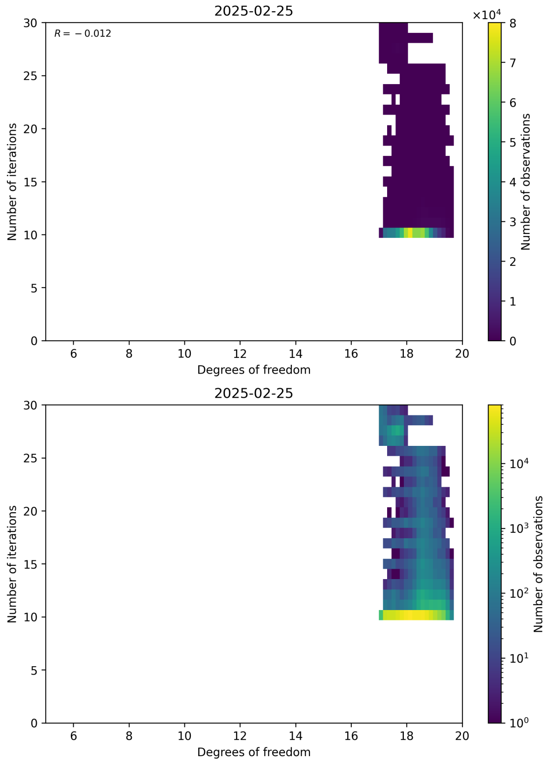
Figure 52: Scatter density plot of “Degrees of freedom” against “Number of iterations” for 2025-02-24 to 2025-02-26.
