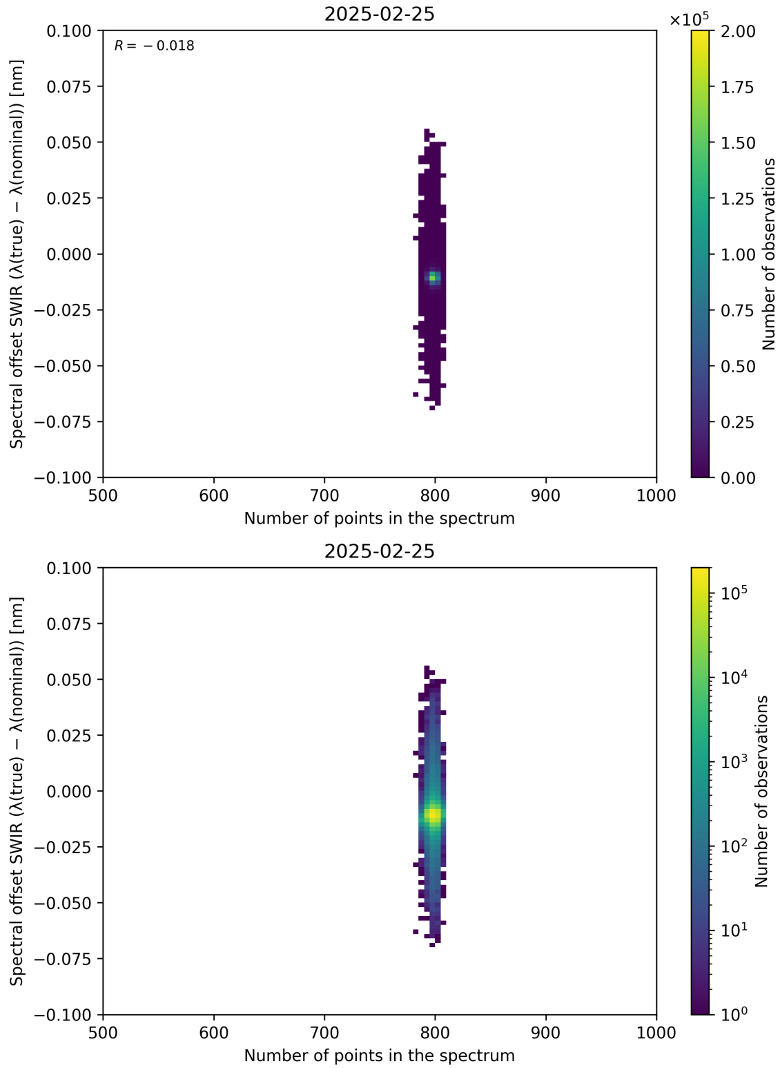
Figure 93: Scatter density plot of “Number of points in the spectrum” against “Spectral offset SWIR ( \lambda_{\text{true}} - \lambda_{\text{nominal}} )” for 2025-02-24 to 2025-02-26.
