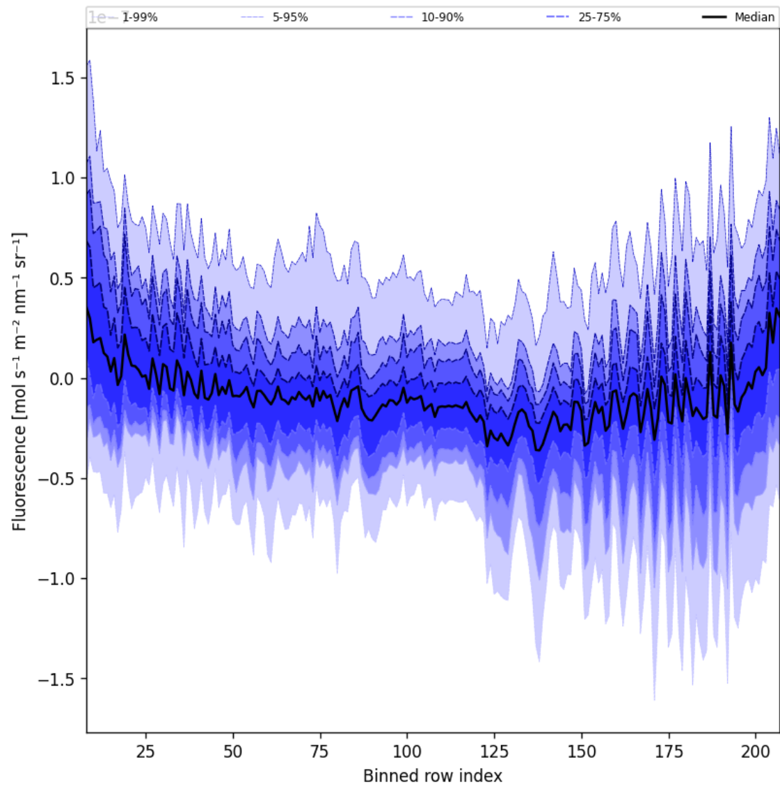
Figure 43: Along track statistics of “Fluorescence” for 2025-02-24 to 2025-02-26
