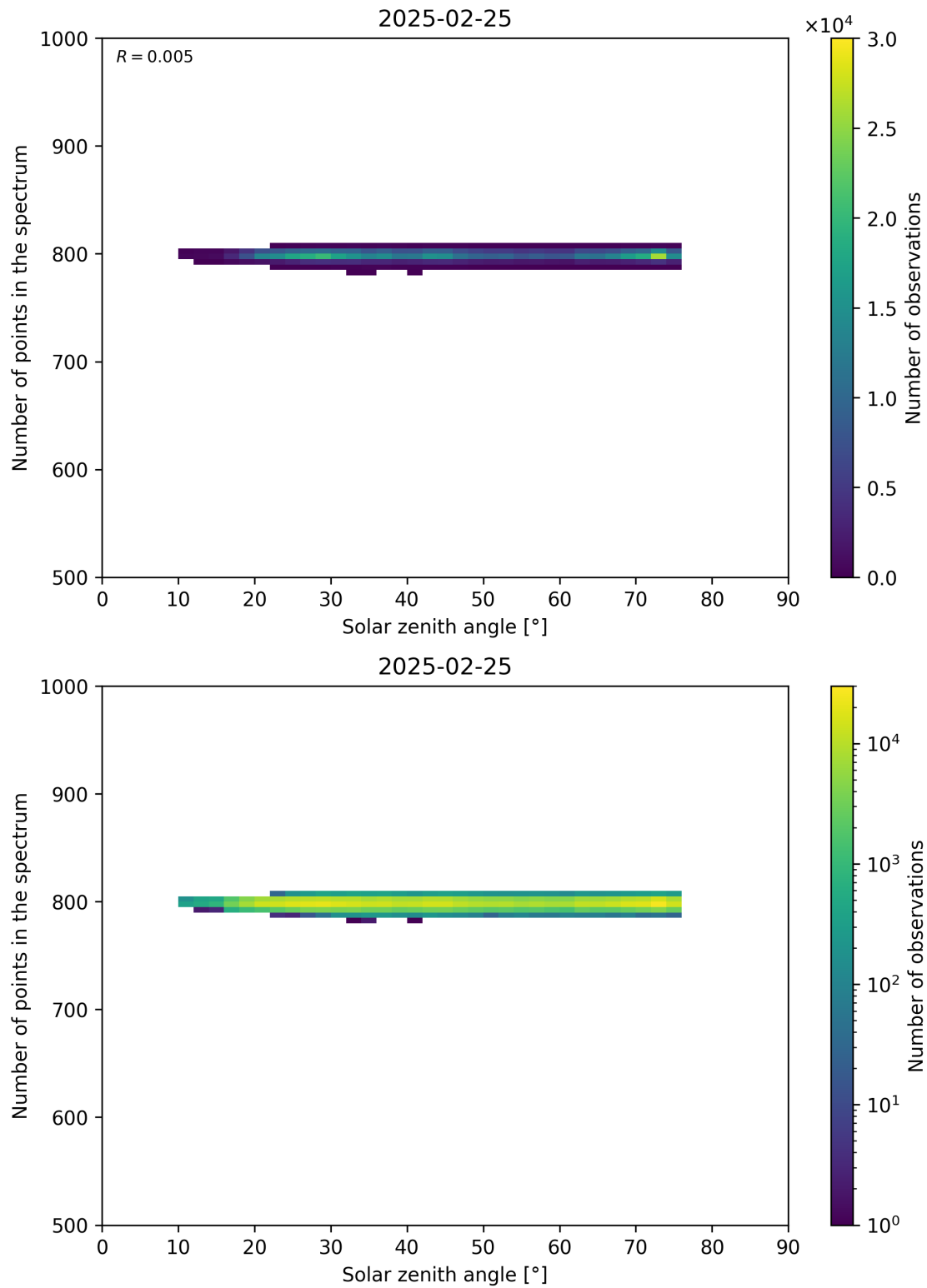
Figure 103: Scatter density plot of “Solar zenith angle” against “Number of points in the spectrum” for 2025-02-24 to 2025-02-26.
