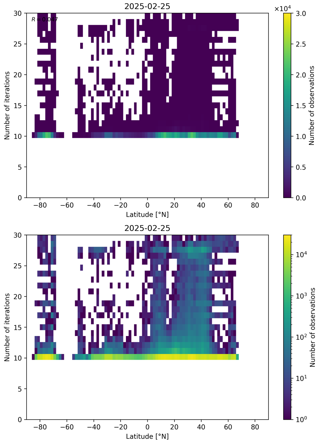
Figure 60: Scatter density plot of “Latitude” against “Number of iterations” for 2025-02-24 to 2025-02-26.
