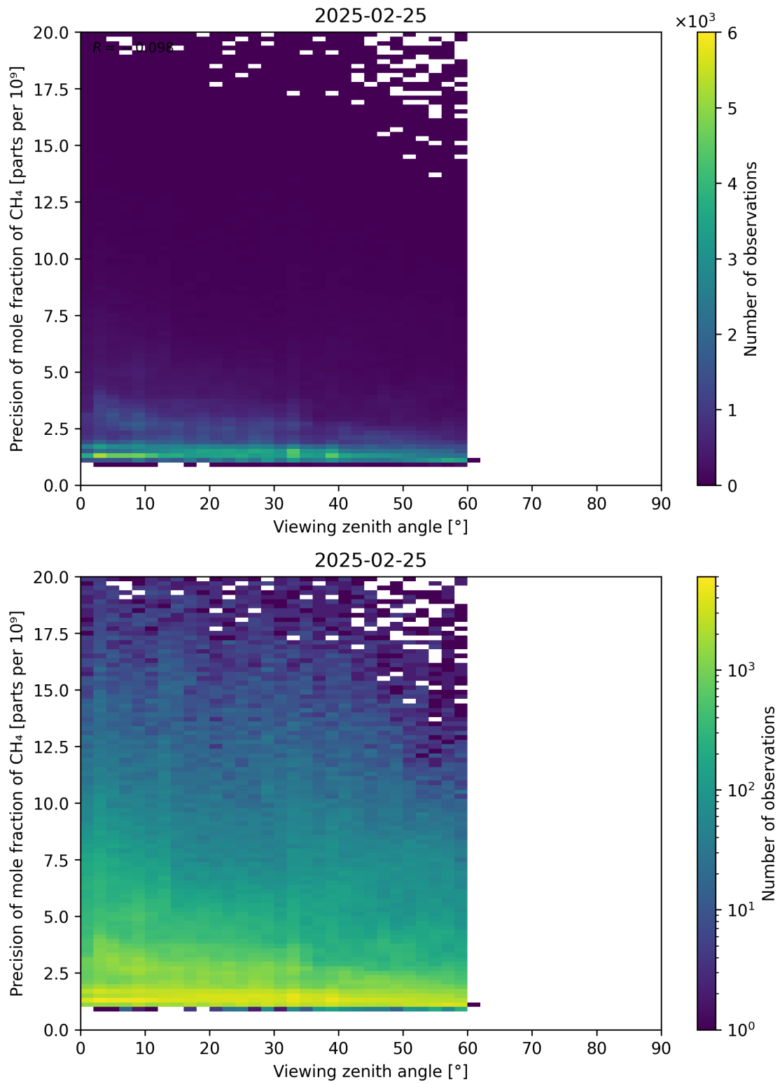
Figure 112: Scatter density plot of “Viewing zenith angle” against “Precision of mole fraction of CH 4 ” for 2025-02-24 to 2025-02-26.
