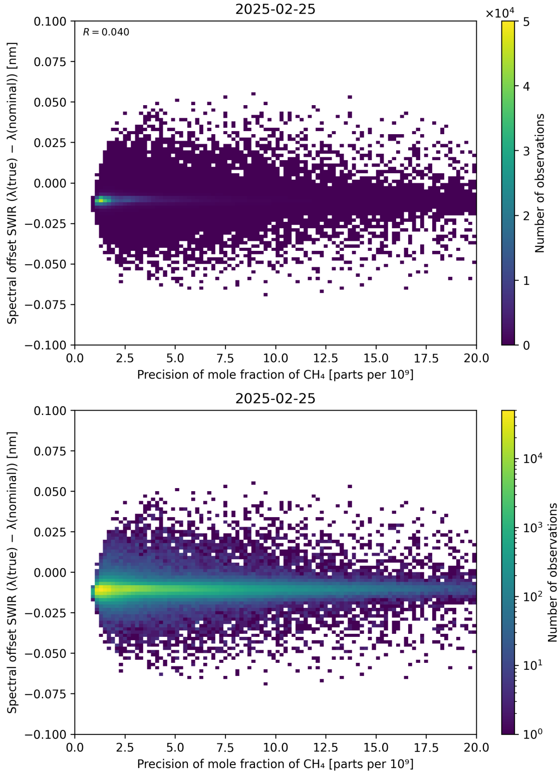
Figure 85: Scatter density plot of “Precision of mole fraction of CH 4 ” against “Spectral offset SWIR ( \lambda_{\text{true}} - \lambda_{\text{nominal}} )” for 2025-02-24 to 2025-02-26.
