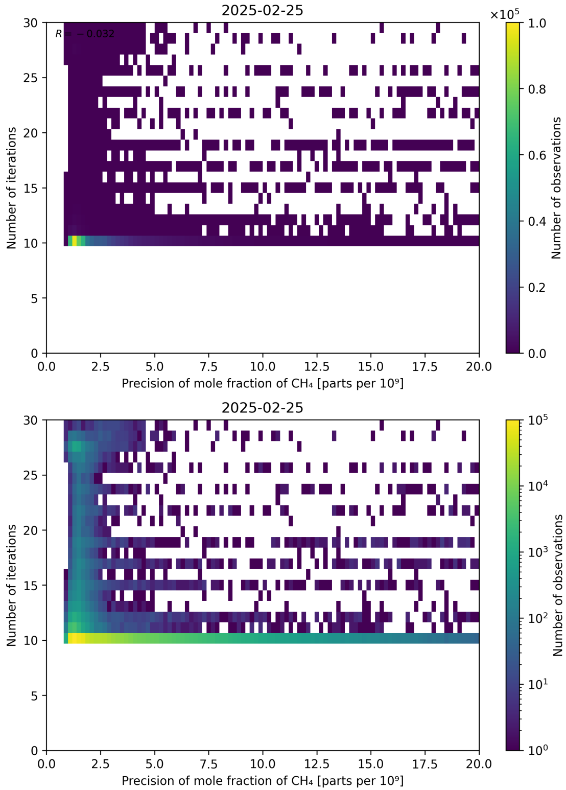
Figure 83: Scatter density plot of “Precision of mole fraction of CH 4 ” against “Number of iterations” for 2025-02-24 to 2025-02-26.
