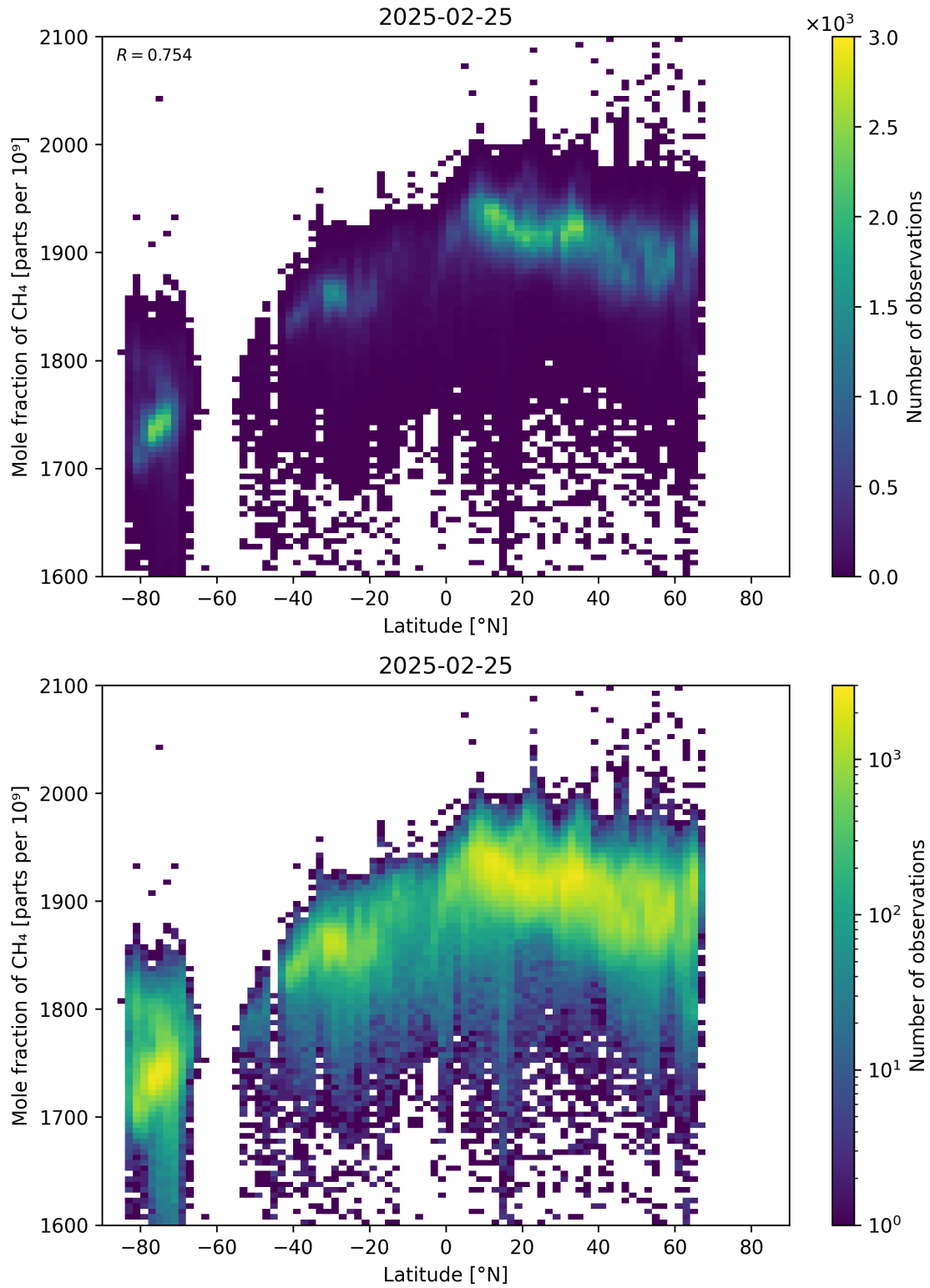
Figure 57: Scatter density plot of “Latitude” against “Mole fraction of CH 4 ” for 2025-02-24 to 2025-02-26.
