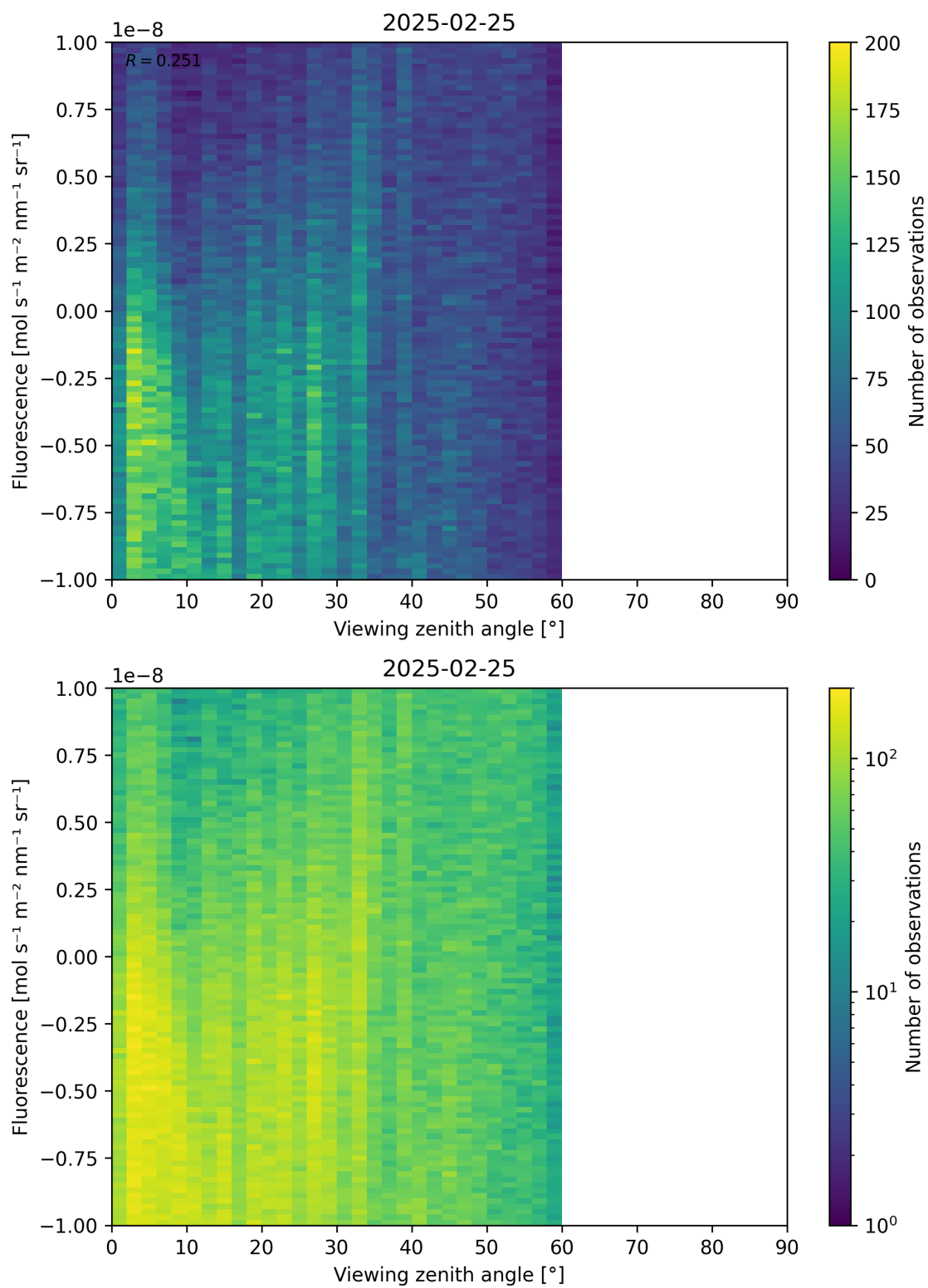
Figure 108: Scatter density plot of “Viewing zenith angle” against “Fluorescence” for 2025-02-24 to 2025-02-26.
