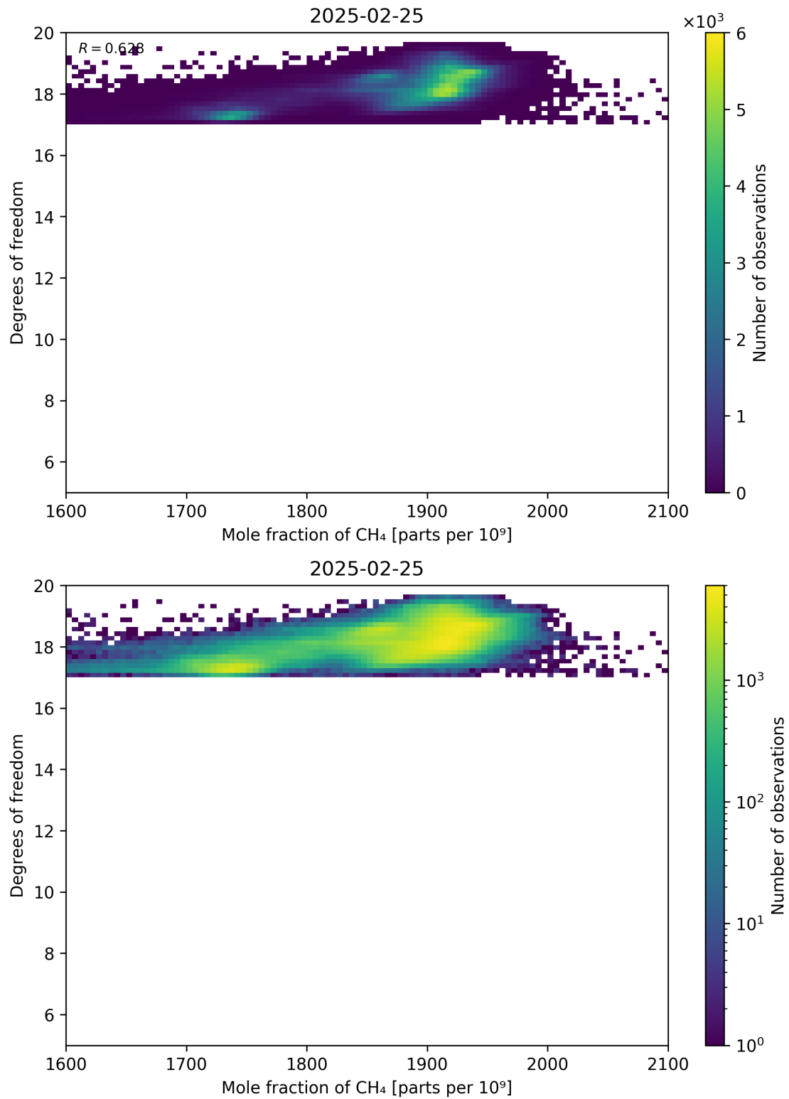
Figure 72: Scatter density plot of “Mole fraction of CH 4 ” against “Degrees of freedom” for 2025-02-24 to 2025-02-26.
