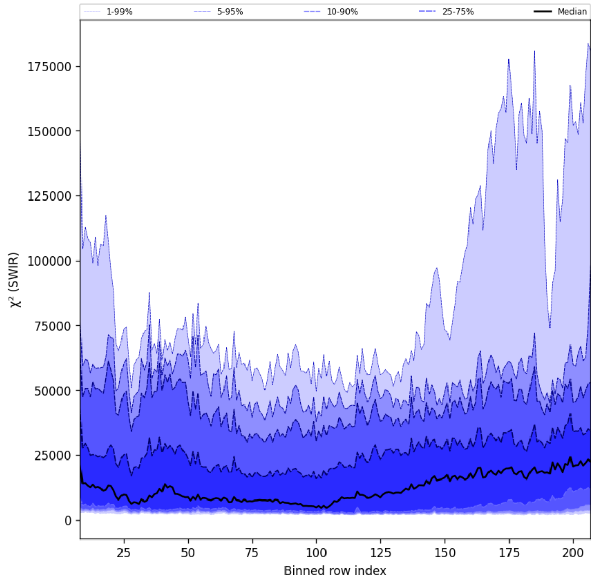
Figure 39: Along track statistics of " \chi^2 (SWIR)" for 2025-02-24 to 2025-02-26
