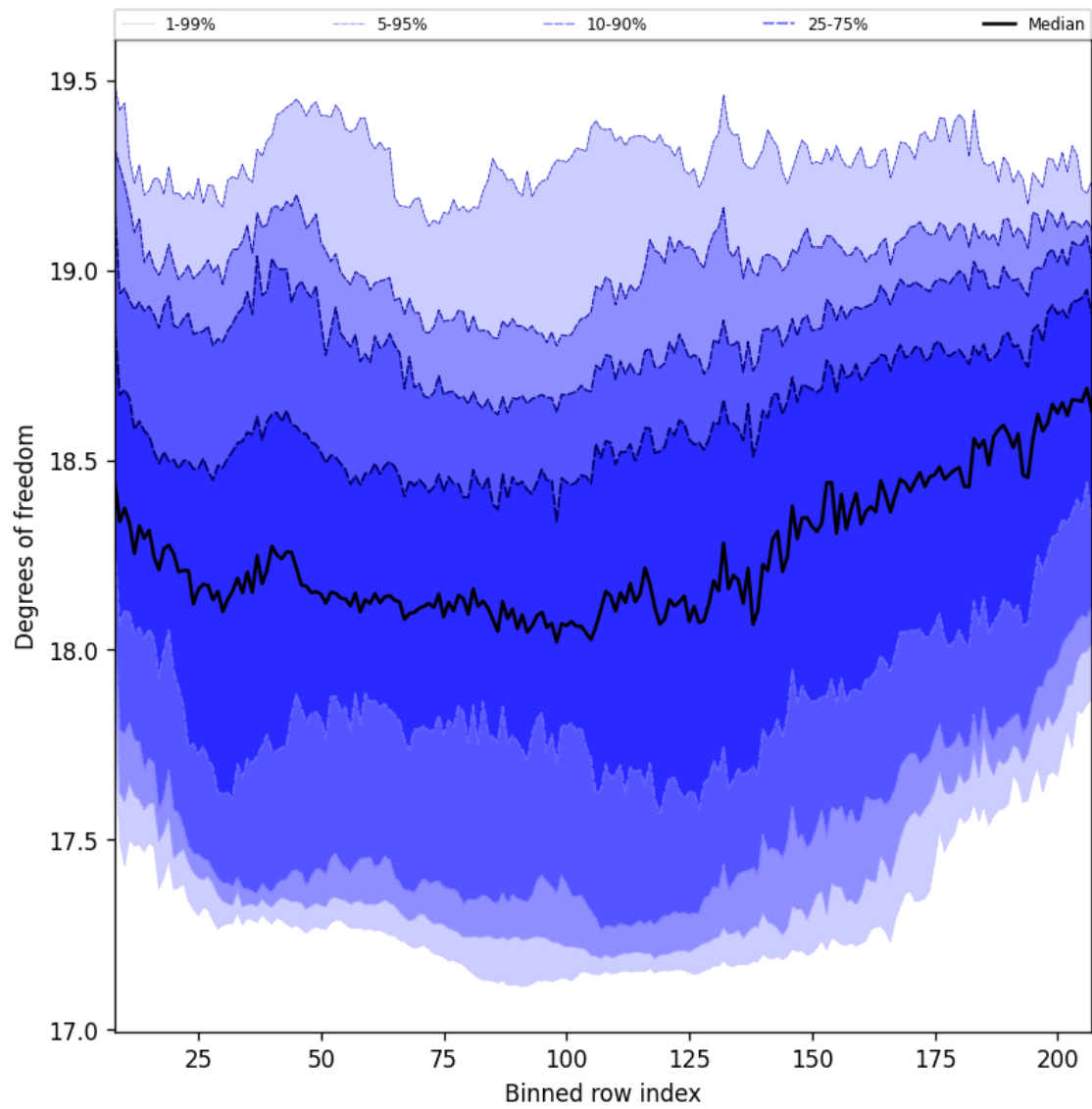
Figure 41: Along track statistics of “Degrees of freedom” for 2025-02-24 to 2025-02-26
