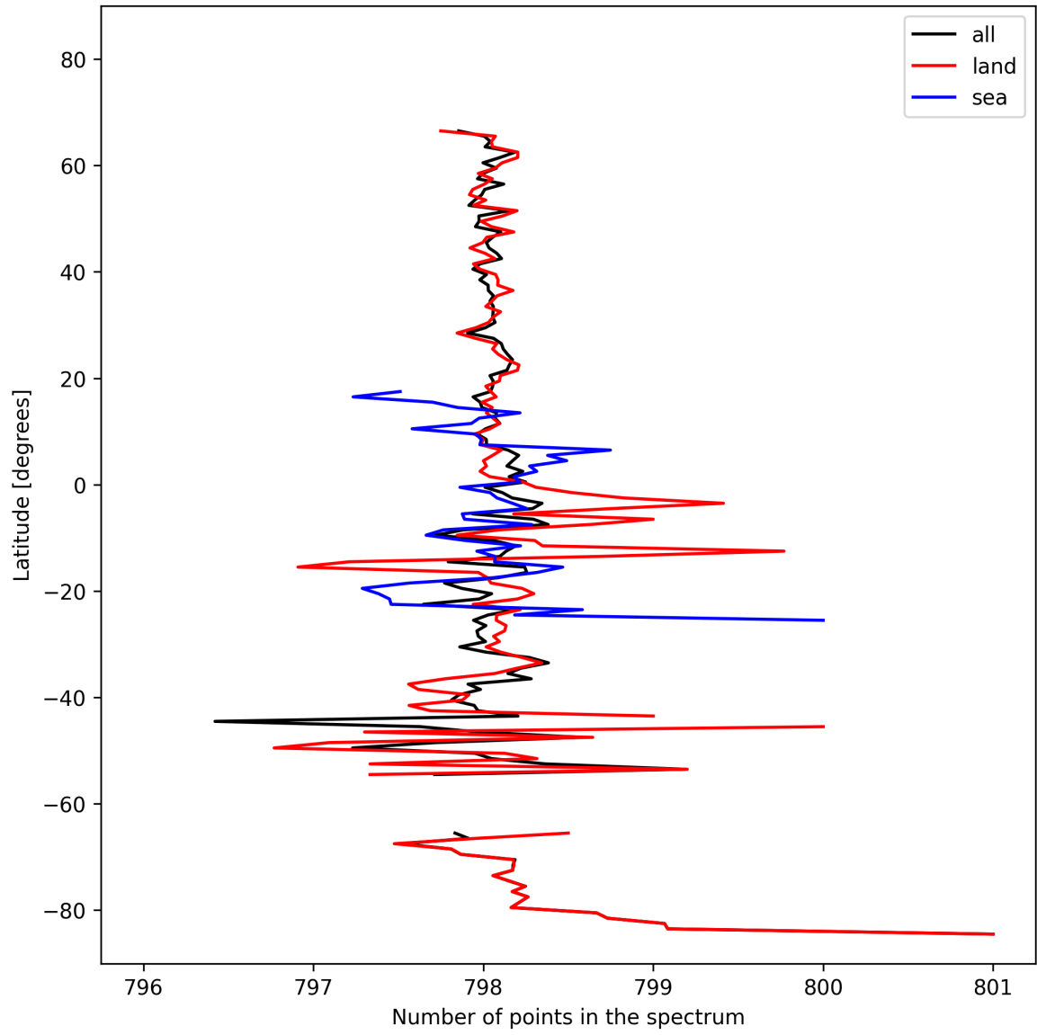
Figure 15: Zonal average of “Number of points in the spectrum” for 2025-02-24 to 2025-02-26.
