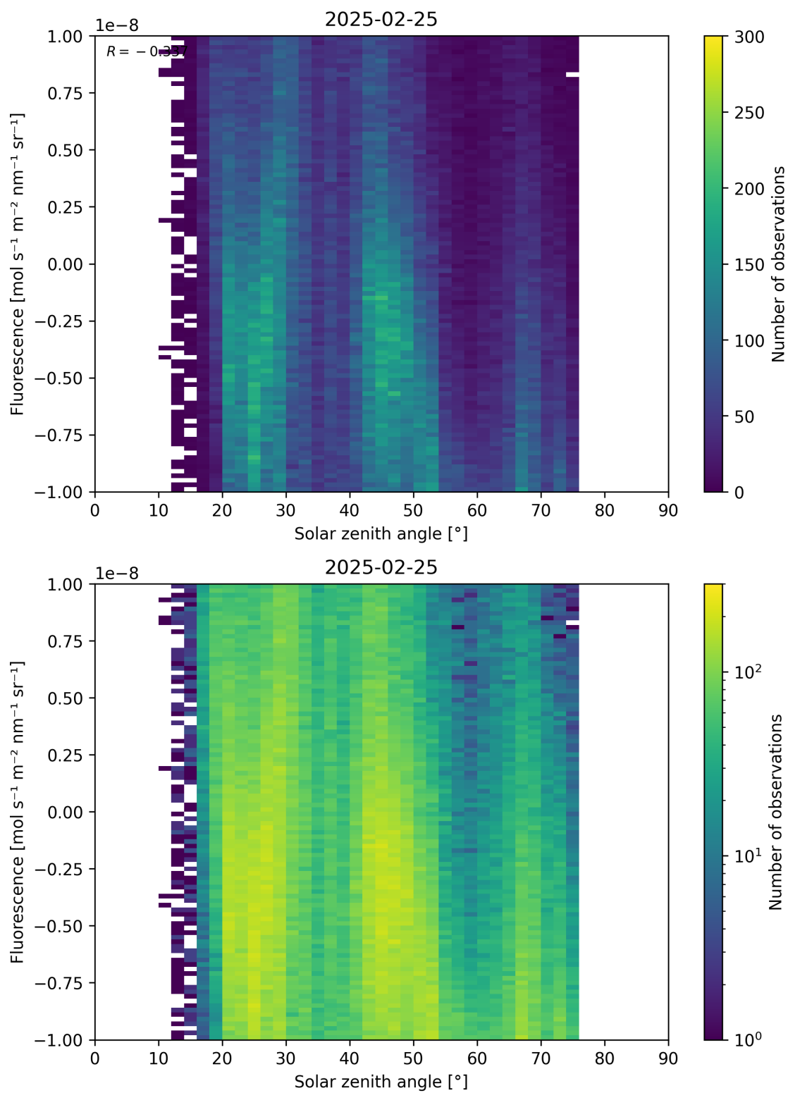
Figure 97: Scatter density plot of “Solar zenith angle” against “Fluorescence” for 2025-02-24 to 2025-02-26.
