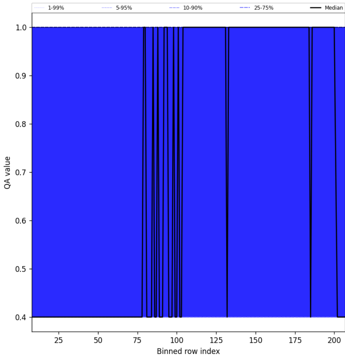
Figure 33: Along track statistics of “QA value” for 2025-02-24 to 2025-02-26
