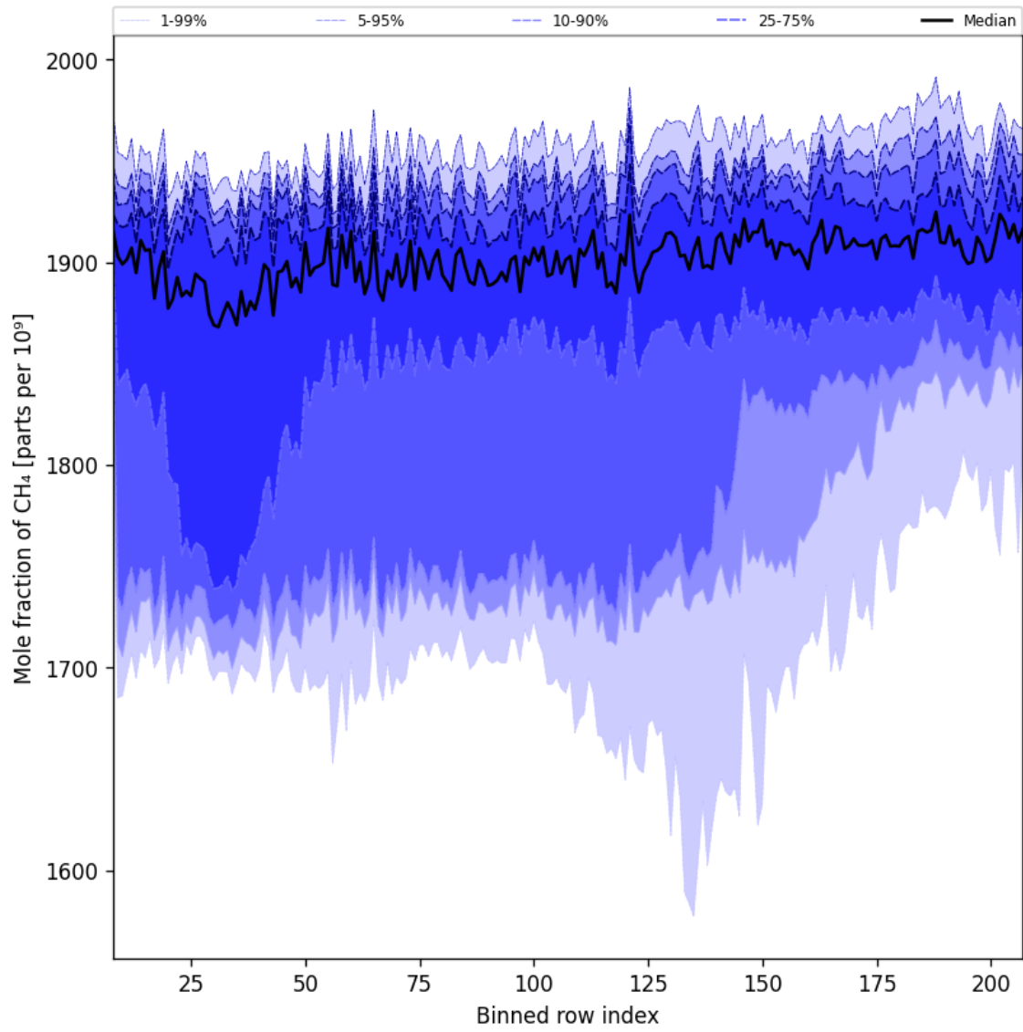
Figure 34: Along track statistics of “Mole fraction of CH 4 ” for 2025-02-24 to 2025-02-26
