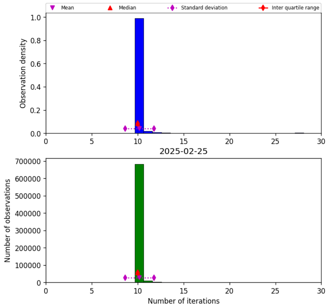
Figure 31: Histogram of “Number of iterations” for 2025-02-24 to 2025-02-26
