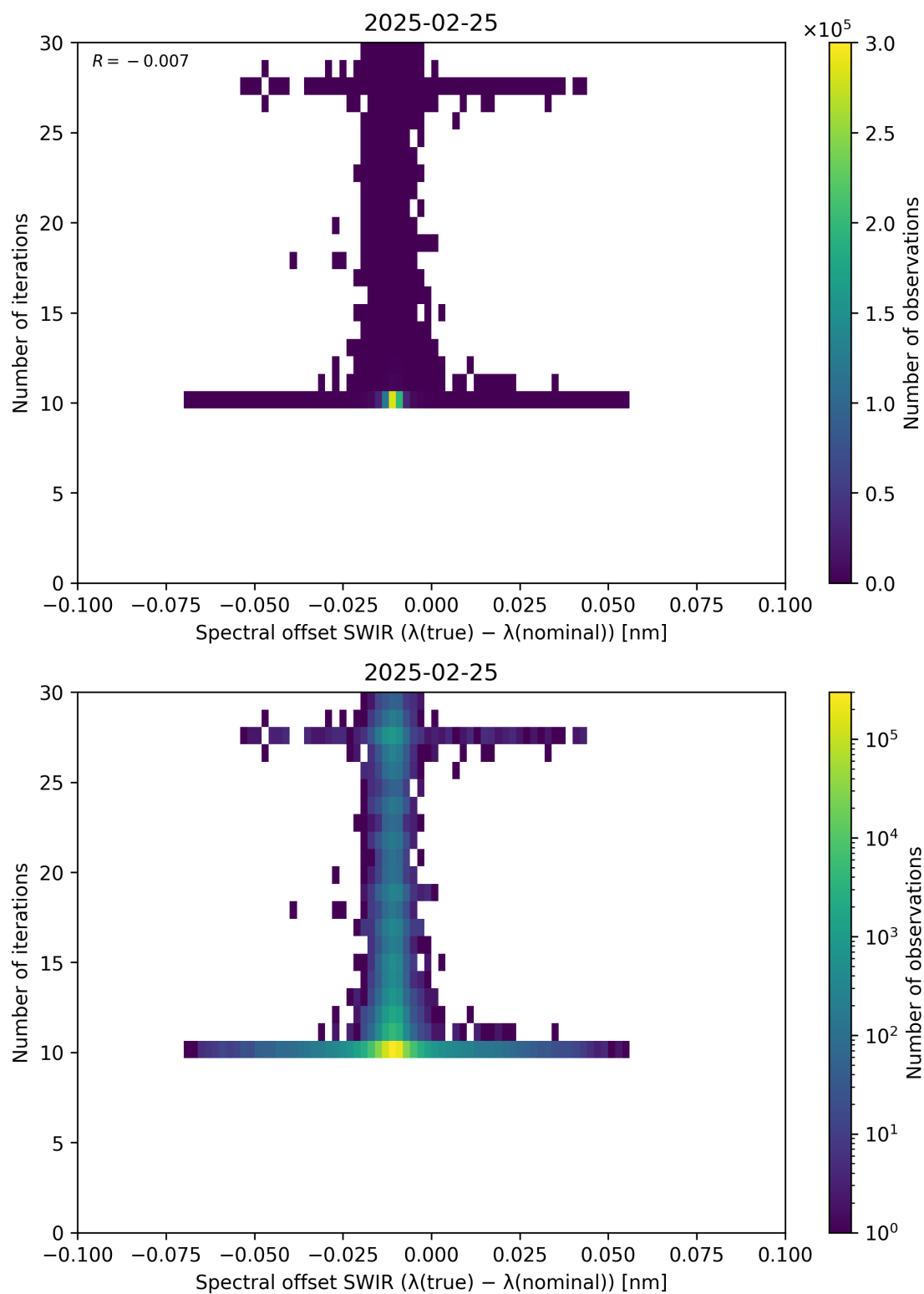
Figure 121: Scatter density plot of “Spectral offset SWIR ( \lambda_{\text{true}} - \lambda_{\text{nominal}} )” against “Number of iterations” for 2025-02-24 to 2025-02-26.
