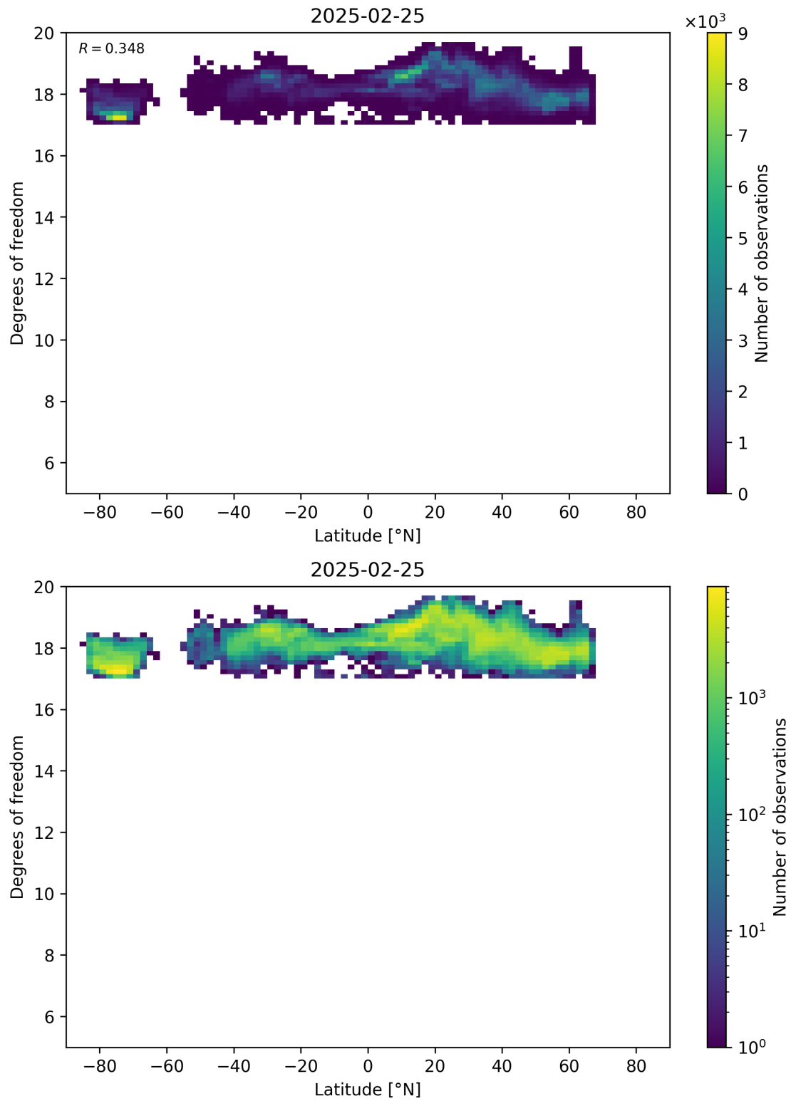
Figure 55: Scatter density plot of “Latitude” against “Degrees of freedom” for 2025-02-24 to 2025-02-26.
