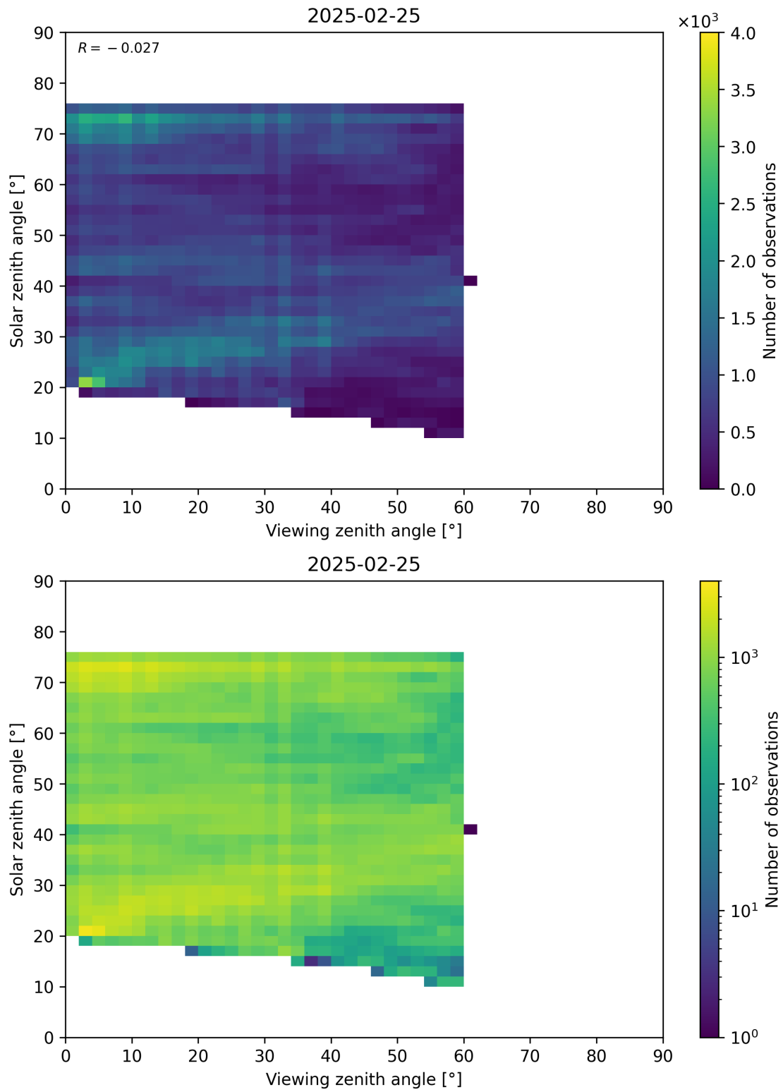
Figure 115: Scatter density plot of “Viewing zenith angle” against “Solar zenith angle” for 2025-02-24 to 2025-02-26.
