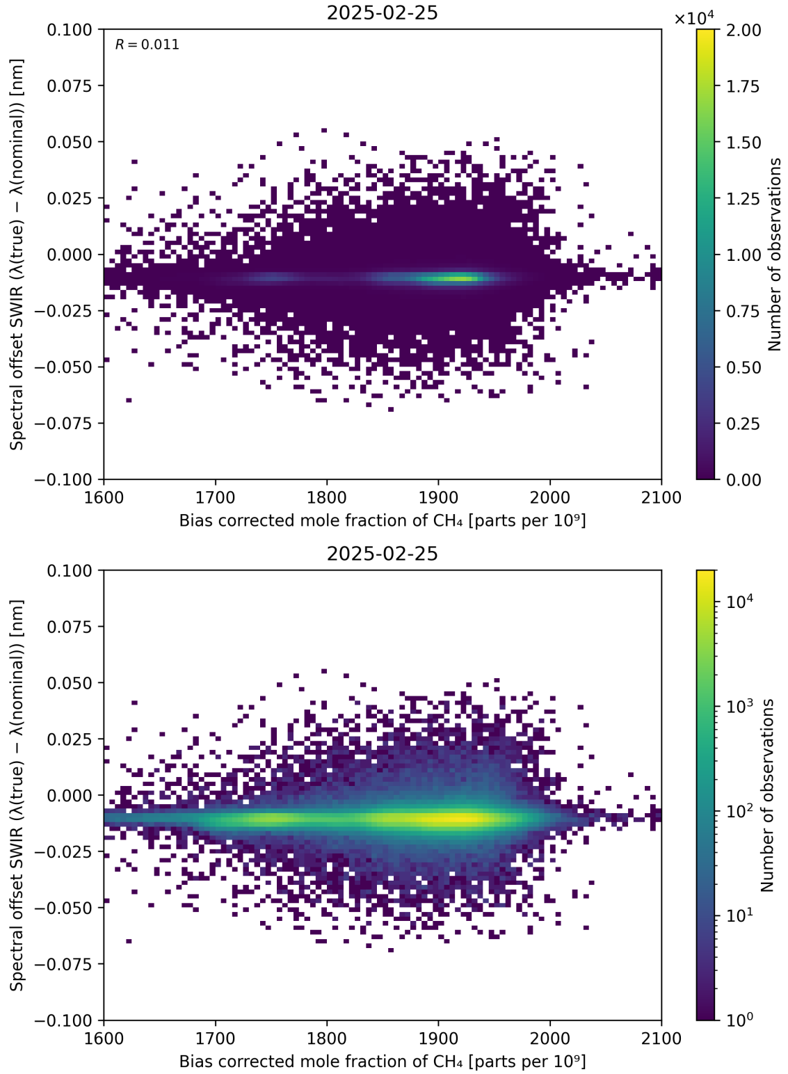
Figure 69: Scatter density plot of “Bias corrected mole fraction of \text{CH}_4 ” against “Spectral offset SWIR ( \lambda_{\text{true}} - \lambda_{\text{nominal}} )” for 2025-02-24 to 2025-02-26.
