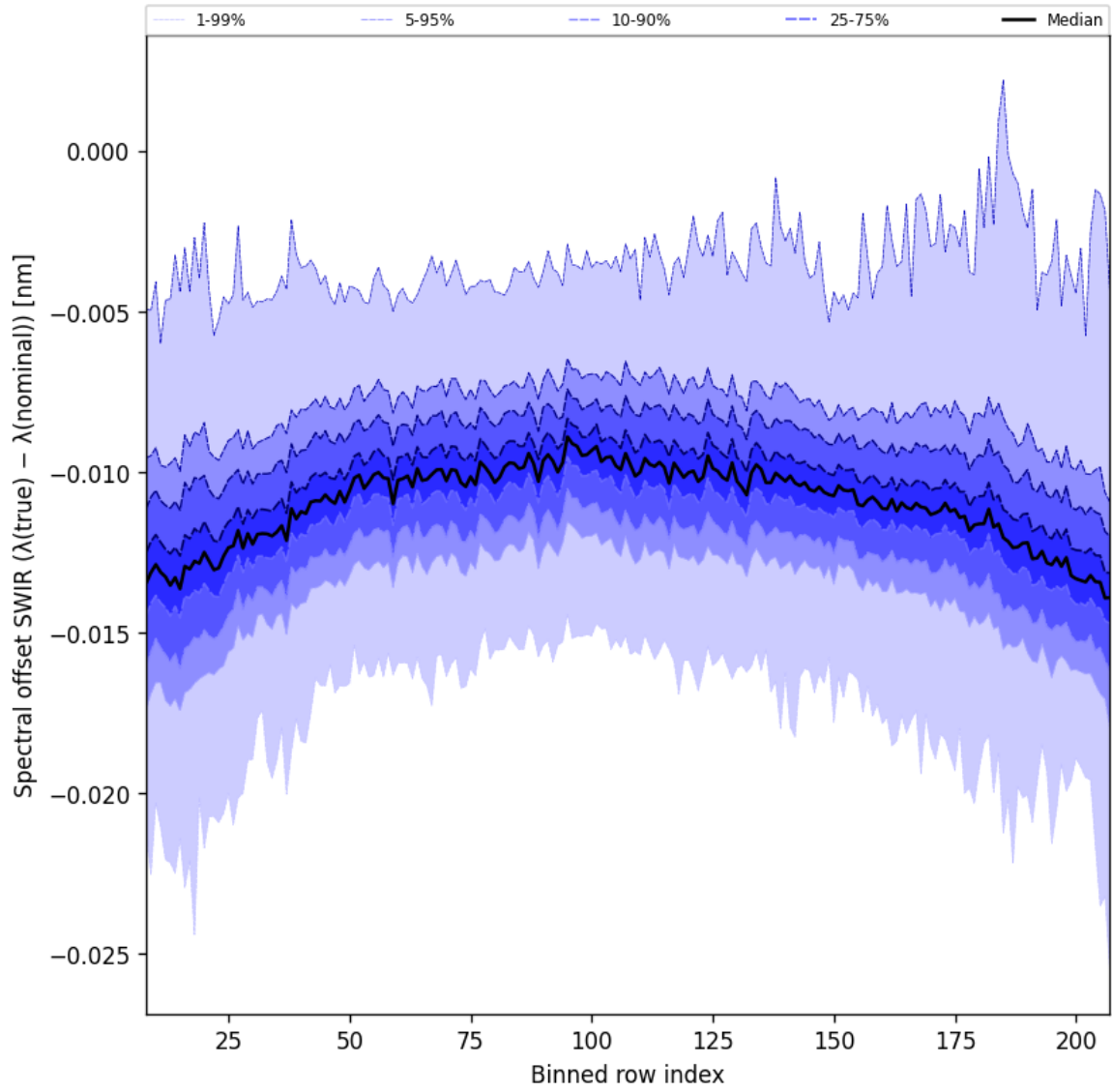
Figure 38: Along track statistics of “Spectral offset SWIR ( \lambda_{\text{true}} - \lambda_{\text{nominal}} )” for 2025-02-24 to 2025-02-26
