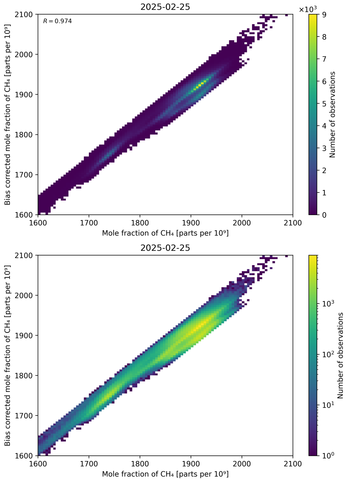
Figure 74: Scatter density plot of “Mole fraction of CH 4 ” against “Bias corrected mole fraction of CH 4 ” for 2025-02-24 to 2025-02-26.
