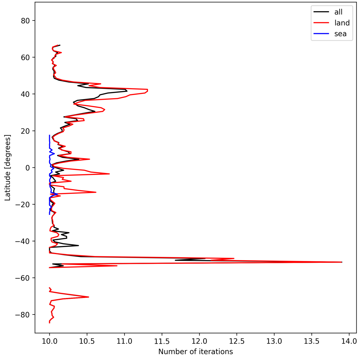
Figure 20: Zonal average of “Number of iterations” for 2025-02-24 to 2025-02-26.
