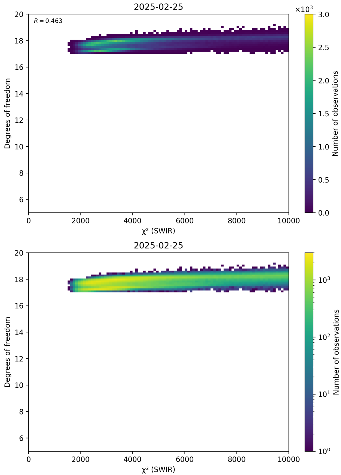
Figure 48: Scatter density plot of “ \chi^2 (SWIR)” against “Degrees of freedom” for 2025-02-24 to 2025-02-26.
