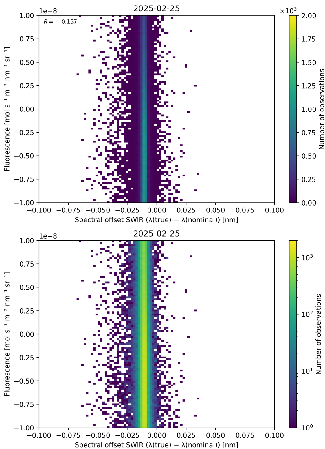
Figure 120: Scatter density plot of “Spectral offset SWIR ( \lambda_{\text{true}} - \lambda_{\text{nominal}} )” against “Fluorescence” for 2025-02-24 to 2025-02-26.
