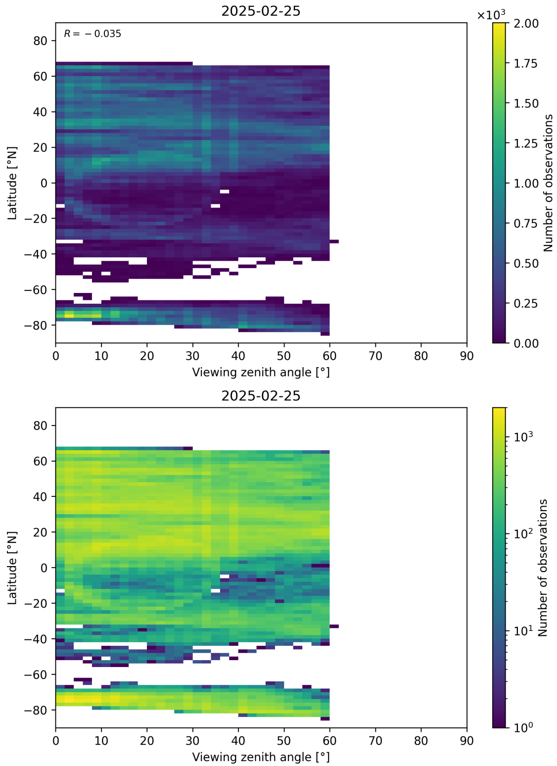
Figure 109: Scatter density plot of “Viewing zenith angle” against “Latitude” for 2025-02-24 to 2025-02-26.
