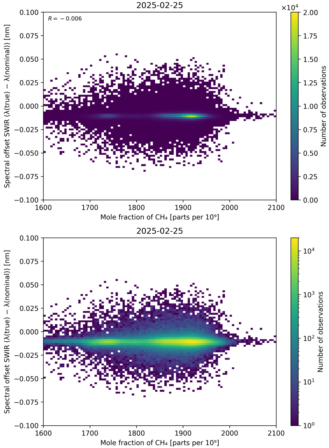
Figure 86: Scatter density plot of “Mole fraction of \text{CH}_4 ” against “Spectral offset SWIR ( \lambda_{\text{true}} - \lambda_{\text{nominal}} )” for 2025-02-24 to 2025-02-26.
