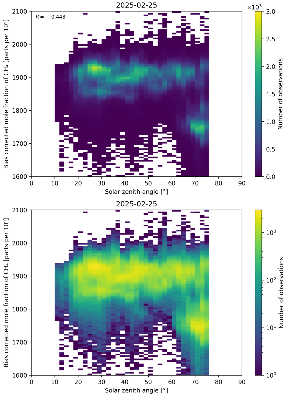
Figure 100: Scatter density plot of “Solar zenith angle” against “Bias corrected mole fraction of \text{CH}_4 ” for 2025-02-24 to 2025-02-26.
