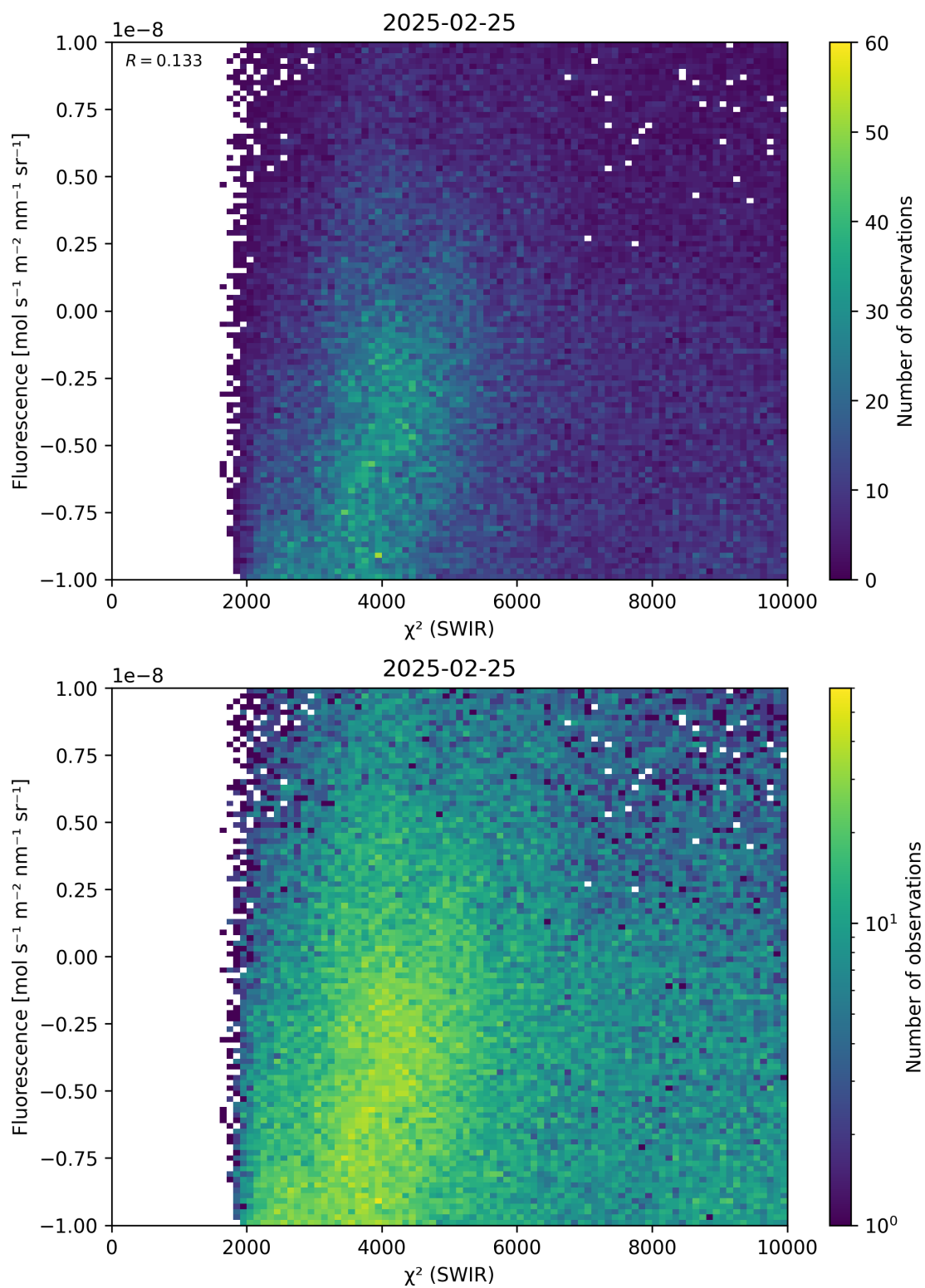
Figure 49: Scatter density plot of “ \chi^2 (SWIR)” against “Fluorescence” for 2025-02-24 to 2025-02-26.
