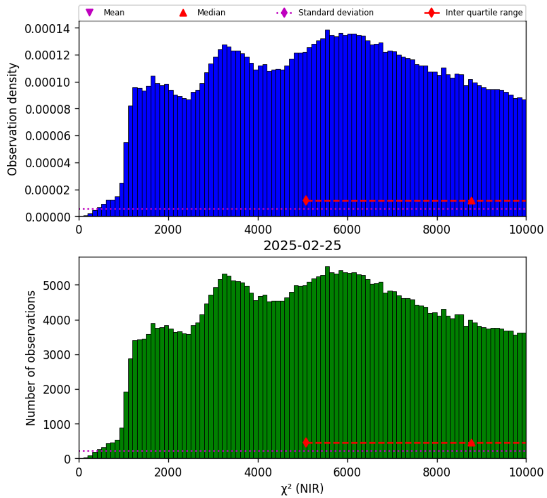
Figure 29: Histogram of “ \chi^2 (NIR)” for 2025-02-24 to 2025-02-26
