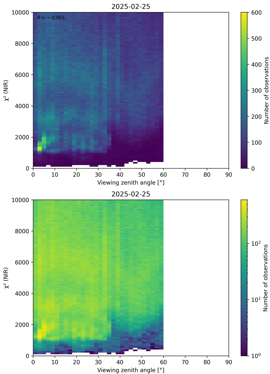
Figure 105: Scatter density plot of “Viewing zenith angle” against “ \chi^2 (NIR)” for 2025-02-24 to 2025-02-26.
