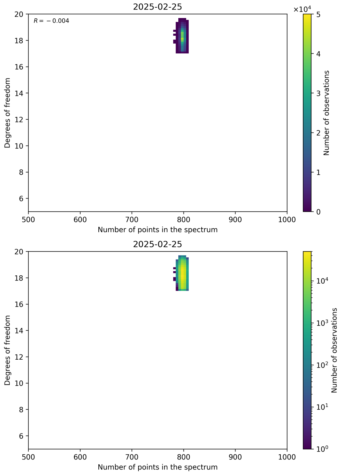
Figure 90: Scatter density plot of “Number of points in the spectrum” against “Degrees of freedom” for 2025-02-24 to 2025-02-26.
