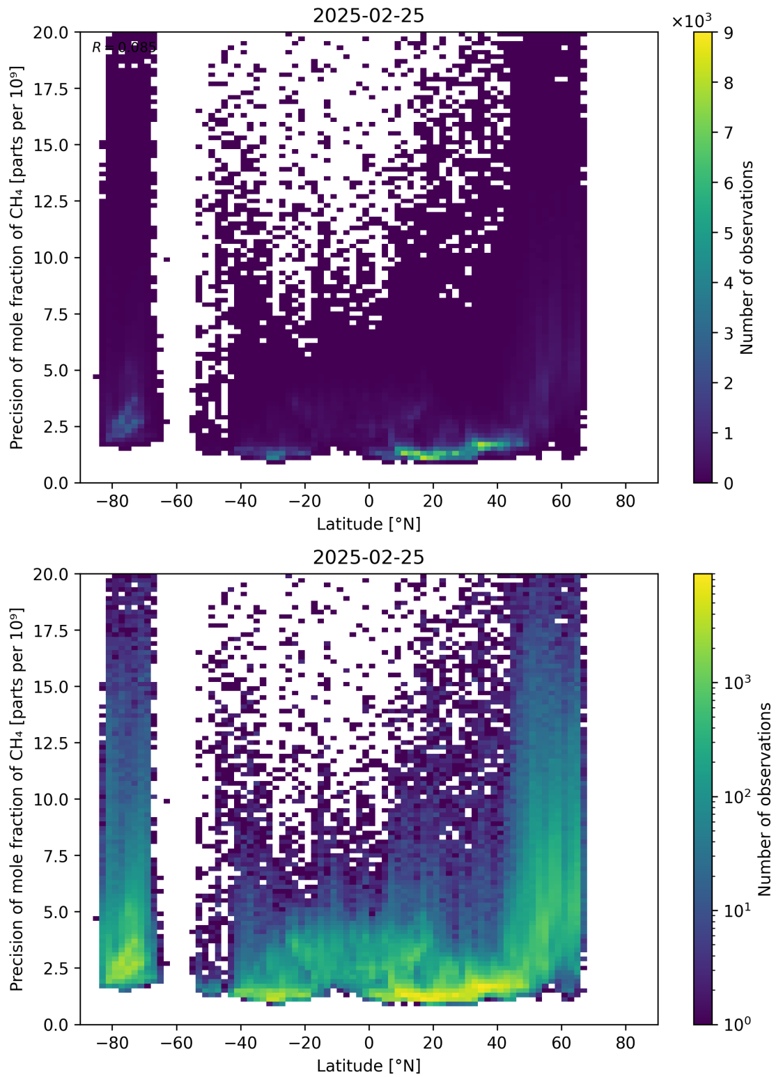
Figure 59: Scatter density plot of “Latitude” against “Precision of mole fraction of CH 4 ” for 2025-02-24 to 2025-02-26.
