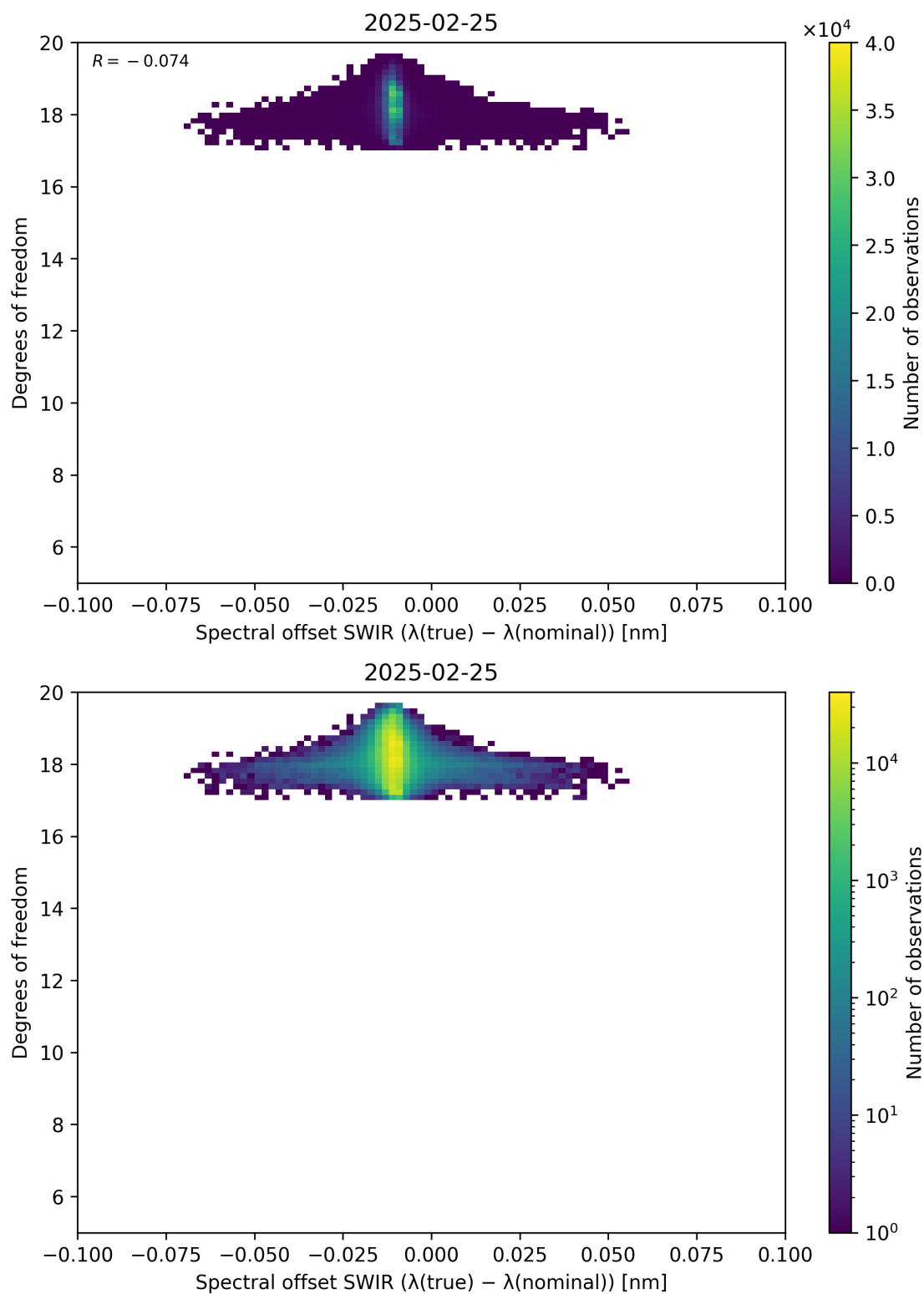
Figure 119: Scatter density plot of “Spectral offset SWIR ( \lambda_{\text{true}} - \lambda_{\text{nominal}} )” against “Degrees of freedom” for 2025-02-24 to 2025-02-26.
