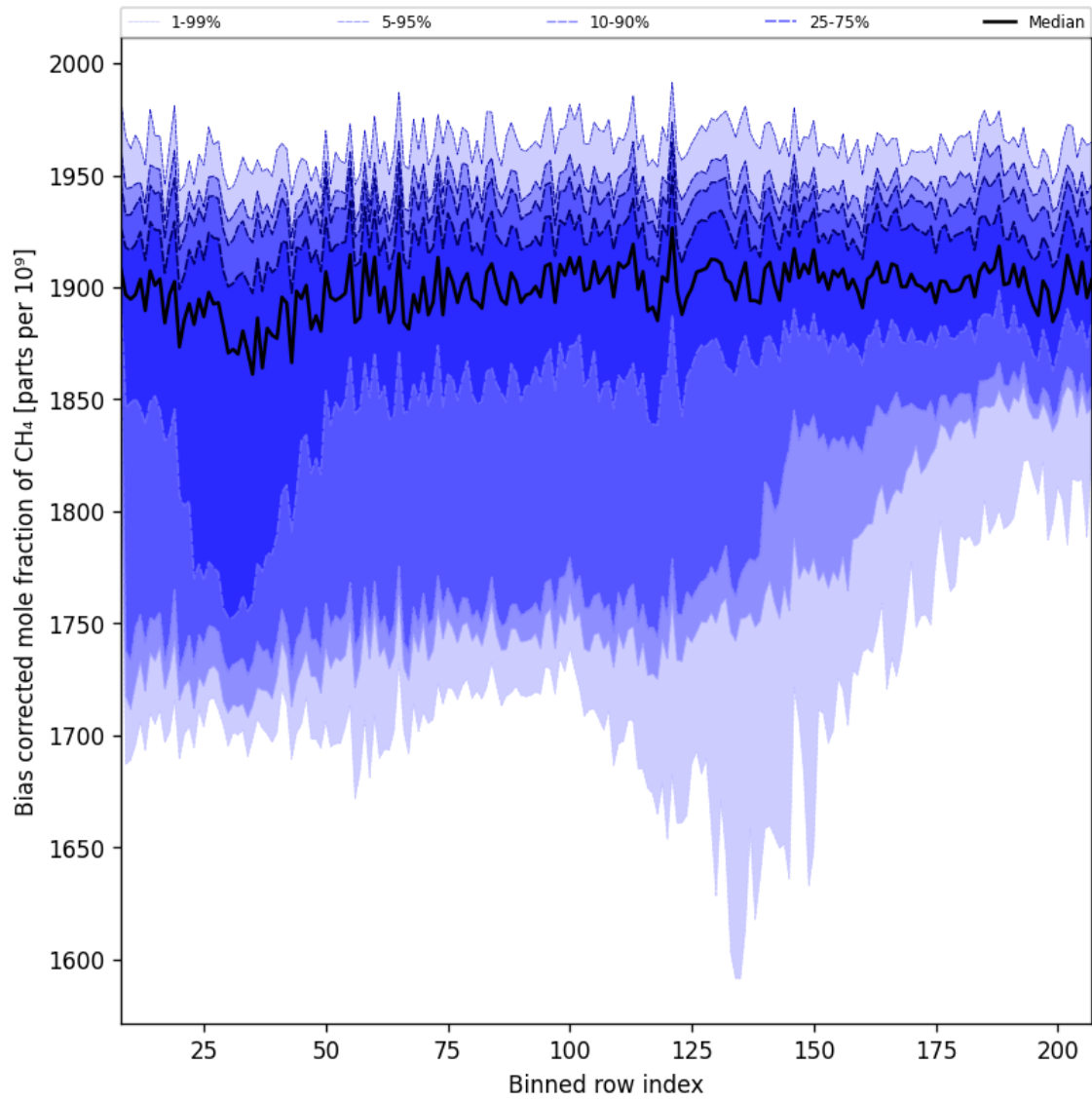
Figure 36: Along track statistics of “Bias corrected mole fraction of CH 4 ” for 2025-02-24 to 2025-02-26
