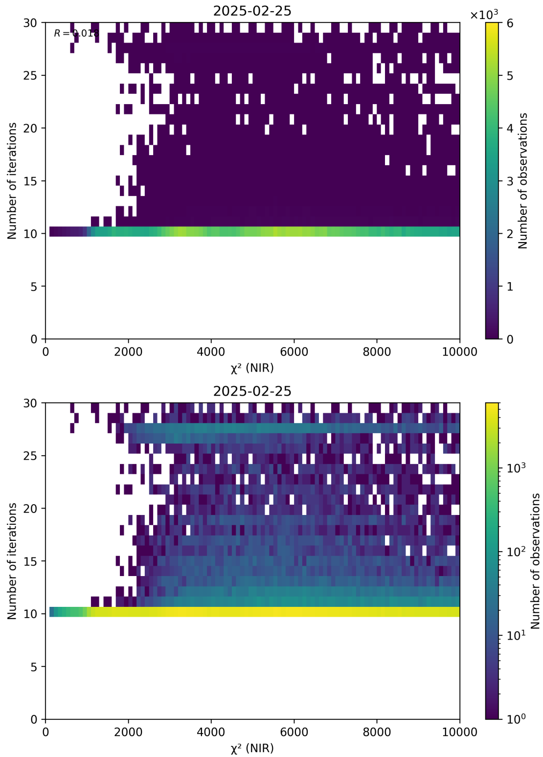
Figure 46: Scatter density plot of “ \chi^2 (NIR)” against “Number of iterations” for 2025-02-24 to 2025-02-26.
