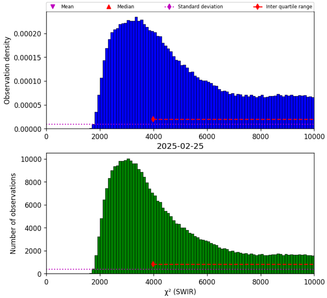
Figure 28: Histogram of “ \chi^2 (SWIR)” for 2025-02-24 to 2025-02-26
