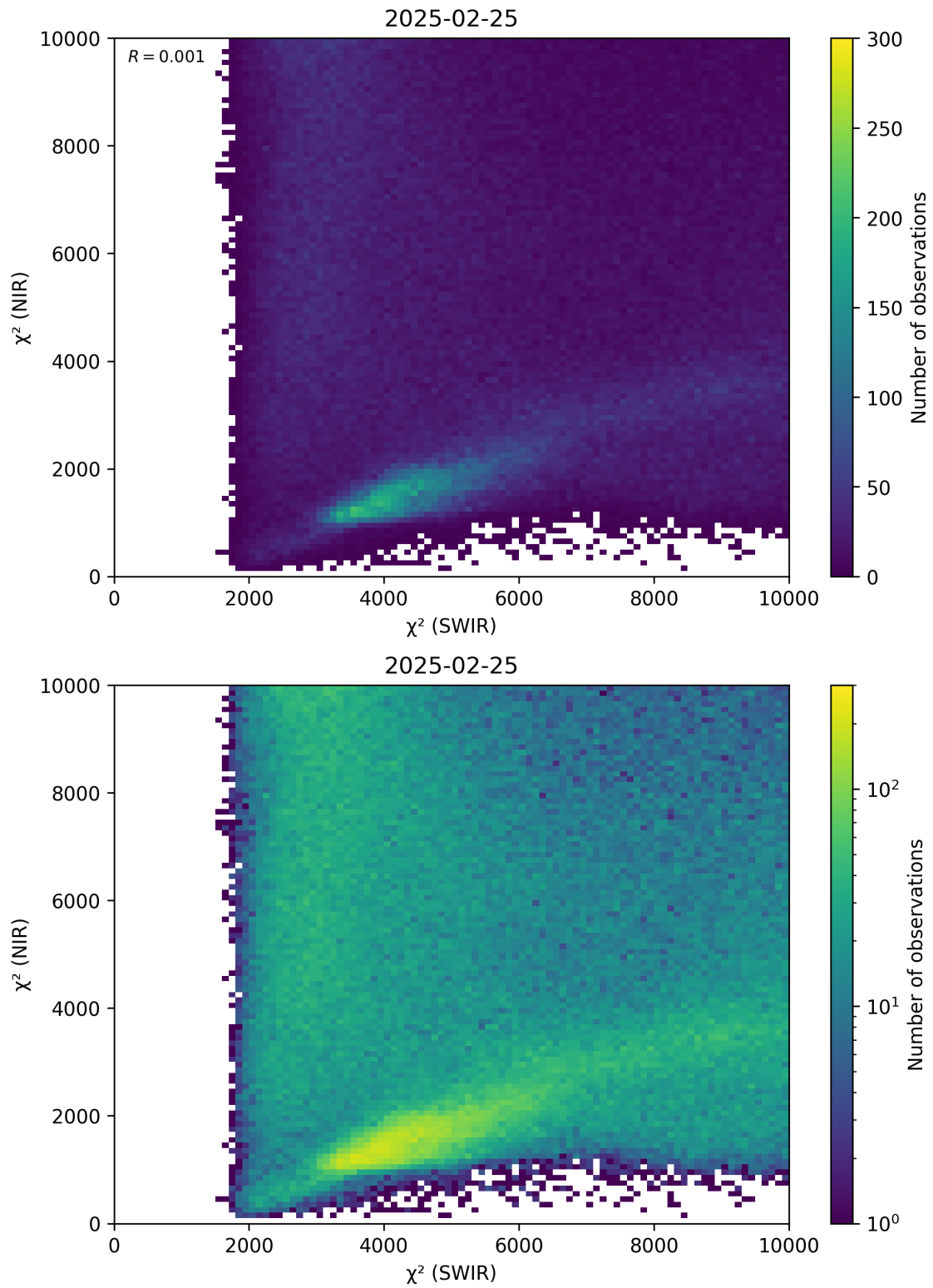
Figure 47: Scatter density plot of “ \chi^2 (SWIR)” against “ \chi^2 (NIR)” for 2025-02-24 to 2025-02-26.
