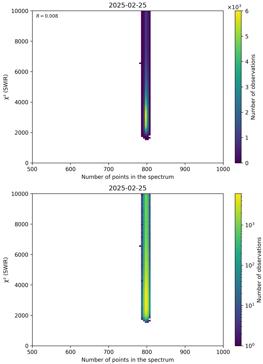
Figure 89: Scatter density plot of “Number of points in the spectrum” against “ \chi^2 (SWIR)” for 2025-02-24 to 2025-02-26.
