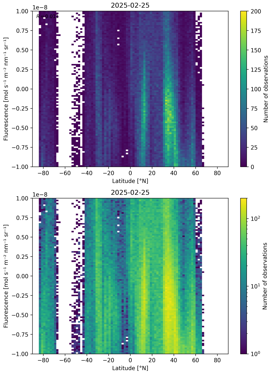
Figure 56: Scatter density plot of “Latitude” against “Fluorescence” for 2025-02-24 to 2025-02-26.
