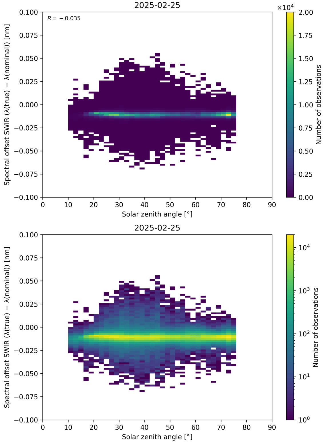
Figure 104: Scatter density plot of “Solar zenith angle” against “Spectral offset SWIR ( \lambda_{\text{true}} - \lambda_{\text{nominal}} )” for 2025-02-24 to 2025-02-26.
