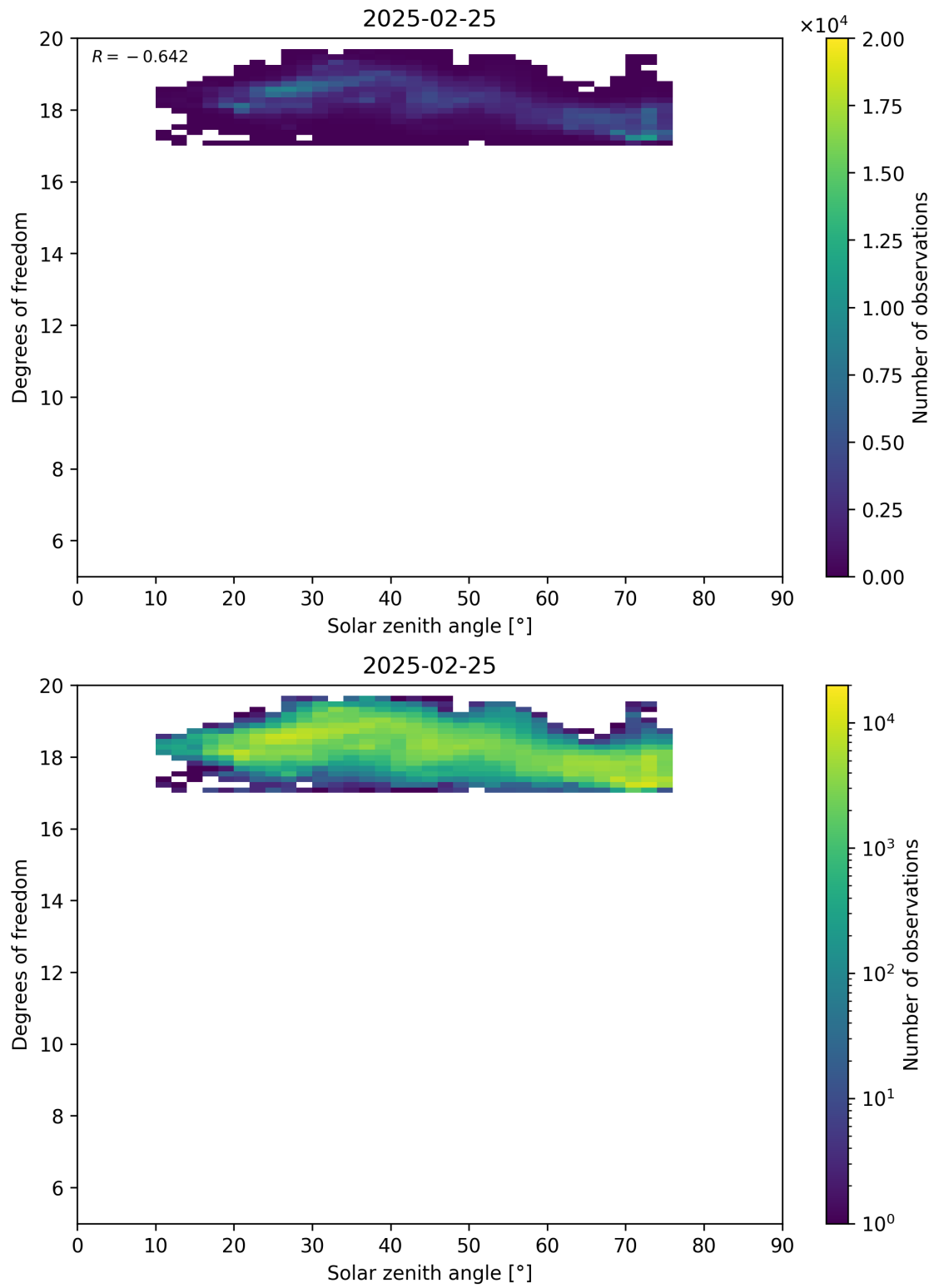
Figure 96: Scatter density plot of “Solar zenith angle” against “Degrees of freedom” for 2025-02-24 to 2025-02-26.
