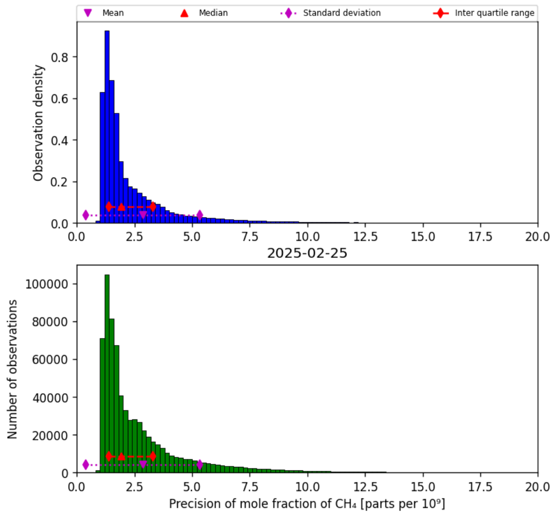
Figure 24: Histogram of “Precision of mole fraction of CH 4 ” for 2025-02-24 to 2025-02-26
