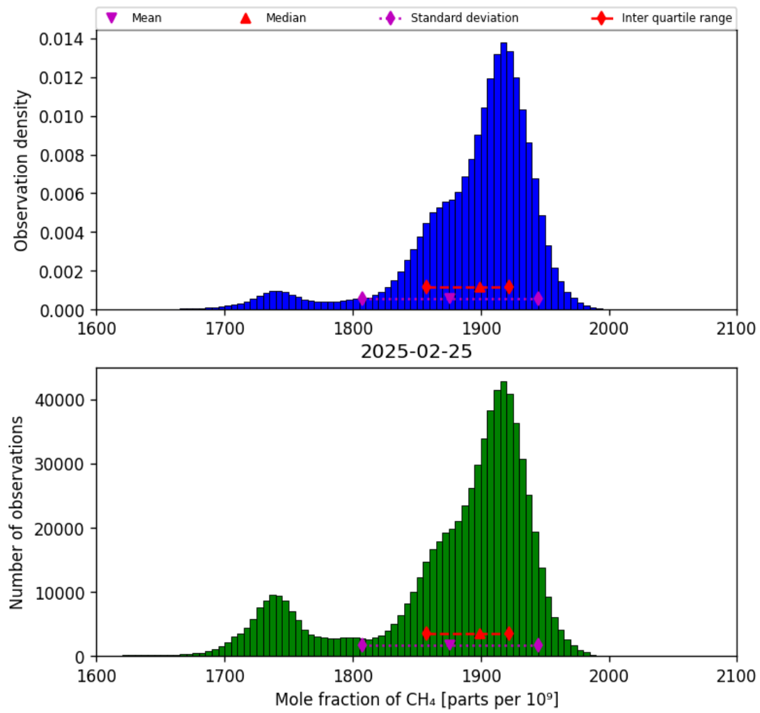
Figure 23: Histogram of “Mole fraction of CH 4 ” for 2025-02-24 to 2025-02-26
