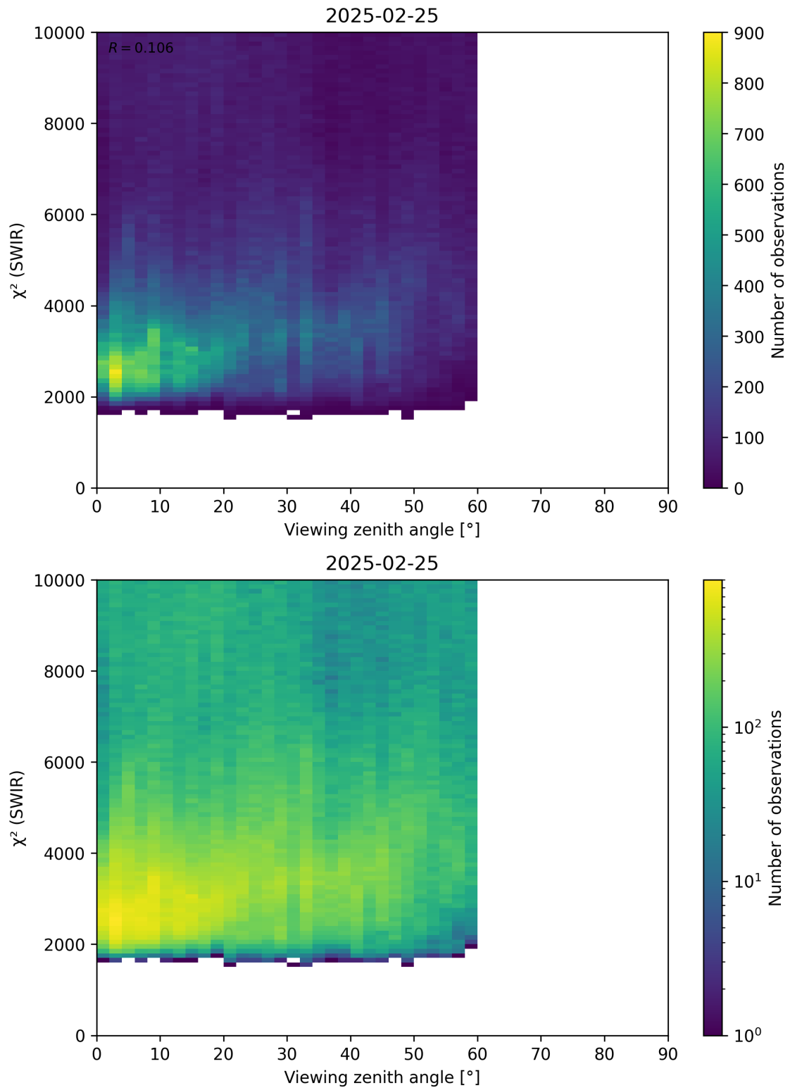
Figure 106: Scatter density plot of “Viewing zenith angle” against “ \chi^2 (SWIR)” for 2025-02-24 to 2025-02-26.
