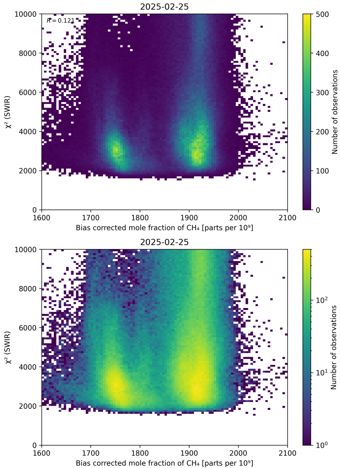
Figure 64: Scatter density plot of “Bias corrected mole fraction of CH 4 ” against “ \chi^2 (SWIR)” for 2025-02-24 to 2025-02-26.
