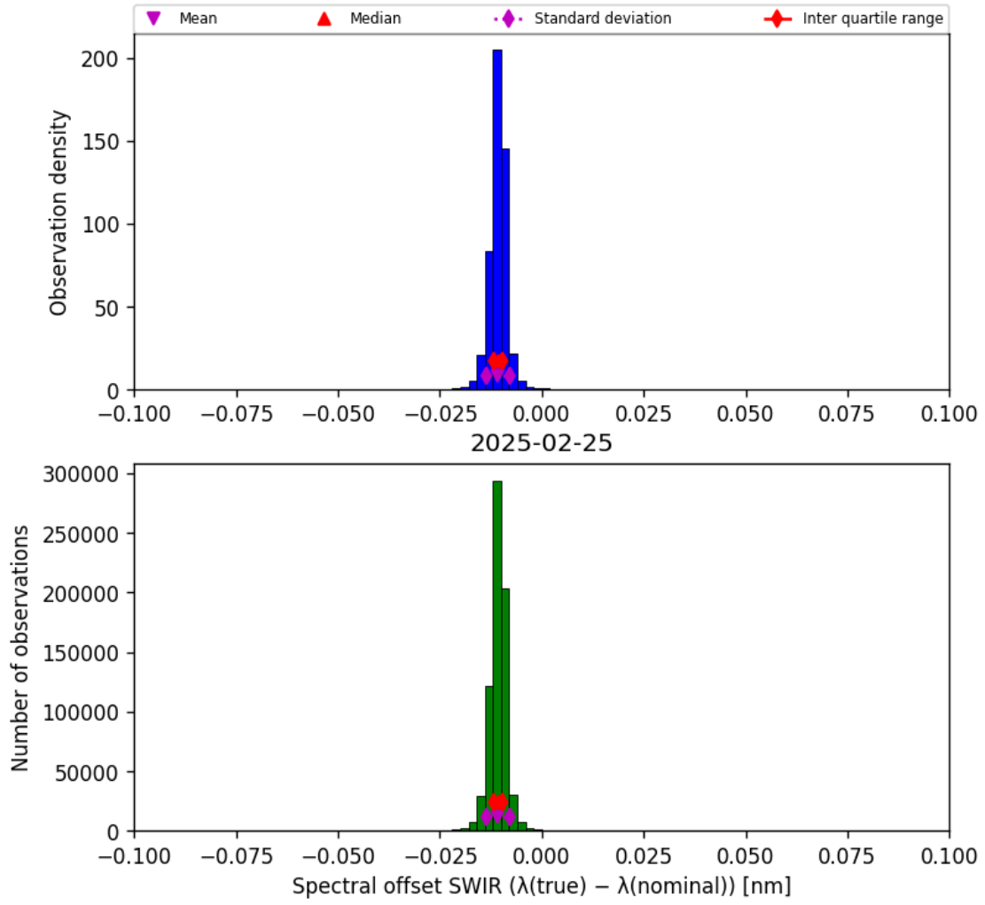
Figure 27: Histogram of “Spectral offset SWIR ( \lambda_{\text{true}} - \lambda_{\text{nominal}} )” for 2025-02-24 to 2025-02-26
