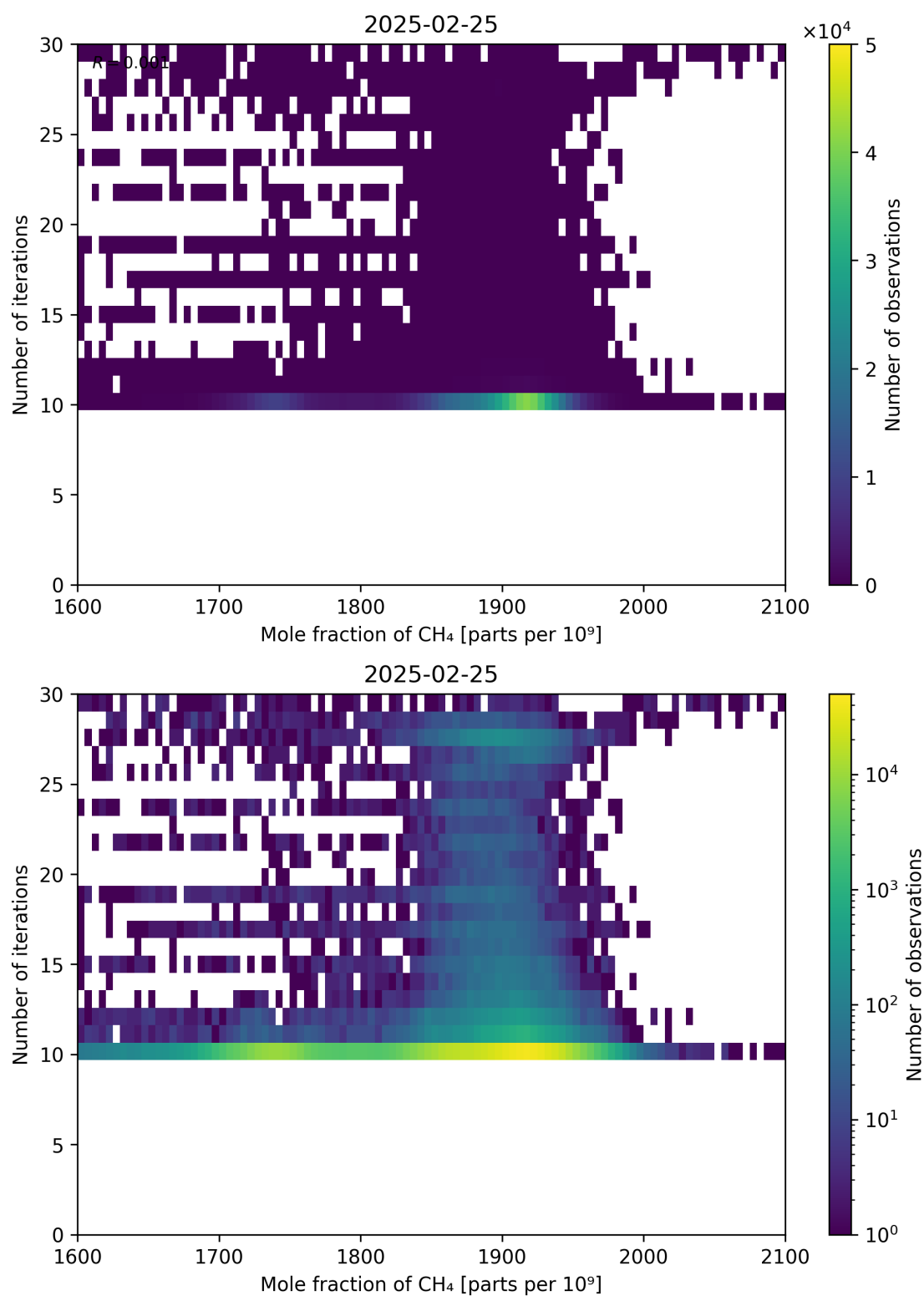
Figure 76: Scatter density plot of “Mole fraction of CH 4 ” against “Number of iterations” for 2025-02-24 to 2025-02-26.
