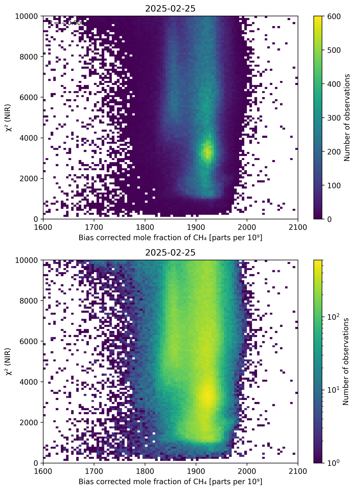
Figure 63: Scatter density plot of “Bias corrected mole fraction of \text{CH}_4 ” against “ \chi^2 (NIR)” for 2025-02-24 to 2025-02-26.
