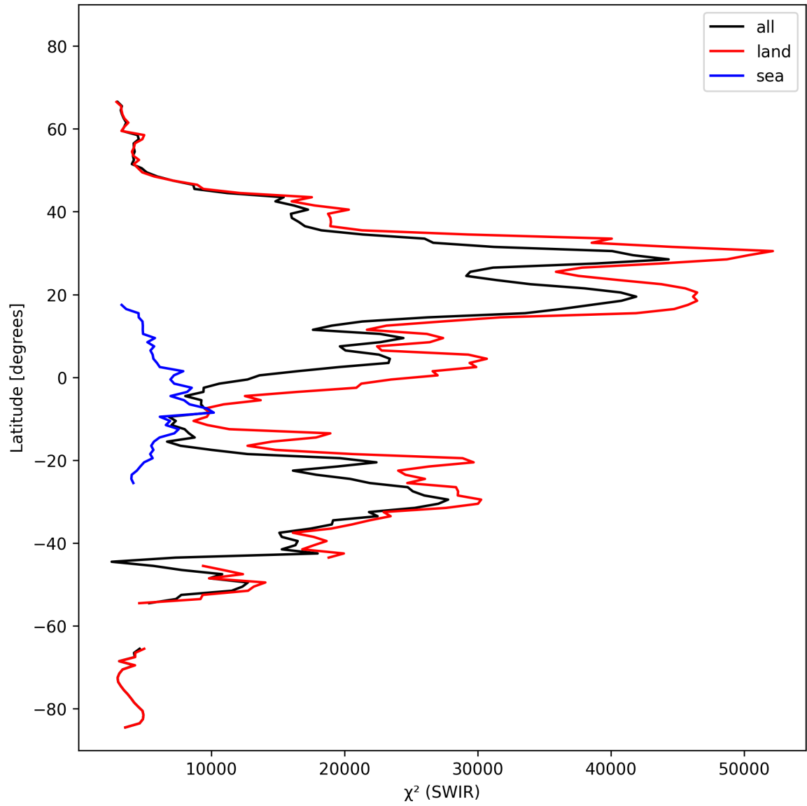
Figure 17: Zonal average of “ \chi^2 (SWIR)” for 2025-02-24 to 2025-02-26.
