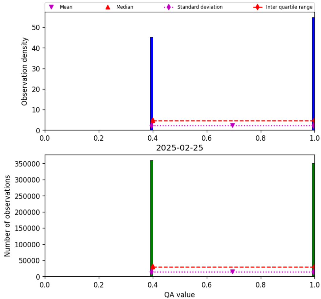
Figure 22: Histogram of “QA value” for 2025-02-24 to 2025-02-26
