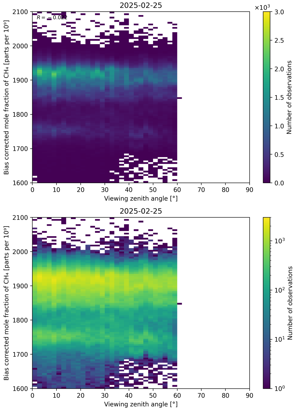
Figure 111: Scatter density plot of “Viewing zenith angle” against “Bias corrected mole fraction of CH 4 ” for 2025-02-24 to 2025-02-26.
