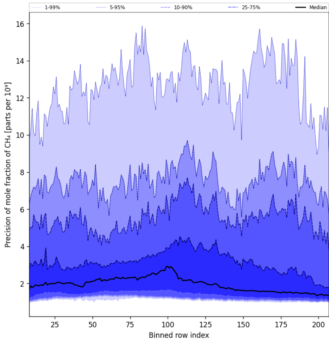
Figure 35: Along track statistics of “Precision of mole fraction of CH 4 ” for 2025-02-24 to 2025-02-26
