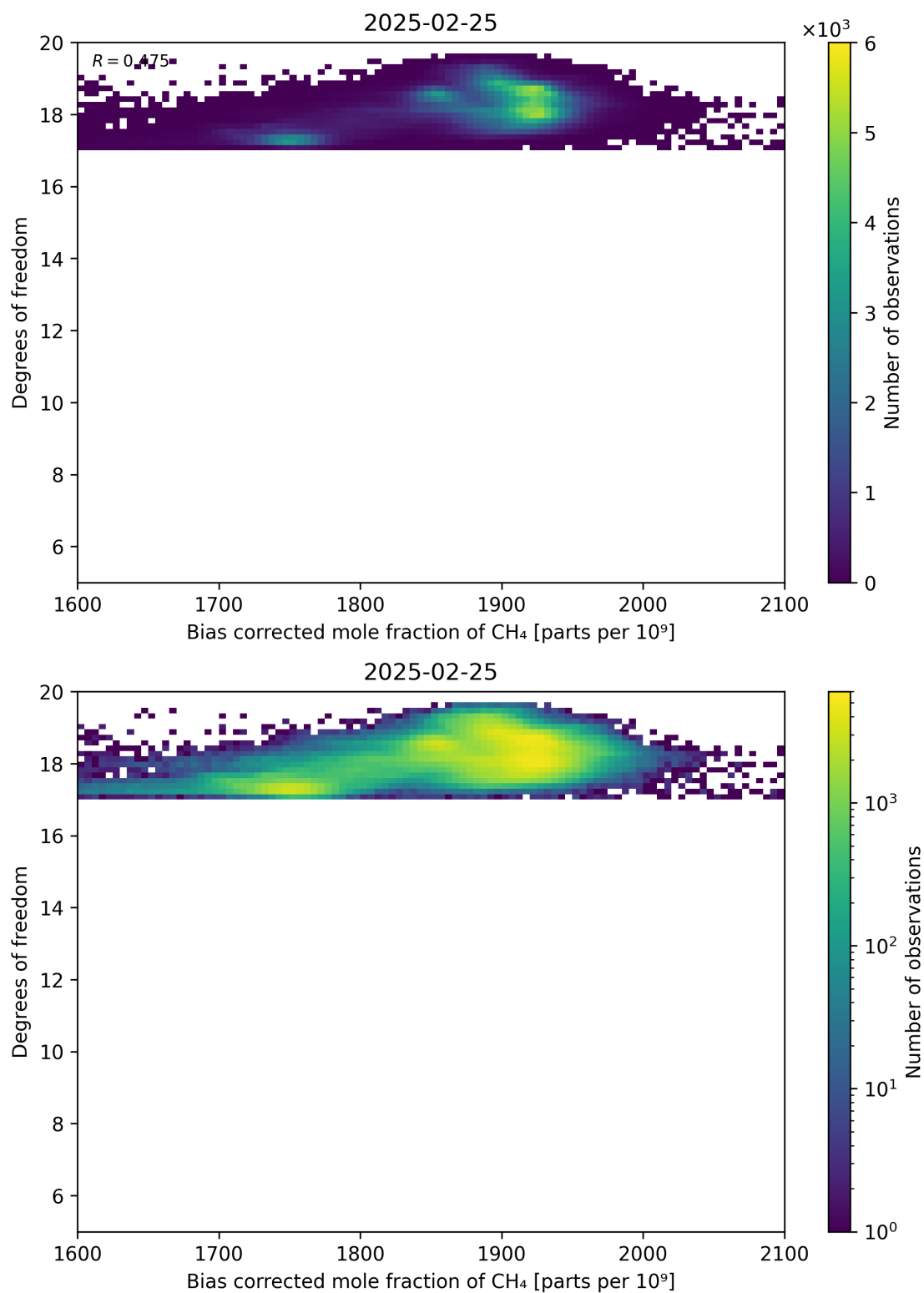
Figure 65: Scatter density plot of “Bias corrected mole fraction of CH 4 ” against “Degrees of freedom” for 2025-02-24 to 2025-02-26.
