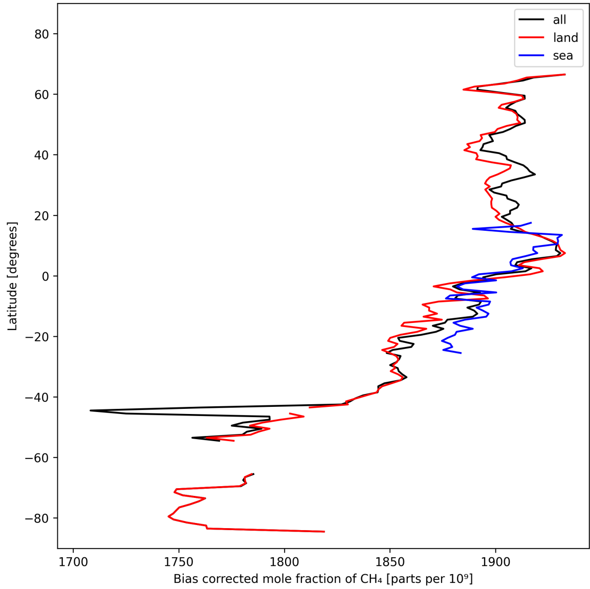
Figure 14: Zonal average of “Bias corrected mole fraction of CH 4 ” for 2025-02-24 to 2025-02-26.
