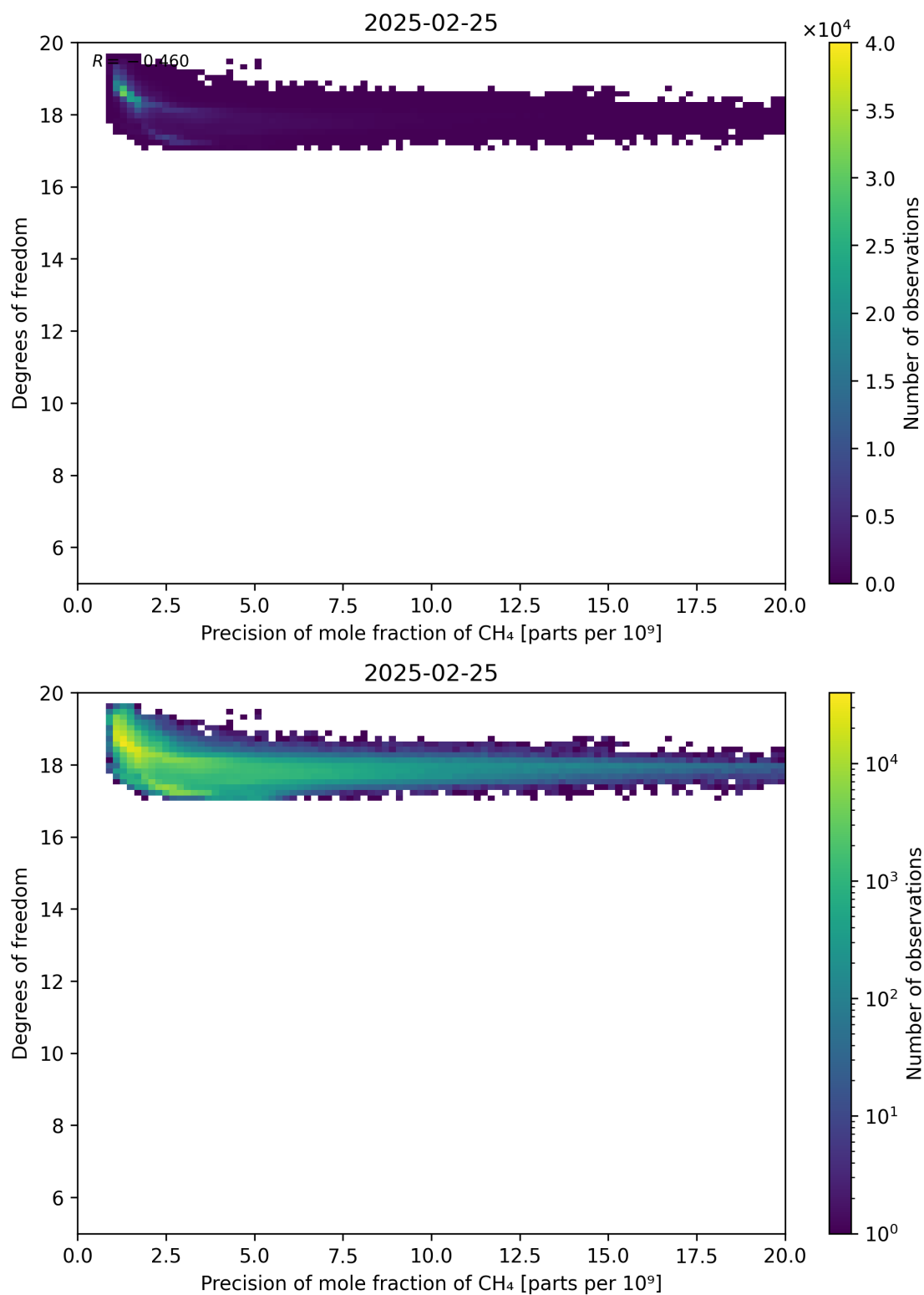
Figure 80: Scatter density plot of “Precision of mole fraction of CH 4 ” against “Degrees of freedom” for 2025-02-24 to 2025-02-26.
