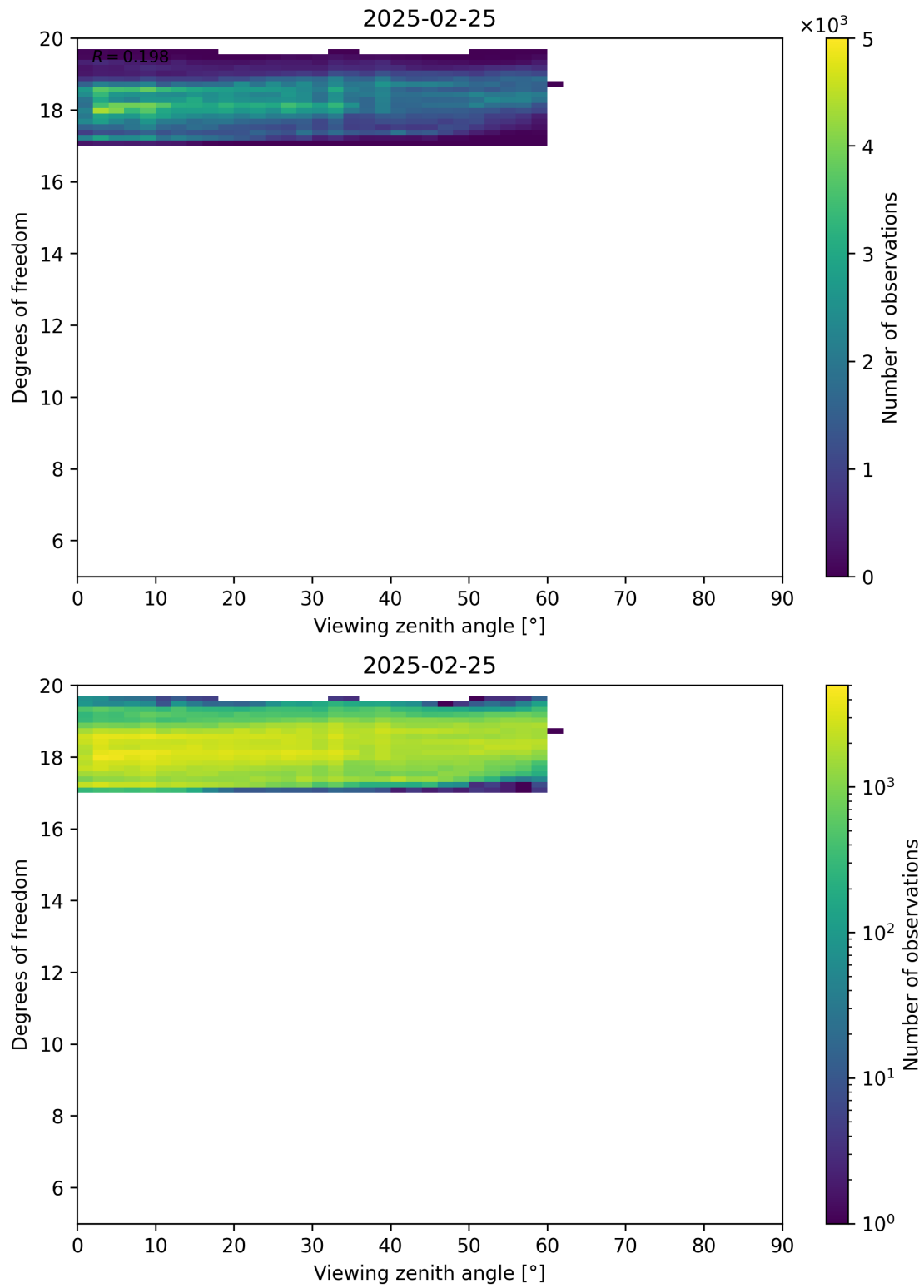
Figure 107: Scatter density plot of “Viewing zenith angle” against “Degrees of freedom” for 2025-02-24 to 2025-02-26.
