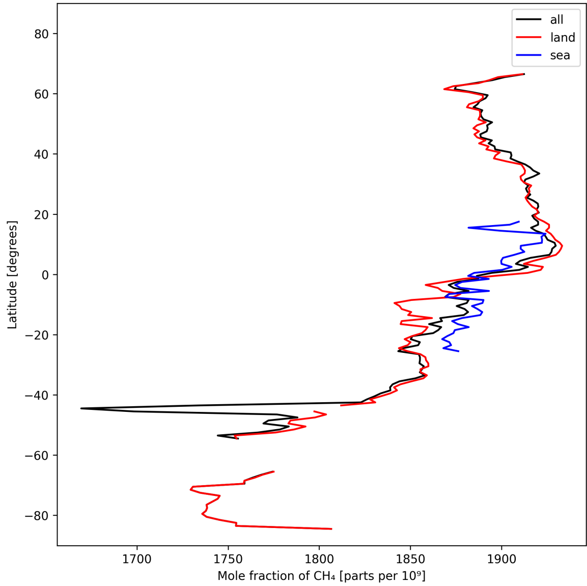
Figure 12: Zonal average of “Mole fraction of CH 4 ” for 2025-02-24 to 2025-02-26.
