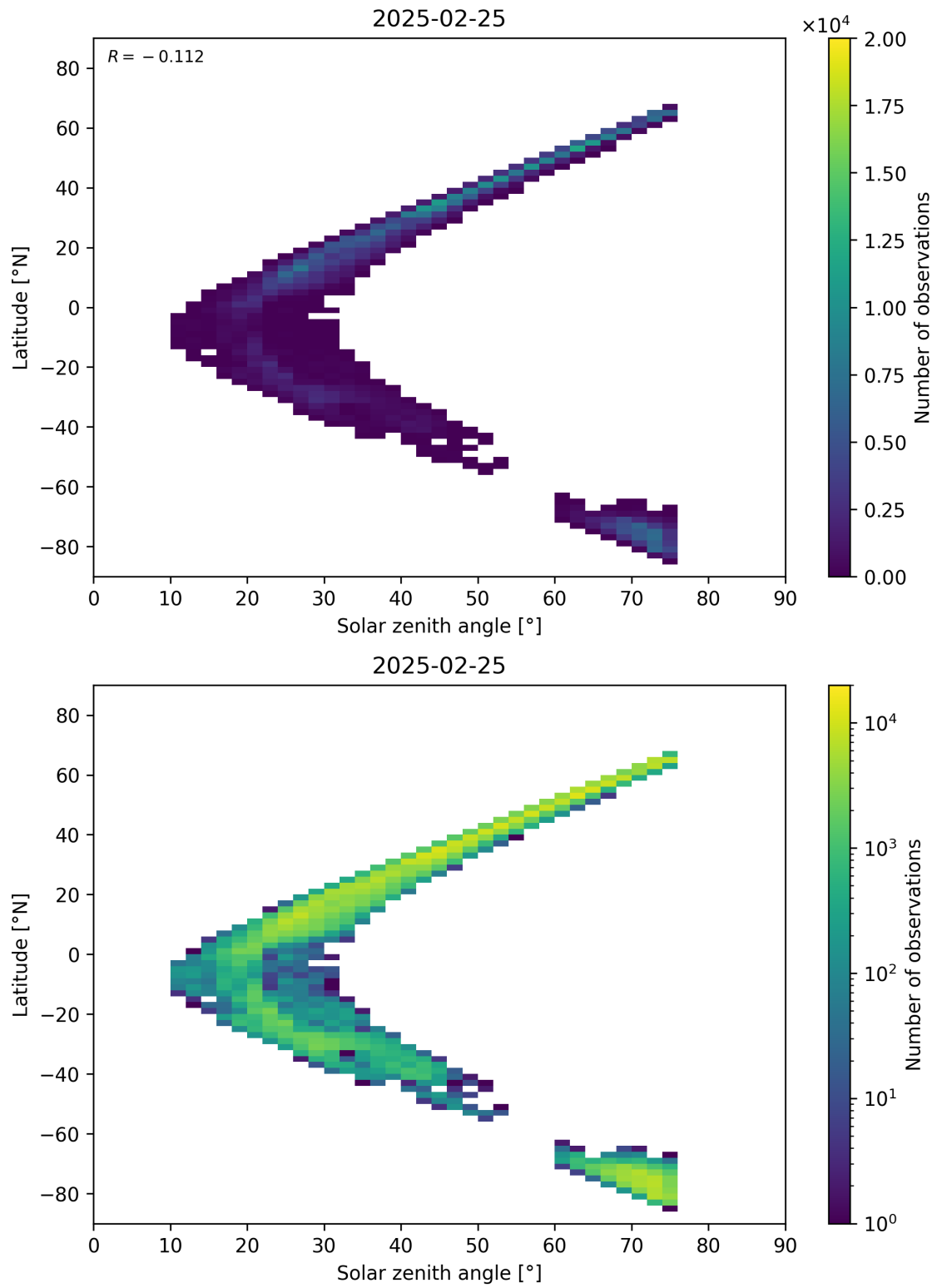
Figure 98: Scatter density plot of “Solar zenith angle” against “Latitude” for 2025-02-24 to 2025-02-26.
