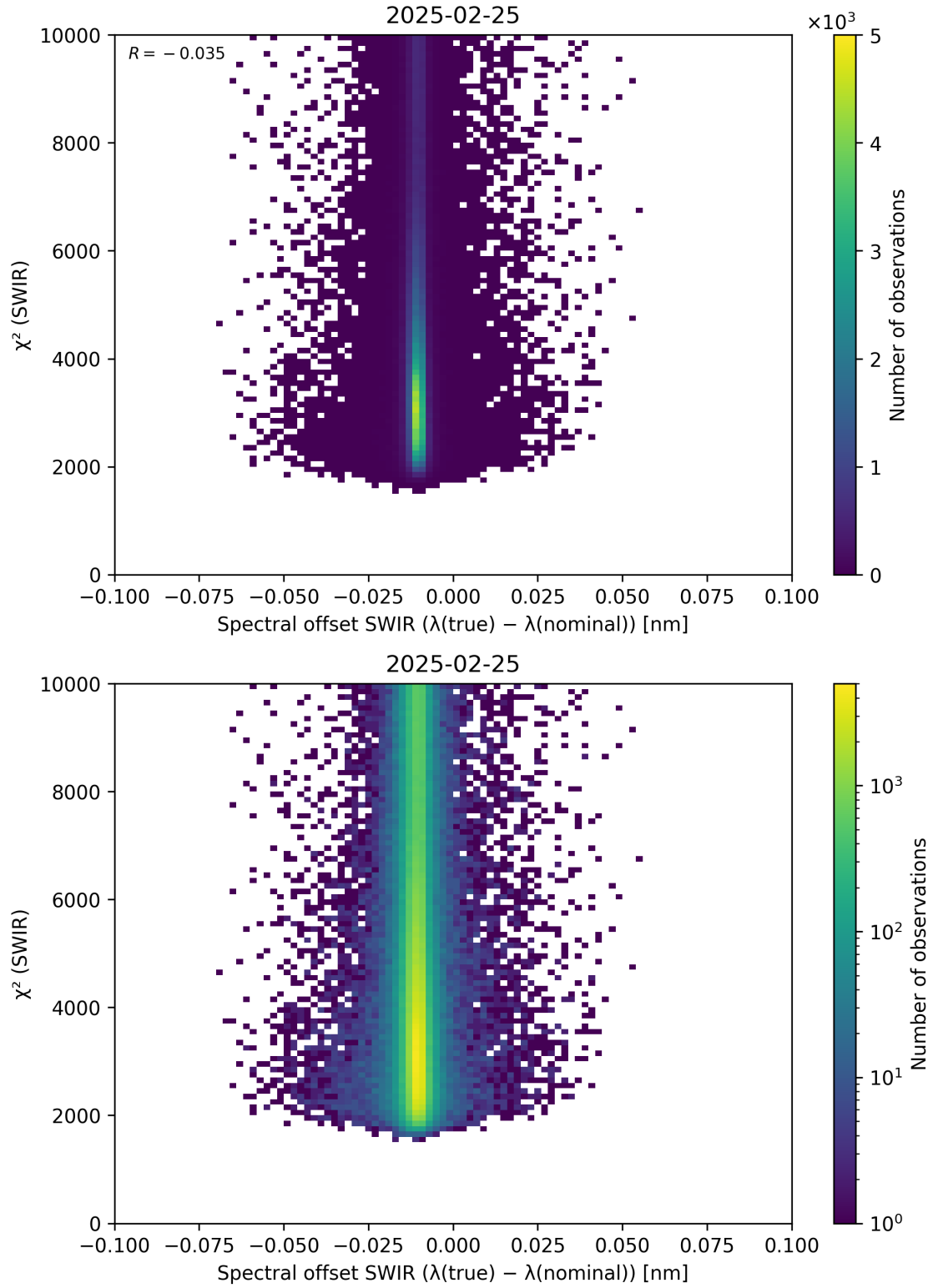
Figure 118: Scatter density plot of “Spectral offset SWIR ( \lambda_{\text{true}} - \lambda_{\text{nominal}} )” against “ \chi^2 (SWIR)” for 2025-02-24 to 2025-02-26.
