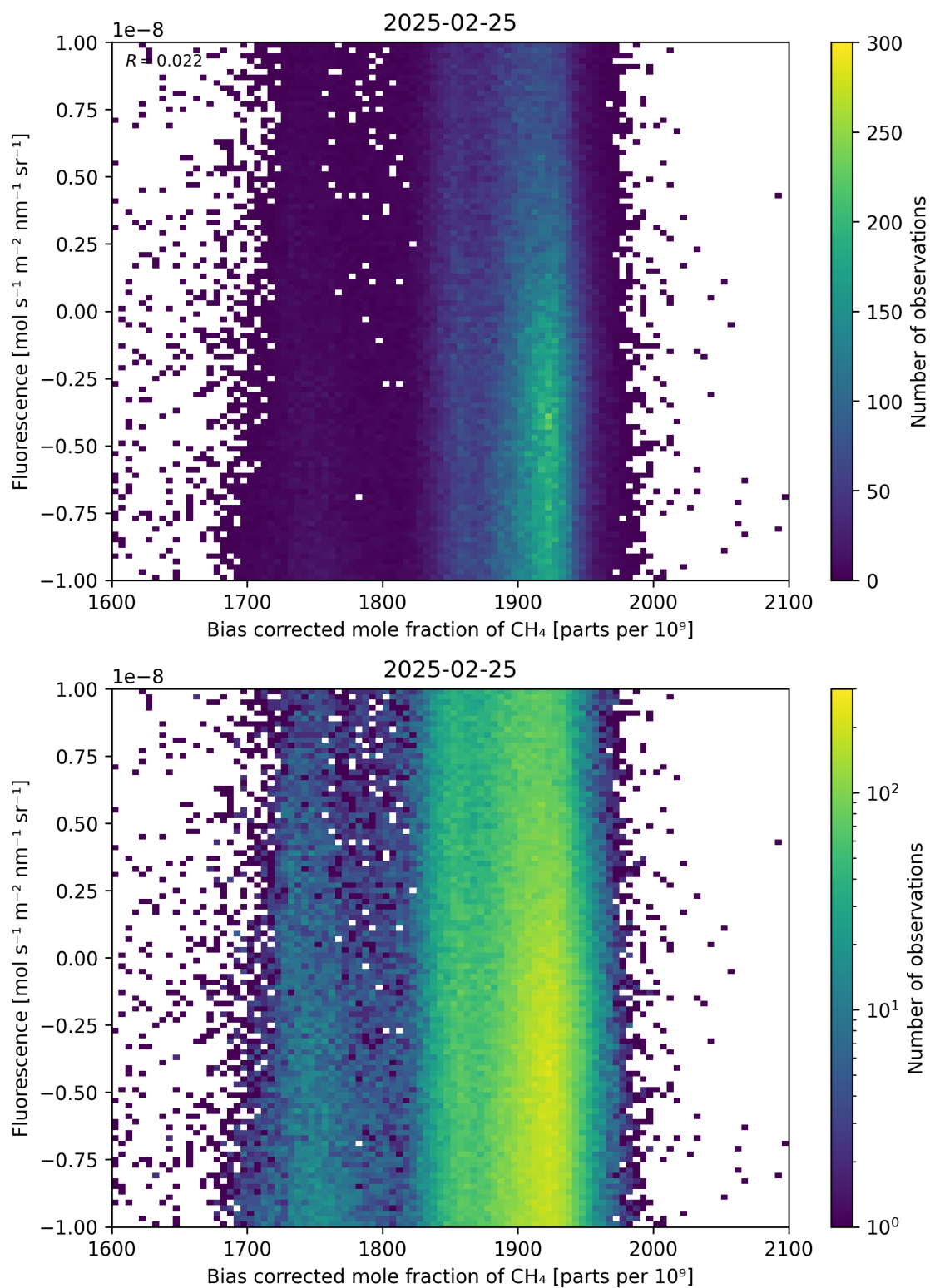
Figure 66: Scatter density plot of “Bias corrected mole fraction of \text{CH}_4 ” against “Fluorescence” for 2025-02-24 to 2025-02-26.
