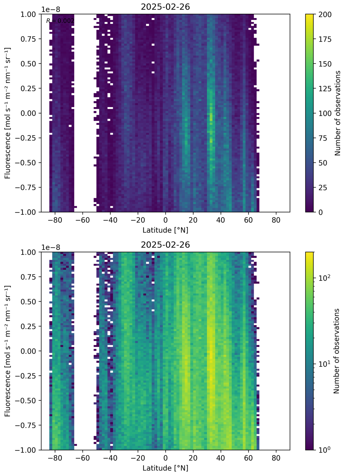
Figure 56: Scatter density plot of “Latitude” against “Fluorescence” for 2025-02-25 to 2025-02-27.
