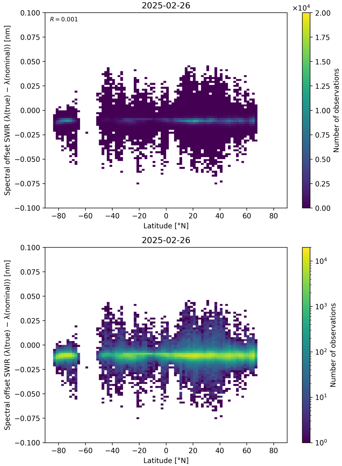
Figure 62: Scatter density plot of “Latitude” against “Spectral offset SWIR ( \lambda_{\text{true}} - \lambda_{\text{nominal}} )” for 2025-02-25 to 2025-02-27.
