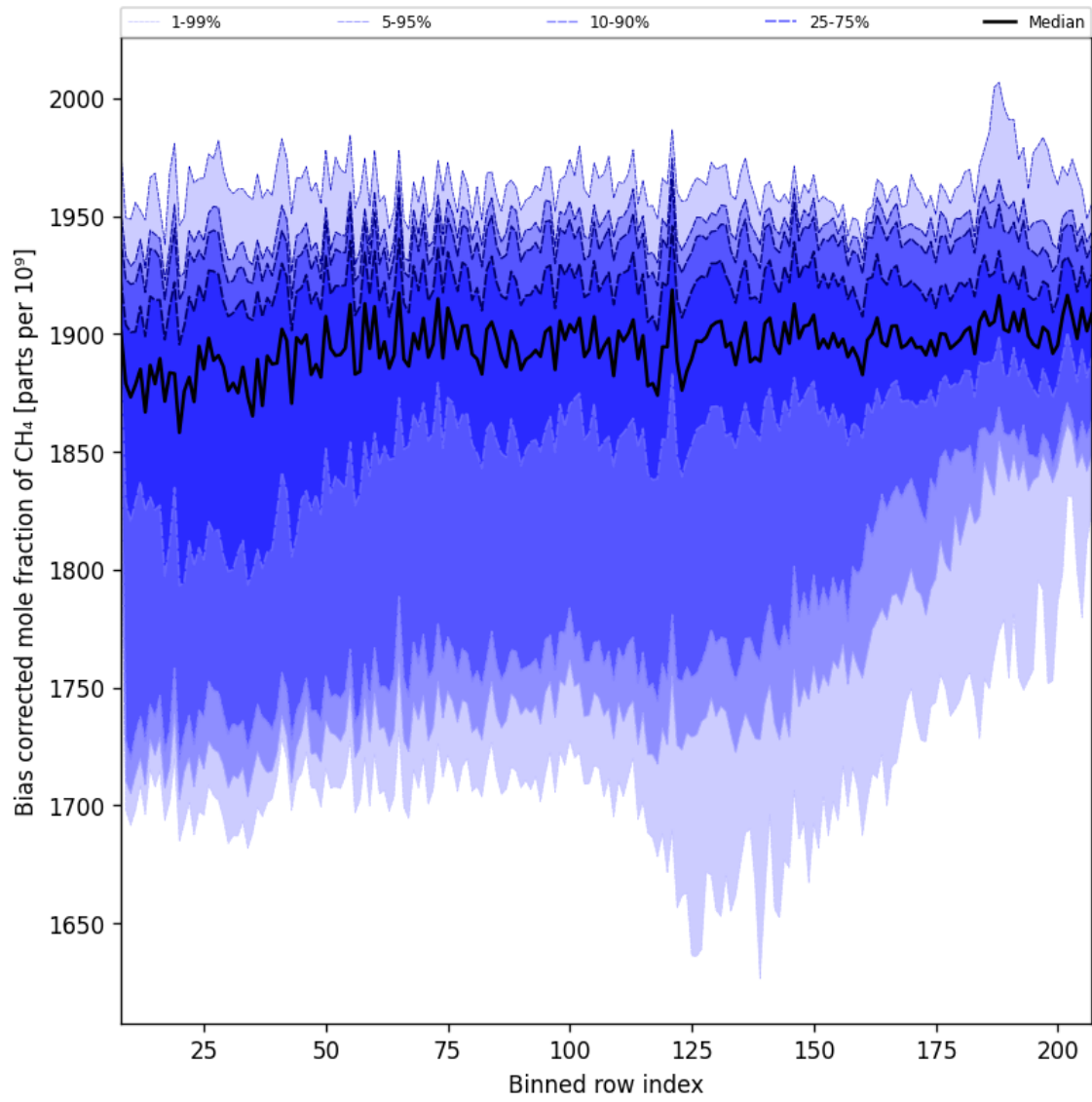
Figure 36: Along track statistics of “Bias corrected mole fraction of CH 4 ” for 2025-02-25 to 2025-02-27
