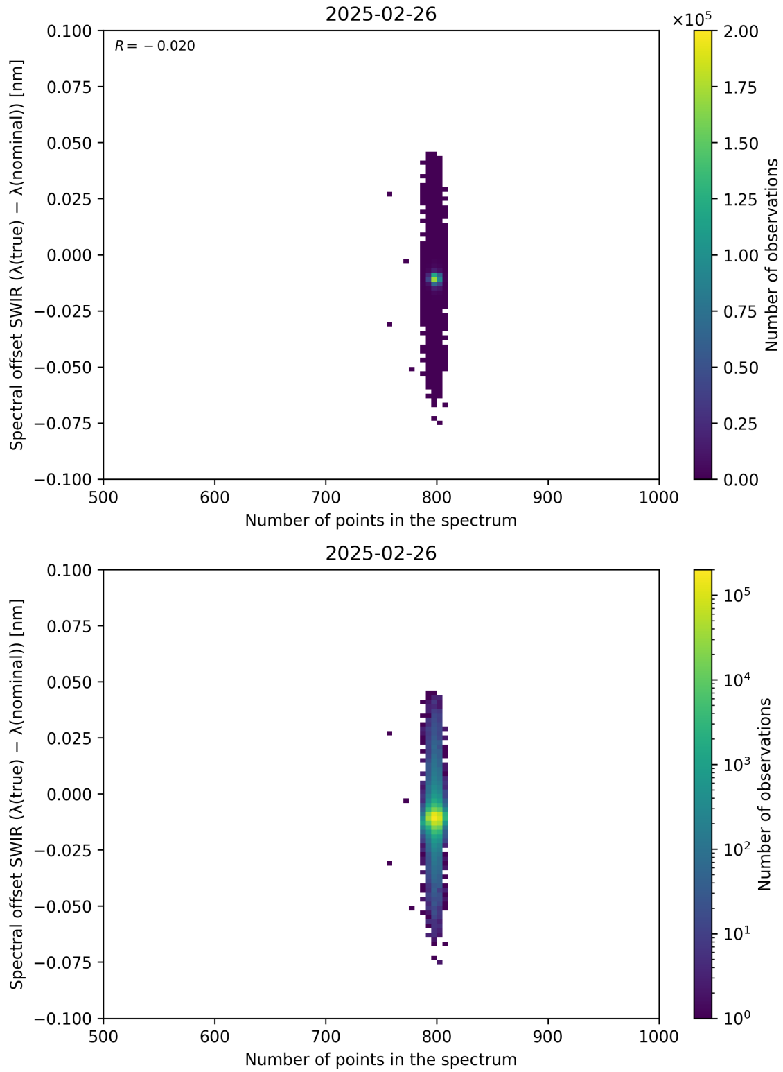
Figure 93: Scatter density plot of “Number of points in the spectrum” against “Spectral offset SWIR ( \lambda_{\text{true}} - \lambda_{\text{nominal}} )” for 2025-02-25 to 2025-02-27.
