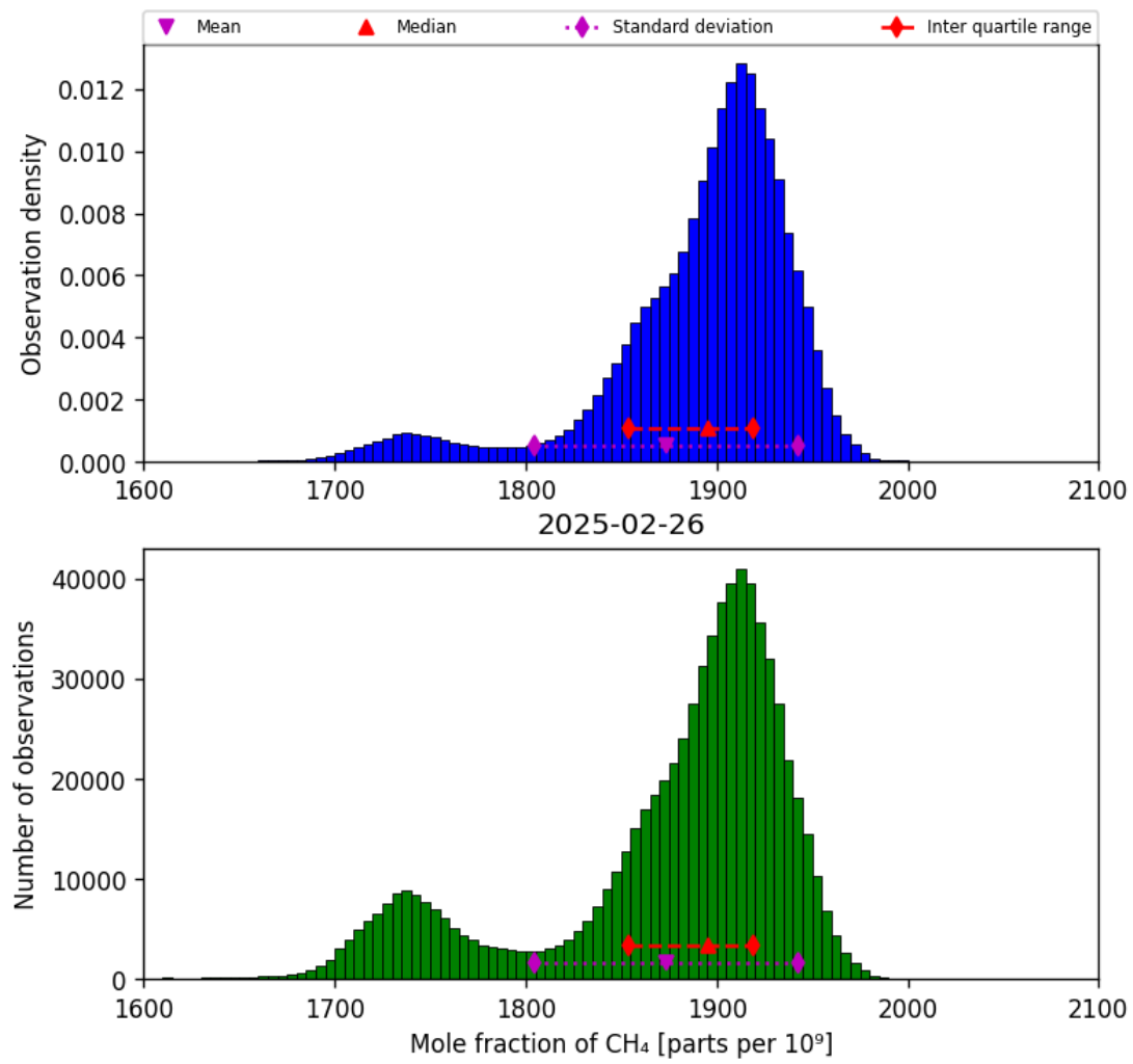
Figure 23: Histogram of “Mole fraction of CH 4 ” for 2025-02-25 to 2025-02-27
