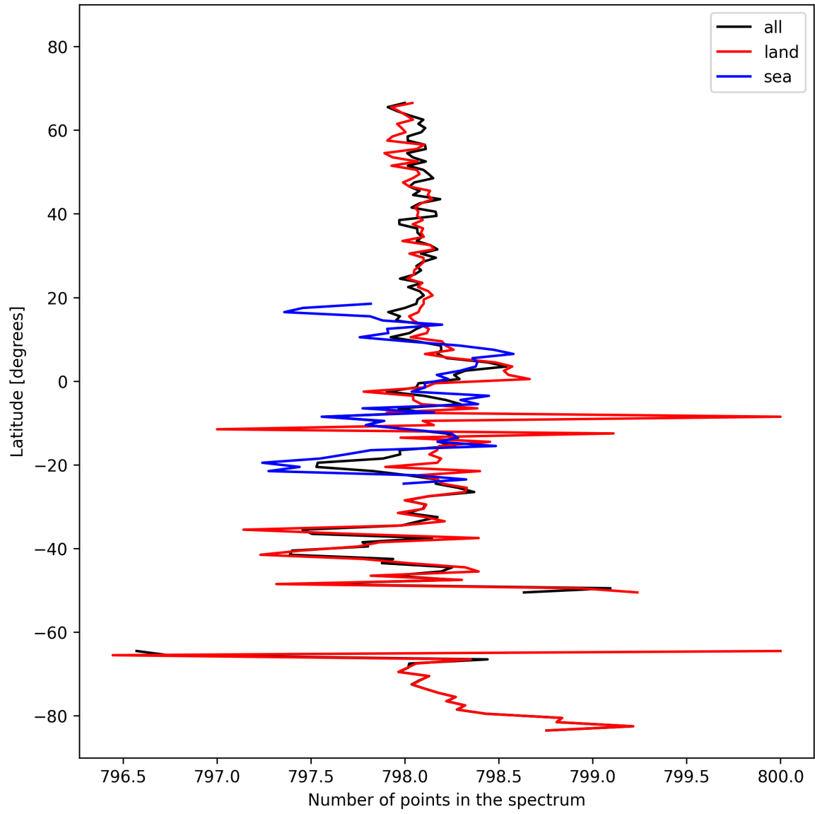
Figure 15: Zonal average of “Number of points in the spectrum” for 2025-02-25 to 2025-02-27.
