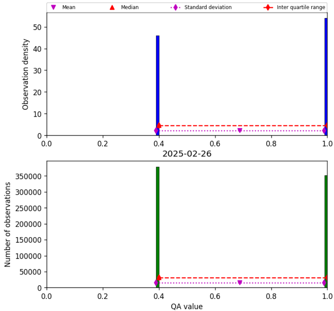
Figure 22: Histogram of “QA value” for 2025-02-25 to 2025-02-27
