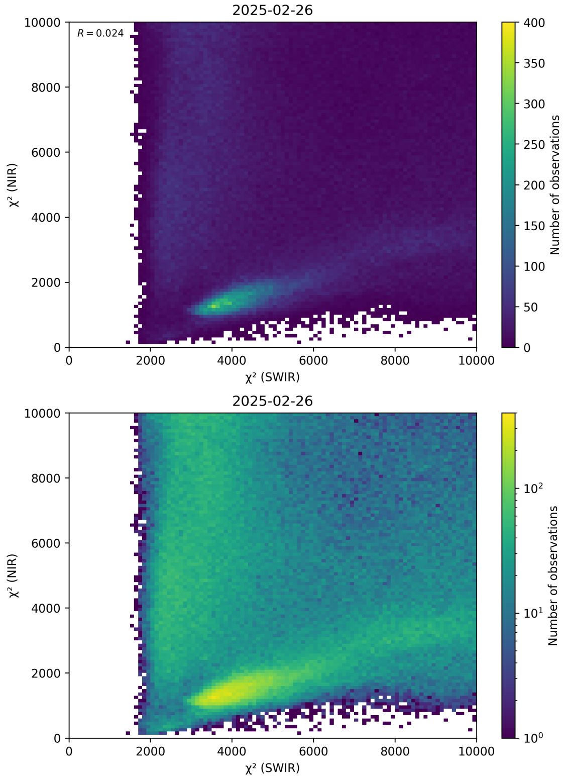
Figure 47: Scatter density plot of “ \chi^2 (SWIR)” against “ \chi^2 (NIR)” for 2025-02-25 to 2025-02-27.
