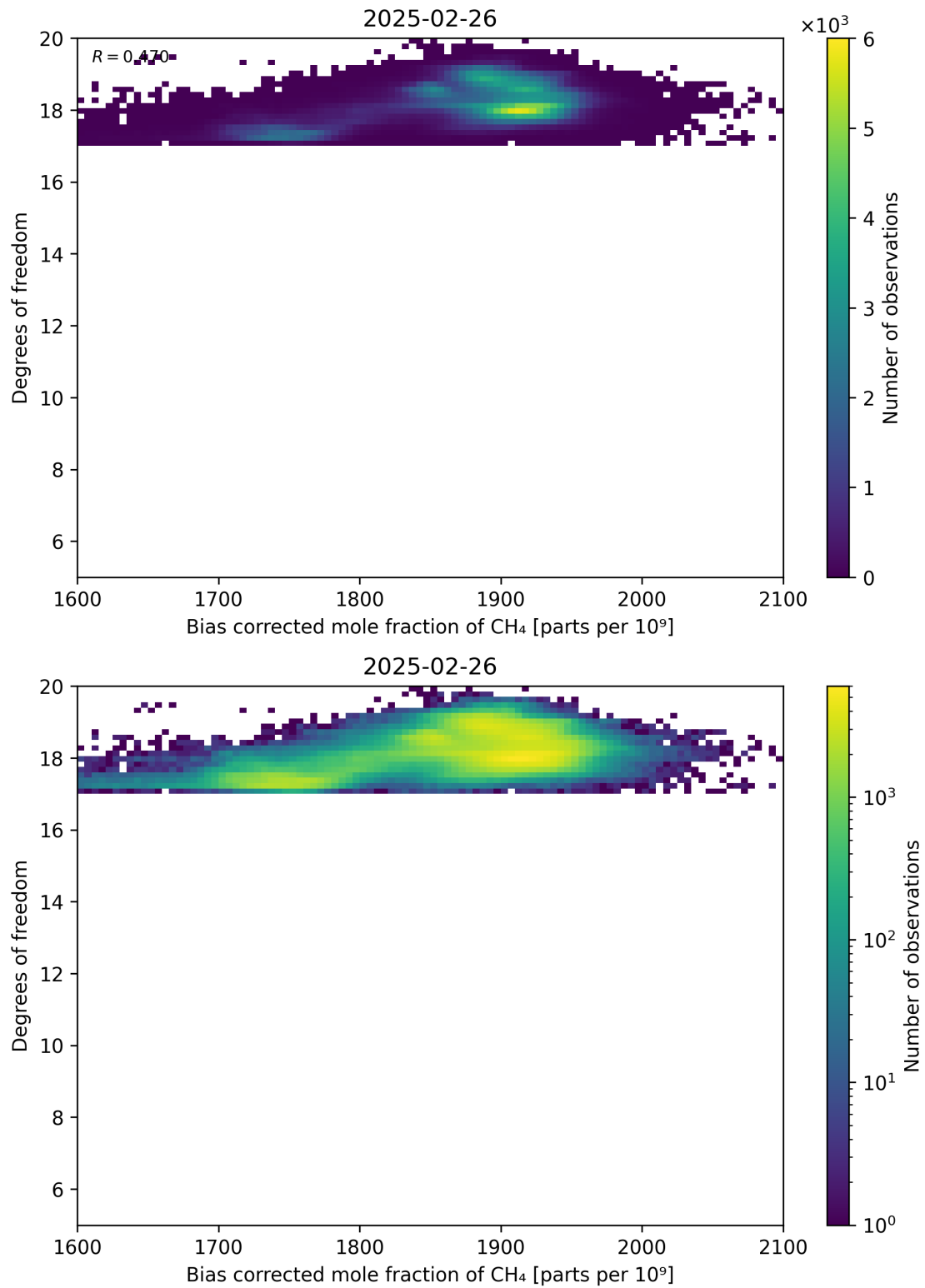
Figure 65: Scatter density plot of “Bias corrected mole fraction of CH 4 ” against “Degrees of freedom” for 2025-02-25 to 2025-02-27.
