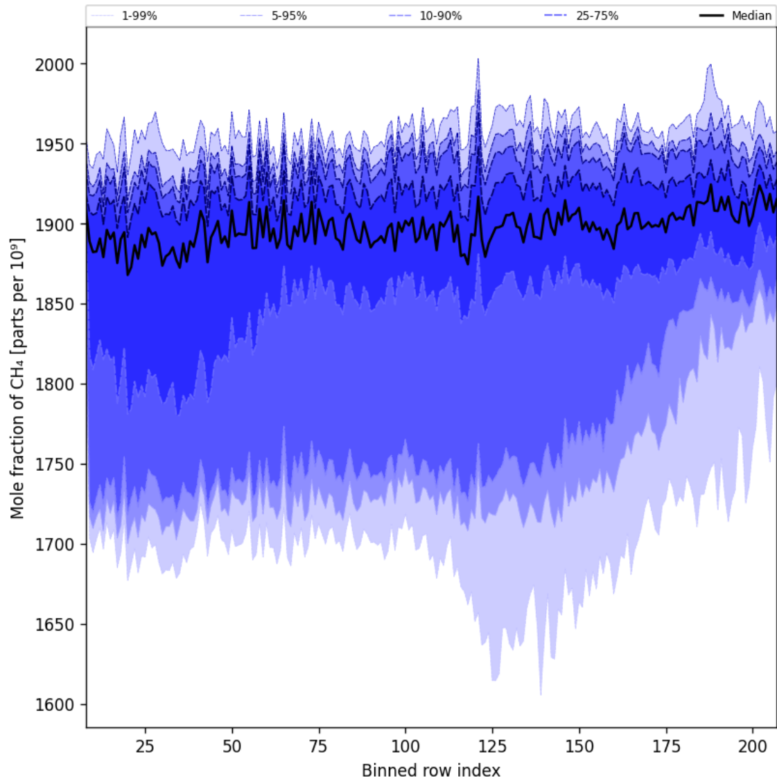
Figure 34: Along track statistics of “Mole fraction of CH 4 ” for 2025-02-25 to 2025-02-27
