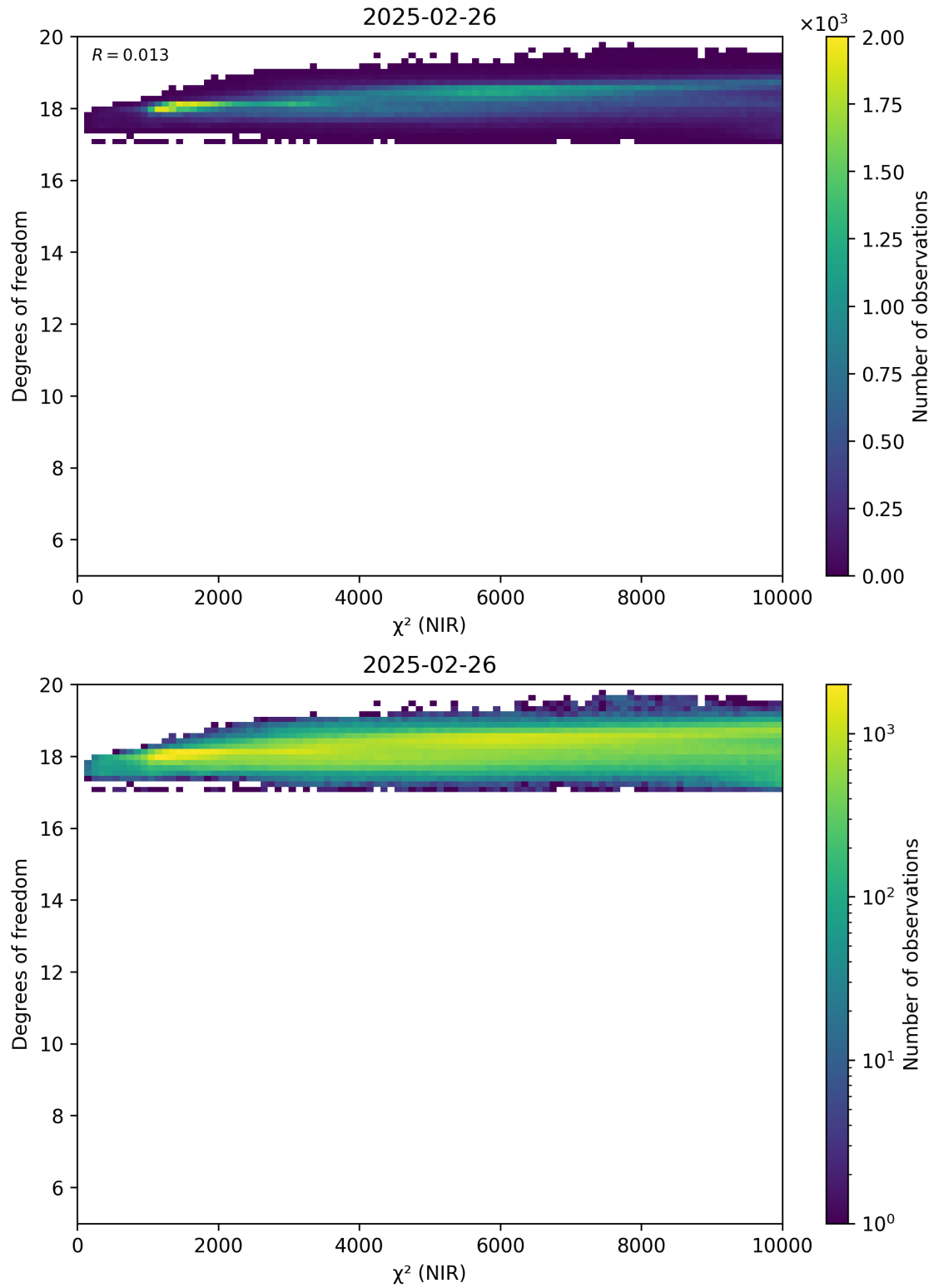
Figure 44: Scatter density plot of “ \chi^2 (NIR)” against “Degrees of freedom” for 2025-02-25 to 2025-02-27.
