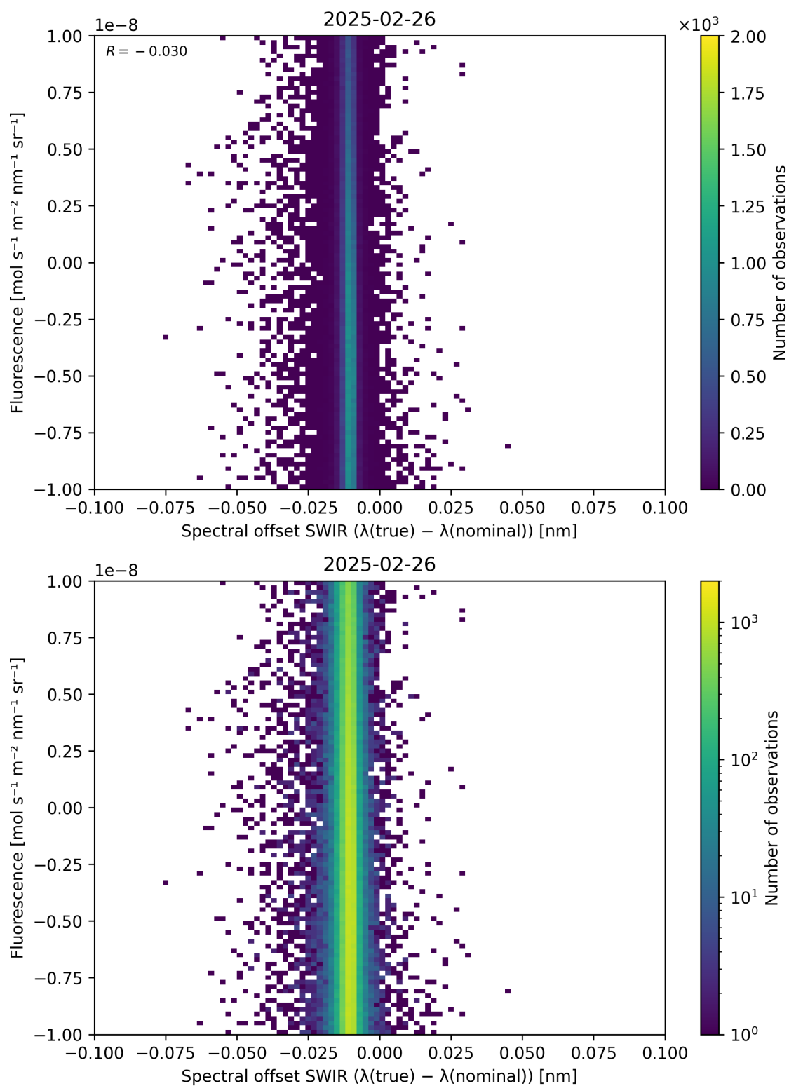
Figure 120: Scatter density plot of “Spectral offset SWIR ( \lambda_{\text{true}} - \lambda_{\text{nominal}} )” against “Fluorescence” for 2025-02-25 to 2025-02-27.
