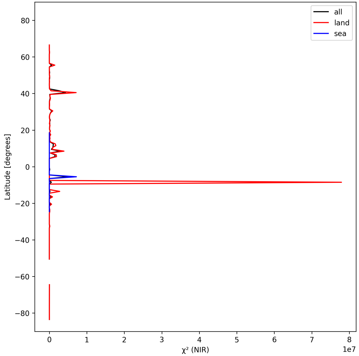
Figure 18: Zonal average of “ \chi^2 (NIR)” for 2025-02-25 to 2025-02-27.
