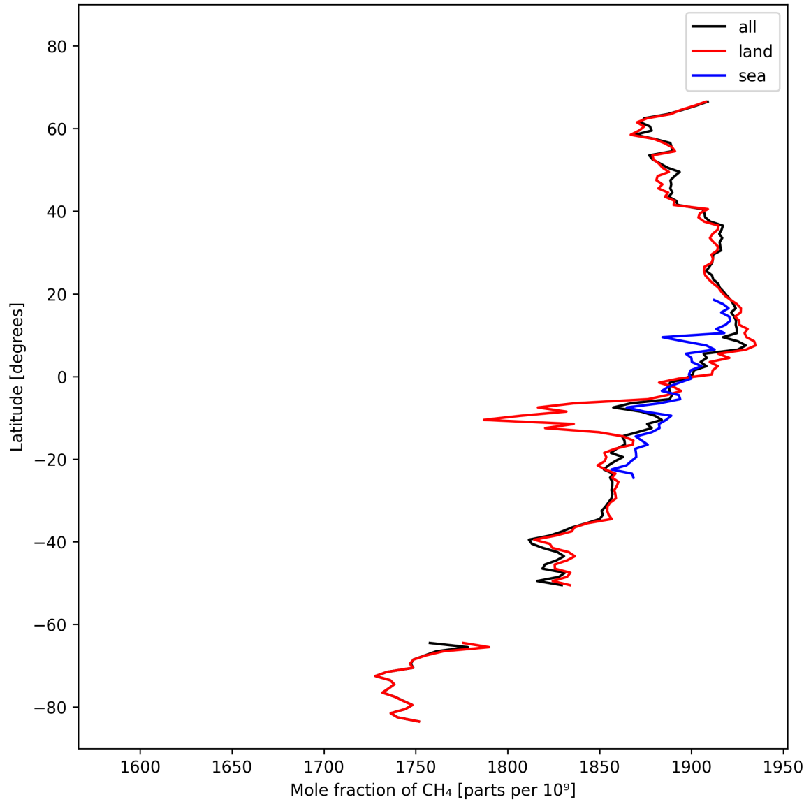
Figure 12: Zonal average of “Mole fraction of \text{CH}_4 ” for 2025-02-25 to 2025-02-27.
