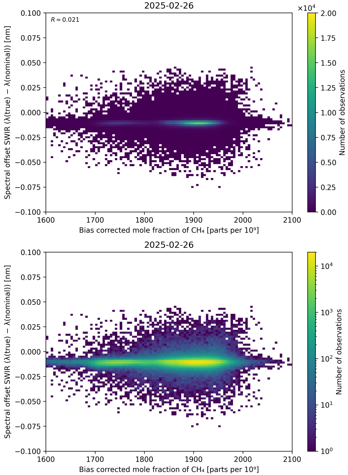
Figure 69: Scatter density plot of “Bias corrected mole fraction of \text{CH}_4 ” against “Spectral offset SWIR ( \lambda_{\text{true}} - \lambda_{\text{nominal}} )” for 2025-02-25 to 2025-02-27.
