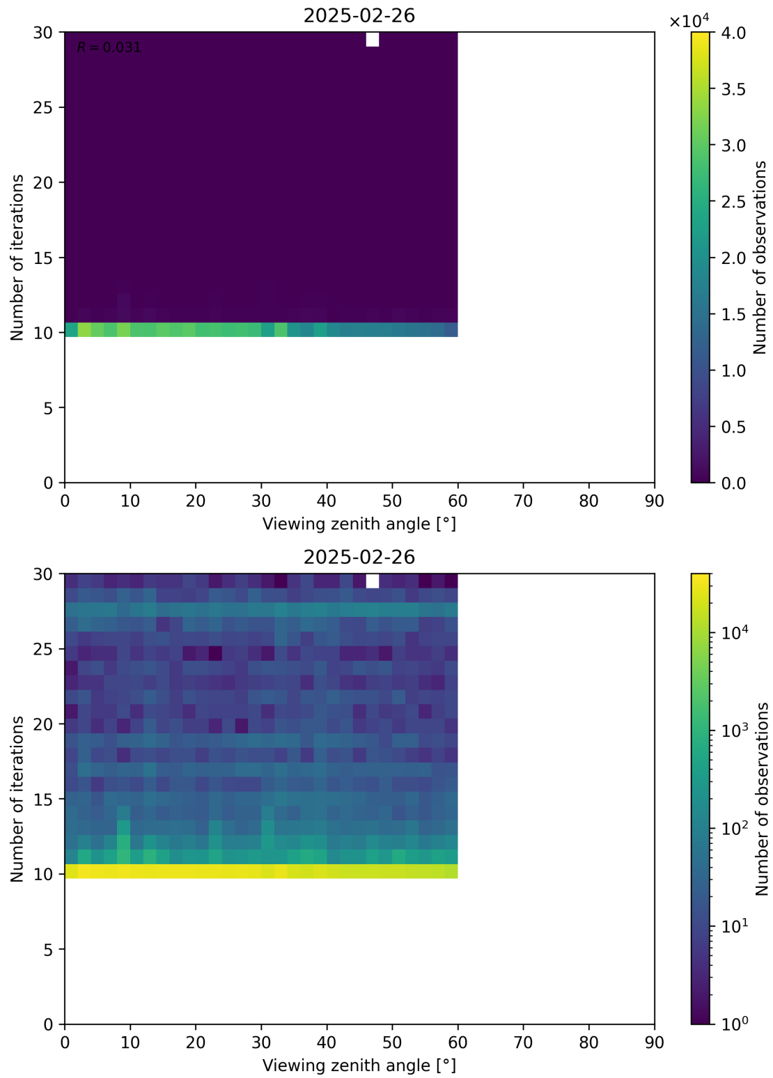
Figure 113: Scatter density plot of “Viewing zenith angle” against “Number of iterations” for 2025-02-25 to 2025-02-27.
