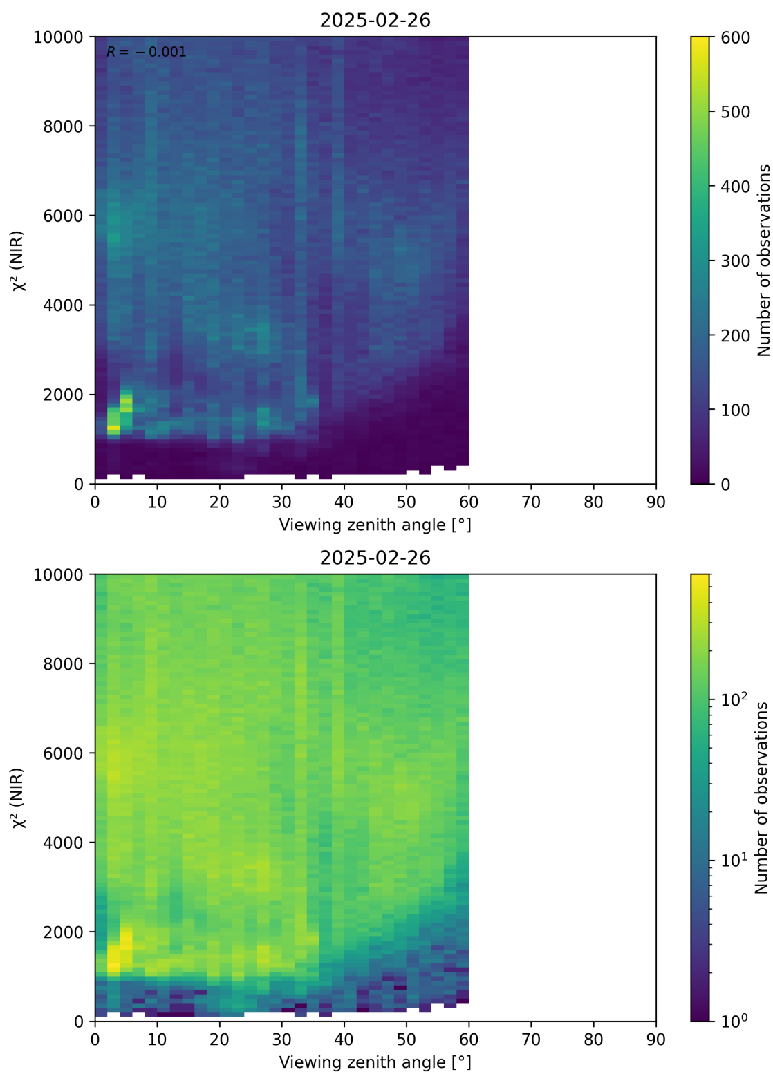
Figure 105: Scatter density plot of “Viewing zenith angle” against “ \chi^2 (NIR)” for 2025-02-25 to 2025-02-27.
