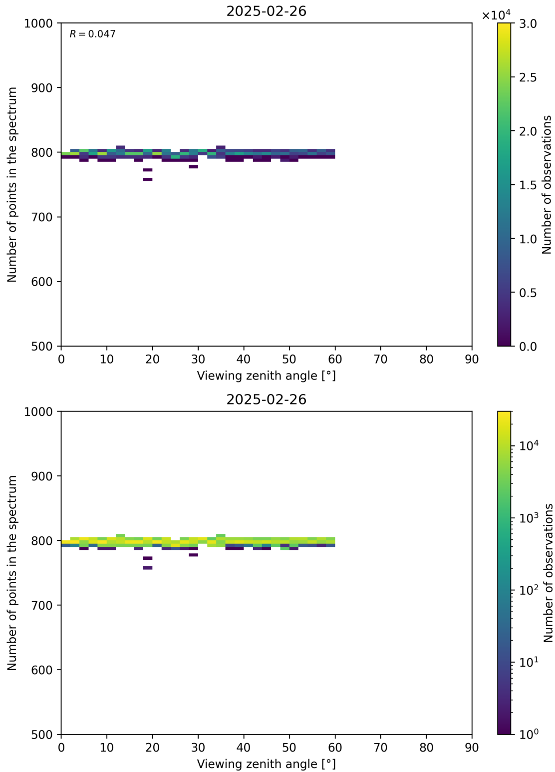
Figure 114: Scatter density plot of “Viewing zenith angle” against “Number of points in the spectrum” for 2025-02-25 to 2025-02-27.
