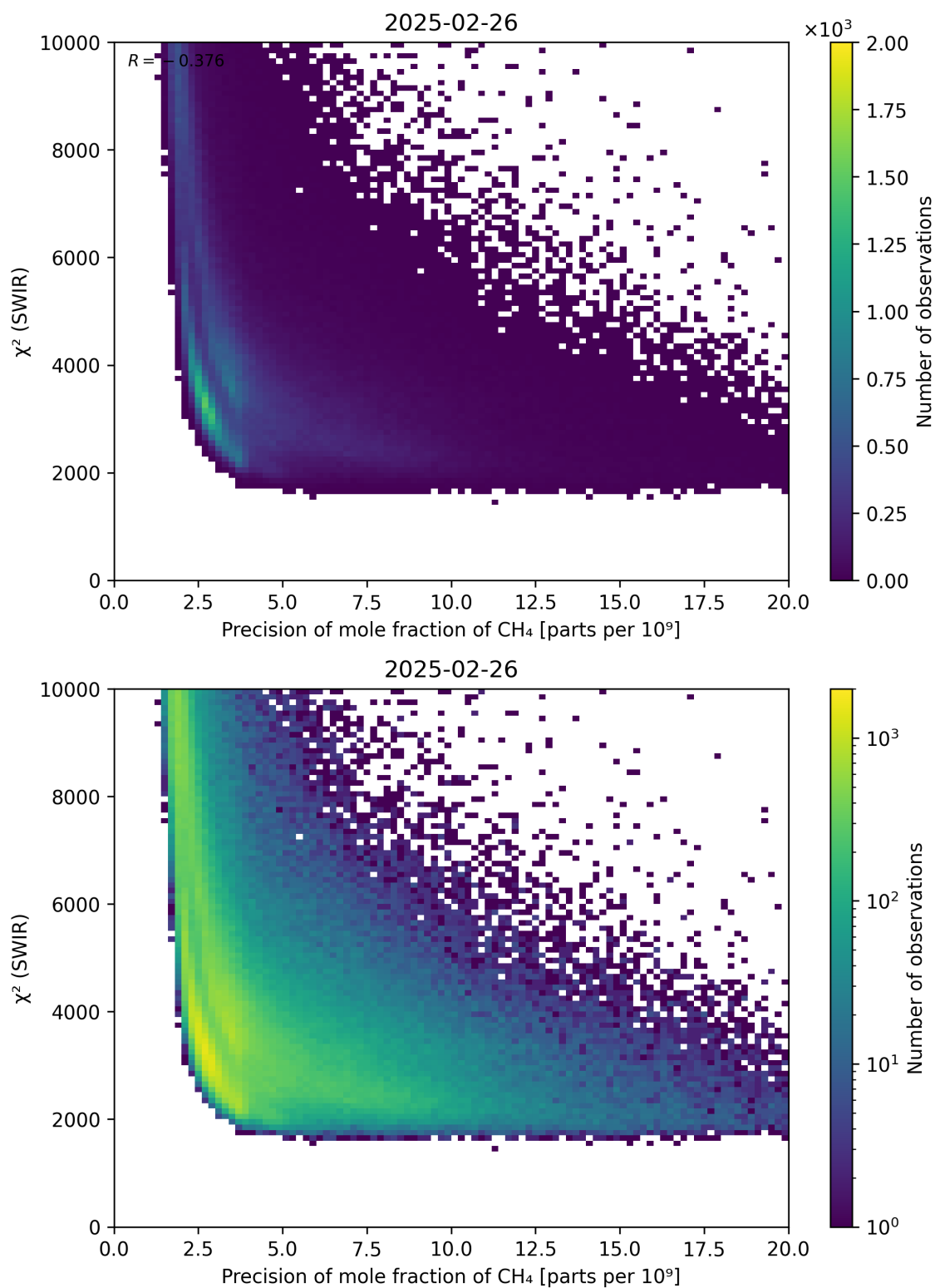
Figure 79: Scatter density plot of “Precision of mole fraction of \text{CH}_4 ” against “ \chi^2 (SWIR)” for 2025-02-25 to 2025-02-27.
