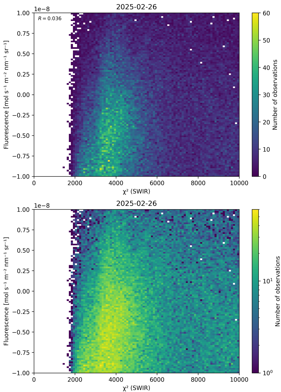
Figure 49: Scatter density plot of “ \chi^2 (SWIR)” against “Fluorescence” for 2025-02-25 to 2025-02-27.
