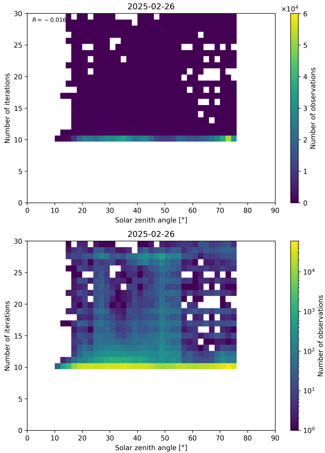
Figure 102: Scatter density plot of “Solar zenith angle” against “Number of iterations” for 2025-02-25 to 2025-02-27.
