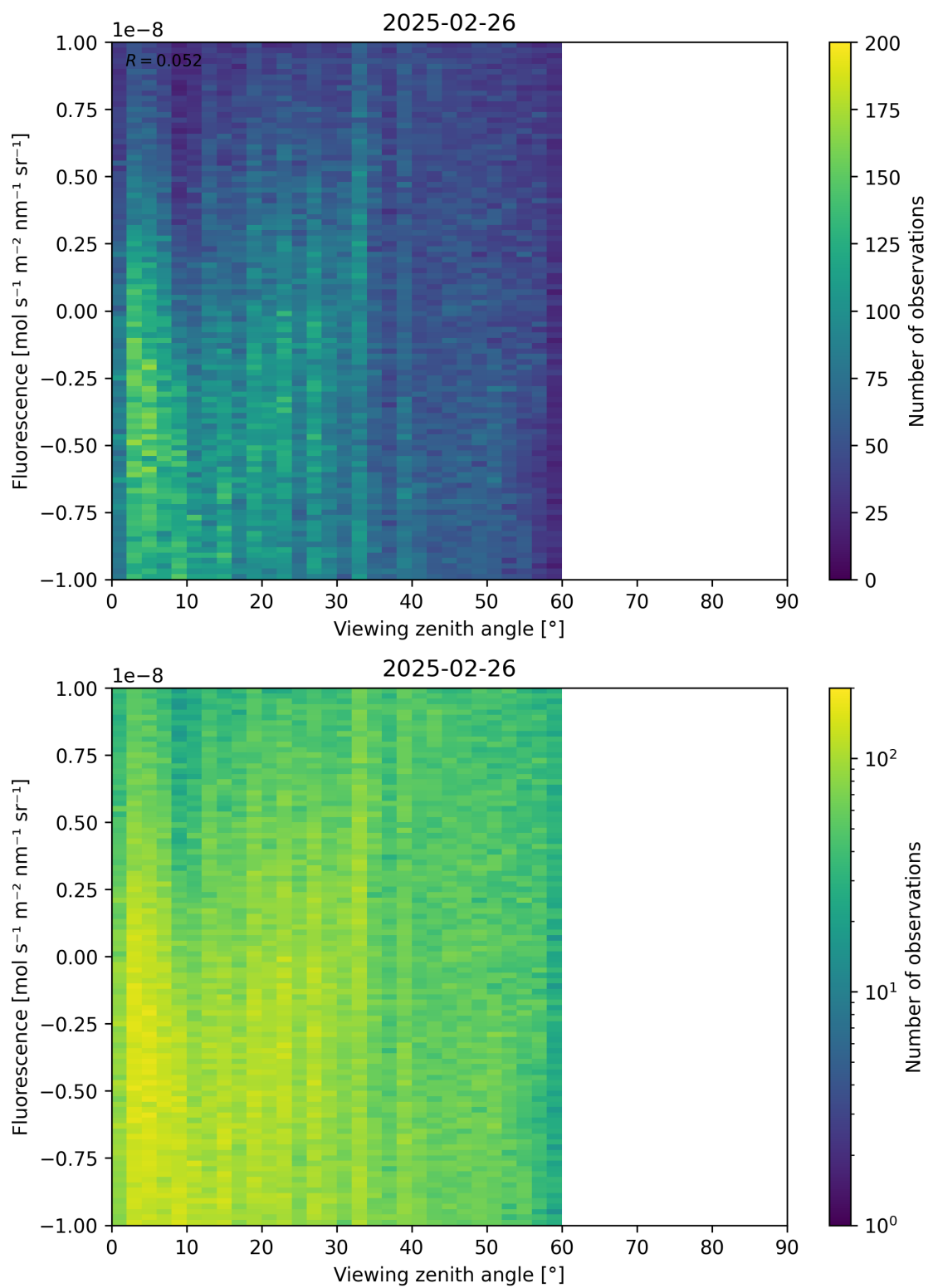
Figure 108: Scatter density plot of “Viewing zenith angle” against “Fluorescence” for 2025-02-25 to 2025-02-27.
