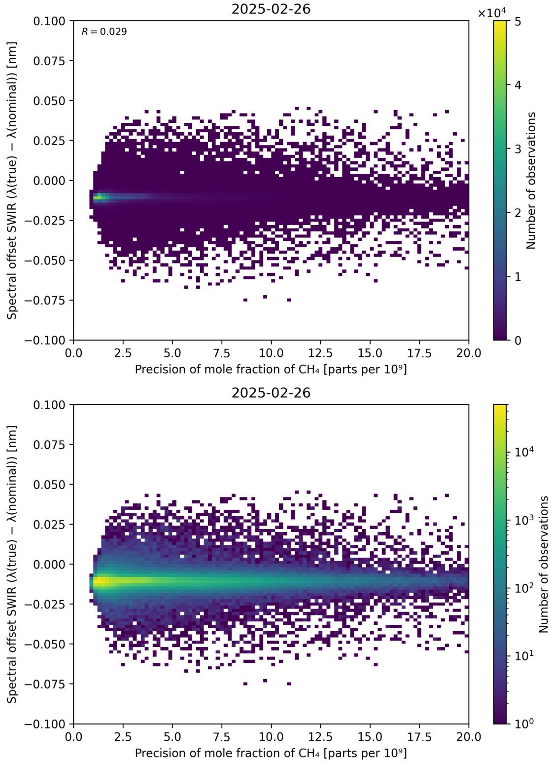
Figure 85: Scatter density plot of “Precision of mole fraction of CH 4 ” against “Spectral offset SWIR ( \lambda_{\text{true}} - \lambda_{\text{nominal}} )” for 2025-02-25 to 2025-02-27.
