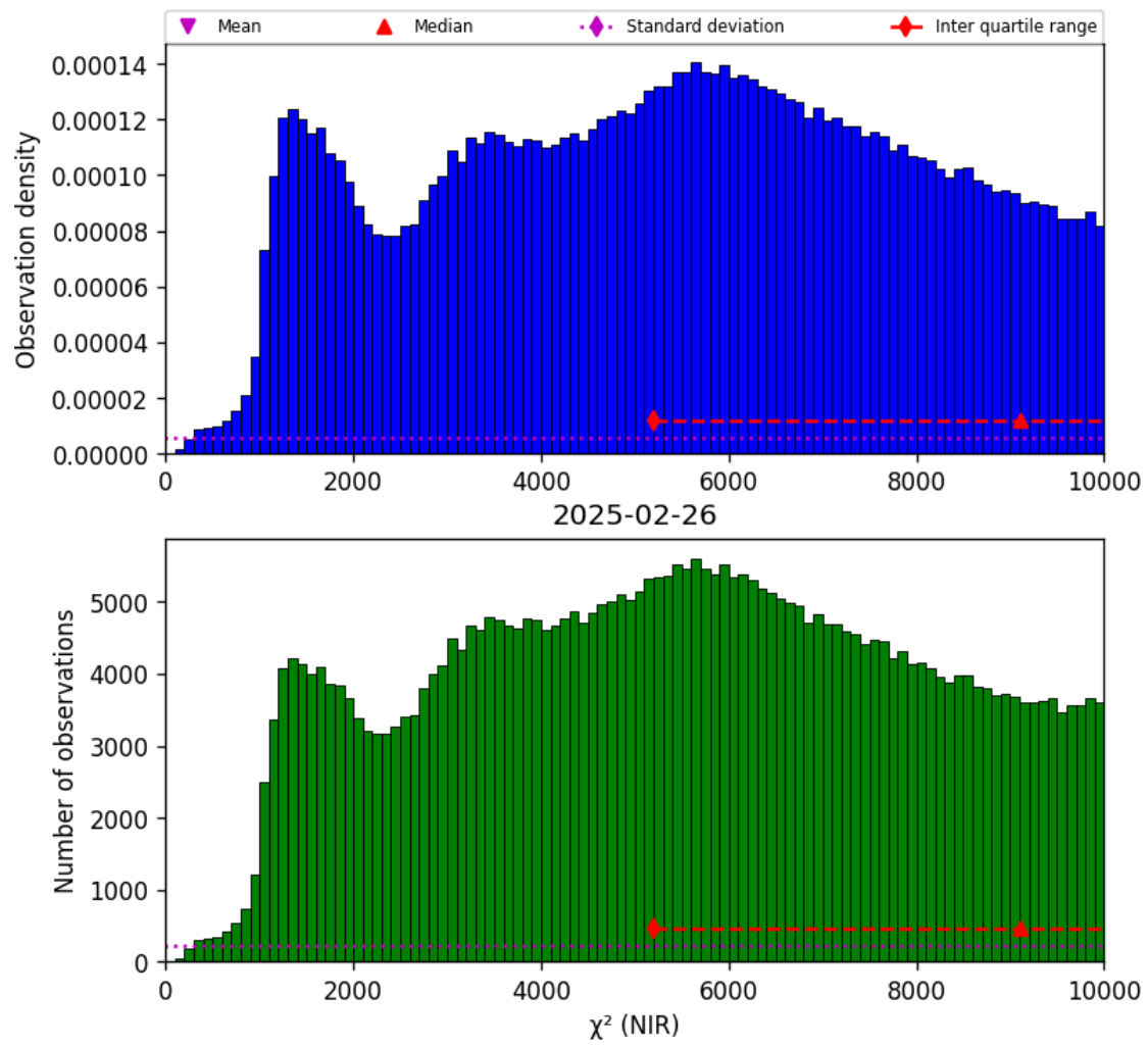
Figure 29: Histogram of “ \chi^2 (NIR)” for 2025-02-25 to 2025-02-27
