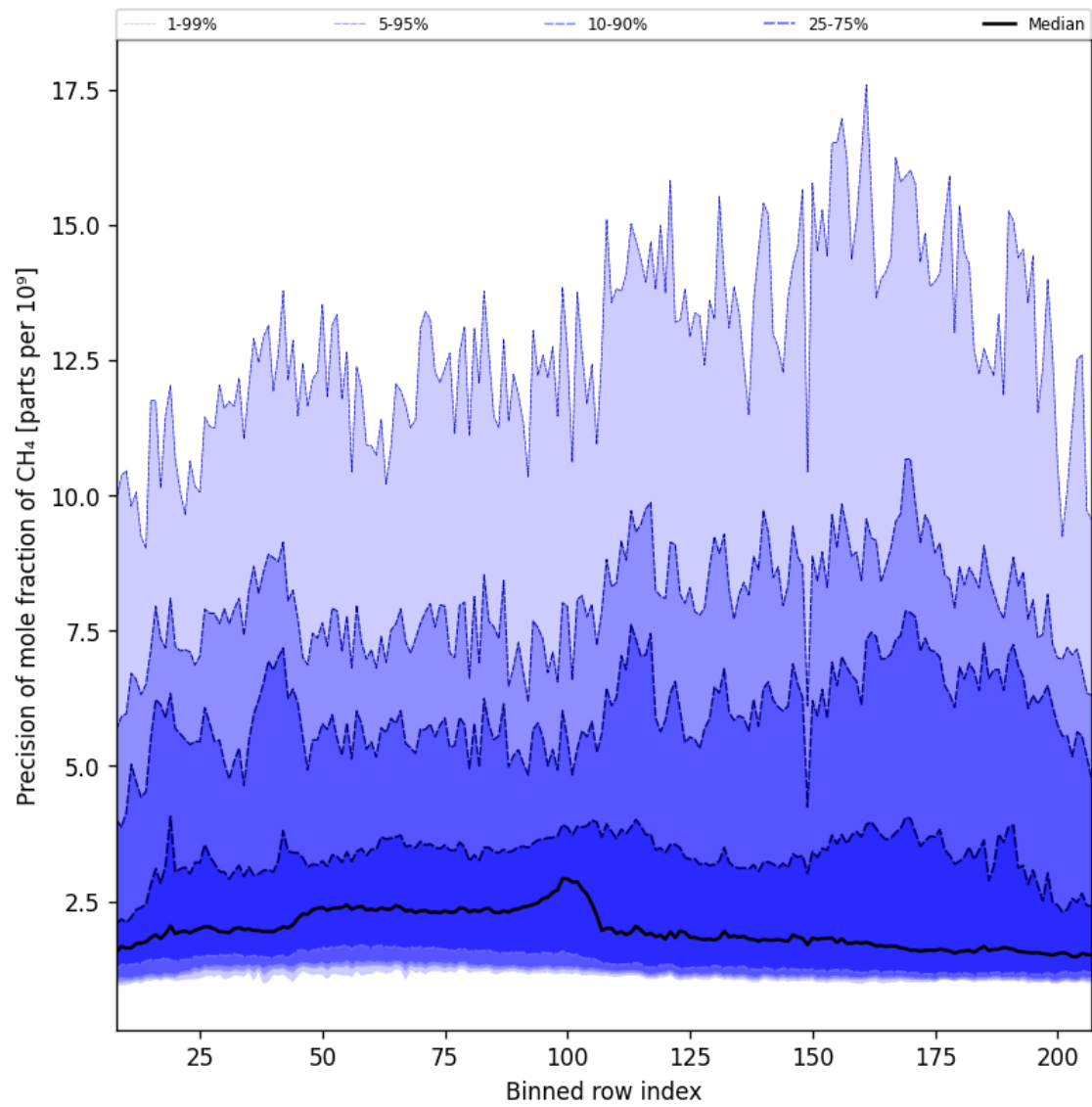
Figure 35: Along track statistics of “Precision of mole fraction of CH 4 ” for 2025-02-25 to 2025-02-27
