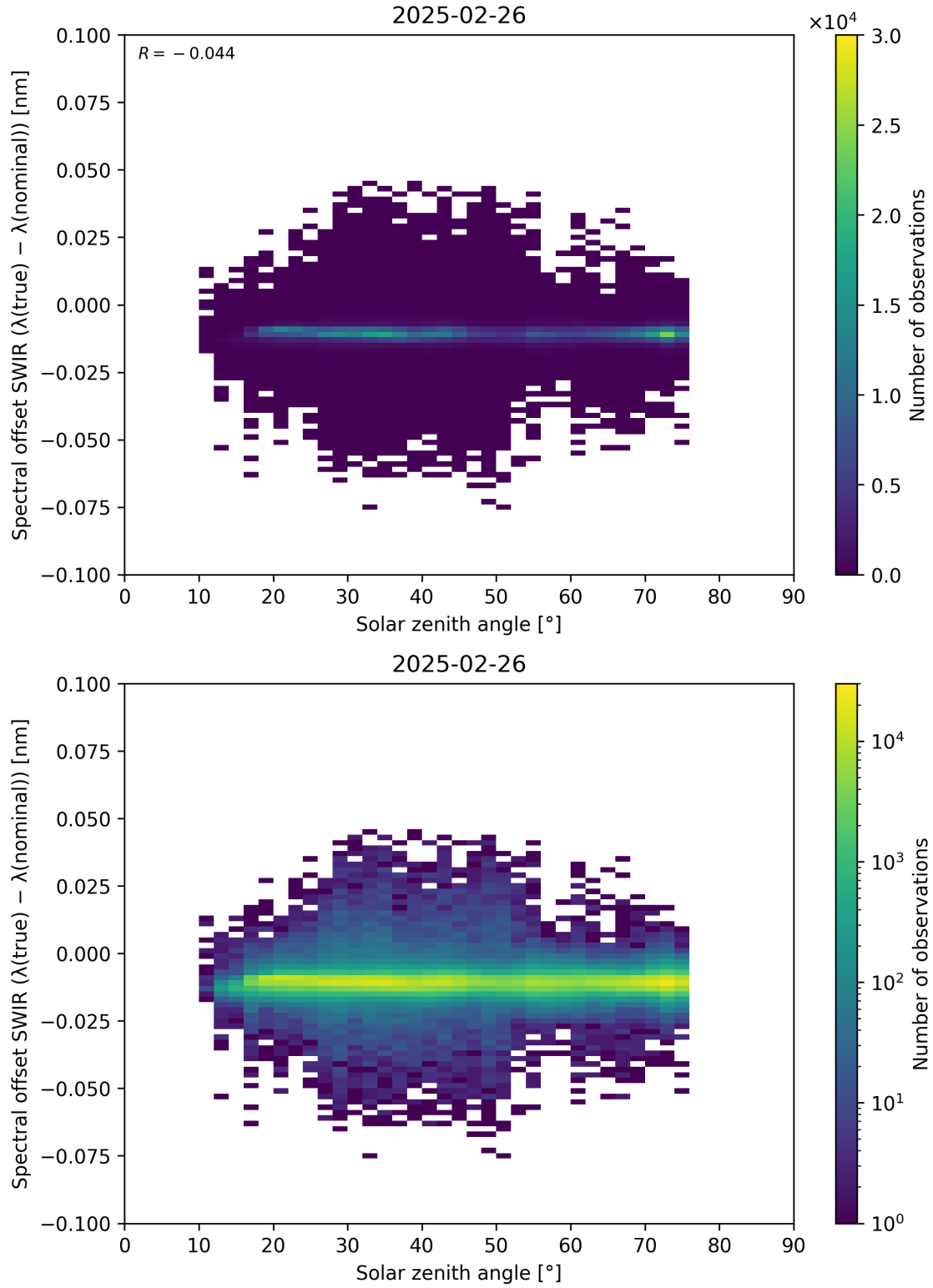
Figure 104: Scatter density plot of “Solar zenith angle” against “Spectral offset SWIR ( \lambda_{\text{true}} - \lambda_{\text{nominal}} )” for 2025-02-25 to 2025-02-27.
