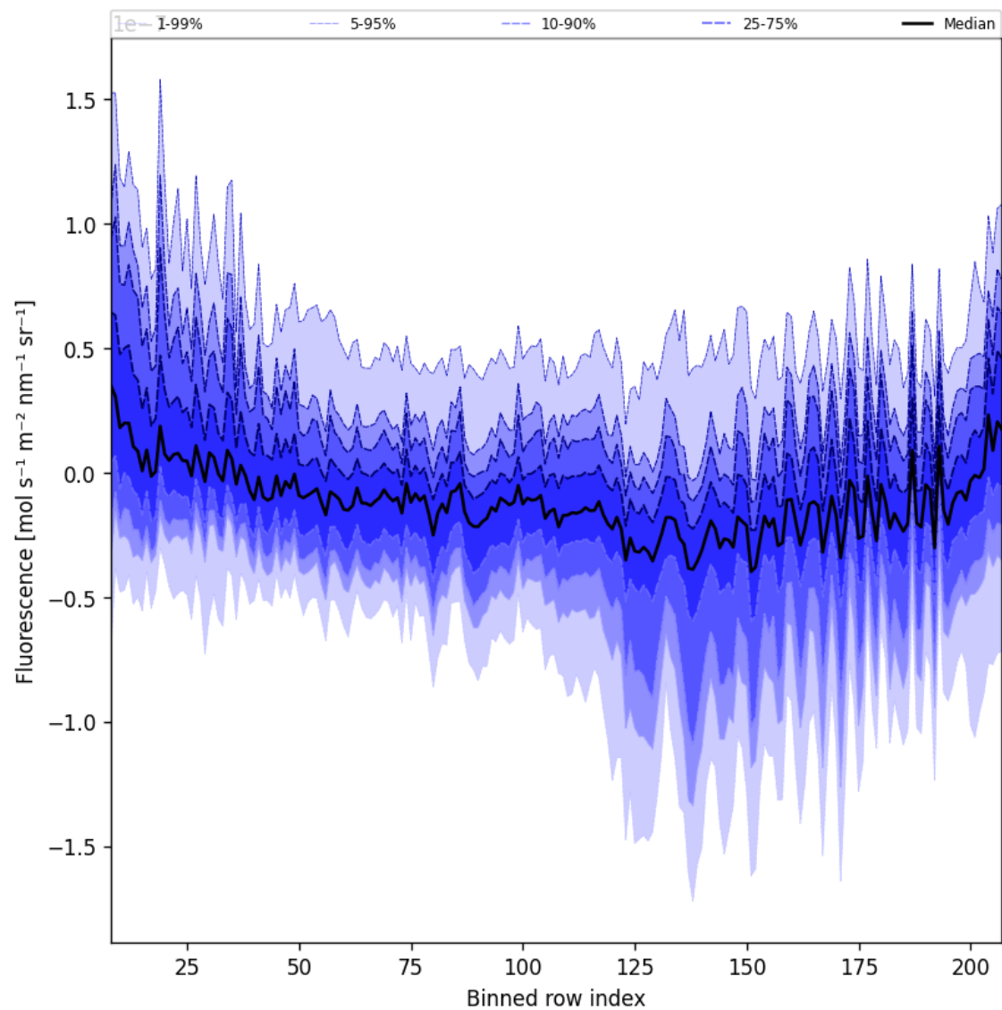
Figure 43: Along track statistics of “Fluorescence” for 2025-02-25 to 2025-02-27
