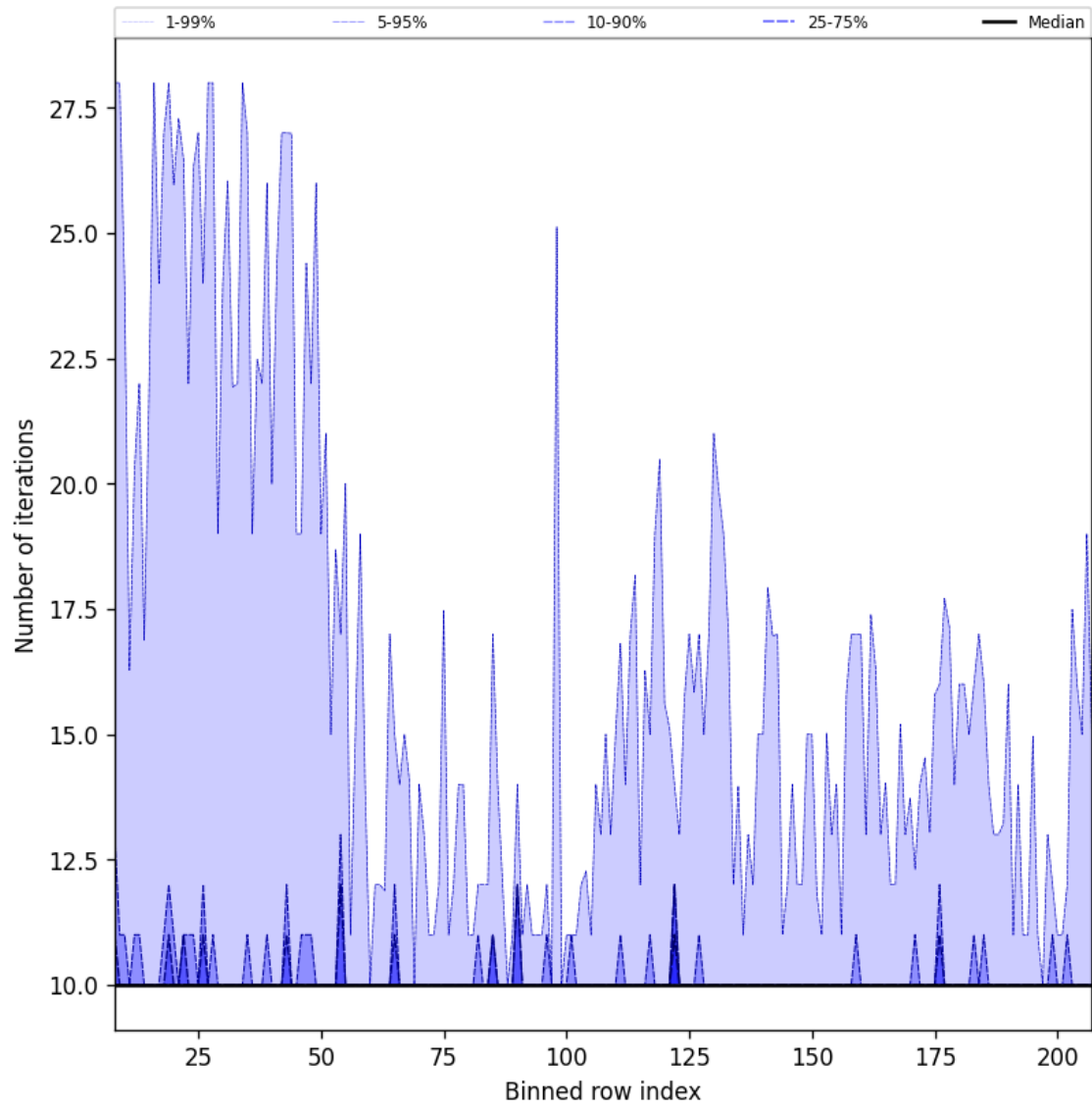
Figure 42: Along track statistics of “Number of iterations” for 2025-02-25 to 2025-02-27
