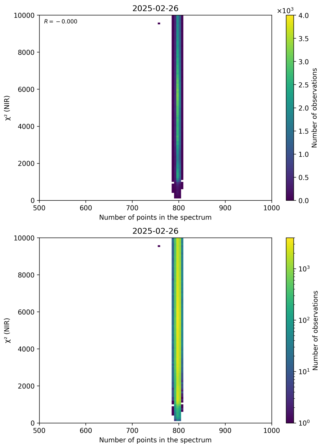
Figure 88: Scatter density plot of “Number of points in the spectrum” against “ \chi^2 (NIR)” for 2025-02-25 to 2025-02-27.
