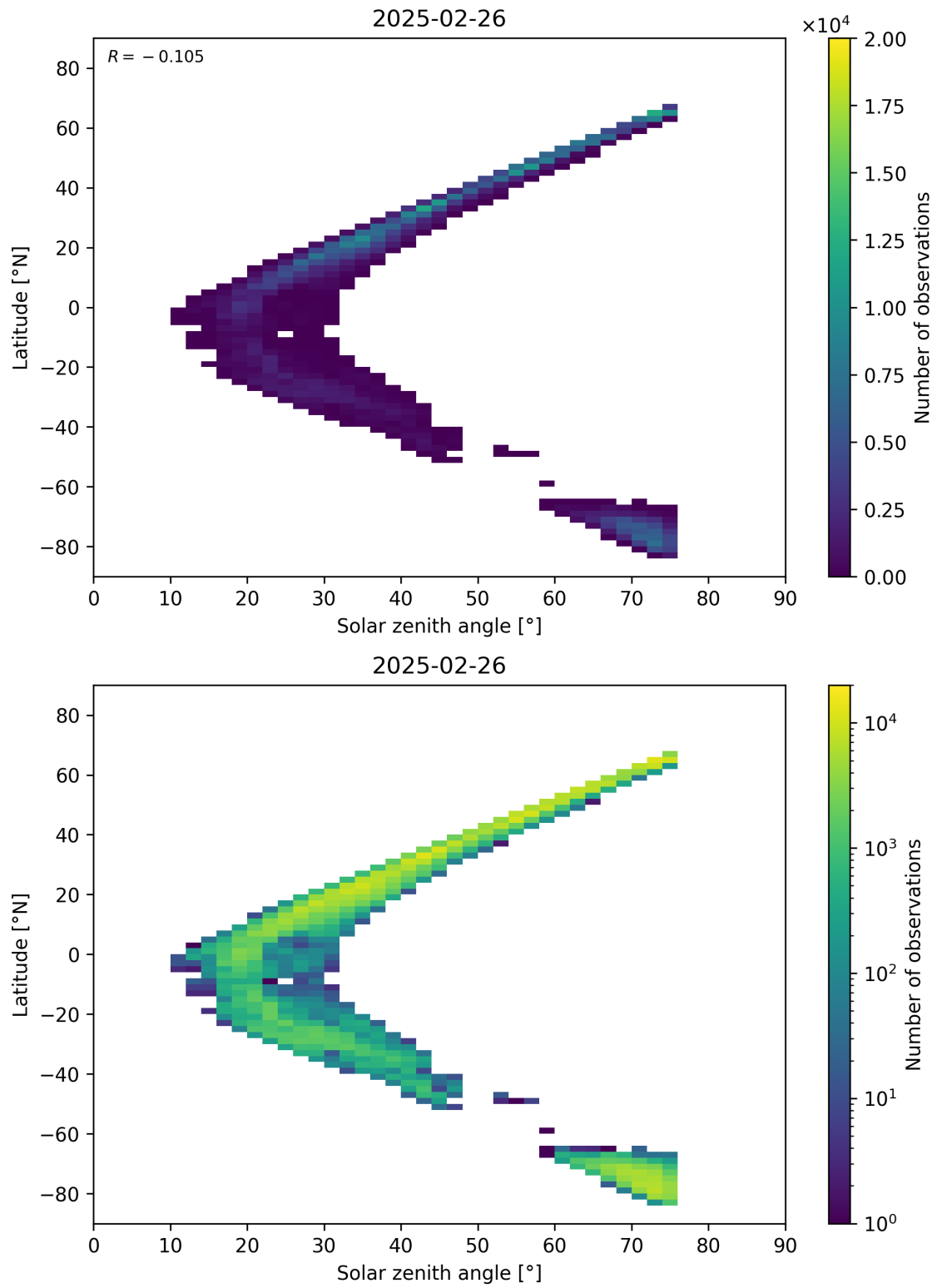
Figure 98: Scatter density plot of “Solar zenith angle” against “Latitude” for 2025-02-25 to 2025-02-27.
