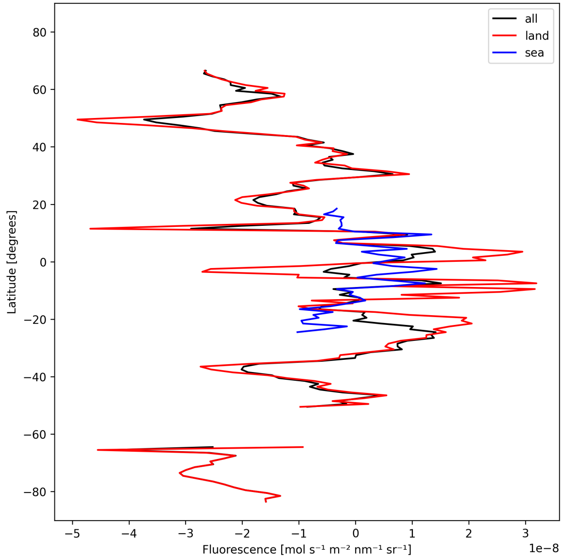
Figure 21: Zonal average of “Fluorescence” for 2025-02-25 to 2025-02-27.
