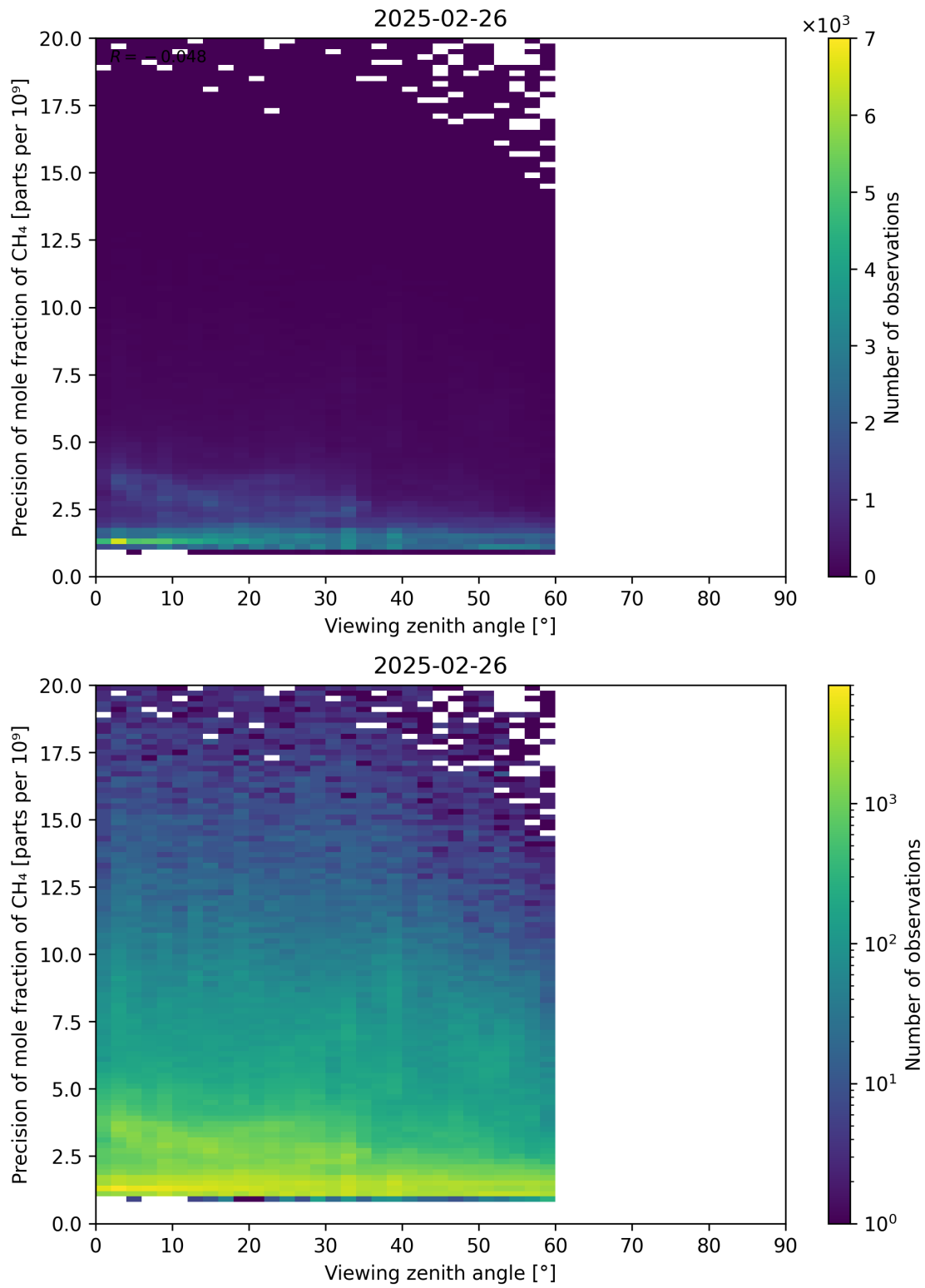
Figure 112: Scatter density plot of “Viewing zenith angle” against “Precision of mole fraction of CH 4 ” for 2025-02-25 to 2025-02-27.
