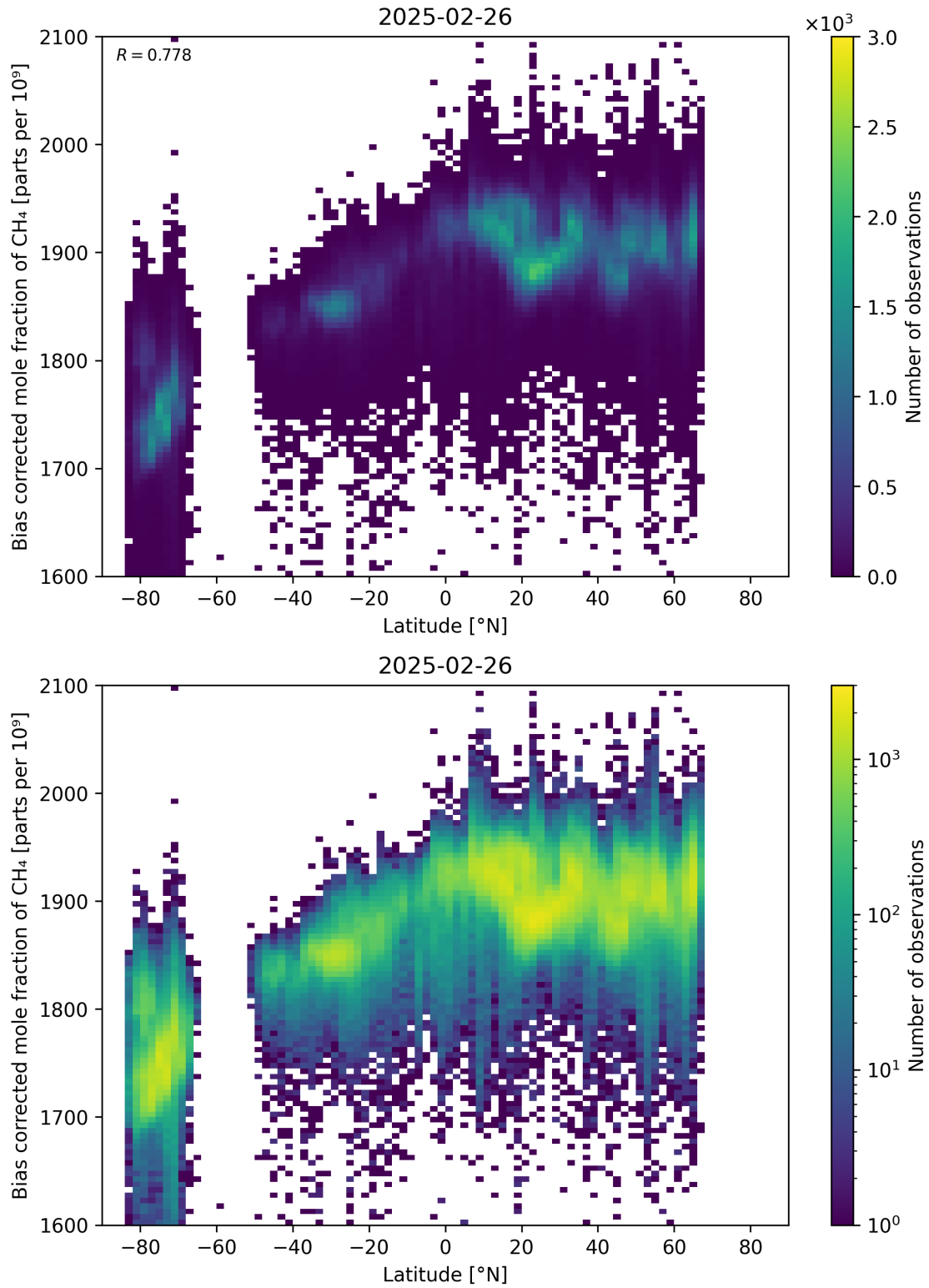
Figure 58: Scatter density plot of “Latitude” against “Bias corrected mole fraction of CH 4 ” for 2025-02-25 to 2025-02-27.
