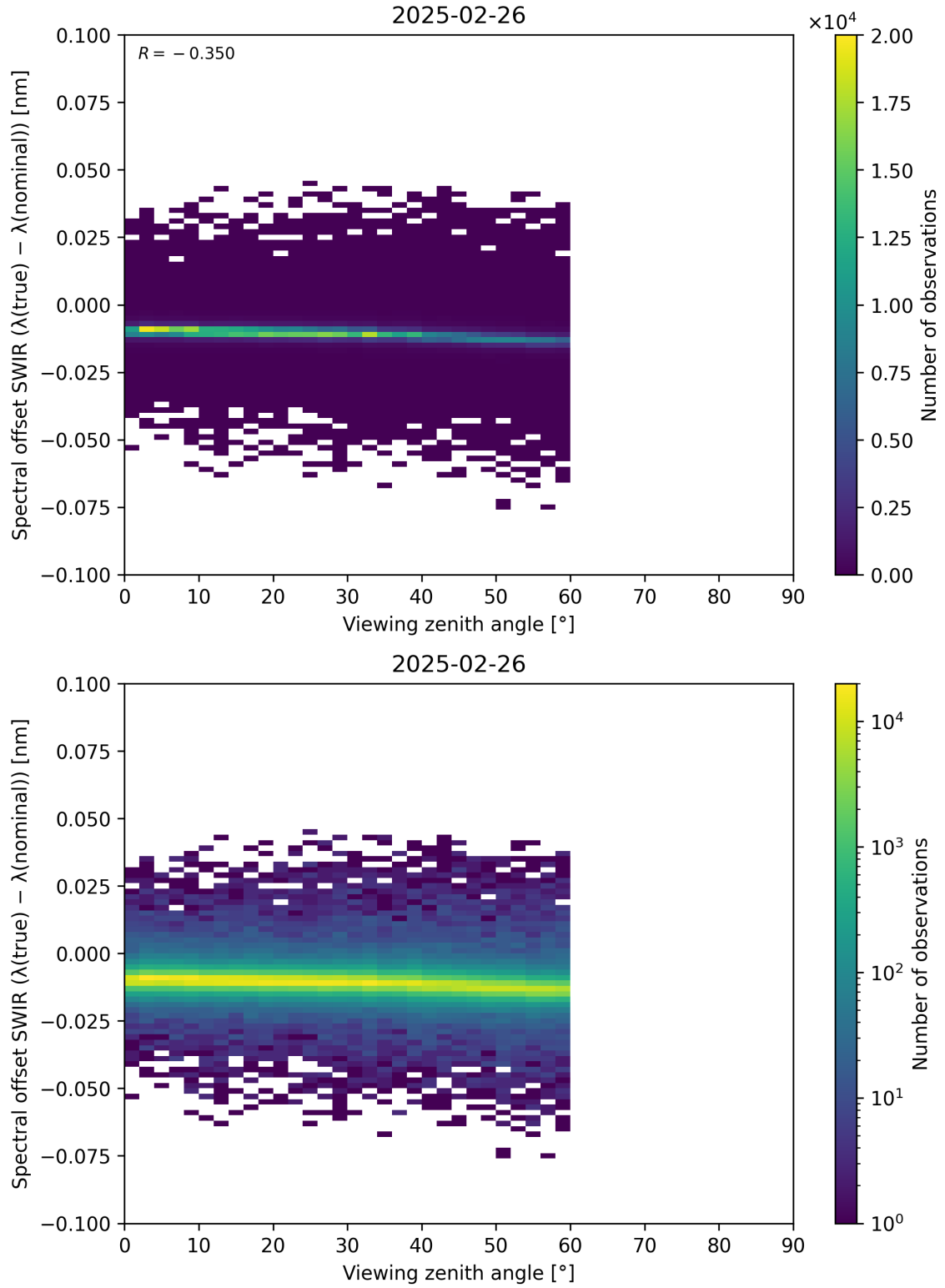
Figure 116: Scatter density plot of “Viewing zenith angle” against “Spectral offset SWIR ( \lambda_{\text{true}} - \lambda_{\text{nominal}} )” for 2025-02-25 to 2025-02-27.
