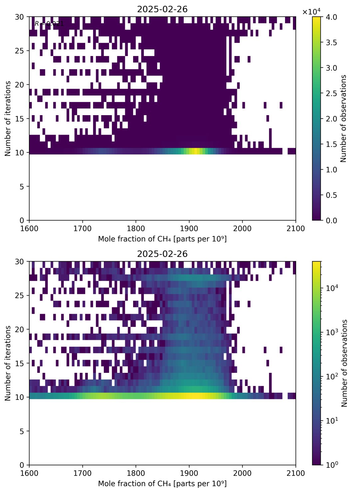
Figure 76: Scatter density plot of “Mole fraction of CH 4 ” against “Number of iterations” for 2025-02-25 to 2025-02-27.
