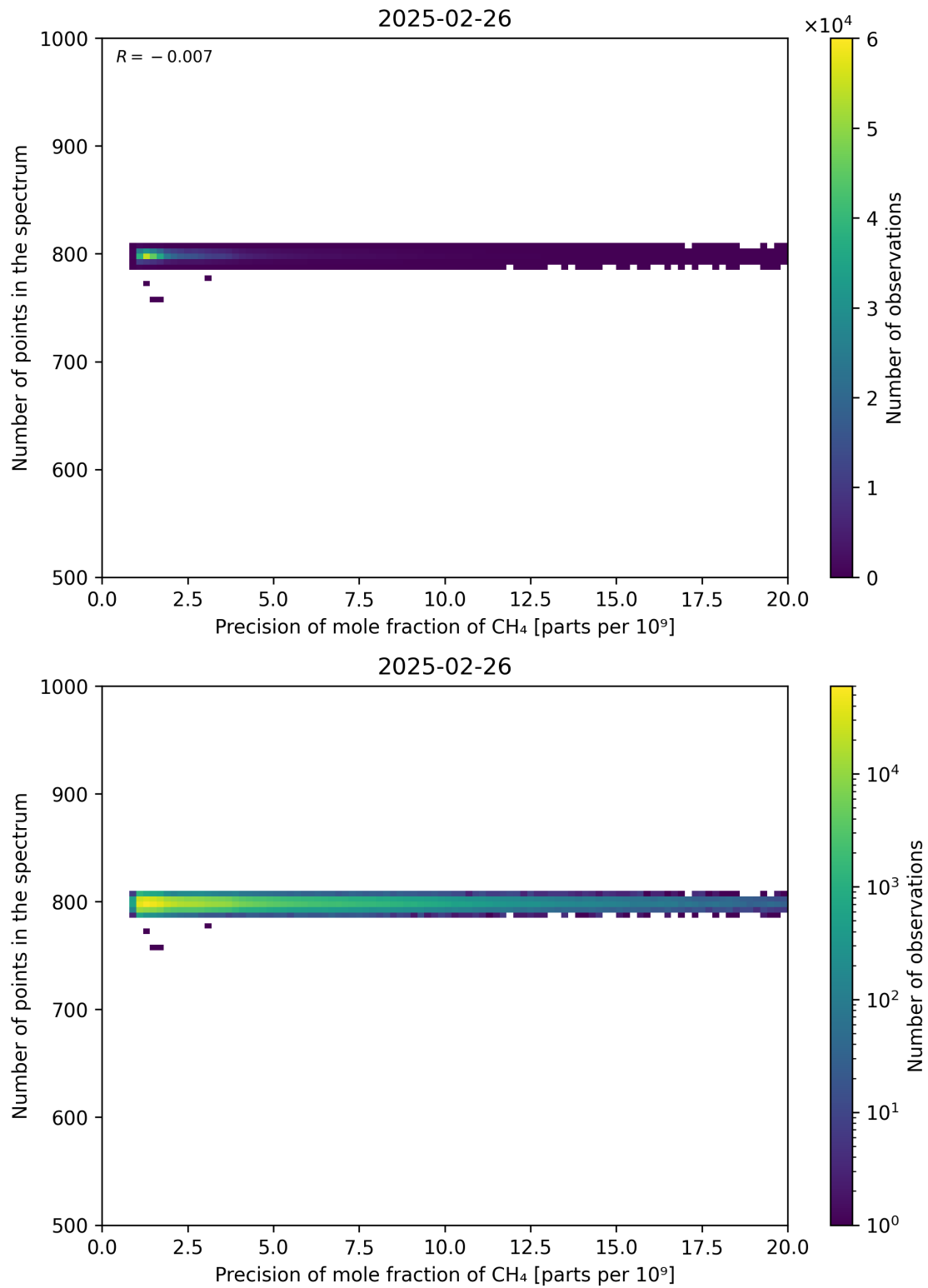
Figure 84: Scatter density plot of “Precision of mole fraction of CH 4 ” against “Number of points in the spectrum” for 2025-02-25 to 2025-02-27.
