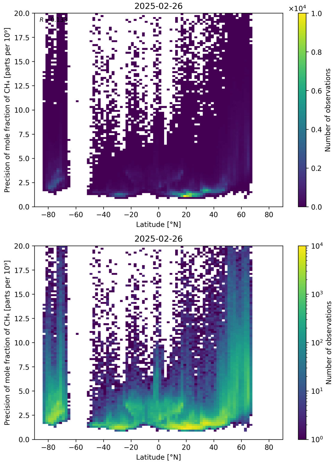
Figure 59: Scatter density plot of “Latitude” against “Precision of mole fraction of CH 4 ” for 2025-02-25 to 2025-02-27.
