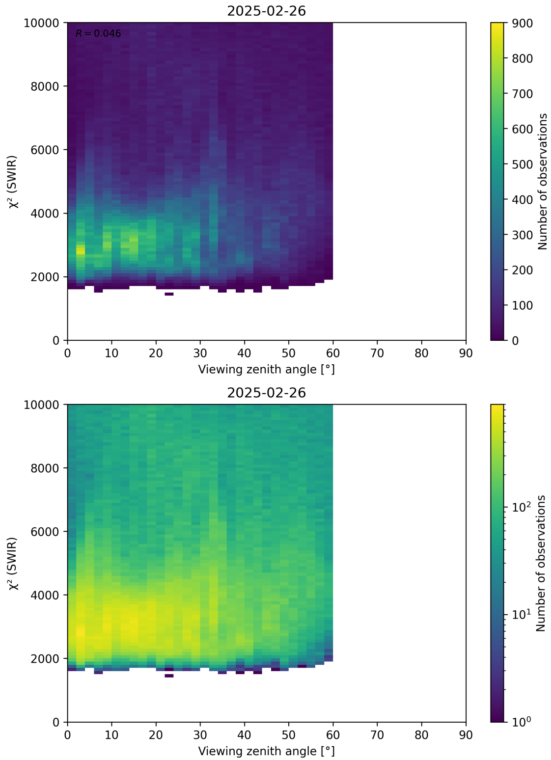
Figure 106: Scatter density plot of “Viewing zenith angle” against “ \chi^2 (SWIR)” for 2025-02-25 to 2025-02-27.
