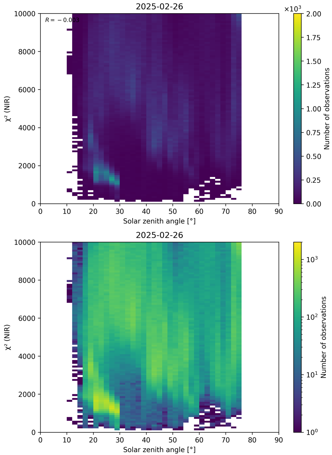
Figure 94: Scatter density plot of “Solar zenith angle” against “ \chi^2 (NIR)” for 2025-02-25 to 2025-02-27.
