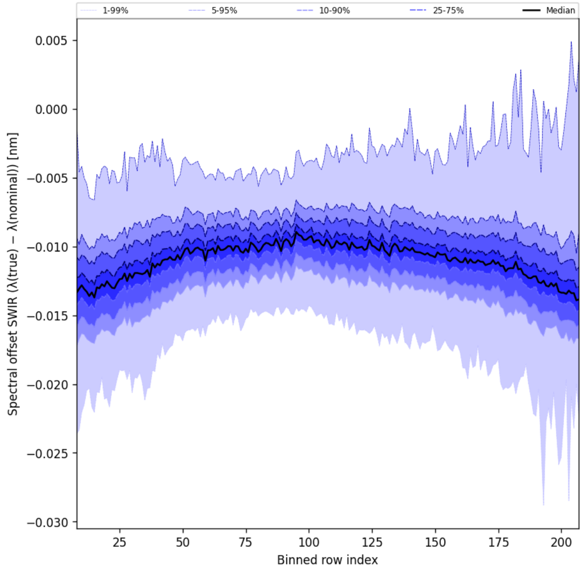
Figure 38: Along track statistics of “Spectral offset SWIR ( \lambda_{\text{true}} - \lambda_{\text{nominal}} )” for 2025-02-25 to 2025-02-27
