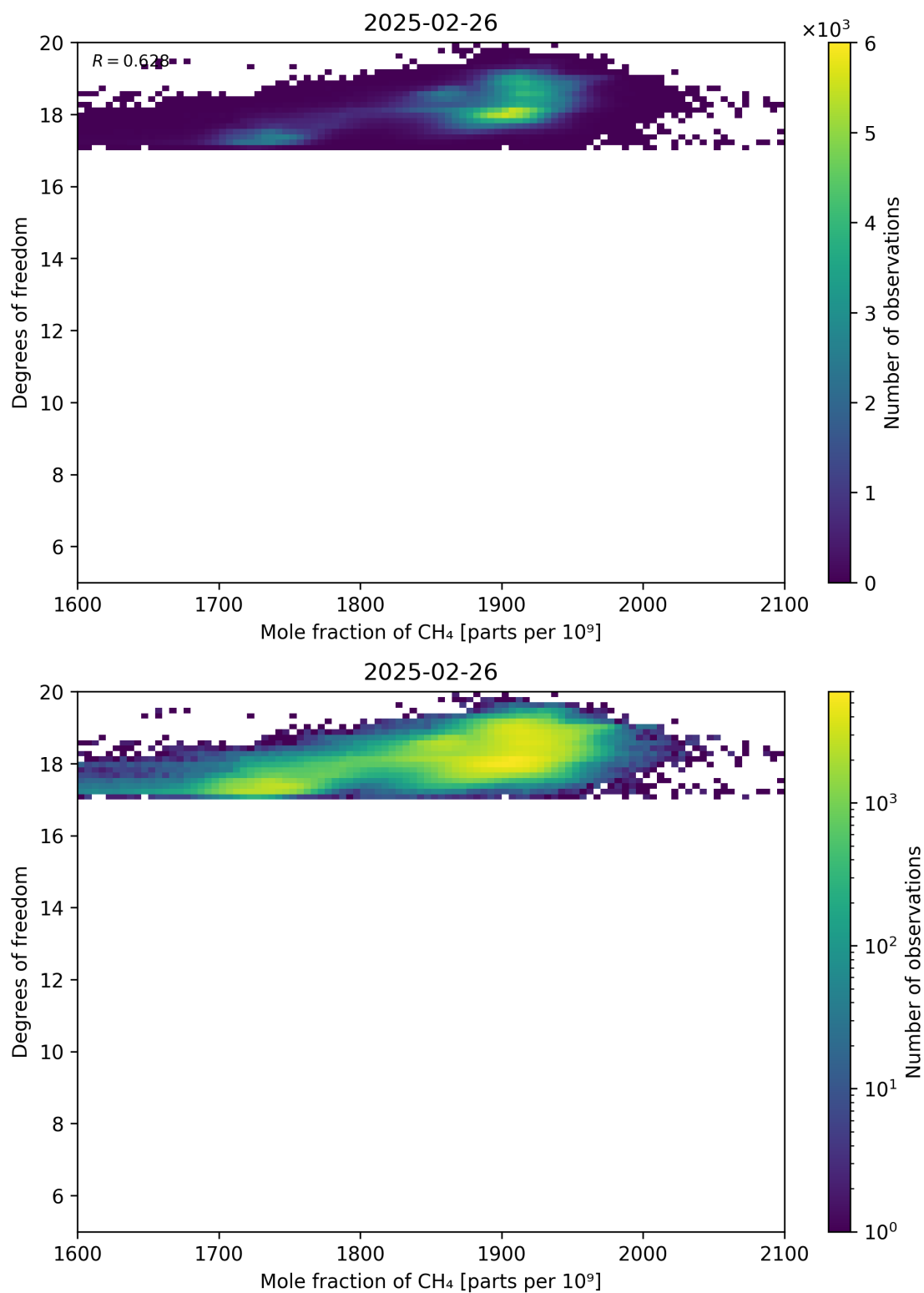
Figure 72: Scatter density plot of “Mole fraction of CH 4 ” against “Degrees of freedom” for 2025-02-25 to 2025-02-27.
