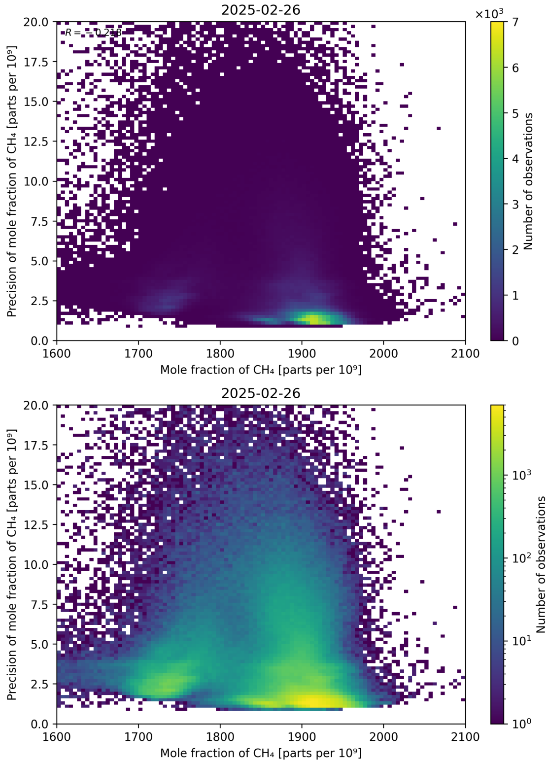
Figure 75: Scatter density plot of “Mole fraction of CH 4 ” against “Precision of mole fraction of CH 4 ” for 2025-02-25 to 2025-02-27.
