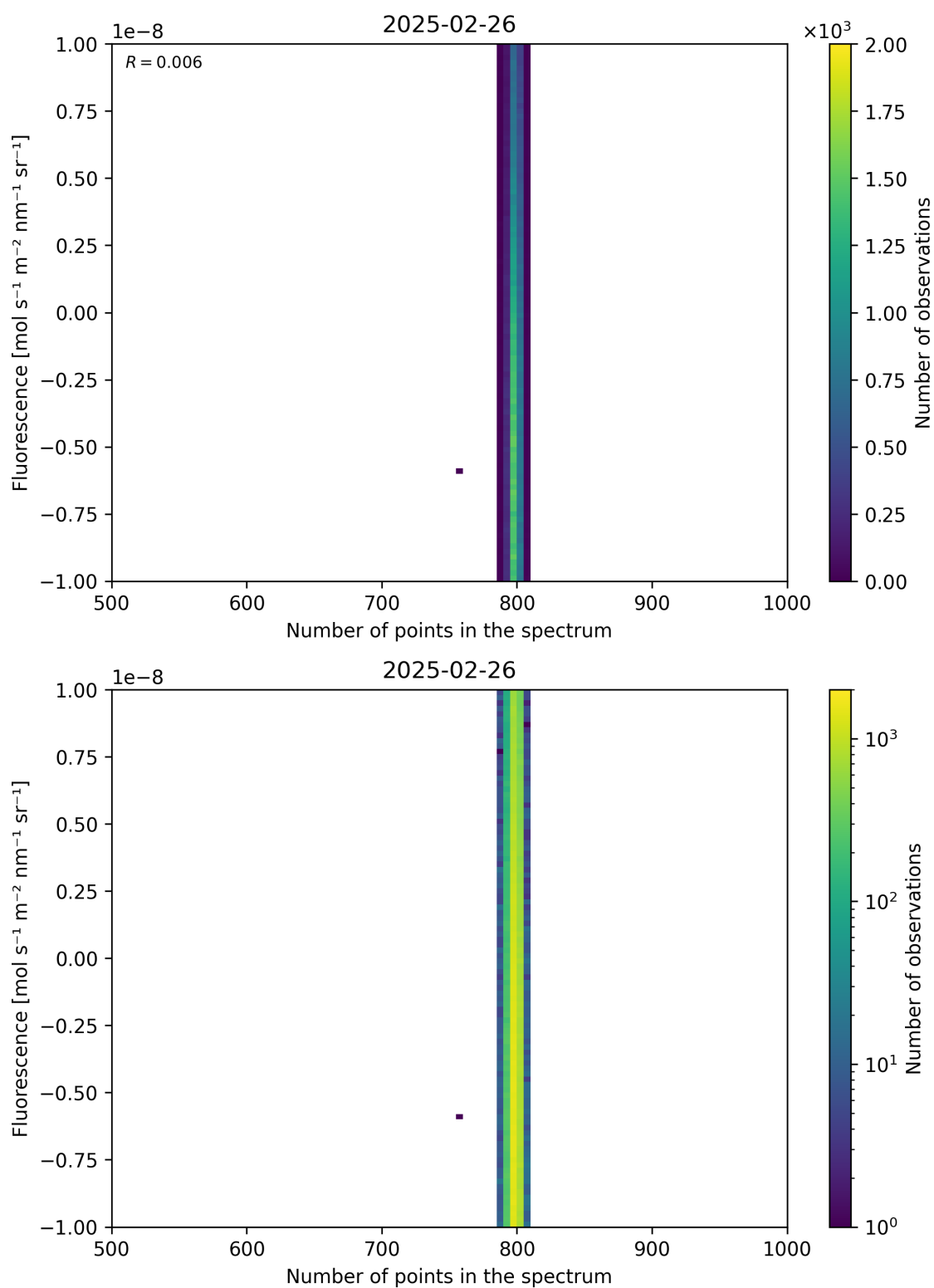
Figure 91: Scatter density plot of “Number of points in the spectrum” against “Fluorescence” for 2025-02-25 to 2025-02-27.
