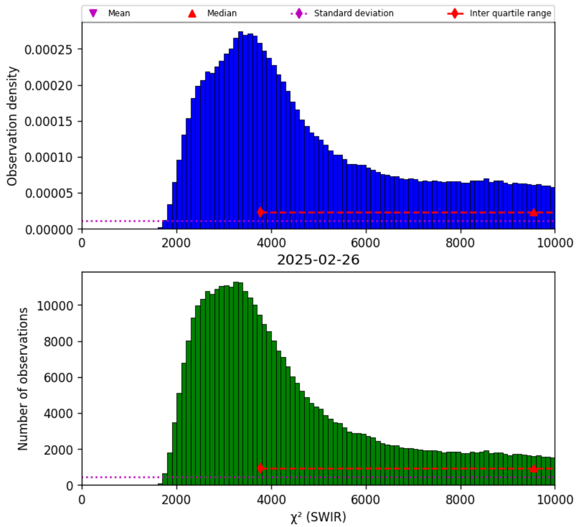
Figure 28: Histogram of “ \chi^2 (SWIR)” for 2025-02-25 to 2025-02-27
