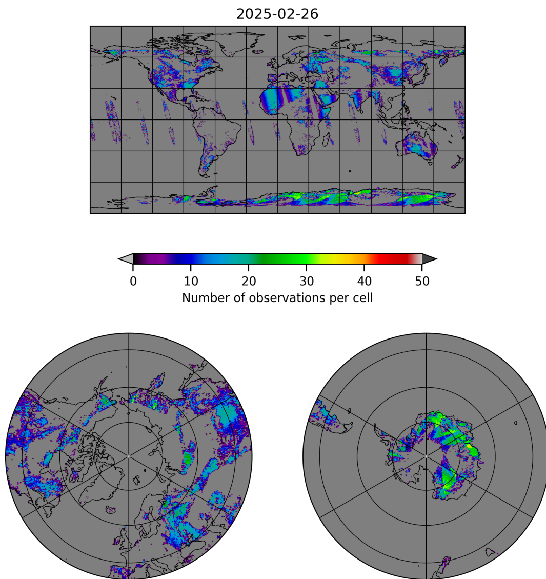
Figure 10: Map of the number of observations for 2025-02-25 to 2025-02-27
