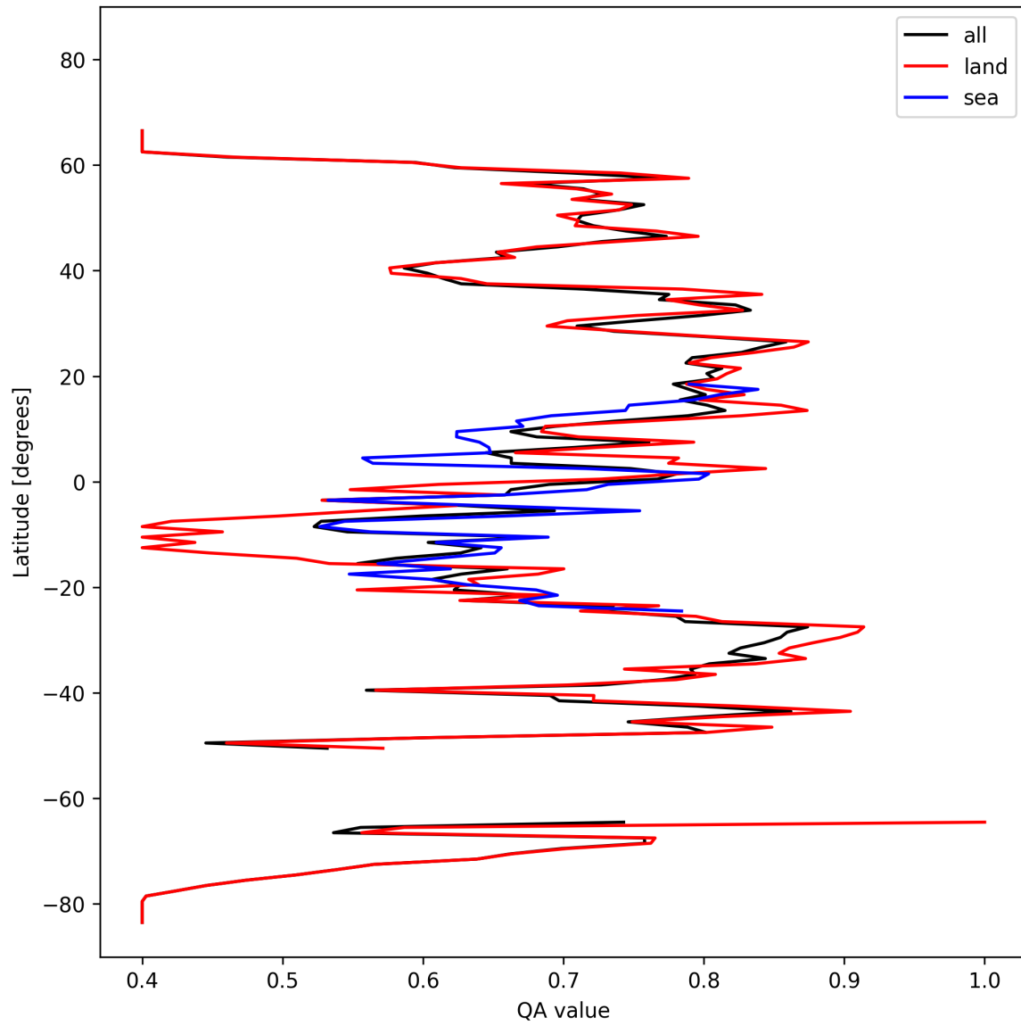
Figure 11: Zonal average of “QA value” for 2025-02-25 to 2025-02-27.
