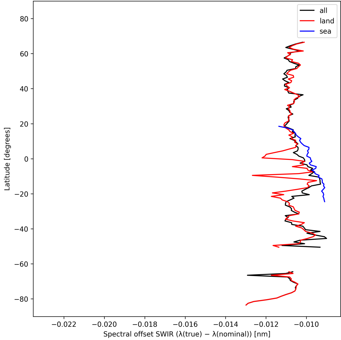
Figure 16: Zonal average of “Spectral offset SWIR ( \lambda_{\text{true}} - \lambda_{\text{nominal}} )” for 2025-02-25 to 2025-02-27.
