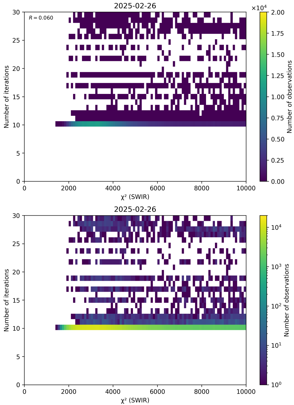
Figure 50: Scatter density plot of “ \chi^2 (SWIR)” against “Number of iterations” for 2025-02-25 to 2025-02-27.
