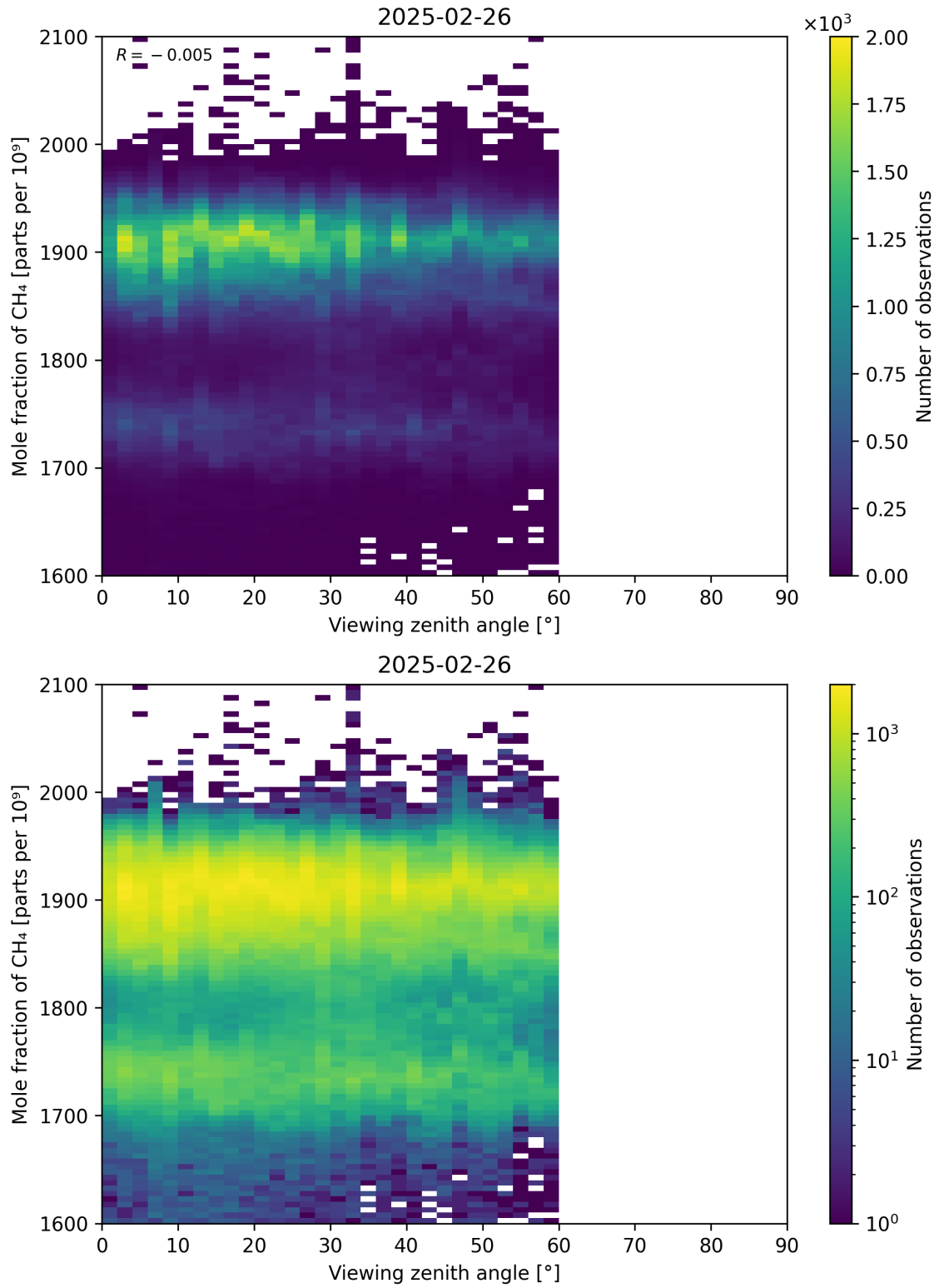
Figure 110: Scatter density plot of “Viewing zenith angle” against “Mole fraction of CH 4 ” for 2025-02-25 to 2025-02-27.
