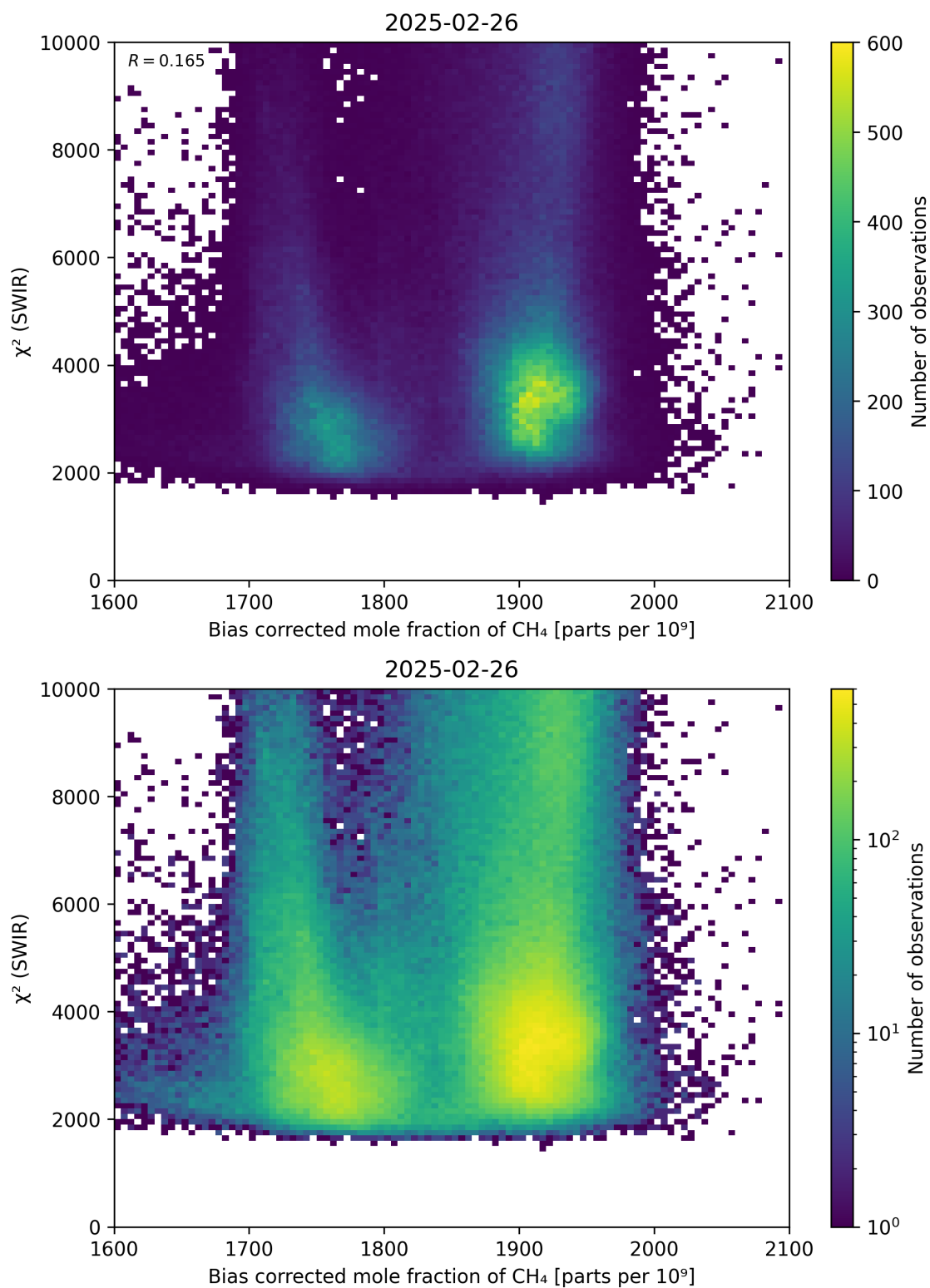
Figure 64: Scatter density plot of “Bias corrected mole fraction of CH 4 ” against “ \chi^2 (SWIR)” for 2025-02-25 to 2025-02-27.
