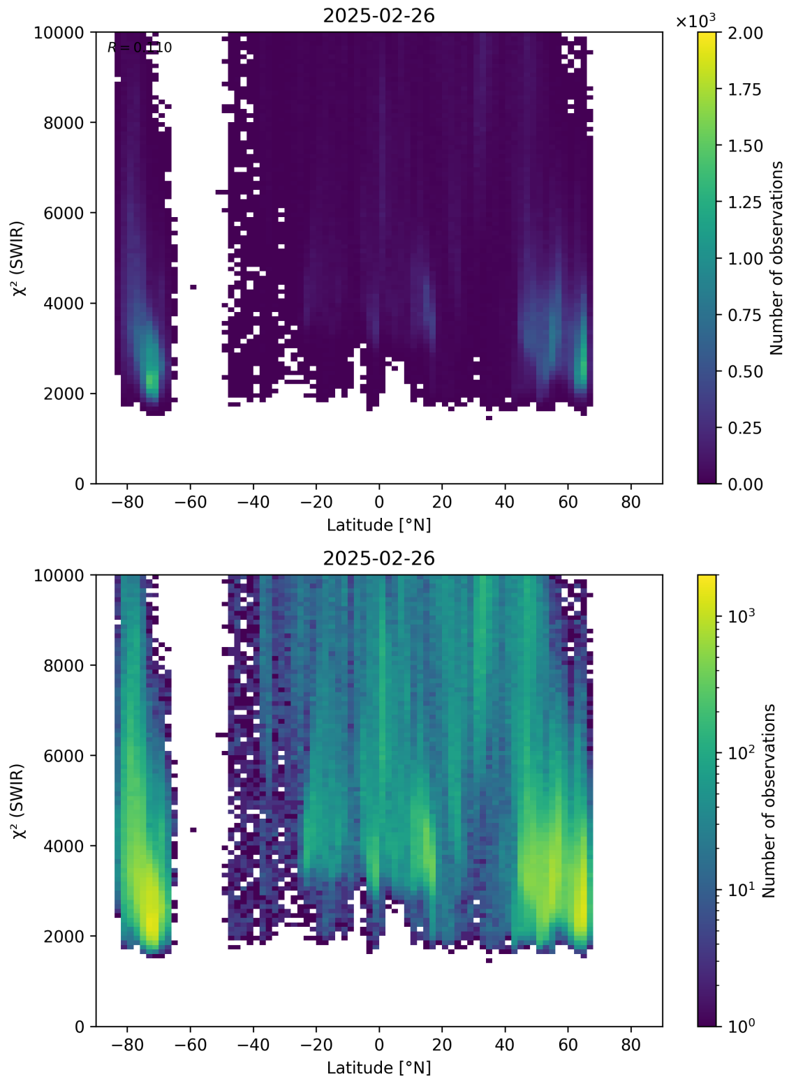
Figure 54: Scatter density plot of “Latitude” against “ \chi^2 (SWIR)” for 2025-02-25 to 2025-02-27.
