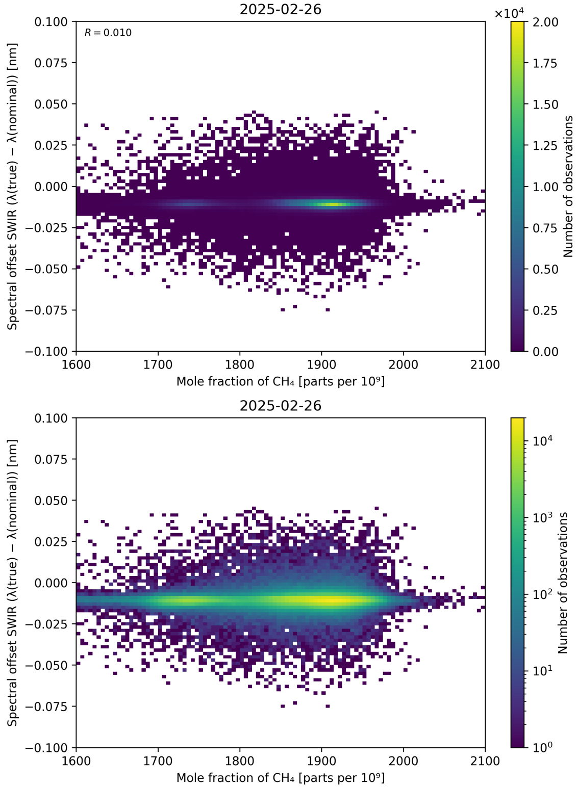
Figure 86: Scatter density plot of “Mole fraction of \text{CH}_4 ” against “Spectral offset SWIR ( \lambda_{\text{true}} - \lambda_{\text{nominal}} )” for 2025-02-25 to 2025-02-27.
