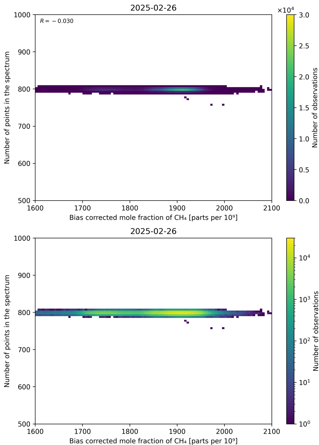
Figure 68: Scatter density plot of “Bias corrected mole fraction of CH 4 ” against “Number of points in the spectrum” for 2025-02-25 to 2025-02-27.
