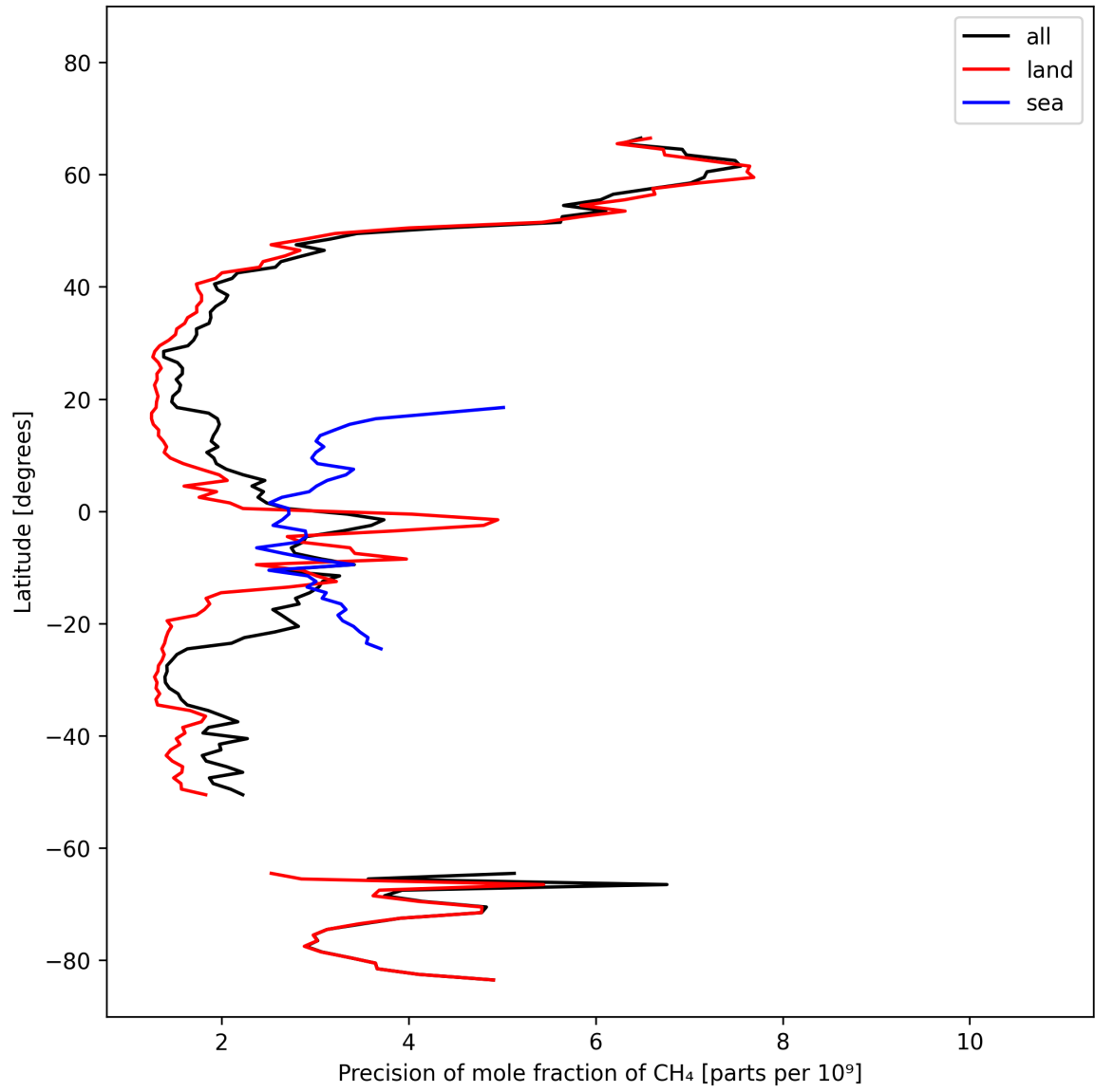
Figure 13: Zonal average of “Precision of mole fraction of CH 4 ” for 2025-02-25 to 2025-02-27.
