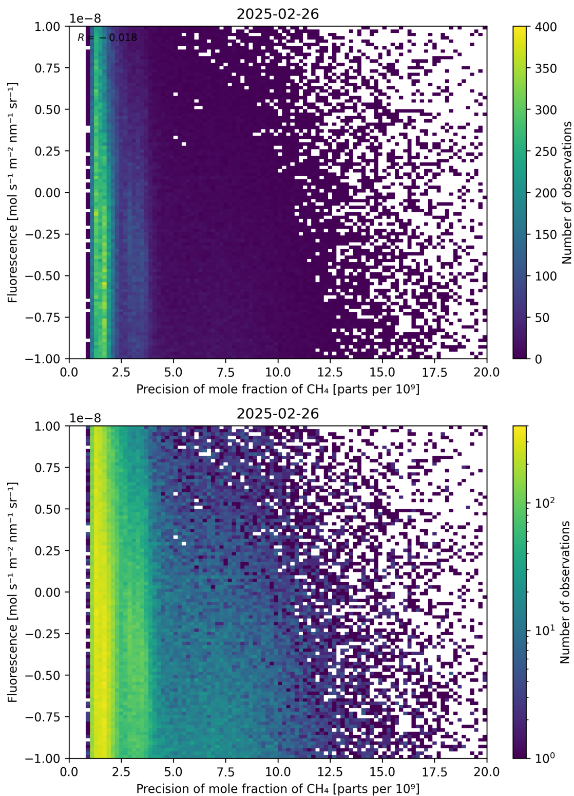
Figure 81: Scatter density plot of “Precision of mole fraction of CH 4 ” against “Fluorescence” for 2025-02-25 to 2025-02-27.
