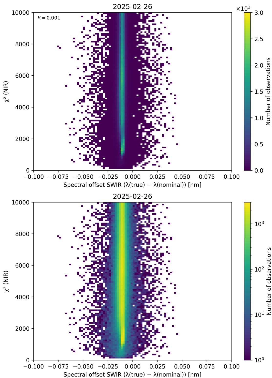
Figure 117: Scatter density plot of “Spectral offset SWIR ( \lambda_{\text{true}} - \lambda_{\text{nominal}} )” against “ \chi^2 (NIR)” for 2025-02-25 to 2025-02-27.
