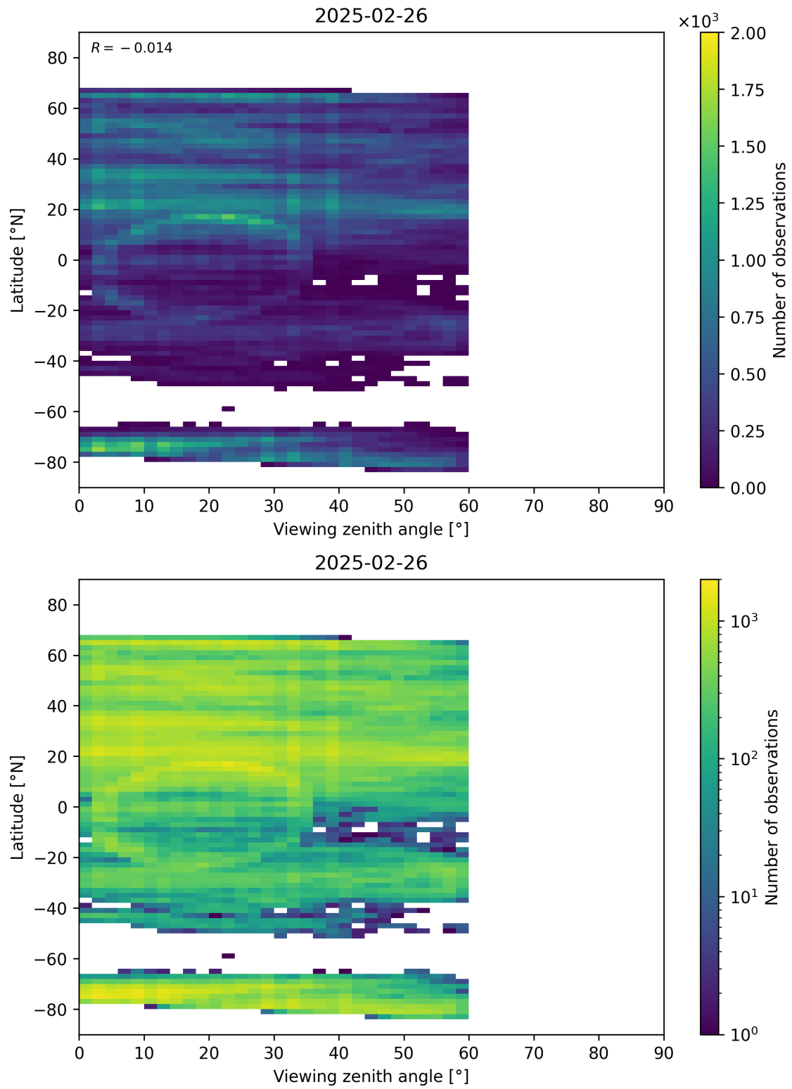
Figure 109: Scatter density plot of “Viewing zenith angle” against “Latitude” for 2025-02-25 to 2025-02-27.
