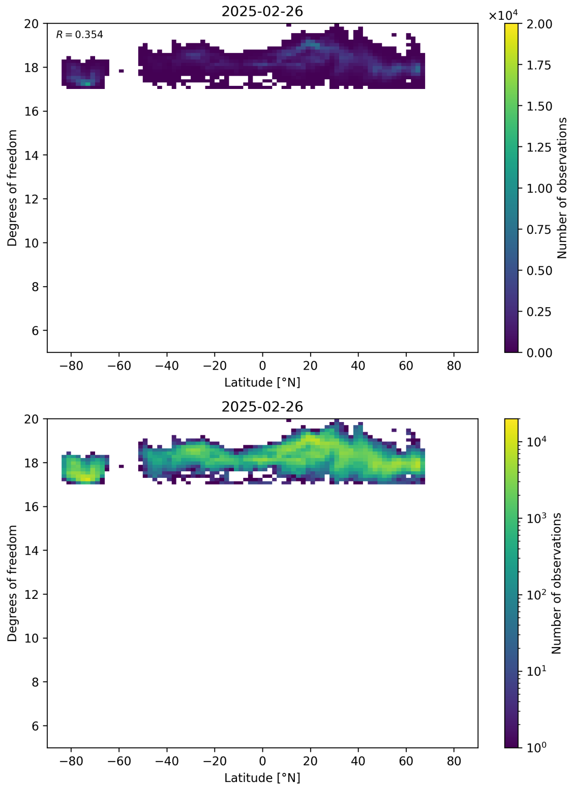
Figure 55: Scatter density plot of “Latitude” against “Degrees of freedom” for 2025-02-25 to 2025-02-27.
