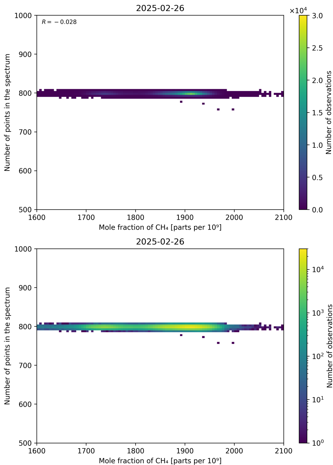
Figure 77: Scatter density plot of “Mole fraction of CH 4 ” against “Number of points in the spectrum” for 2025-02-25 to 2025-02-27.
