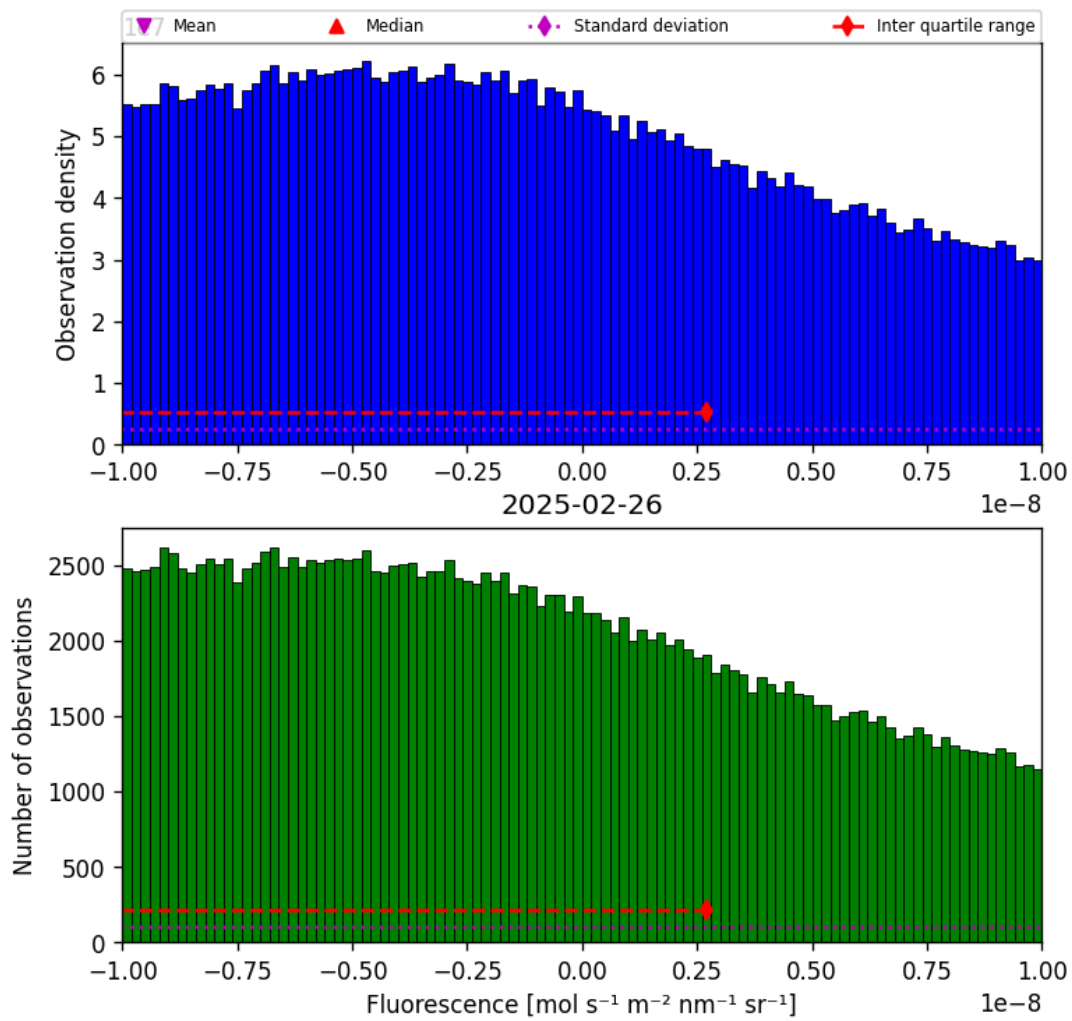
Figure 32: Histogram of “Fluorescence” for 2025-02-25 to 2025-02-27
