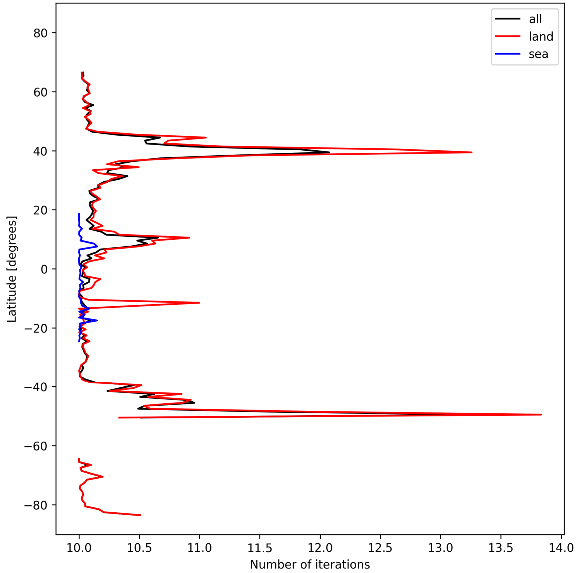
Figure 20: Zonal average of “Number of iterations” for 2025-02-25 to 2025-02-27.
