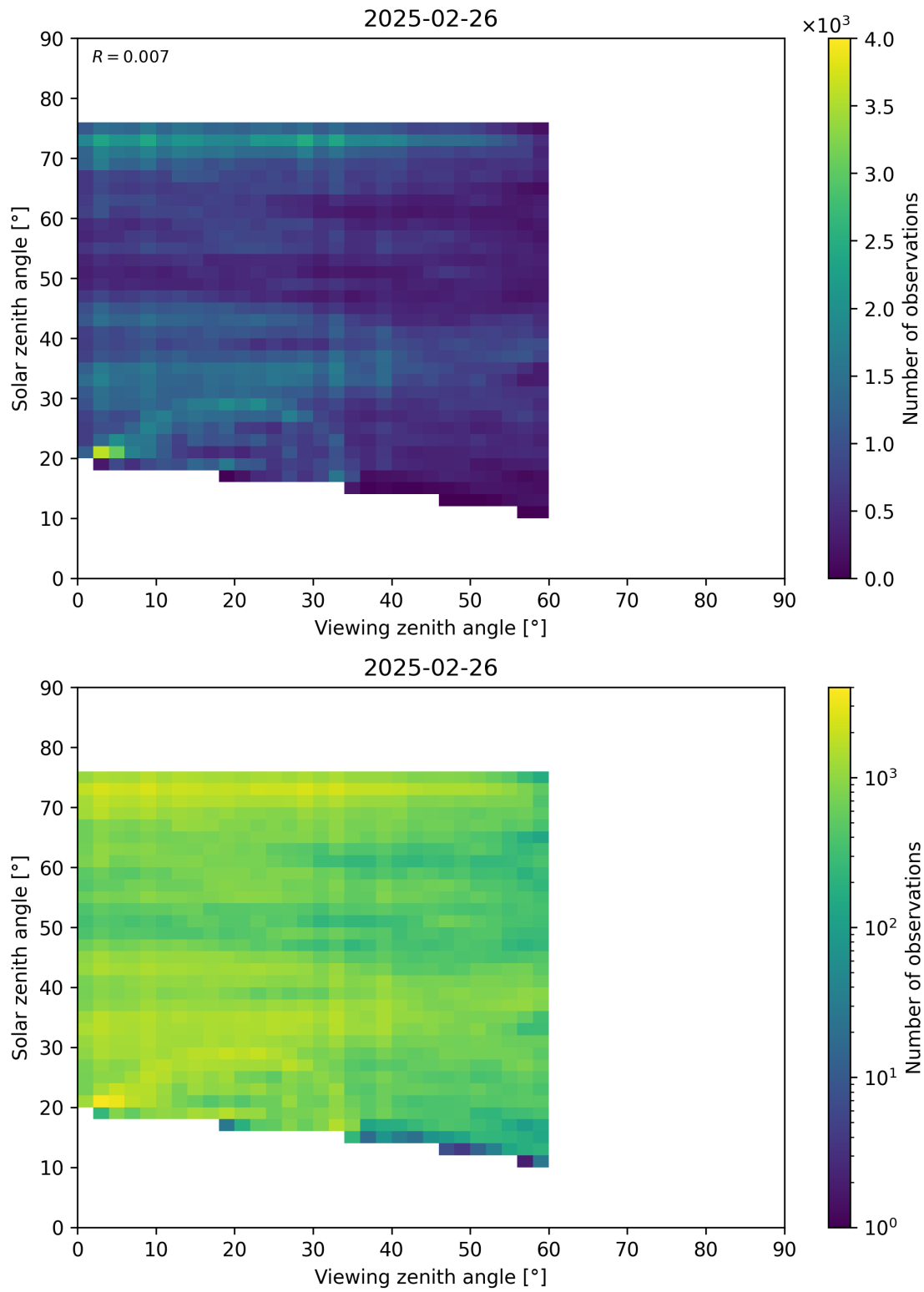
Figure 115: Scatter density plot of “Viewing zenith angle” against “Solar zenith angle” for 2025-02-25 to 2025-02-27.
