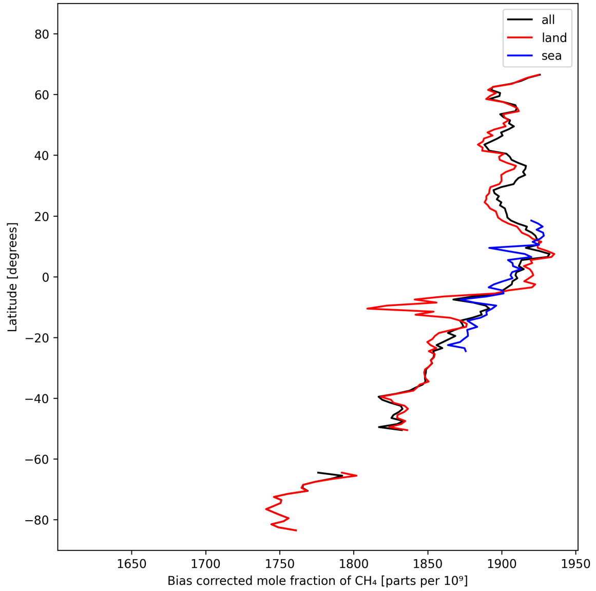
Figure 14: Zonal average of “Bias corrected mole fraction of CH 4 ” for 2025-02-25 to 2025-02-27.
