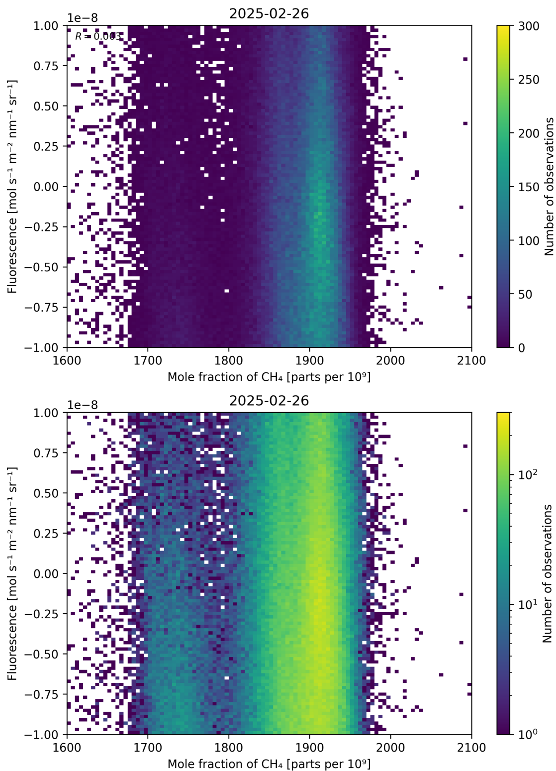
Figure 73: Scatter density plot of “Mole fraction of \text{CH}_4 ” against “Fluorescence” for 2025-02-25 to 2025-02-27.
