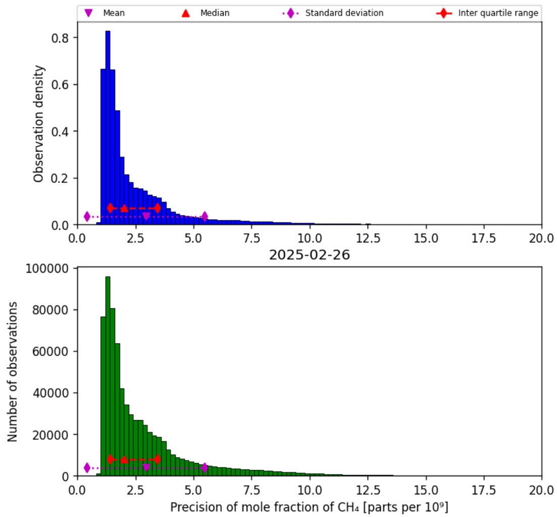
Figure 24: Histogram of “Precision of mole fraction of CH 4 ” for 2025-02-25 to 2025-02-27
