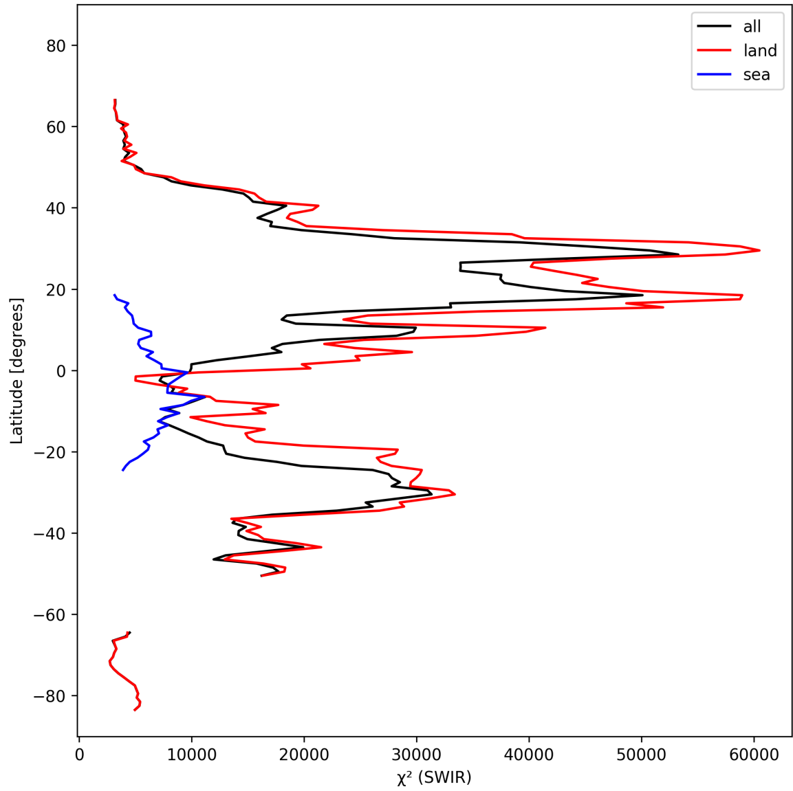
Figure 17: Zonal average of “ \chi^2 (SWIR)” for 2025-02-25 to 2025-02-27.
