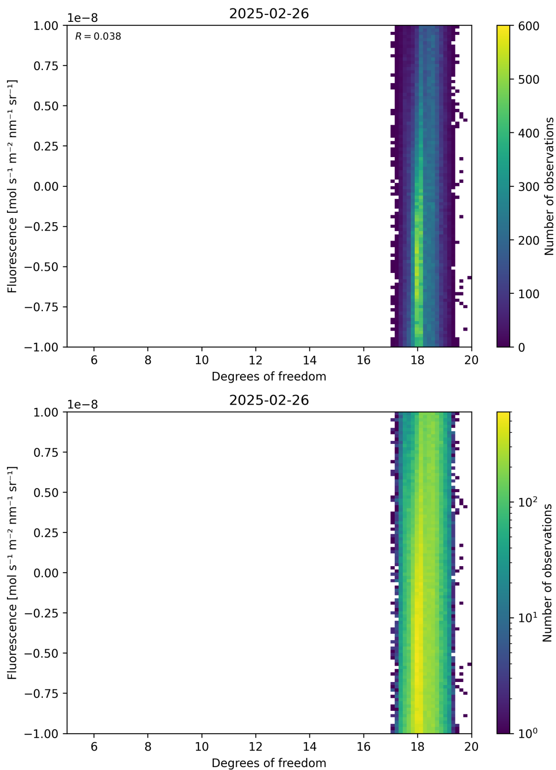
Figure 51: Scatter density plot of “Degrees of freedom” against “Fluorescence” for 2025-02-25 to 2025-02-27.
