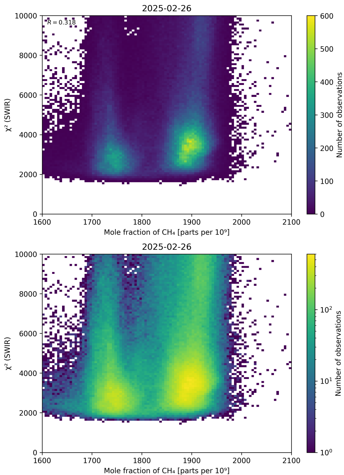
Figure 71: Scatter density plot of “Mole fraction of \text{CH}_4 ” against “ \chi^2 (SWIR)” for 2025-02-25 to 2025-02-27.
