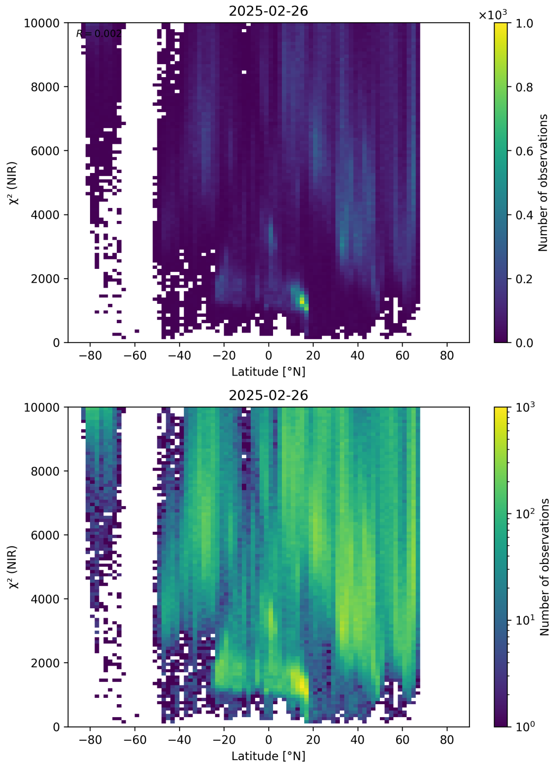
Figure 53: Scatter density plot of “Latitude” against “ \chi^2 (NIR)” for 2025-02-25 to 2025-02-27.
