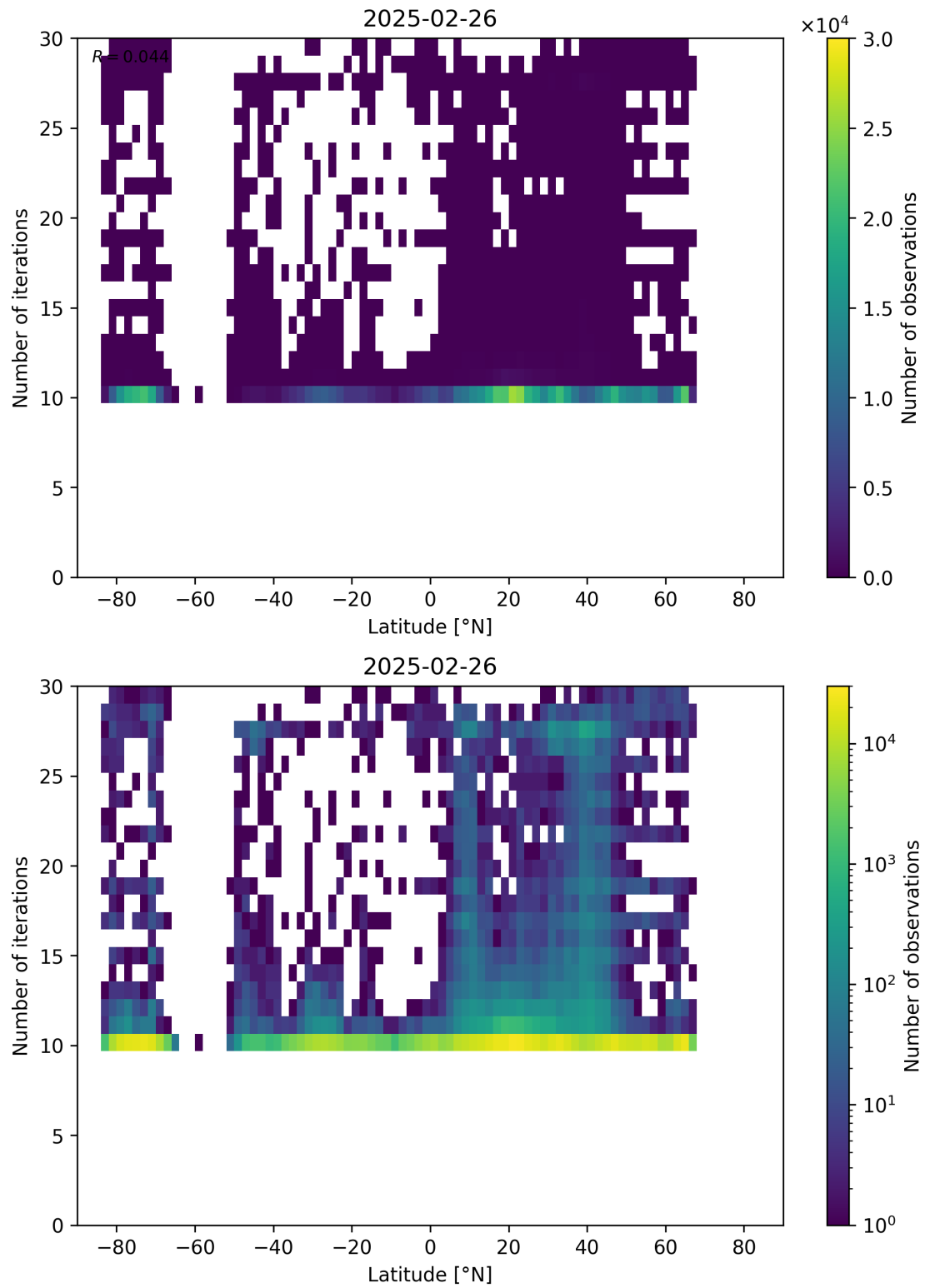
Figure 60: Scatter density plot of “Latitude” against “Number of iterations” for 2025-02-25 to 2025-02-27.
