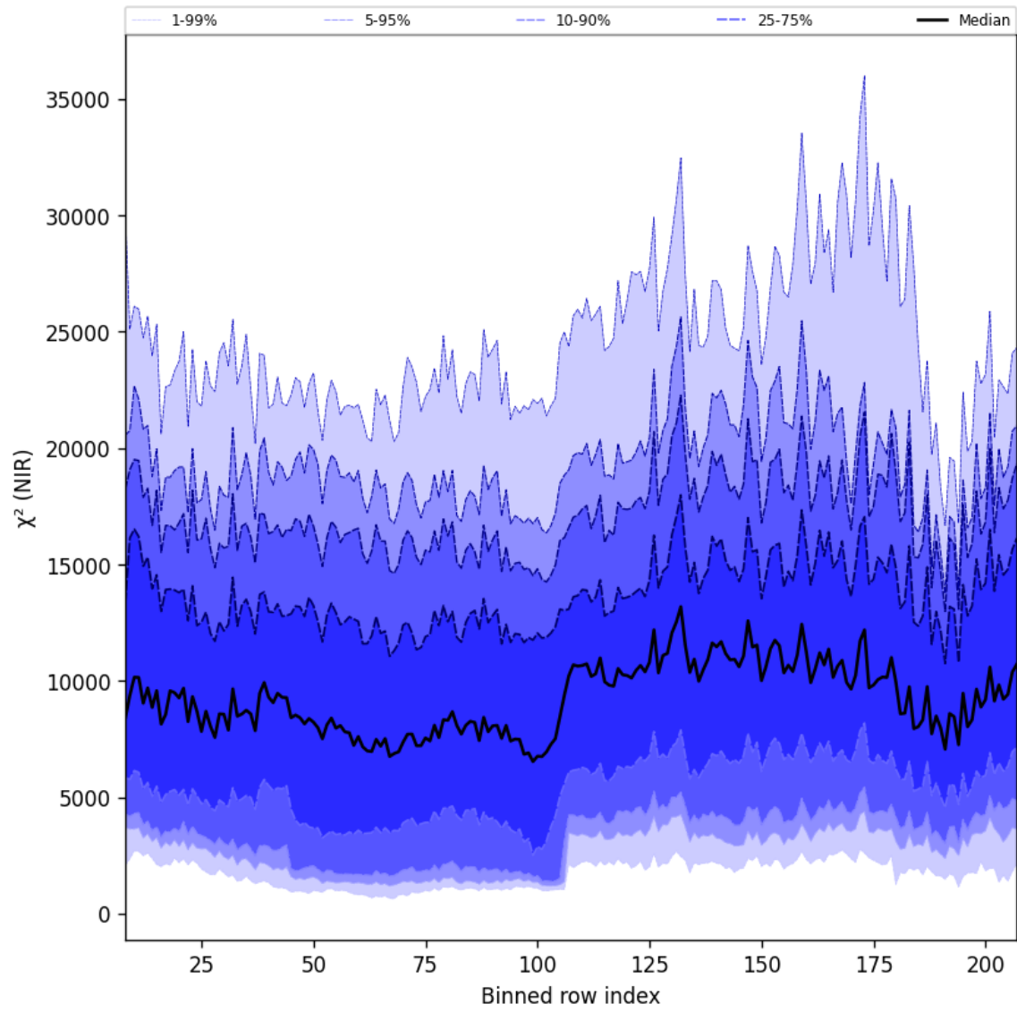
Figure 40: Along track statistics of “ \chi^2 (NIR)” for 2025-02-25 to 2025-02-27
