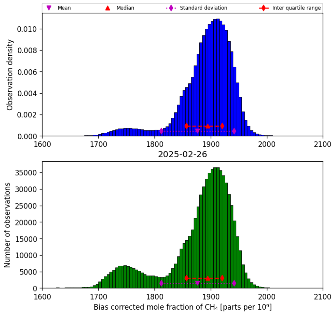
Figure 25: Histogram of “Bias corrected mole fraction of CH 4 ” for 2025-02-25 to 2025-02-27
