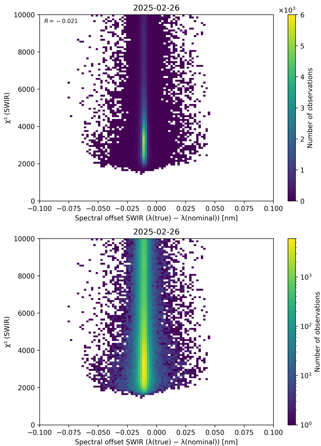
Figure 118: Scatter density plot of “Spectral offset SWIR ( \lambda_{\text{true}} - \lambda_{\text{nominal}} )” against “ \chi^2 (SWIR)” for 2025-02-25 to 2025-02-27.
