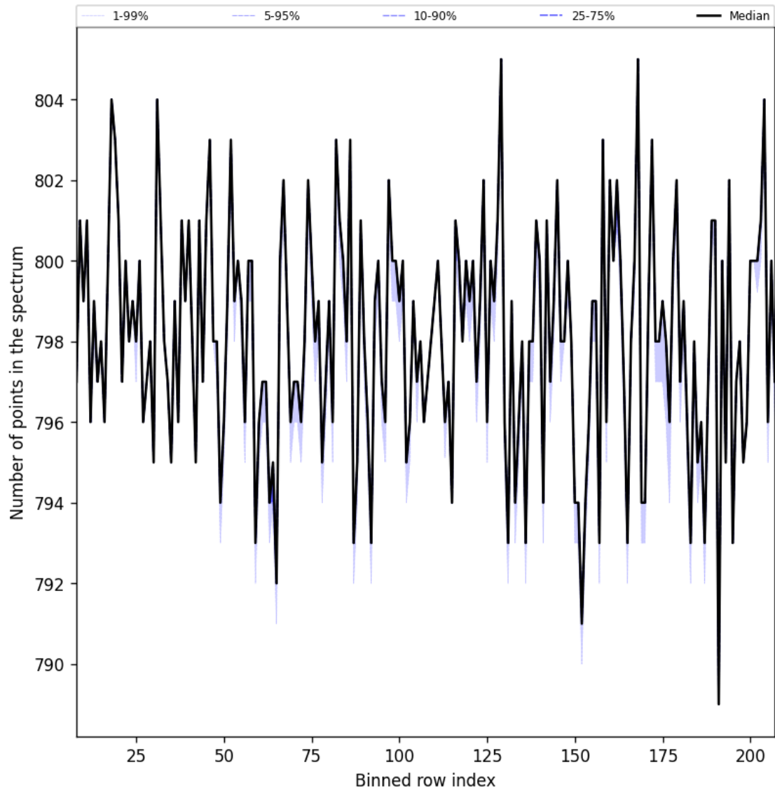
Figure 37: Along track statistics of “Number of points in the spectrum” for 2025-02-25 to 2025-02-27
