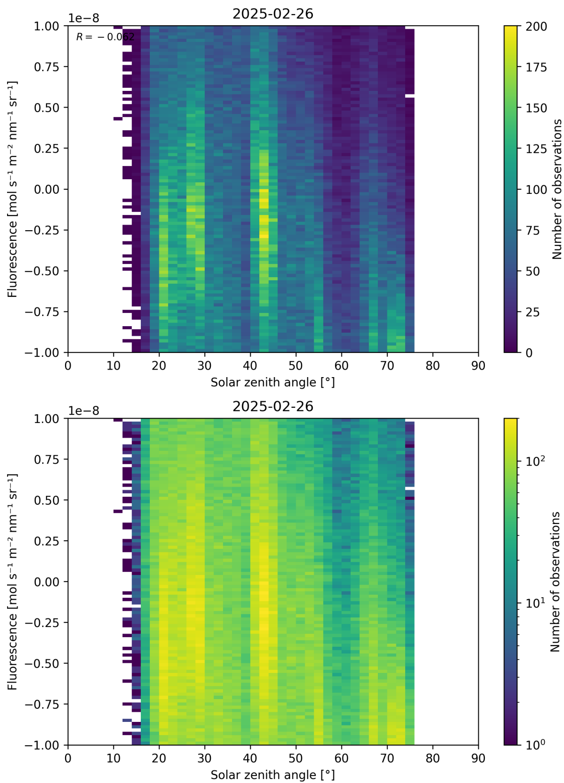
Figure 97: Scatter density plot of “Solar zenith angle” against “Fluorescence” for 2025-02-25 to 2025-02-27.
