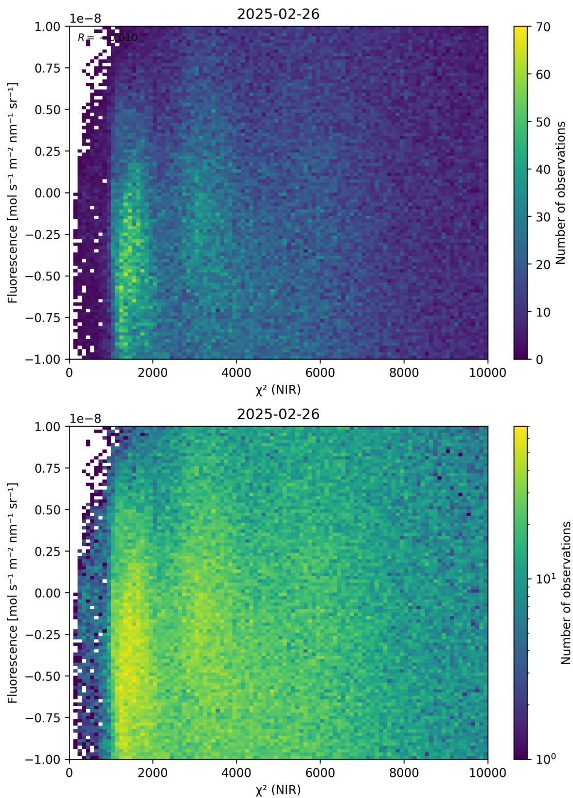
Figure 45: Scatter density plot of “ \chi^2 (NIR)” against “Fluorescence” for 2025-02-25 to 2025-02-27.
