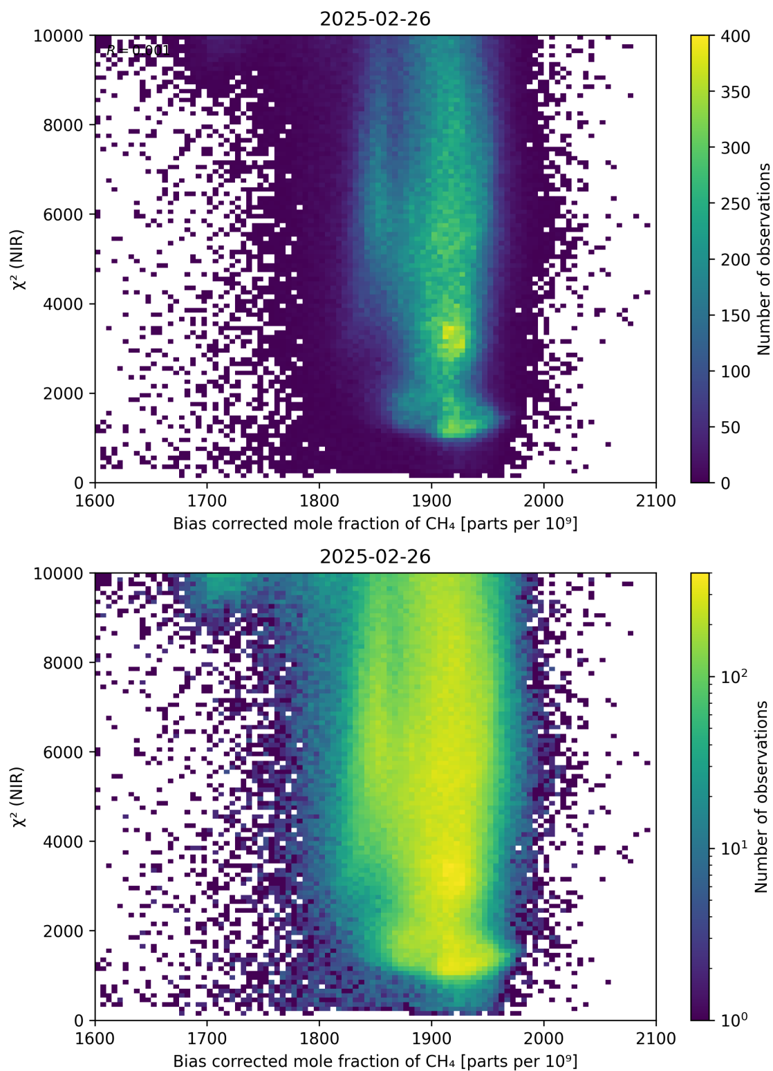
Figure 63: Scatter density plot of “Bias corrected mole fraction of CH 4 ” against “ \chi^2 (NIR)” for 2025-02-25 to 2025-02-27.
