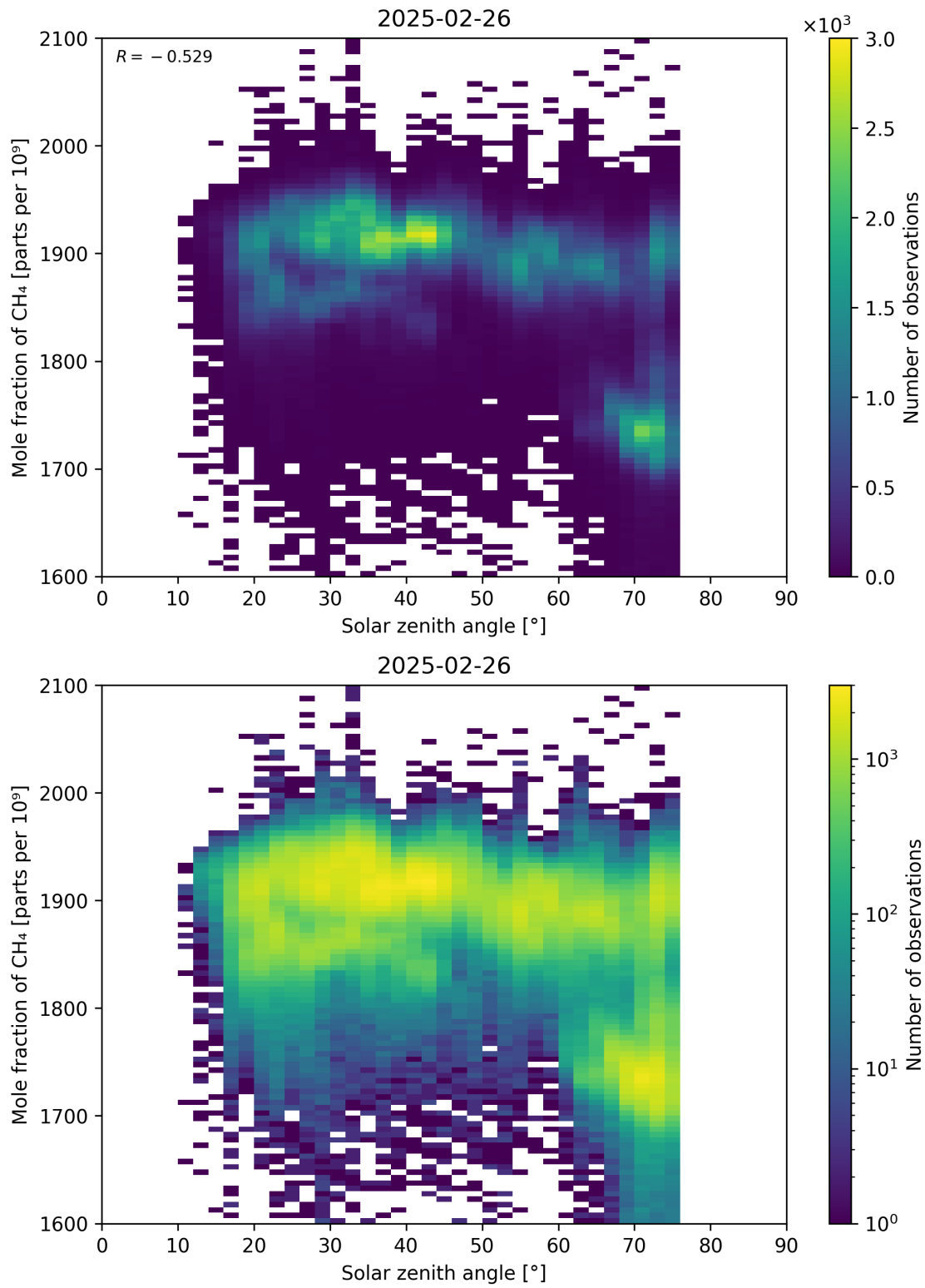
Figure 99: Scatter density plot of “Solar zenith angle” against “Mole fraction of CH 4 ” for 2025-02-25 to 2025-02-27.
