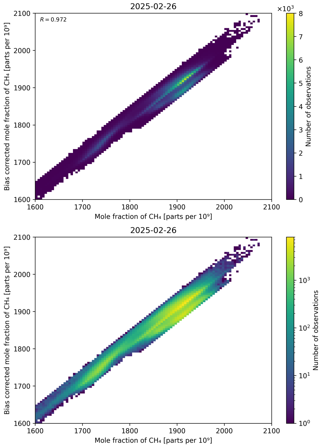
Figure 74: Scatter density plot of “Mole fraction of CH 4 ” against “Bias corrected mole fraction of CH 4 ” for 2025-02-25 to 2025-02-27.
