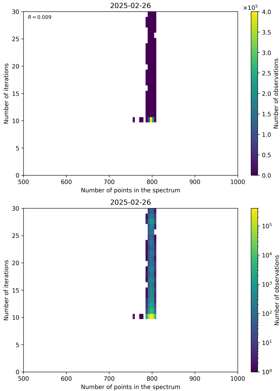
Figure 92: Scatter density plot of “Number of points in the spectrum” against “Number of iterations” for 2025-02-25 to 2025-02-27.
