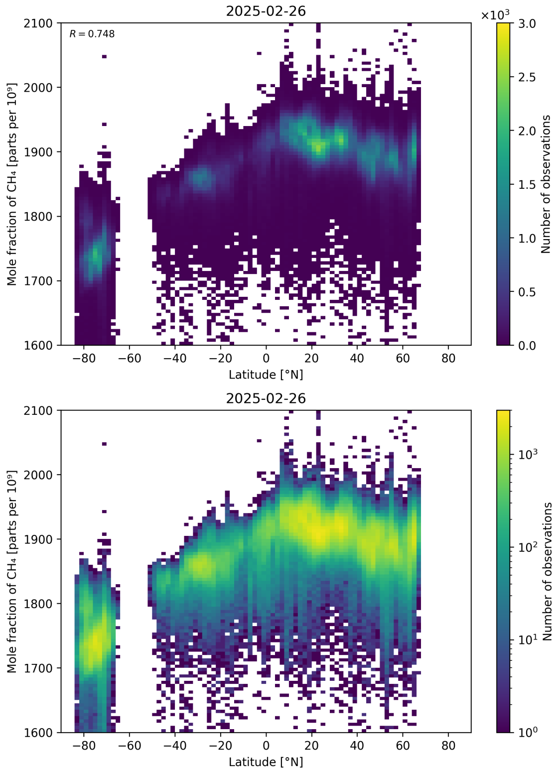
Figure 57: Scatter density plot of “Latitude” against “Mole fraction of CH 4 ” for 2025-02-25 to 2025-02-27.
