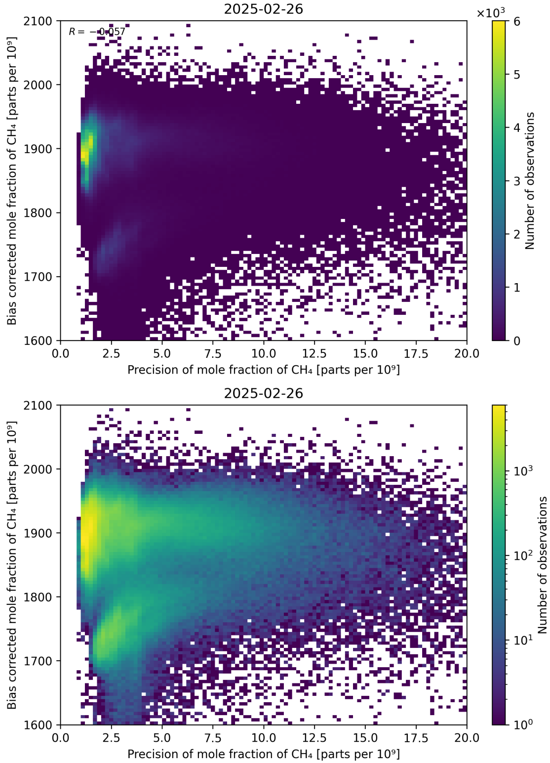
Figure 82: Scatter density plot of “Precision of mole fraction of CH 4 ” against “Bias corrected mole fraction of CH 4 ” for 2025-02-25 to 2025-02-27.
