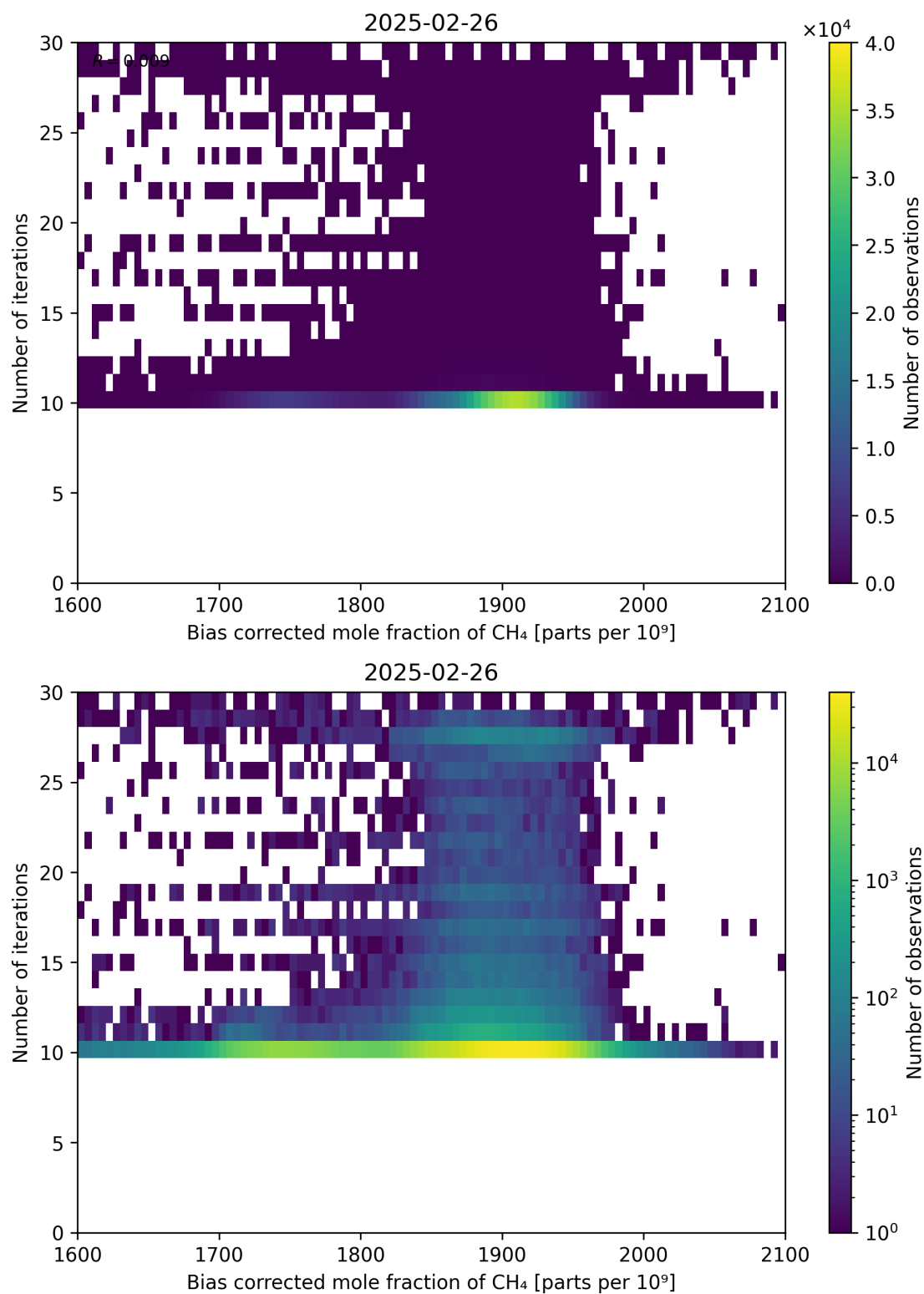
Figure 67: Scatter density plot of “Bias corrected mole fraction of \text{CH}_4 ” against “Number of iterations” for 2025-02-25 to 2025-02-27.
