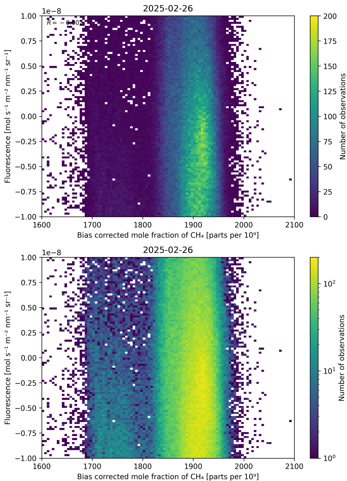
Figure 66: Scatter density plot of “Bias corrected mole fraction of \text{CH}_4 ” against “Fluorescence” for 2025-02-25 to 2025-02-27.
