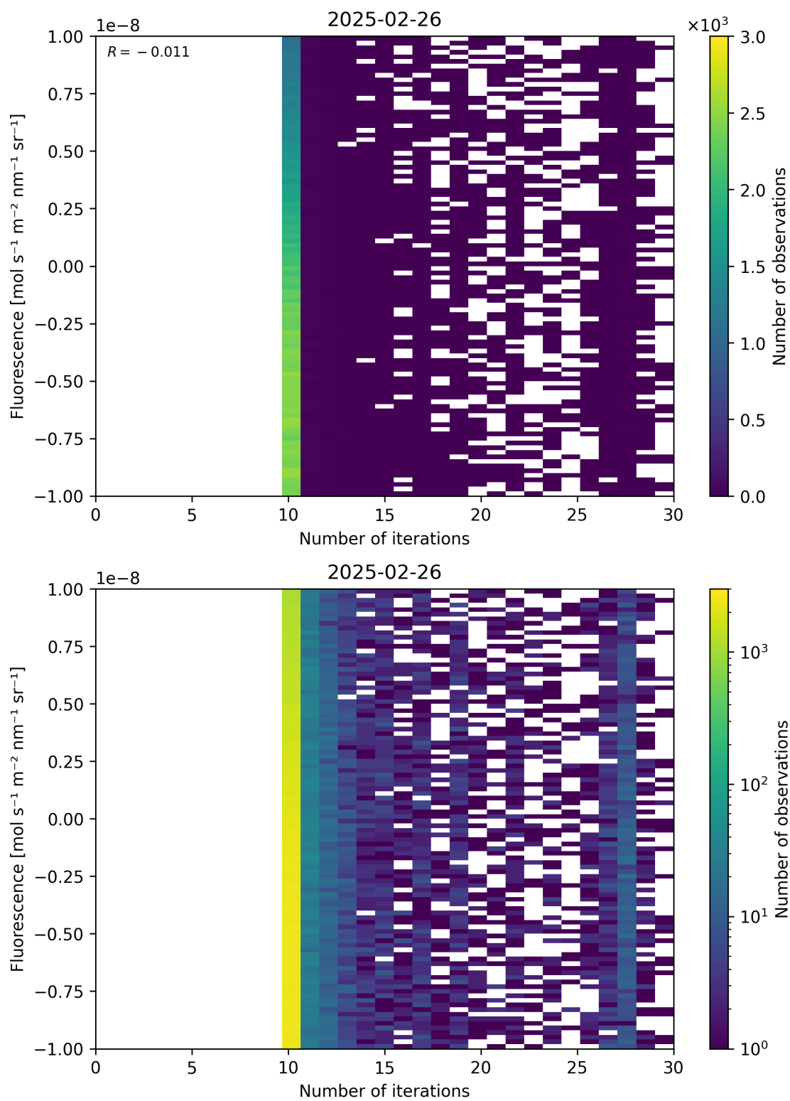
Figure 87: Scatter density plot of “Number of iterations” against “Fluorescence” for 2025-02-25 to 2025-02-27.
