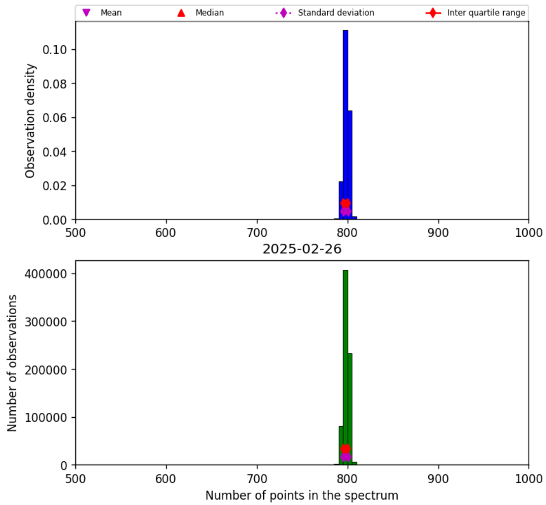
Figure 26: Histogram of “Number of points in the spectrum” for 2025-02-25 to 2025-02-27
