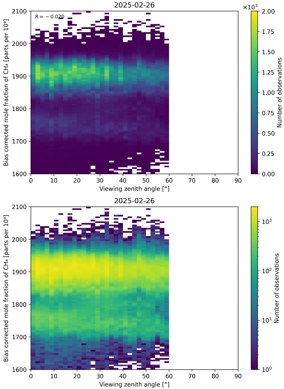
Figure 111: Scatter density plot of “Viewing zenith angle” against “Bias corrected mole fraction of CH 4 ” for 2025-02-25 to 2025-02-27.
