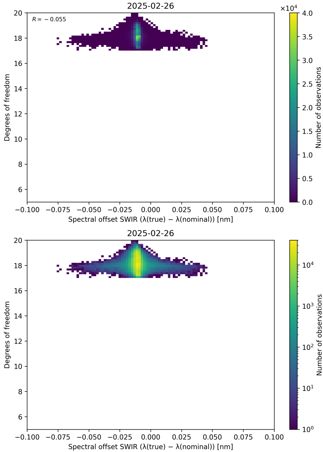
Figure 119: Scatter density plot of “Spectral offset SWIR ( \lambda_{\text{true}} - \lambda_{\text{nominal}} )” against “Degrees of freedom” for 2025-02-25 to 2025-02-27.
