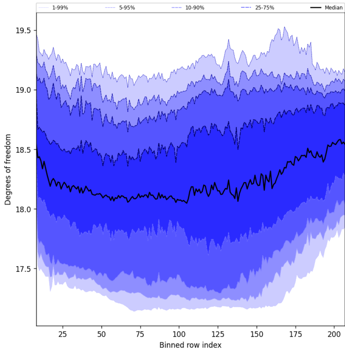
Figure 41: Along track statistics of “Degrees of freedom” for 2025-02-25 to 2025-02-27
