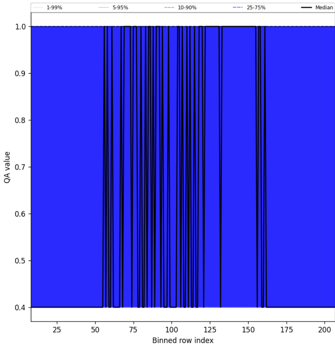
Figure 33: Along track statistics of “QA value” for 2025-02-25 to 2025-02-27
