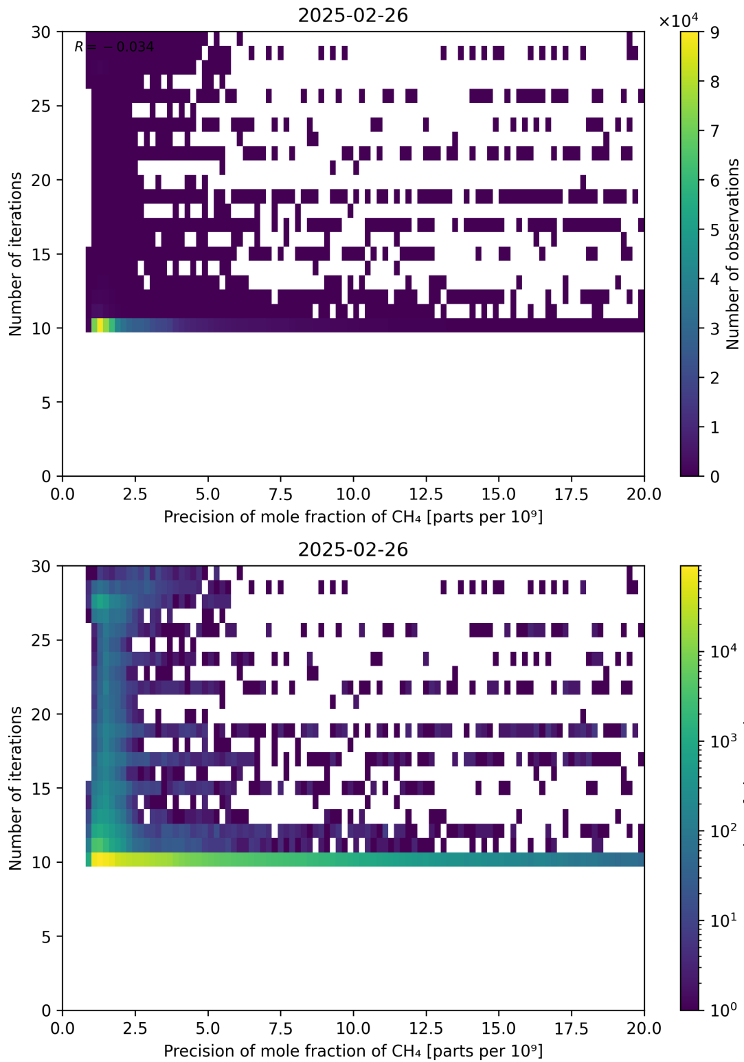
Figure 83: Scatter density plot of “Precision of mole fraction of CH 4 ” against “Number of iterations” for 2025-02-25 to 2025-02-27.
