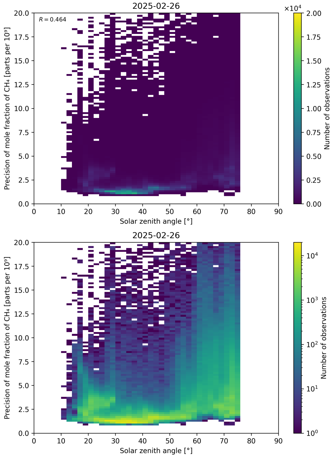
Figure 101: Scatter density plot of “Solar zenith angle” against “Precision of mole fraction of CH 4 ” for 2025-02-25 to 2025-02-27.
