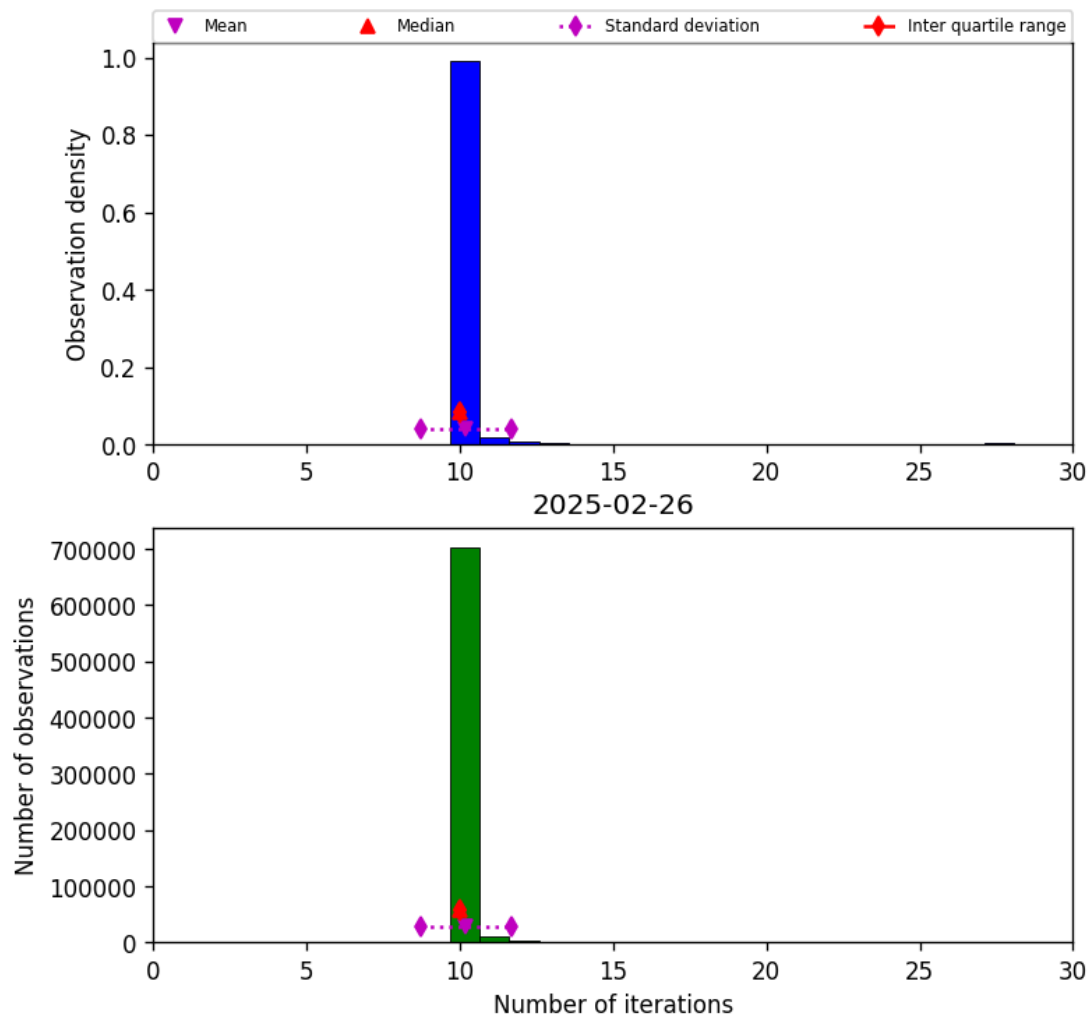
Figure 31: Histogram of “Number of iterations” for 2025-02-25 to 2025-02-27
