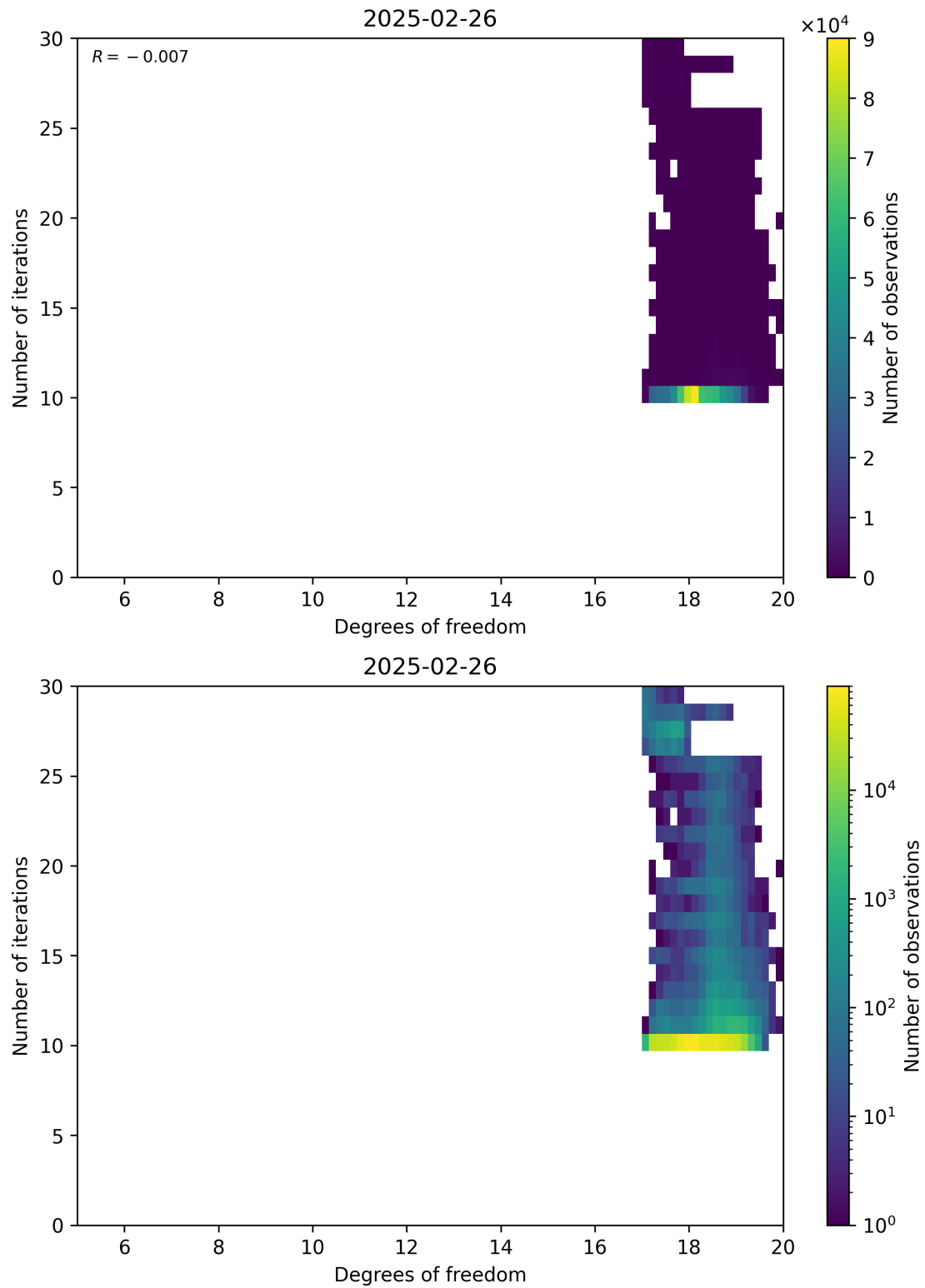
Figure 52: Scatter density plot of “Degrees of freedom” against “Number of iterations” for 2025-02-25 to 2025-02-27.
