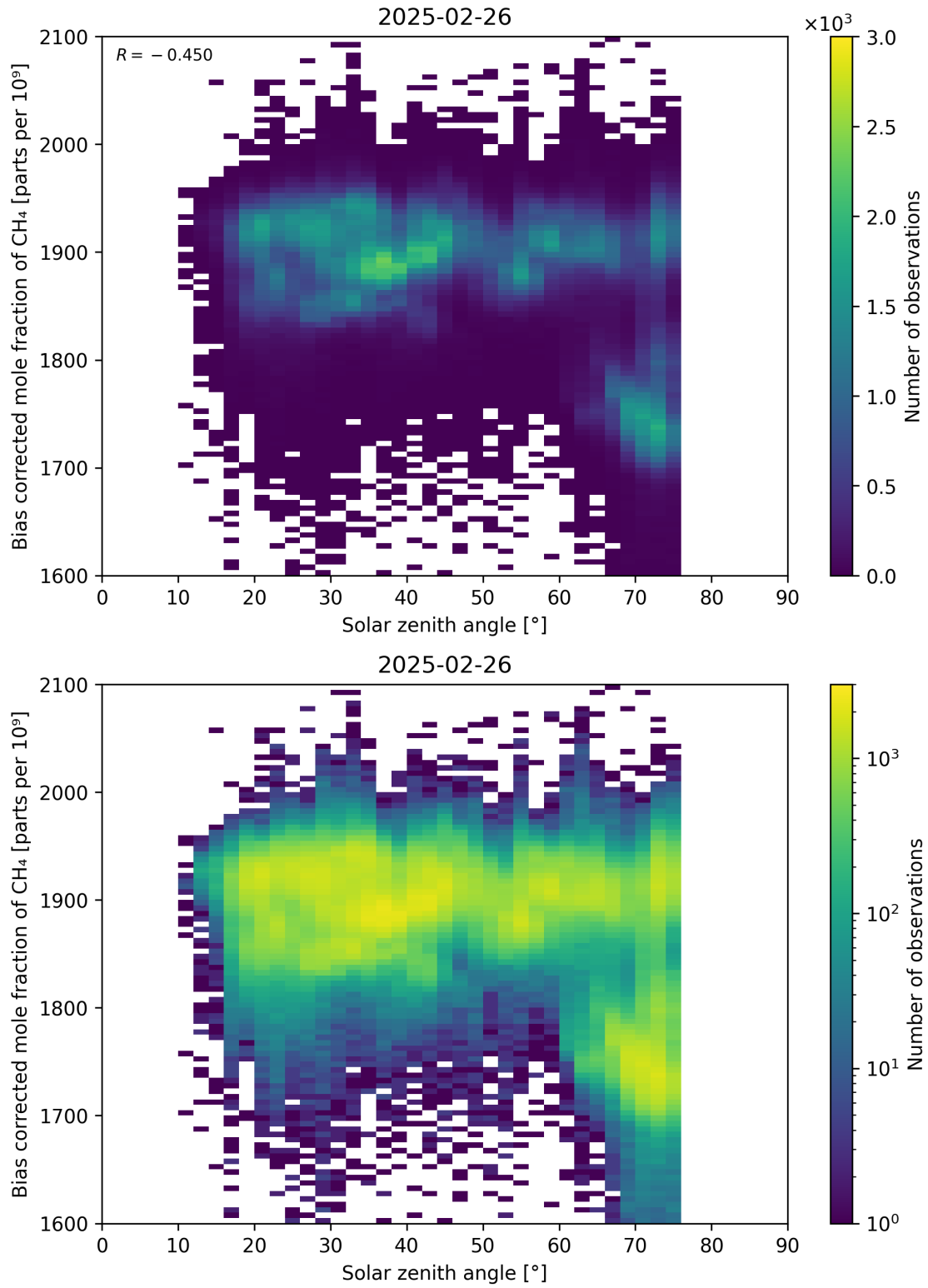
Figure 100: Scatter density plot of “Solar zenith angle” against “Bias corrected mole fraction of \text{CH}_4 ” for 2025-02-25 to 2025-02-27.
