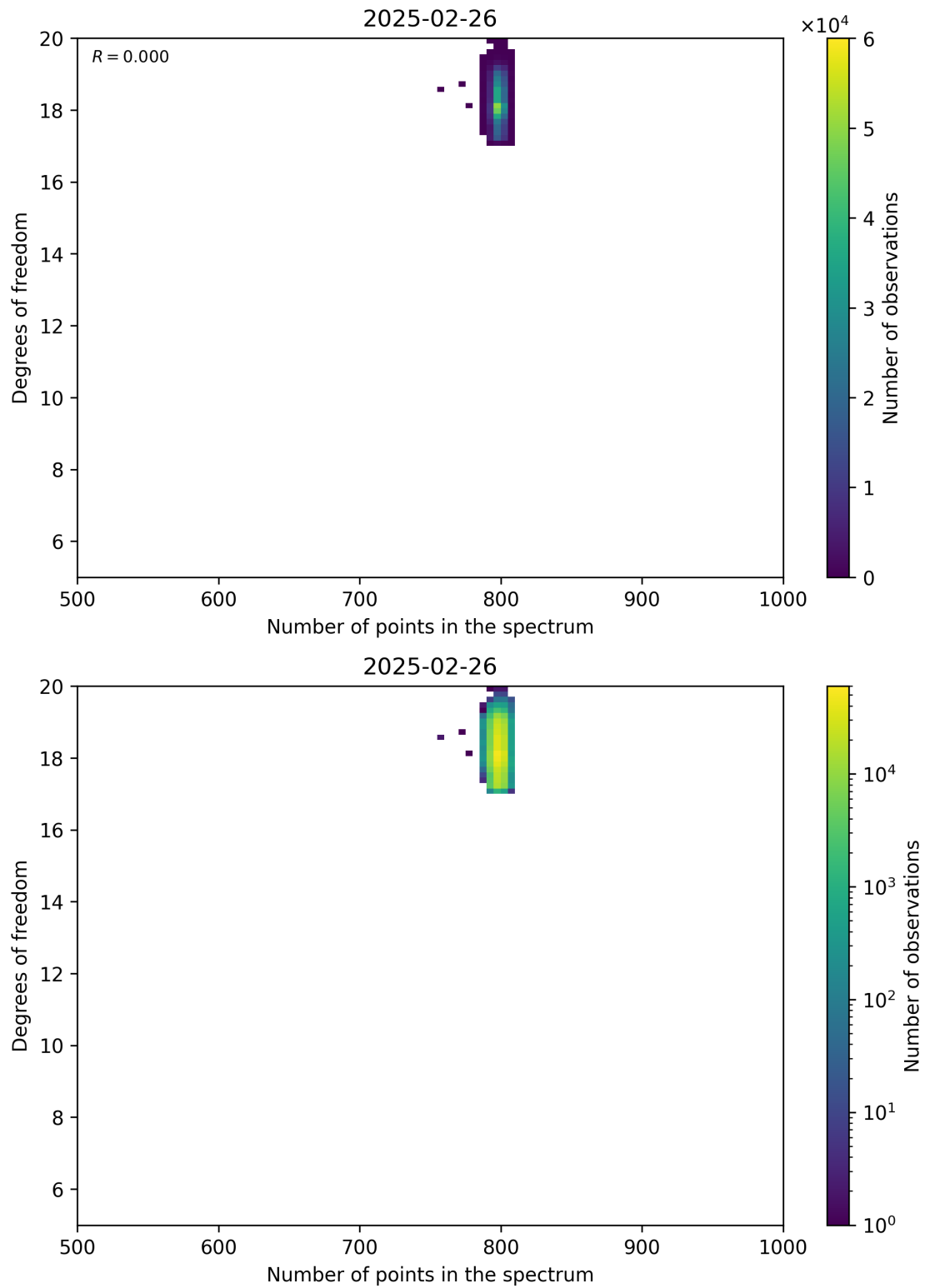
Figure 90: Scatter density plot of “Number of points in the spectrum” against “Degrees of freedom” for 2025-02-25 to 2025-02-27.
