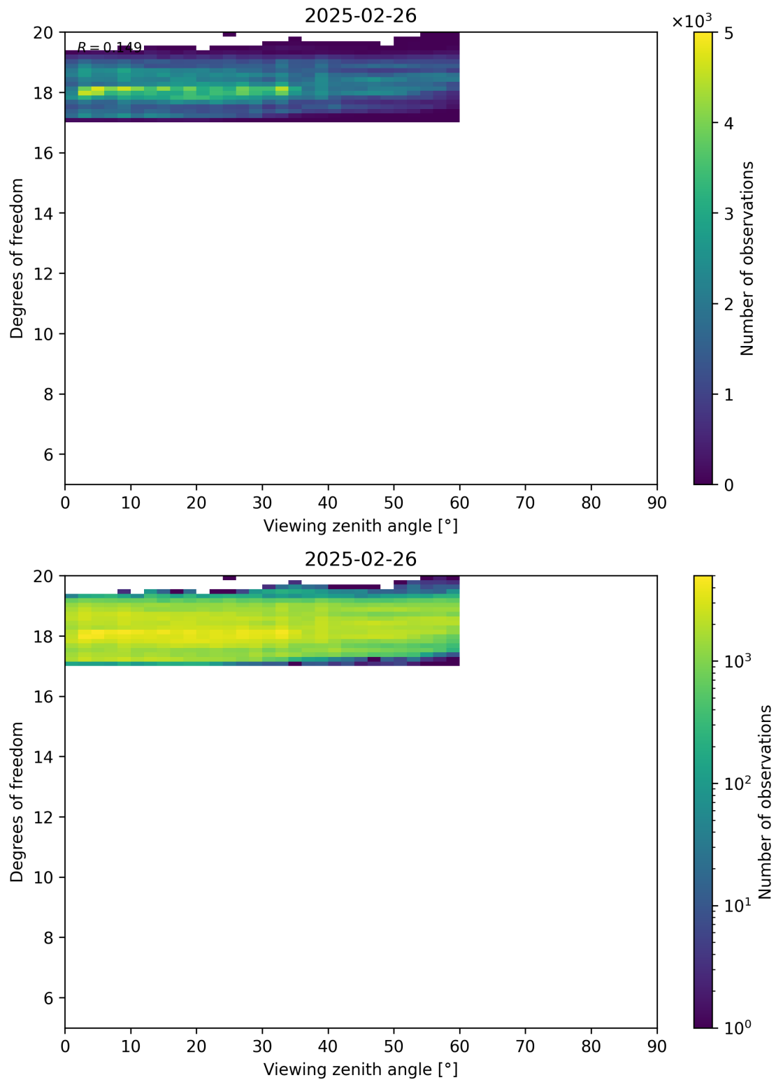
Figure 107: Scatter density plot of “Viewing zenith angle” against “Degrees of freedom” for 2025-02-25 to 2025-02-27.
