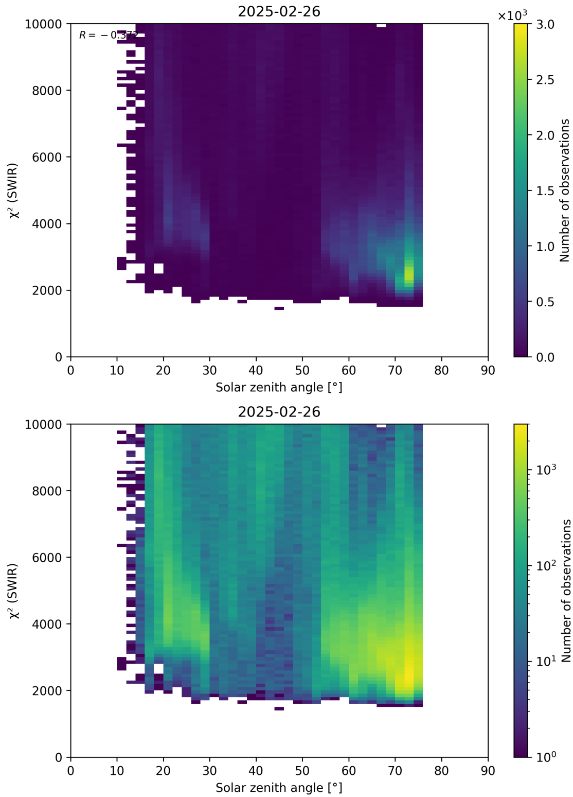
Figure 95: Scatter density plot of “Solar zenith angle” against “ \chi^2 (SWIR)” for 2025-02-25 to 2025-02-27.
