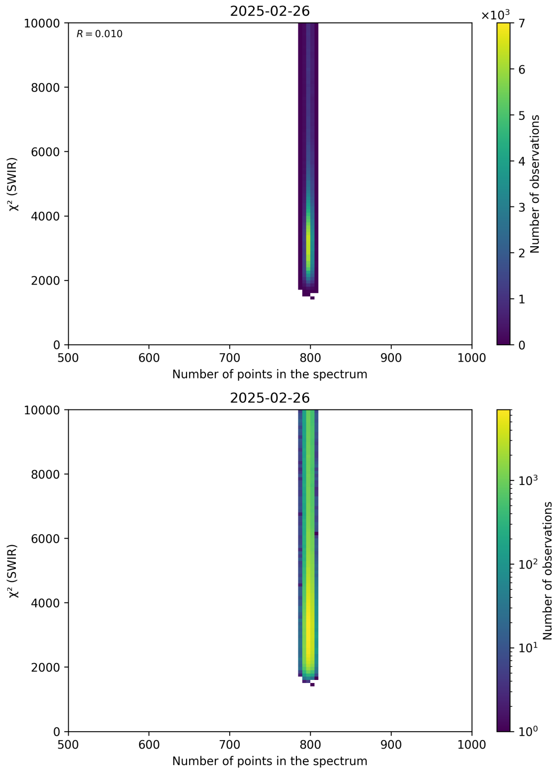
Figure 89: Scatter density plot of “Number of points in the spectrum” against “ \chi^2 (SWIR)” for 2025-02-25 to 2025-02-27.
