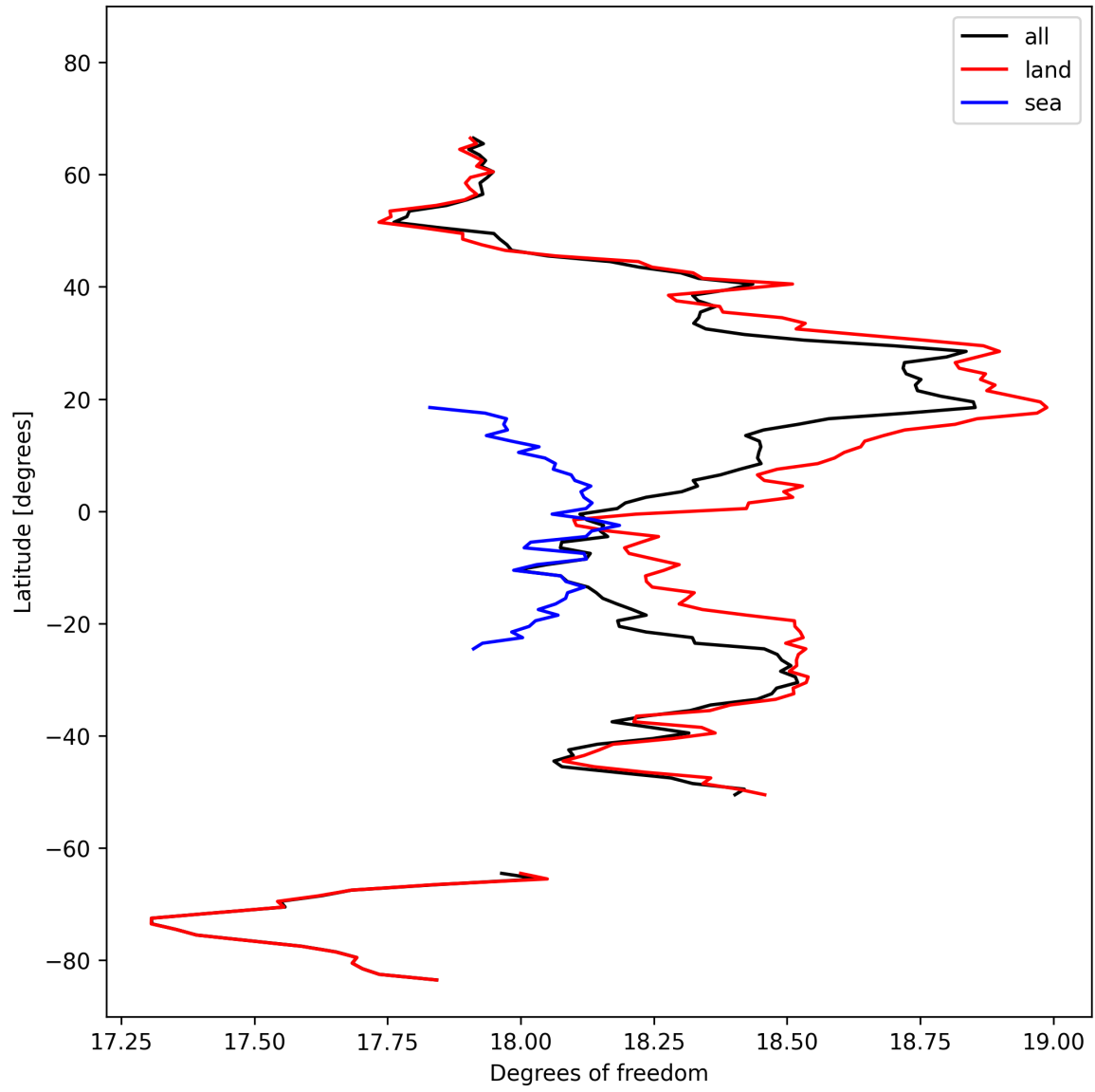
Figure 19: Zonal average of “Degrees of freedom” for 2025-02-25 to 2025-02-27.
