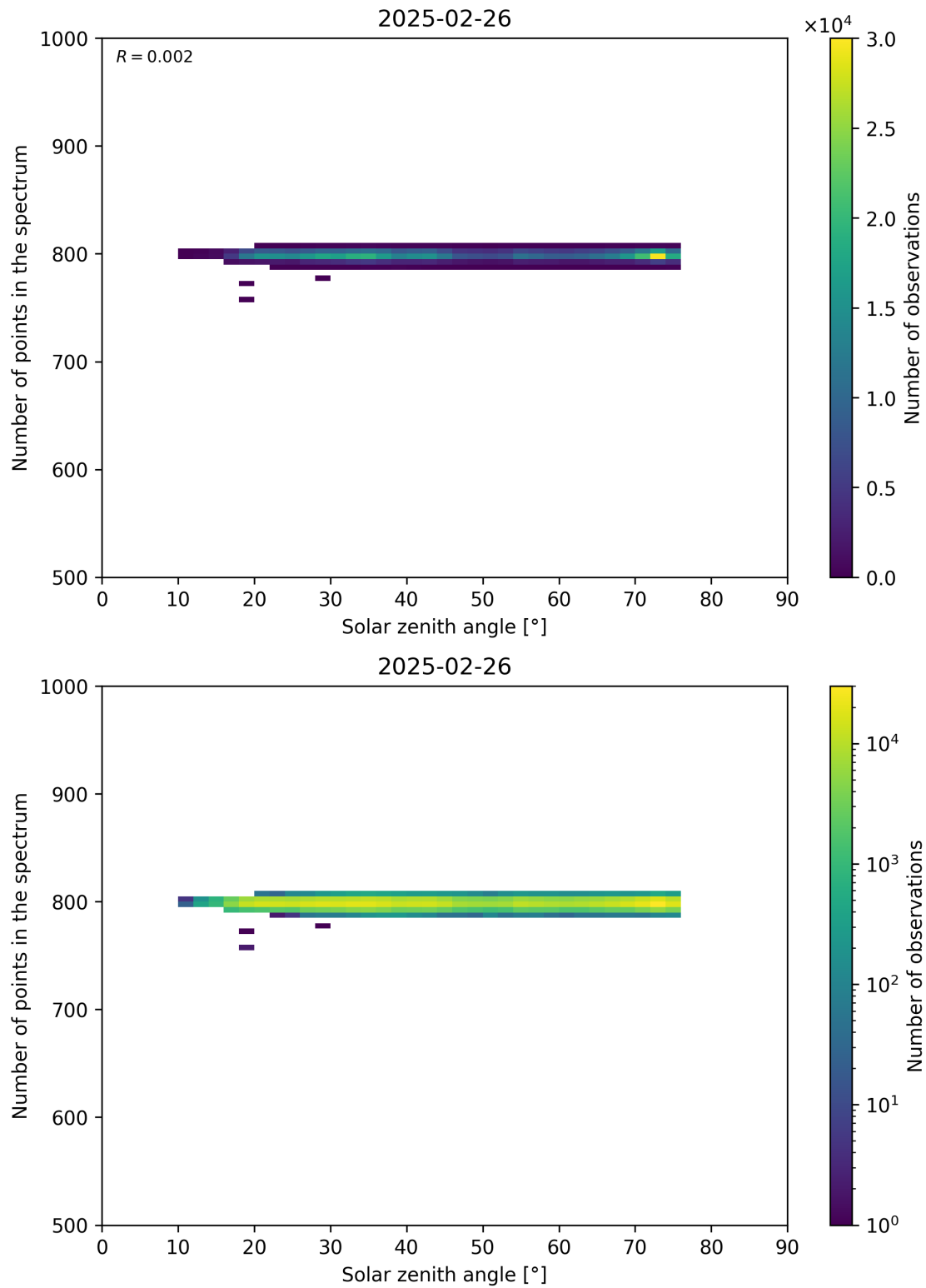
Figure 103: Scatter density plot of “Solar zenith angle” against “Number of points in the spectrum” for 2025-02-25 to 2025-02-27.
