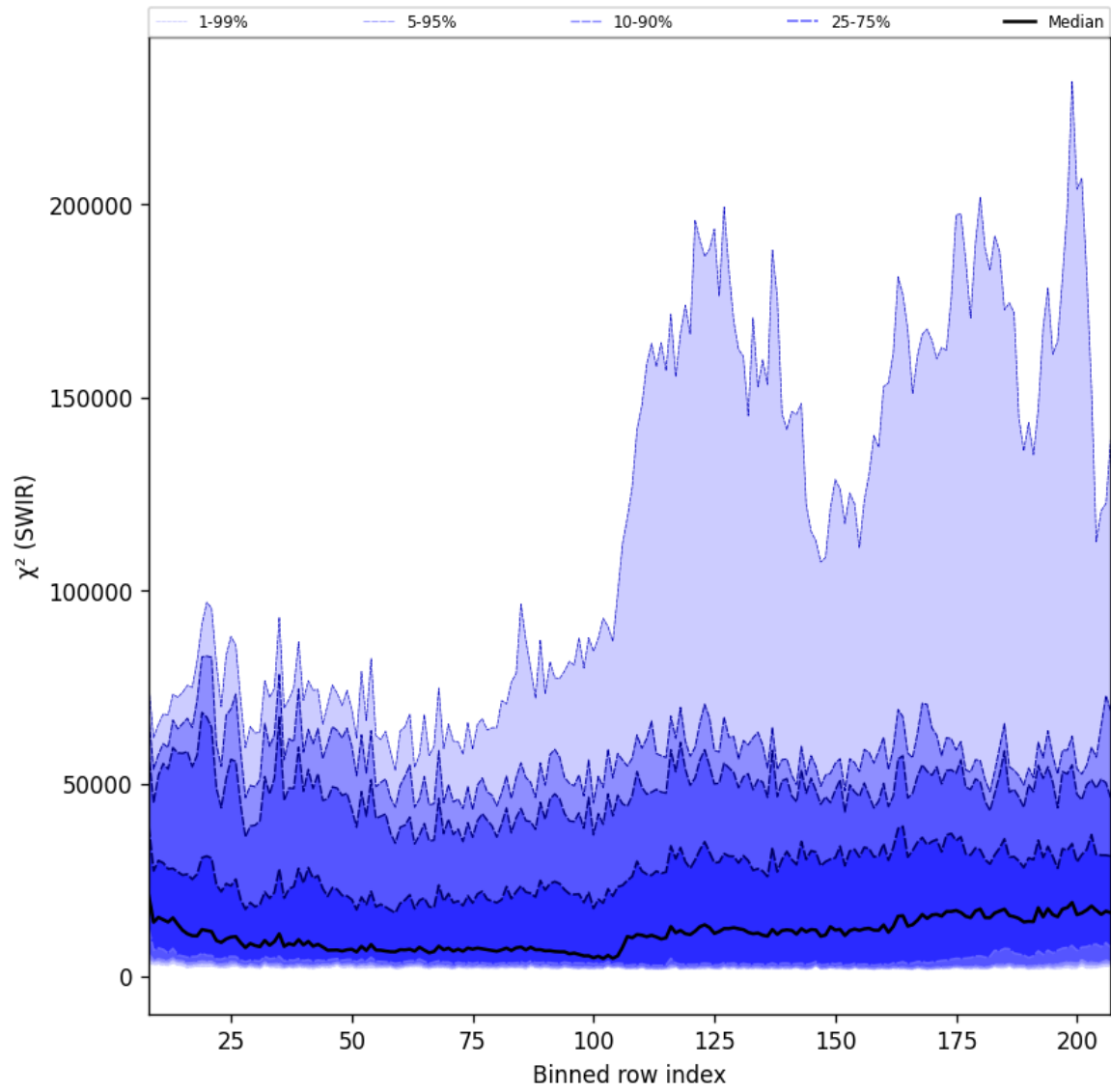
Figure 39: Along track statistics of “ \chi^2 (SWIR)” for 2025-02-25 to 2025-02-27
