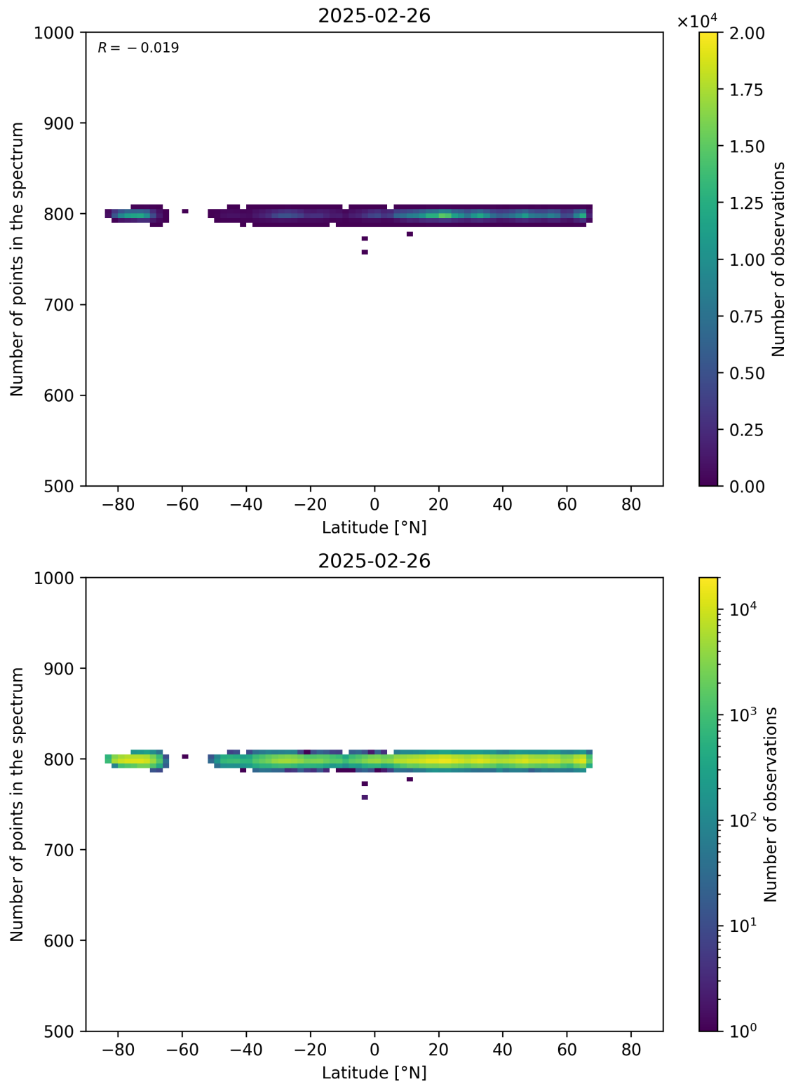
Figure 61: Scatter density plot of “Latitude” against “Number of points in the spectrum” for 2025-02-25 to 2025-02-27.
