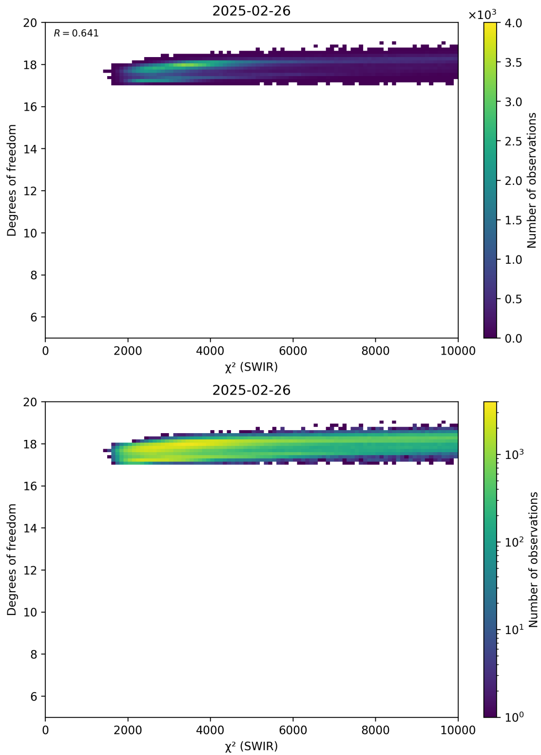
Figure 48: Scatter density plot of “ \chi^2 (SWIR)” against “Degrees of freedom” for 2025-02-25 to 2025-02-27.
