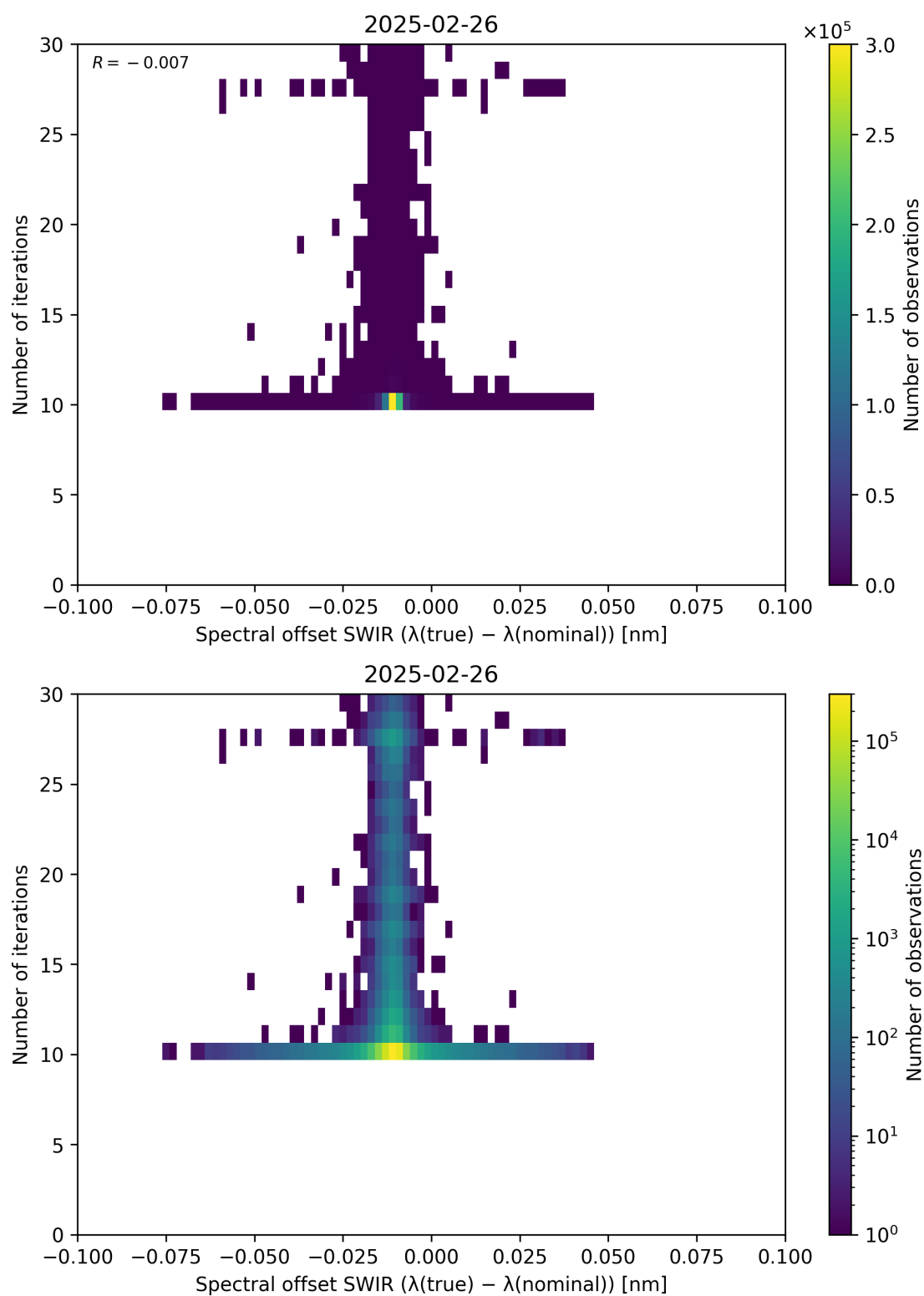
Figure 121: Scatter density plot of “Spectral offset SWIR ( \lambda_{\text{true}} - \lambda_{\text{nominal}} )” against “Number of iterations” for 2025-02-25 to 2025-02-27.
