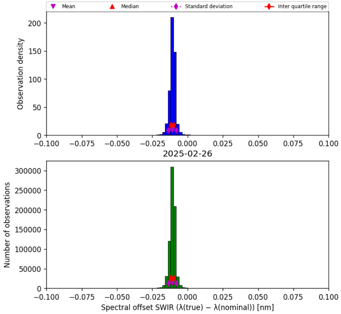
Figure 27: Histogram of “Spectral offset SWIR ( \lambda_{\text{true}} - \lambda_{\text{nominal}} )” for 2025-02-25 to 2025-02-27
