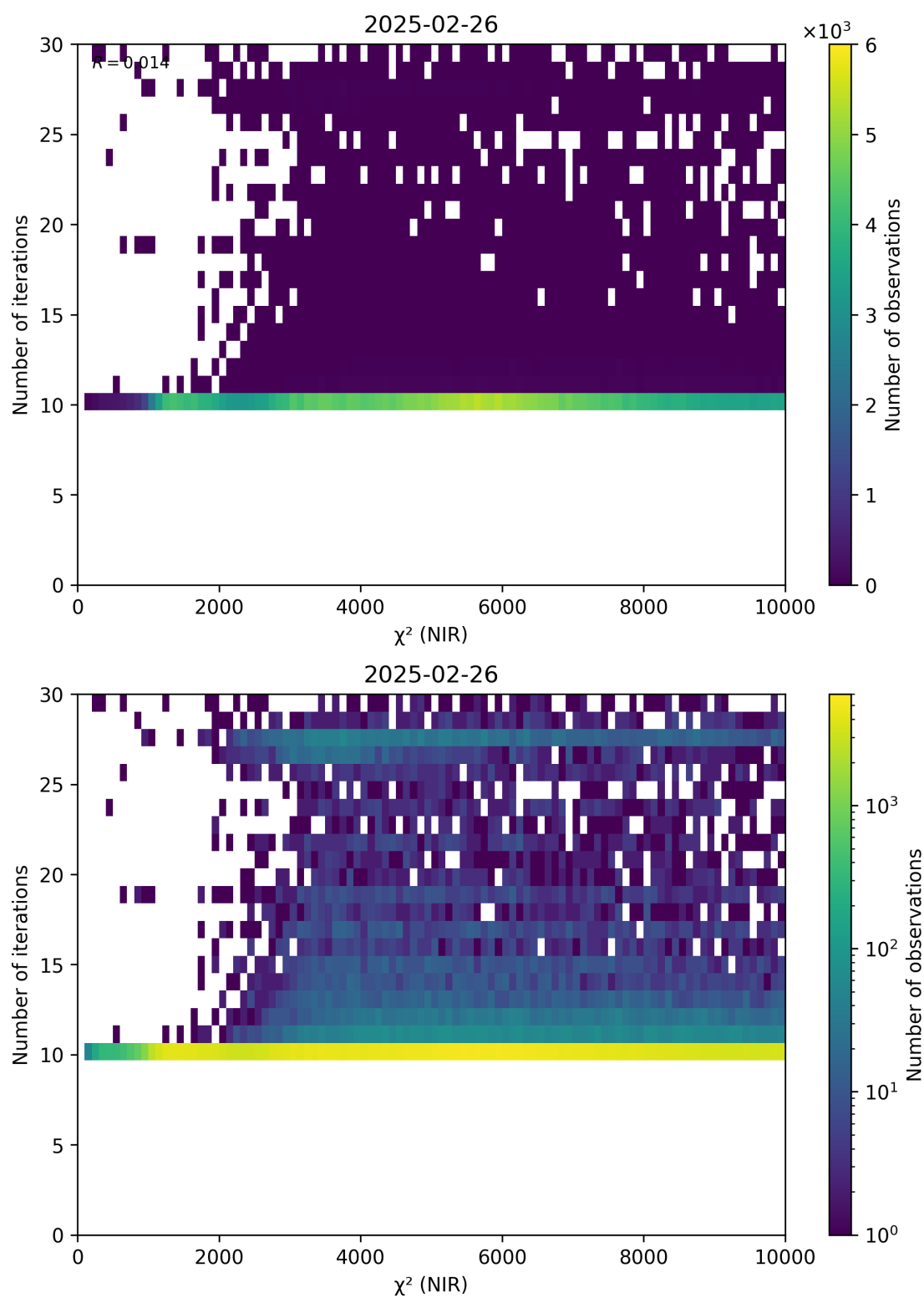
Figure 46: Scatter density plot of “ \chi^2 (NIR)” against “Number of iterations” for 2025-02-25 to 2025-02-27.
