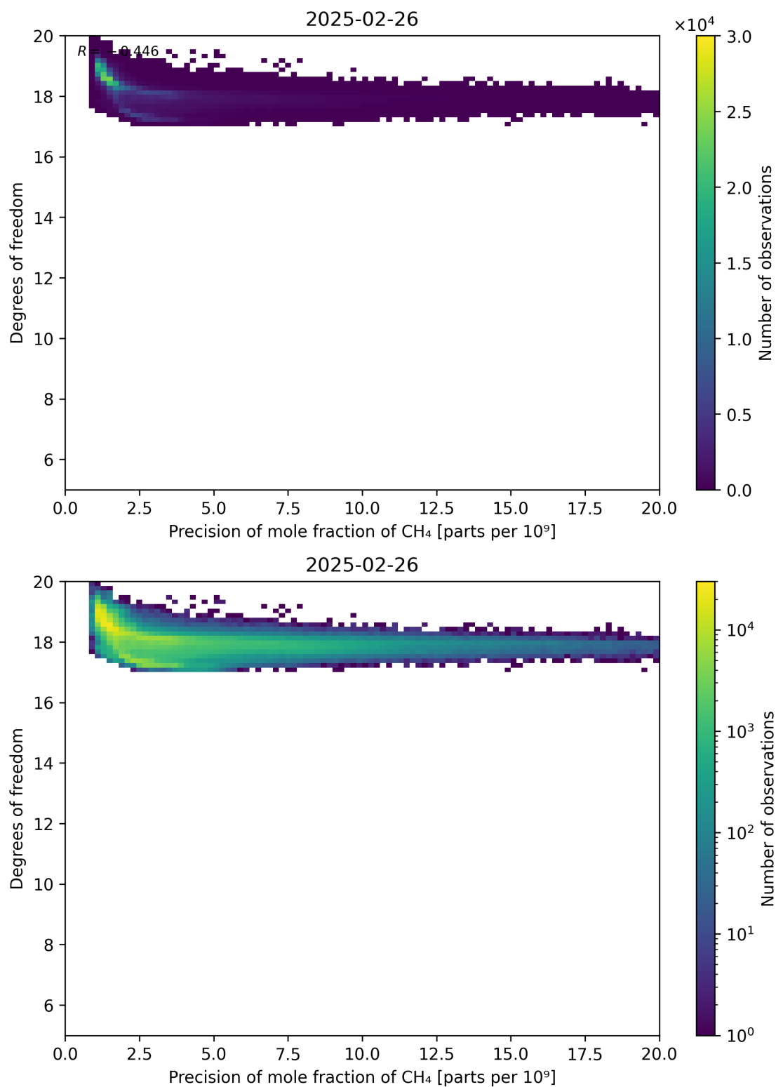
Figure 80: Scatter density plot of “Precision of mole fraction of CH 4 ” against “Degrees of freedom” for 2025-02-25 to 2025-02-27.
