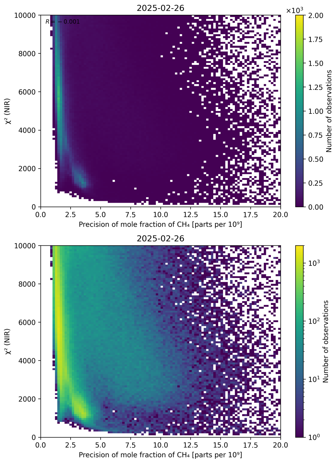
Figure 78: Scatter density plot of “Precision of mole fraction of CH 4 ” against “ \chi^2 (NIR)” for 2025-02-25 to 2025-02-27.
