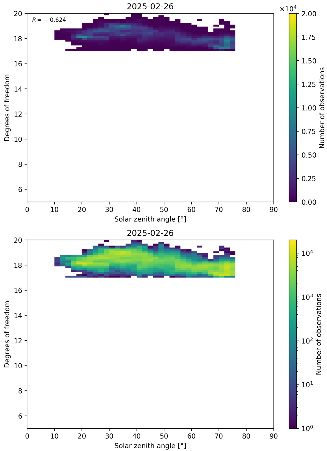
Figure 96: Scatter density plot of “Solar zenith angle” against “Degrees of freedom” for 2025-02-25 to 2025-02-27.
