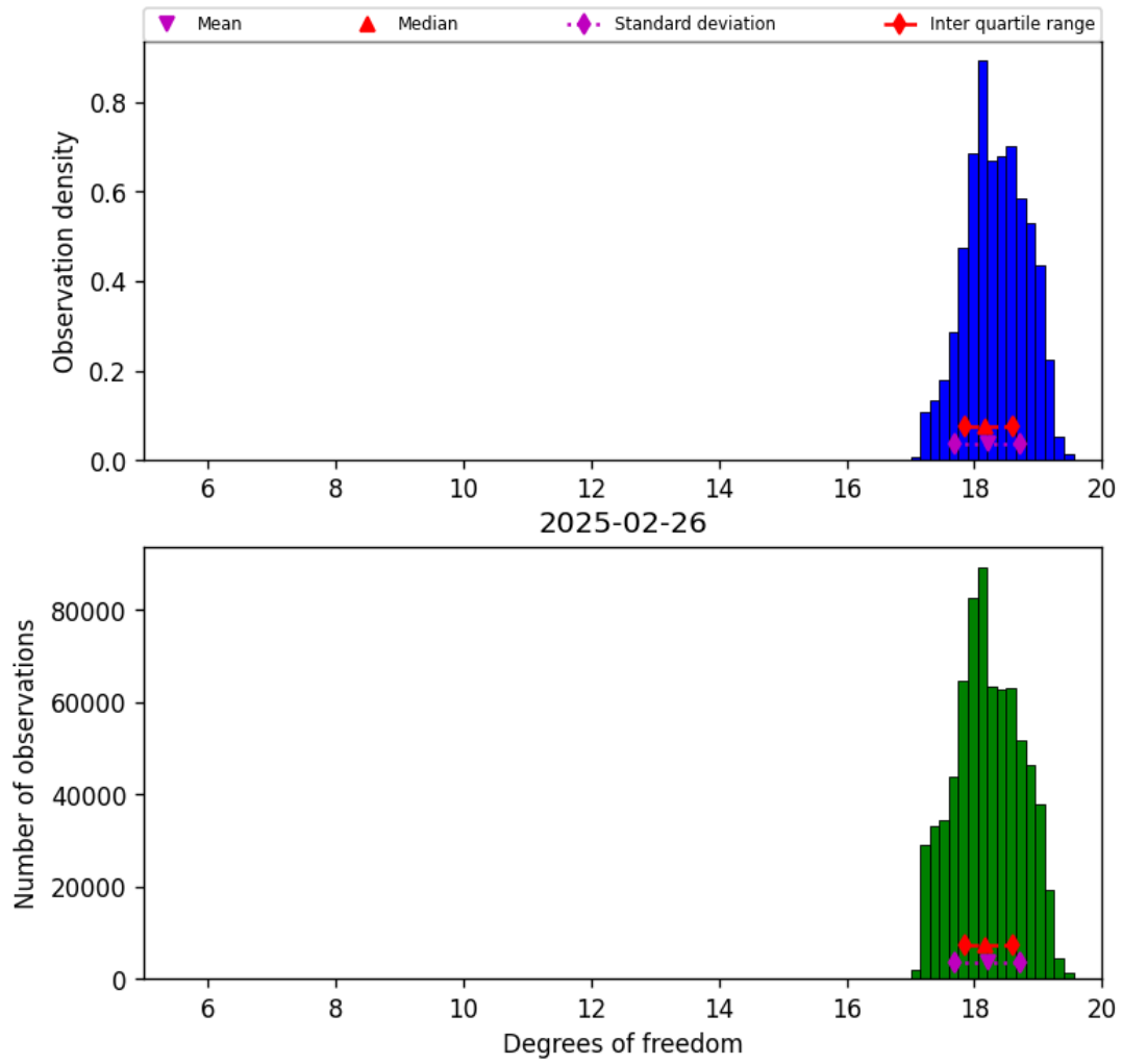
Figure 30: Histogram of “Degrees of freedom” for 2025-02-25 to 2025-02-27
