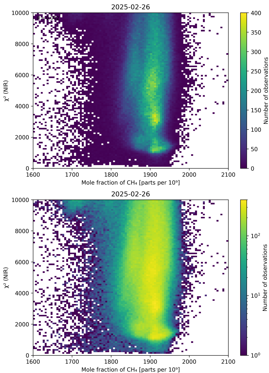
Figure 70: Scatter density plot of “Mole fraction of CH 4 ” against “ \chi^2 (NIR)” for 2025-02-25 to 2025-02-27.
