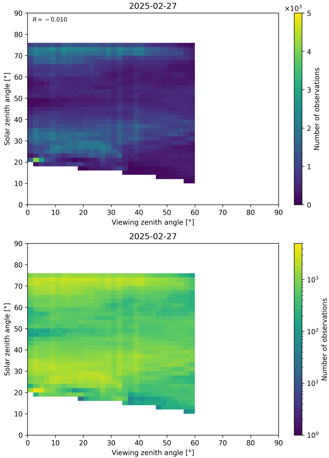
Figure 115: Scatter density plot of “Viewing zenith angle” against “Solar zenith angle” for 2025-02-26 to 2025-02-28.
