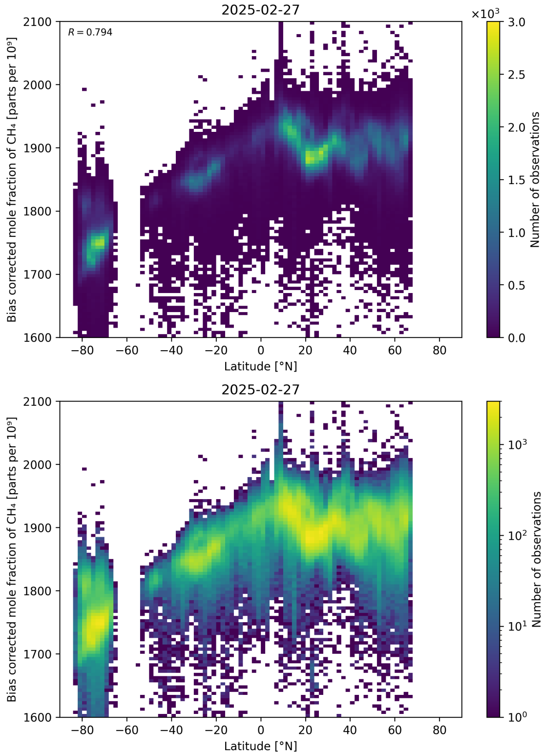
Figure 58: Scatter density plot of “Latitude” against “Bias corrected mole fraction of \text{CH}_4 ” for 2025-02-26 to 2025-02-28.
