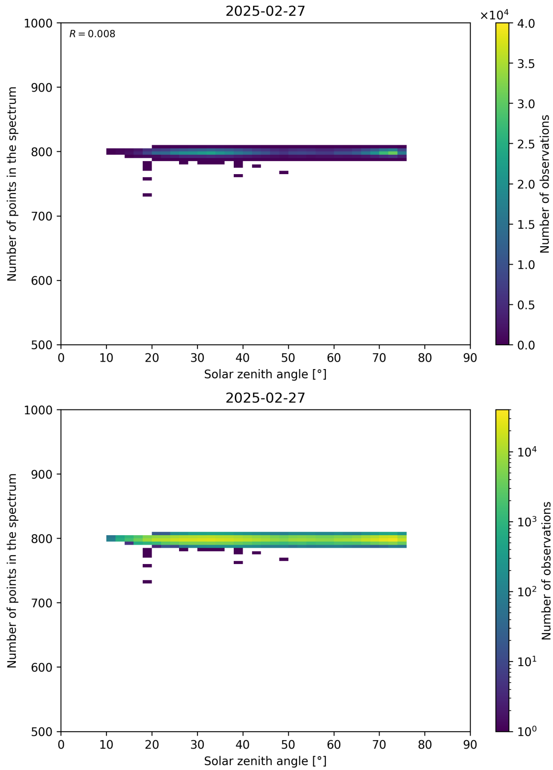
Figure 103: Scatter density plot of “Solar zenith angle” against “Number of points in the spectrum” for 2025-02-26 to 2025-02-28.
