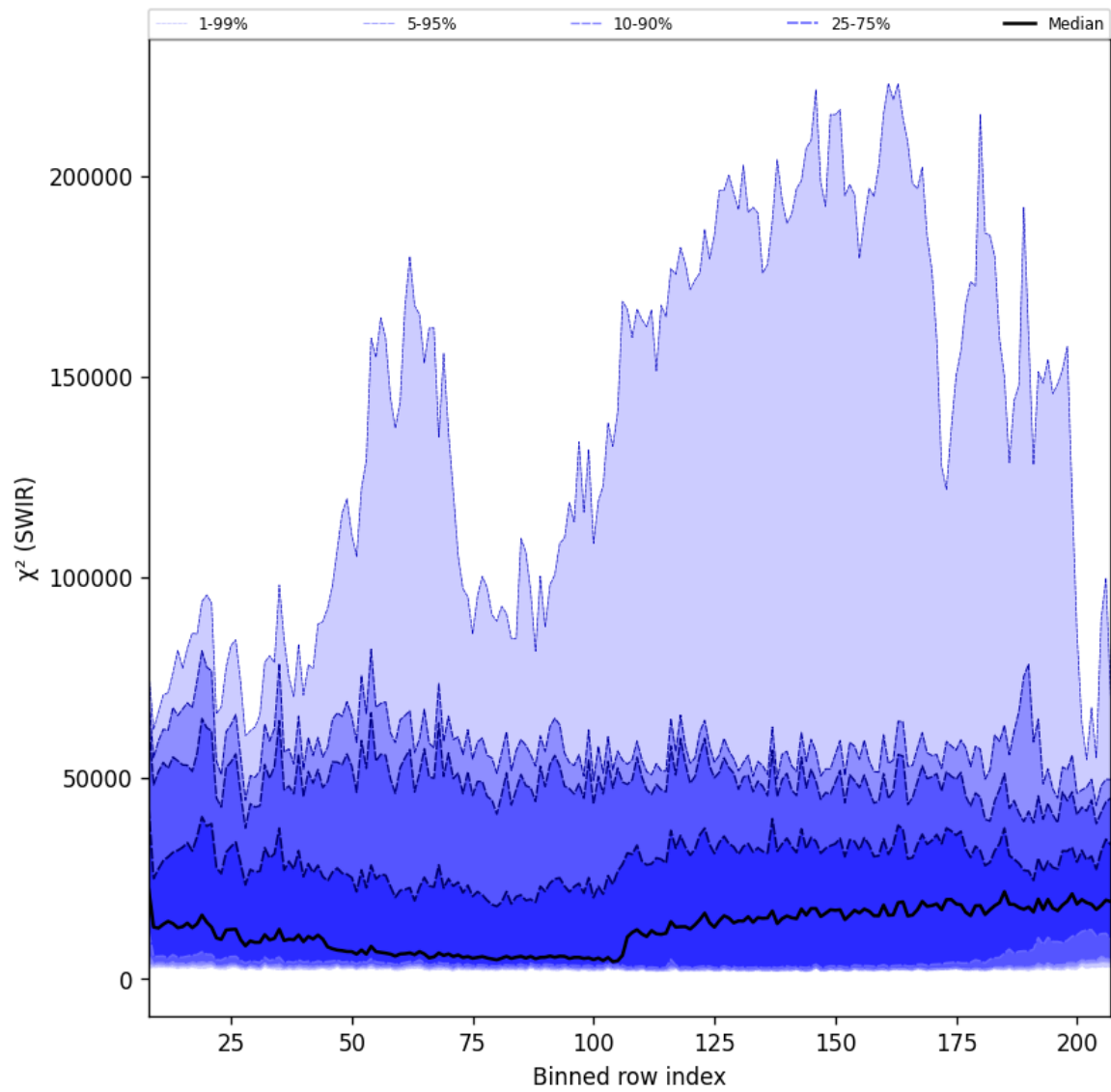
Figure 39: Along track statistics of “ \chi^2 (SWIR)” for 2025-02-26 to 2025-02-28
