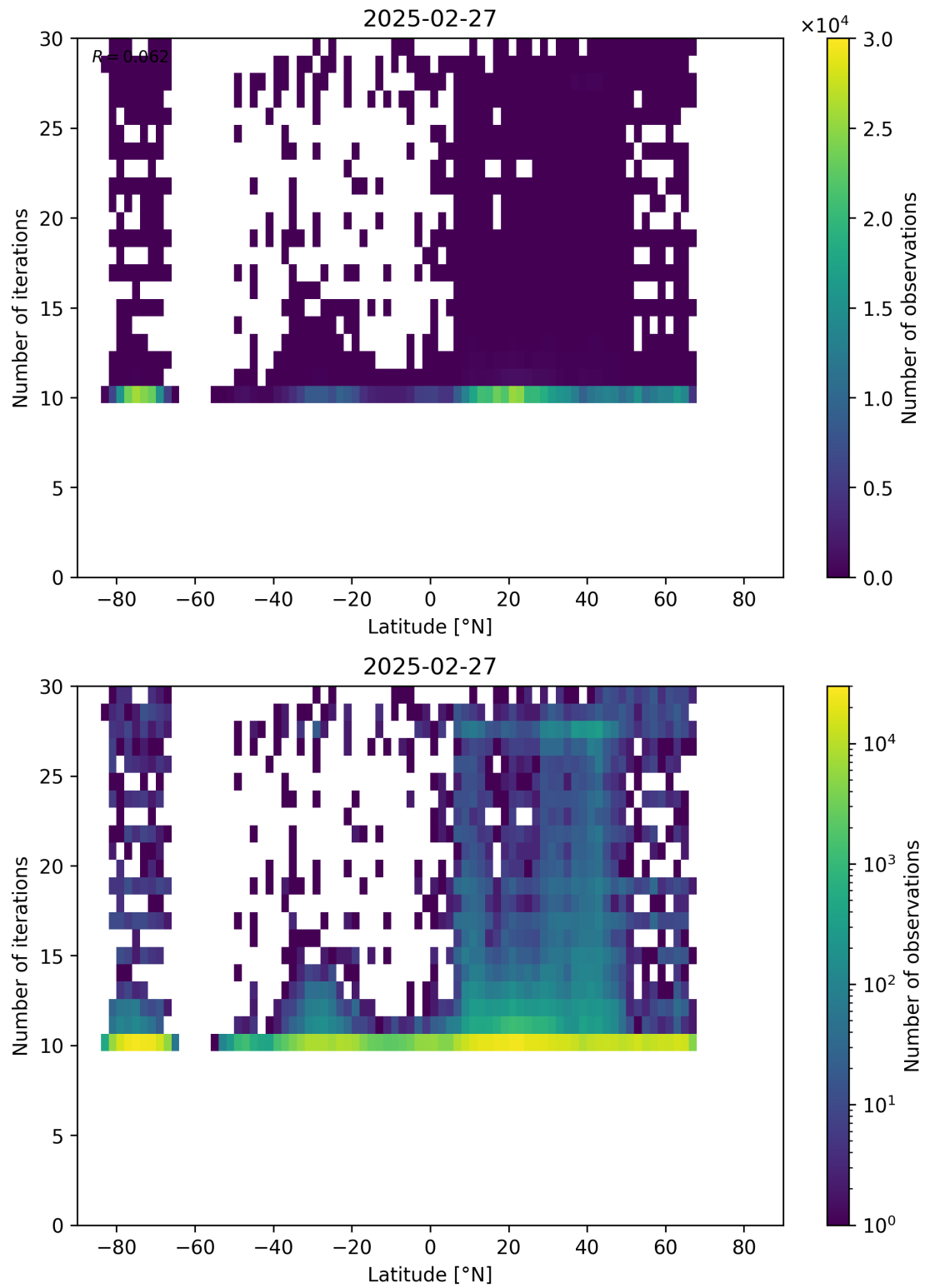
Figure 60: Scatter density plot of “Latitude” against “Number of iterations” for 2025-02-26 to 2025-02-28.
