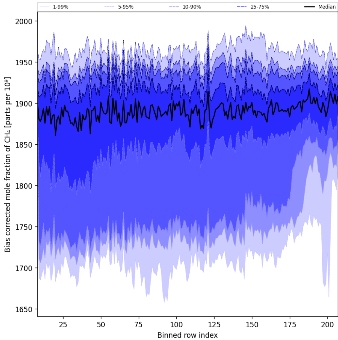
Figure 36: Along track statistics of “Bias corrected mole fraction of CH 4 ” for 2025-02-26 to 2025-02-28
