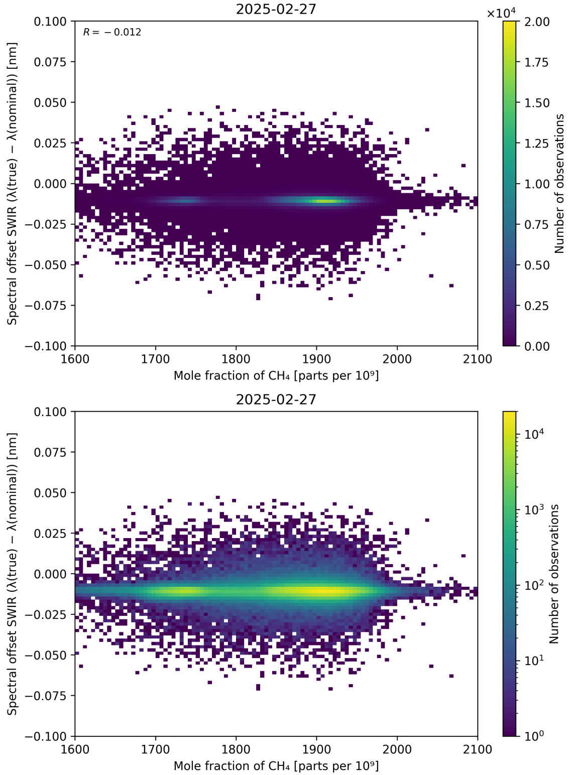
Figure 86: Scatter density plot of “Mole fraction of CH 4 ” against “Spectral offset SWIR ( \lambda_{\text{true}} - \lambda_{\text{nominal}} )” for 2025-02-26 to 2025-02-28.
