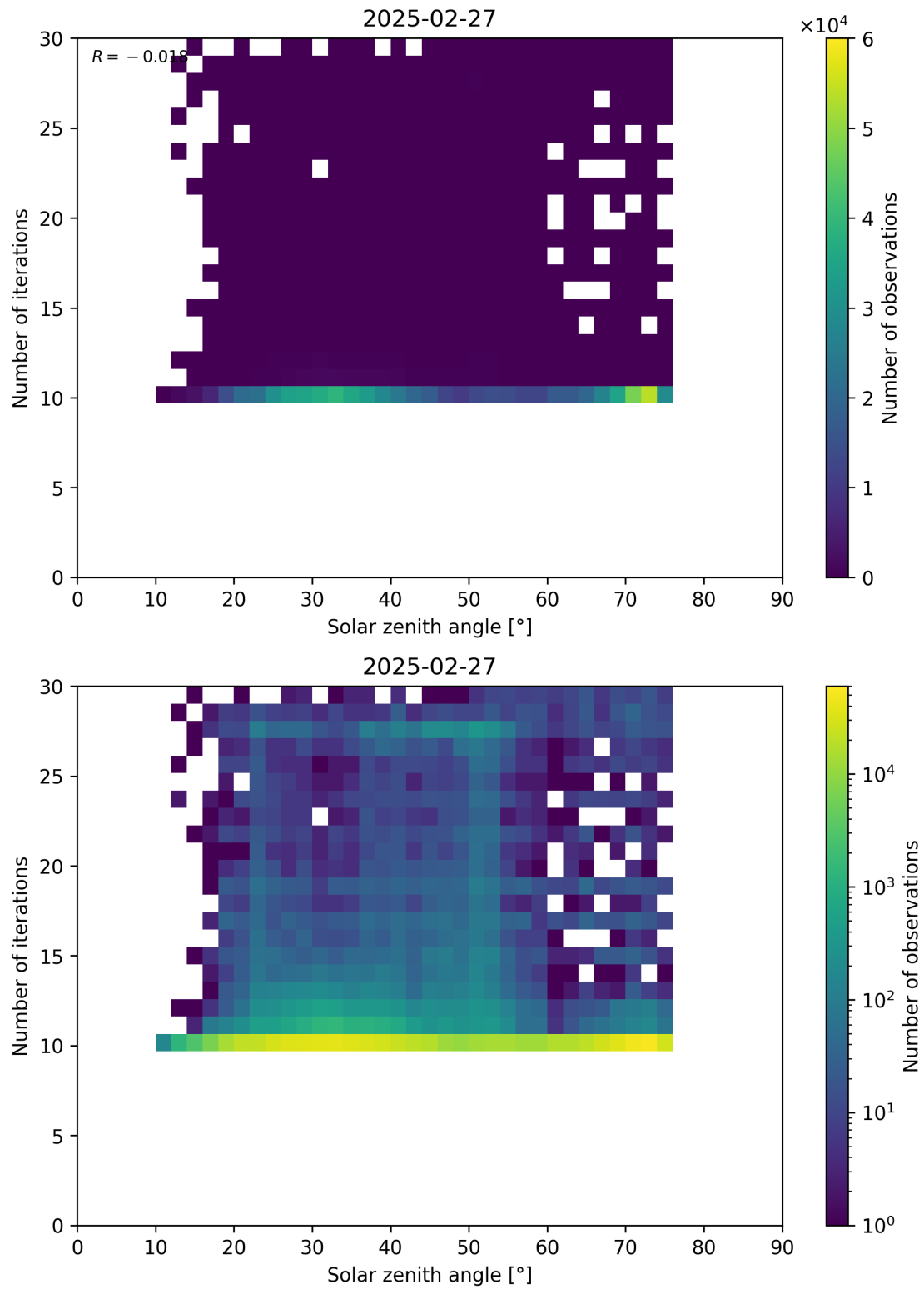
Figure 102: Scatter density plot of “Solar zenith angle” against “Number of iterations” for 2025-02-26 to 2025-02-28.
