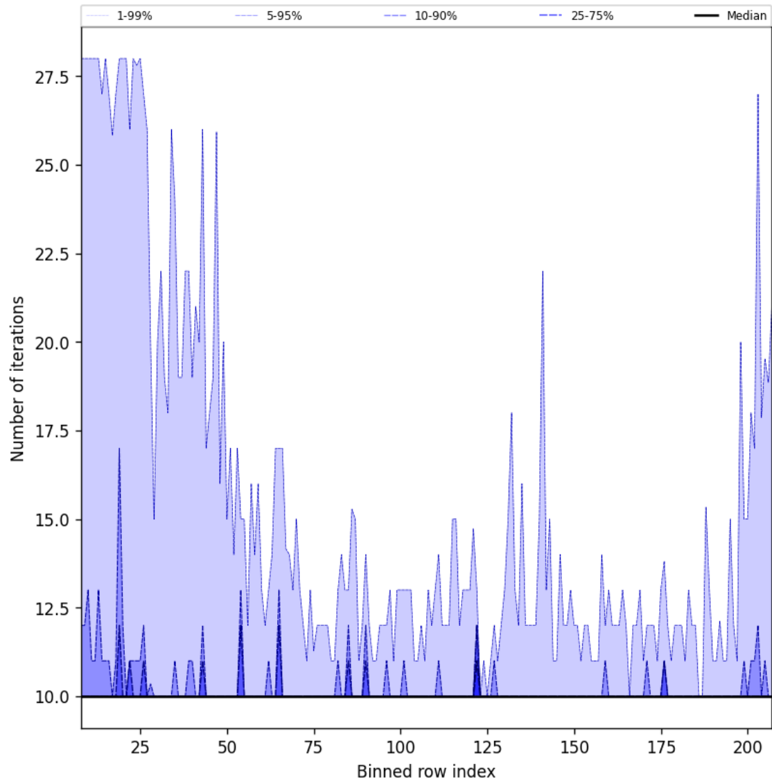
Figure 42: Along track statistics of “Number of iterations” for 2025-02-26 to 2025-02-28
