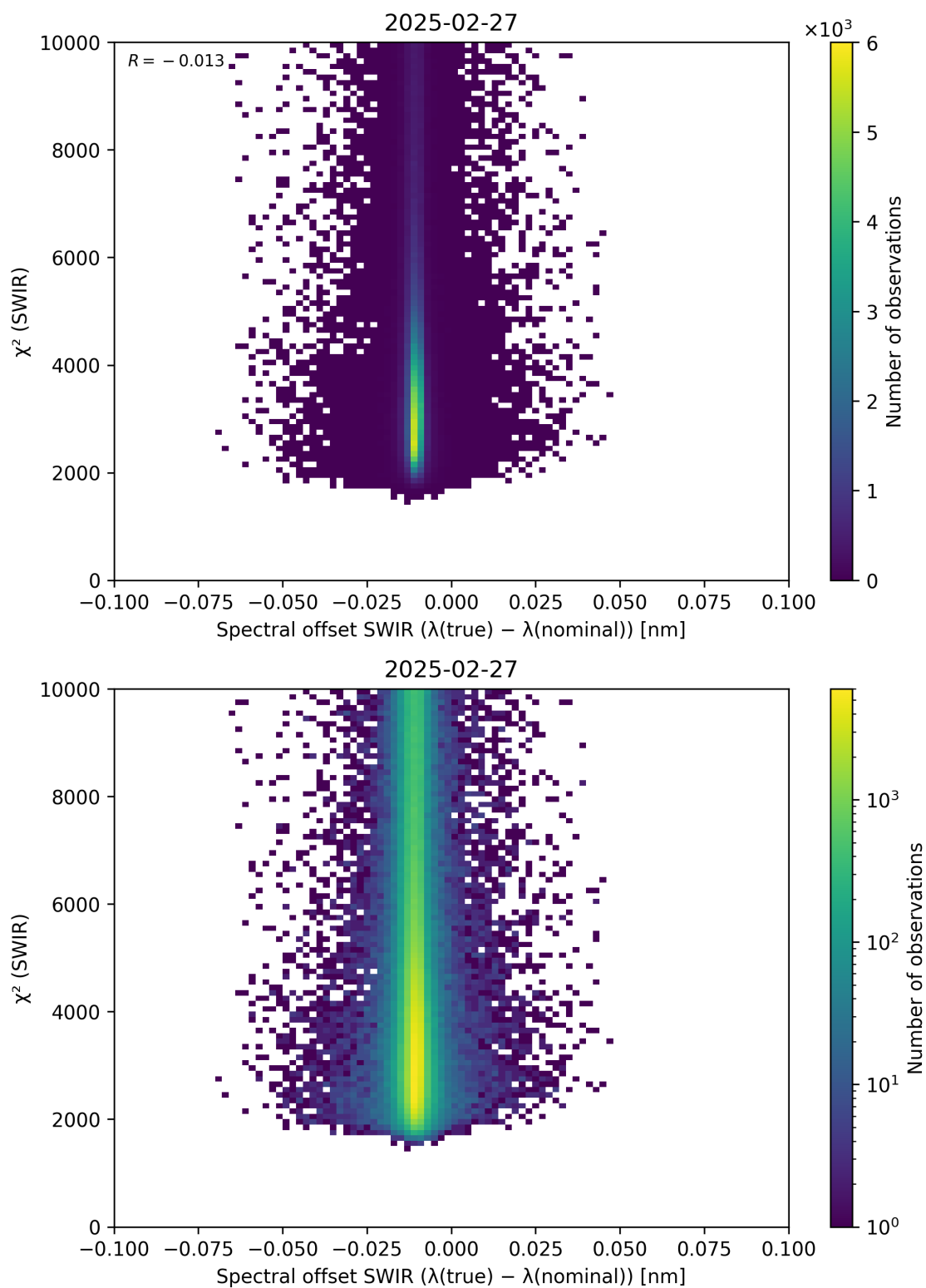
Figure 118: Scatter density plot of “Spectral offset SWIR ( \lambda_{\text{true}} - \lambda_{\text{nominal}} )” against “ \chi^2 (SWIR)” for 2025-02-26 to 2025-02-28.
