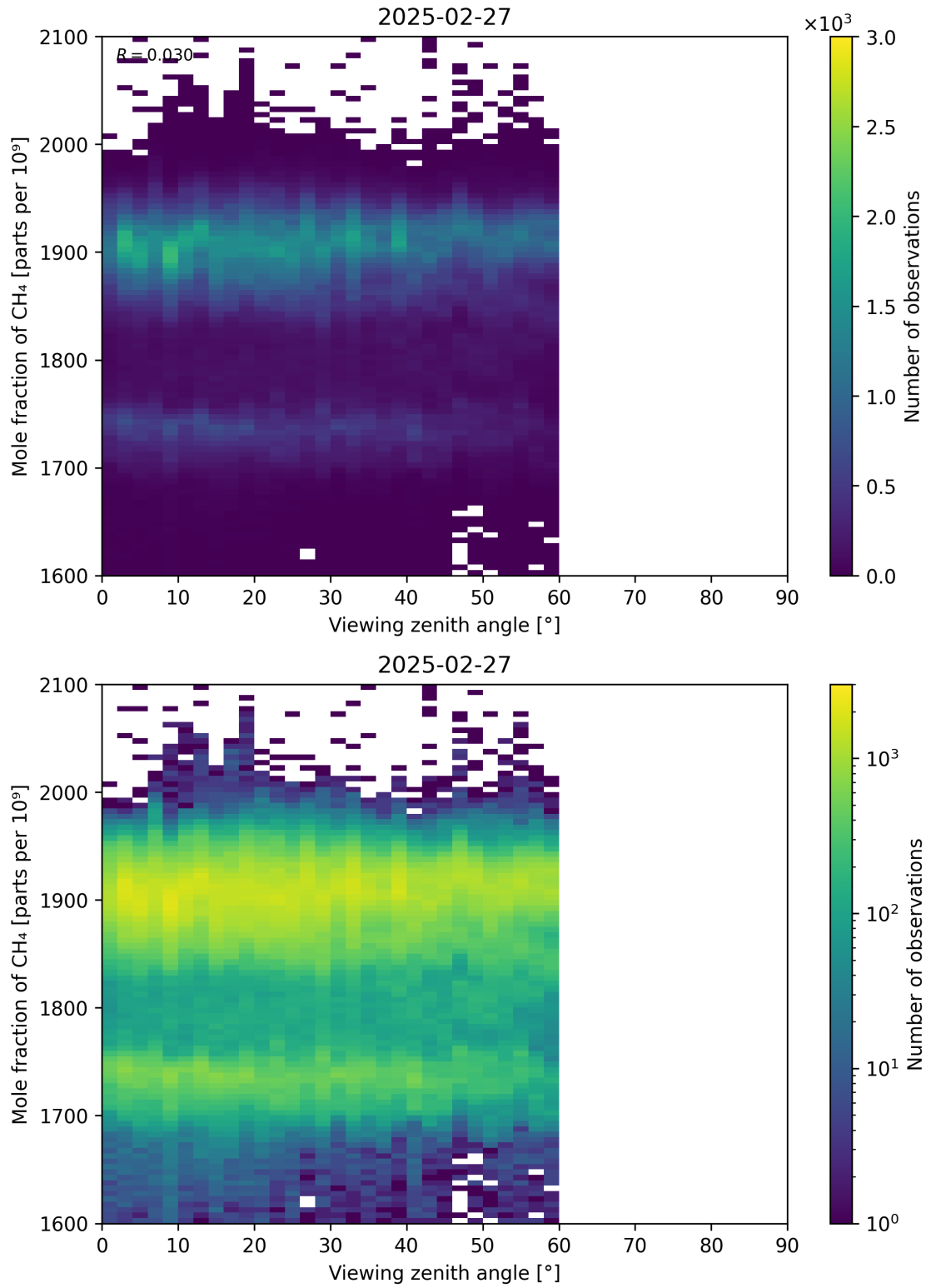
Figure 110: Scatter density plot of “Viewing zenith angle” against “Mole fraction of CH 4 ” for 2025-02-26 to 2025-02-28.
