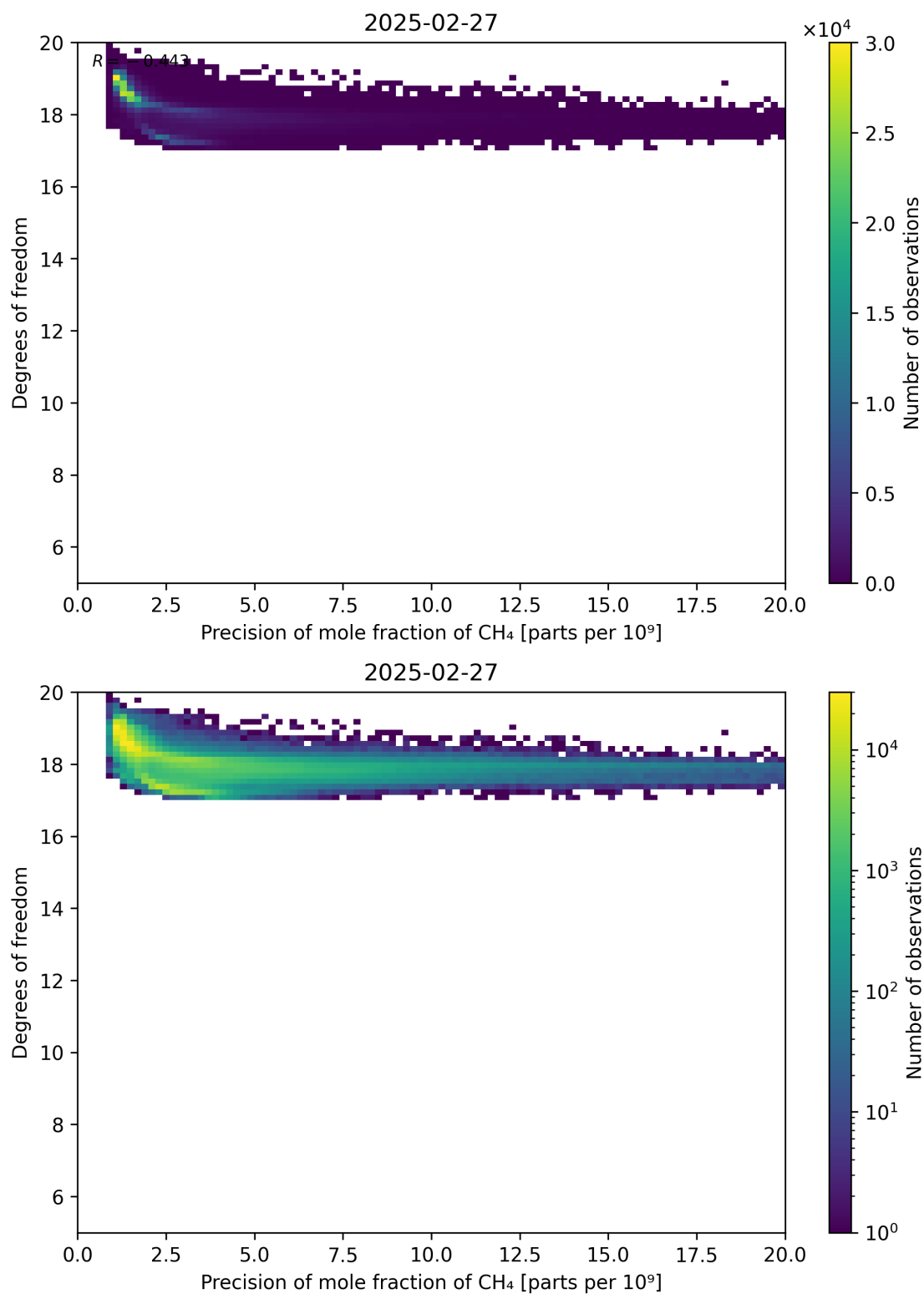
Figure 80: Scatter density plot of “Precision of mole fraction of CH 4 ” against “Degrees of freedom” for 2025-02-26 to 2025-02-28.
