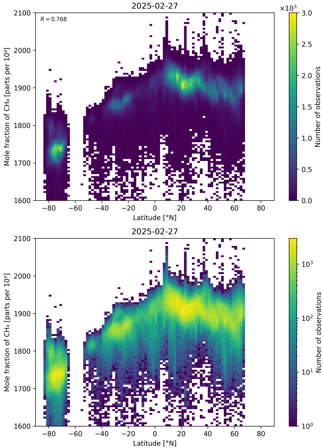
Figure 57: Scatter density plot of “Latitude” against “Mole fraction of CH 4 ” for 2025-02-26 to 2025-02-28.
