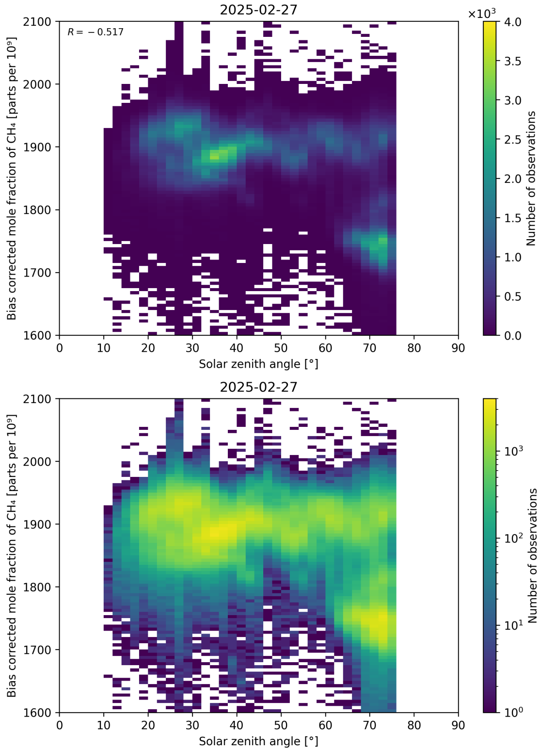
Figure 100: Scatter density plot of “Solar zenith angle” against “Bias corrected mole fraction of CH 4 ” for 2025-02-26 to 2025-02-28.
