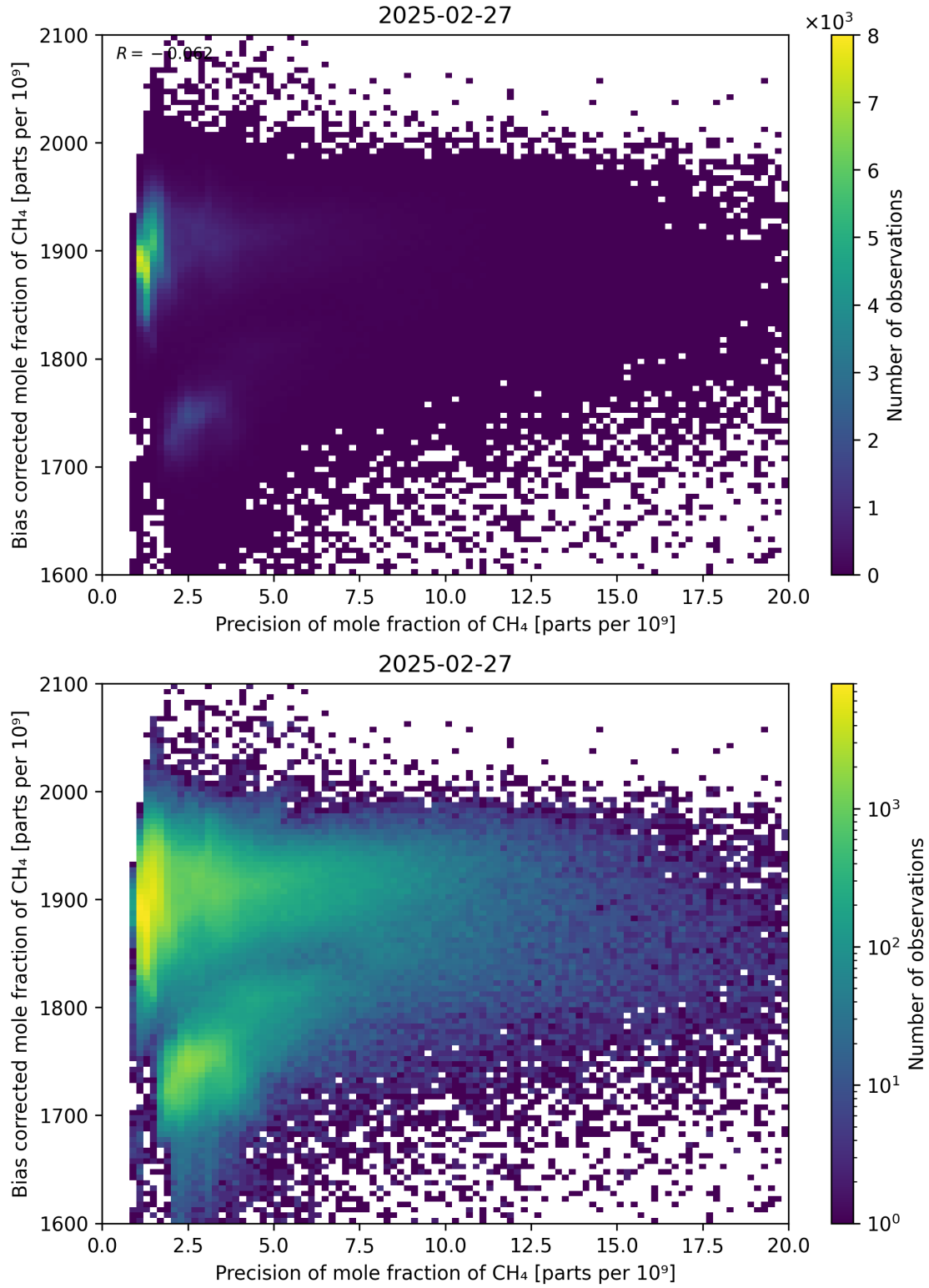
Figure 82: Scatter density plot of “Precision of mole fraction of CH 4 ” against “Bias corrected mole fraction of CH 4 ” for 2025-02-26 to 2025-02-28.
