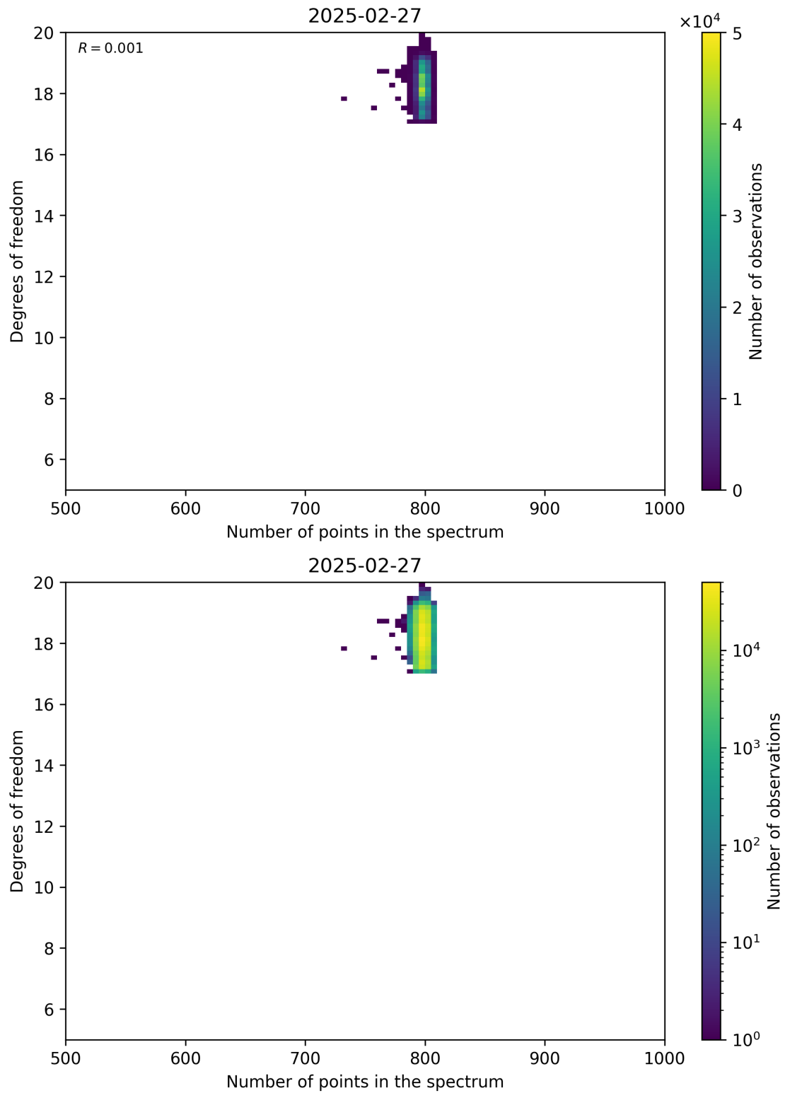
Figure 90: Scatter density plot of “Number of points in the spectrum” against “Degrees of freedom” for 2025-02-26 to 2025-02-28.
