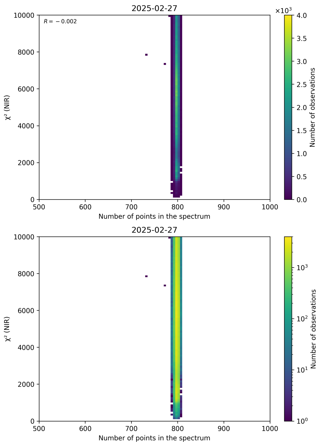
Figure 88: Scatter density plot of “Number of points in the spectrum” against “ \chi^2 (NIR)” for 2025-02-26 to 2025-02-28.
