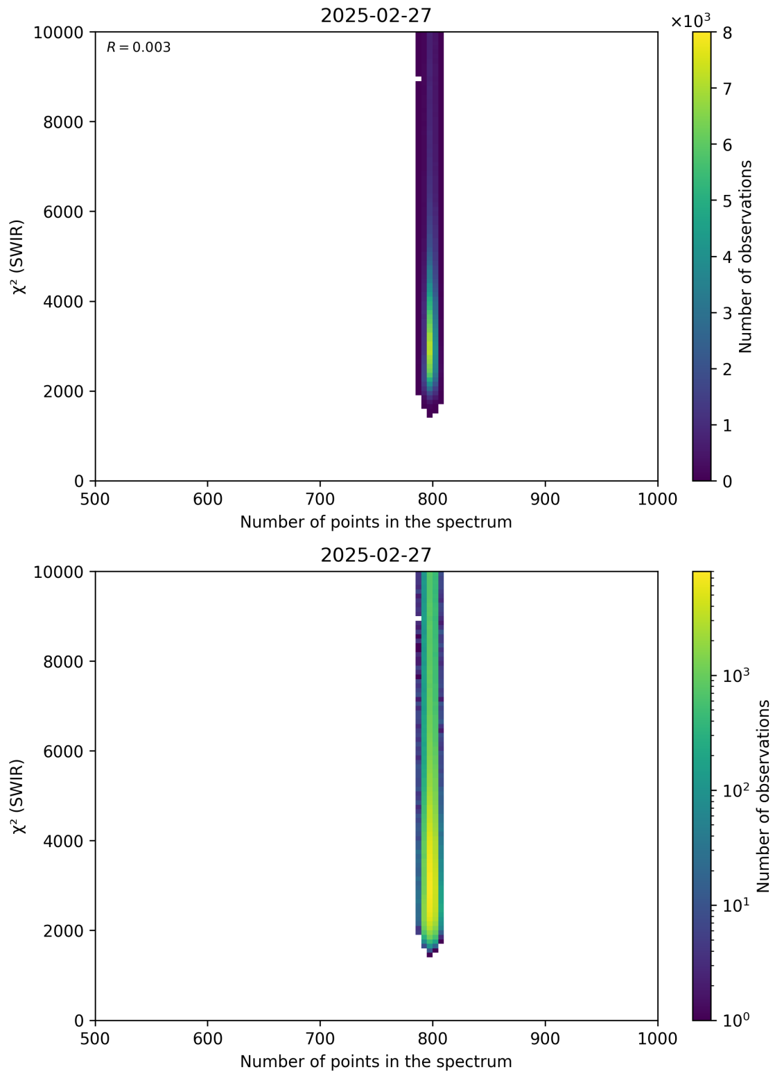
Figure 89: Scatter density plot of “Number of points in the spectrum” against “ \chi^2 (SWIR)” for 2025-02-26 to 2025-02-28.
