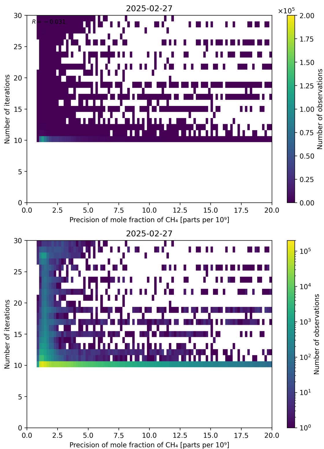
Figure 83: Scatter density plot of “Precision of mole fraction of CH 4 ” against “Number of iterations” for 2025-02-26 to 2025-02-28.
