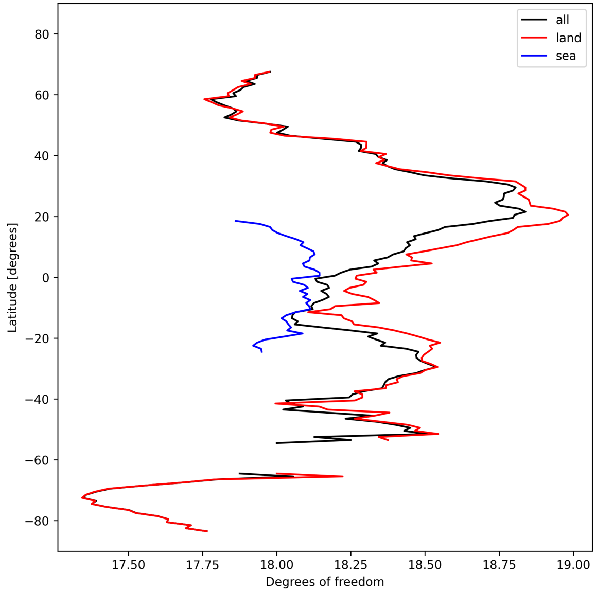
Figure 19: Zonal average of “Degrees of freedom” for 2025-02-26 to 2025-02-28.
