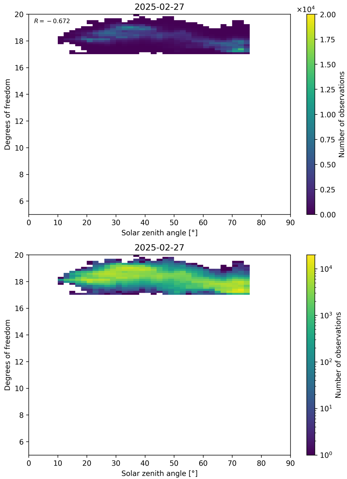
Figure 96: Scatter density plot of “Solar zenith angle” against “Degrees of freedom” for 2025-02-26 to 2025-02-28.
