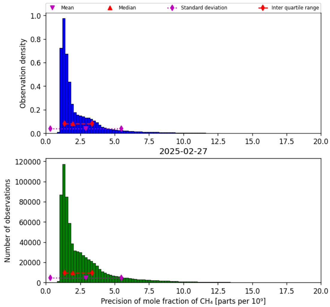
Figure 24: Histogram of “Precision of mole fraction of CH 4 ” for 2025-02-26 to 2025-02-28
