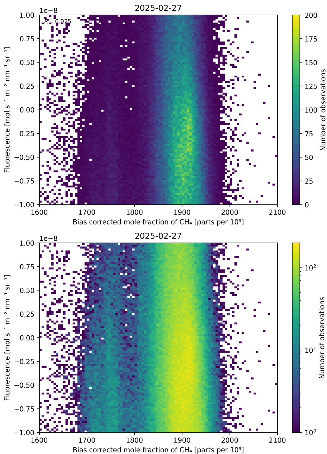
Figure 66: Scatter density plot of “Bias corrected mole fraction of \text{CH}_4 ” against “Fluorescence” for 2025-02-26 to 2025-02-28.
