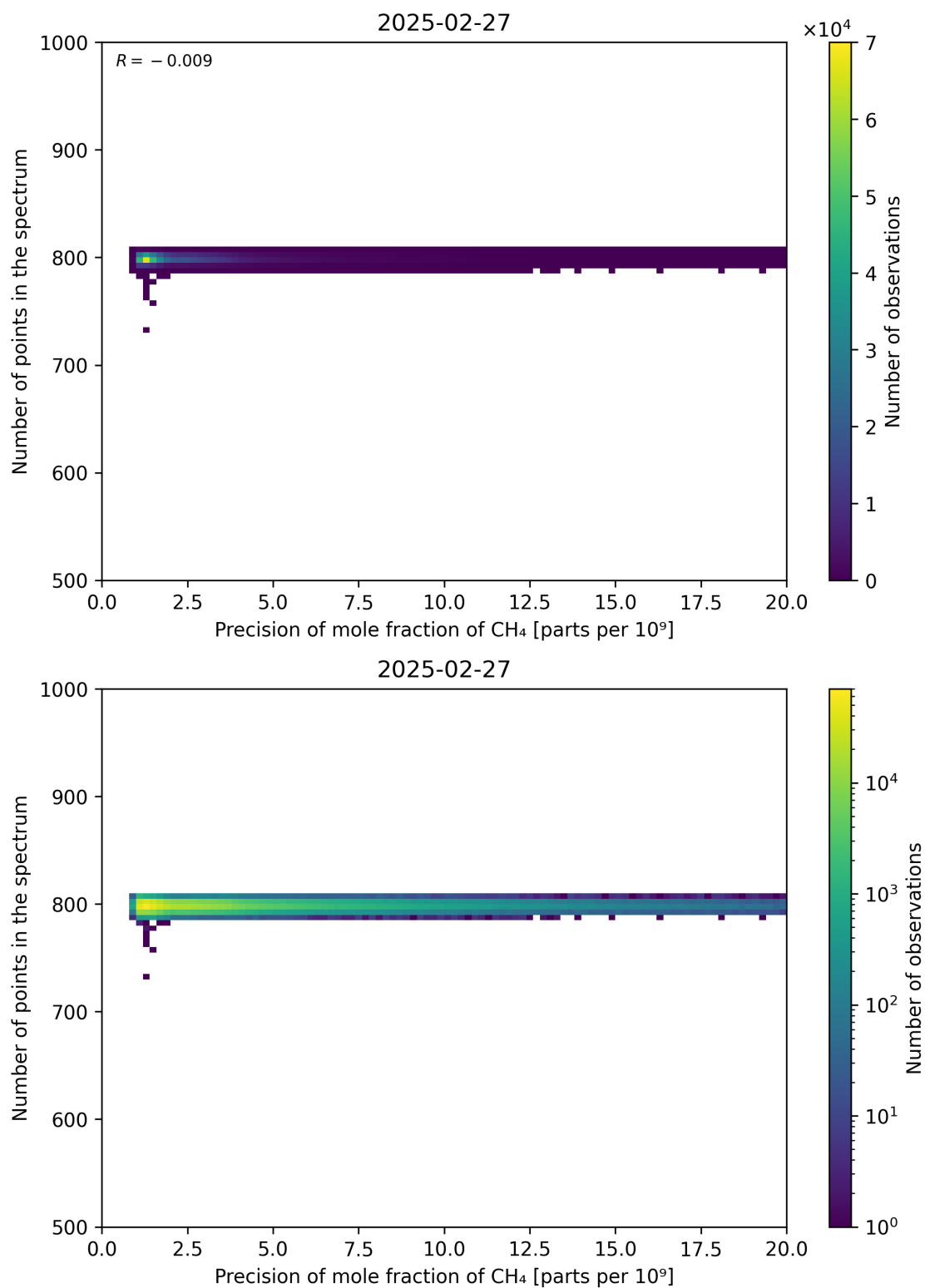
Figure 84: Scatter density plot of “Precision of mole fraction of CH 4 ” against “Number of points in the spectrum” for 2025-02-26 to 2025-02-28.
