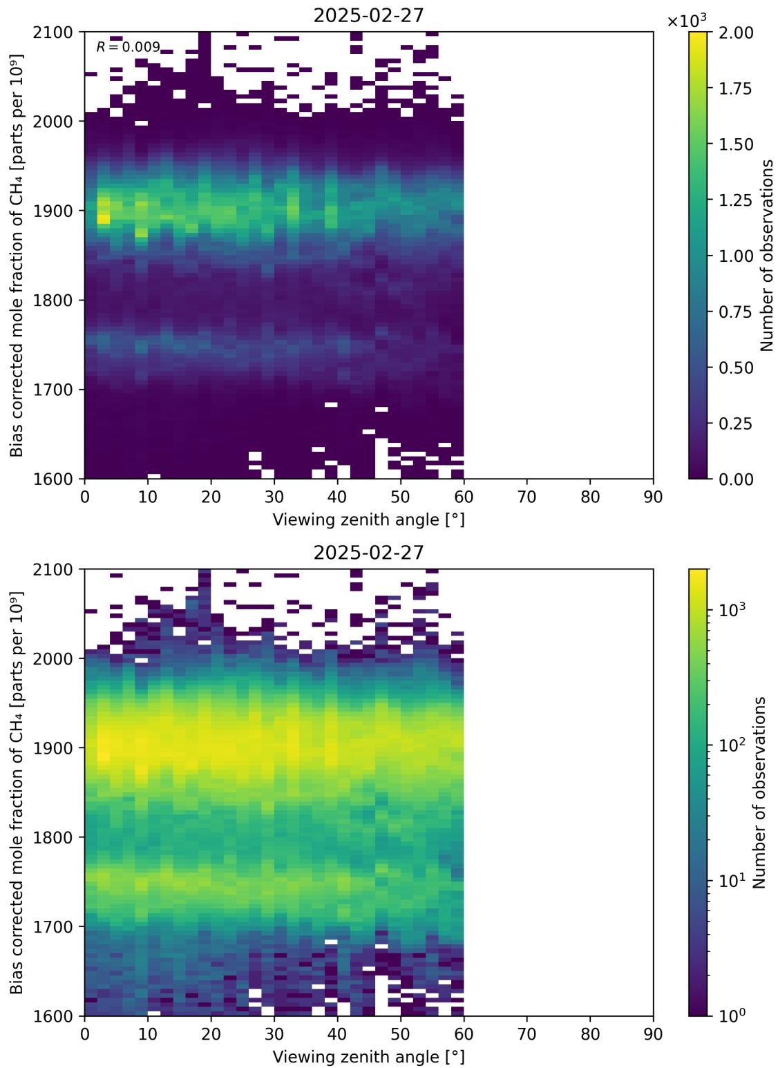
Figure 111: Scatter density plot of “Viewing zenith angle” against “Bias corrected mole fraction of CH 4 ” for 2025-02-26 to 2025-02-28.
