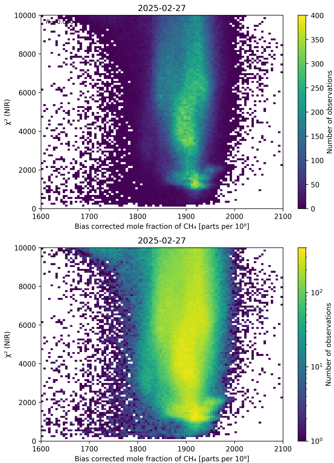
Figure 63: Scatter density plot of “Bias corrected mole fraction of CH 4 ” against “ \chi^2 (NIR)” for 2025-02-26 to 2025-02-28.
