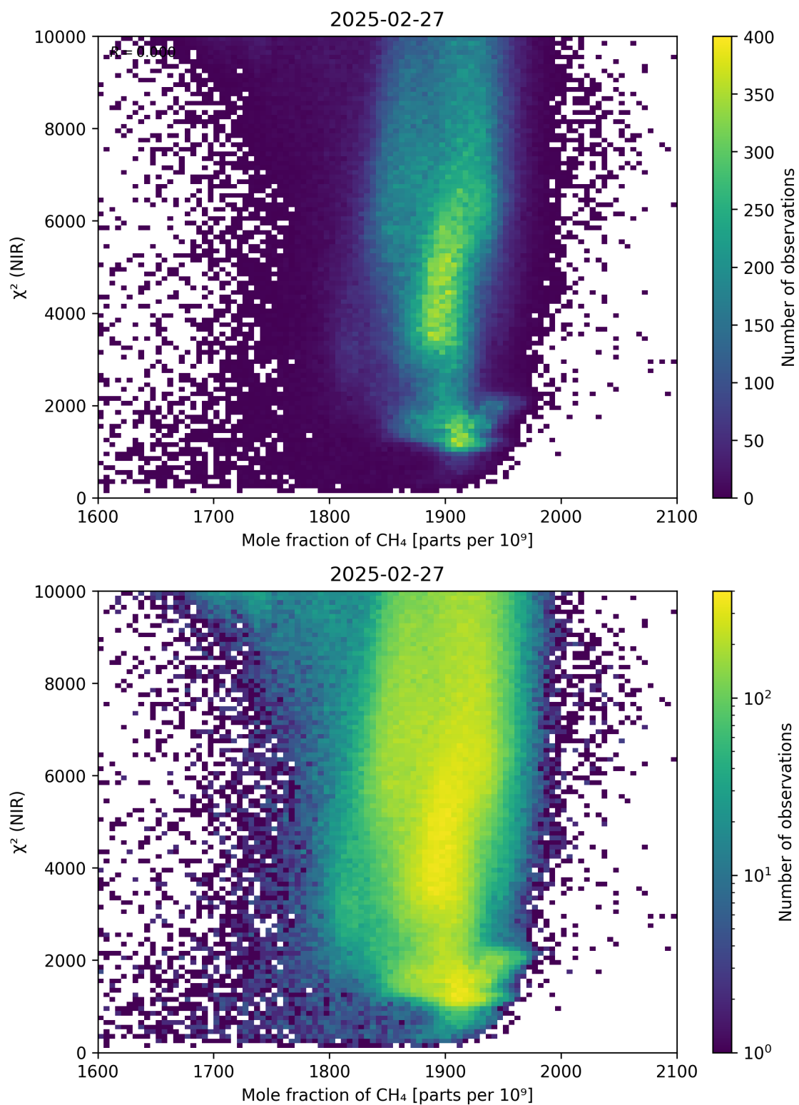
Figure 70: Scatter density plot of “Mole fraction of CH 4 ” against “ \chi^2 (NIR)” for 2025-02-26 to 2025-02-28.
