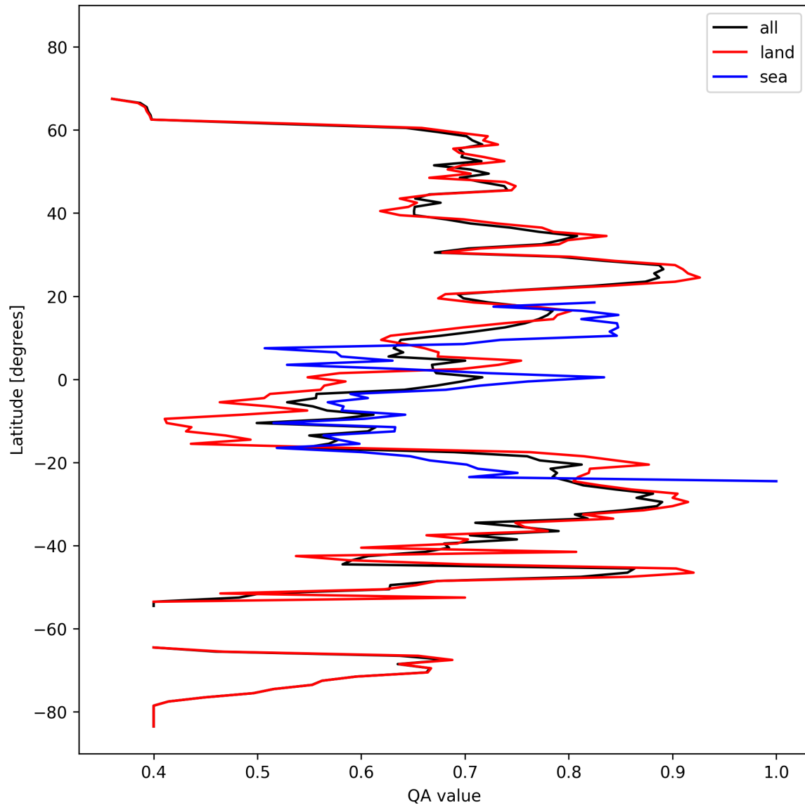
Figure 11: Zonal average of “QA value” for 2025-02-26 to 2025-02-28.
