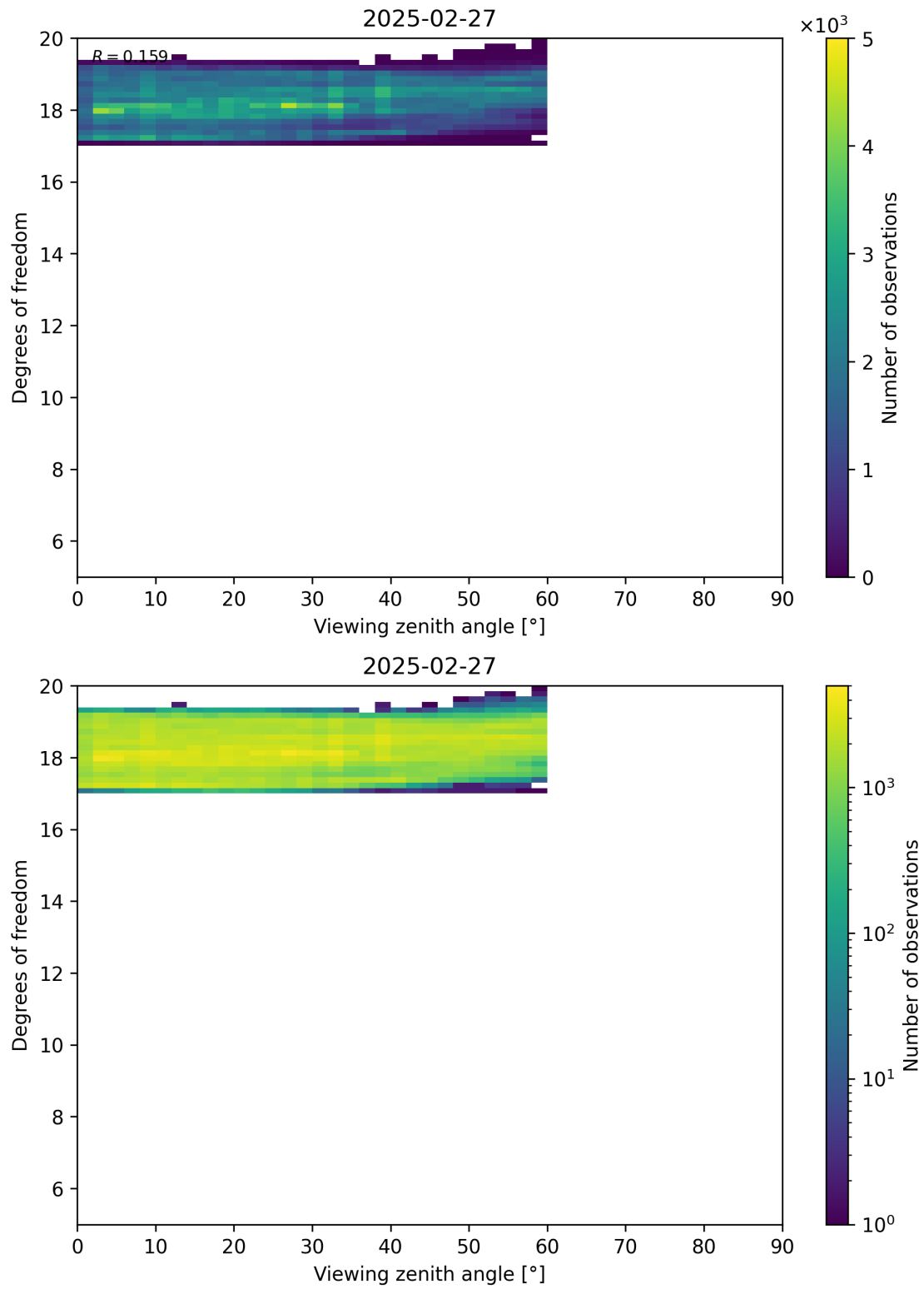
Figure 107: Scatter density plot of “Viewing zenith angle” against “Degrees of freedom” for 2025-02-26 to 2025-02-28.
