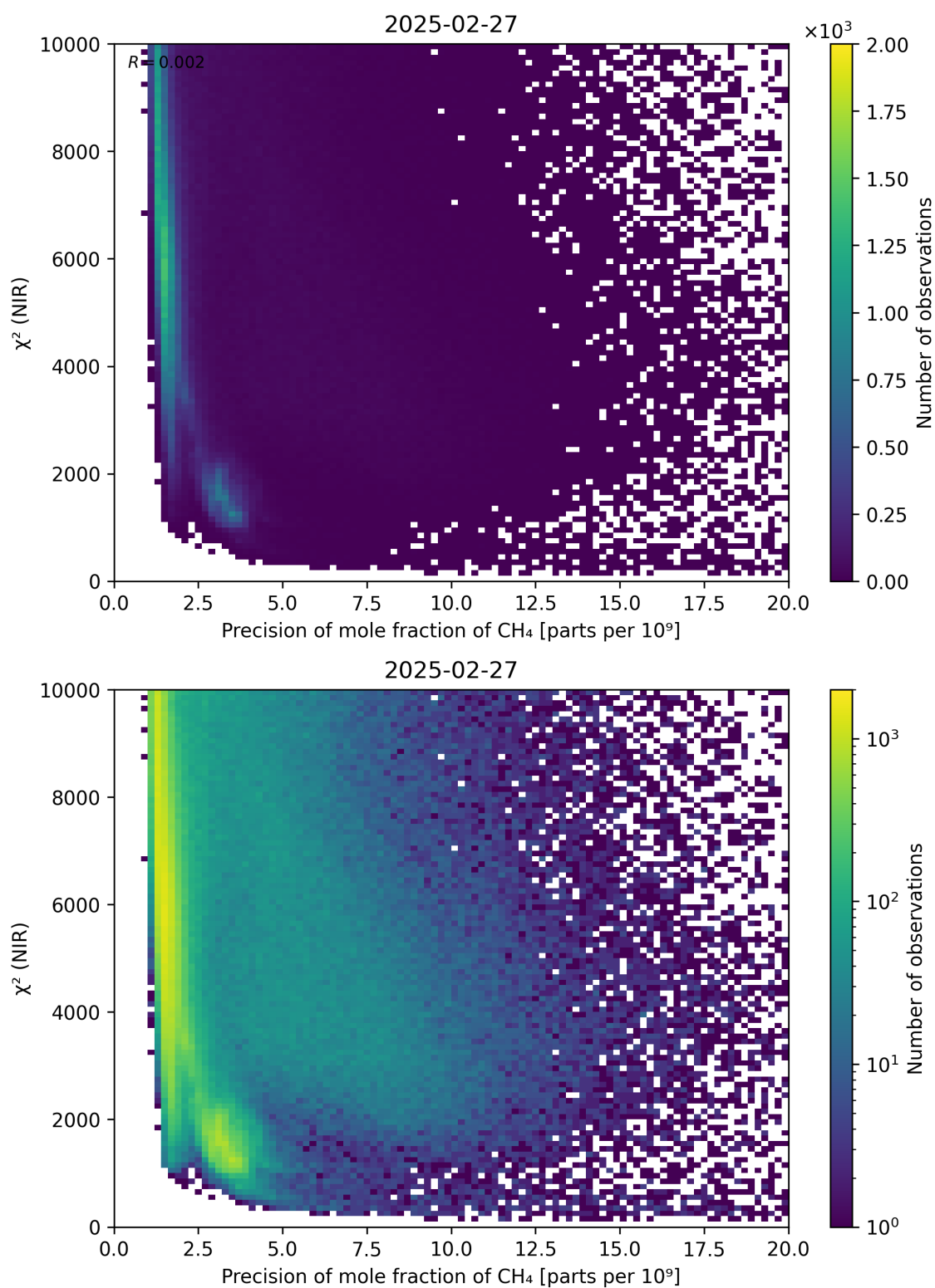
Figure 78: Scatter density plot of “Precision of mole fraction of \text{CH}_4 ” against “ \chi^2 (NIR)” for 2025-02-26 to 2025-02-28.
