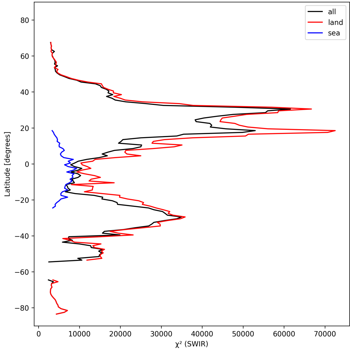
Figure 17: Zonal average of “ \chi^2 (SWIR)” for 2025-02-26 to 2025-02-28.
