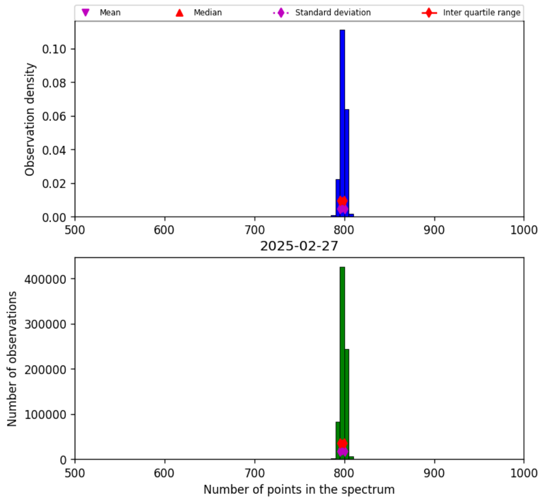
Figure 26: Histogram of “Number of points in the spectrum” for 2025-02-26 to 2025-02-28
