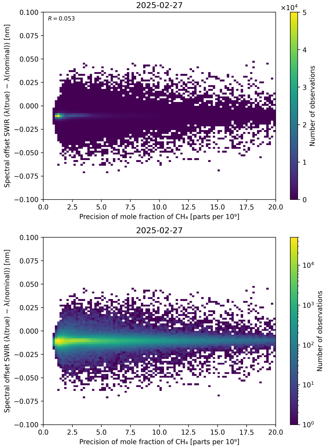
Figure 85: Scatter density plot of “Precision of mole fraction of CH 4 ” against “Spectral offset SWIR ( \lambda_{\text{true}} - \lambda_{\text{nominal}} )” for 2025-02-26 to 2025-02-28.
