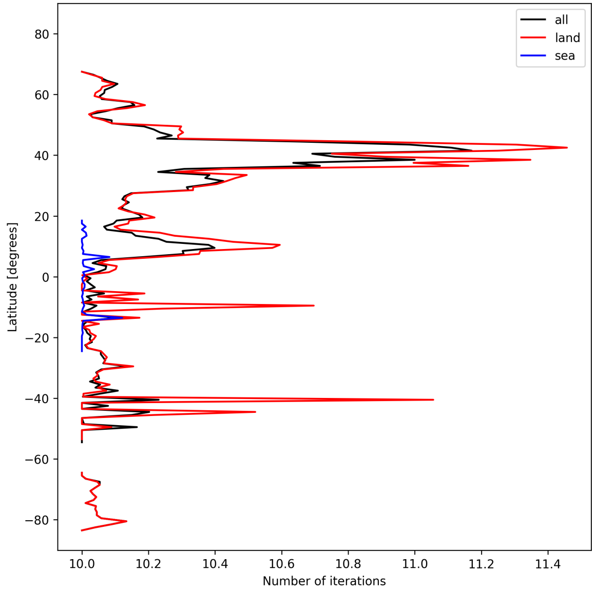
Figure 20: Zonal average of “Number of iterations” for 2025-02-26 to 2025-02-28.
