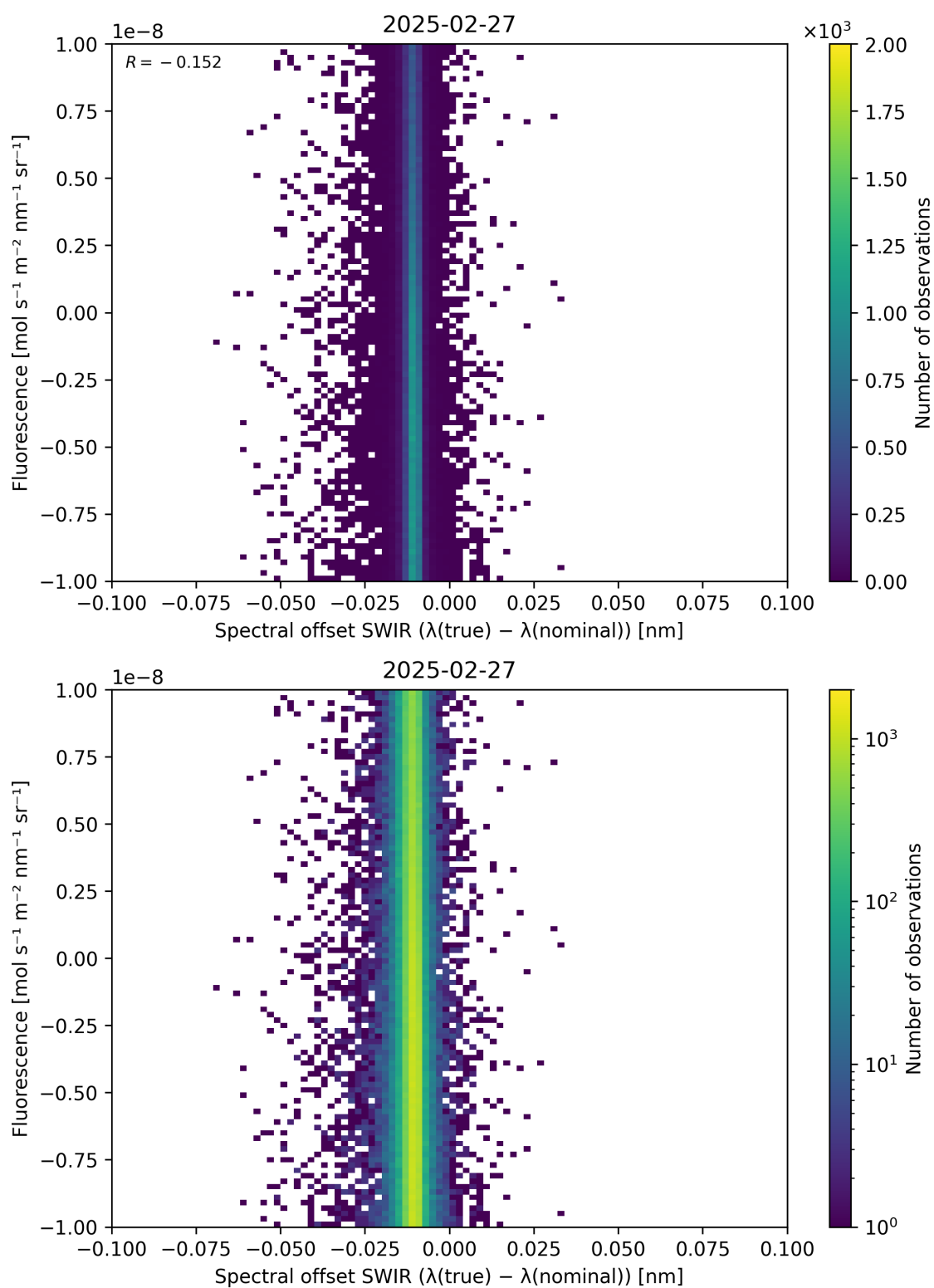
Figure 120: Scatter density plot of “Spectral offset SWIR ( \lambda_{\text{true}} - \lambda_{\text{nominal}} )” against “Fluorescence” for 2025-02-26 to 2025-02-28.
