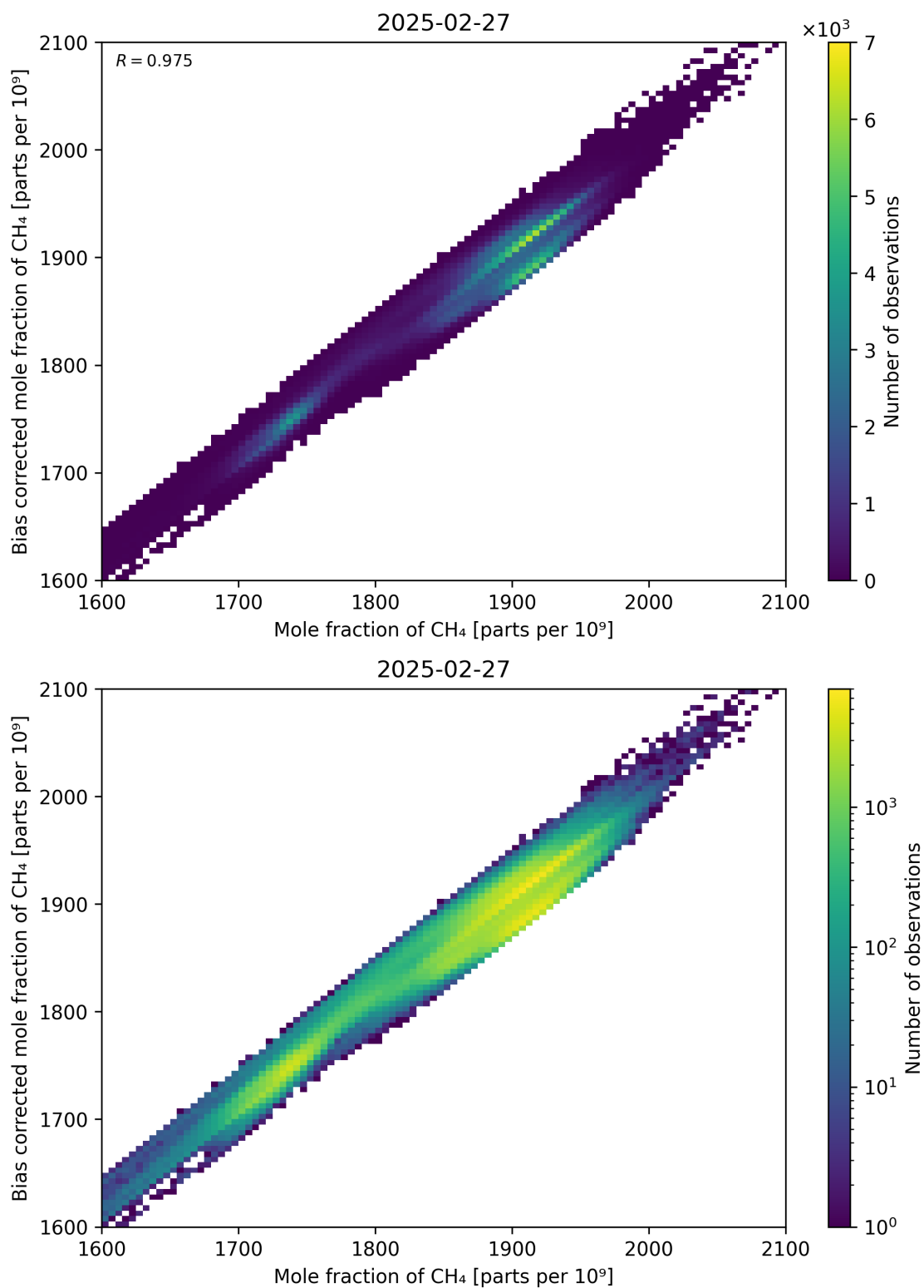
Figure 74: Scatter density plot of “Mole fraction of CH 4 ” against “Bias corrected mole fraction of CH 4 ” for 2025-02-26 to 2025-02-28.
