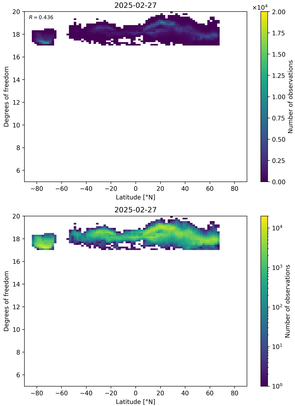
Figure 55: Scatter density plot of “Latitude” against “Degrees of freedom” for 2025-02-26 to 2025-02-28.
