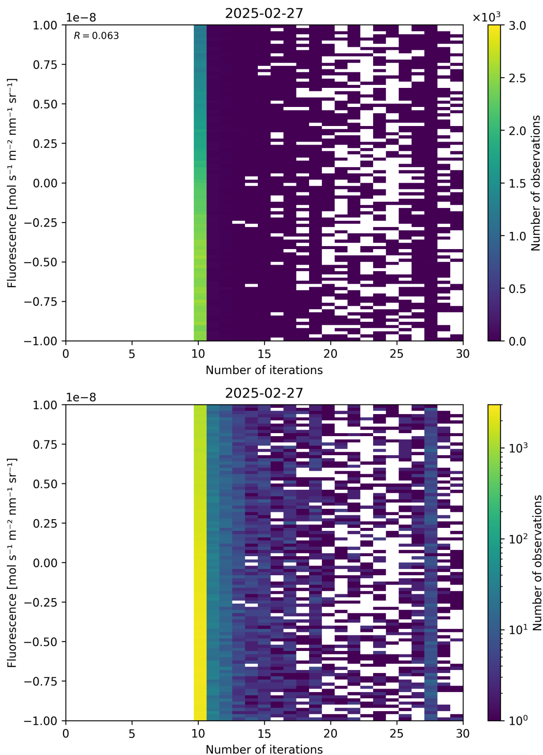
Figure 87: Scatter density plot of “Number of iterations” against “Fluorescence” for 2025-02-26 to 2025-02-28.
