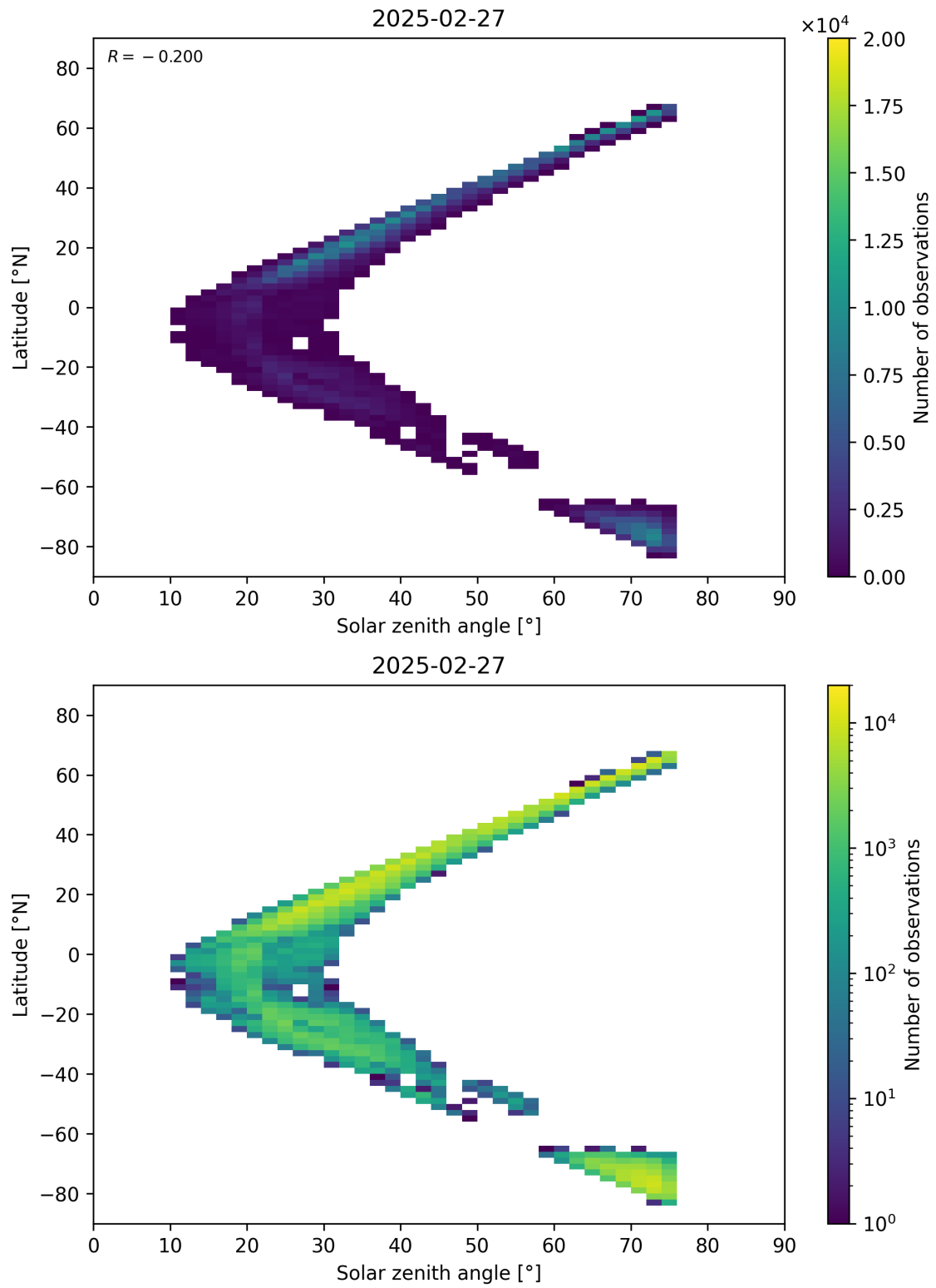
Figure 98: Scatter density plot of “Solar zenith angle” against “Latitude” for 2025-02-26 to 2025-02-28.
