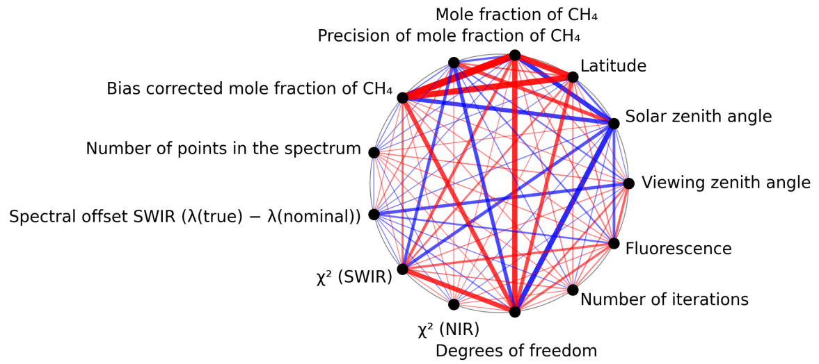
Figure 1: Map of correlation graph for 2025-02-26 to 2025-02-28.
