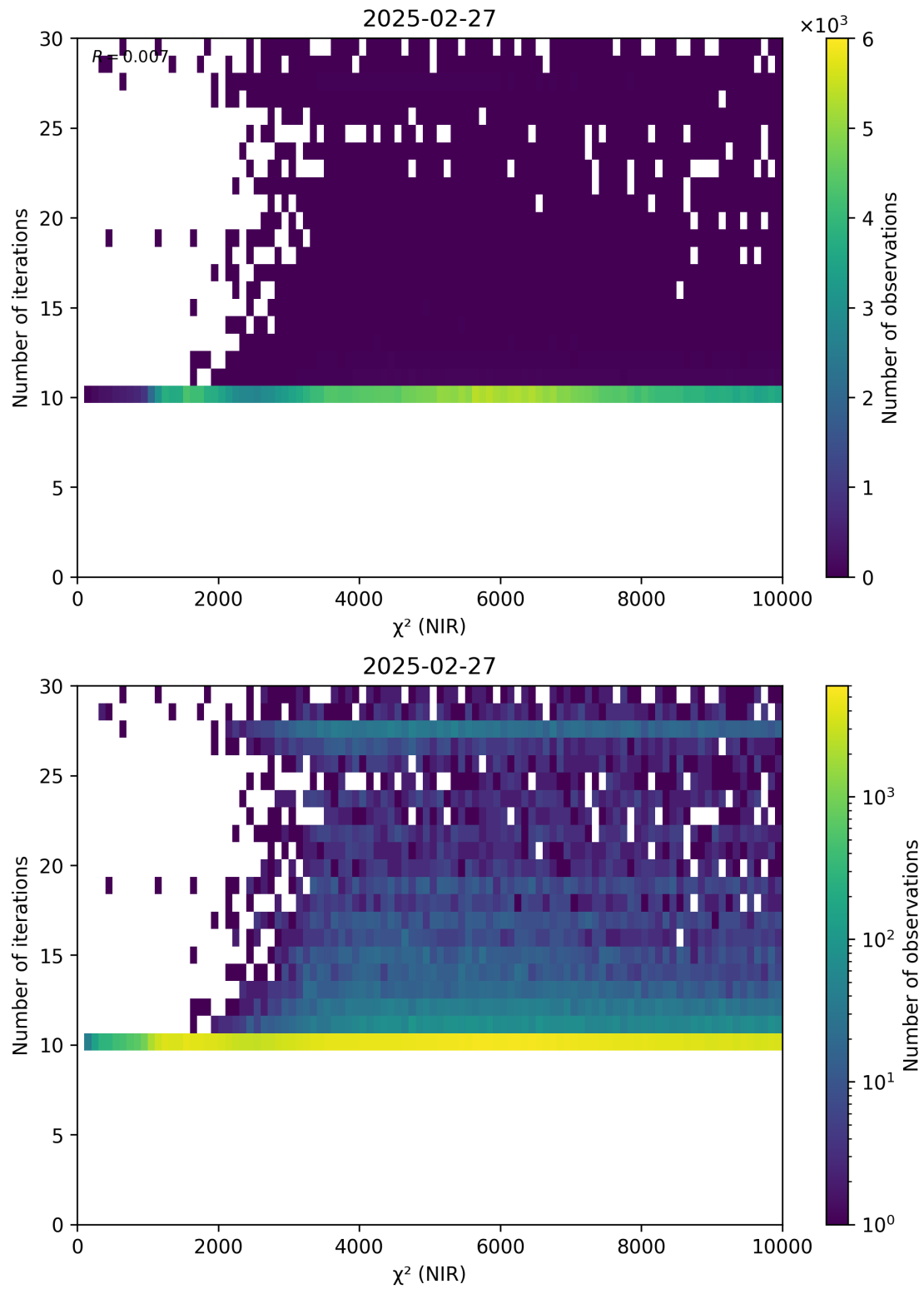
Figure 46: Scatter density plot of “ \chi^2 (NIR)” against “Number of iterations” for 2025-02-26 to 2025-02-28.
