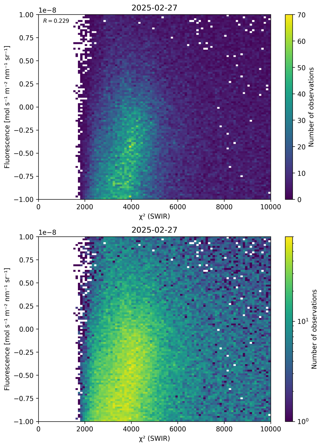
Figure 49: Scatter density plot of “ \chi^2 (SWIR)” against “Fluorescence” for 2025-02-26 to 2025-02-28.
