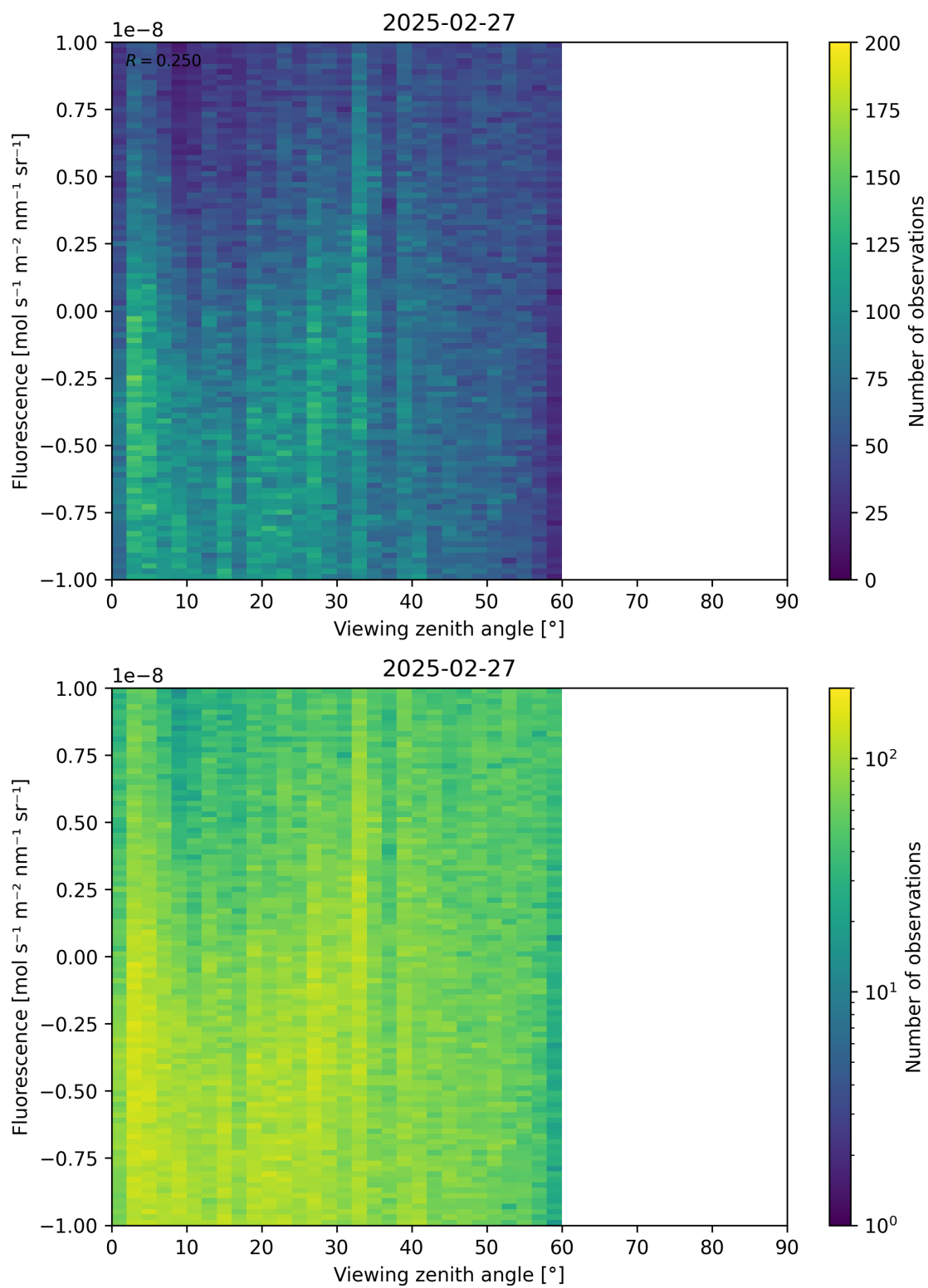
Figure 108: Scatter density plot of “Viewing zenith angle” against “Fluorescence” for 2025-02-26 to 2025-02-28.
