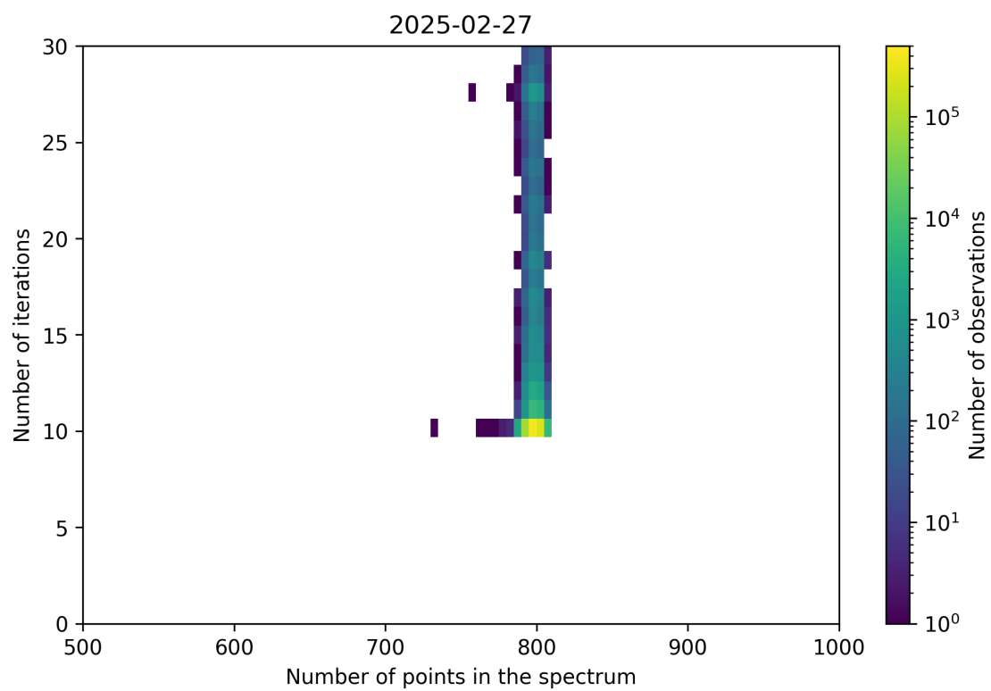
Figure 92: Scatter density plot of “Number of points in the spectrum” against “Number of iterations” for 2025-02-26 to 2025-02-28.
