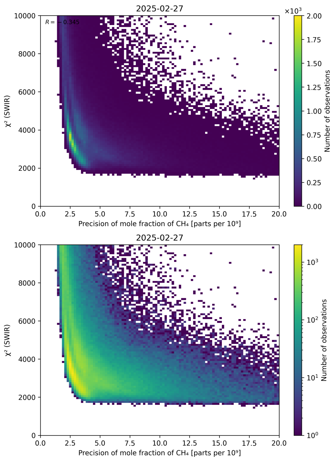
Figure 79: Scatter density plot of “Precision of mole fraction of \text{CH}_4 ” against “ \chi^2 (SWIR)” for 2025-02-26 to 2025-02-28.
