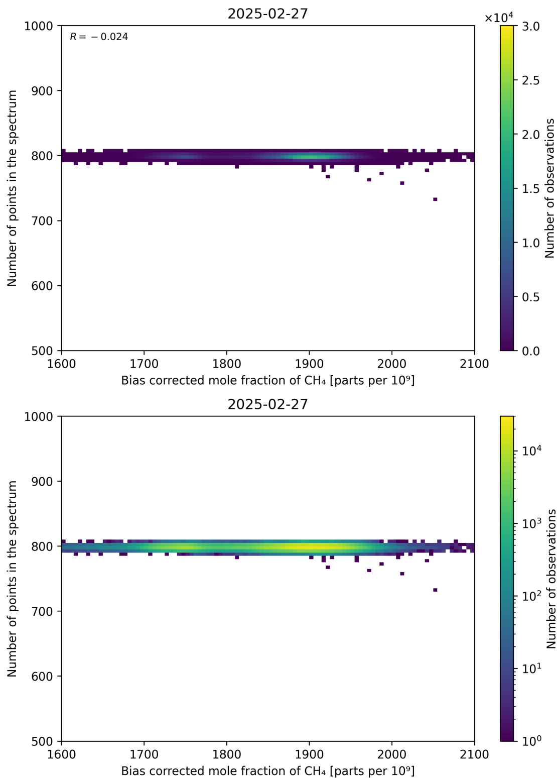
Figure 68: Scatter density plot of “Bias corrected mole fraction of CH 4 ” against “Number of points in the spectrum” for 2025-02-26 to 2025-02-28.
