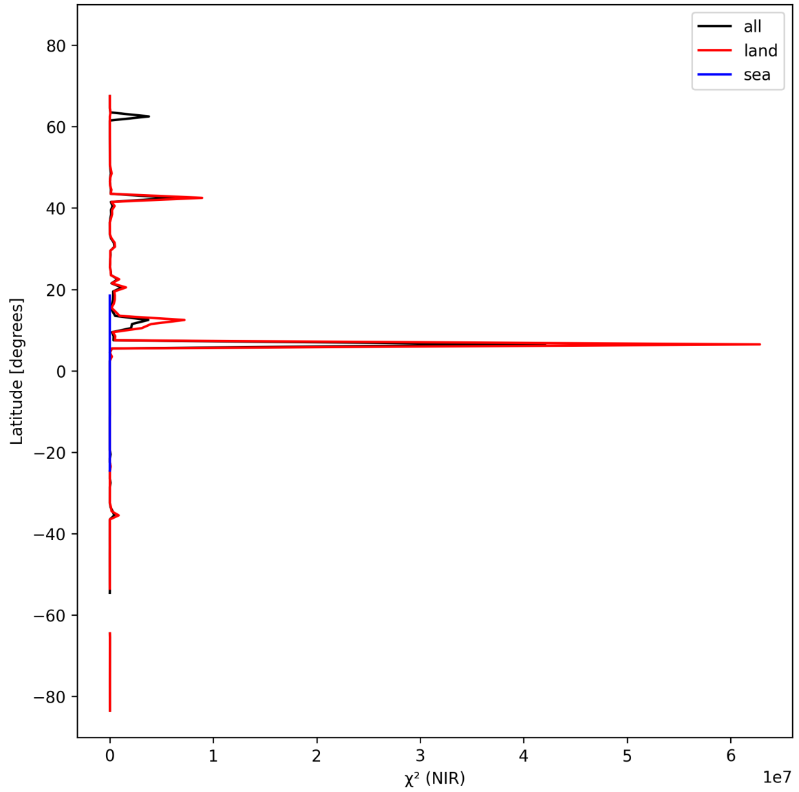
Figure 18: Zonal average of “ \chi^2 (NIR)” for 2025-02-26 to 2025-02-28.
