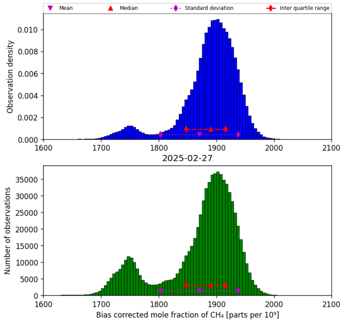
Figure 25: Histogram of “Bias corrected mole fraction of CH 4 ” for 2025-02-26 to 2025-02-28
