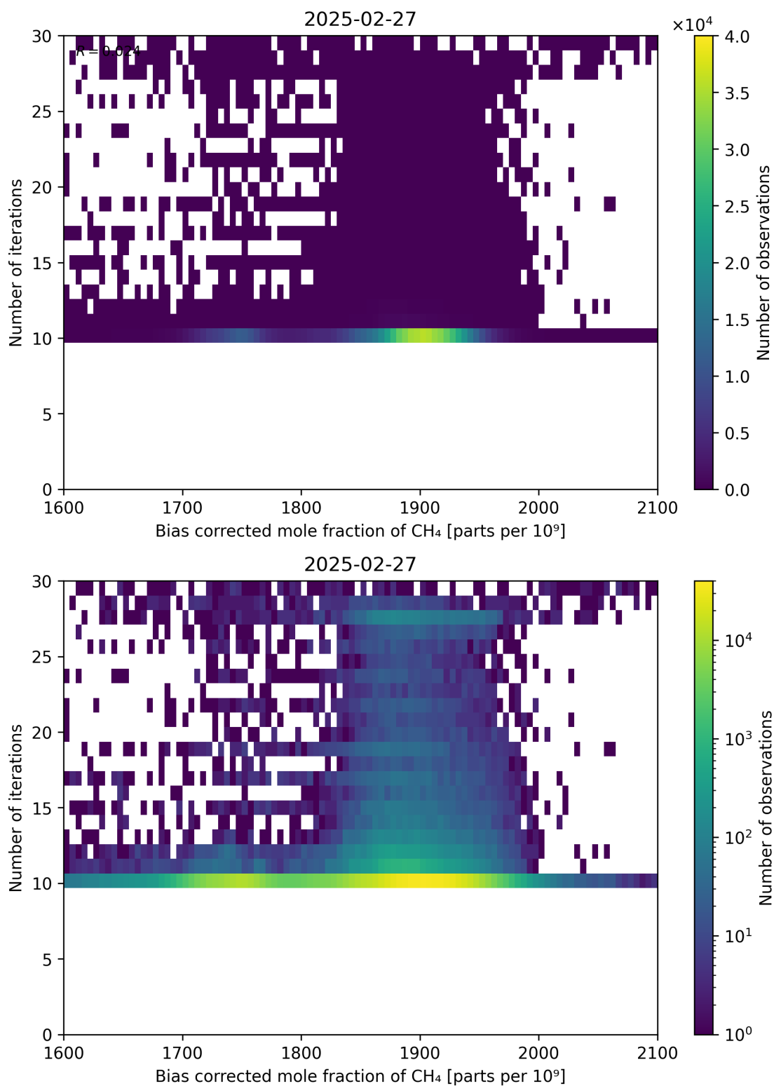
Figure 67: Scatter density plot of “Bias corrected mole fraction of \text{CH}_4 ” against “Number of iterations” for 2025-02-26 to 2025-02-28.
