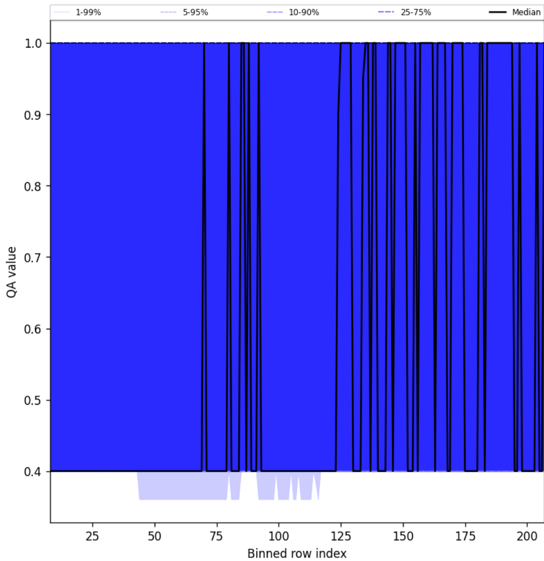
Figure 33: Along track statistics of “QA value” for 2025-02-26 to 2025-02-28
