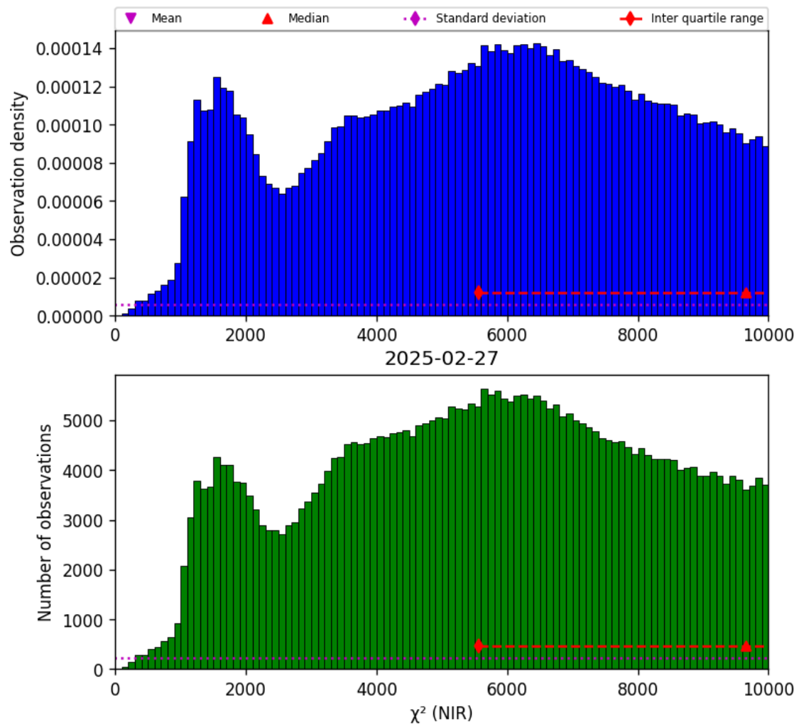
Figure 29: Histogram of “ \chi^2 (NIR)” for 2025-02-26 to 2025-02-28
