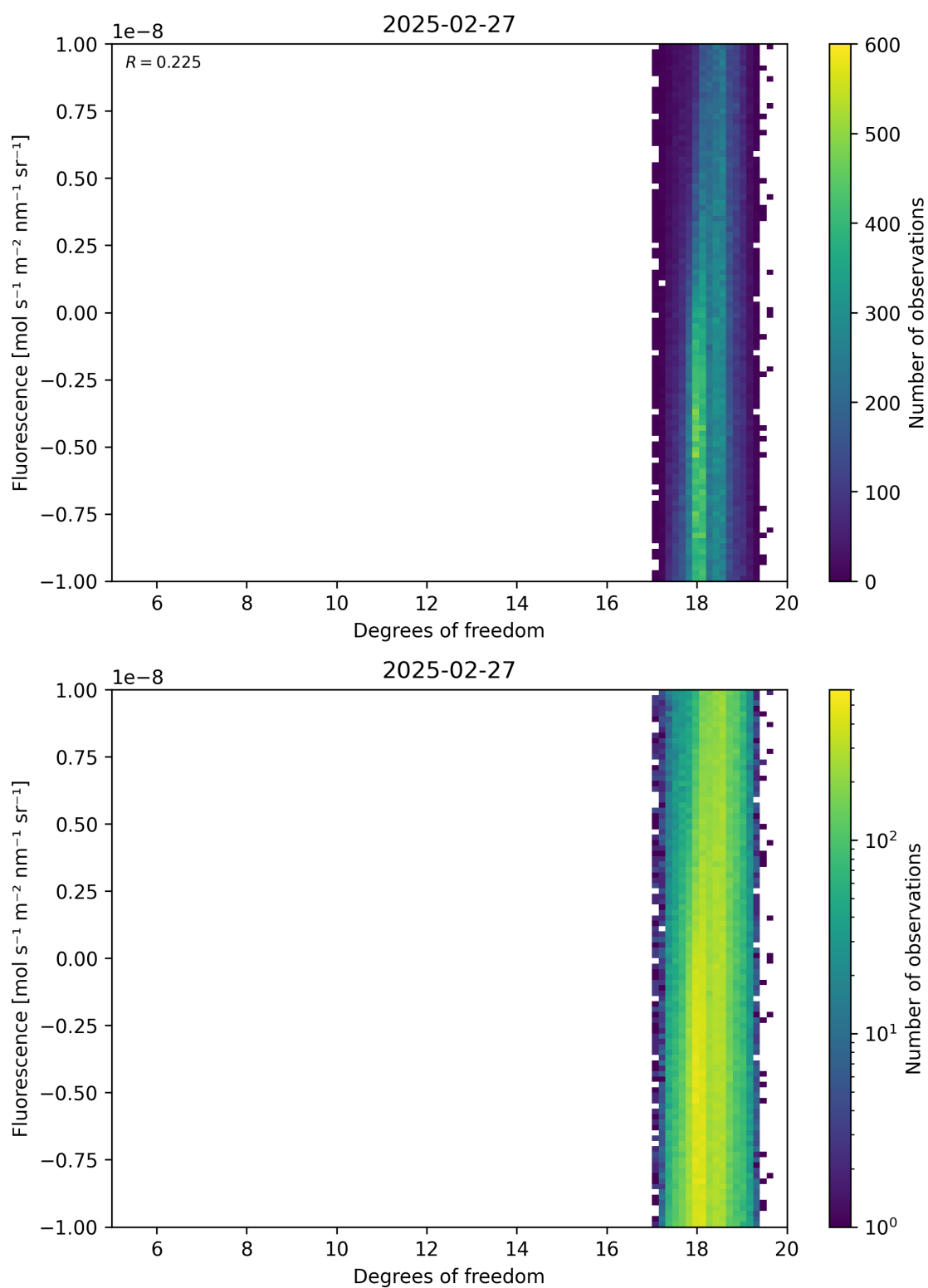
Figure 51: Scatter density plot of “Degrees of freedom” against “Fluorescence” for 2025-02-26 to 2025-02-28.
