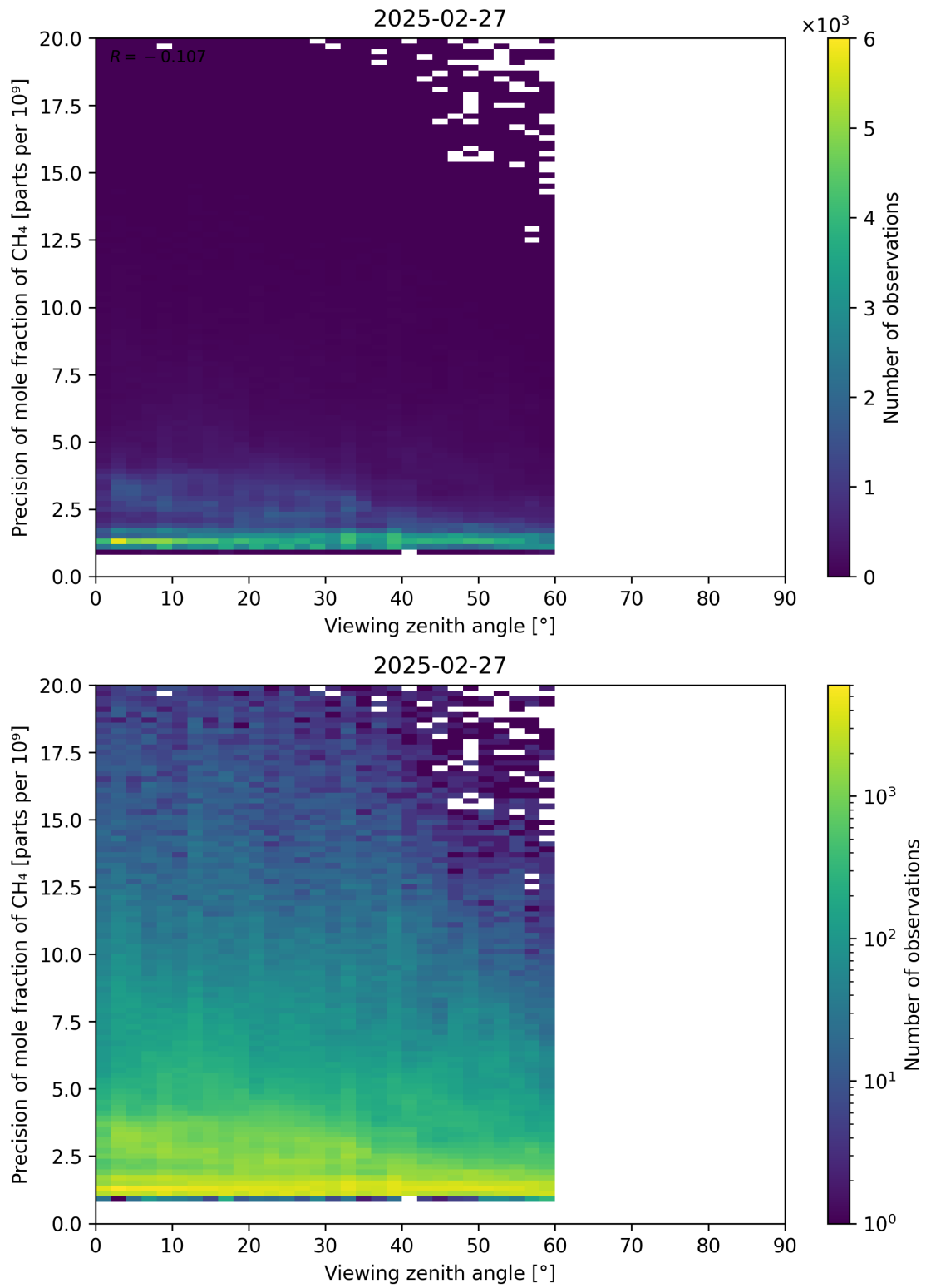
Figure 112: Scatter density plot of “Viewing zenith angle” against “Precision of mole fraction of CH 4 ” for 2025-02-26 to 2025-02-28.
