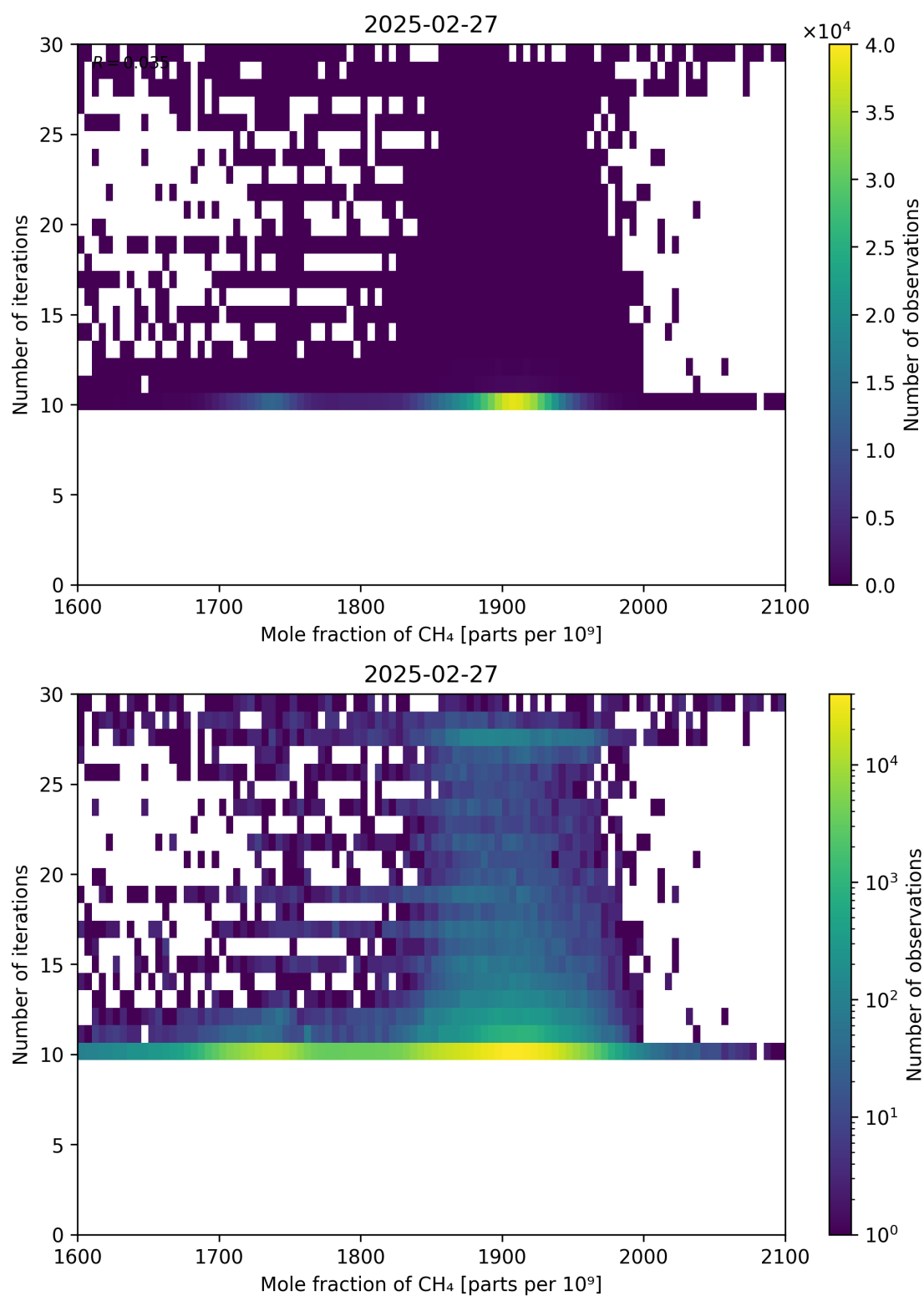
Figure 76: Scatter density plot of “Mole fraction of CH 4 ” against “Number of iterations” for 2025-02-26 to 2025-02-28.
