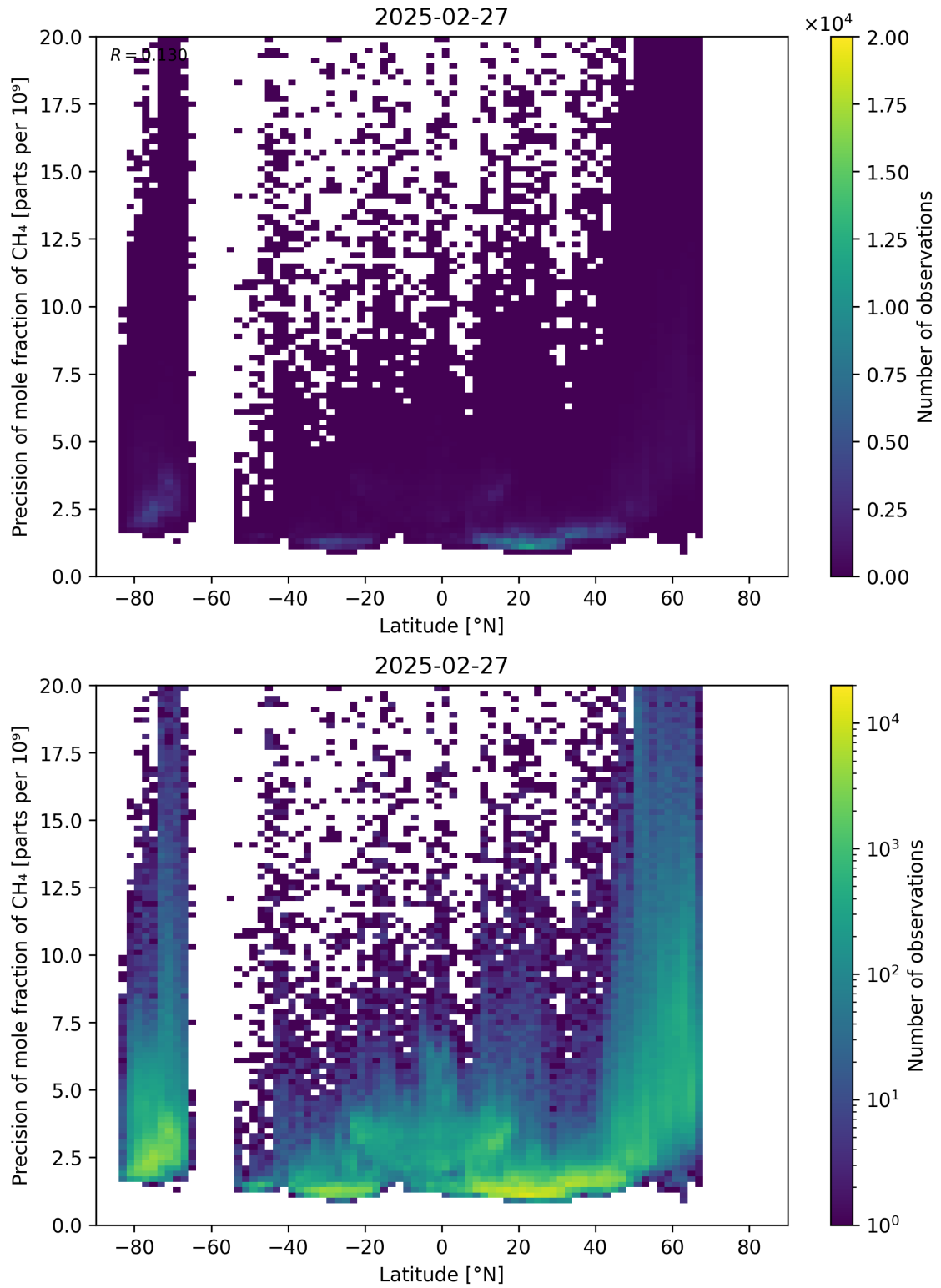
Figure 59: Scatter density plot of “Latitude” against “Precision of mole fraction of CH 4 ” for 2025-02-26 to 2025-02-28.
