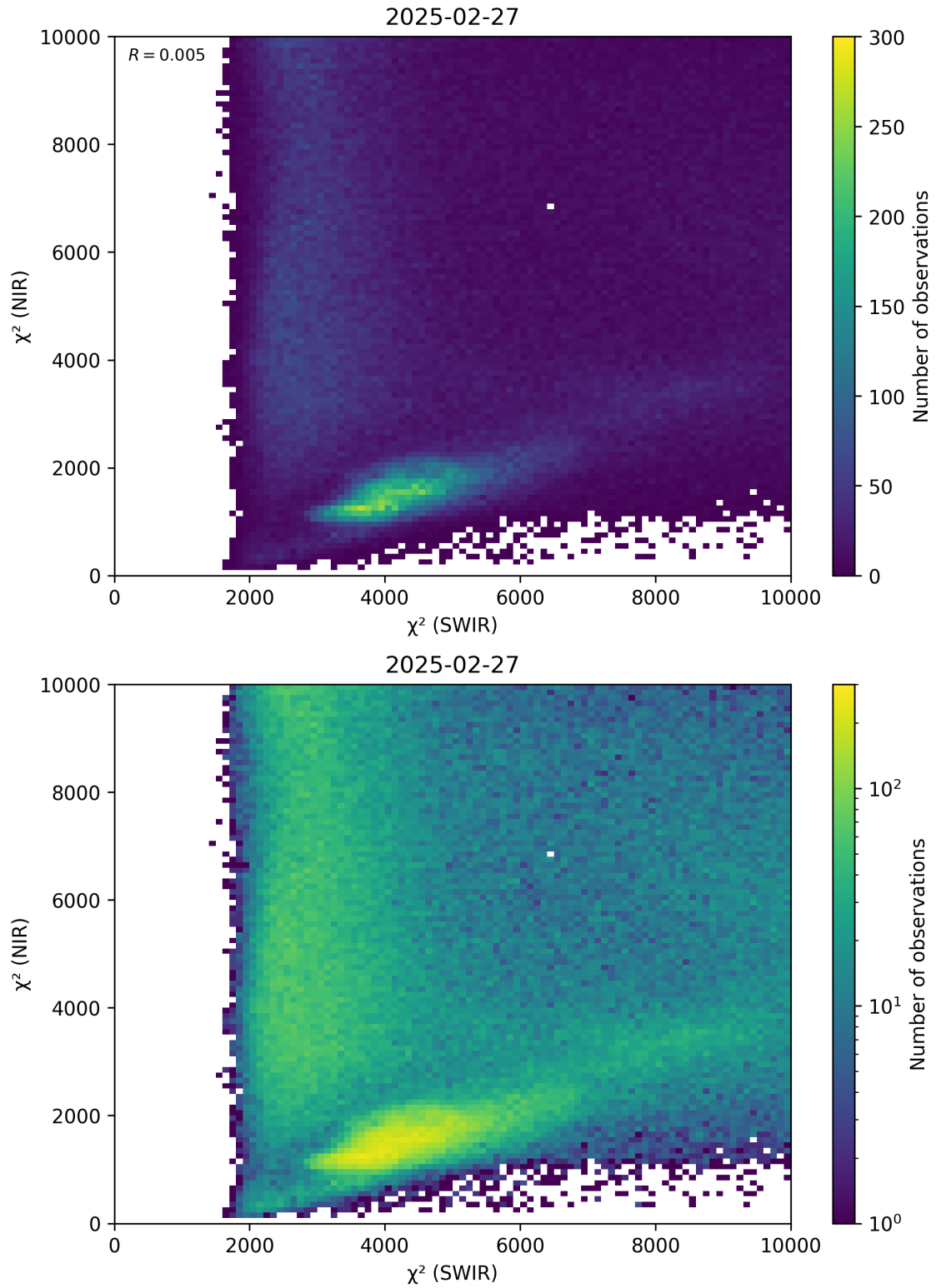
Figure 47: Scatter density plot of “ \chi^2 (SWIR)” against “ \chi^2 (NIR)” for 2025-02-26 to 2025-02-28.
