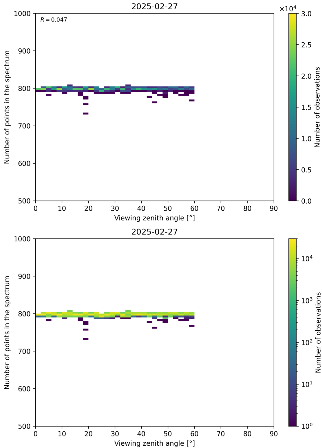
Figure 114: Scatter density plot of “Viewing zenith angle” against “Number of points in the spectrum” for 2025-02-26 to 2025-02-28.
