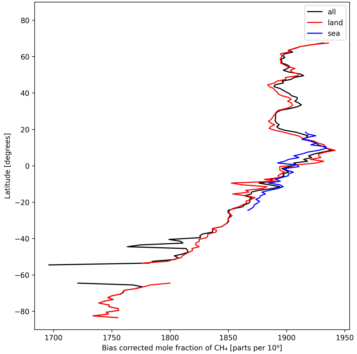
Figure 14: Zonal average of “Bias corrected mole fraction of CH 4 ” for 2025-02-26 to 2025-02-28.
