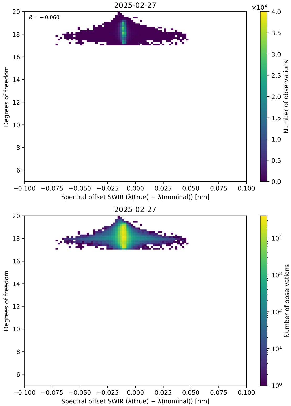
Figure 119: Scatter density plot of “Spectral offset SWIR ( \lambda_{\text{true}} - \lambda_{\text{nominal}} )” against “Degrees of freedom” for 2025-02-26 to 2025-02-28.
