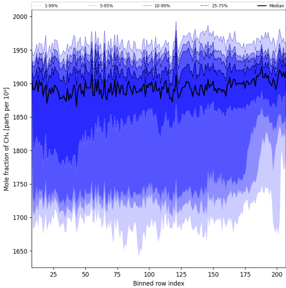
Figure 34: Along track statistics of “Mole fraction of CH 4 ” for 2025-02-26 to 2025-02-28
