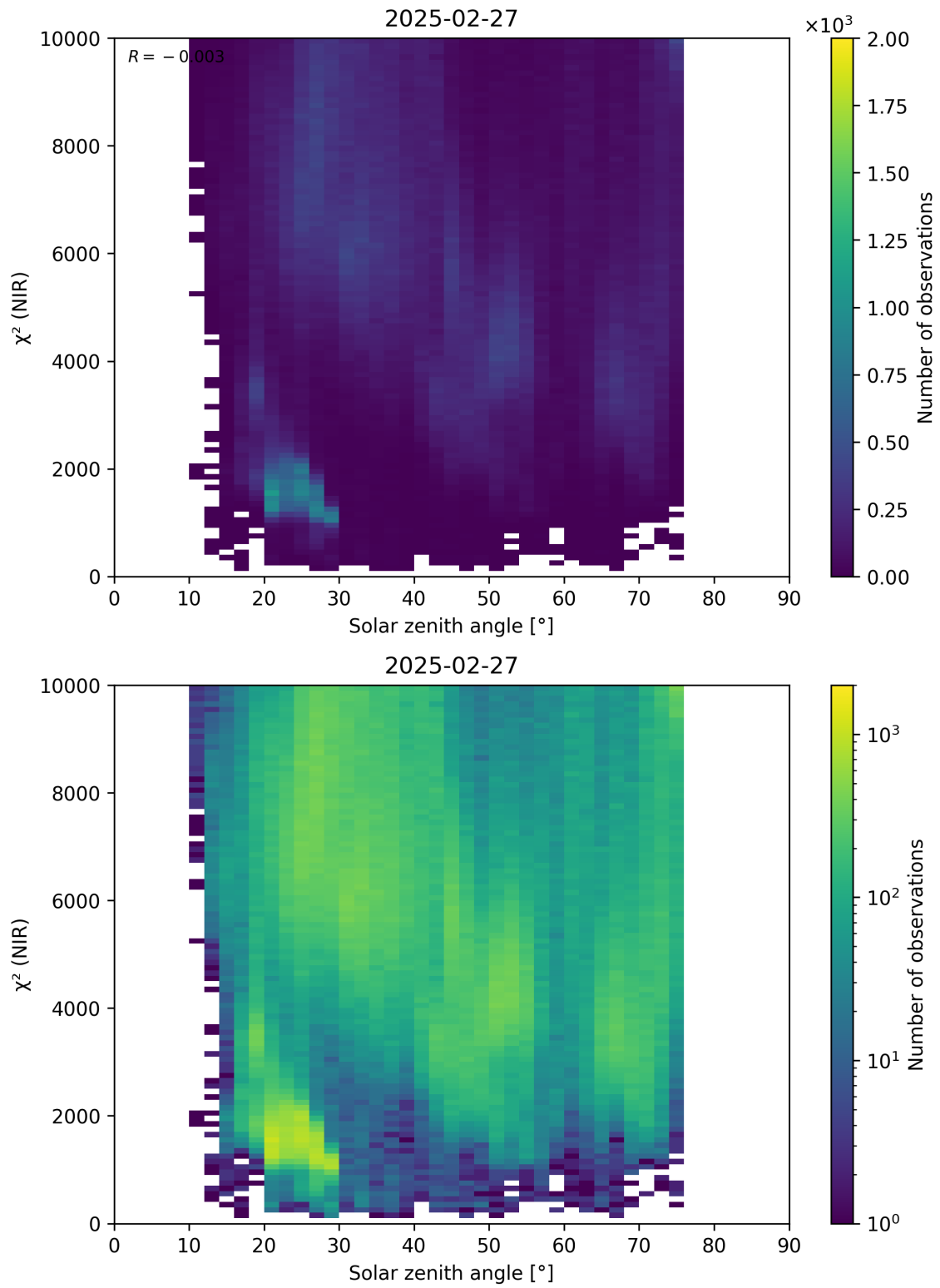
Figure 94: Scatter density plot of “Solar zenith angle” against “ \chi^2 (NIR)” for 2025-02-26 to 2025-02-28.
