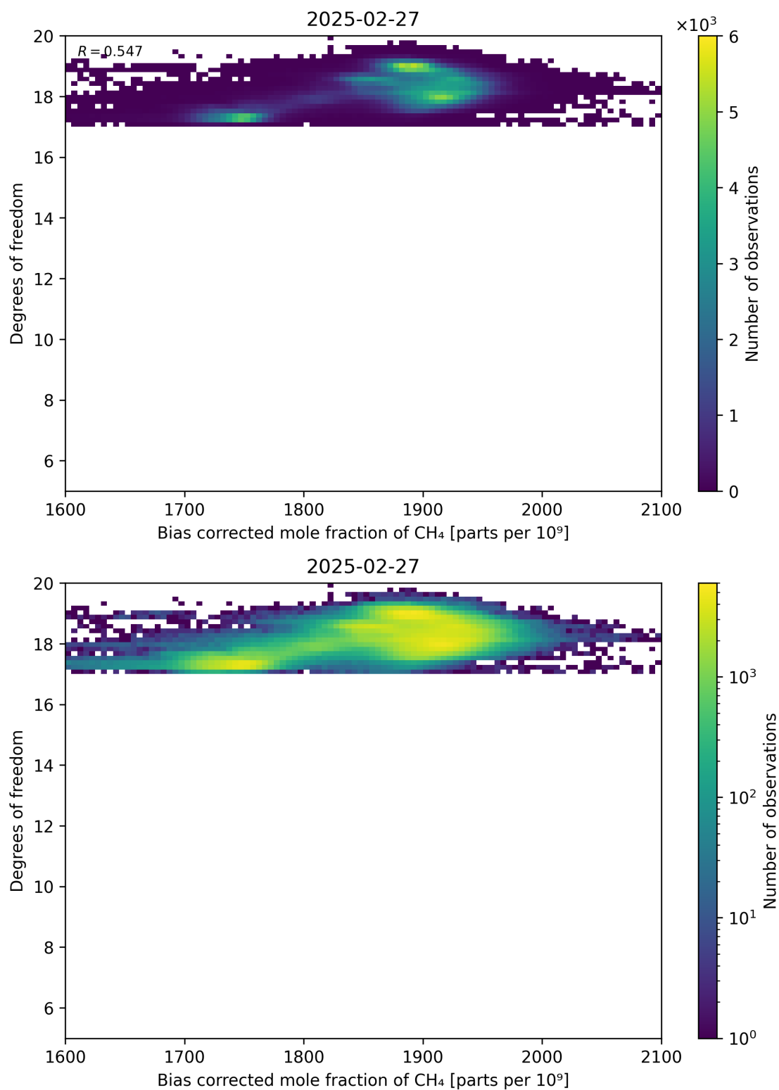
Figure 65: Scatter density plot of “Bias corrected mole fraction of CH 4 ” against “Degrees of freedom” for 2025-02-26 to 2025-02-28.
