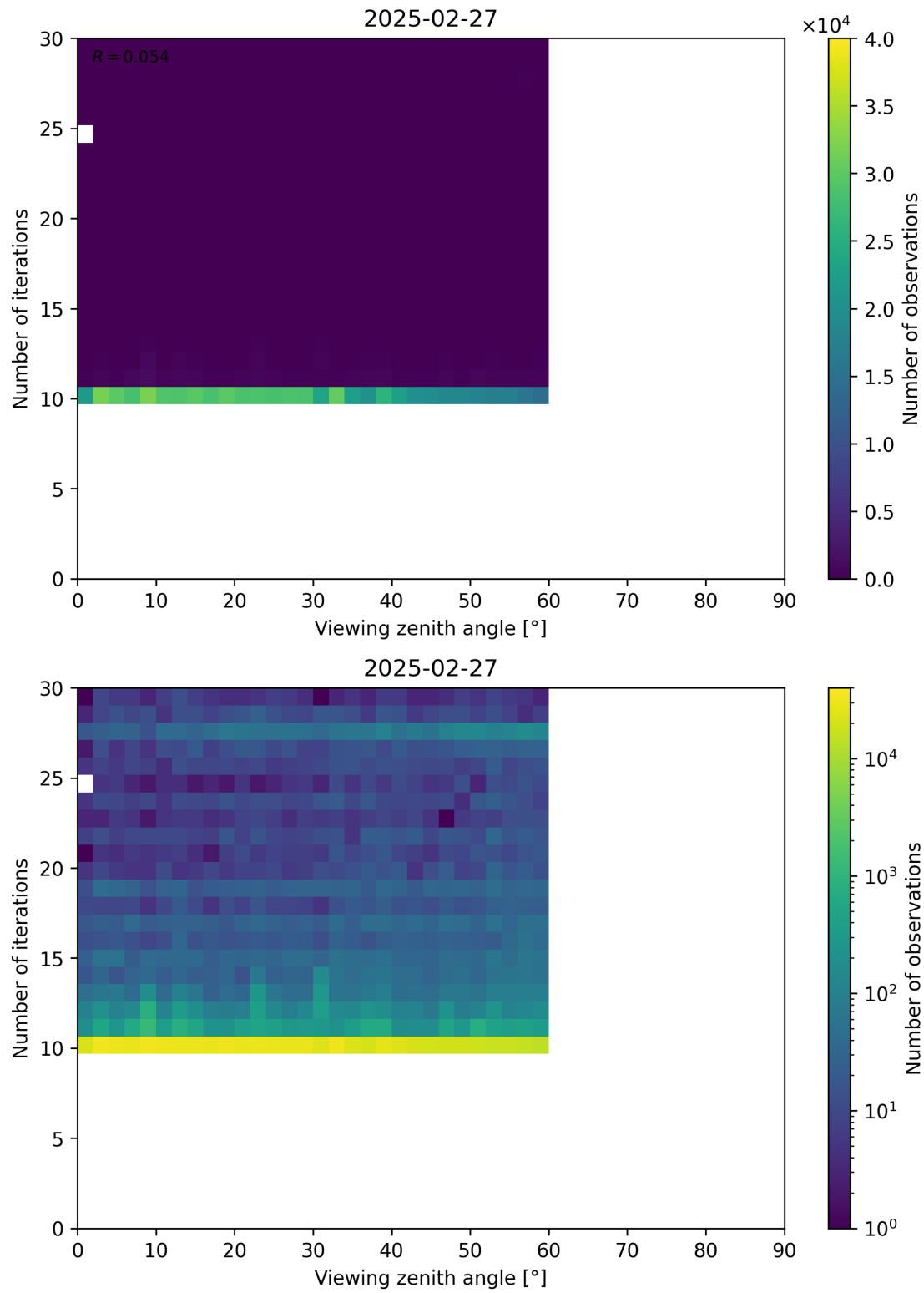
Figure 113: Scatter density plot of “Viewing zenith angle” against “Number of iterations” for 2025-02-26 to 2025-02-28.
