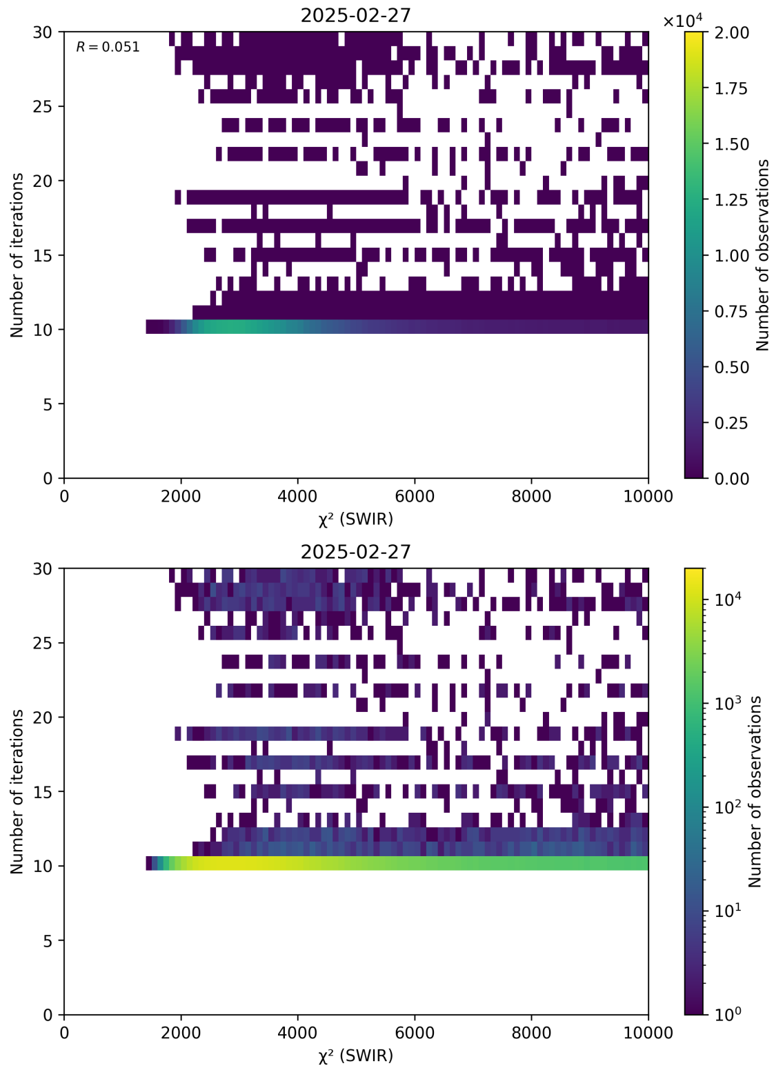
Figure 50: Scatter density plot of “ \chi^2 (SWIR)” against “Number of iterations” for 2025-02-26 to 2025-02-28.
