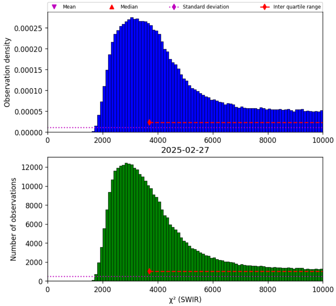
Figure 28: Histogram of “ \chi^2 (SWIR)” for 2025-02-26 to 2025-02-28
