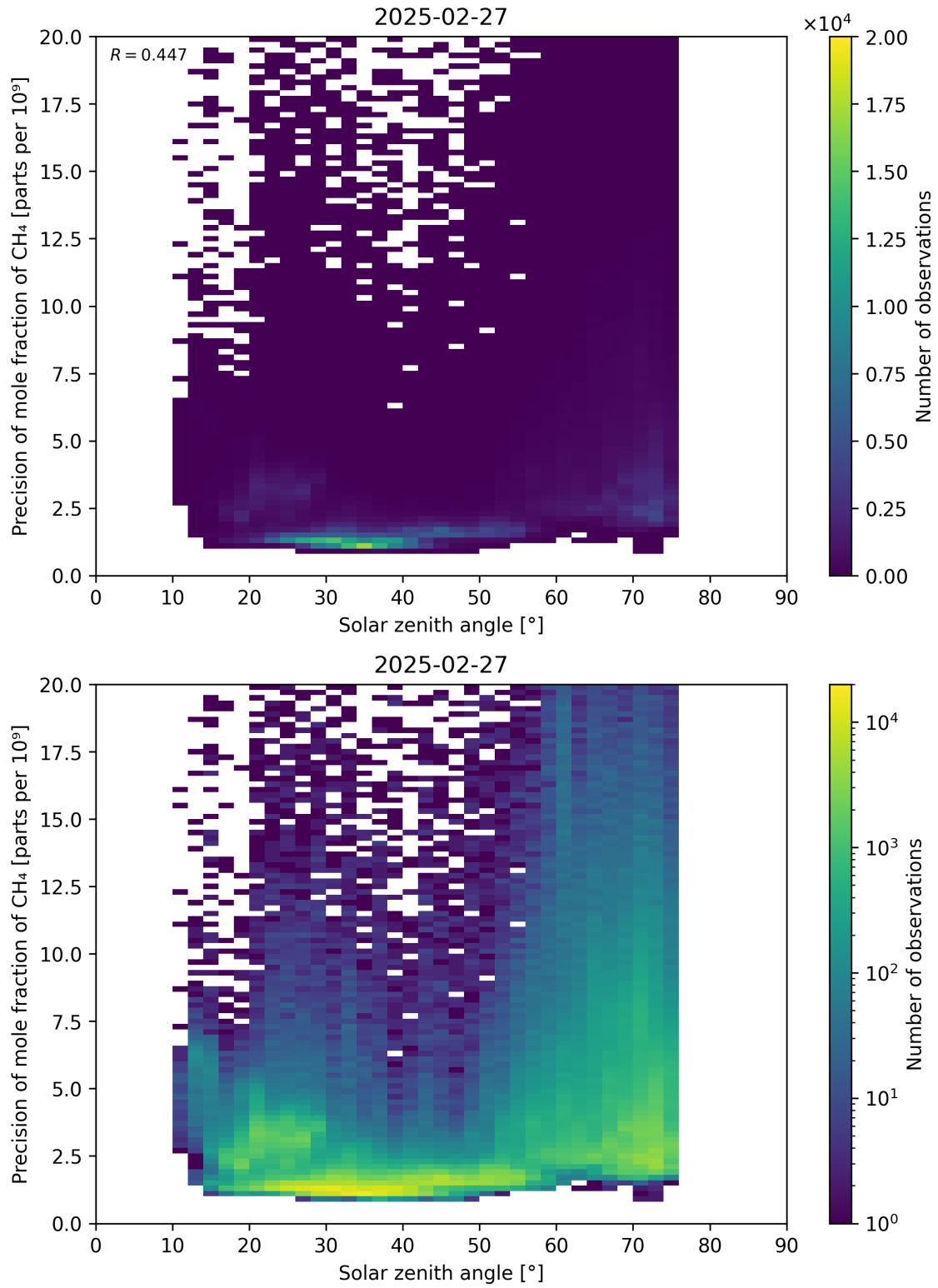
Figure 101: Scatter density plot of “Solar zenith angle” against “Precision of mole fraction of CH 4 ” for 2025-02-26 to 2025-02-28.
