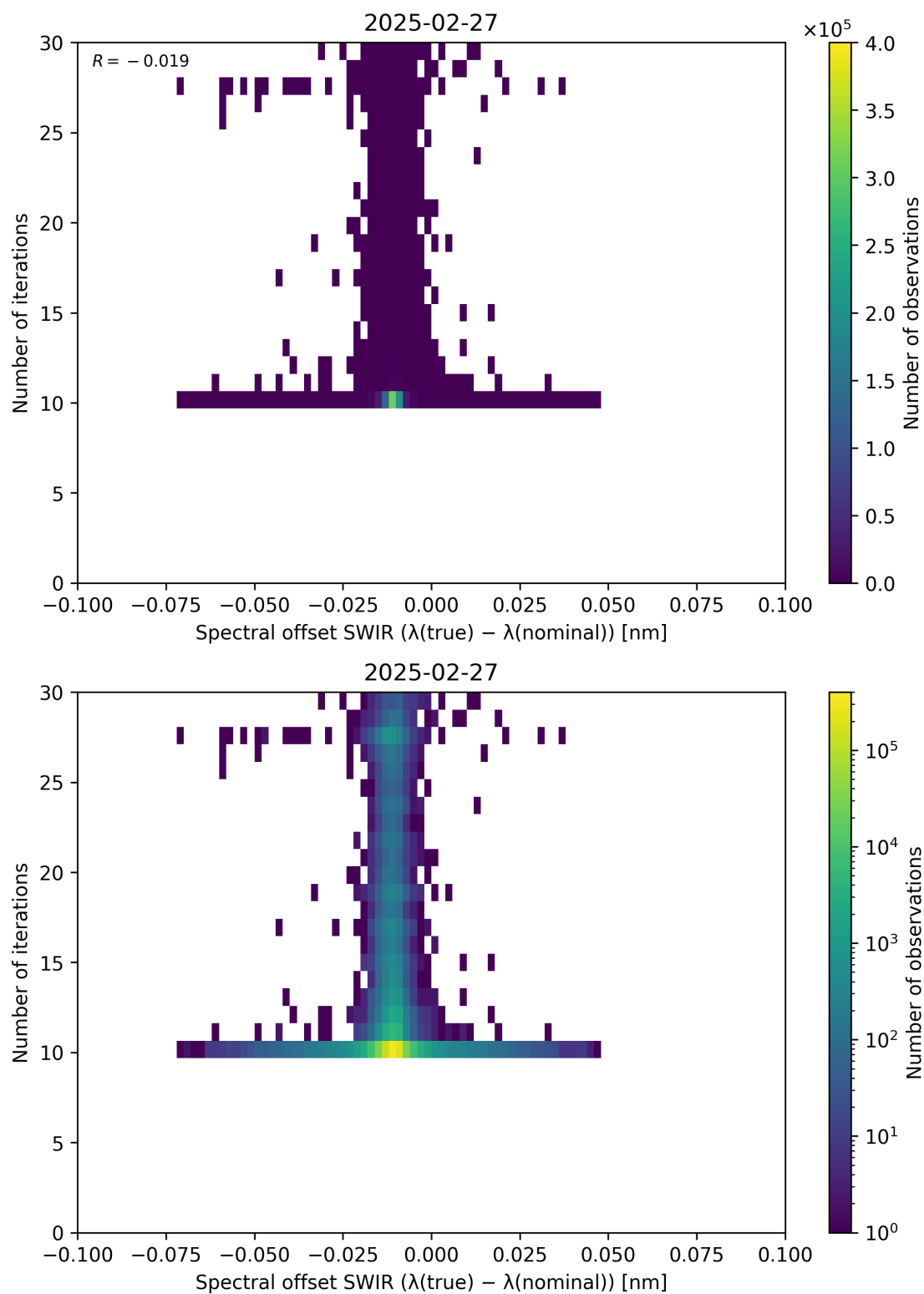
Figure 121: Scatter density plot of “Spectral offset SWIR ( \lambda_{\text{true}} - \lambda_{\text{nominal}} )” against “Number of iterations” for 2025-02-26 to 2025-02-28.
