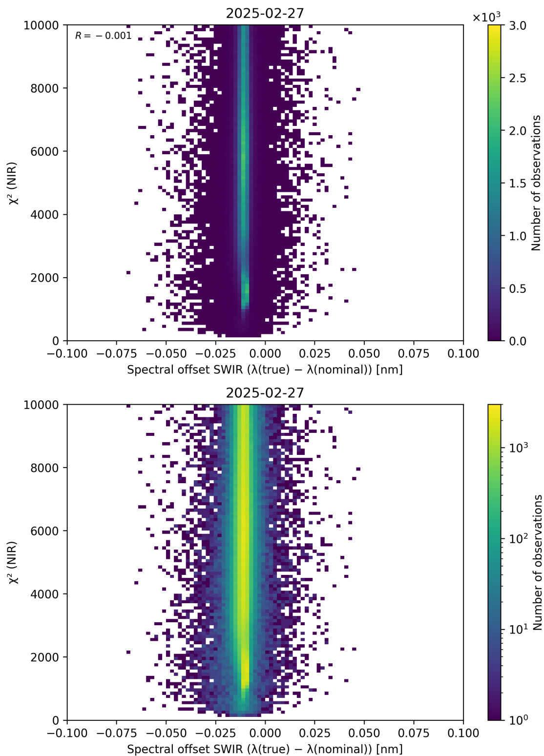
Figure 117: Scatter density plot of “Spectral offset SWIR ( \lambda_{\text{true}} - \lambda_{\text{nominal}} )” against “ \chi^2 (NIR)” for 2025-02-26 to 2025-02-28.
