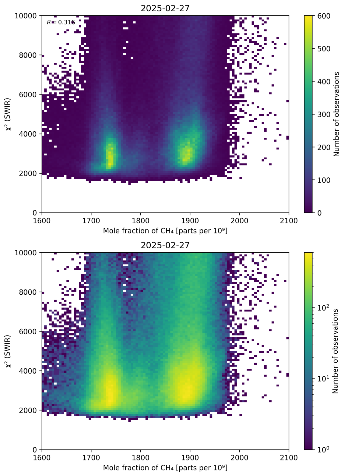
Figure 71: Scatter density plot of “Mole fraction of \text{CH}_4 ” against “ \chi^2 (SWIR)” for 2025-02-26 to 2025-02-28.
