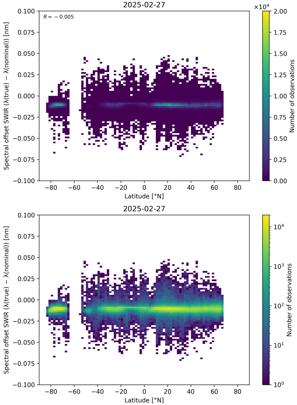
Figure 62: Scatter density plot of “Latitude” against “Spectral offset SWIR ( \lambda_{\text{true}} - \lambda_{\text{nominal}} )” for 2025-02-26 to 2025-02-28.
