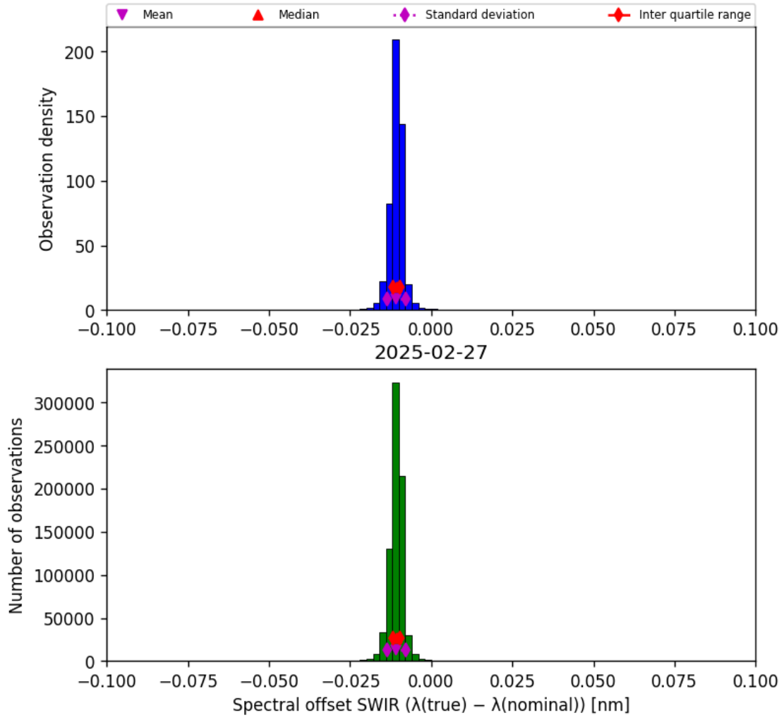
Figure 27: Histogram of “Spectral offset SWIR ( \lambda_{\text{true}} - \lambda_{\text{nominal}} )” for 2025-02-26 to 2025-02-28
