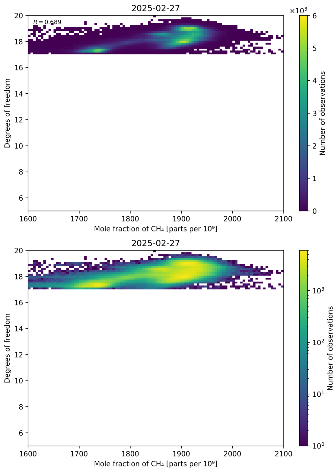
Figure 72: Scatter density plot of “Mole fraction of CH 4 ” against “Degrees of freedom” for 2025-02-26 to 2025-02-28.
