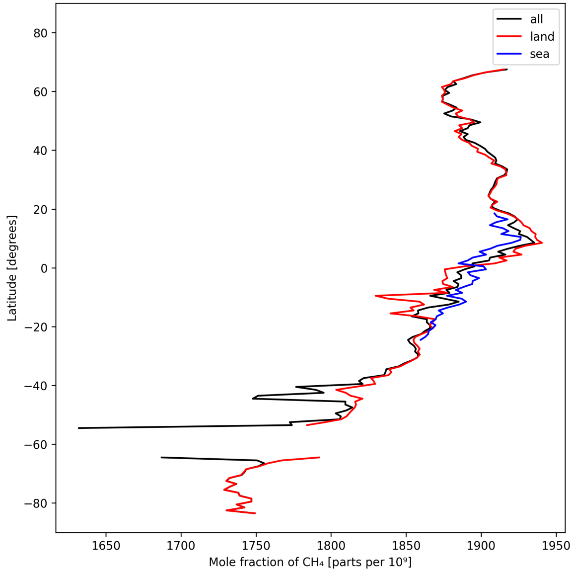
Figure 12: Zonal average of “Mole fraction of CH 4 ” for 2025-02-26 to 2025-02-28.
