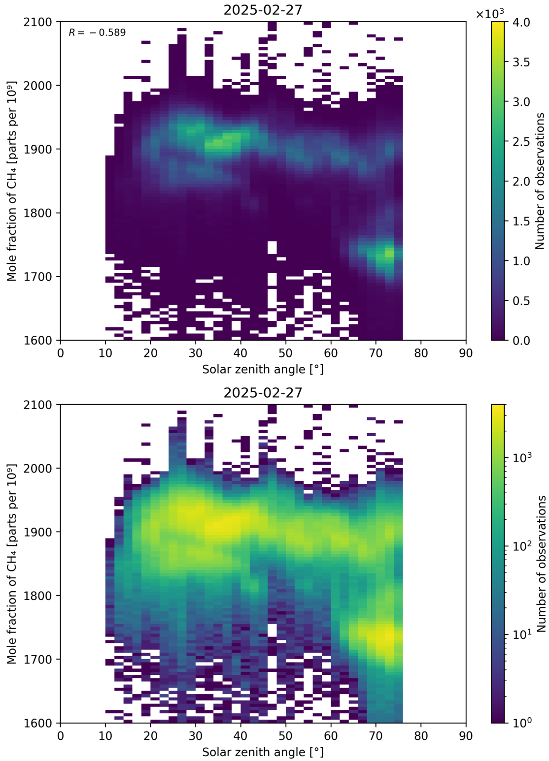
Figure 99: Scatter density plot of “Solar zenith angle” against “Mole fraction of CH 4 ” for 2025-02-26 to 2025-02-28.
