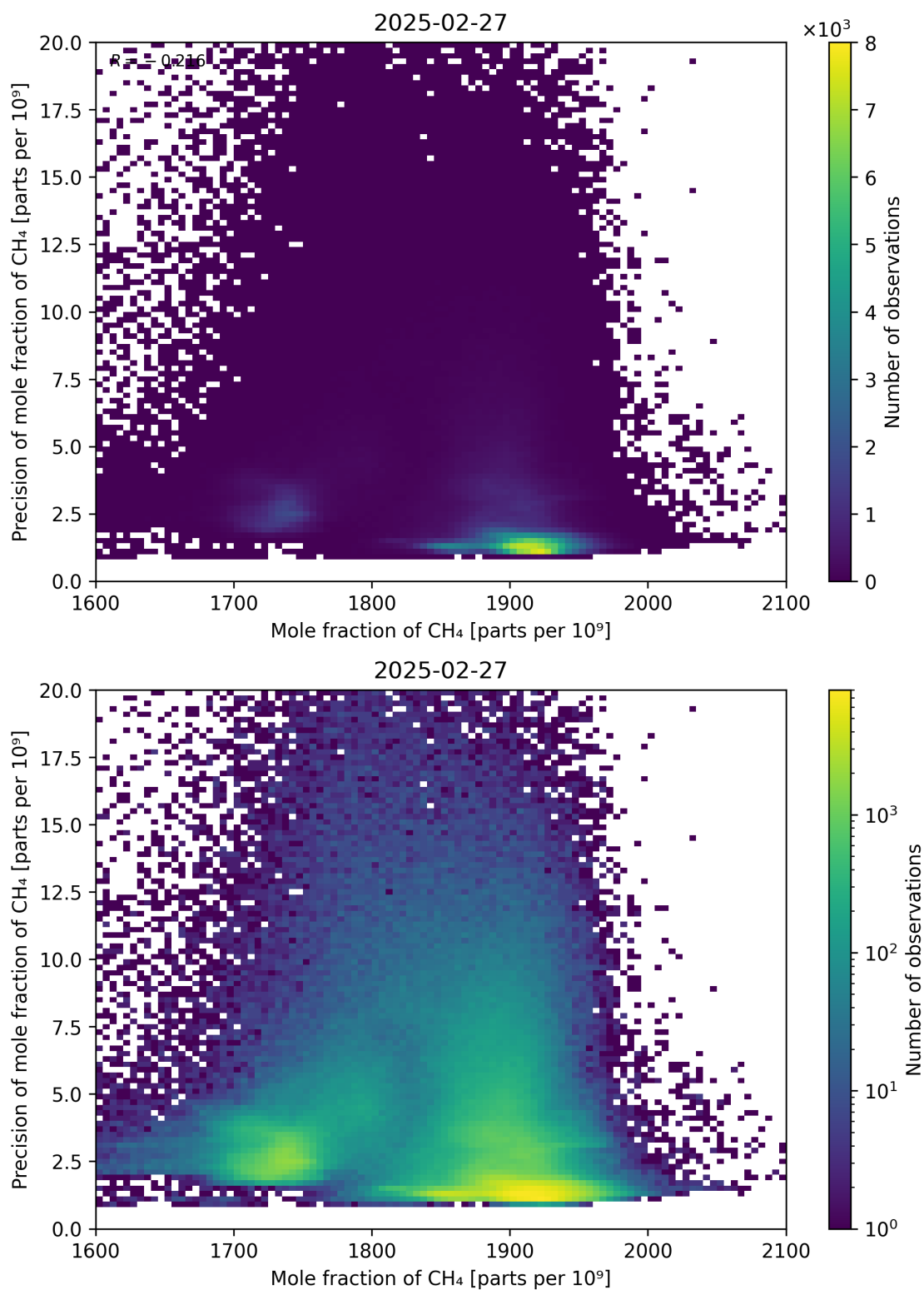
Figure 75: Scatter density plot of “Mole fraction of CH 4 ” against “Precision of mole fraction of CH 4 ” for 2025-02-26 to 2025-02-28.
