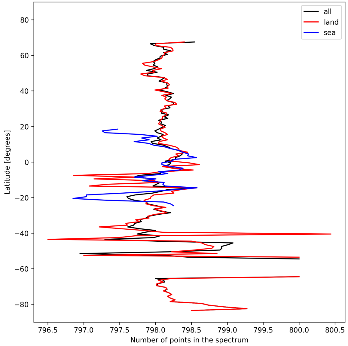
Figure 15: Zonal average of “Number of points in the spectrum” for 2025-02-26 to 2025-02-28.
