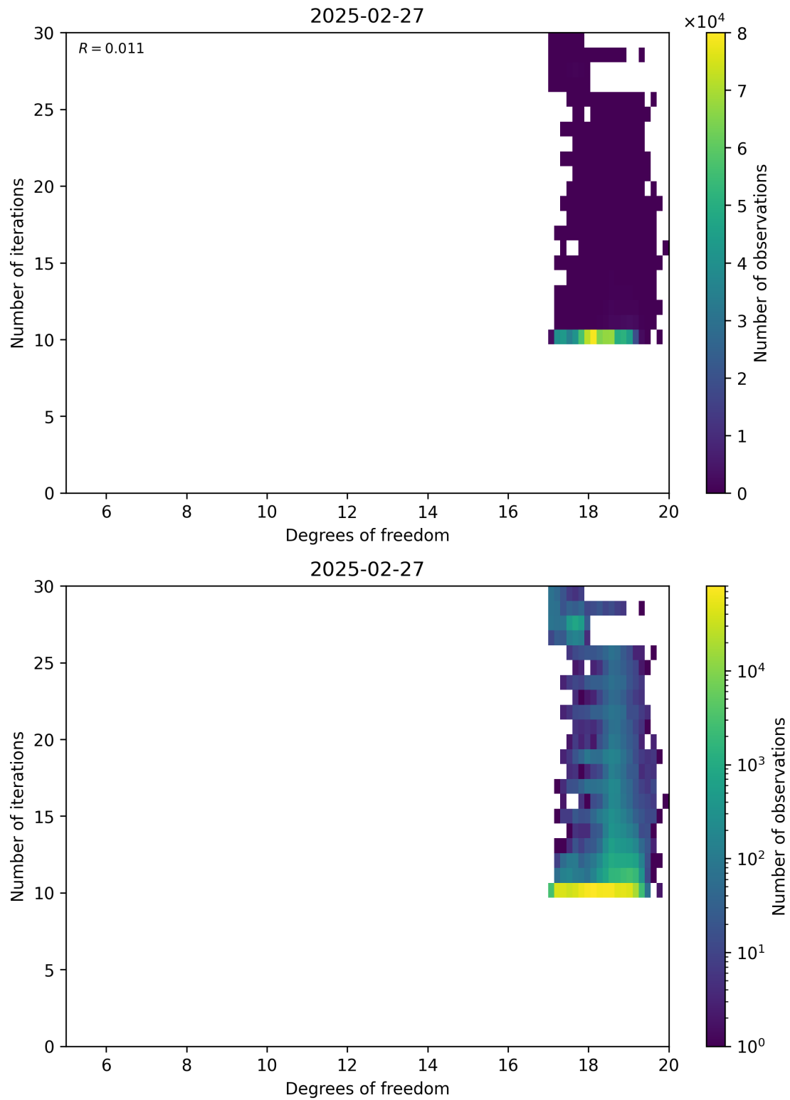
Figure 52: Scatter density plot of “Degrees of freedom” against “Number of iterations” for 2025-02-26 to 2025-02-28.
