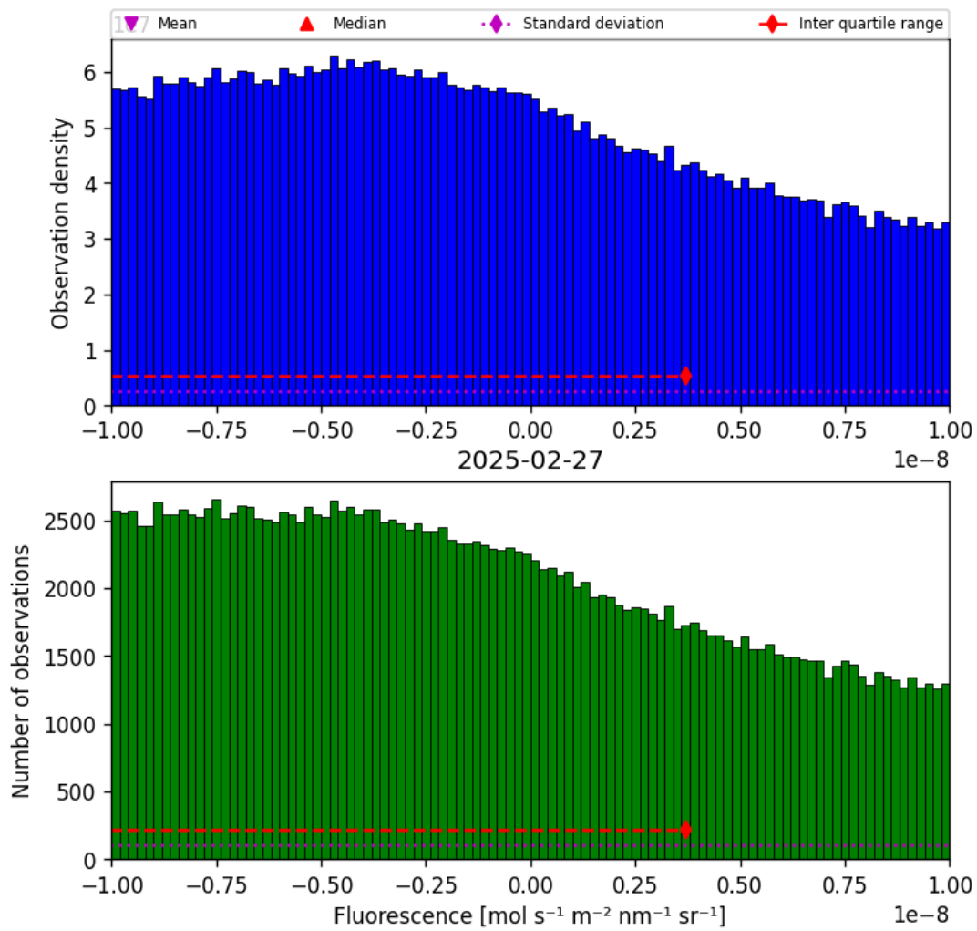
Figure 32: Histogram of “Fluorescence” for 2025-02-26 to 2025-02-28
