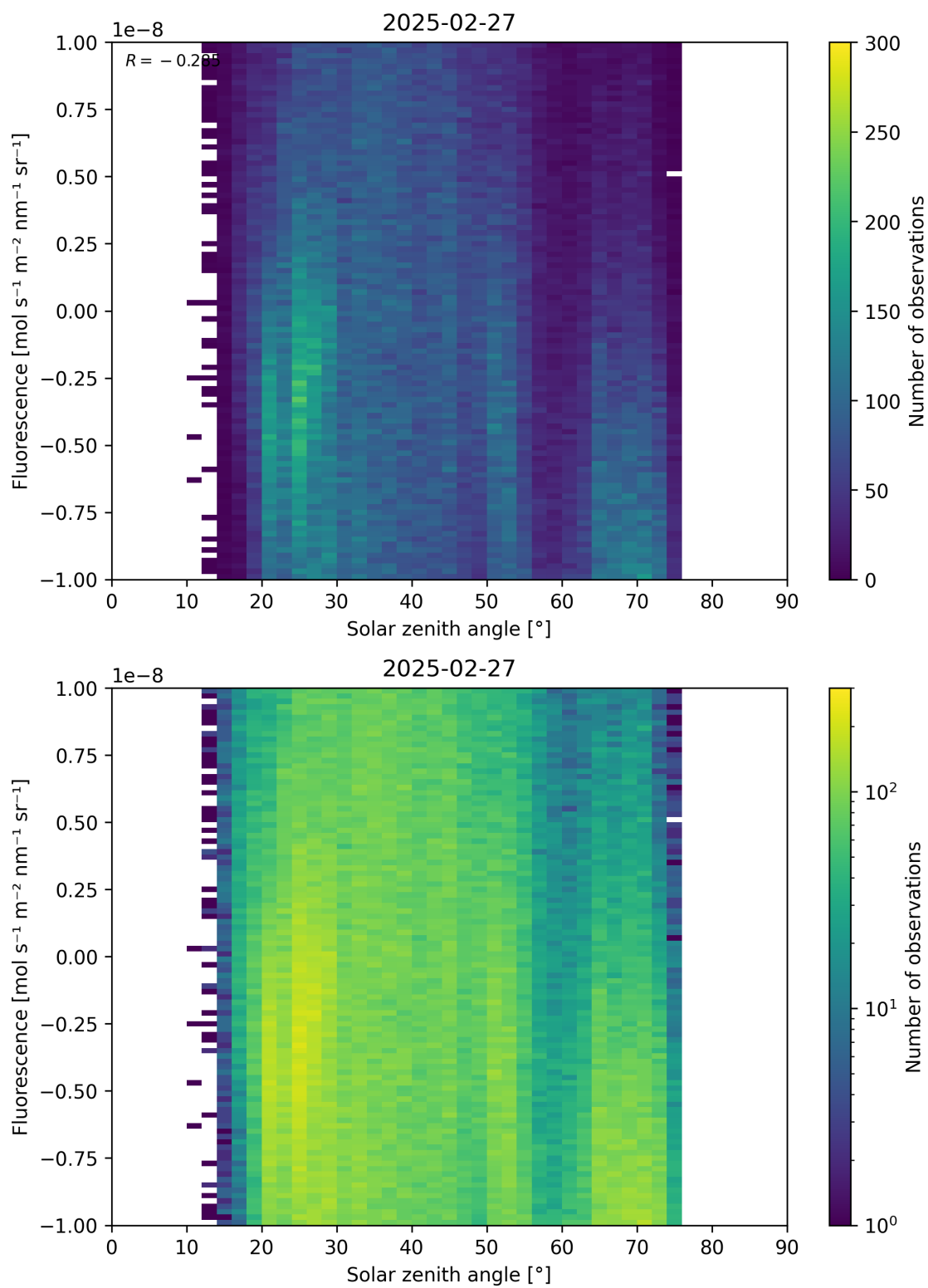
Figure 97: Scatter density plot of “Solar zenith angle” against “Fluorescence” for 2025-02-26 to 2025-02-28.
