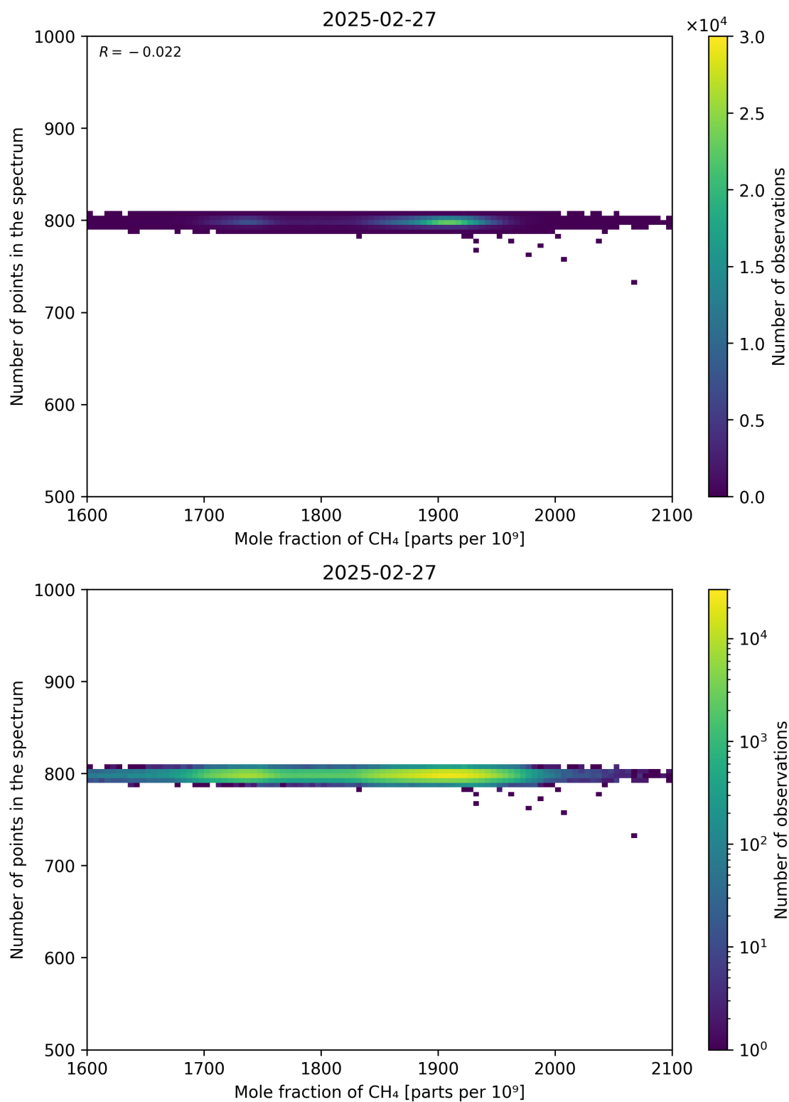
Figure 77: Scatter density plot of “Mole fraction of CH 4 ” against “Number of points in the spectrum” for 2025-02-26 to 2025-02-28.
