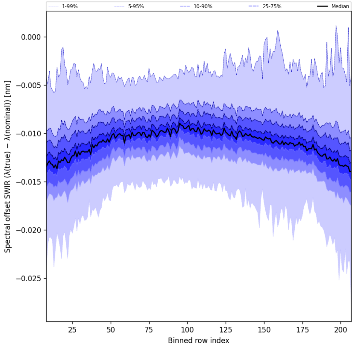
Figure 38: Along track statistics of “Spectral offset SWIR ( \lambda_{\text{true}} - \lambda_{\text{nominal}} )” for 2025-02-26 to 2025-02-28
