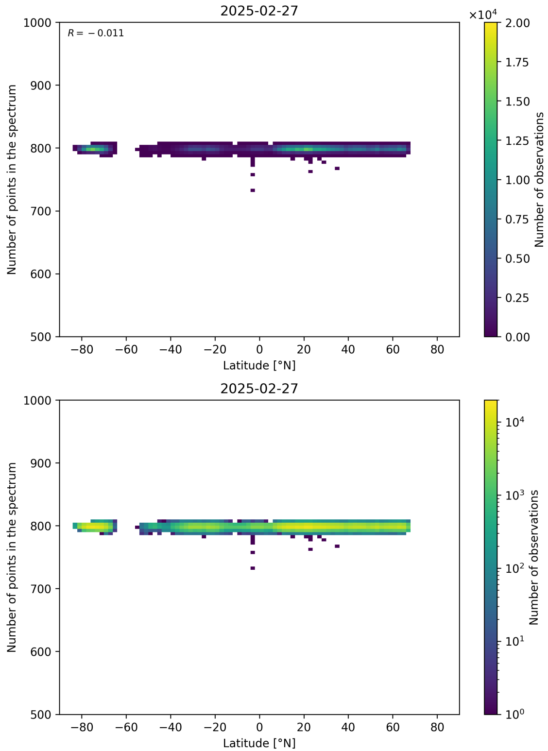
Figure 61: Scatter density plot of “Latitude” against “Number of points in the spectrum” for 2025-02-26 to 2025-02-28.
