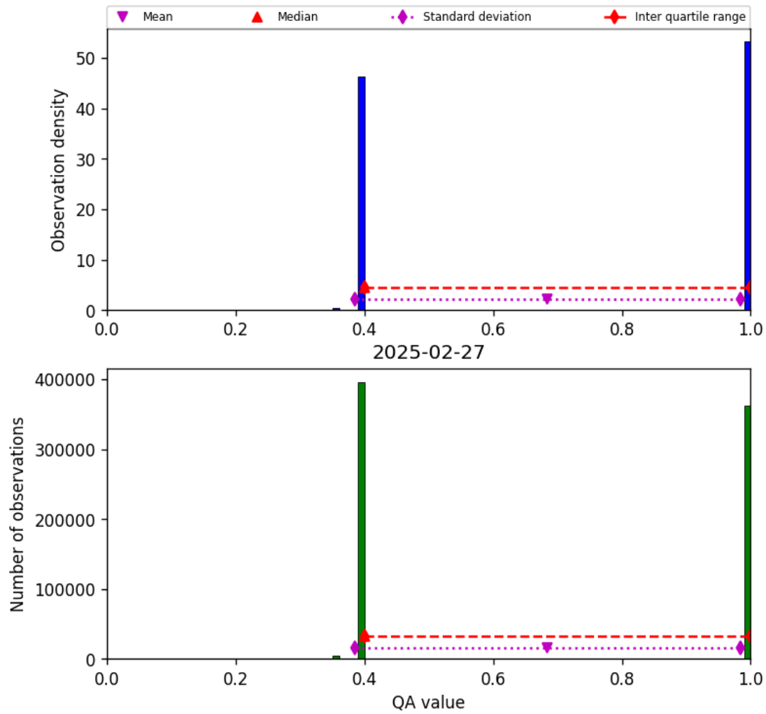
Figure 22: Histogram of “QA value” for 2025-02-26 to 2025-02-28
