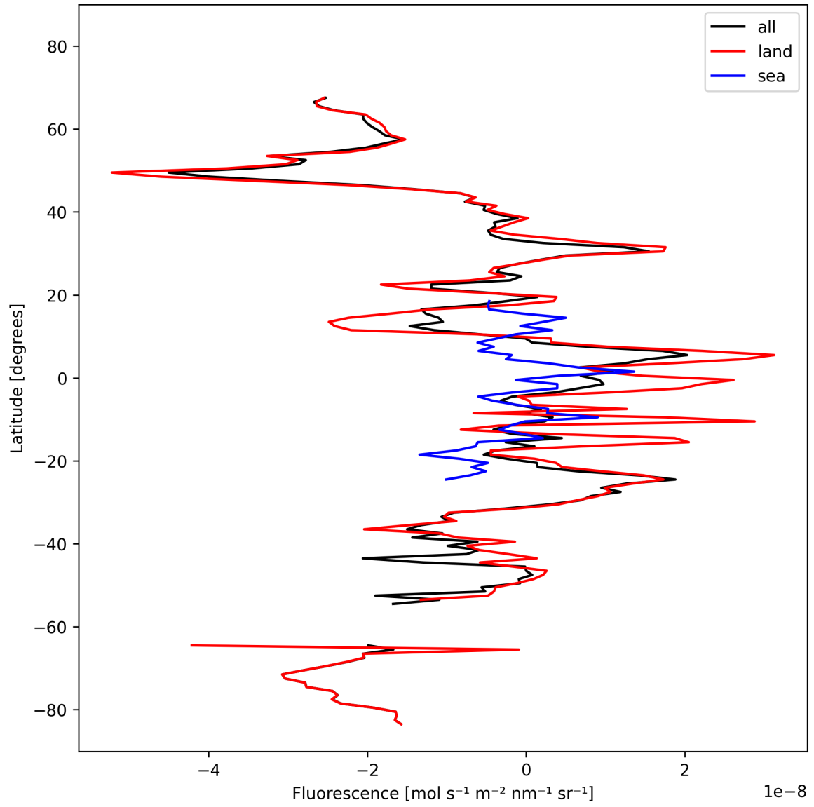
Figure 21: Zonal average of “Fluorescence” for 2025-02-26 to 2025-02-28.
