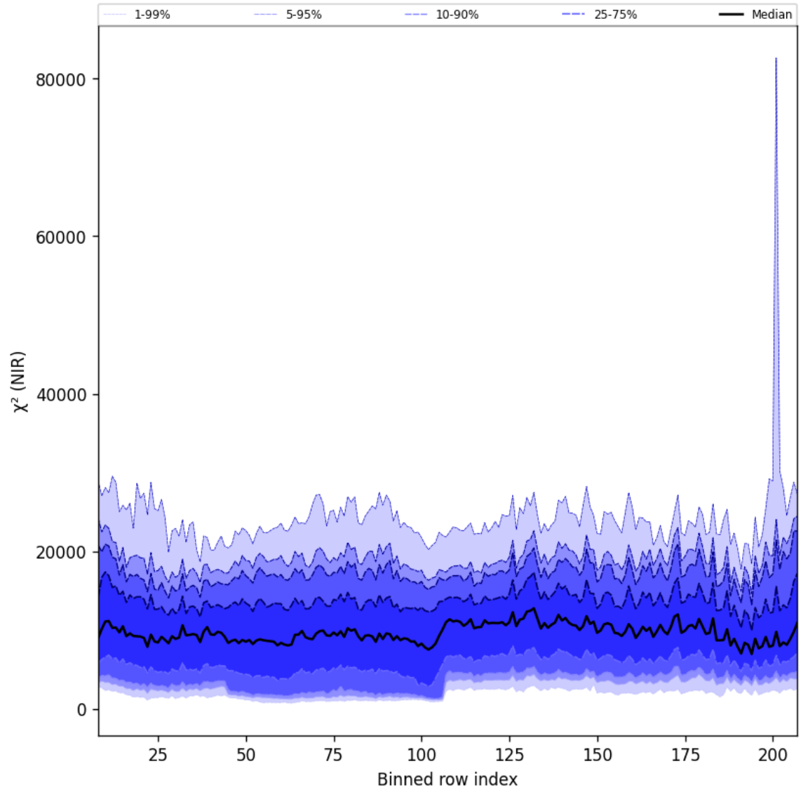
Figure 40: Along track statistics of “ \chi^2 (NIR)” for 2025-02-26 to 2025-02-28
