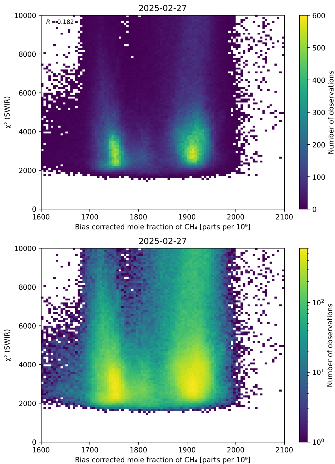
Figure 64: Scatter density plot of “Bias corrected mole fraction of CH 4 ” against “ \chi^2 (SWIR)” for 2025-02-26 to 2025-02-28.
