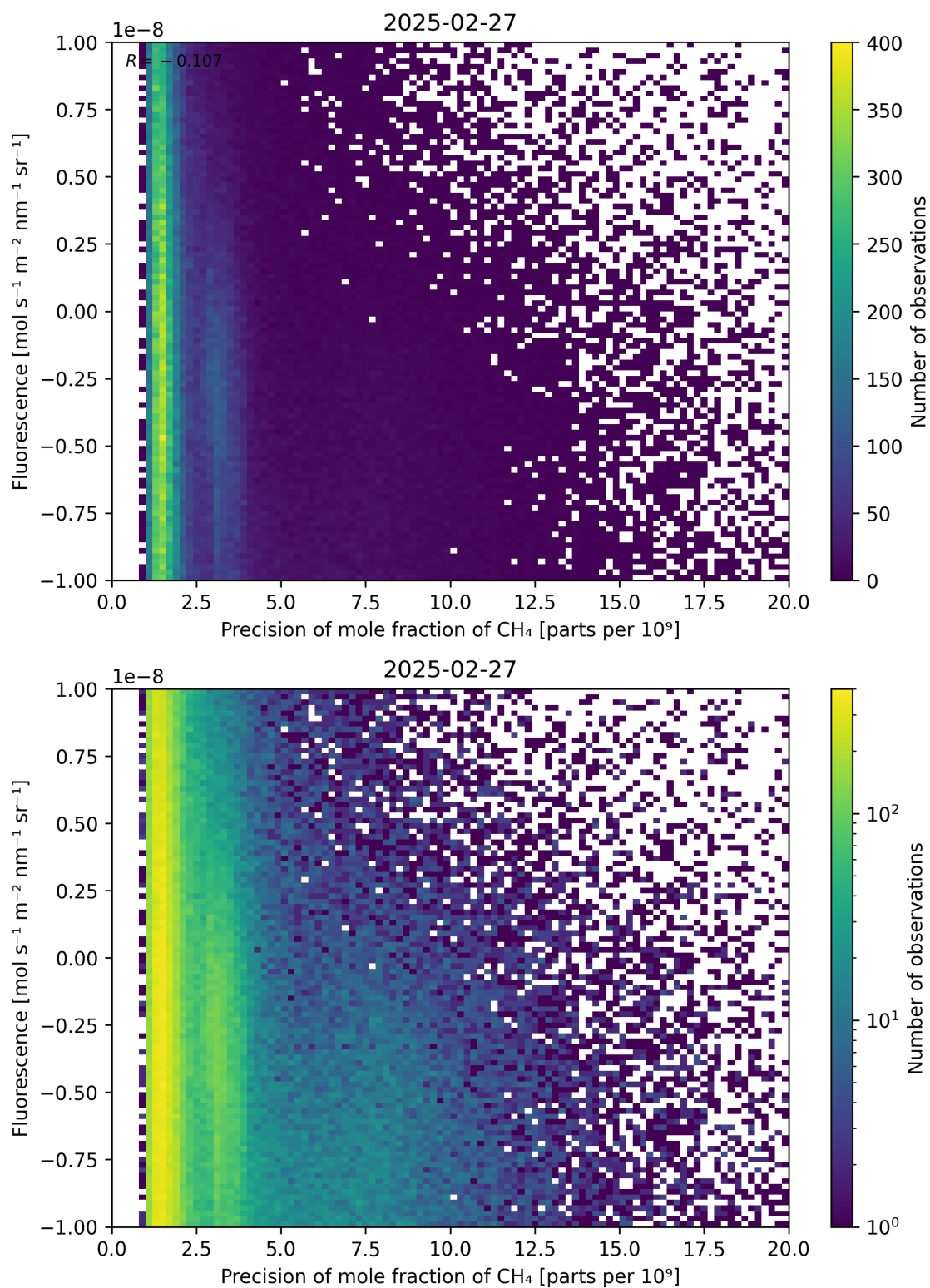
Figure 81: Scatter density plot of “Precision of mole fraction of CH 4 ” against “Fluorescence” for 2025-02-26 to 2025-02-28.
