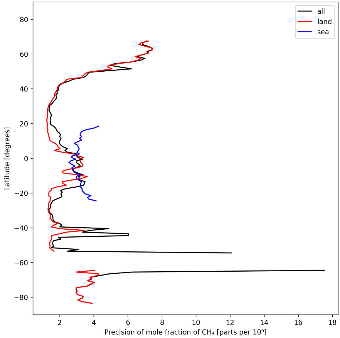
Figure 13: Zonal average of “Precision of mole fraction of CH 4 ” for 2025-02-26 to 2025-02-28.
