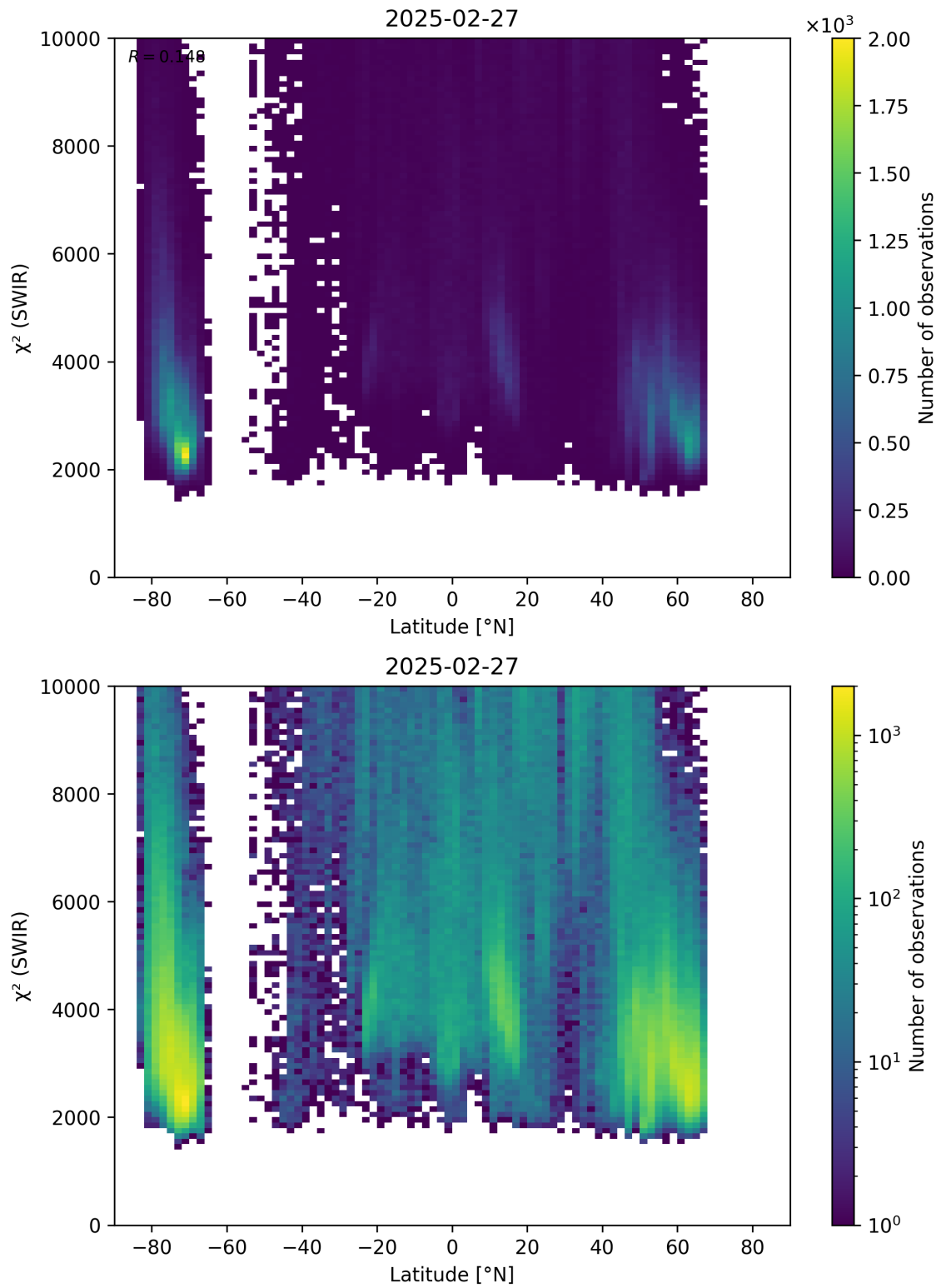
Figure 54: Scatter density plot of “Latitude” against “ \chi^2 (SWIR)” for 2025-02-26 to 2025-02-28.
