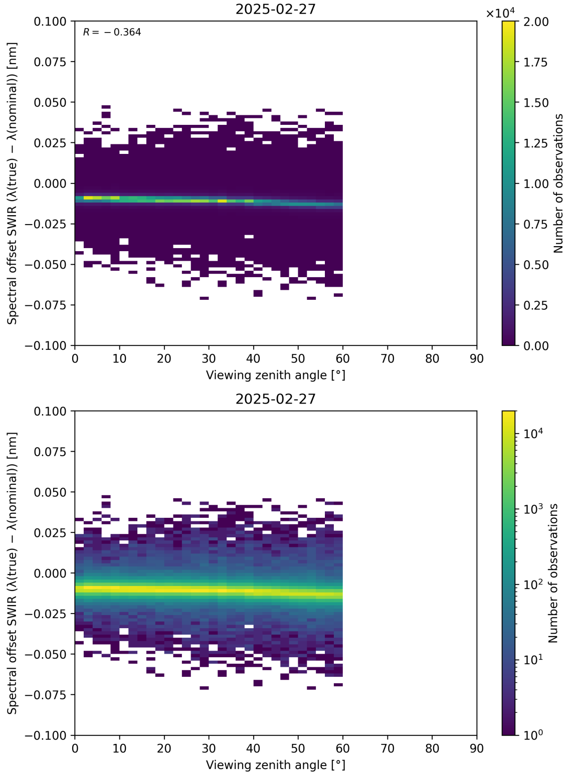
Figure 116: Scatter density plot of “Viewing zenith angle” against “Spectral offset SWIR ( \lambda_{\text{true}} - \lambda_{\text{nominal}} )” for 2025-02-26 to 2025-02-28.
