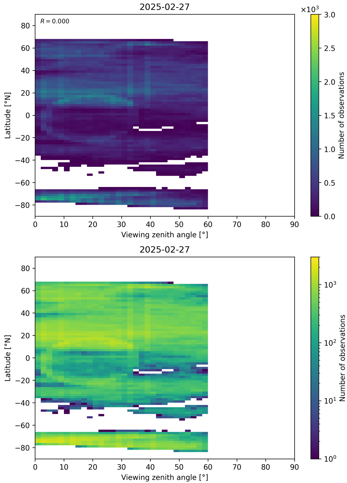
Figure 109: Scatter density plot of “Viewing zenith angle” against “Latitude” for 2025-02-26 to 2025-02-28.
