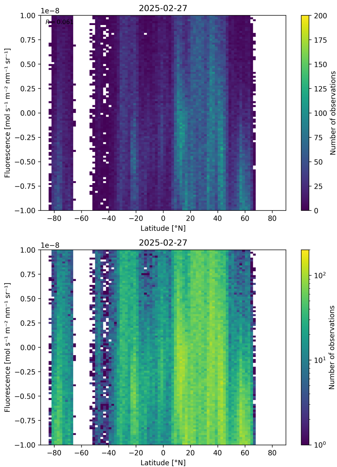
Figure 56: Scatter density plot of “Latitude” against “Fluorescence” for 2025-02-26 to 2025-02-28.
