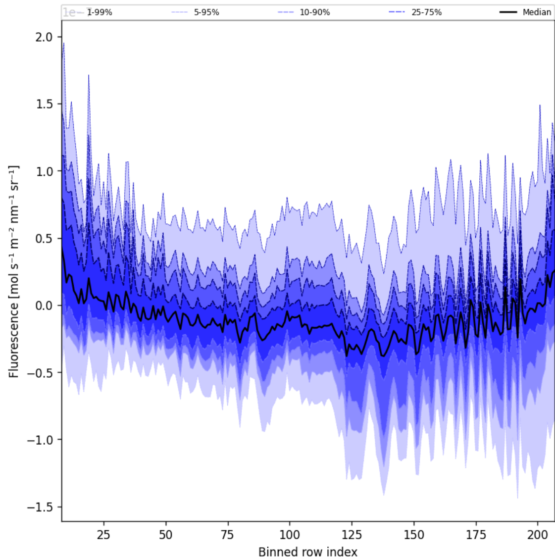
Figure 43: Along track statistics of “Fluorescence” for 2025-02-26 to 2025-02-28
