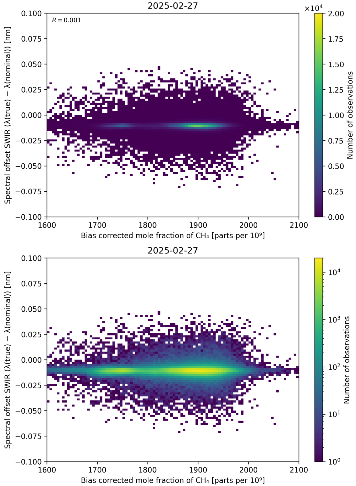
Figure 69: Scatter density plot of “Bias corrected mole fraction of \text{CH}_4 ” against “Spectral offset SWIR ( \lambda_{\text{true}} - \lambda_{\text{nominal}} )” for 2025-02-26 to 2025-02-28.
