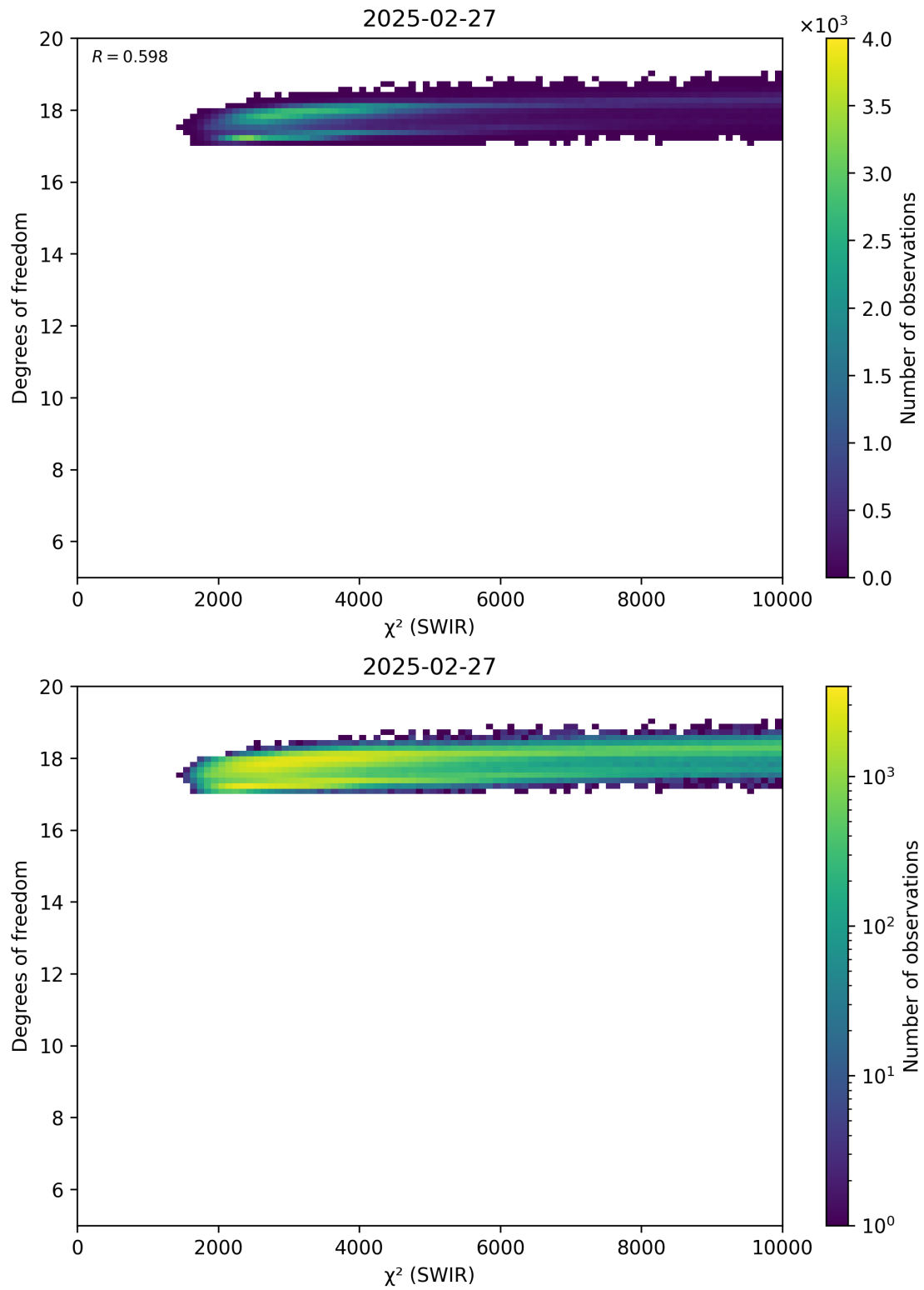
Figure 48: Scatter density plot of “ \chi^2 (SWIR)” against “Degrees of freedom” for 2025-02-26 to 2025-02-28.
