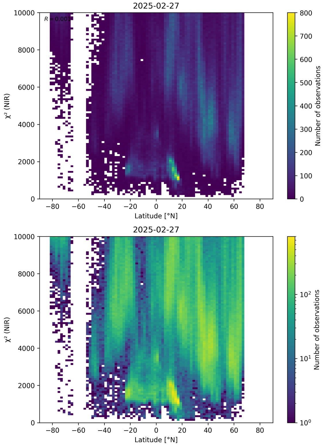
Figure 53: Scatter density plot of “Latitude” against “ \chi^2 (NIR)” for 2025-02-26 to 2025-02-28.
