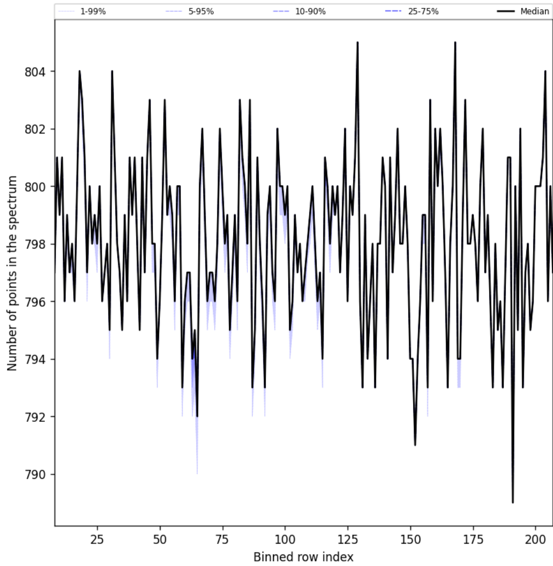
Figure 37: Along track statistics of “Number of points in the spectrum” for 2025-02-26 to 2025-02-28
