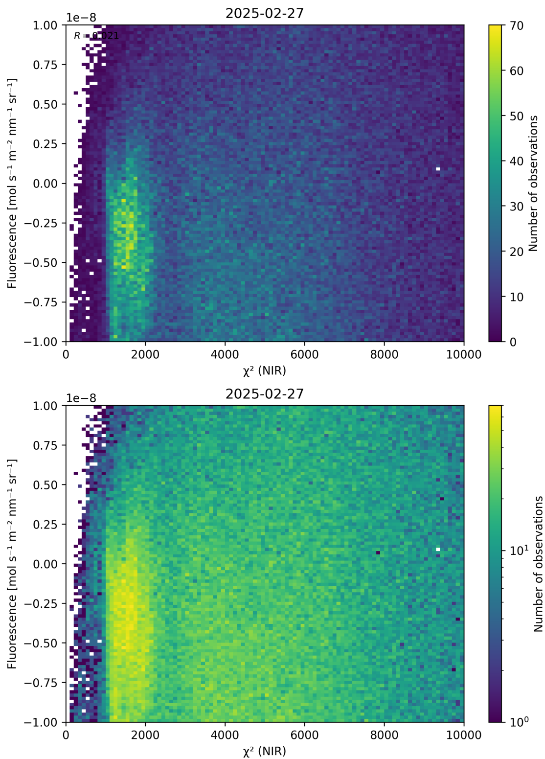
Figure 45: Scatter density plot of “ \chi^2 (NIR)” against “Fluorescence” for 2025-02-26 to 2025-02-28.
