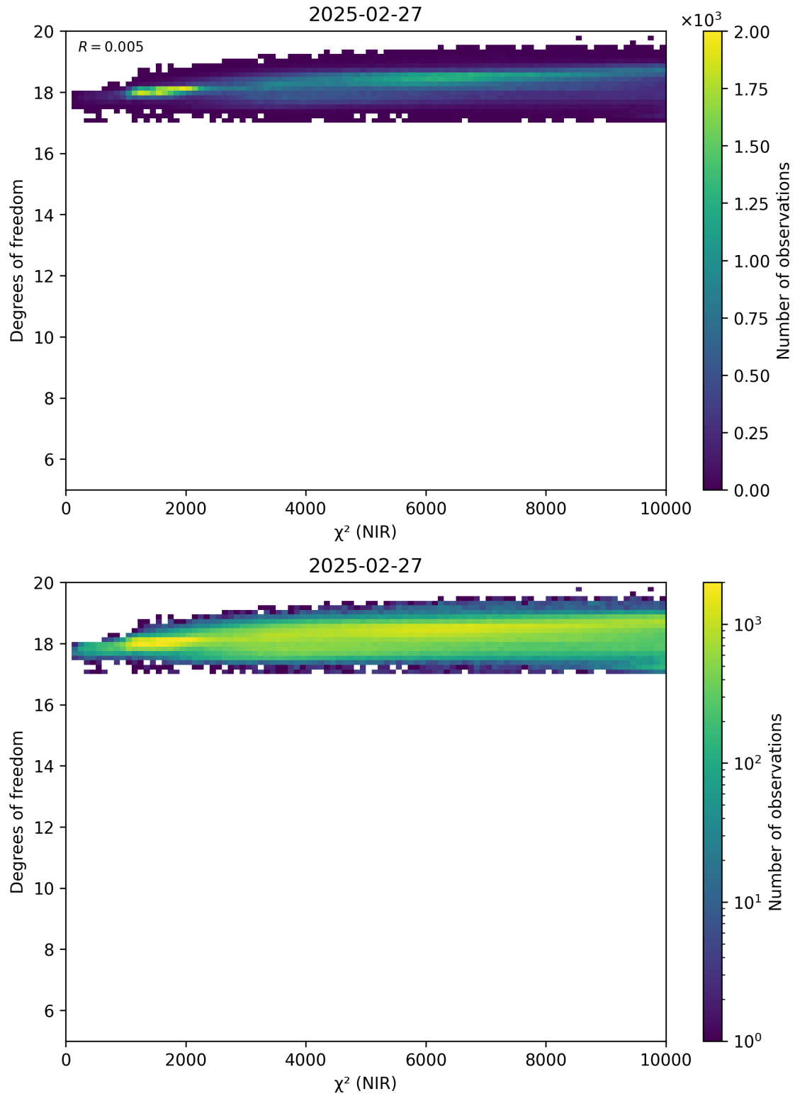
Figure 44: Scatter density plot of “ \chi^2 (NIR)” against “Degrees of freedom” for 2025-02-26 to 2025-02-28.
