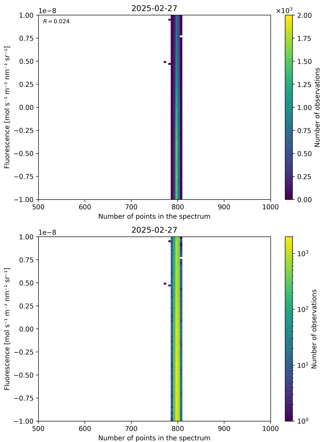
Figure 91: Scatter density plot of “Number of points in the spectrum” against “Fluorescence” for 2025-02-26 to 2025-02-28.
