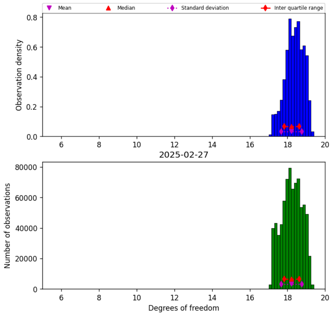
Figure 30: Histogram of “Degrees of freedom” for 2025-02-26 to 2025-02-28
