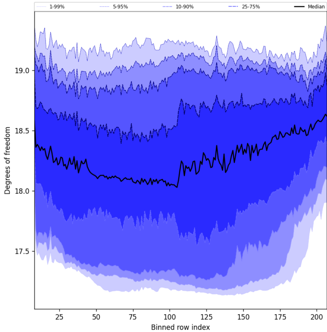
Figure 41: Along track statistics of “Degrees of freedom” for 2025-02-26 to 2025-02-28
