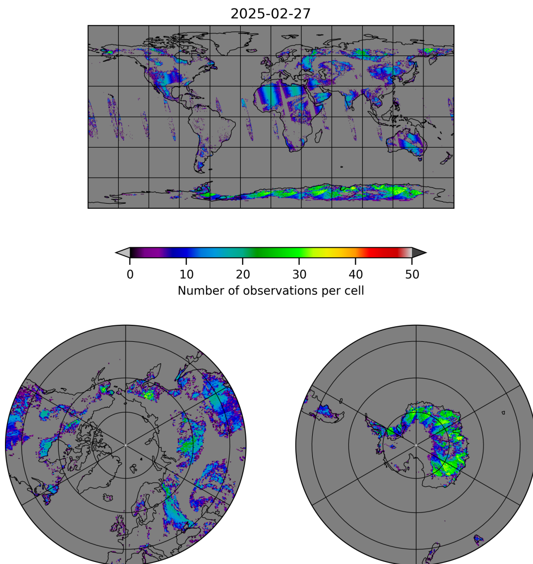
Figure 10: Map of the number of observations for 2025-02-26 to 2025-02-28
