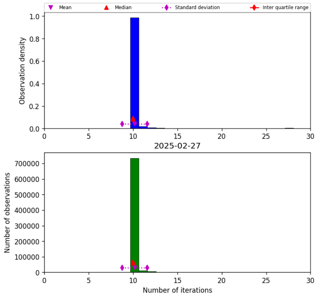
Figure 31: Histogram of “Number of iterations” for 2025-02-26 to 2025-02-28
