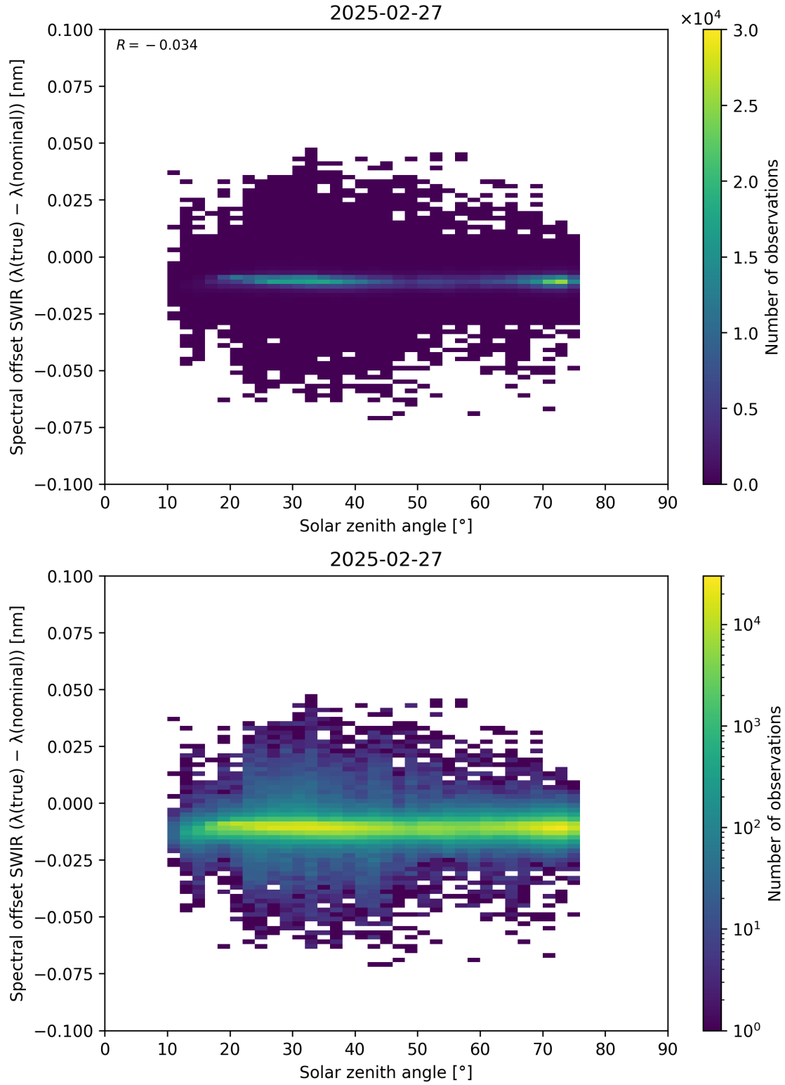
Figure 104: Scatter density plot of “Solar zenith angle” against “Spectral offset SWIR ( \lambda_{\text{true}} - \lambda_{\text{nominal}} )” for 2025-02-26 to 2025-02-28.
