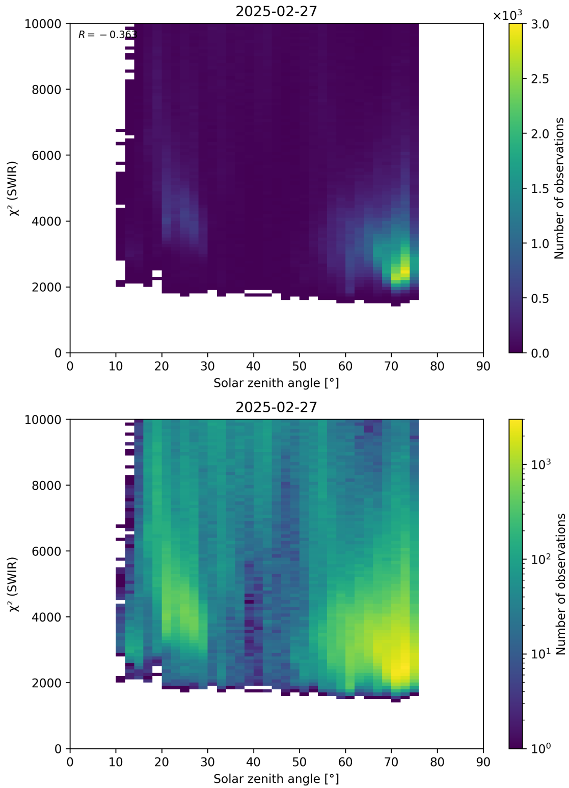
Figure 95: Scatter density plot of “Solar zenith angle” against “ \chi^2 (SWIR)” for 2025-02-26 to 2025-02-28.
