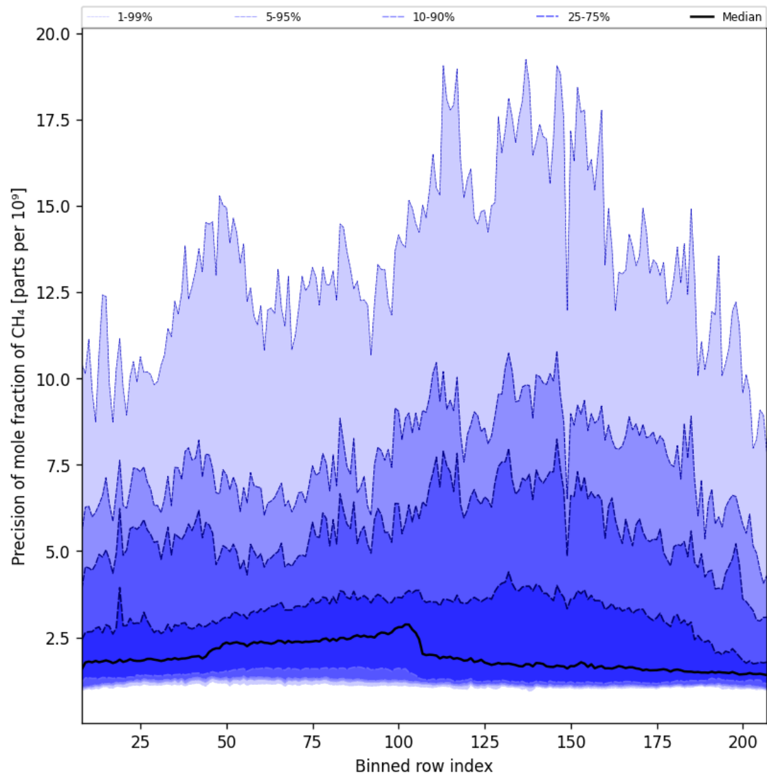
Figure 35: Along track statistics of “Precision of mole fraction of CH 4 ” for 2025-02-26 to 2025-02-28
