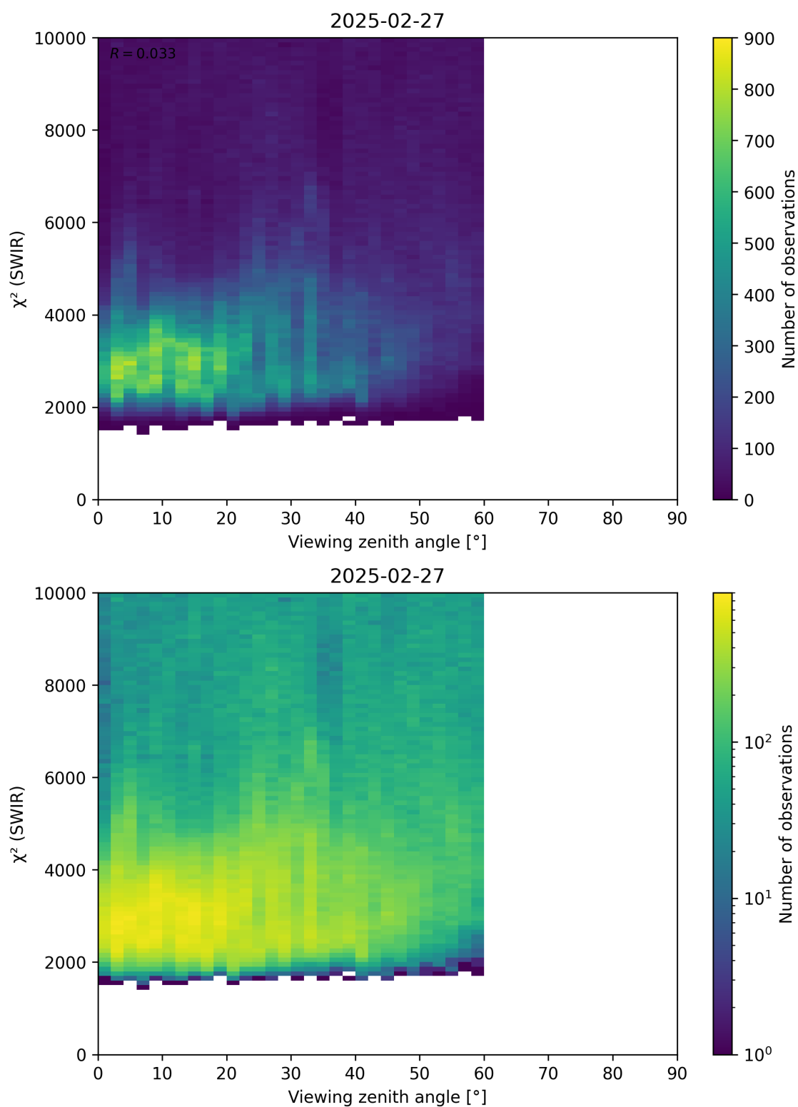
Figure 106: Scatter density plot of “Viewing zenith angle” against “ \chi^2 (SWIR)” for 2025-02-26 to 2025-02-28.
