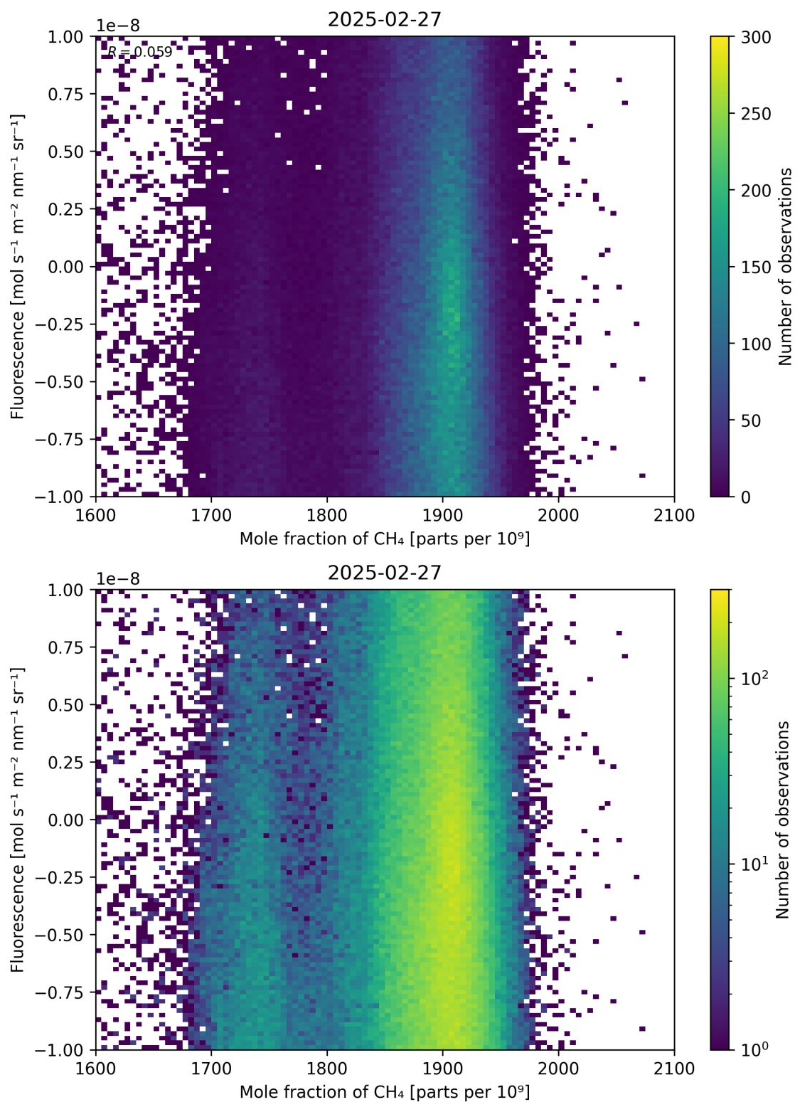
Figure 73: Scatter density plot of “Mole fraction of \text{CH}_4 ” against “Fluorescence” for 2025-02-26 to 2025-02-28.
