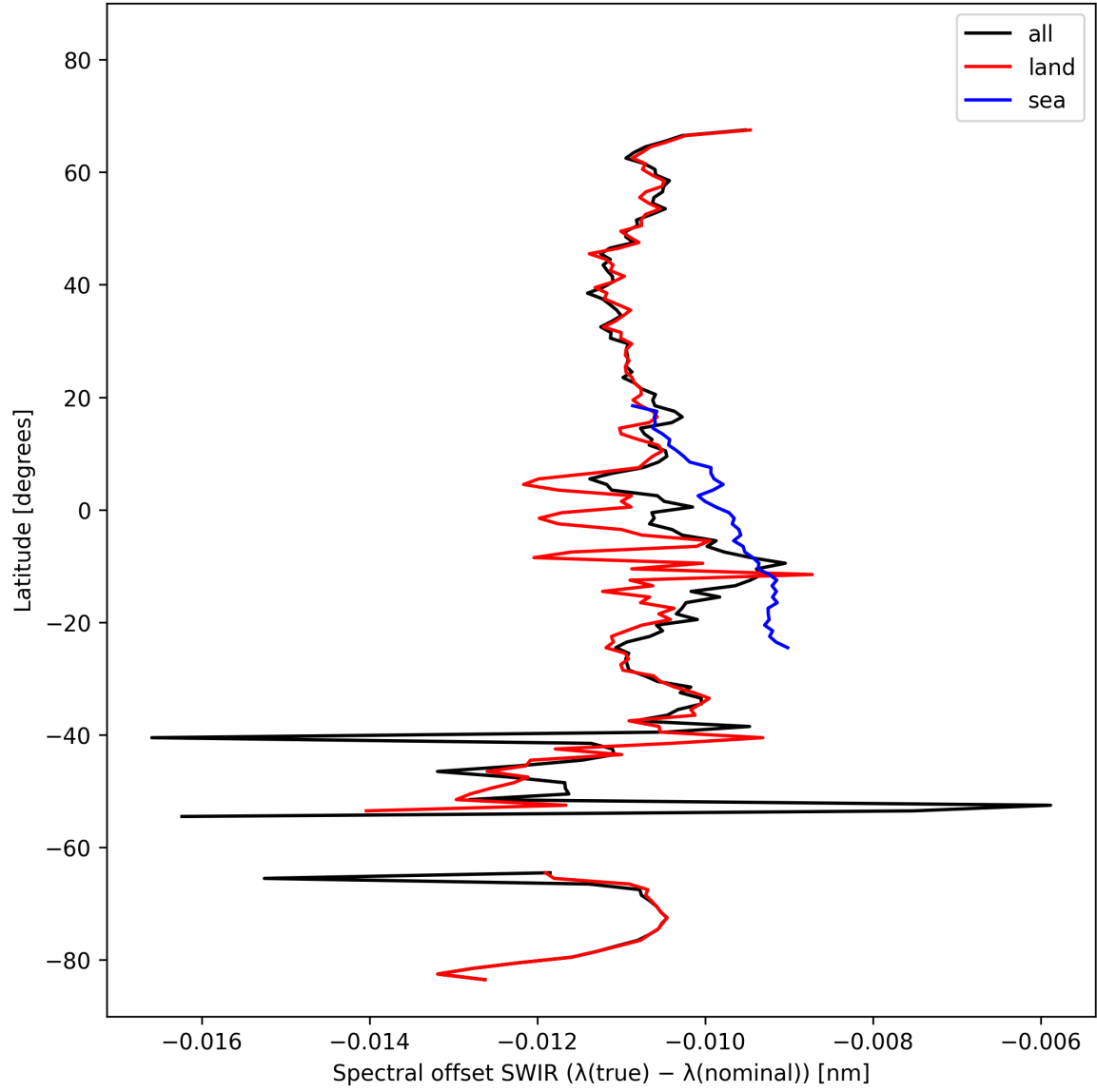
Figure 16: Zonal average of “Spectral offset SWIR ( \lambda_{\text{true}} - \lambda_{\text{nominal}} )” for 2025-02-26 to 2025-02-28.
