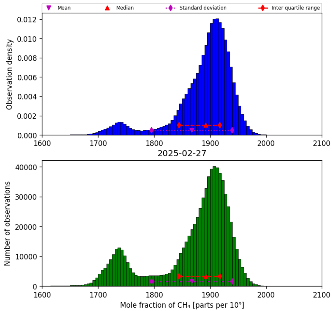
Figure 23: Histogram of “Mole fraction of CH 4 ” for 2025-02-26 to 2025-02-28
