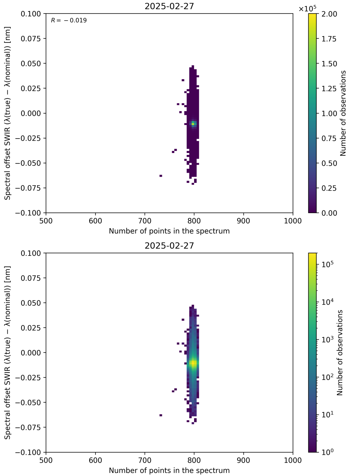
Figure 93: Scatter density plot of “Number of points in the spectrum” against “Spectral offset SWIR ( \lambda_{\text{true}} - \lambda_{\text{nominal}} )” for 2025-02-26 to 2025-02-28.
