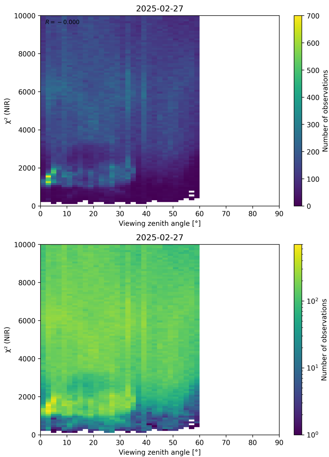
Figure 105: Scatter density plot of “Viewing zenith angle” against “ \chi^2 (NIR)” for 2025-02-26 to 2025-02-28.
