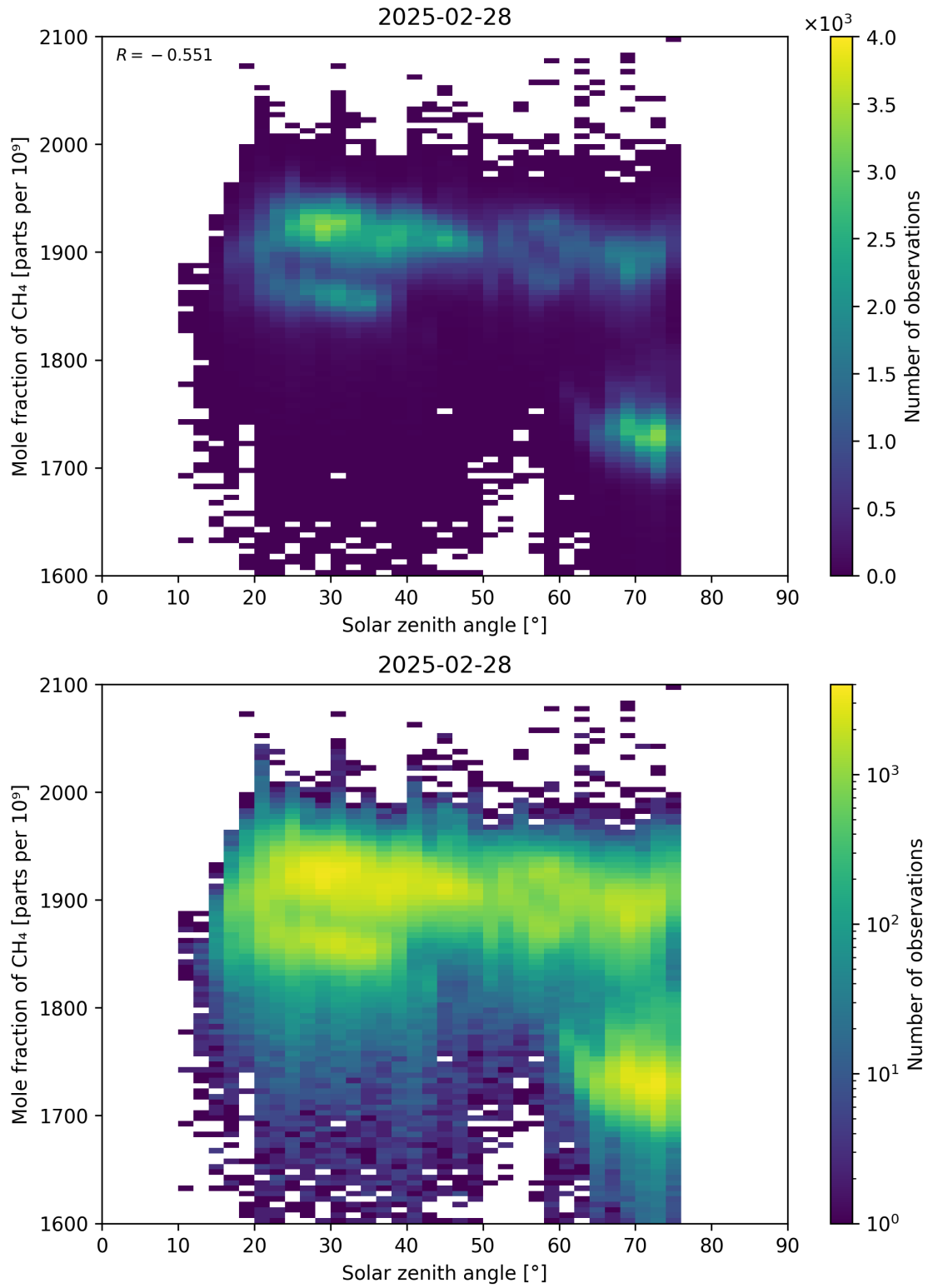
Figure 99: Scatter density plot of “Solar zenith angle” against “Mole fraction of CH 4 ” for 2025-02-27 to 2025-03-01.
