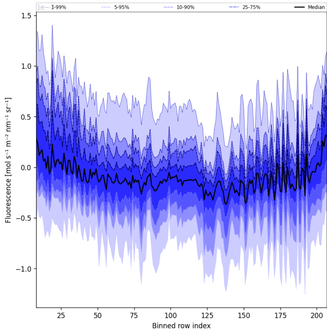
Figure 43: Along track statistics of "Fluorescence" for 2025-02-27 to 2025-03-01
