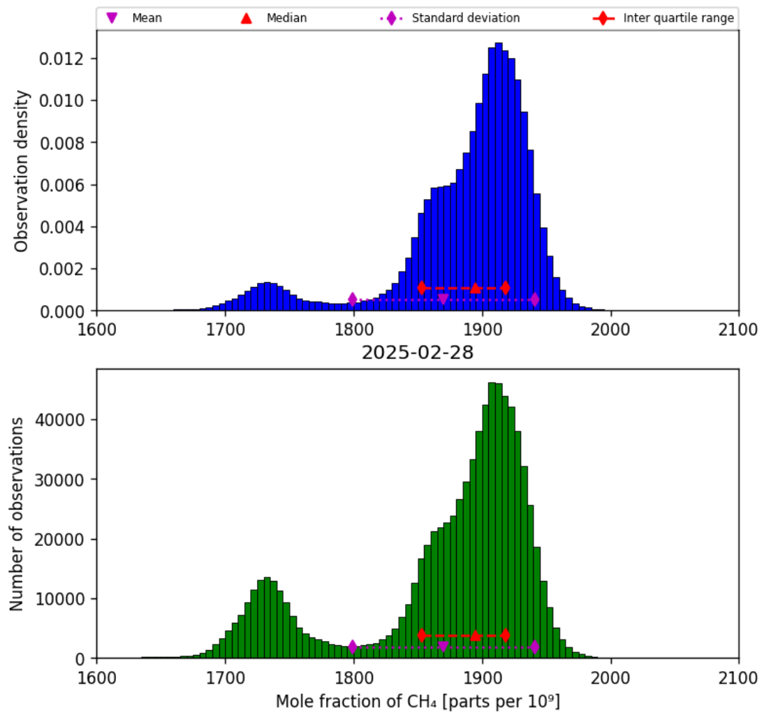
Figure 23: Histogram of “Mole fraction of CH 4 ” for 2025-02-27 to 2025-03-01
