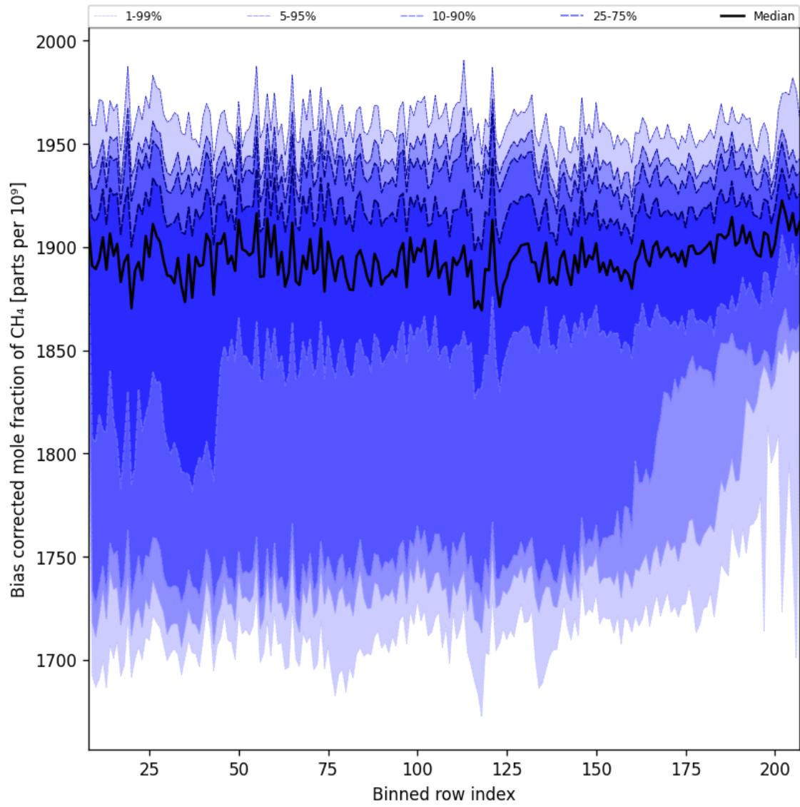
Figure 36: Along track statistics of “Bias corrected mole fraction of CH 4 ” for 2025-02-27 to 2025-03-01
