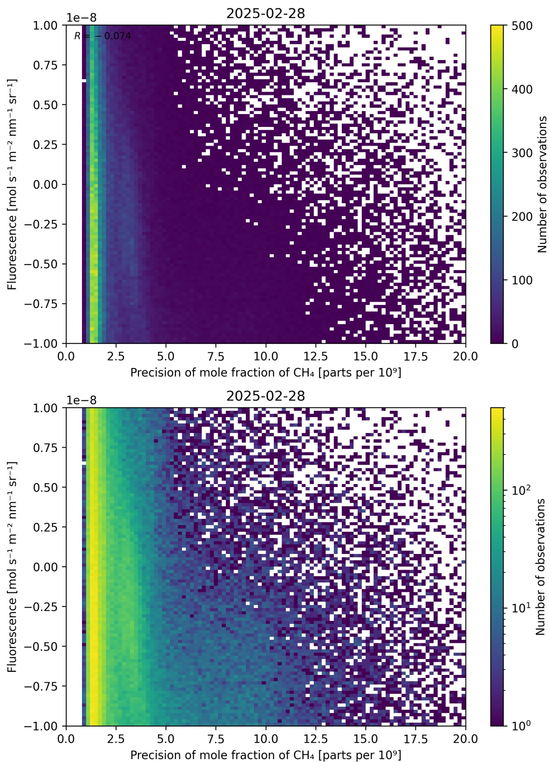
Figure 81: Scatter density plot of “Precision of mole fraction of CH 4 ” against “Fluorescence” for 2025-02-27 to 2025-03-01.
