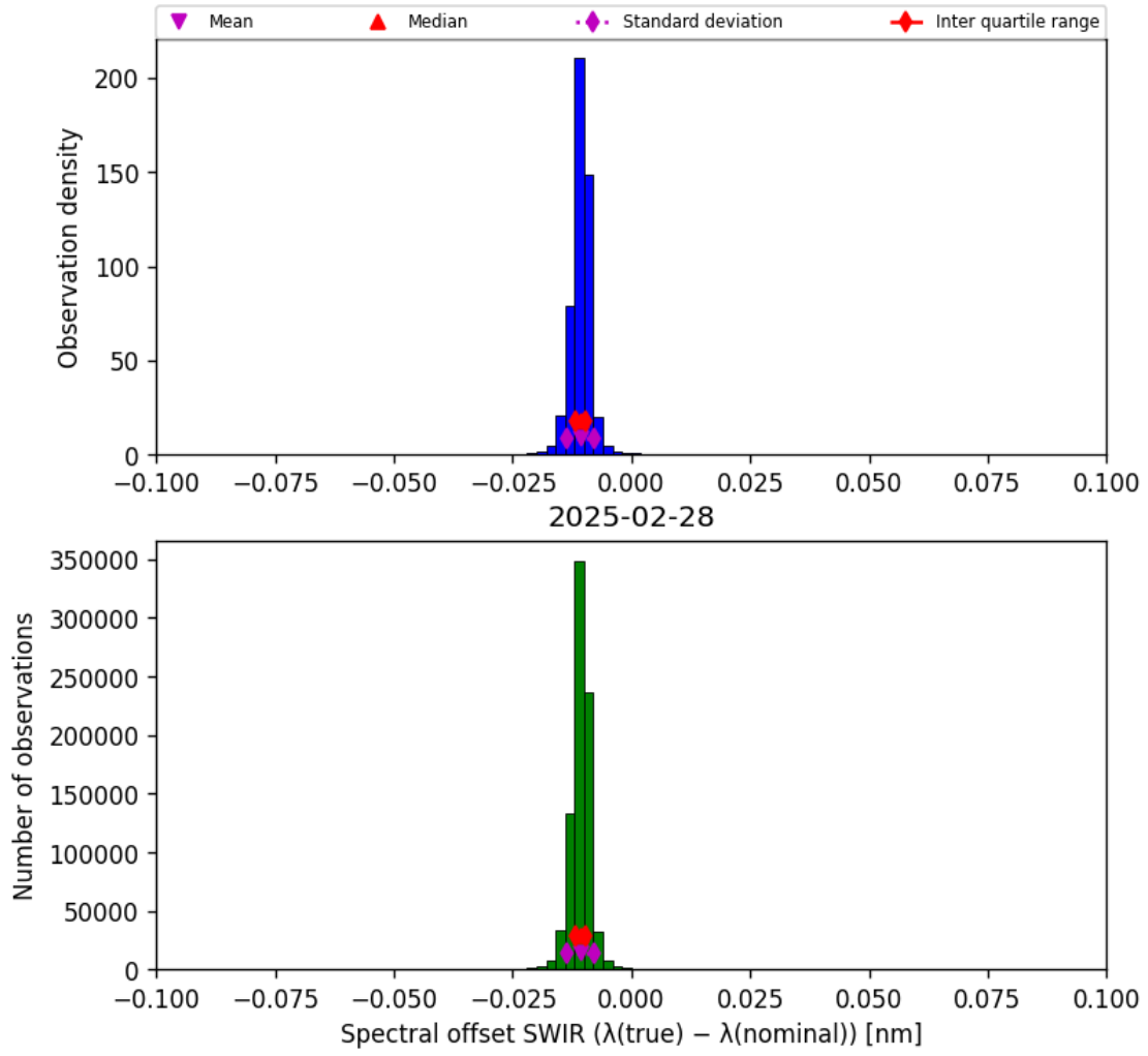
Figure 27: Histogram of “Spectral offset SWIR ( \lambda_{\text{true}} - \lambda_{\text{nominal}} )” for 2025-02-27 to 2025-03-01
