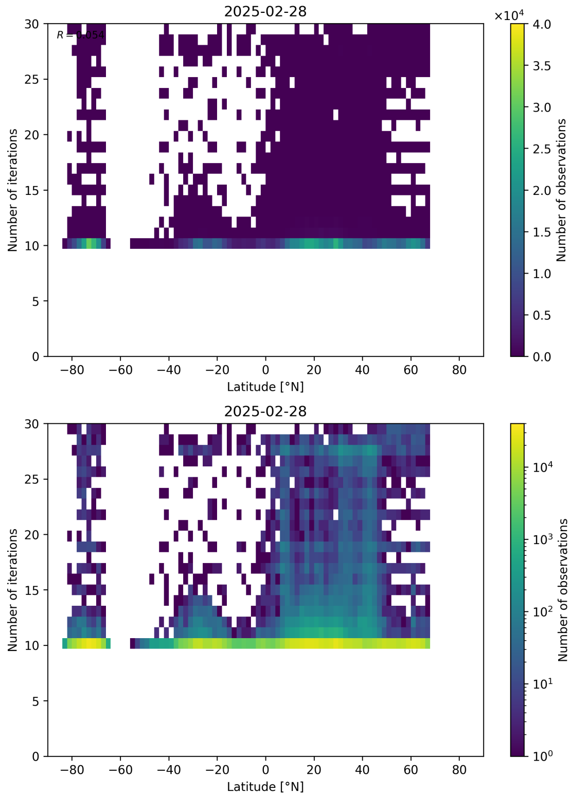
Figure 60: Scatter density plot of “Latitude” against “Number of iterations” for 2025-02-27 to 2025-03-01.
