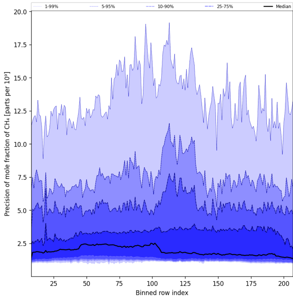
Figure 35: Along track statistics of “Precision of mole fraction of CH 4 ” for 2025-02-27 to 2025-03-01
