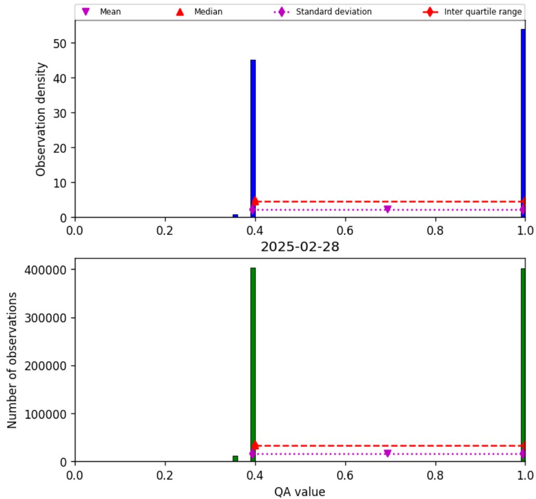
Figure 22: Histogram of “QA value” for 2025-02-27 to 2025-03-01
