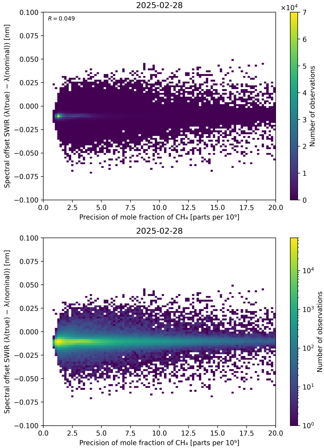
Figure 85: Scatter density plot of “Precision of mole fraction of \text{CH}_4 ” against “Spectral offset SWIR ( \lambda_{\text{true}} - \lambda_{\text{nominal}} )” for 2025-02-27 to 2025-03-01.
