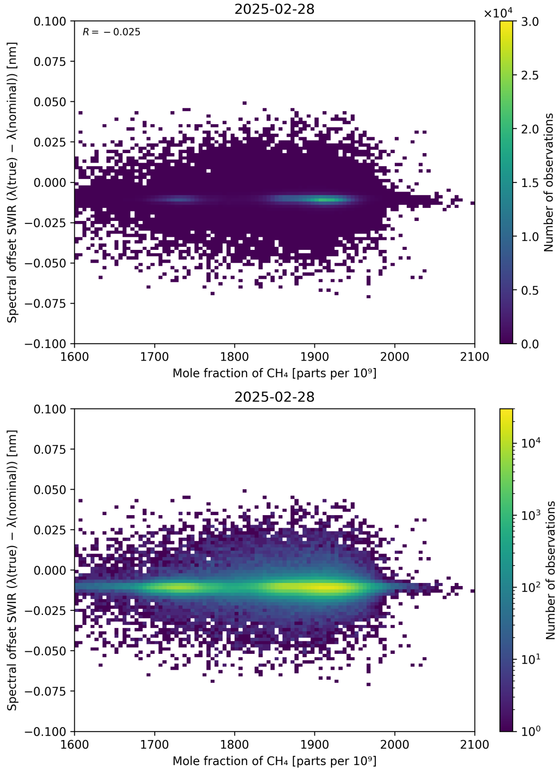
Figure 86: Scatter density plot of “Mole fraction of CH 4 ” against “Spectral offset SWIR ( \lambda_{\text{true}} - \lambda_{\text{nominal}} )” for 2025-02-27 to 2025-03-01.
