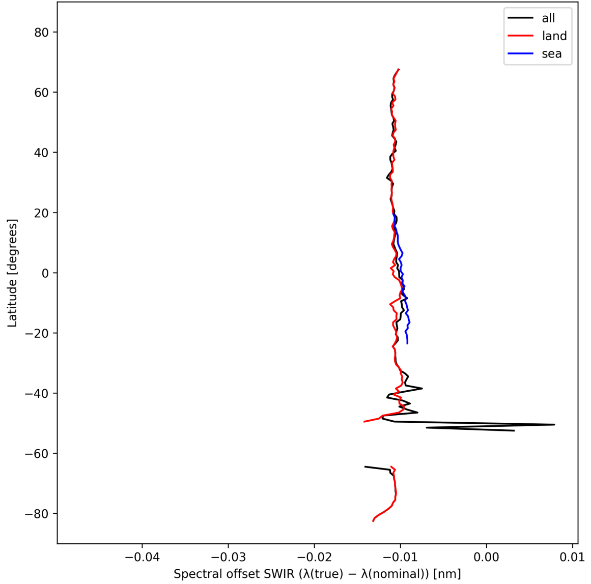
Figure 16: Zonal average of “Spectral offset SWIR ( \lambda_{\text{true}} - \lambda_{\text{nominal}} )” for 2025-02-27 to 2025-03-01.
