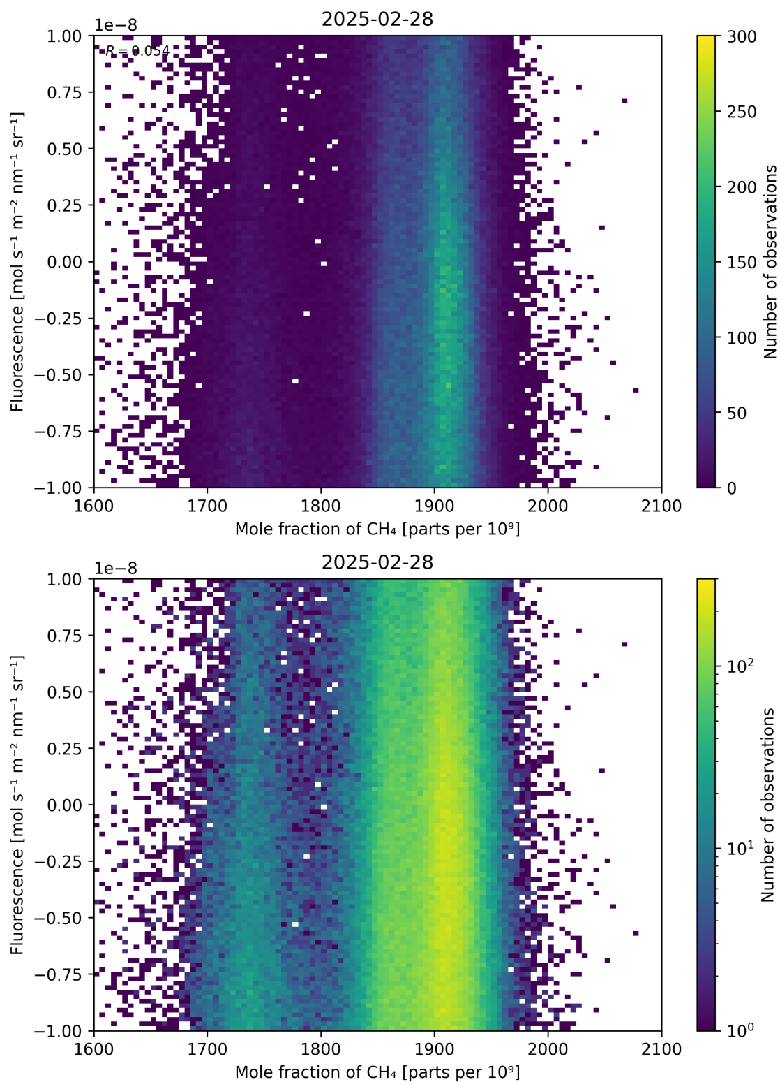
Figure 73: Scatter density plot of “Mole fraction of \text{CH}_4 ” against “Fluorescence” for 2025-02-27 to 2025-03-01.
