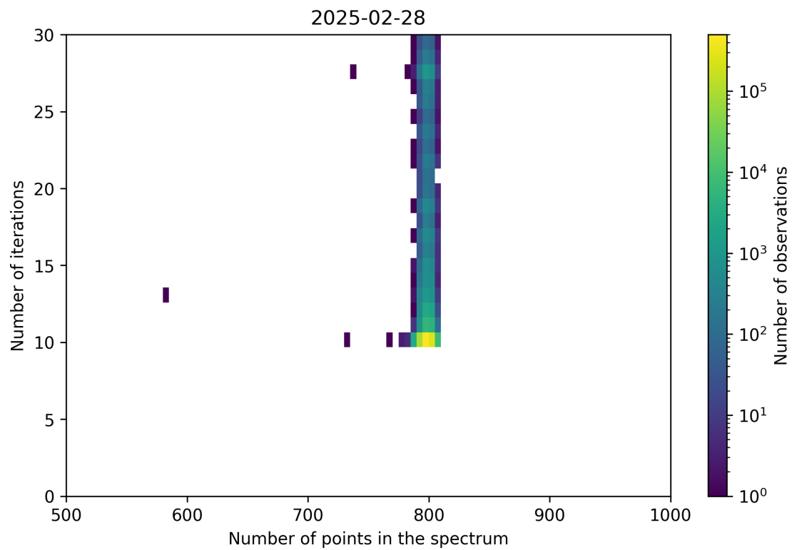
Figure 92: Scatter density plot of “Number of points in the spectrum” against “Number of iterations” for 2025-02-27 to 2025-03-01.
