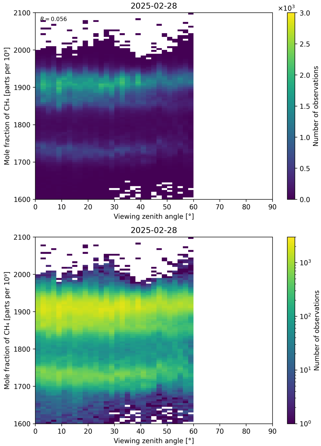
Figure 110: Scatter density plot of “Viewing zenith angle” against “Mole fraction of CH 4 ” for 2025-02-27 to 2025-03-01.
