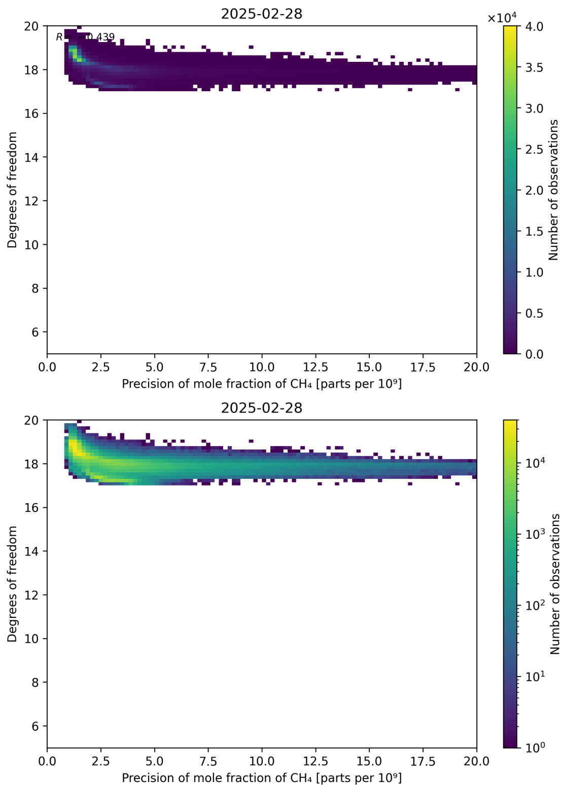
Figure 80: Scatter density plot of “Precision of mole fraction of CH 4 ” against “Degrees of freedom” for 2025-02-27 to 2025-03-01.
