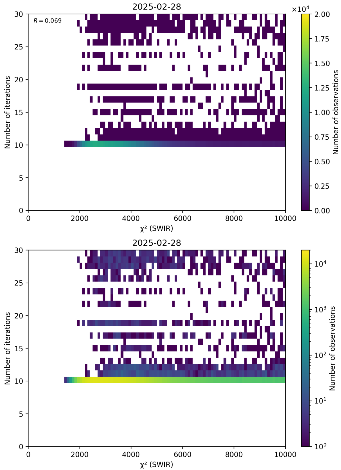
Figure 50: Scatter density plot of “ \chi^2 (SWIR)” against “Number of iterations” for 2025-02-27 to 2025-03-01.
