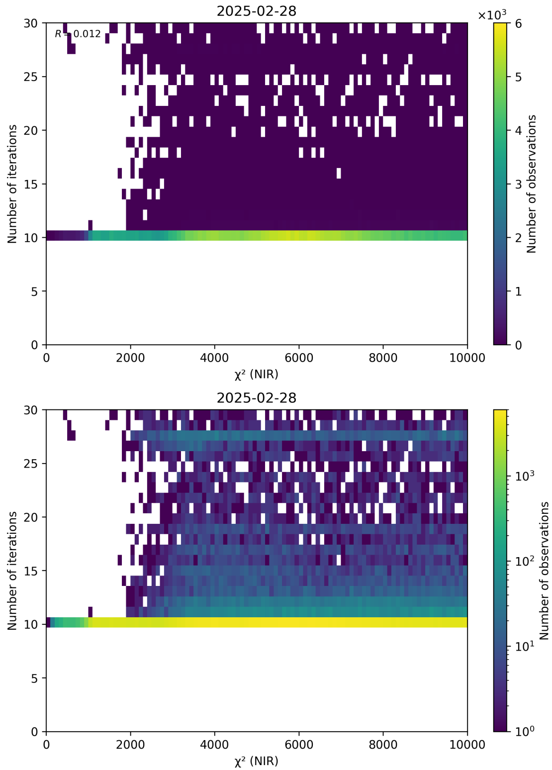
Figure 46: Scatter density plot of “ \chi^2 (NIR)” against “Number of iterations” for 2025-02-27 to 2025-03-01.
