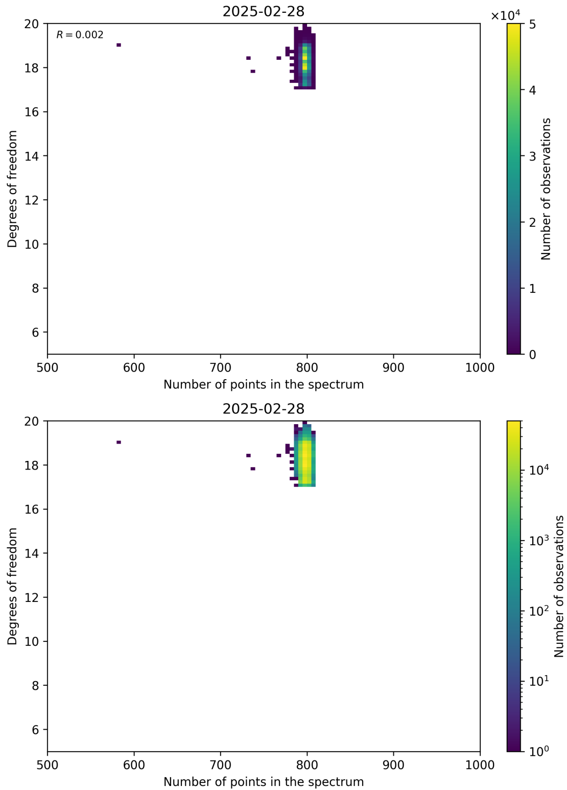
Figure 90: Scatter density plot of “Number of points in the spectrum” against “Degrees of freedom” for 2025-02-27 to 2025-03-01.
