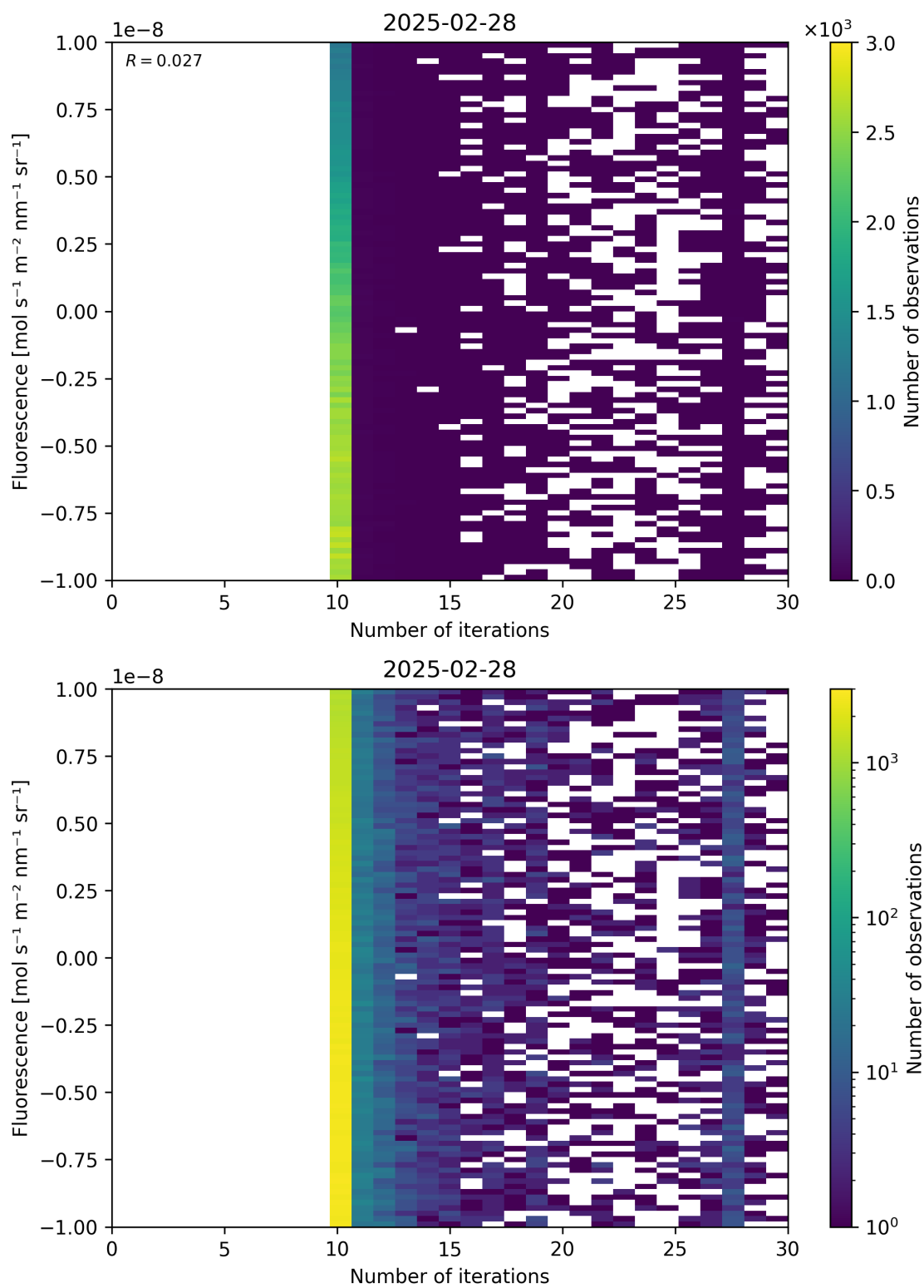
Figure 87: Scatter density plot of "Number of iterations" against "Fluorescence" for 2025-02-27 to 2025-03-01.
