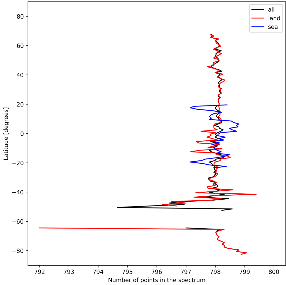
Figure 15: Zonal average of “Number of points in the spectrum” for 2025-02-27 to 2025-03-01.
