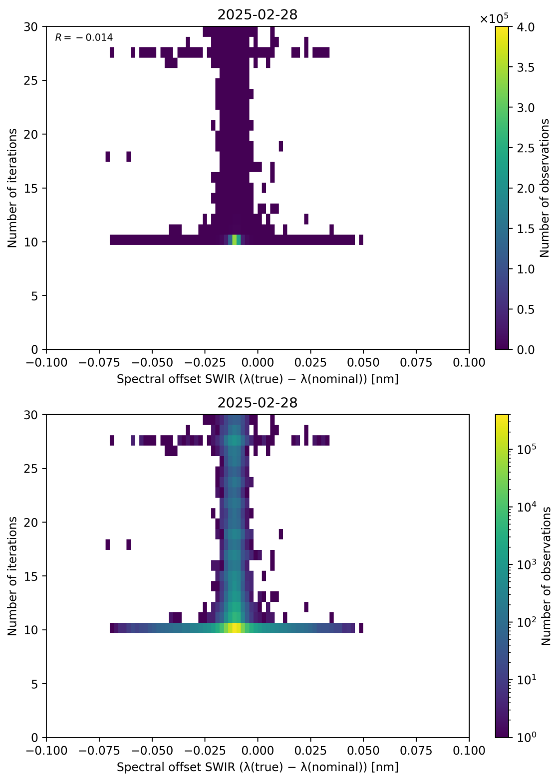
Figure 121: Scatter density plot of “Spectral offset SWIR ( \lambda_{\text{true}} - \lambda_{\text{nominal}} )” against “Number of iterations” for 2025-02-27 to 2025-03-01.
