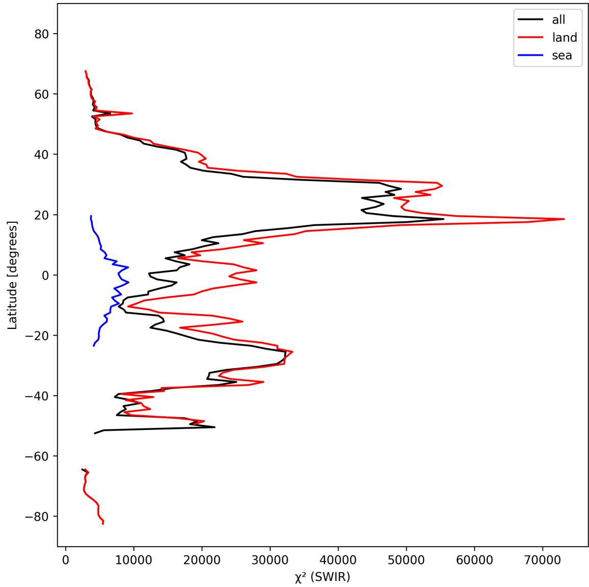
Figure 17: Zonal average of “ \chi^2 (SWIR)” for 2025-02-27 to 2025-03-01.
