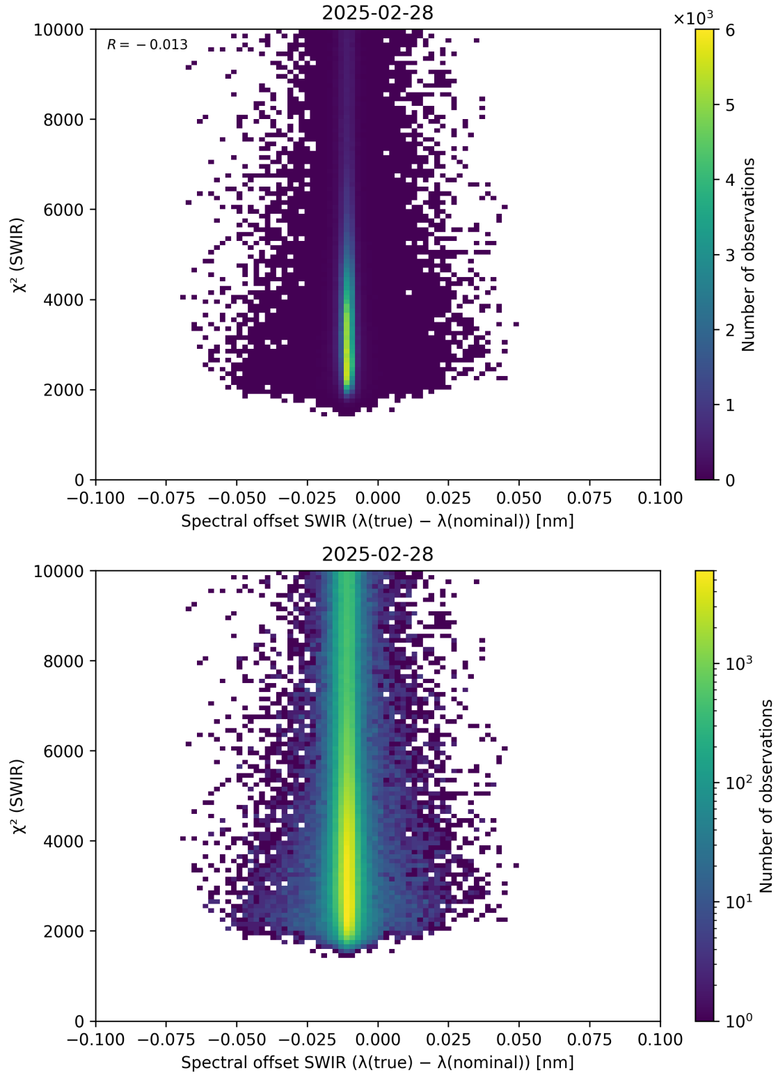
Figure 118: Scatter density plot of “Spectral offset SWIR ( \lambda_{\text{true}} - \lambda_{\text{nominal}} )” against “ \chi^2 (SWIR)” for 2025-02-27 to 2025-03-01.
