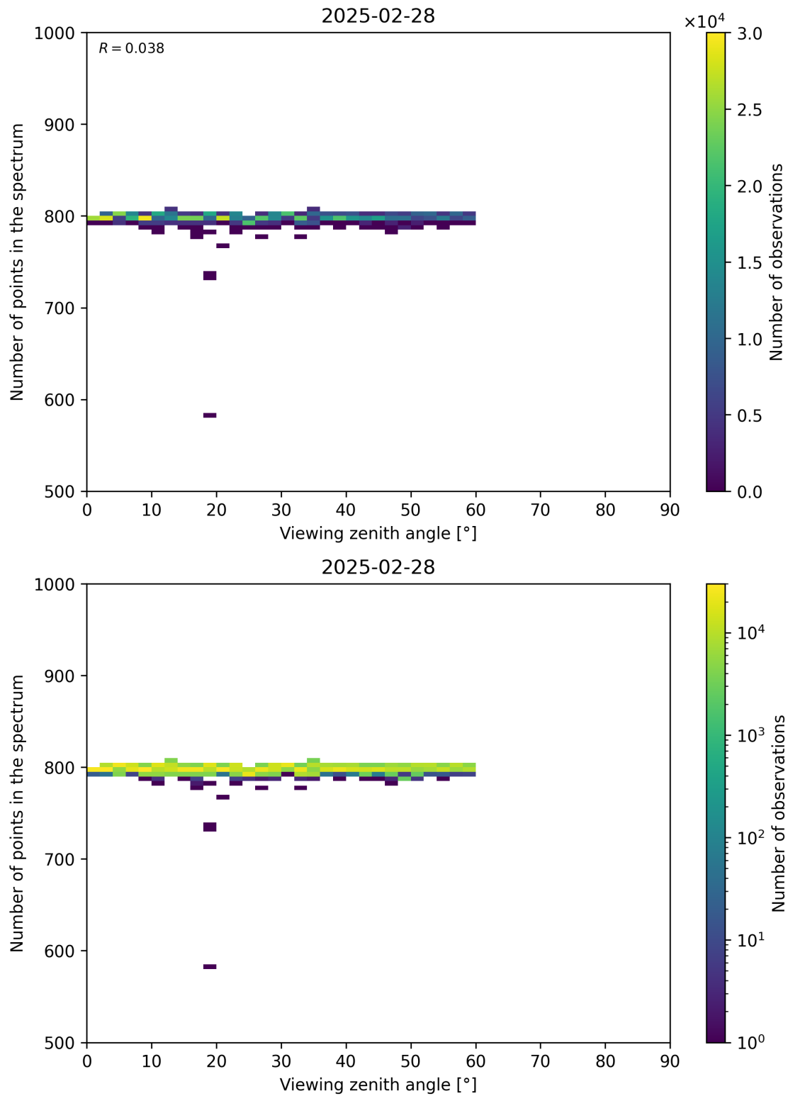
Figure 114: Scatter density plot of “Viewing zenith angle” against “Number of points in the spectrum” for 2025-02-27 to 2025-03-01.
