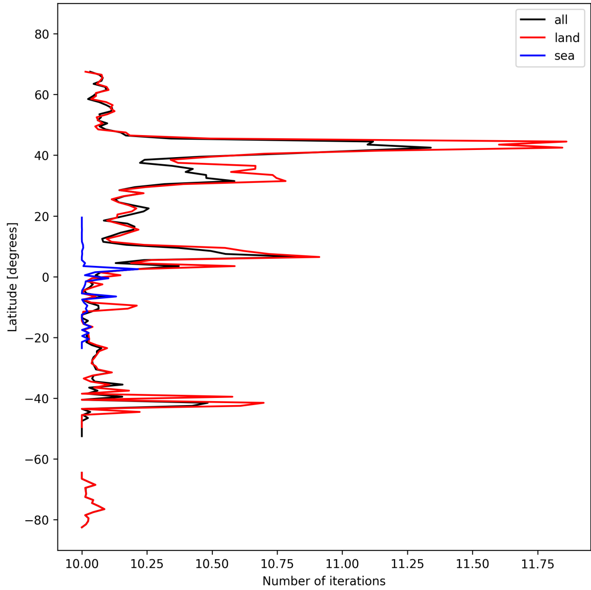
Figure 20: Zonal average of “Number of iterations” for 2025-02-27 to 2025-03-01.
