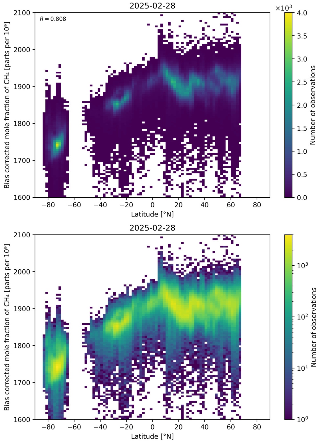
Figure 58: Scatter density plot of “Latitude” against “Bias corrected mole fraction of CH 4 ” for 2025-02-27 to 2025-03-01.
