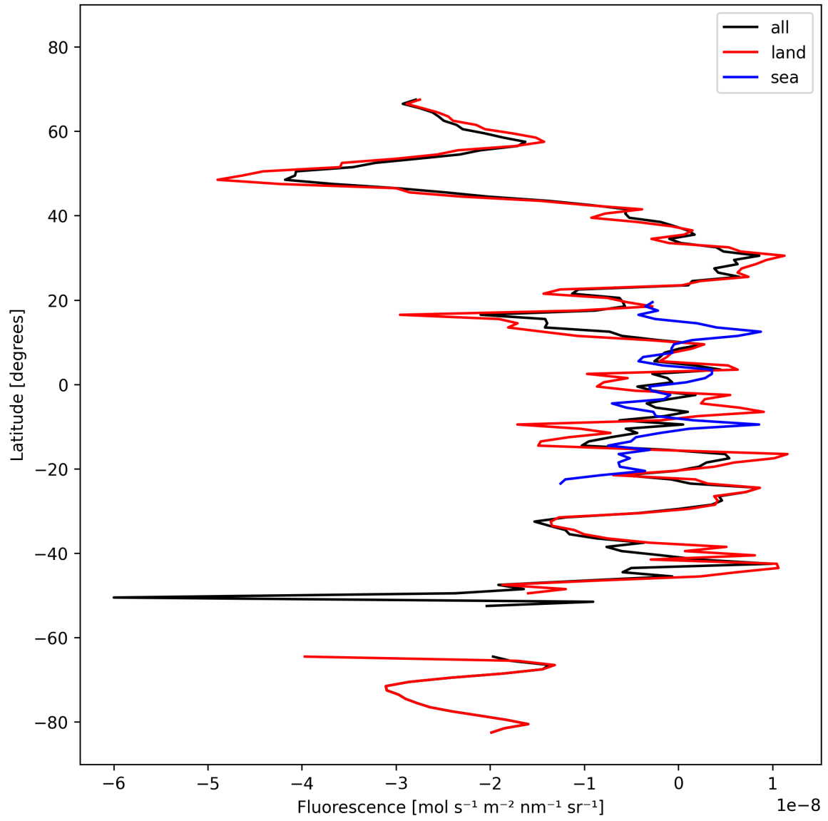
Figure 21: Zonal average of “Fluorescence” for 2025-02-27 to 2025-03-01.
