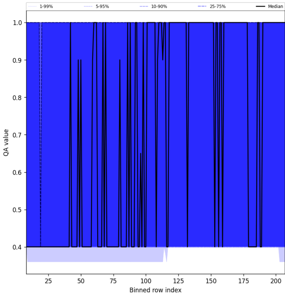
Figure 33: Along track statistics of "QA value" for 2025-02-27 to 2025-03-01
