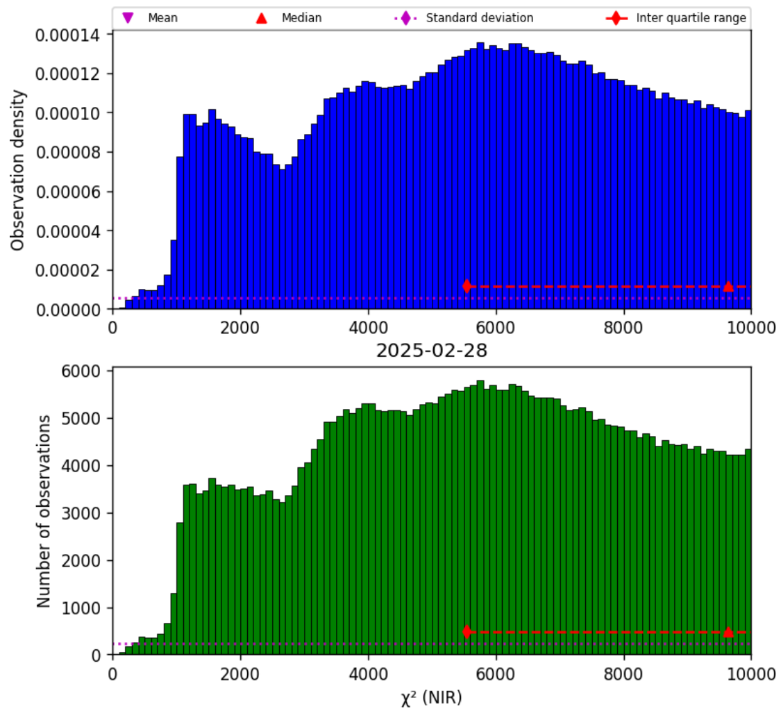
Figure 29: Histogram of " \chi^2 (NIR)" for 2025-02-27 to 2025-03-01
