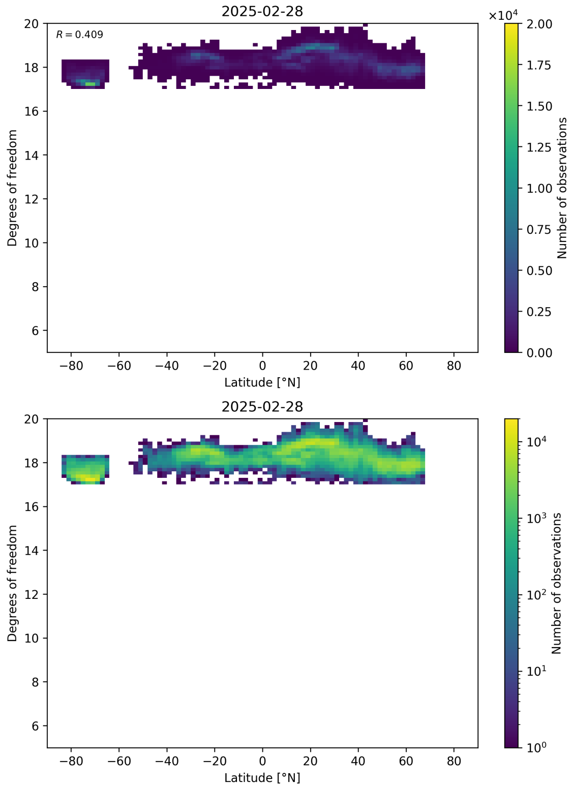
Figure 55: Scatter density plot of “Latitude” against “Degrees of freedom” for 2025-02-27 to 2025-03-01.
