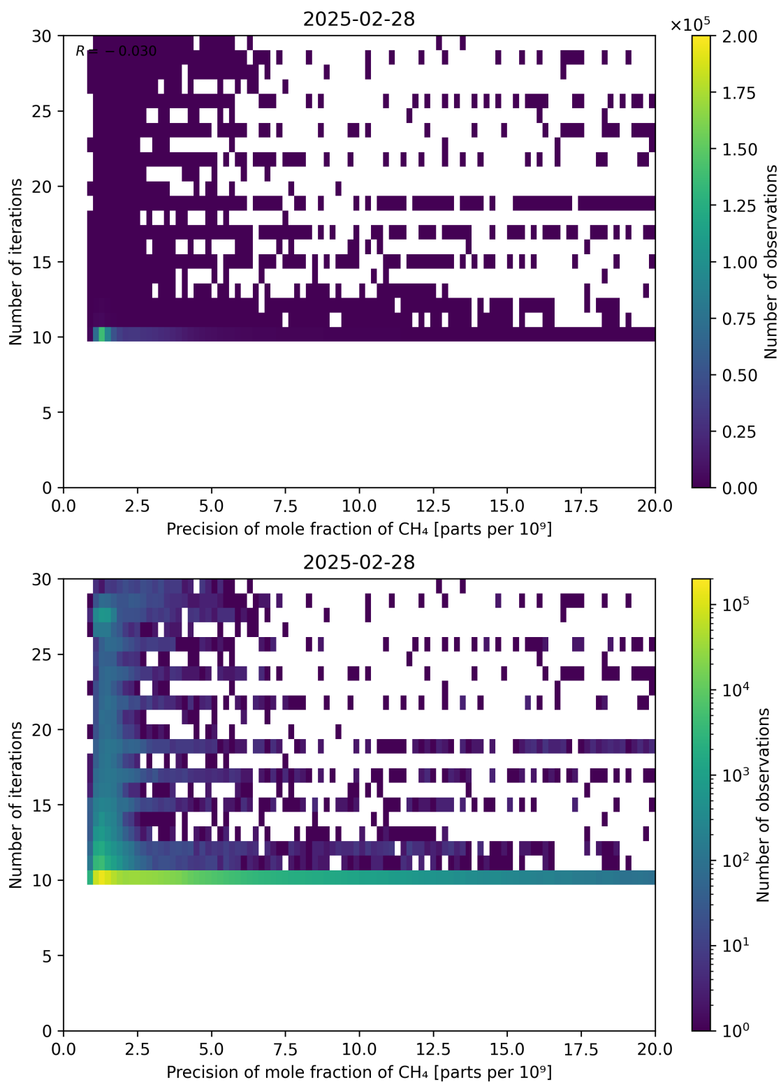
Figure 83: Scatter density plot of “Precision of mole fraction of CH 4 ” against “Number of iterations” for 2025-02-27 to 2025-03-01.
