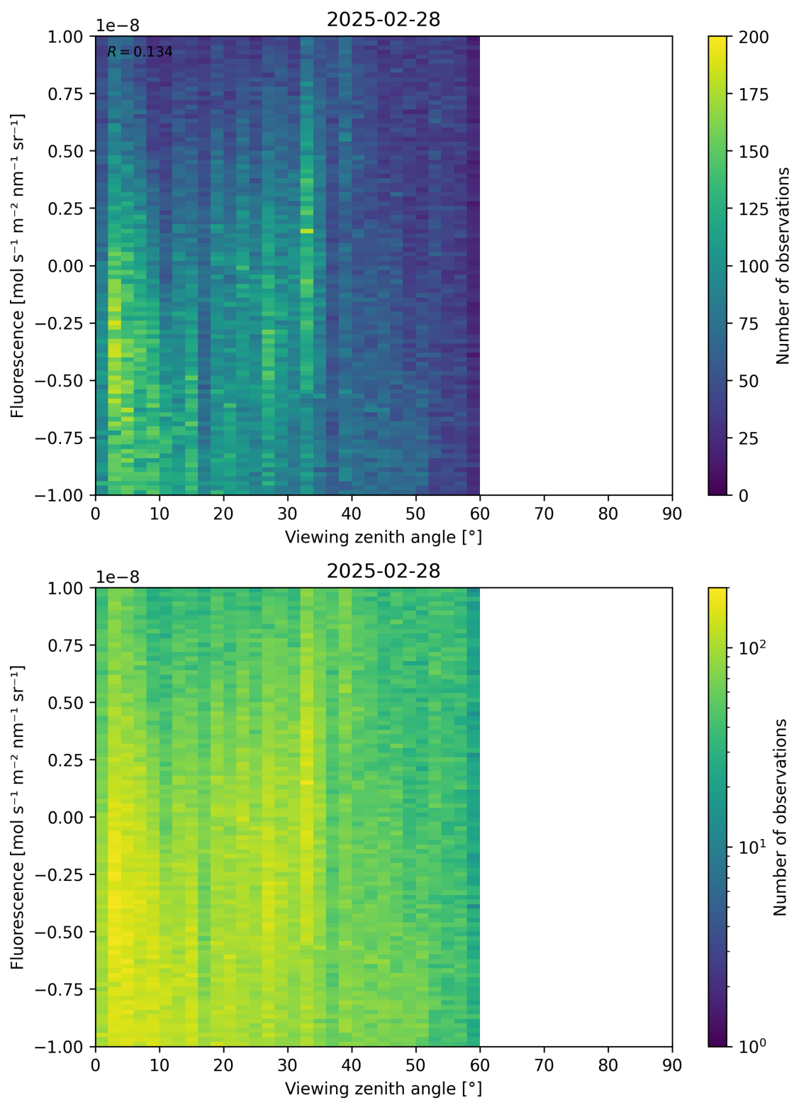
Figure 108: Scatter density plot of “Viewing zenith angle” against “Fluorescence” for 2025-02-27 to 2025-03-01.
