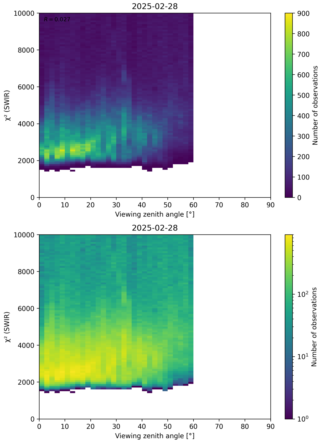
Figure 106: Scatter density plot of “Viewing zenith angle” against “ \chi^2 (SWIR)” for 2025-02-27 to 2025-03-01.
