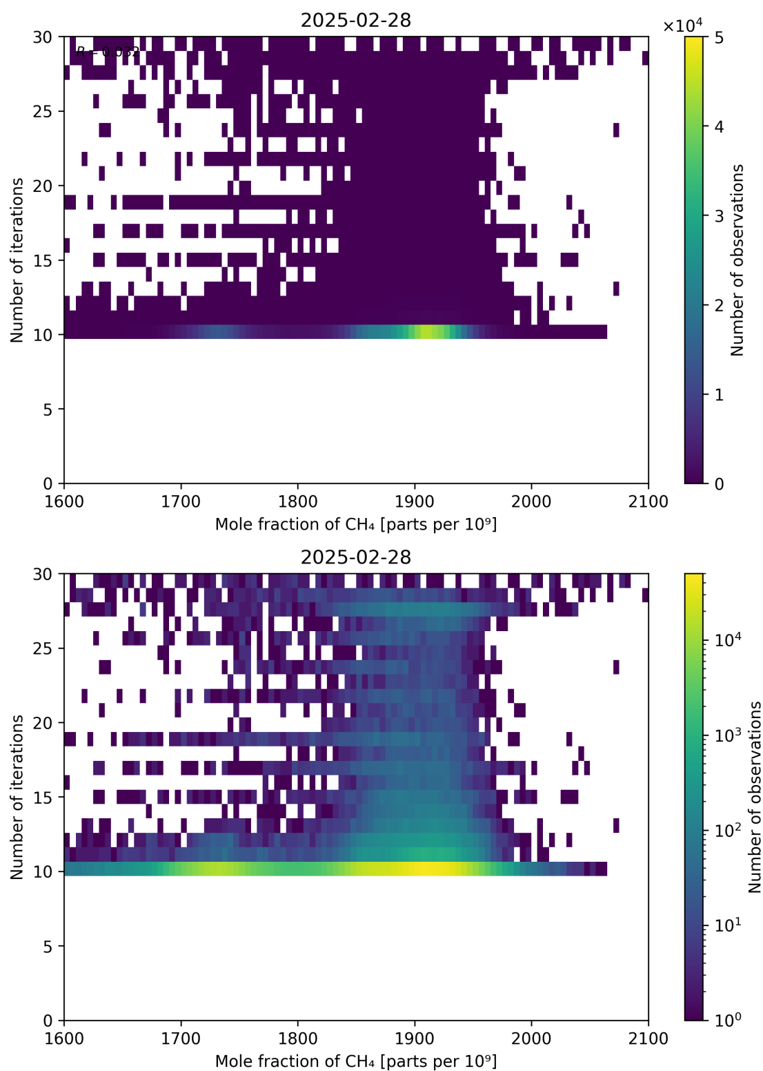
Figure 76: Scatter density plot of “Mole fraction of CH 4 ” against “Number of iterations” for 2025-02-27 to 2025-03-01.
