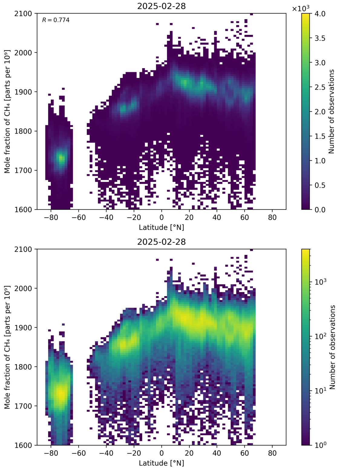
Figure 57: Scatter density plot of “Latitude” against “Mole fraction of \text{CH}_4 ” for 2025-02-27 to 2025-03-01.
