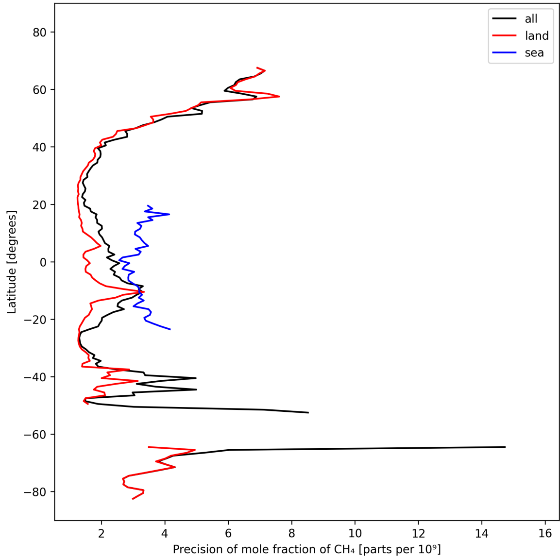
Figure 13: Zonal average of “Precision of mole fraction of CH 4 ” for 2025-02-27 to 2025-03-01.
