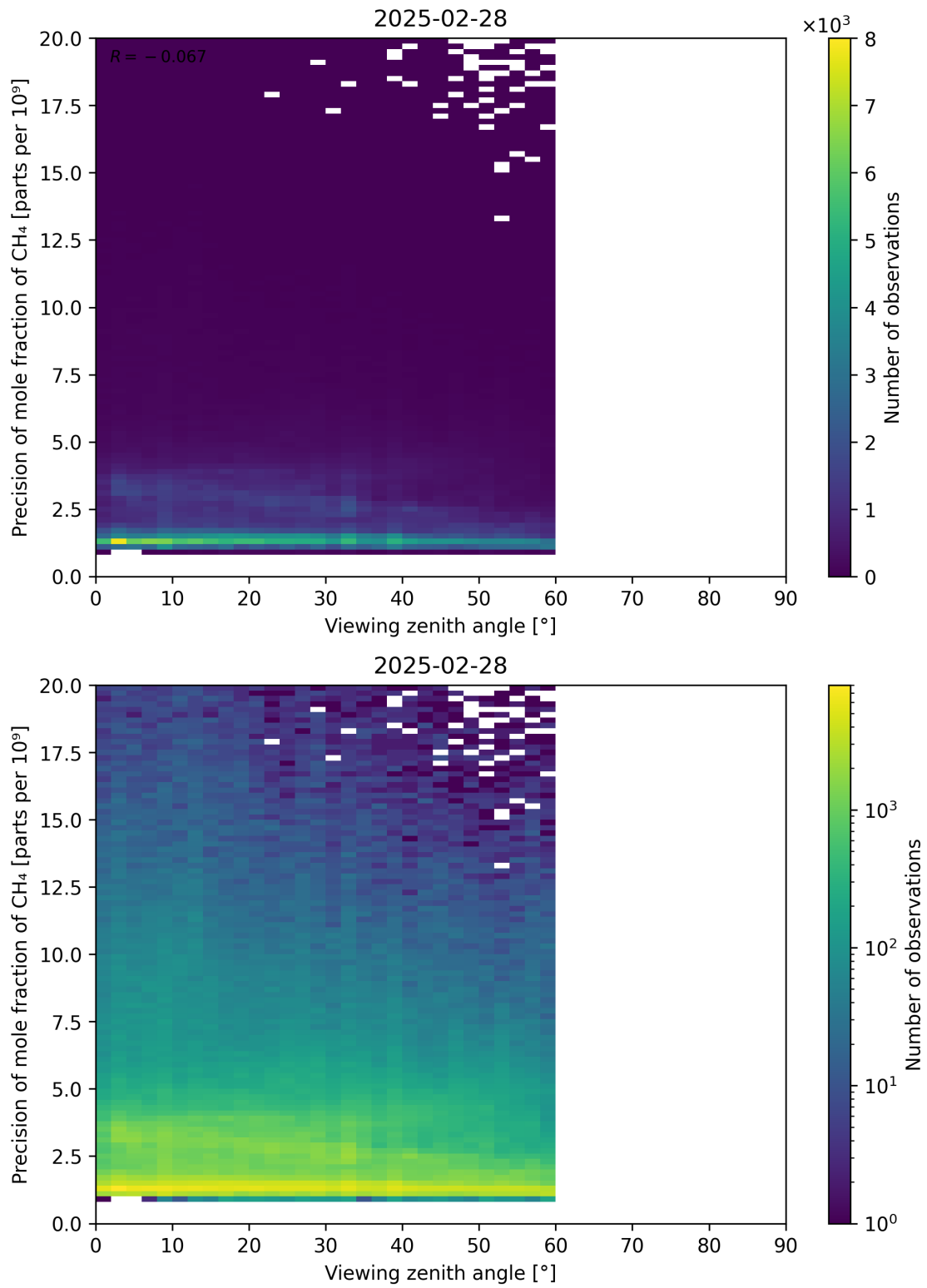
Figure 112: Scatter density plot of “Viewing zenith angle” against “Precision of mole fraction of CH 4 ” for 2025-02-27 to 2025-03-01.
