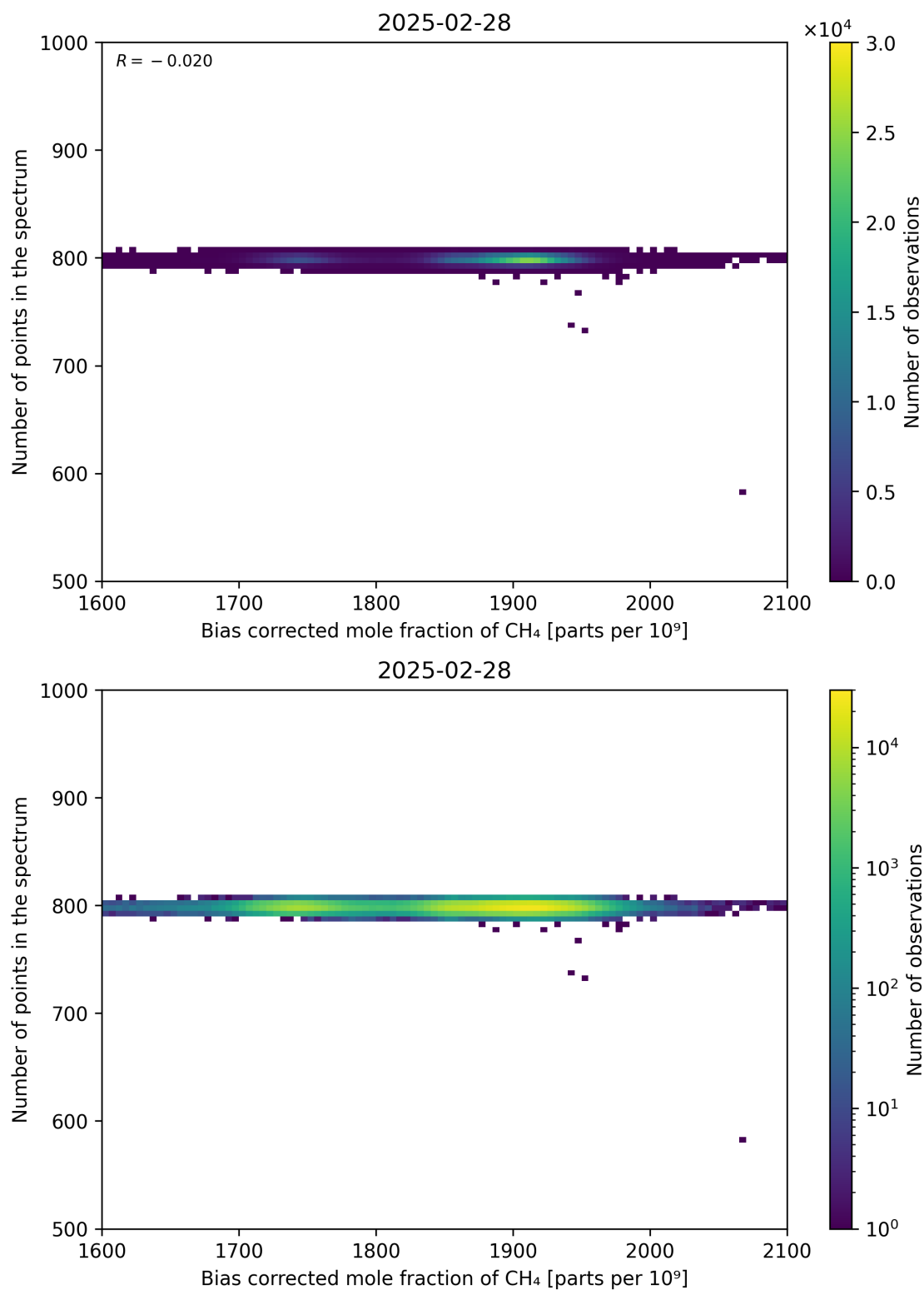
Figure 68: Scatter density plot of “Bias corrected mole fraction of CH 4 ” against “Number of points in the spectrum” for 2025-02-27 to 2025-03-01.
