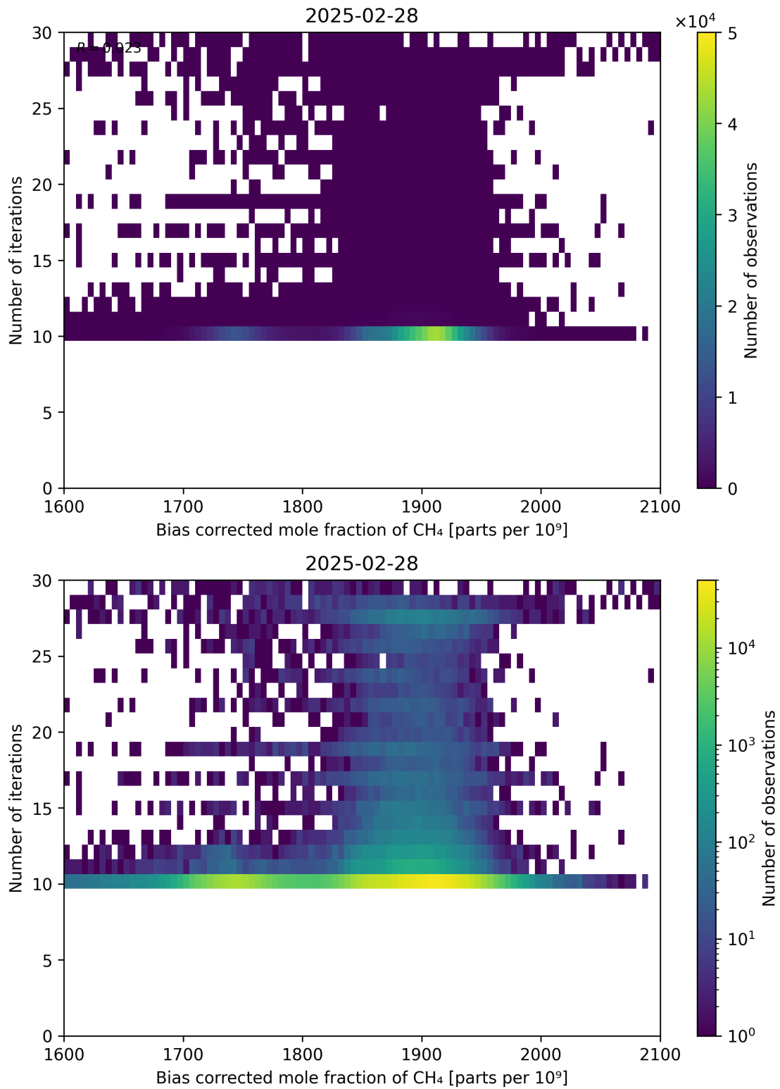
Figure 67: Scatter density plot of “Bias corrected mole fraction of \text{CH}_4 ” against “Number of iterations” for 2025-02-27 to 2025-03-01.
