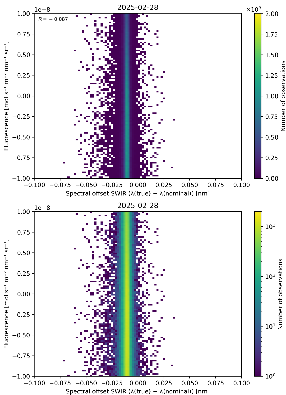
Figure 120: Scatter density plot of “Spectral offset SWIR ( \lambda_{\text{true}} - \lambda_{\text{nominal}} )” against “Fluorescence” for 2025-02-27 to 2025-03-01.
