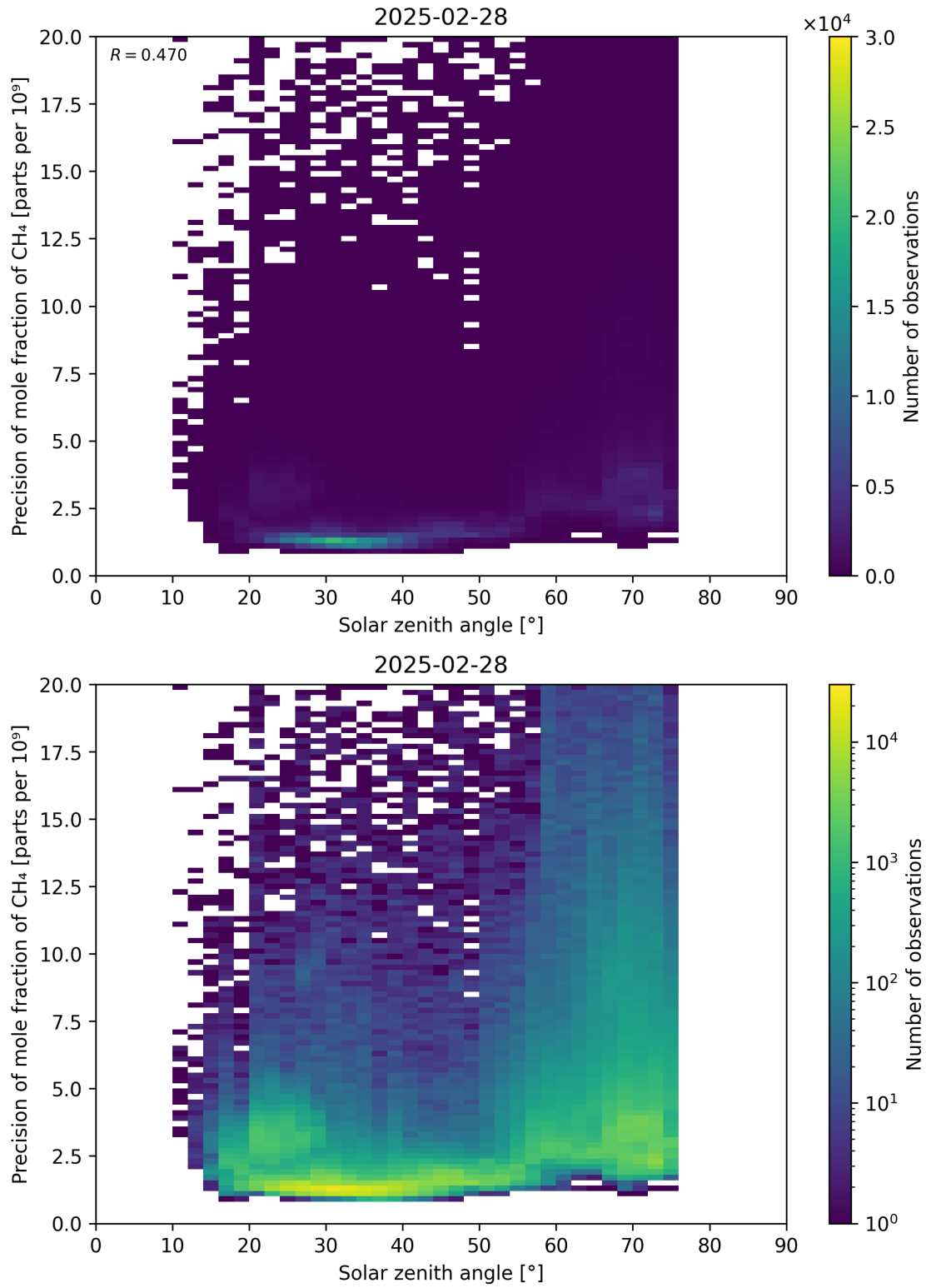
Figure 101: Scatter density plot of “Solar zenith angle” against “Precision of mole fraction of \text{CH}_4 ” for 2025-02-27 to 2025-03-01.
