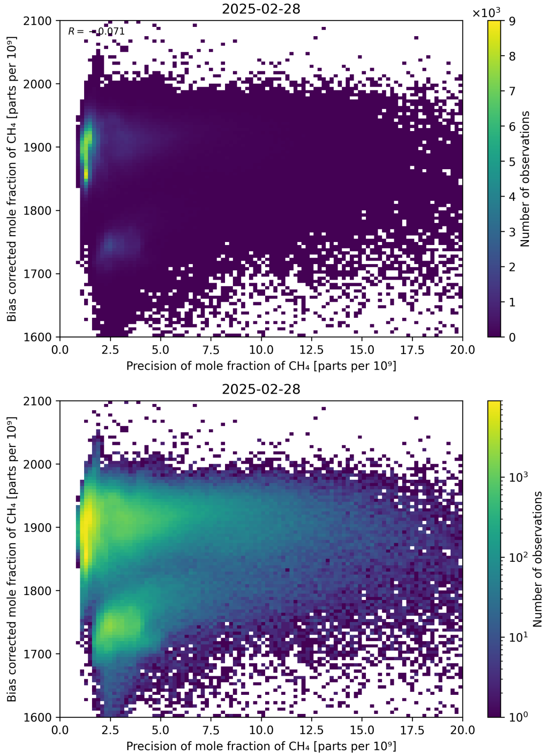
Figure 82: Scatter density plot of “Precision of mole fraction of CH 4 ” against “Bias corrected mole fraction of CH 4 ” for 2025-02-27 to 2025-03-01.
