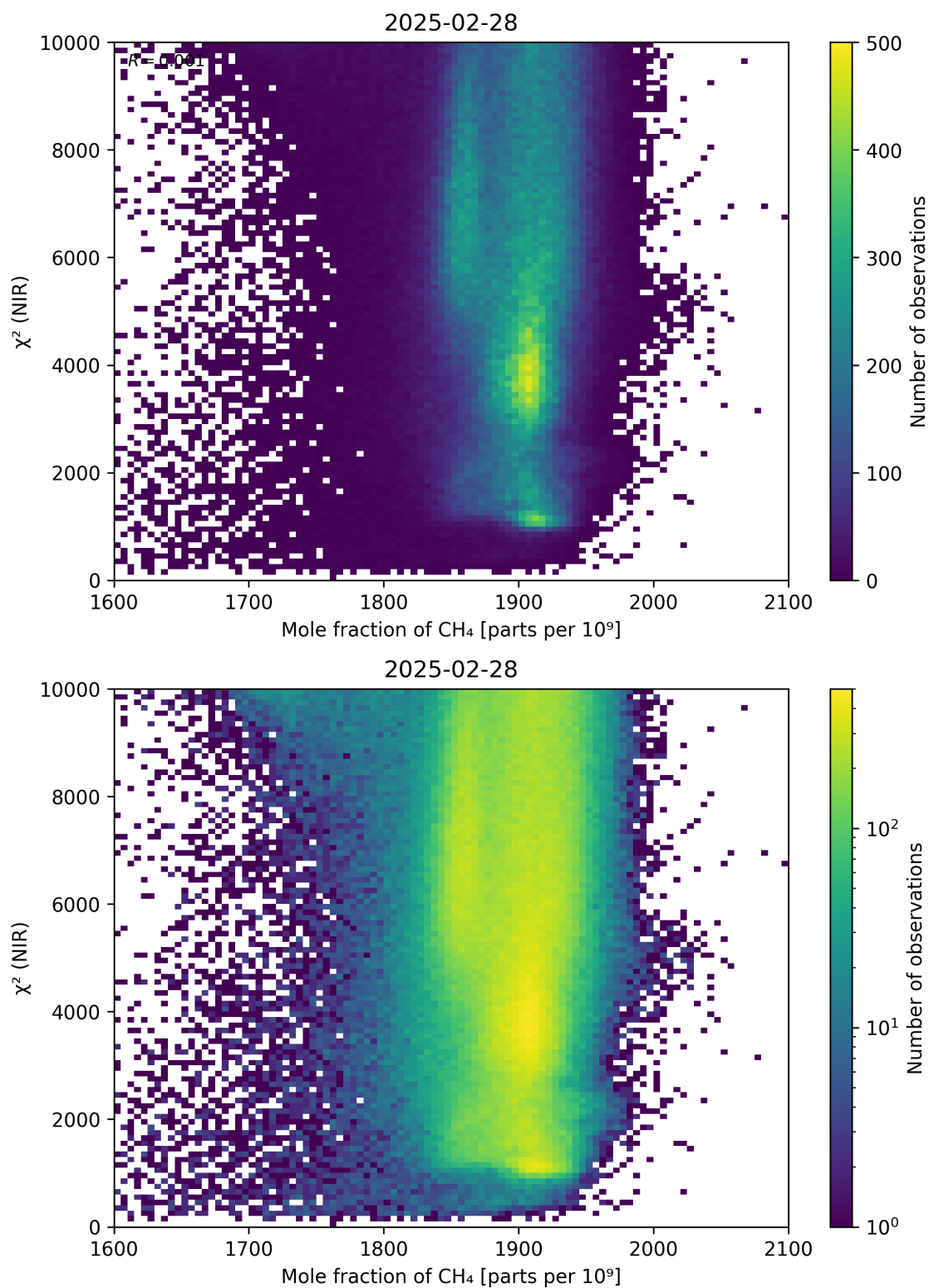
Figure 70: Scatter density plot of “Mole fraction of \text{CH}_4 ” against “ \chi^2 (NIR)” for 2025-02-27 to 2025-03-01.
