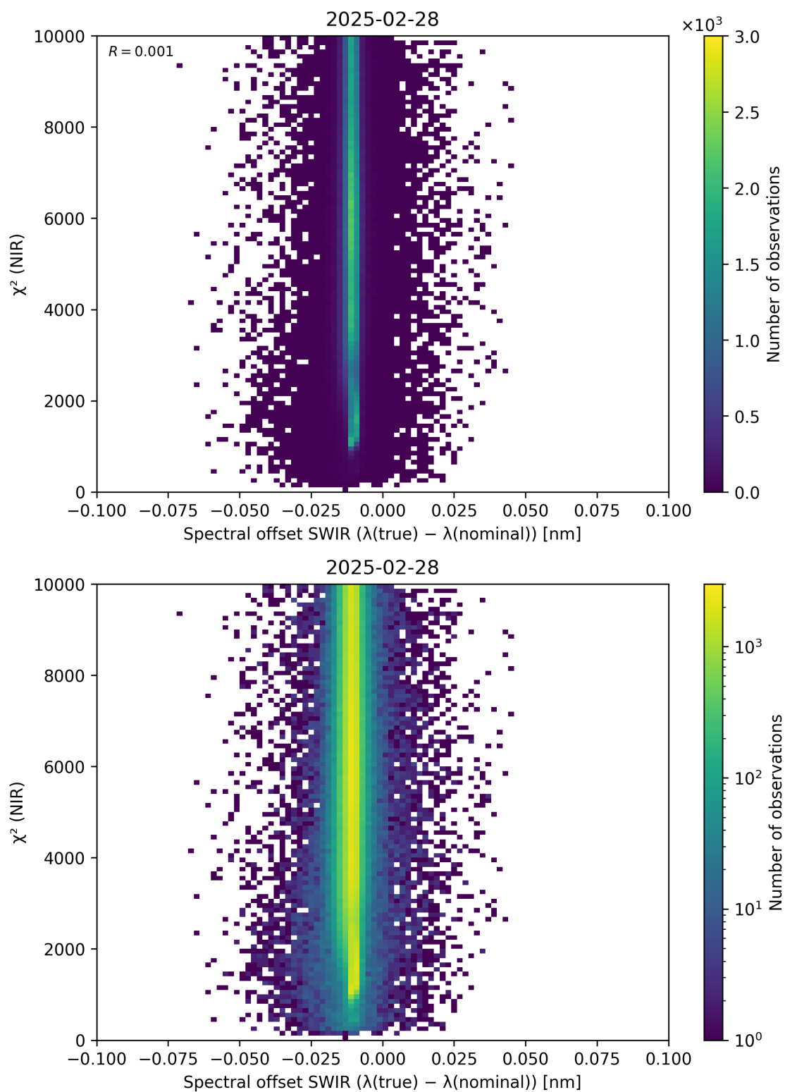
Figure 117: Scatter density plot of “Spectral offset SWIR ( \lambda_{\text{true}} - \lambda_{\text{nominal}} )” against “ \chi^2 (NIR)” for 2025-02-27 to 2025-03-01.
