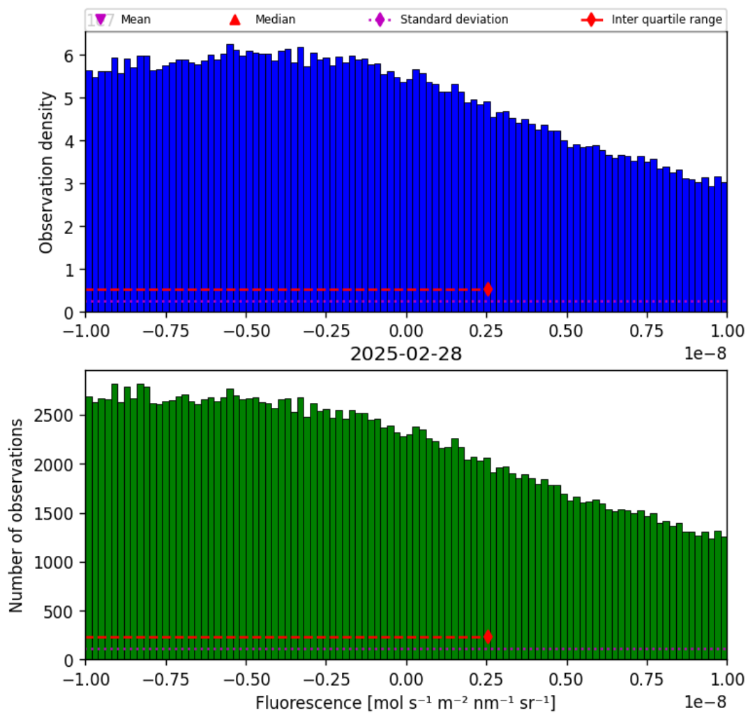
Figure 32: Histogram of “Fluorescence” for 2025-02-27 to 2025-03-01
