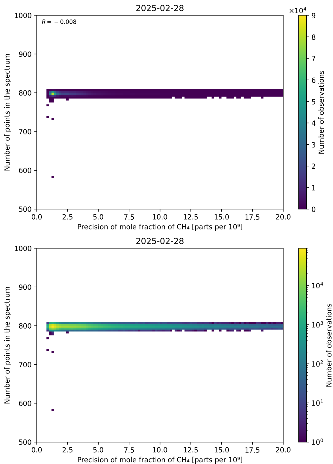
Figure 84: Scatter density plot of “Precision of mole fraction of CH 4 ” against “Number of points in the spectrum” for 2025-02-27 to 2025-03-01.
