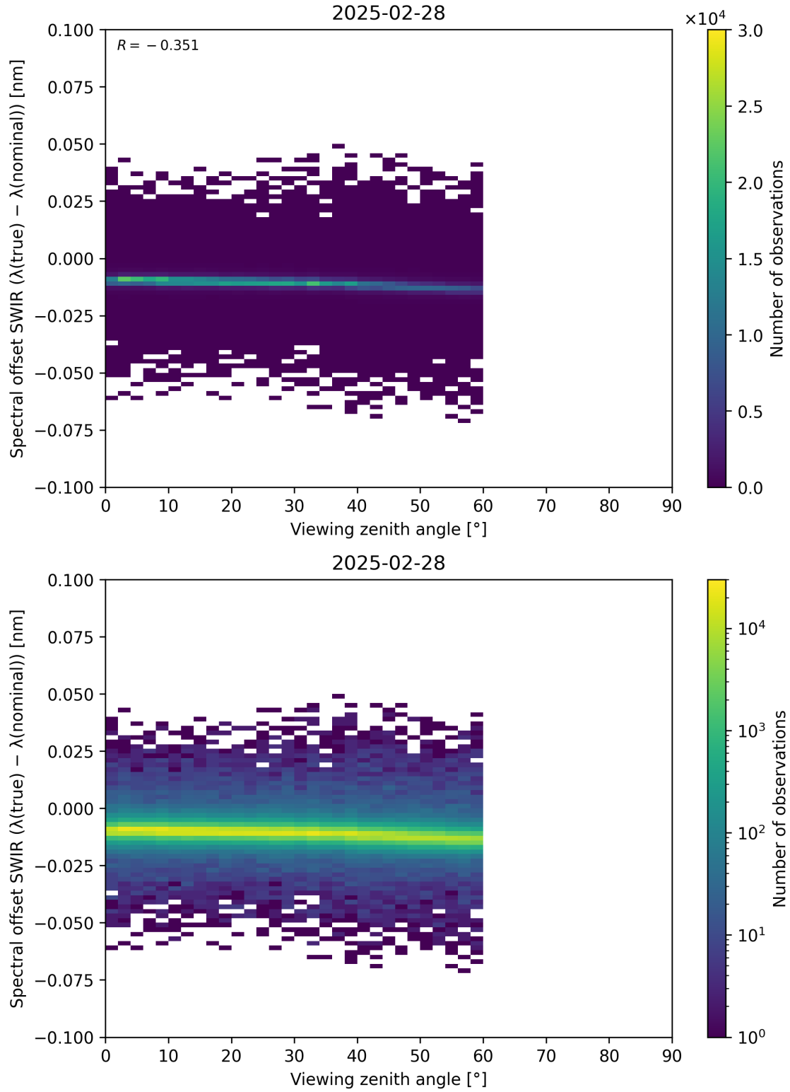
Figure 116: Scatter density plot of “Viewing zenith angle” against “Spectral offset SWIR ( \lambda_{\text{true}} - \lambda_{\text{nominal}} )” for 2025-02-27 to 2025-03-01.
