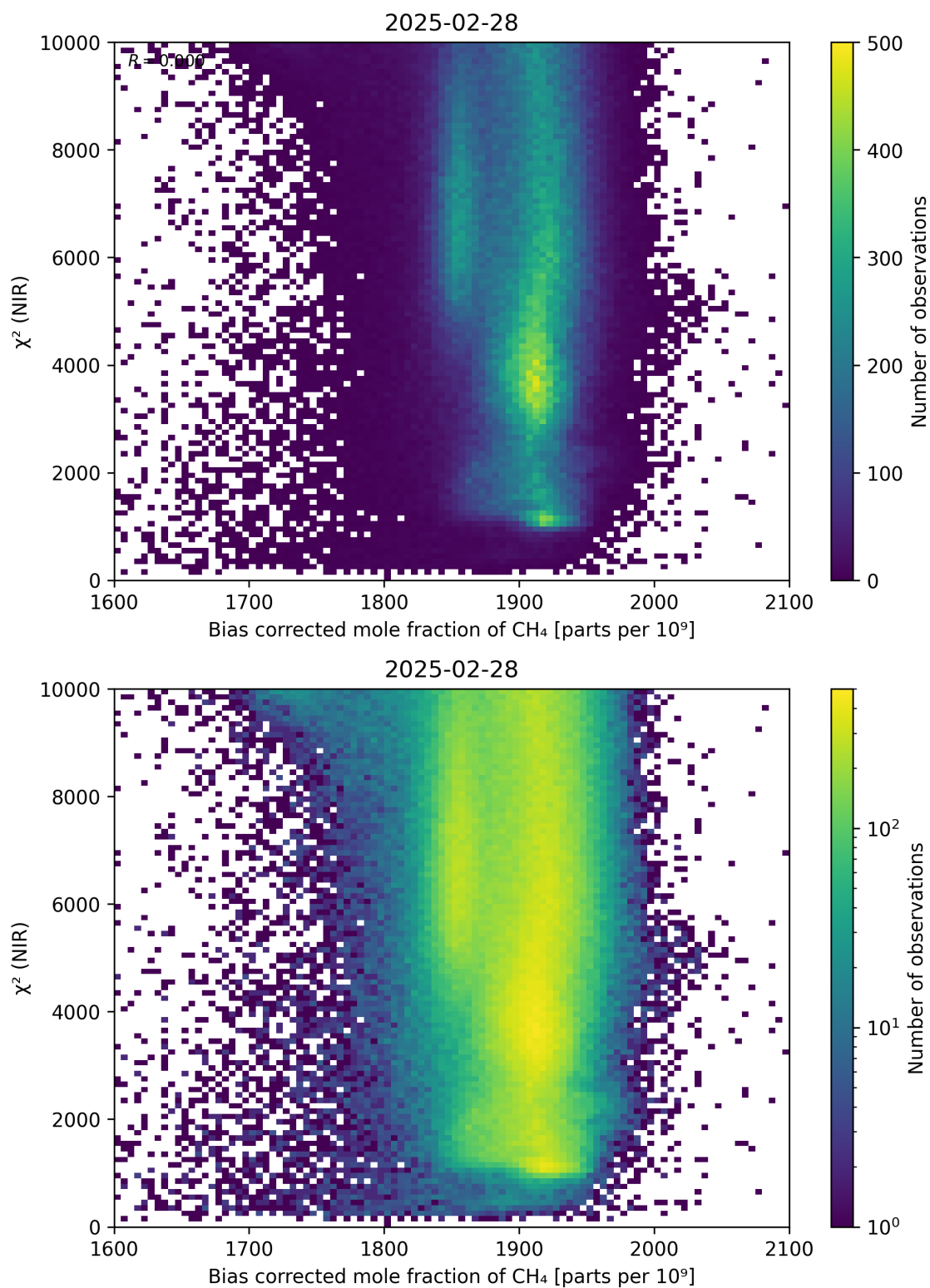
Figure 63: Scatter density plot of “Bias corrected mole fraction of \text{CH}_4 ” against “ \chi^2 (NIR)” for 2025-02-27 to 2025-03-01.
