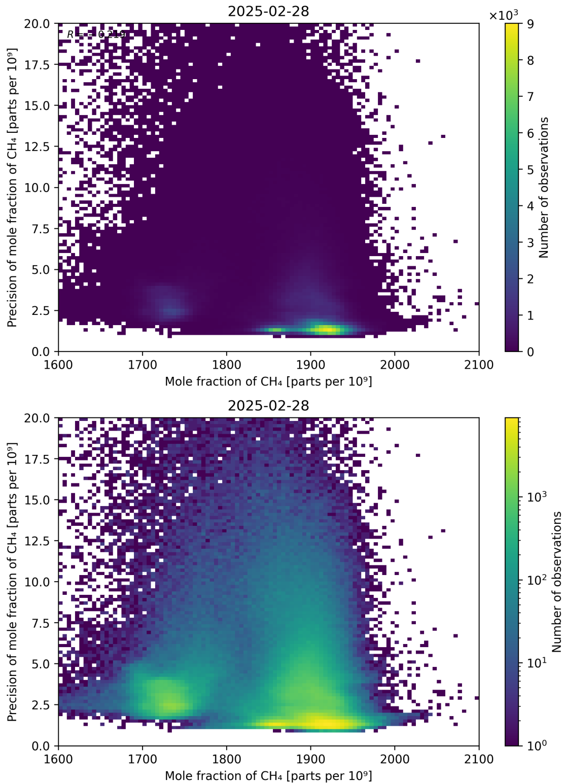
Figure 75: Scatter density plot of “Mole fraction of CH 4 ” against “Precision of mole fraction of CH 4 ” for 2025-02-27 to 2025-03-01.
