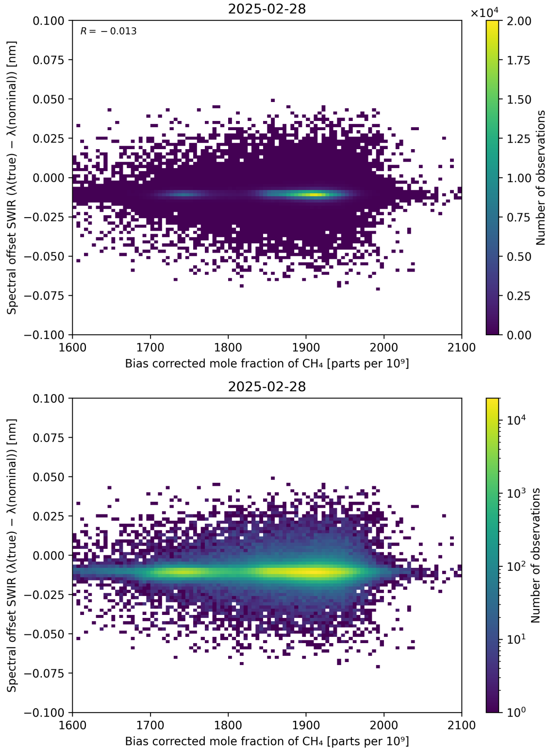
Figure 69: Scatter density plot of “Bias corrected mole fraction of \text{CH}_4 ” against “Spectral offset SWIR ( \lambda_{\text{true}} - \lambda_{\text{nominal}} )” for 2025-02-27 to 2025-03-01.
