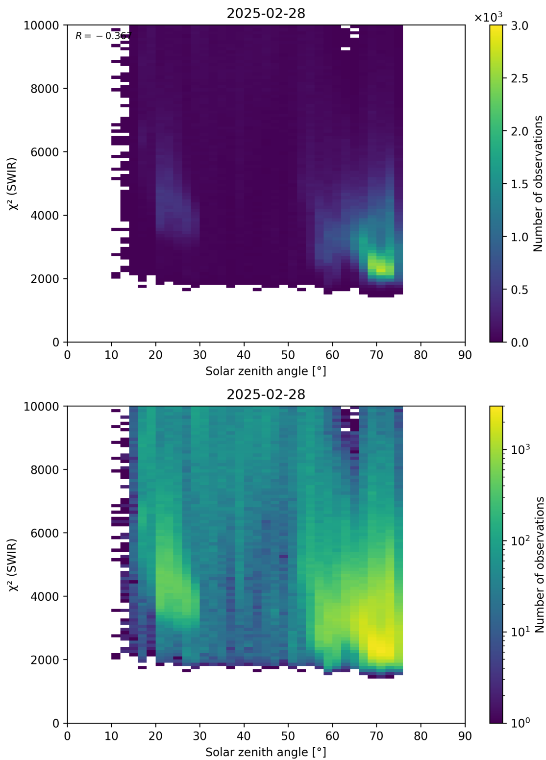
Figure 95: Scatter density plot of “Solar zenith angle” against “ \chi^2 (SWIR)” for 2025-02-27 to 2025-03-01.
