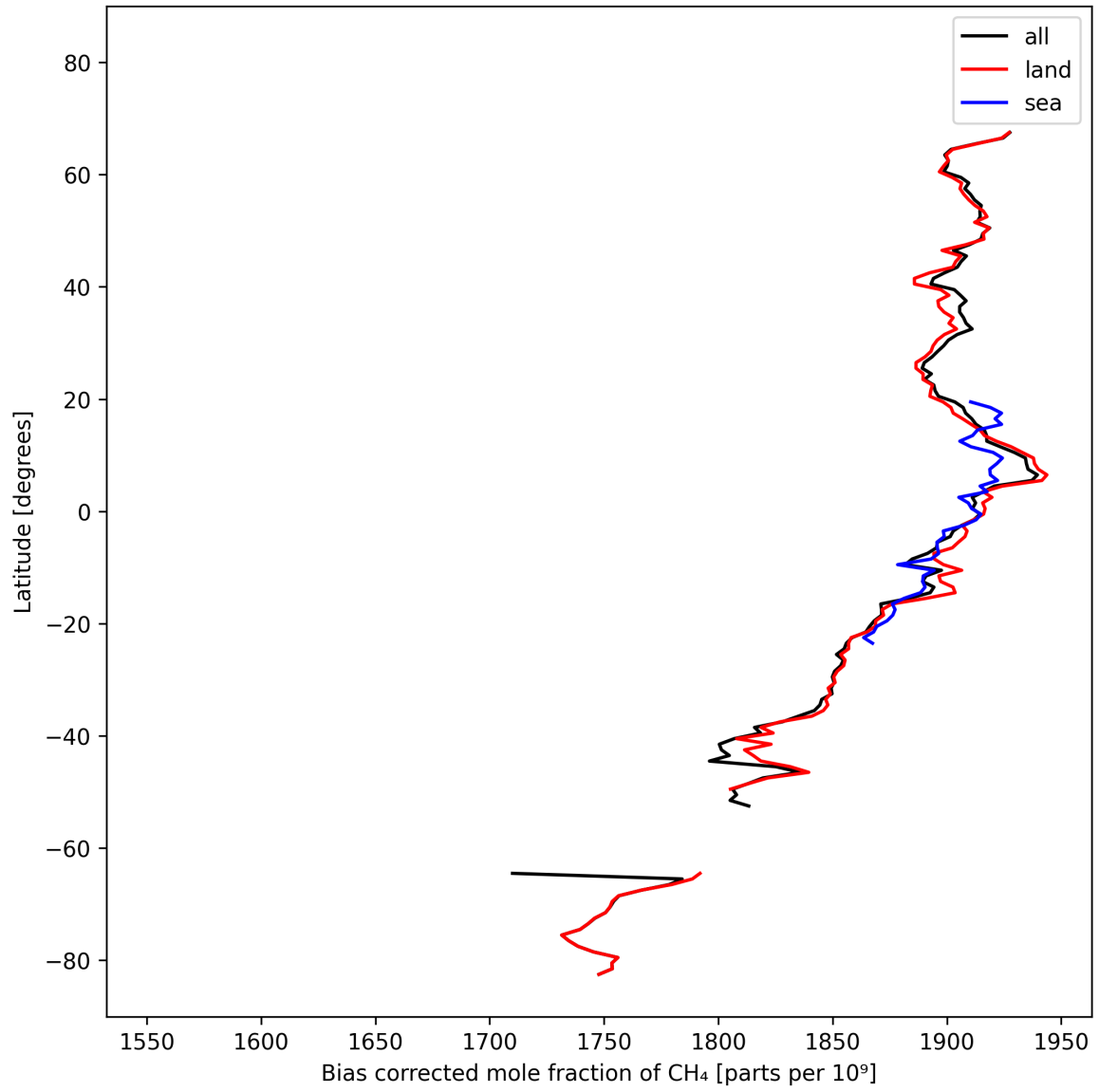
Figure 14: Zonal average of “Bias corrected mole fraction of \text{CH}_4 ” for 2025-02-27 to 2025-03-01.
