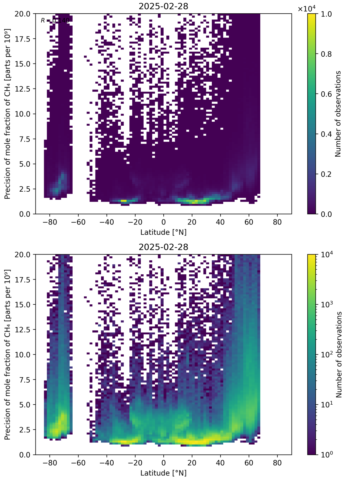
Figure 59: Scatter density plot of “Latitude” against “Precision of mole fraction of CH 4 ” for 2025-02-27 to 2025-03-01.
