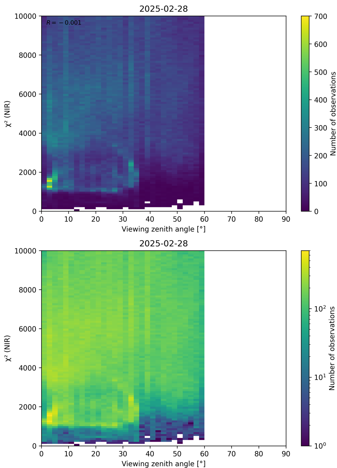
Figure 105: Scatter density plot of “Viewing zenith angle” against “ \chi^2 (NIR)” for 2025-02-27 to 2025-03-01.
