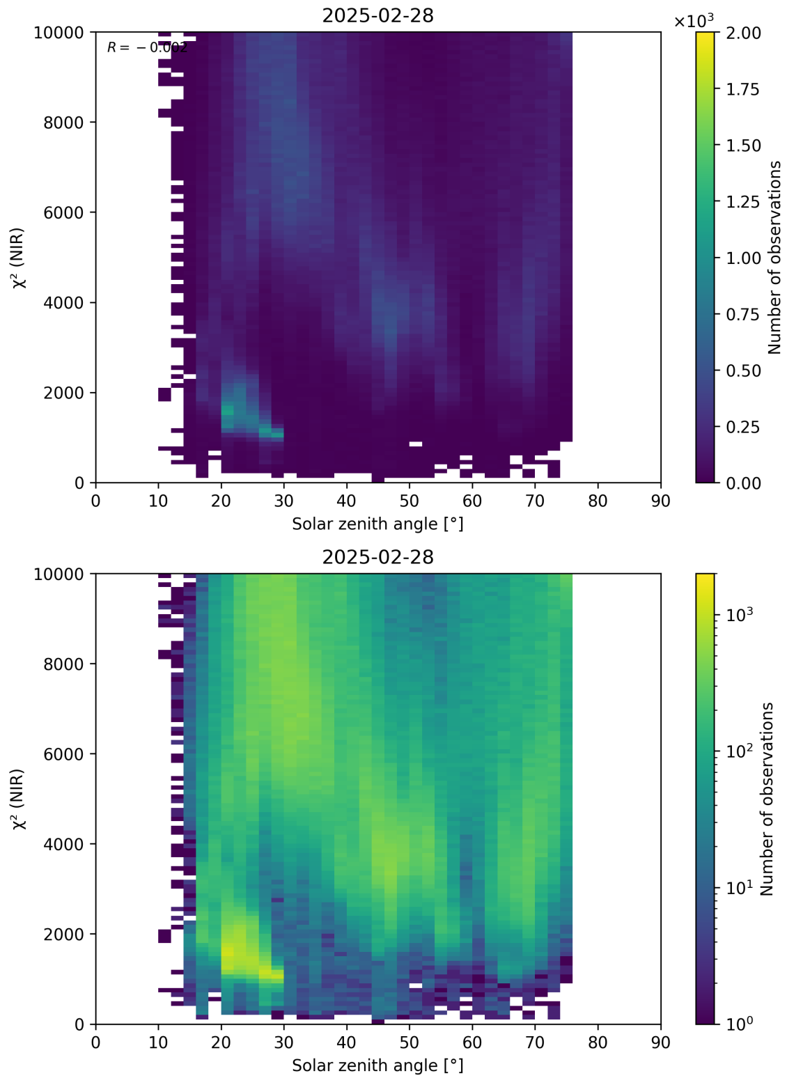
Figure 94: Scatter density plot of “Solar zenith angle” against “ \chi^2 (NIR)” for 2025-02-27 to 2025-03-01.
