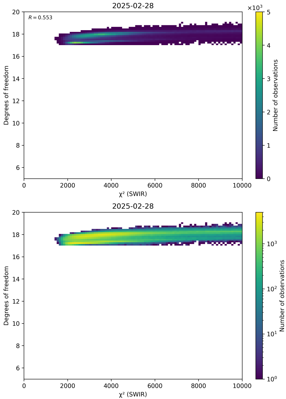
Figure 48: Scatter density plot of “ \chi^2 (SWIR)” against “Degrees of freedom” for 2025-02-27 to 2025-03-01.
