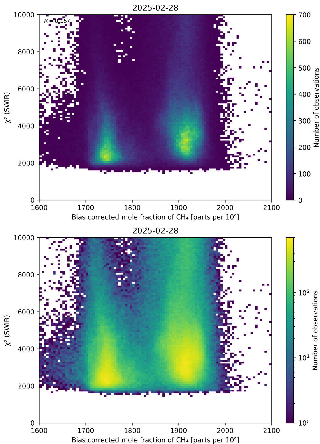
Figure 64: Scatter density plot of “Bias corrected mole fraction of \text{CH}_4 ” against “ \chi^2 (SWIR)” for 2025-02-27 to 2025-03-01.
