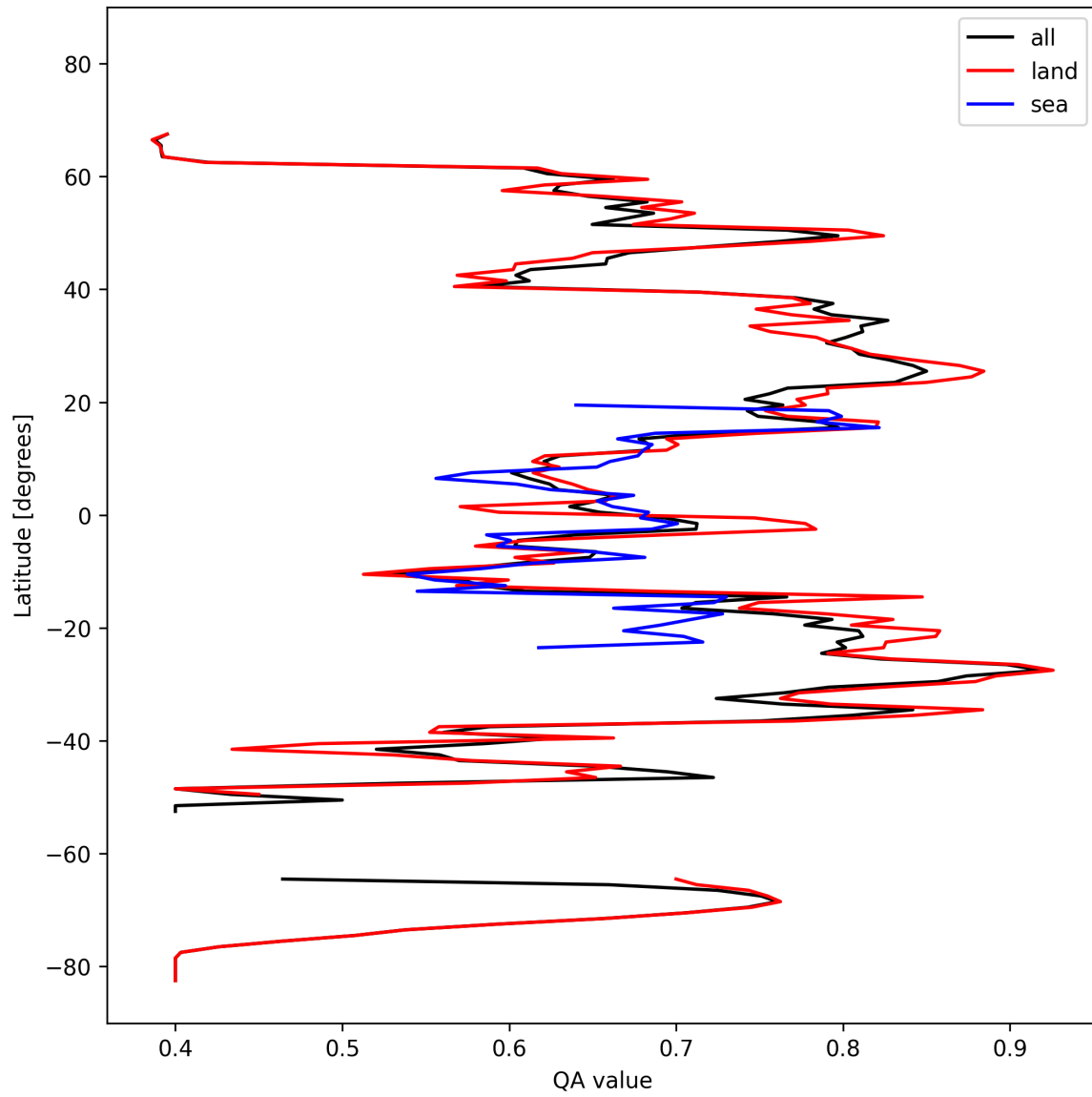
Figure 11: Zonal average of “QA value” for 2025-02-27 to 2025-03-01.
