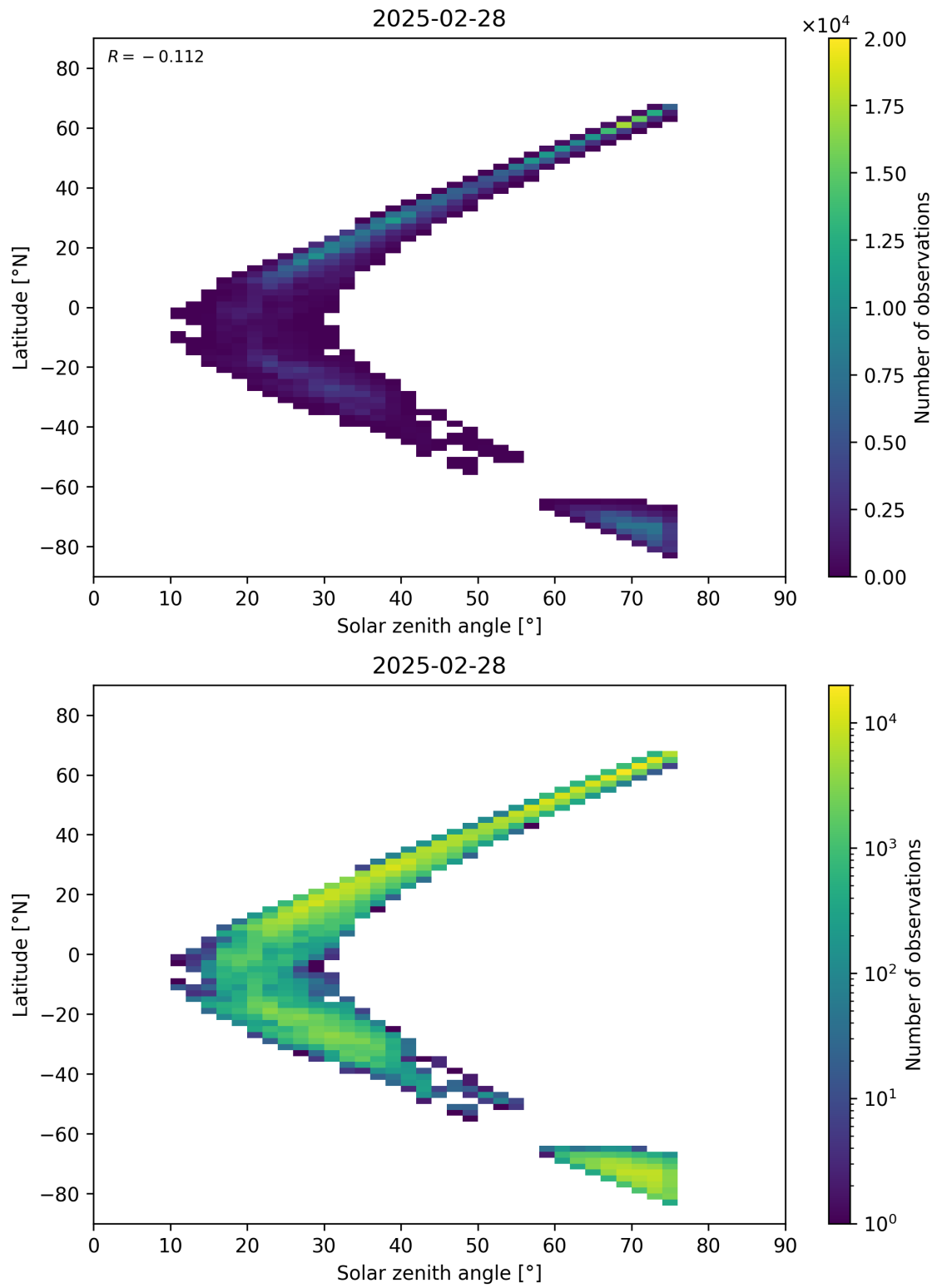
Figure 98: Scatter density plot of “Solar zenith angle” against “Latitude” for 2025-02-27 to 2025-03-01.
