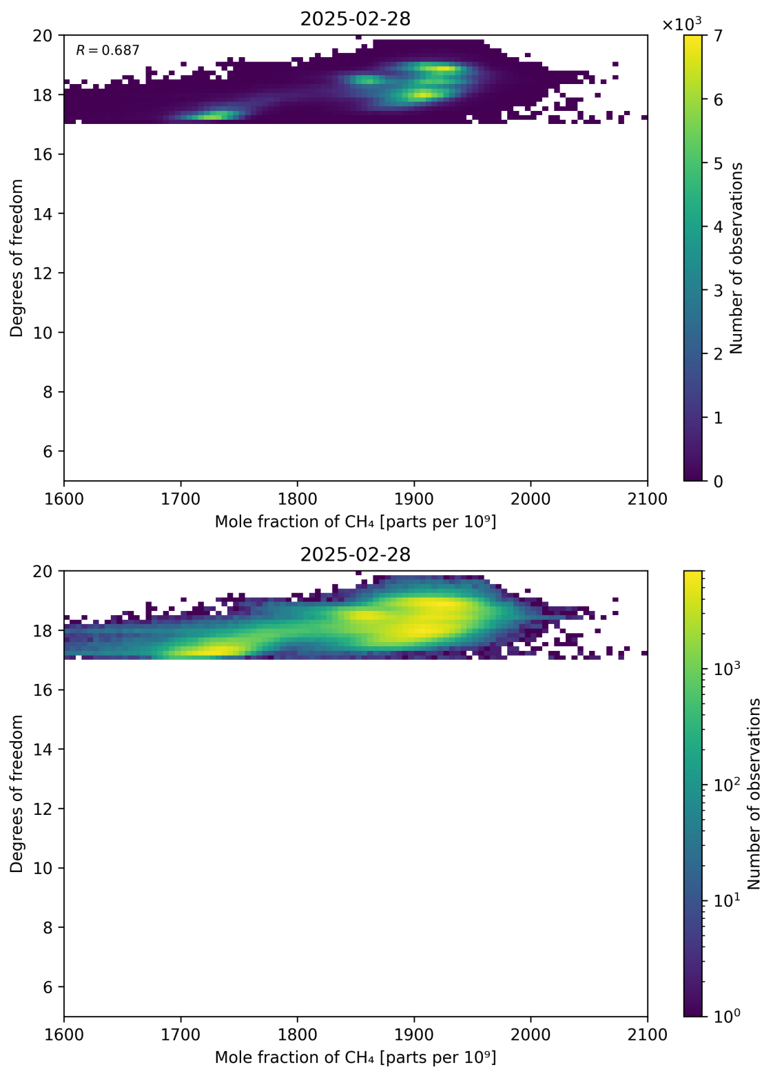
Figure 72: Scatter density plot of “Mole fraction of CH 4 ” against “Degrees of freedom” for 2025-02-27 to 2025-03-01.
