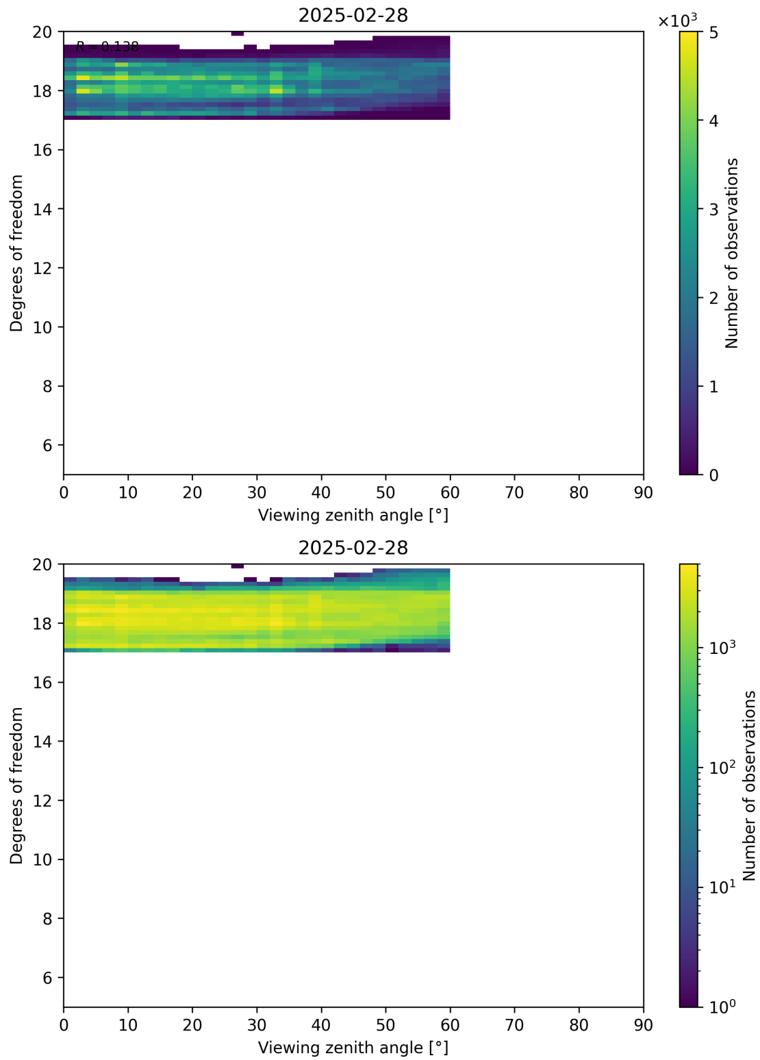
Figure 107: Scatter density plot of “Viewing zenith angle” against “Degrees of freedom” for 2025-02-27 to 2025-03-01.
