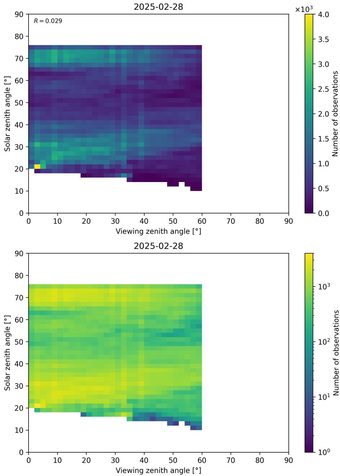
Figure 115: Scatter density plot of “Viewing zenith angle” against “Solar zenith angle” for 2025-02-27 to 2025-03-01.
