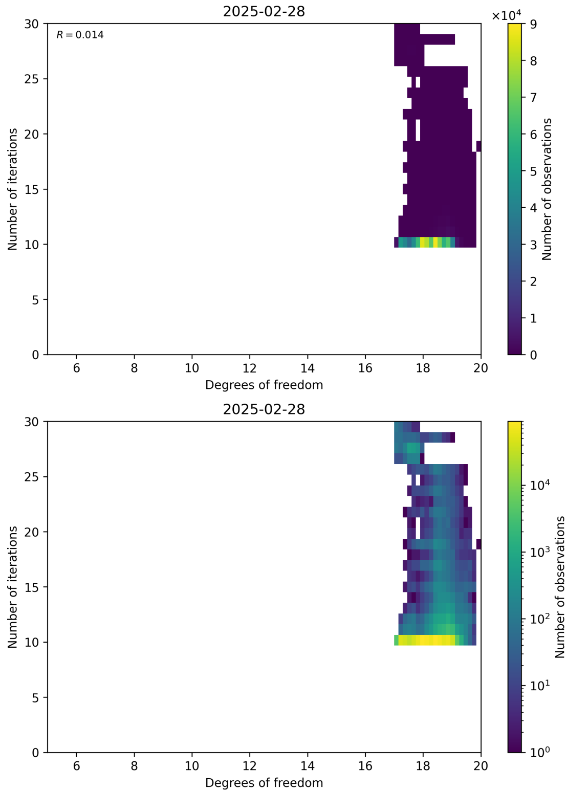
Figure 52: Scatter density plot of “Degrees of freedom” against “Number of iterations” for 2025-02-27 to 2025-03-01.
