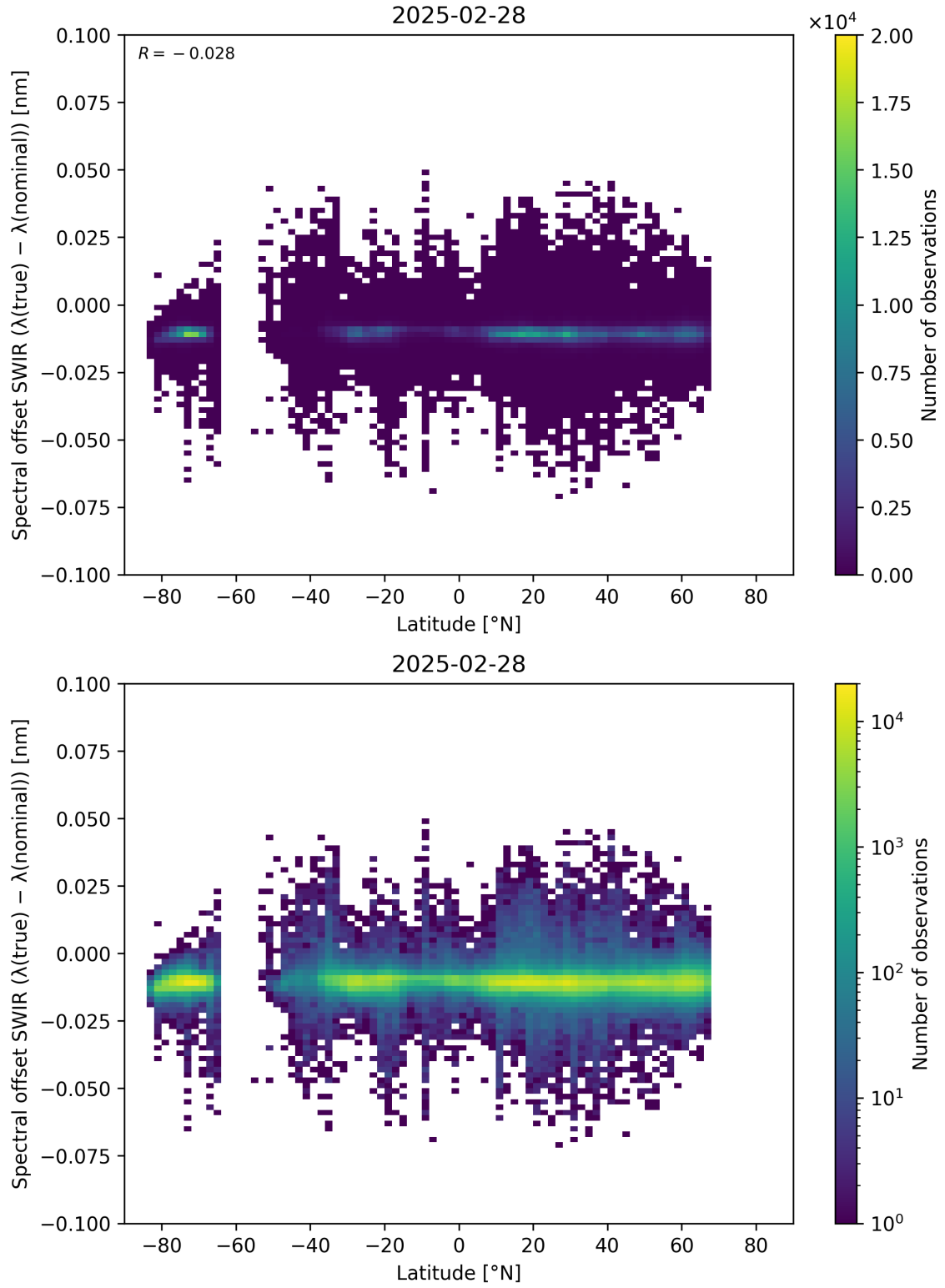
Figure 62: Scatter density plot of “Latitude” against “Spectral offset SWIR ( \lambda_{\text{true}} - \lambda_{\text{nominal}} )” for 2025-02-27 to 2025-03-01.
