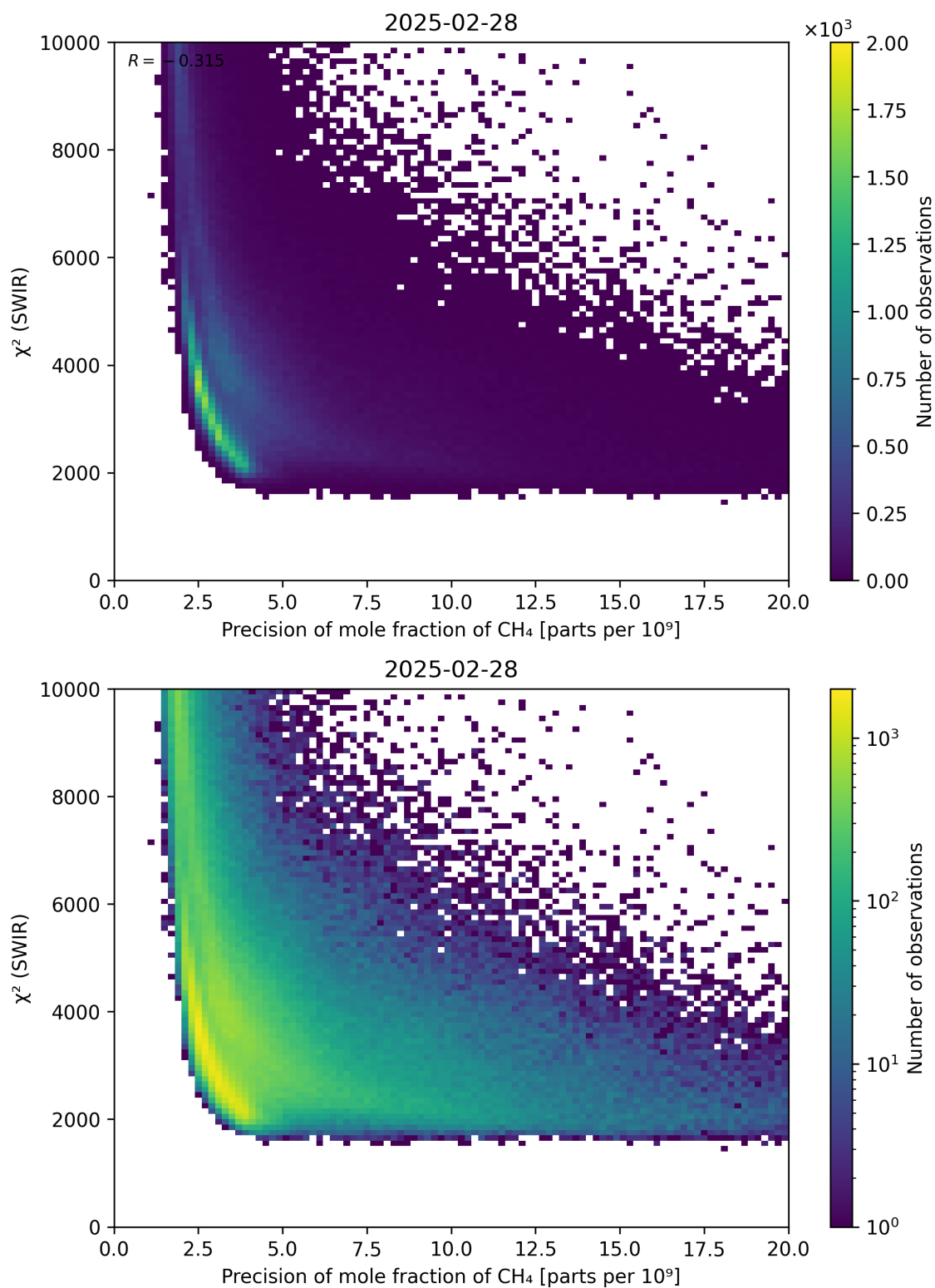
Figure 79: Scatter density plot of “Precision of mole fraction of \text{CH}_4 ” against “ \chi^2 (SWIR)” for 2025-02-27 to 2025-03-01.
