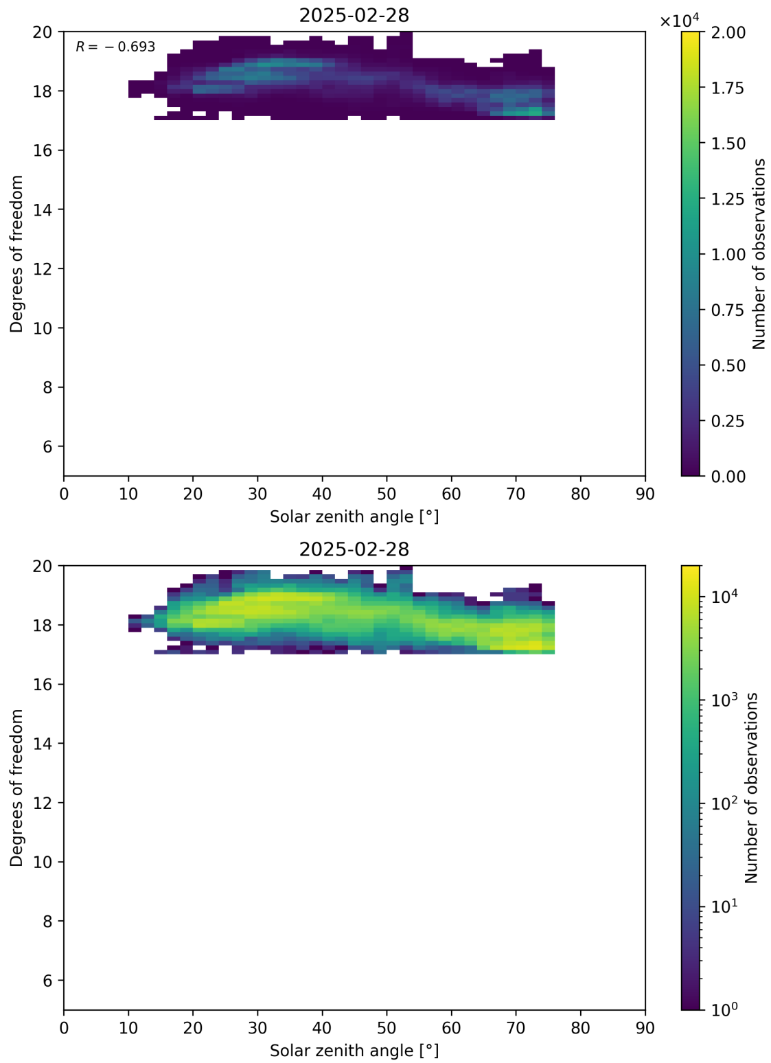
Figure 96: Scatter density plot of “Solar zenith angle” against “Degrees of freedom” for 2025-02-27 to 2025-03-01.
