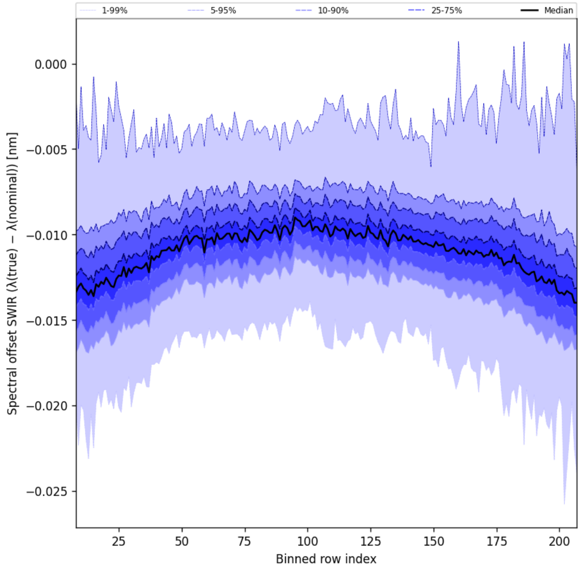
Figure 38: Along track statistics of “Spectral offset SWIR ( \lambda_{\text{true}} - \lambda_{\text{nominal}} )” for 2025-02-27 to 2025-03-01
