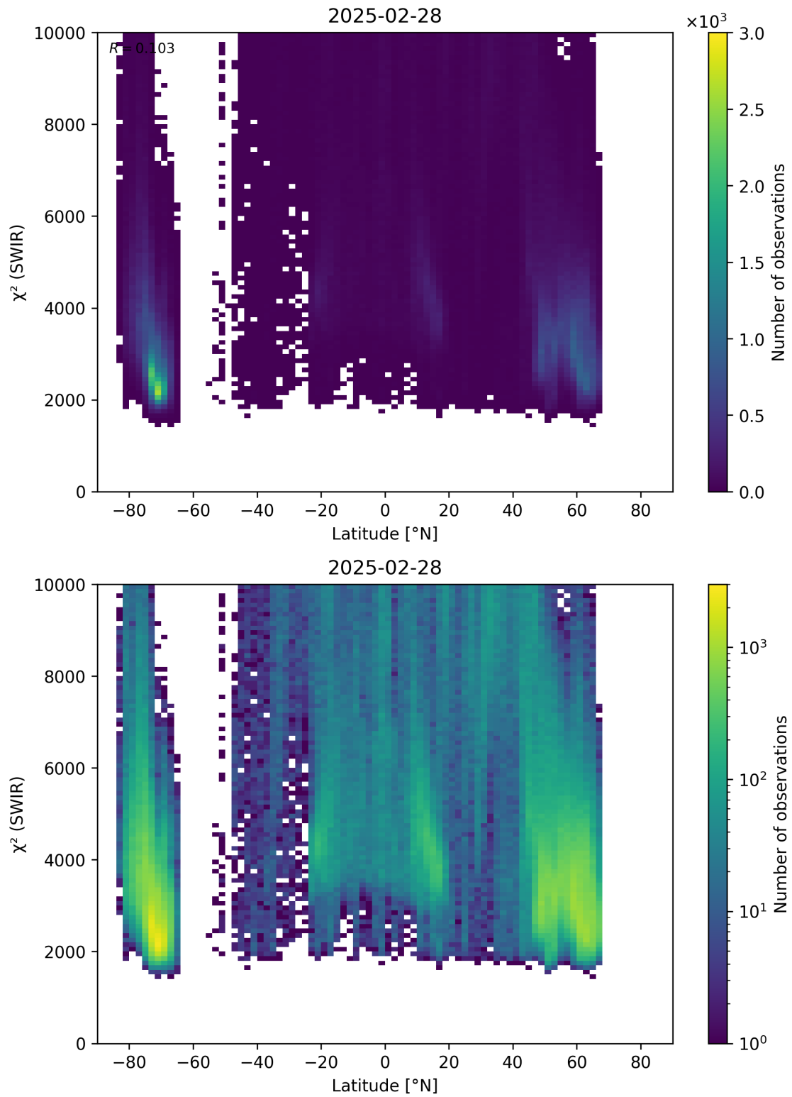
Figure 54: Scatter density plot of “Latitude” against “ \chi^2 (SWIR)” for 2025-02-27 to 2025-03-01.
