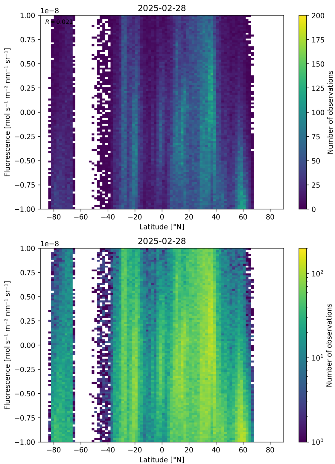
Figure 56: Scatter density plot of “Latitude” against “Fluorescence” for 2025-02-27 to 2025-03-01.
