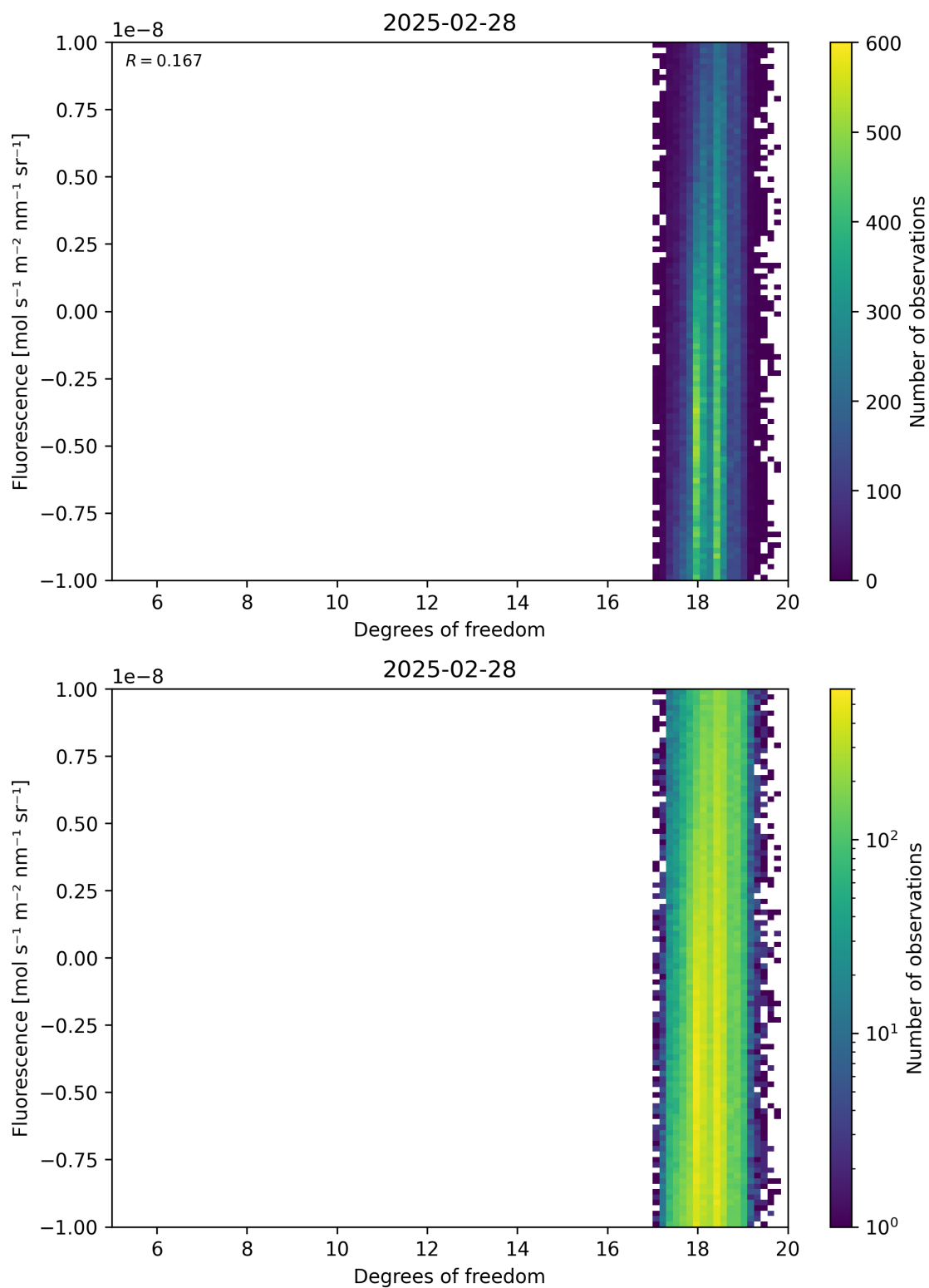
Figure 51: Scatter density plot of “Degrees of freedom” against “Fluorescence” for 2025-02-27 to 2025-03-01.
