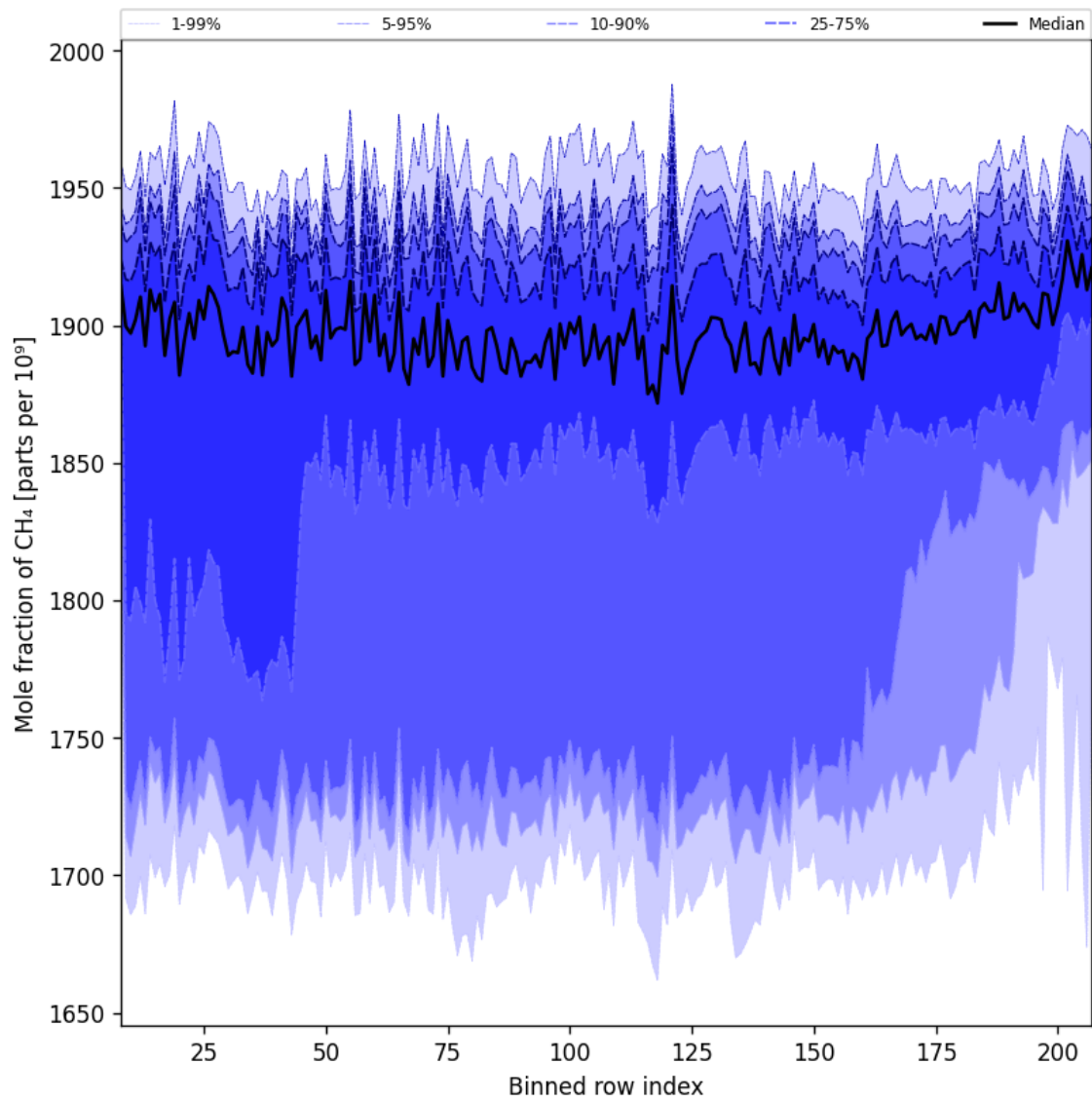
Figure 34: Along track statistics of “Mole fraction of CH 4 ” for 2025-02-27 to 2025-03-01
