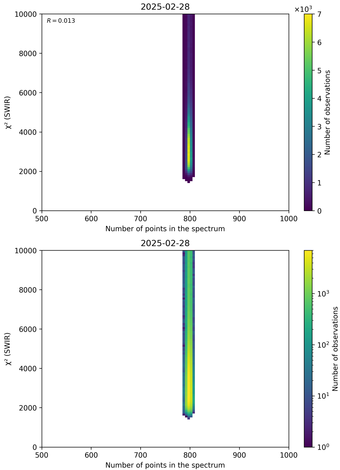
Figure 89: Scatter density plot of “Number of points in the spectrum” against “ \chi^2 (SWIR)” for 2025-02-27 to 2025-03-01.
