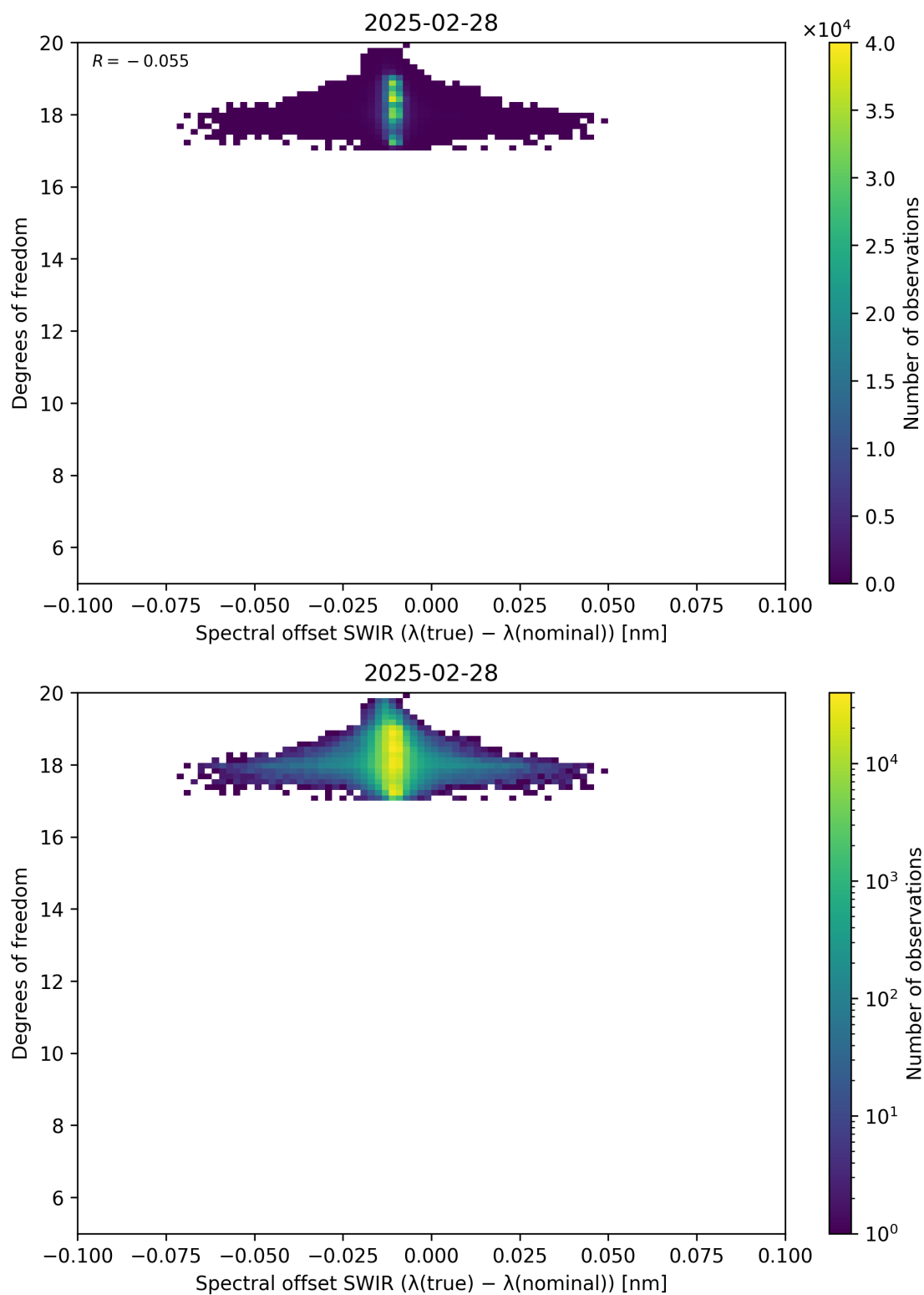
Figure 119: Scatter density plot of “Spectral offset SWIR ( \lambda_{\text{true}} - \lambda_{\text{nominal}} )” against “Degrees of freedom” for 2025-02-27 to 2025-03-01.
