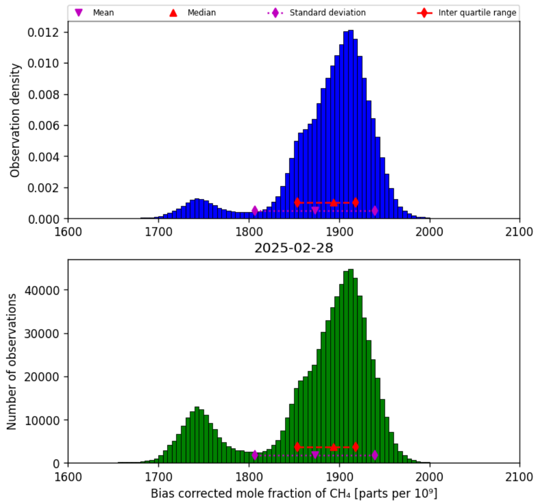
Figure 25: Histogram of “Bias corrected mole fraction of CH 4 ” for 2025-02-27 to 2025-03-01
