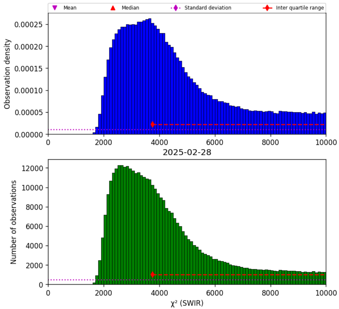
Figure 28: Histogram of “ \chi^2 (SWIR)” for 2025-02-27 to 2025-03-01
