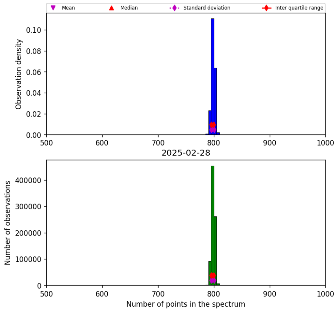
Figure 26: Histogram of “Number of points in the spectrum” for 2025-02-27 to 2025-03-01
