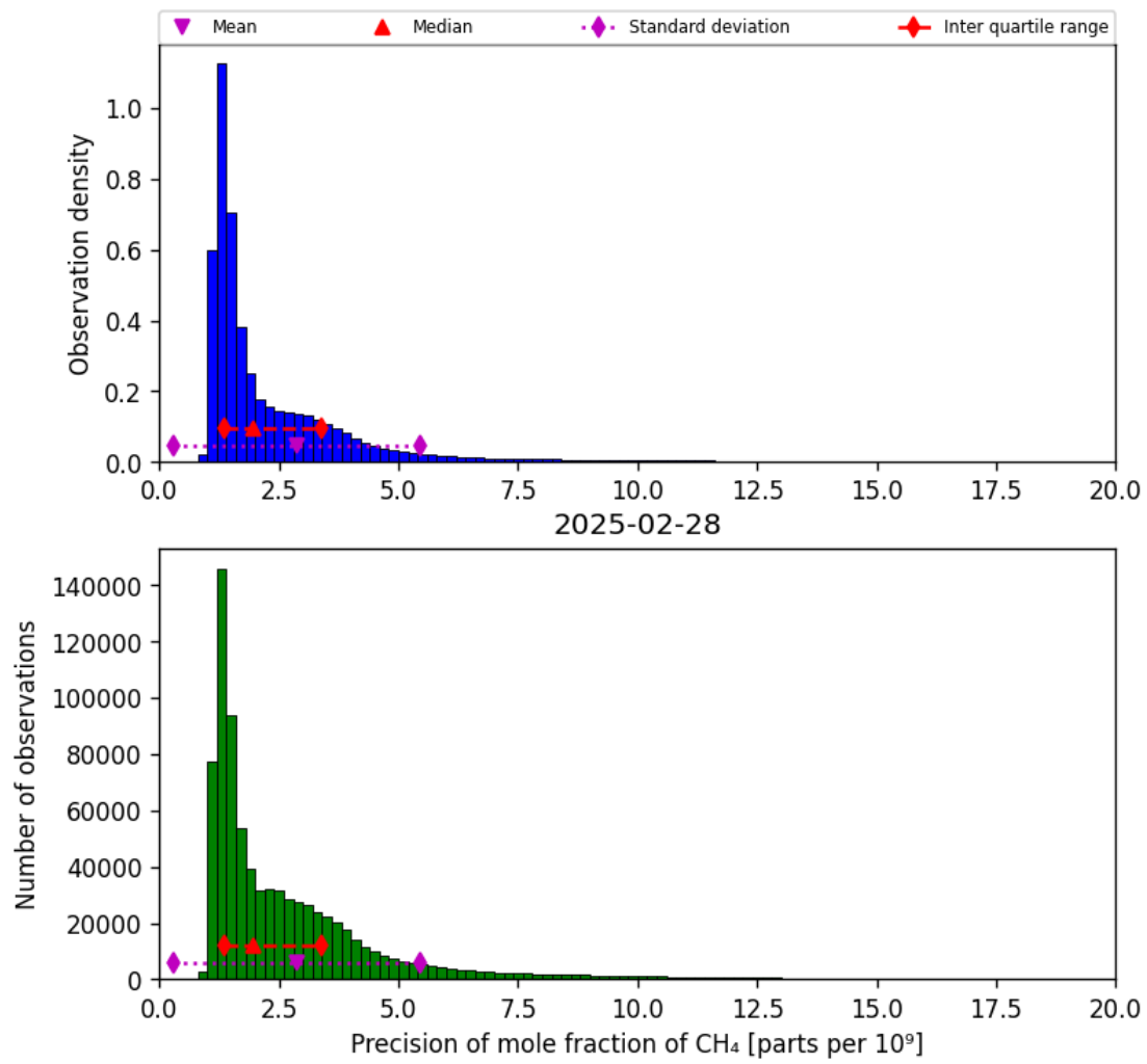
Figure 24: Histogram of “Precision of mole fraction of CH 4 ” for 2025-02-27 to 2025-03-01
