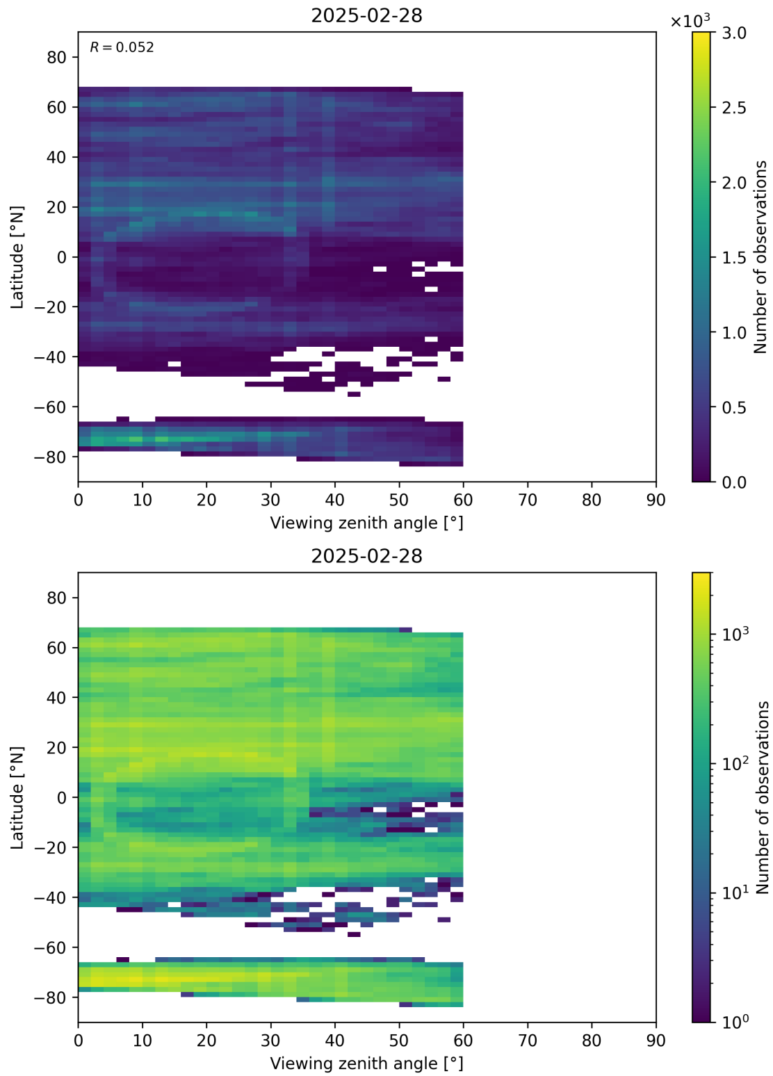
Figure 109: Scatter density plot of “Viewing zenith angle” against “Latitude” for 2025-02-27 to 2025-03-01.
