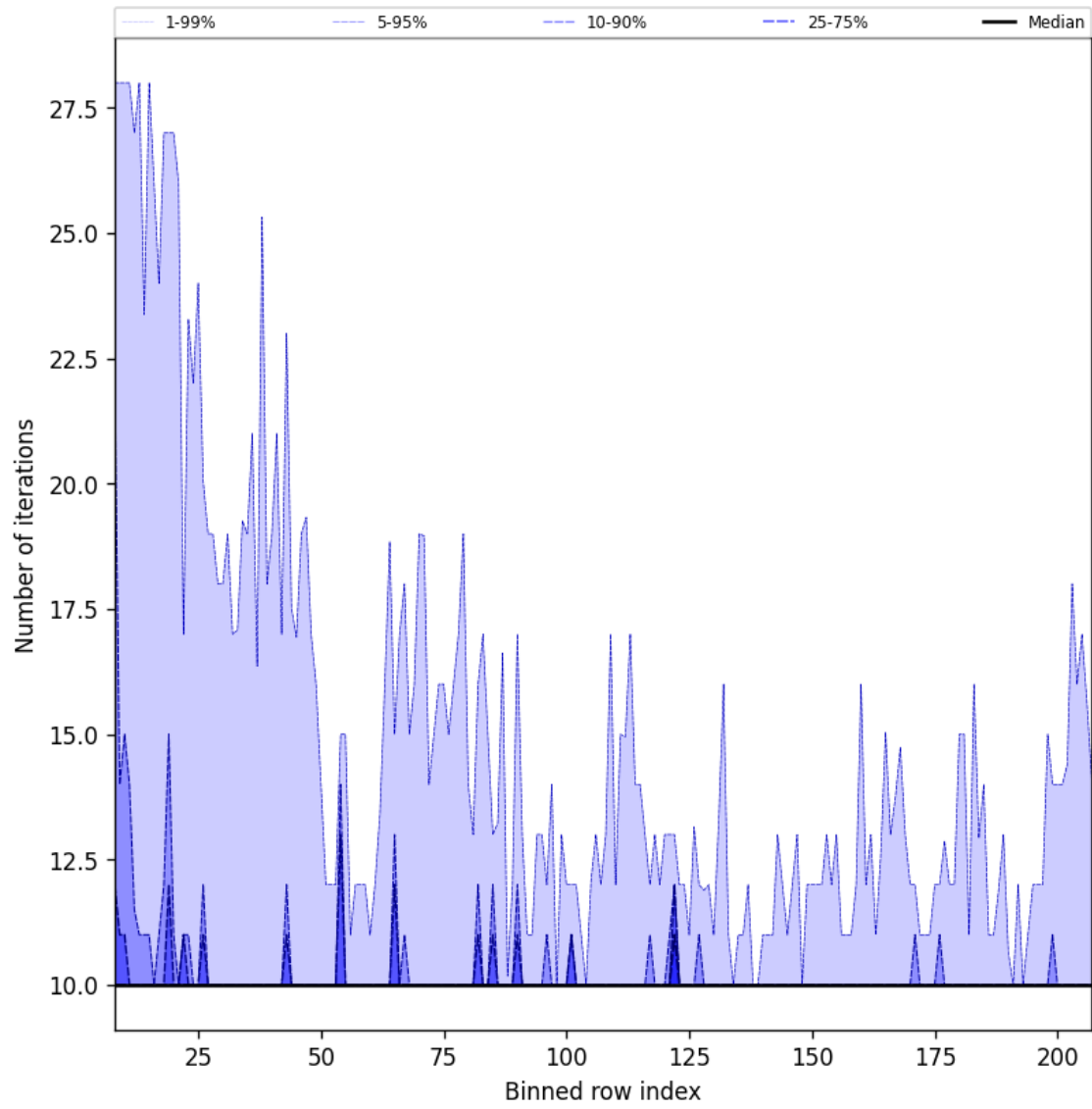
Figure 42: Along track statistics of “Number of iterations” for 2025-02-27 to 2025-03-01
