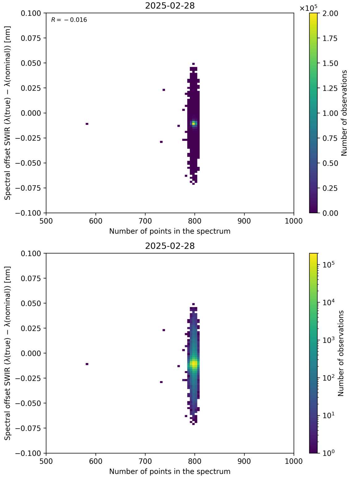
Figure 93: Scatter density plot of “Number of points in the spectrum” against “Spectral offset SWIR ( \lambda_{\text{true}} - \lambda_{\text{nominal}} )” for 2025-02-27 to 2025-03-01.
