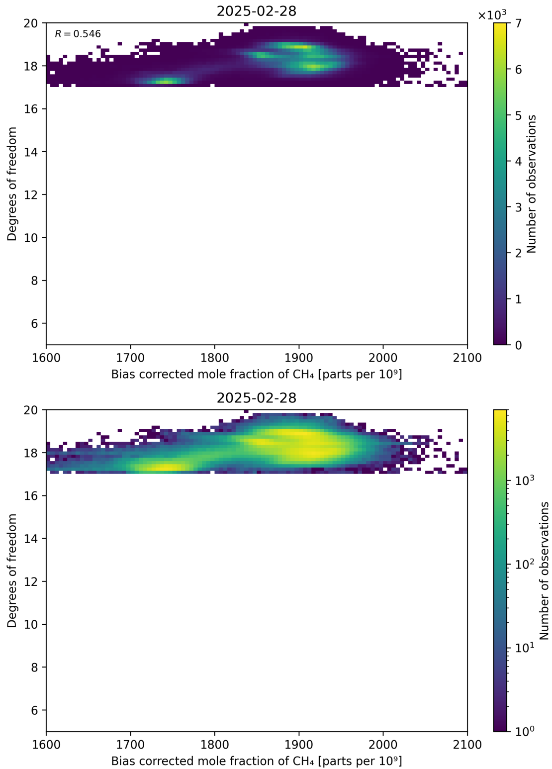
Figure 65: Scatter density plot of “Bias corrected mole fraction of CH 4 ” against “Degrees of freedom” for 2025-02-27 to 2025-03-01.
