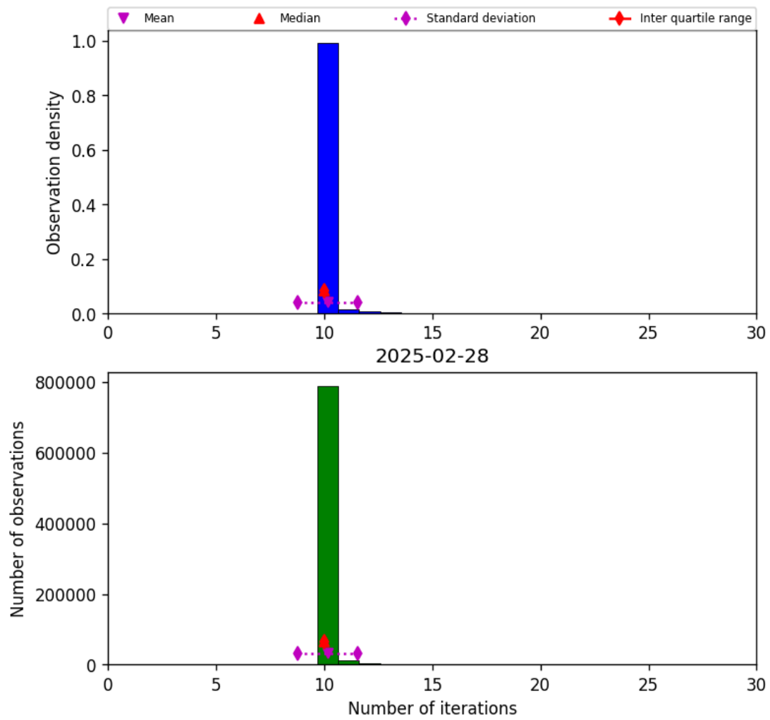
Figure 31: Histogram of “Number of iterations” for 2025-02-27 to 2025-03-01
