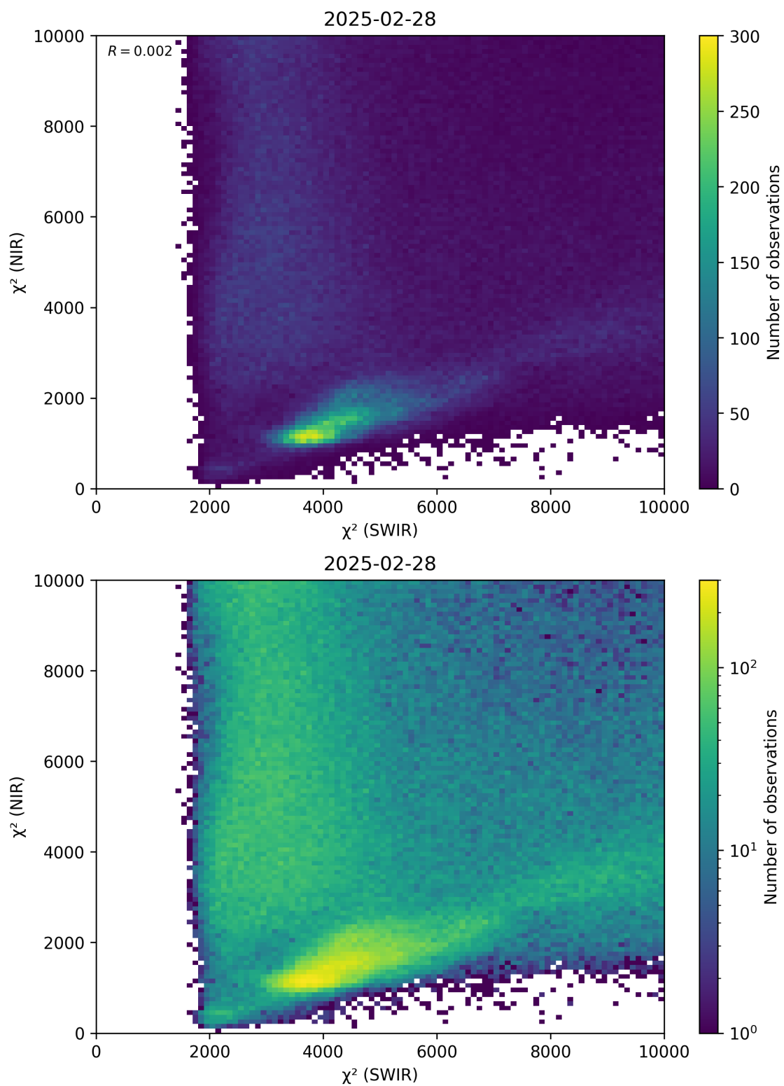
Figure 47: Scatter density plot of “ \chi^2 (SWIR)” against “ \chi^2 (NIR)” for 2025-02-27 to 2025-03-01.
