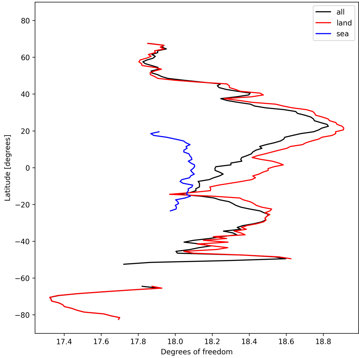
Figure 19: Zonal average of “Degrees of freedom” for 2025-02-27 to 2025-03-01.
