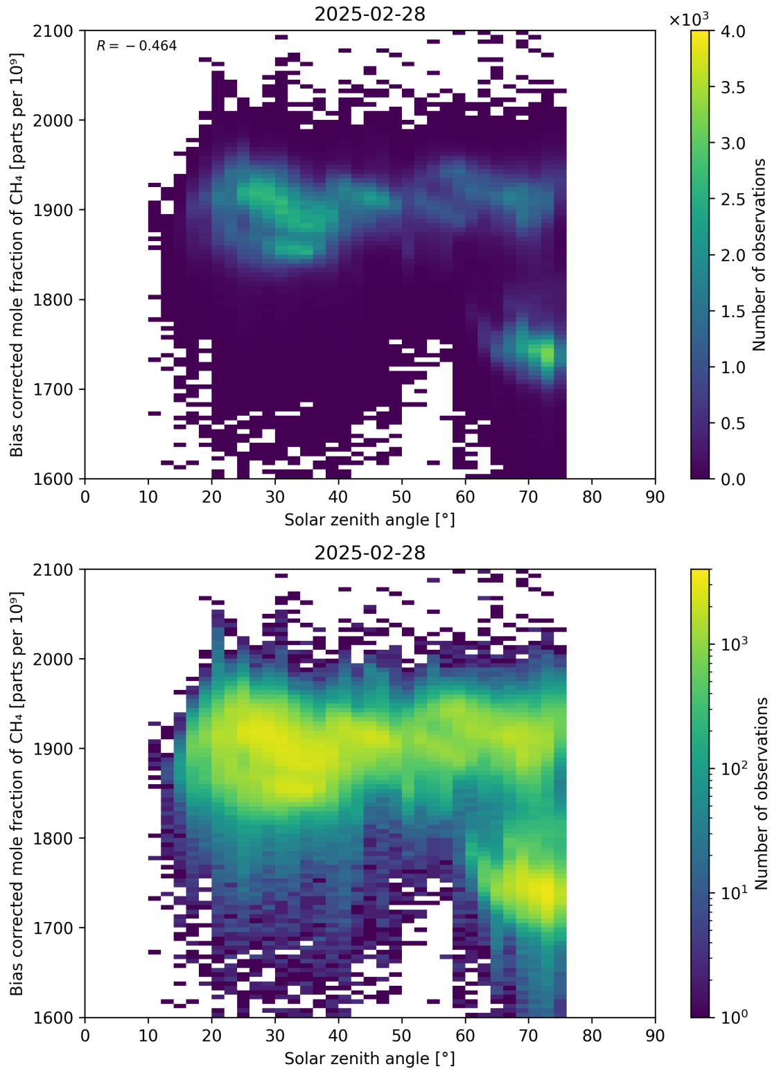
Figure 100: Scatter density plot of “Solar zenith angle” against “Bias corrected mole fraction of \text{CH}_4 ” for 2025-02-27 to 2025-03-01.
