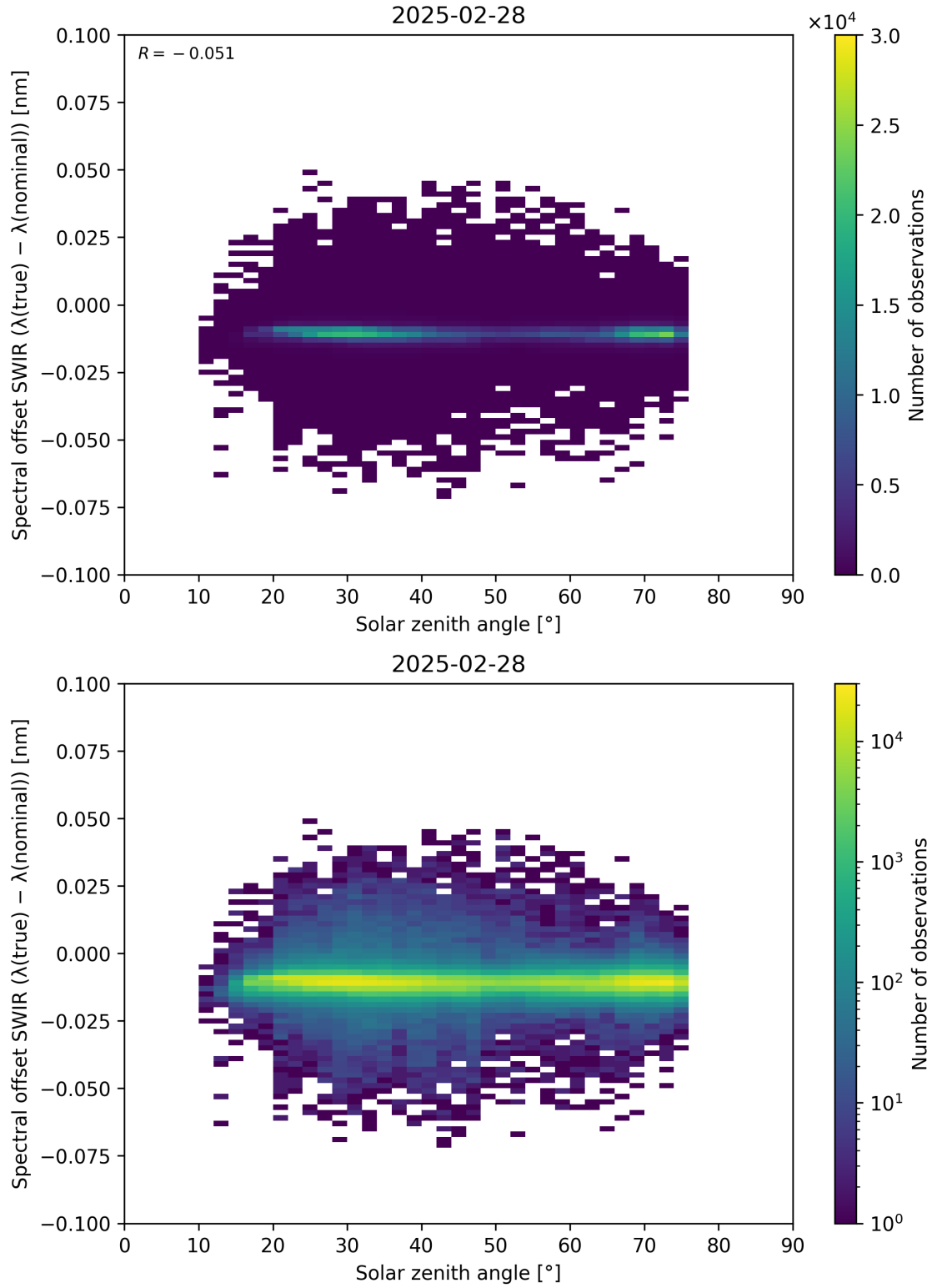
Figure 104: Scatter density plot of “Solar zenith angle” against “Spectral offset SWIR ( \lambda_{\text{true}} - \lambda_{\text{nominal}} )” for 2025-02-27 to 2025-03-01.
