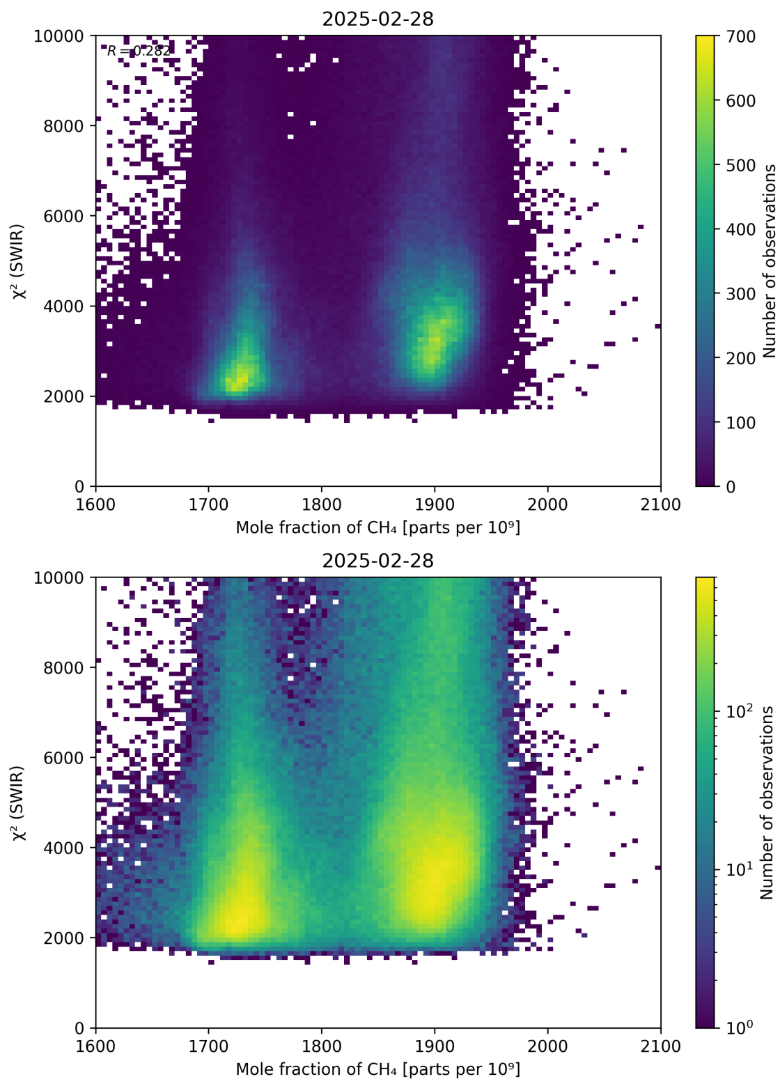
Figure 71: Scatter density plot of “Mole fraction of \text{CH}_4 ” against “ \chi^2 (SWIR)” for 2025-02-27 to 2025-03-01.
