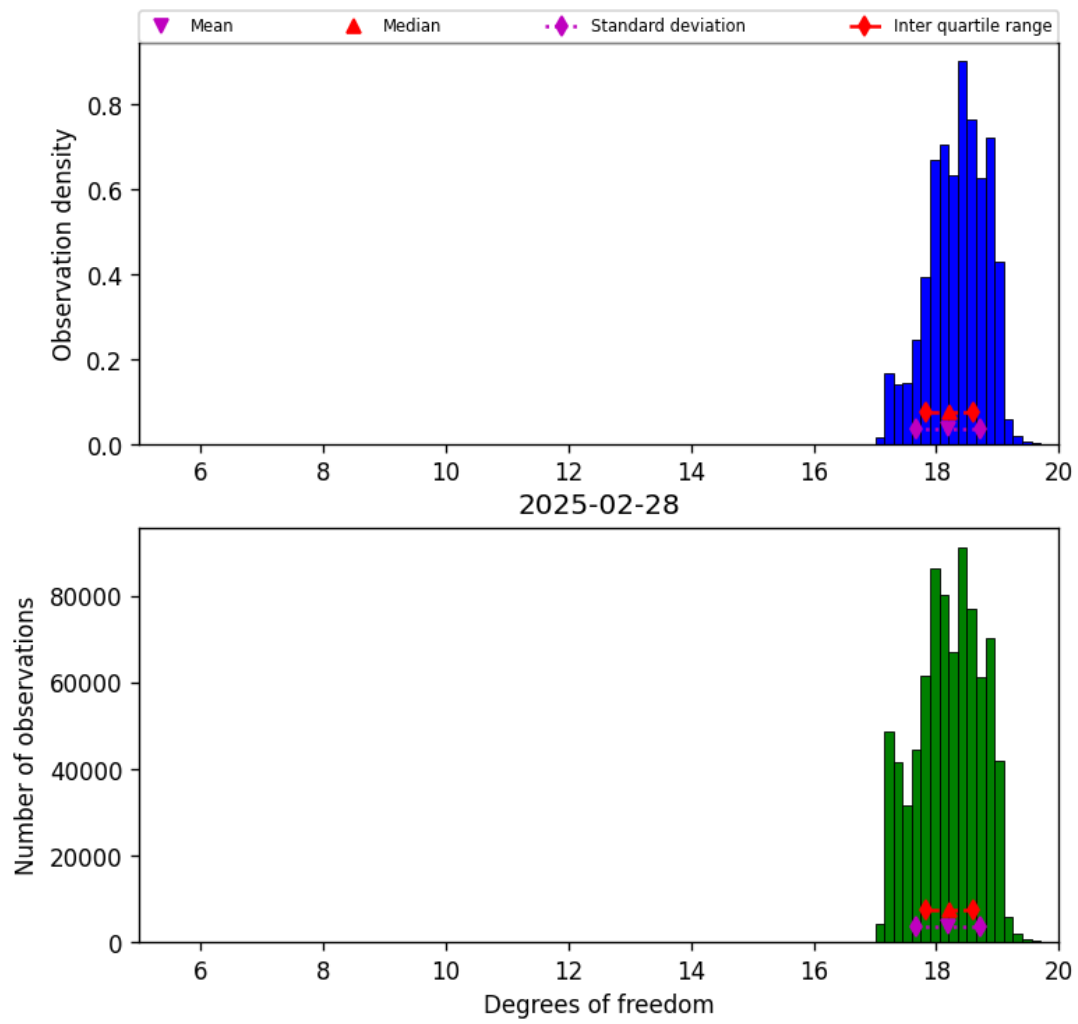
Figure 30: Histogram of “Degrees of freedom” for 2025-02-27 to 2025-03-01
