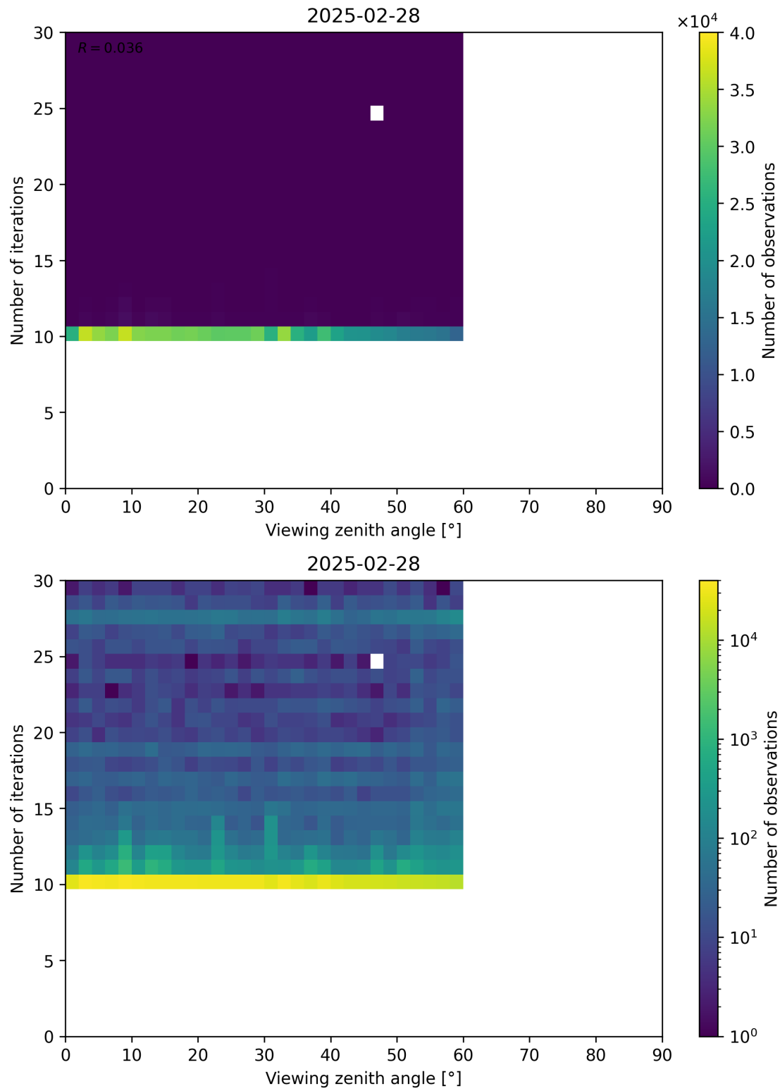
Figure 113: Scatter density plot of “Viewing zenith angle” against “Number of iterations” for 2025-02-27 to 2025-03-01.
