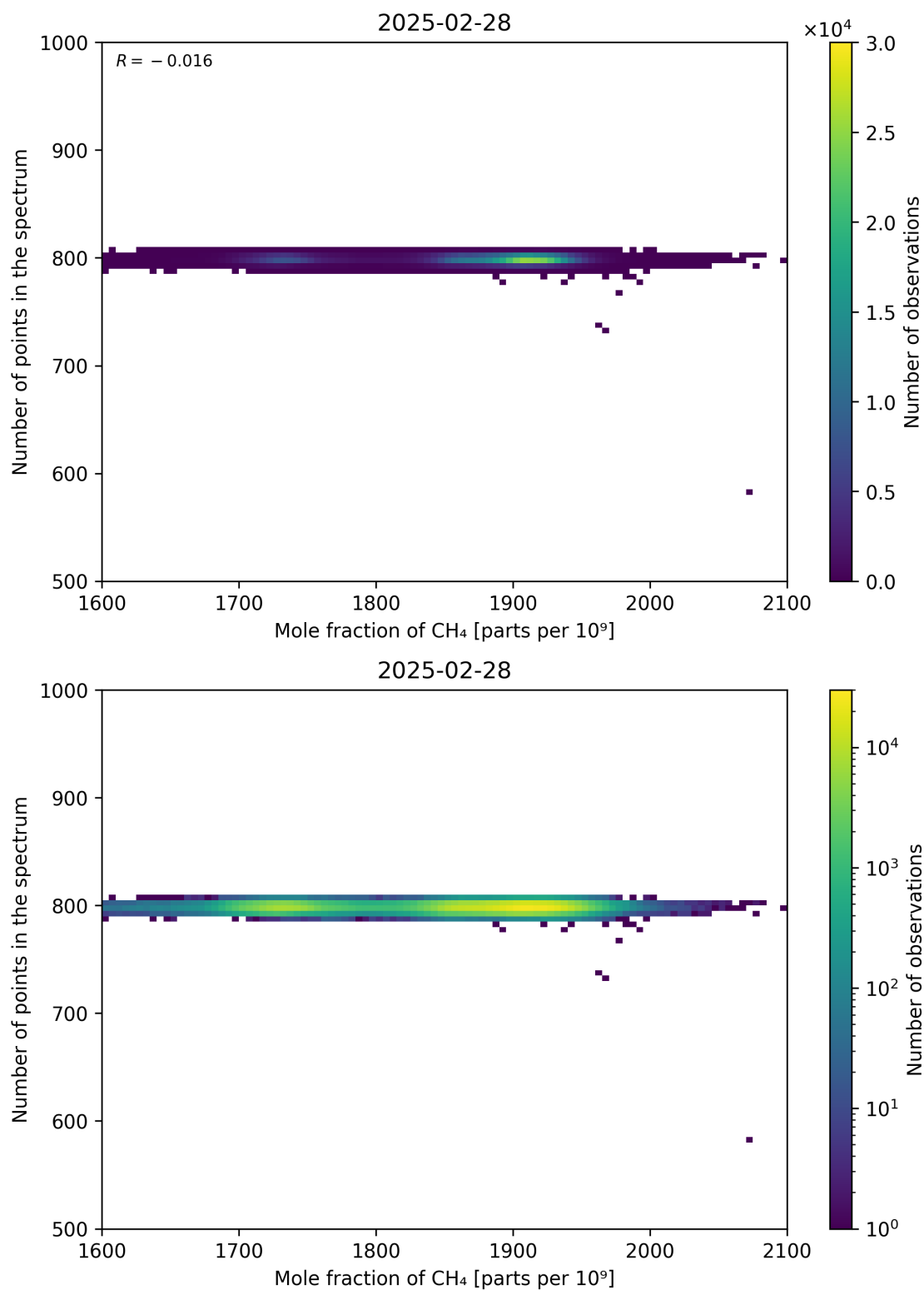
Figure 77: Scatter density plot of “Mole fraction of CH 4 ” against “Number of points in the spectrum” for 2025-02-27 to 2025-03-01.
