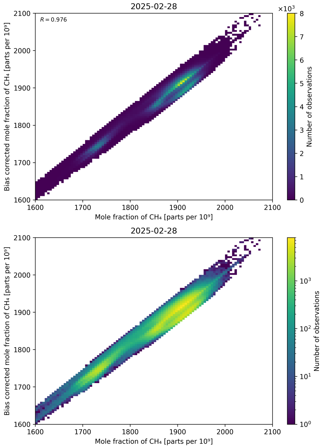
Figure 74: Scatter density plot of “Mole fraction of CH 4 ” against “Bias corrected mole fraction of CH 4 ” for 2025-02-27 to 2025-03-01.
