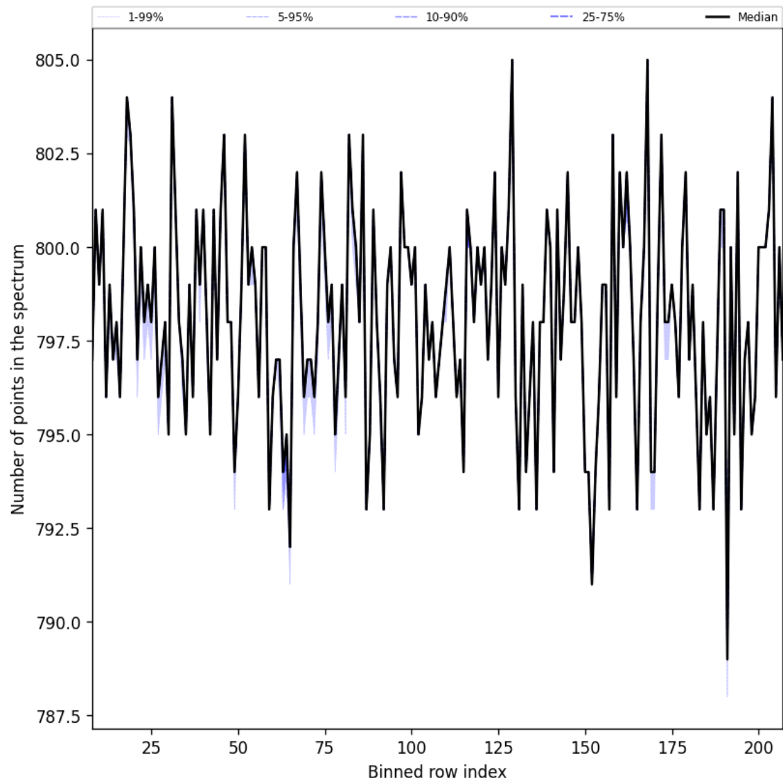
Figure 37: Along track statistics of “Number of points in the spectrum” for 2025-02-27 to 2025-03-01
