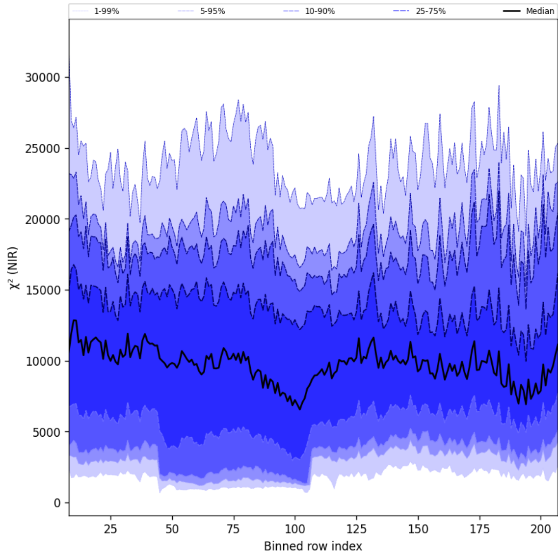
Figure 40: Along track statistics of “ \chi^2 (NIR)” for 2025-02-27 to 2025-03-01
