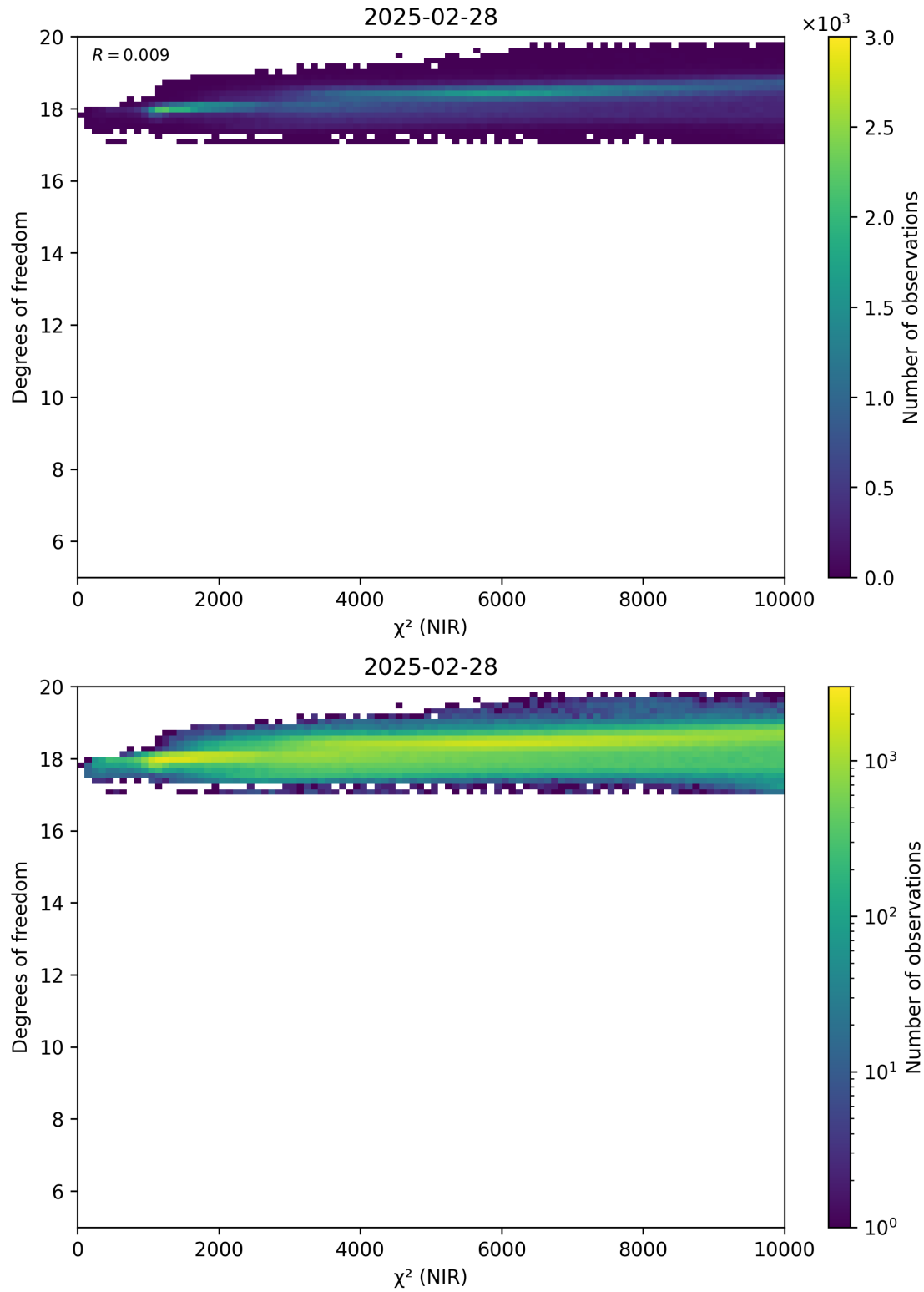
Figure 44: Scatter density plot of “ \chi^2 (NIR)” against “Degrees of freedom” for 2025-02-27 to 2025-03-01.
