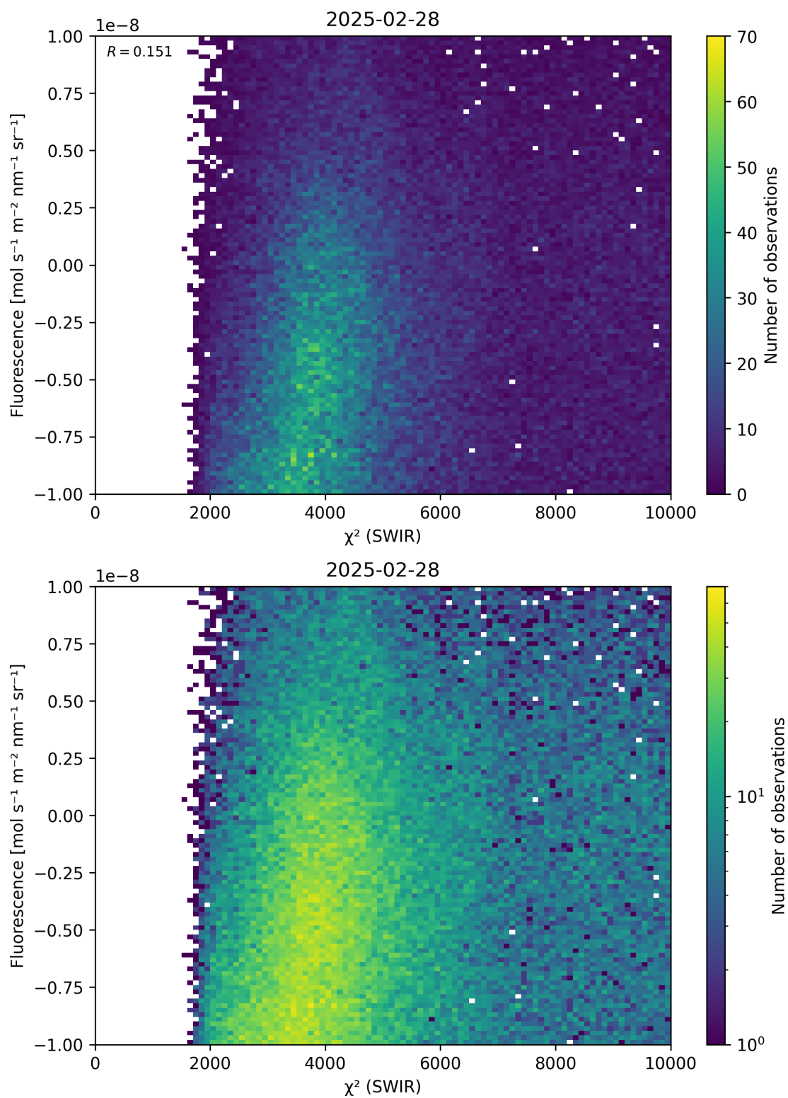
Figure 49: Scatter density plot of “ \chi^2 (SWIR)” against “Fluorescence” for 2025-02-27 to 2025-03-01.
