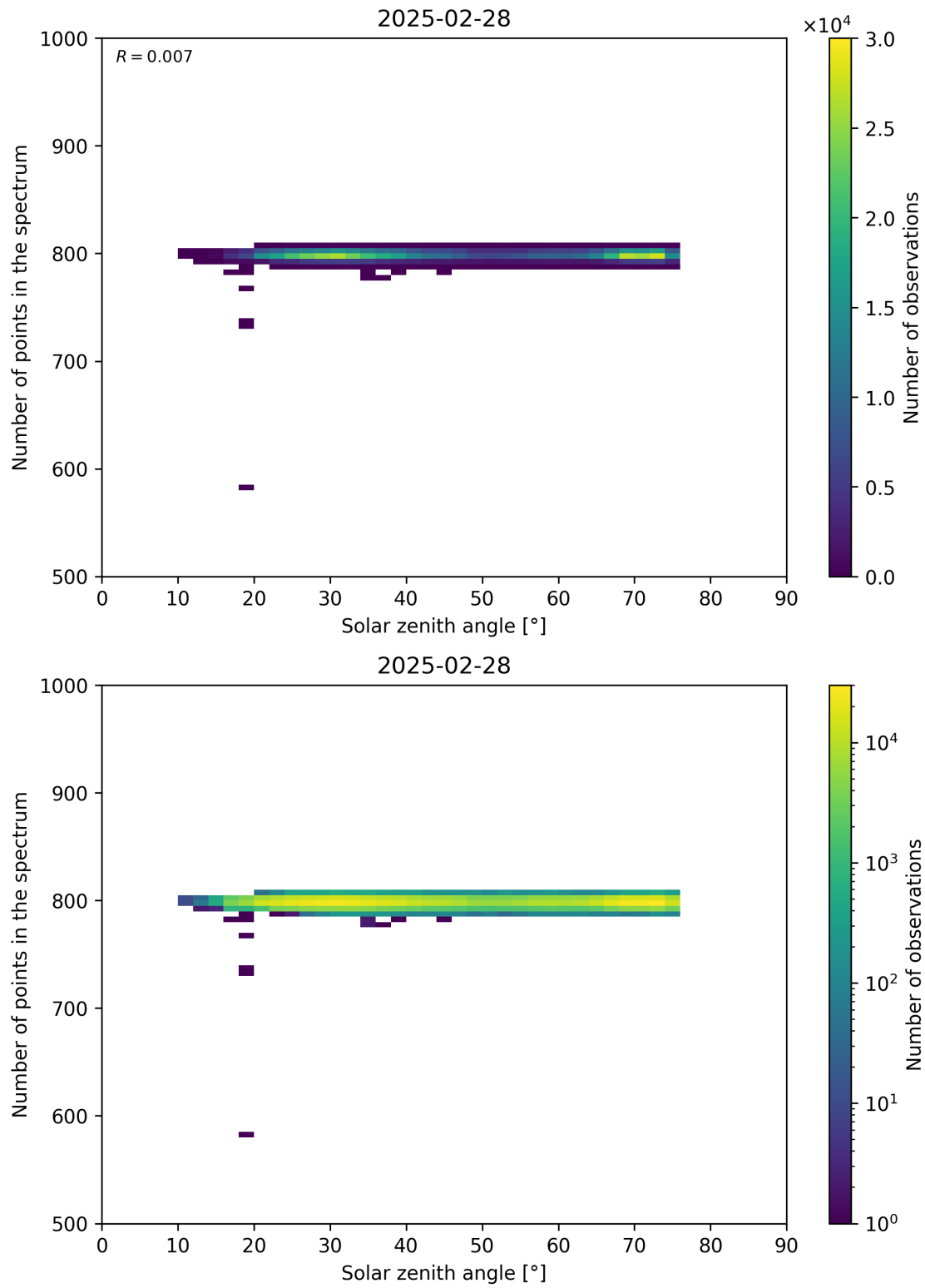
Figure 103: Scatter density plot of “Solar zenith angle” against “Number of points in the spectrum” for 2025-02-27 to 2025-03-01.
