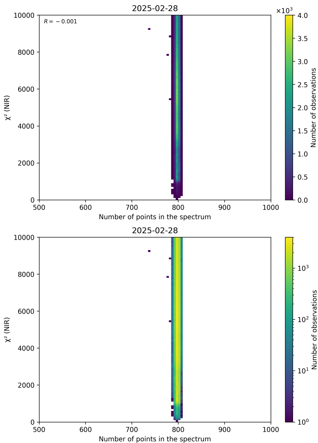
Figure 88: Scatter density plot of “Number of points in the spectrum” against “ \chi^2 (NIR)” for 2025-02-27 to 2025-03-01.
