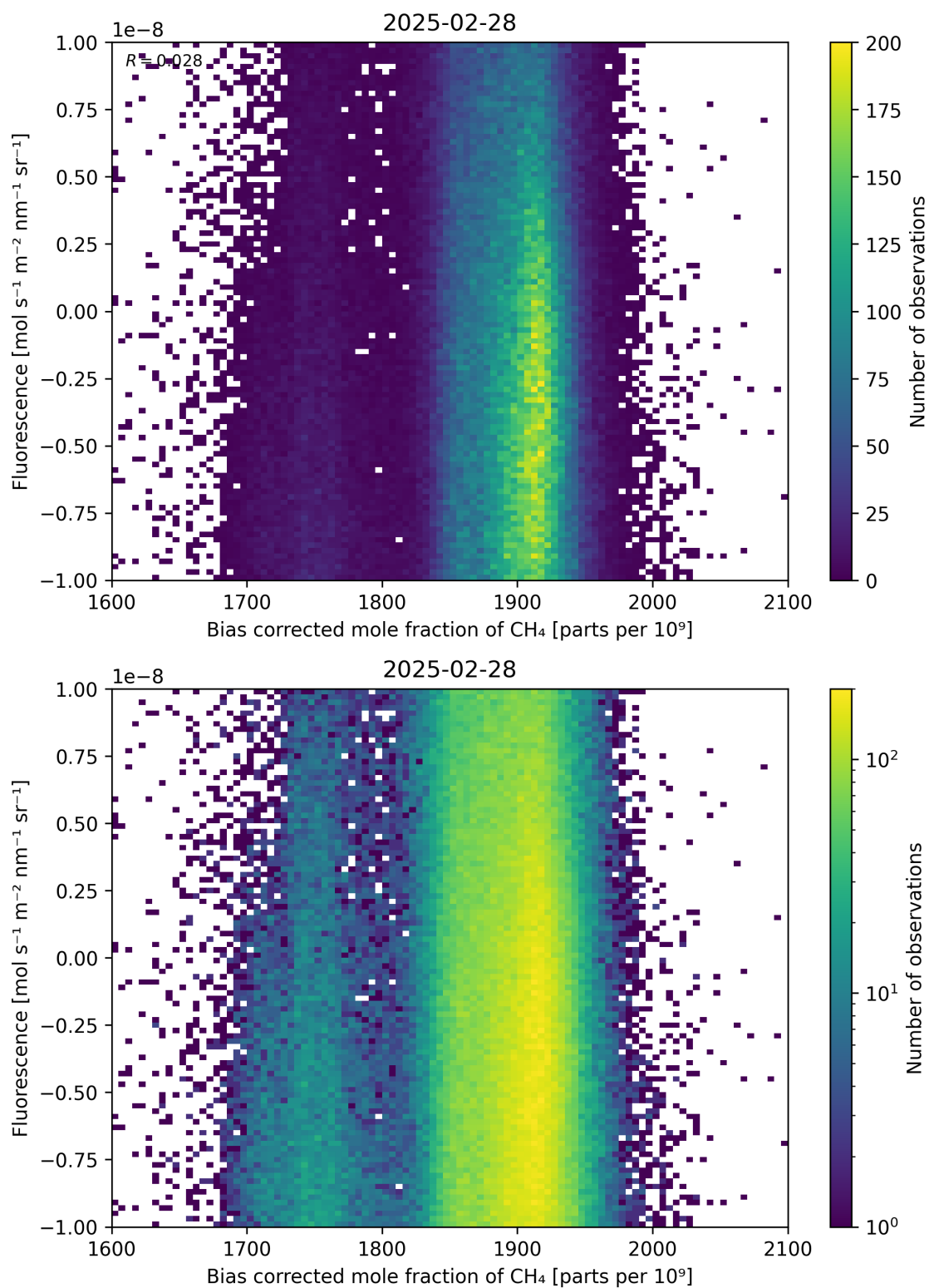
Figure 66: Scatter density plot of “Bias corrected mole fraction of \text{CH}_4 ” against “Fluorescence” for 2025-02-27 to 2025-03-01.
