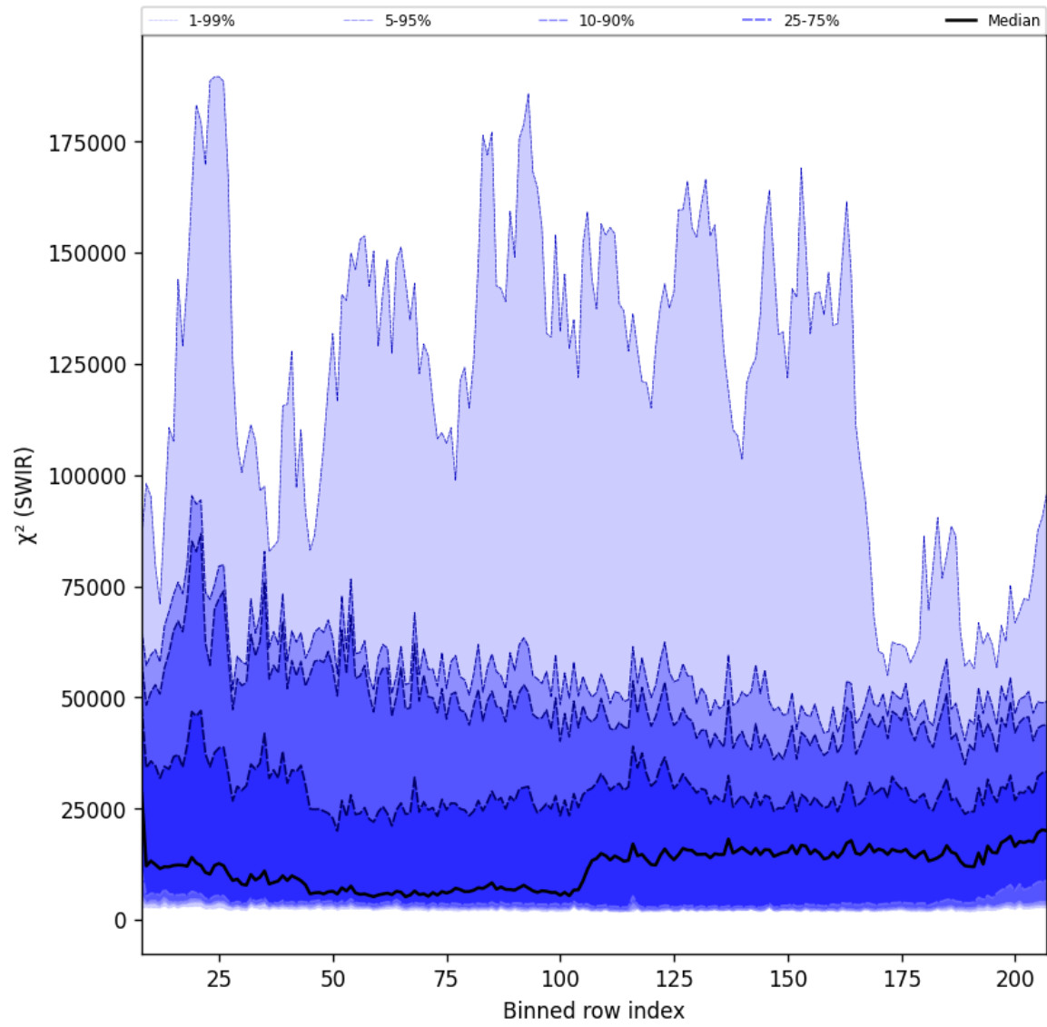
Figure 39: Along track statistics of “ \chi^2 (SWIR)” for 2025-02-27 to 2025-03-01
