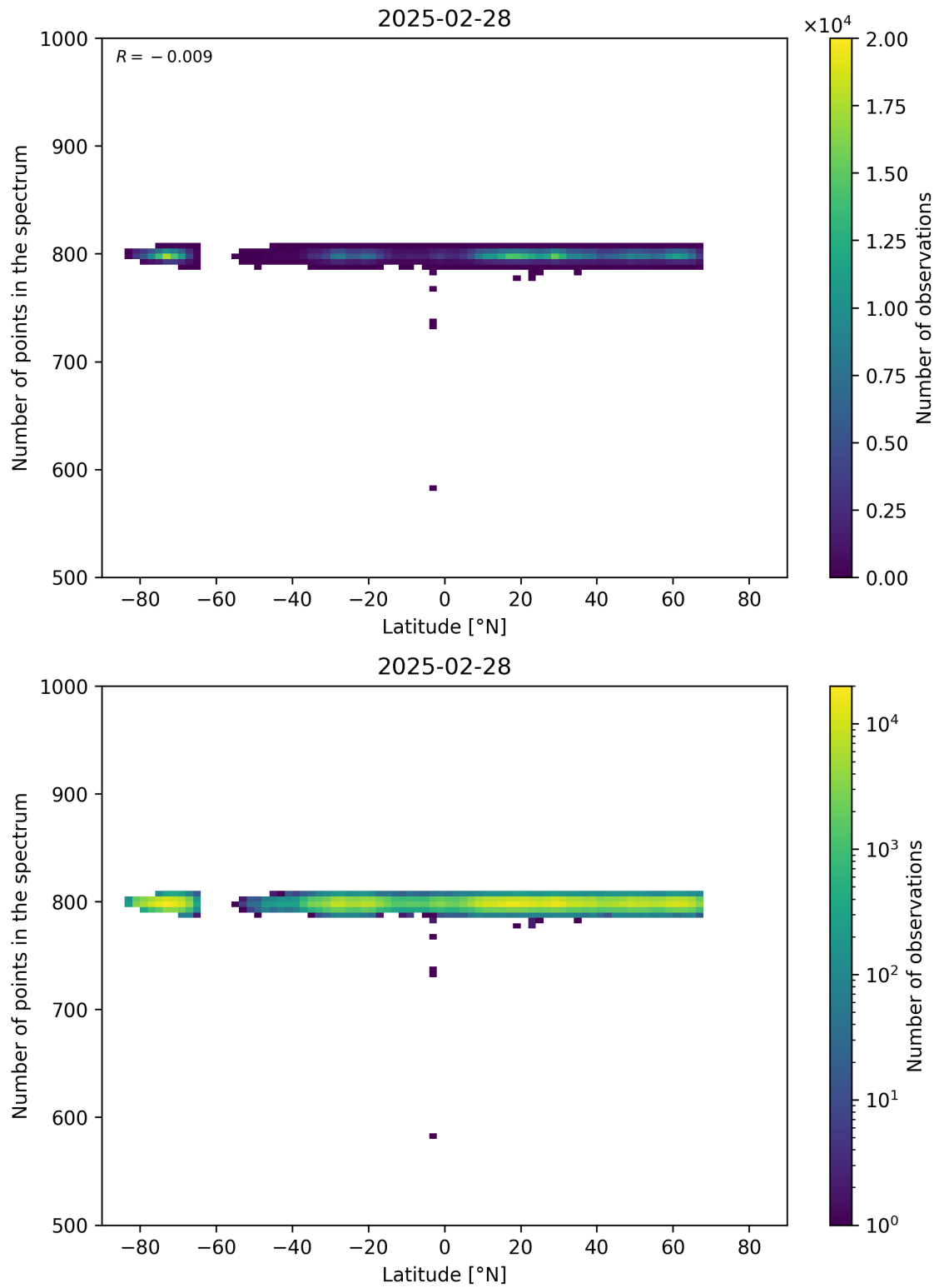
Figure 61: Scatter density plot of “Latitude” against “Number of points in the spectrum” for 2025-02-27 to 2025-03-01.
