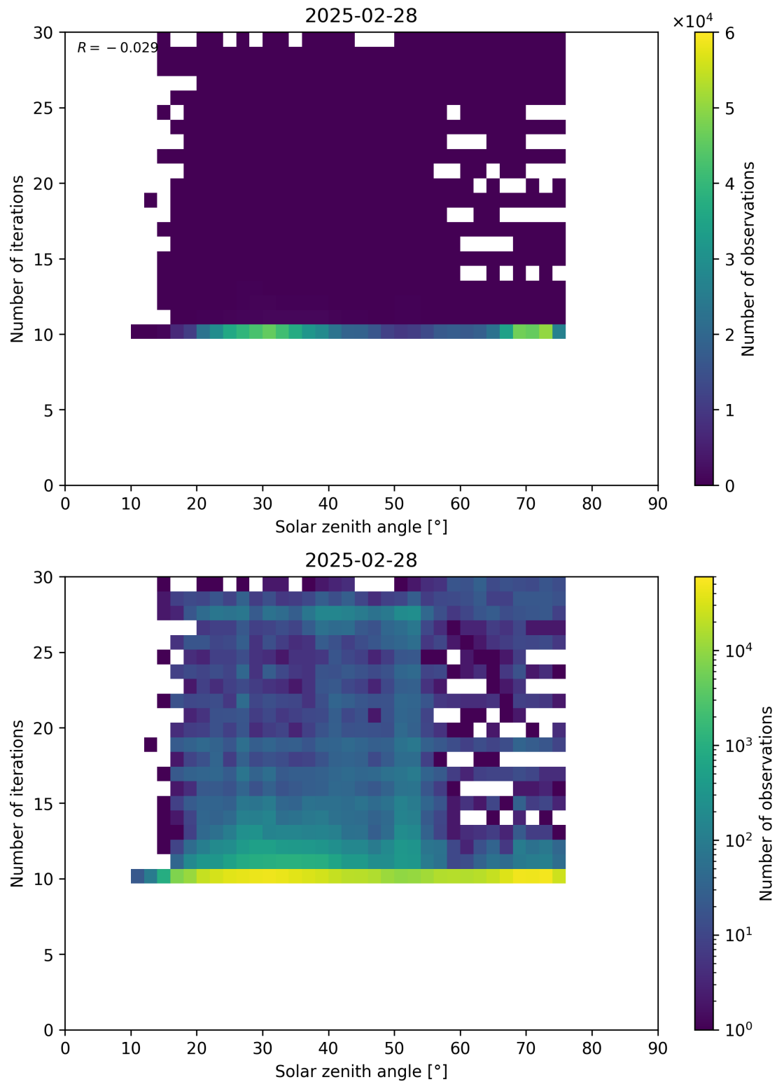
Figure 102: Scatter density plot of “Solar zenith angle” against “Number of iterations” for 2025-02-27 to 2025-03-01.
