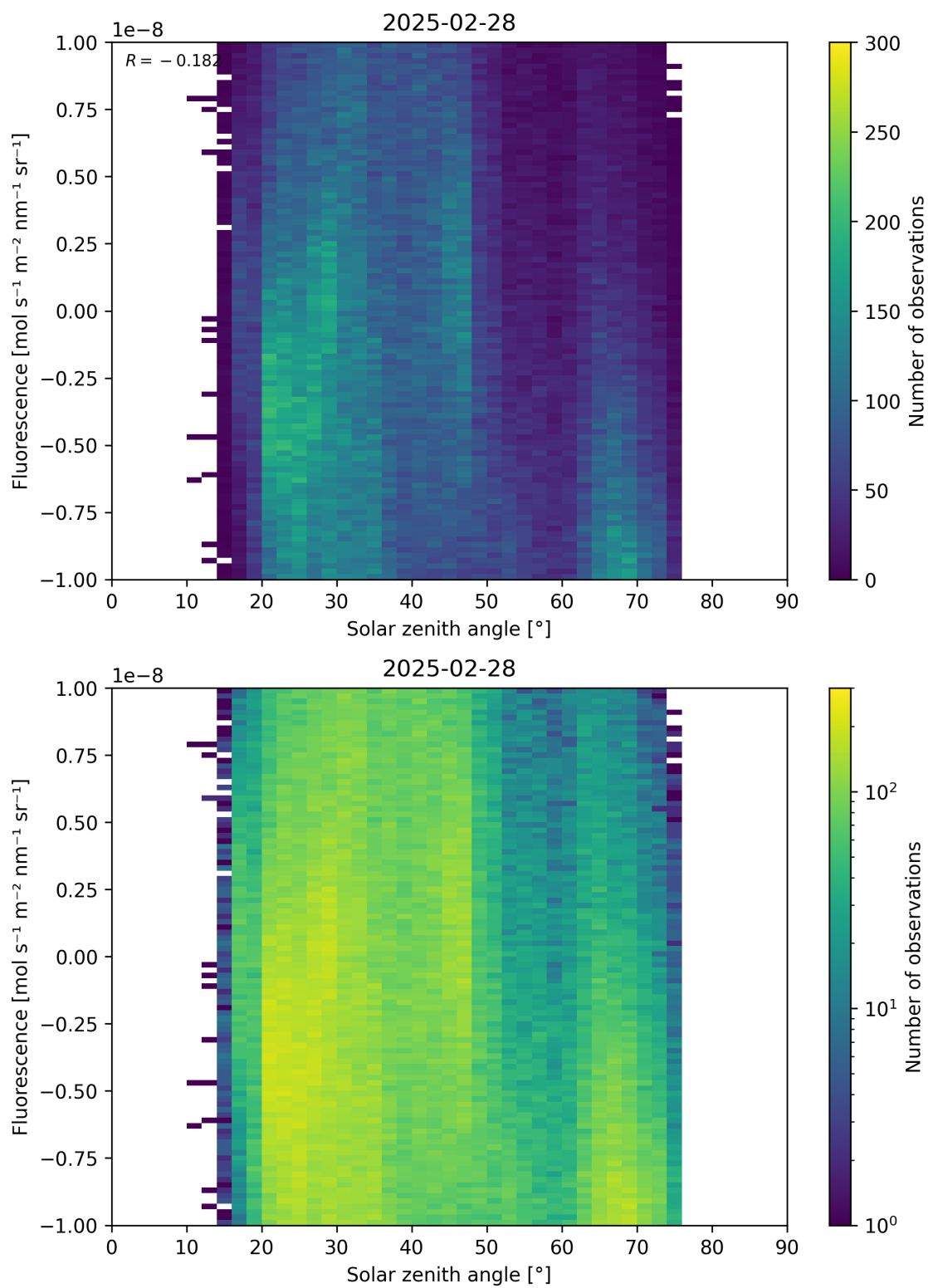
Figure 97: Scatter density plot of “Solar zenith angle” against “Fluorescence” for 2025-02-27 to 2025-03-01.
