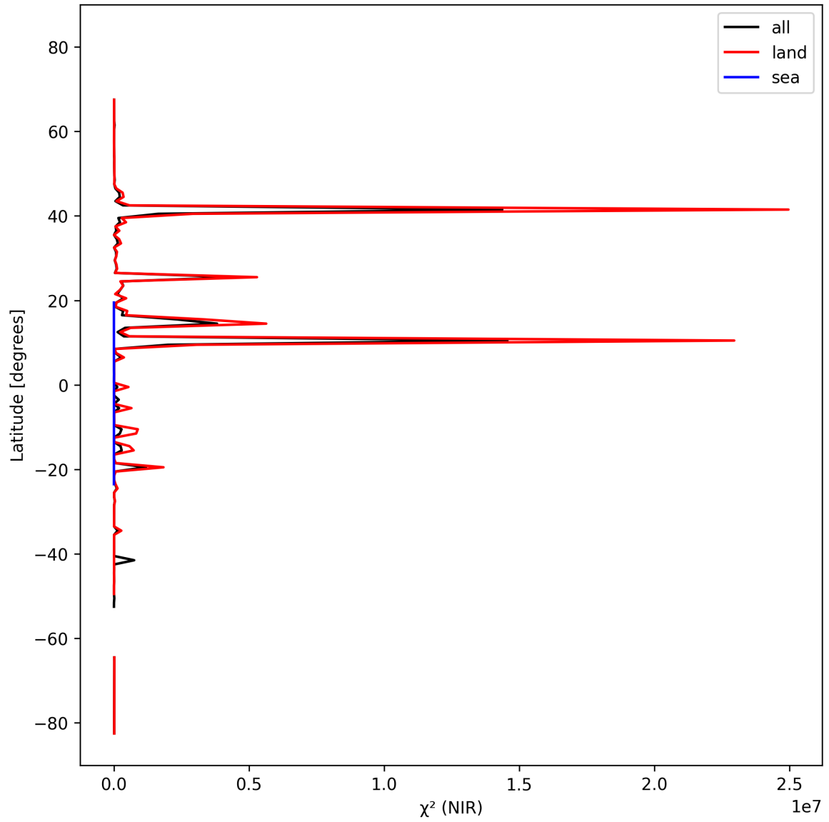
Figure 18: Zonal average of “ \chi^2 (NIR)” for 2025-02-27 to 2025-03-01.
