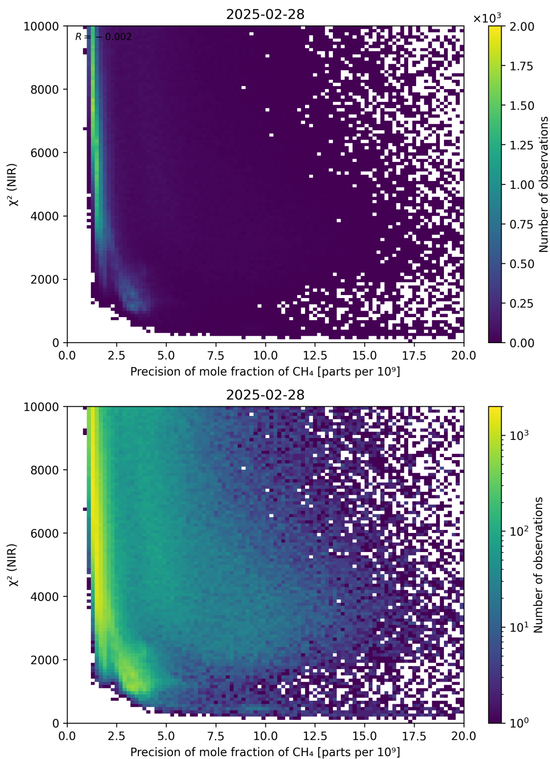
Figure 78: Scatter density plot of “Precision of mole fraction of CH 4 ” against “ \chi^2 (NIR)” for 2025-02-27 to 2025-03-01.
