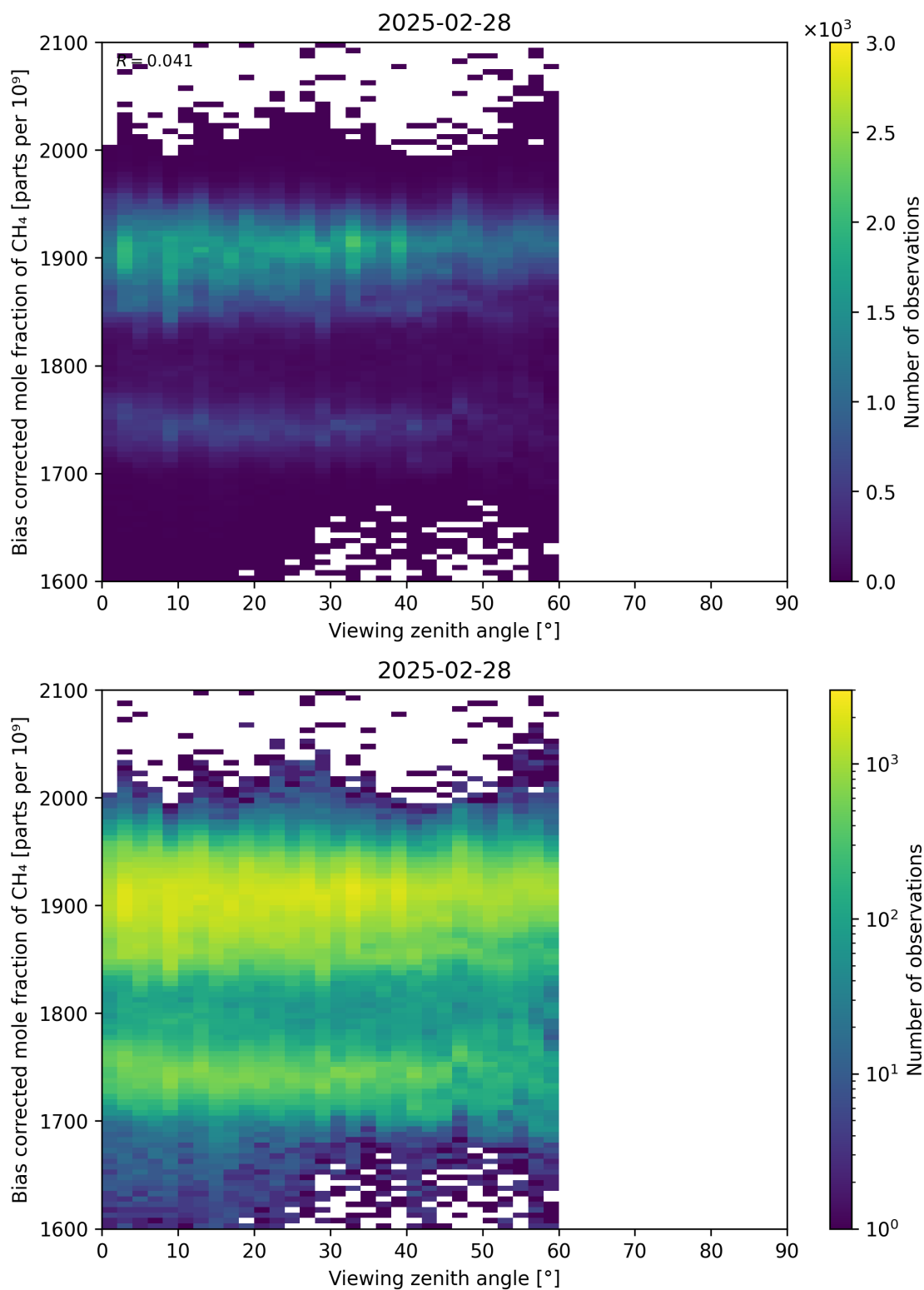
Figure 111: Scatter density plot of “Viewing zenith angle” against “Bias corrected mole fraction of CH 4 ” for 2025-02-27 to 2025-03-01.
