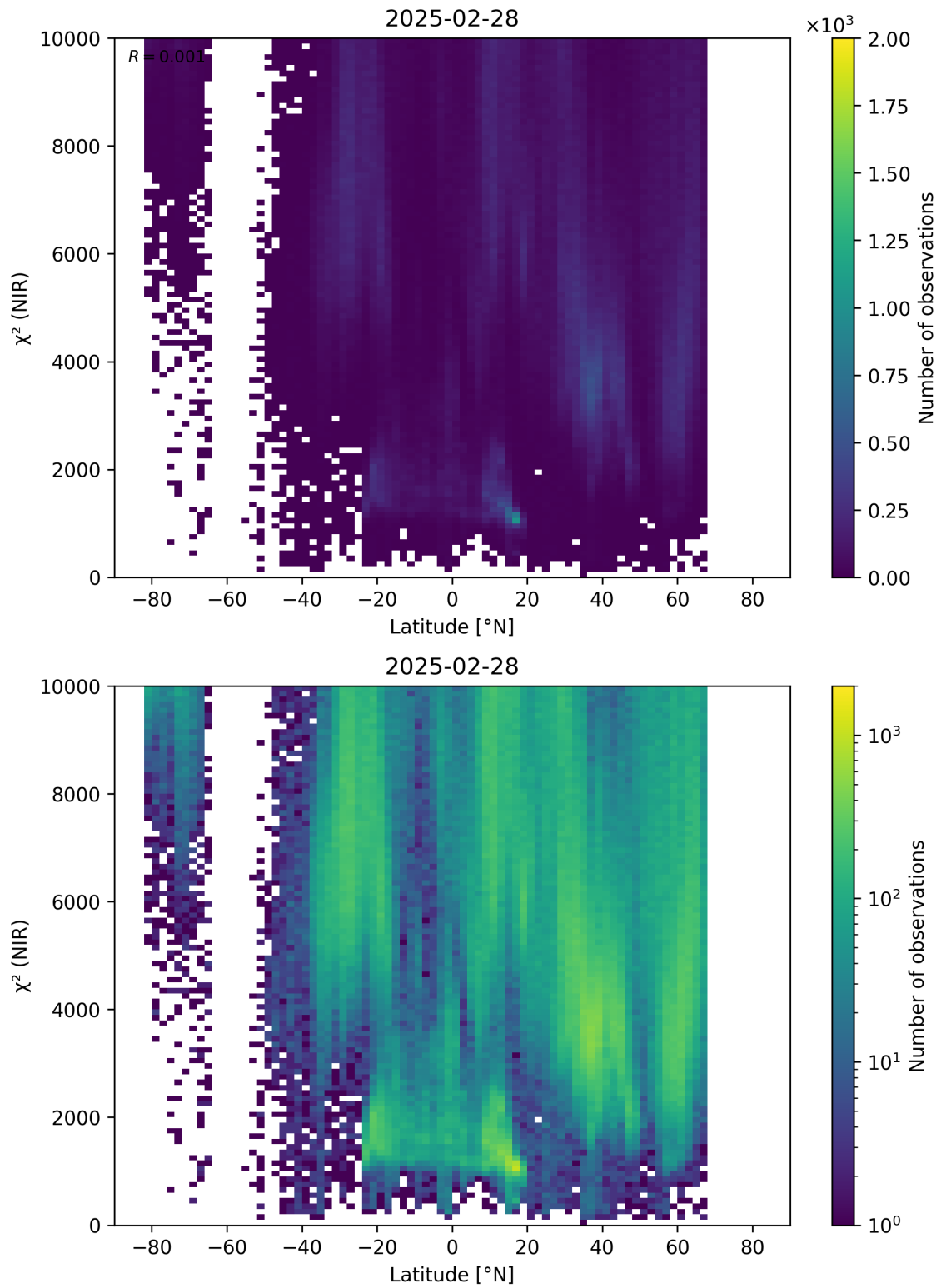
Figure 53: Scatter density plot of “Latitude” against “ \chi^2 (NIR)” for 2025-02-27 to 2025-03-01.
