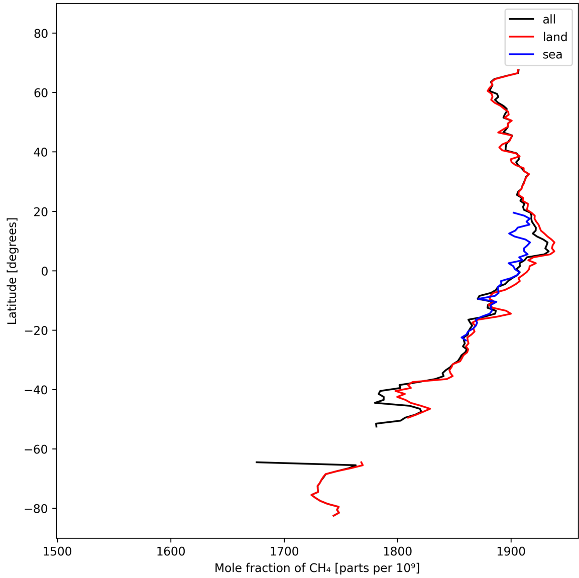
Figure 12: Zonal average of “Mole fraction of \text{CH}_4 ” for 2025-02-27 to 2025-03-01.
