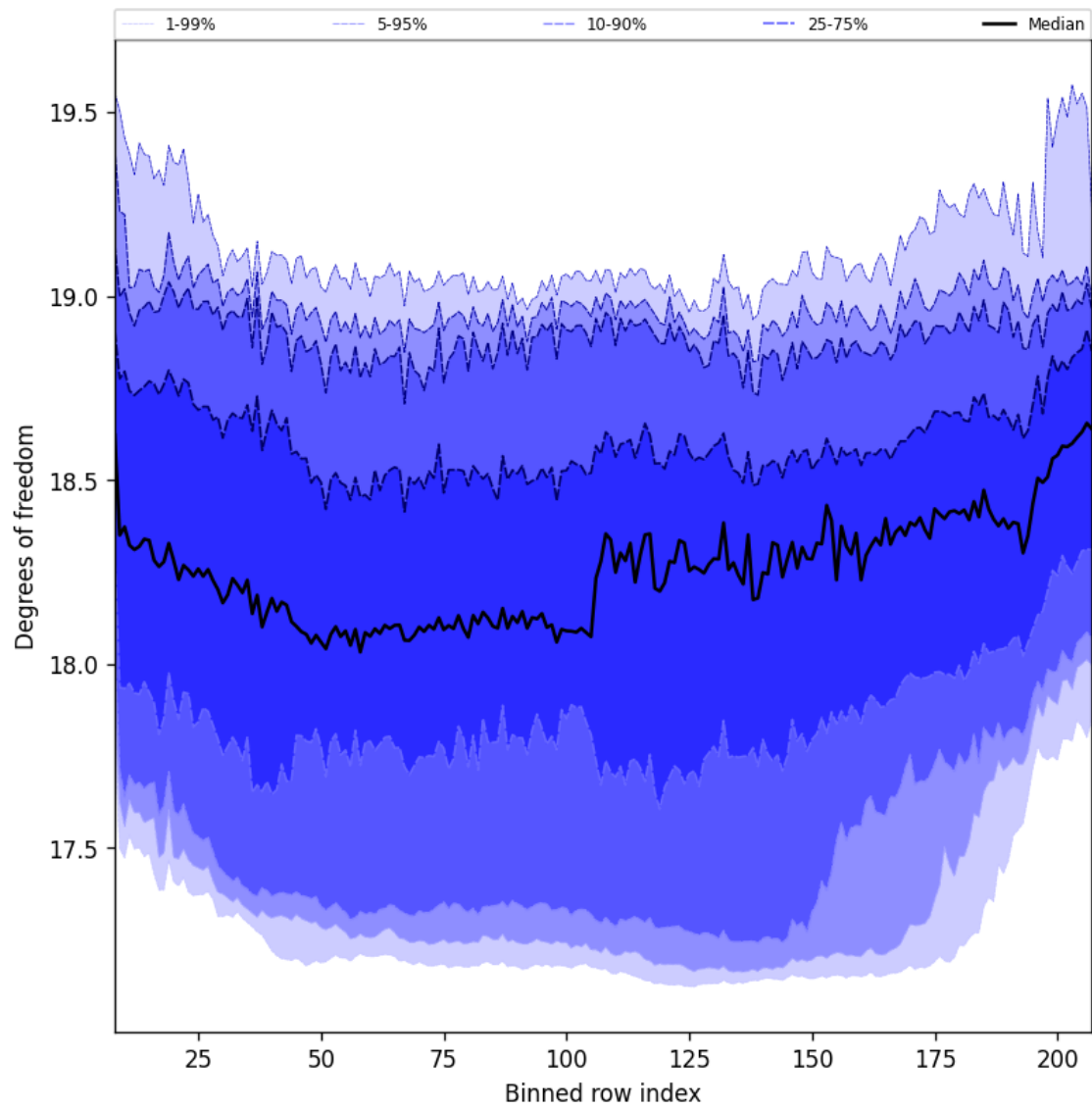
Figure 41: Along track statistics of “Degrees of freedom” for 2025-02-27 to 2025-03-01
