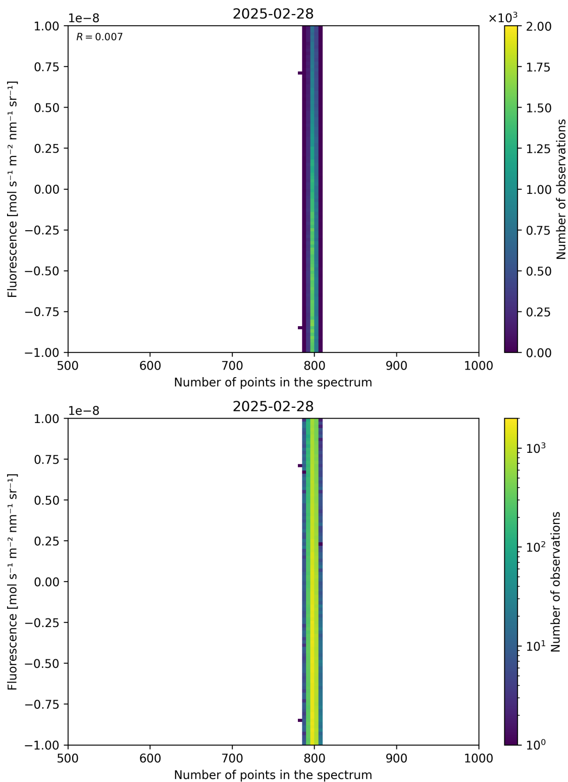
Figure 91: Scatter density plot of “Number of points in the spectrum” against “Fluorescence” for 2025-02-27 to 2025-03-01.
