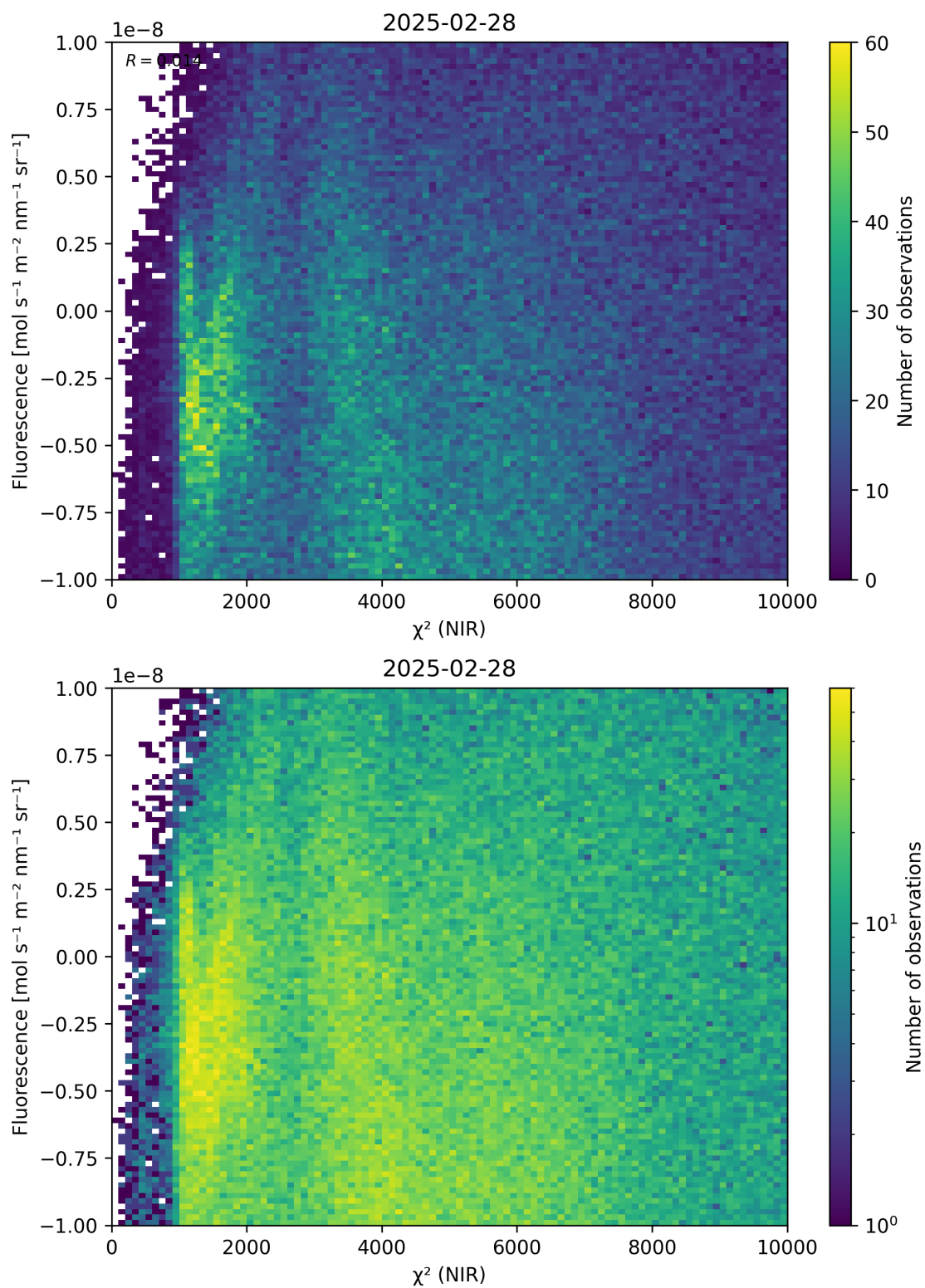
Figure 45: Scatter density plot of “ \chi^2 (NIR)” against “Fluorescence” for 2025-02-27 to 2025-03-01.
