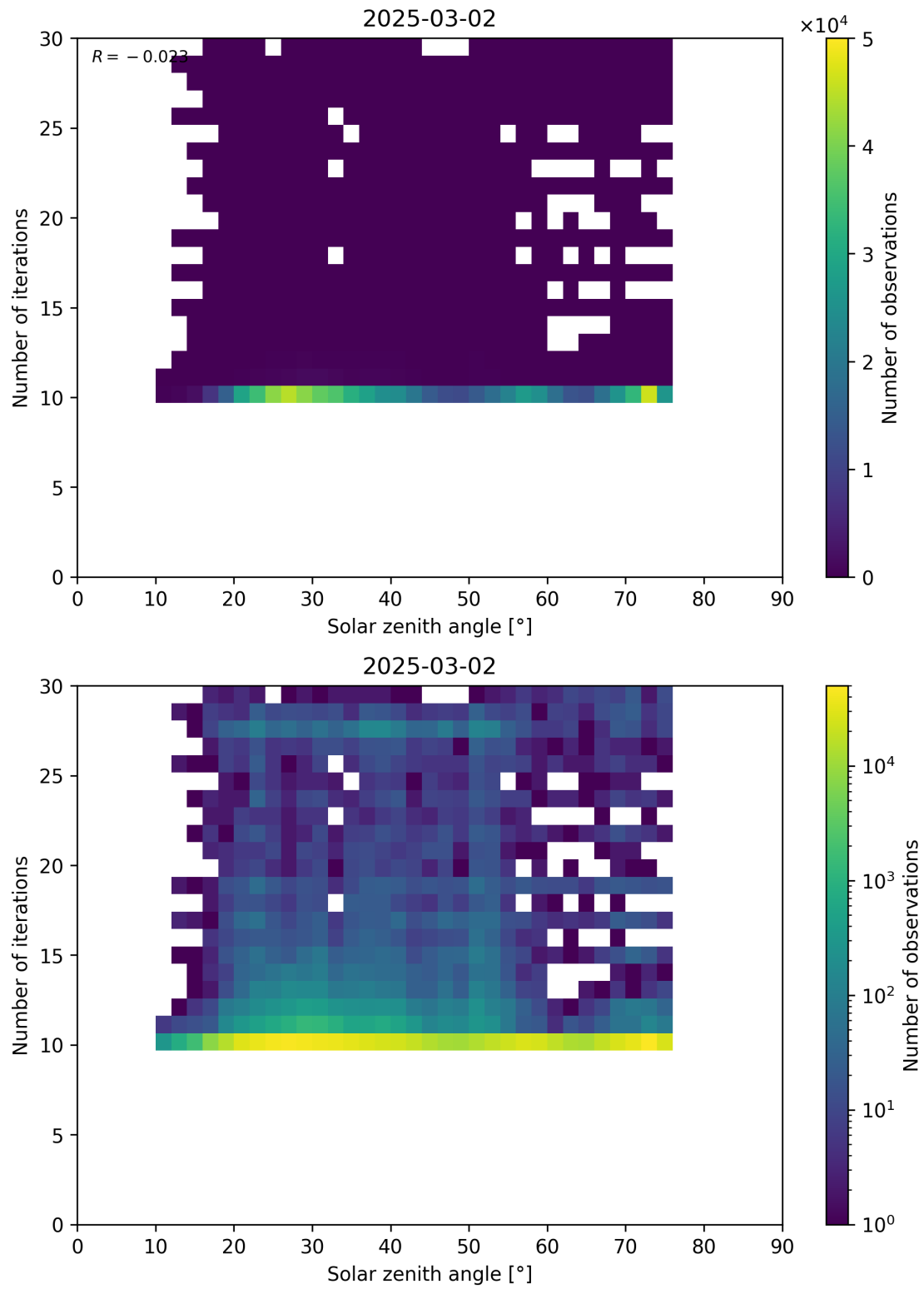
Figure 102: Scatter density plot of “Solar zenith angle” against “Number of iterations” for 2025-03-01 to 2025-03-03.
