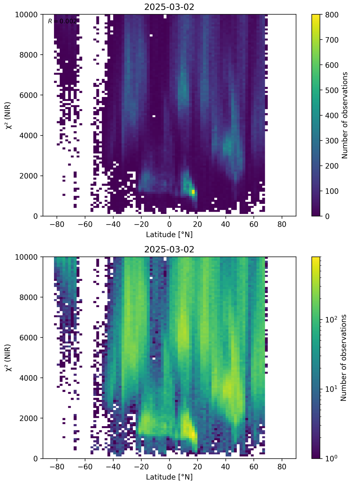
Figure 53: Scatter density plot of “Latitude” against “ \chi^2 (NIR)” for 2025-03-01 to 2025-03-03.
