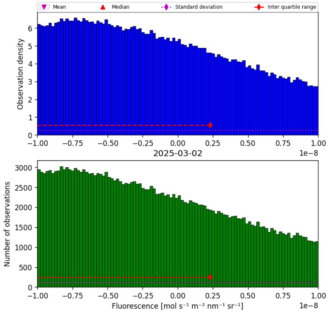
Figure 32: Histogram of “Fluorescence” for 2025-03-01 to 2025-03-03
