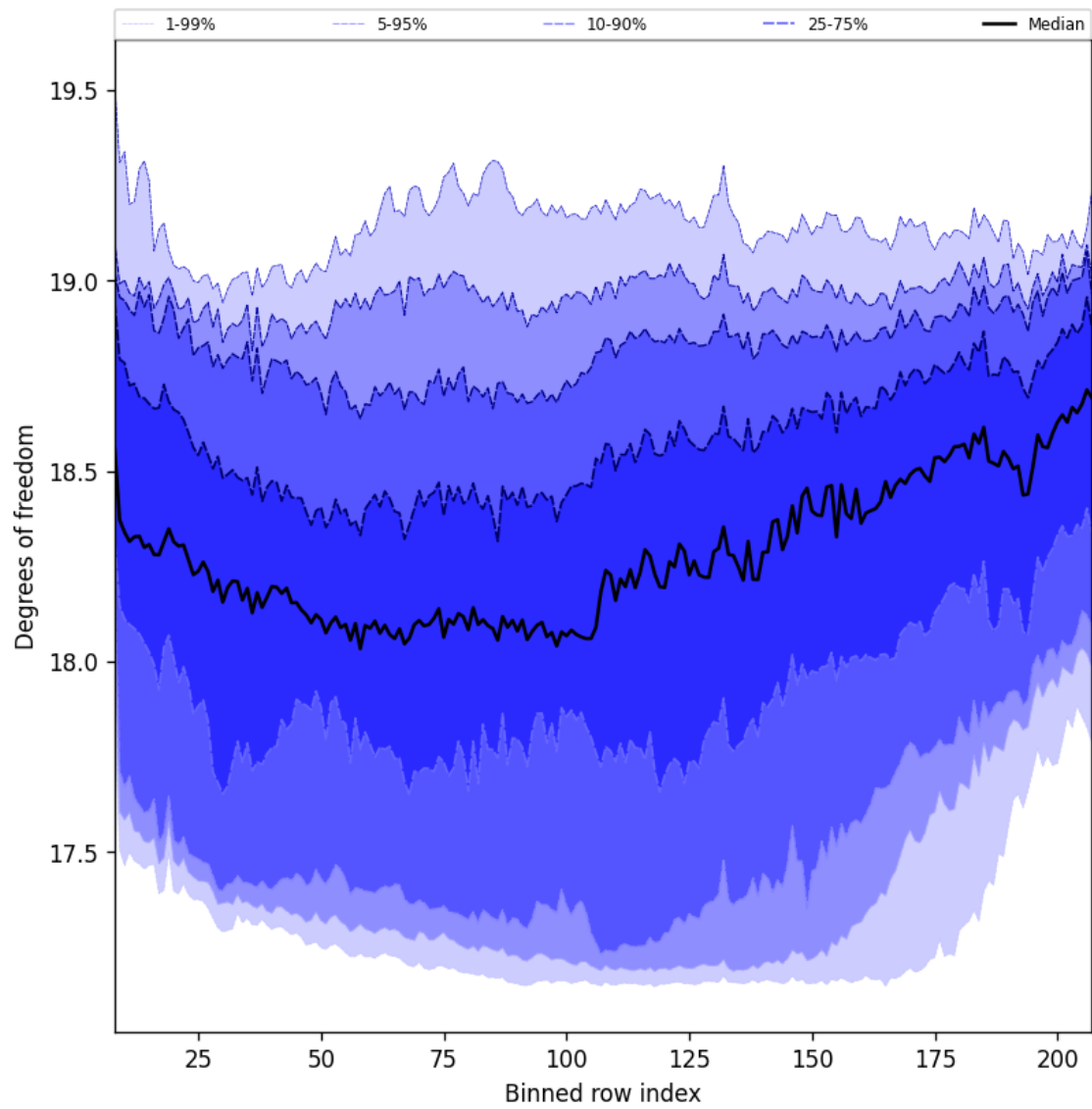
Figure 41: Along track statistics of “Degrees of freedom” for 2025-03-01 to 2025-03-03
