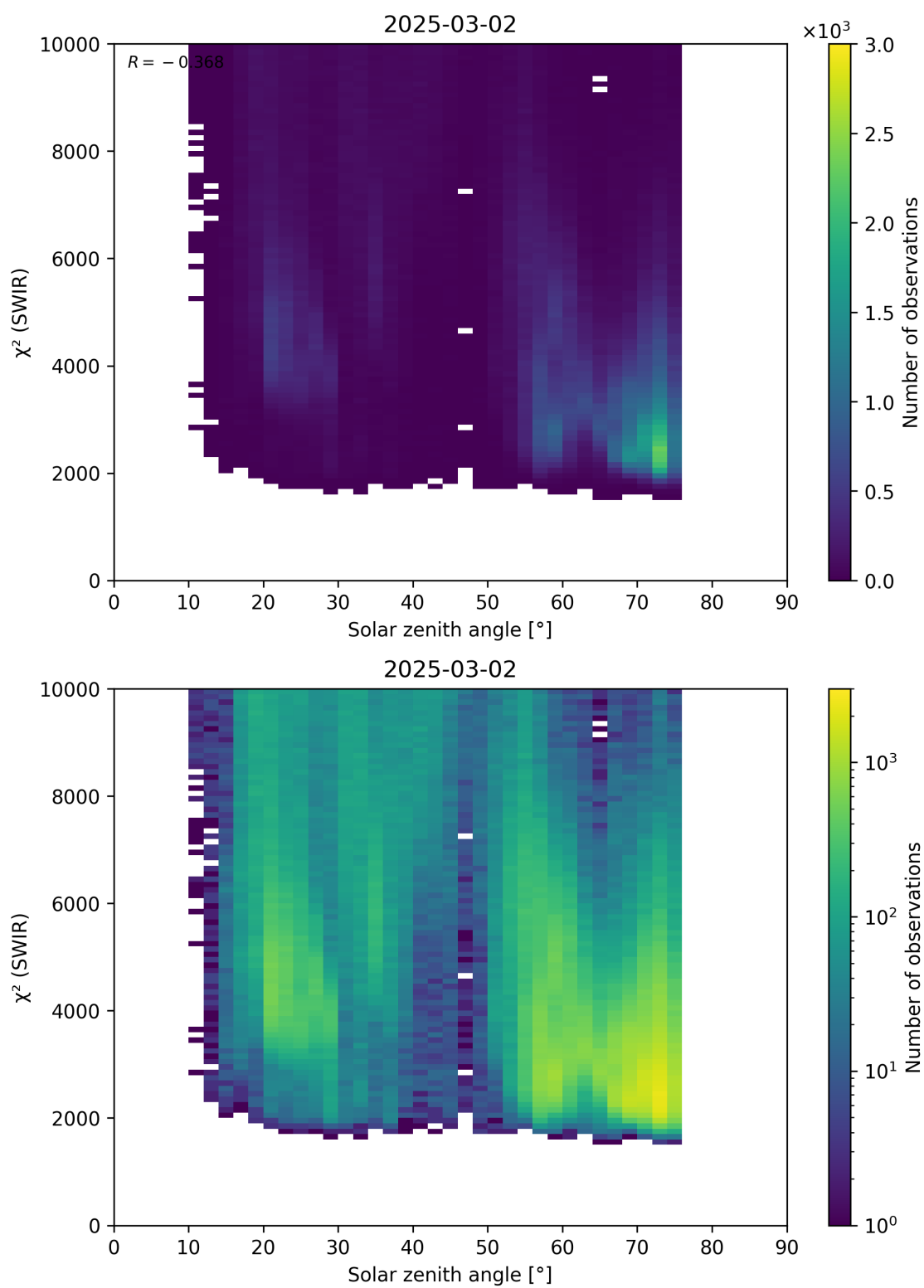
Figure 95: Scatter density plot of “Solar zenith angle” against “ \chi^2 (SWIR)” for 2025-03-01 to 2025-03-03.
