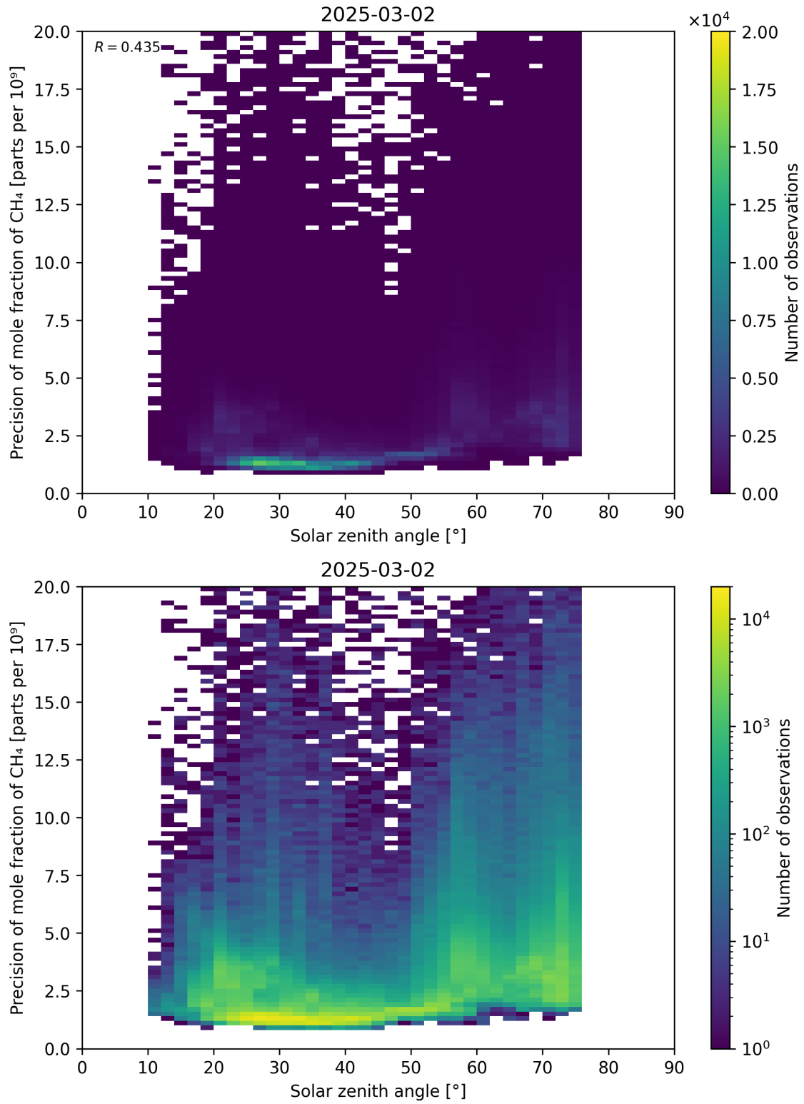
Figure 101: Scatter density plot of “Solar zenith angle” against “Precision of mole fraction of \text{CH}_4 ” for 2025-03-01 to 2025-03-03.
