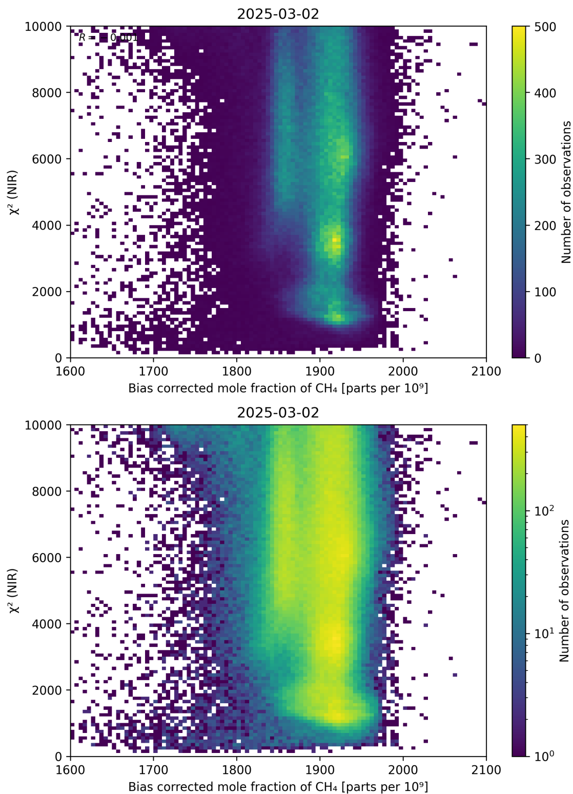
Figure 63: Scatter density plot of “Bias corrected mole fraction of CH 4 ” against “ \chi^2 (NIR)” for 2025-03-01 to 2025-03-03.
