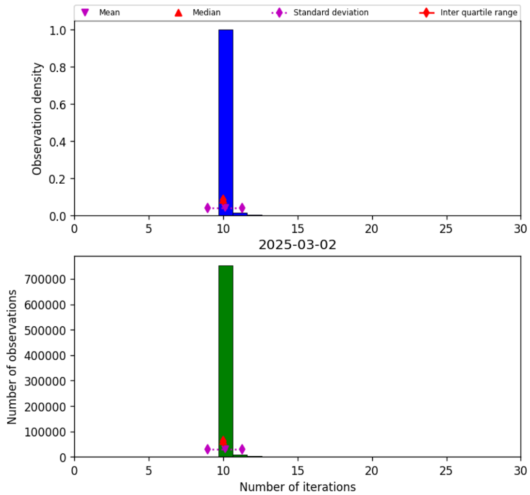
Figure 31: Histogram of “Number of iterations” for 2025-03-01 to 2025-03-03
