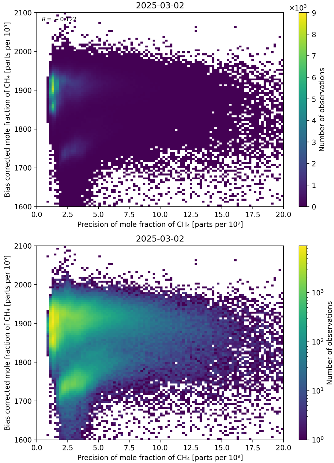
Figure 82: Scatter density plot of “Precision of mole fraction of CH 4 ” against “Bias corrected mole fraction of CH 4 ” for 2025-03-01 to 2025-03-03.
