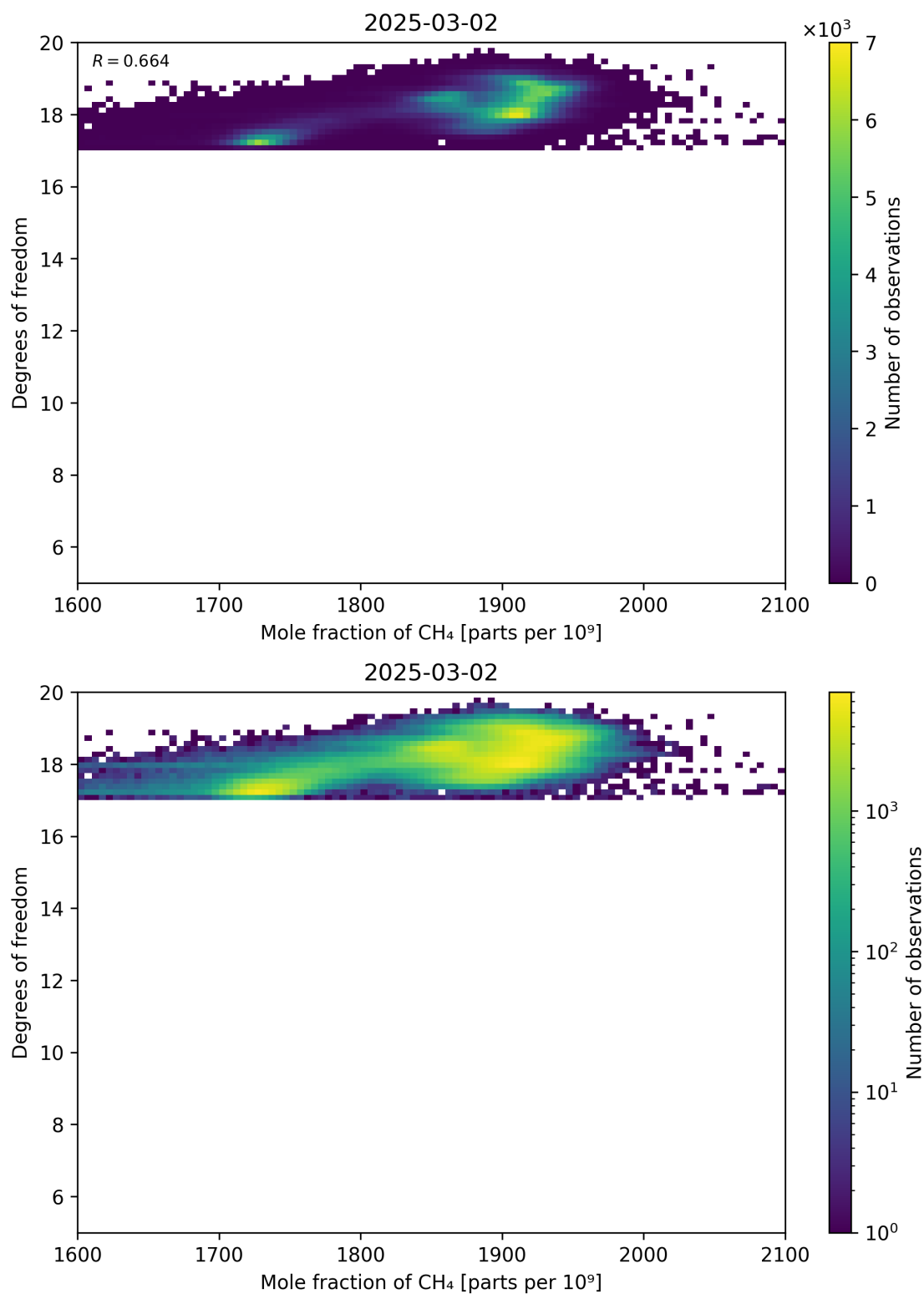
Figure 72: Scatter density plot of “Mole fraction of CH 4 ” against “Degrees of freedom” for 2025-03-01 to 2025-03-03.
