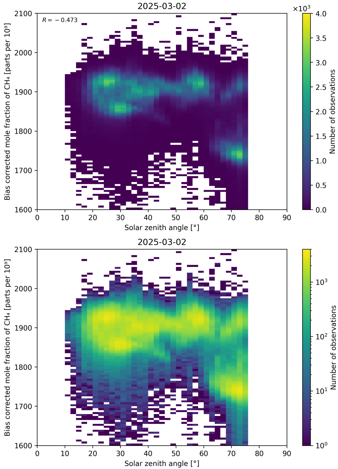
Figure 100: Scatter density plot of “Solar zenith angle” against “Bias corrected mole fraction of CH 4 ” for 2025-03-01 to 2025-03-03.
