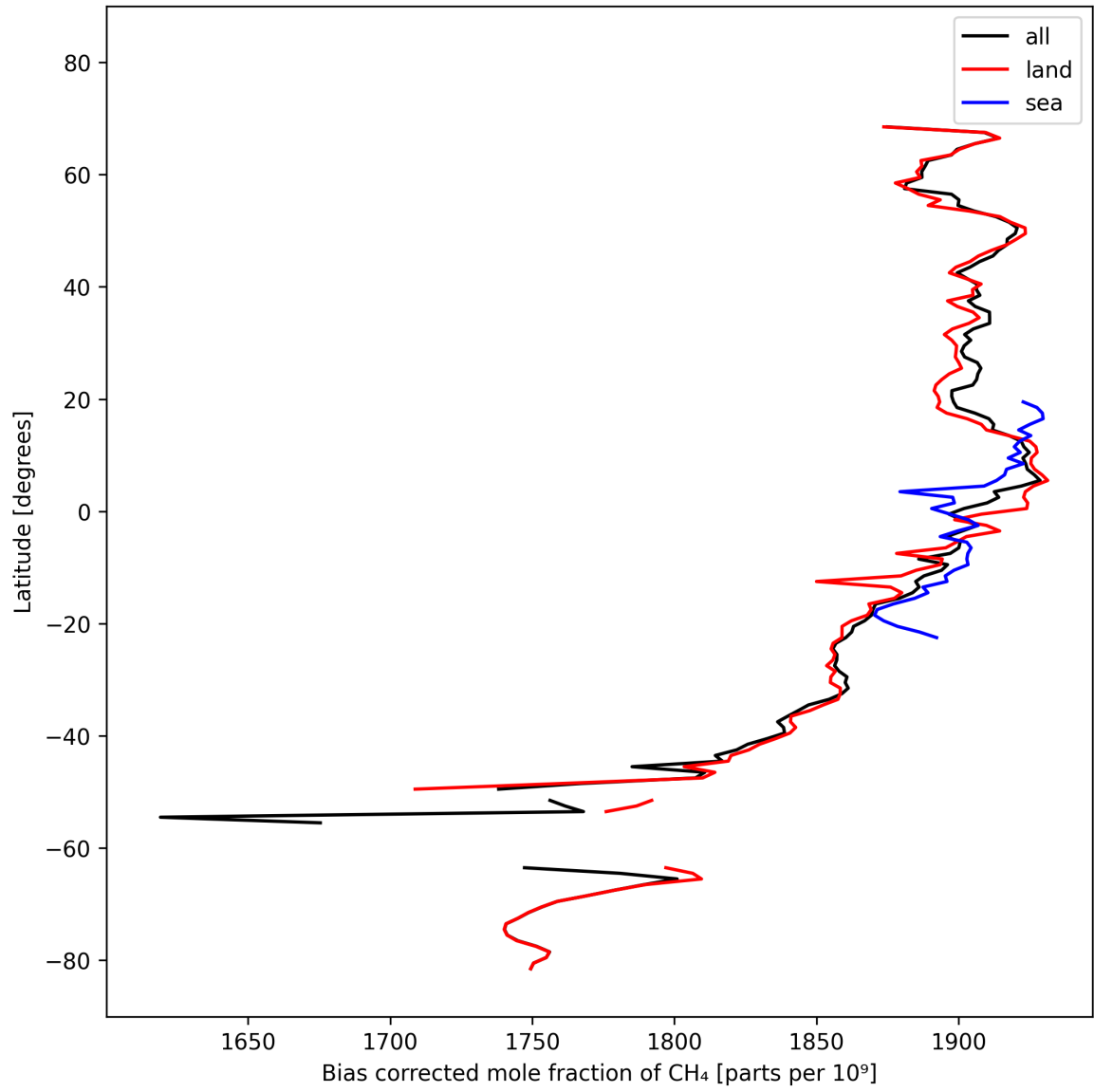
Figure 14: Zonal average of “Bias corrected mole fraction of CH 4 ” for 2025-03-01 to 2025-03-03.
