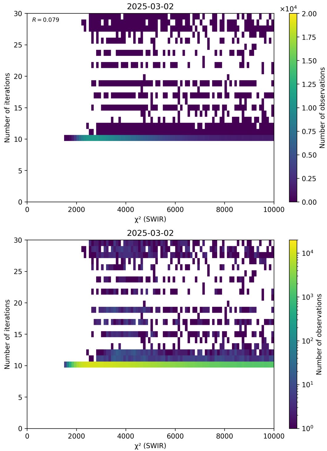
Figure 50: Scatter density plot of “ \chi^2 (SWIR)” against “Number of iterations” for 2025-03-01 to 2025-03-03.
