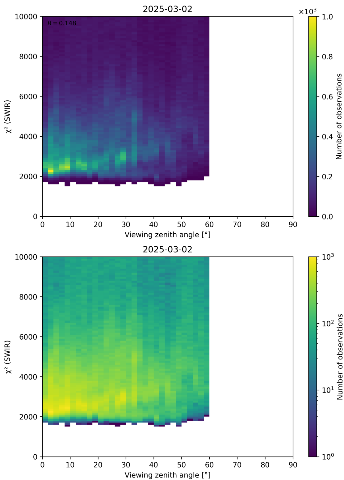
Figure 106: Scatter density plot of “Viewing zenith angle” against “ \chi^2 (SWIR)” for 2025-03-01 to 2025-03-03.
