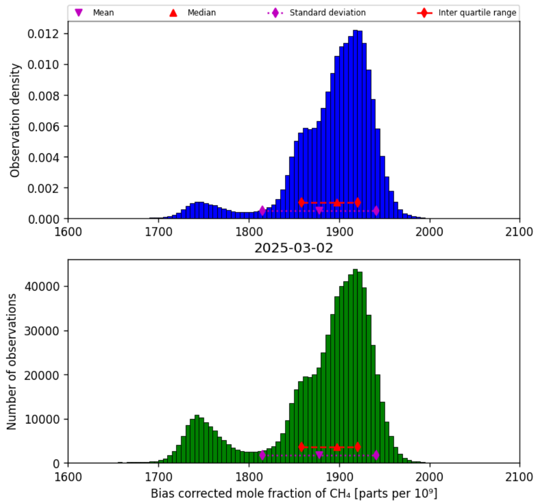
Figure 25: Histogram of “Bias corrected mole fraction of CH 4 ” for 2025-03-01 to 2025-03-03
