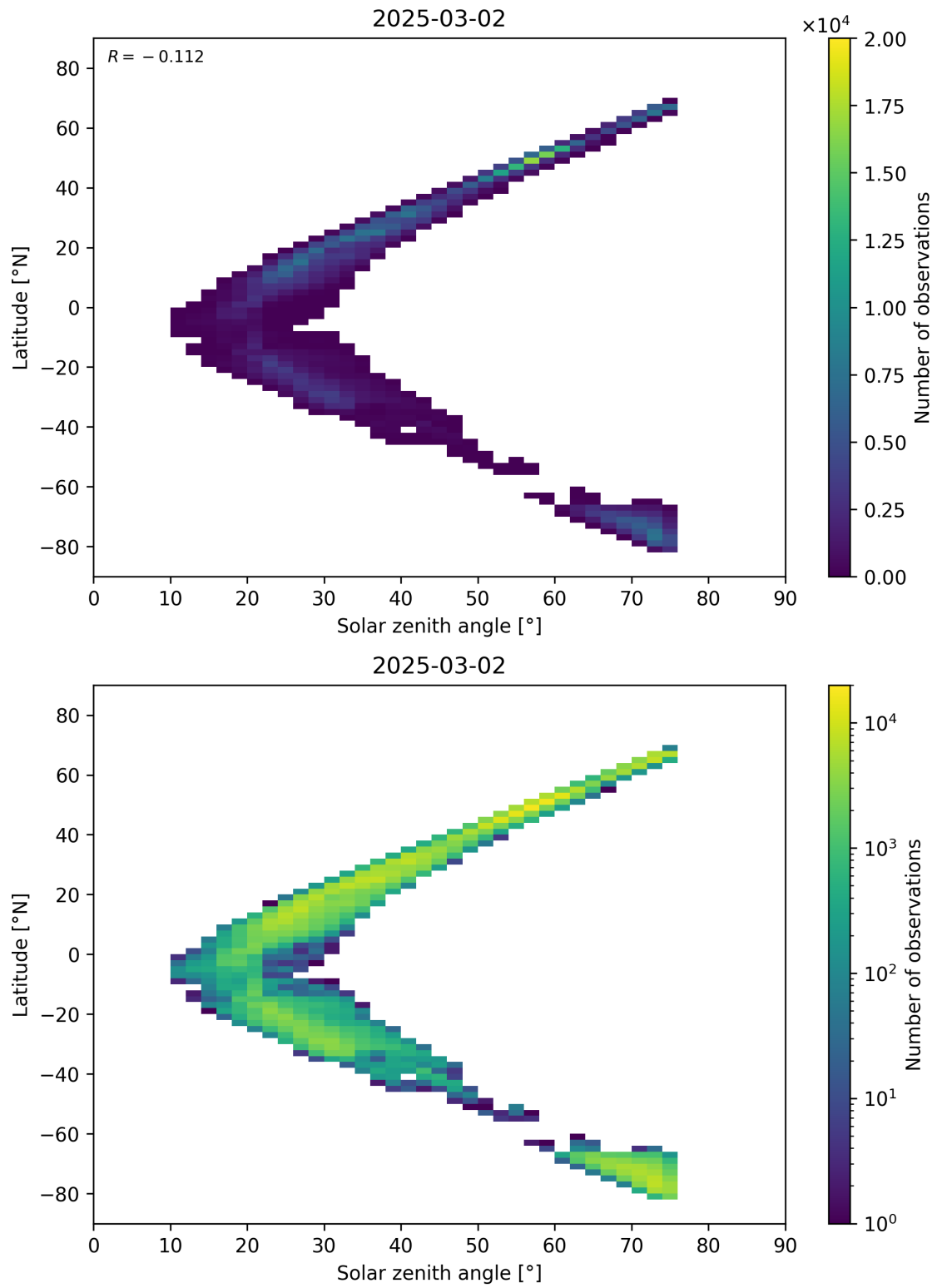
Figure 98: Scatter density plot of “Solar zenith angle” against “Latitude” for 2025-03-01 to 2025-03-03.
