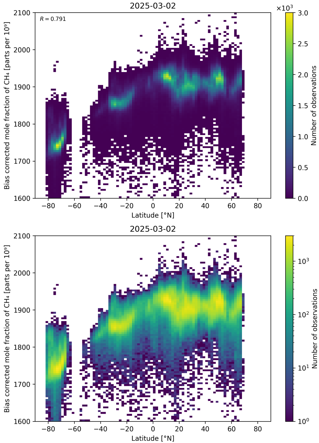
Figure 58: Scatter density plot of “Latitude” against “Bias corrected mole fraction of CH 4 ” for 2025-03-01 to 2025-03-03.
