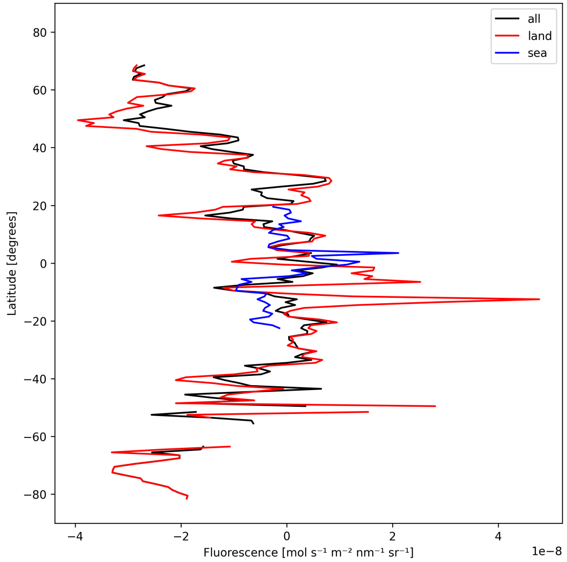
Figure 21: Zonal average of “Fluorescence” for 2025-03-01 to 2025-03-03.
