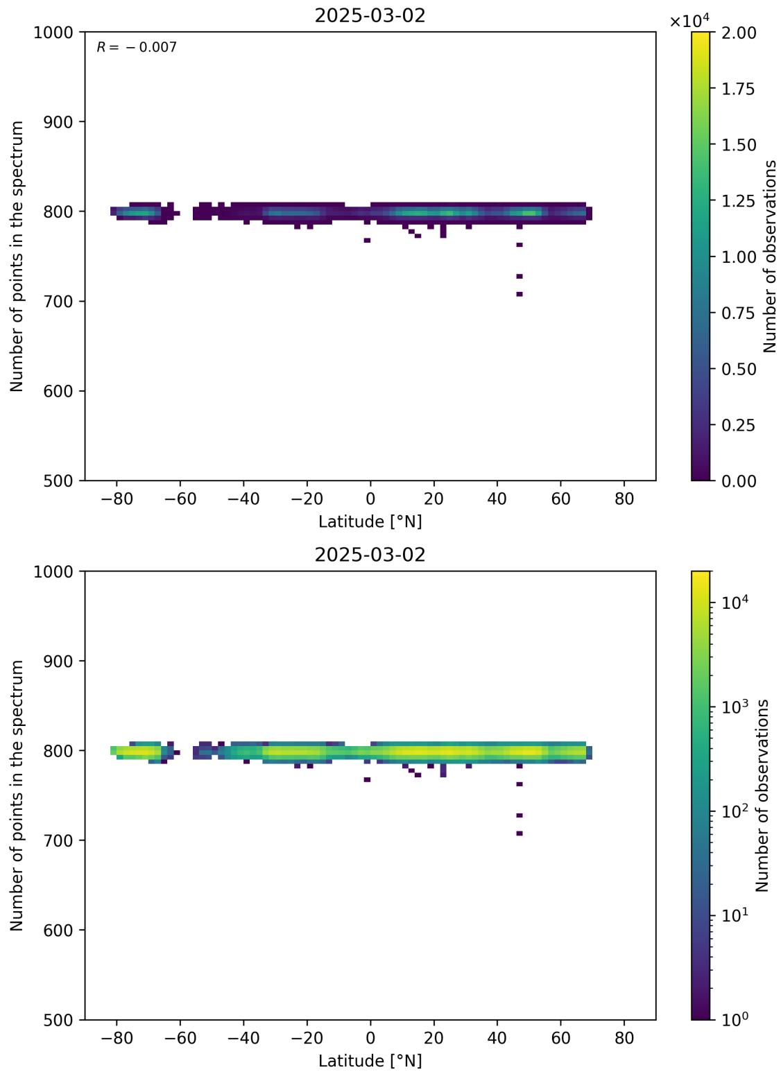
Figure 61: Scatter density plot of “Latitude” against “Number of points in the spectrum” for 2025-03-01 to 2025-03-03.
