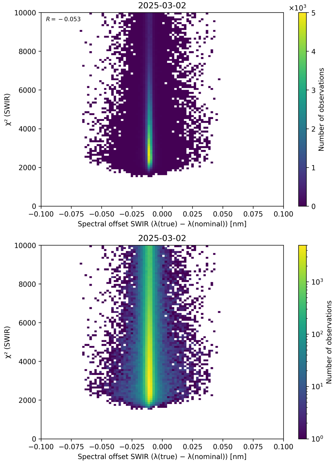
Figure 118: Scatter density plot of “Spectral offset SWIR ( \lambda_{\text{true}} - \lambda_{\text{nominal}} )” against “ \chi^2 (SWIR)” for 2025-03-01 to 2025-03-03.
