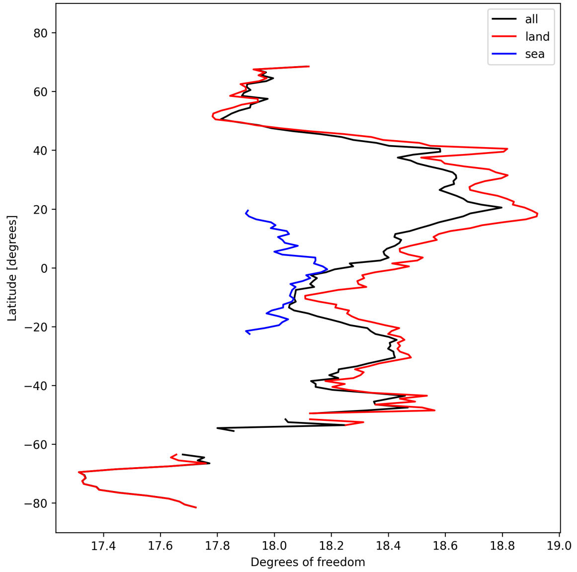
Figure 19: Zonal average of “Degrees of freedom” for 2025-03-01 to 2025-03-03.
