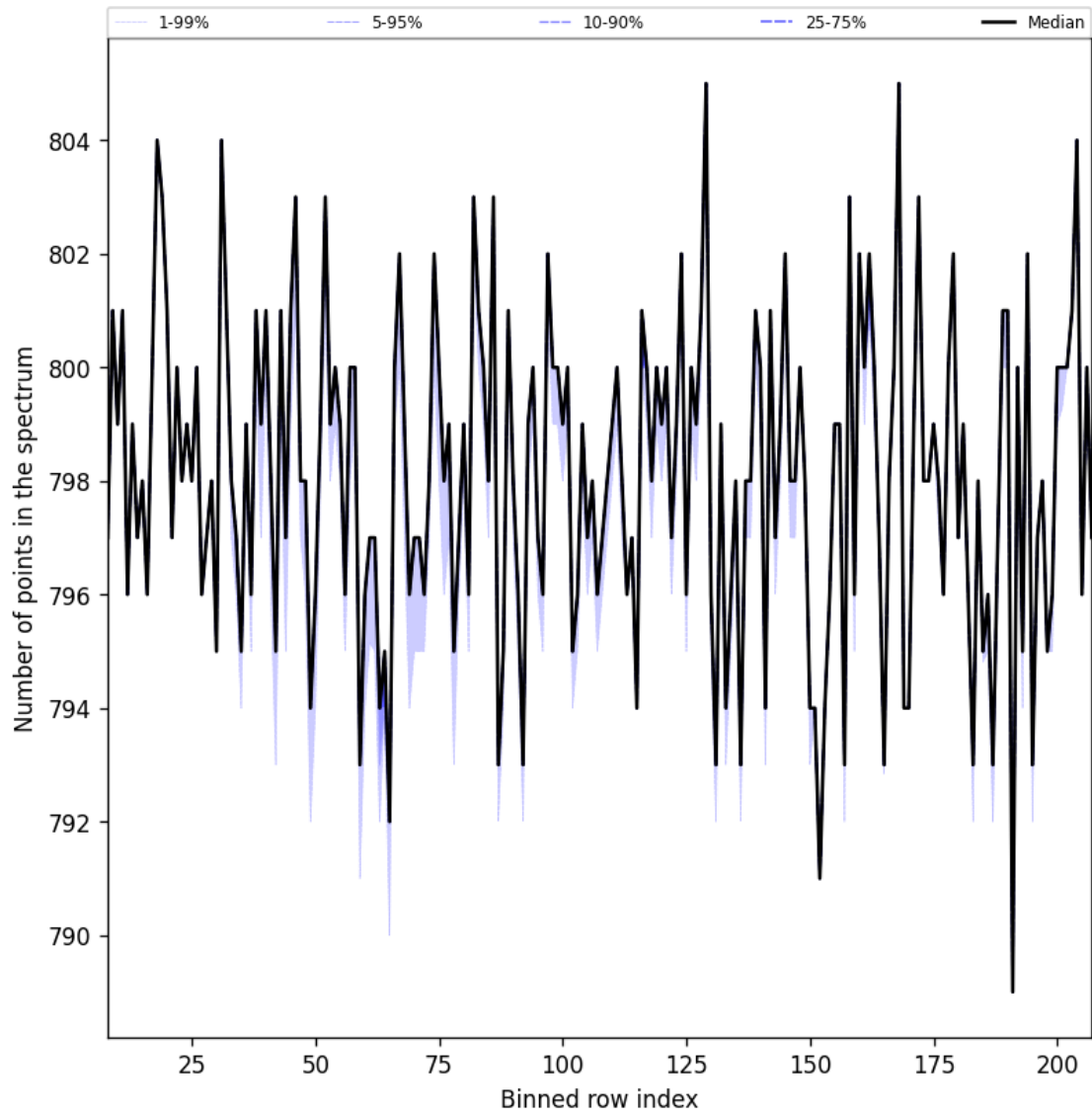
Figure 37: Along track statistics of “Number of points in the spectrum” for 2025-03-01 to 2025-03-03
