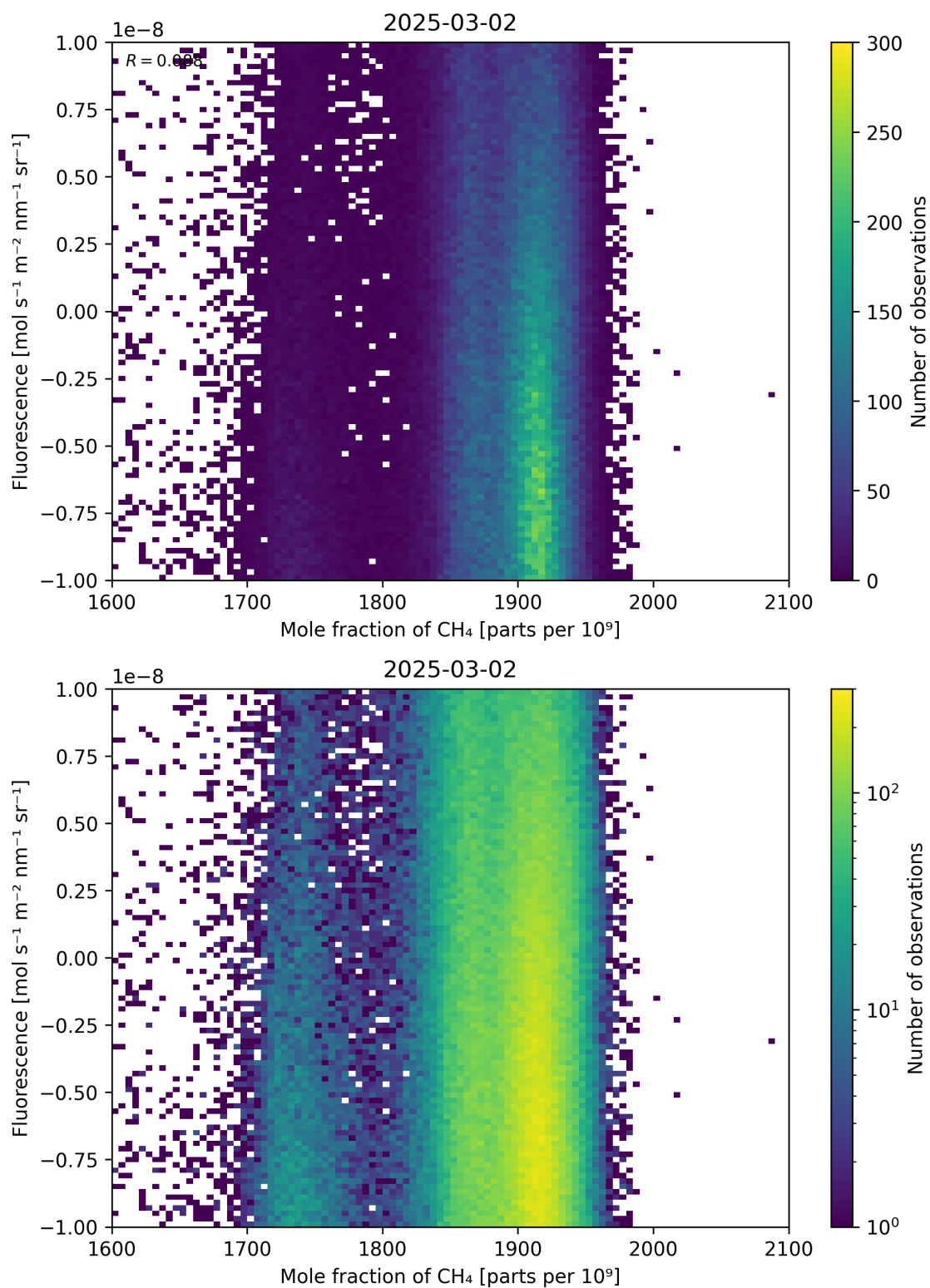
Figure 73: Scatter density plot of “Mole fraction of \text{CH}_4 ” against “Fluorescence” for 2025-03-01 to 2025-03-03.
