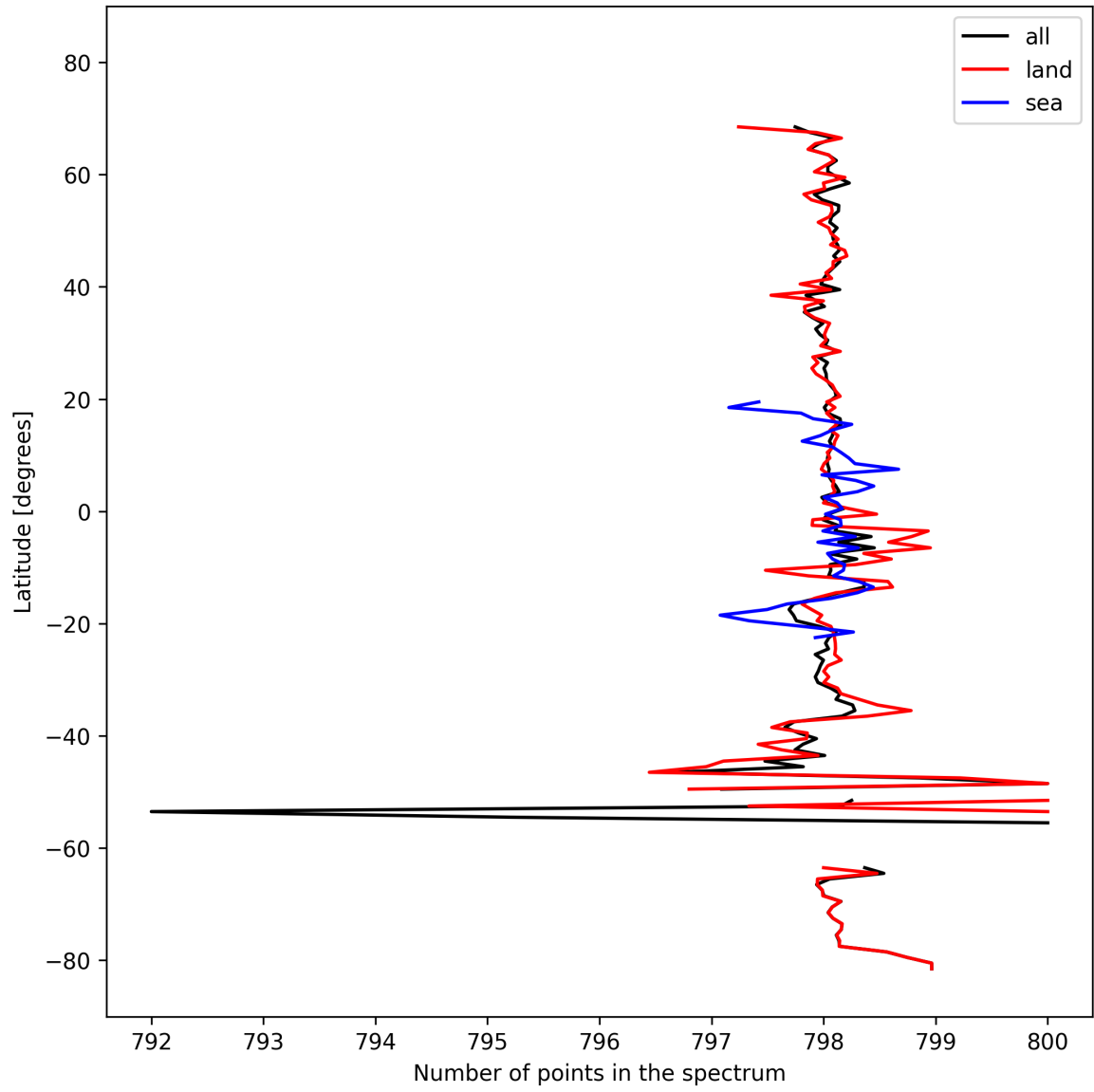
Figure 15: Zonal average of “Number of points in the spectrum” for 2025-03-01 to 2025-03-03.
