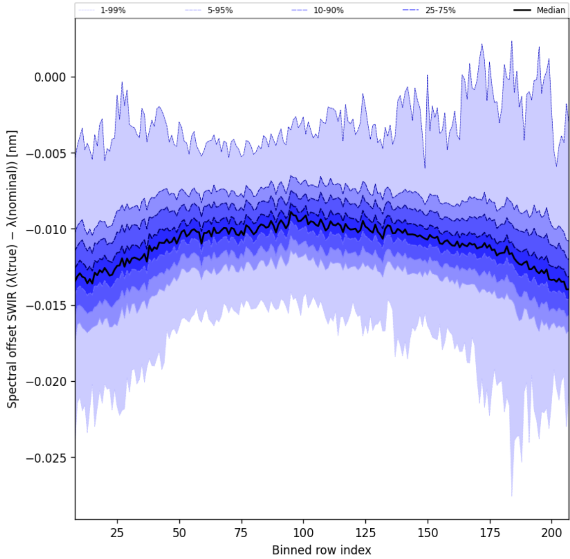
Figure 38: Along track statistics of “Spectral offset SWIR ( \lambda_{\text{true}} - \lambda_{\text{nominal}} )” for 2025-03-01 to 2025-03-03
