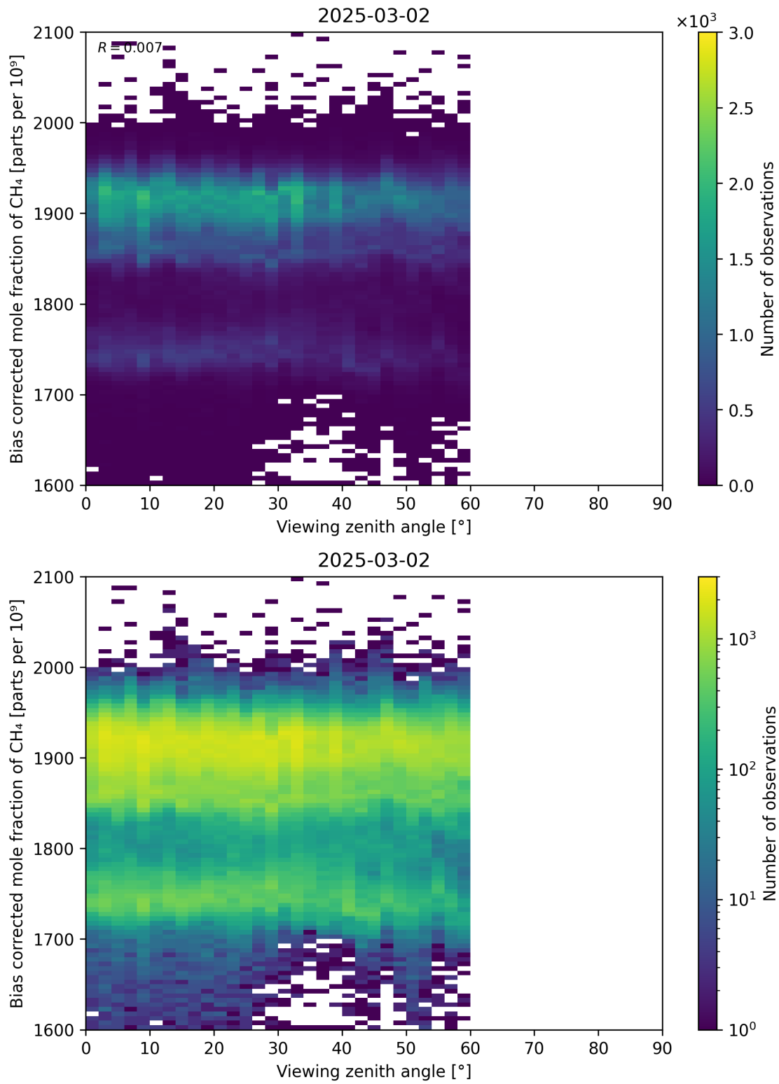
Figure 111: Scatter density plot of “Viewing zenith angle” against “Bias corrected mole fraction of CH 4 ” for 2025-03-01 to 2025-03-03.
