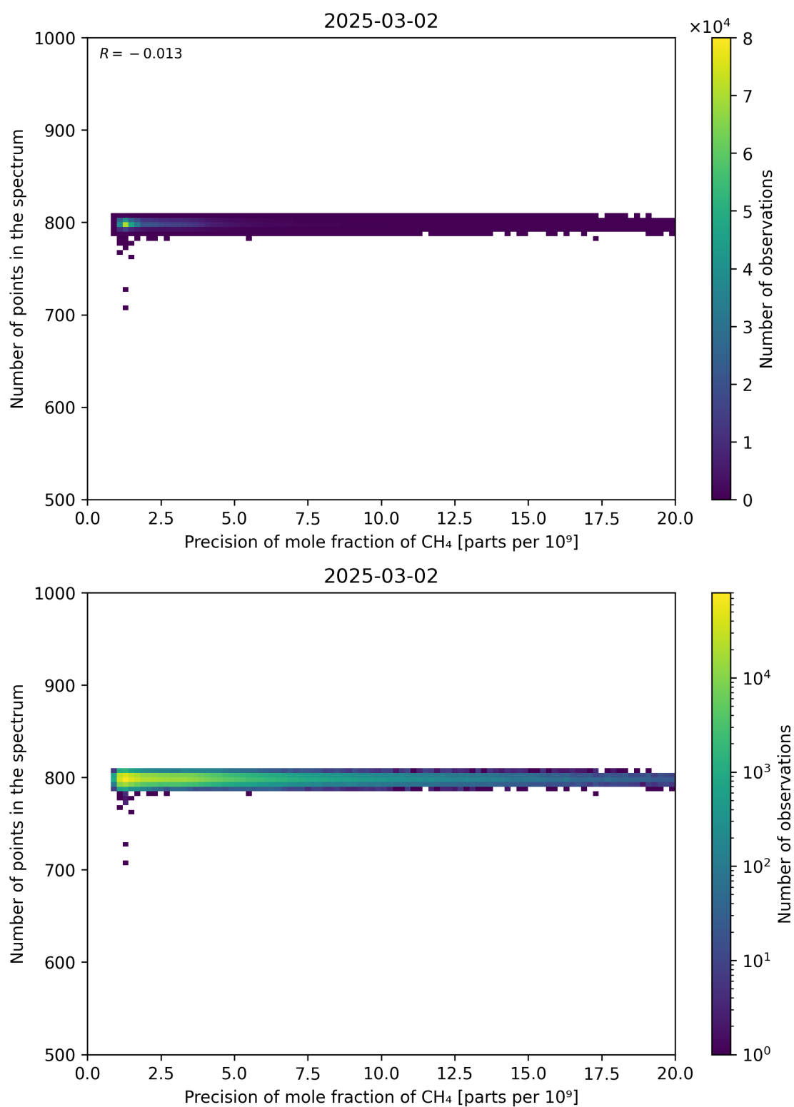
Figure 84: Scatter density plot of “Precision of mole fraction of CH 4 ” against “Number of points in the spectrum” for 2025-03-01 to 2025-03-03.
