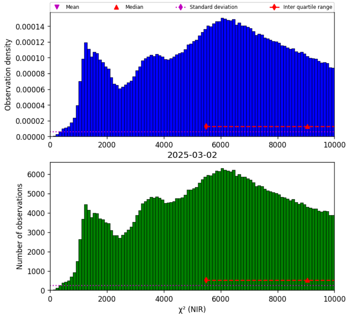
Figure 29: Histogram of " \chi^2 (NIR)" for 2025-03-01 to 2025-03-03
