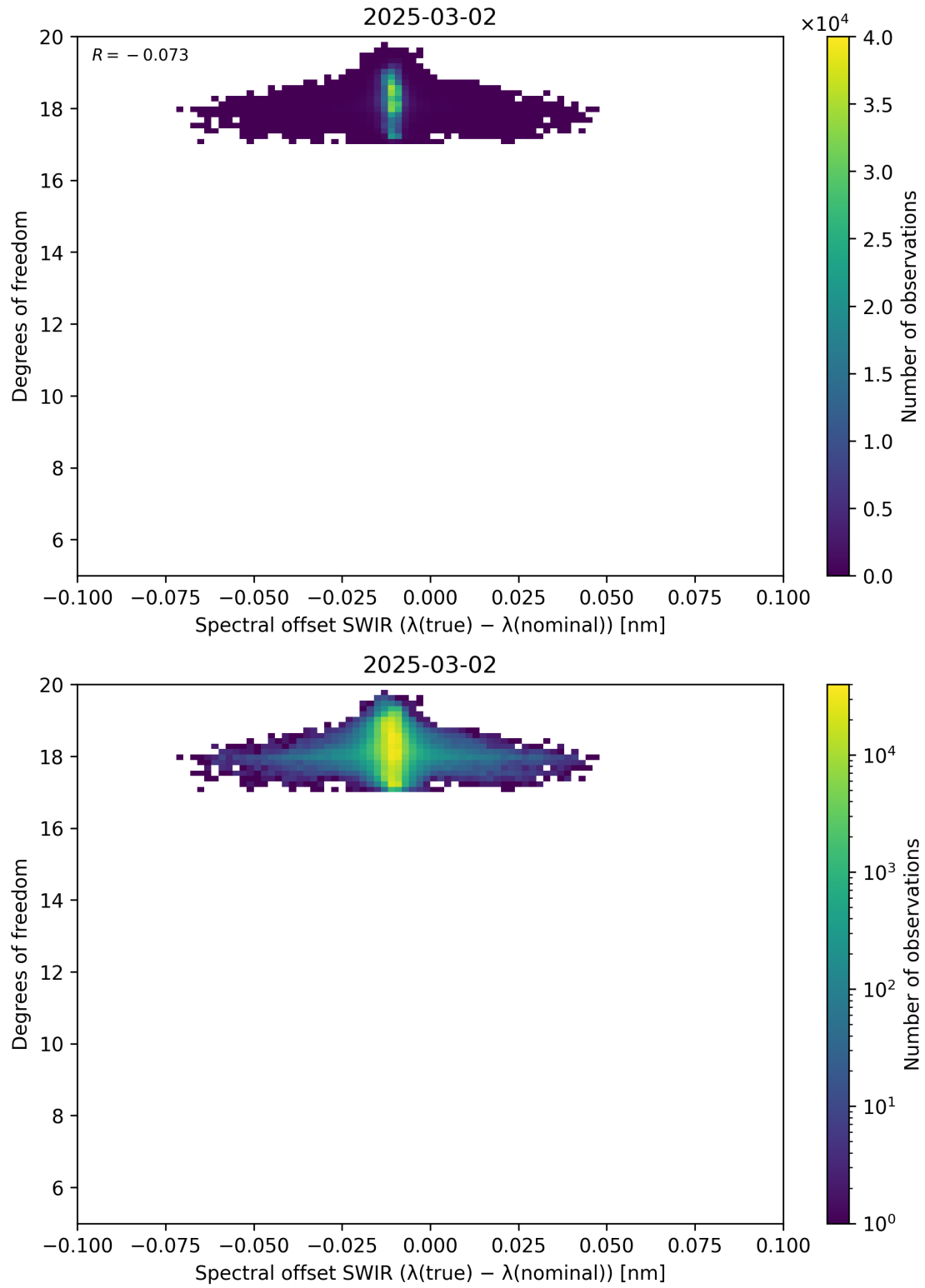
Figure 119: Scatter density plot of “Spectral offset SWIR ( \lambda_{\text{true}} - \lambda_{\text{nominal}} )” against “Degrees of freedom” for 2025-03-01 to 2025-03-03.
