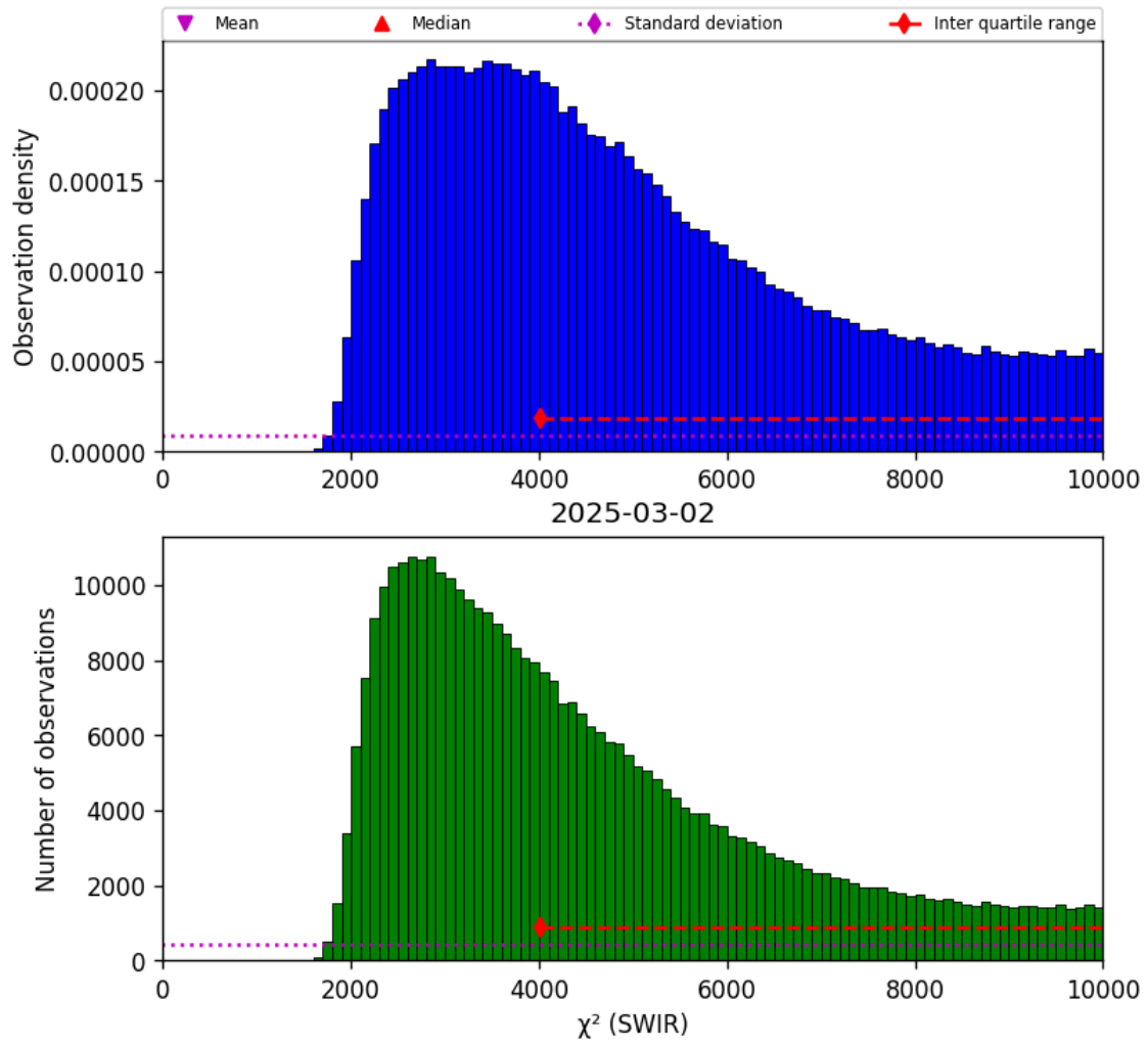
Figure 28: Histogram of “ \chi^2 (SWIR)” for 2025-03-01 to 2025-03-03
