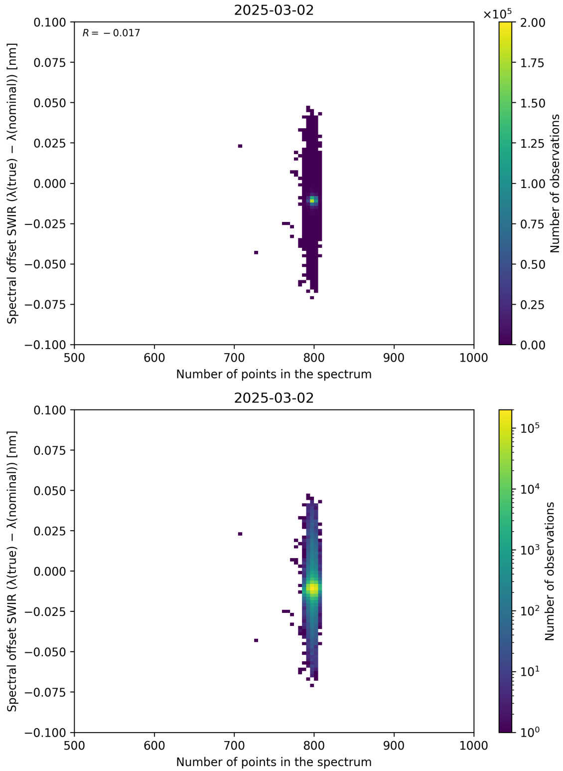
Figure 93: Scatter density plot of “Number of points in the spectrum” against “Spectral offset SWIR ( \lambda_{\text{true}} - \lambda_{\text{nominal}} )” for 2025-03-01 to 2025-03-03.
