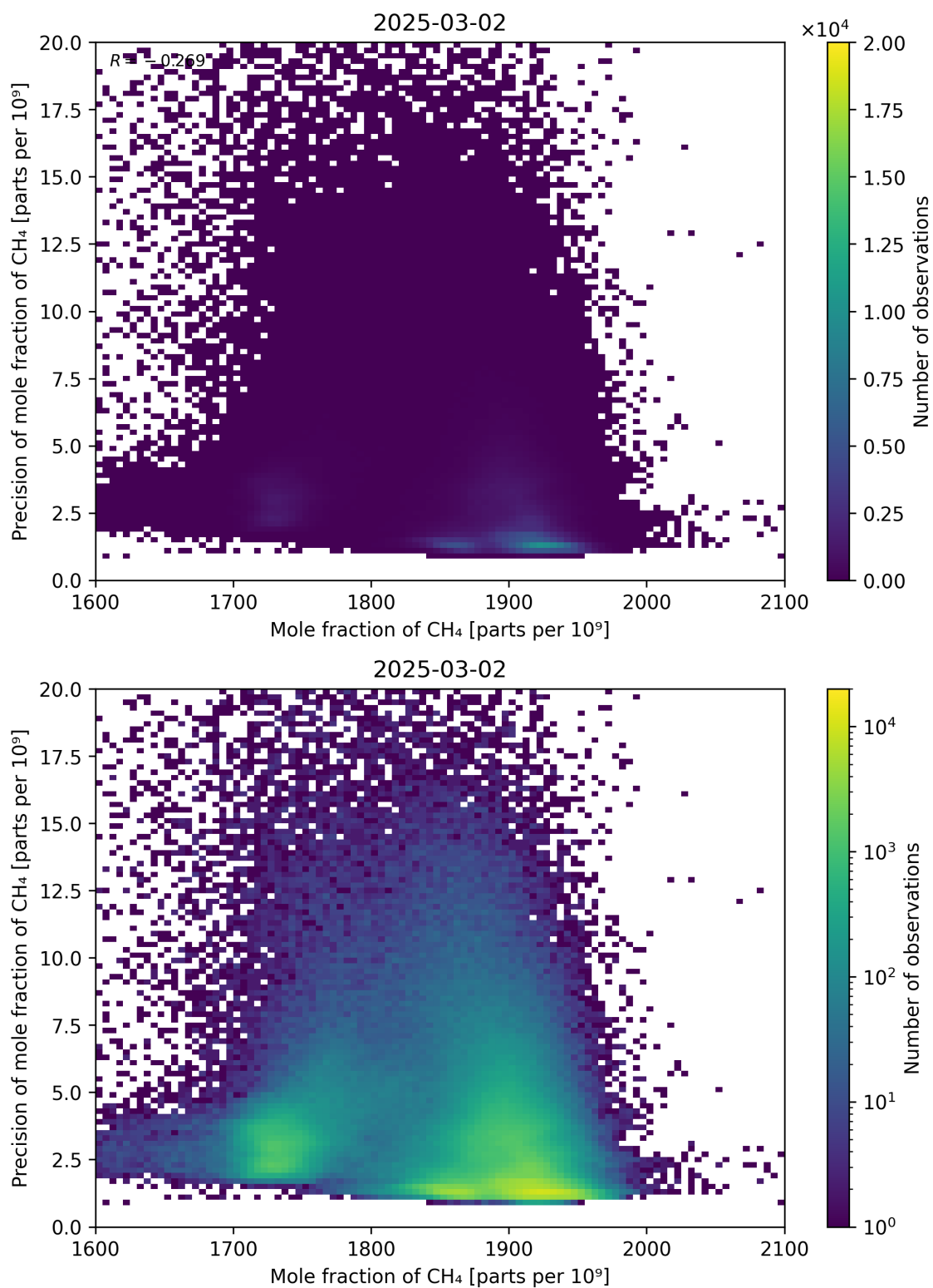
Figure 75: Scatter density plot of “Mole fraction of CH 4 ” against “Precision of mole fraction of CH 4 ” for 2025-03-01 to 2025-03-03.
