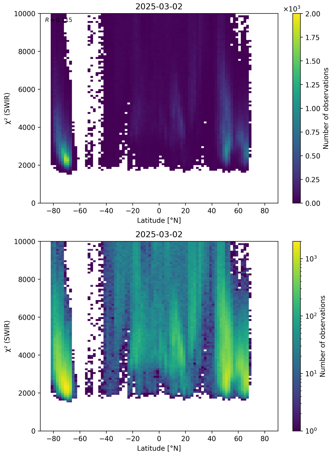
Figure 54: Scatter density plot of “Latitude” against “ \chi^2 (SWIR)” for 2025-03-01 to 2025-03-03.
