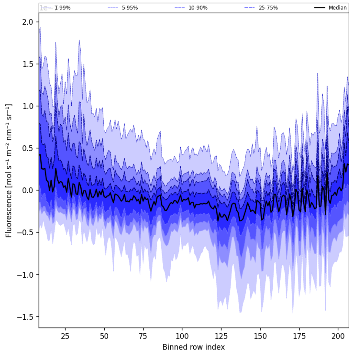
Figure 43: Along track statistics of “Fluorescence” for 2025-03-01 to 2025-03-03
