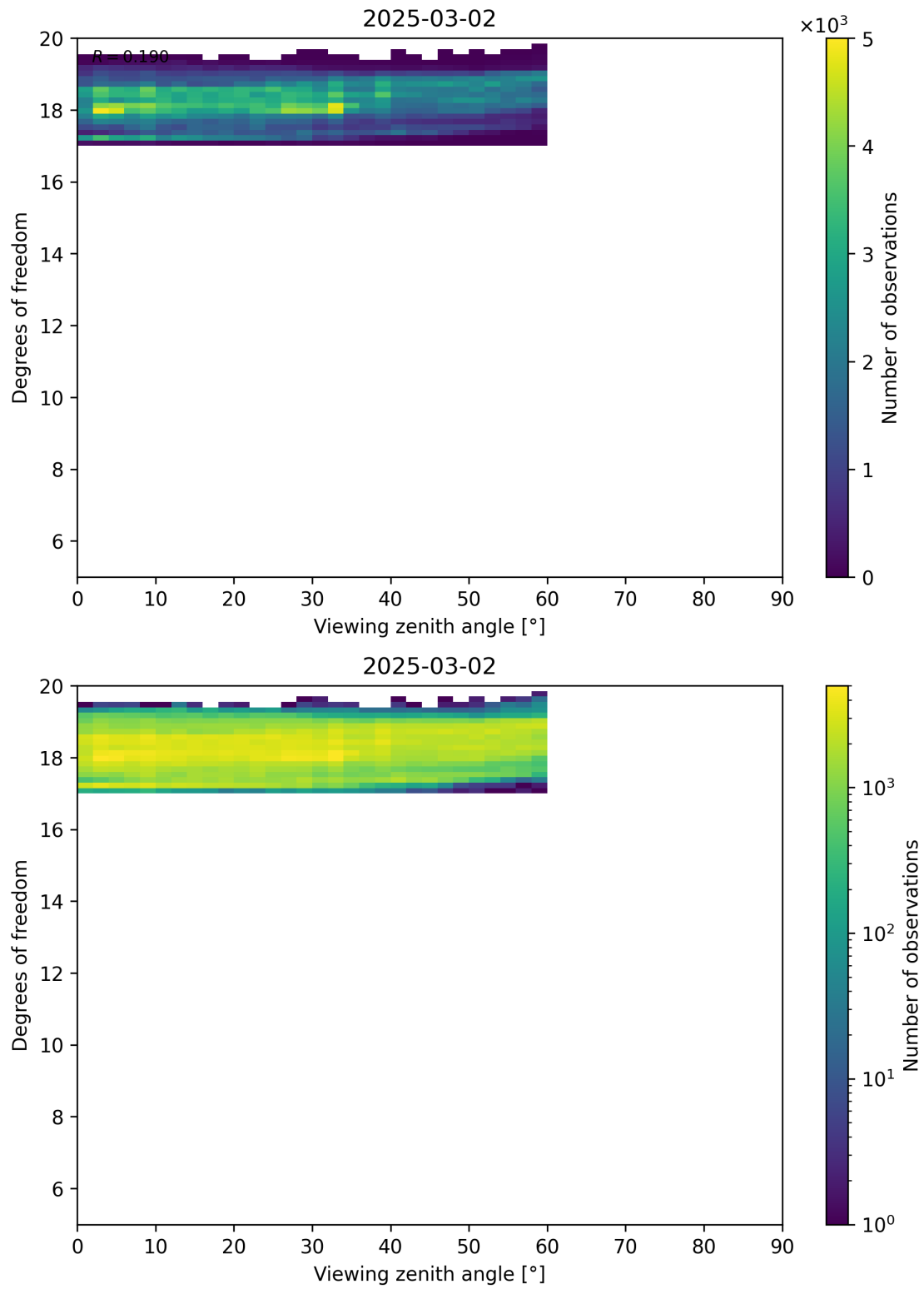
Figure 107: Scatter density plot of “Viewing zenith angle” against “Degrees of freedom” for 2025-03-01 to 2025-03-03.
