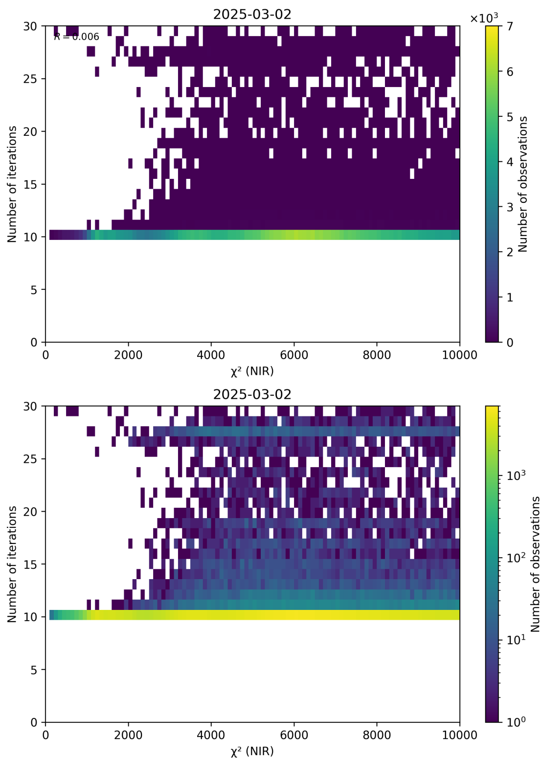
Figure 46: Scatter density plot of “ \chi^2 (NIR)” against “Number of iterations” for 2025-03-01 to 2025-03-03.
