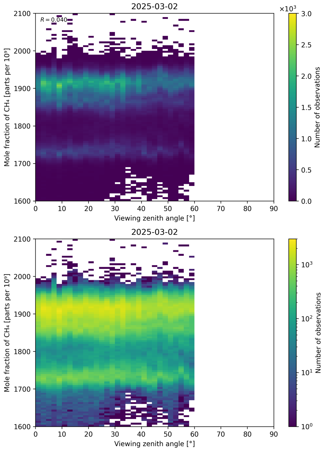
Figure 110: Scatter density plot of “Viewing zenith angle” against “Mole fraction of CH 4 ” for 2025-03-01 to 2025-03-03.
