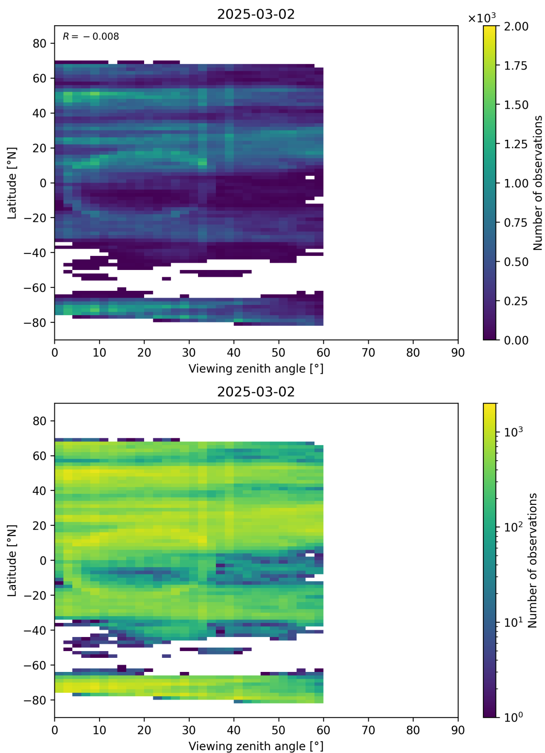
Figure 109: Scatter density plot of “Viewing zenith angle” against “Latitude” for 2025-03-01 to 2025-03-03.
