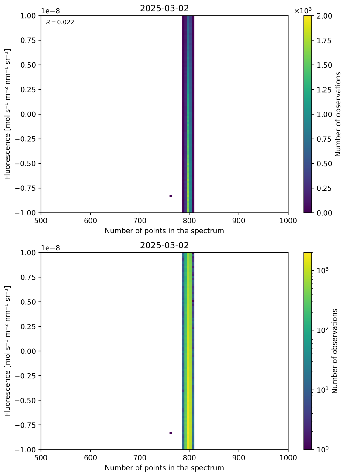
Figure 91: Scatter density plot of “Number of points in the spectrum” against “Fluorescence” for 2025-03-01 to 2025-03-03.
