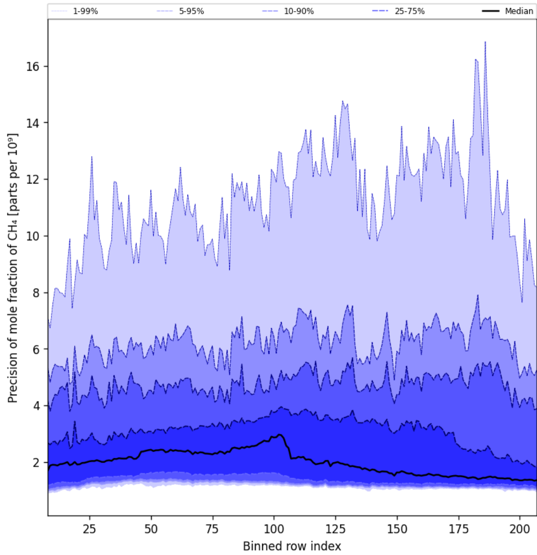
Figure 35: Along track statistics of “Precision of mole fraction of CH 4 ” for 2025-03-01 to 2025-03-03
