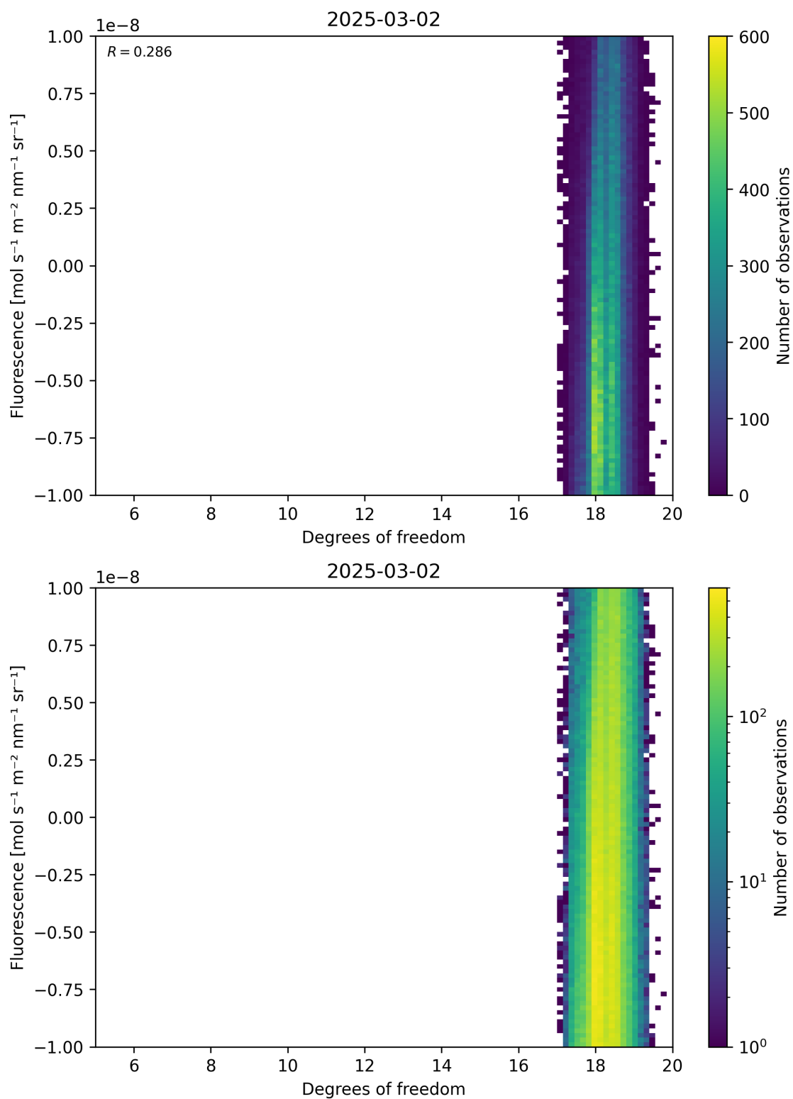
Figure 51: Scatter density plot of “Degrees of freedom” against “Fluorescence” for 2025-03-01 to 2025-03-03.
