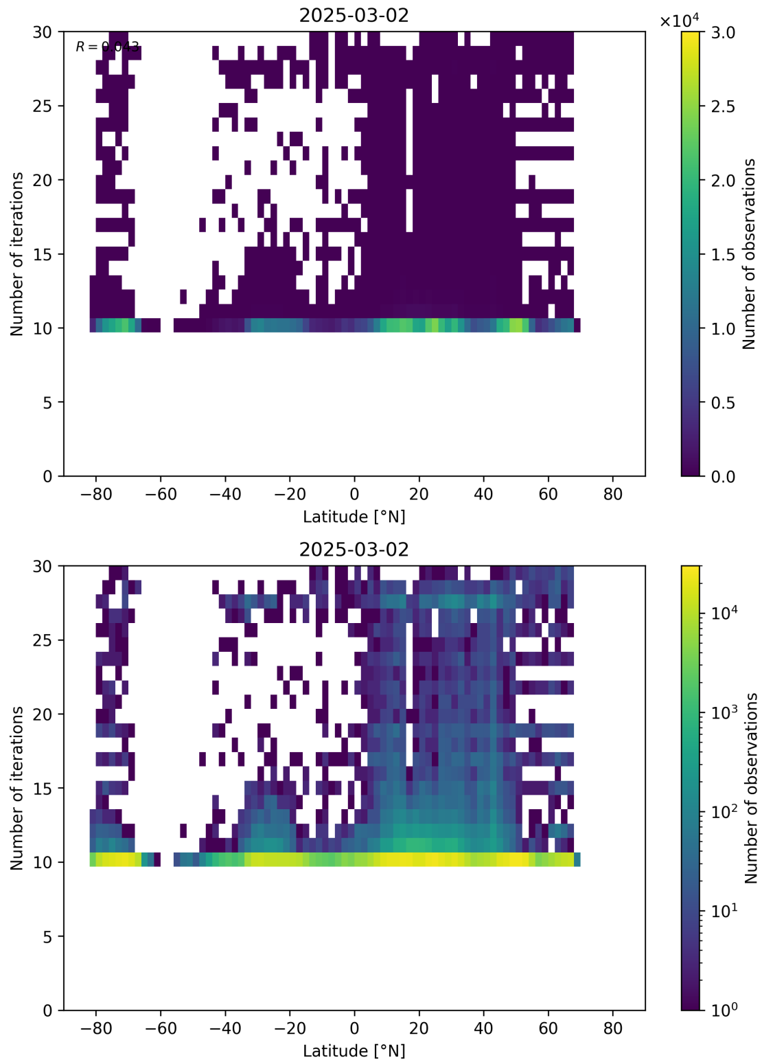
Figure 60: Scatter density plot of “Latitude” against “Number of iterations” for 2025-03-01 to 2025-03-03.
