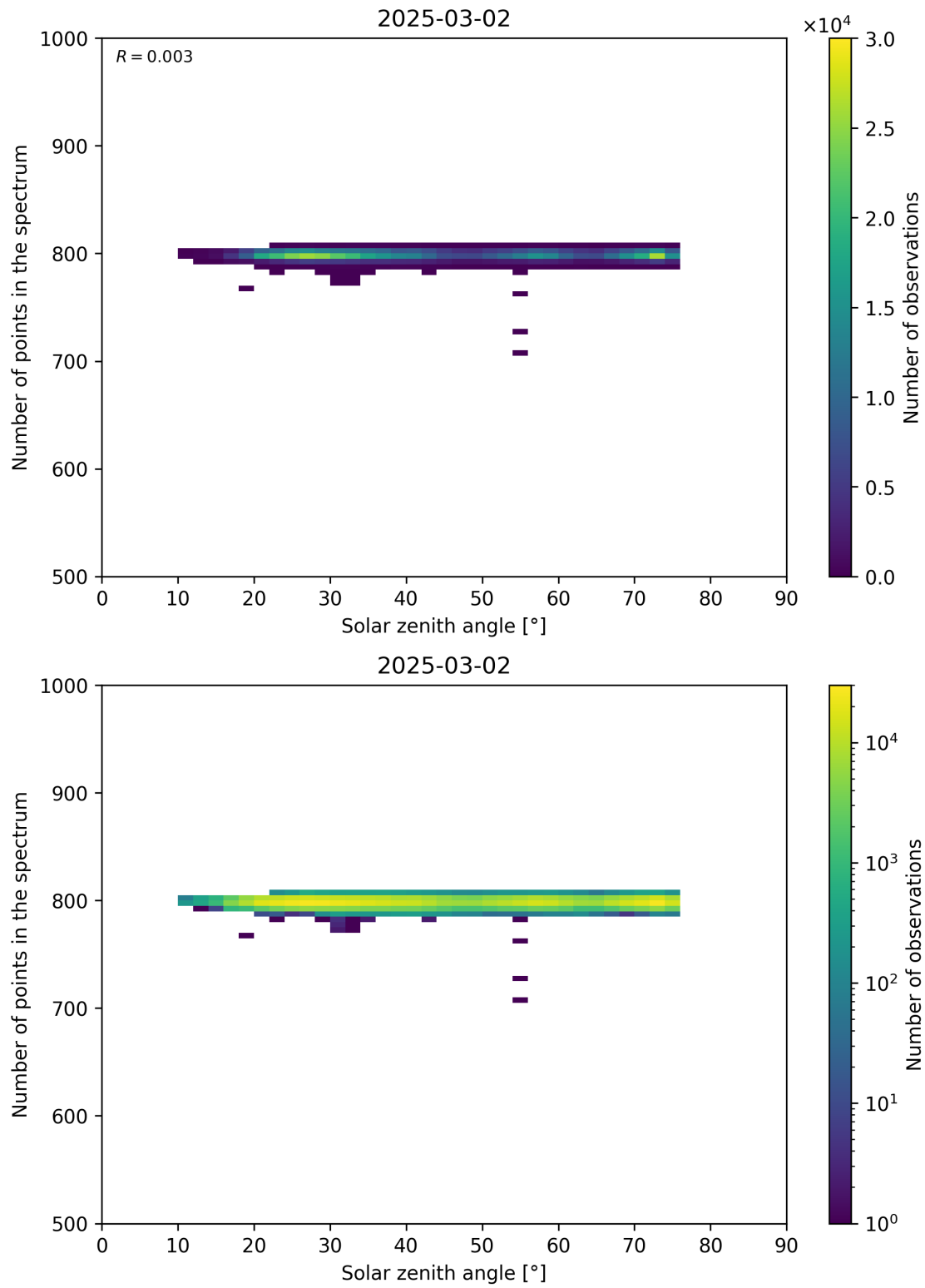
Figure 103: Scatter density plot of “Solar zenith angle” against “Number of points in the spectrum” for 2025-03-01 to 2025-03-03.
