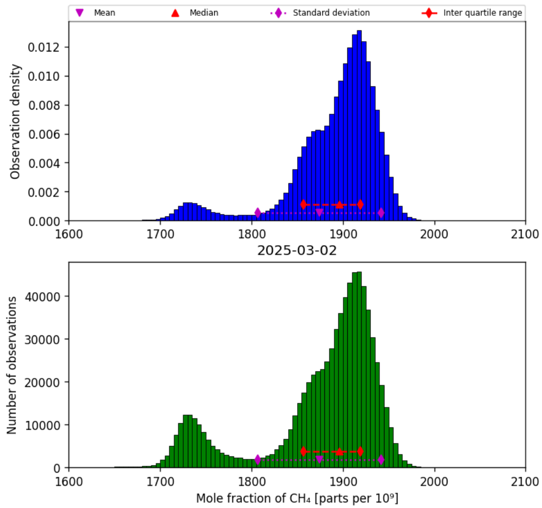
Figure 23: Histogram of “Mole fraction of CH 4 ” for 2025-03-01 to 2025-03-03
