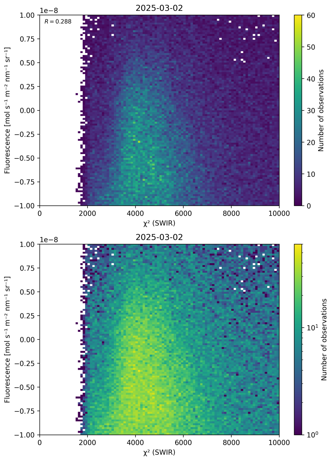
Figure 49: Scatter density plot of “ \chi^2 (SWIR)” against “Fluorescence” for 2025-03-01 to 2025-03-03.
