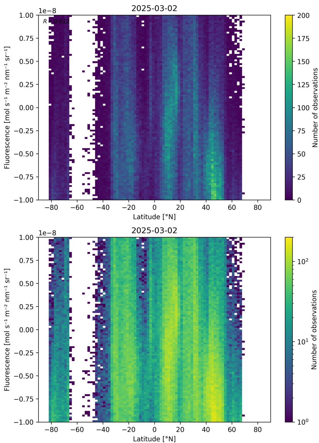
Figure 56: Scatter density plot of “Latitude” against “Fluorescence” for 2025-03-01 to 2025-03-03.
