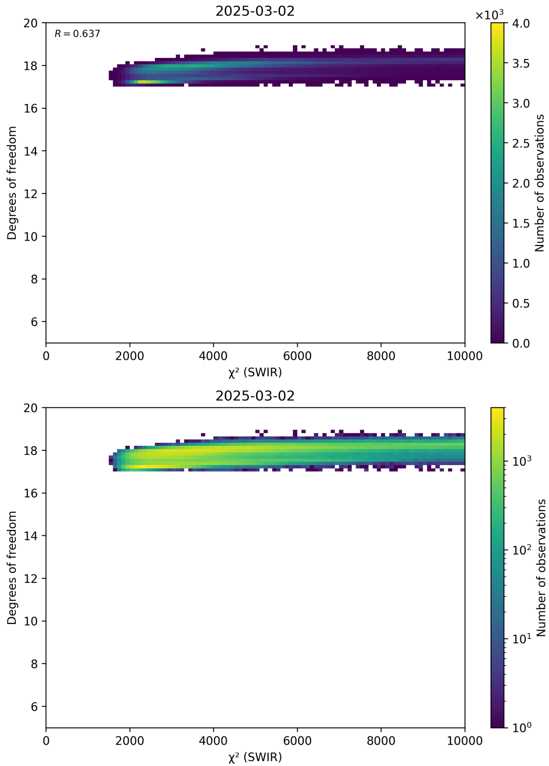
Figure 48: Scatter density plot of “ \chi^2 (SWIR)” against “Degrees of freedom” for 2025-03-01 to 2025-03-03.
