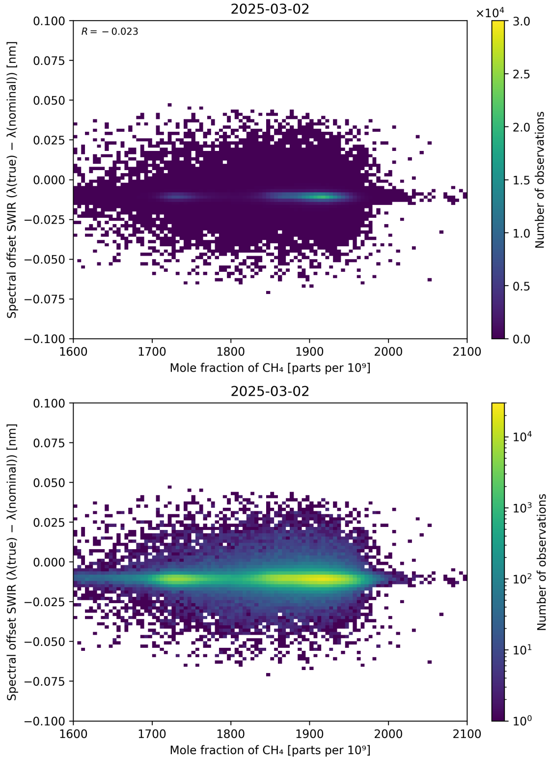
Figure 86: Scatter density plot of “Mole fraction of CH 4 ” against “Spectral offset SWIR ( \lambda_{\text{true}} - \lambda_{\text{nominal}} )” for 2025-03-01 to 2025-03-03.
