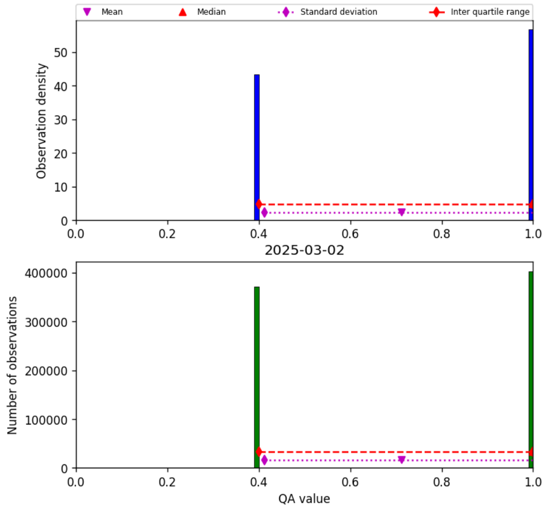
Figure 22: Histogram of “QA value” for 2025-03-01 to 2025-03-03
