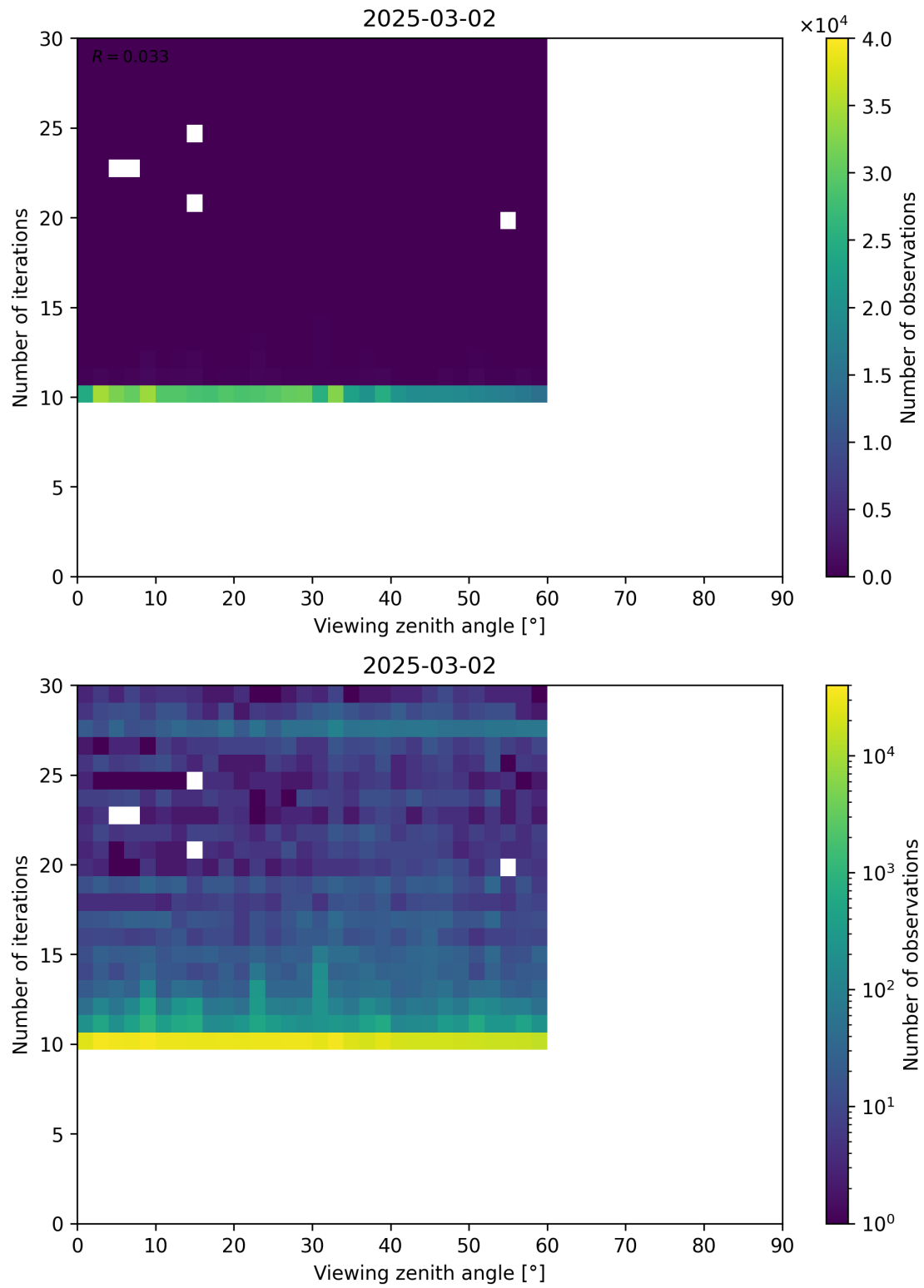
Figure 113: Scatter density plot of “Viewing zenith angle” against “Number of iterations” for 2025-03-01 to 2025-03-03.
