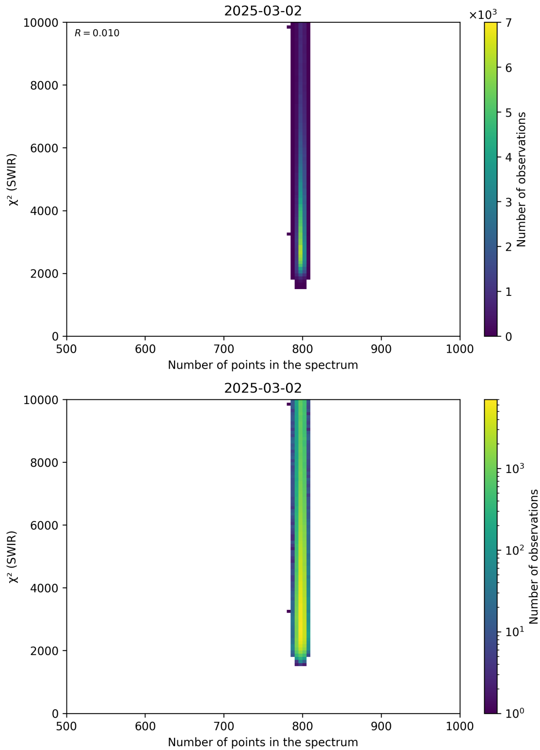
Figure 89: Scatter density plot of “Number of points in the spectrum” against “ \chi^2 (SWIR)” for 2025-03-01 to 2025-03-03.
