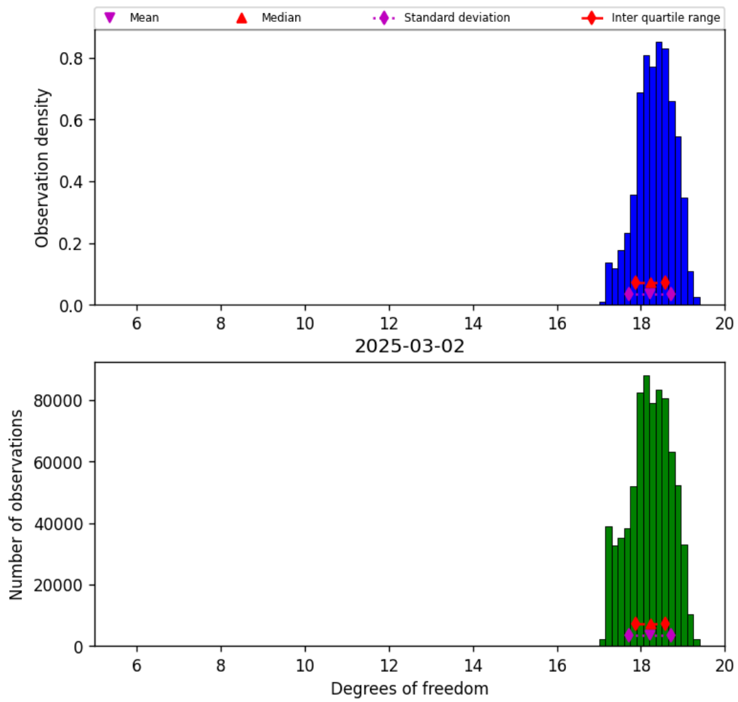
Figure 30: Histogram of “Degrees of freedom” for 2025-03-01 to 2025-03-03
