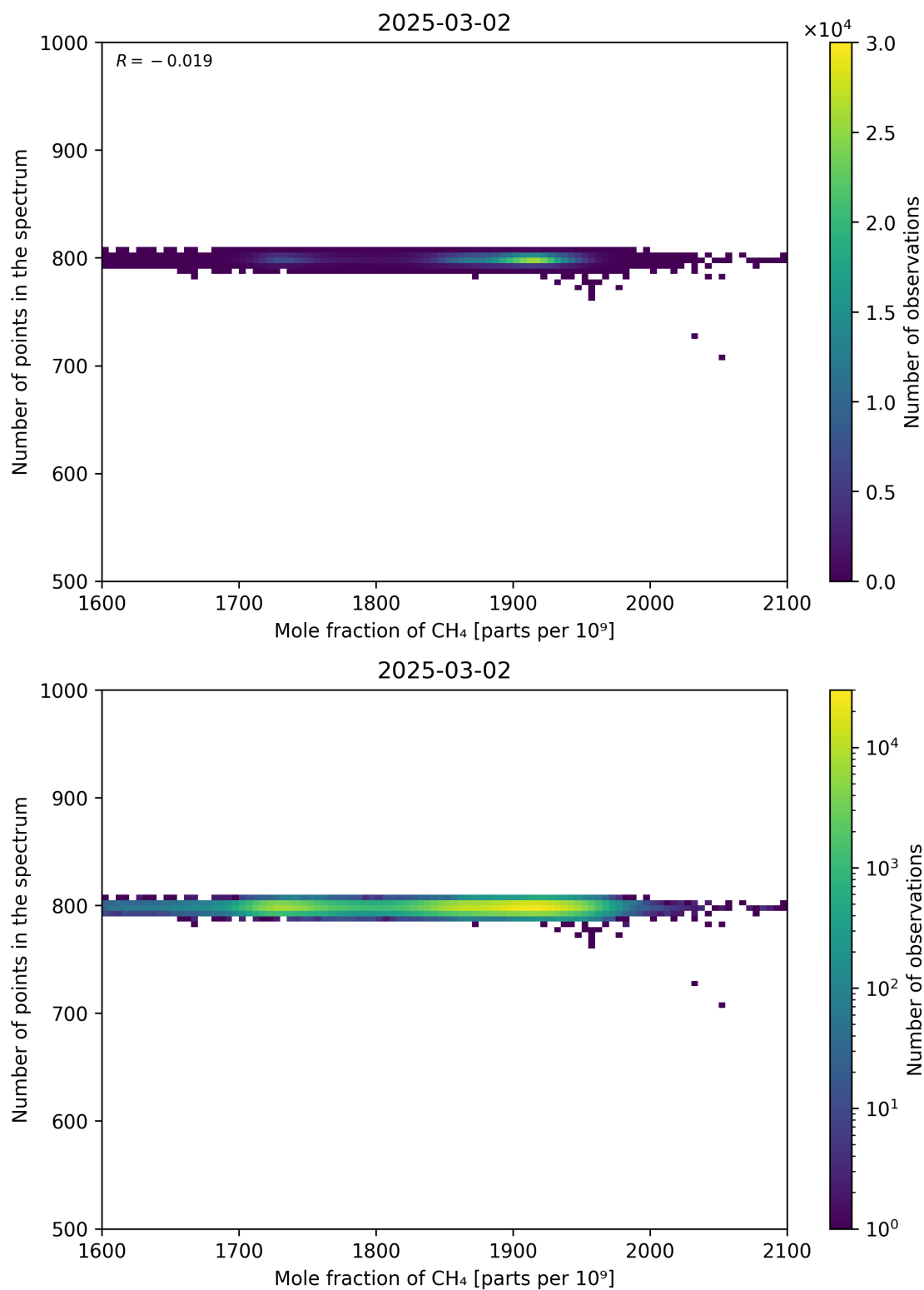
Figure 77: Scatter density plot of “Mole fraction of CH 4 ” against “Number of points in the spectrum” for 2025-03-01 to 2025-03-03.
