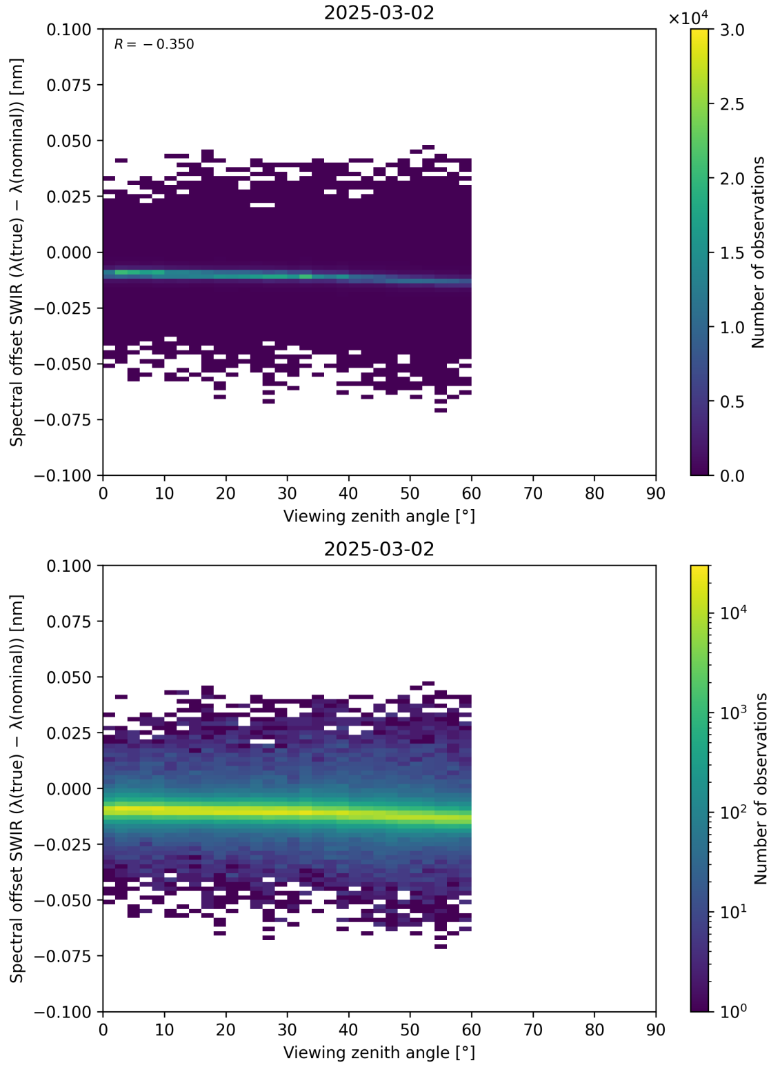
Figure 116: Scatter density plot of “Viewing zenith angle” against “Spectral offset SWIR ( \lambda_{\text{true}} - \lambda_{\text{nominal}} )” for 2025-03-01 to 2025-03-03.
