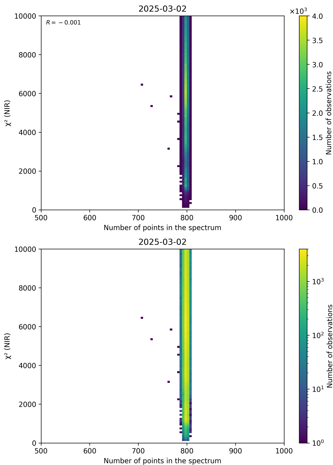
Figure 88: Scatter density plot of “Number of points in the spectrum” against “ \chi^2 (NIR)” for 2025-03-01 to 2025-03-03.
