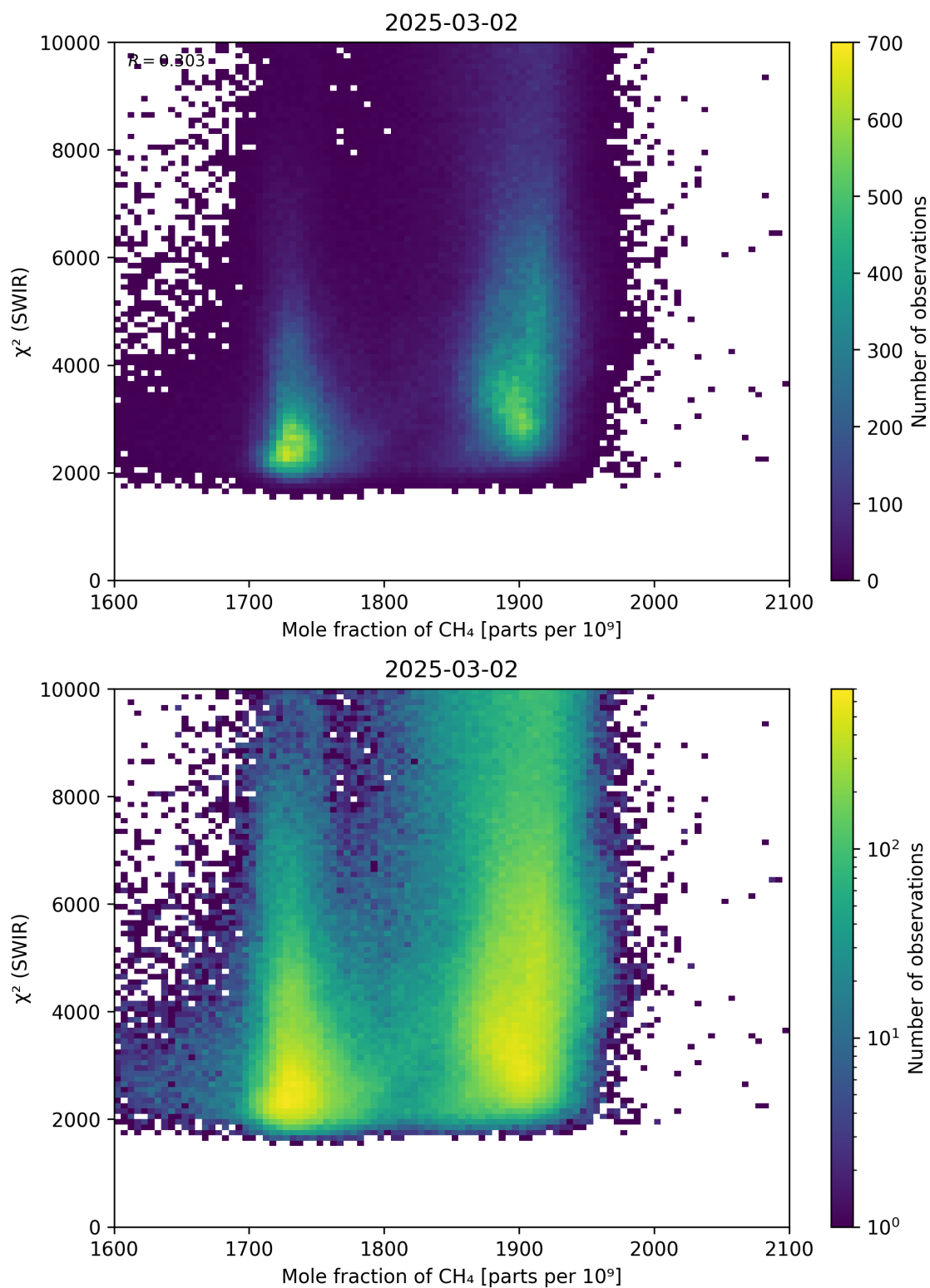
Figure 71: Scatter density plot of “Mole fraction of \text{CH}_4 ” against “ \chi^2 (SWIR)” for 2025-03-01 to 2025-03-03.
