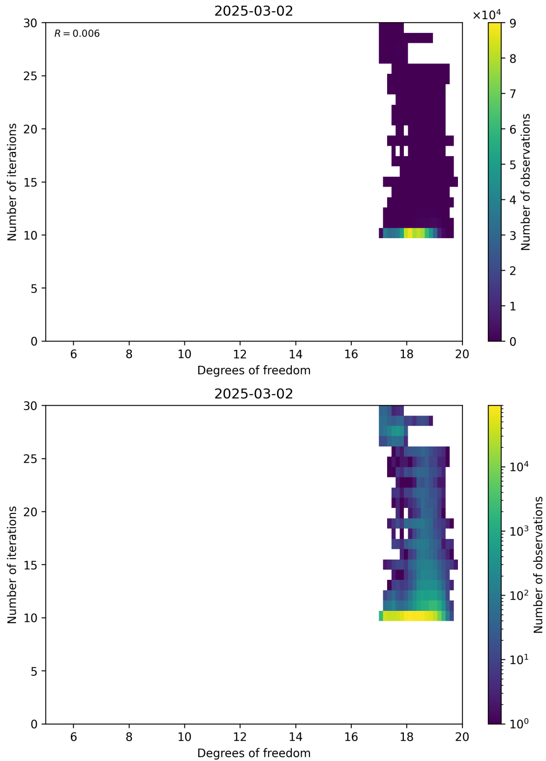
Figure 52: Scatter density plot of “Degrees of freedom” against “Number of iterations” for 2025-03-01 to 2025-03-03.
