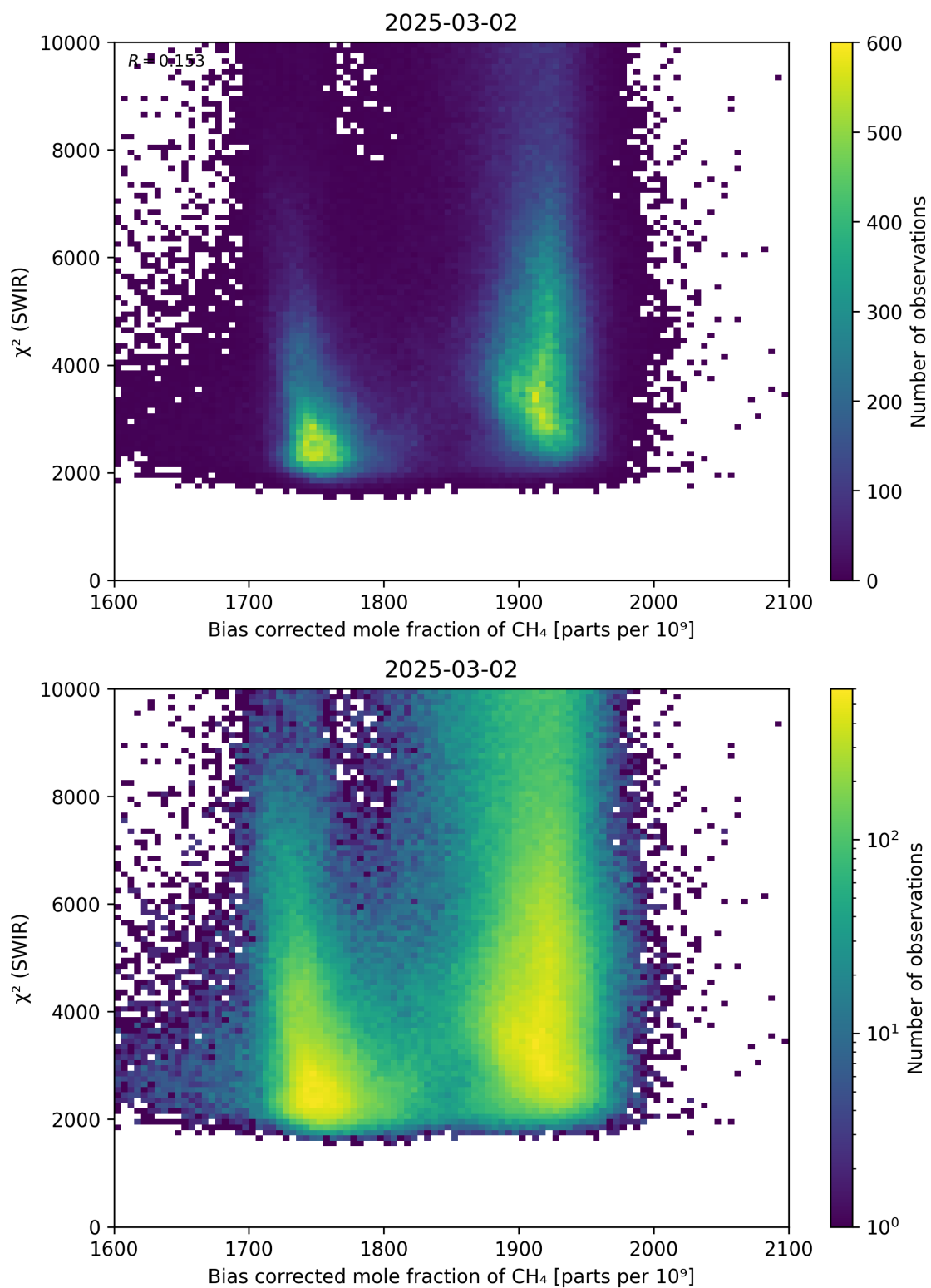
Figure 64: Scatter density plot of “Bias corrected mole fraction of \text{CH}_4 ” against “ \chi^2 (SWIR)” for 2025-03-01 to 2025-03-03.
