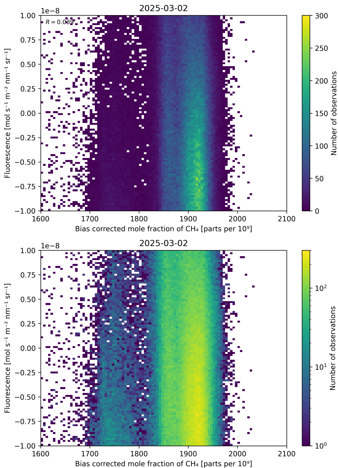
Figure 66: Scatter density plot of “Bias corrected mole fraction of \text{CH}_4 ” against “Fluorescence” for 2025-03-01 to 2025-03-03.
