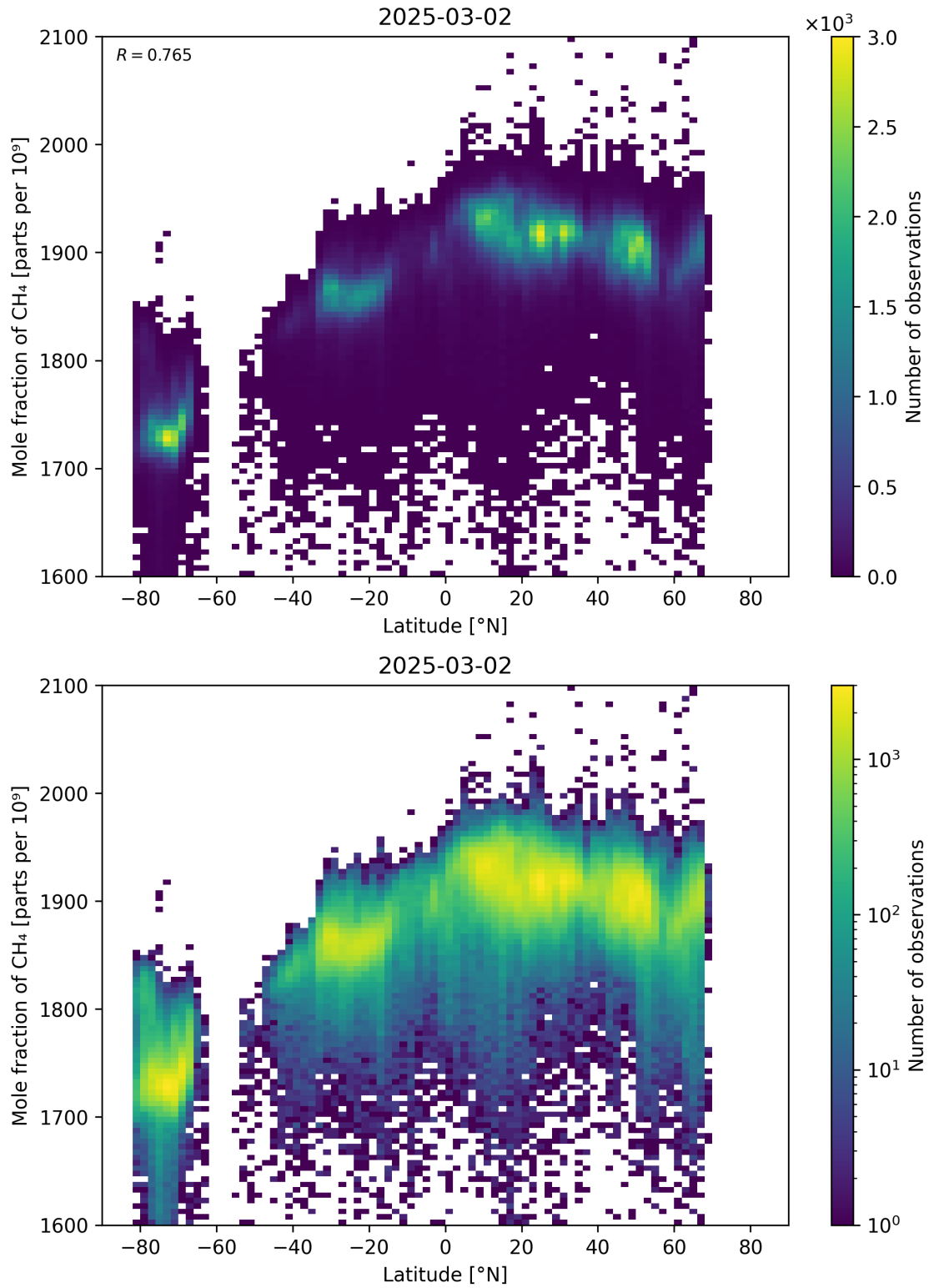
Figure 57: Scatter density plot of “Latitude” against “Mole fraction of CH 4 ” for 2025-03-01 to 2025-03-03.
