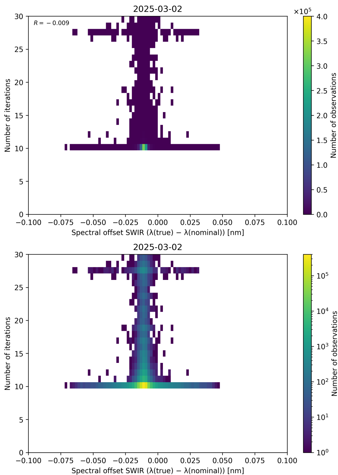
Figure 121: Scatter density plot of “Spectral offset SWIR ( \lambda_{\text{true}} - \lambda_{\text{nominal}} )” against “Number of iterations” for 2025-03-01 to 2025-03-03.
