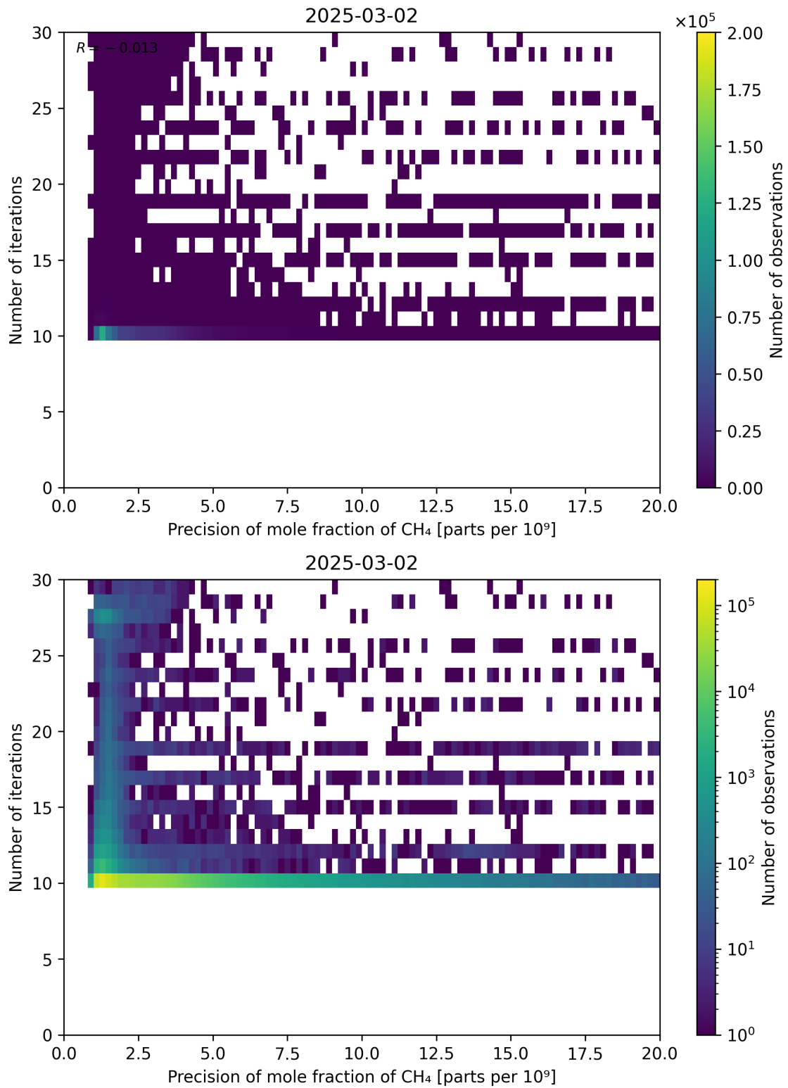
Figure 83: Scatter density plot of “Precision of mole fraction of CH 4 ” against “Number of iterations” for 2025-03-01 to 2025-03-03.
