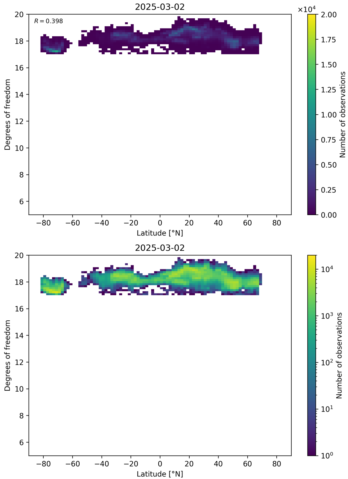
Figure 55: Scatter density plot of “Latitude” against “Degrees of freedom” for 2025-03-01 to 2025-03-03.
