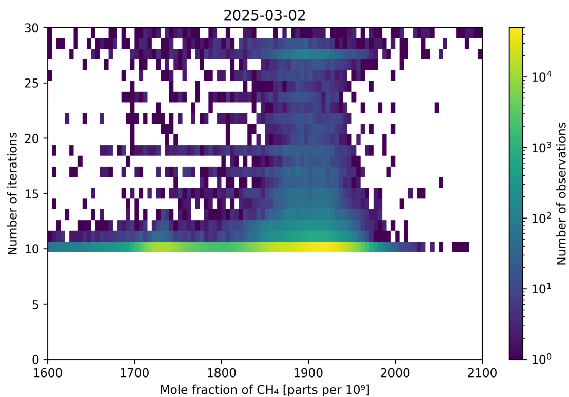
Figure 76: Scatter density plot of “Mole fraction of CH 4 ” against “Number of iterations” for 2025-03-01 to 2025-03-03.
