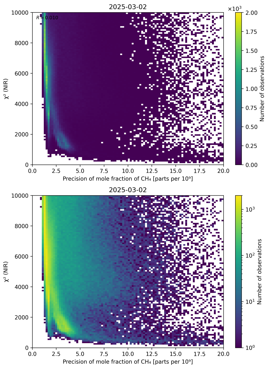
Figure 78: Scatter density plot of “Precision of mole fraction of CH 4 ” against “ \chi^2 (NIR)” for 2025-03-01 to 2025-03-03.
