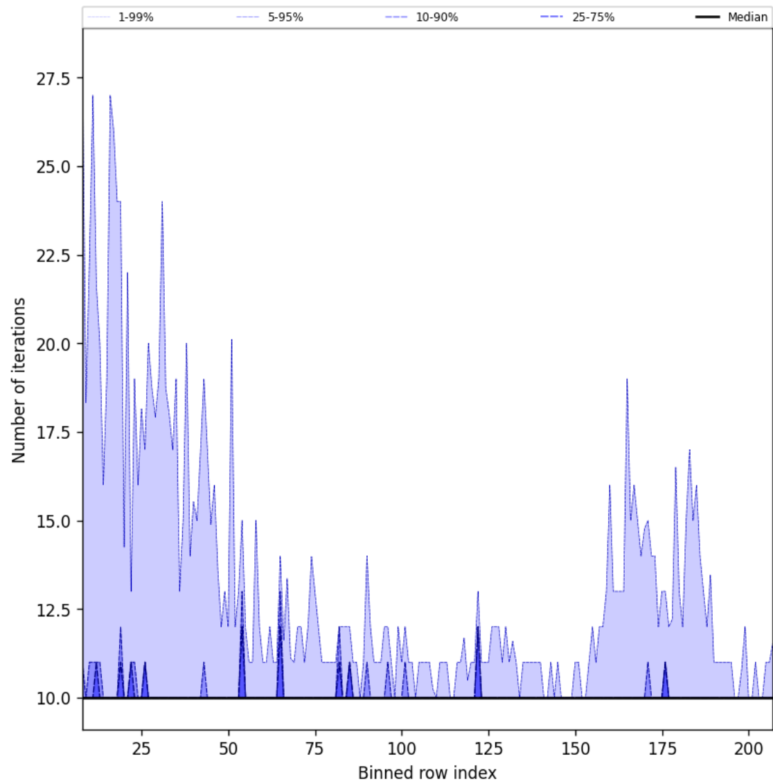
Figure 42: Along track statistics of “Number of iterations” for 2025-03-01 to 2025-03-03
