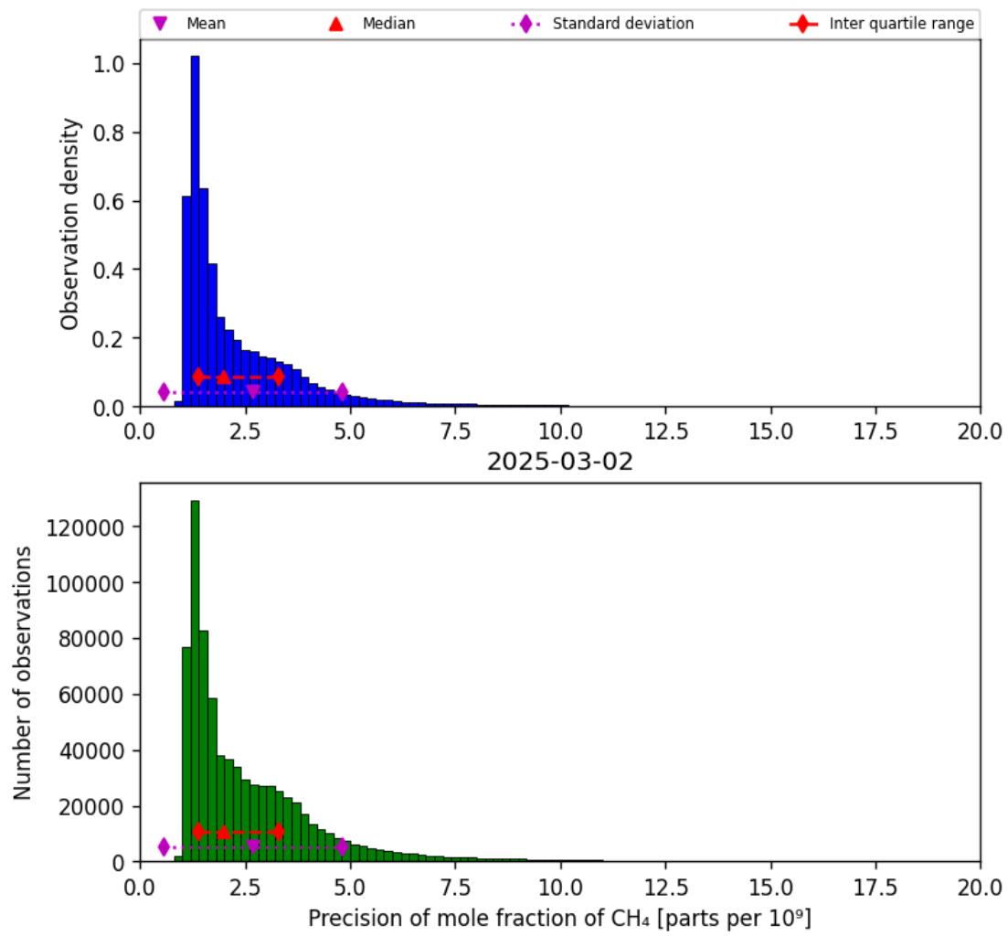
Figure 24: Histogram of “Precision of mole fraction of CH 4 ” for 2025-03-01 to 2025-03-03
