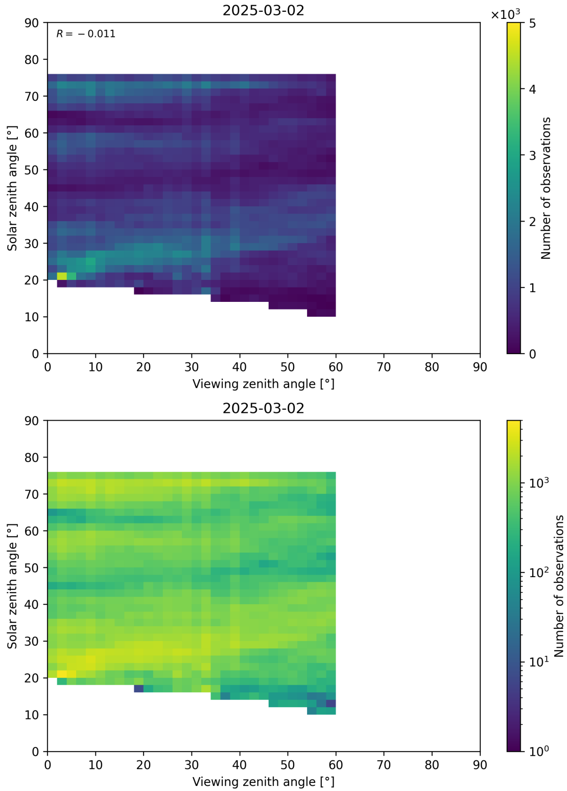
Figure 115: Scatter density plot of “Viewing zenith angle” against “Solar zenith angle” for 2025-03-01 to 2025-03-03.
