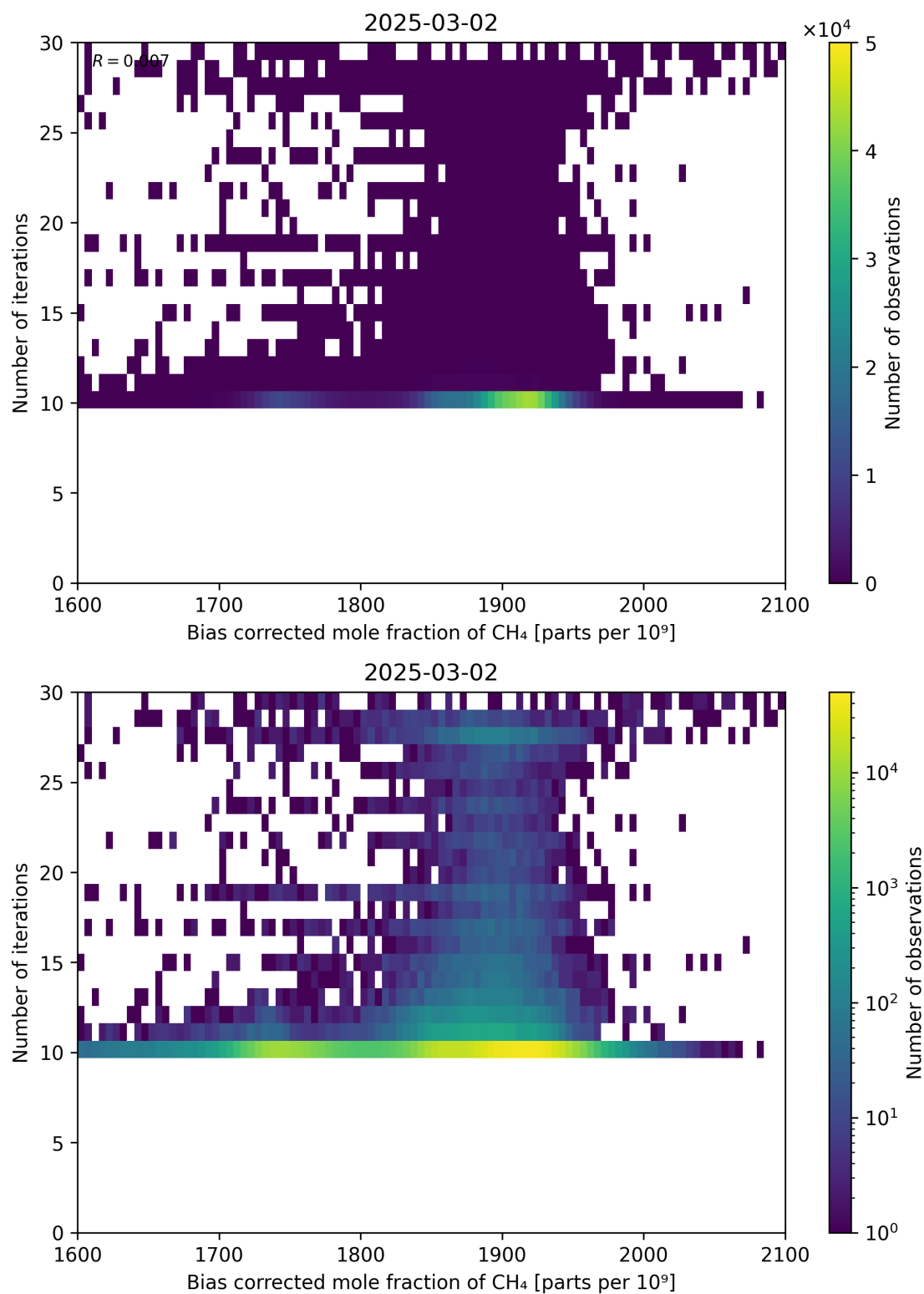
Figure 67: Scatter density plot of “Bias corrected mole fraction of \text{CH}_4 ” against “Number of iterations” for 2025-03-01 to 2025-03-03.
