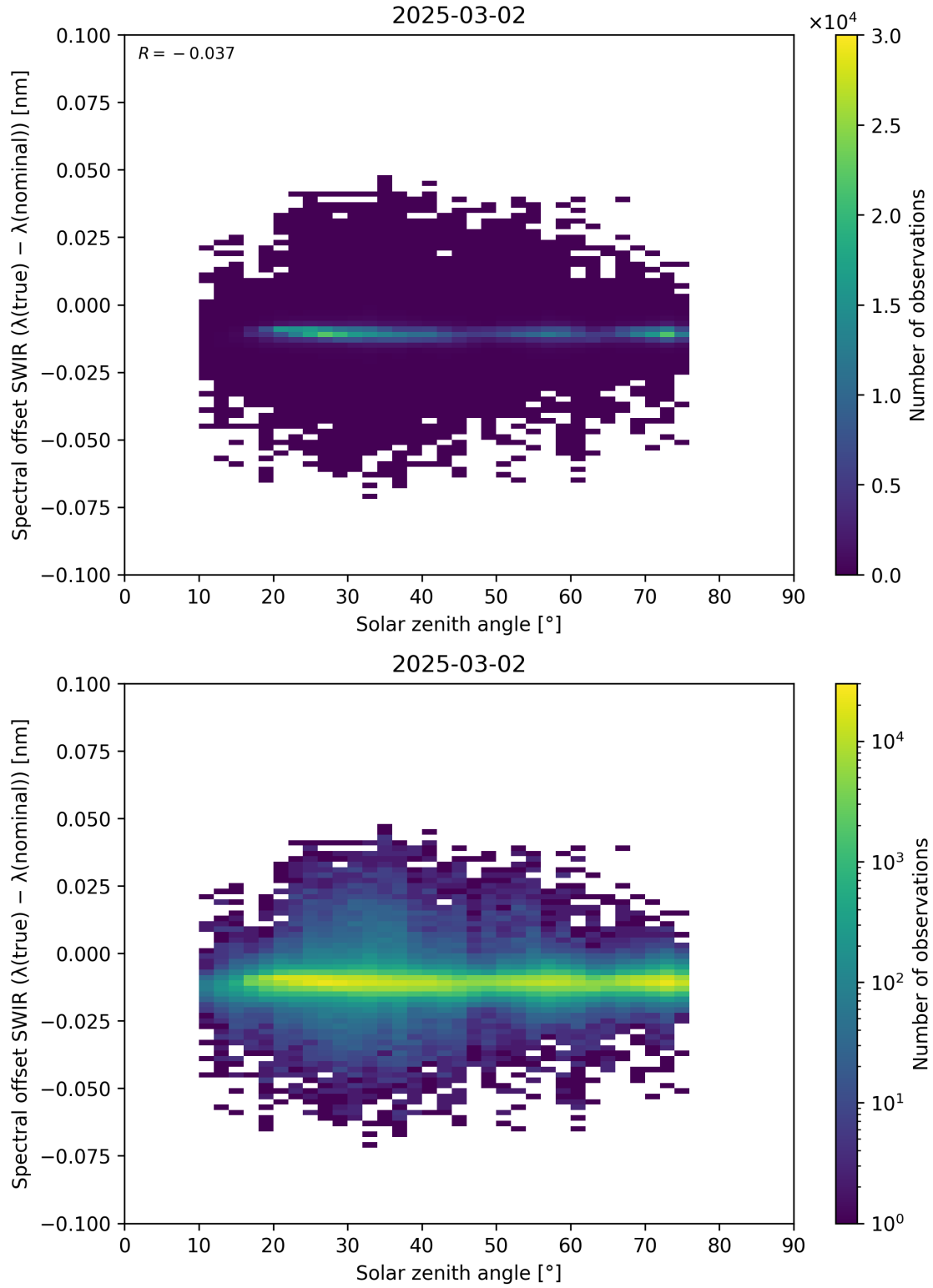
Figure 104: Scatter density plot of “Solar zenith angle” against “Spectral offset SWIR ( \lambda_{\text{true}} - \lambda_{\text{nominal}} )” for 2025-03-01 to 2025-03-03.
