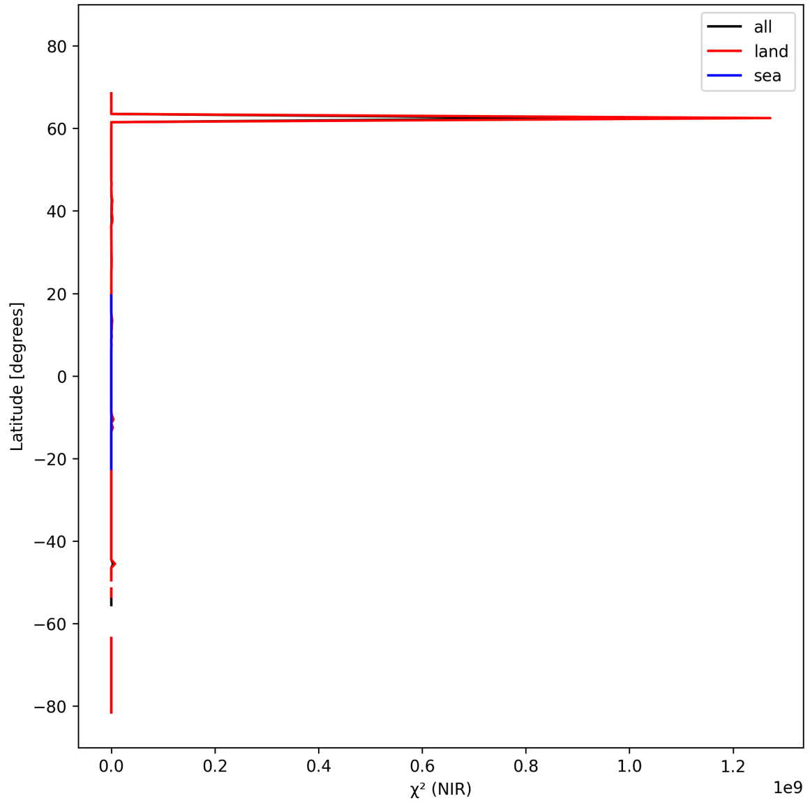
Figure 18: Zonal average of “ \chi^2 (NIR)” for 2025-03-01 to 2025-03-03.
