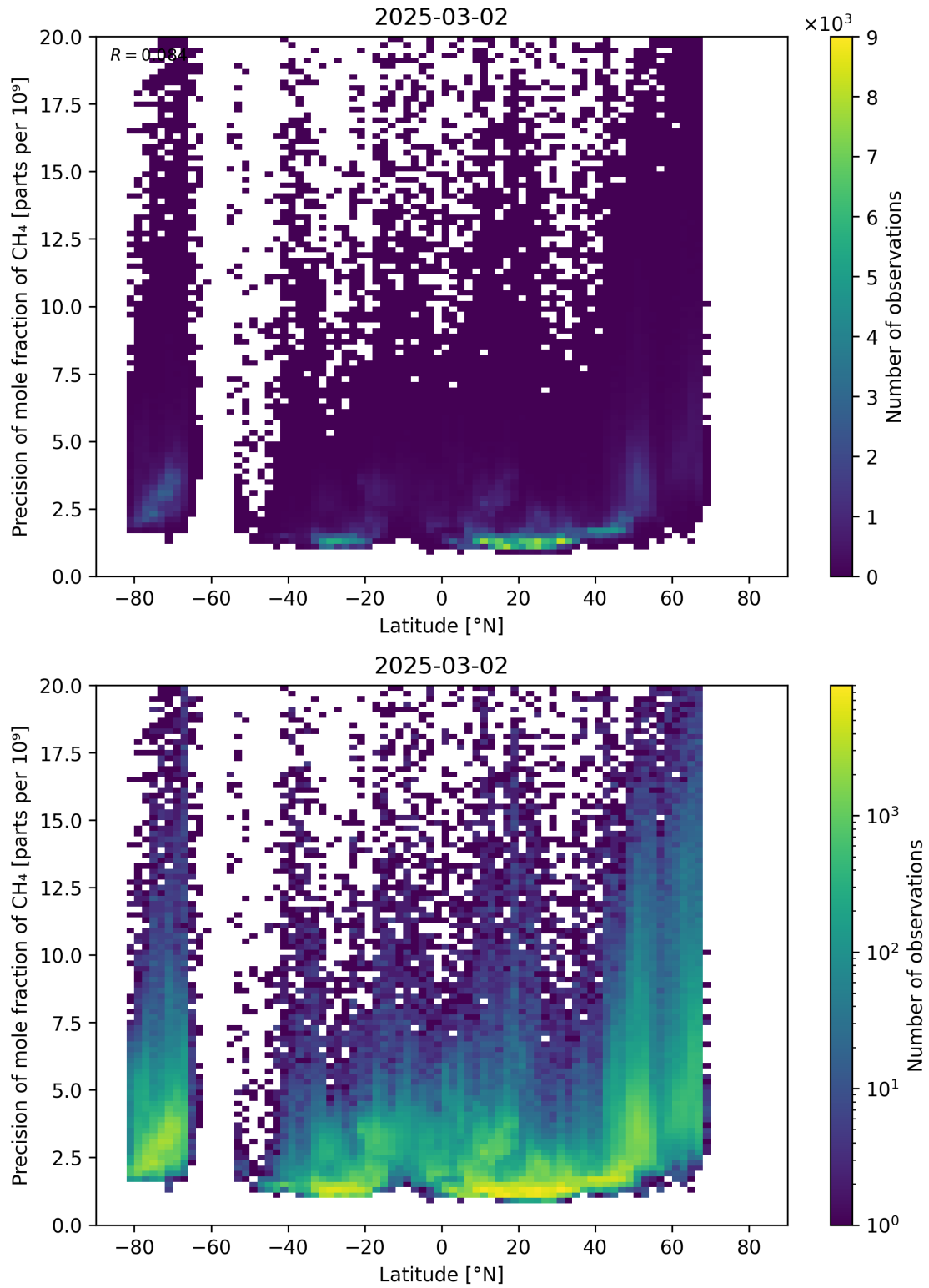
Figure 59: Scatter density plot of “Latitude” against “Precision of mole fraction of CH 4 ” for 2025-03-01 to 2025-03-03.
