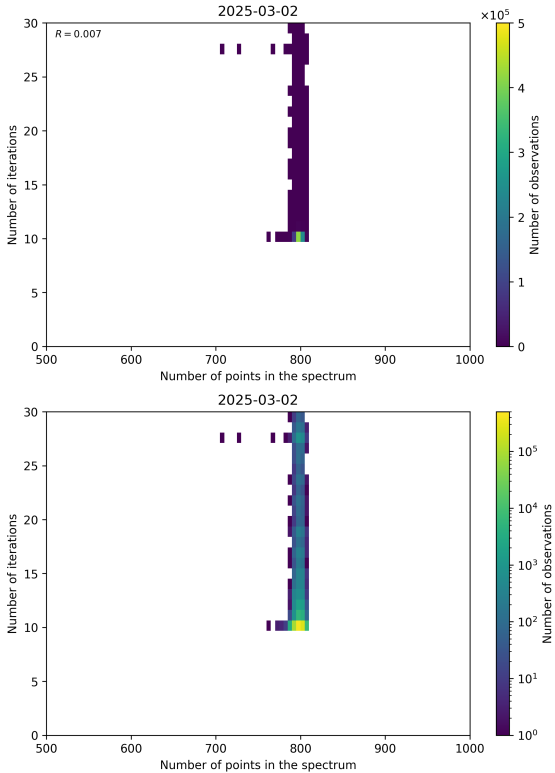
Figure 92: Scatter density plot of “Number of points in the spectrum” against “Number of iterations” for 2025-03-01 to 2025-03-03.
