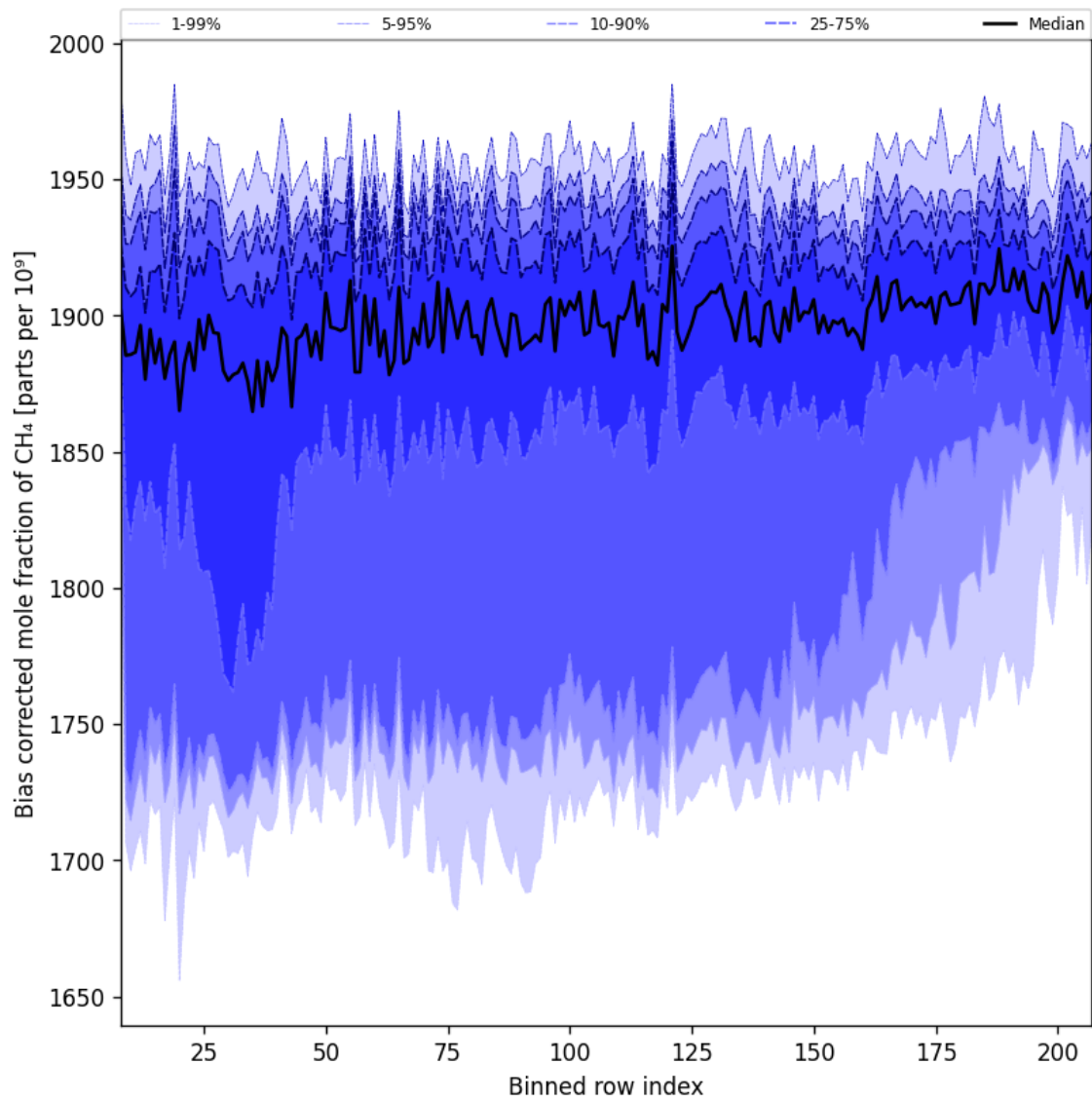
Figure 36: Along track statistics of “Bias corrected mole fraction of CH 4 ” for 2025-03-01 to 2025-03-03
