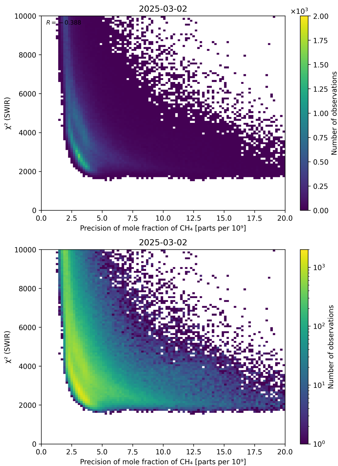
Figure 79: Scatter density plot of “Precision of mole fraction of CH 4 ” against “ \chi^2 (SWIR)” for 2025-03-01 to 2025-03-03.
