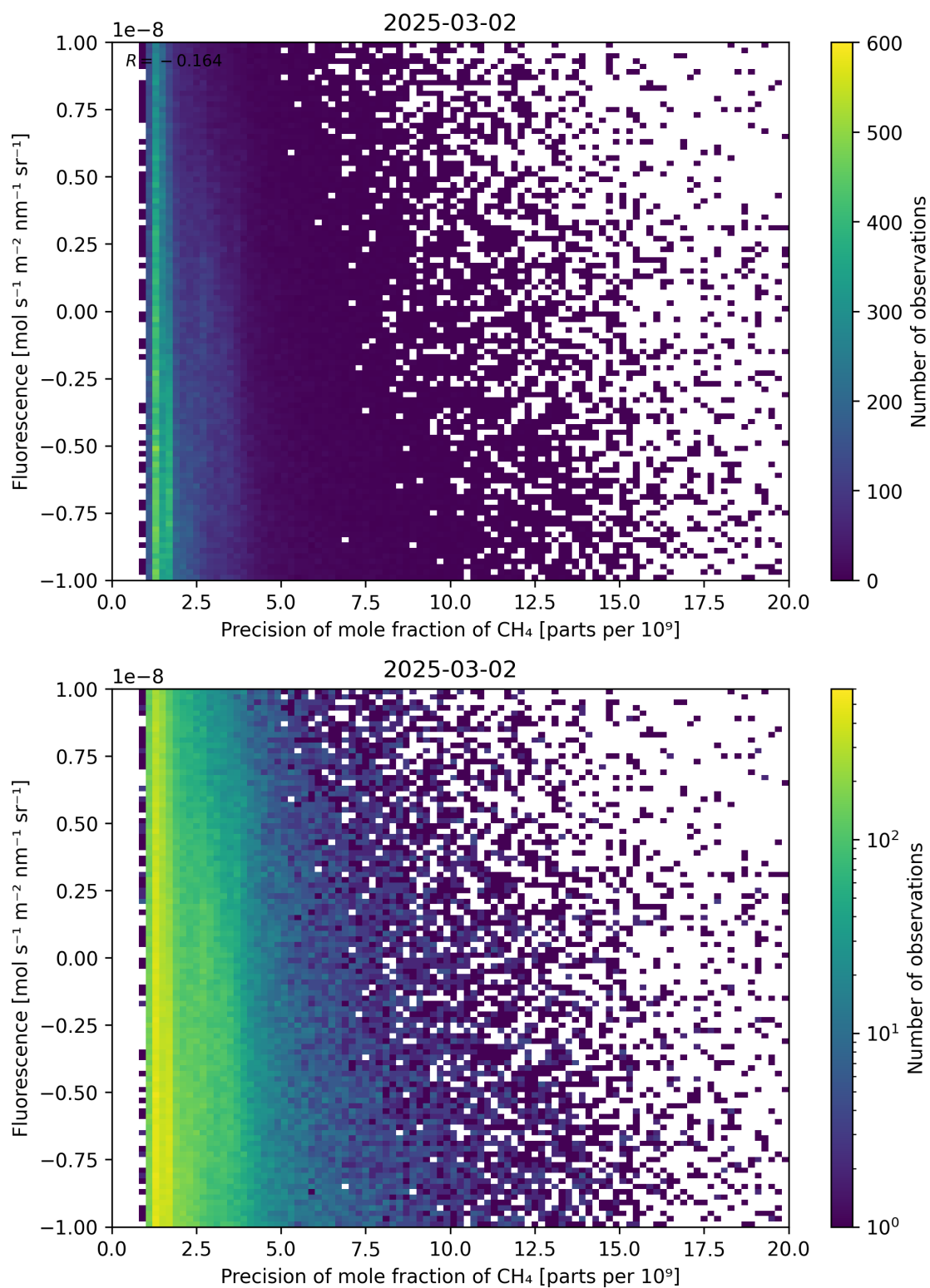
Figure 81: Scatter density plot of “Precision of mole fraction of \text{CH}_4 ” against “Fluorescence” for 2025-03-01 to 2025-03-03.
