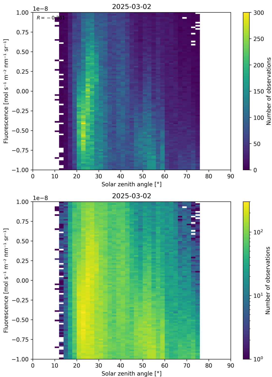
Figure 97: Scatter density plot of “Solar zenith angle” against “Fluorescence” for 2025-03-01 to 2025-03-03.
