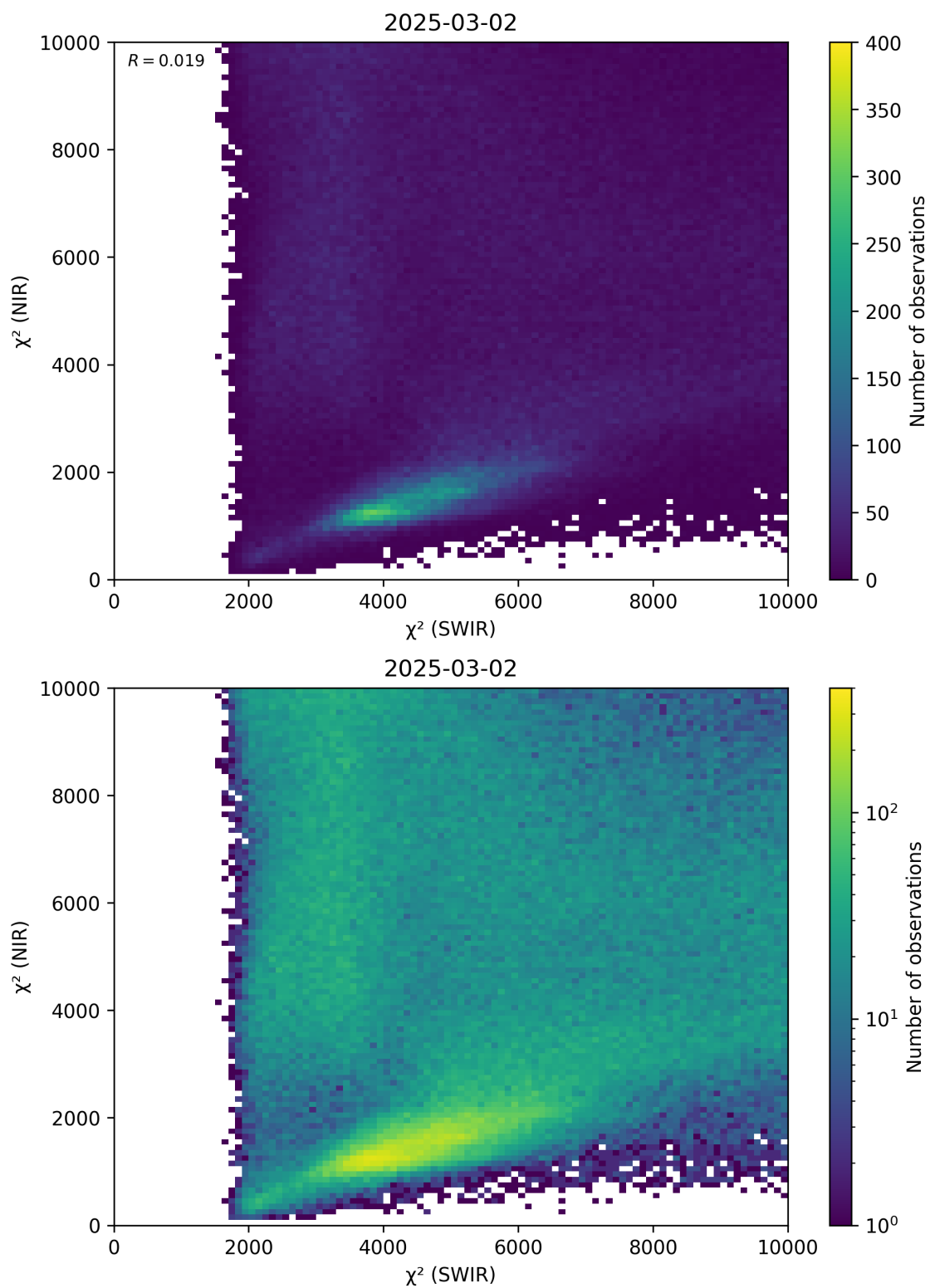
Figure 47: Scatter density plot of “ \chi^2 (SWIR)” against “ \chi^2 (NIR)” for 2025-03-01 to 2025-03-03.
