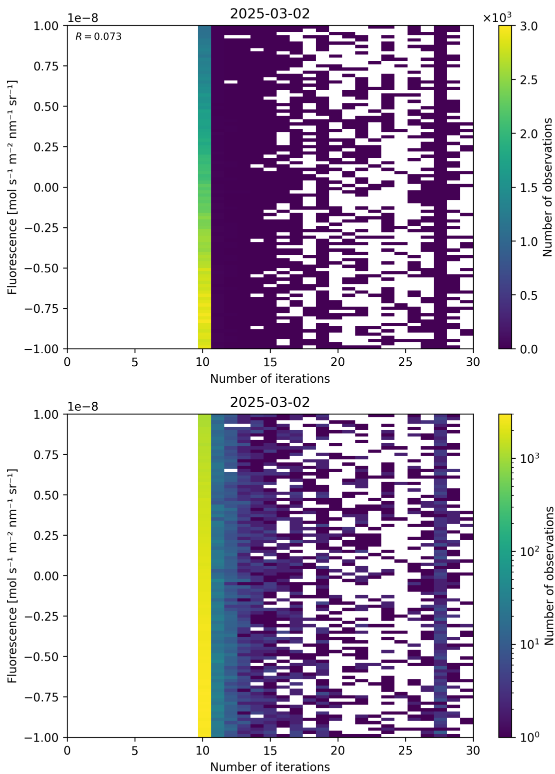
Figure 87: Scatter density plot of "Number of iterations" against "Fluorescence" for 2025-03-01 to 2025-03-03.
