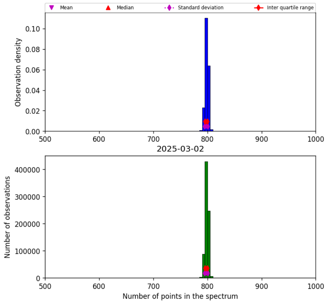
Figure 26: Histogram of “Number of points in the spectrum” for 2025-03-01 to 2025-03-03
