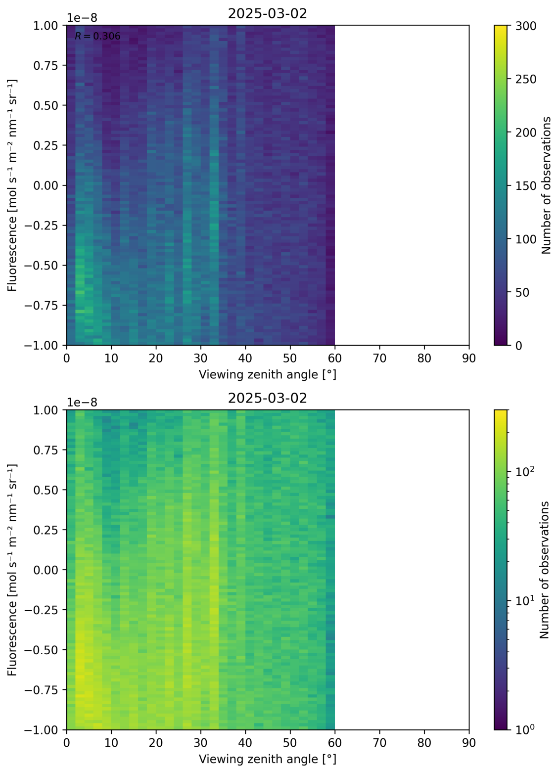
Figure 108: Scatter density plot of “Viewing zenith angle” against “Fluorescence” for 2025-03-01 to 2025-03-03.
