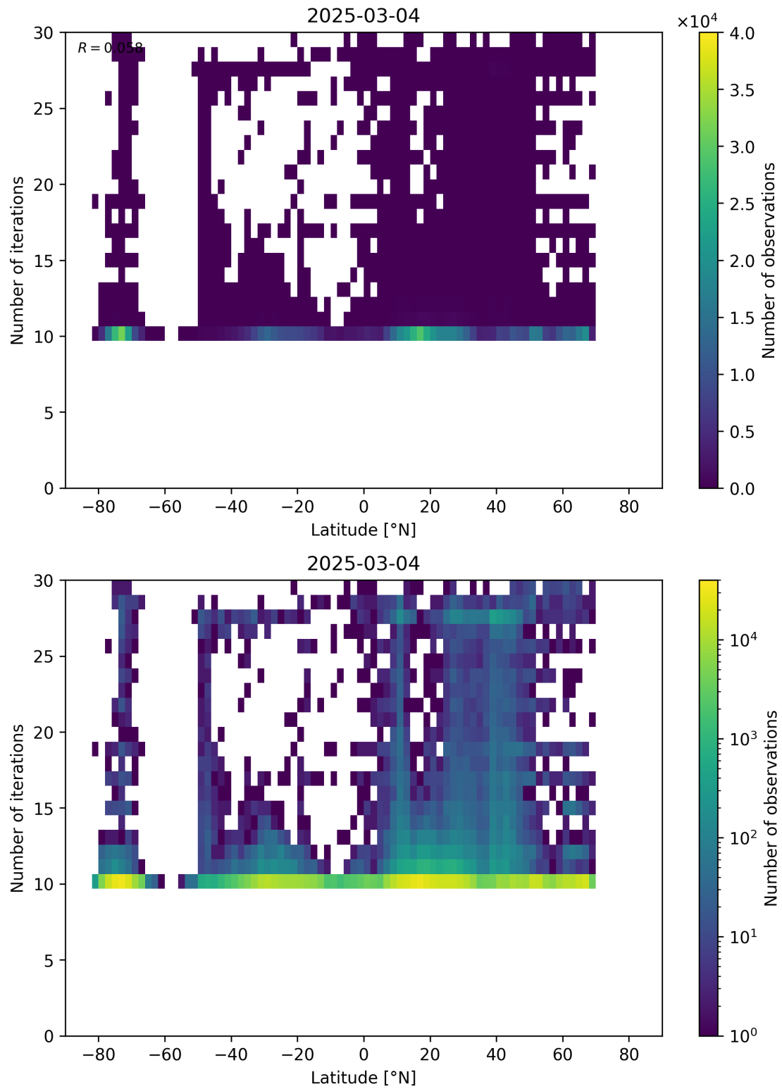
Figure 60: Scatter density plot of “Latitude” against “Number of iterations” for 2025-03-03 to 2025-03-05.
