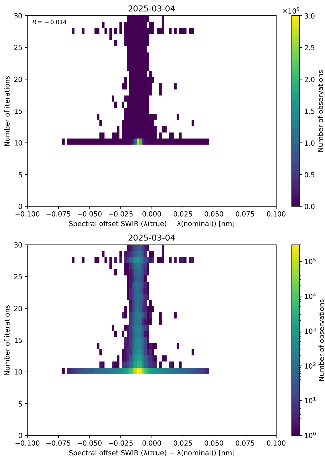
Figure 121: Scatter density plot of “Spectral offset SWIR ( \lambda_{\text{true}} - \lambda_{\text{nominal}} )” against “Number of iterations” for 2025-03-03 to 2025-03-05.
