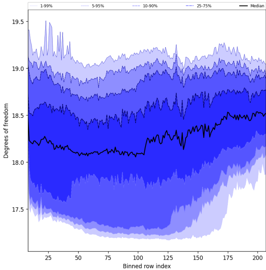
Figure 41: Along track statistics of “Degrees of freedom” for 2025-03-03 to 2025-03-05
