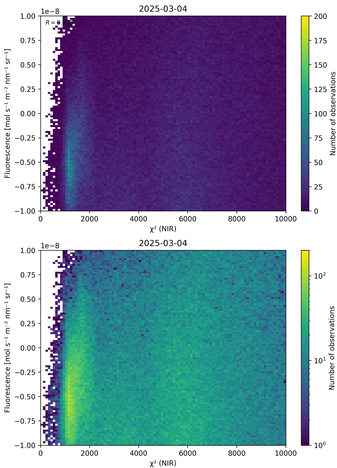
Figure 45: Scatter density plot of “ \chi^2 (NIR)” against “Fluorescence” for 2025-03-03 to 2025-03-05.
