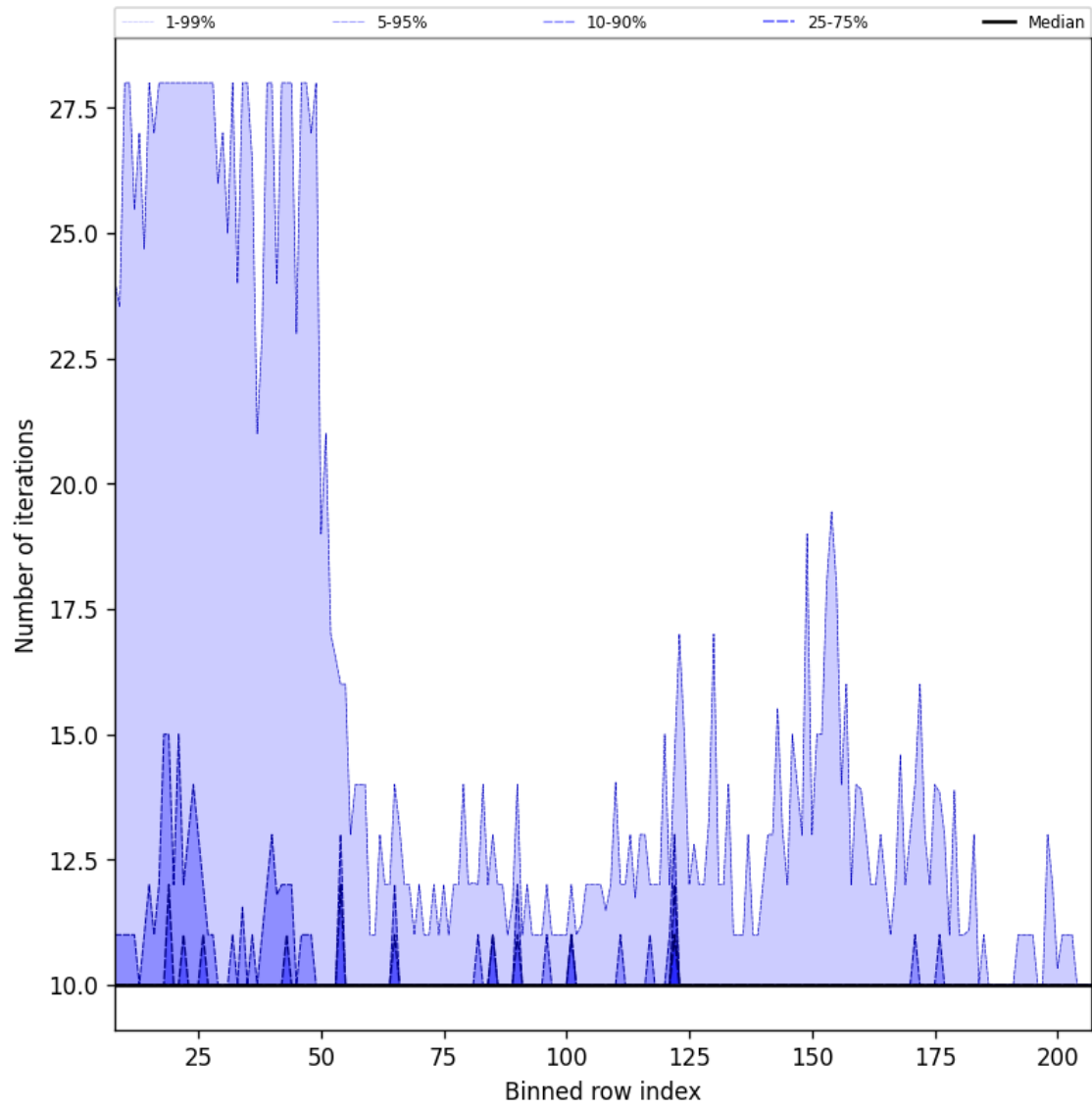
Figure 42: Along track statistics of “Number of iterations” for 2025-03-03 to 2025-03-05
