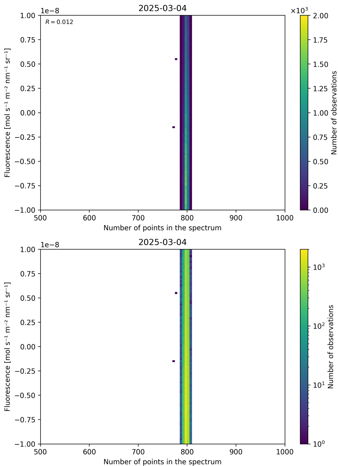
Figure 91: Scatter density plot of “Number of points in the spectrum” against “Fluorescence” for 2025-03-03 to 2025-03-05.
