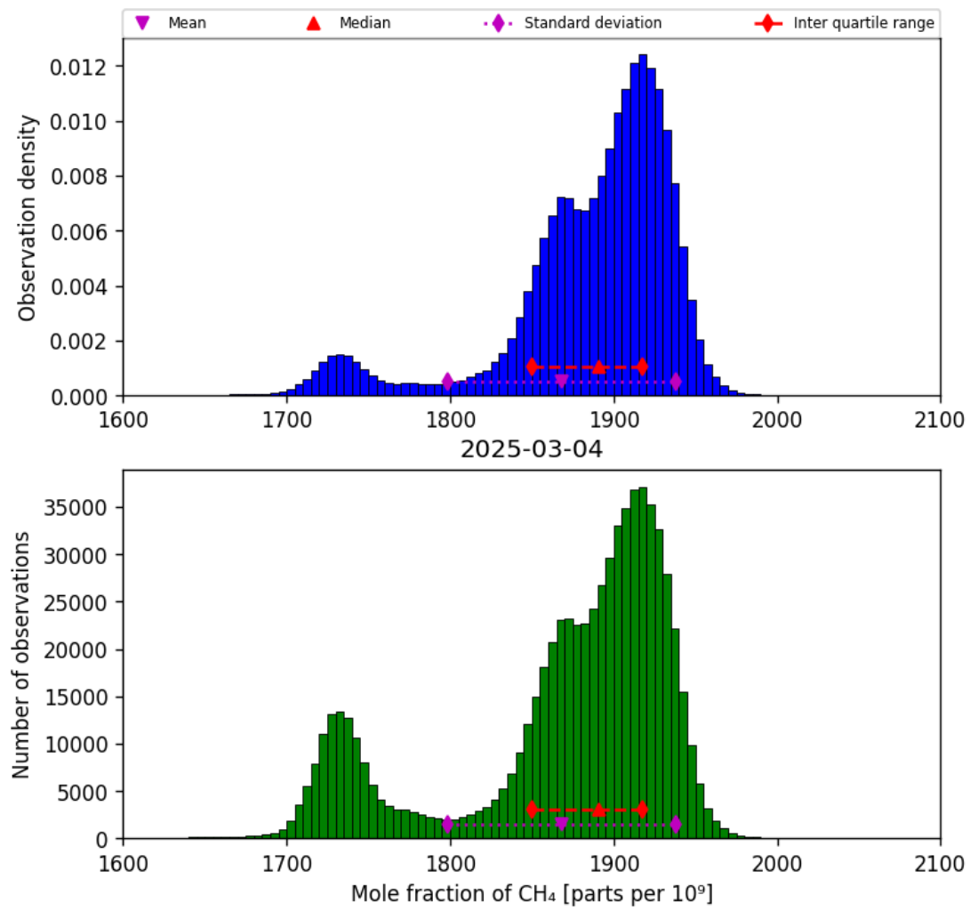
Figure 23: Histogram of “Mole fraction of CH 4 ” for 2025-03-03 to 2025-03-05
