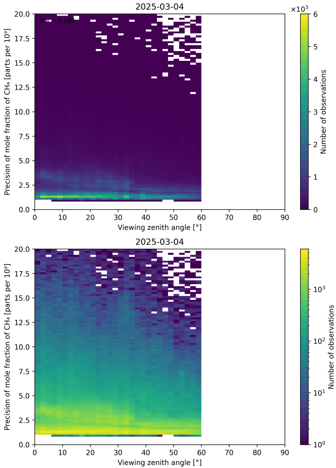
Figure 112: Scatter density plot of “Viewing zenith angle” against “Precision of mole fraction of CH 4 ” for 2025-03-03 to 2025-03-05.
