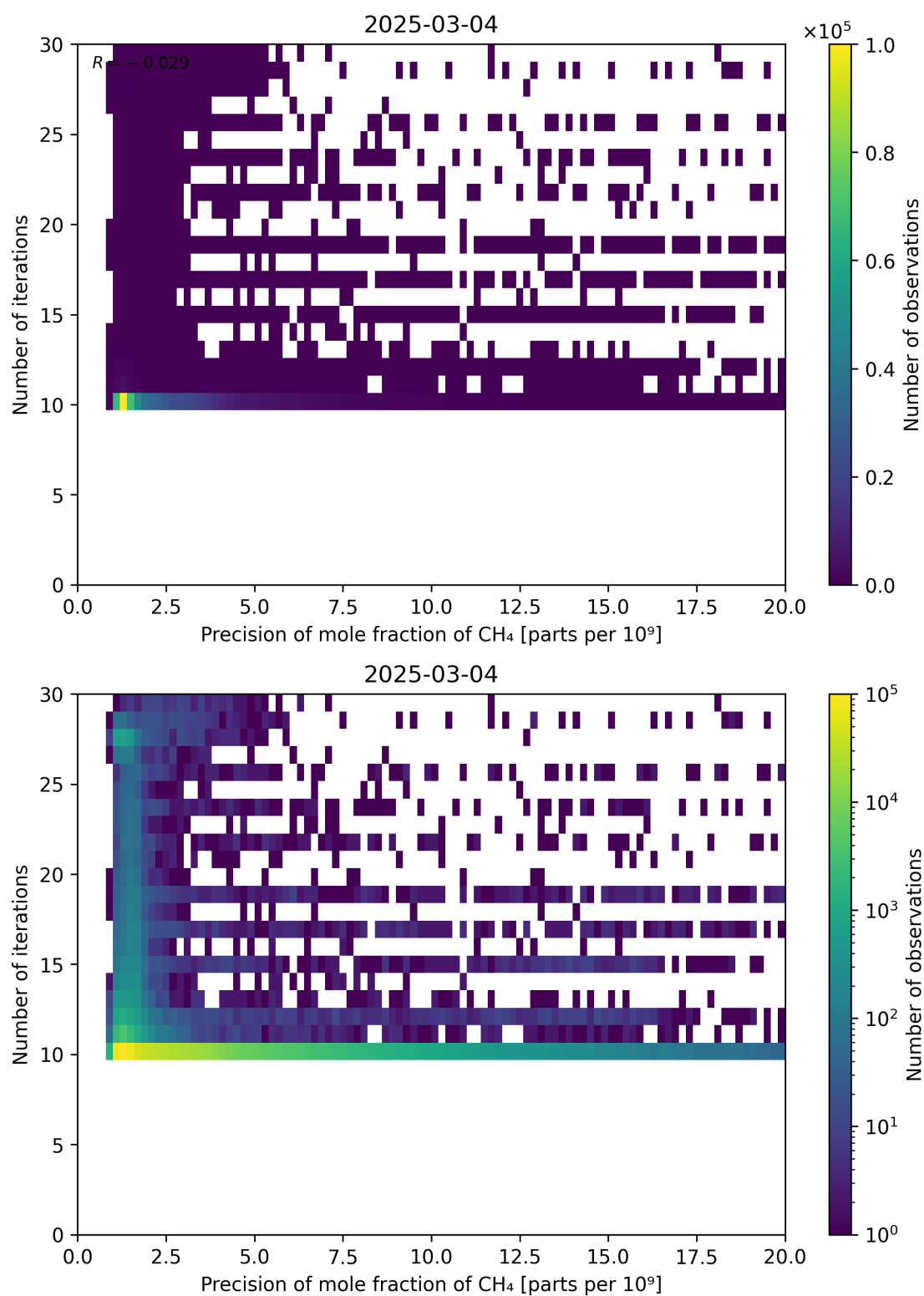
Figure 83: Scatter density plot of “Precision of mole fraction of CH 4 ” against “Number of iterations” for 2025-03-03 to 2025-03-05.
