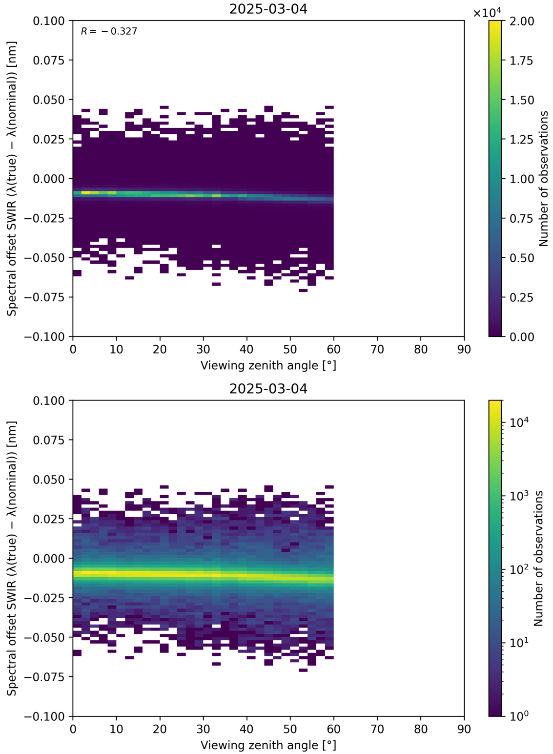
Figure 116: Scatter density plot of “Viewing zenith angle” against “Spectral offset SWIR ( \lambda_{\text{true}} - \lambda_{\text{nominal}} )” for 2025-03-03 to 2025-03-05.
