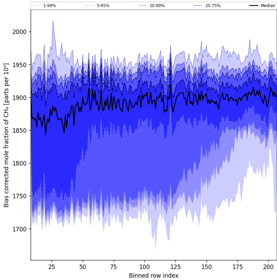
Figure 36: Along track statistics of “Bias corrected mole fraction of CH 4 ” for 2025-03-03 to 2025-03-05
