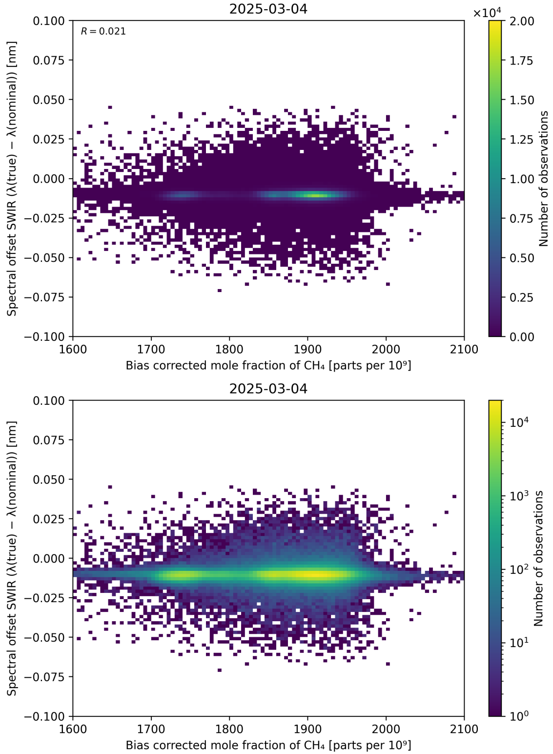
Figure 69: Scatter density plot of “Bias corrected mole fraction of CH 4 ” against “Spectral offset SWIR ( \lambda_{\text{true}} - \lambda_{\text{nominal}} )” for 2025-03-03 to 2025-03-05.
