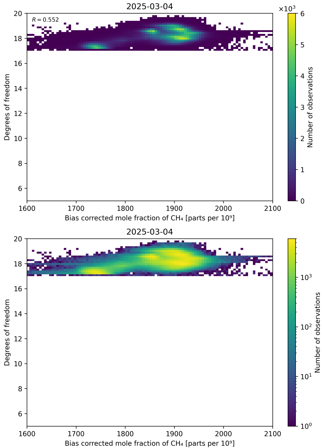
Figure 65: Scatter density plot of “Bias corrected mole fraction of CH 4 ” against “Degrees of freedom” for 2025-03-03 to 2025-03-05.
