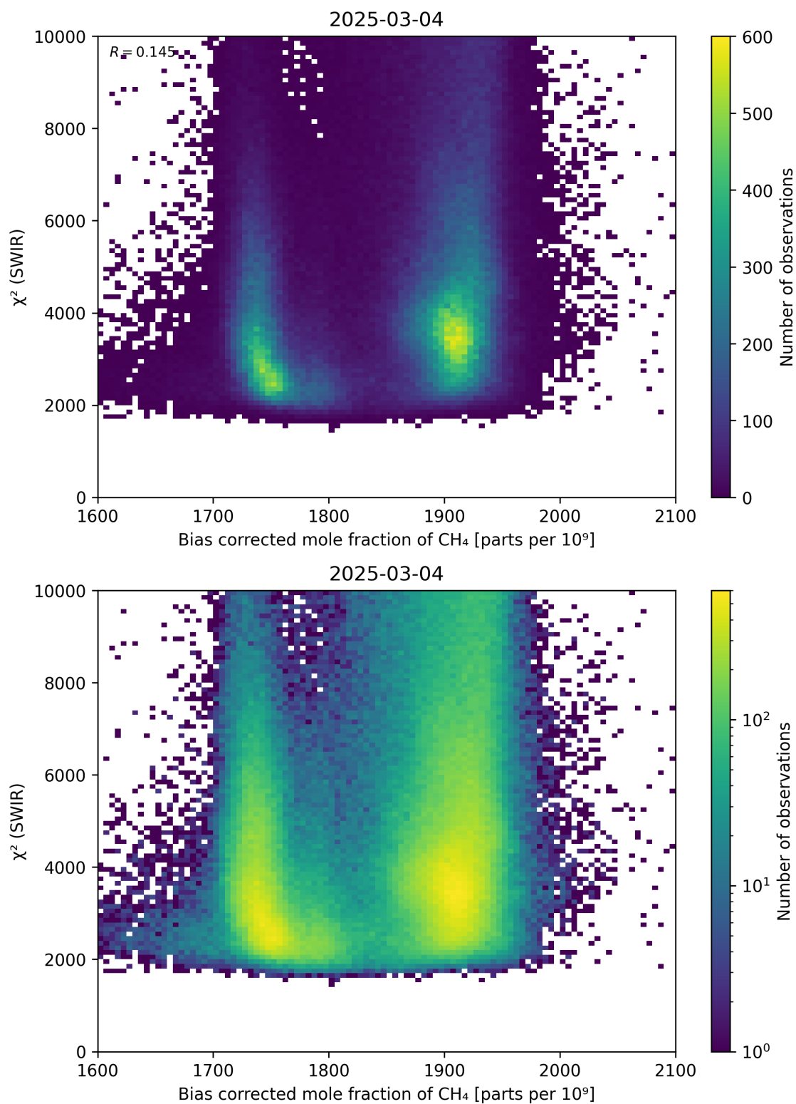
Figure 64: Scatter density plot of “Bias corrected mole fraction of \text{CH}_4 ” against “ \chi^2 (SWIR)” for 2025-03-03 to 2025-03-05.
