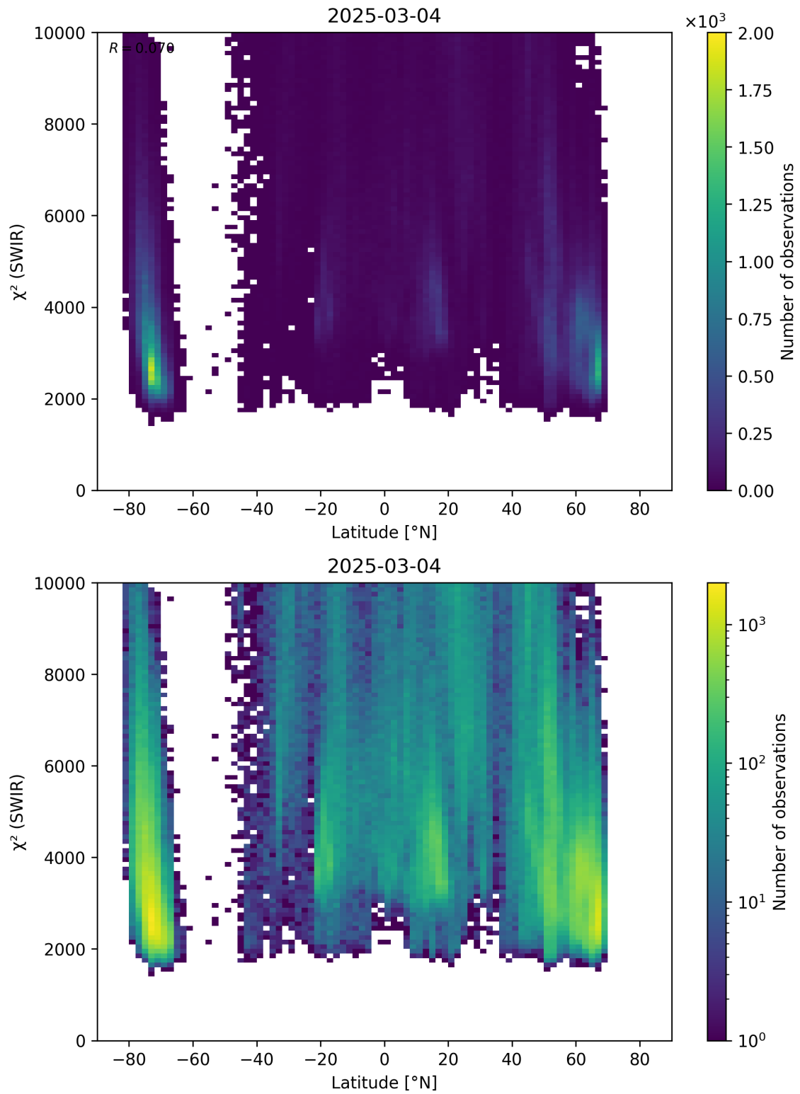
Figure 54: Scatter density plot of “Latitude” against “ \chi^2 (SWIR)” for 2025-03-03 to 2025-03-05.
