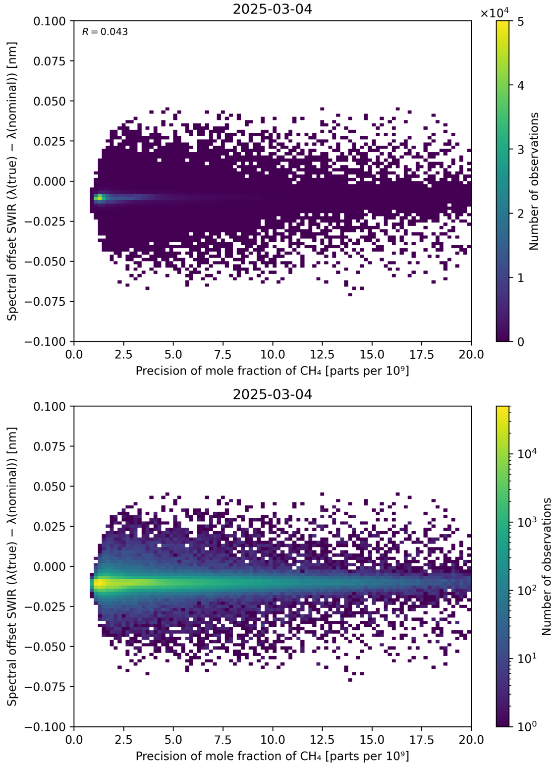
Figure 85: Scatter density plot of “Precision of mole fraction of CH 4 ” against “Spectral offset SWIR ( \lambda_{\text{true}} - \lambda_{\text{nominal}} )” for 2025-03-03 to 2025-03-05.
