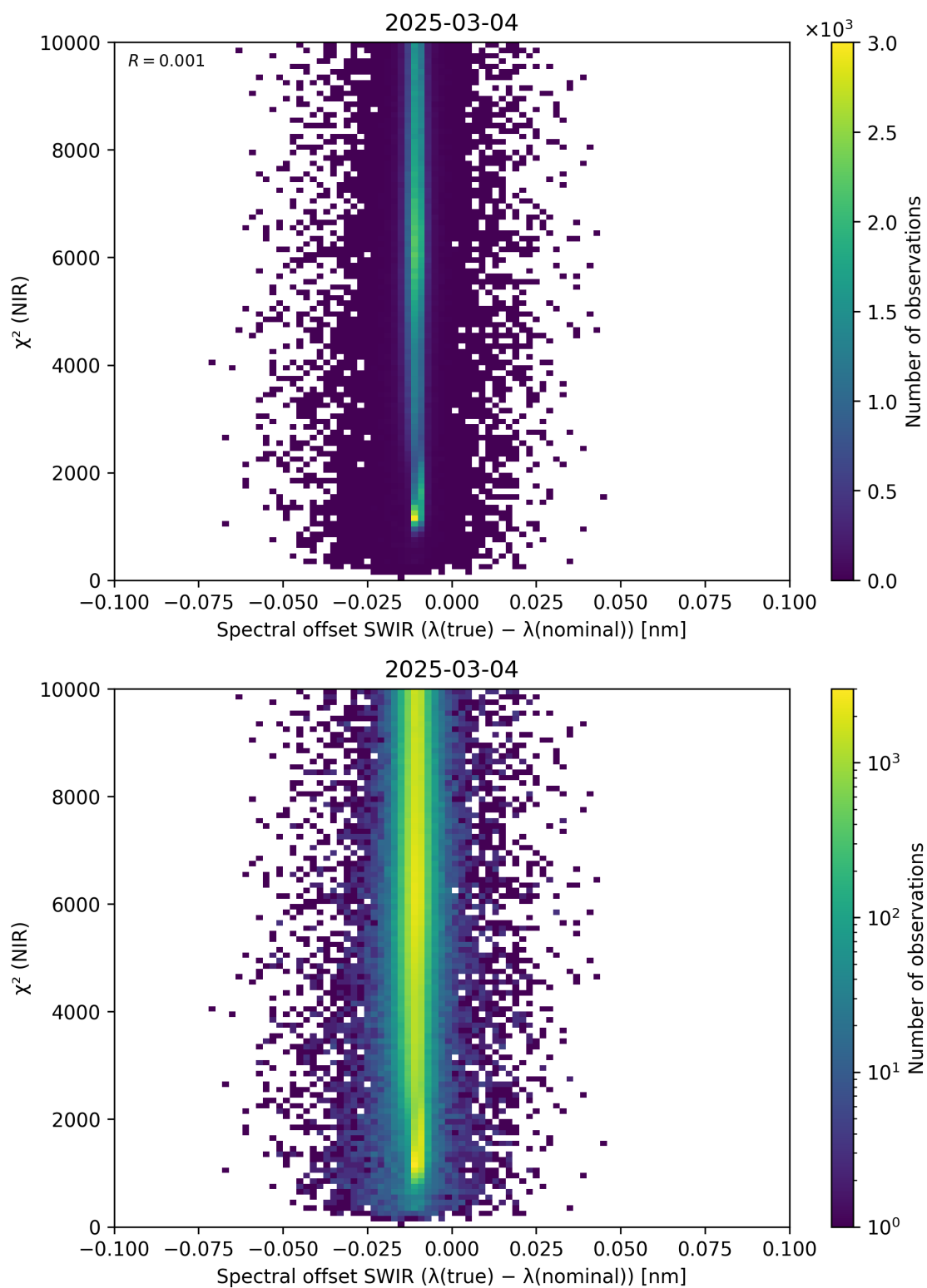
Figure 117: Scatter density plot of “Spectral offset SWIR ( \lambda_{\text{true}} - \lambda_{\text{nominal}} )” against “ \chi^2 (NIR)” for 2025-03-03 to 2025-03-05.
