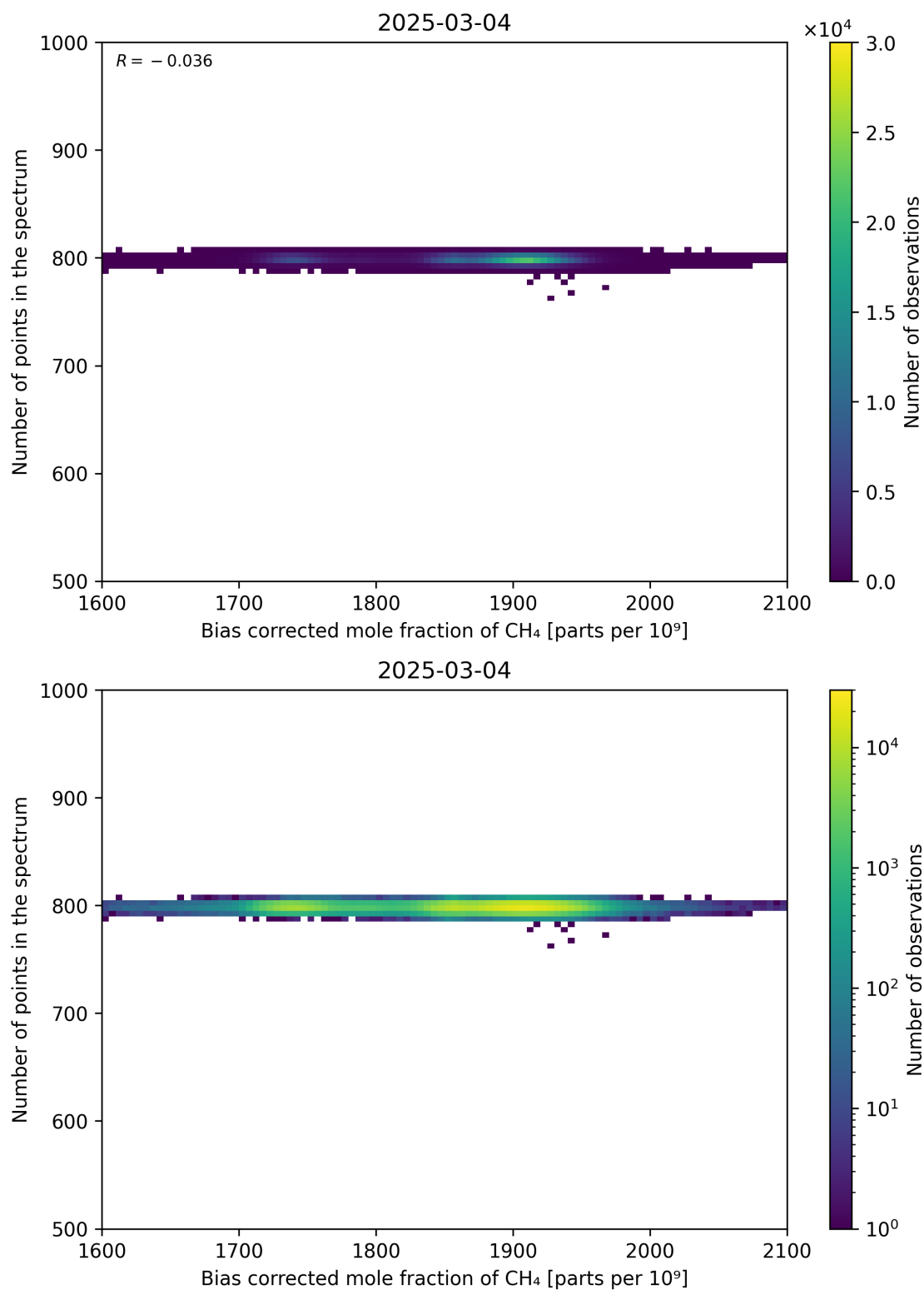
Figure 68: Scatter density plot of “Bias corrected mole fraction of CH 4 ” against “Number of points in the spectrum” for 2025-03-03 to 2025-03-05.
