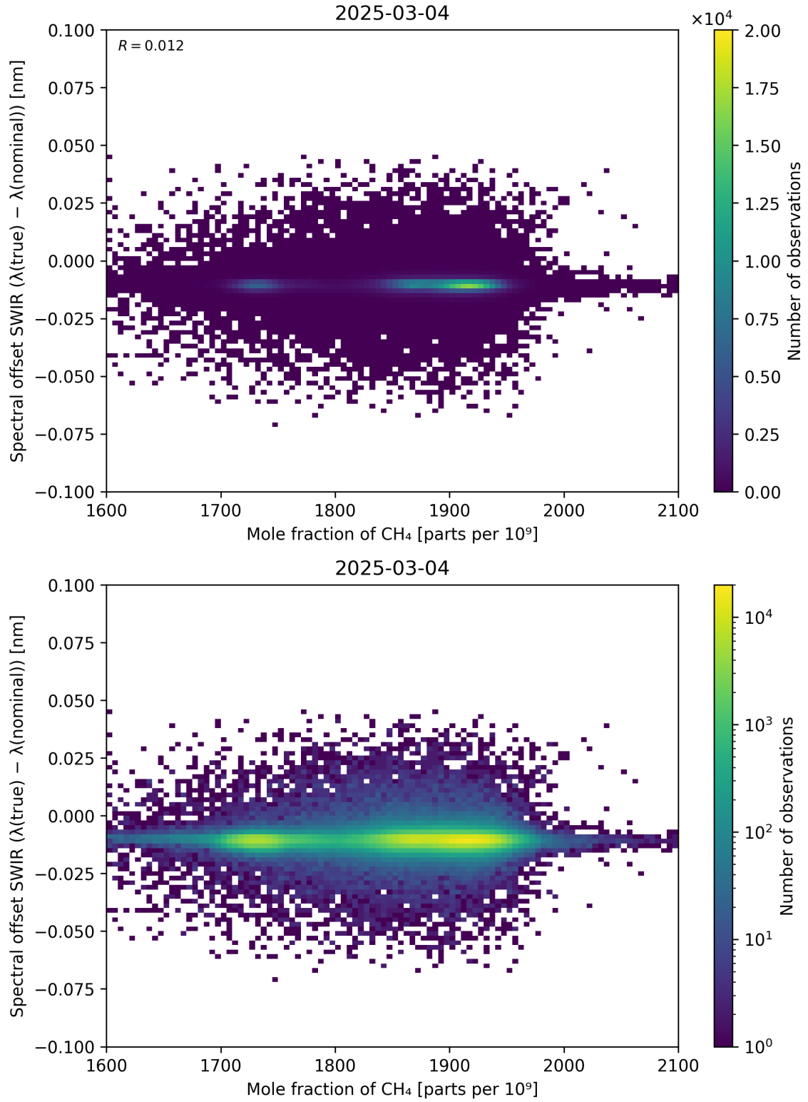
Figure 86: Scatter density plot of “Mole fraction of \text{CH}_4 ” against “Spectral offset SWIR ( \lambda_{\text{true}} - \lambda_{\text{nominal}} )” for 2025-03-03 to 2025-03-05.
