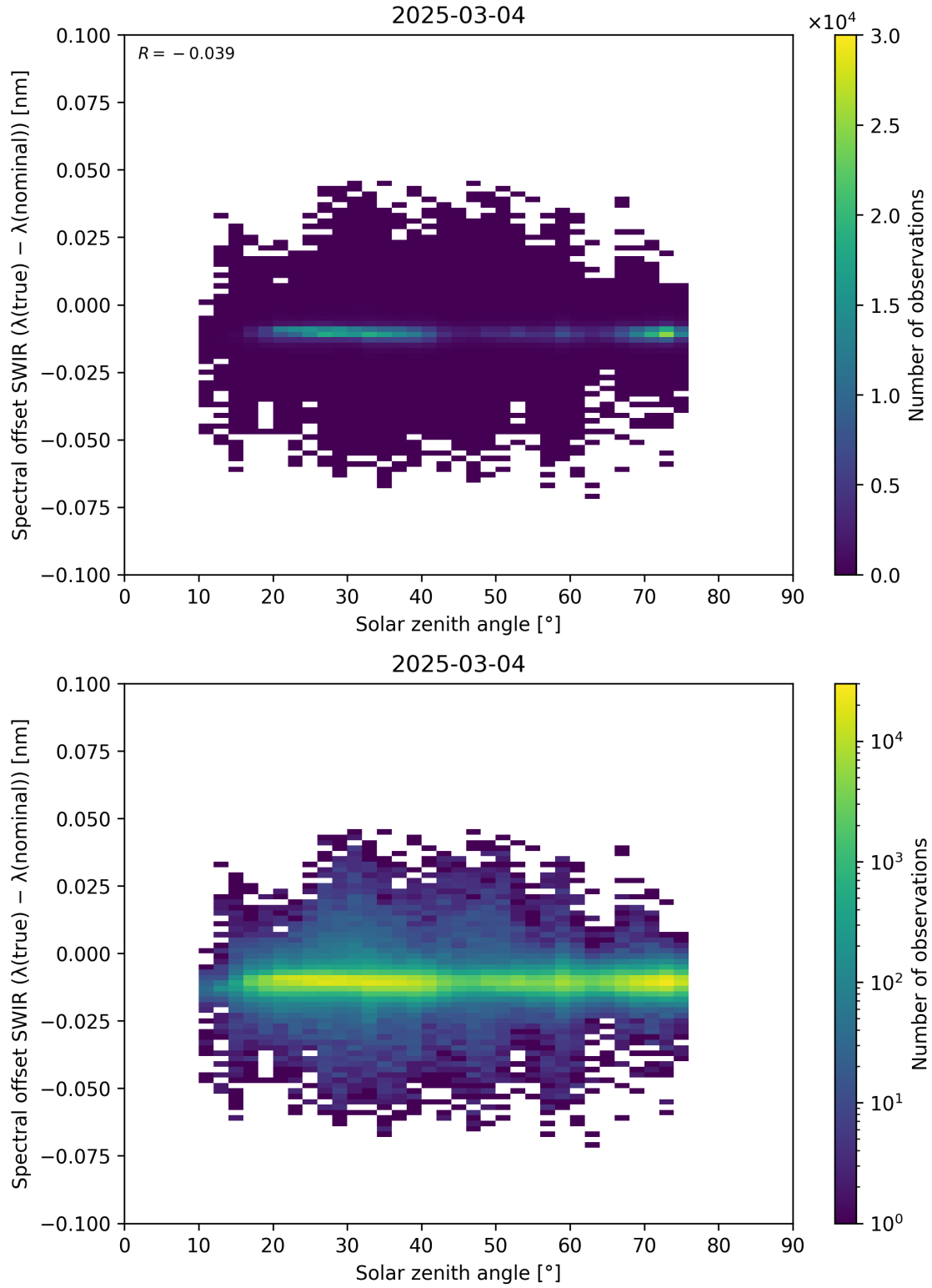
Figure 104: Scatter density plot of “Solar zenith angle” against “Spectral offset SWIR ( \lambda_{\text{true}} - \lambda_{\text{nominal}} )” for 2025-03-03 to 2025-03-05.
