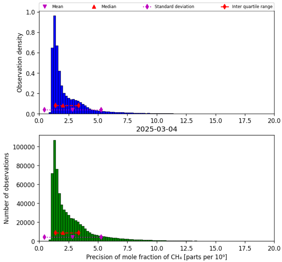
Figure 24: Histogram of “Precision of mole fraction of CH 4 ” for 2025-03-03 to 2025-03-05
