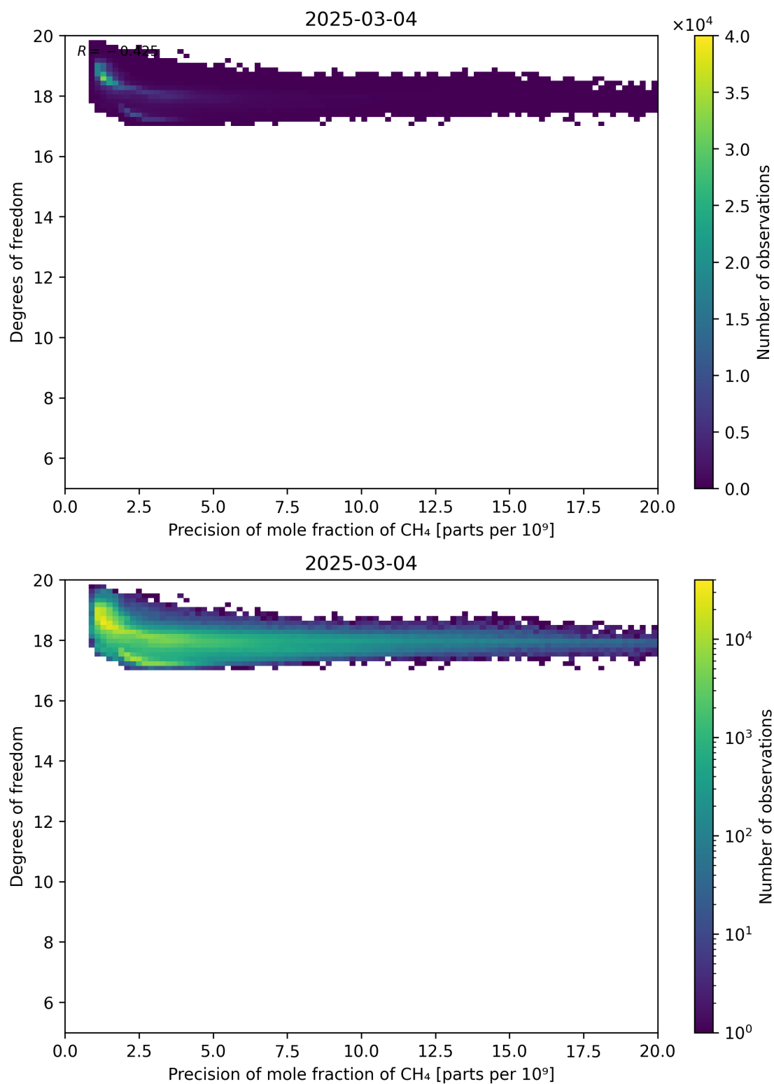
Figure 80: Scatter density plot of “Precision of mole fraction of CH 4 ” against “Degrees of freedom” for 2025-03-03 to 2025-03-05.
