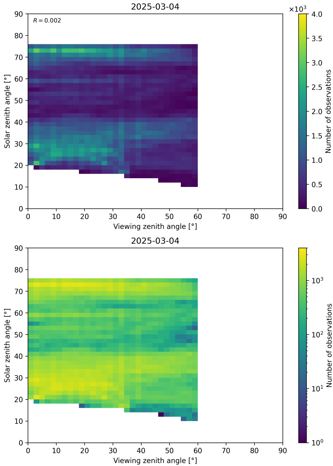
Figure 115: Scatter density plot of “Viewing zenith angle” against “Solar zenith angle” for 2025-03-03 to 2025-03-05.
