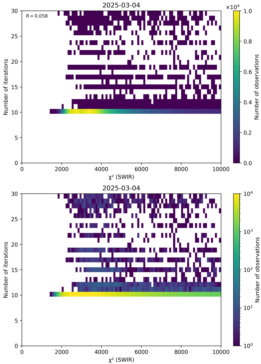
Figure 50: Scatter density plot of “ \chi^2 (SWIR)” against “Number of iterations” for 2025-03-03 to 2025-03-05.
