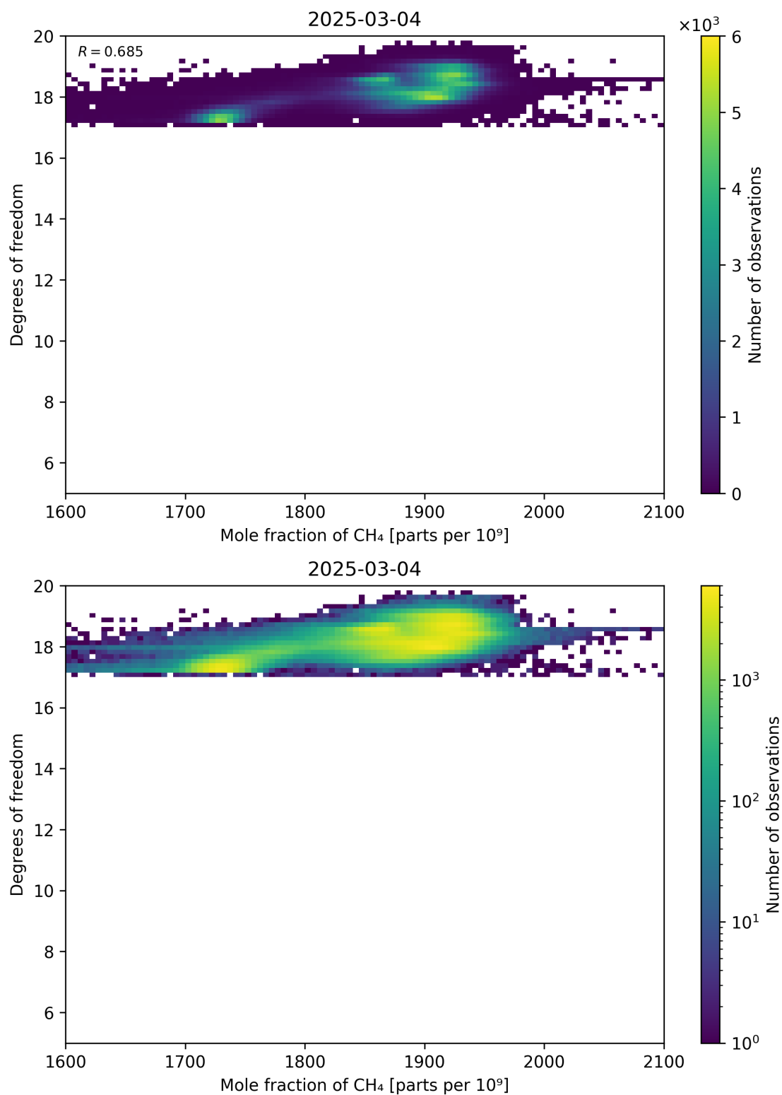
Figure 72: Scatter density plot of “Mole fraction of CH 4 ” against “Degrees of freedom” for 2025-03-03 to 2025-03-05.
