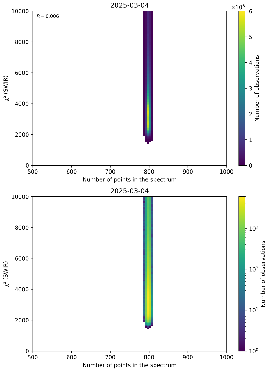
Figure 89: Scatter density plot of “Number of points in the spectrum” against “ \chi^2 (SWIR)” for 2025-03-03 to 2025-03-05.
