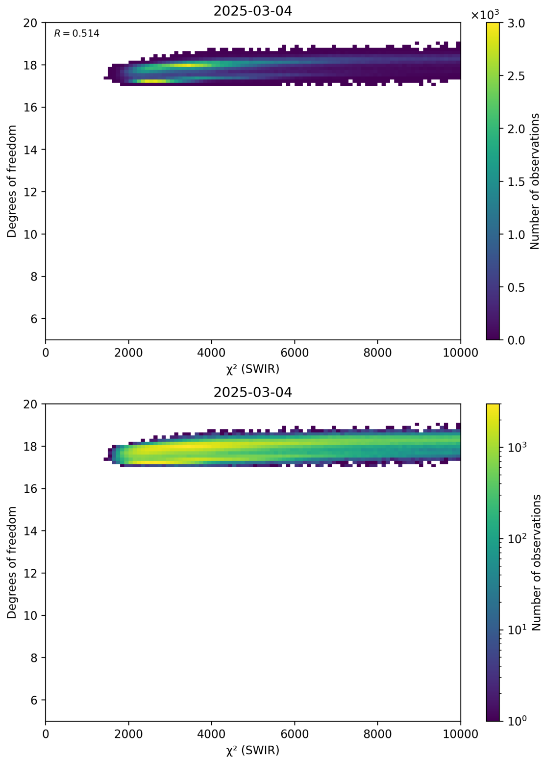
Figure 48: Scatter density plot of “ \chi^2 (SWIR)” against “Degrees of freedom” for 2025-03-03 to 2025-03-05.
