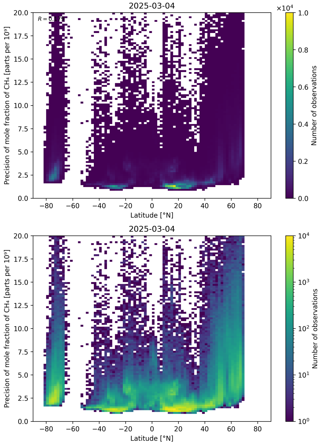
Figure 59: Scatter density plot of “Latitude” against “Precision of mole fraction of CH 4 ” for 2025-03-03 to 2025-03-05.
