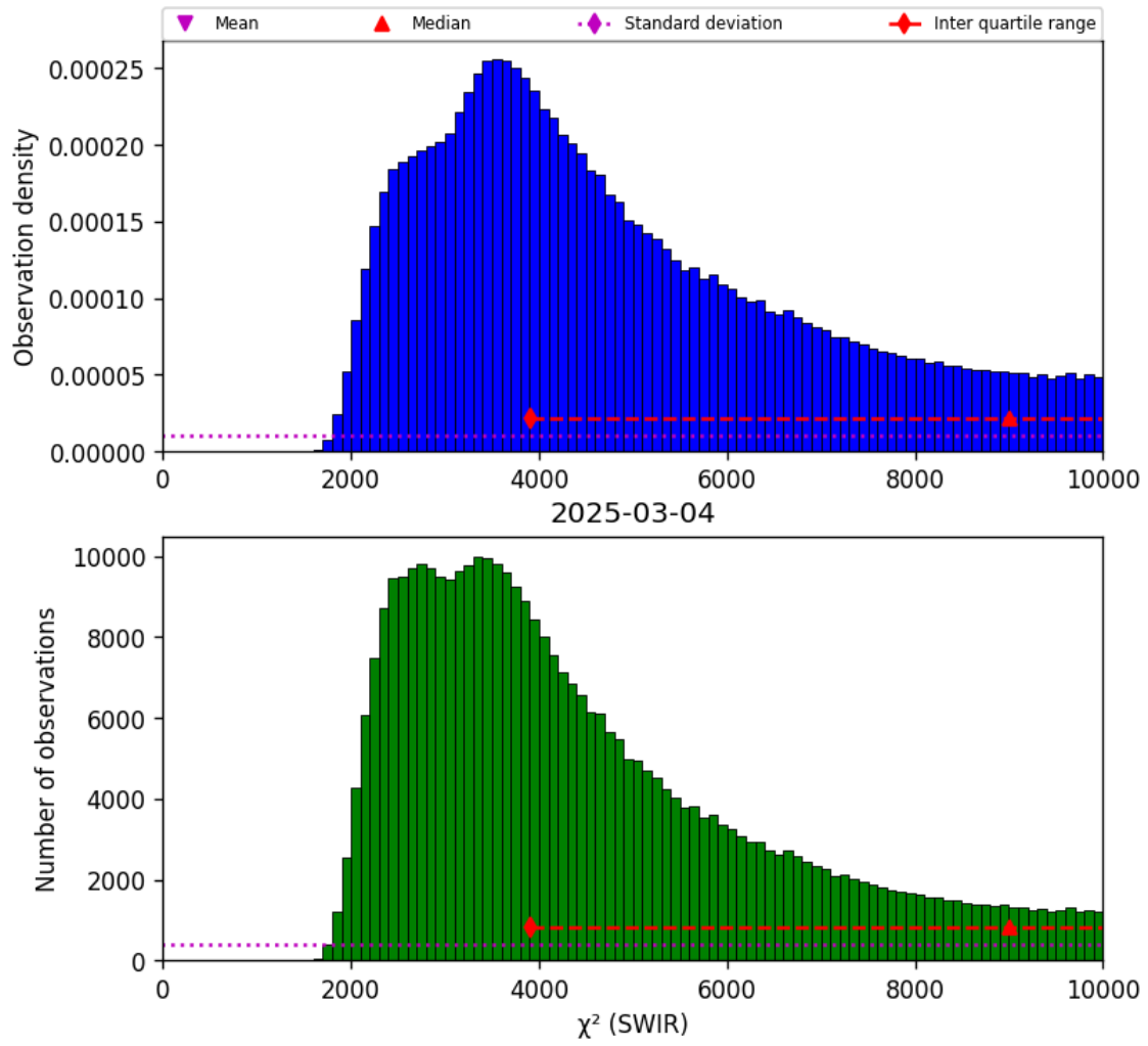
Figure 28: Histogram of " \chi^2 (SWIR)" for 2025-03-03 to 2025-03-05
