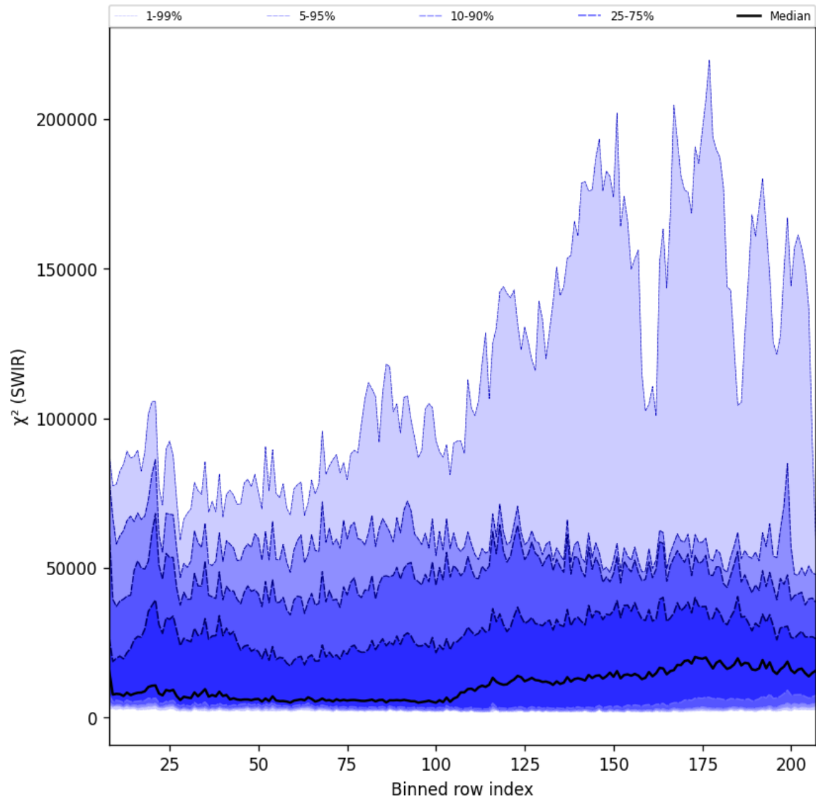
Figure 39: Along track statistics of “ \chi^2 (SWIR)” for 2025-03-03 to 2025-03-05
