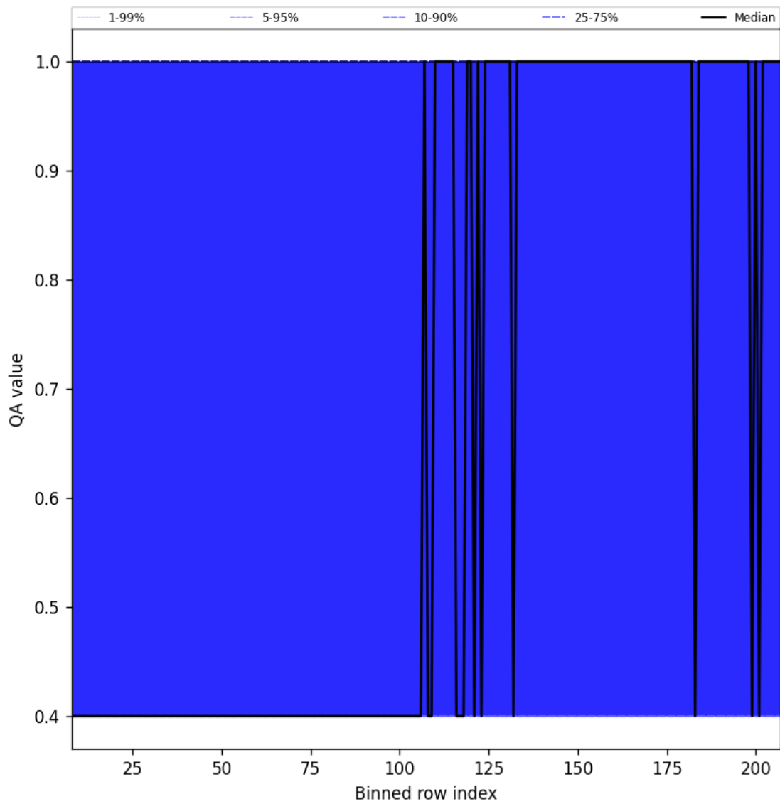
Figure 33: Along track statistics of “QA value” for 2025-03-03 to 2025-03-05
