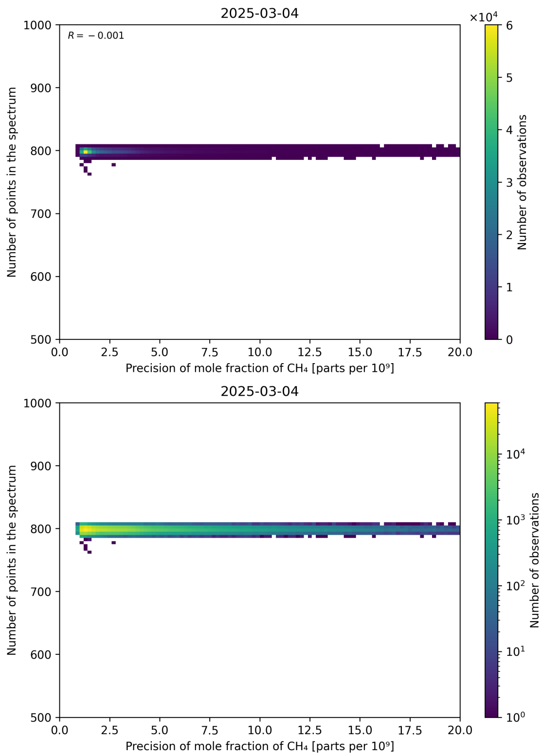
Figure 84: Scatter density plot of “Precision of mole fraction of CH 4 ” against “Number of points in the spectrum” for 2025-03-03 to 2025-03-05.
