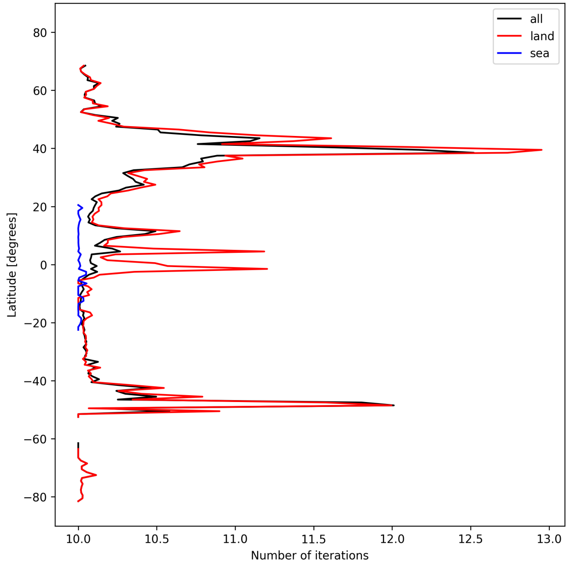
Figure 20: Zonal average of “Number of iterations” for 2025-03-03 to 2025-03-05.
