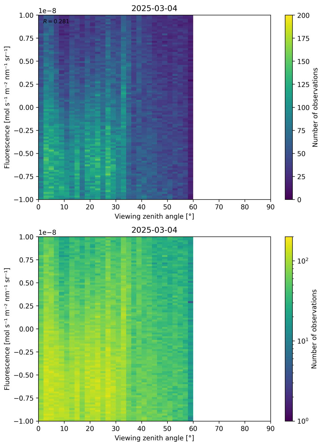
Figure 108: Scatter density plot of “Viewing zenith angle” against “Fluorescence” for 2025-03-03 to 2025-03-05.
