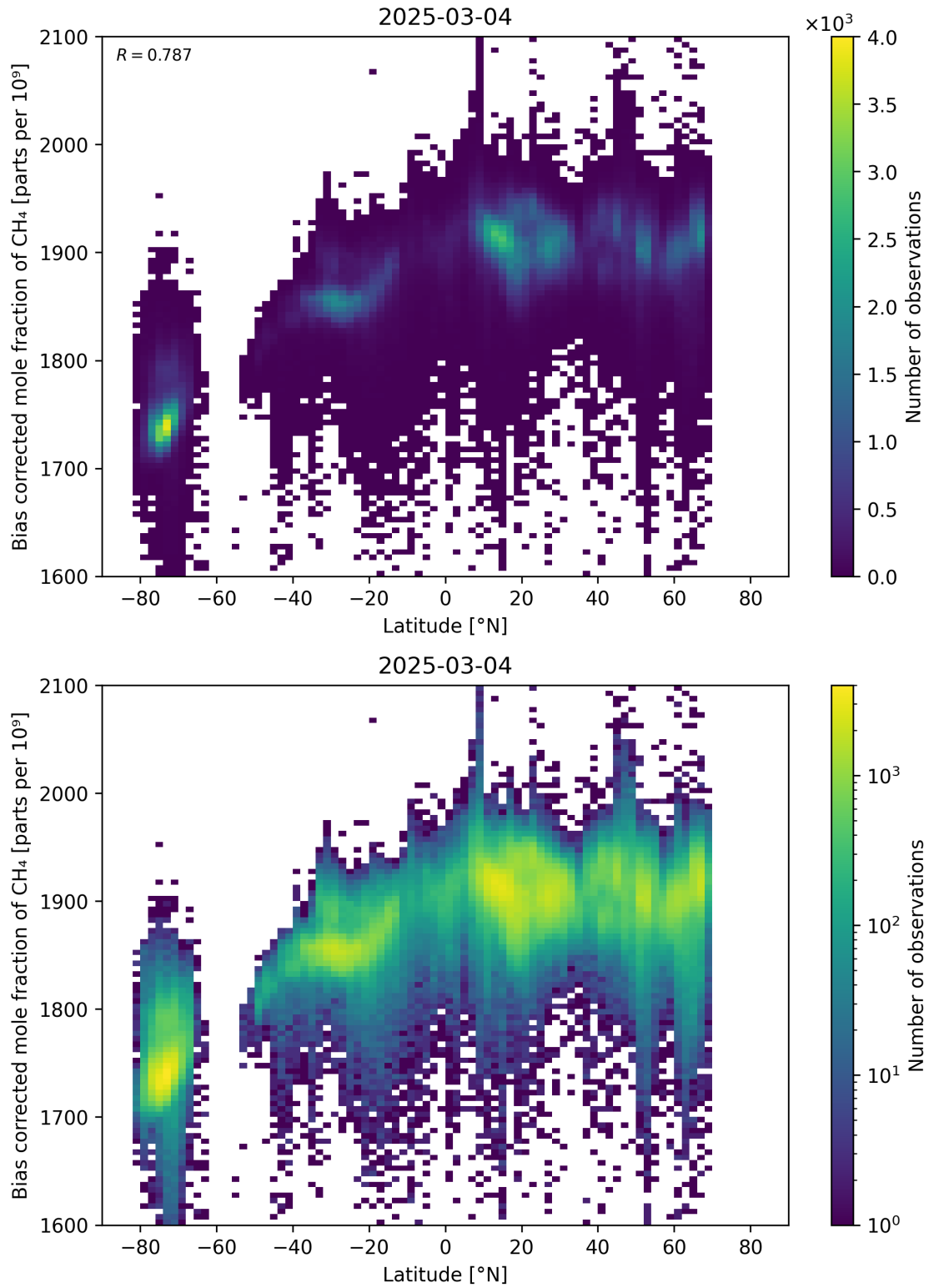
Figure 58: Scatter density plot of “Latitude” against “Bias corrected mole fraction of CH 4 ” for 2025-03-03 to 2025-03-05.
