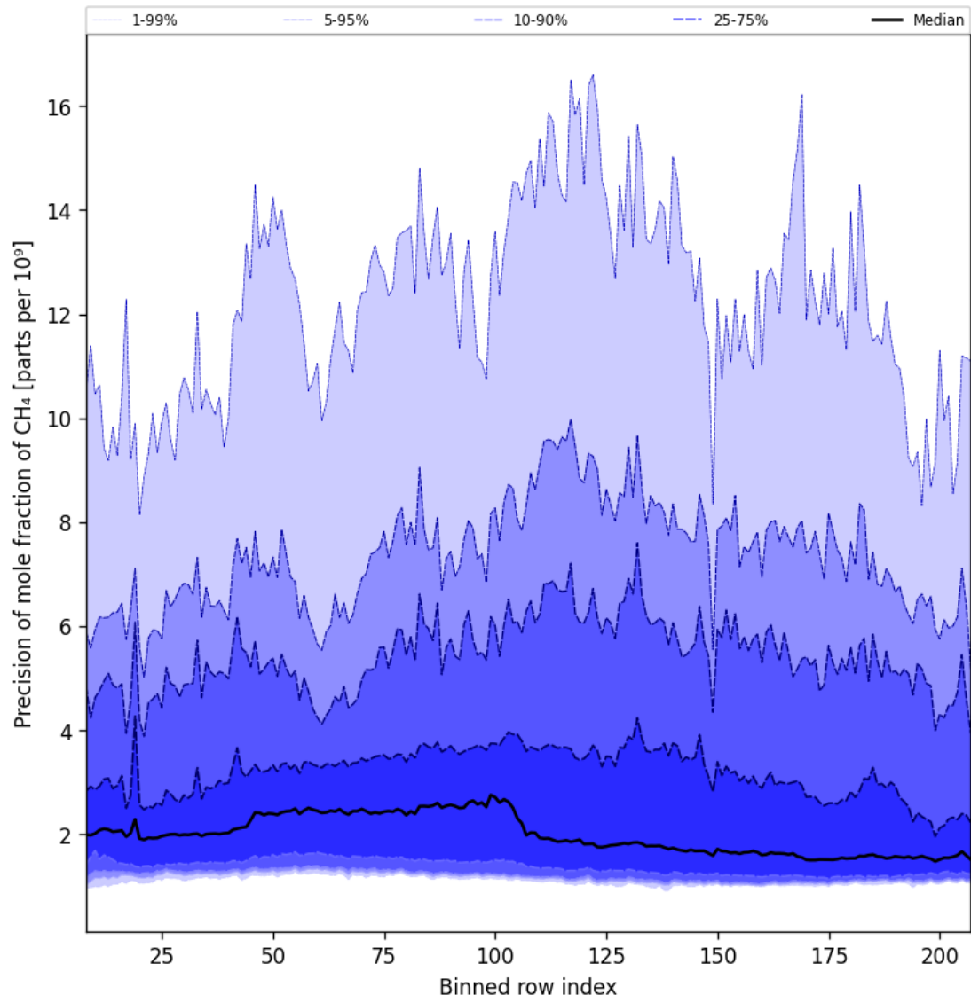
Figure 35: Along track statistics of “Precision of mole fraction of CH 4 ” for 2025-03-03 to 2025-03-05
