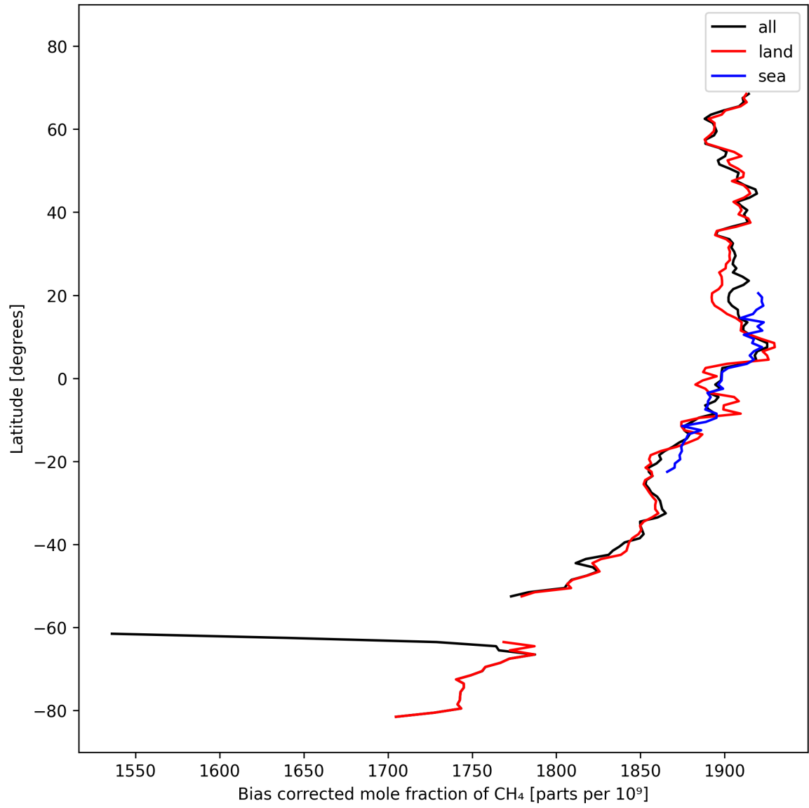
Figure 14: Zonal average of “Bias corrected mole fraction of \text{CH}_4 ” for 2025-03-03 to 2025-03-05.
