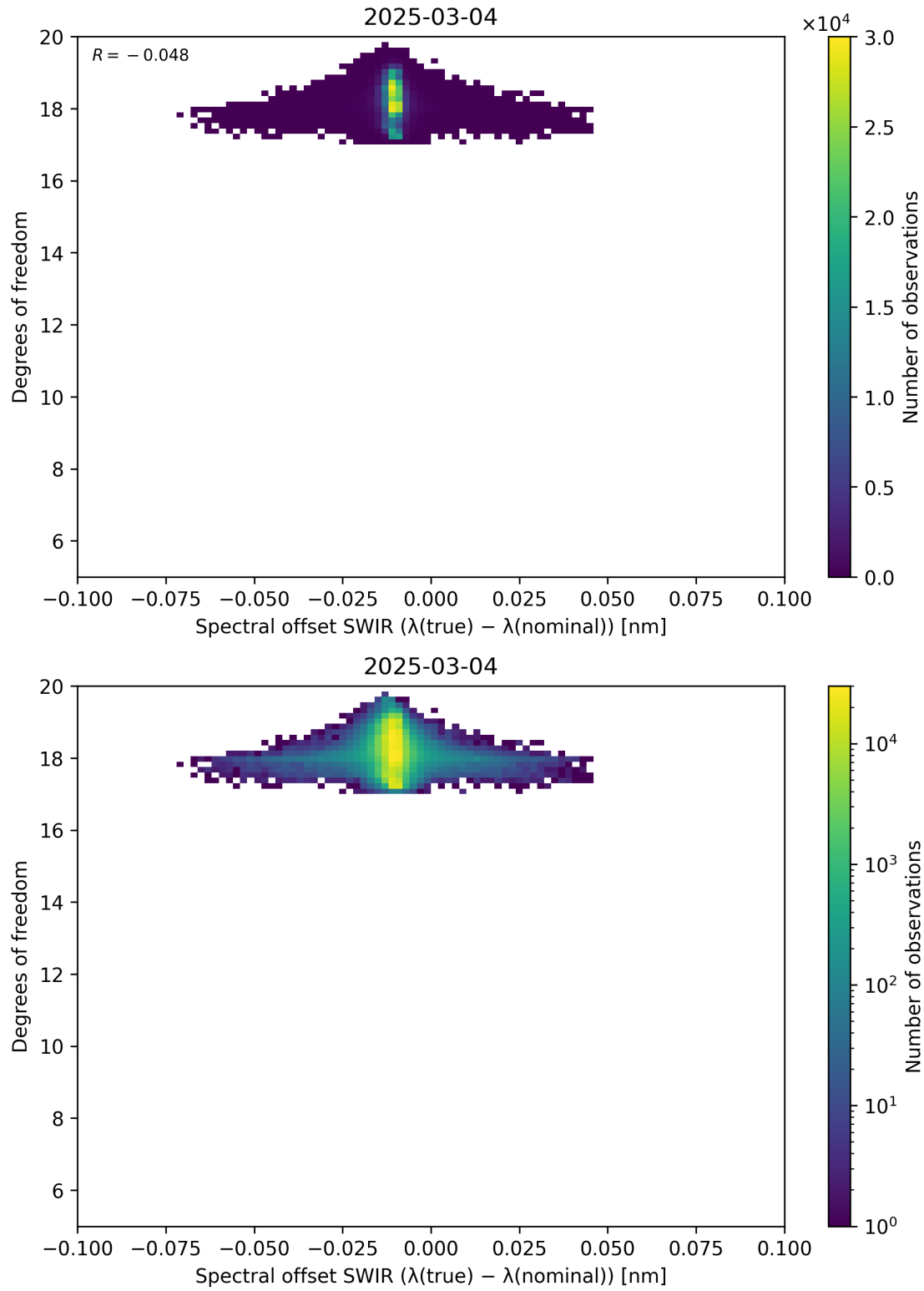
Figure 119: Scatter density plot of “Spectral offset SWIR ( \lambda_{\text{true}} - \lambda_{\text{nominal}} )” against “Degrees of freedom” for 2025-03-03 to 2025-03-05.
