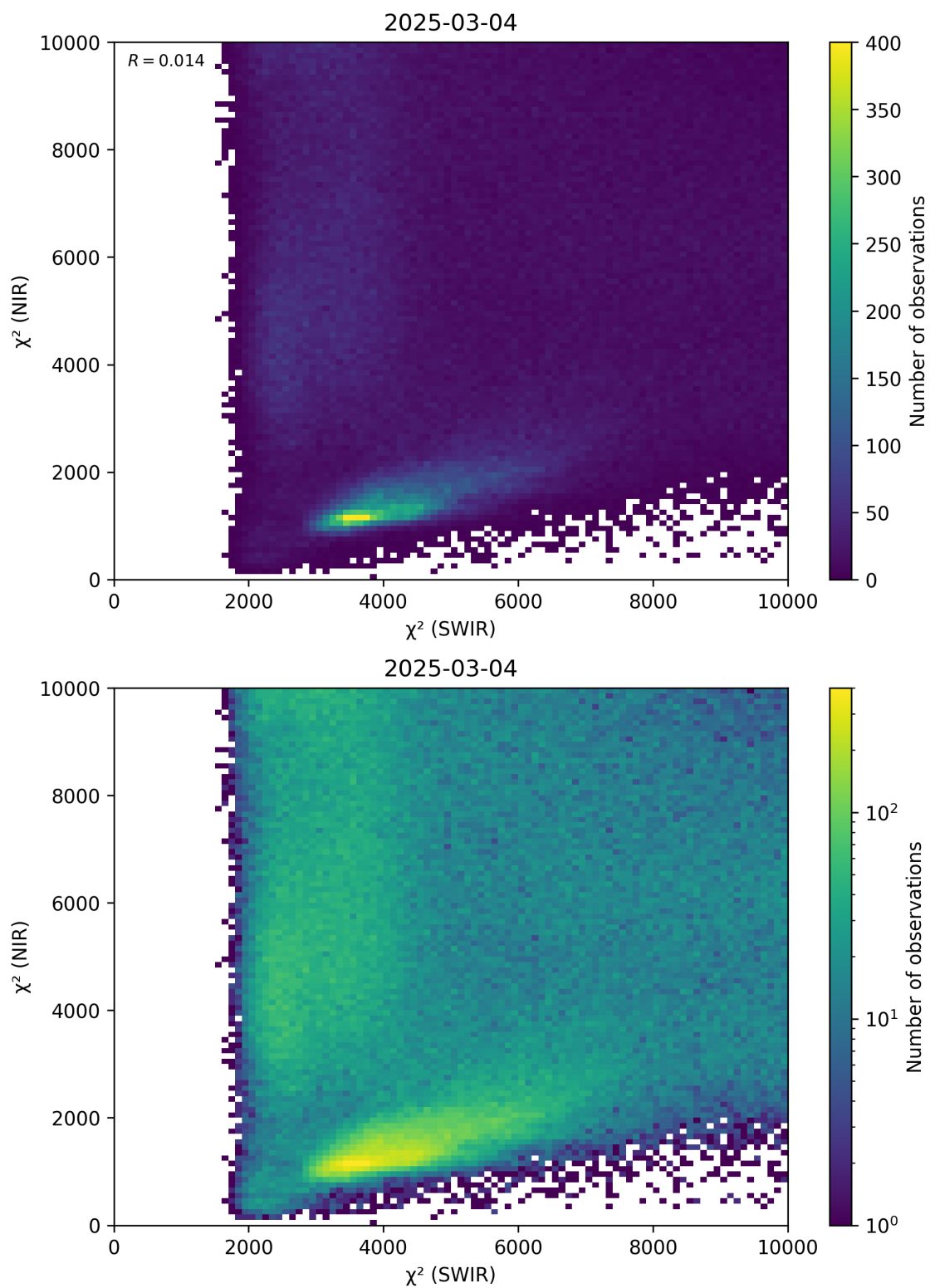
Figure 47: Scatter density plot of “ \chi^2 (SWIR)” against “ \chi^2 (NIR)” for 2025-03-03 to 2025-03-05.
