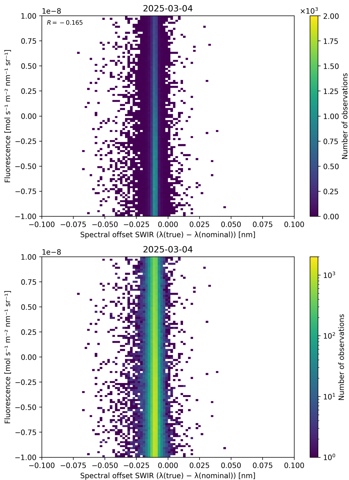
Figure 120: Scatter density plot of “Spectral offset SWIR ( \lambda_{\text{true}} - \lambda_{\text{nominal}} )” against “Fluorescence” for 2025-03-03 to 2025-03-05.
