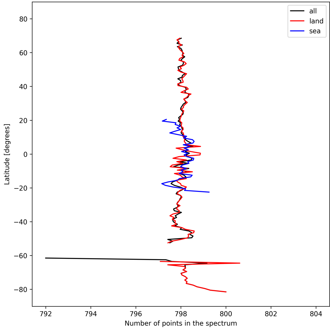
Figure 15: Zonal average of “Number of points in the spectrum” for 2025-03-03 to 2025-03-05.
