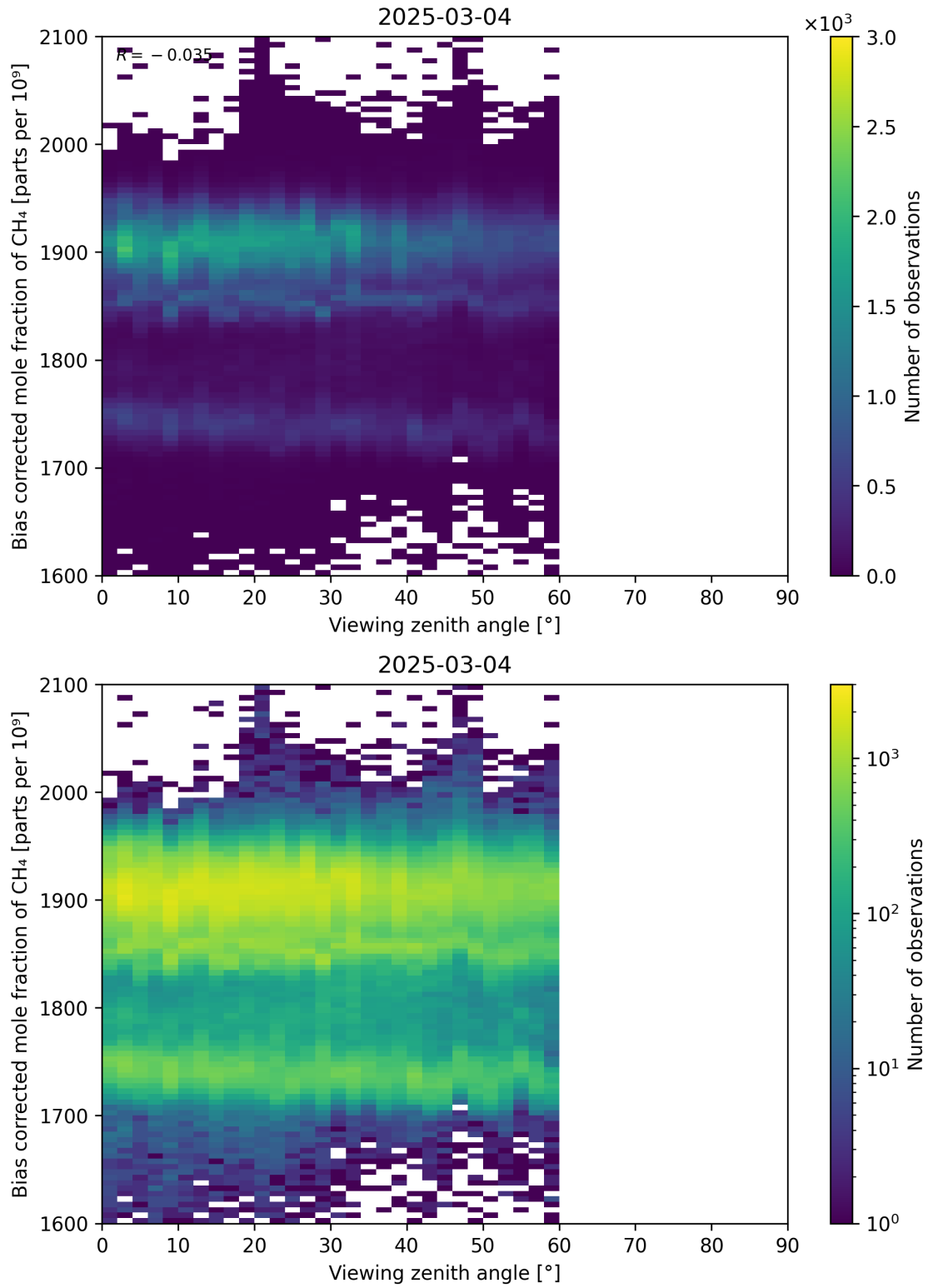
Figure 111: Scatter density plot of “Viewing zenith angle” against “Bias corrected mole fraction of CH 4 ” for 2025-03-03 to 2025-03-05.
