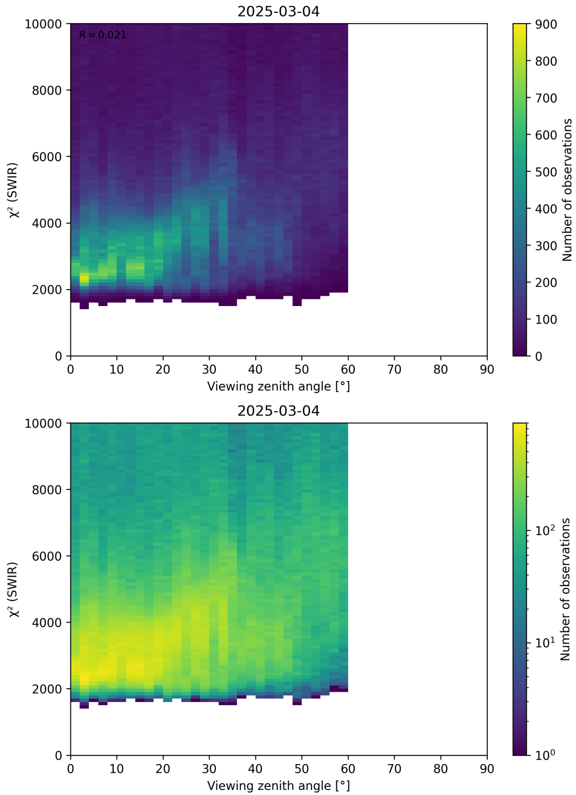
Figure 106: Scatter density plot of “Viewing zenith angle” against “ \chi^2 (SWIR)” for 2025-03-03 to 2025-03-05.
