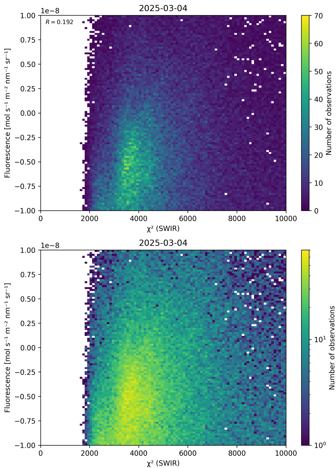
Figure 49: Scatter density plot of “ \chi^2 (SWIR)” against “Fluorescence” for 2025-03-03 to 2025-03-05.
