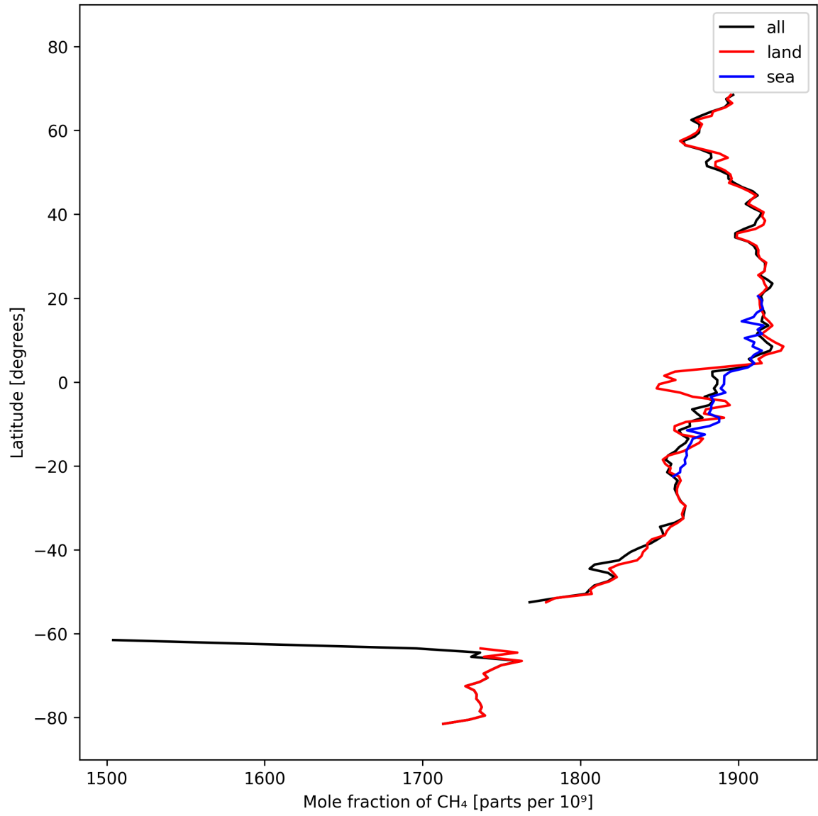
Figure 12: Zonal average of “Mole fraction of \text{CH}_4 ” for 2025-03-03 to 2025-03-05.
