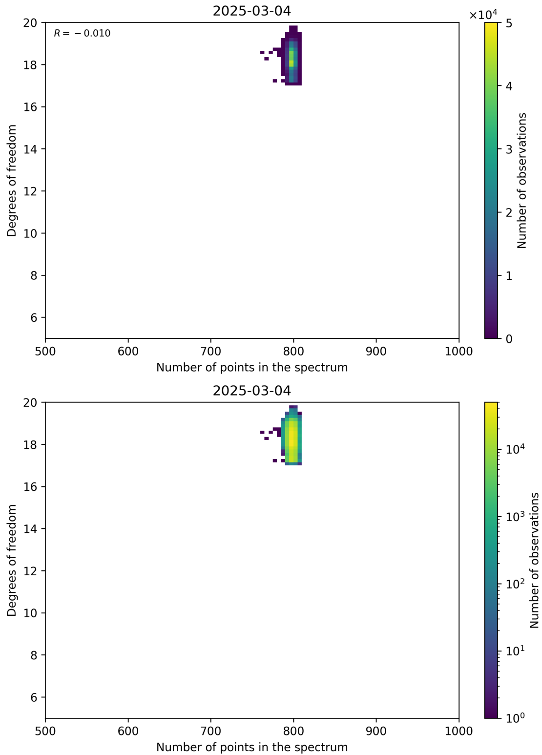
Figure 90: Scatter density plot of “Number of points in the spectrum” against “Degrees of freedom” for 2025-03-03 to 2025-03-05.
