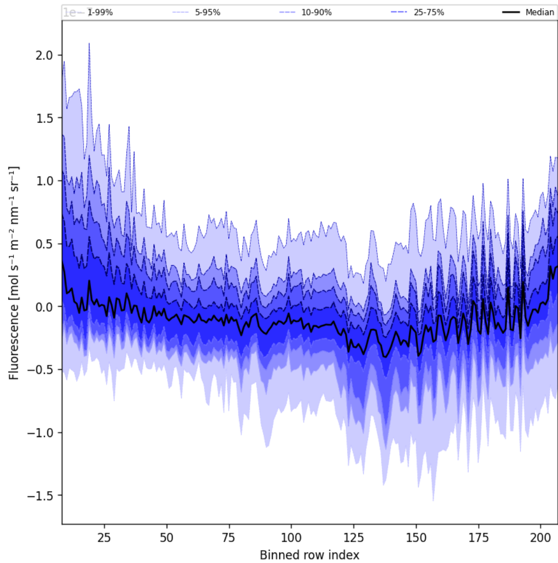
Figure 43: Along track statistics of “Fluorescence” for 2025-03-03 to 2025-03-05
