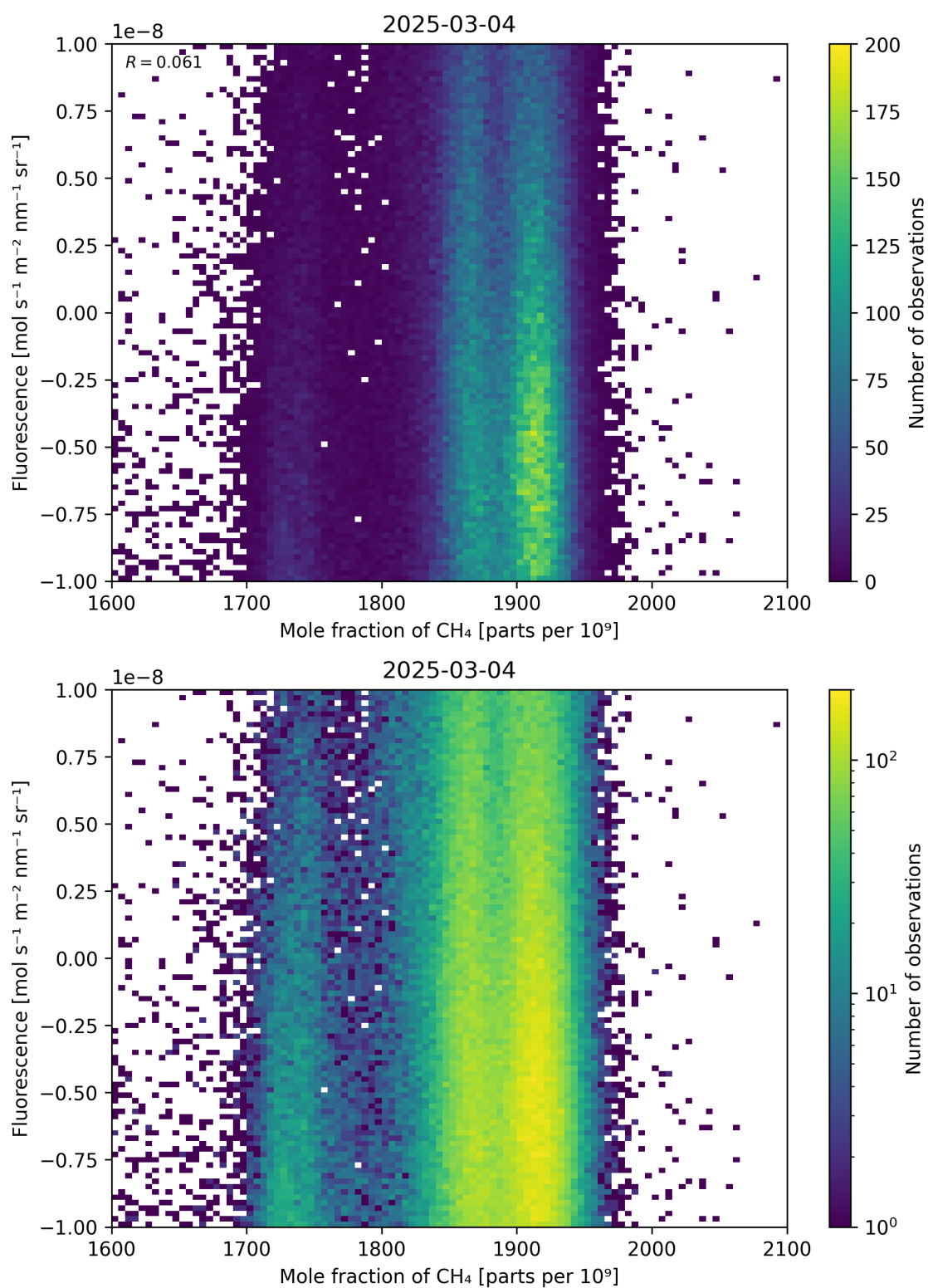
Figure 73: Scatter density plot of “Mole fraction of \text{CH}_4 ” against “Fluorescence” for 2025-03-03 to 2025-03-05.
