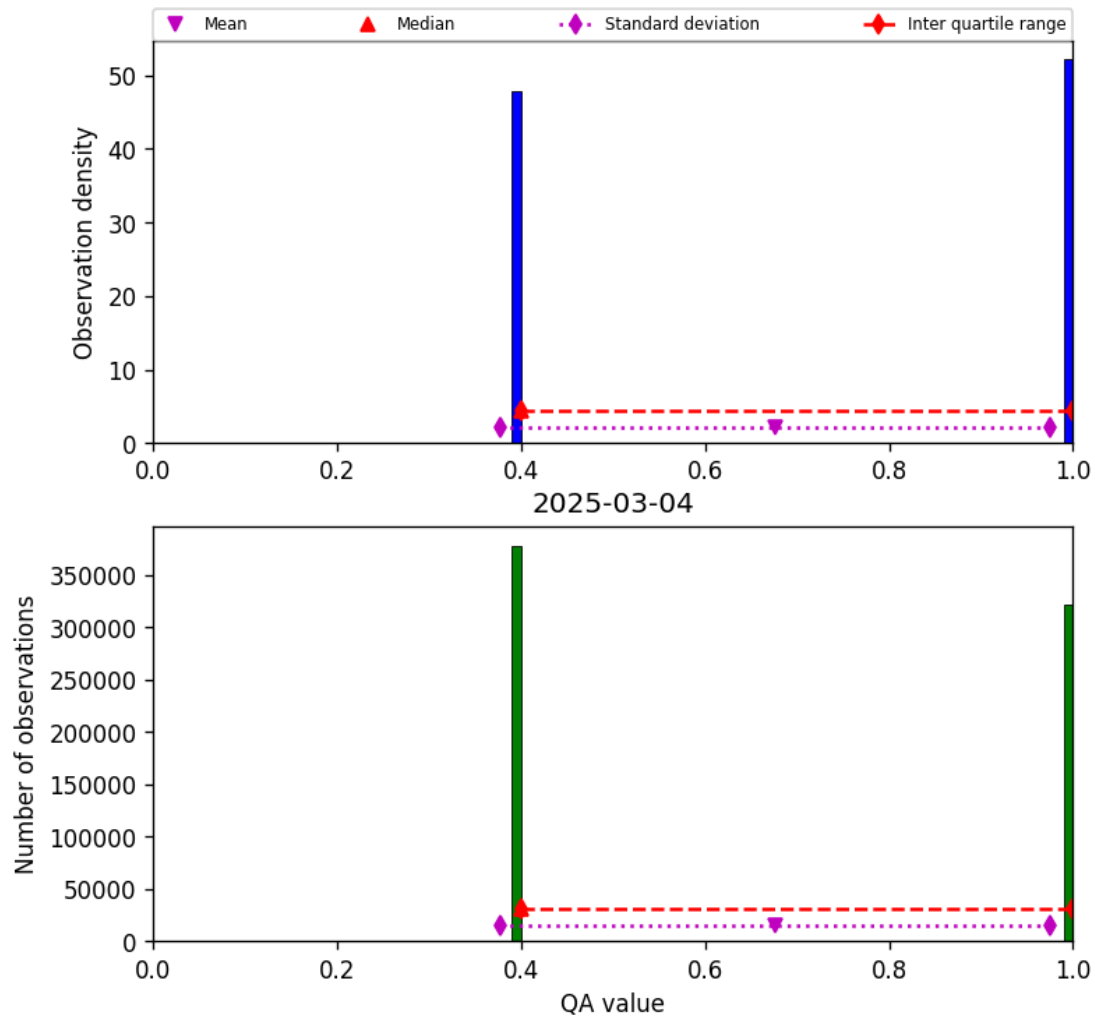
Figure 22: Histogram of “QA value” for 2025-03-03 to 2025-03-05
