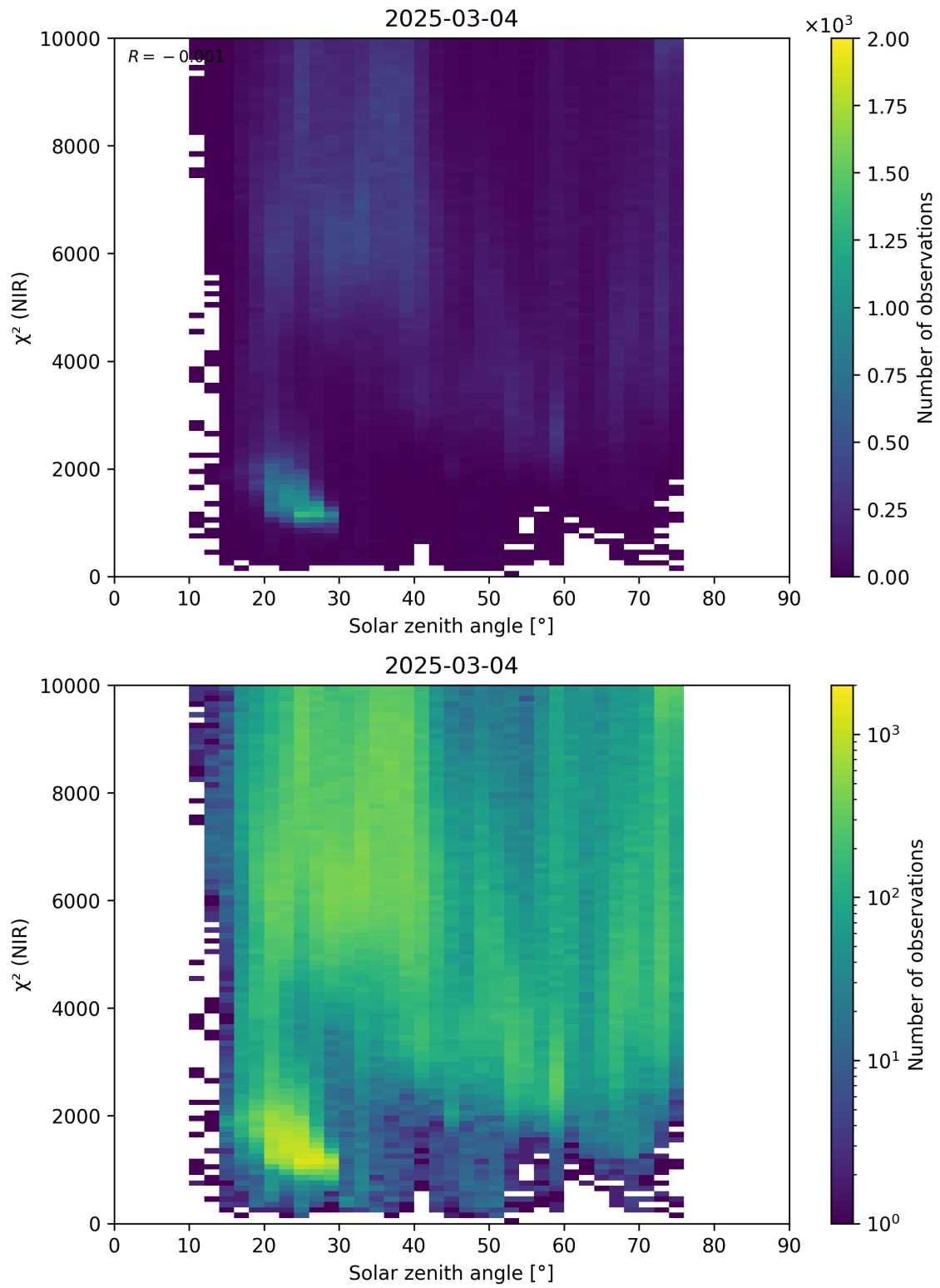
Figure 94: Scatter density plot of “Solar zenith angle” against “ \chi^2 (NIR)” for 2025-03-03 to 2025-03-05.
