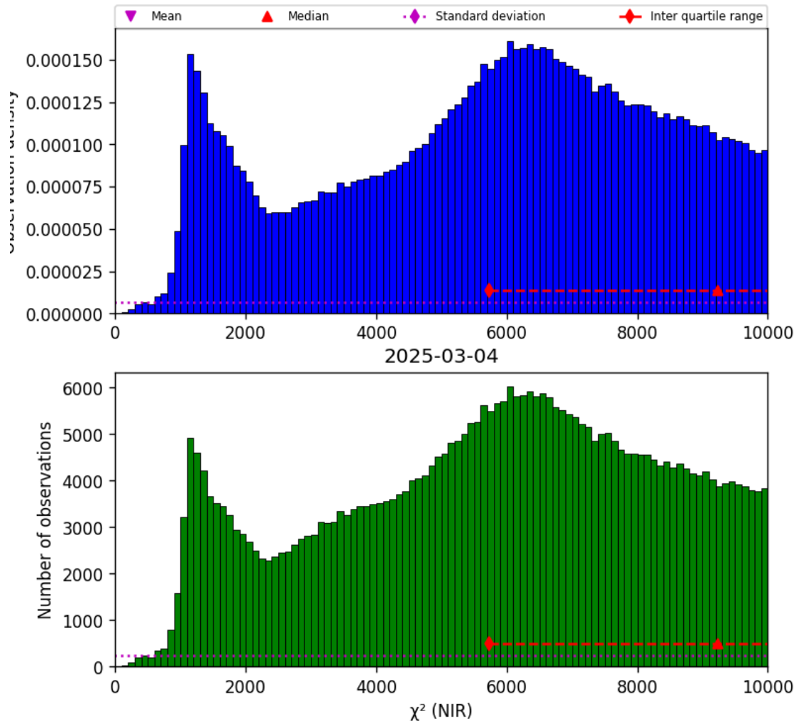
Figure 29: Histogram of “ \chi^2 (NIR)” for 2025-03-03 to 2025-03-05
