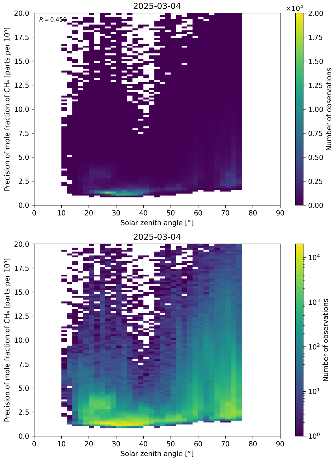
Figure 101: Scatter density plot of “Solar zenith angle” against “Precision of mole fraction of CH 4 ” for 2025-03-03 to 2025-03-05.
