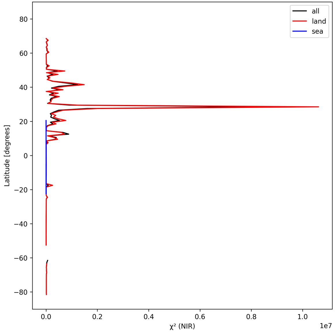
Figure 18: Zonal average of “ \chi^2 (NIR)” for 2025-03-03 to 2025-03-05.
