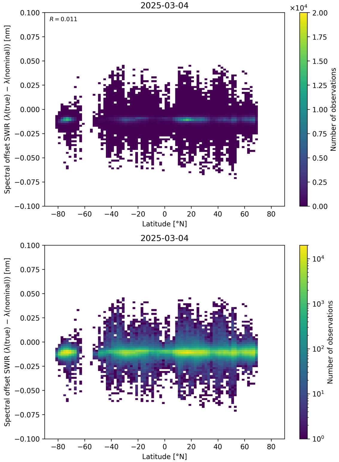
Figure 62: Scatter density plot of “Latitude” against “Spectral offset SWIR ( \lambda_{\text{true}} - \lambda_{\text{nominal}} )” for 2025-03-03 to 2025-03-05.
