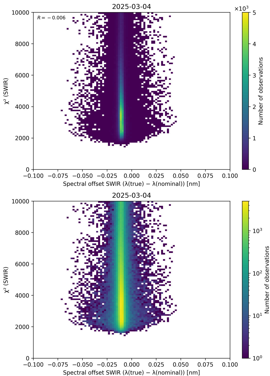
Figure 118: Scatter density plot of “Spectral offset SWIR ( \lambda_{\text{true}} - \lambda_{\text{nominal}} )” against “ \chi^2 (SWIR)” for 2025-03-03 to 2025-03-05.
