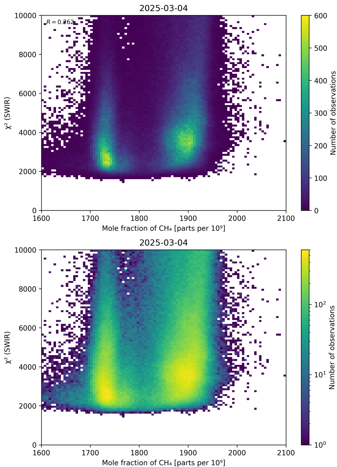
Figure 71: Scatter density plot of “Mole fraction of CH 4 ” against “ \chi^2 (SWIR)” for 2025-03-03 to 2025-03-05.
