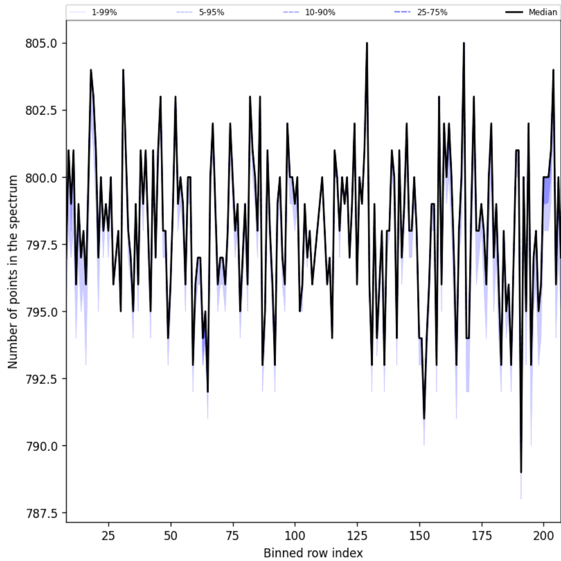
Figure 37: Along track statistics of “Number of points in the spectrum” for 2025-03-03 to 2025-03-05
