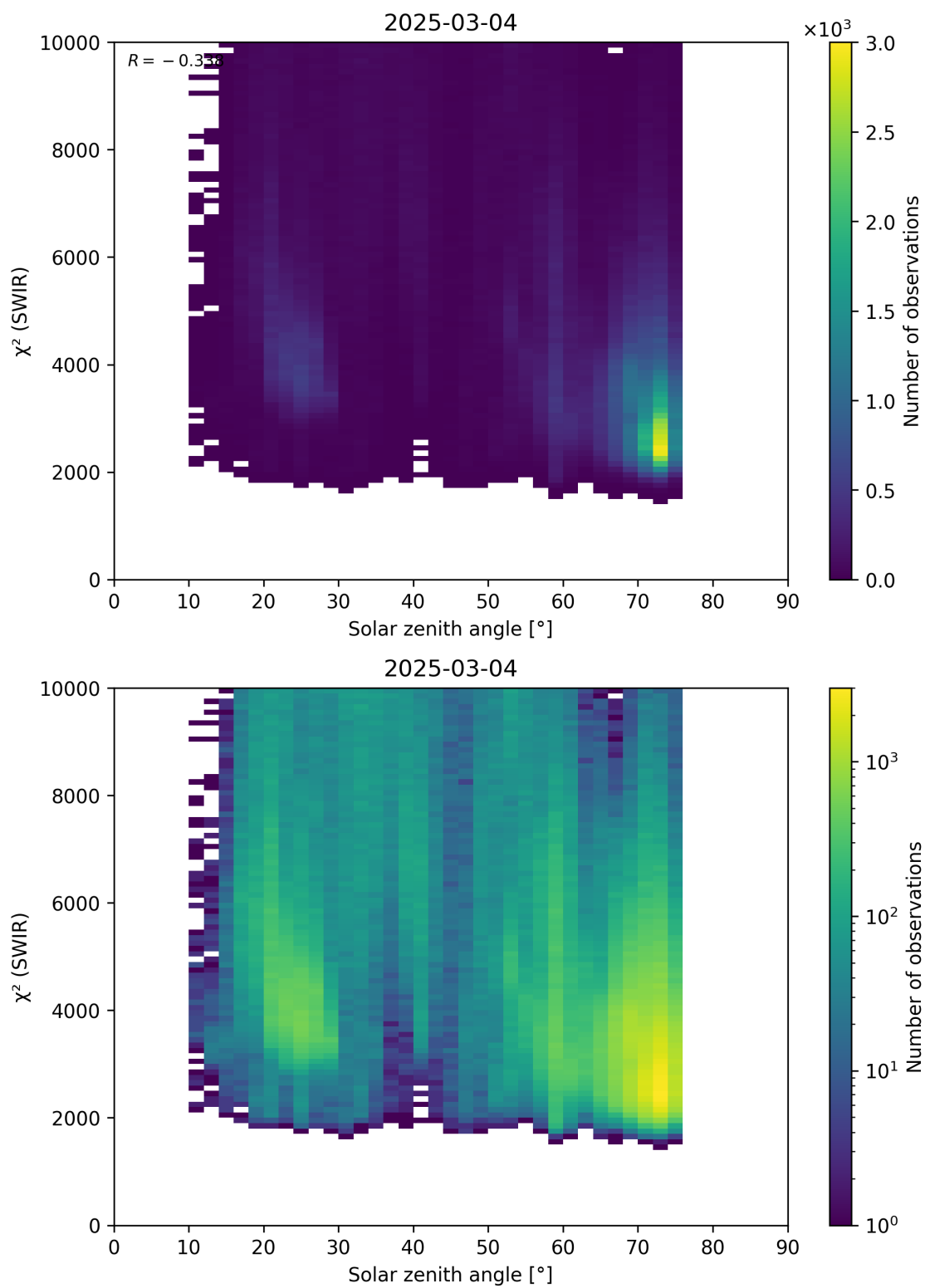
Figure 95: Scatter density plot of “Solar zenith angle” against “ \chi^2 (SWIR)” for 2025-03-03 to 2025-03-05.
