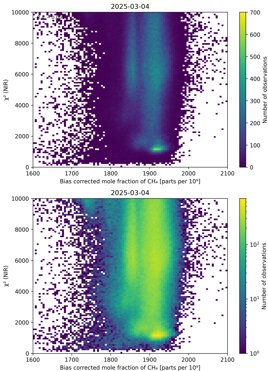
Figure 63: Scatter density plot of “Bias corrected mole fraction of \text{CH}_4 ” against “ \chi^2 (NIR)” for 2025-03-03 to 2025-03-05.
