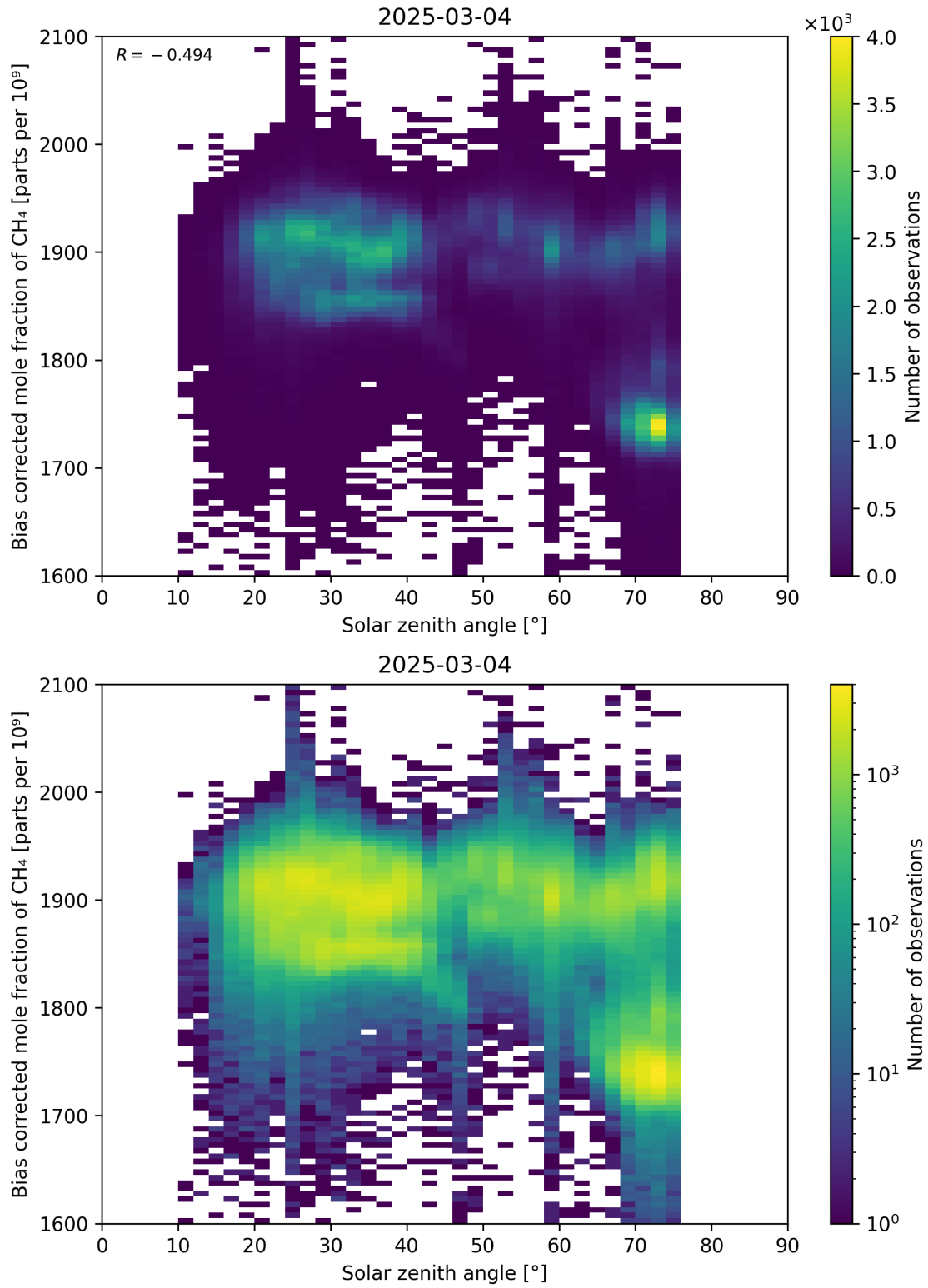
Figure 100: Scatter density plot of “Solar zenith angle” against “Bias corrected mole fraction of \text{CH}_4 ” for 2025-03-03 to 2025-03-05.
