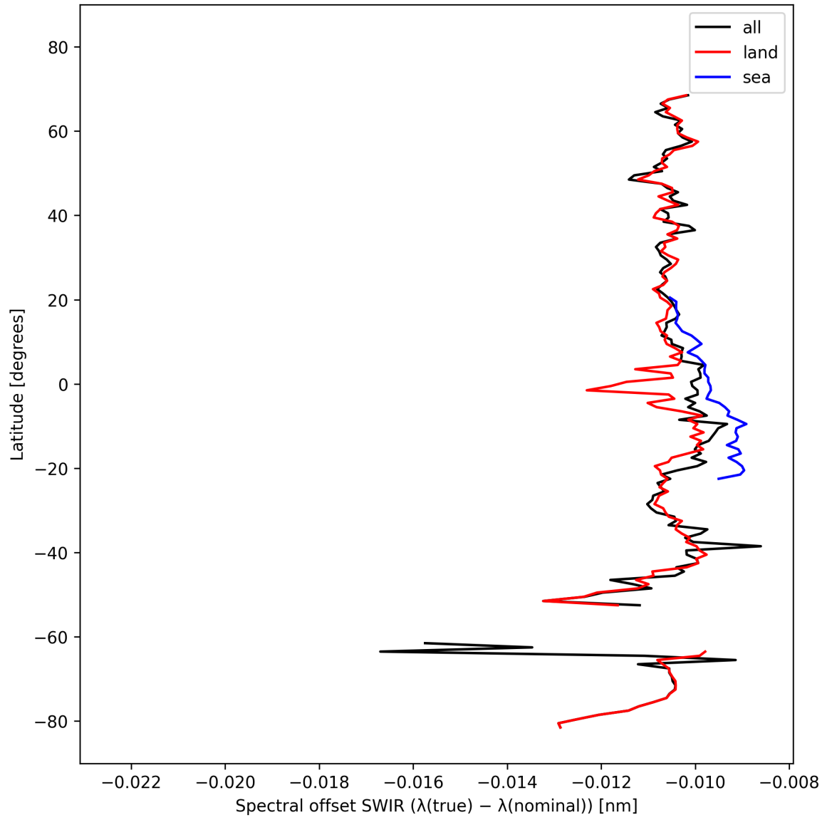
Figure 16: Zonal average of “Spectral offset SWIR ( \lambda_{\text{true}} - \lambda_{\text{nominal}} )” for 2025-03-03 to 2025-03-05.
