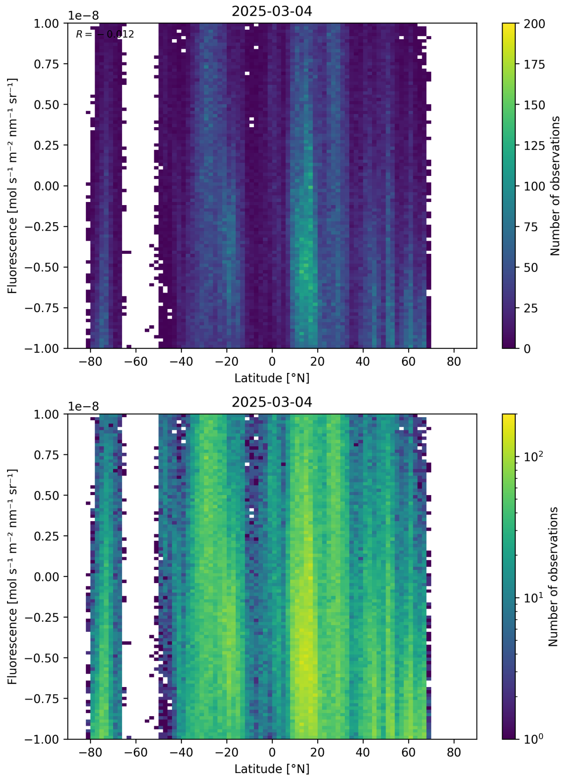
Figure 56: Scatter density plot of “Latitude” against “Fluorescence” for 2025-03-03 to 2025-03-05.
