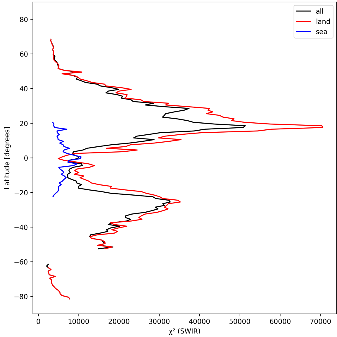
Figure 17: Zonal average of “ \chi^2 (SWIR)” for 2025-03-03 to 2025-03-05.
