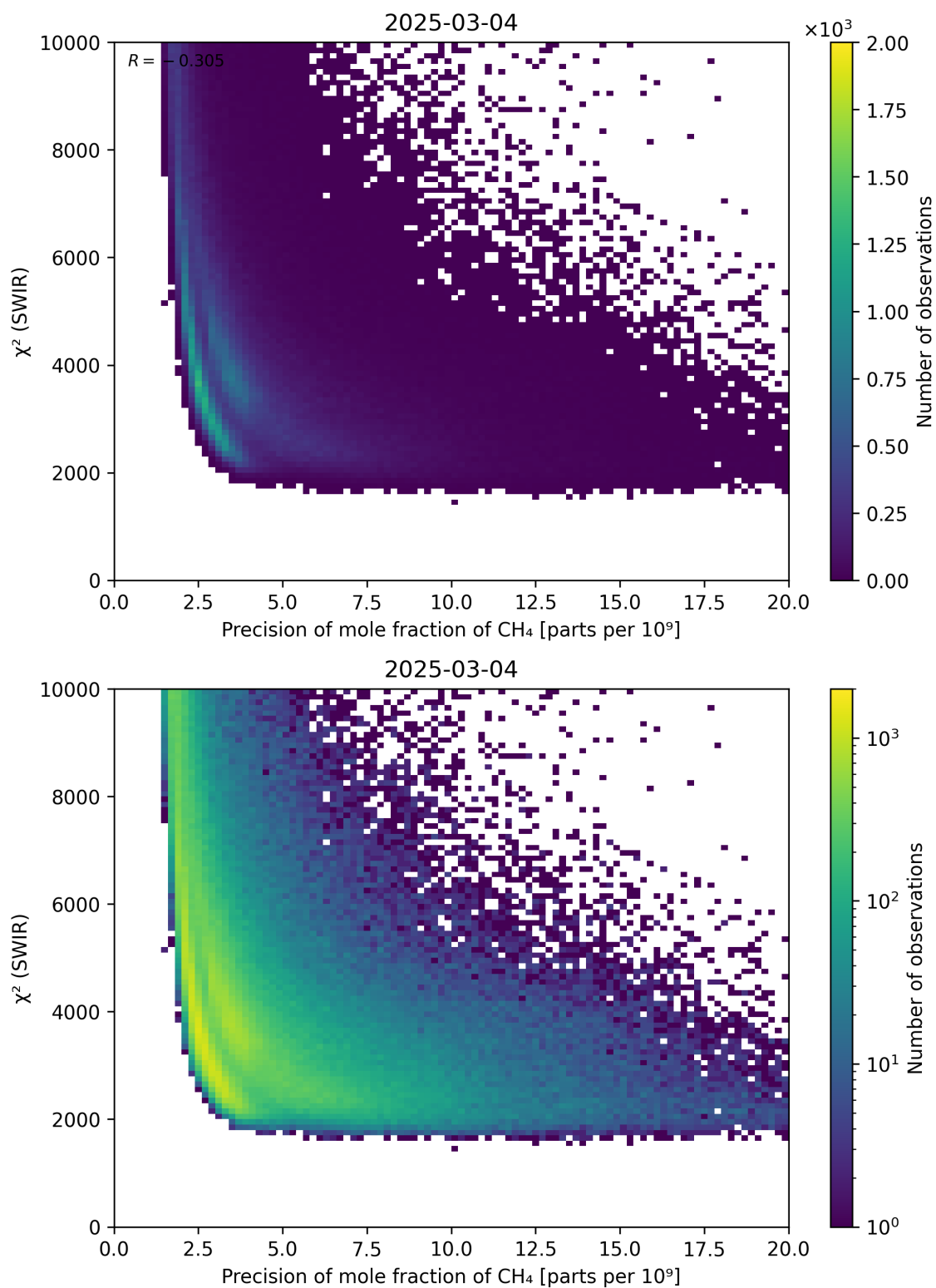
Figure 79: Scatter density plot of “Precision of mole fraction of \text{CH}_4 ” against “ \chi^2 (SWIR)” for 2025-03-03 to 2025-03-05.
