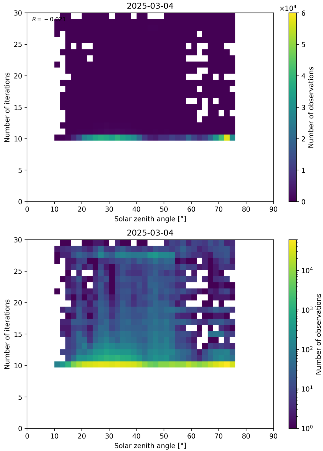
Figure 102: Scatter density plot of “Solar zenith angle” against “Number of iterations” for 2025-03-03 to 2025-03-05.
