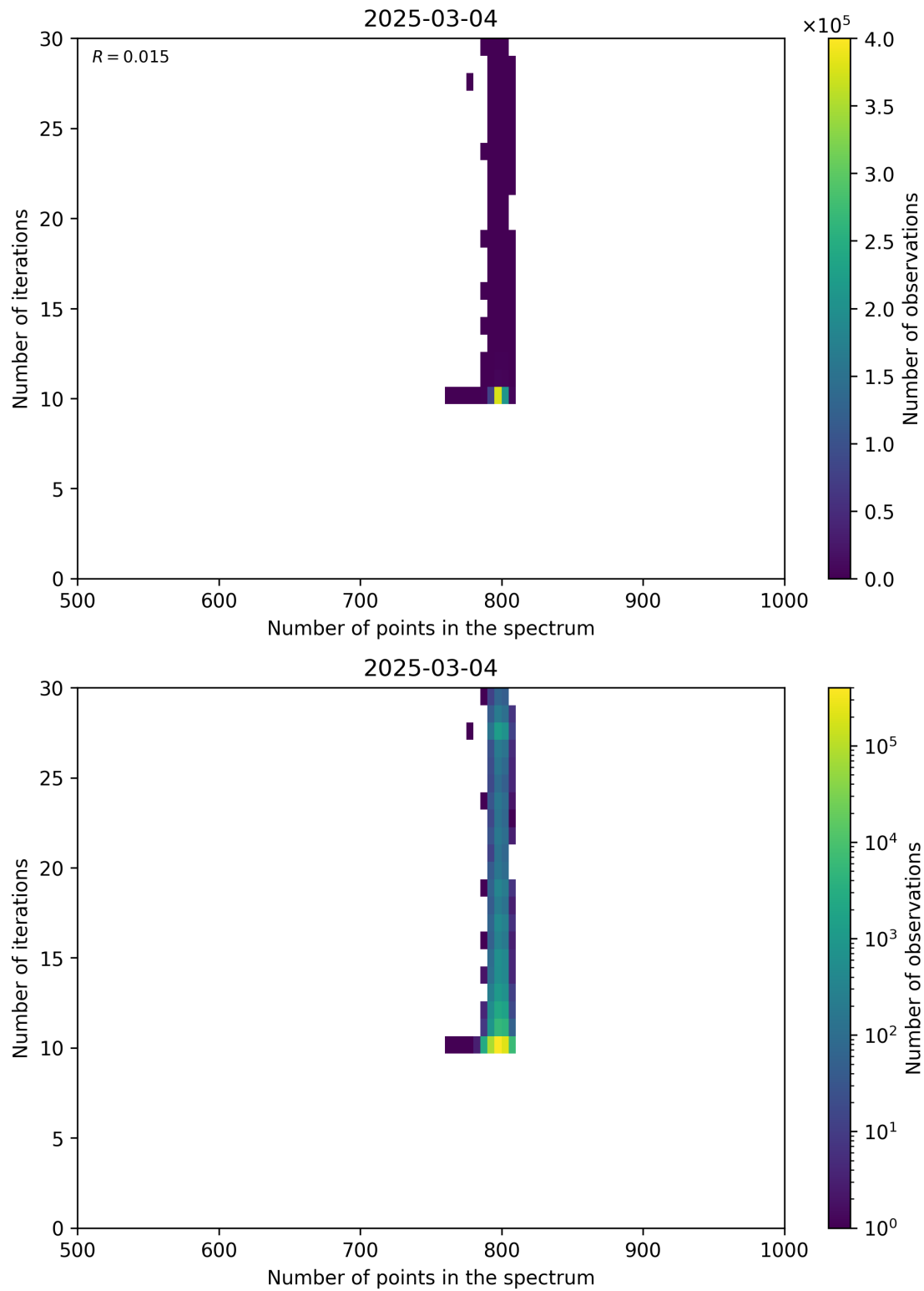
Figure 92: Scatter density plot of “Number of points in the spectrum” against “Number of iterations” for 2025-03-03 to 2025-03-05.
