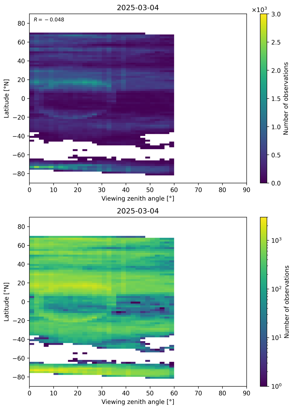
Figure 109: Scatter density plot of “Viewing zenith angle” against “Latitude” for 2025-03-03 to 2025-03-05.
