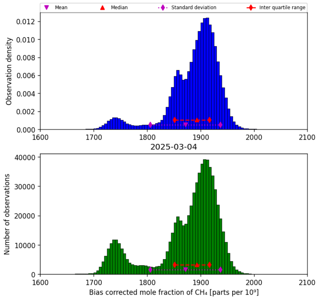
Figure 25: Histogram of “Bias corrected mole fraction of CH 4 ” for 2025-03-03 to 2025-03-05
