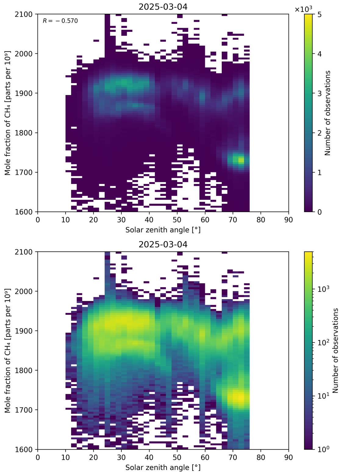
Figure 99: Scatter density plot of “Solar zenith angle” against “Mole fraction of CH 4 ” for 2025-03-03 to 2025-03-05.
