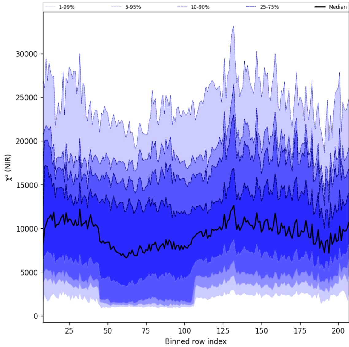
Figure 40: Along track statistics of “ \chi^2 (NIR)” for 2025-03-03 to 2025-03-05
