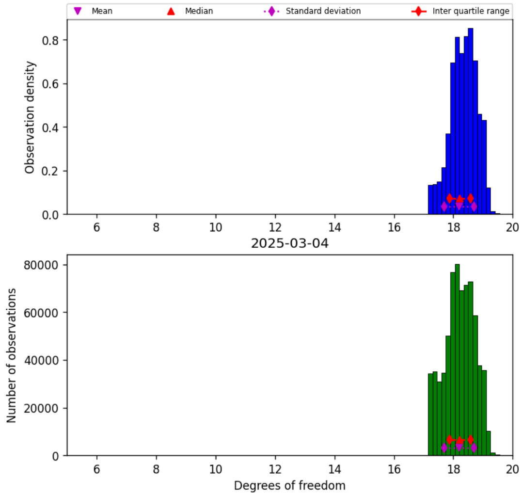
Figure 30: Histogram of “Degrees of freedom” for 2025-03-03 to 2025-03-05
