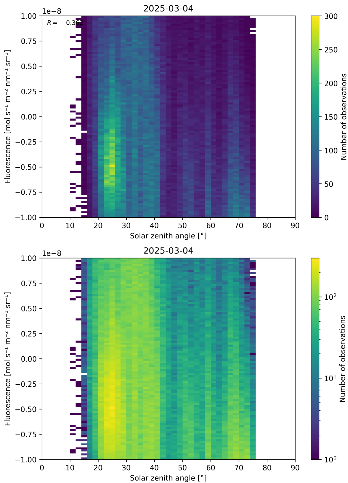
Figure 97: Scatter density plot of “Solar zenith angle” against “Fluorescence” for 2025-03-03 to 2025-03-05.
