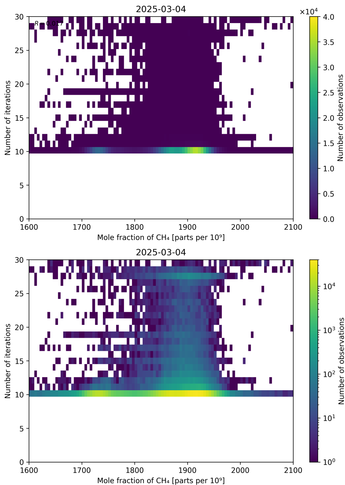
Figure 76: Scatter density plot of “Mole fraction of CH 4 ” against “Number of iterations” for 2025-03-03 to 2025-03-05.
