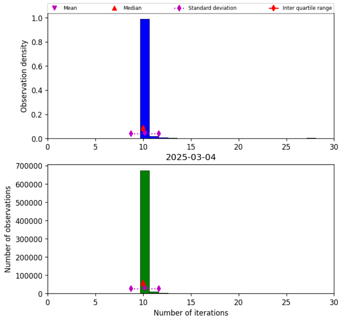
Figure 31: Histogram of “Number of iterations” for 2025-03-03 to 2025-03-05
