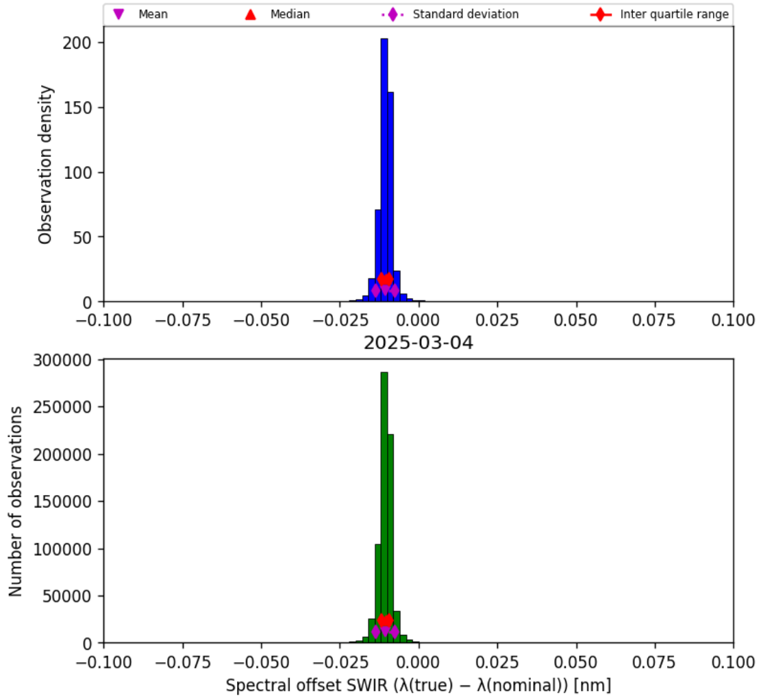
Figure 27: Histogram of “Spectral offset SWIR ( \lambda_{\text{true}} - \lambda_{\text{nominal}} )” for 2025-03-03 to 2025-03-05
