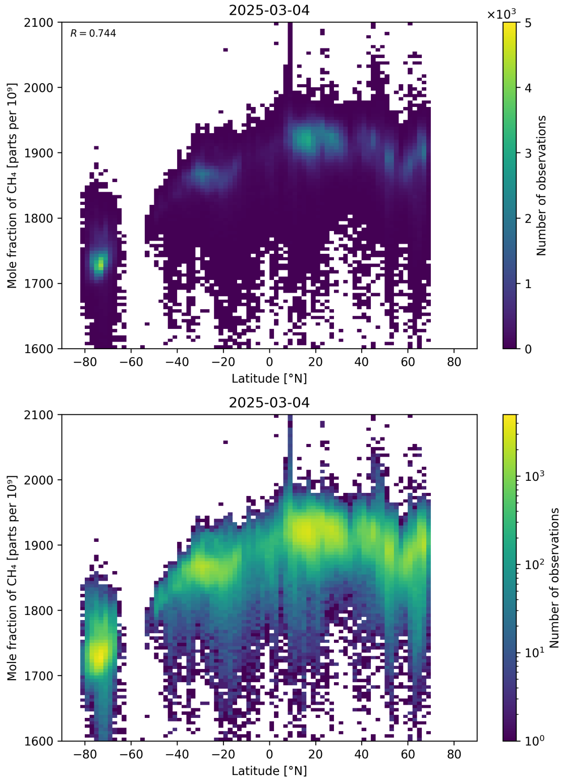
Figure 57: Scatter density plot of “Latitude” against “Mole fraction of CH 4 ” for 2025-03-03 to 2025-03-05.
