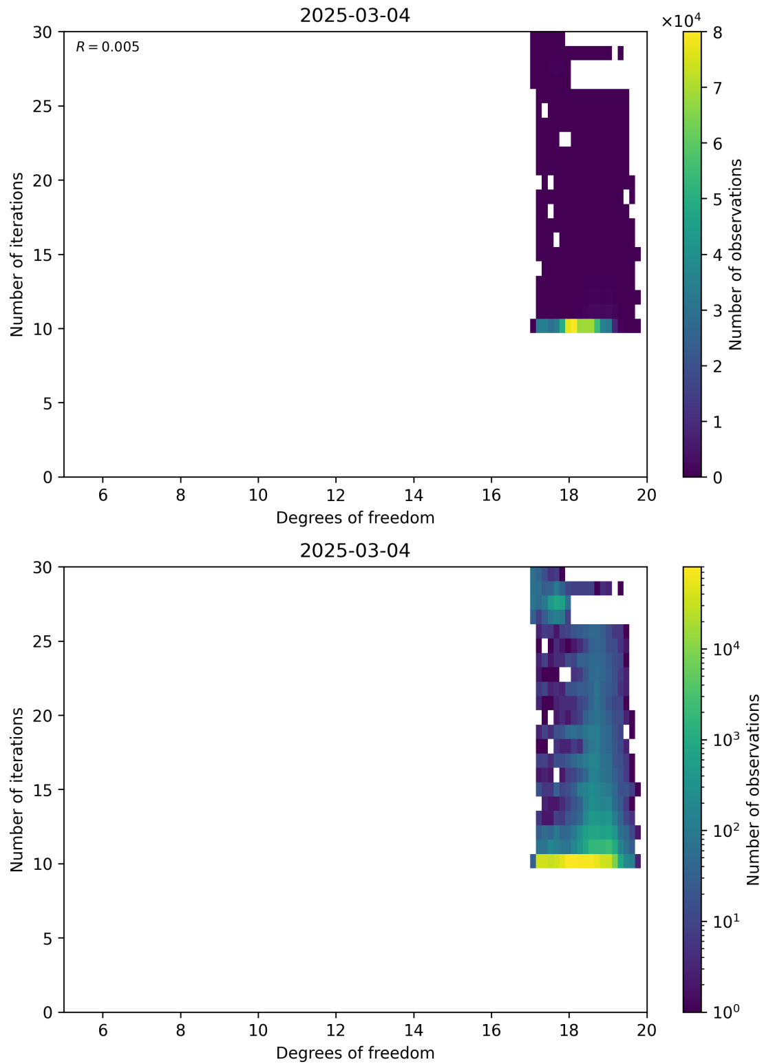
Figure 52: Scatter density plot of “Degrees of freedom” against “Number of iterations” for 2025-03-03 to 2025-03-05.
