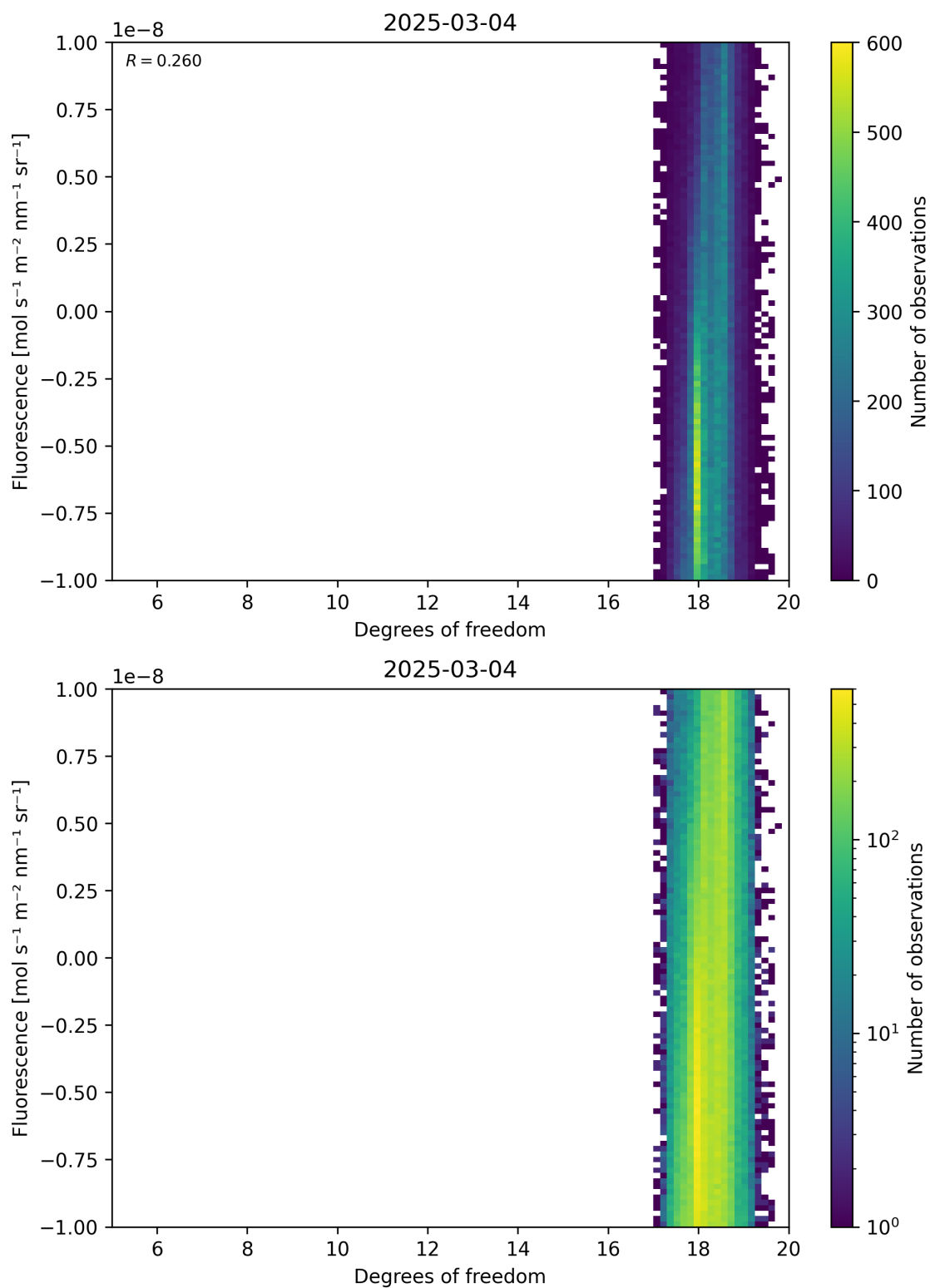
Figure 51: Scatter density plot of “Degrees of freedom” against “Fluorescence” for 2025-03-03 to 2025-03-05.
