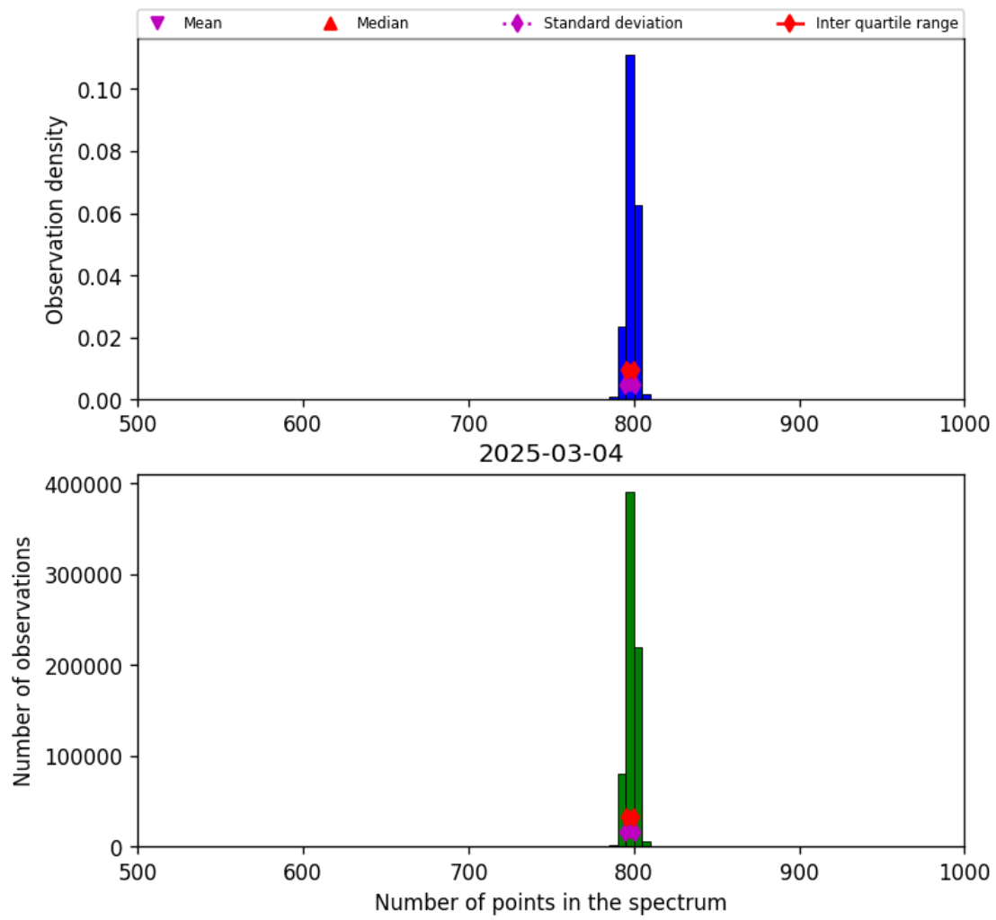
Figure 26: Histogram of “Number of points in the spectrum” for 2025-03-03 to 2025-03-05
