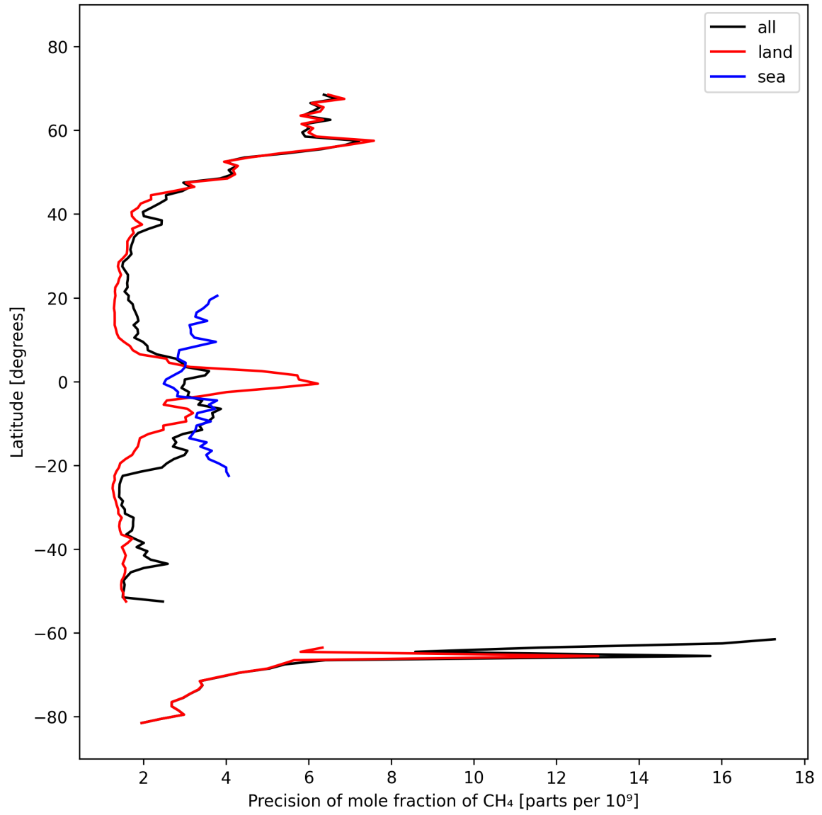
Figure 13: Zonal average of “Precision of mole fraction of CH 4 ” for 2025-03-03 to 2025-03-05.
