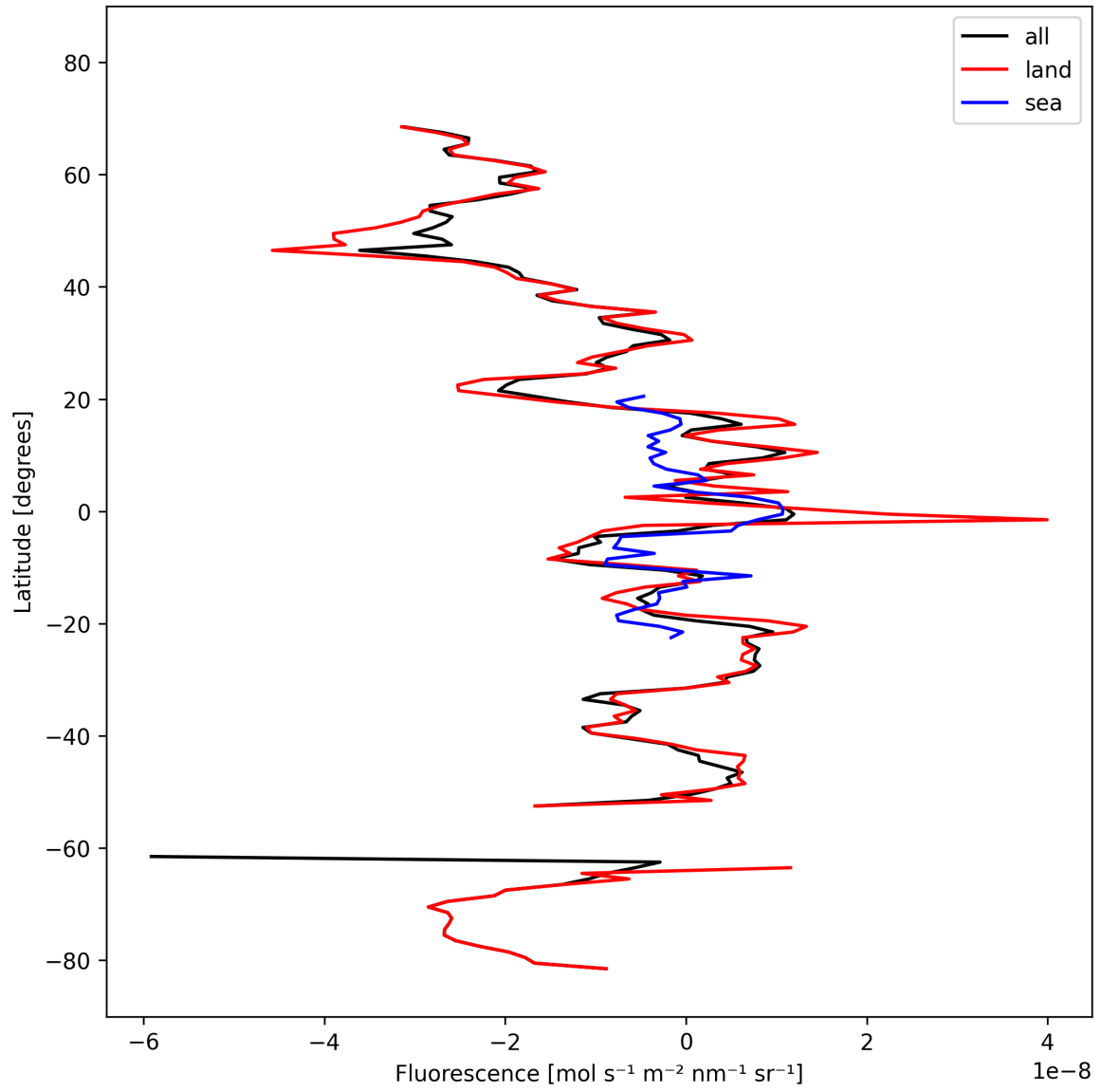
Figure 21: Zonal average of “Fluorescence” for 2025-03-03 to 2025-03-05.
