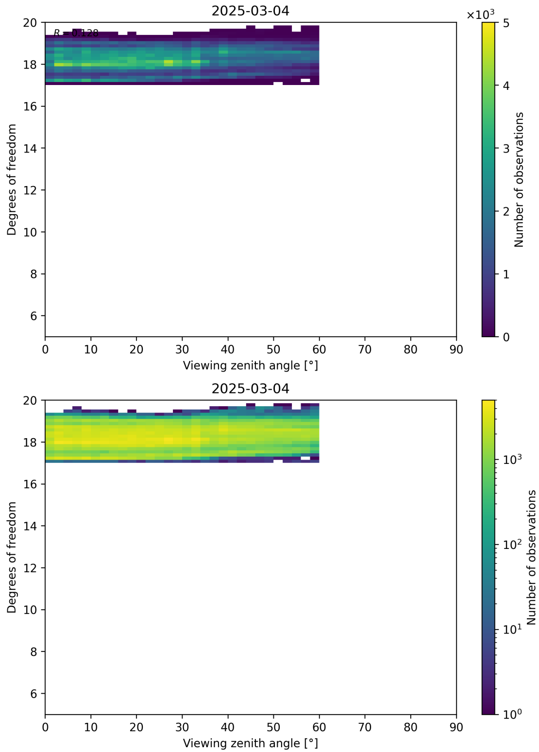
Figure 107: Scatter density plot of “Viewing zenith angle” against “Degrees of freedom” for 2025-03-03 to 2025-03-05.
