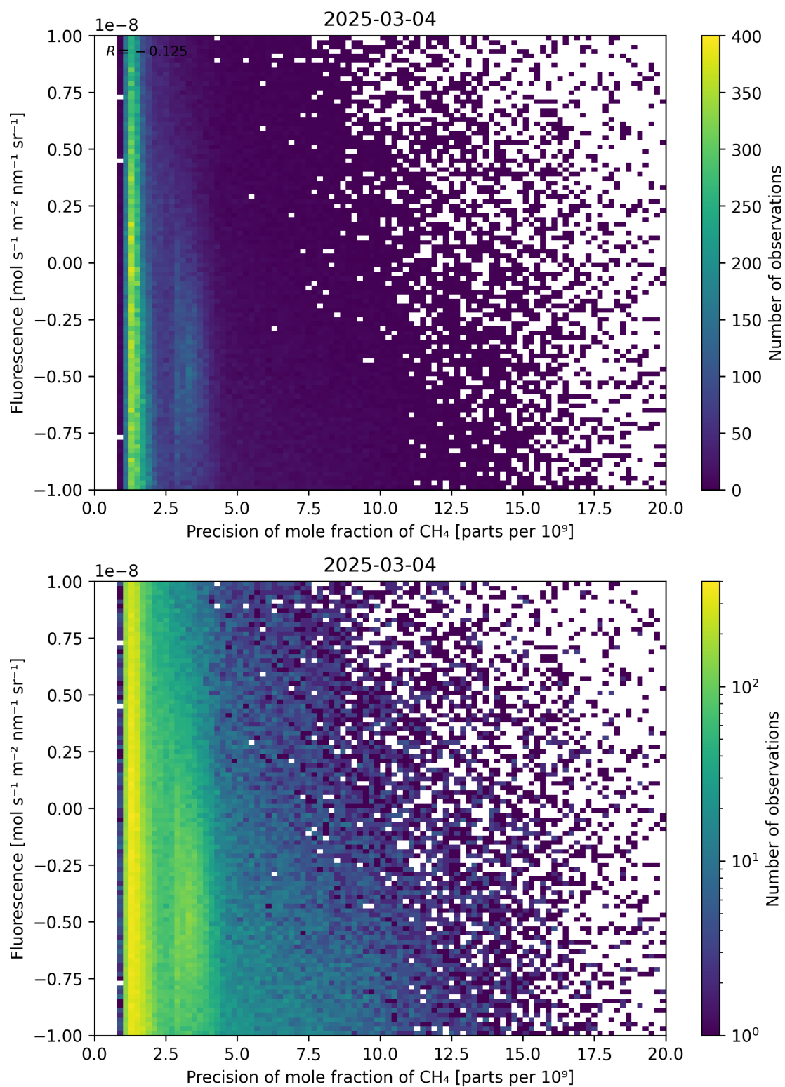
Figure 81: Scatter density plot of “Precision of mole fraction of \text{CH}_4 ” against “Fluorescence” for 2025-03-03 to 2025-03-05.
