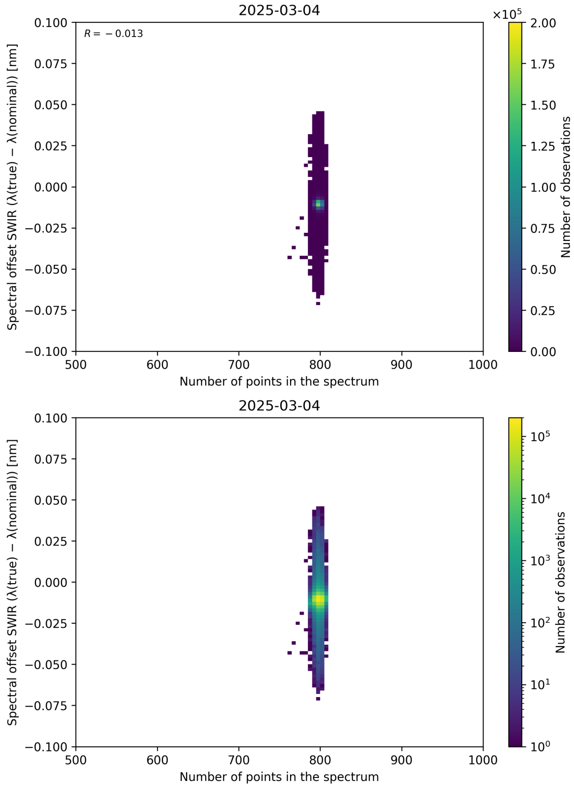
Figure 93: Scatter density plot of “Number of points in the spectrum” against “Spectral offset SWIR ( \lambda_{\text{true}} - \lambda_{\text{nominal}} )” for 2025-03-03 to 2025-03-05.
