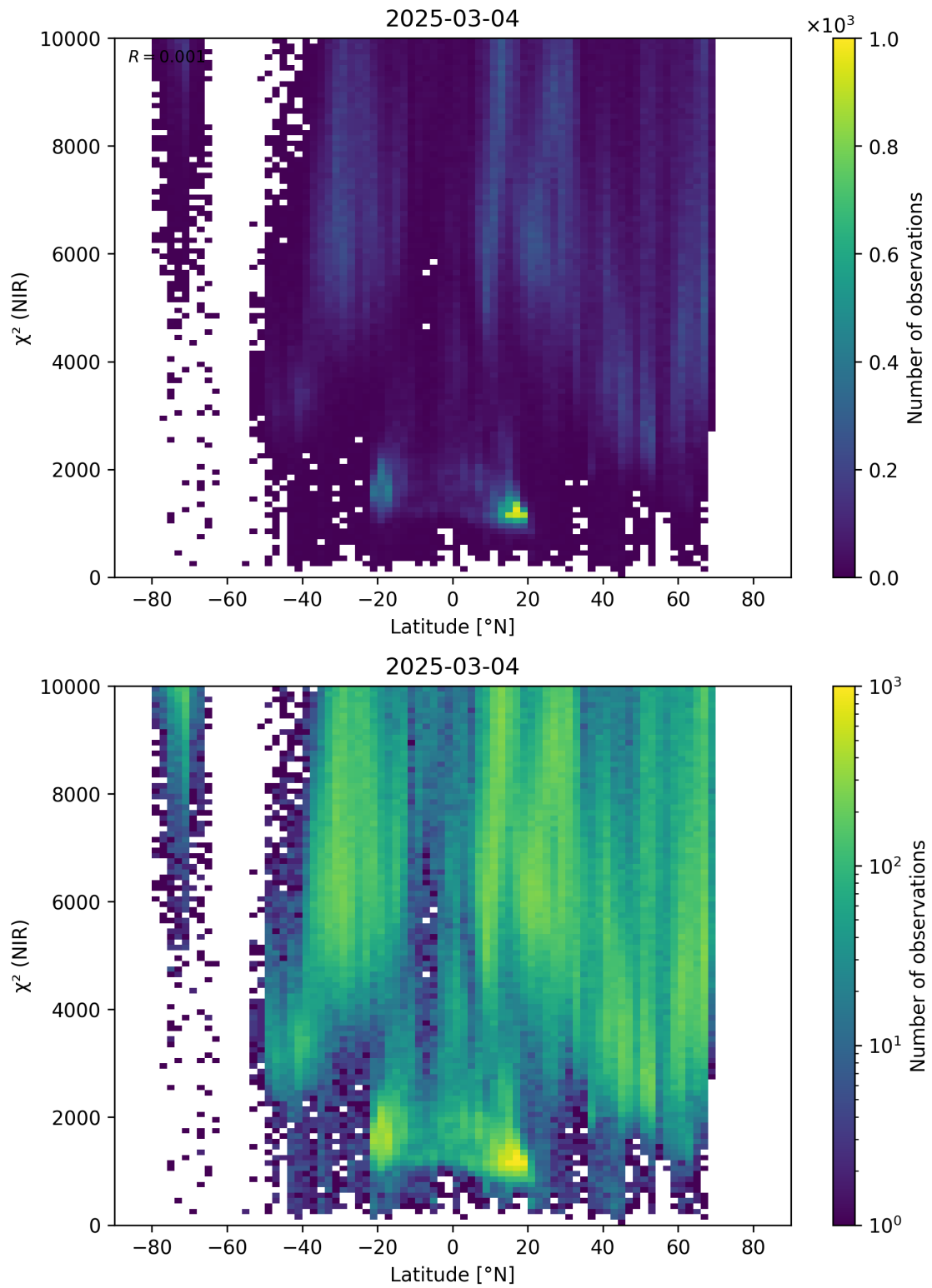
Figure 53: Scatter density plot of “Latitude” against “ \chi^2 (NIR)” for 2025-03-03 to 2025-03-05.
