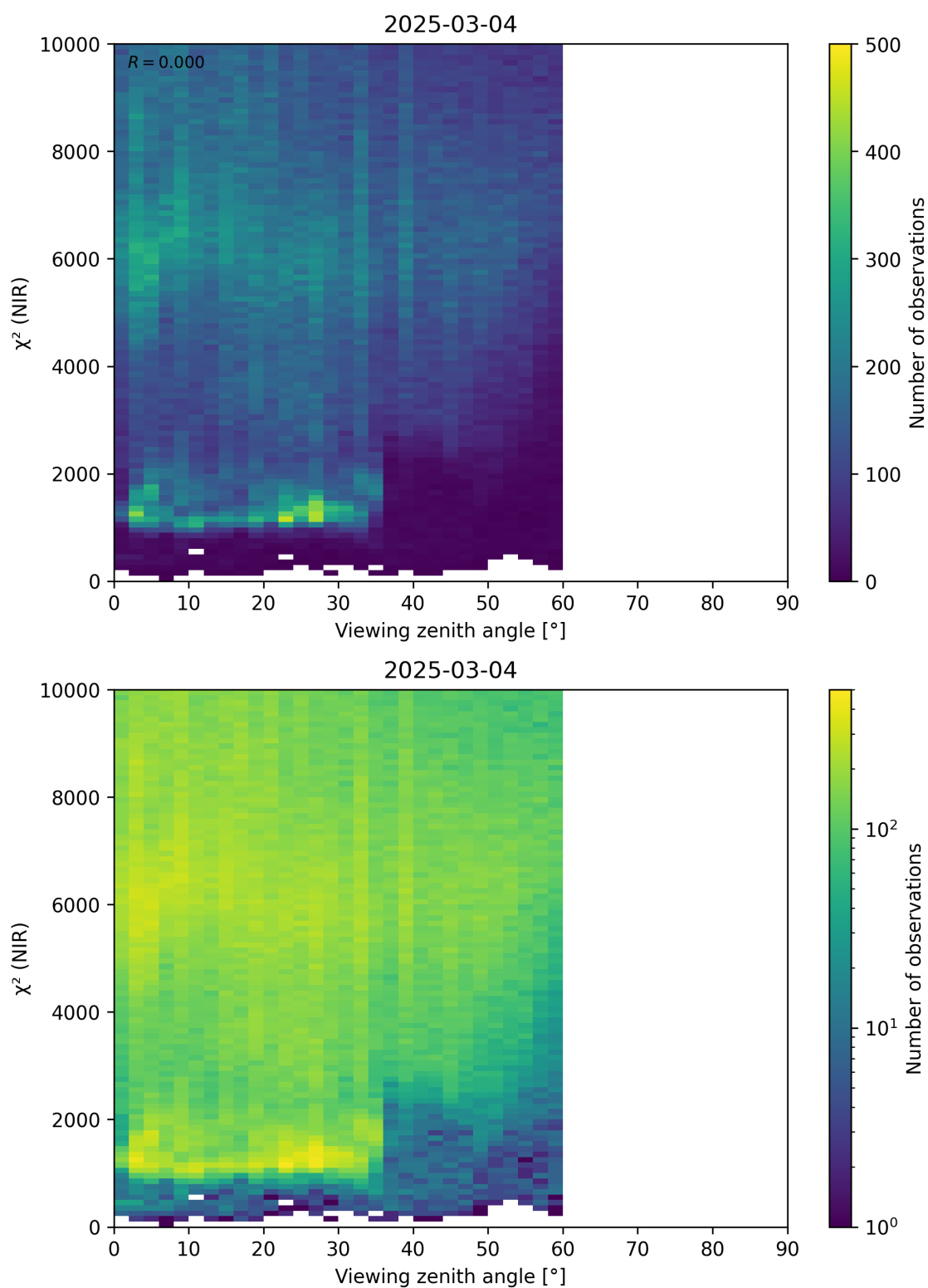
Figure 105: Scatter density plot of “Viewing zenith angle” against “ \chi^2 (NIR)” for 2025-03-03 to 2025-03-05.
