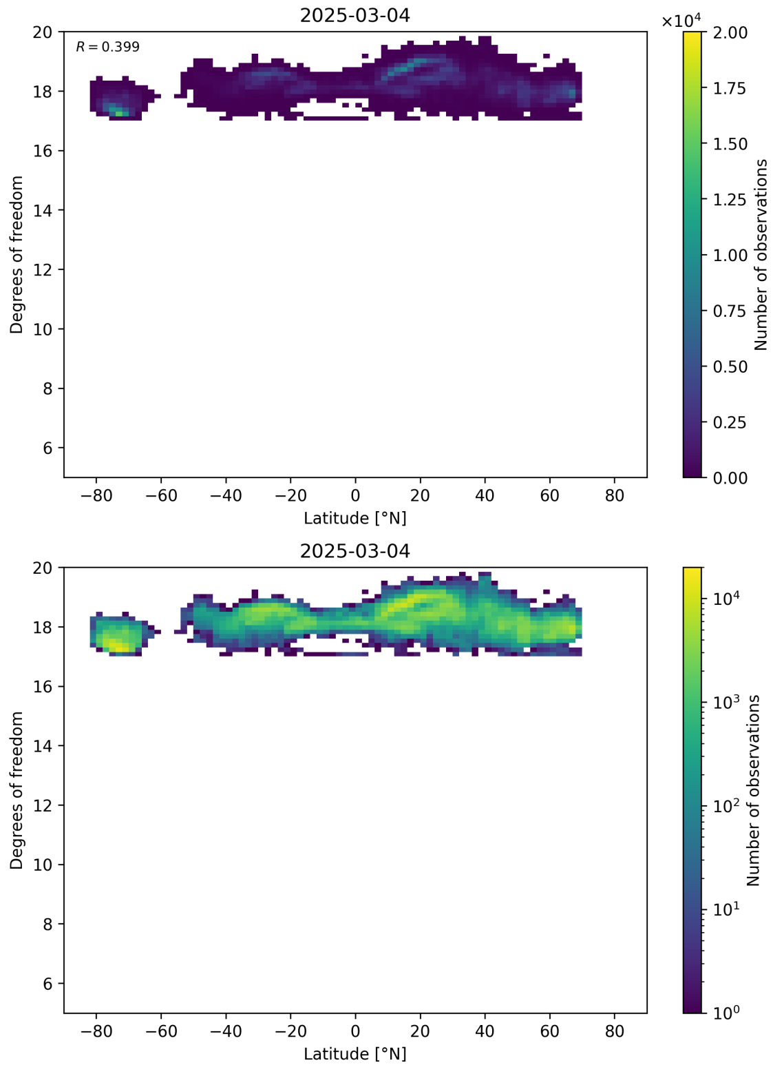
Figure 55: Scatter density plot of “Latitude” against “Degrees of freedom” for 2025-03-03 to 2025-03-05.
