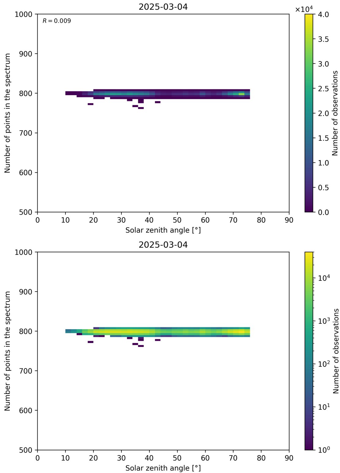
Figure 103: Scatter density plot of “Solar zenith angle” against “Number of points in the spectrum” for 2025-03-03 to 2025-03-05.
