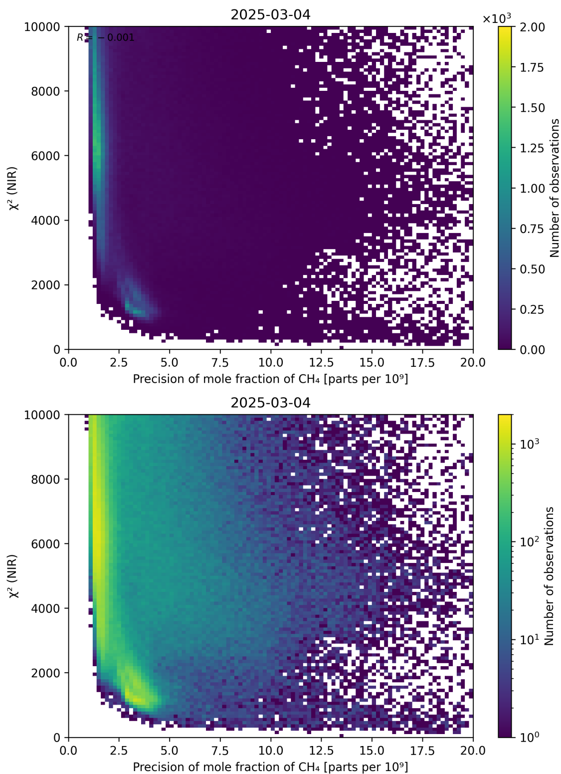
Figure 78: Scatter density plot of “Precision of mole fraction of CH 4 ” against “ \chi^2 (NIR)” for 2025-03-03 to 2025-03-05.
