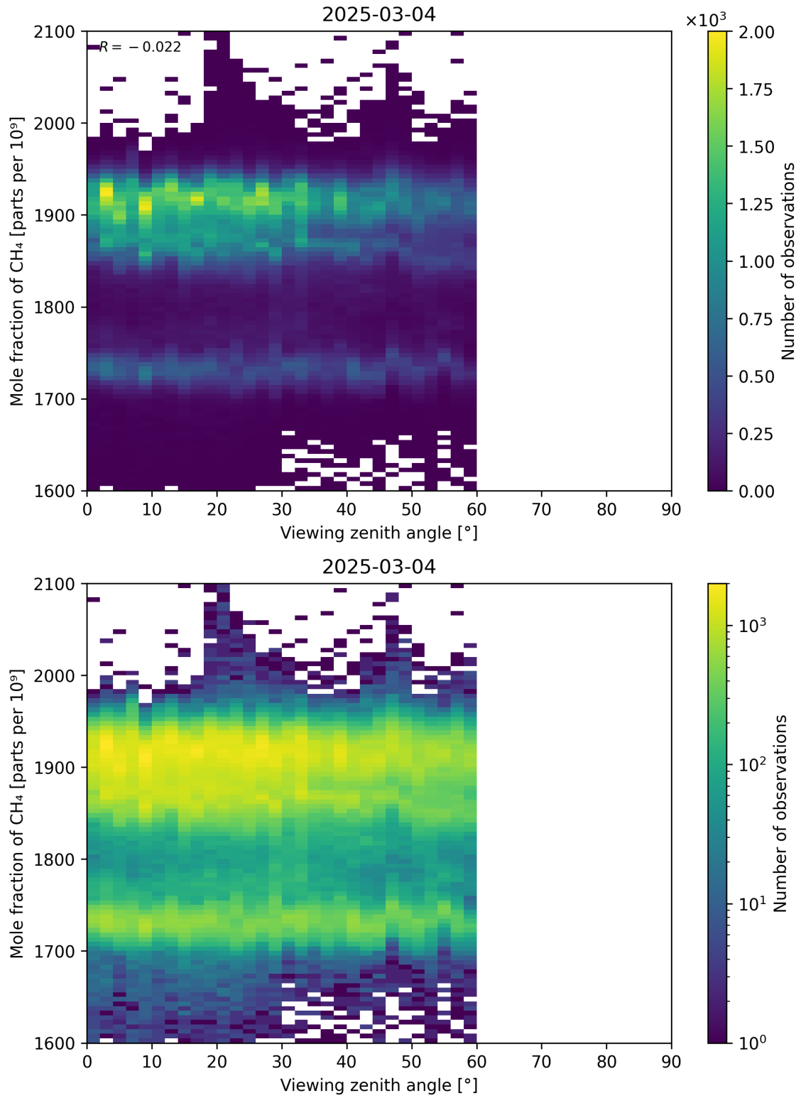
Figure 110: Scatter density plot of “Viewing zenith angle” against “Mole fraction of CH 4 ” for 2025-03-03 to 2025-03-05.
