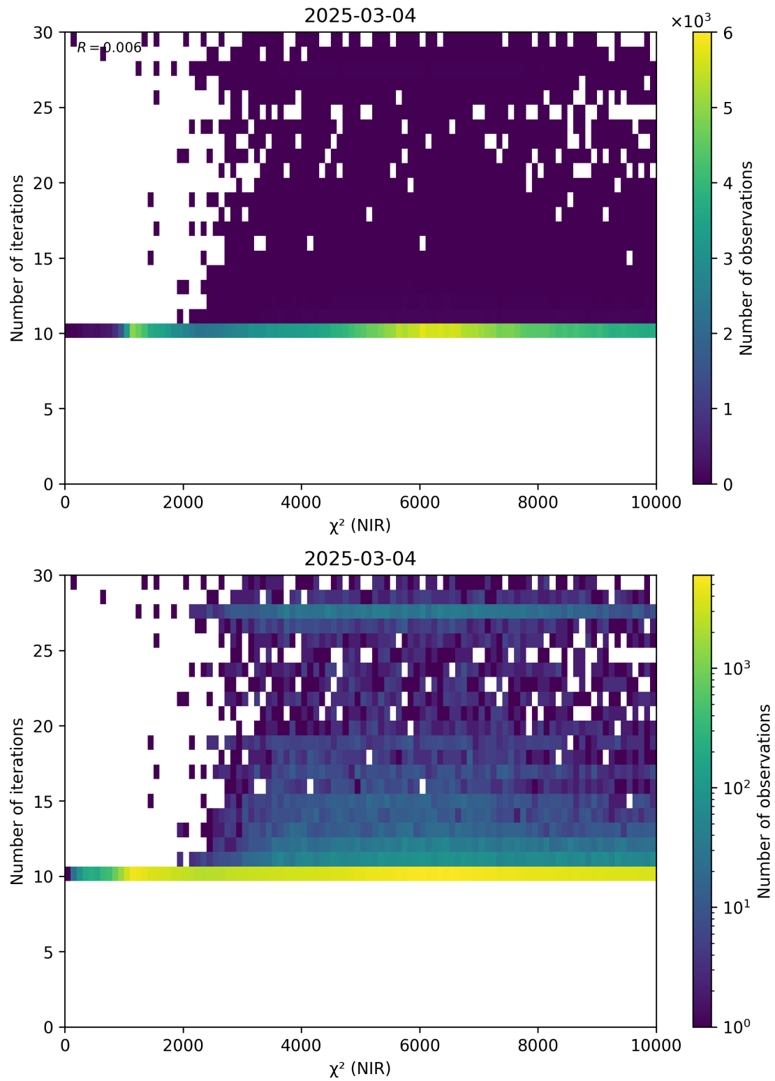
Figure 46: Scatter density plot of “ \chi^2 (NIR)” against “Number of iterations” for 2025-03-03 to 2025-03-05.
