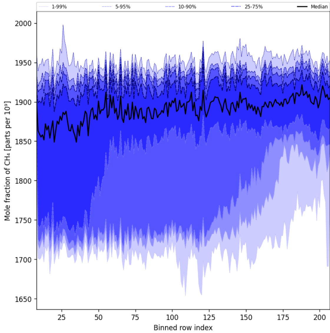
Figure 34: Along track statistics of “Mole fraction of CH 4 ” for 2025-03-03 to 2025-03-05
