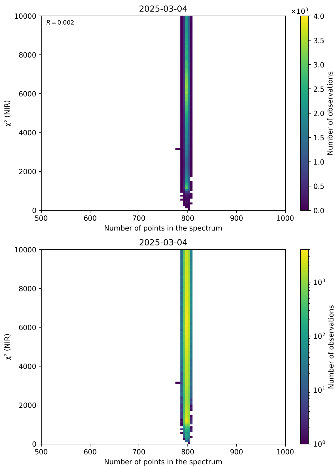
Figure 88: Scatter density plot of “Number of points in the spectrum” against “ \chi^2 (NIR)” for 2025-03-03 to 2025-03-05.
