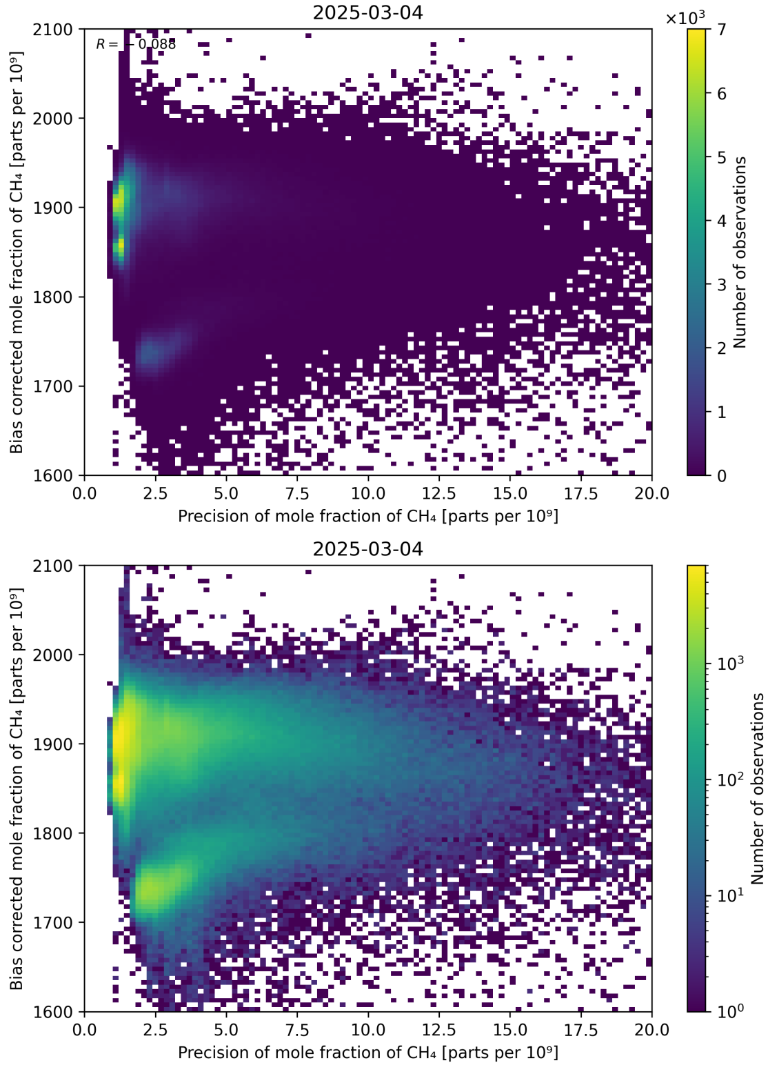
Figure 82: Scatter density plot of “Precision of mole fraction of CH 4 ” against “Bias corrected mole fraction of CH 4 ” for 2025-03-03 to 2025-03-05.
