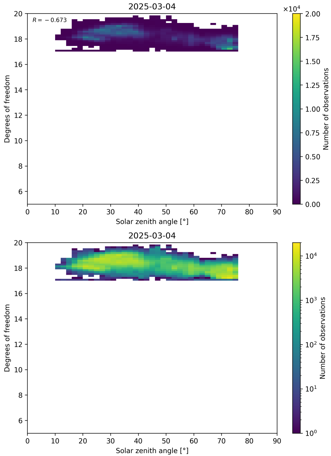
Figure 96: Scatter density plot of “Solar zenith angle” against “Degrees of freedom” for 2025-03-03 to 2025-03-05.
