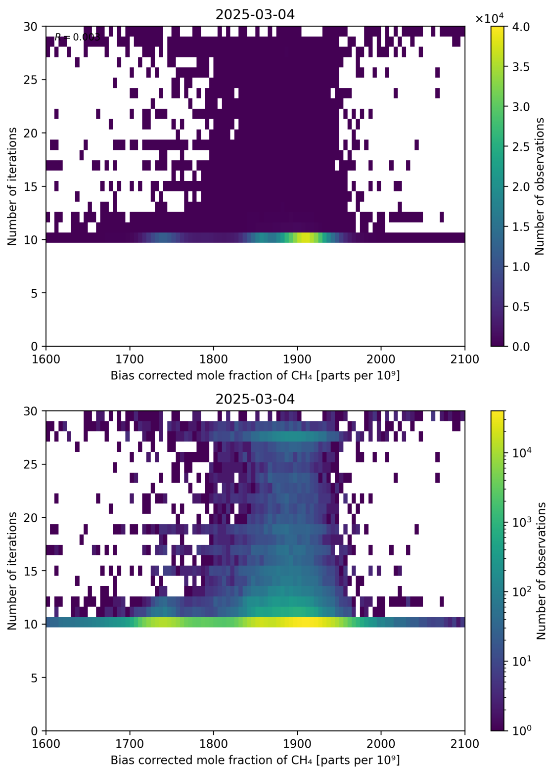
Figure 67: Scatter density plot of “Bias corrected mole fraction of CH 4 ” against “Number of iterations” for 2025-03-03 to 2025-03-05.
