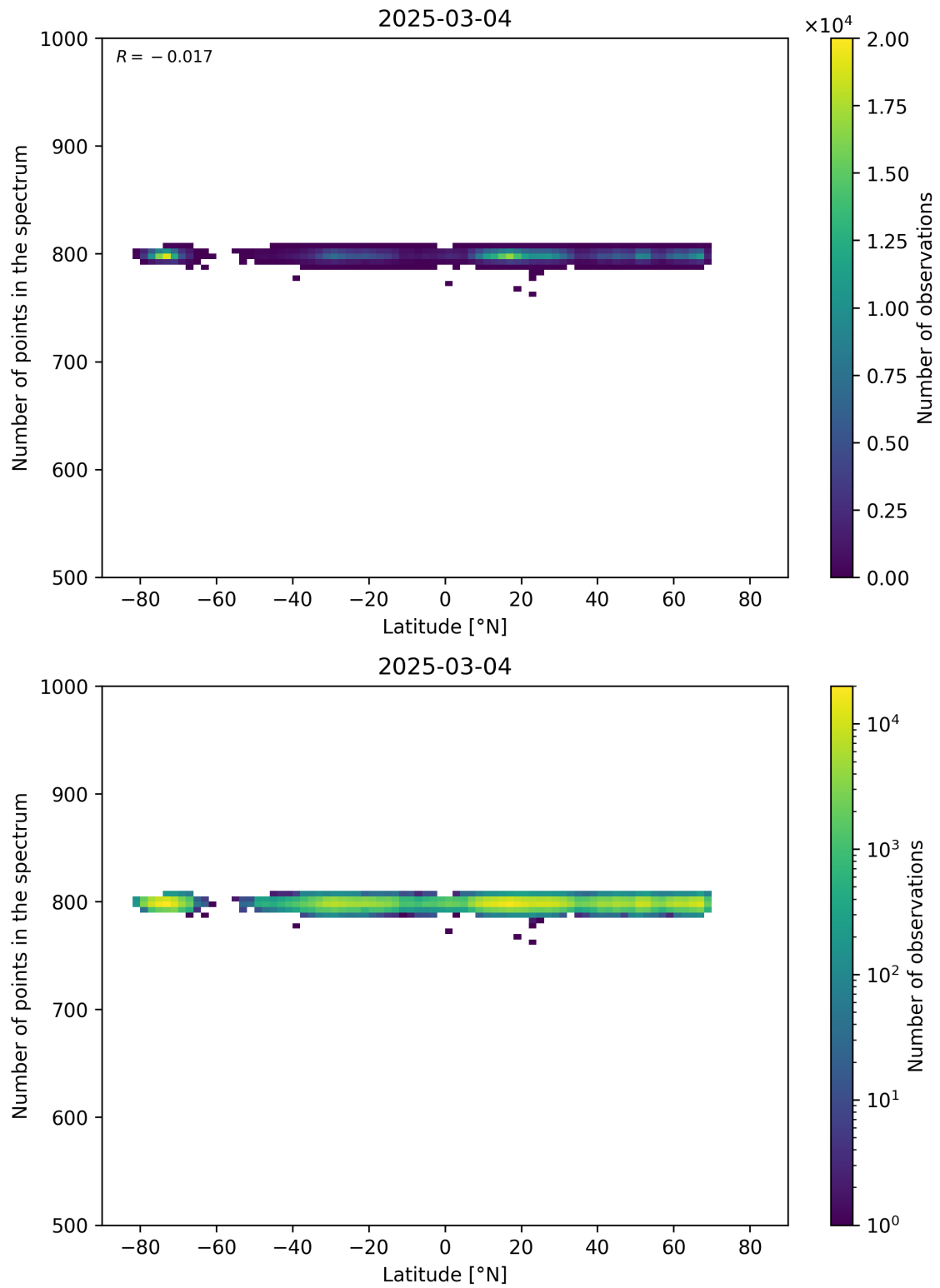
Figure 61: Scatter density plot of “Latitude” against “Number of points in the spectrum” for 2025-03-03 to 2025-03-05.
