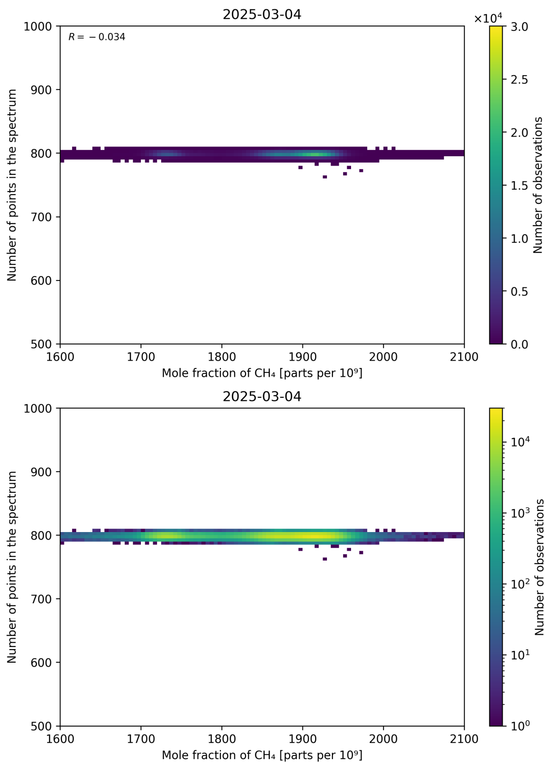
Figure 77: Scatter density plot of “Mole fraction of CH 4 ” against “Number of points in the spectrum” for 2025-03-03 to 2025-03-05.
