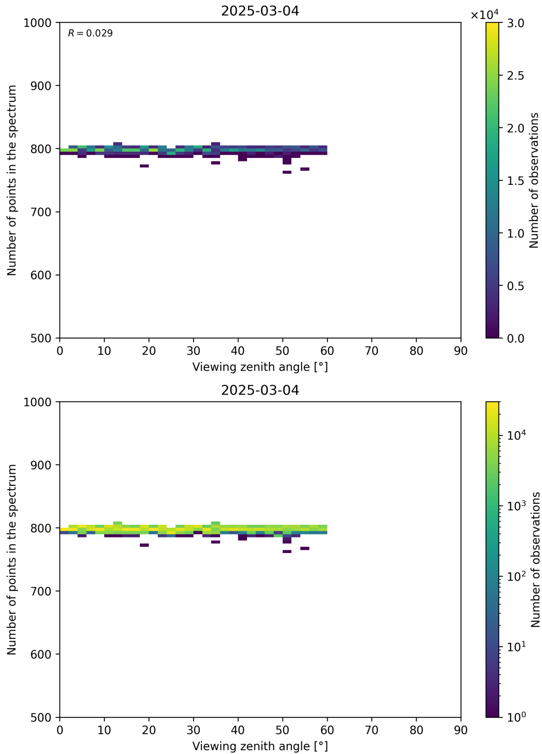
Figure 114: Scatter density plot of “Viewing zenith angle” against “Number of points in the spectrum” for 2025-03-03 to 2025-03-05.
