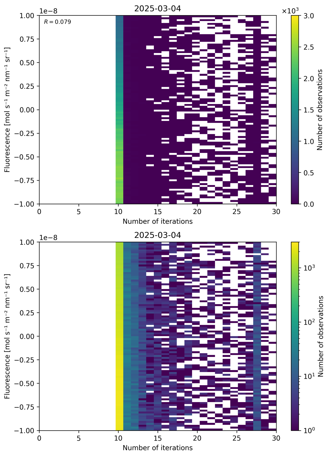
Figure 87: Scatter density plot of “Number of iterations” against “Fluorescence” for 2025-03-03 to 2025-03-05.
