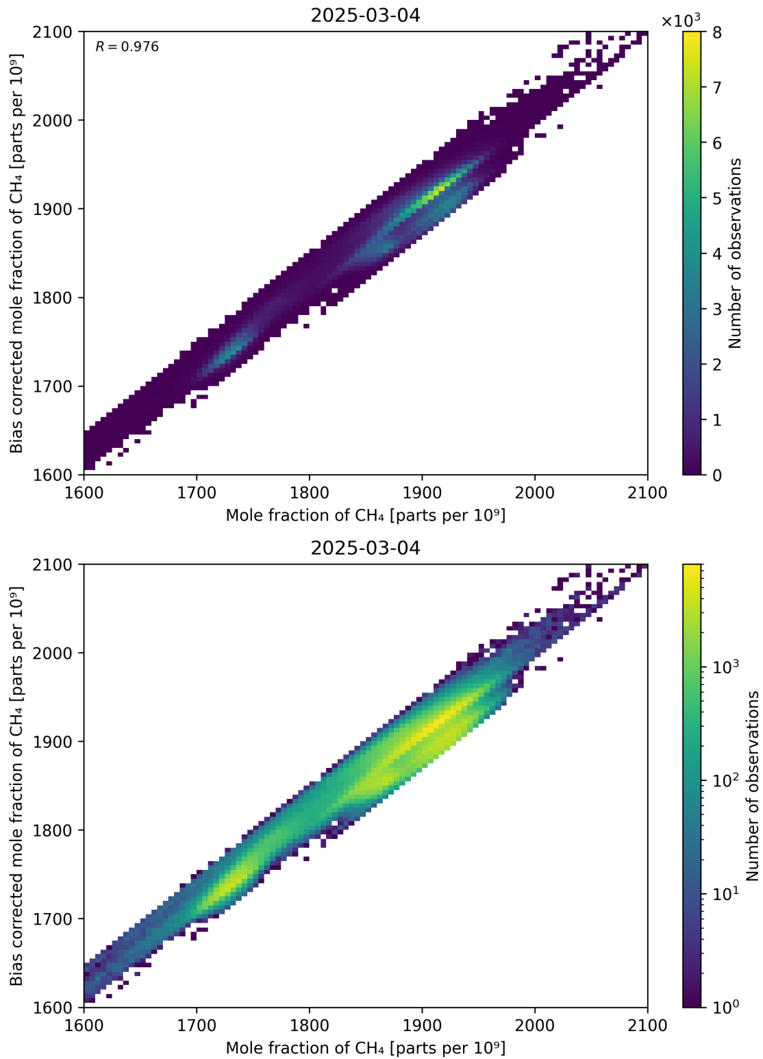
Figure 74: Scatter density plot of “Mole fraction of CH 4 ” against “Bias corrected mole fraction of CH 4 ” for 2025-03-03 to 2025-03-05.
