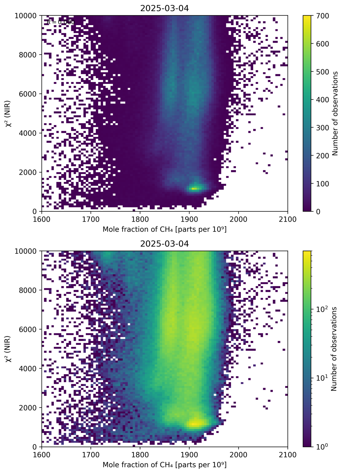
Figure 70: Scatter density plot of “Mole fraction of CH 4 ” against “ \chi^2 (NIR)” for 2025-03-03 to 2025-03-05.
