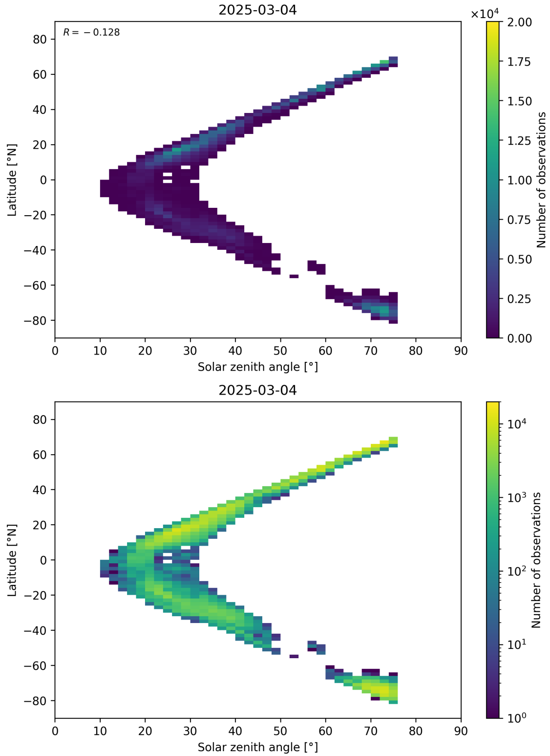
Figure 98: Scatter density plot of “Solar zenith angle” against “Latitude” for 2025-03-03 to 2025-03-05.
