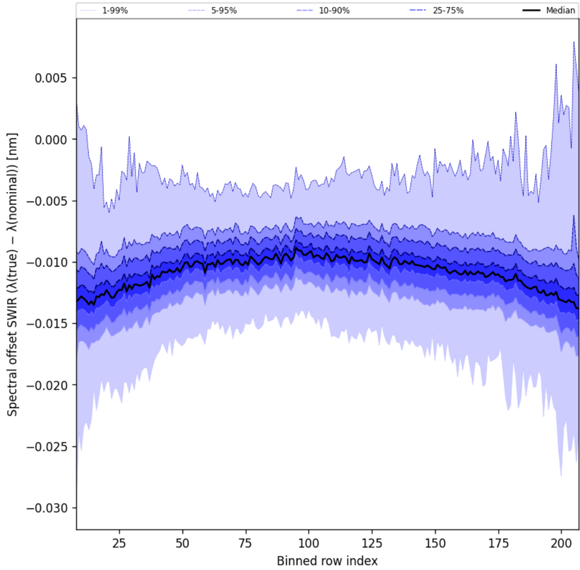
Figure 38: Along track statistics of “Spectral offset SWIR ( \lambda_{\text{true}} - \lambda_{\text{nominal}} )” for 2025-03-03 to 2025-03-05
