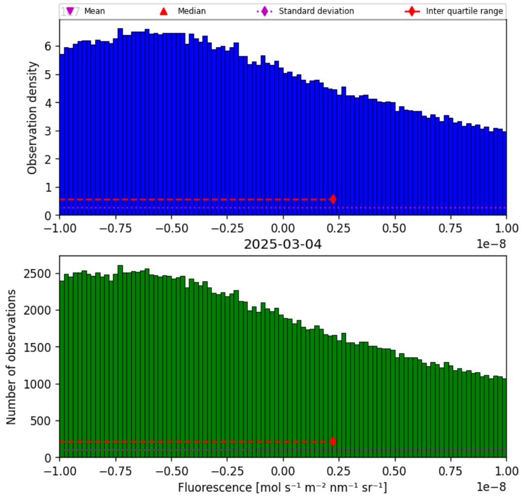
Figure 32: Histogram of “Fluorescence” for 2025-03-03 to 2025-03-05
