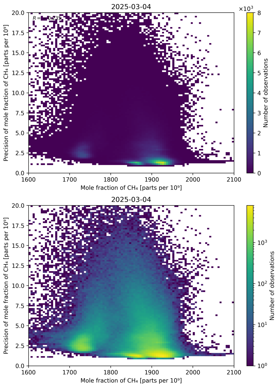
Figure 75: Scatter density plot of “Mole fraction of CH 4 ” against “Precision of mole fraction of CH 4 ” for 2025-03-03 to 2025-03-05.
