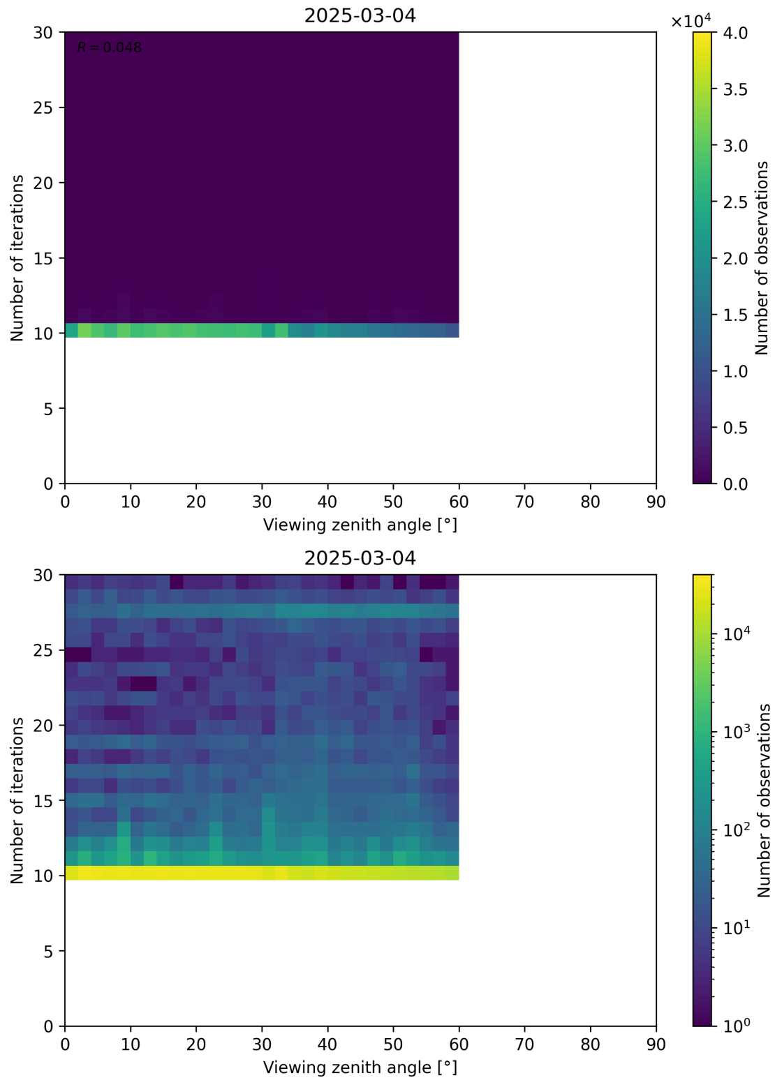
Figure 113: Scatter density plot of “Viewing zenith angle” against “Number of iterations” for 2025-03-03 to 2025-03-05.
