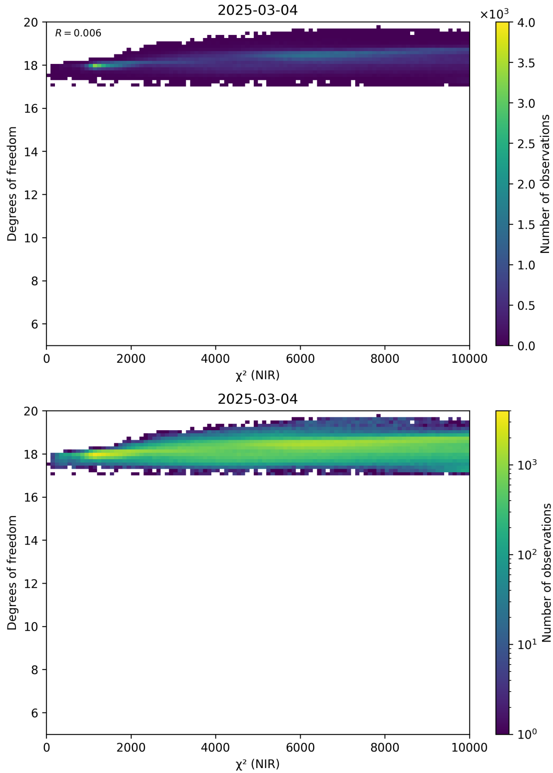
Figure 44: Scatter density plot of “ \chi^2 (NIR)” against “Degrees of freedom” for 2025-03-03 to 2025-03-05.
