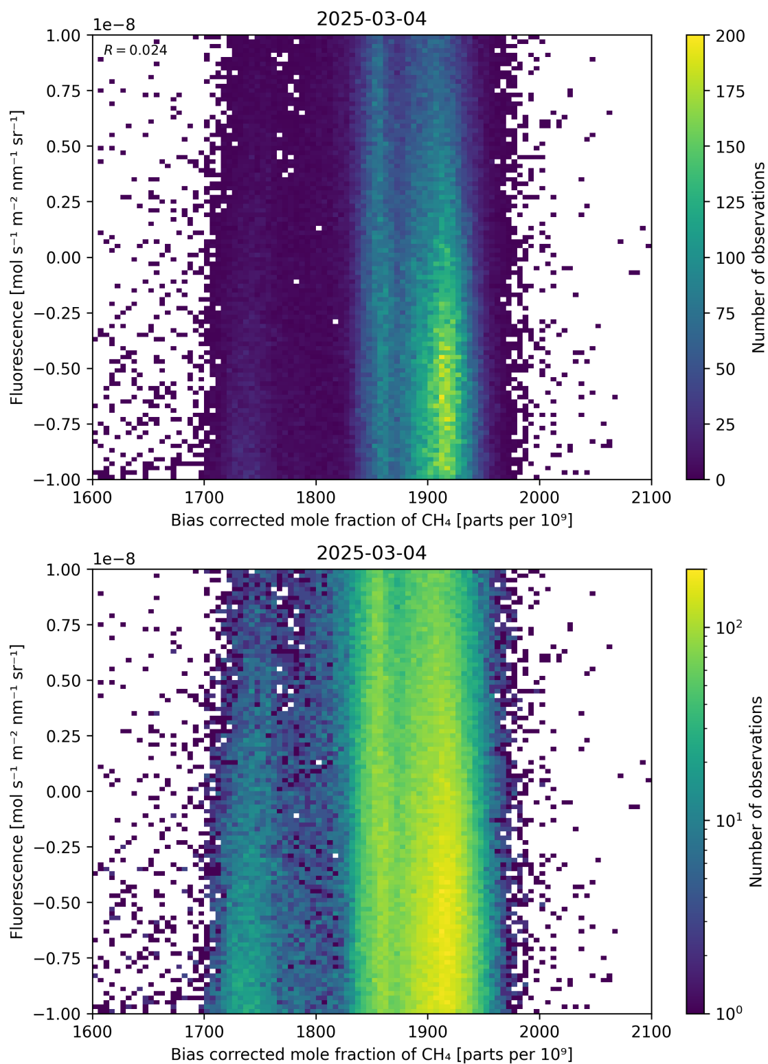
Figure 66: Scatter density plot of “Bias corrected mole fraction of \text{CH}_4 ” against “Fluorescence” for 2025-03-03 to 2025-03-05.
