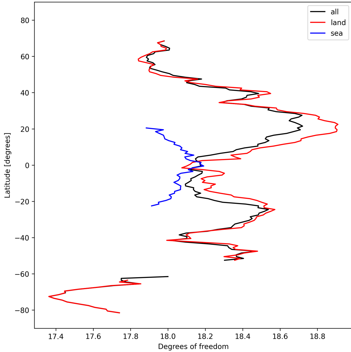
Figure 19: Zonal average of “Degrees of freedom” for 2025-03-03 to 2025-03-05.
