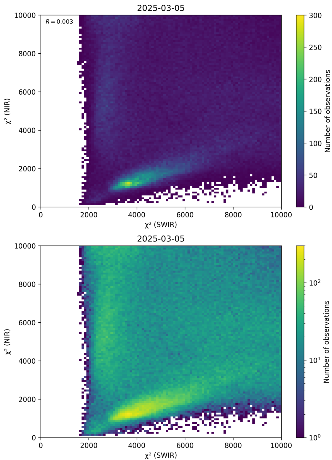
Figure 47: Scatter density plot of “ \chi^2 (SWIR)” against “ \chi^2 (NIR)” for 2025-03-04 to 2025-03-06.
