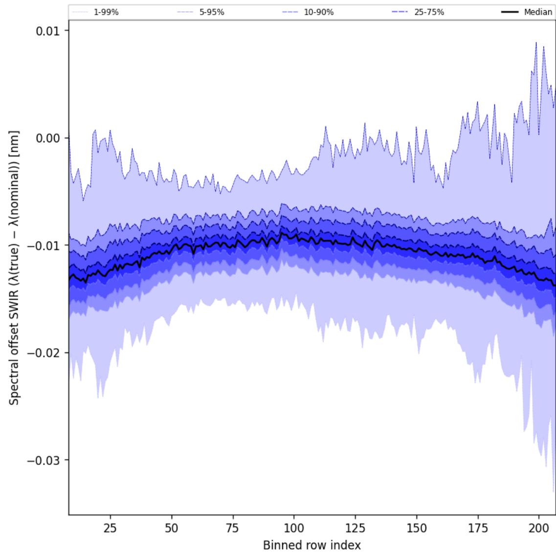
Figure 38: Along track statistics of “Spectral offset SWIR ( \lambda_{\text{true}} - \lambda_{\text{nominal}} )” for 2025-03-04 to 2025-03-06
