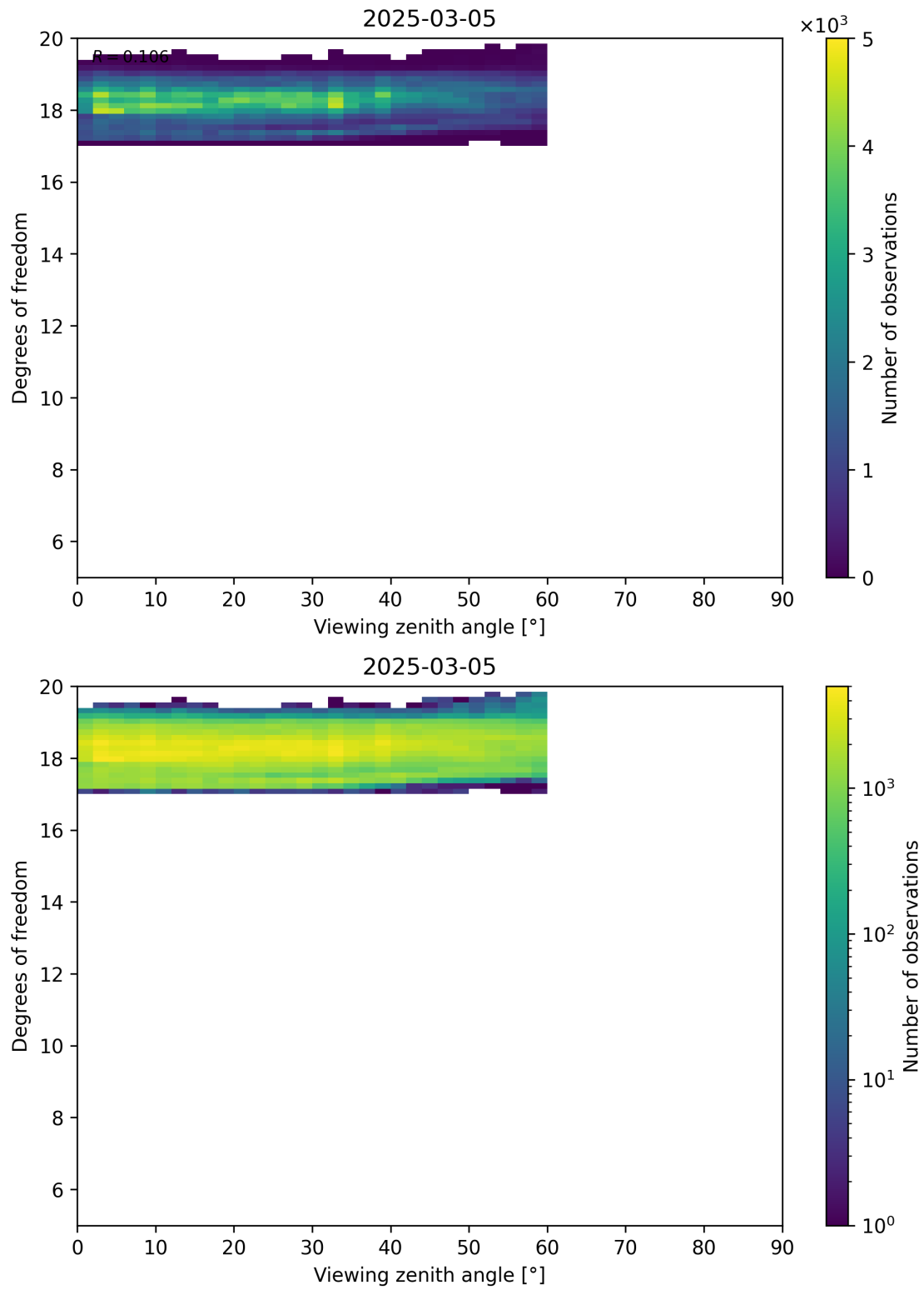
Figure 107: Scatter density plot of “Viewing zenith angle” against “Degrees of freedom” for 2025-03-04 to 2025-03-06.
