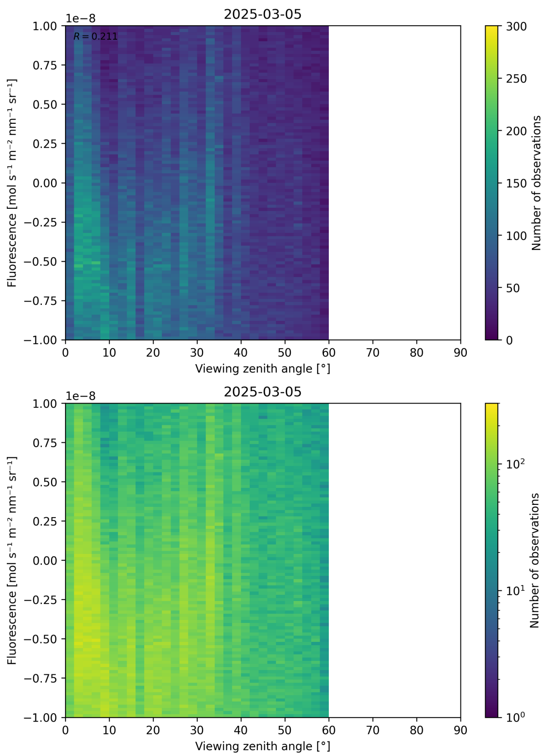
Figure 108: Scatter density plot of “Viewing zenith angle” against “Fluorescence” for 2025-03-04 to 2025-03-06.
