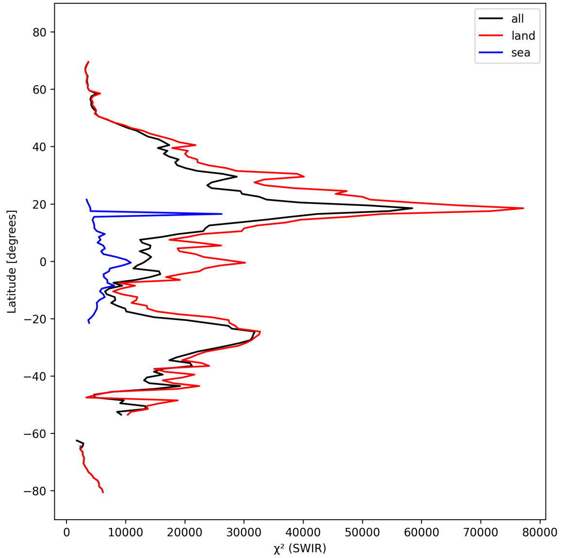
Figure 17: Zonal average of “ \chi^2 (SWIR)” for 2025-03-04 to 2025-03-06.
