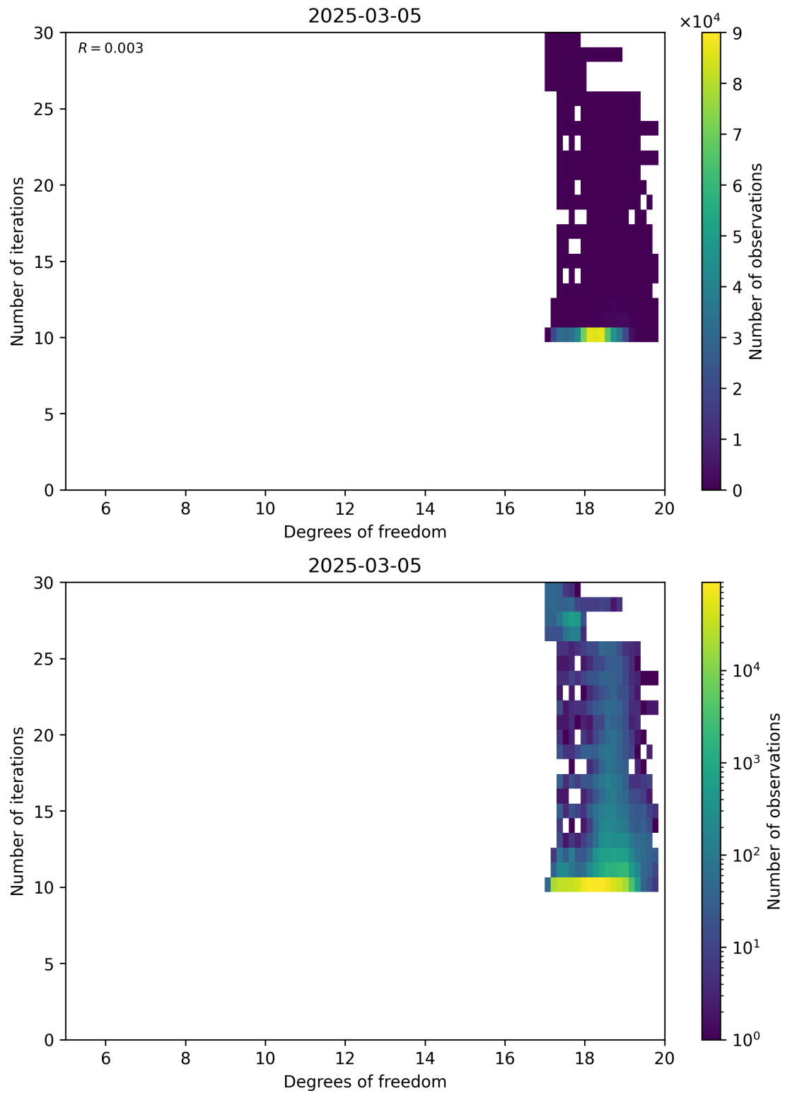
Figure 52: Scatter density plot of “Degrees of freedom” against “Number of iterations” for 2025-03-04 to 2025-03-06.
