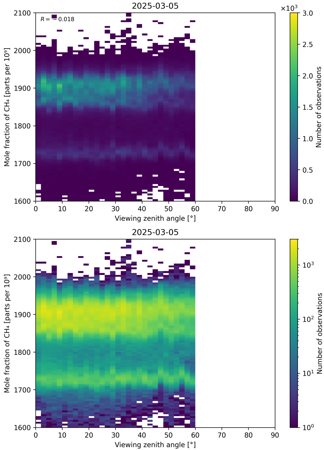
Figure 110: Scatter density plot of “Viewing zenith angle” against “Mole fraction of CH 4 ” for 2025-03-04 to 2025-03-06.
