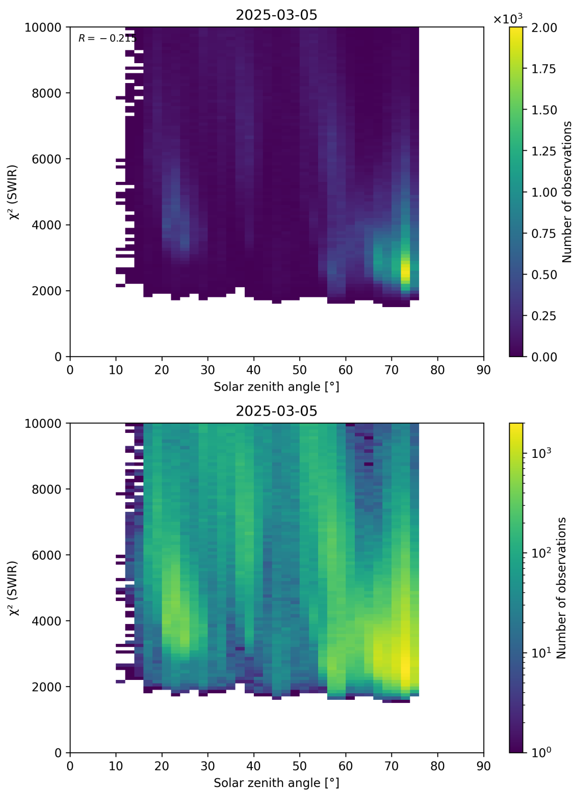
Figure 95: Scatter density plot of “Solar zenith angle” against “ \chi^2 (SWIR)” for 2025-03-04 to 2025-03-06.
