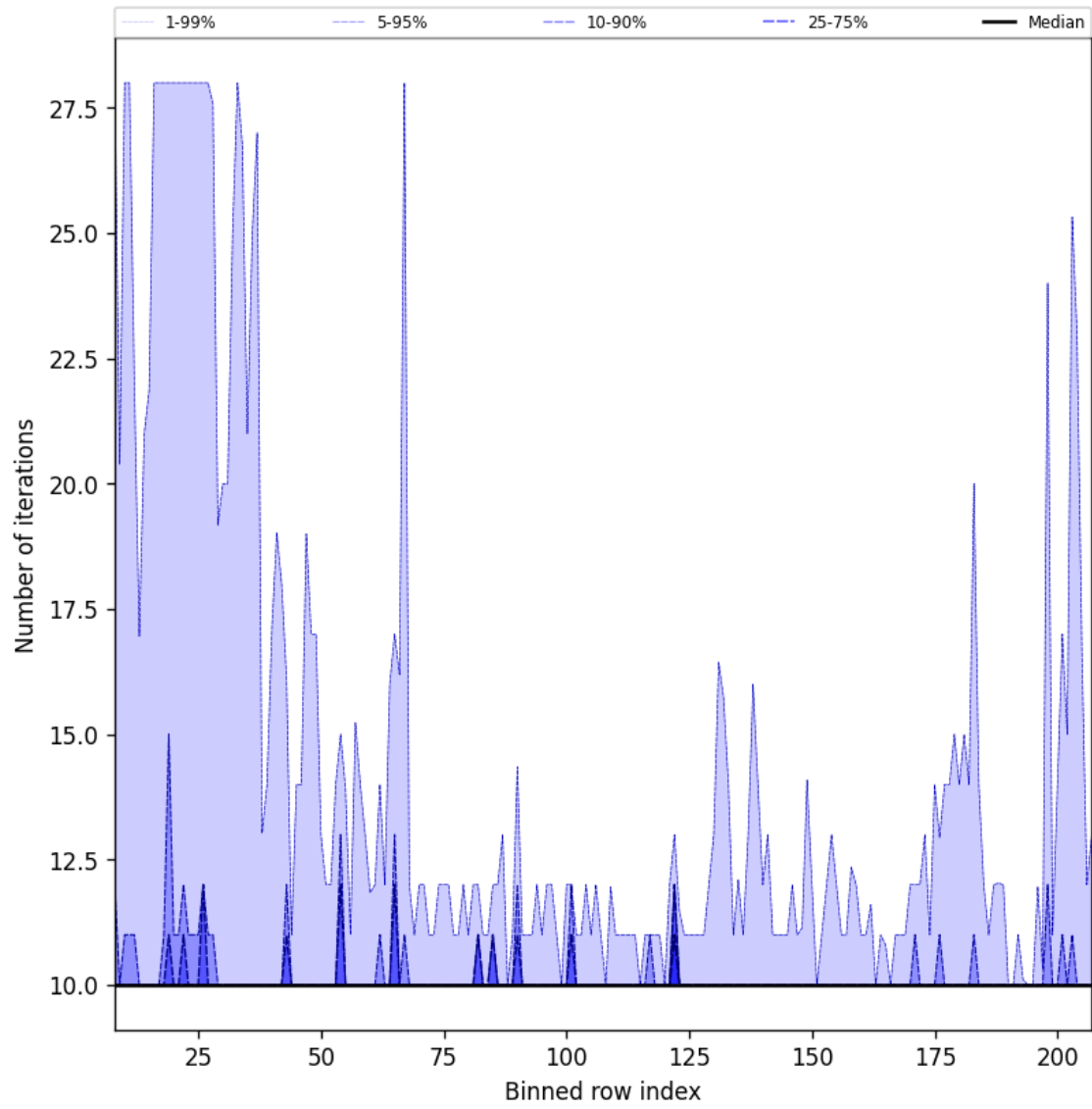
Figure 42: Along track statistics of “Number of iterations” for 2025-03-04 to 2025-03-06
