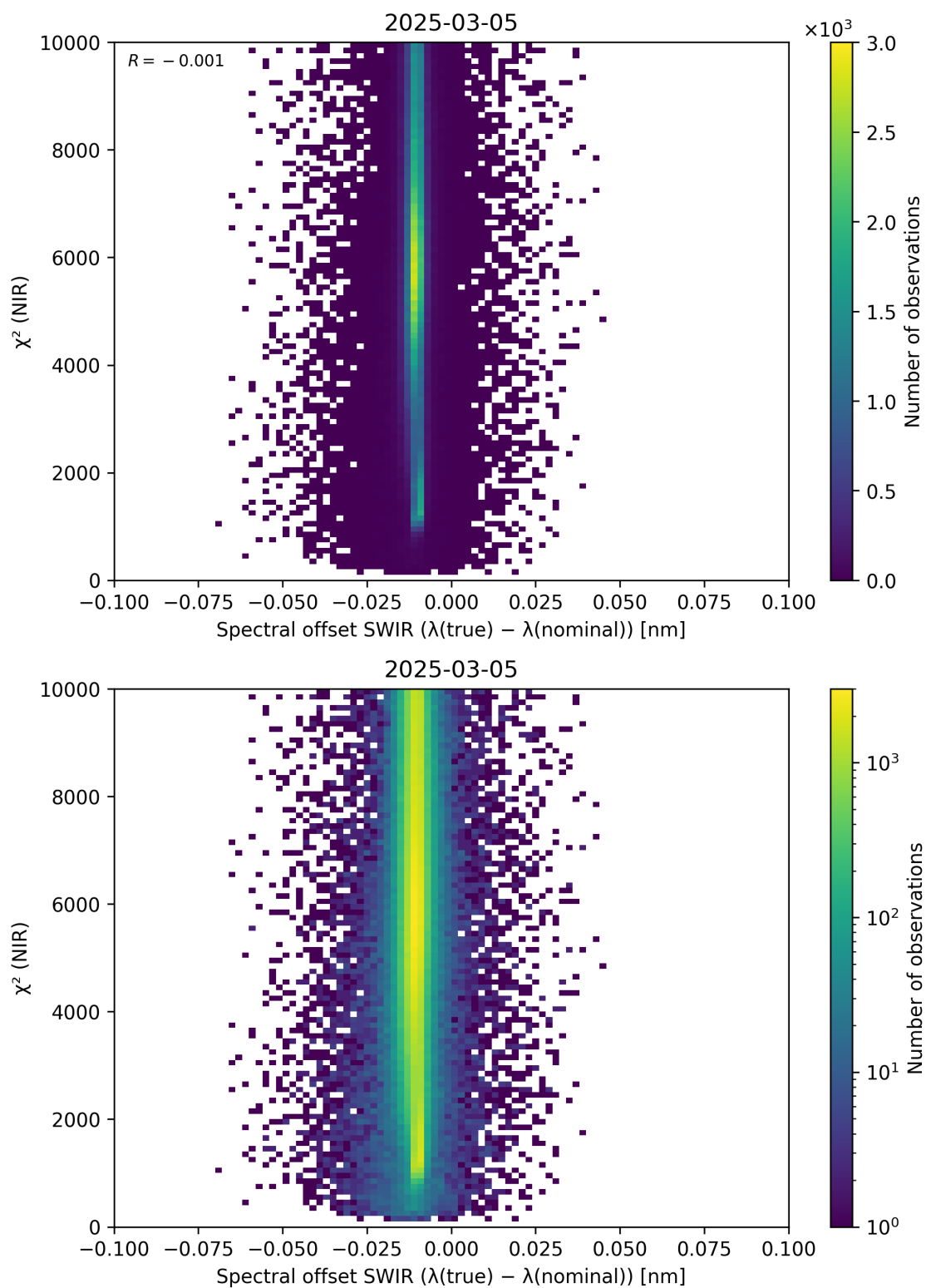
Figure 117: Scatter density plot of “Spectral offset SWIR ( \lambda_{\text{true}} - \lambda_{\text{nominal}} )” against “ \chi^2 (NIR)” for 2025-03-04 to 2025-03-06.
