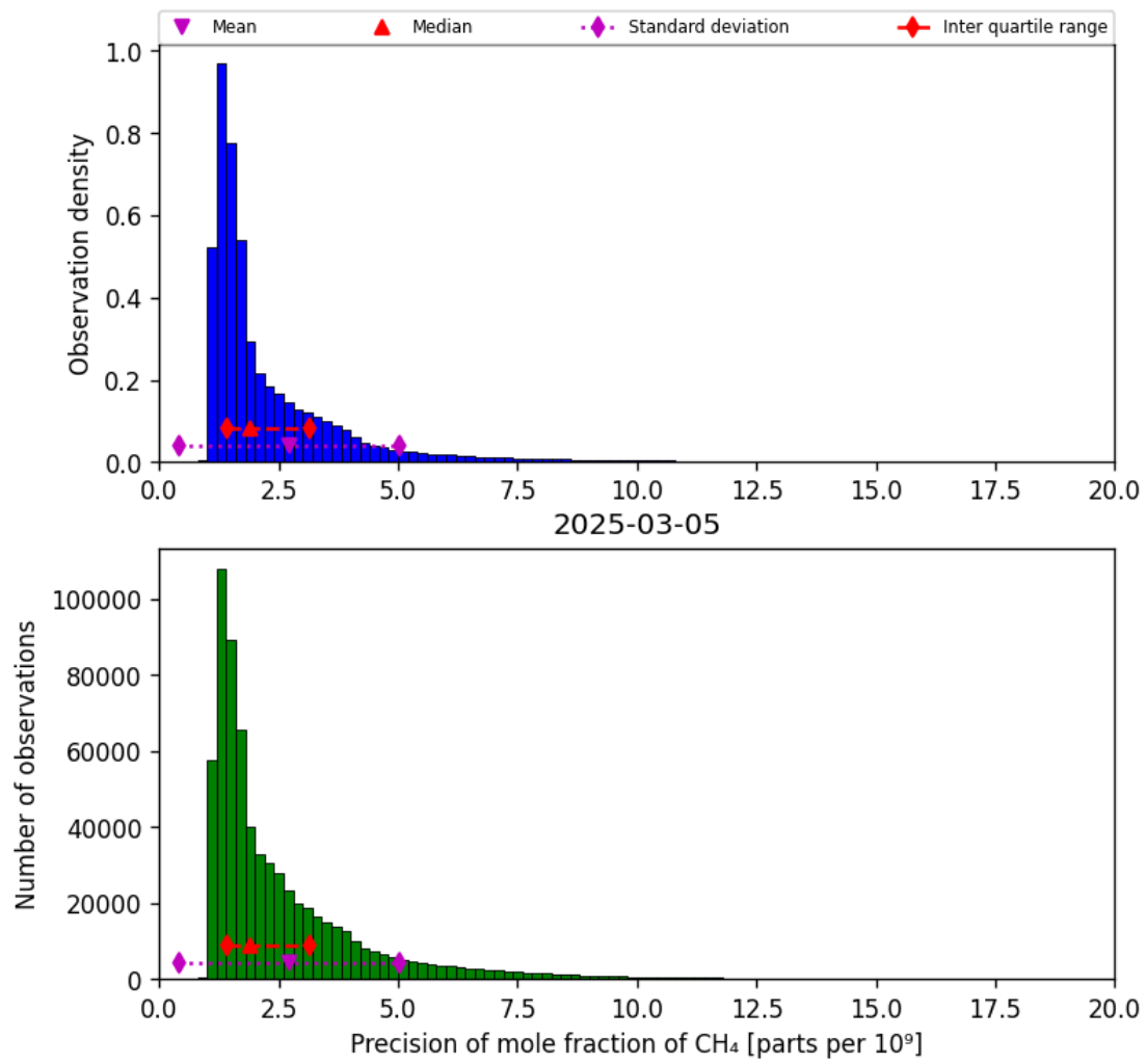
Figure 24: Histogram of “Precision of mole fraction of CH 4 ” for 2025-03-04 to 2025-03-06
