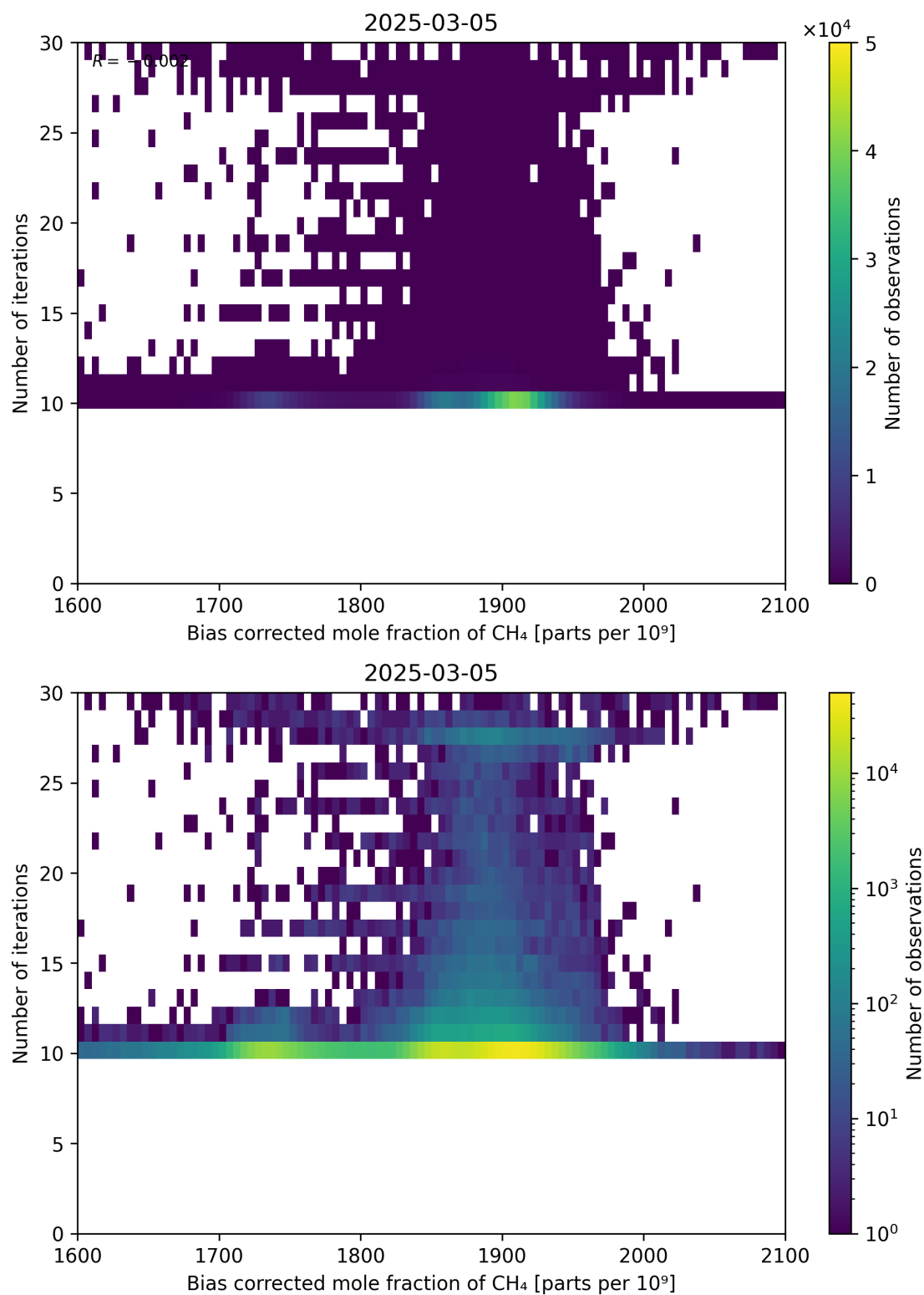
Figure 67: Scatter density plot of “Bias corrected mole fraction of \text{CH}_4 ” against “Number of iterations” for 2025-03-04 to 2025-03-06.
