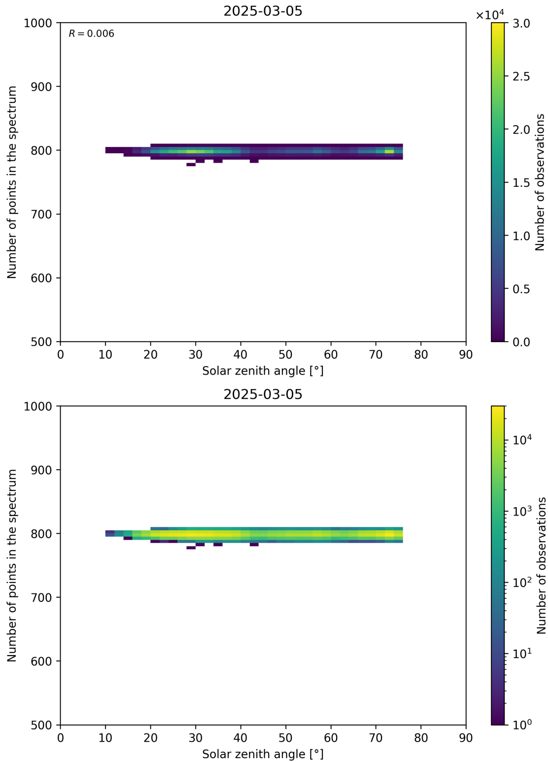
Figure 103: Scatter density plot of “Solar zenith angle” against “Number of points in the spectrum” for 2025-03-04 to 2025-03-06.
