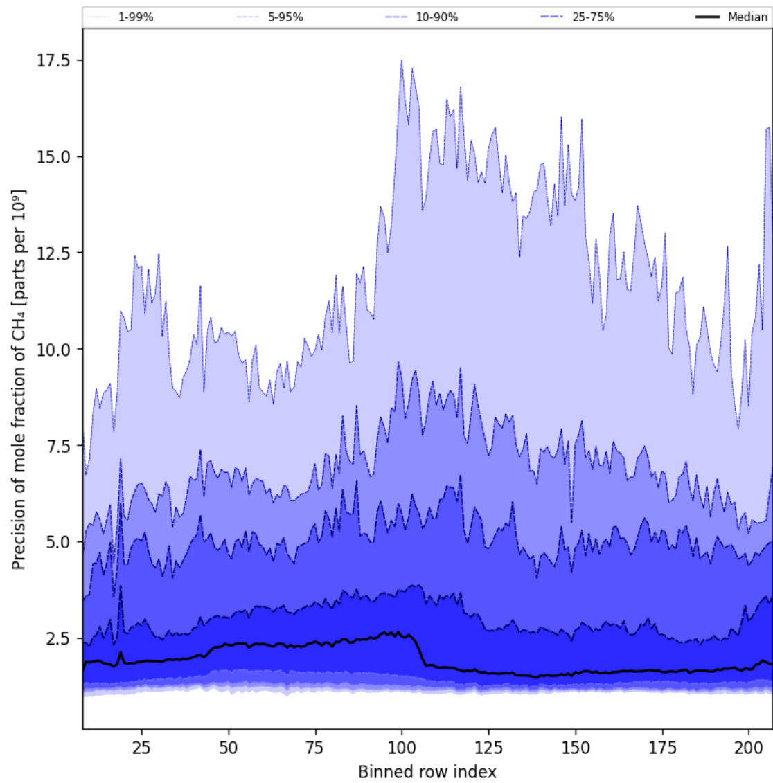
Figure 35: Along track statistics of “Precision of mole fraction of CH 4 ” for 2025-03-04 to 2025-03-06
