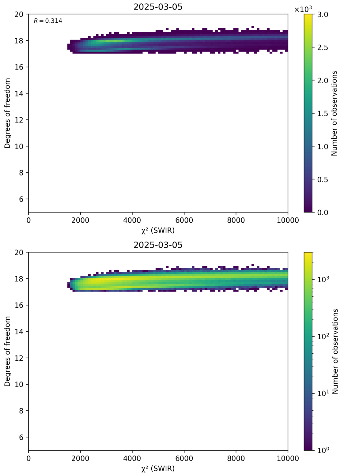
Figure 48: Scatter density plot of “ \chi^2 (SWIR)” against “Degrees of freedom” for 2025-03-04 to 2025-03-06.
