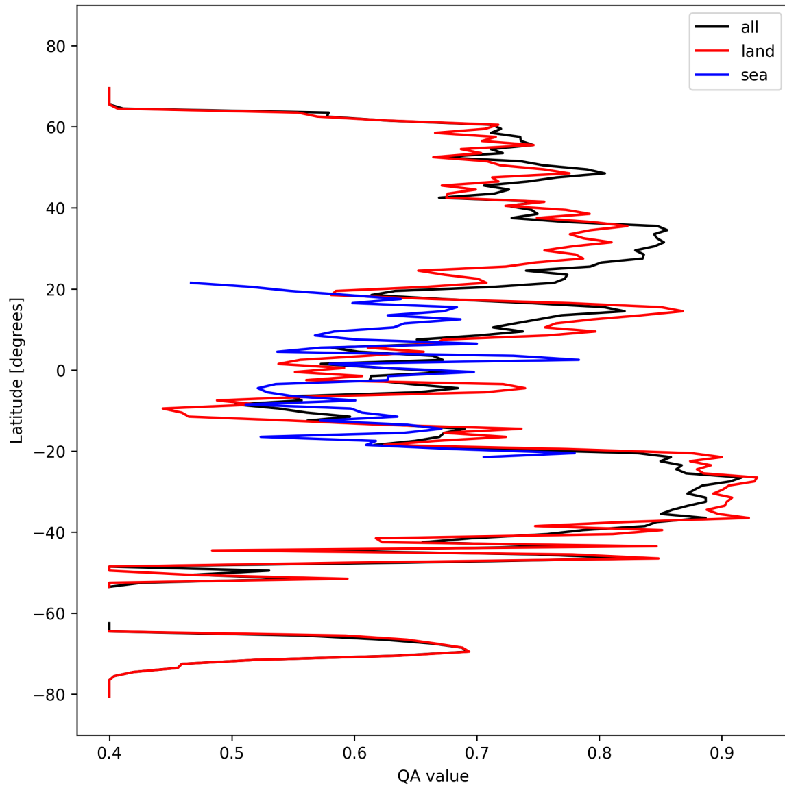
Figure 11: Zonal average of “QA value” for 2025-03-04 to 2025-03-06.
