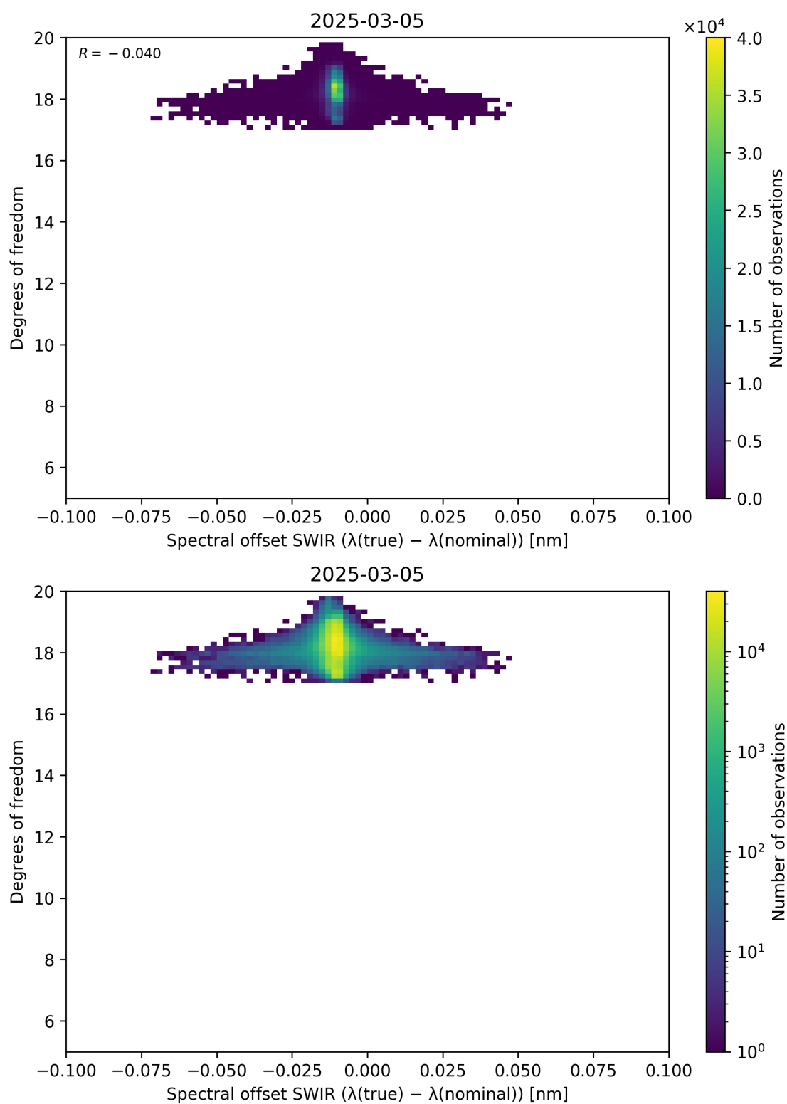
Figure 119: Scatter density plot of “Spectral offset SWIR ( \lambda_{\text{true}} - \lambda_{\text{nominal}} )” against “Degrees of freedom” for 2025-03-04 to 2025-03-06.
