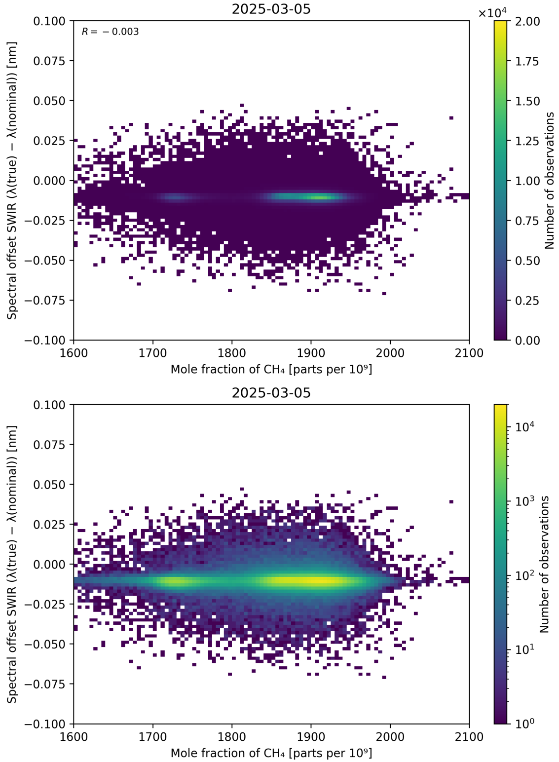
Figure 86: Scatter density plot of “Mole fraction of CH 4 ” against “Spectral offset SWIR ( \lambda_{\text{true}} - \lambda_{\text{nominal}} )” for 2025-03-04 to 2025-03-06.
