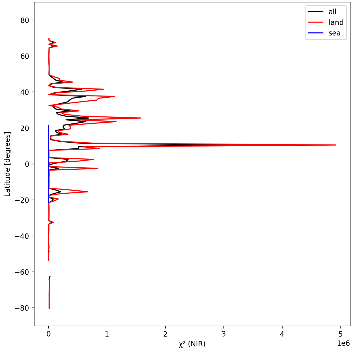
Figure 18: Zonal average of “ \chi^2 (NIR)” for 2025-03-04 to 2025-03-06.
