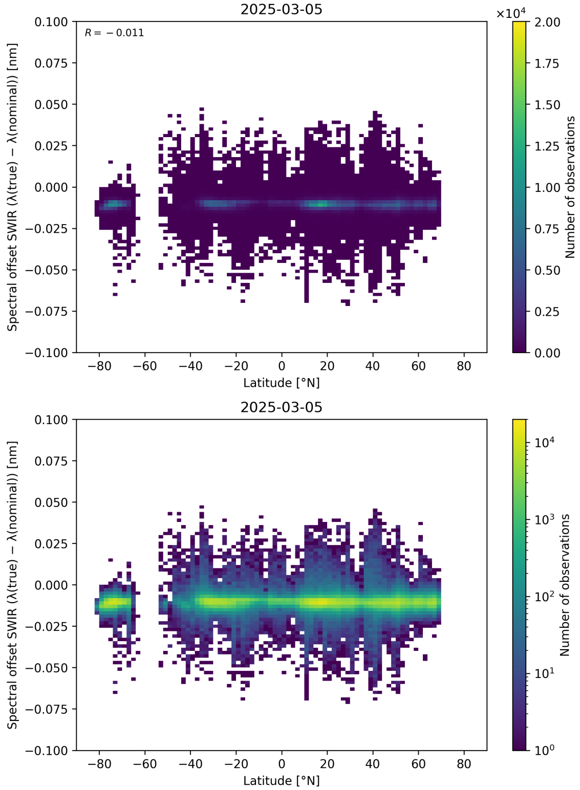
Figure 62: Scatter density plot of “Latitude” against “Spectral offset SWIR ( \lambda_{\text{true}} - \lambda_{\text{nominal}} )” for 2025-03-04 to 2025-03-06.
