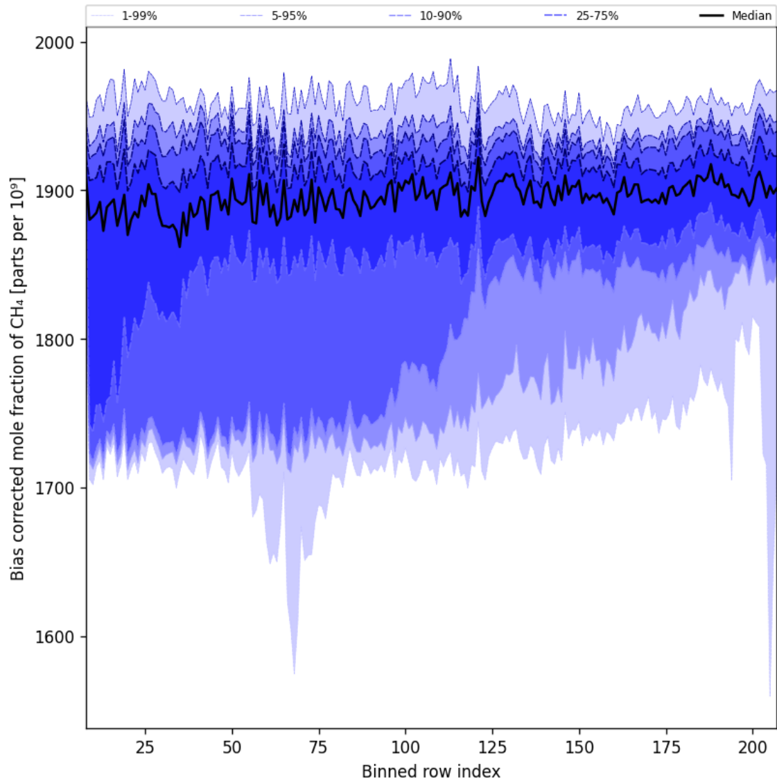
Figure 36: Along track statistics of “Bias corrected mole fraction of CH 4 ” for 2025-03-04 to 2025-03-06
