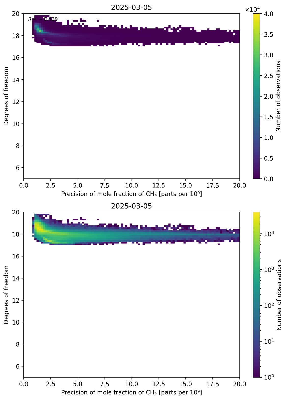
Figure 80: Scatter density plot of “Precision of mole fraction of CH 4 ” against “Degrees of freedom” for 2025-03-04 to 2025-03-06.
