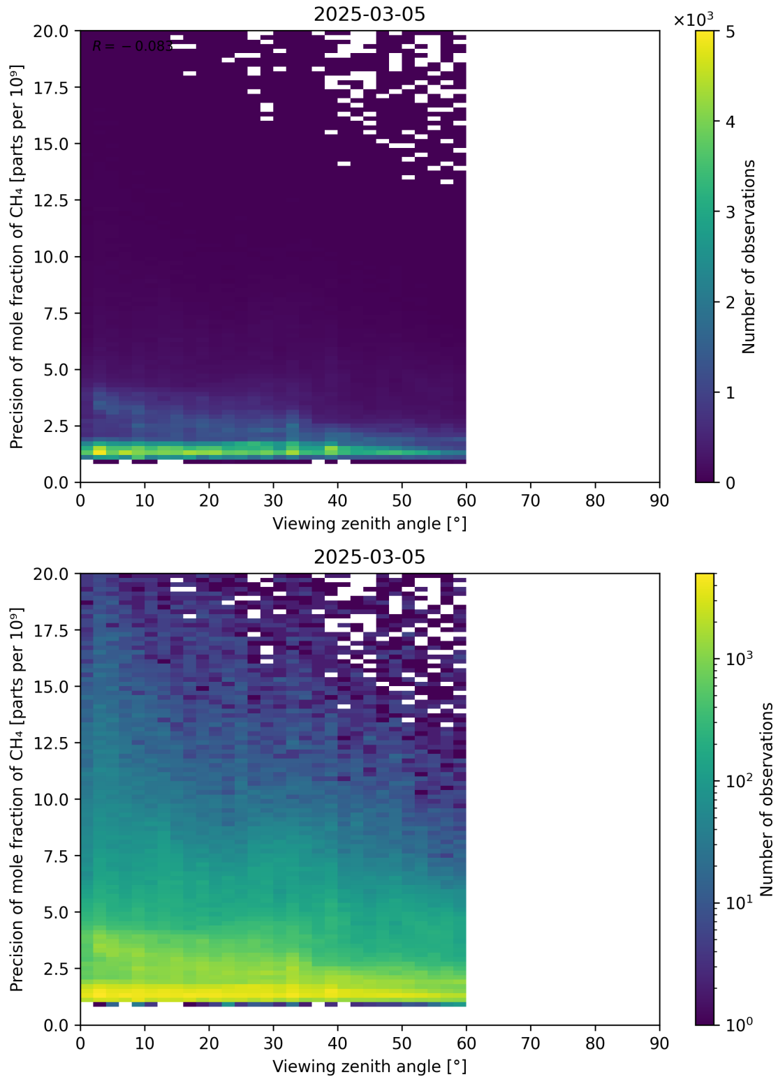
Figure 112: Scatter density plot of “Viewing zenith angle” against “Precision of mole fraction of CH 4 ” for 2025-03-04 to 2025-03-06.
