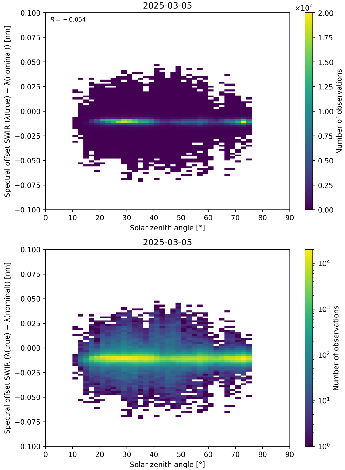
Figure 104: Scatter density plot of “Solar zenith angle” against “Spectral offset SWIR ( \lambda_{\text{true}} - \lambda_{\text{nominal}} )” for 2025-03-04 to 2025-03-06.
