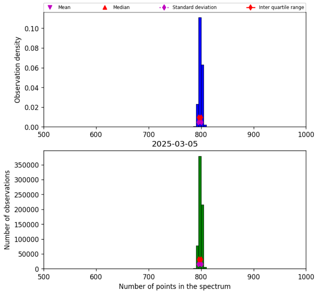
Figure 26: Histogram of “Number of points in the spectrum” for 2025-03-04 to 2025-03-06
