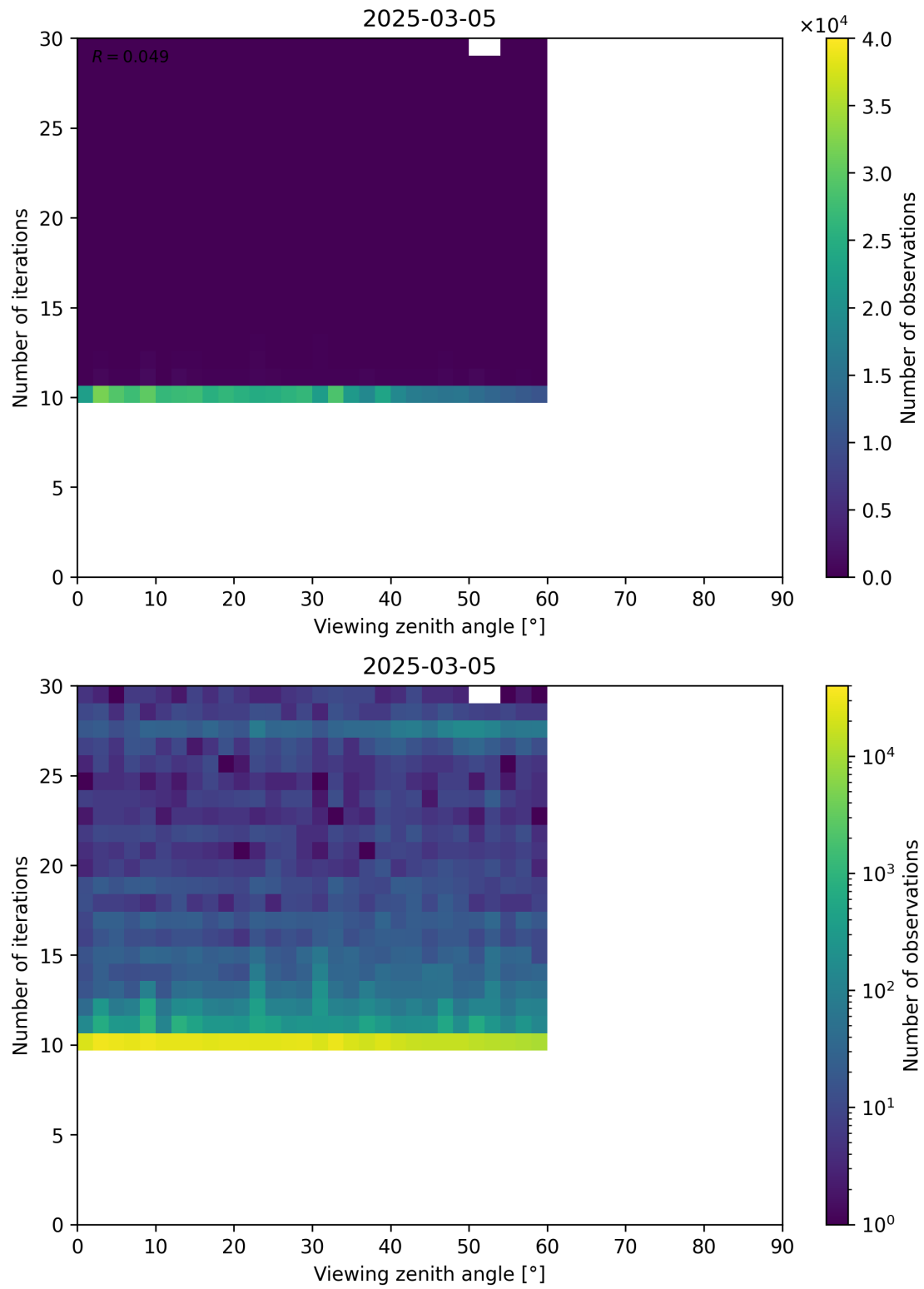
Figure 113: Scatter density plot of “Viewing zenith angle” against “Number of iterations” for 2025-03-04 to 2025-03-06.
