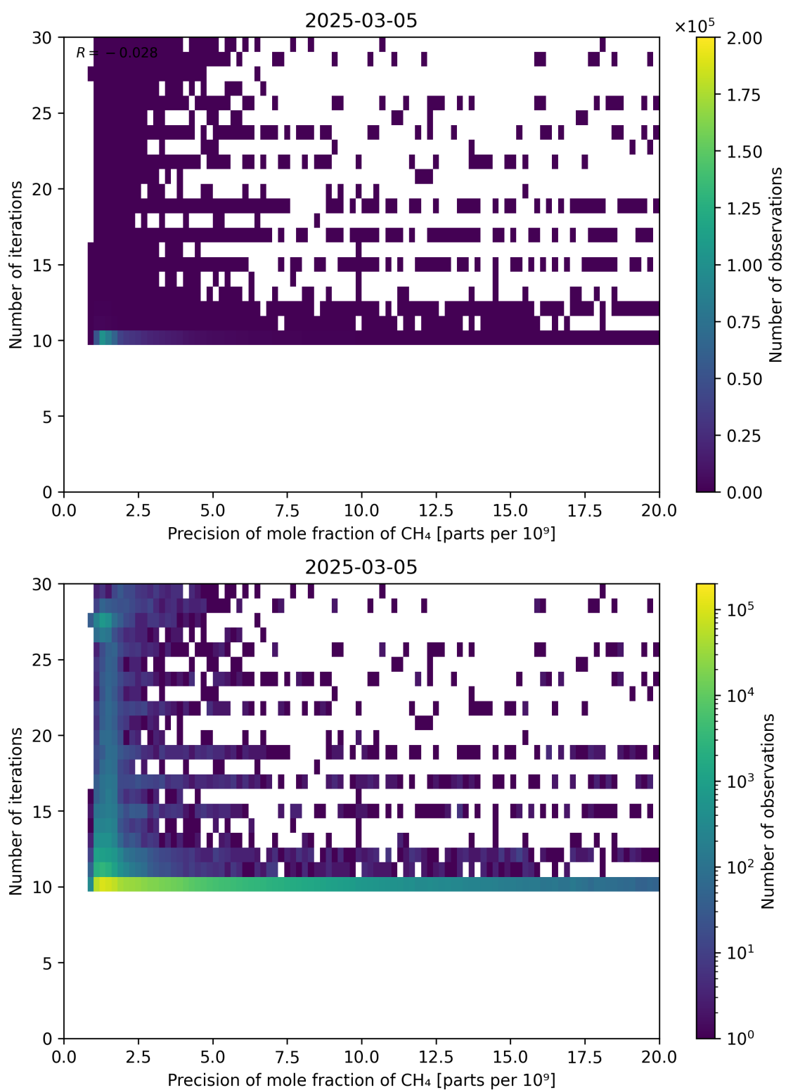
Figure 83: Scatter density plot of “Precision of mole fraction of CH 4 ” against “Number of iterations” for 2025-03-04 to 2025-03-06.
