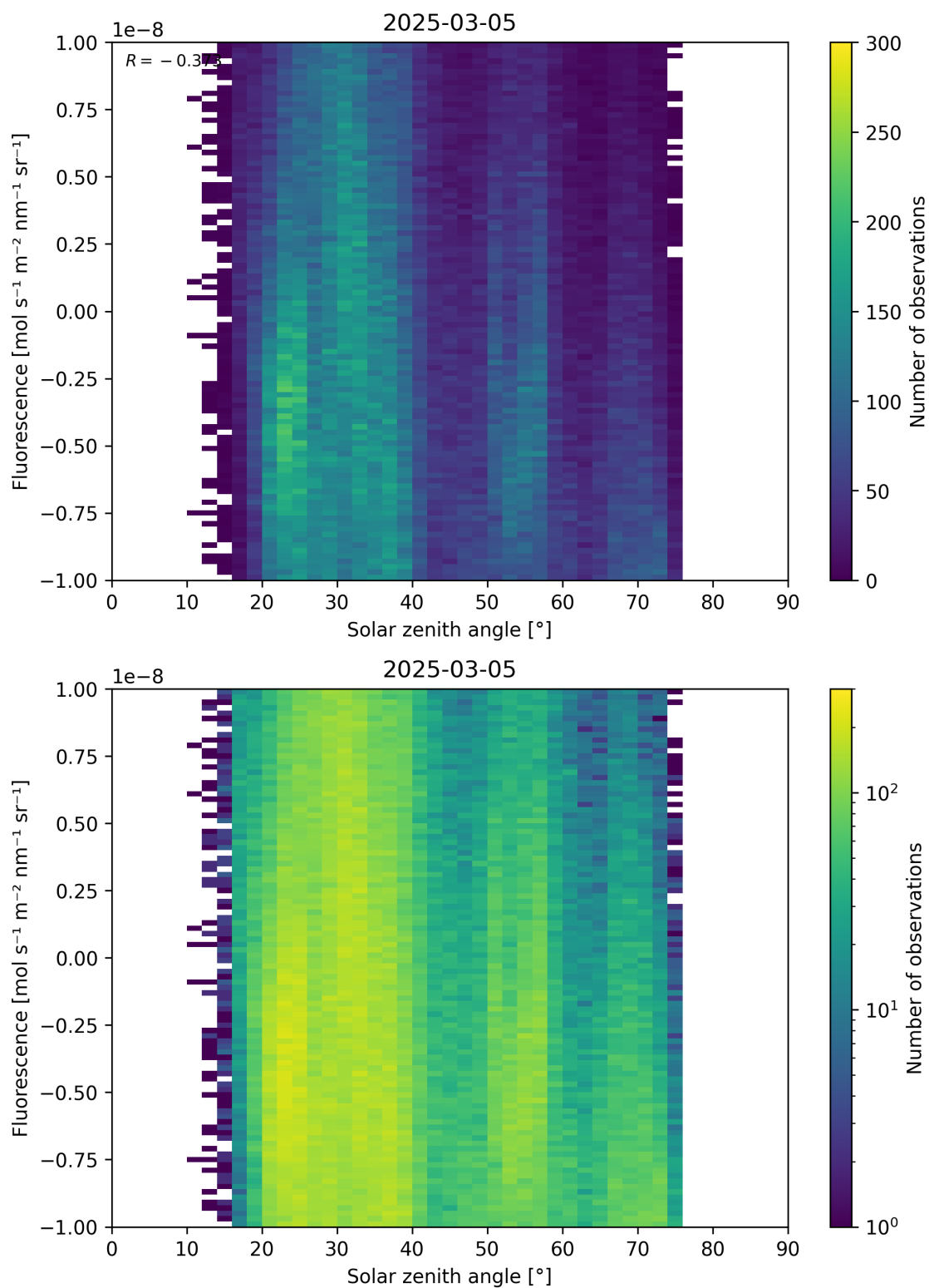
Figure 97: Scatter density plot of “Solar zenith angle” against “Fluorescence” for 2025-03-04 to 2025-03-06.
