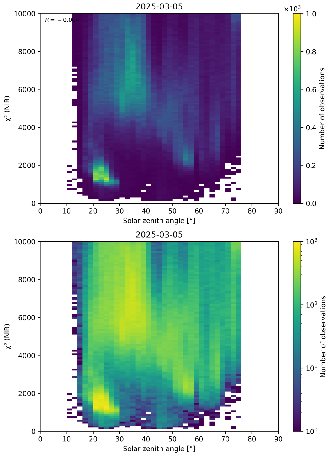
Figure 94: Scatter density plot of “Solar zenith angle” against “ \chi^2 (NIR)” for 2025-03-04 to 2025-03-06.
