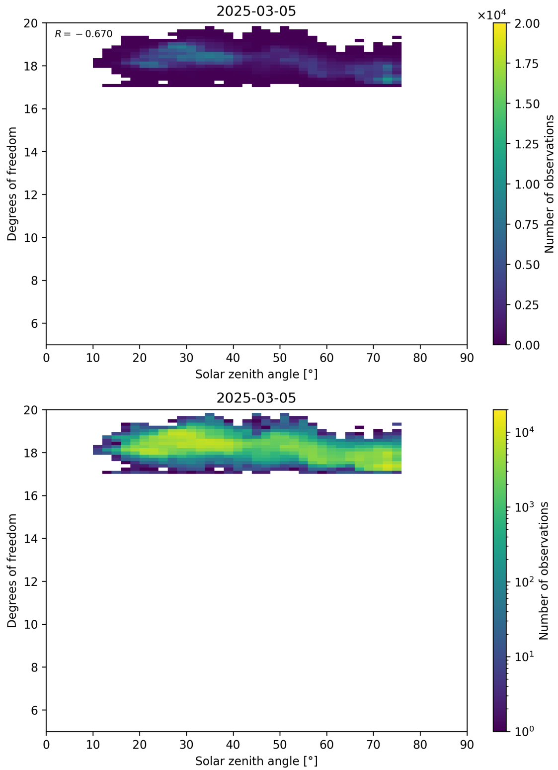
Figure 96: Scatter density plot of “Solar zenith angle” against “Degrees of freedom” for 2025-03-04 to 2025-03-06.
