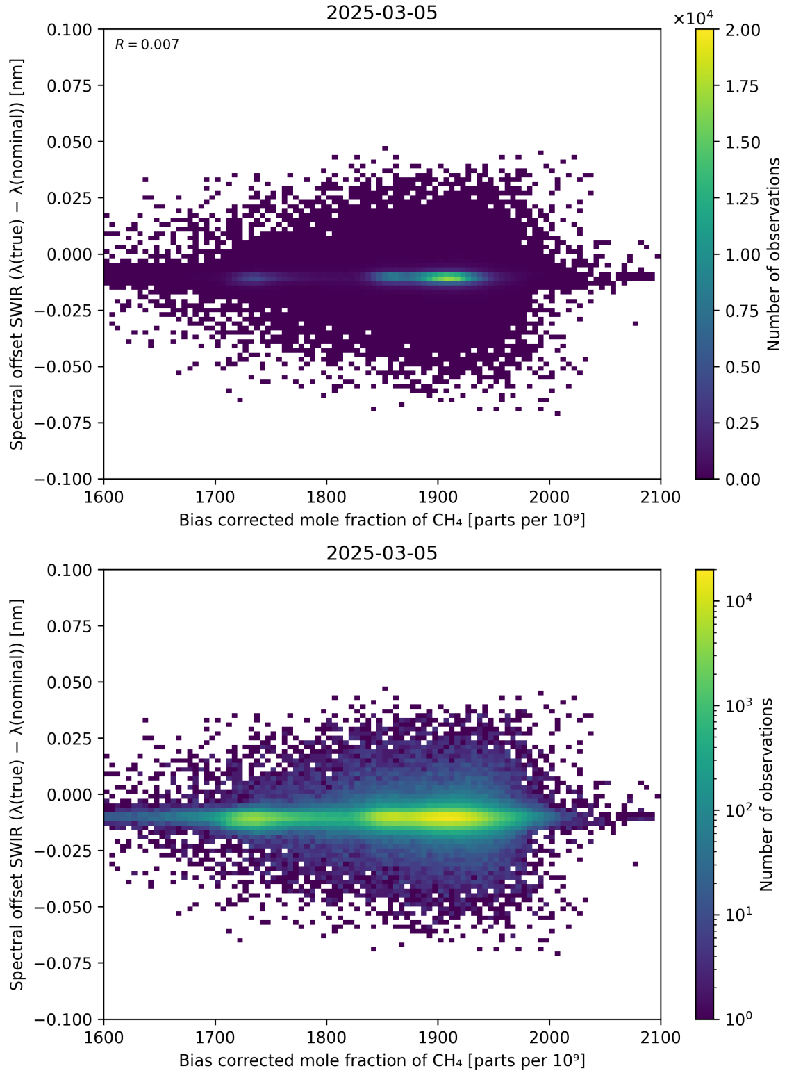
Figure 69: Scatter density plot of “Bias corrected mole fraction of \text{CH}_4 ” against “Spectral offset SWIR ( \lambda_{\text{true}} - \lambda_{\text{nominal}} )” for 2025-03-04 to 2025-03-06.
