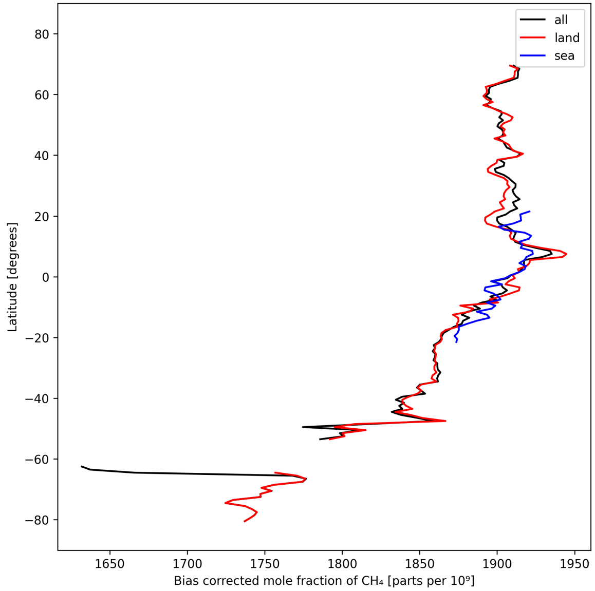
Figure 14: Zonal average of “Bias corrected mole fraction of CH 4 ” for 2025-03-04 to 2025-03-06.
