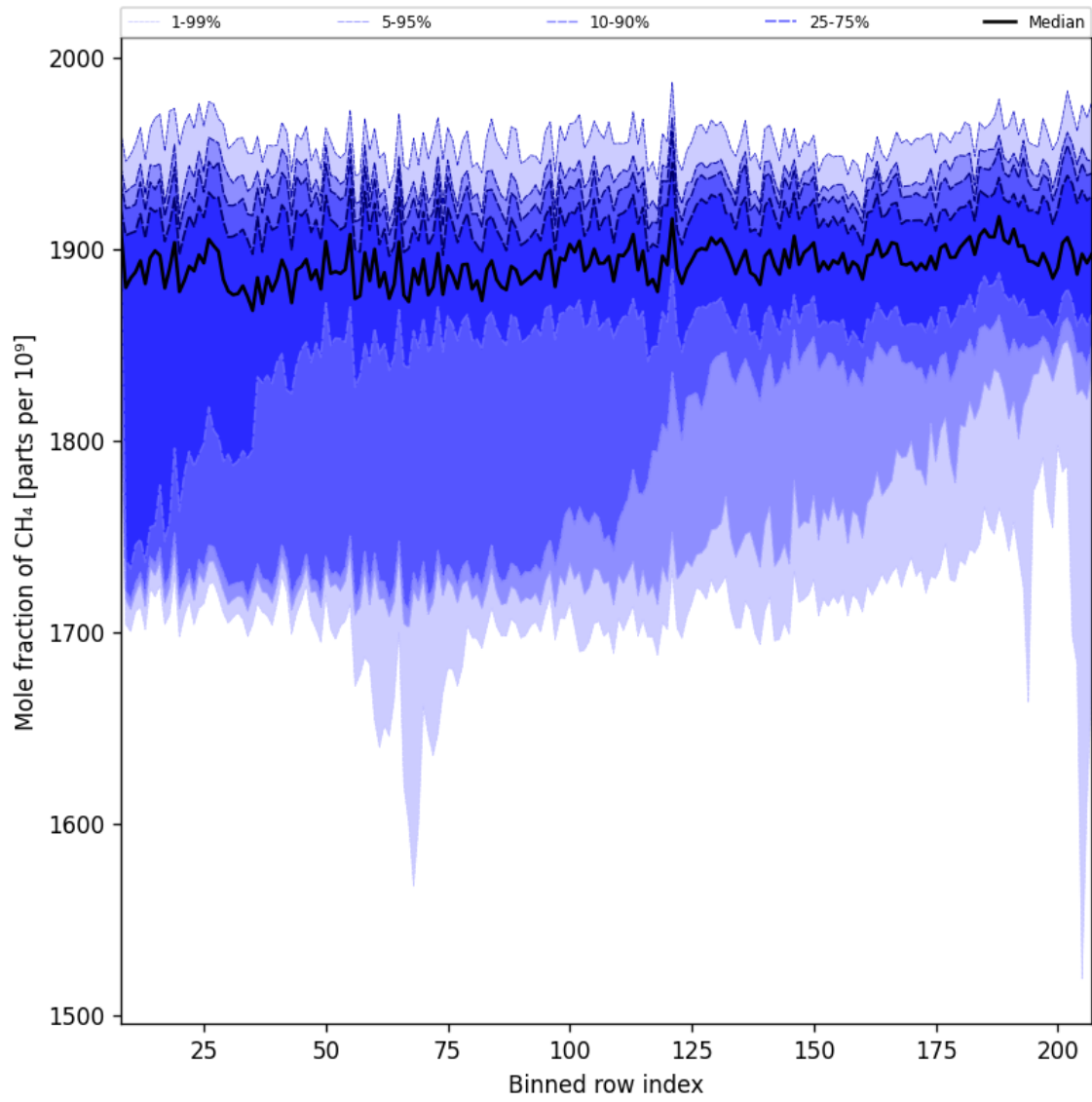
Figure 34: Along track statistics of “Mole fraction of CH 4 ” for 2025-03-04 to 2025-03-06
