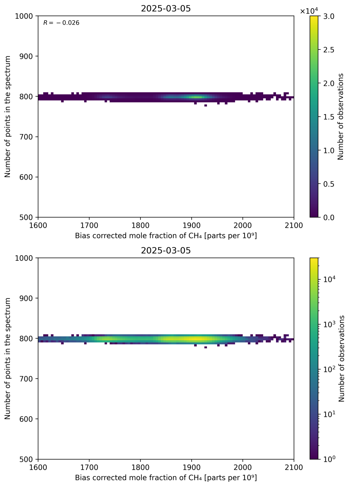
Figure 68: Scatter density plot of “Bias corrected mole fraction of CH 4 ” against “Number of points in the spectrum” for 2025-03-04 to 2025-03-06.
