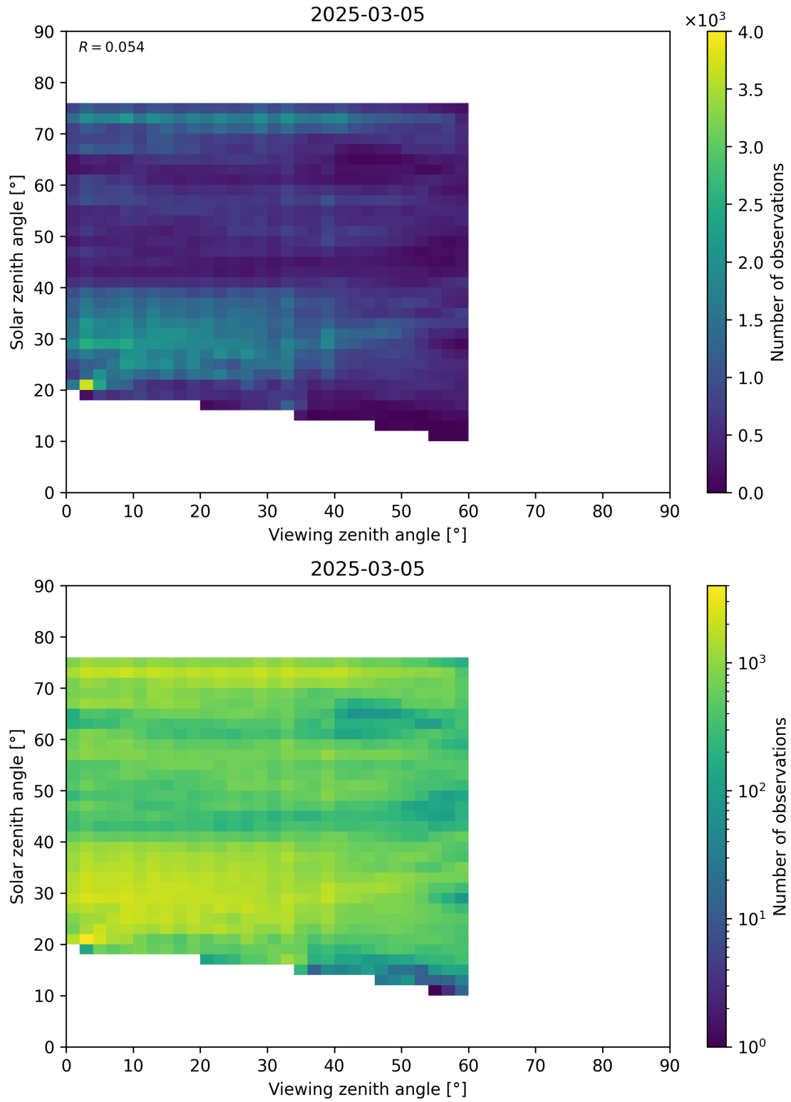
Figure 115: Scatter density plot of “Viewing zenith angle” against “Solar zenith angle” for 2025-03-04 to 2025-03-06.
