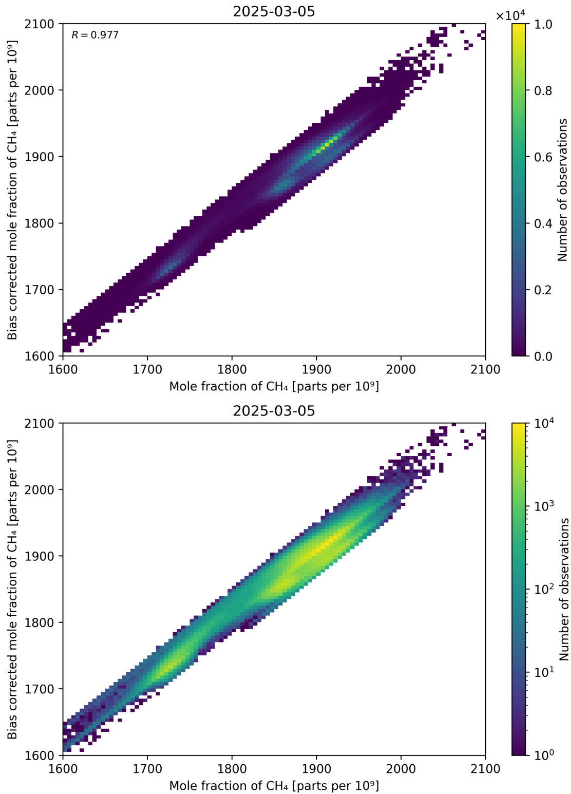
Figure 74: Scatter density plot of “Mole fraction of CH 4 ” against “Bias corrected mole fraction of CH 4 ” for 2025-03-04 to 2025-03-06.
