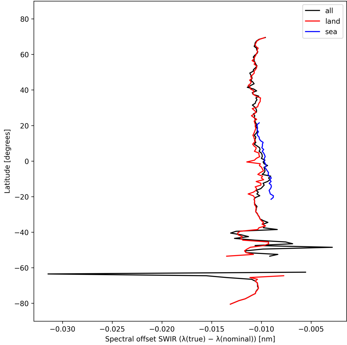
Figure 16: Zonal average of “Spectral offset SWIR ( \lambda_{\text{true}} - \lambda_{\text{nominal}} )” for 2025-03-04 to 2025-03-06.
