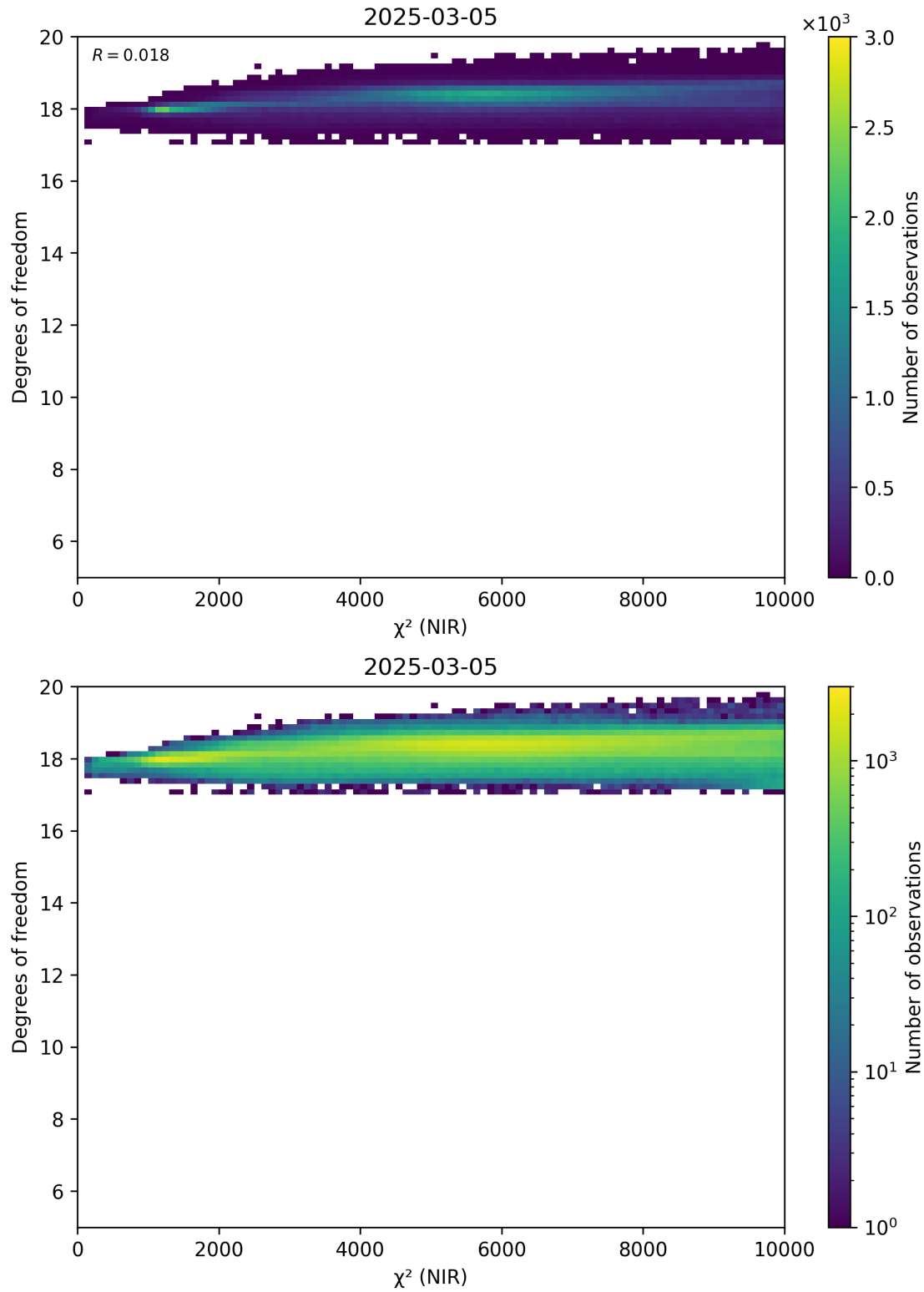
Figure 44: Scatter density plot of “ \chi^2 (NIR)” against “Degrees of freedom” for 2025-03-04 to 2025-03-06.
