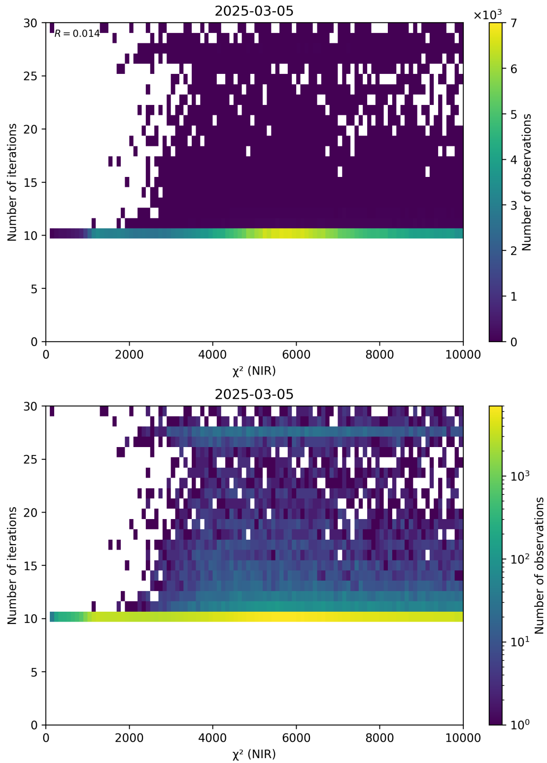
Figure 46: Scatter density plot of “ \chi^2 (NIR)” against “Number of iterations” for 2025-03-04 to 2025-03-06.
