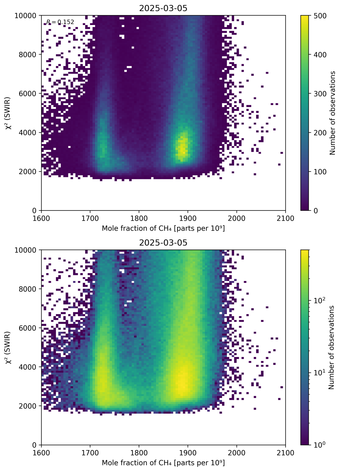
Figure 71: Scatter density plot of “Mole fraction of \text{CH}_4 ” against “ \chi^2 (SWIR)” for 2025-03-04 to 2025-03-06.
