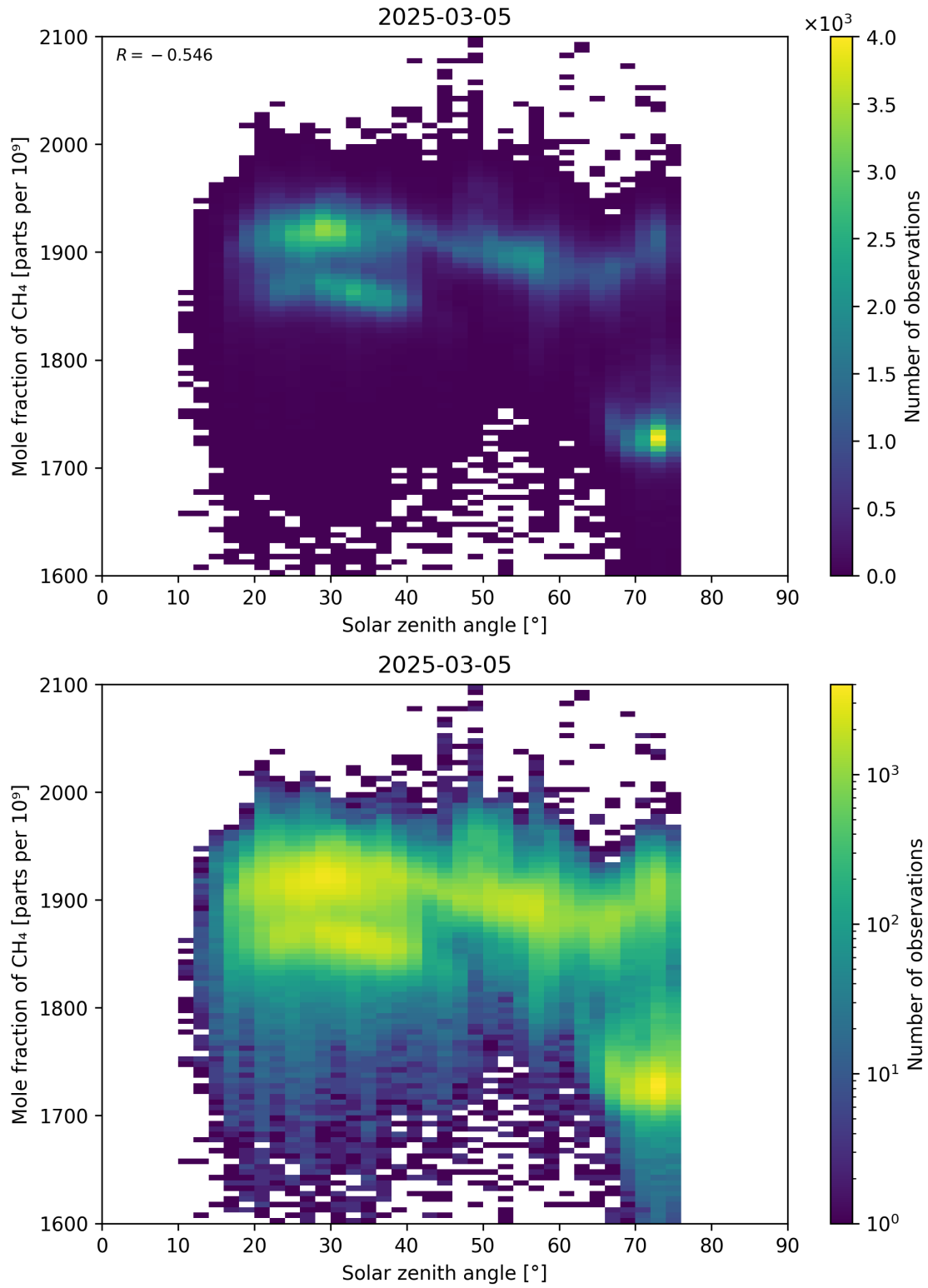
Figure 99: Scatter density plot of “Solar zenith angle” against “Mole fraction of CH 4 ” for 2025-03-04 to 2025-03-06.
