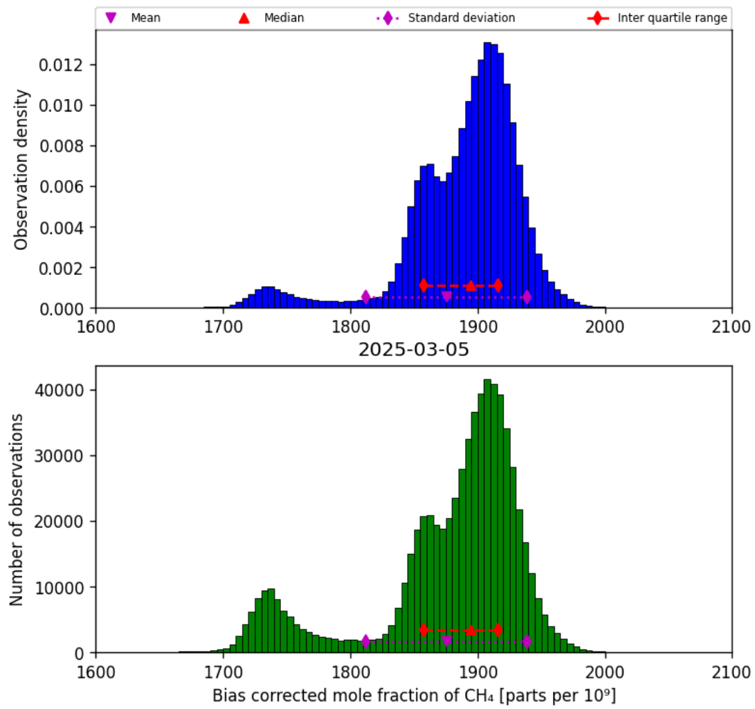
Figure 25: Histogram of “Bias corrected mole fraction of CH 4 ” for 2025-03-04 to 2025-03-06
