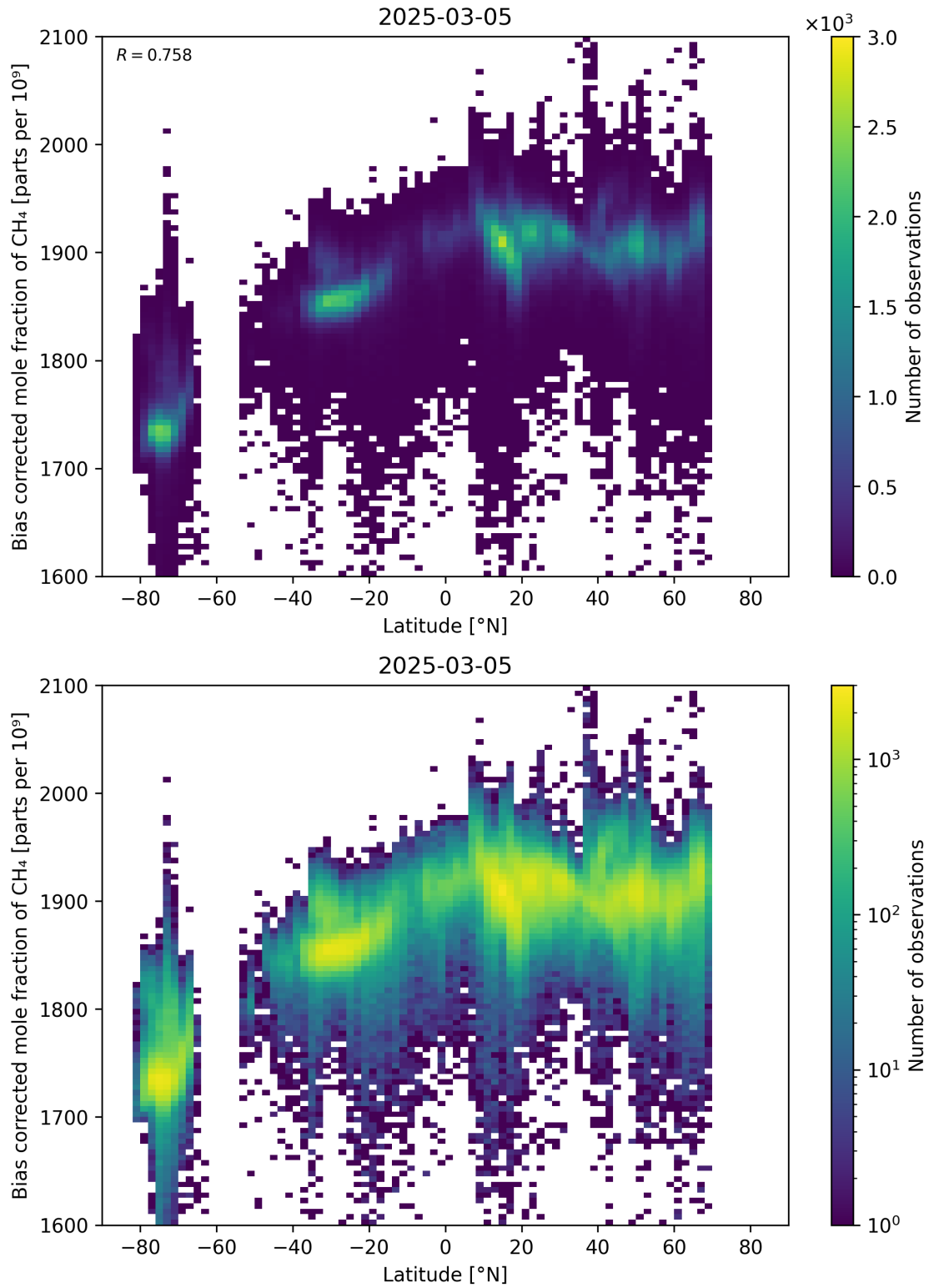
Figure 58: Scatter density plot of “Latitude” against “Bias corrected mole fraction of CH 4 ” for 2025-03-04 to 2025-03-06.
