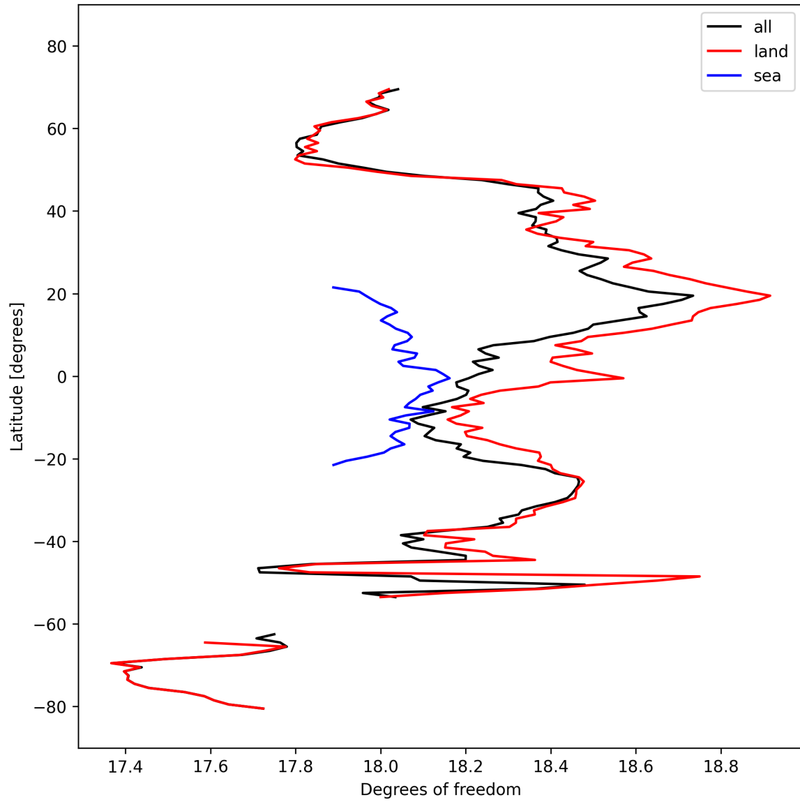
Figure 19: Zonal average of “Degrees of freedom” for 2025-03-04 to 2025-03-06.
