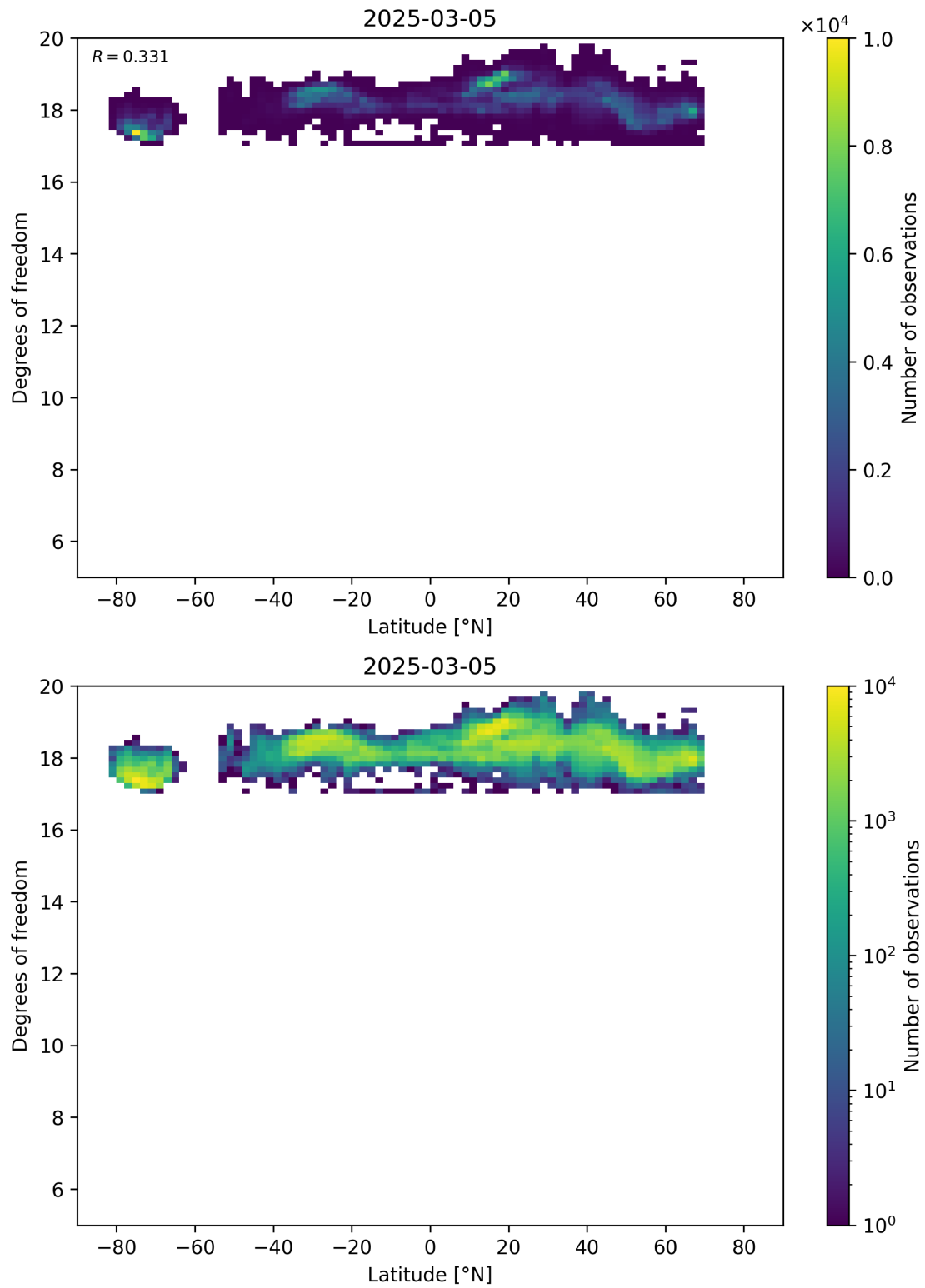
Figure 55: Scatter density plot of “Latitude” against “Degrees of freedom” for 2025-03-04 to 2025-03-06.
