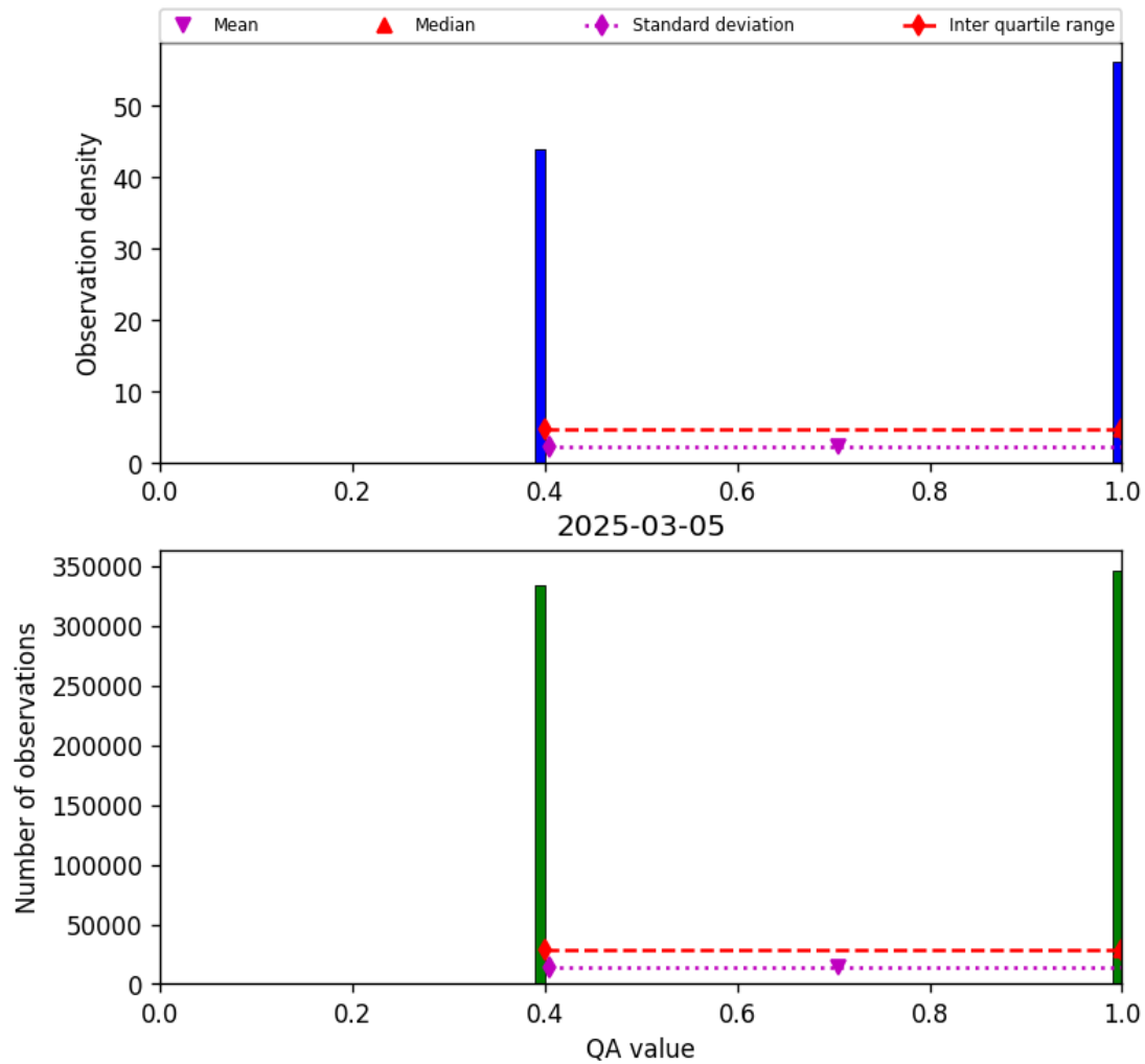
Figure 22: Histogram of “QA value” for 2025-03-04 to 2025-03-06
