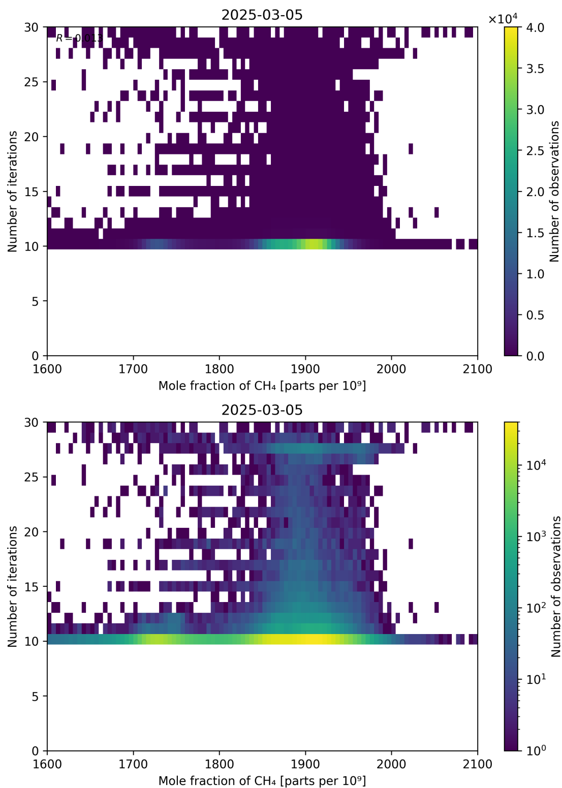
Figure 76: Scatter density plot of “Mole fraction of CH 4 ” against “Number of iterations” for 2025-03-04 to 2025-03-06.
