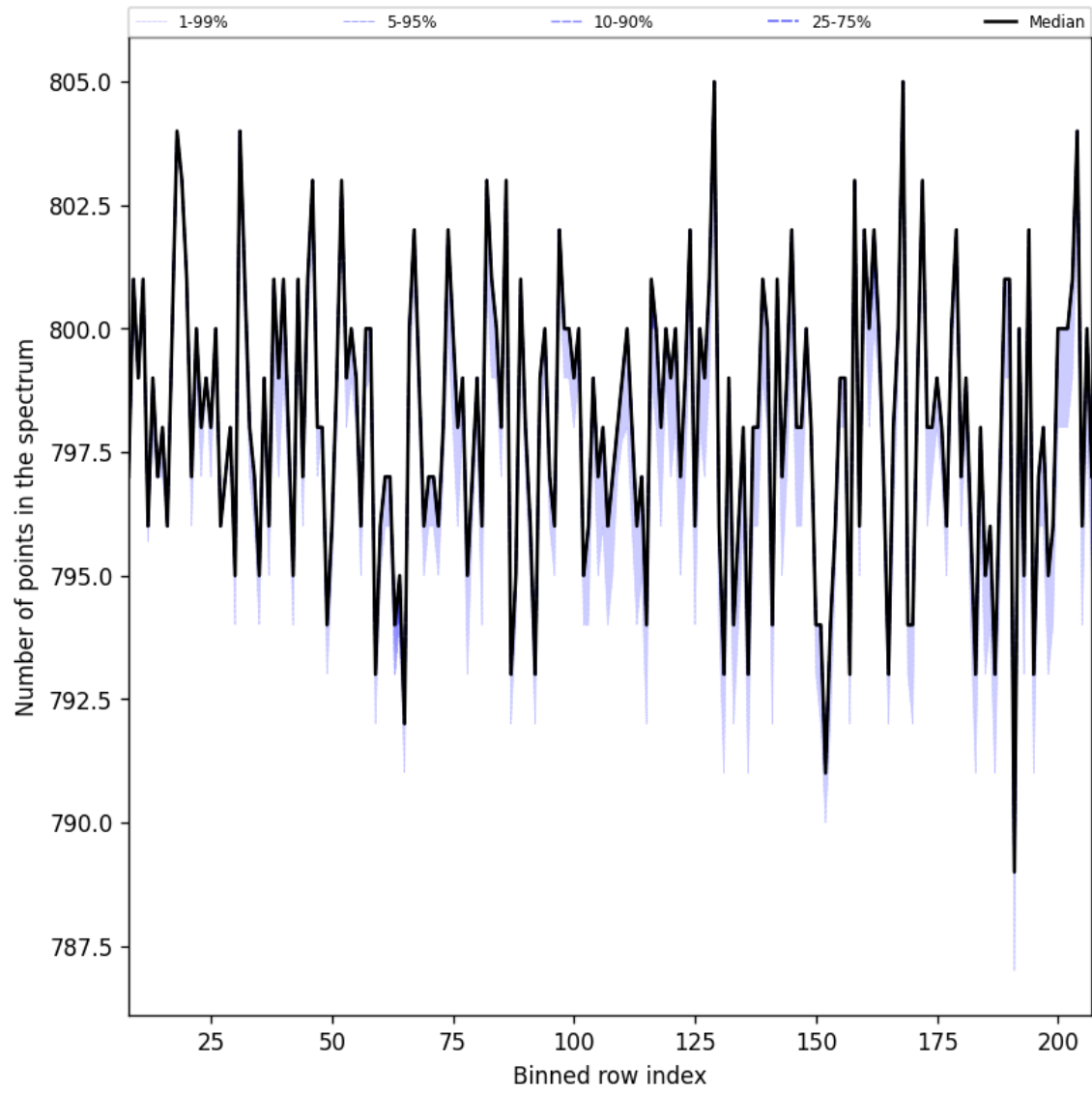
Figure 37: Along track statistics of “Number of points in the spectrum” for 2025-03-04 to 2025-03-06
