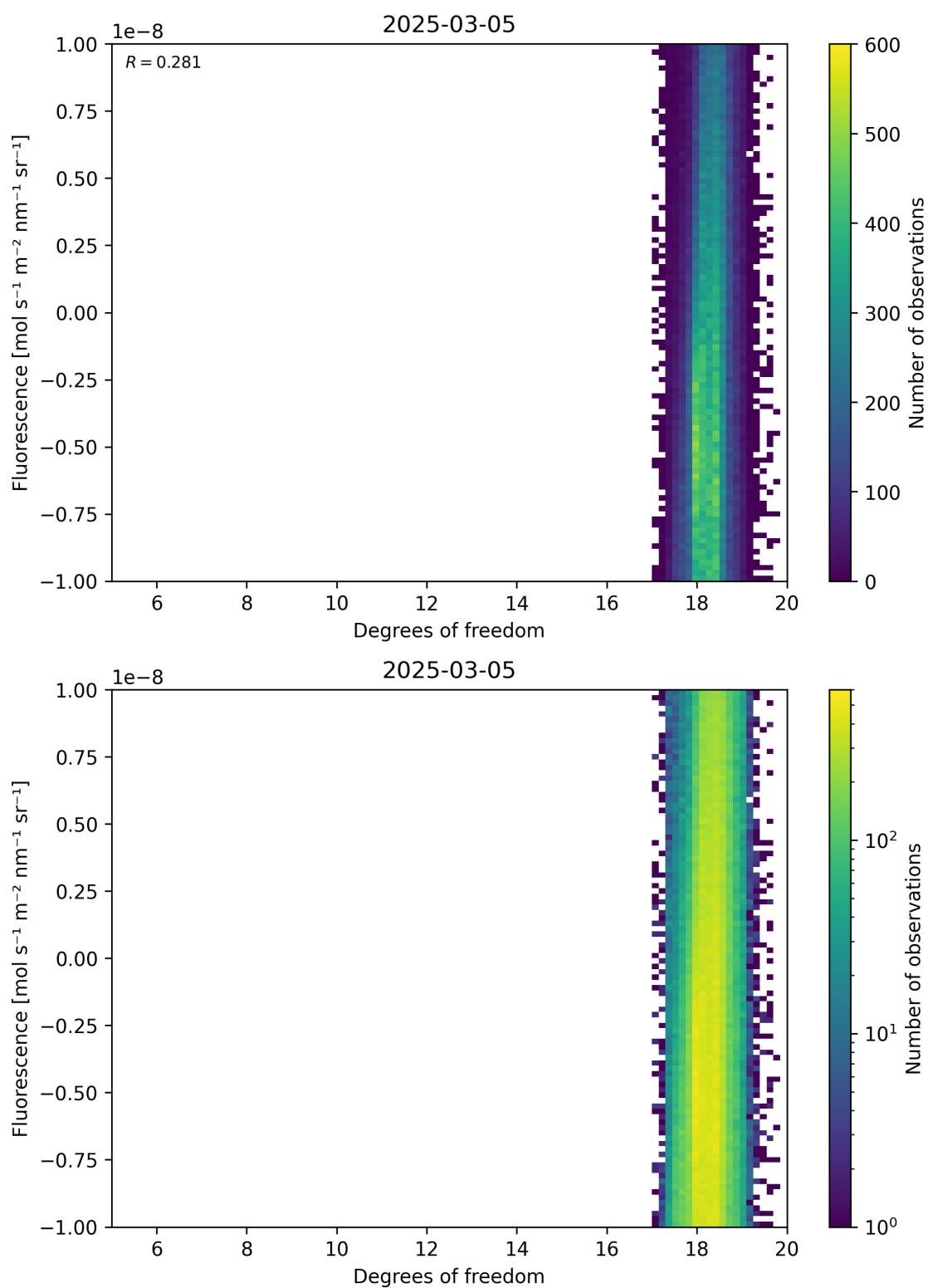
Figure 51: Scatter density plot of “Degrees of freedom” against “Fluorescence” for 2025-03-04 to 2025-03-06.
