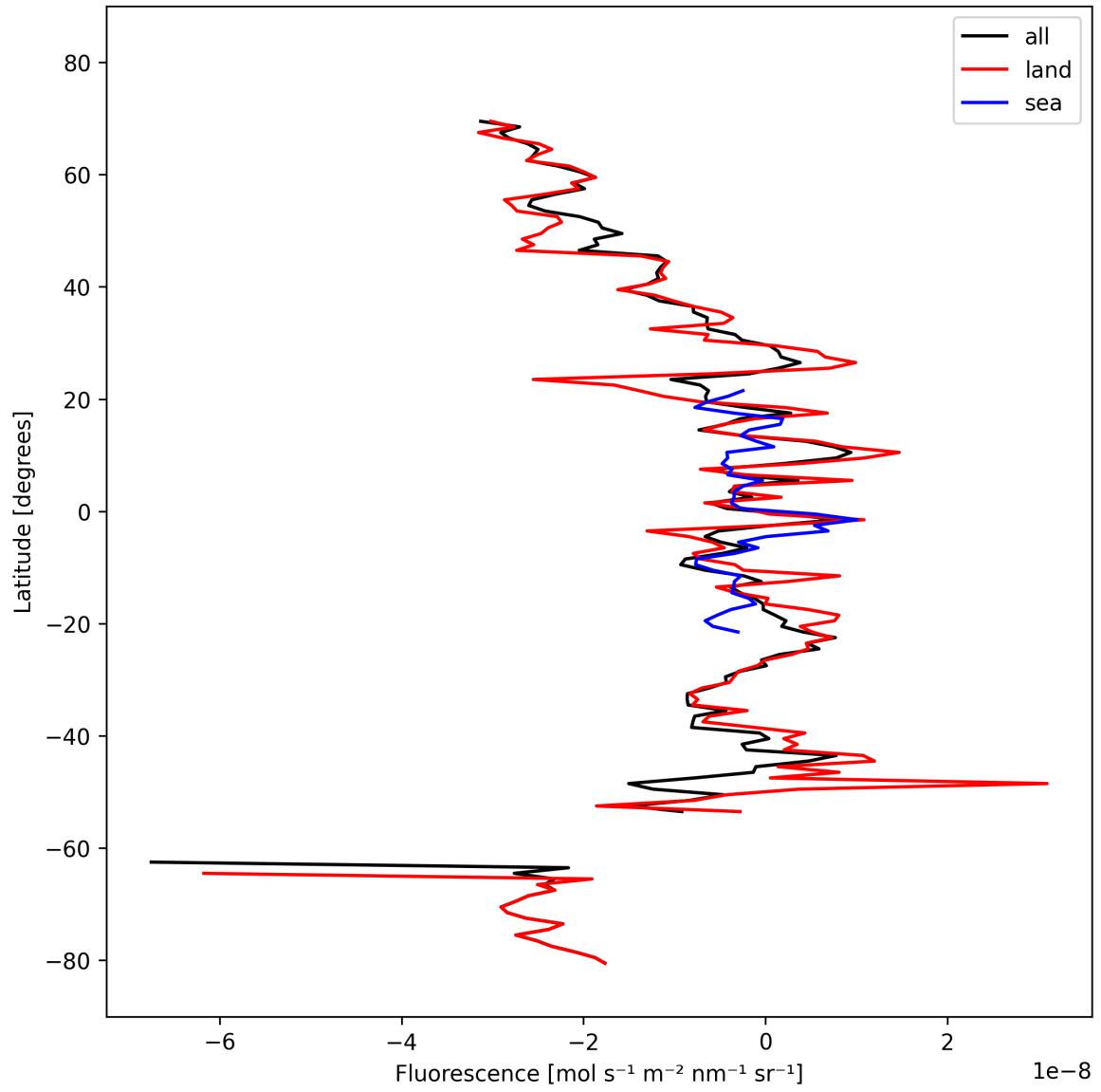
Figure 21: Zonal average of “Fluorescence” for 2025-03-04 to 2025-03-06.
