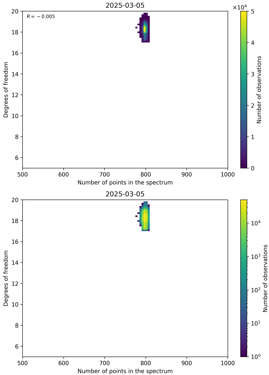
Figure 90: Scatter density plot of “Number of points in the spectrum” against “Degrees of freedom” for 2025-03-04 to 2025-03-06.
