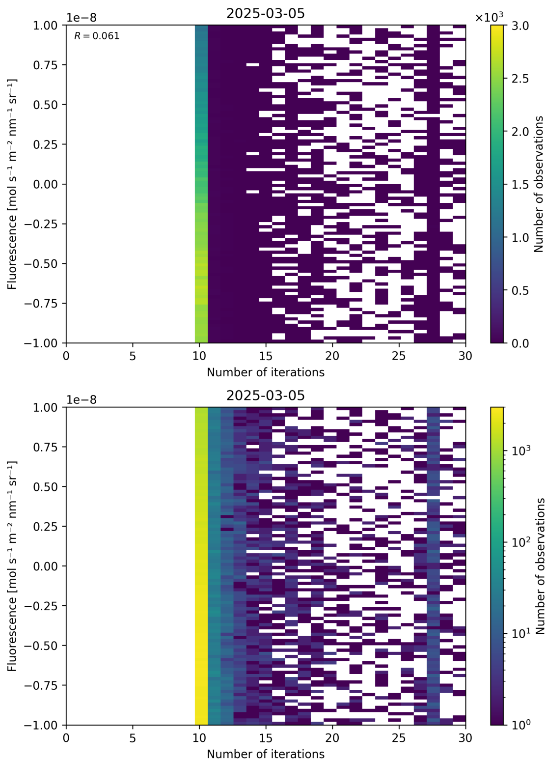
Figure 87: Scatter density plot of “Number of iterations” against “Fluorescence” for 2025-03-04 to 2025-03-06.
