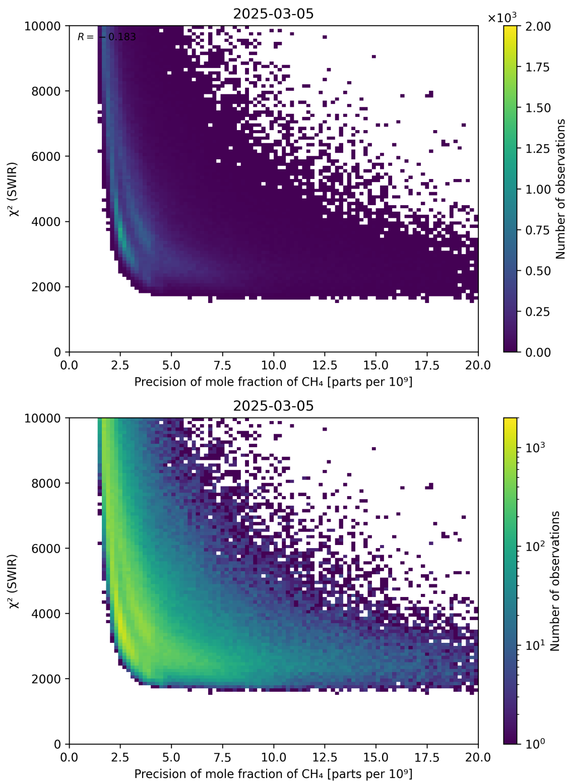
Figure 79: Scatter density plot of “Precision of mole fraction of \text{CH}_4 ” against “ \chi^2 (SWIR)” for 2025-03-04 to 2025-03-06.
