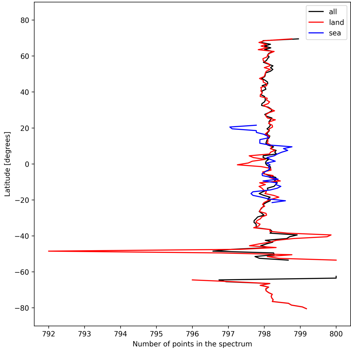
Figure 15: Zonal average of “Number of points in the spectrum” for 2025-03-04 to 2025-03-06.
