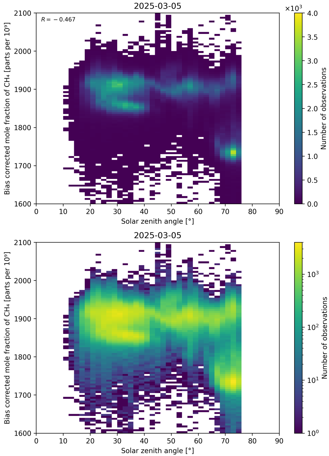
Figure 100: Scatter density plot of “Solar zenith angle” against “Bias corrected mole fraction of CH 4 ” for 2025-03-04 to 2025-03-06.
