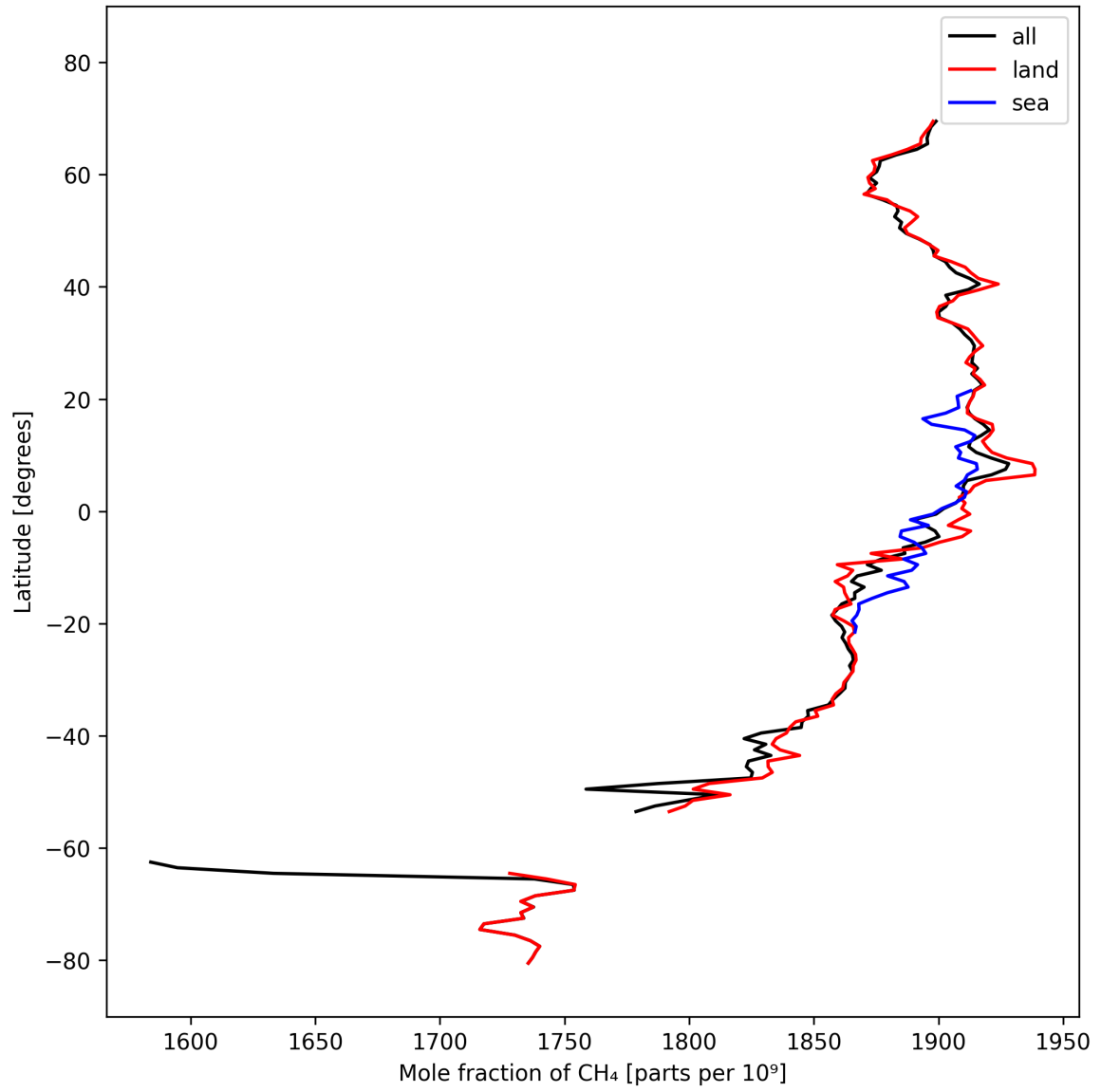
Figure 12: Zonal average of “Mole fraction of CH 4 ” for 2025-03-04 to 2025-03-06.
