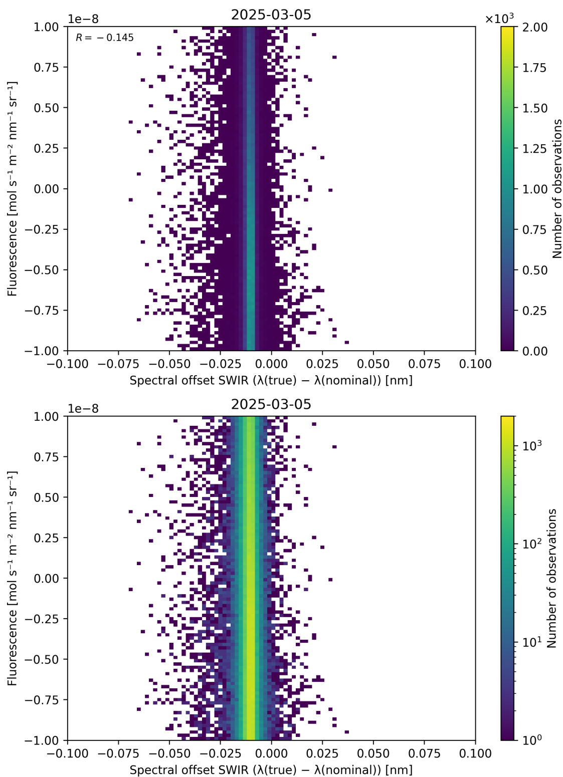
Figure 120: Scatter density plot of “Spectral offset SWIR ( \lambda_{\text{true}} - \lambda_{\text{nominal}} )” against “Fluorescence” for 2025-03-04 to 2025-03-06.
