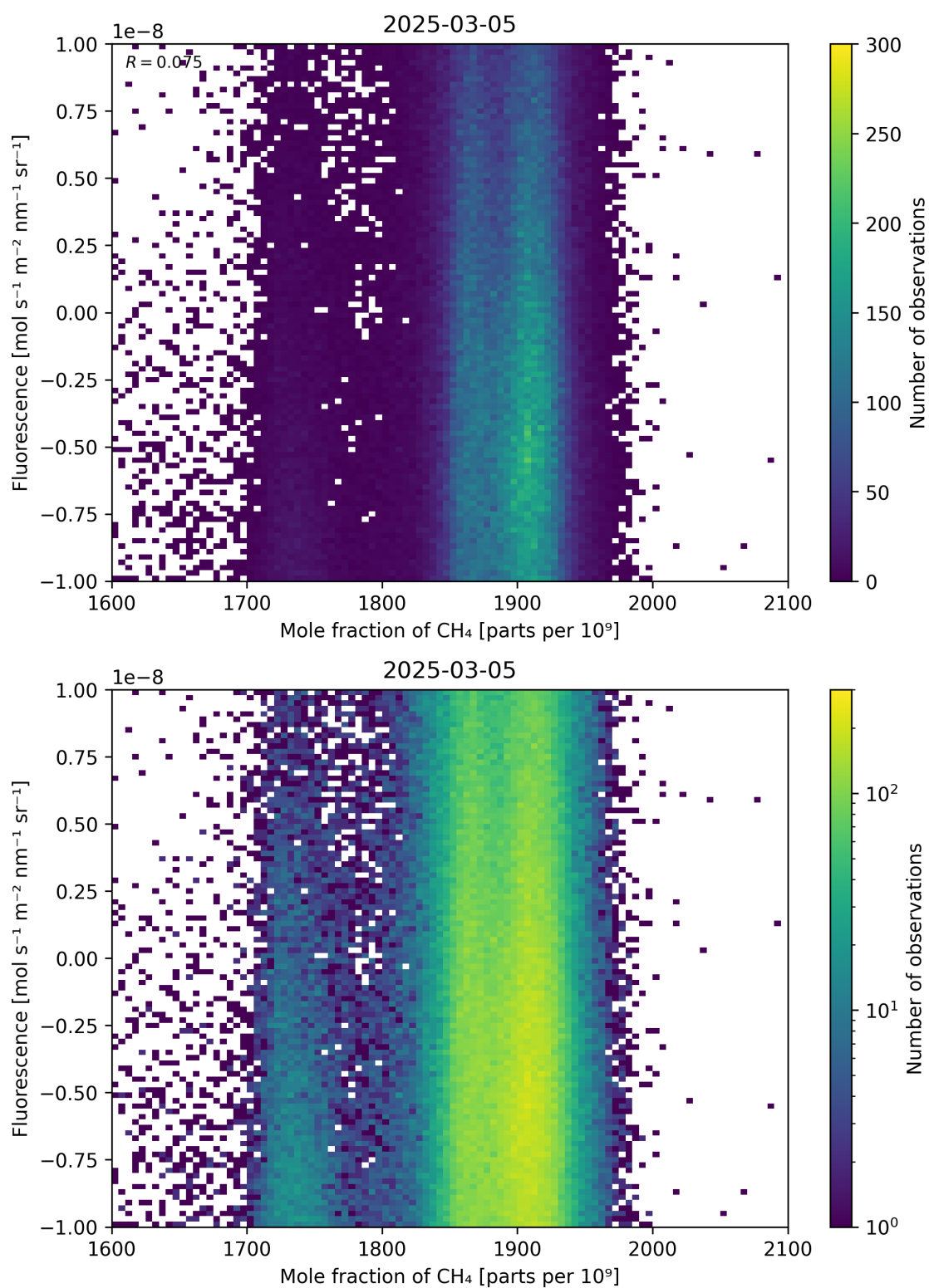
Figure 73: Scatter density plot of “Mole fraction of \text{CH}_4 ” against “Fluorescence” for 2025-03-04 to 2025-03-06.
