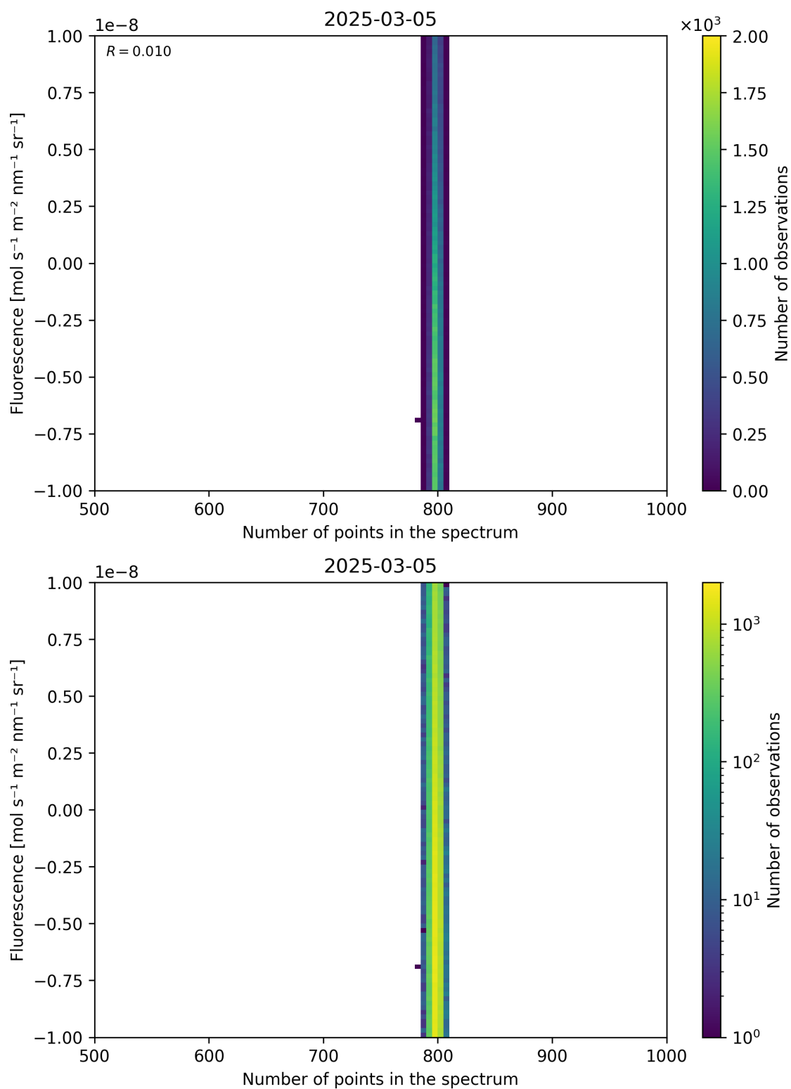
Figure 91: Scatter density plot of “Number of points in the spectrum” against “Fluorescence” for 2025-03-04 to 2025-03-06.
