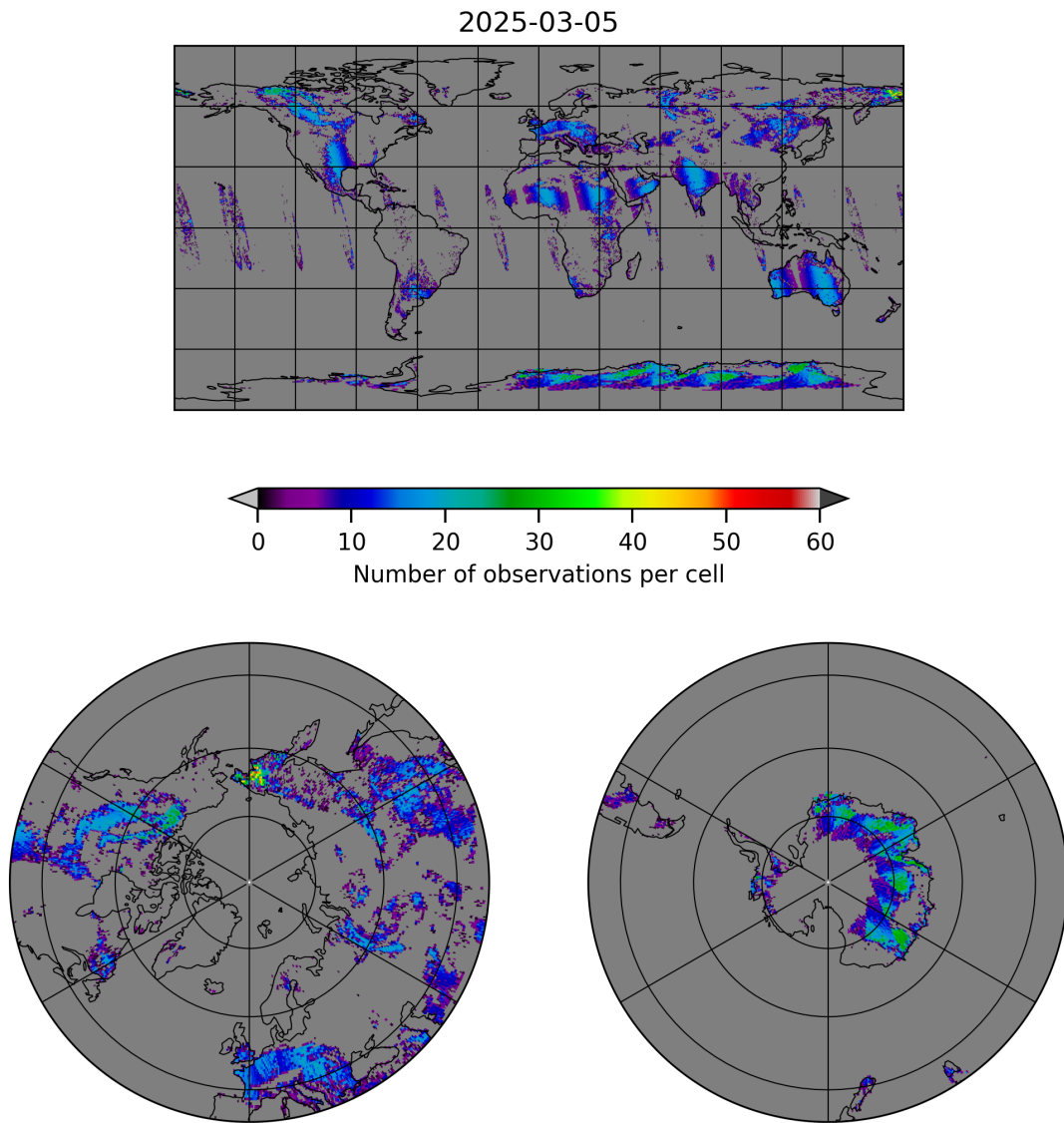
Figure 10: Map of the number of observations for 2025-03-04 to 2025-03-06
