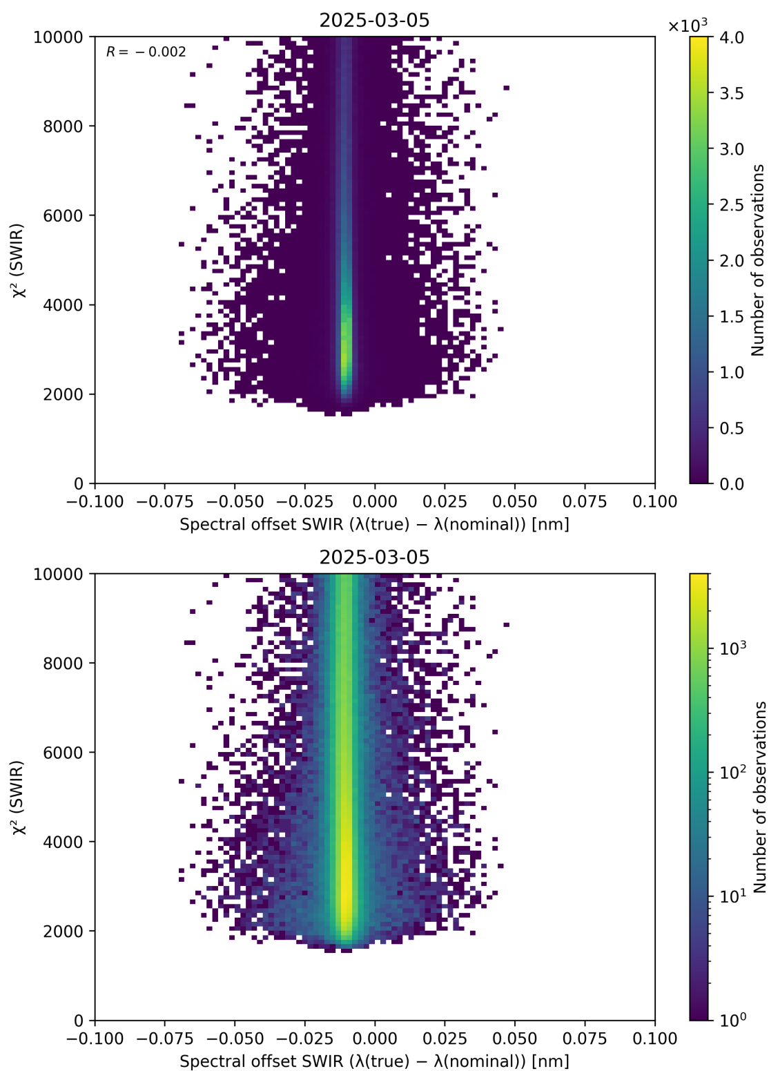
Figure 118: Scatter density plot of “Spectral offset SWIR ( \lambda_{\text{true}} - \lambda_{\text{nominal}} )” against “ \chi^2 (SWIR)” for 2025-03-04 to 2025-03-06.
