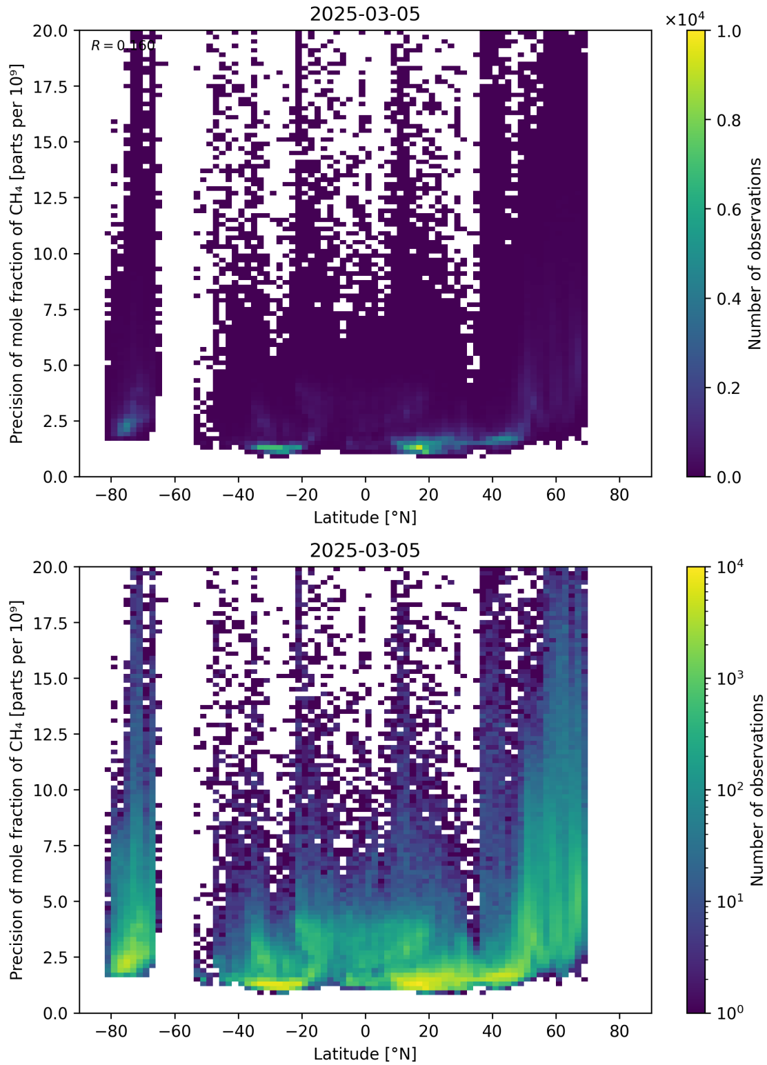
Figure 59: Scatter density plot of “Latitude” against “Precision of mole fraction of CH 4 ” for 2025-03-04 to 2025-03-06.
