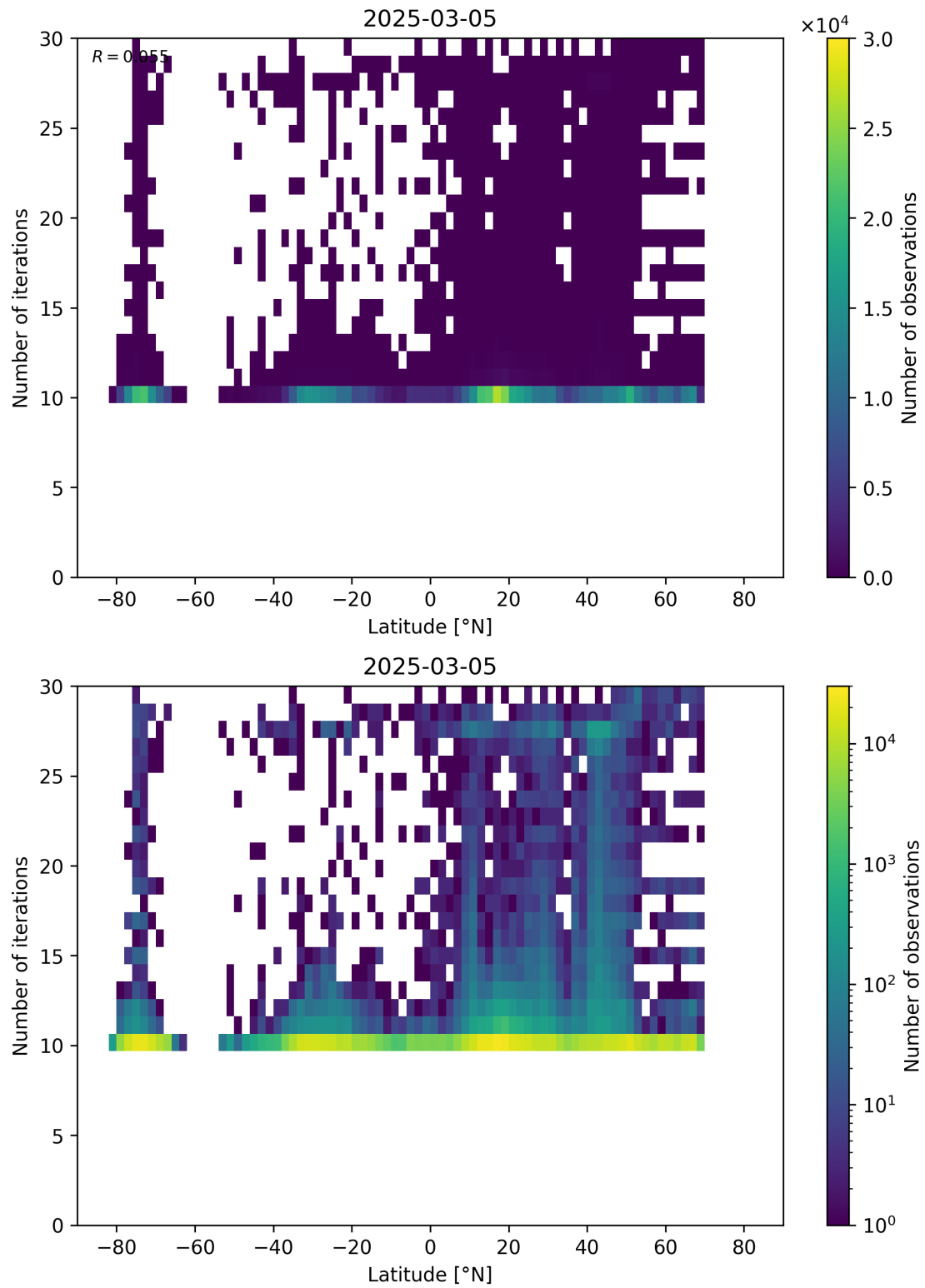
Figure 60: Scatter density plot of “Latitude” against “Number of iterations” for 2025-03-04 to 2025-03-06.
