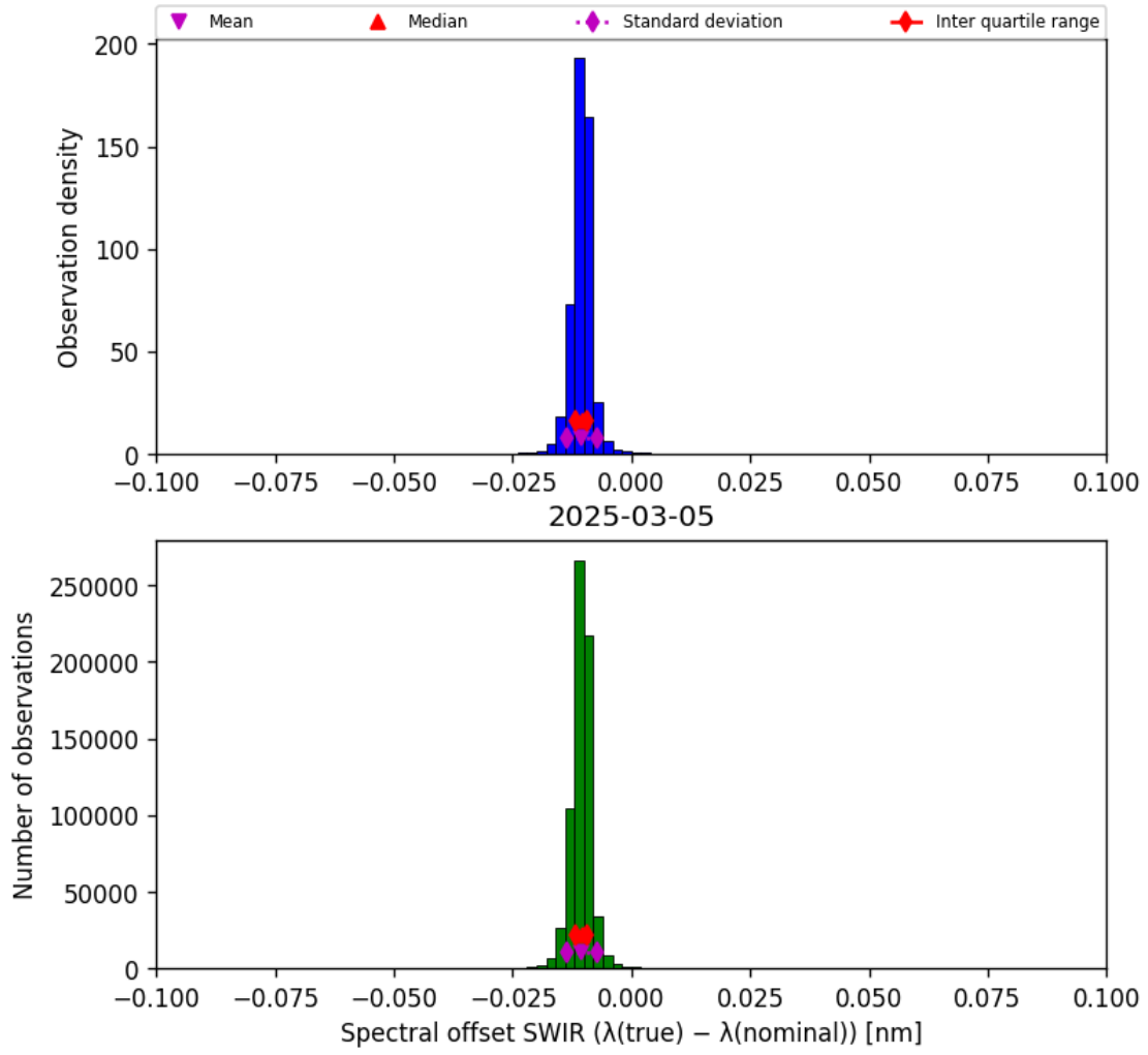
Figure 27: Histogram of “Spectral offset SWIR ( \lambda_{\text{true}} - \lambda_{\text{nominal}} )” for 2025-03-04 to 2025-03-06
