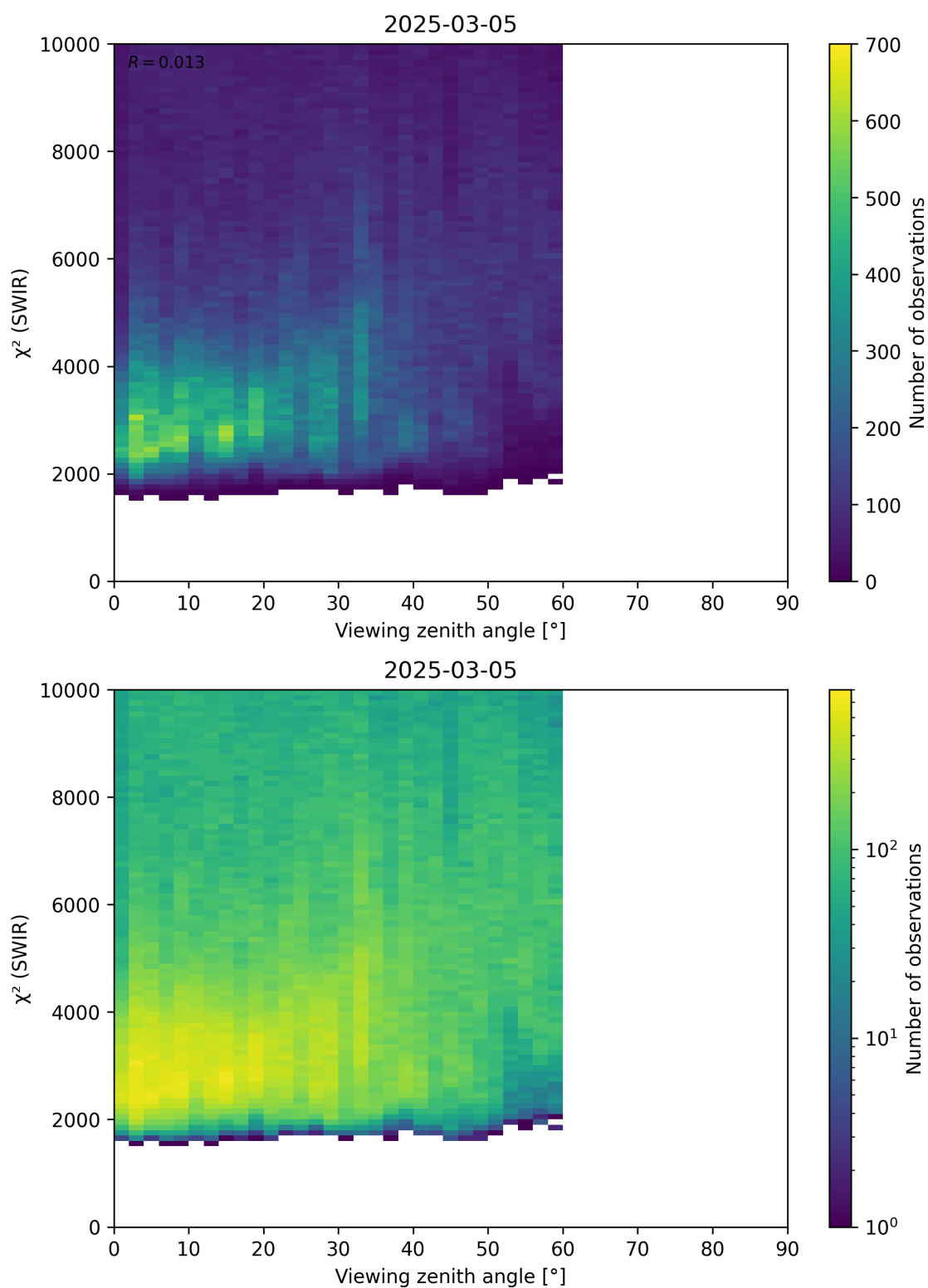
Figure 106: Scatter density plot of “Viewing zenith angle” against “ \chi^2 (SWIR)” for 2025-03-04 to 2025-03-06.
