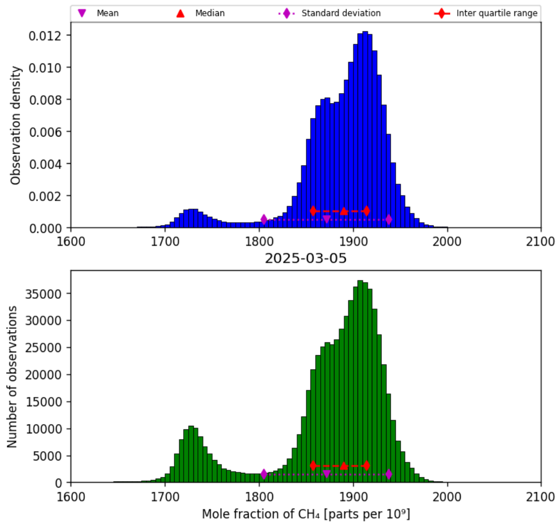
Figure 23: Histogram of “Mole fraction of CH 4 ” for 2025-03-04 to 2025-03-06
