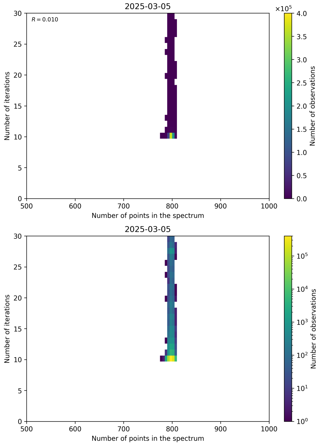
Figure 92: Scatter density plot of “Number of points in the spectrum” against “Number of iterations” for 2025-03-04 to 2025-03-06.
