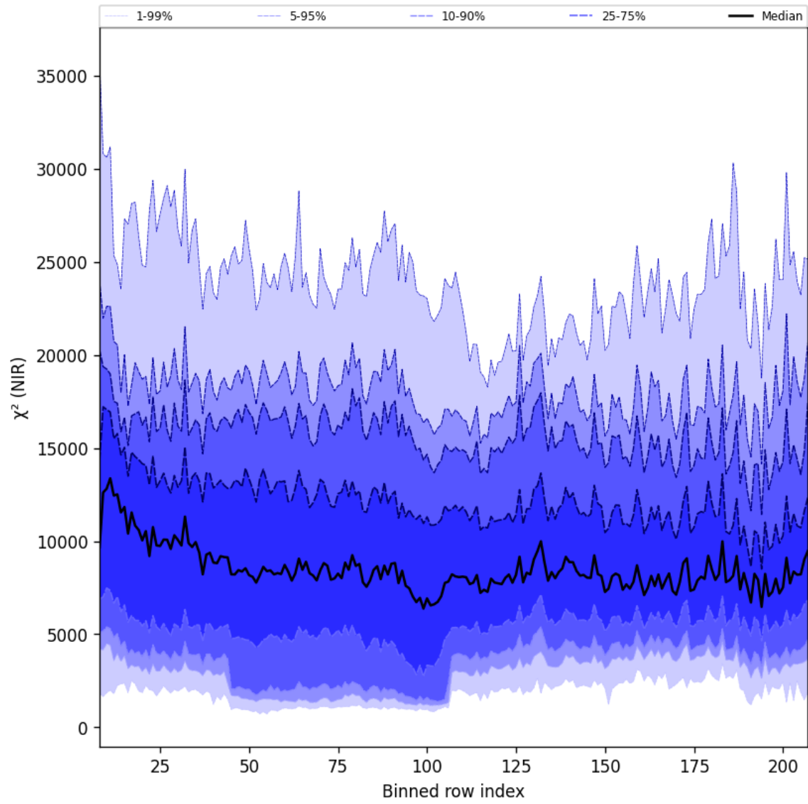
Figure 40: Along track statistics of “ \chi^2 (NIR)” for 2025-03-04 to 2025-03-06
