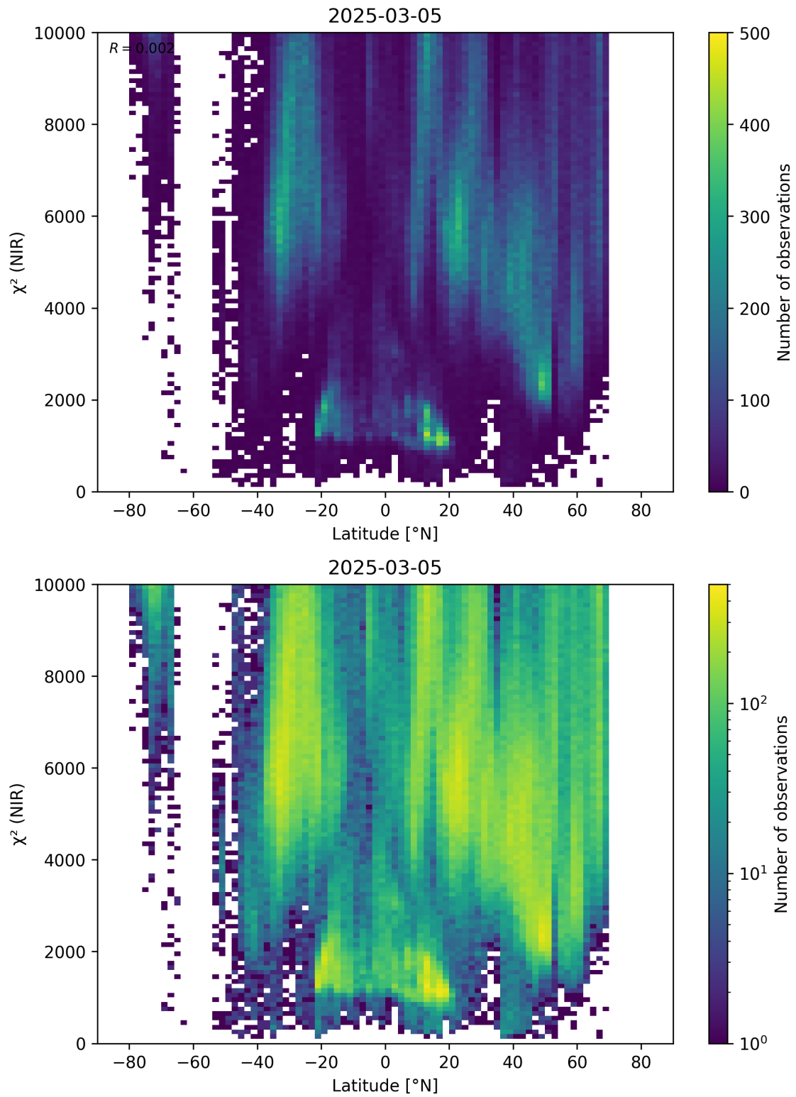
Figure 53: Scatter density plot of “Latitude” against “ \chi^2 (NIR)” for 2025-03-04 to 2025-03-06.
