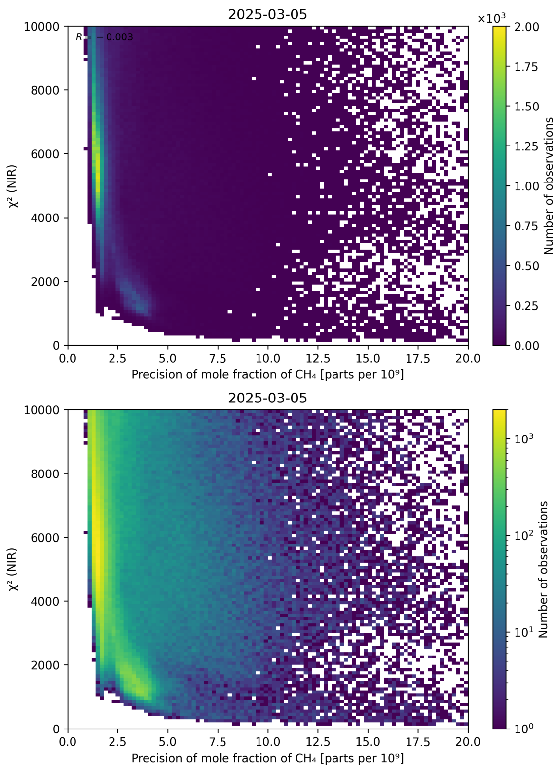
Figure 78: Scatter density plot of “Precision of mole fraction of CH 4 ” against “ \chi^2 (NIR)” for 2025-03-04 to 2025-03-06.
