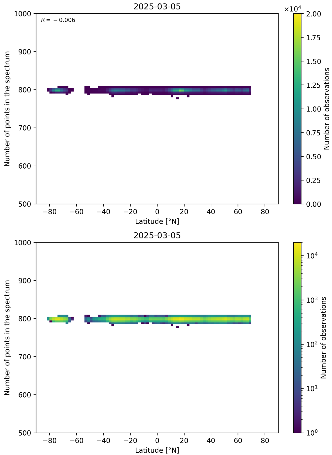
Figure 61: Scatter density plot of “Latitude” against “Number of points in the spectrum” for 2025-03-04 to 2025-03-06.
