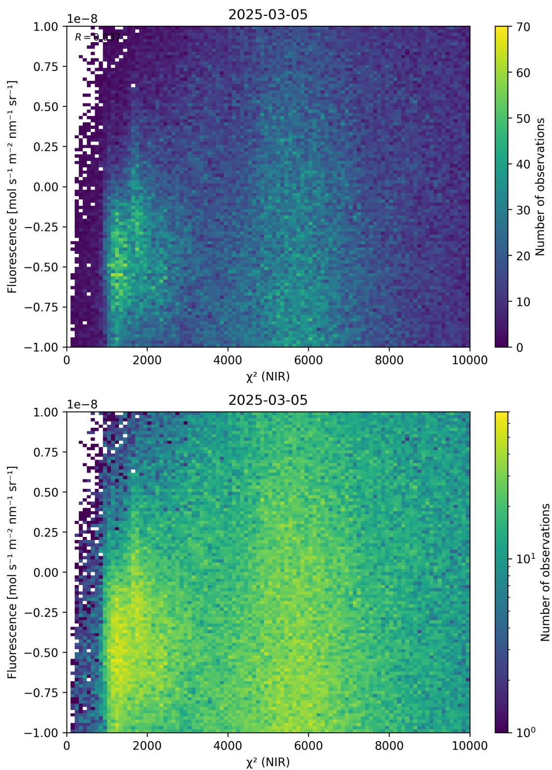
Figure 45: Scatter density plot of “ \chi^2 (NIR)” against “Fluorescence” for 2025-03-04 to 2025-03-06.
