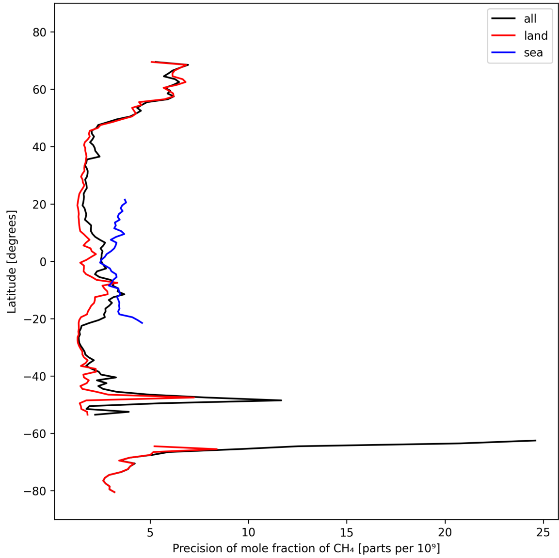
Figure 13: Zonal average of “Precision of mole fraction of CH 4 ” for 2025-03-04 to 2025-03-06.
