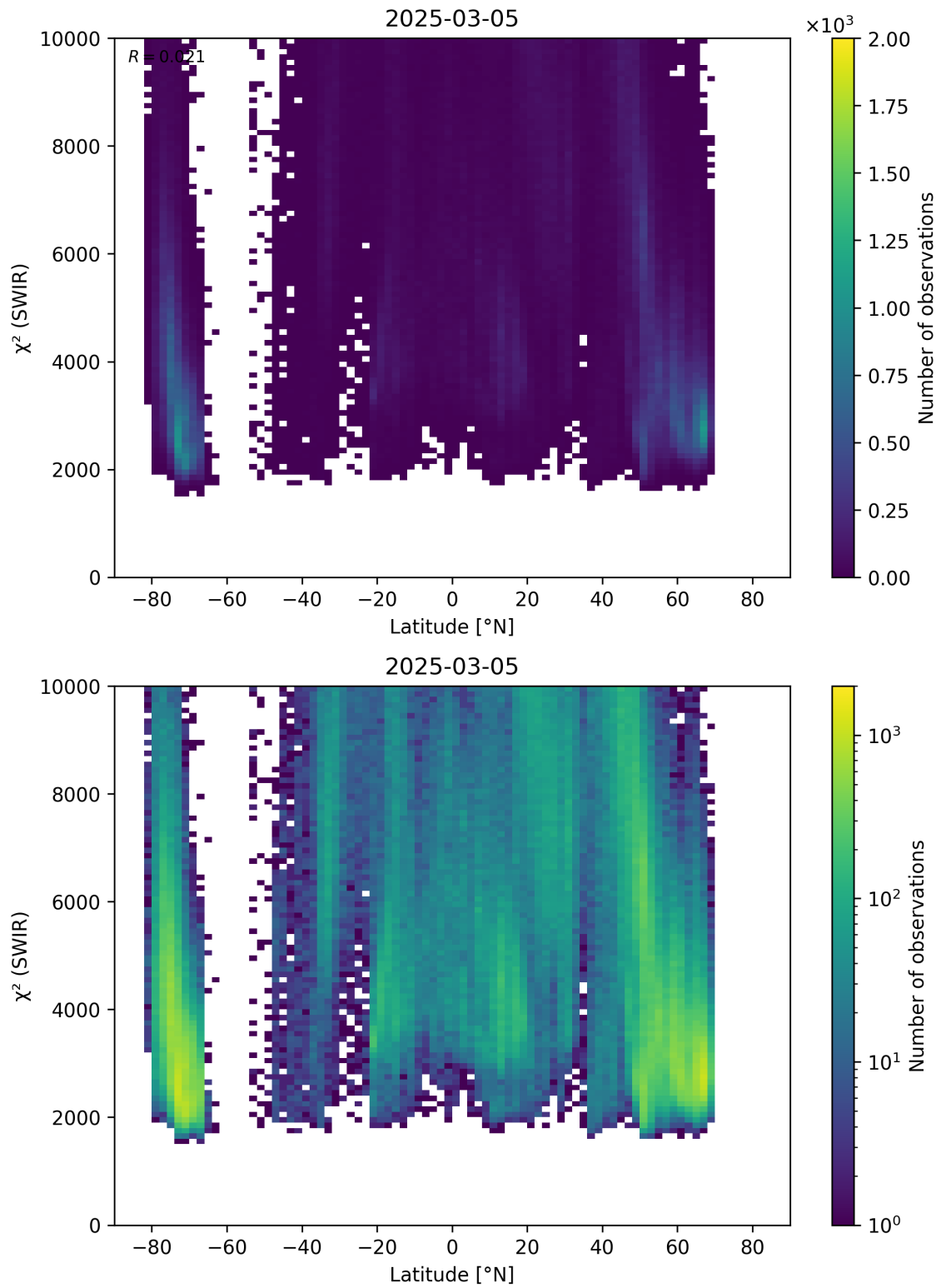
Figure 54: Scatter density plot of “Latitude” against “ \chi^2 (SWIR)” for 2025-03-04 to 2025-03-06.
