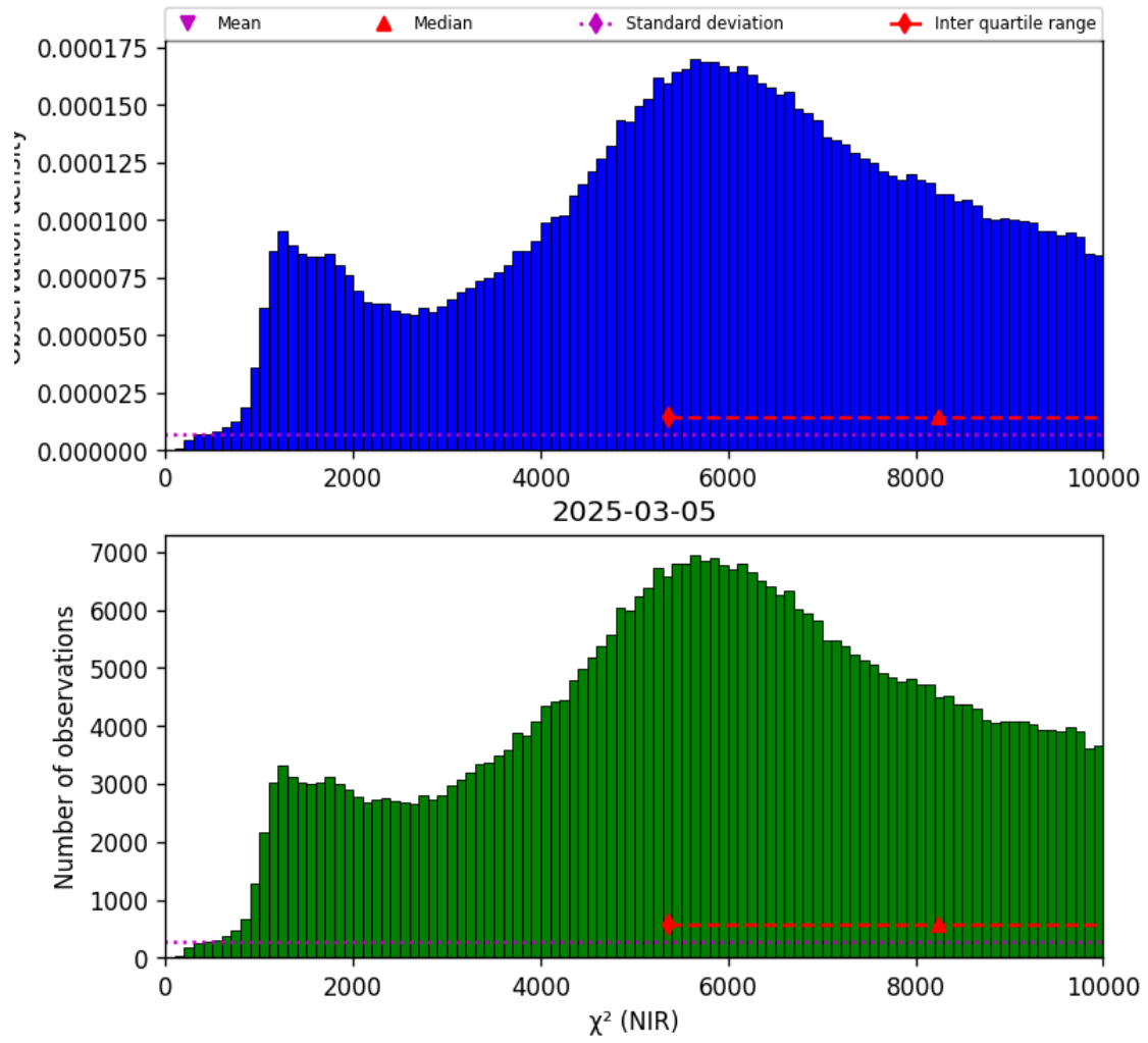
Figure 29: Histogram of “ \chi^2 (NIR)” for 2025-03-04 to 2025-03-06
