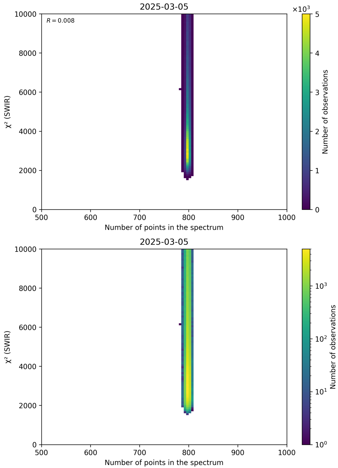
Figure 89: Scatter density plot of “Number of points in the spectrum” against “ \chi^2 (SWIR)” for 2025-03-04 to 2025-03-06.
