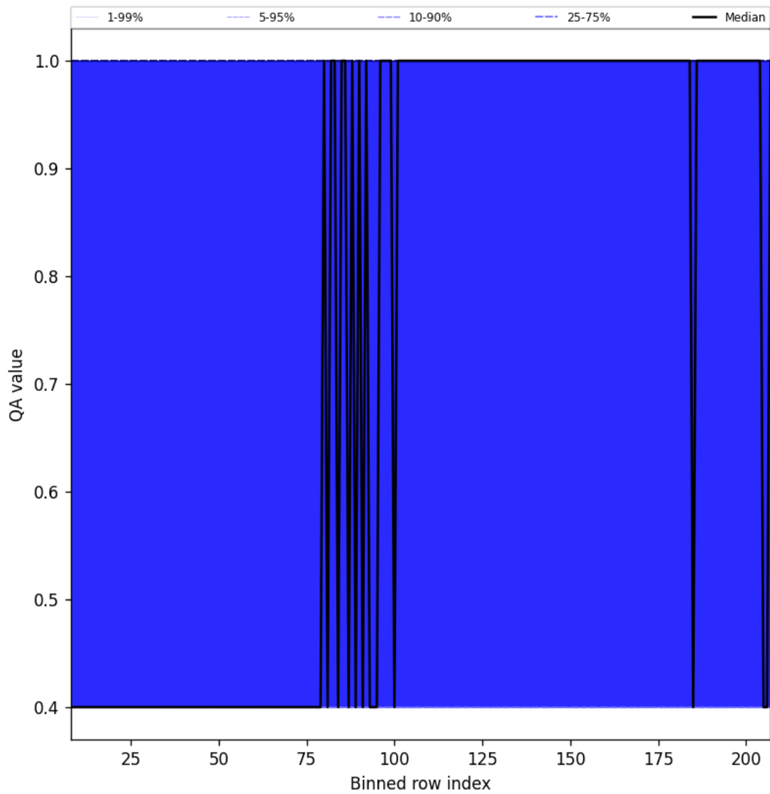
Figure 33: Along track statistics of “QA value” for 2025-03-04 to 2025-03-06
