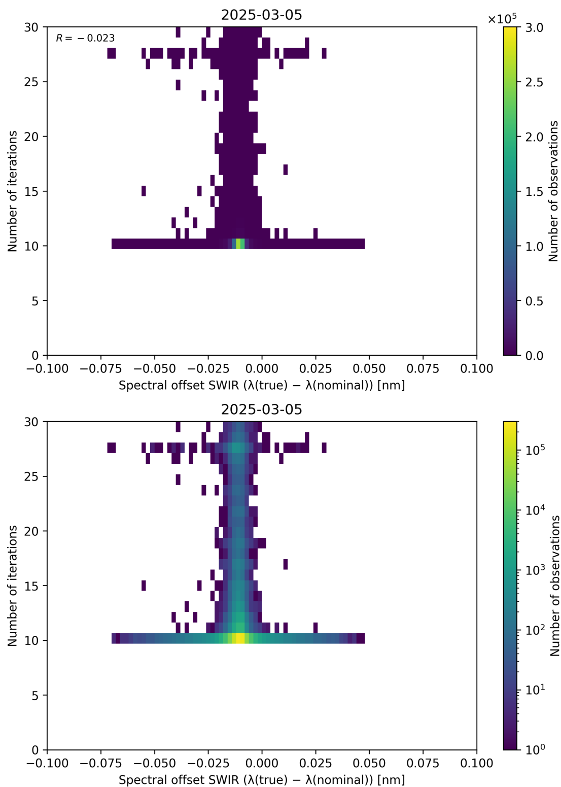
Figure 121: Scatter density plot of “Spectral offset SWIR ( \lambda_{\text{true}} - \lambda_{\text{nominal}} )” against “Number of iterations” for 2025-03-04 to 2025-03-06.
