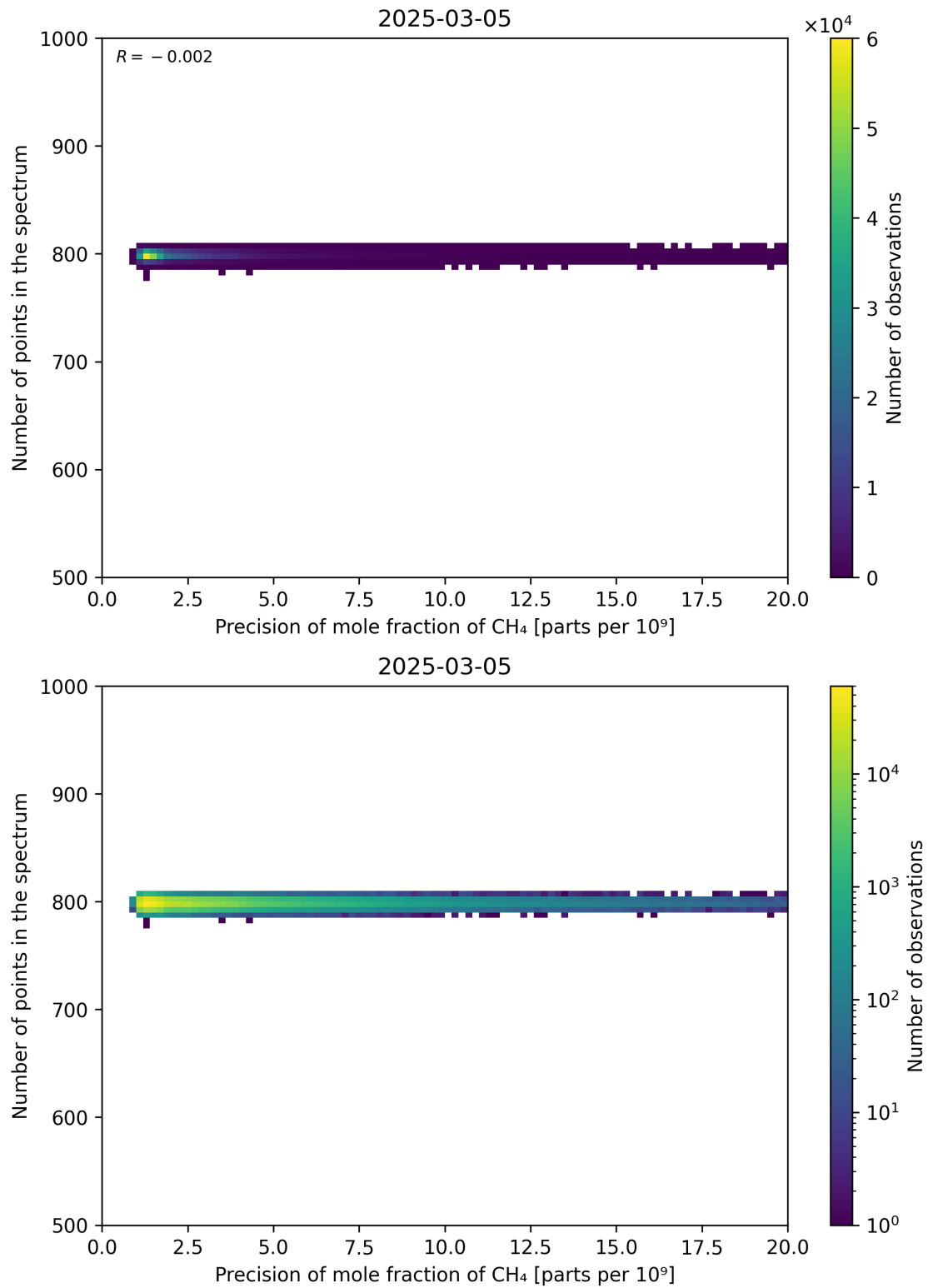
Figure 84: Scatter density plot of “Precision of mole fraction of CH 4 ” against “Number of points in the spectrum” for 2025-03-04 to 2025-03-06.
