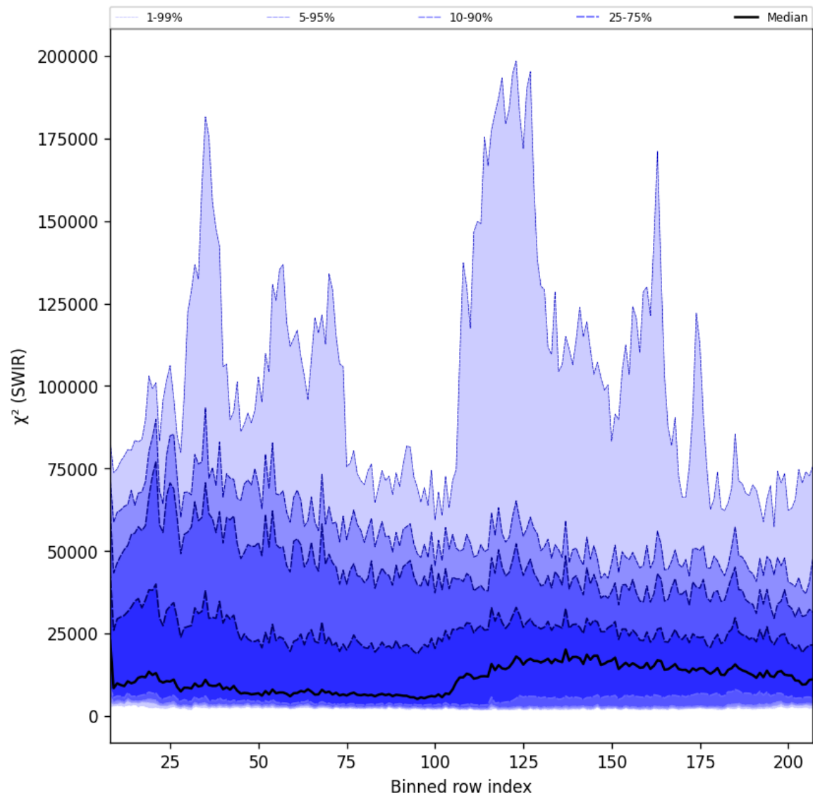
Figure 39: Along track statistics of " \chi^2 (SWIR)" for 2025-03-04 to 2025-03-06
