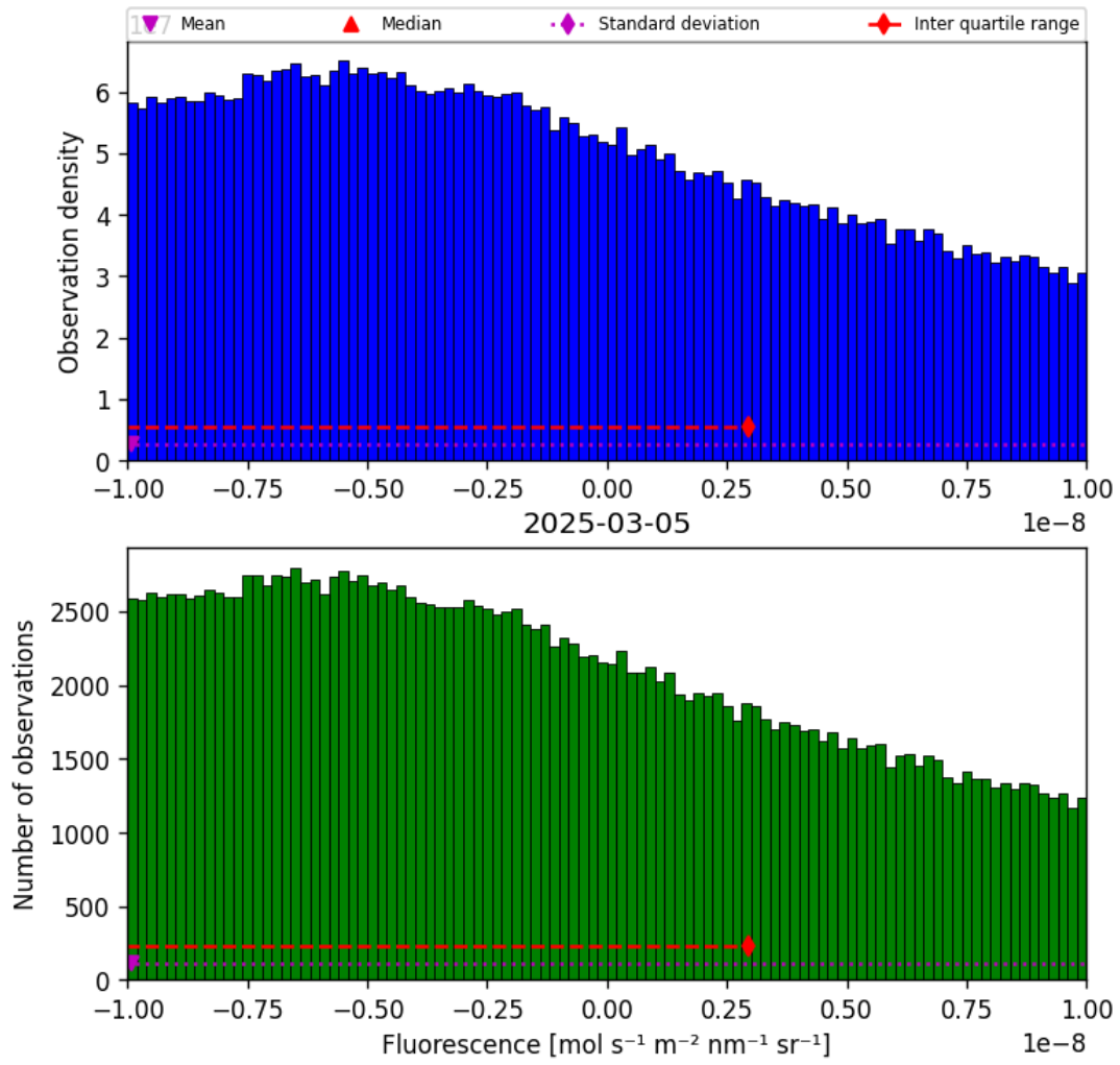
Figure 32: Histogram of “Fluorescence” for 2025-03-04 to 2025-03-06
