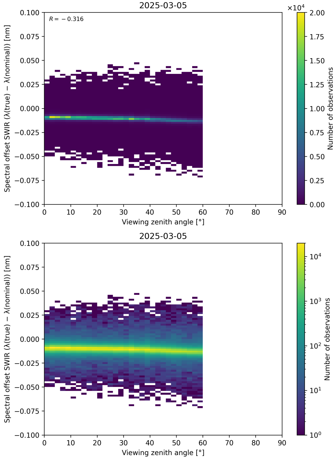
Figure 116: Scatter density plot of “Viewing zenith angle” against “Spectral offset SWIR ( \lambda_{\text{true}} - \lambda_{\text{nominal}} )” for 2025-03-04 to 2025-03-06.
