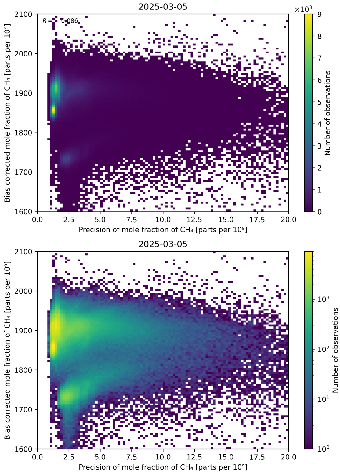
Figure 82: Scatter density plot of “Precision of mole fraction of CH 4 ” against “Bias corrected mole fraction of CH 4 ” for 2025-03-04 to 2025-03-06.
