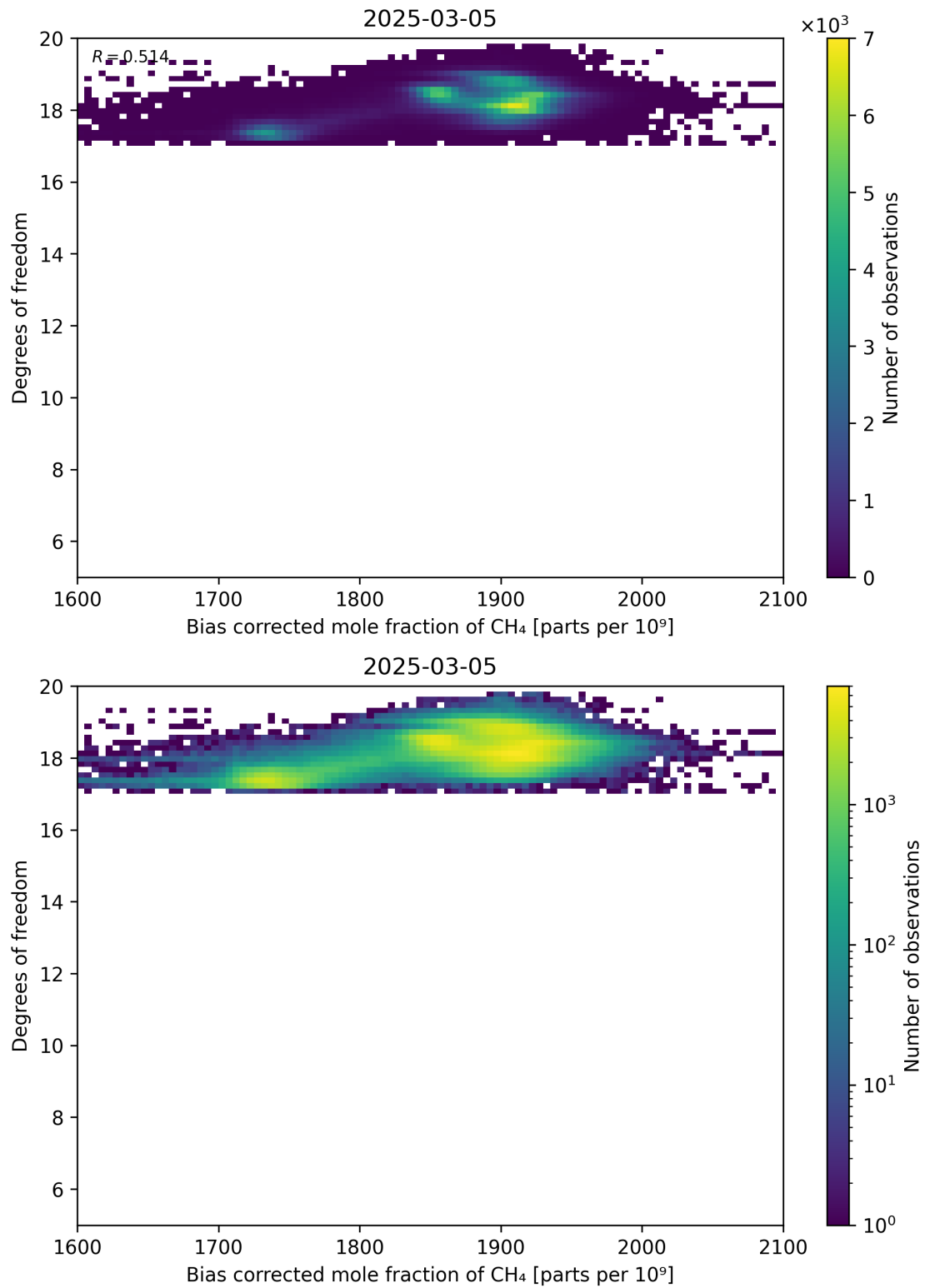
Figure 65: Scatter density plot of “Bias corrected mole fraction of CH 4 ” against “Degrees of freedom” for 2025-03-04 to 2025-03-06.
