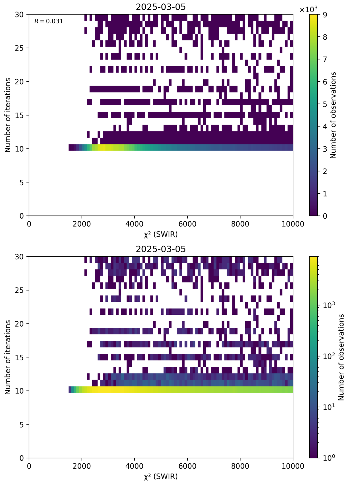
Figure 50: Scatter density plot of “ \chi^2 (SWIR)” against “Number of iterations” for 2025-03-04 to 2025-03-06.
