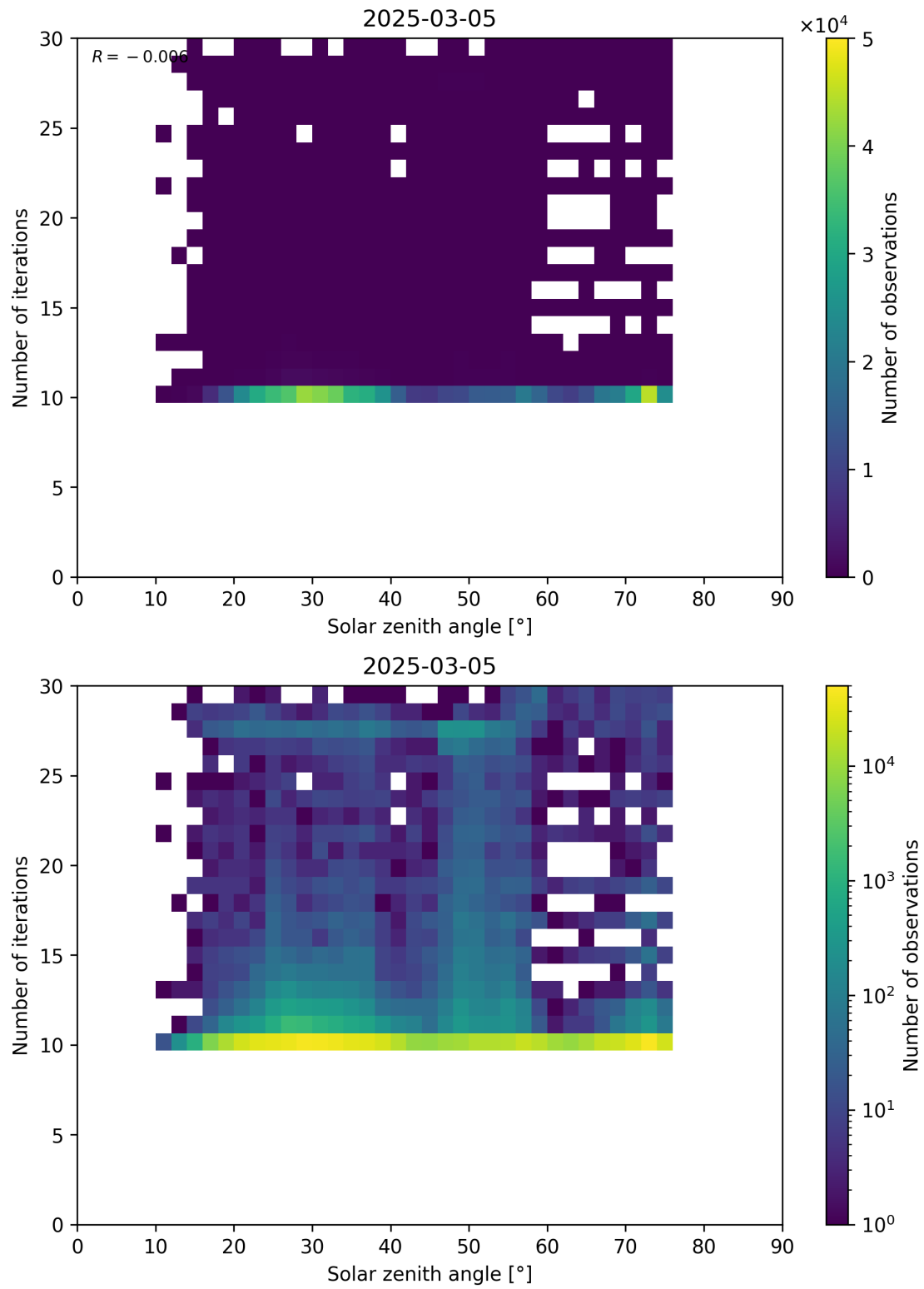
Figure 102: Scatter density plot of “Solar zenith angle” against “Number of iterations” for 2025-03-04 to 2025-03-06.
