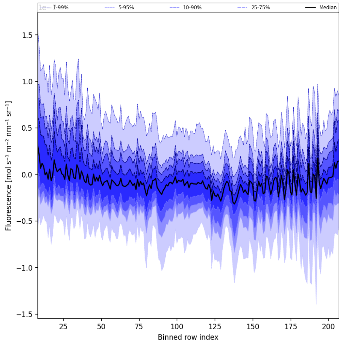
Figure 43: Along track statistics of “Fluorescence” for 2025-03-04 to 2025-03-06
