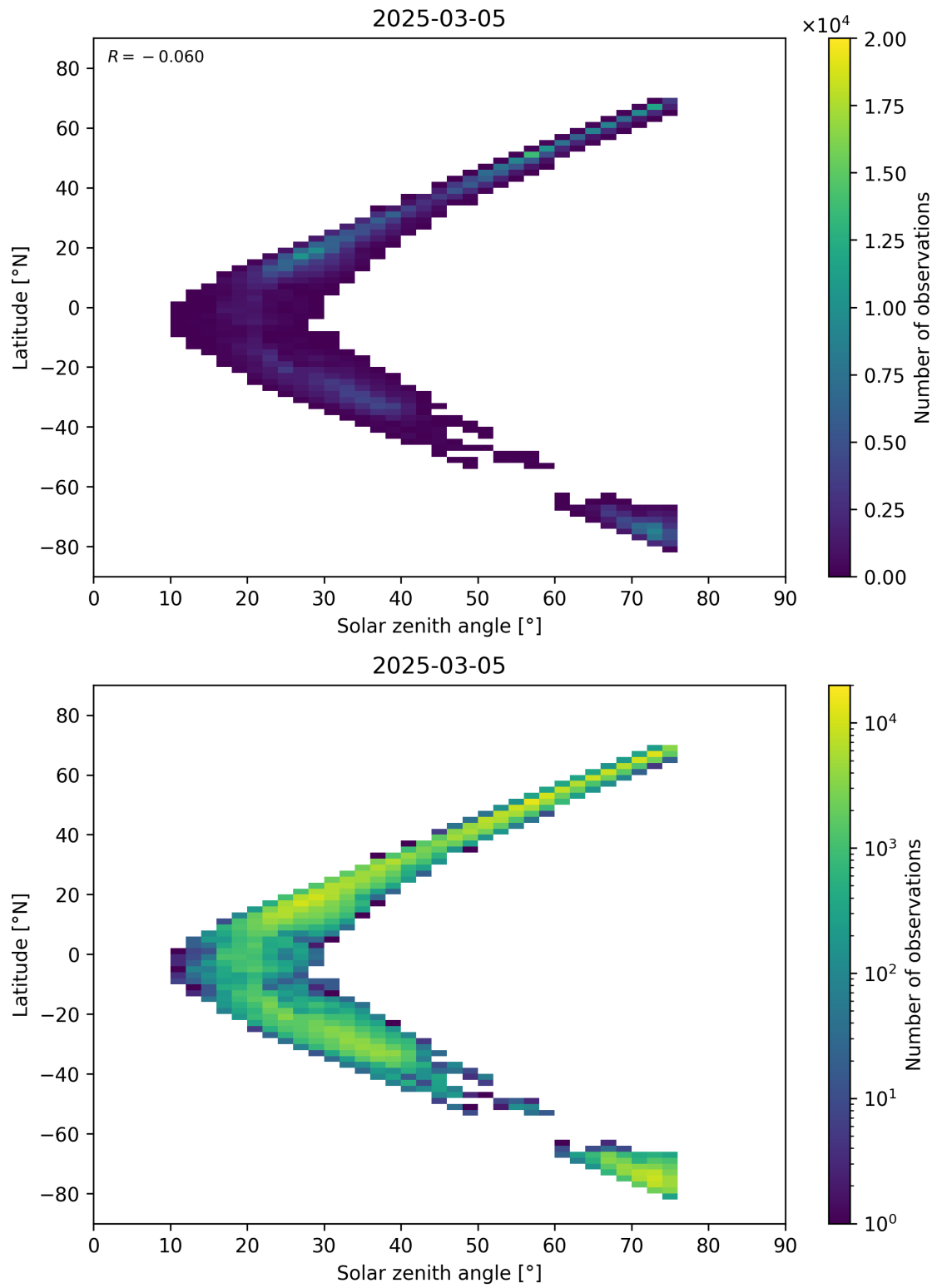
Figure 98: Scatter density plot of “Solar zenith angle” against “Latitude” for 2025-03-04 to 2025-03-06.
