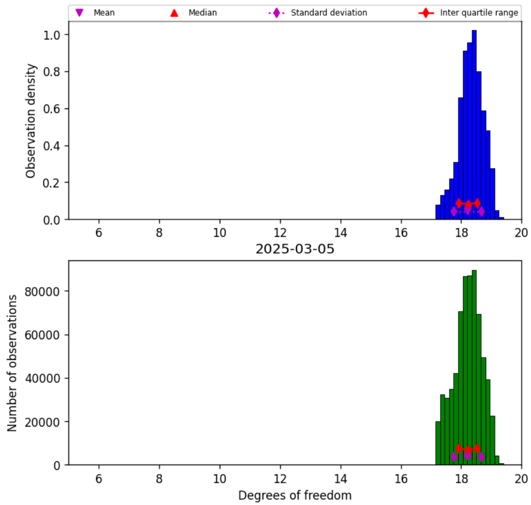
Figure 30: Histogram of “Degrees of freedom” for 2025-03-04 to 2025-03-06
