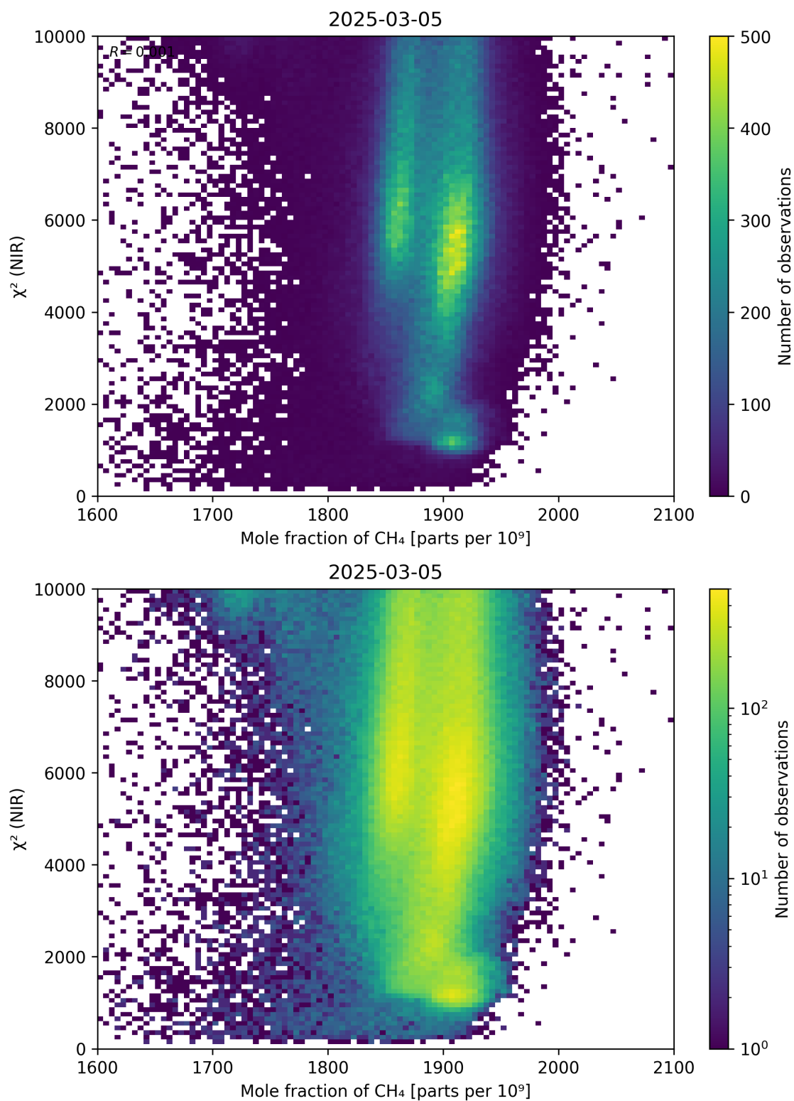
Figure 70: Scatter density plot of “Mole fraction of \text{CH}_4 ” against “ \chi^2 (NIR)” for 2025-03-04 to 2025-03-06.
