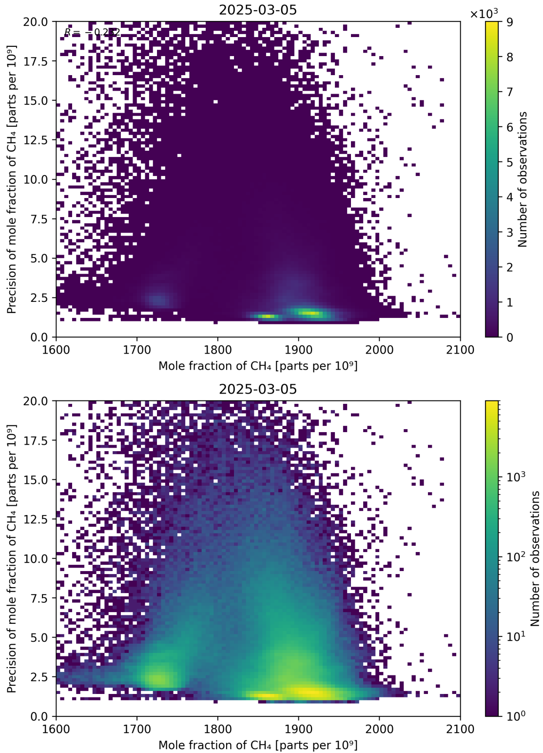
Figure 75: Scatter density plot of “Mole fraction of CH 4 ” against “Precision of mole fraction of CH 4 ” for 2025-03-04 to 2025-03-06.
