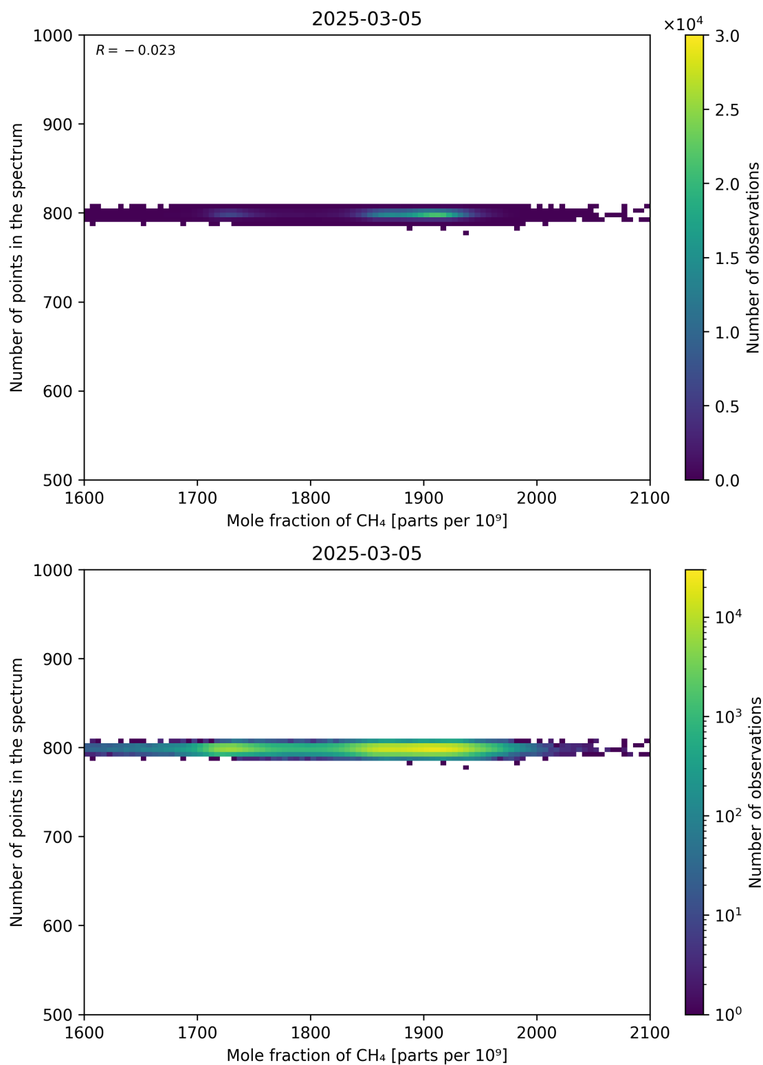
Figure 77: Scatter density plot of “Mole fraction of CH 4 ” against “Number of points in the spectrum” for 2025-03-04 to 2025-03-06.
