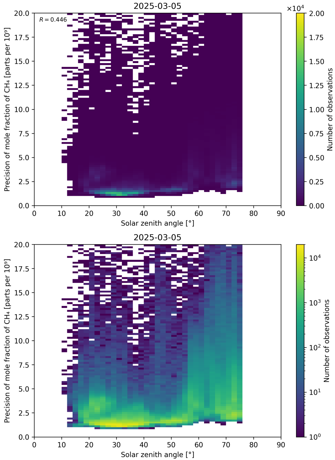
Figure 101: Scatter density plot of “Solar zenith angle” against “Precision of mole fraction of CH 4 ” for 2025-03-04 to 2025-03-06.
