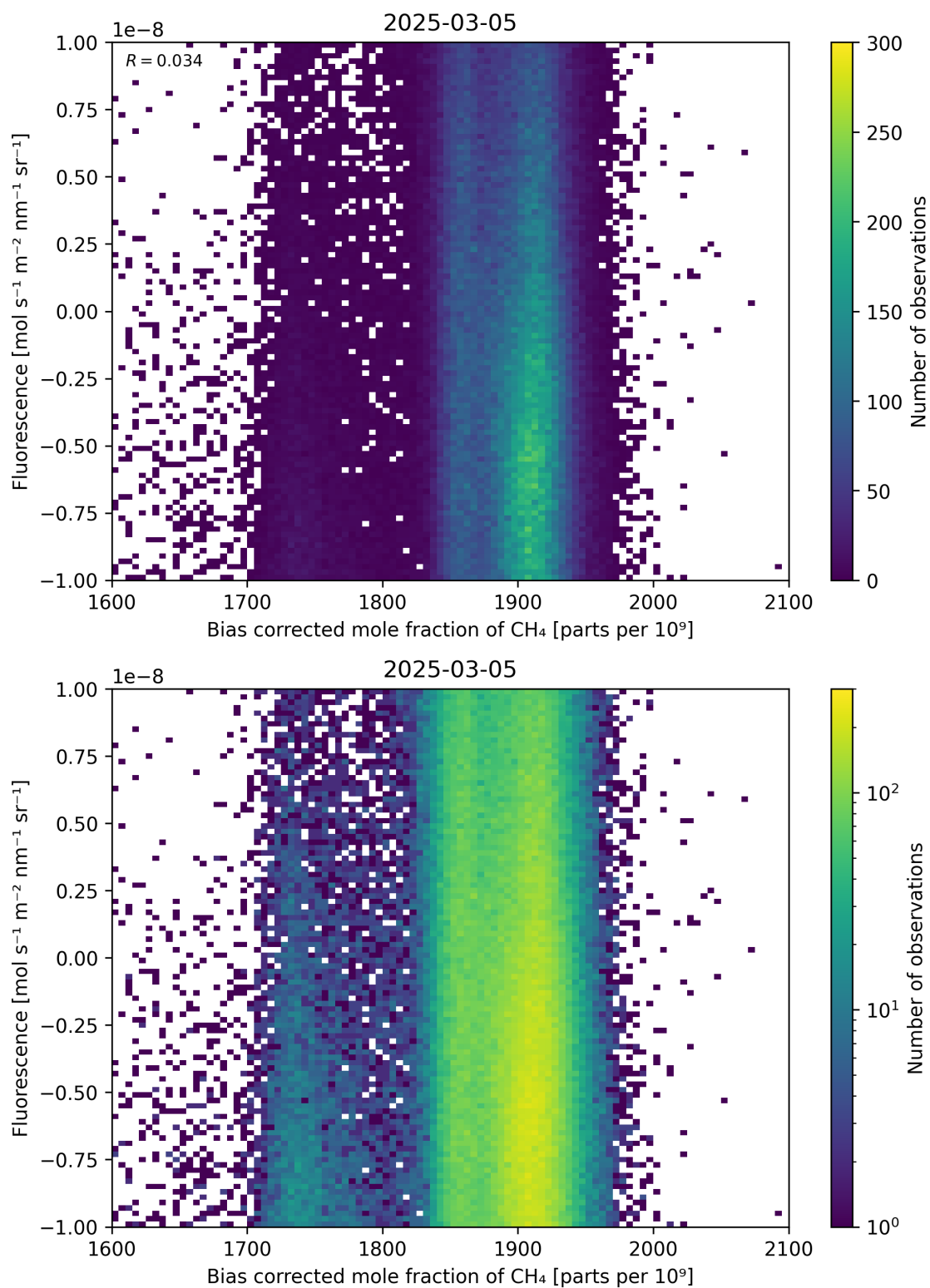
Figure 66: Scatter density plot of “Bias corrected mole fraction of \text{CH}_4 ” against “Fluorescence” for 2025-03-04 to 2025-03-06.
