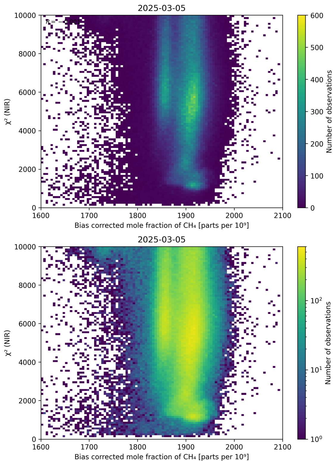
Figure 63: Scatter density plot of “Bias corrected mole fraction of \text{CH}_4 ” against “ \chi^2 (NIR)” for 2025-03-04 to 2025-03-06.
