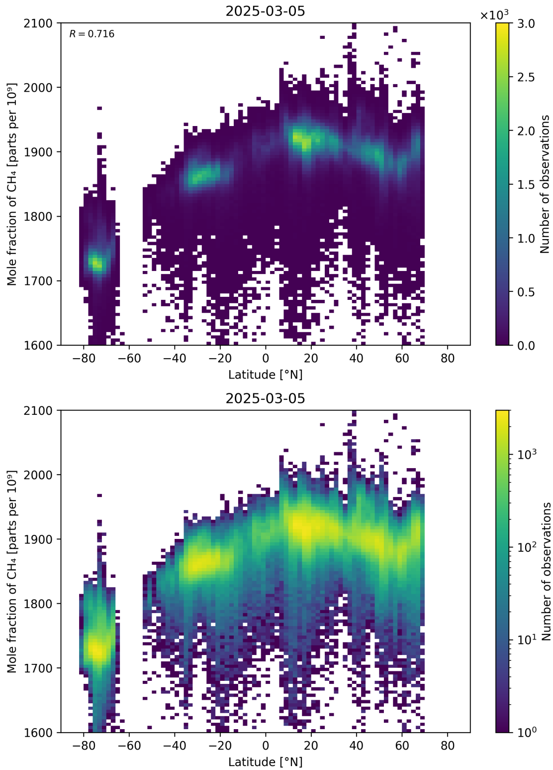
Figure 57: Scatter density plot of “Latitude” against “Mole fraction of \text{CH}_4 ” for 2025-03-04 to 2025-03-06.
