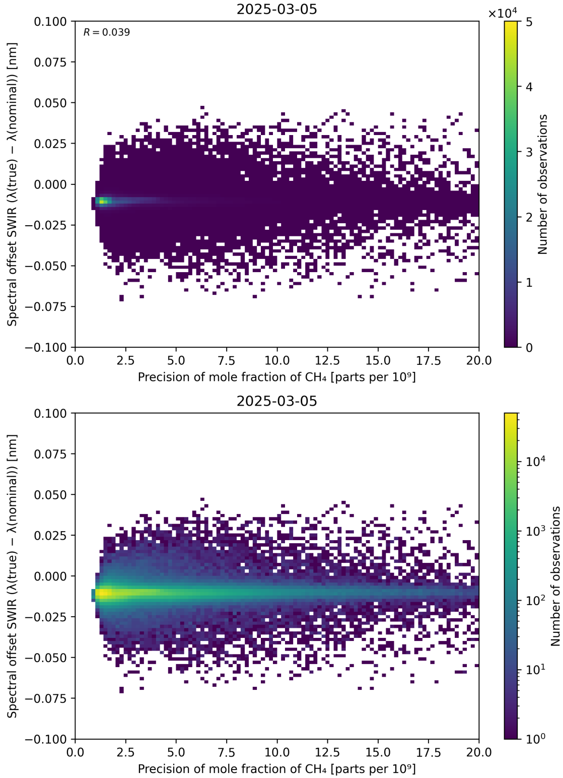
Figure 85: Scatter density plot of “Precision of mole fraction of \text{CH}_4 ” against “Spectral offset SWIR ( \lambda_{\text{true}} - \lambda_{\text{nominal}} )” for 2025-03-04 to 2025-03-06.
