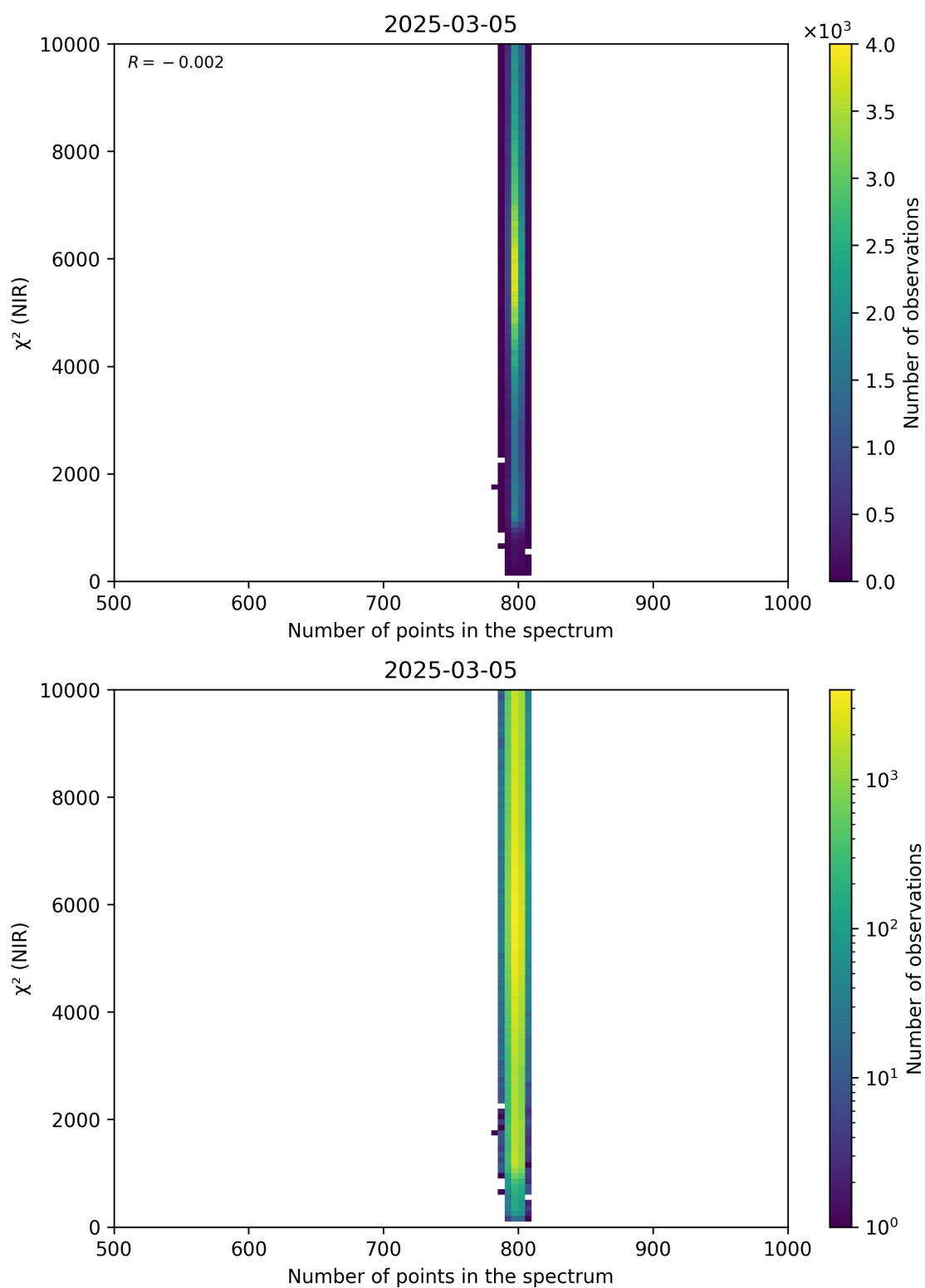
Figure 88: Scatter density plot of “Number of points in the spectrum” against “ \chi^2 (NIR)” for 2025-03-04 to 2025-03-06.
