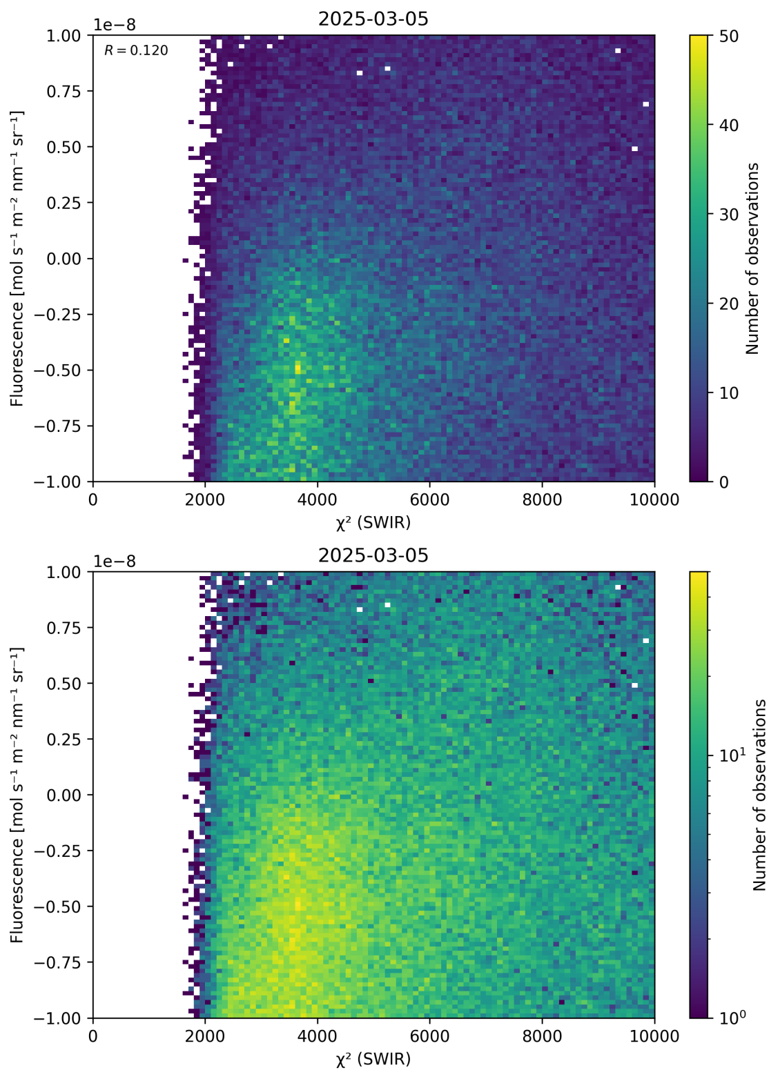
Figure 49: Scatter density plot of “ \chi^2 (SWIR)” against “Fluorescence” for 2025-03-04 to 2025-03-06.
