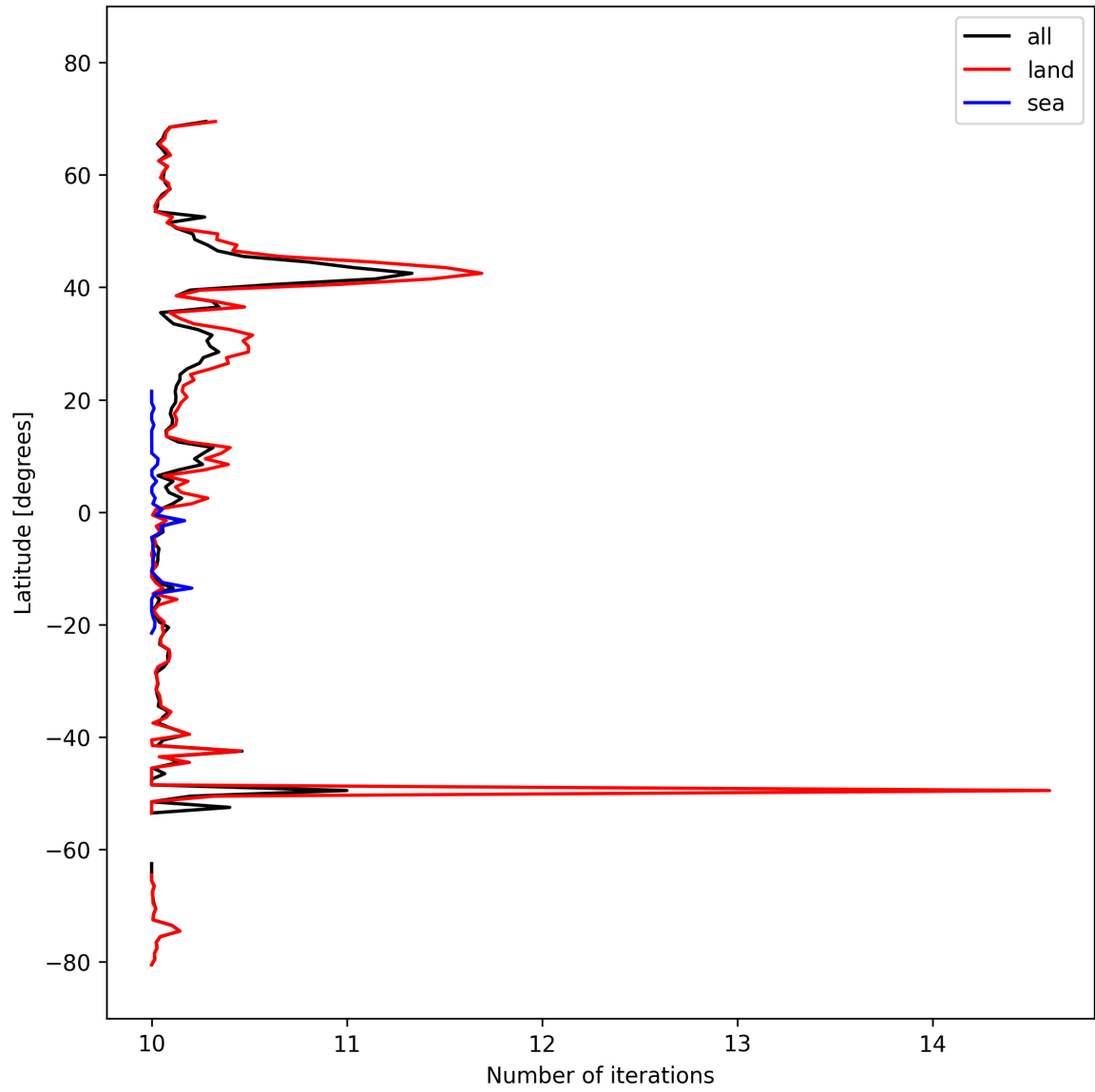
Figure 20: Zonal average of “Number of iterations” for 2025-03-04 to 2025-03-06.
