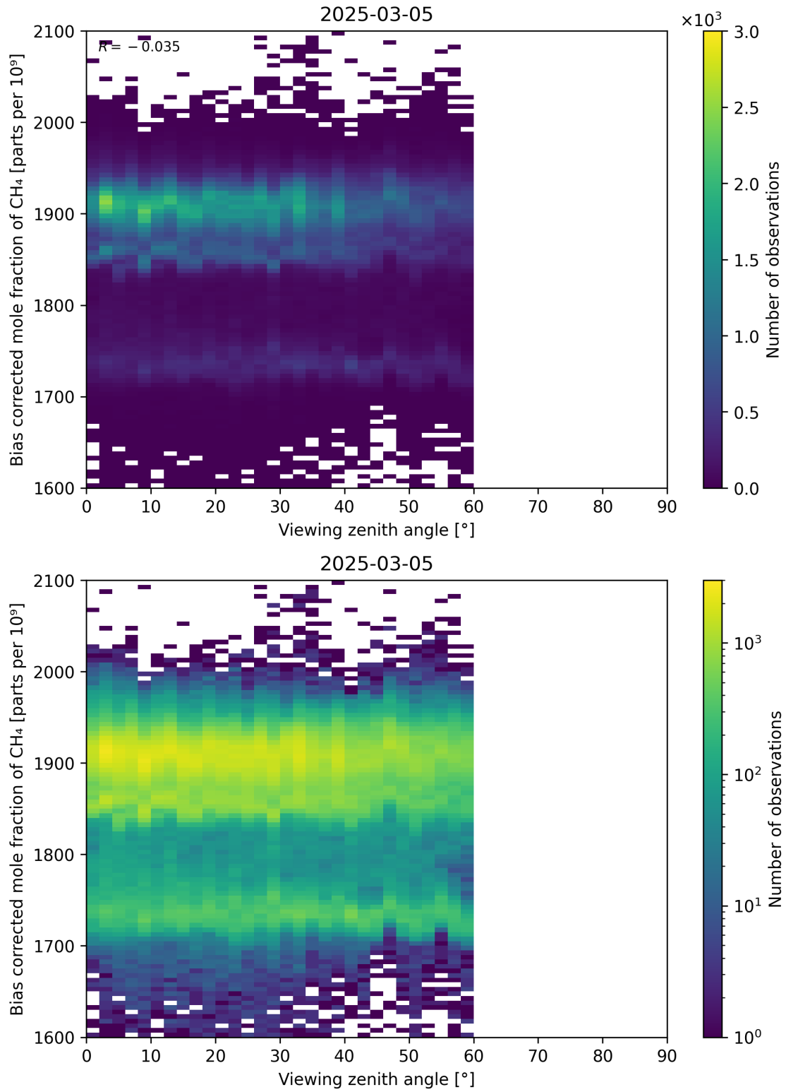
Figure 111: Scatter density plot of “Viewing zenith angle” against “Bias corrected mole fraction of CH 4 ” for 2025-03-04 to 2025-03-06.
