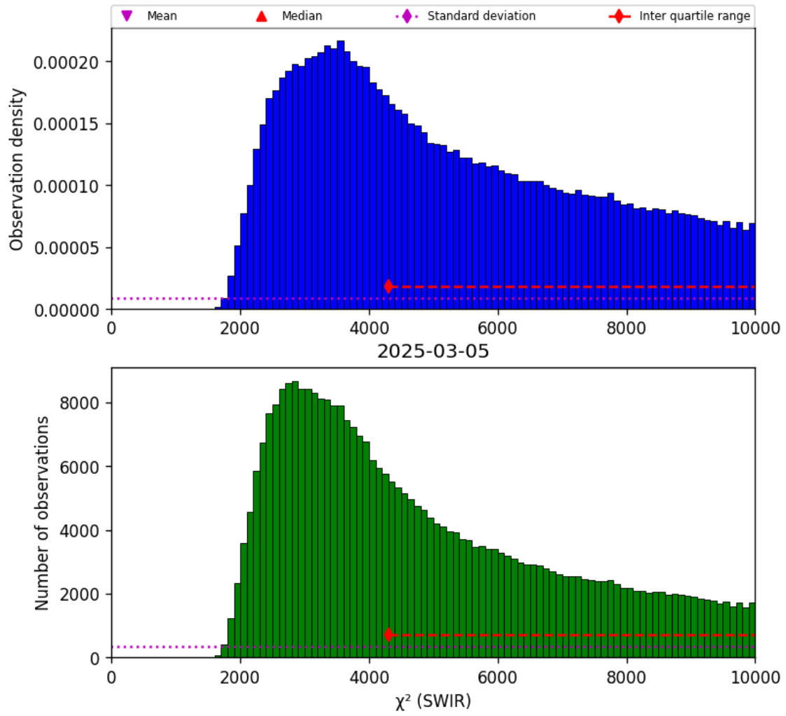
Figure 28: Histogram of " \chi^2 (SWIR)" for 2025-03-04 to 2025-03-06
