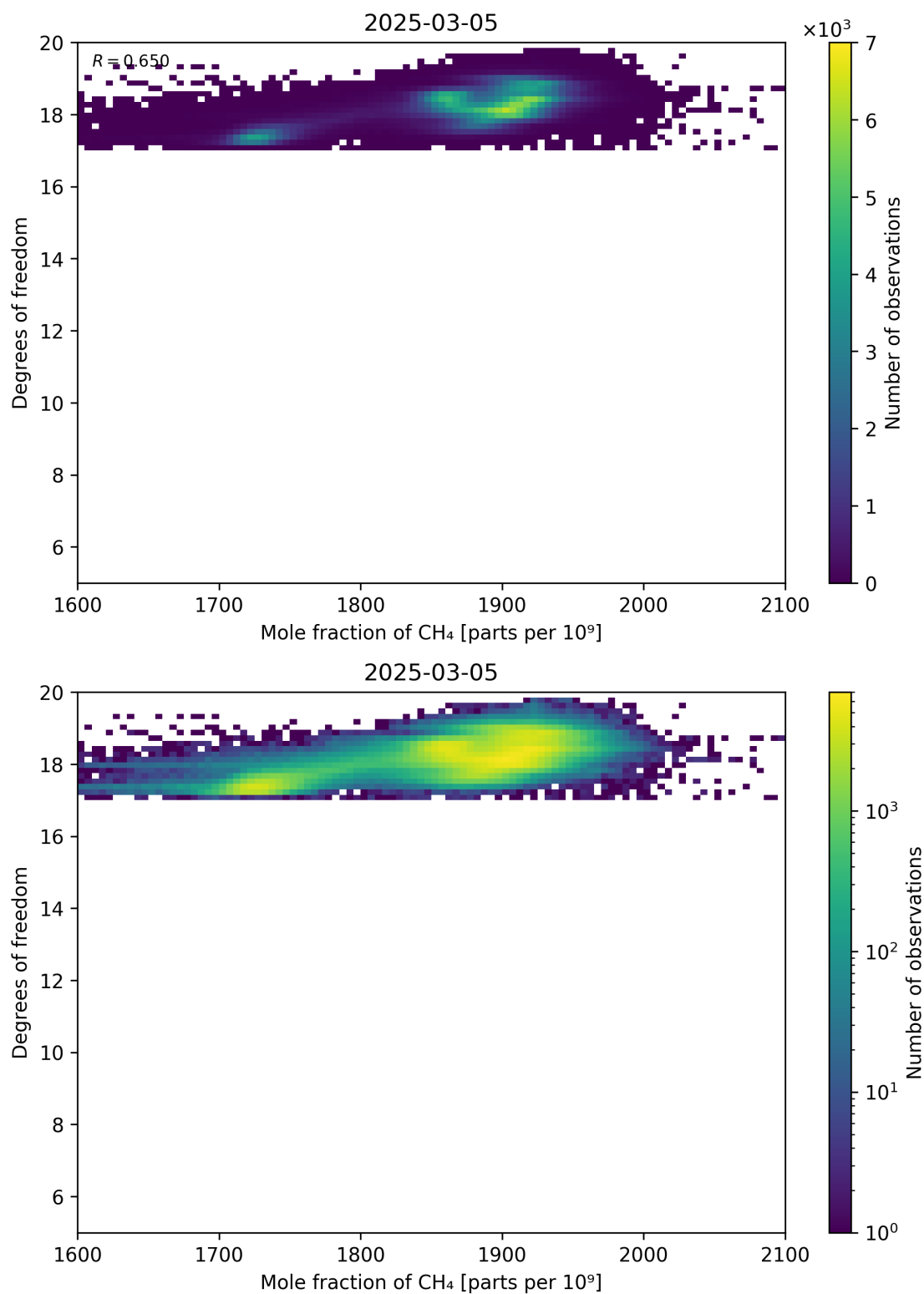
Figure 72: Scatter density plot of “Mole fraction of CH 4 ” against “Degrees of freedom” for 2025-03-04 to 2025-03-06.
