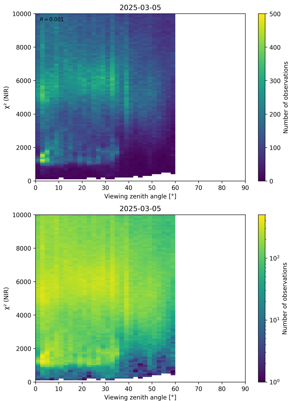
Figure 105: Scatter density plot of “Viewing zenith angle” against “ \chi^2 (NIR)” for 2025-03-04 to 2025-03-06.
