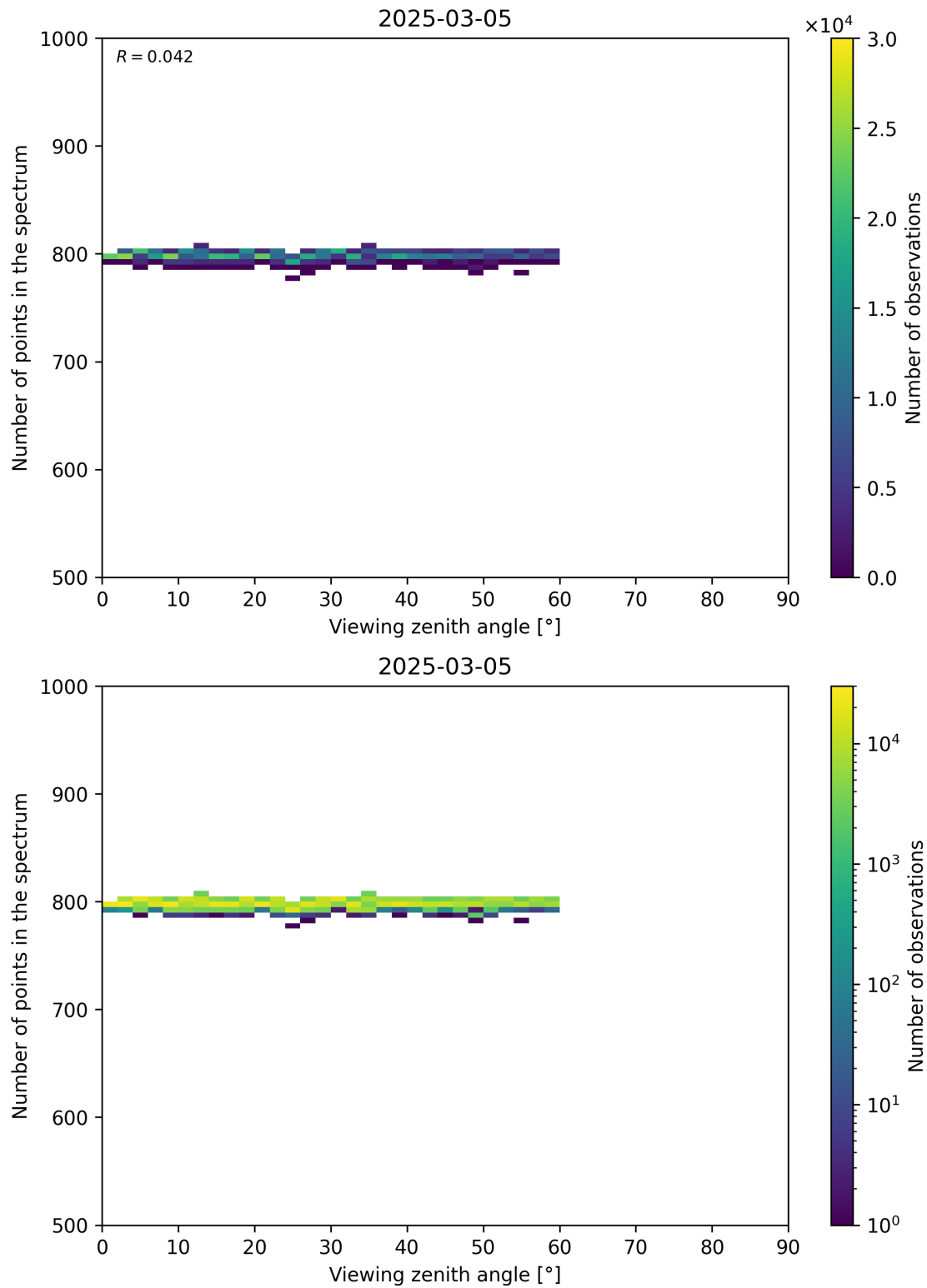
Figure 114: Scatter density plot of “Viewing zenith angle” against “Number of points in the spectrum” for 2025-03-04 to 2025-03-06.
