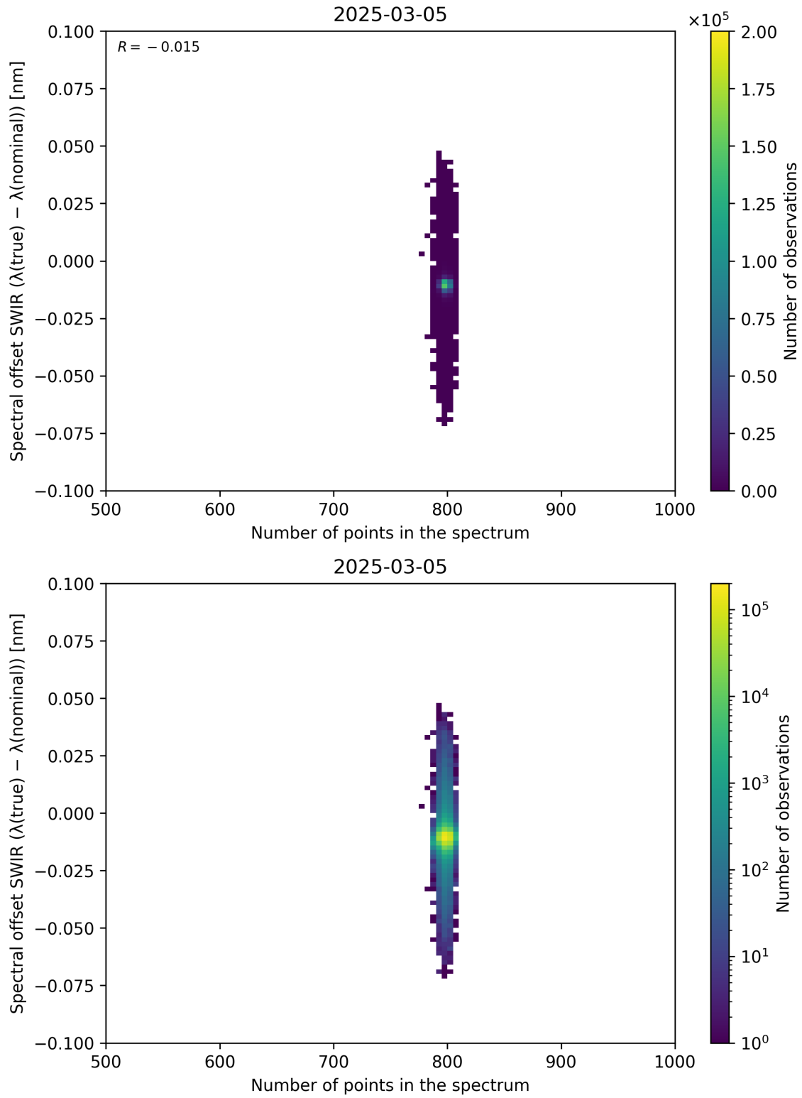
Figure 93: Scatter density plot of “Number of points in the spectrum” against “Spectral offset SWIR ( \lambda_{\text{true}} - \lambda_{\text{nominal}} )” for 2025-03-04 to 2025-03-06.
