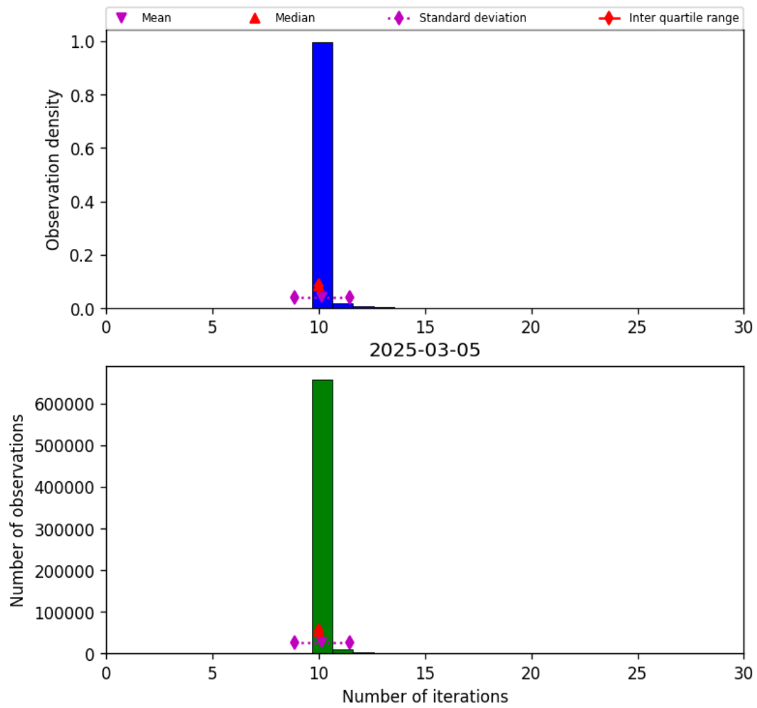
Figure 31: Histogram of “Number of iterations” for 2025-03-04 to 2025-03-06
