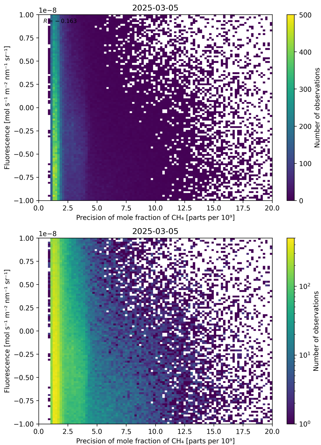
Figure 81: Scatter density plot of “Precision of mole fraction of \text{CH}_4 ” against “Fluorescence” for 2025-03-04 to 2025-03-06.
