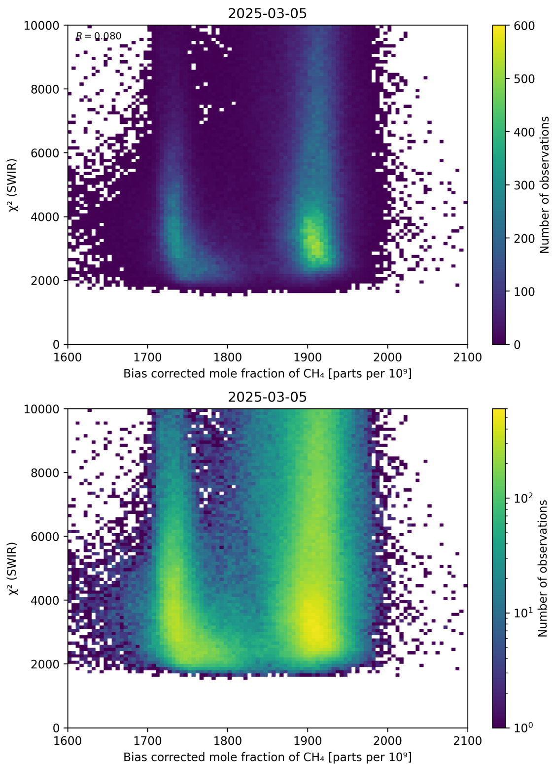
Figure 64: Scatter density plot of “Bias corrected mole fraction of CH 4 ” against “ \chi^2 (SWIR)” for 2025-03-04 to 2025-03-06.
