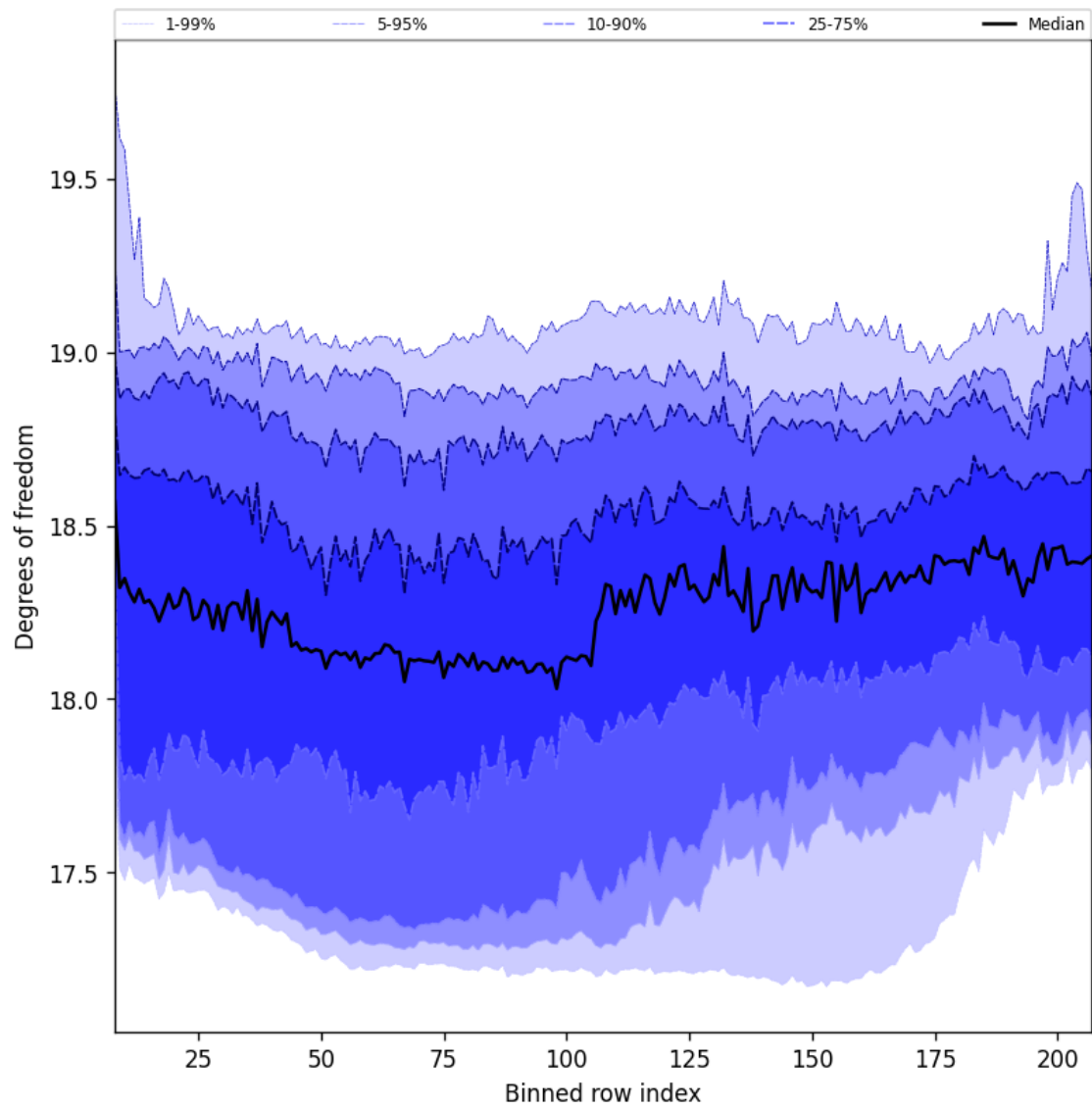
Figure 41: Along track statistics of “Degrees of freedom” for 2025-03-04 to 2025-03-06
