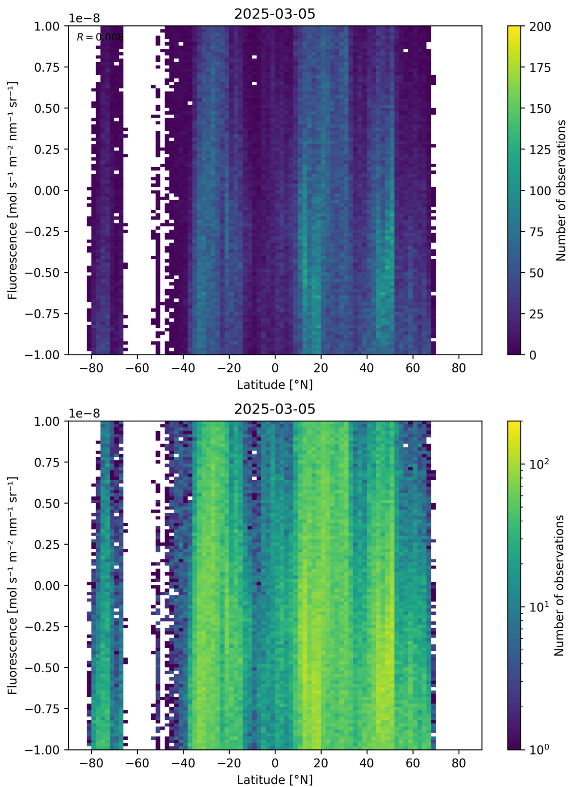
Figure 56: Scatter density plot of “Latitude” against “Fluorescence” for 2025-03-04 to 2025-03-06.
