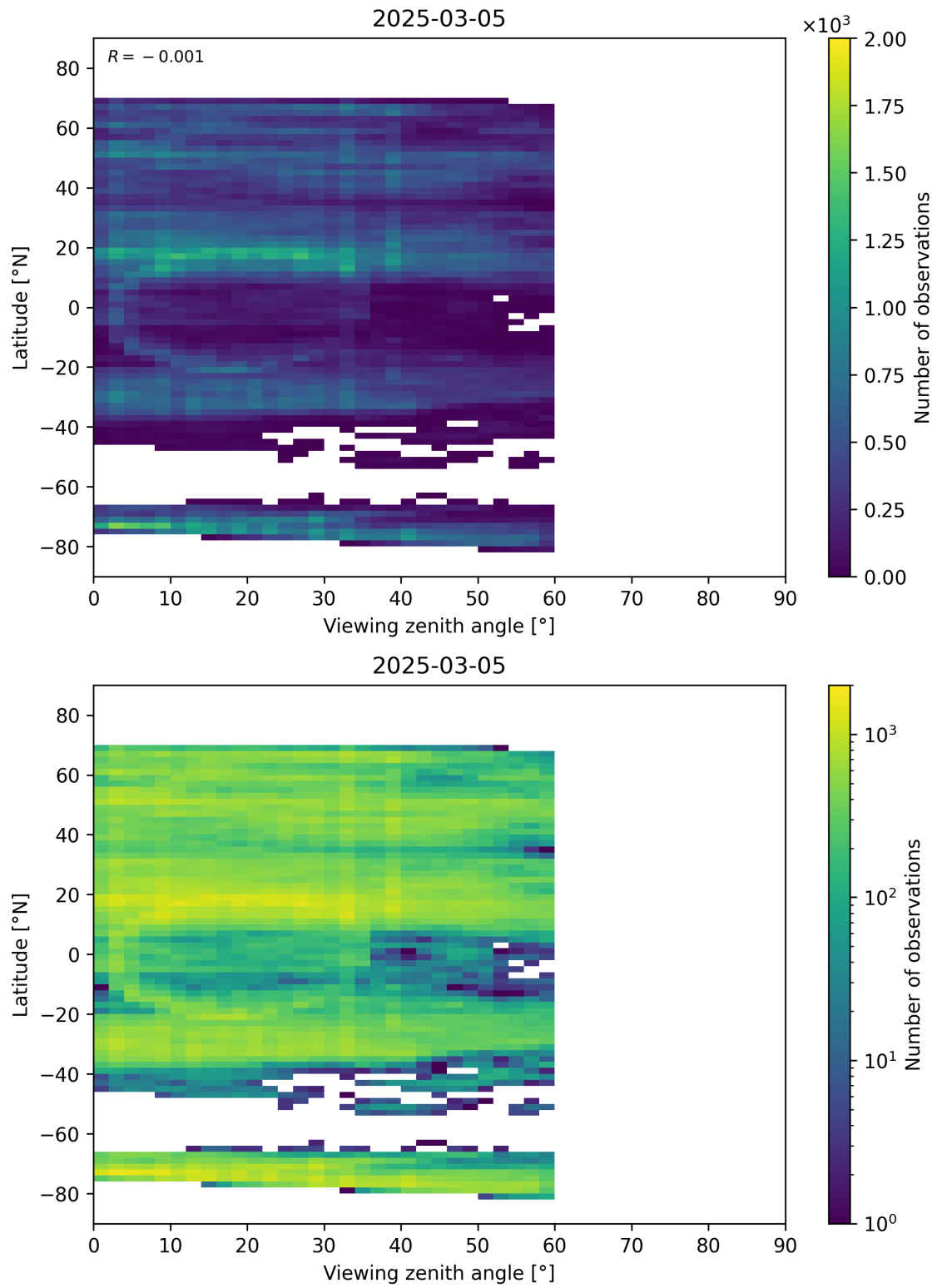
Figure 109: Scatter density plot of “Viewing zenith angle” against “Latitude” for 2025-03-04 to 2025-03-06.
