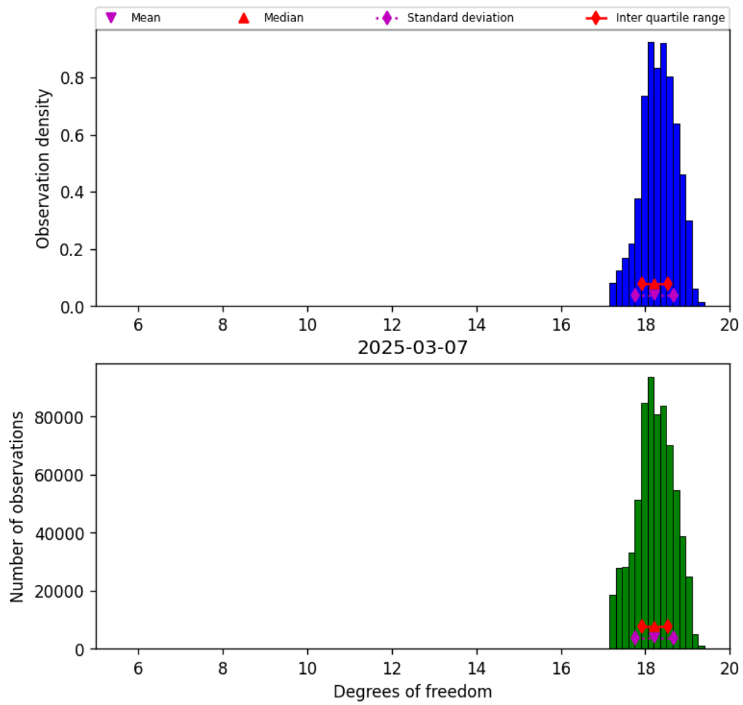
Figure 30: Histogram of “Degrees of freedom” for 2025-03-07 to 2025-03-08
