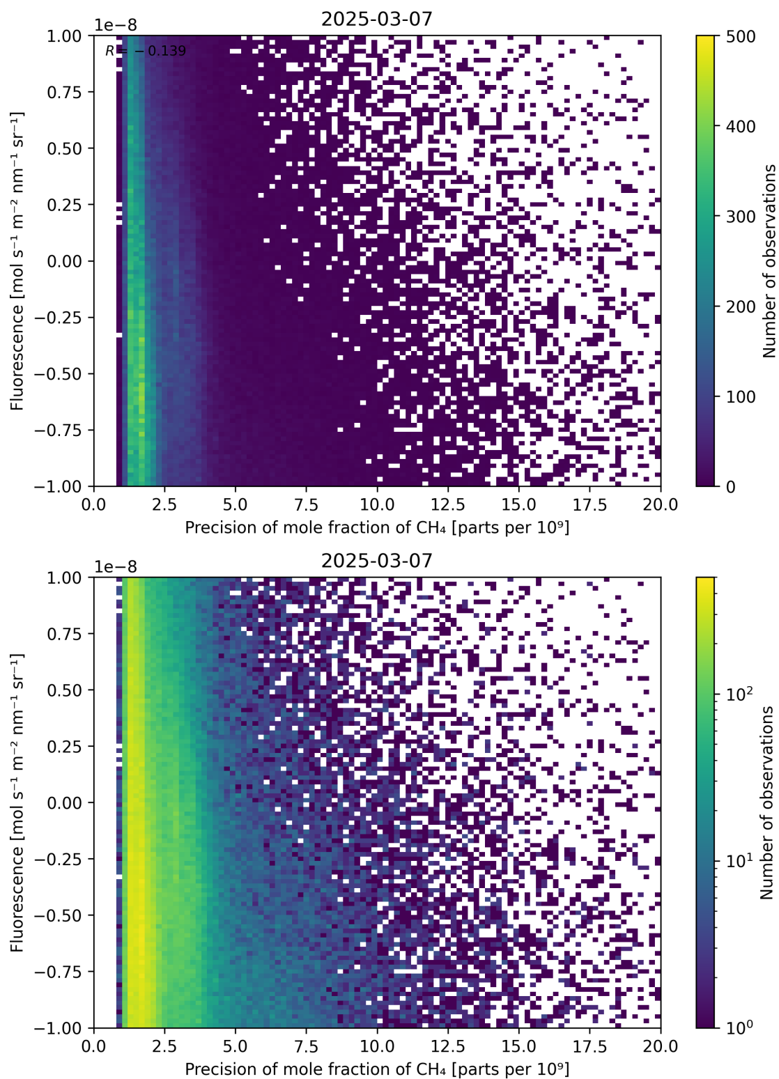
Figure 81: Scatter density plot of “Precision of mole fraction of CH 4 ” against “Fluorescence” for 2025-03-07 to 2025-03-08.
