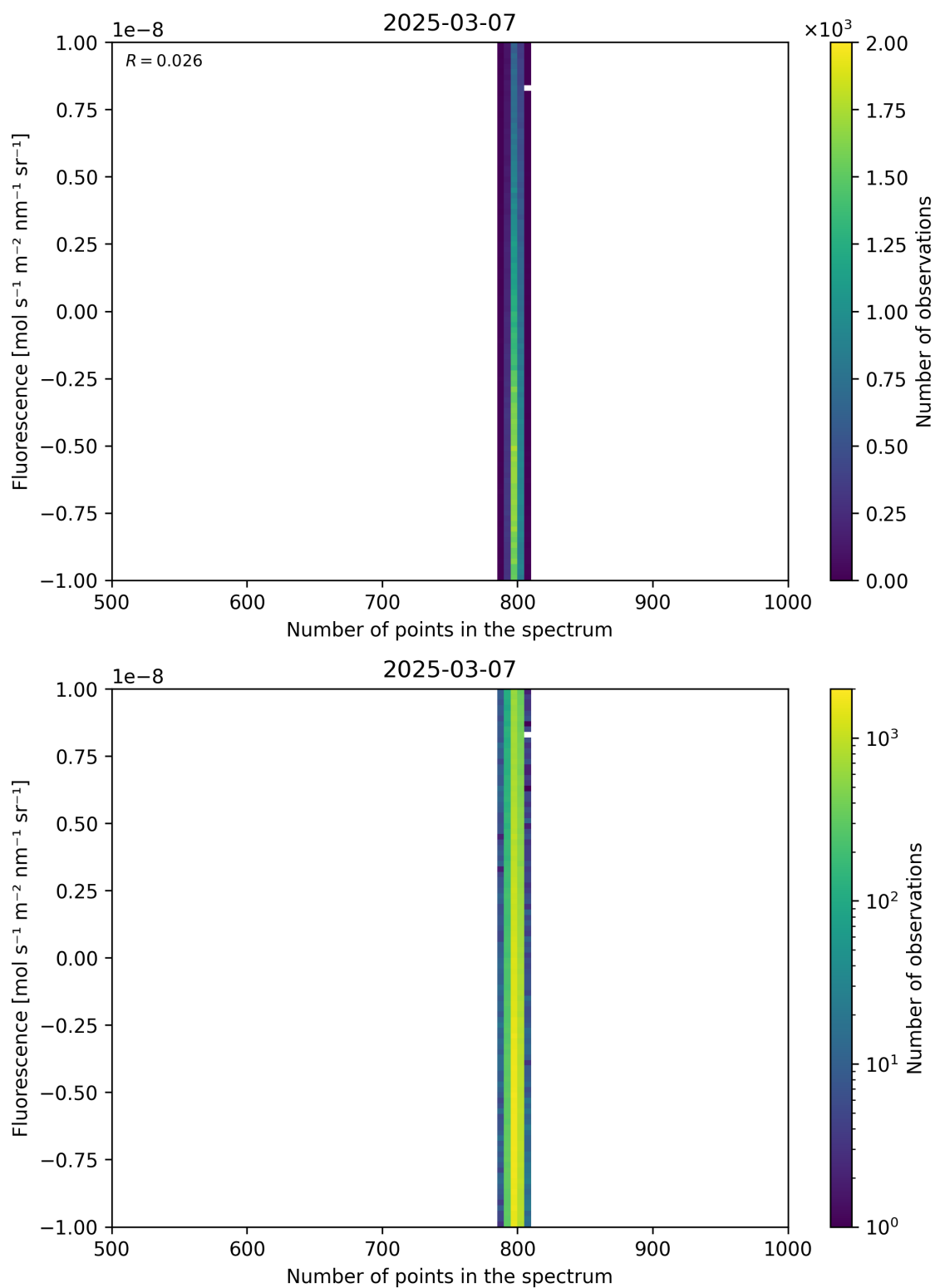
Figure 91: Scatter density plot of “Number of points in the spectrum” against “Fluorescence” for 2025-03-07 to 2025-03-08.
