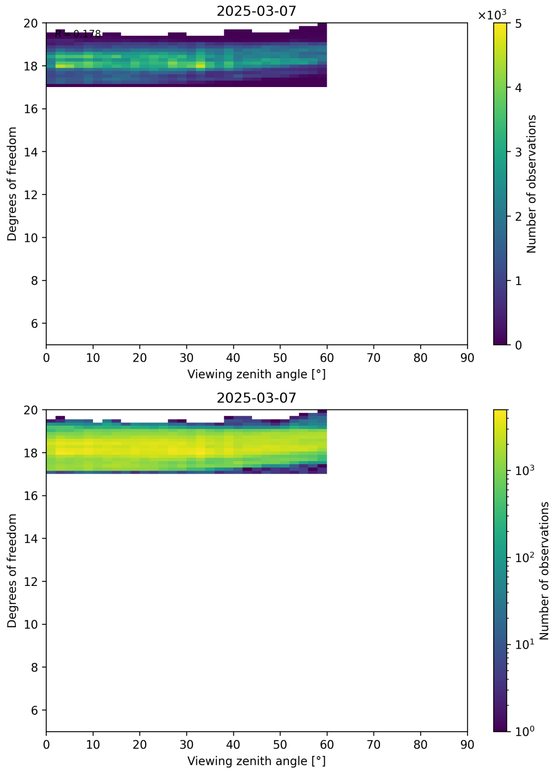
Figure 107: Scatter density plot of “Viewing zenith angle” against “Degrees of freedom” for 2025-03-07 to 2025-03-08.
