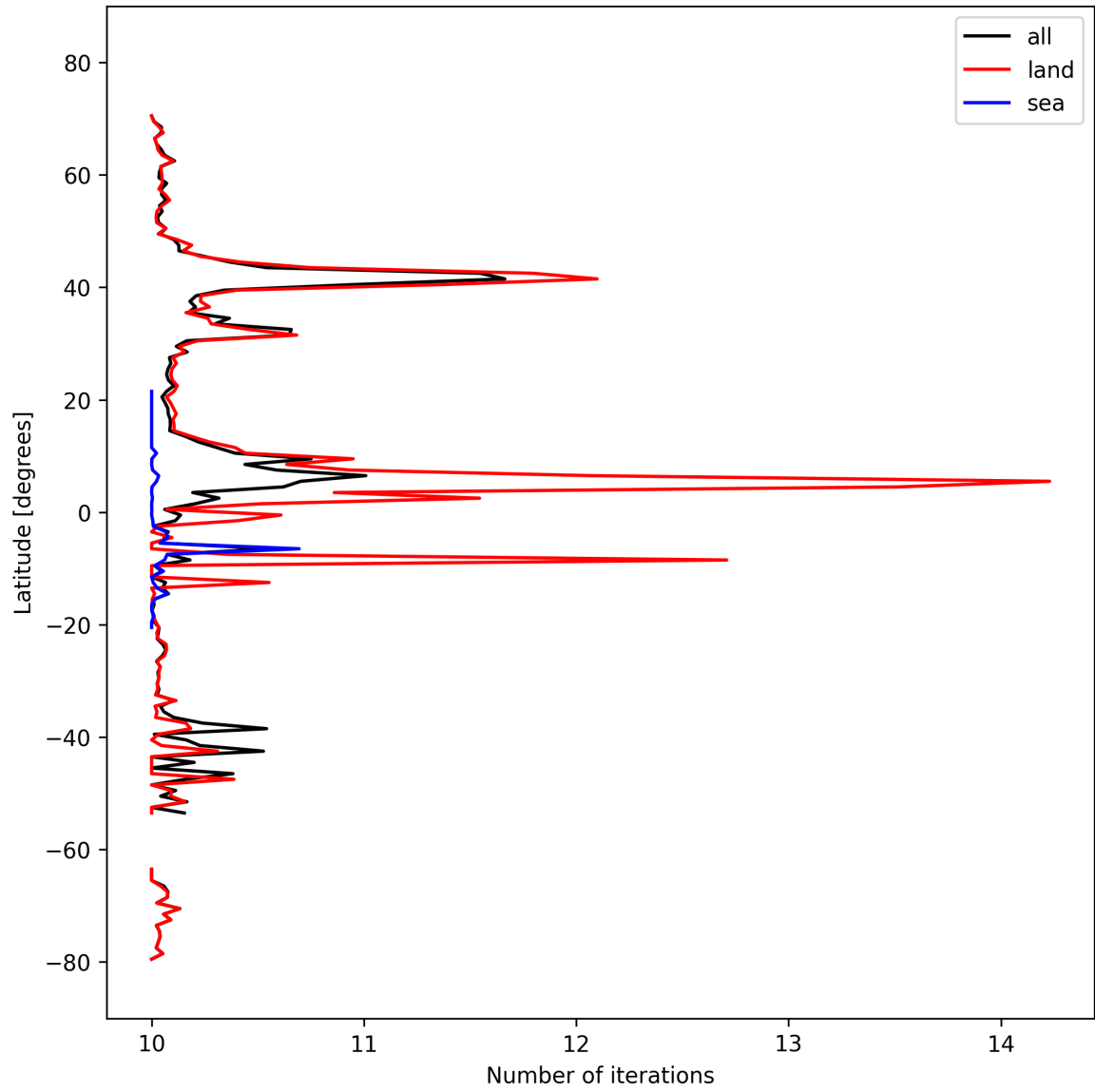
Figure 20: Zonal average of “Number of iterations” for 2025-03-07 to 2025-03-08.
