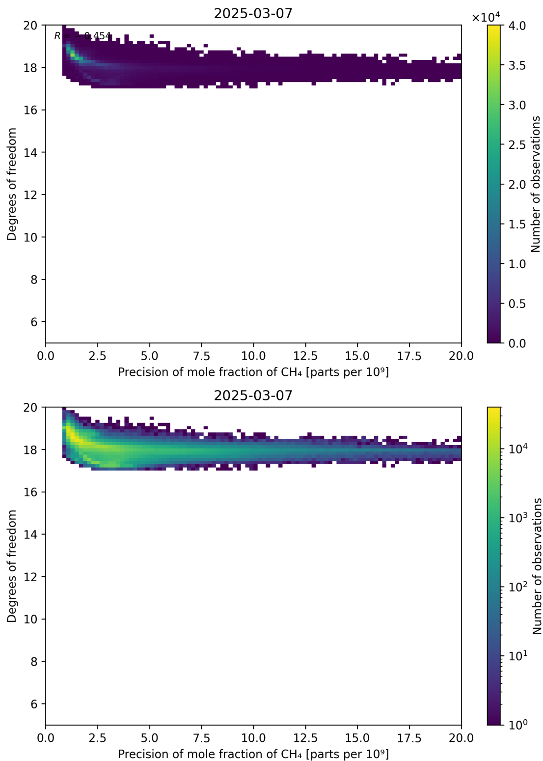
Figure 80: Scatter density plot of “Precision of mole fraction of CH 4 ” against “Degrees of freedom” for 2025-03-07 to 2025-03-08.
