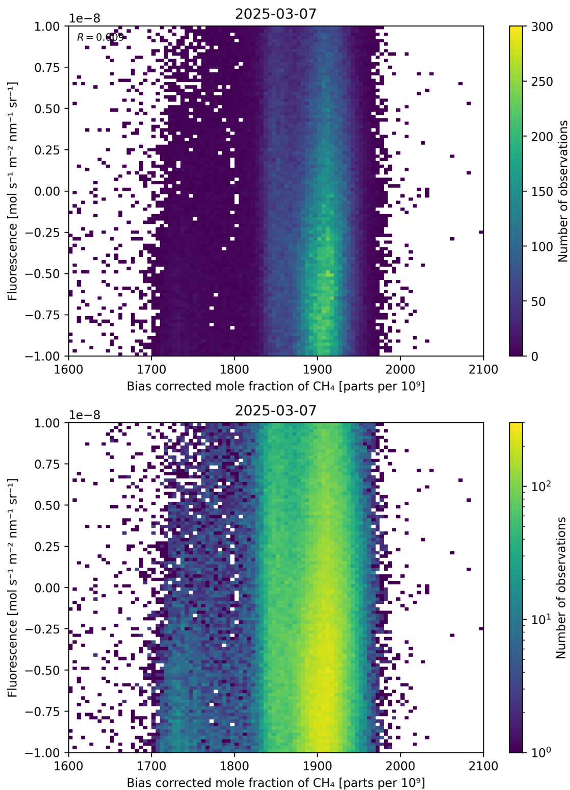
Figure 66: Scatter density plot of “Bias corrected mole fraction of \text{CH}_4 ” against “Fluorescence” for 2025-03-07 to 2025-03-08.
