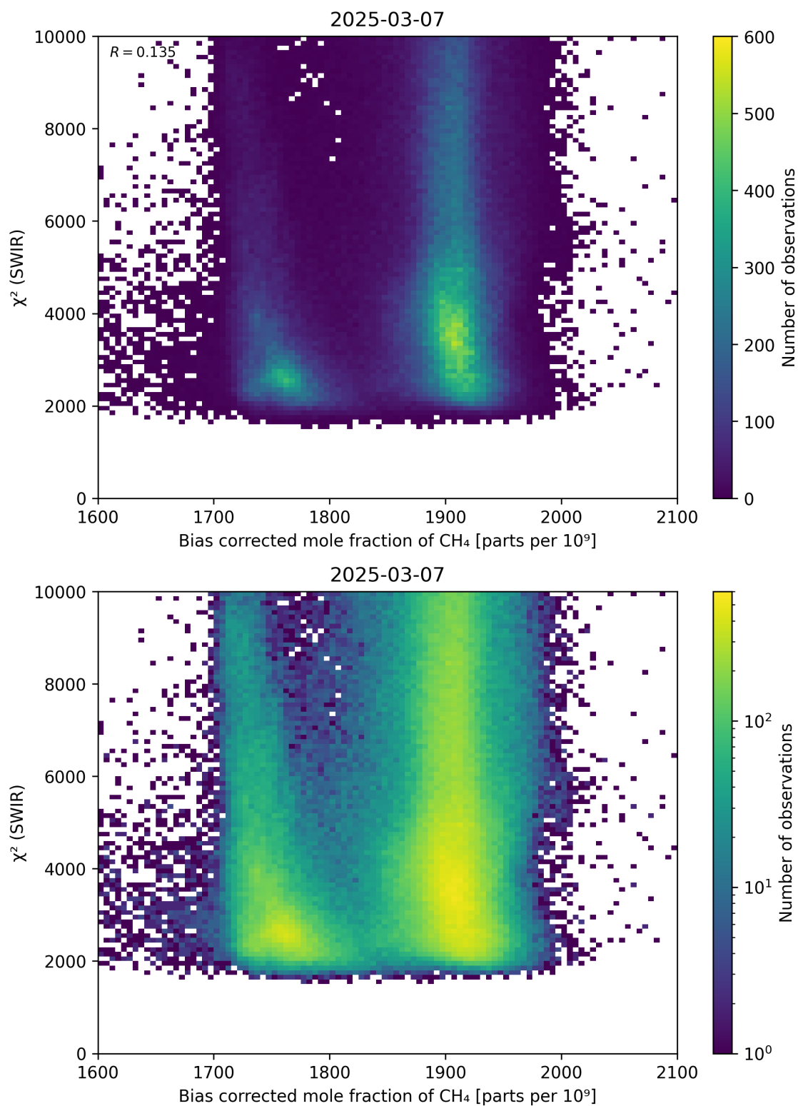
Figure 64: Scatter density plot of “Bias corrected mole fraction of \text{CH}_4 ” against “ \chi^2 (SWIR)” for 2025-03-07 to 2025-03-08.
