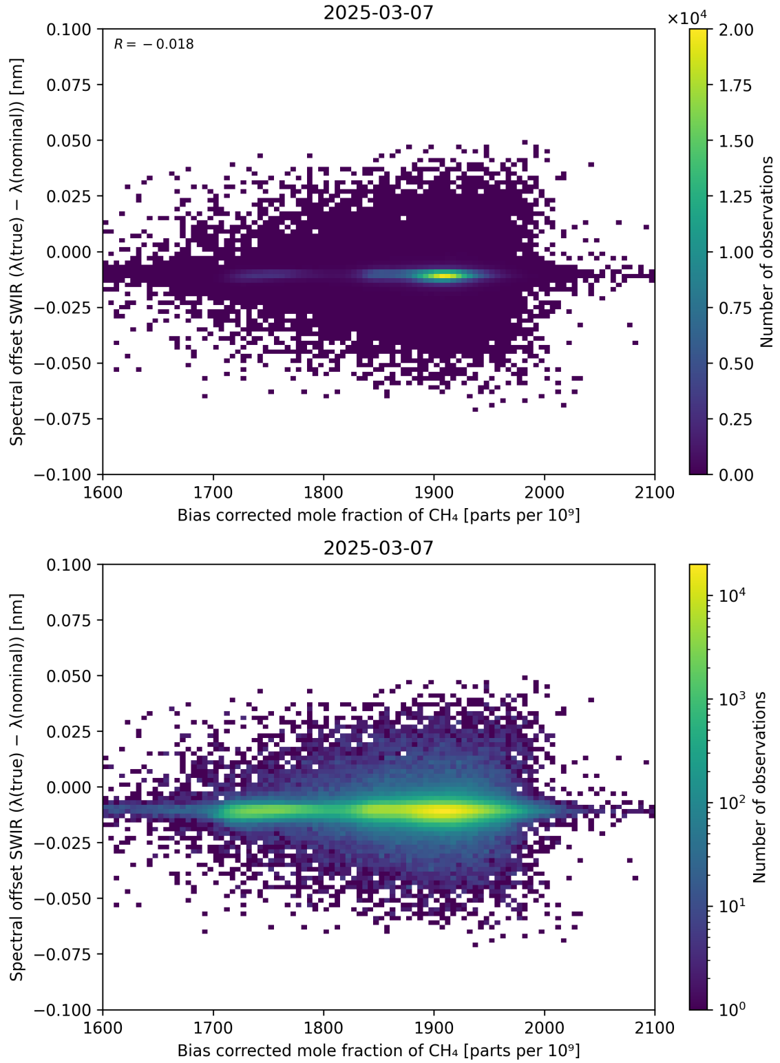
Figure 69: Scatter density plot of “Bias corrected mole fraction of \text{CH}_4 ” against “Spectral offset SWIR ( \lambda_{\text{true}} - \lambda_{\text{nominal}} )” for 2025-03-07 to 2025-03-08.
