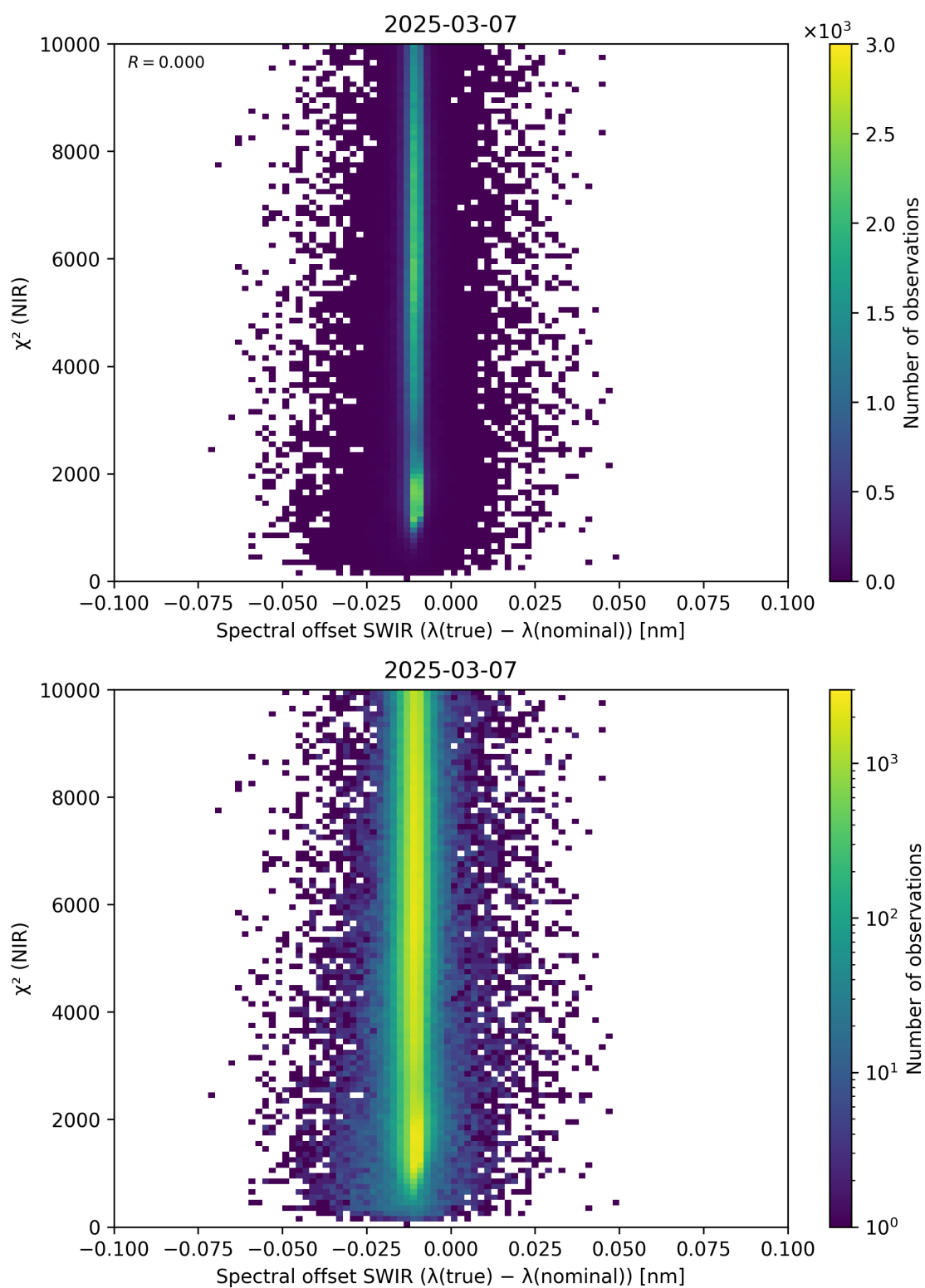
Figure 117: Scatter density plot of “Spectral offset SWIR ( \lambda_{\text{true}} - \lambda_{\text{nominal}} )” against “ \chi^2 (NIR)” for 2025-03-07 to 2025-03-08.
