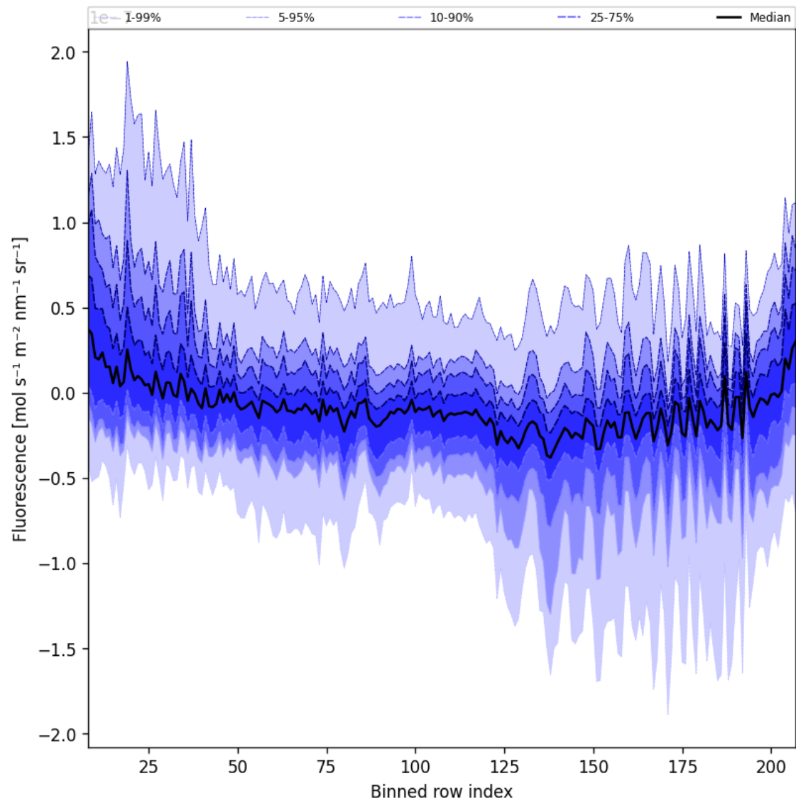
Figure 43: Along track statistics of “Fluorescence” for 2025-03-07 to 2025-03-08
