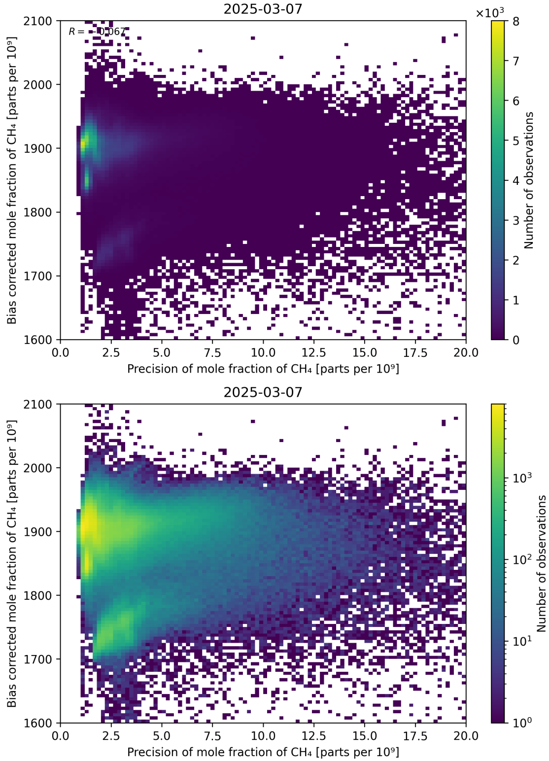
Figure 82: Scatter density plot of “Precision of mole fraction of CH 4 ” against “Bias corrected mole fraction of CH 4 ” for 2025-03-07 to 2025-03-08.
