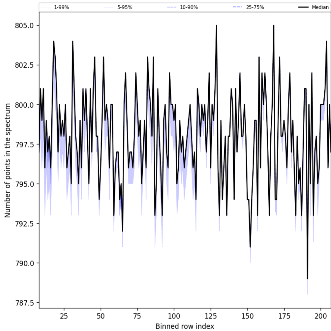
Figure 37: Along track statistics of “Number of points in the spectrum” for 2025-03-07 to 2025-03-08
