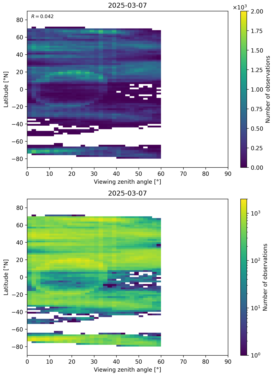
Figure 109: Scatter density plot of “Viewing zenith angle” against “Latitude” for 2025-03-07 to 2025-03-08.
