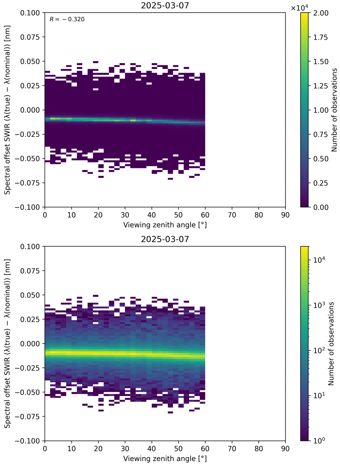
Figure 116: Scatter density plot of “Viewing zenith angle” against “Spectral offset SWIR ( \lambda_{\text{true}} - \lambda_{\text{nominal}} )” for 2025-03-07 to 2025-03-08.
