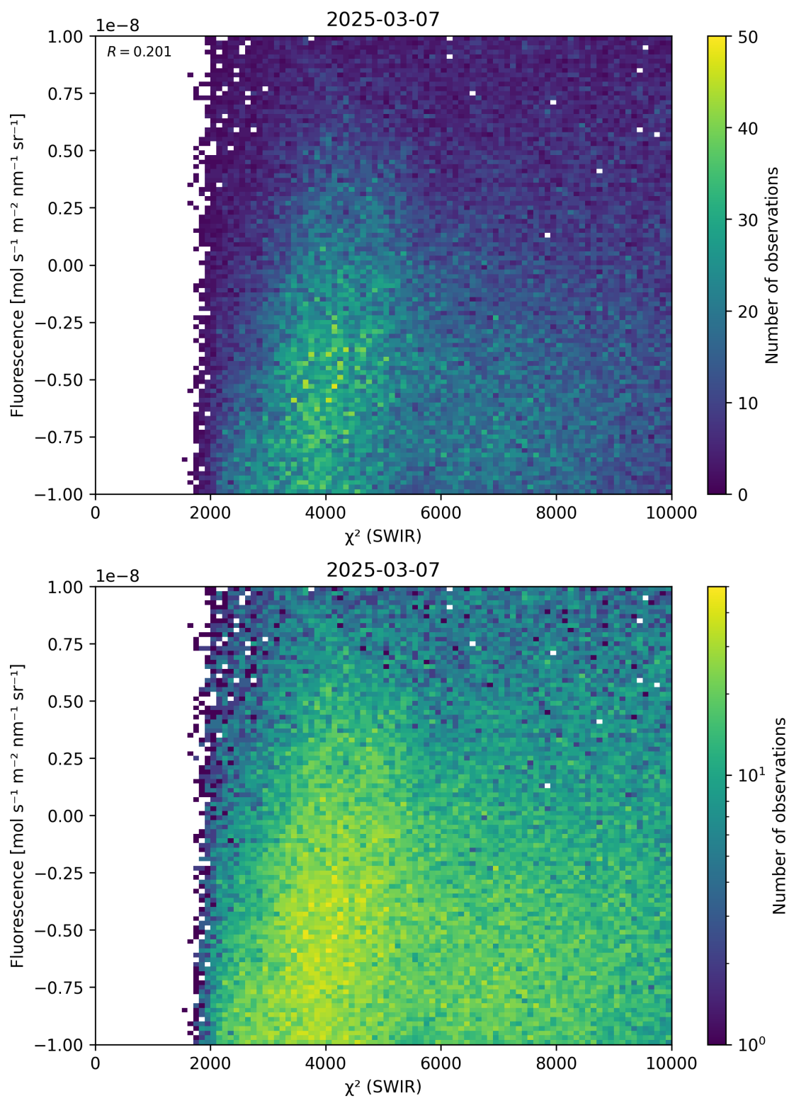
Figure 49: Scatter density plot of “ \chi^2 (SWIR)” against “Fluorescence” for 2025-03-07 to 2025-03-08.
