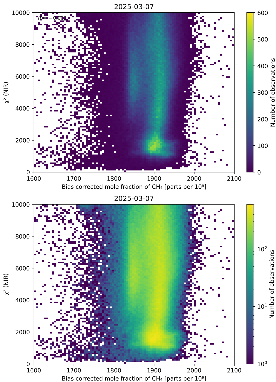
Figure 63: Scatter density plot of “Bias corrected mole fraction of \text{CH}_4 ” against “ \chi^2 (NIR)” for 2025-03-07 to 2025-03-08.
