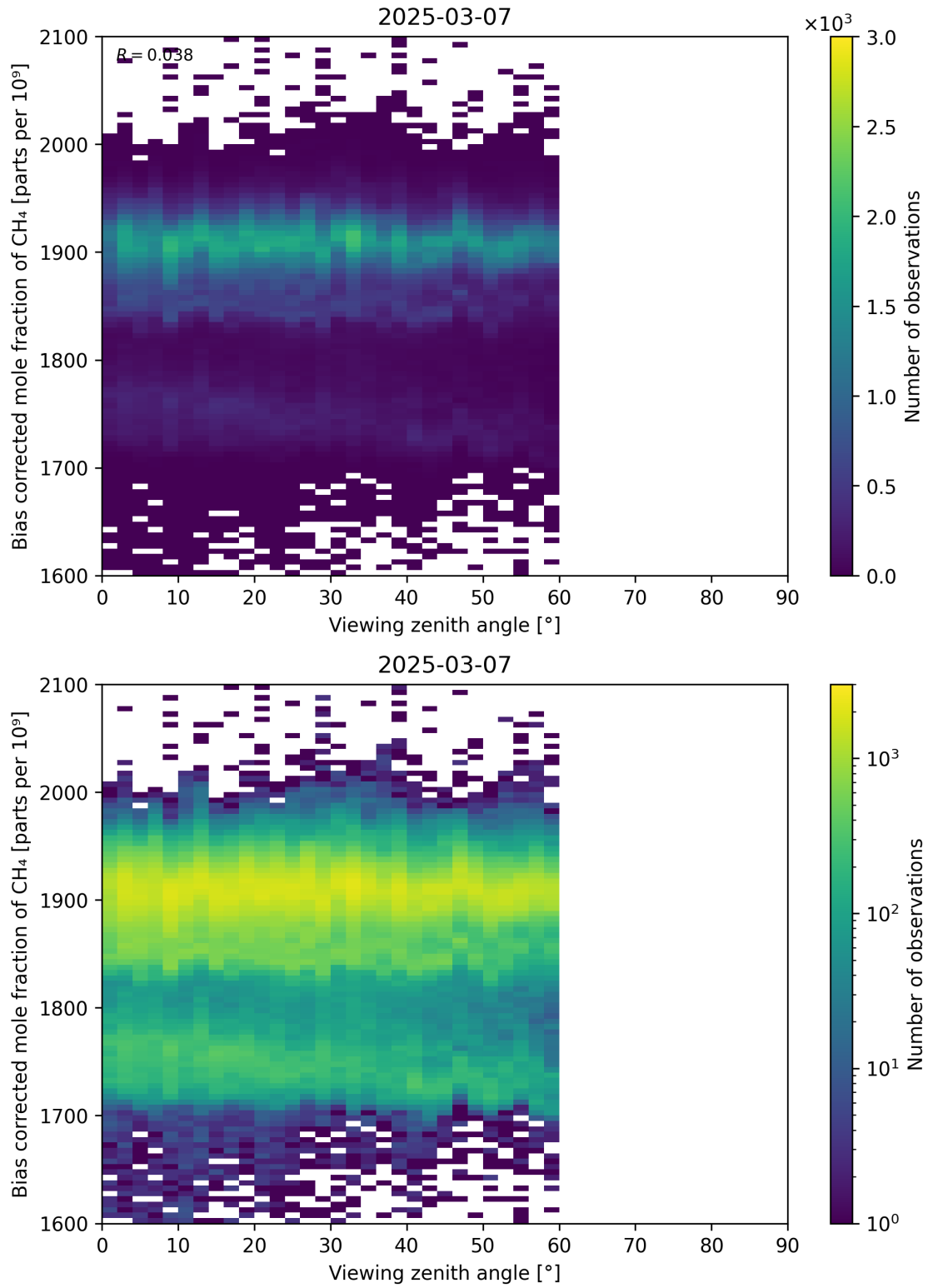
Figure 111: Scatter density plot of “Viewing zenith angle” against “Bias corrected mole fraction of CH 4 ” for 2025-03-07 to 2025-03-08.
