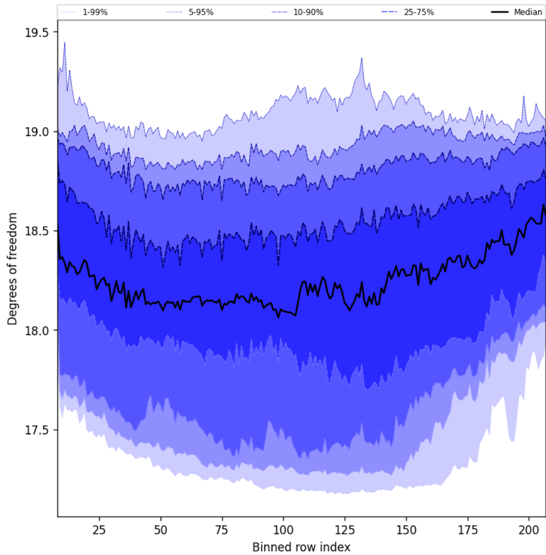
Figure 41: Along track statistics of “Degrees of freedom” for 2025-03-07 to 2025-03-08
