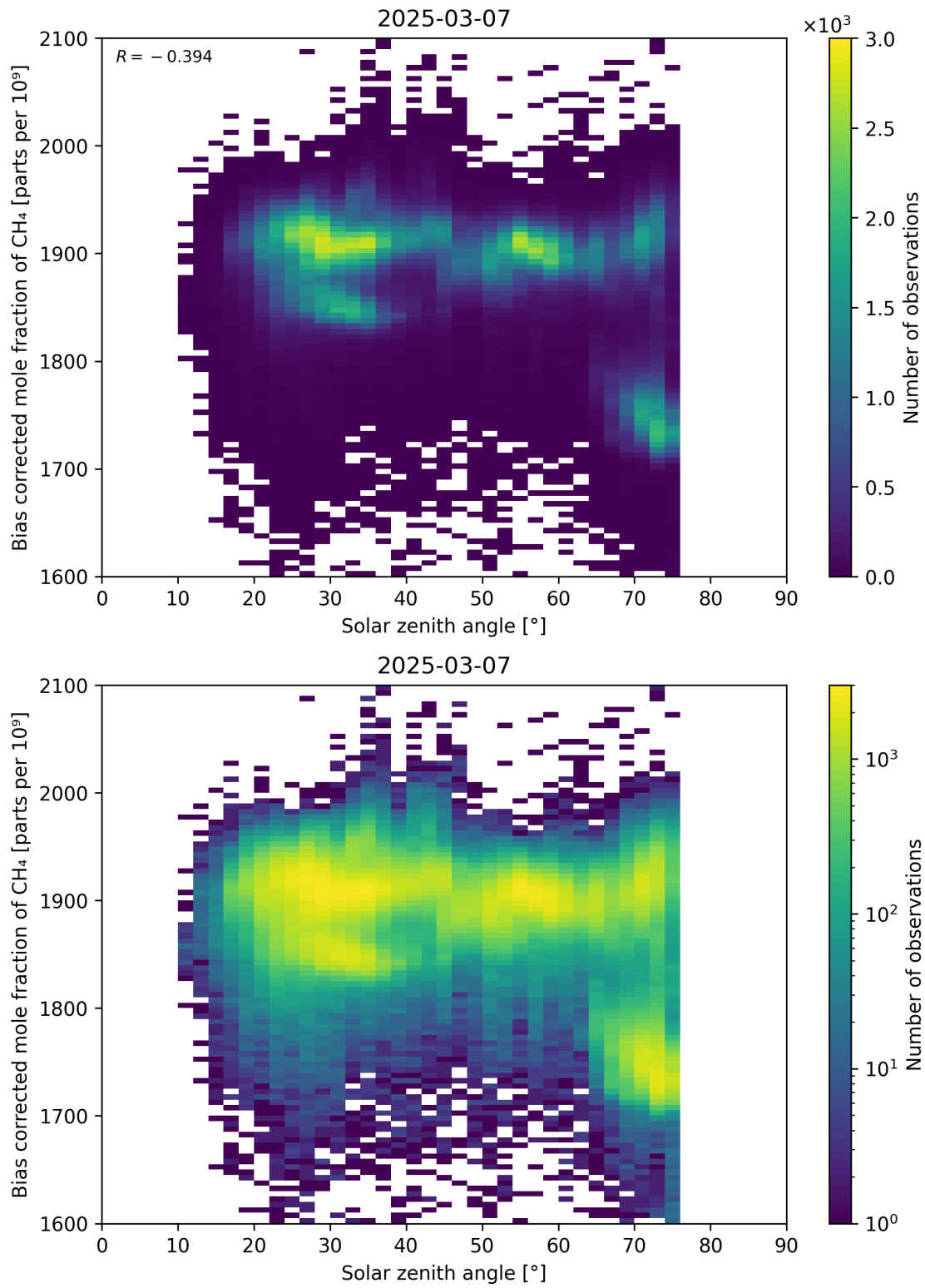
Figure 100: Scatter density plot of “Solar zenith angle” against “Bias corrected mole fraction of CH 4 ” for 2025-03-07 to 2025-03-08.
