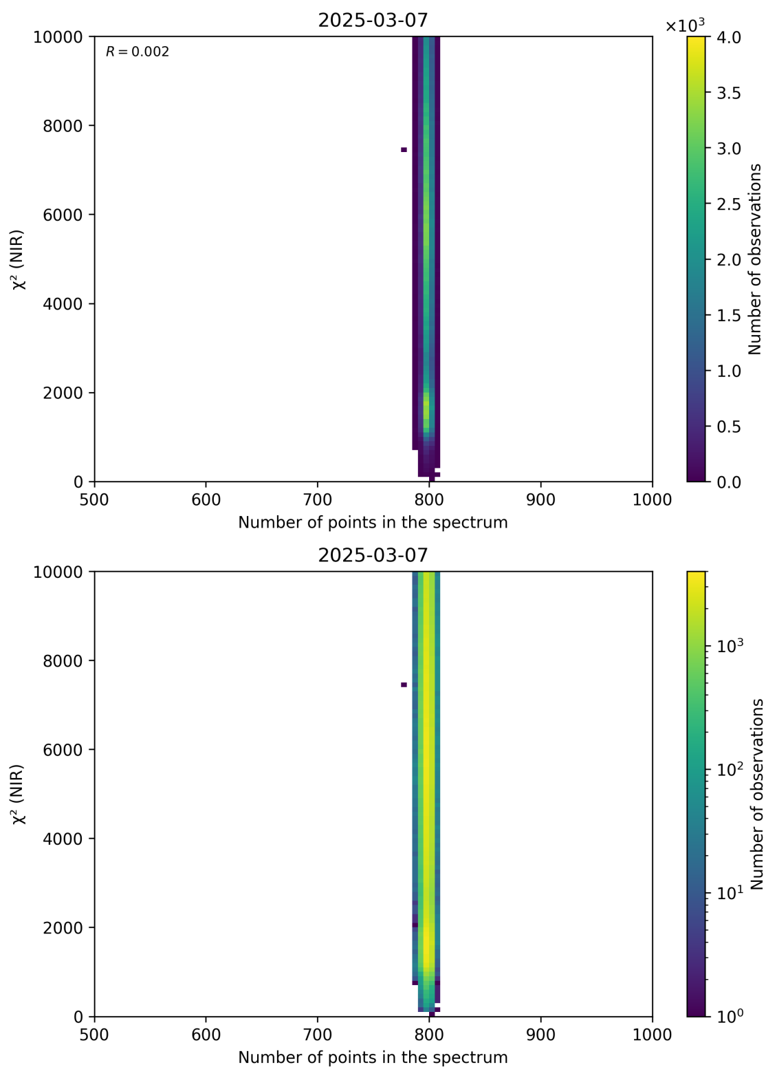
Figure 88: Scatter density plot of “Number of points in the spectrum” against “ \chi^2 (NIR)” for 2025-03-07 to 2025-03-08.
