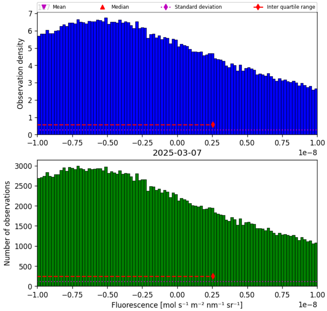
Figure 32: Histogram of “Fluorescence” for 2025-03-07 to 2025-03-08
