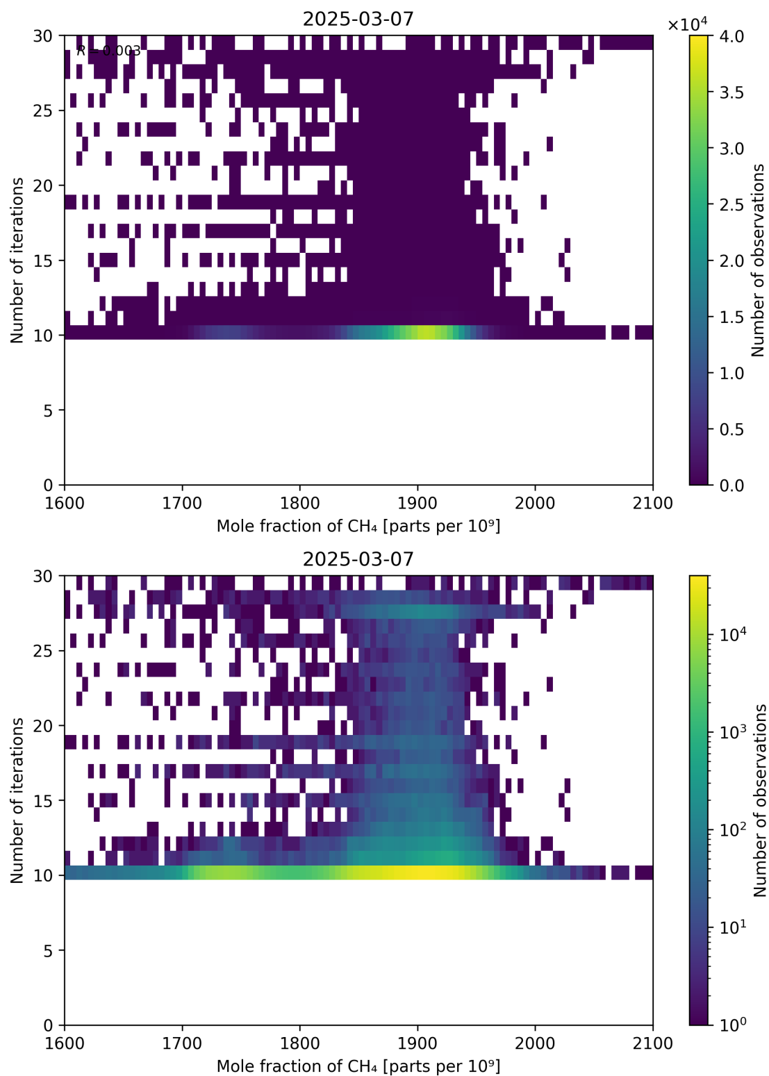
Figure 76: Scatter density plot of “Mole fraction of CH 4 ” against “Number of iterations” for 2025-03-07 to 2025-03-08.
