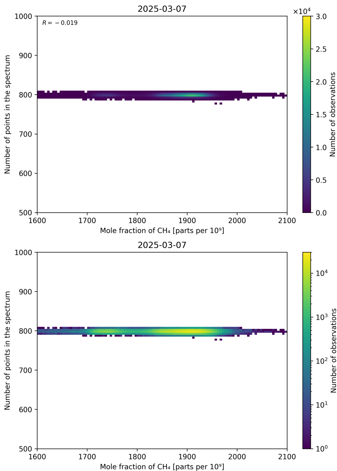
Figure 77: Scatter density plot of “Mole fraction of CH 4 ” against “Number of points in the spectrum” for 2025-03-07 to 2025-03-08.
