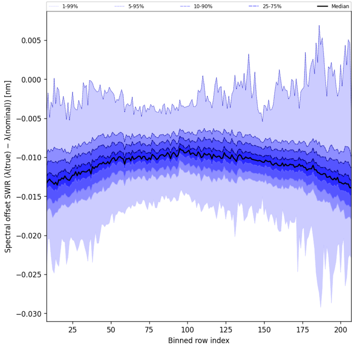
Figure 38: Along track statistics of “Spectral offset SWIR ( \lambda_{\text{true}} - \lambda_{\text{nominal}} )” for 2025-03-07 to 2025-03-08
