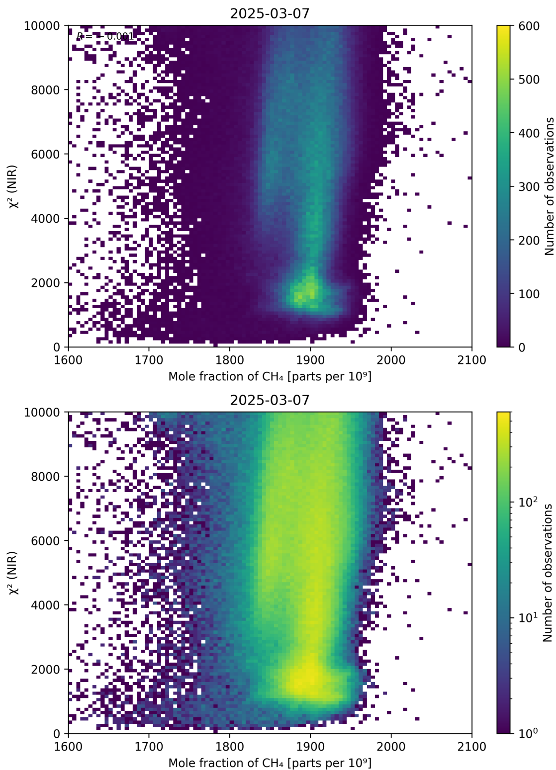
Figure 70: Scatter density plot of “Mole fraction of \text{CH}_4 ” against “ \chi^2 (NIR)” for 2025-03-07 to 2025-03-08.
