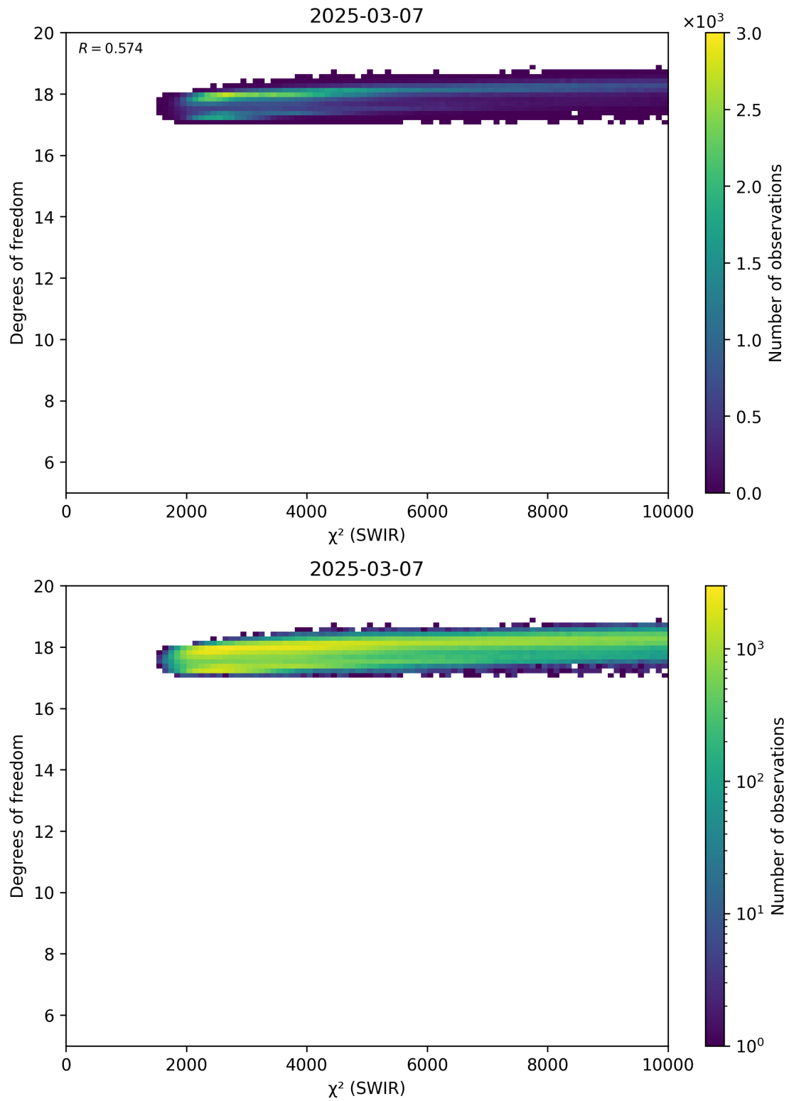
Figure 48: Scatter density plot of “ \chi^2 (SWIR)” against “Degrees of freedom” for 2025-03-07 to 2025-03-08.
