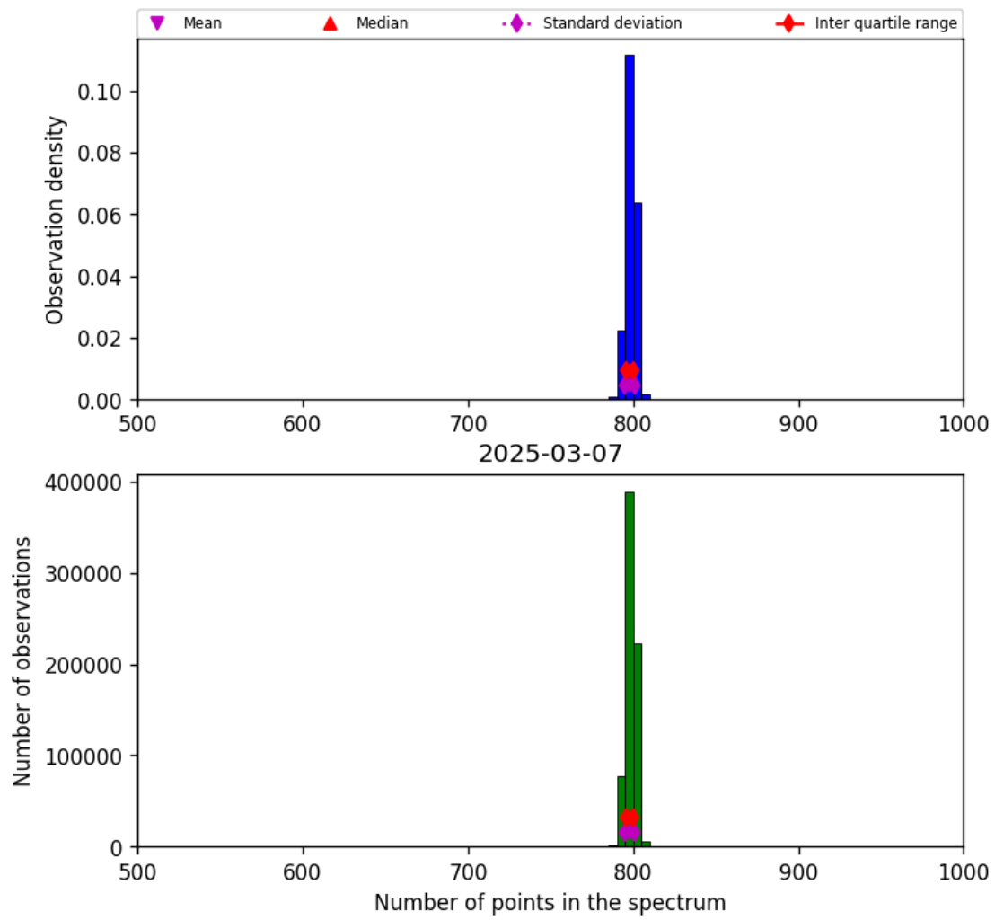
Figure 26: Histogram of “Number of points in the spectrum” for 2025-03-07 to 2025-03-08
