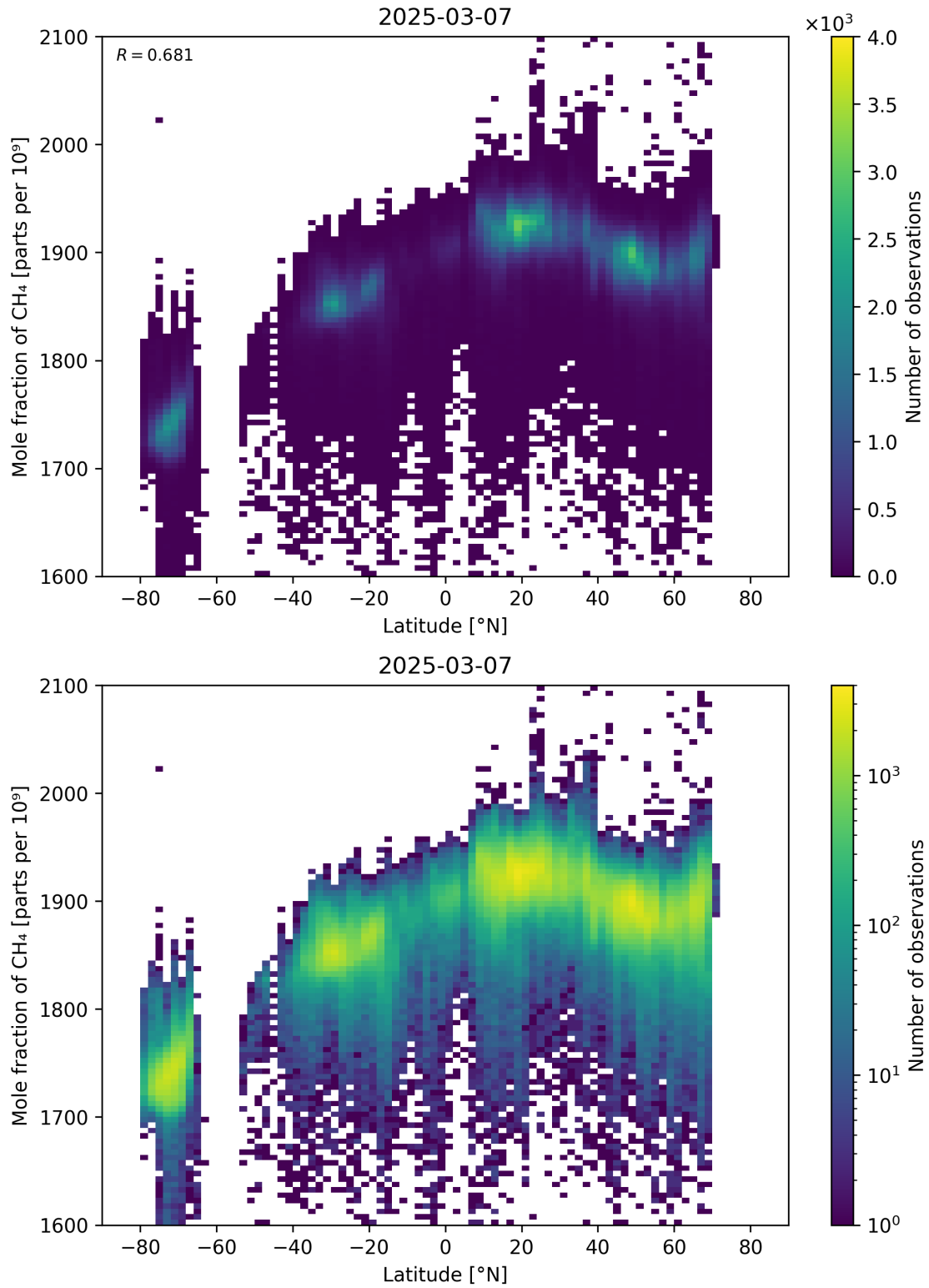
Figure 57: Scatter density plot of “Latitude” against “Mole fraction of CH 4 ” for 2025-03-07 to 2025-03-08.
