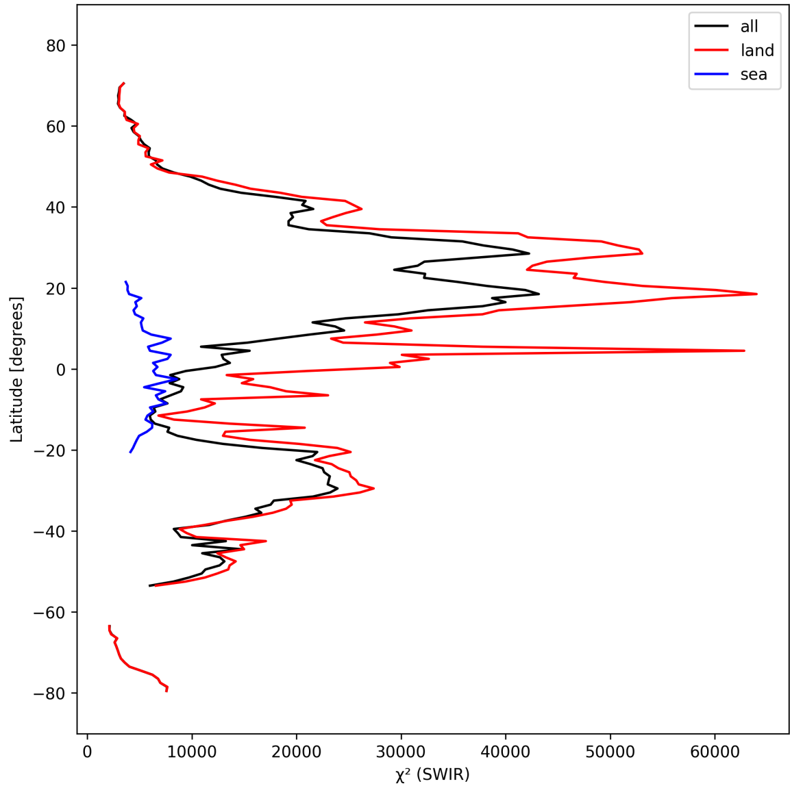
Figure 17: Zonal average of “ \chi^2 (SWIR)” for 2025-03-07 to 2025-03-08.
