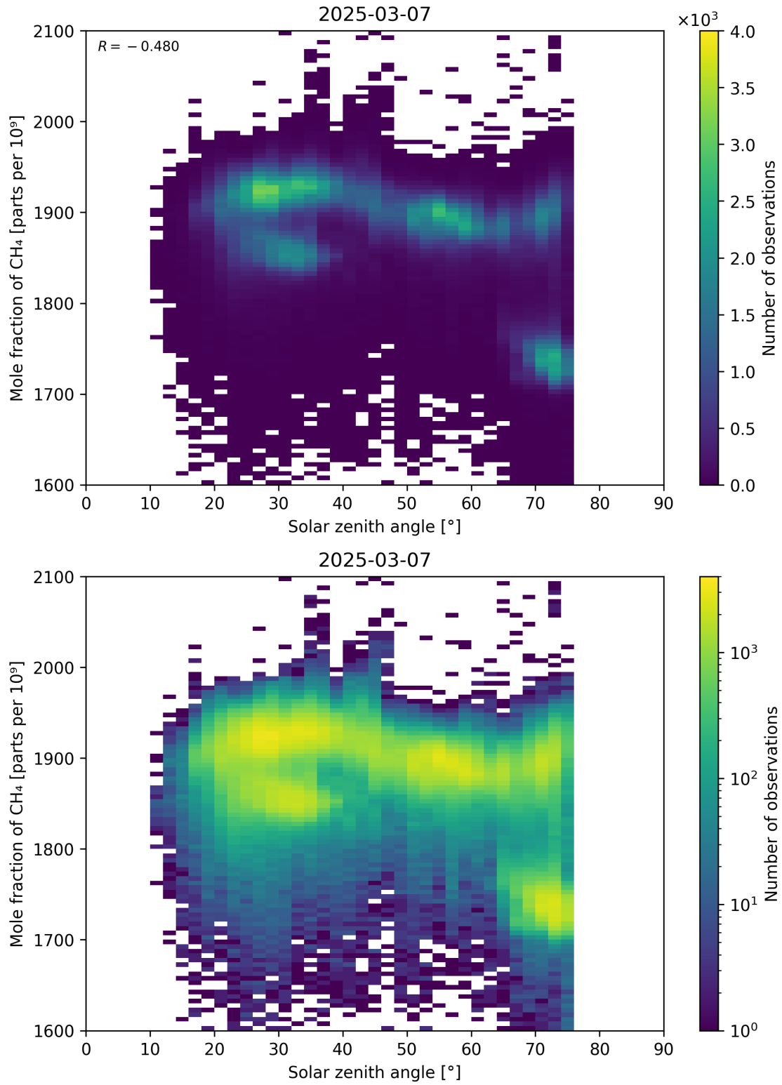
Figure 99: Scatter density plot of “Solar zenith angle” against “Mole fraction of CH 4 ” for 2025-03-07 to 2025-03-08.
