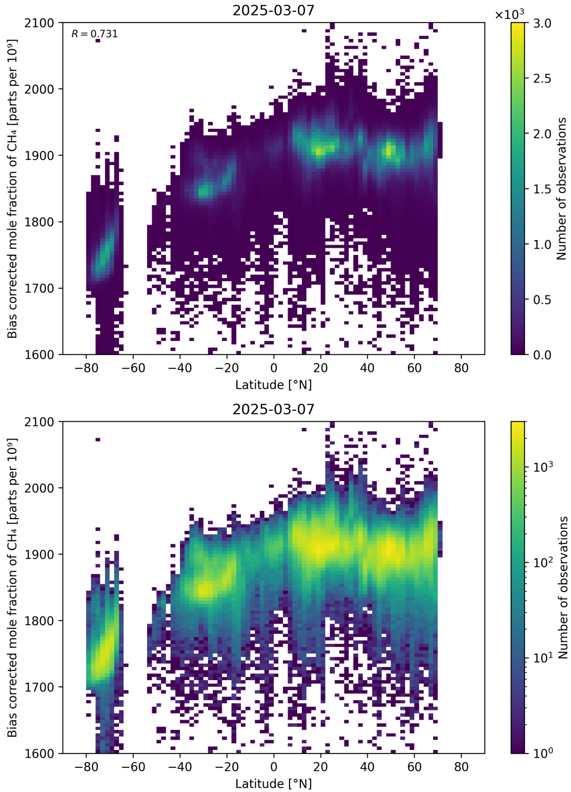
Figure 58: Scatter density plot of “Latitude” against “Bias corrected mole fraction of CH 4 ” for 2025-03-07 to 2025-03-08.
