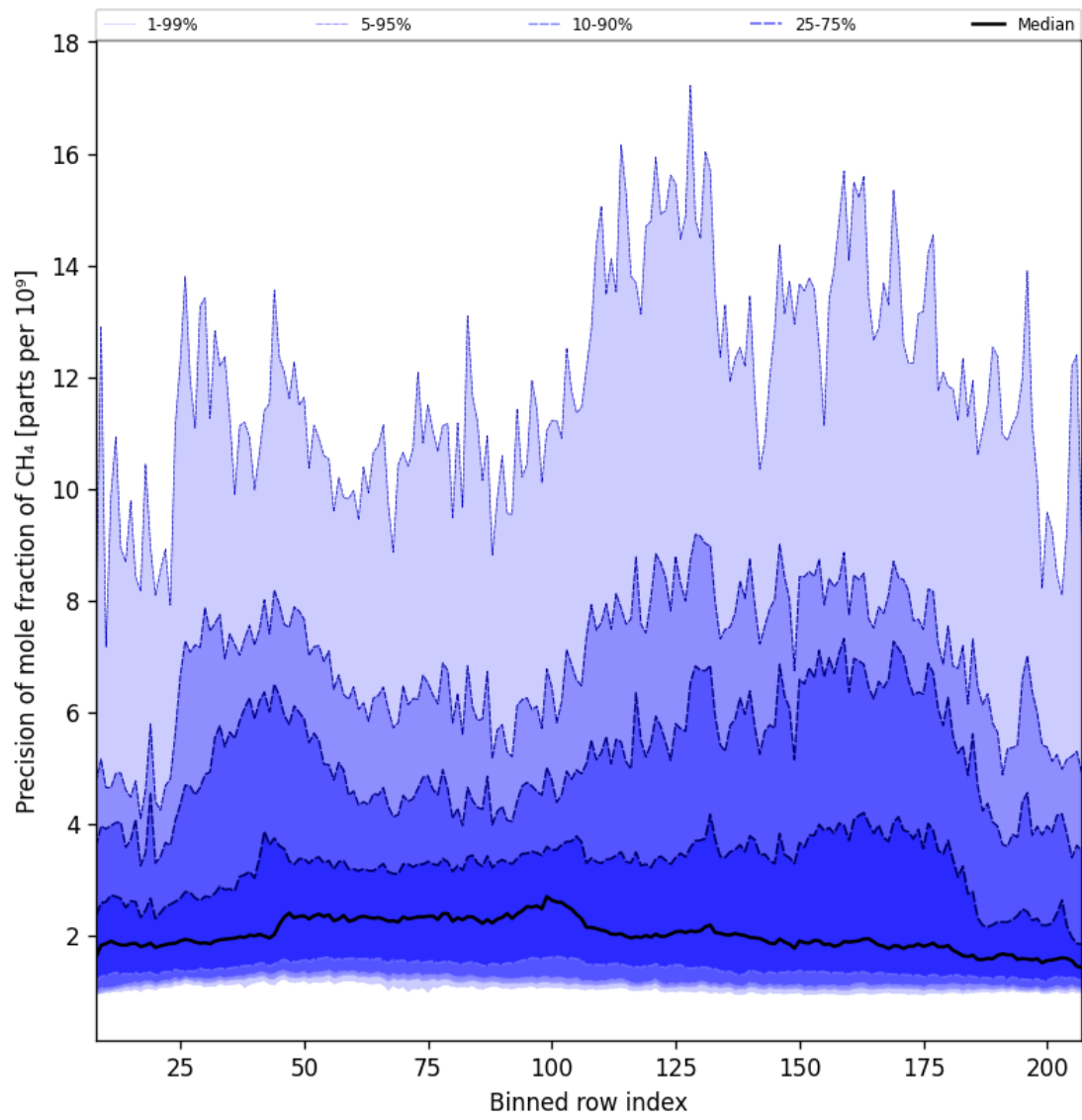
Figure 35: Along track statistics of “Precision of mole fraction of CH 4 ” for 2025-03-07 to 2025-03-08
