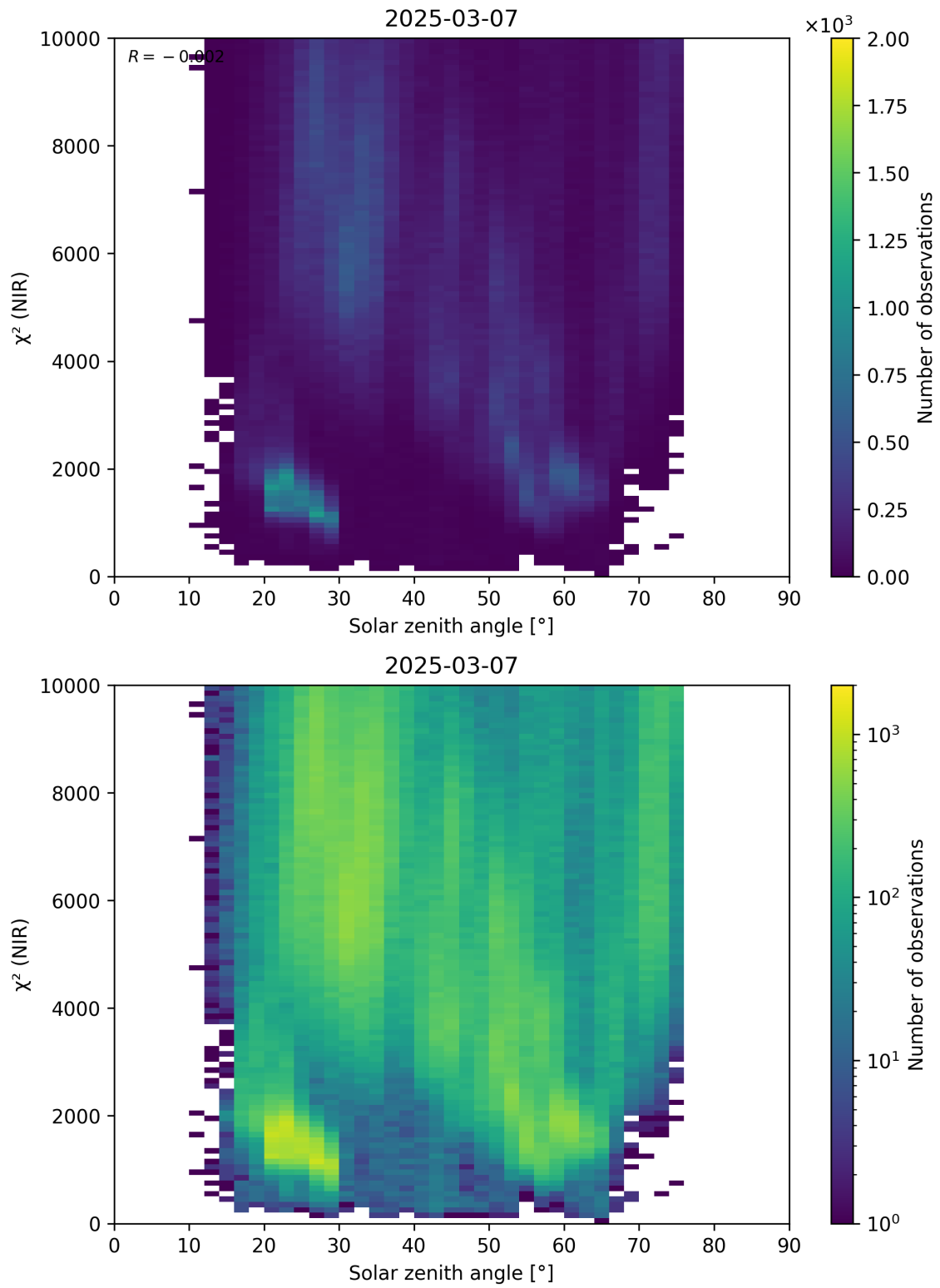
Figure 94: Scatter density plot of “Solar zenith angle” against “ \chi^2 (NIR)” for 2025-03-07 to 2025-03-08.
