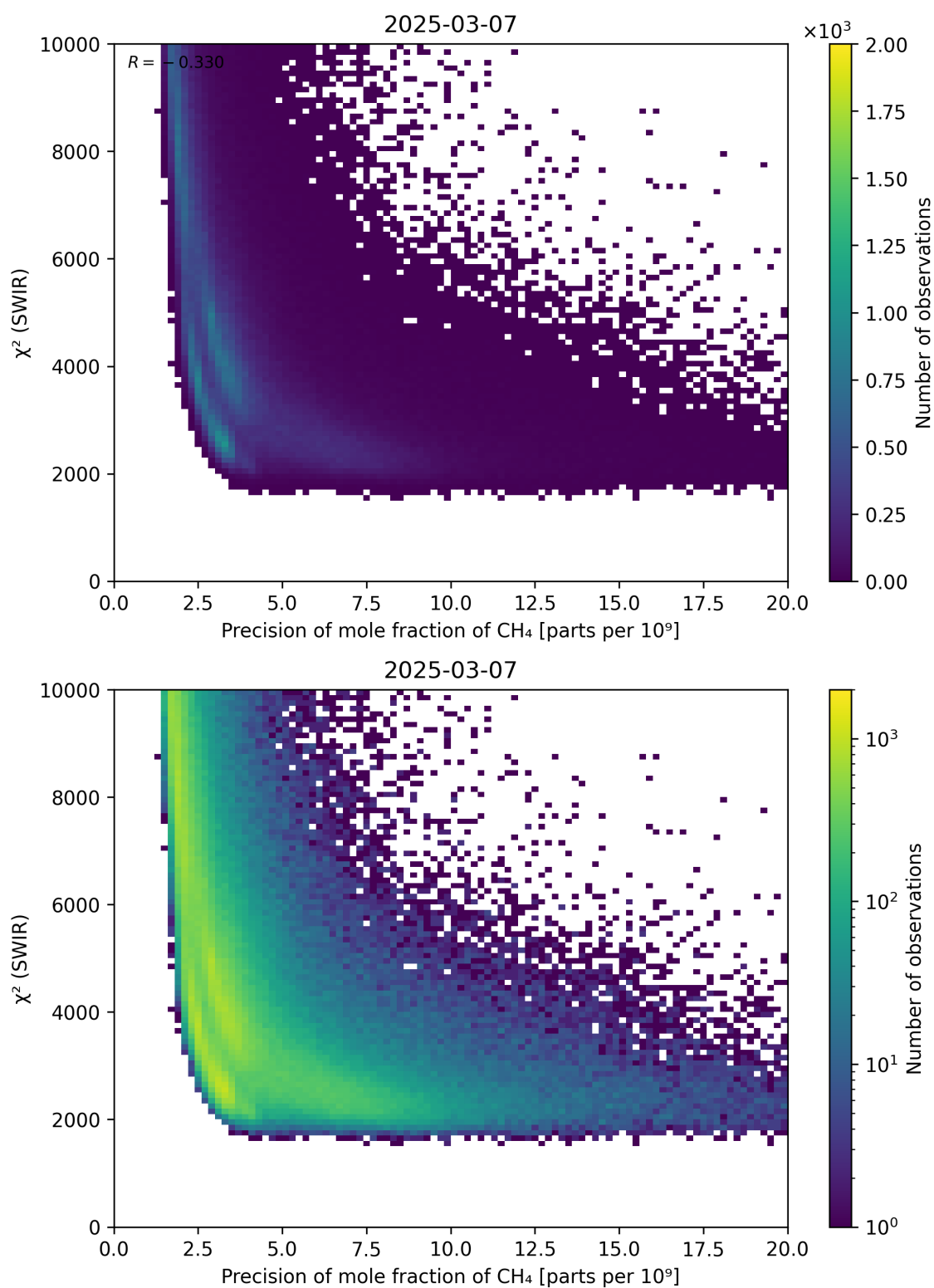
Figure 79: Scatter density plot of “Precision of mole fraction of CH 4 ” against “ \chi^2 (SWIR)” for 2025-03-07 to 2025-03-08.
