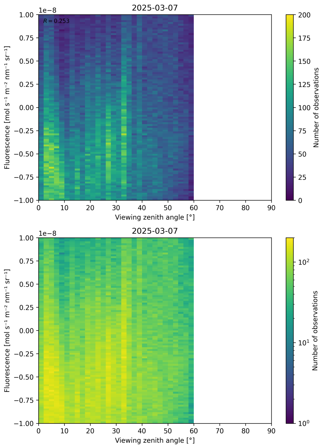
Figure 108: Scatter density plot of “Viewing zenith angle” against “Fluorescence” for 2025-03-07 to 2025-03-08.
