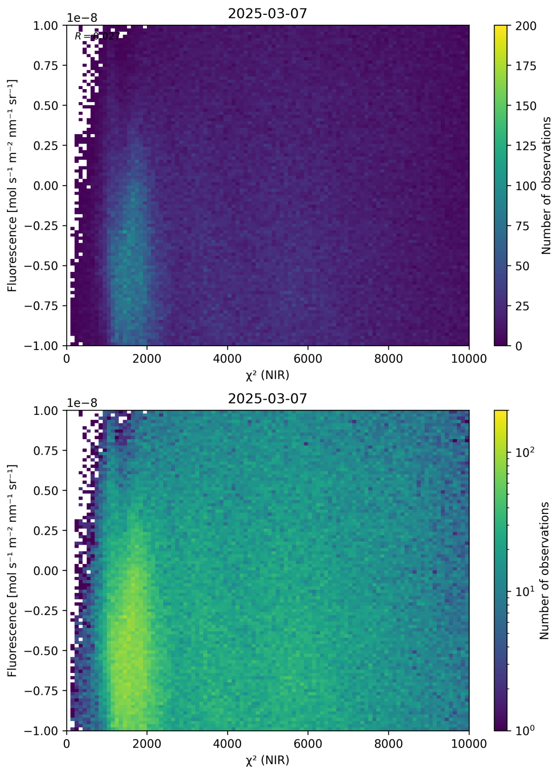
Figure 45: Scatter density plot of “ \chi^2 (NIR)” against “Fluorescence” for 2025-03-07 to 2025-03-08.
