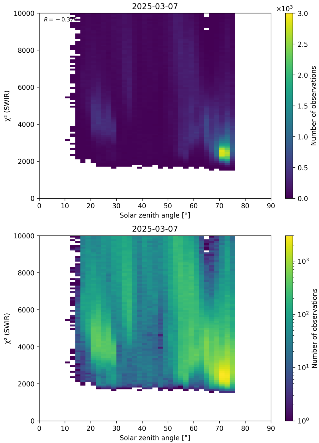
Figure 95: Scatter density plot of “Solar zenith angle” against “ \chi^2 (SWIR)” for 2025-03-07 to 2025-03-08.
