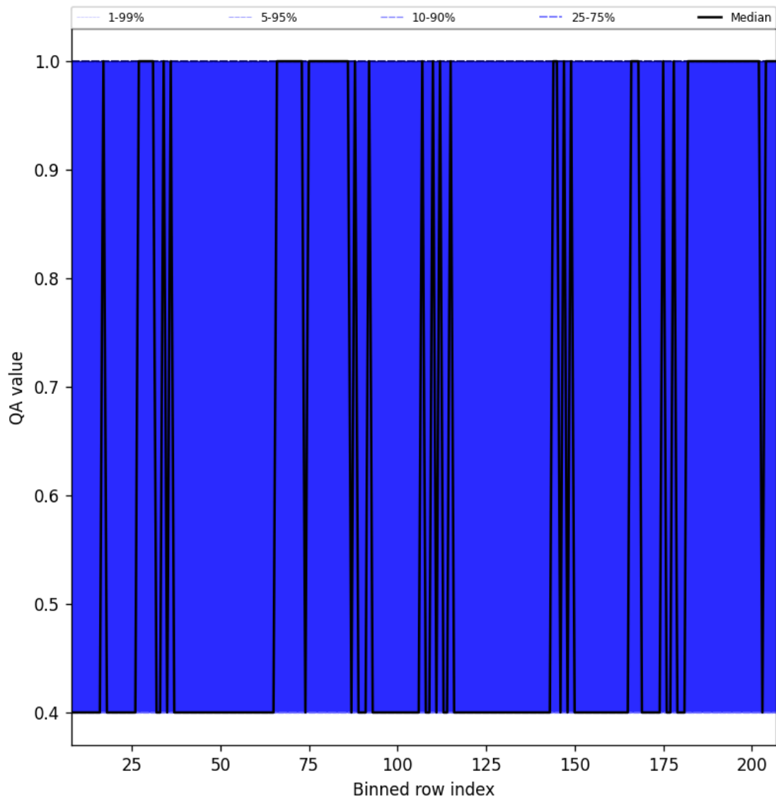
Figure 33: Along track statistics of “QA value” for 2025-03-07 to 2025-03-08
