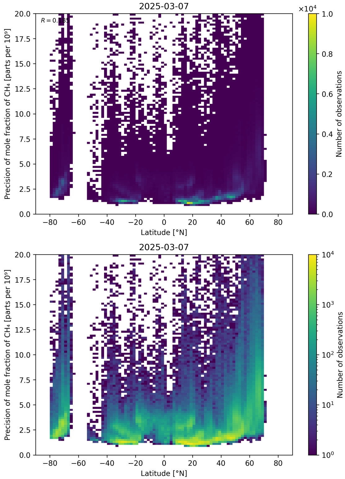
Figure 59: Scatter density plot of “Latitude” against “Precision of mole fraction of \text{CH}_4 ” for 2025-03-07 to 2025-03-08.
