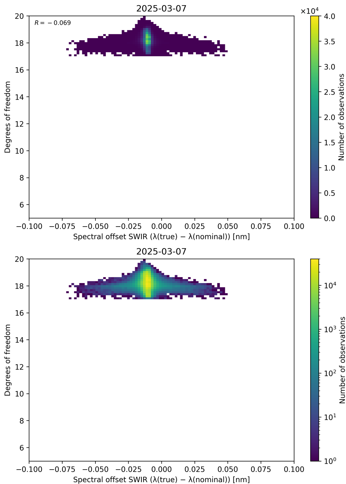
Figure 119: Scatter density plot of “Spectral offset SWIR ( \lambda_{\text{true}} - \lambda_{\text{nominal}} )” against “Degrees of freedom” for 2025-03-07 to 2025-03-08.
