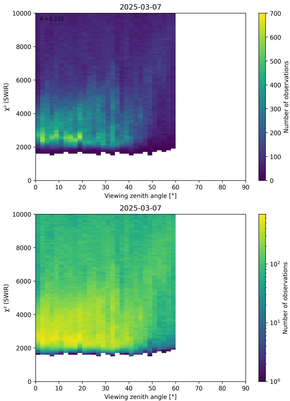
Figure 106: Scatter density plot of “Viewing zenith angle” against “ \chi^2 (SWIR)” for 2025-03-07 to 2025-03-08.
