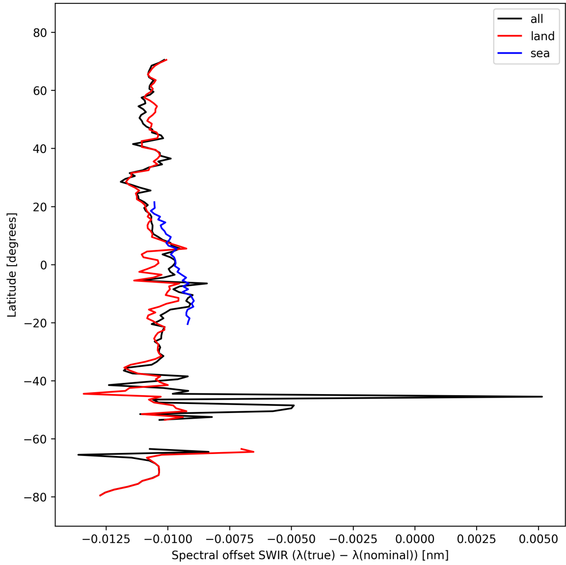
Figure 16: Zonal average of “Spectral offset SWIR ( \lambda_{\text{true}} - \lambda_{\text{nominal}} )” for 2025-03-07 to 2025-03-08.
