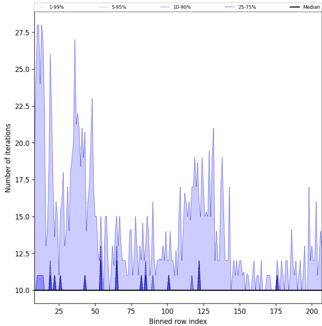
Figure 42: Along track statistics of “Number of iterations” for 2025-03-07 to 2025-03-08
