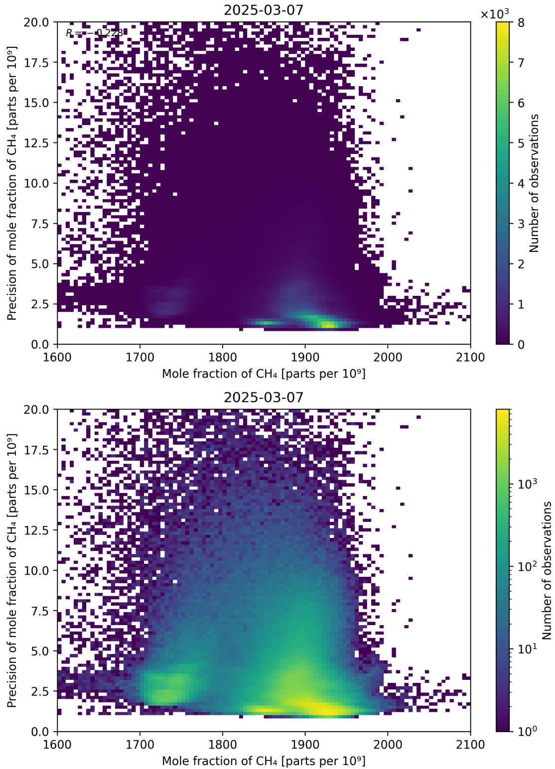
Figure 75: Scatter density plot of “Mole fraction of CH 4 ” against “Precision of mole fraction of CH 4 ” for 2025-03-07 to 2025-03-08.
