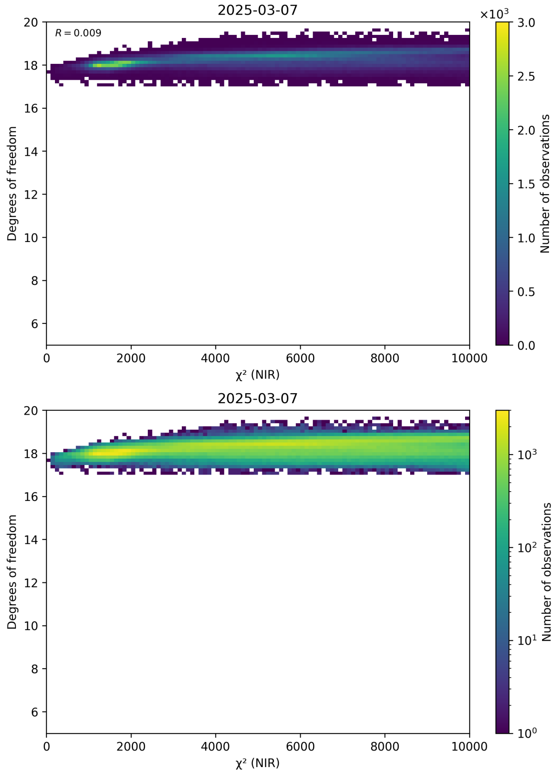
Figure 44: Scatter density plot of “ \chi^2 (NIR)” against “Degrees of freedom” for 2025-03-07 to 2025-03-08.
