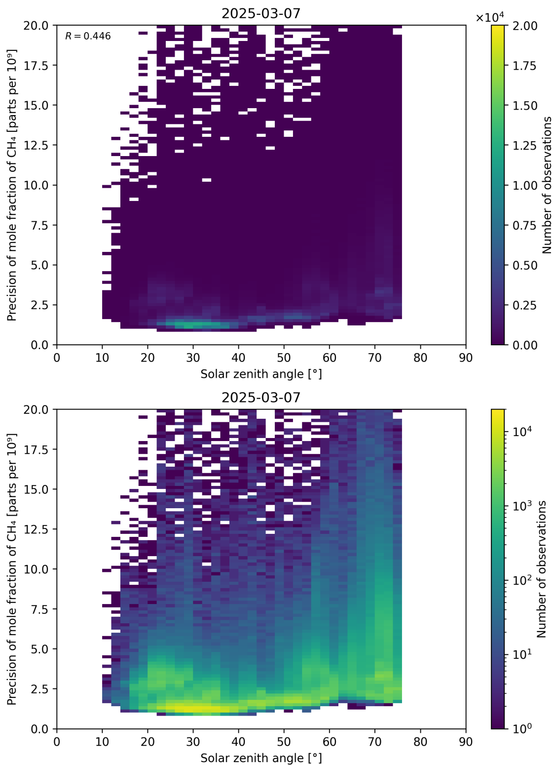
Figure 101: Scatter density plot of “Solar zenith angle” against “Precision of mole fraction of CH 4 ” for 2025-03-07 to 2025-03-08.
