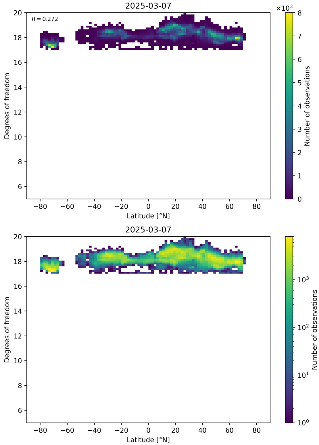
Figure 55: Scatter density plot of “Latitude” against “Degrees of freedom” for 2025-03-07 to 2025-03-08.
