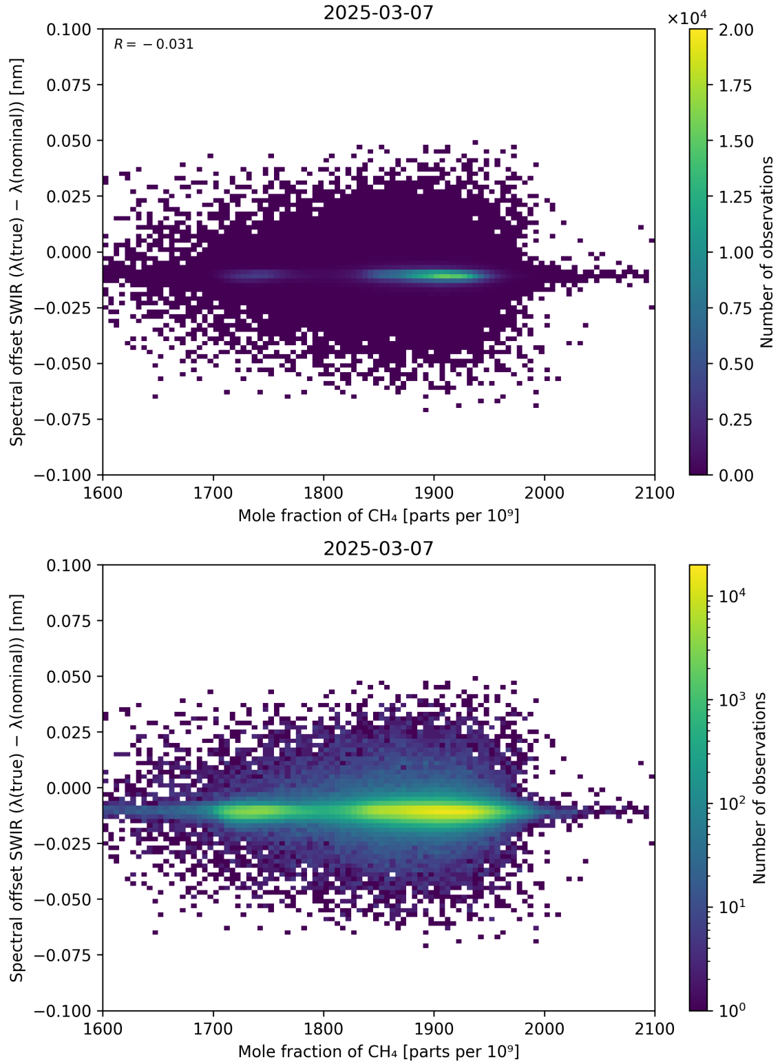
Figure 86: Scatter density plot of “Mole fraction of CH 4 ” against “Spectral offset SWIR ( \lambda_{\text{true}} - \lambda_{\text{nominal}} )” for 2025-03-07 to 2025-03-08.
