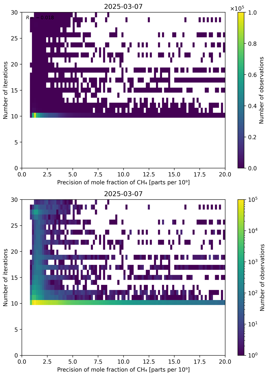
Figure 83: Scatter density plot of “Precision of mole fraction of CH 4 ” against “Number of iterations” for 2025-03-07 to 2025-03-08.
