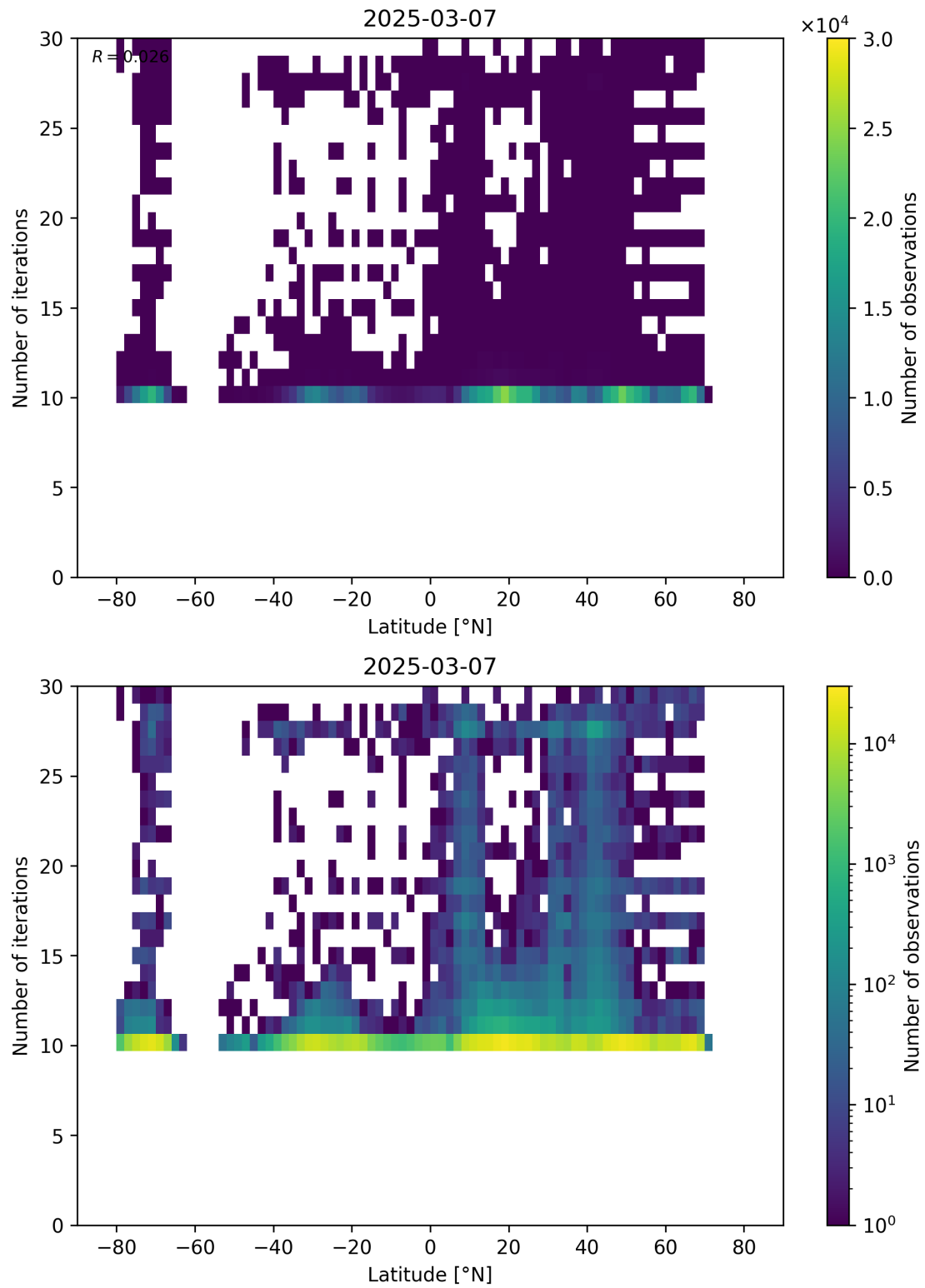
Figure 60: Scatter density plot of “Latitude” against “Number of iterations” for 2025-03-07 to 2025-03-08.
