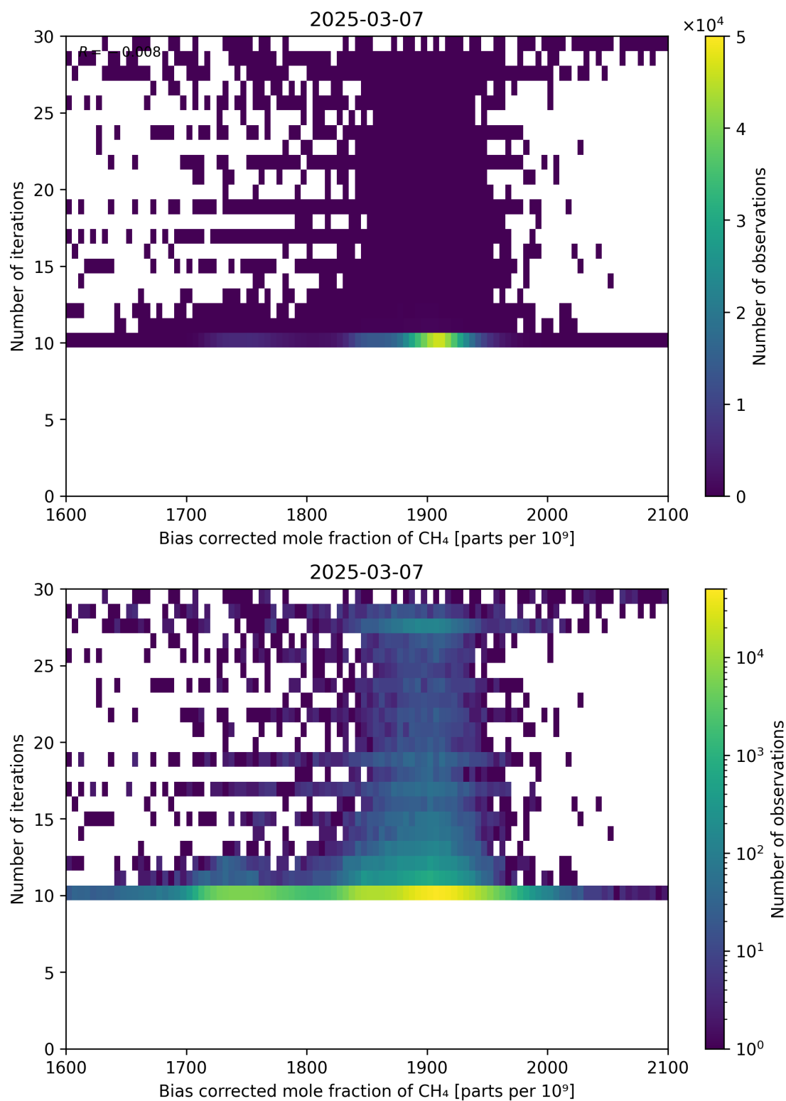
Figure 67: Scatter density plot of “Bias corrected mole fraction of CH 4 ” against “Number of iterations” for 2025-03-07 to 2025-03-08.
