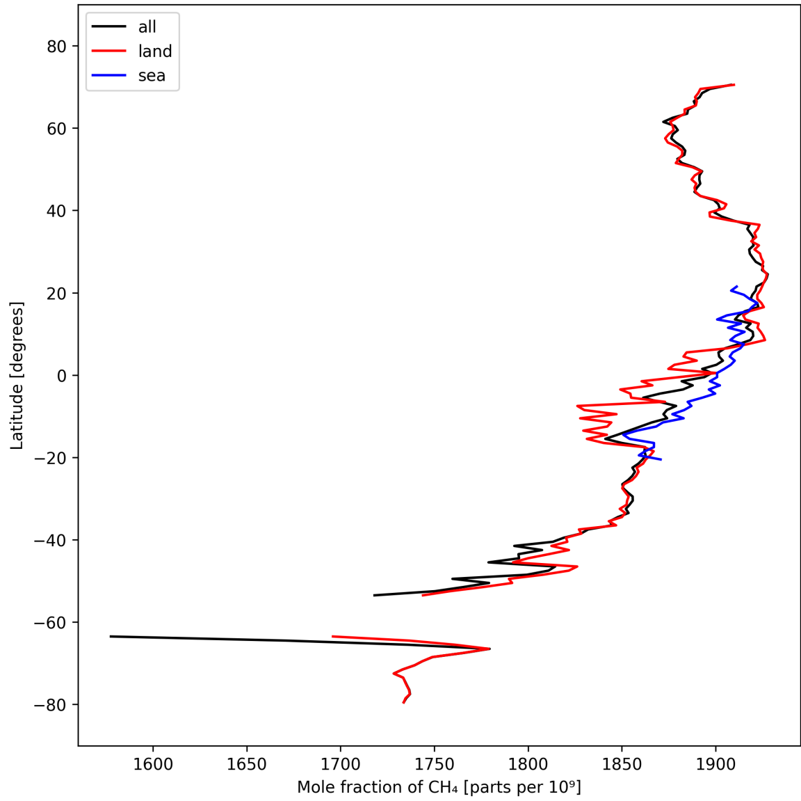
Figure 12: Zonal average of “Mole fraction of \text{CH}_4 ” for 2025-03-07 to 2025-03-08.
