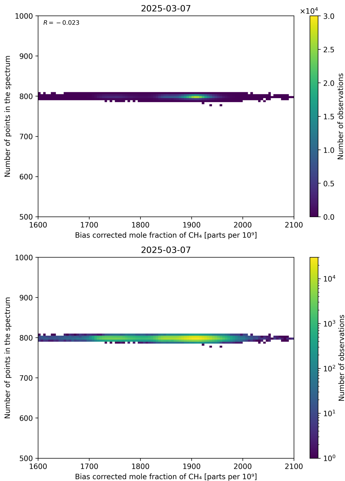
Figure 68: Scatter density plot of “Bias corrected mole fraction of CH 4 ” against “Number of points in the spectrum” for 2025-03-07 to 2025-03-08.
