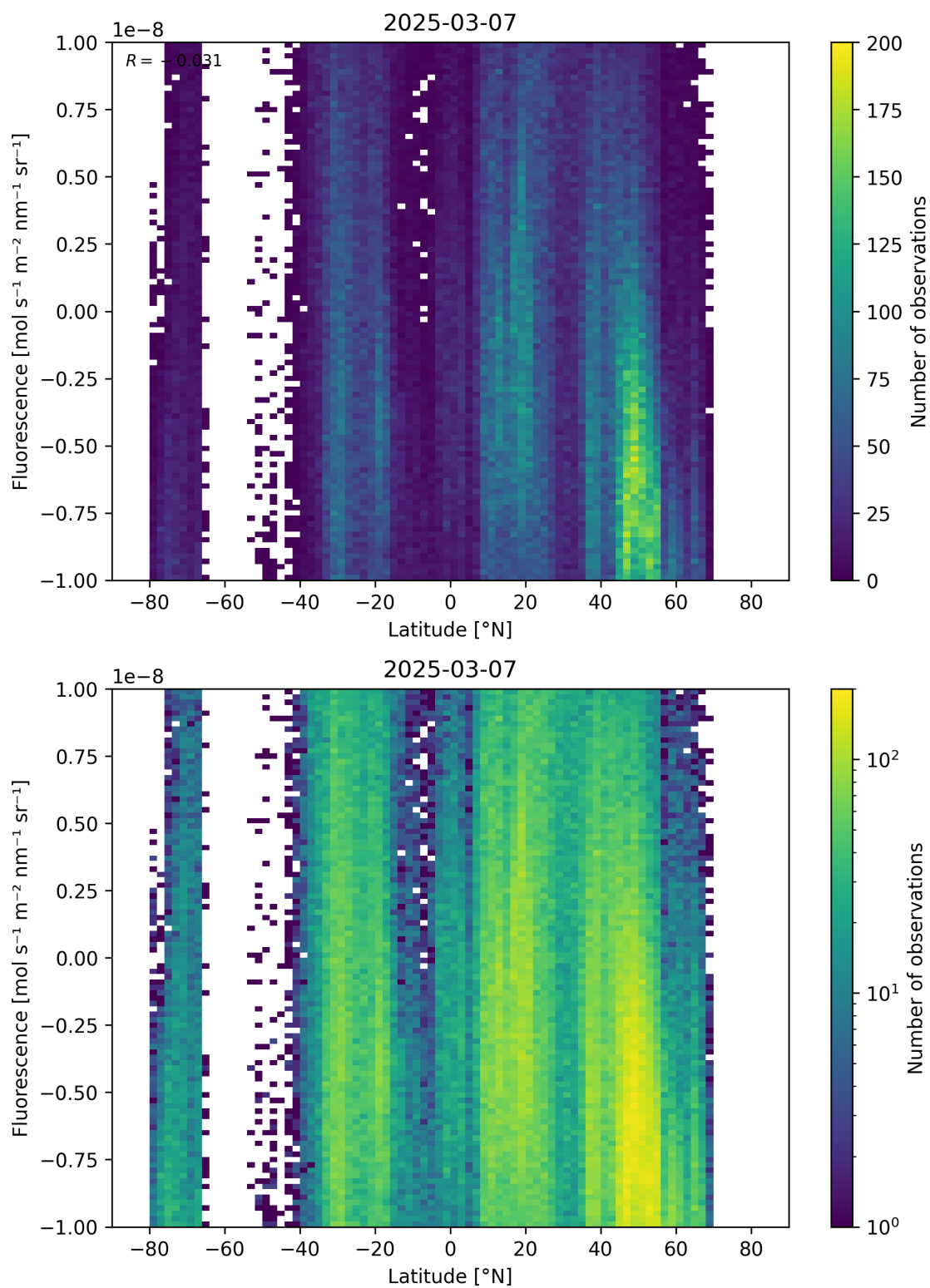
Figure 56: Scatter density plot of “Latitude” against “Fluorescence” for 2025-03-07 to 2025-03-08.
