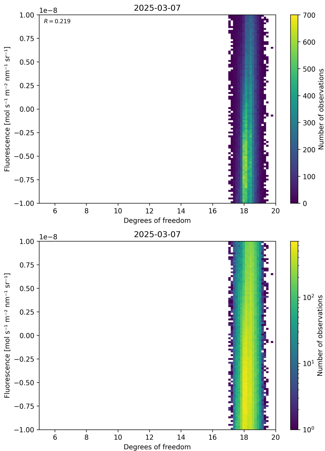
Figure 51: Scatter density plot of “Degrees of freedom” against “Fluorescence” for 2025-03-07 to 2025-03-08.
