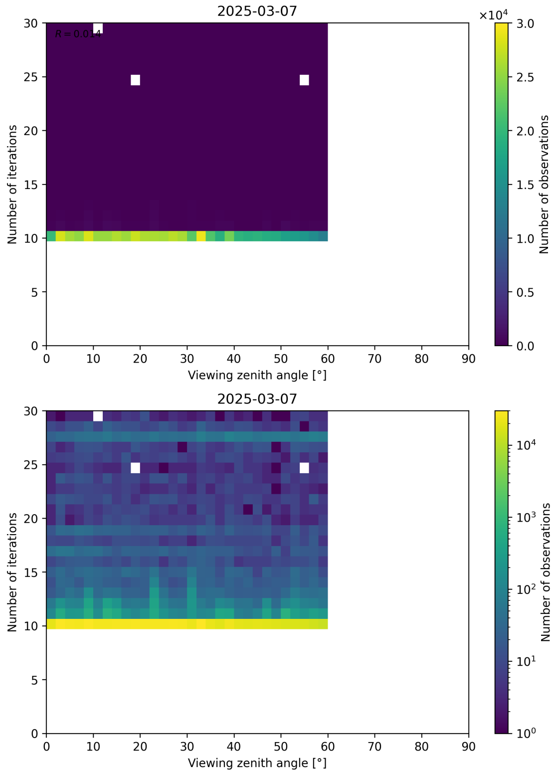
Figure 113: Scatter density plot of “Viewing zenith angle” against “Number of iterations” for 2025-03-07 to 2025-03-08.
