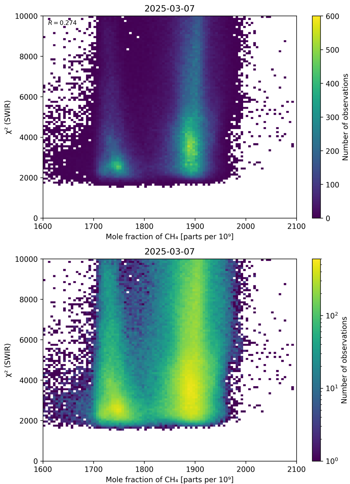
Figure 71: Scatter density plot of “Mole fraction of \text{CH}_4 ” against “ \chi^2 (SWIR)” for 2025-03-07 to 2025-03-08.
