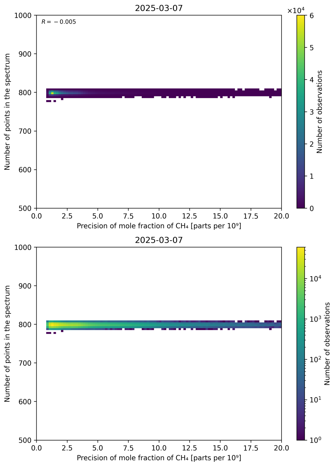
Figure 84: Scatter density plot of “Precision of mole fraction of CH 4 ” against “Number of points in the spectrum” for 2025-03-07 to 2025-03-08.
