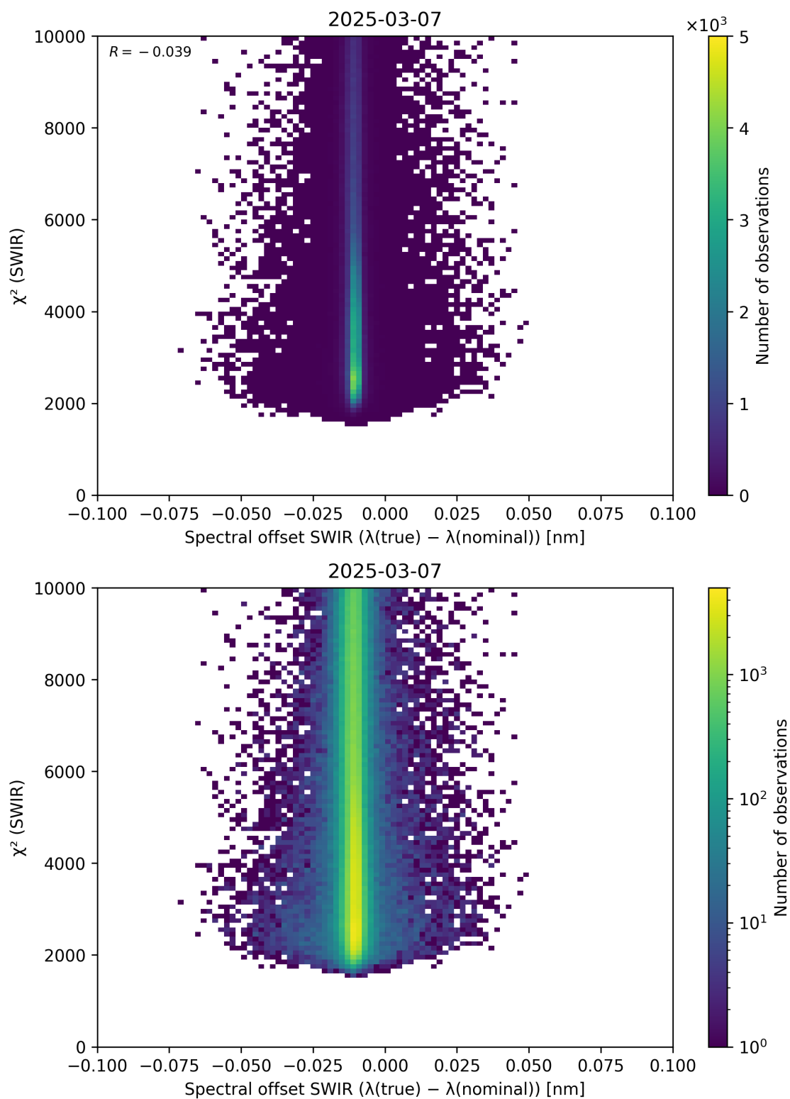
Figure 118: Scatter density plot of “Spectral offset SWIR ( \lambda_{\text{true}} - \lambda_{\text{nominal}} )” against “ \chi^2 (SWIR)” for 2025-03-07 to 2025-03-08.
