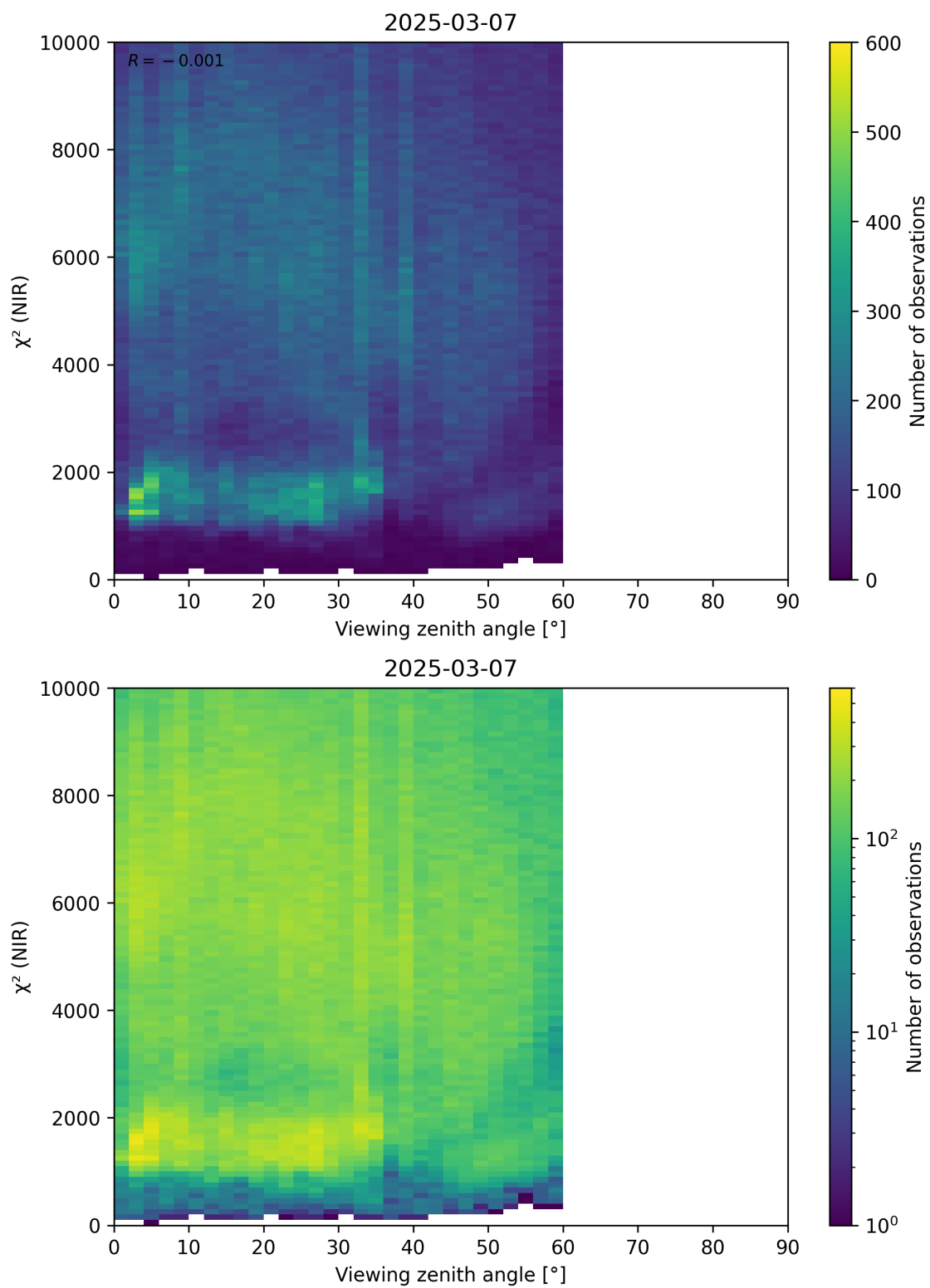
Figure 105: Scatter density plot of “Viewing zenith angle” against “ \chi^2 (NIR)” for 2025-03-07 to 2025-03-08.
