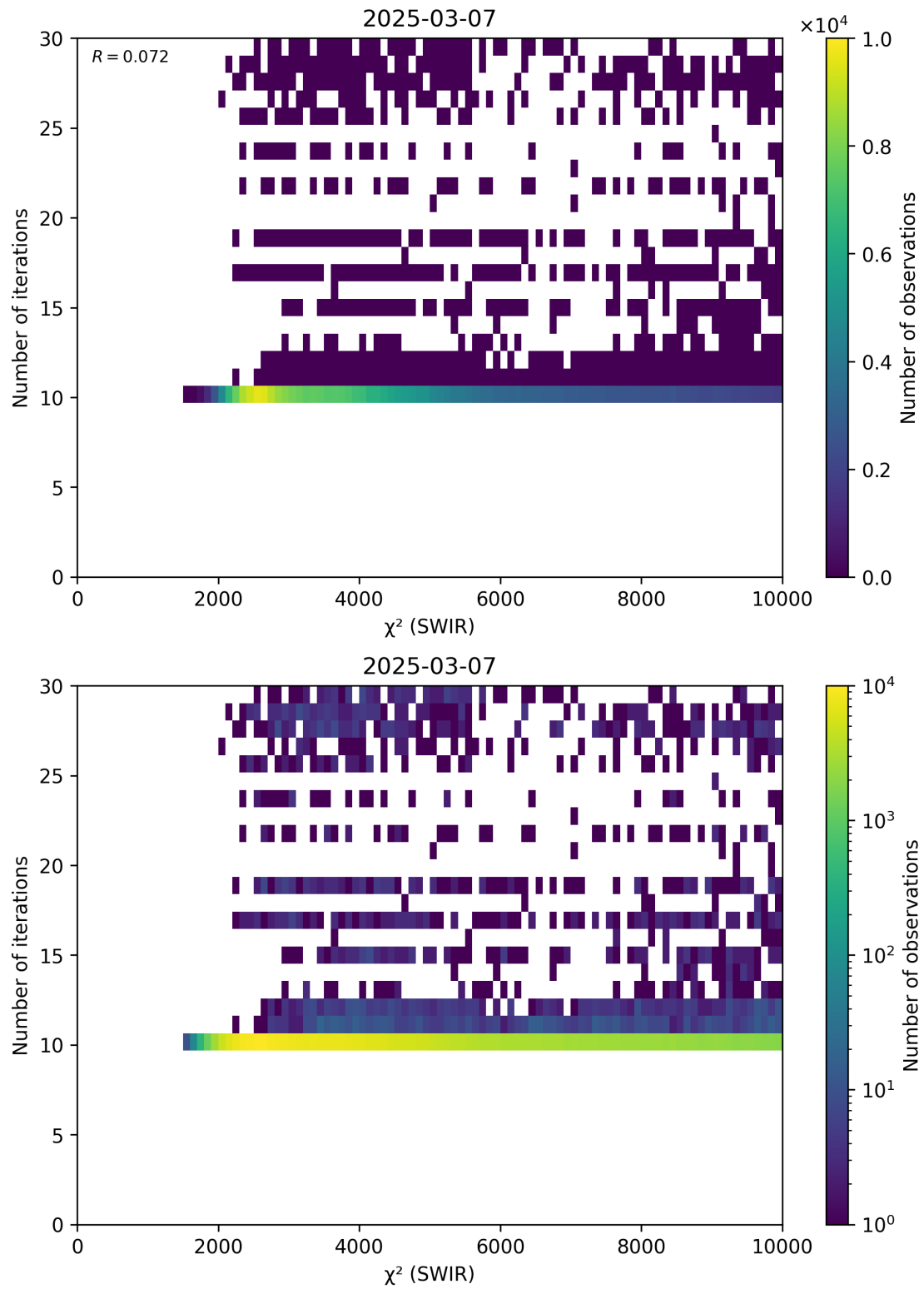
Figure 50: Scatter density plot of “ \chi^2 (SWIR)” against “Number of iterations” for 2025-03-07 to 2025-03-08.
