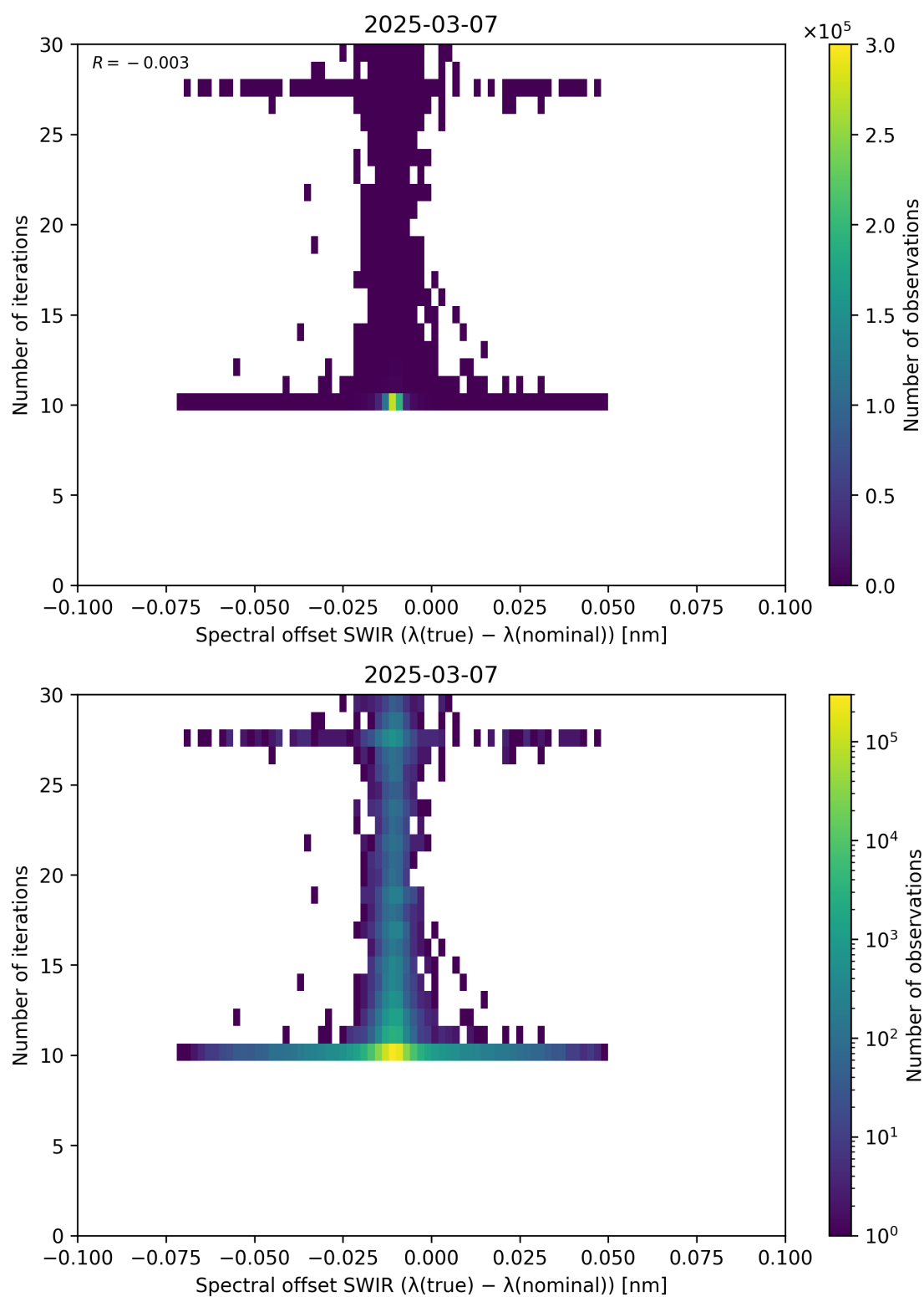
Figure 121: Scatter density plot of “Spectral offset SWIR ( \lambda_{\text{true}} - \lambda_{\text{nominal}} )” against “Number of iterations” for 2025-03-07 to 2025-03-08.
