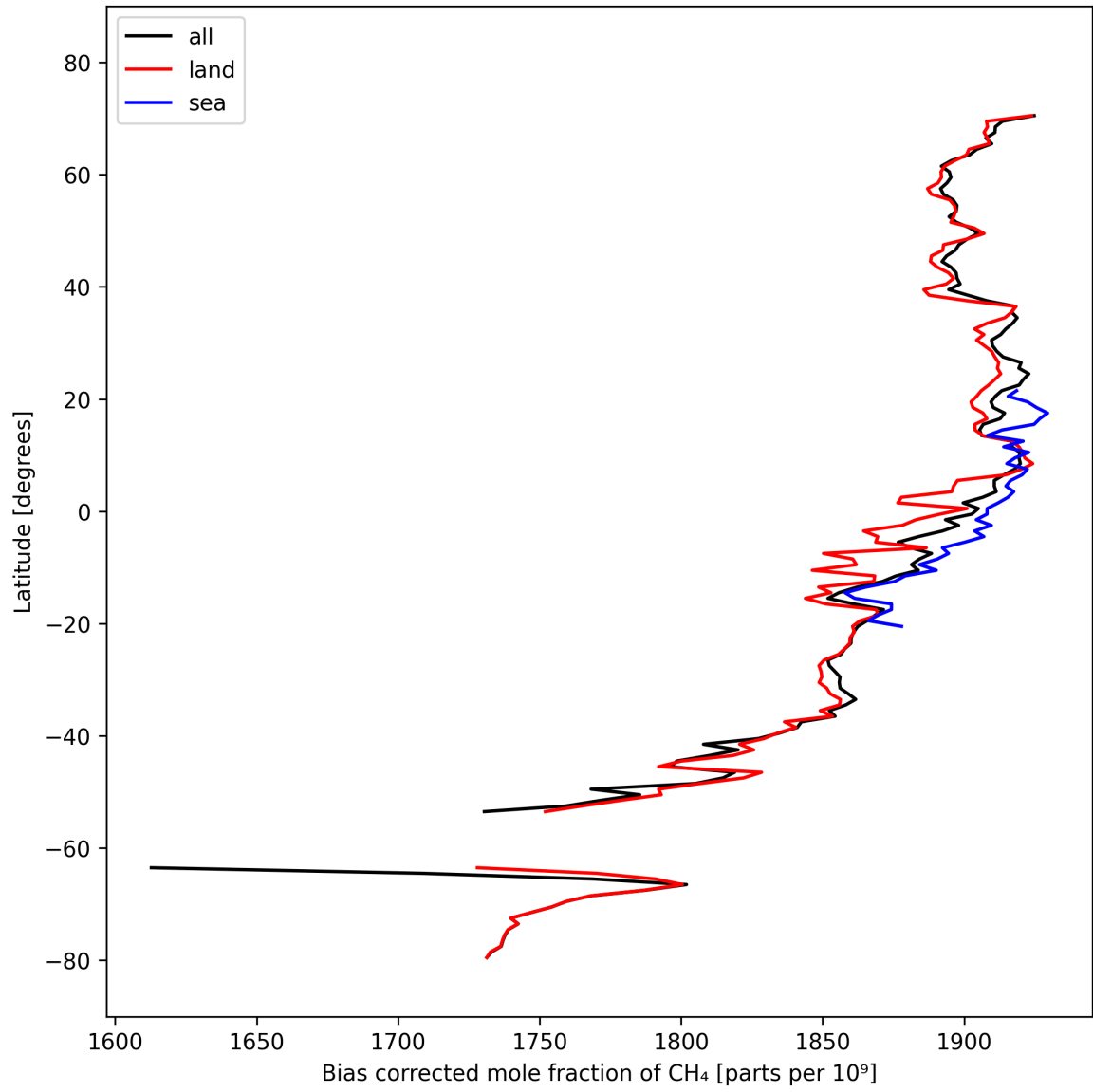
Figure 14: Zonal average of “Bias corrected mole fraction of \text{CH}_4 ” for 2025-03-07 to 2025-03-08.
