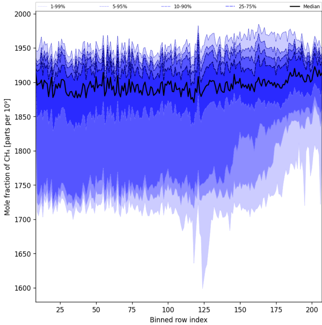
Figure 34: Along track statistics of “Mole fraction of CH 4 ” for 2025-03-07 to 2025-03-08
