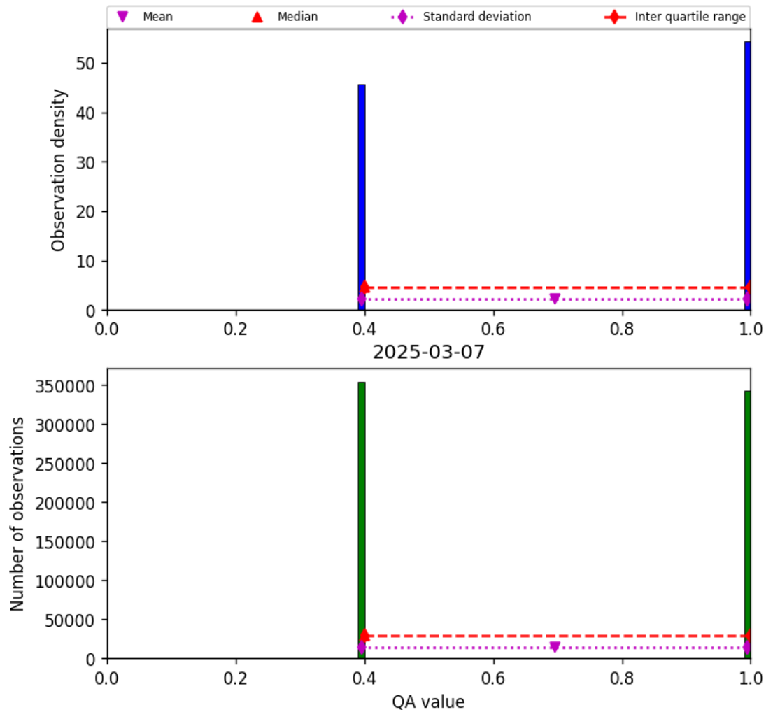
Figure 22: Histogram of “QA value” for 2025-03-07 to 2025-03-08
