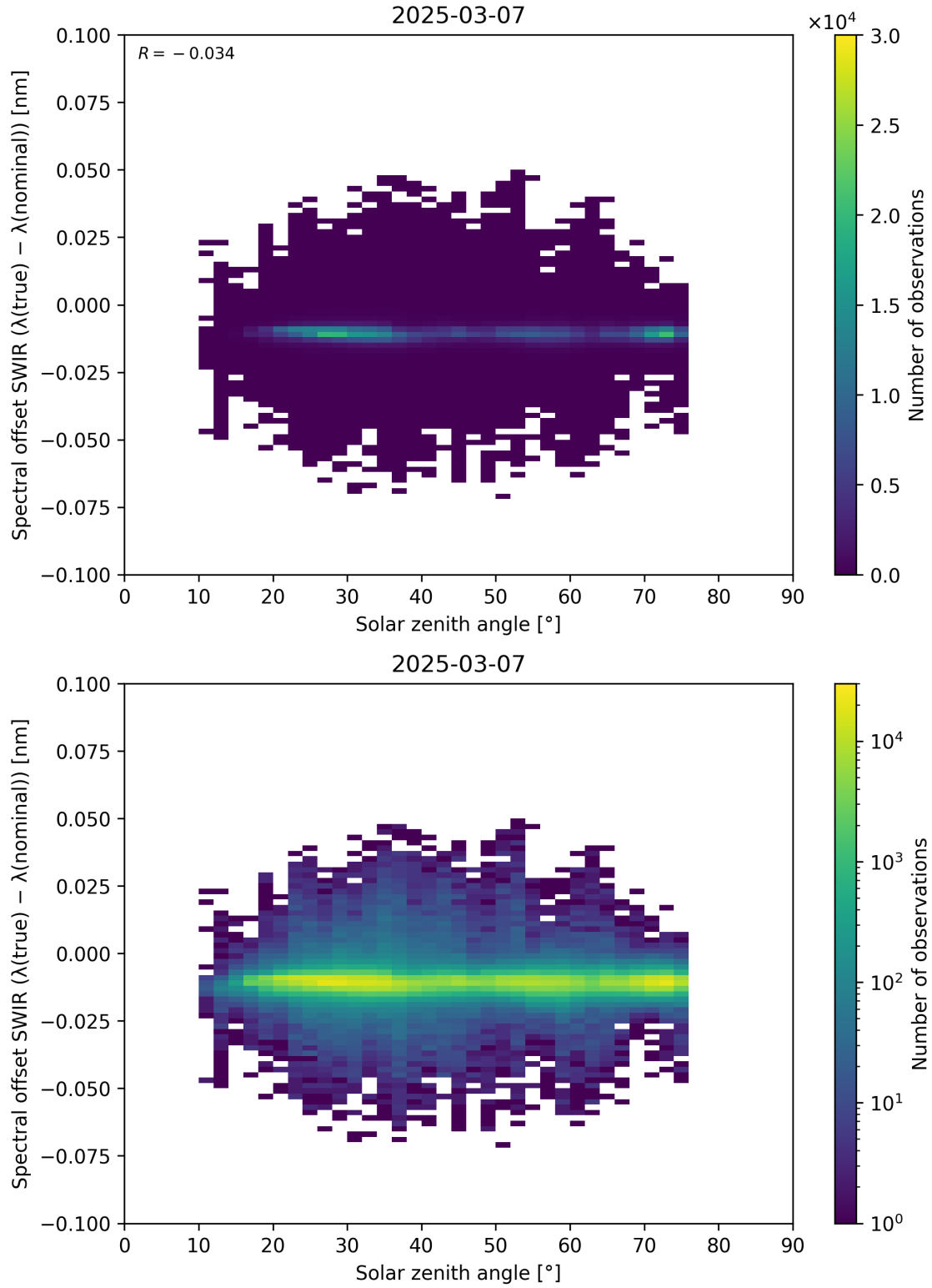
Figure 104: Scatter density plot of “Solar zenith angle” against “Spectral offset SWIR ( \lambda_{\text{true}} - \lambda_{\text{nominal}} )” for 2025-03-07 to 2025-03-08.
