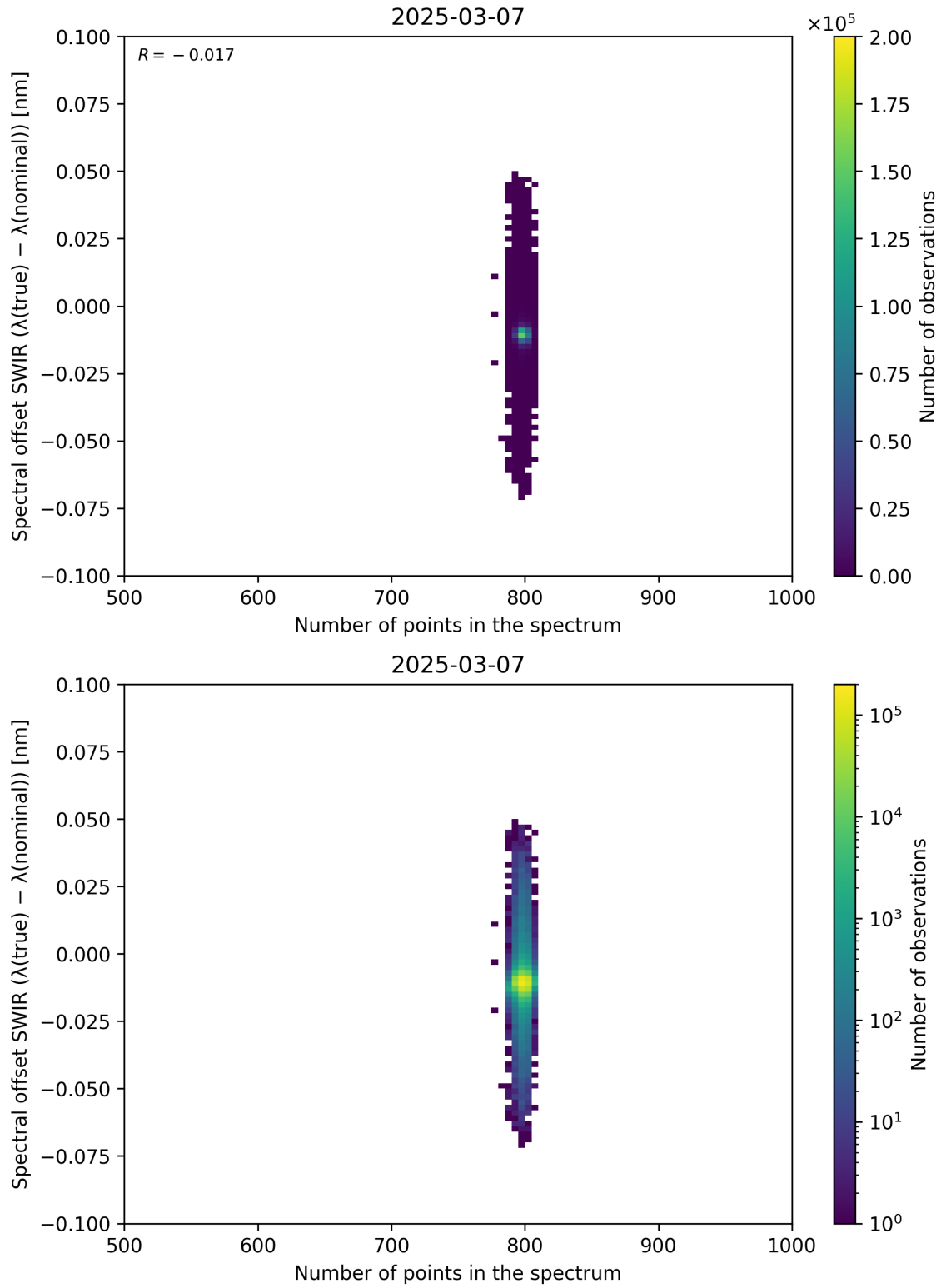
Figure 93: Scatter density plot of “Number of points in the spectrum” against “Spectral offset SWIR ( \lambda_{\text{true}} - \lambda_{\text{nominal}} )” for 2025-03-07 to 2025-03-08.
