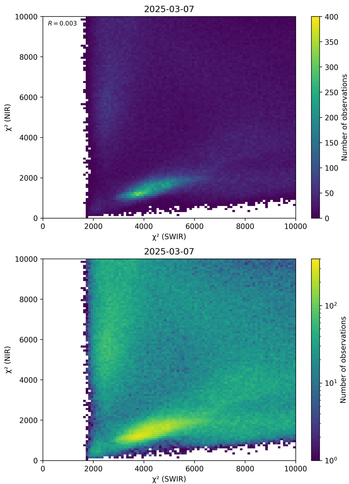
Figure 47: Scatter density plot of “ \chi^2 (SWIR)” against “ \chi^2 (NIR)” for 2025-03-07 to 2025-03-08.
