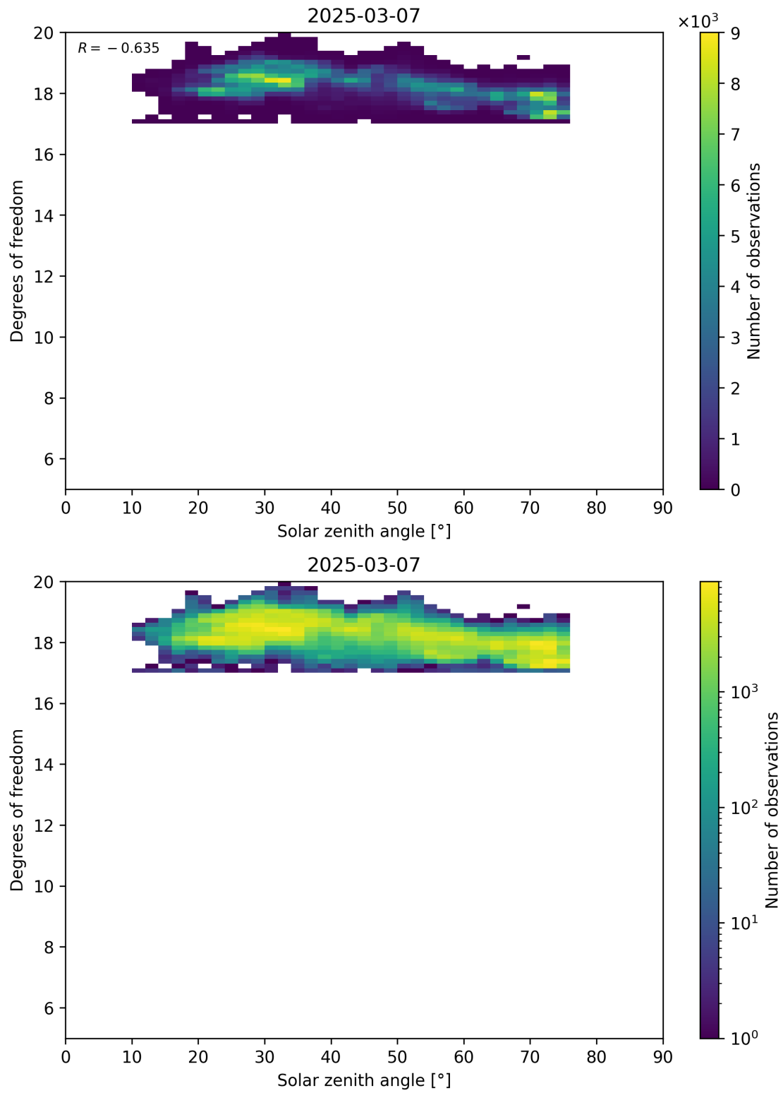
Figure 96: Scatter density plot of “Solar zenith angle” against “Degrees of freedom” for 2025-03-07 to 2025-03-08.
