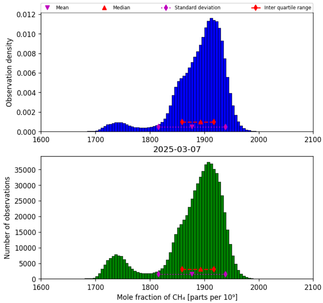
Figure 23: Histogram of “Mole fraction of CH 4 ” for 2025-03-07 to 2025-03-08
