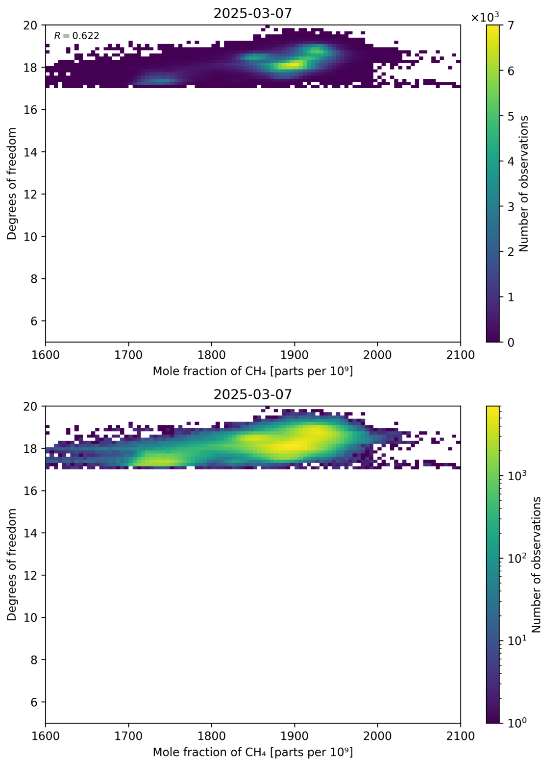
Figure 72: Scatter density plot of “Mole fraction of CH 4 ” against “Degrees of freedom” for 2025-03-07 to 2025-03-08.
