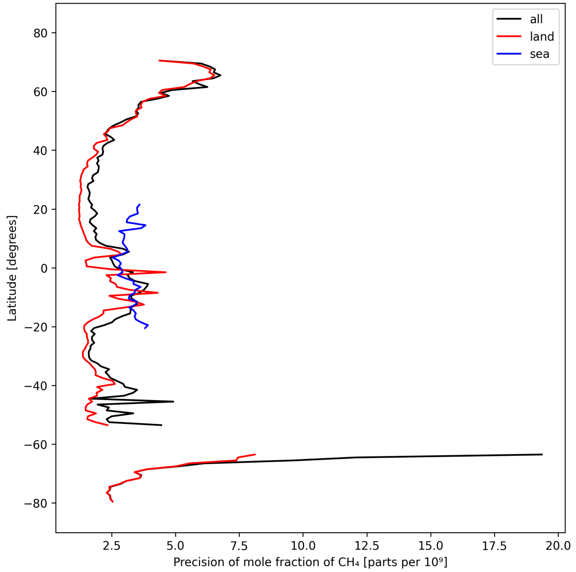
Figure 13: Zonal average of “Precision of mole fraction of CH 4 ” for 2025-03-07 to 2025-03-08.
