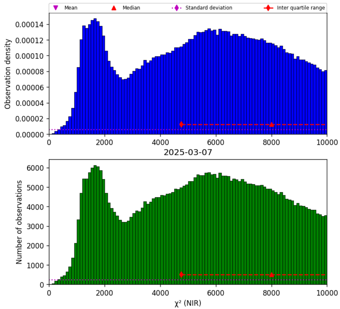
Figure 29: Histogram of “ \chi^2 (NIR)” for 2025-03-07 to 2025-03-08
