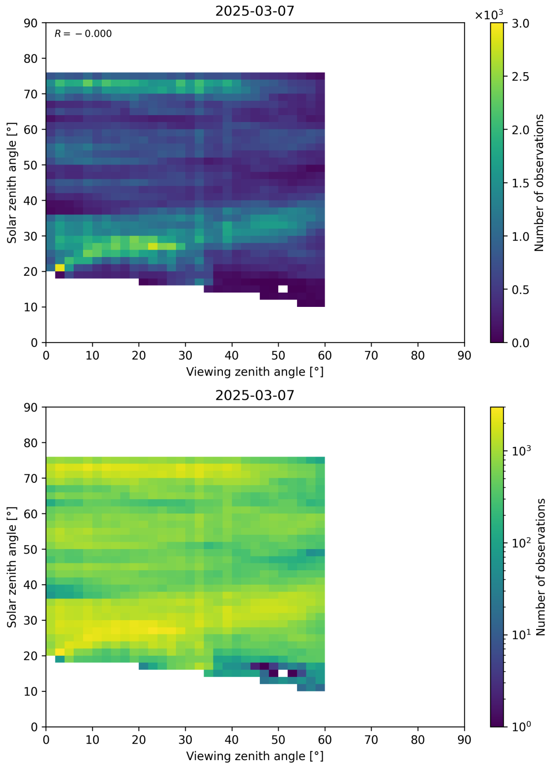
Figure 115: Scatter density plot of “Viewing zenith angle” against “Solar zenith angle” for 2025-03-07 to 2025-03-08.
