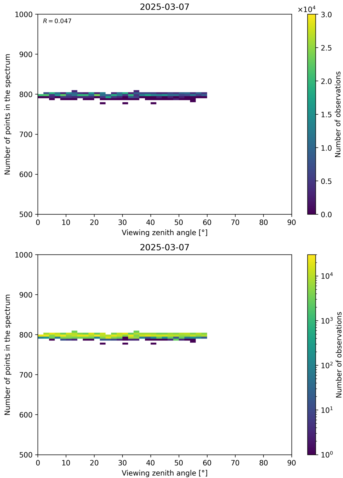
Figure 114: Scatter density plot of “Viewing zenith angle” against “Number of points in the spectrum” for 2025-03-07 to 2025-03-08.
