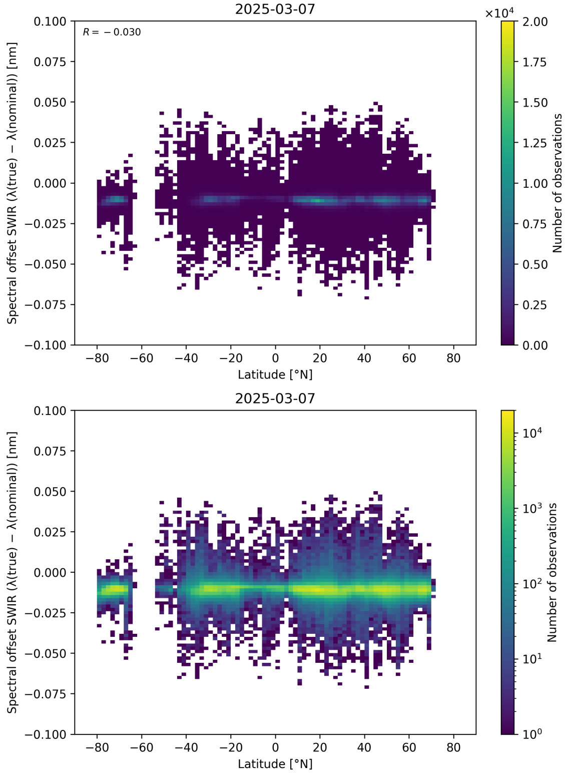
Figure 62: Scatter density plot of “Latitude” against “Spectral offset SWIR ( \lambda_{\text{true}} - \lambda_{\text{nominal}} )” for 2025-03-07 to 2025-03-08.
