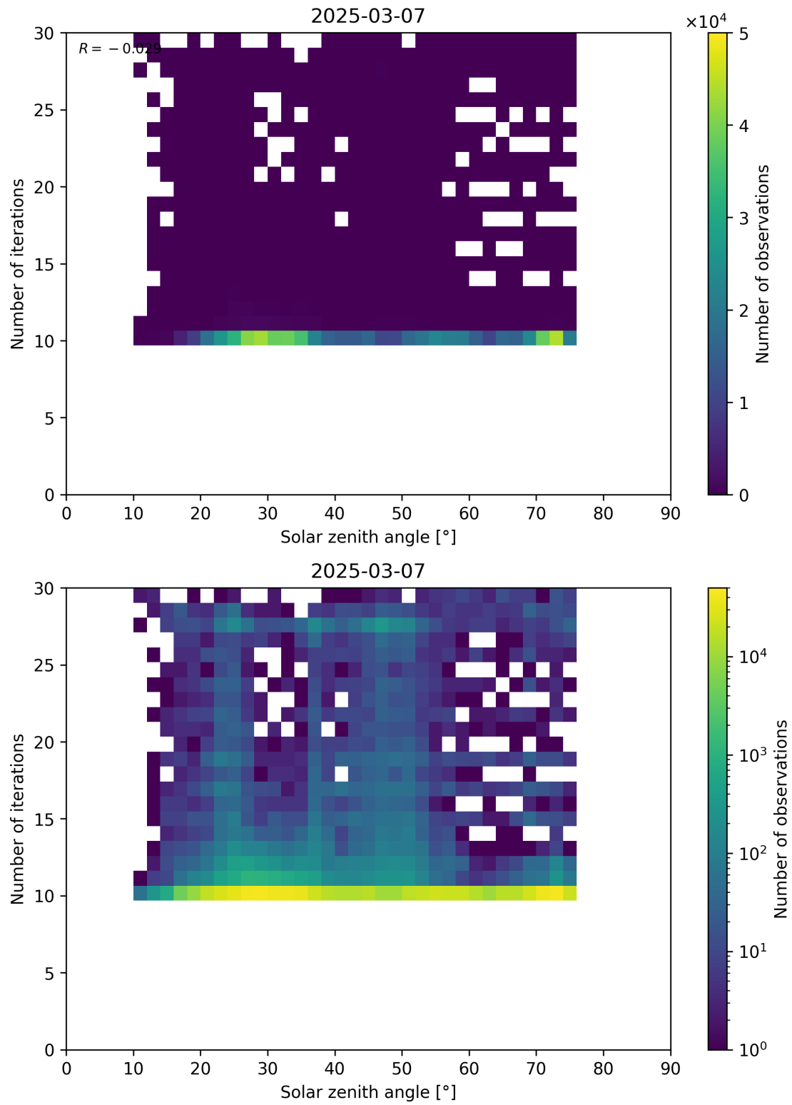
Figure 102: Scatter density plot of “Solar zenith angle” against “Number of iterations” for 2025-03-07 to 2025-03-08.
