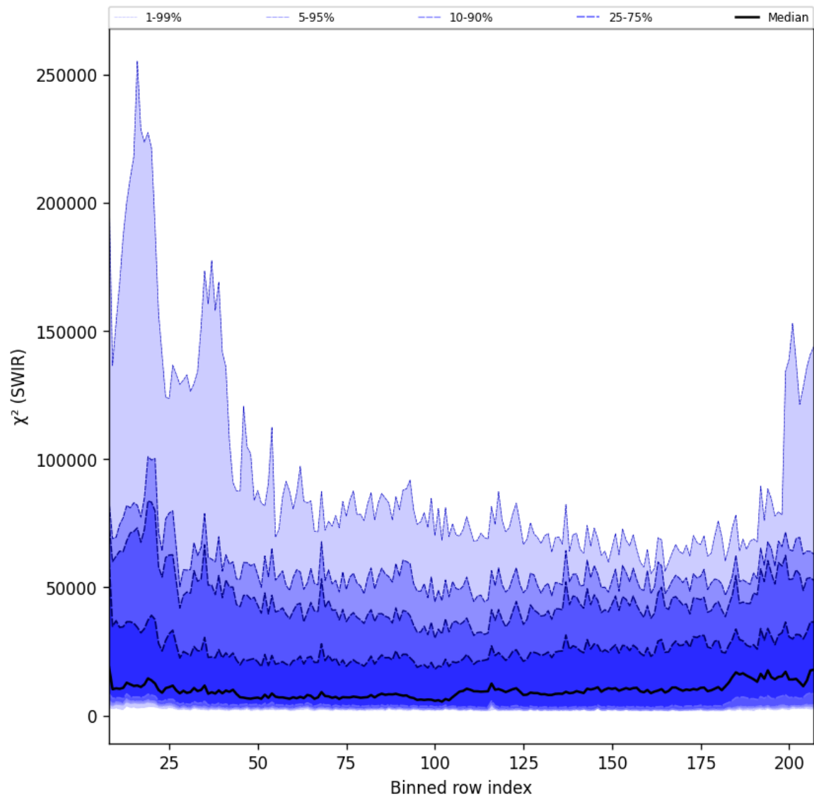
Figure 39: Along track statistics of " \chi^2 (SWIR)" for 2025-03-07 to 2025-03-08
