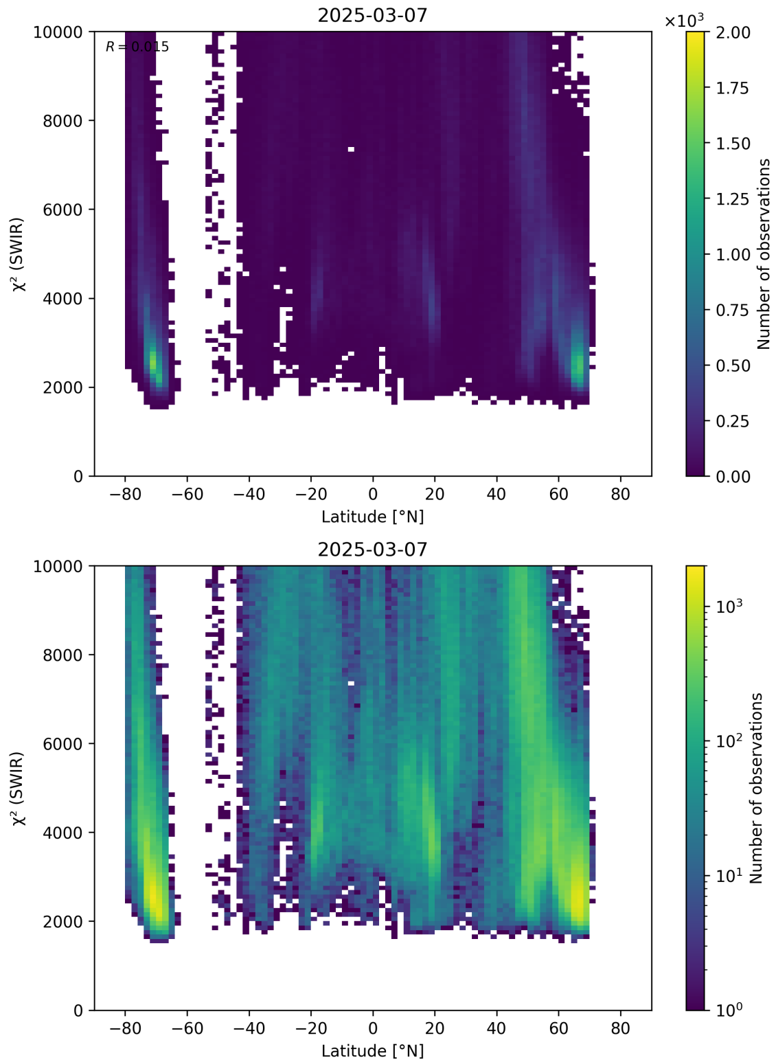
Figure 54: Scatter density plot of “Latitude” against “ \chi^2 (SWIR)” for 2025-03-07 to 2025-03-08.
