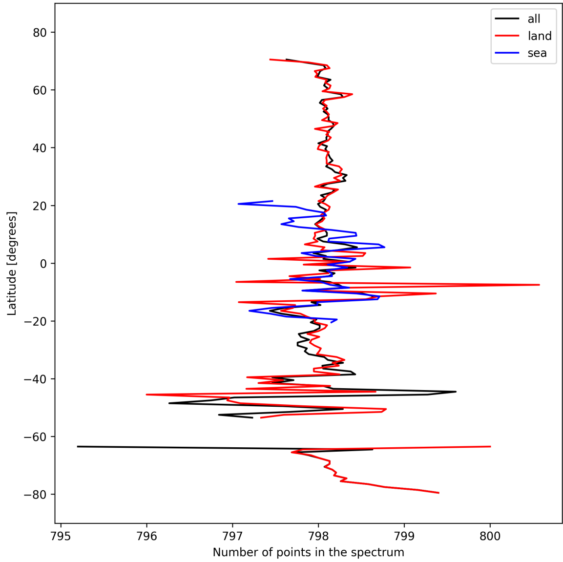
Figure 15: Zonal average of “Number of points in the spectrum” for 2025-03-07 to 2025-03-08.
