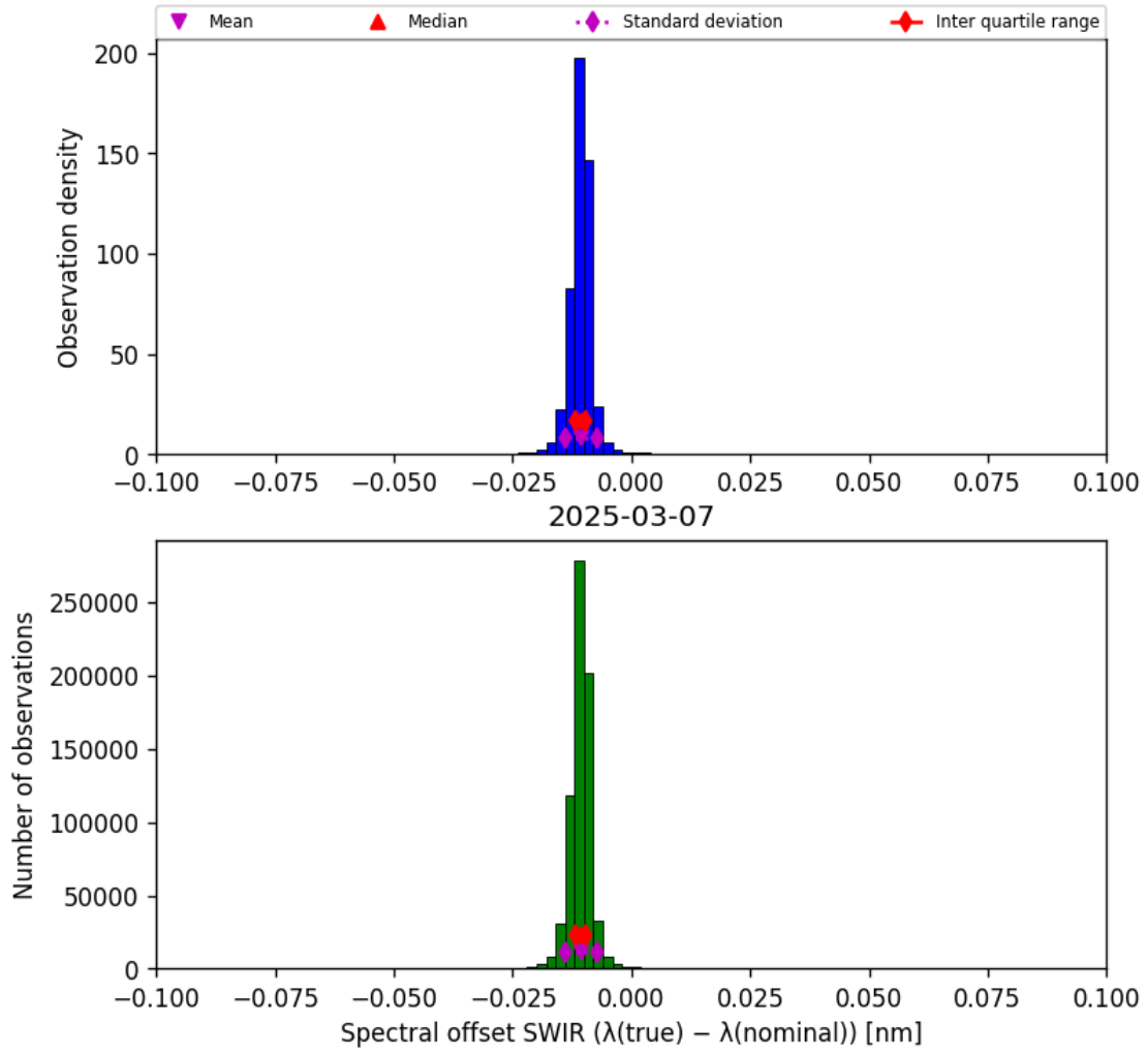
Figure 27: Histogram of “Spectral offset SWIR ( \lambda_{\text{true}} - \lambda_{\text{nominal}} )” for 2025-03-07 to 2025-03-08
