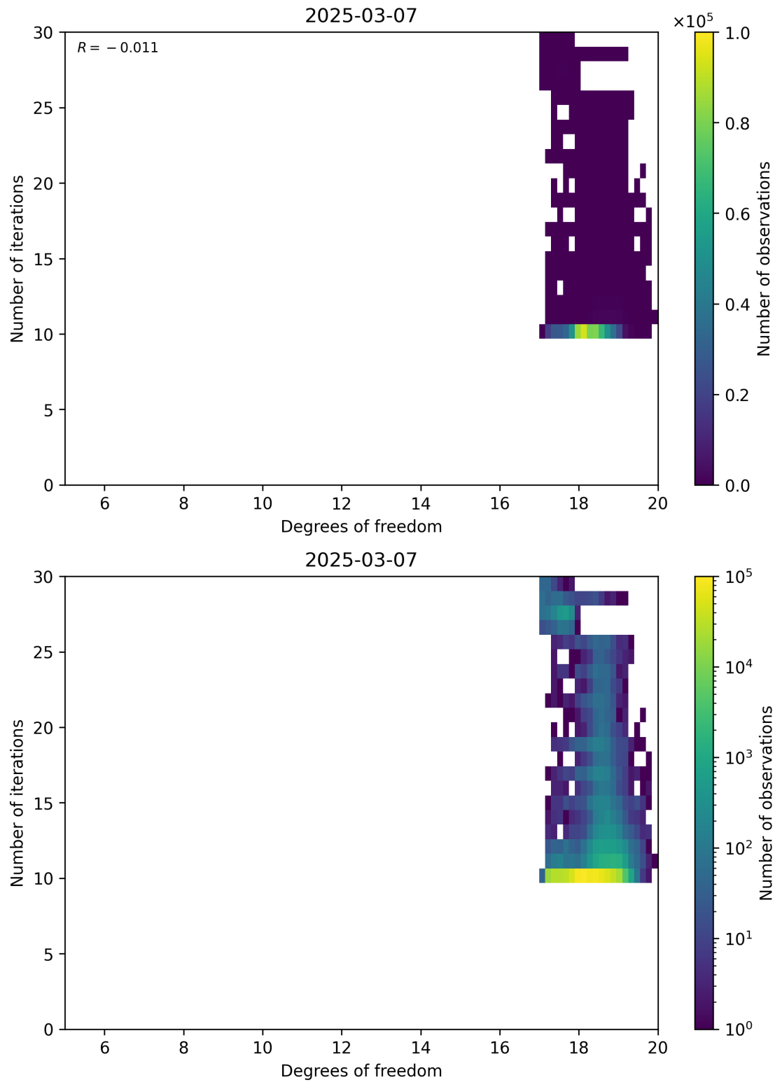
Figure 52: Scatter density plot of “Degrees of freedom” against “Number of iterations” for 2025-03-07 to 2025-03-08.
