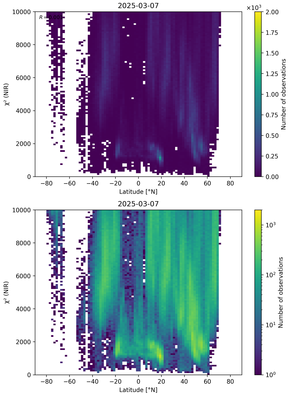
Figure 53: Scatter density plot of “Latitude” against “ \chi^2 (NIR)” for 2025-03-07 to 2025-03-08.
