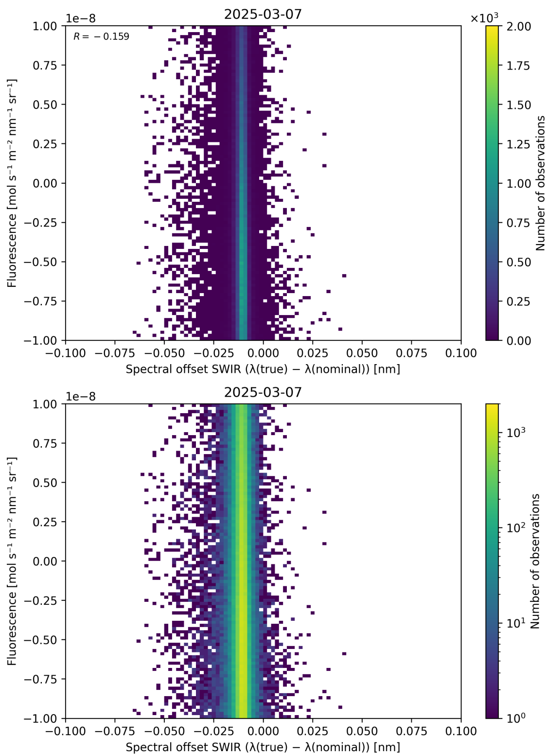
Figure 120: Scatter density plot of “Spectral offset SWIR ( \lambda_{\text{true}} - \lambda_{\text{nominal}} )” against “Fluorescence” for 2025-03-07 to 2025-03-08.
