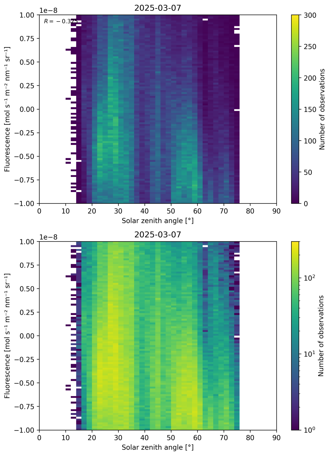
Figure 97: Scatter density plot of “Solar zenith angle” against “Fluorescence” for 2025-03-07 to 2025-03-08.
