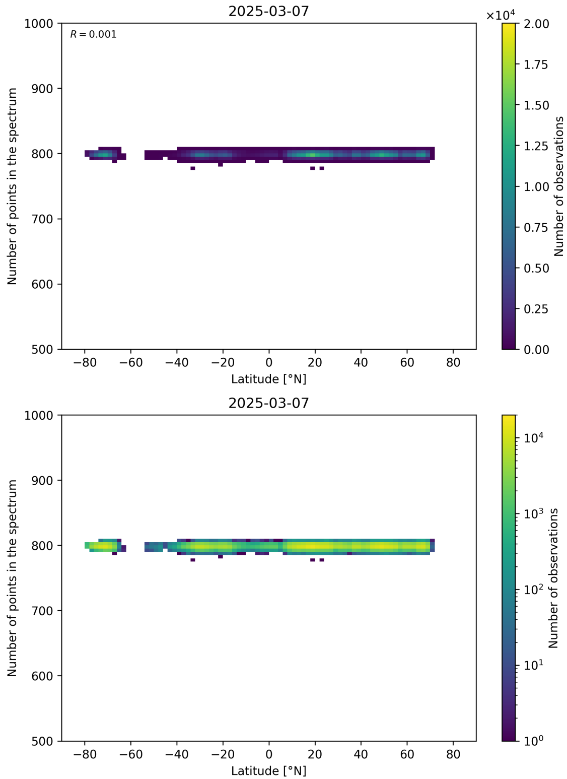
Figure 61: Scatter density plot of “Latitude” against “Number of points in the spectrum” for 2025-03-07 to 2025-03-08.
