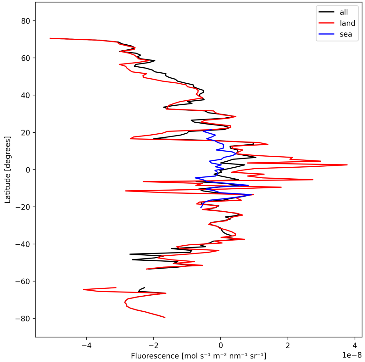
Figure 21: Zonal average of “Fluorescence” for 2025-03-07 to 2025-03-08.
