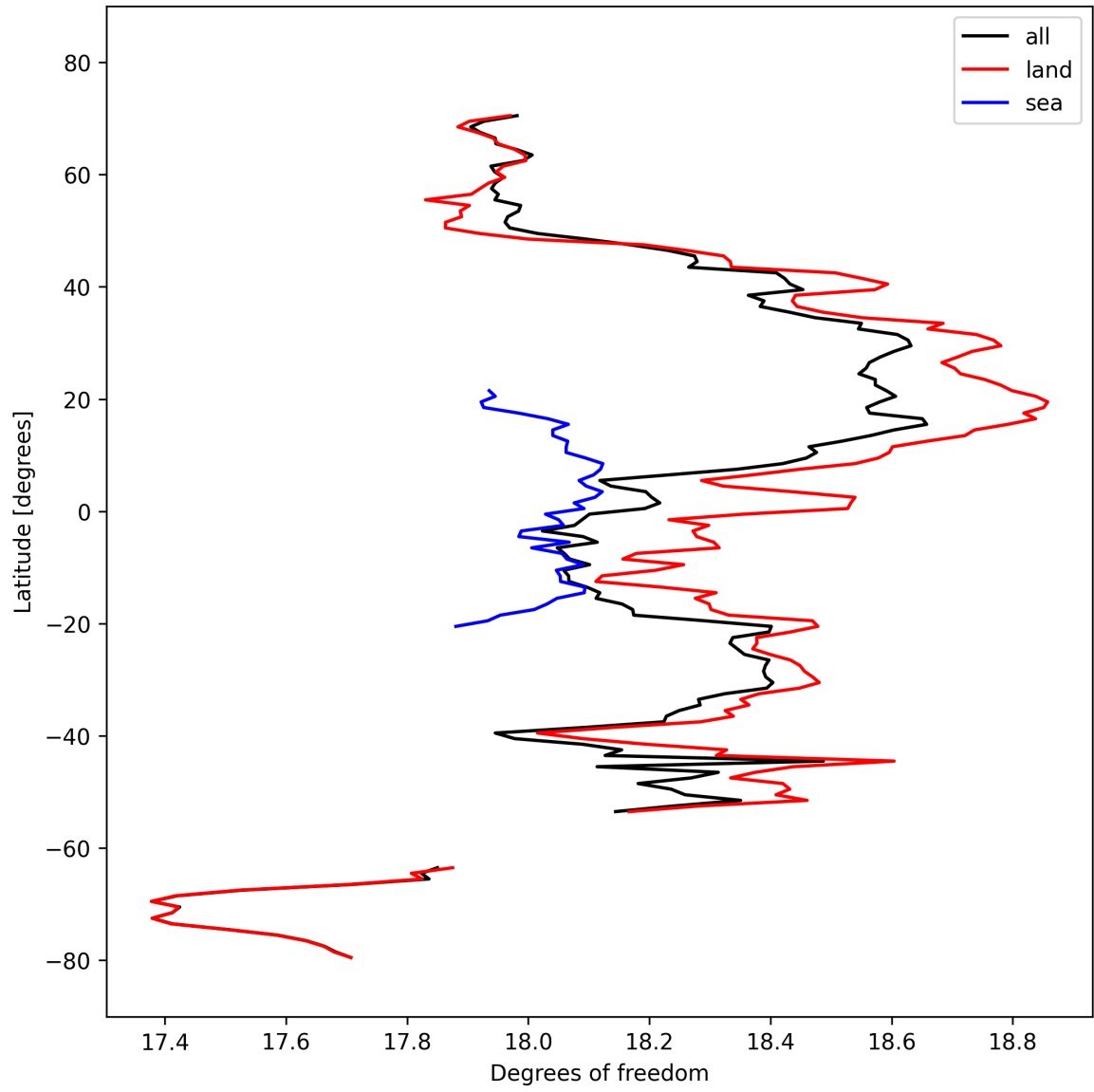
Figure 19: Zonal average of “Degrees of freedom” for 2025-03-07 to 2025-03-08.
