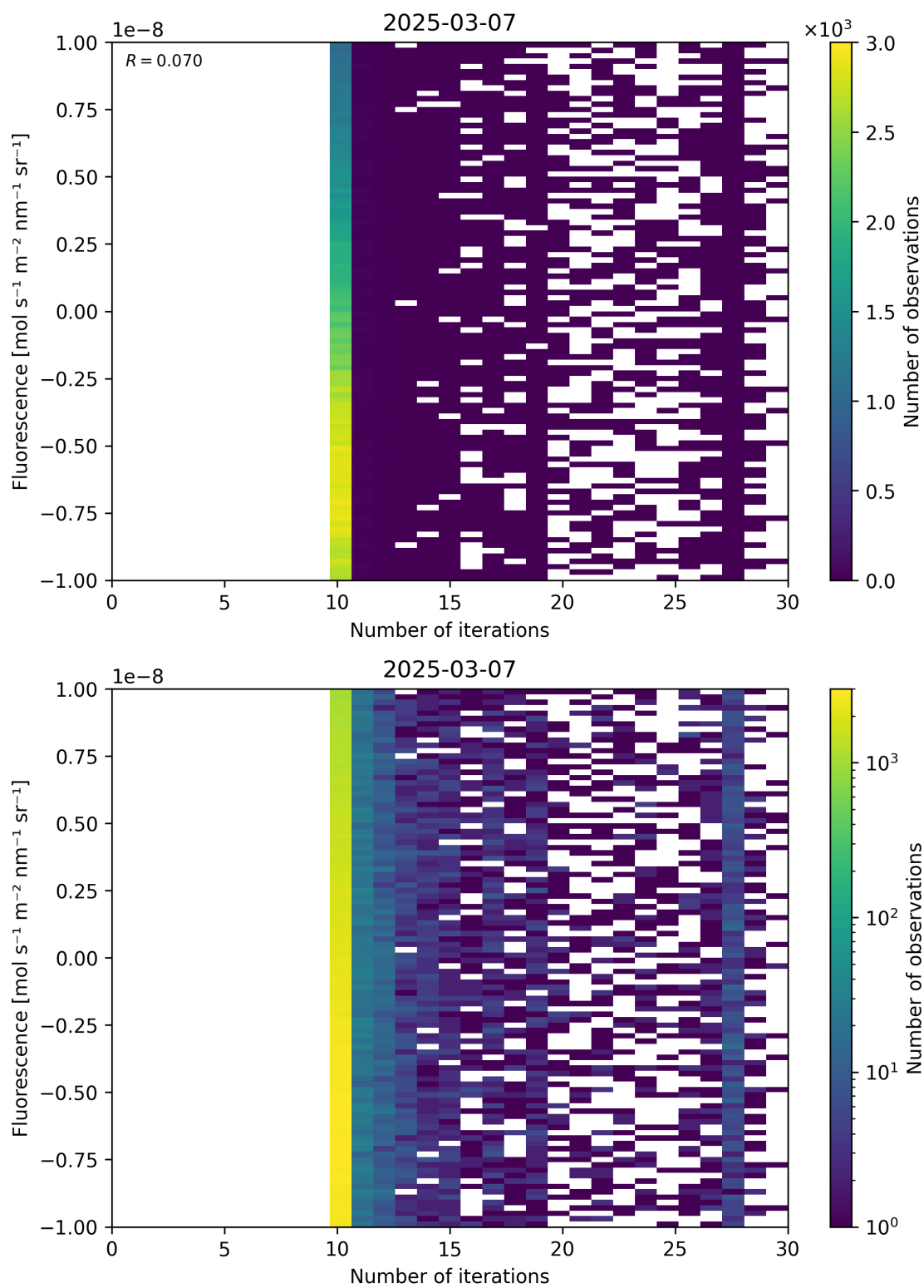
Figure 87: Scatter density plot of “Number of iterations” against “Fluorescence” for 2025-03-07 to 2025-03-08.
