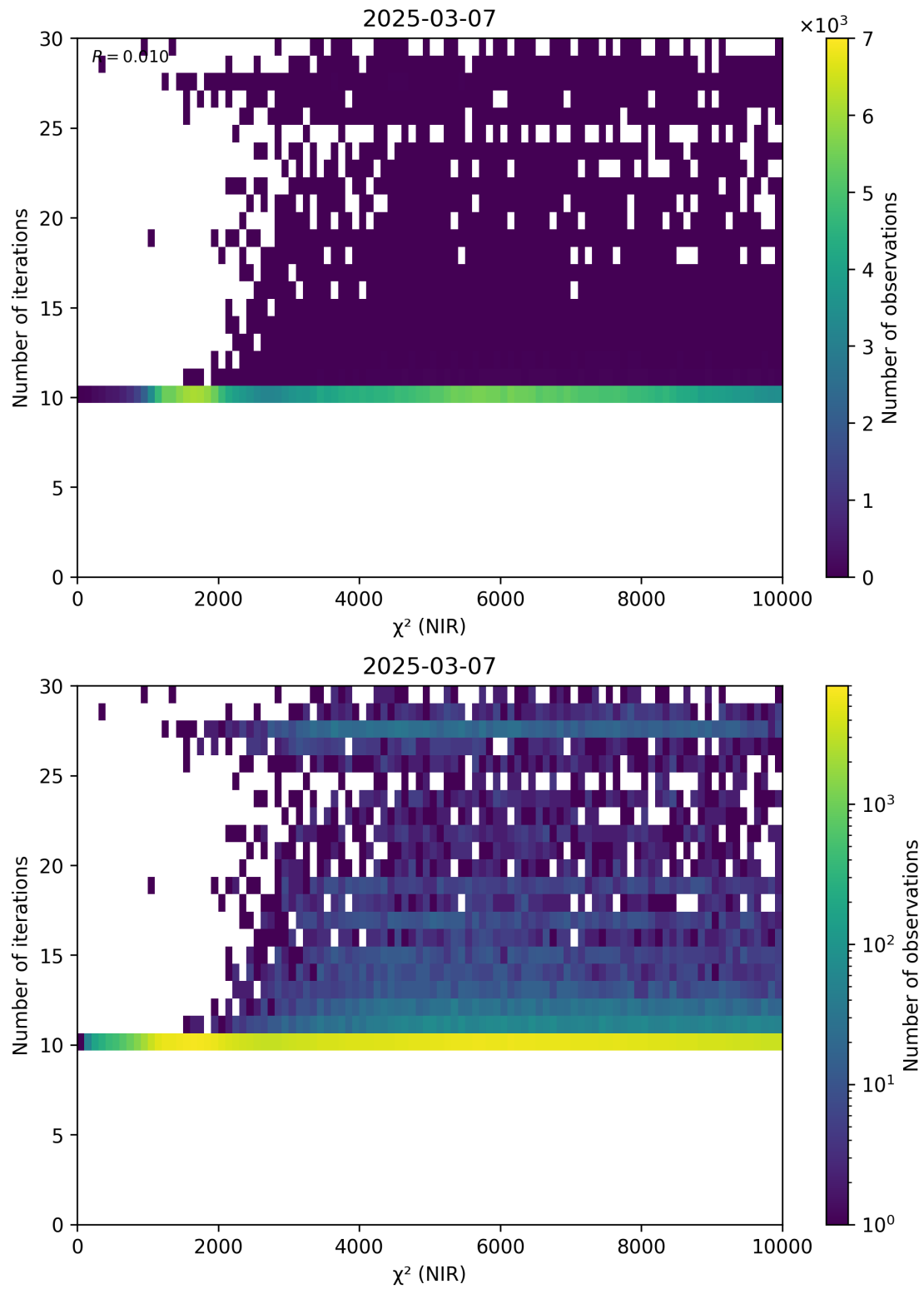
Figure 46: Scatter density plot of “ \chi^2 (NIR)” against “Number of iterations” for 2025-03-07 to 2025-03-08.
