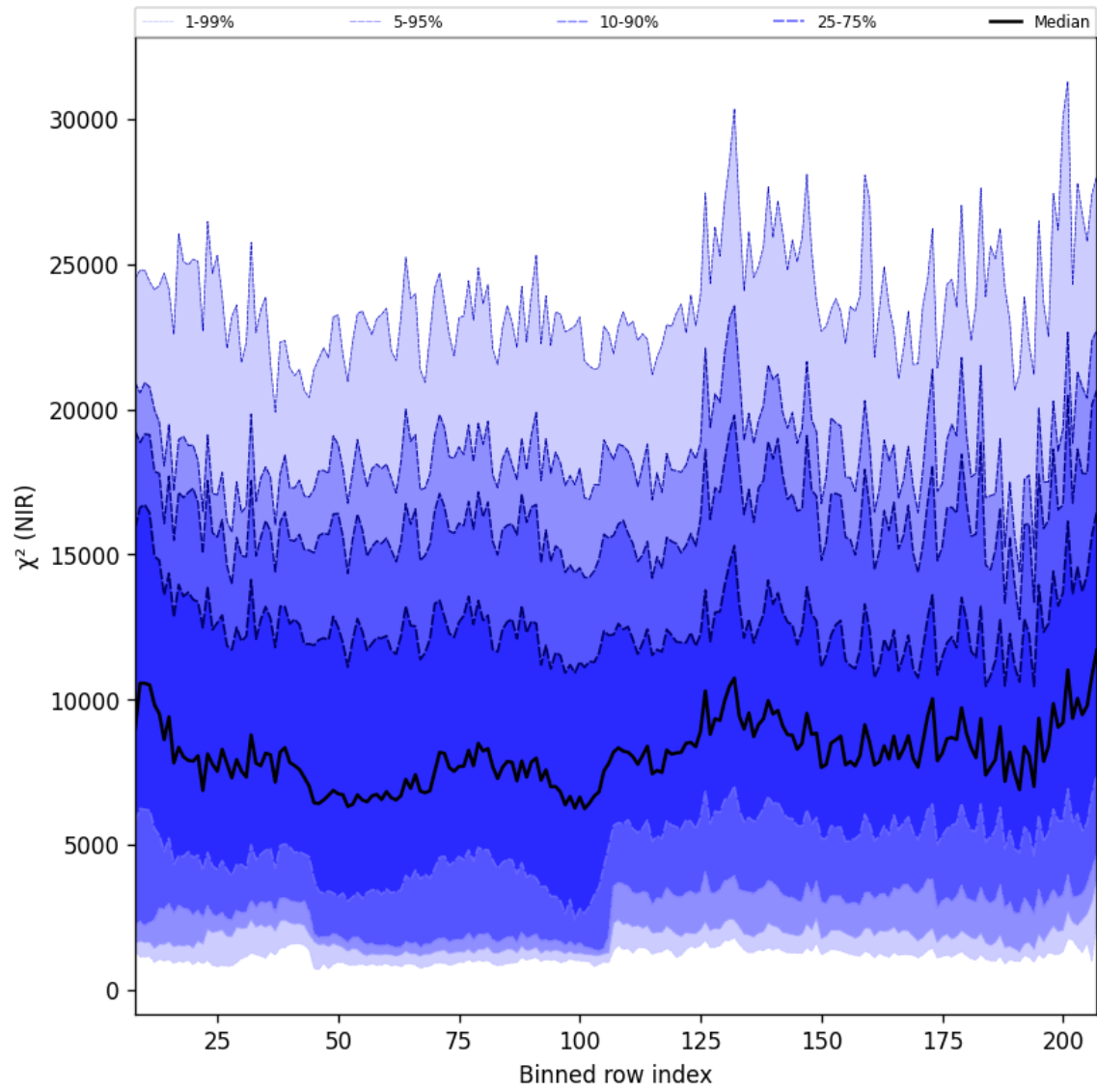
Figure 40: Along track statistics of “ \chi^2 (NIR)” for 2025-03-07 to 2025-03-08
