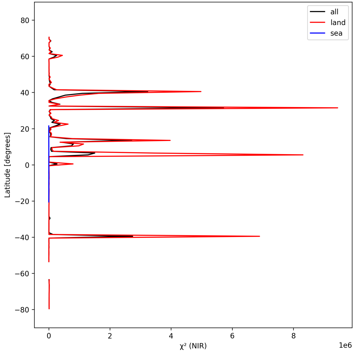
Figure 18: Zonal average of “ \chi^2 (NIR)” for 2025-03-07 to 2025-03-08.
