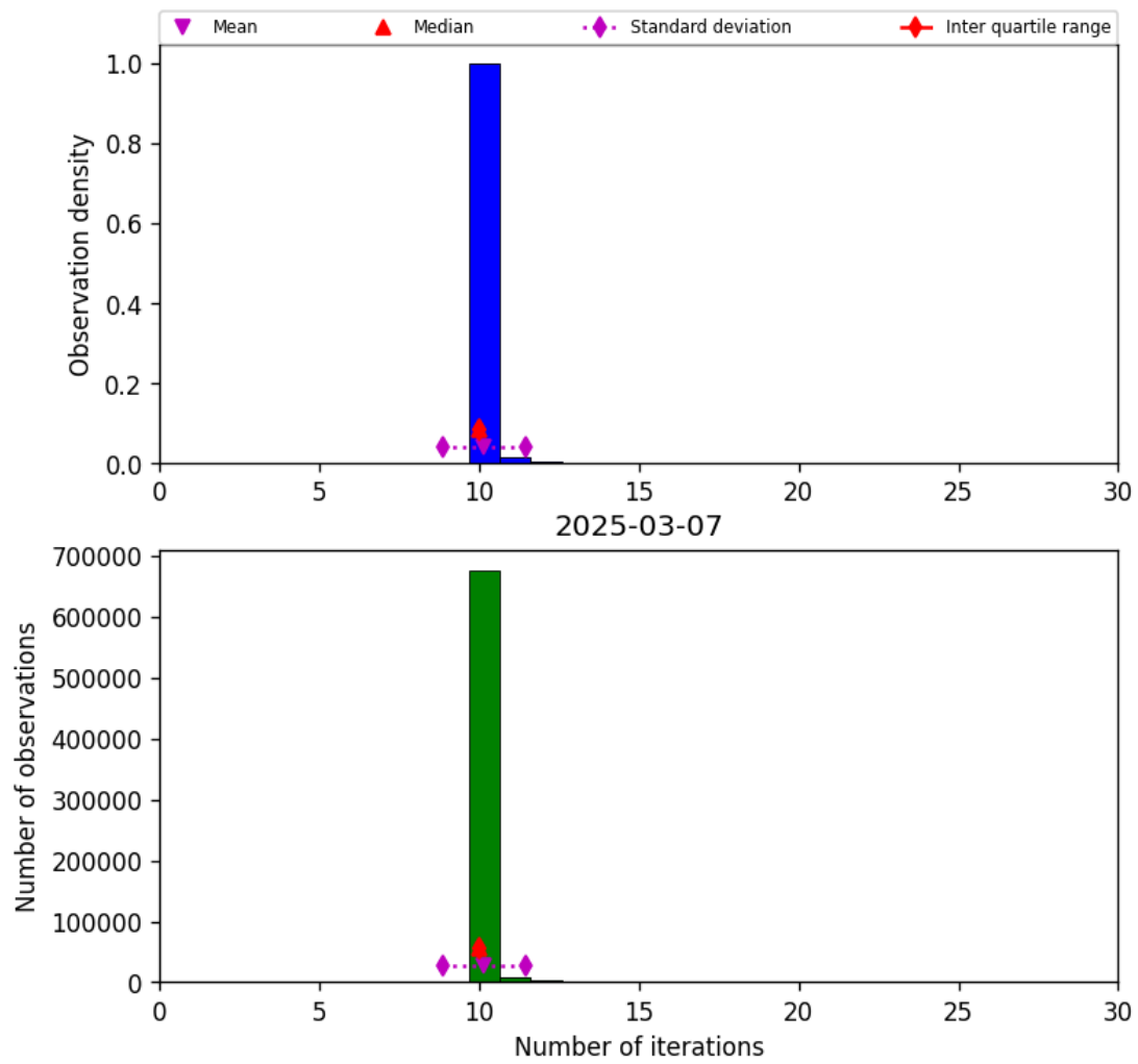
Figure 31: Histogram of “Number of iterations” for 2025-03-07 to 2025-03-08
