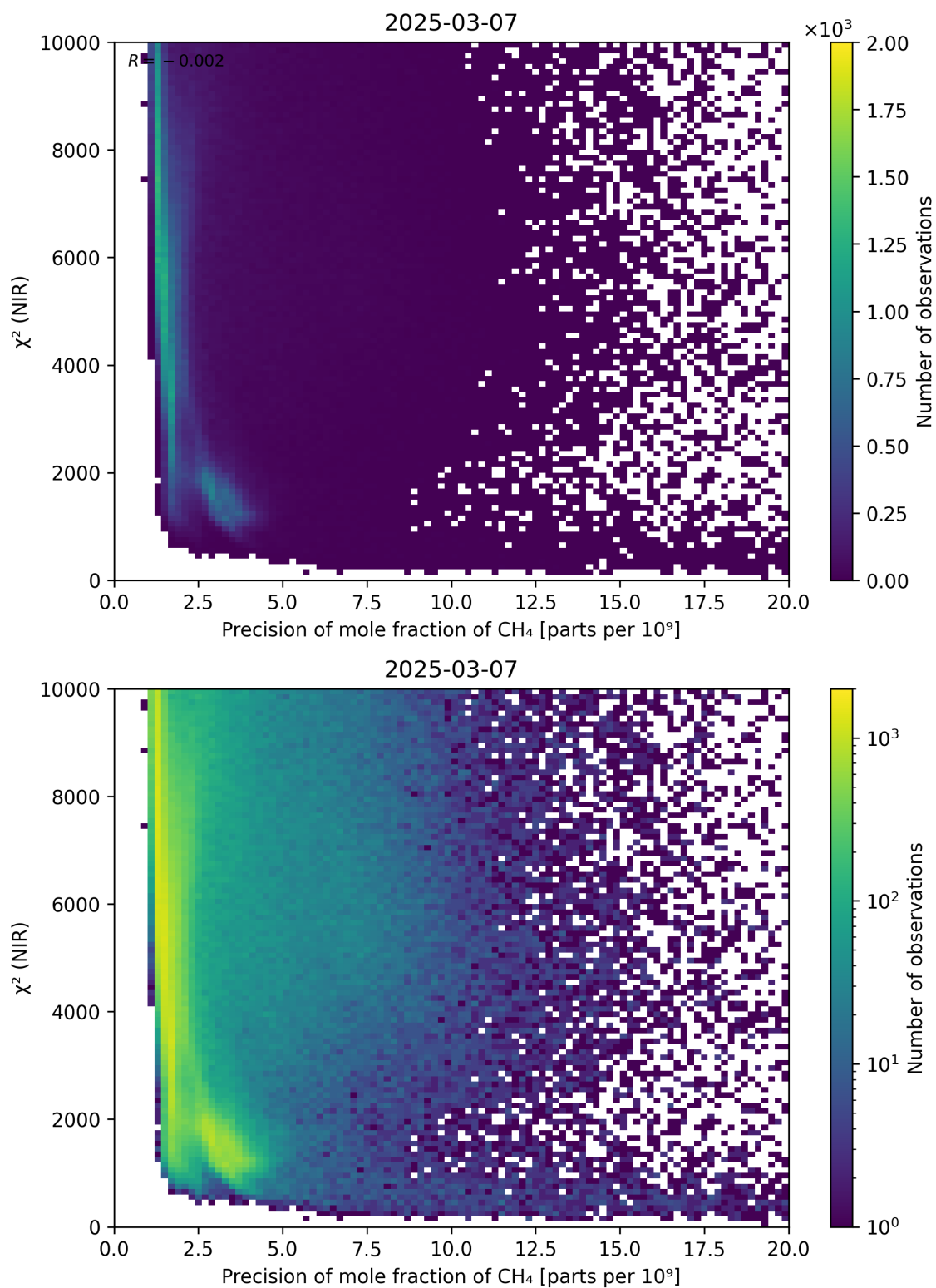
Figure 78: Scatter density plot of “Precision of mole fraction of \text{CH}_4 ” against “ \chi^2 (NIR)” for 2025-03-07 to 2025-03-08.
