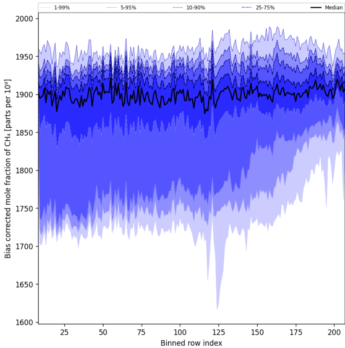
Figure 36: Along track statistics of “Bias corrected mole fraction of CH 4 ” for 2025-03-07 to 2025-03-08
