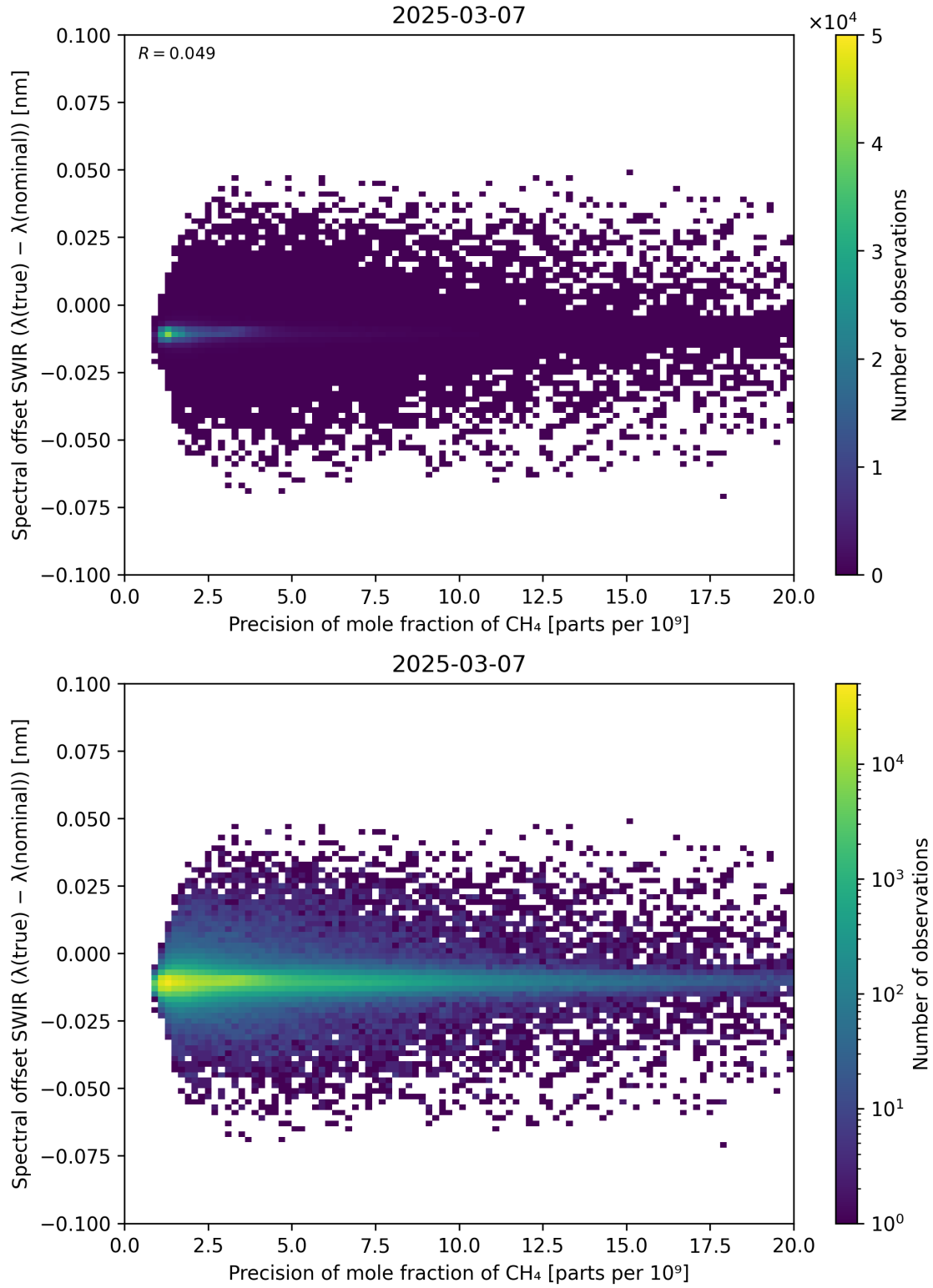
Figure 85: Scatter density plot of “Precision of mole fraction of CH 4 ” against “Spectral offset SWIR ( \lambda_{\text{true}} - \lambda_{\text{nominal}} )” for 2025-03-07 to 2025-03-08.
