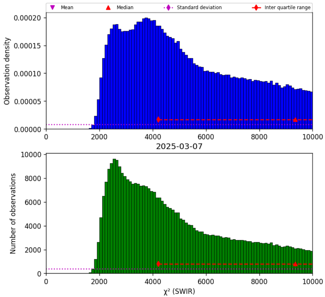
Figure 28: Histogram of “ \chi^2 (SWIR)” for 2025-03-07 to 2025-03-08
