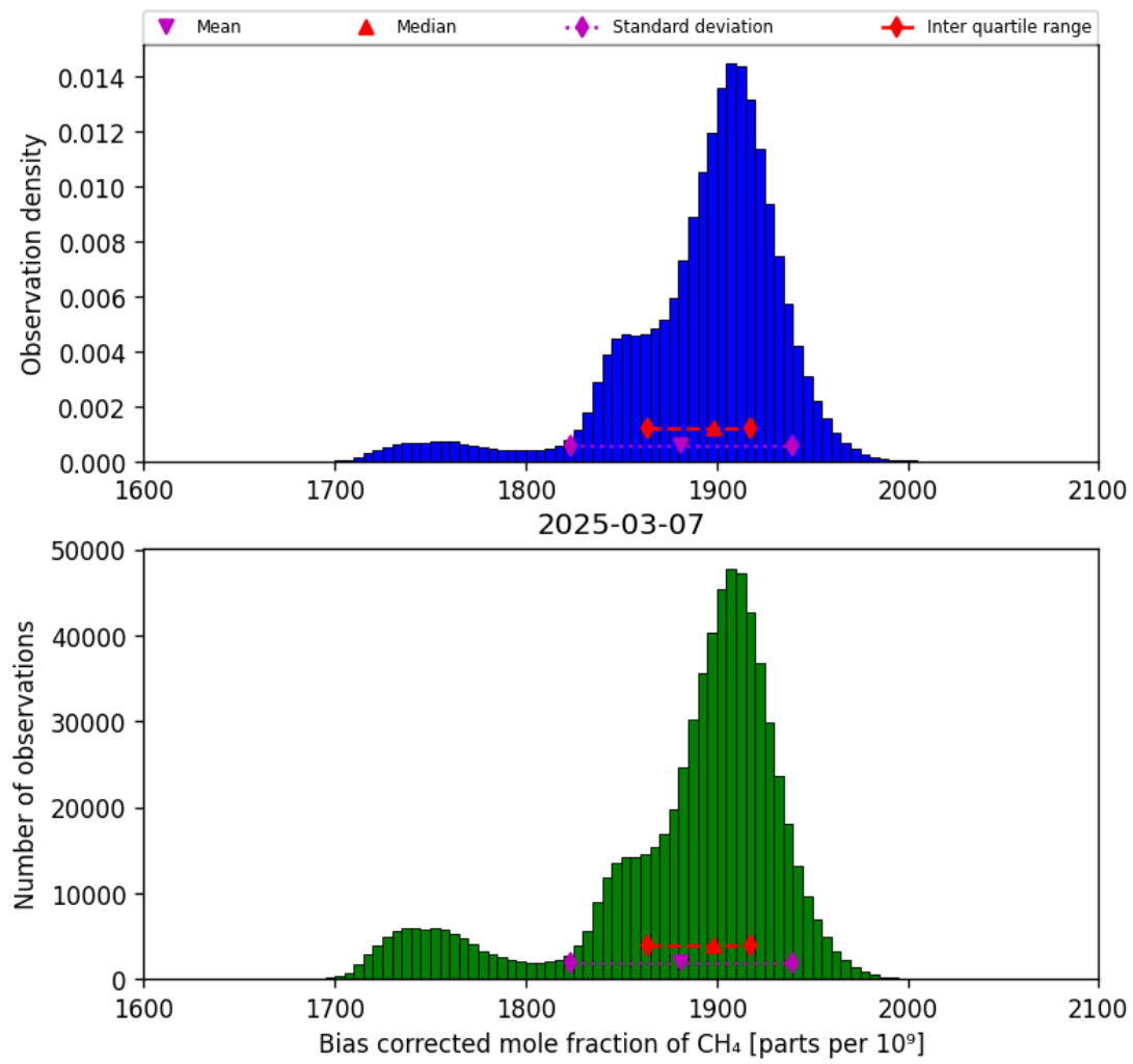
Figure 25: Histogram of “Bias corrected mole fraction of CH 4 ” for 2025-03-07 to 2025-03-08
