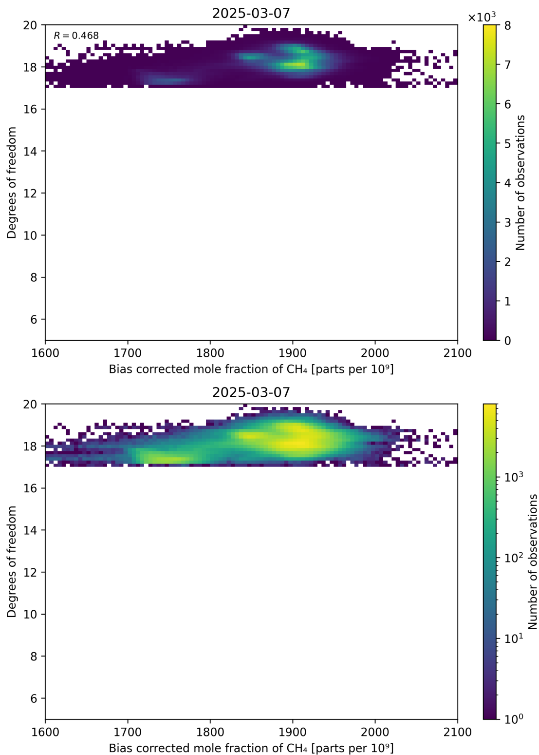
Figure 65: Scatter density plot of “Bias corrected mole fraction of CH 4 ” against “Degrees of freedom” for 2025-03-07 to 2025-03-08.
