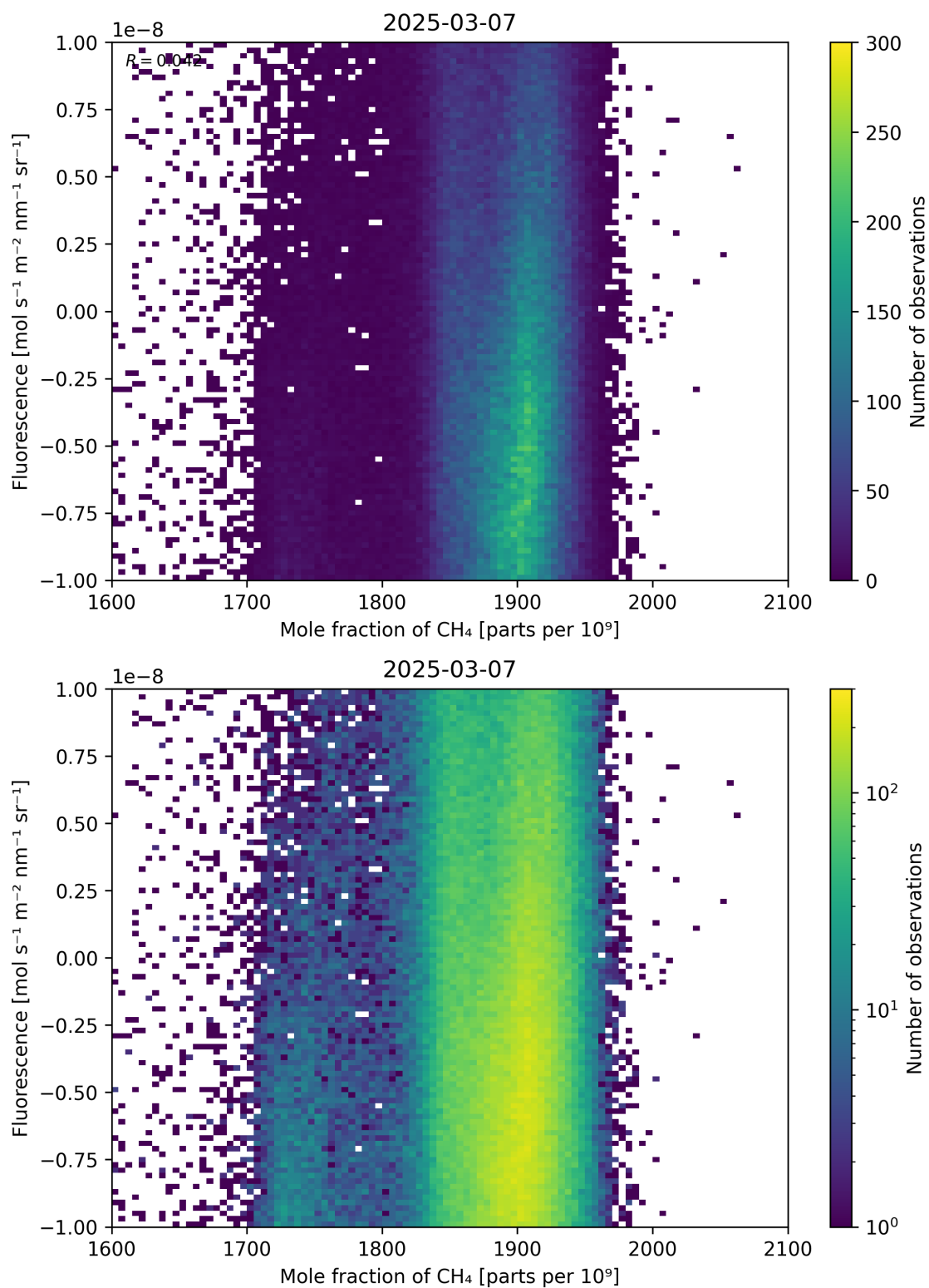
Figure 73: Scatter density plot of “Mole fraction of \text{CH}_4 ” against “Fluorescence” for 2025-03-07 to 2025-03-08.
