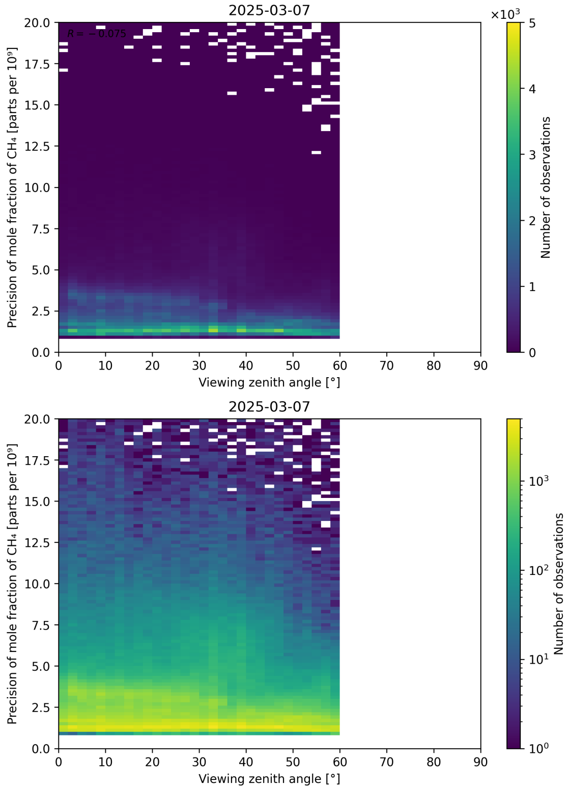
Figure 112: Scatter density plot of “Viewing zenith angle” against “Precision of mole fraction of CH 4 ” for 2025-03-07 to 2025-03-08.
