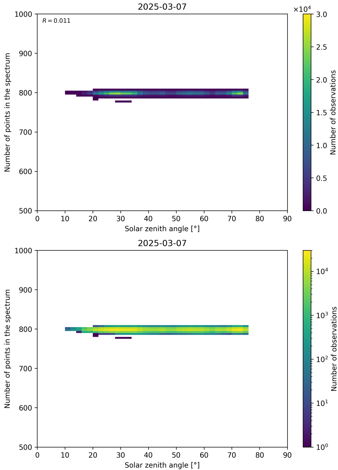
Figure 103: Scatter density plot of “Solar zenith angle” against “Number of points in the spectrum” for 2025-03-07 to 2025-03-08.
