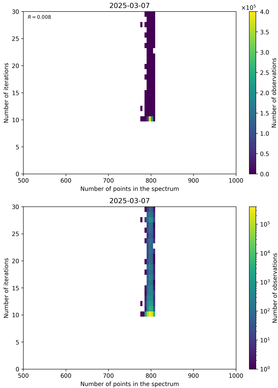
Figure 92: Scatter density plot of “Number of points in the spectrum” against “Number of iterations” for 2025-03-07 to 2025-03-08.
