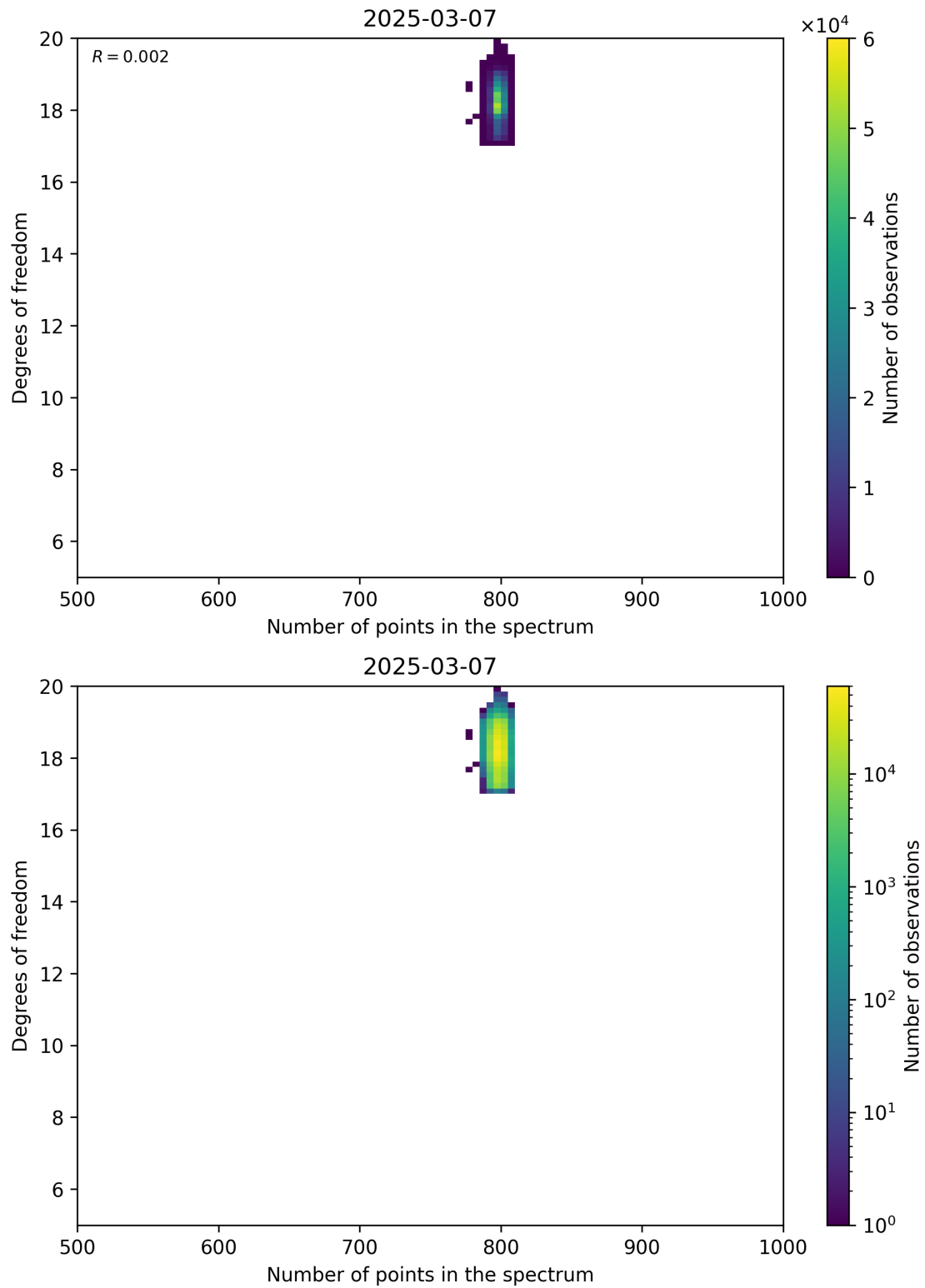
Figure 90: Scatter density plot of “Number of points in the spectrum” against “Degrees of freedom” for 2025-03-07 to 2025-03-08.
