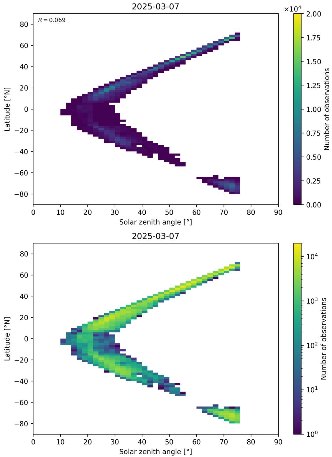
Figure 98: Scatter density plot of “Solar zenith angle” against “Latitude” for 2025-03-07 to 2025-03-08.
