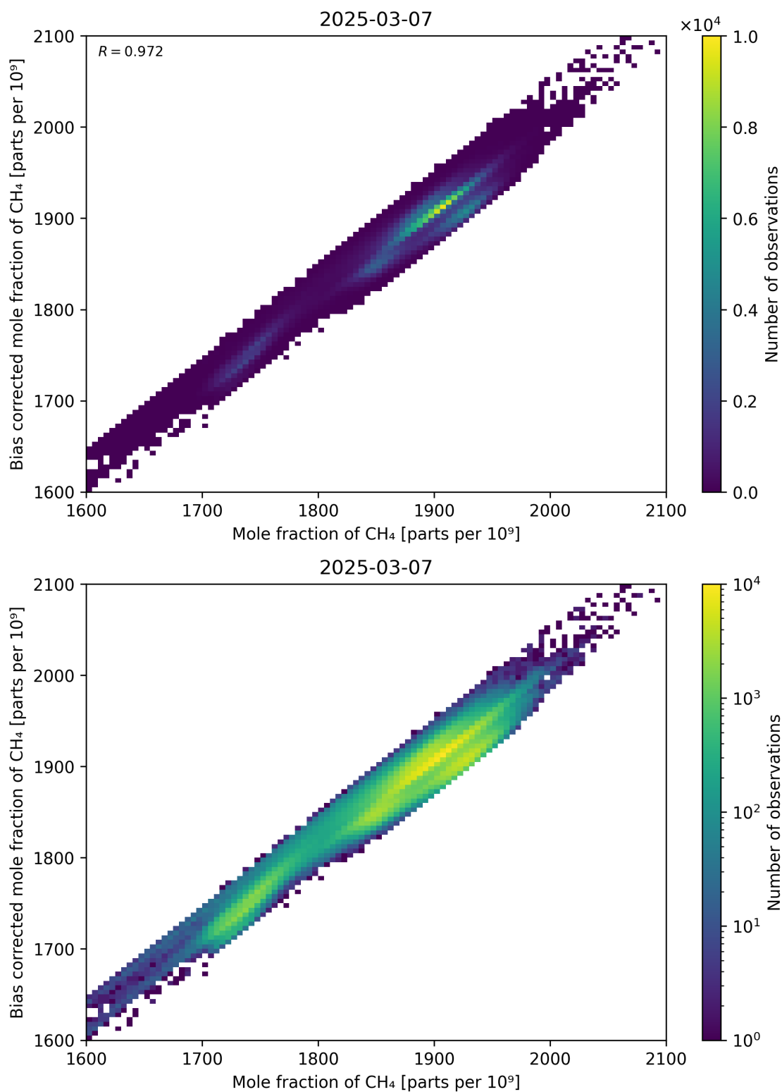
Figure 74: Scatter density plot of “Mole fraction of CH 4 ” against “Bias corrected mole fraction of CH 4 ” for 2025-03-07 to 2025-03-08.
