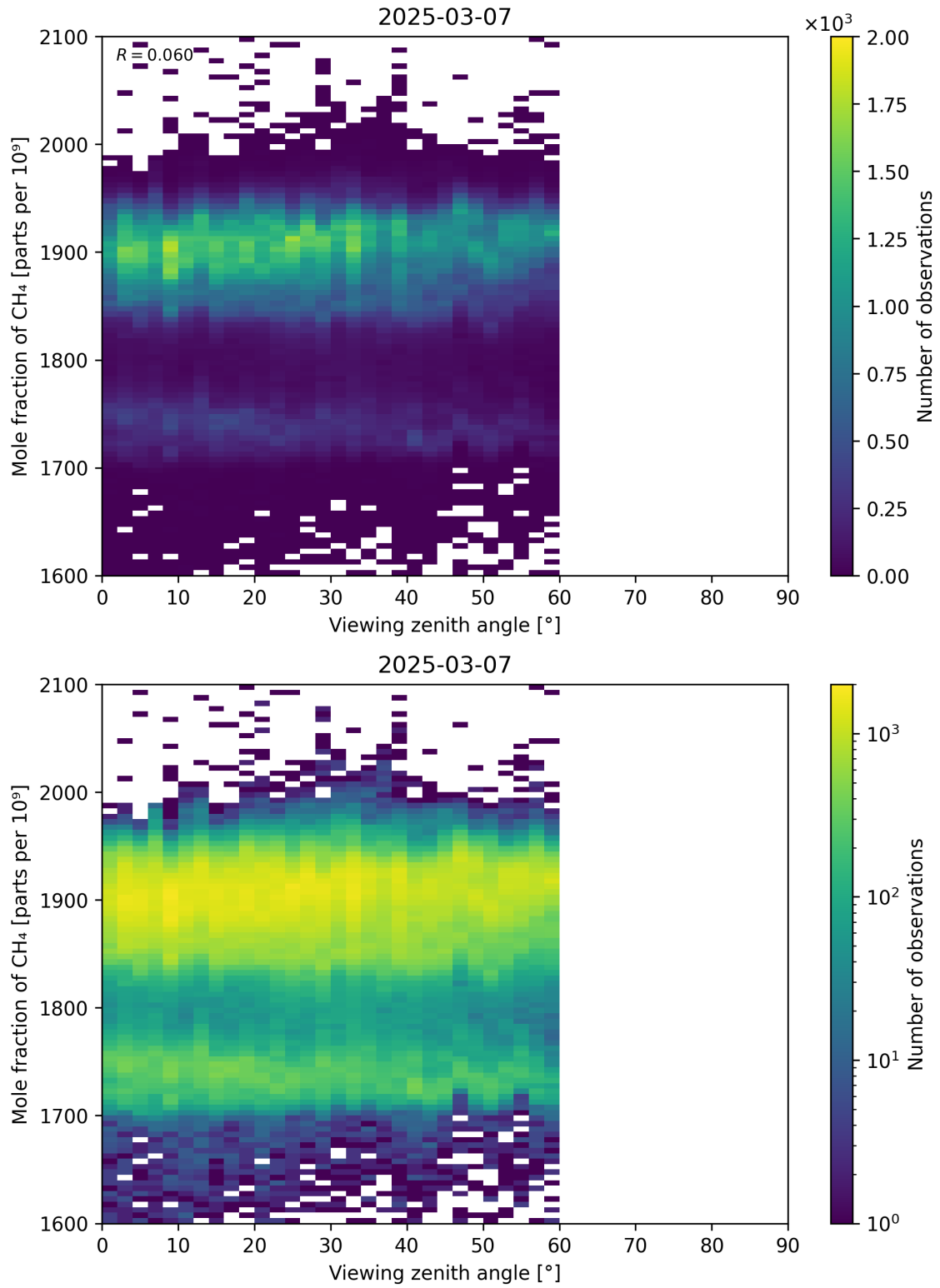
Figure 110: Scatter density plot of “Viewing zenith angle” against “Mole fraction of CH 4 ” for 2025-03-07 to 2025-03-08.
