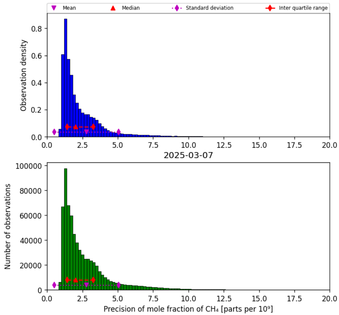
Figure 24: Histogram of “Precision of mole fraction of CH 4 ” for 2025-03-07 to 2025-03-08
