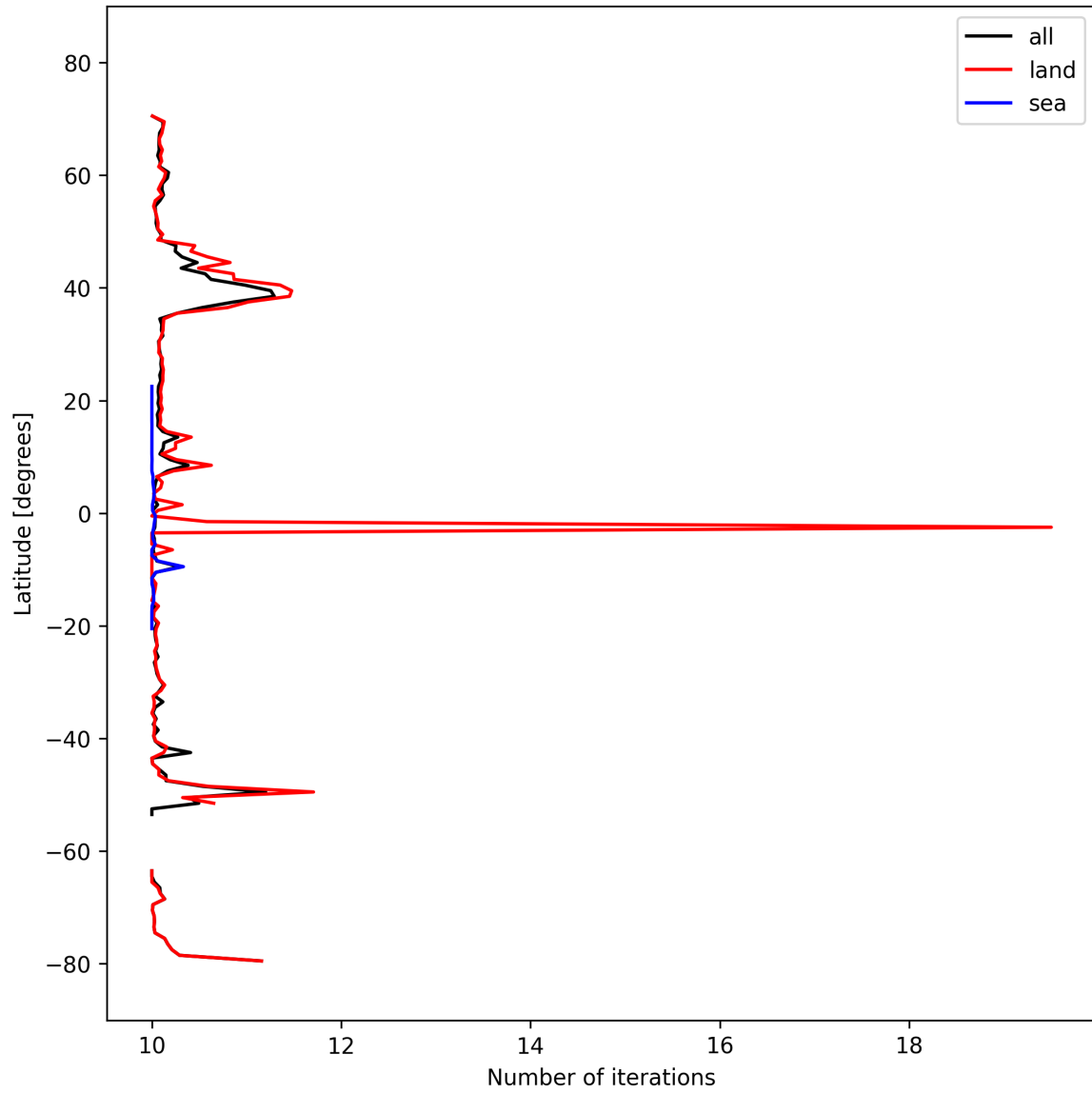
Figure 20: Zonal average of “Number of iterations” for 2025-03-07 to 2025-03-09.
