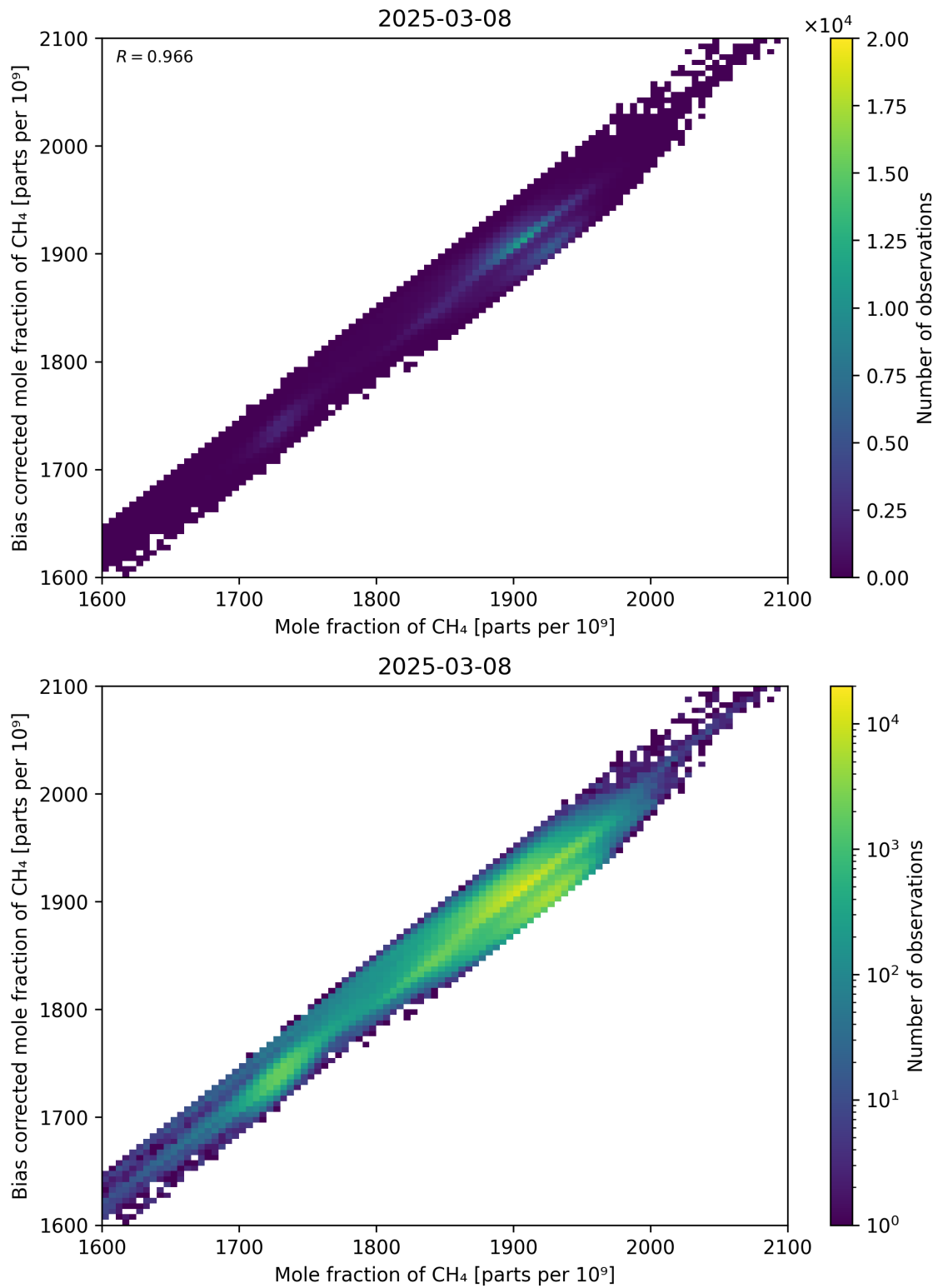
Figure 74: Scatter density plot of “Mole fraction of CH 4 ” against “Bias corrected mole fraction of CH 4 ” for 2025-03-07 to 2025-03-09.
