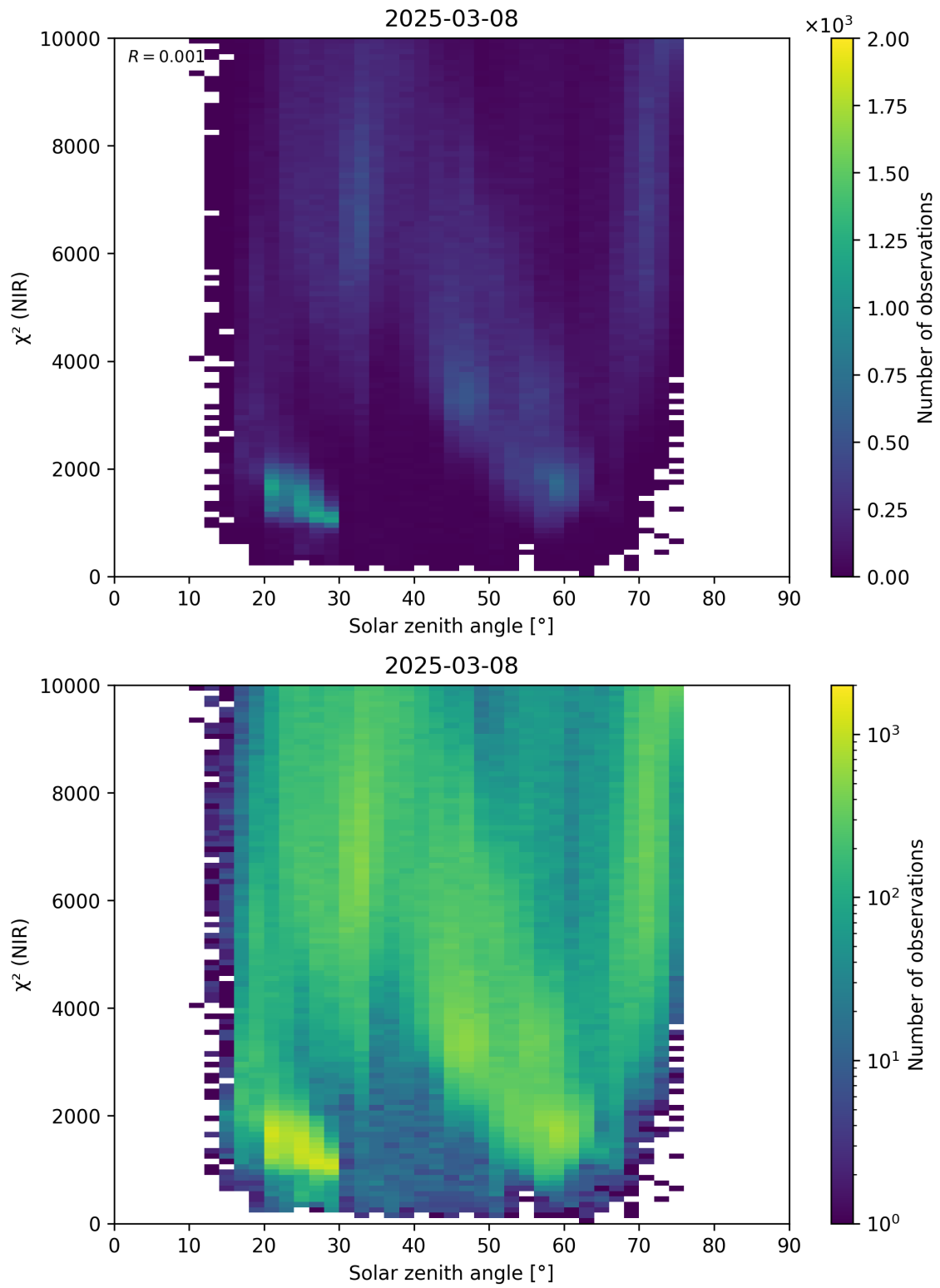
Figure 94: Scatter density plot of “Solar zenith angle” against “ \chi^2 (NIR)” for 2025-03-07 to 2025-03-09.
