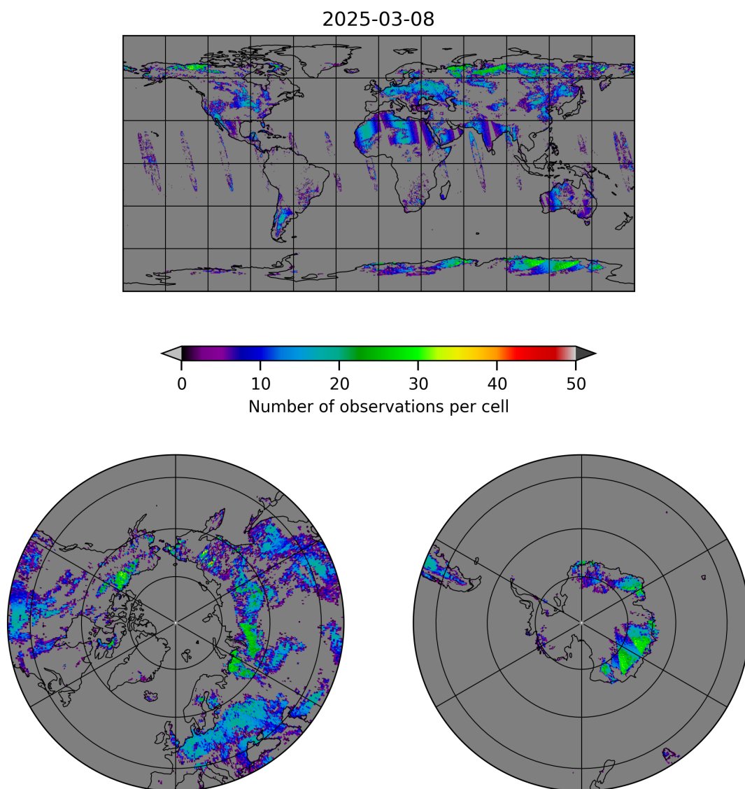
Figure 10: Map of the number of observations for 2025-03-07 to 2025-03-09
