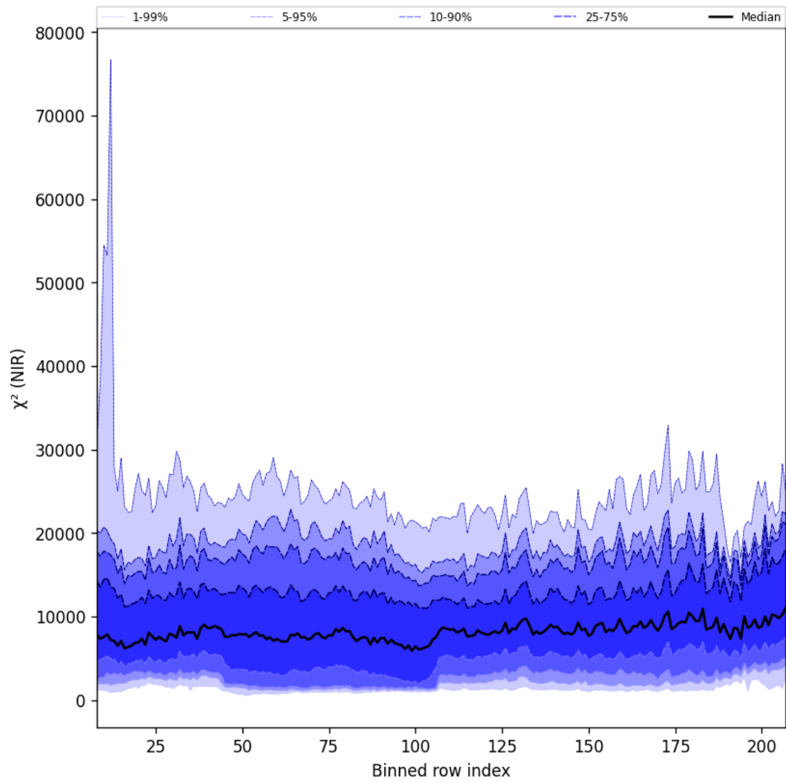
Figure 40: Along track statistics of “ \chi^2 (NIR)” for 2025-03-07 to 2025-03-09
