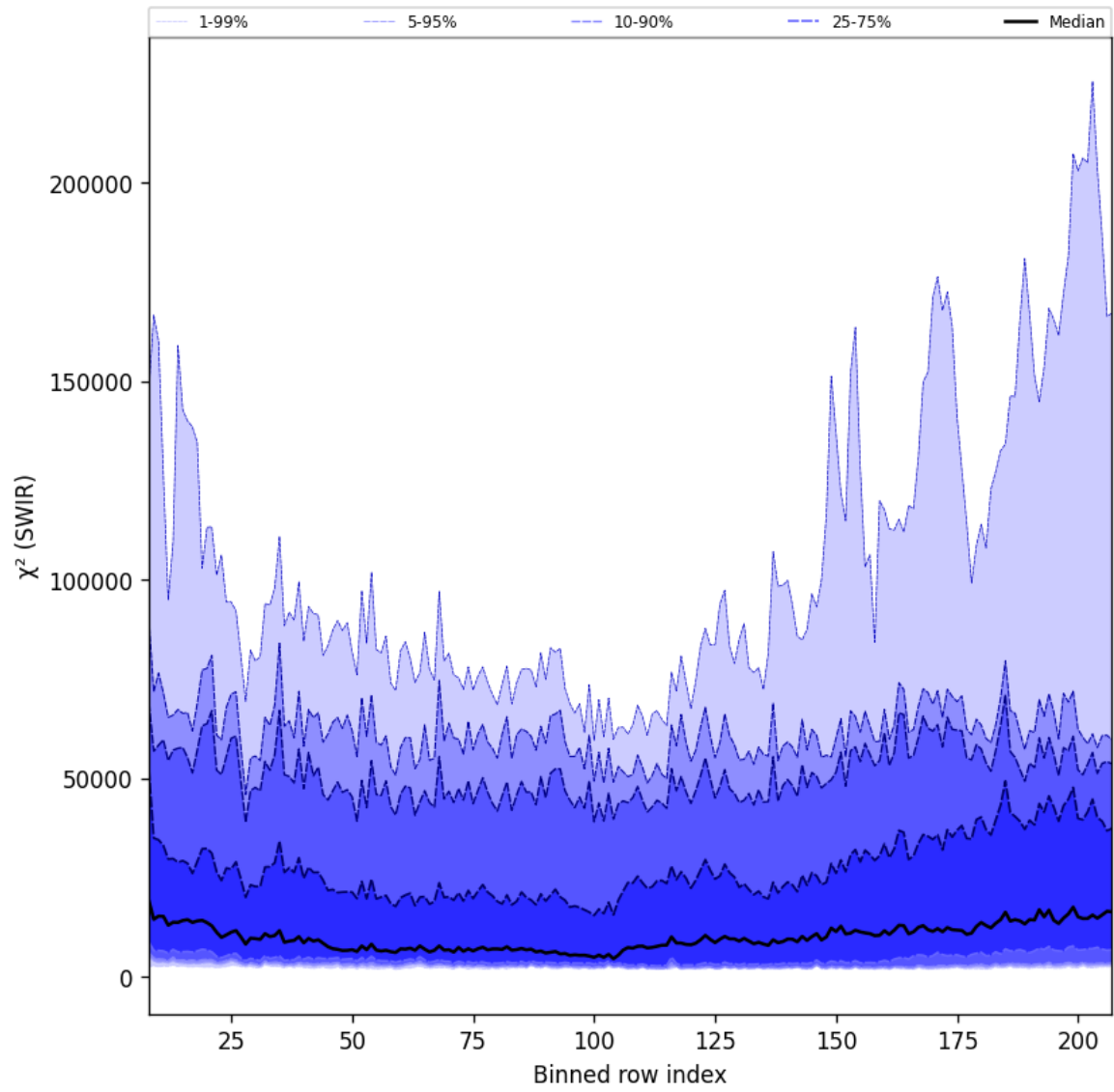
Figure 39: Along track statistics of “ \chi^2 (SWIR)” for 2025-03-07 to 2025-03-09
