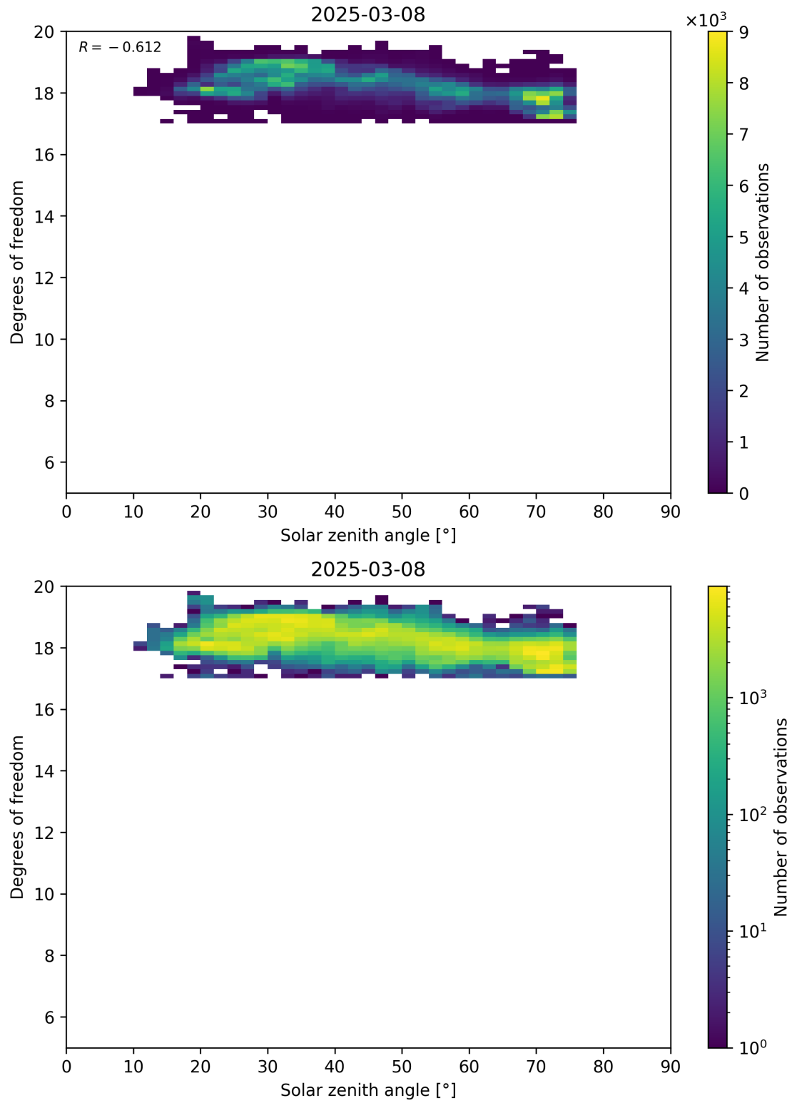
Figure 96: Scatter density plot of “Solar zenith angle” against “Degrees of freedom” for 2025-03-07 to 2025-03-09.
