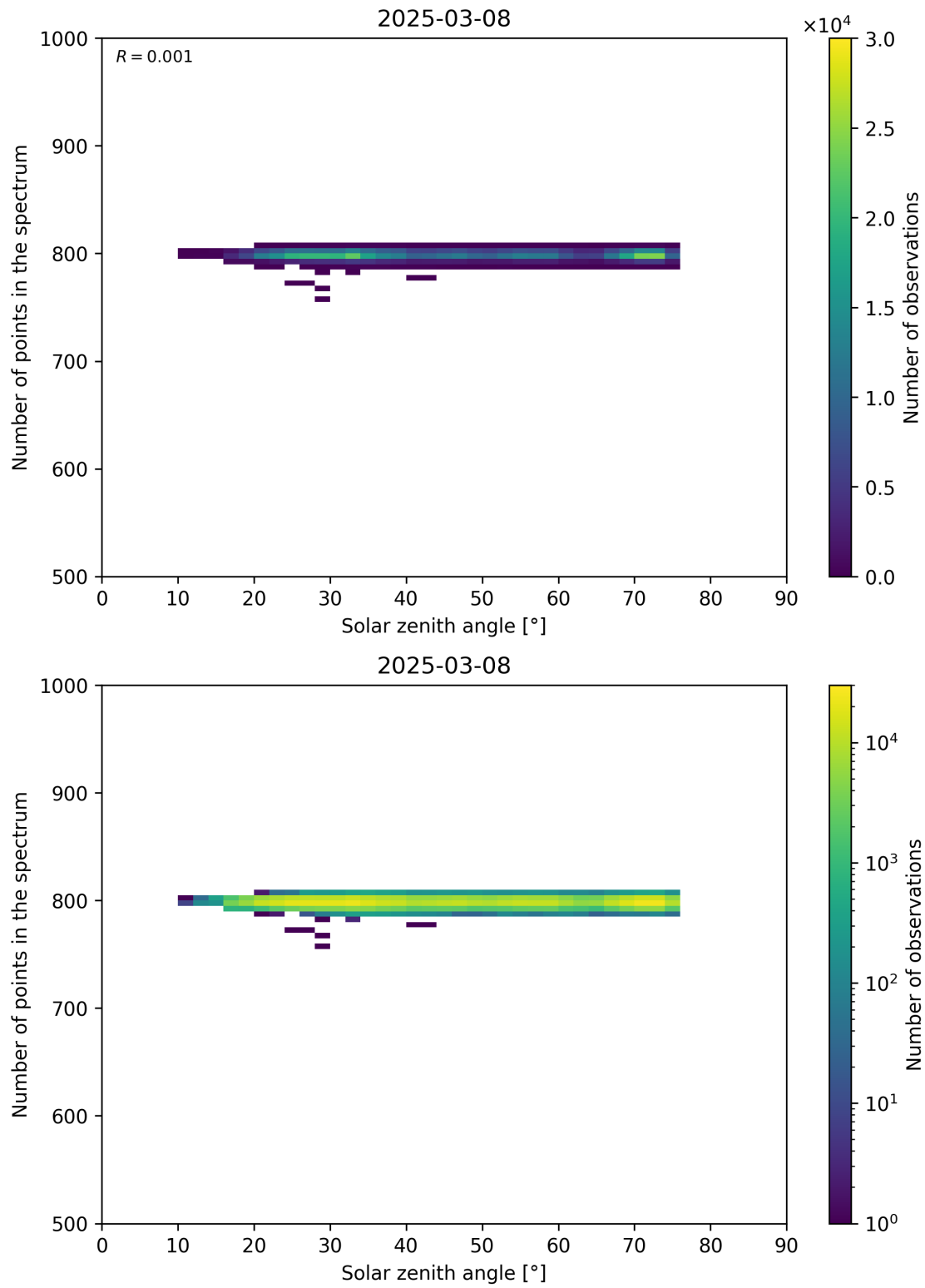
Figure 103: Scatter density plot of “Solar zenith angle” against “Number of points in the spectrum” for 2025-03-07 to 2025-03-09.
