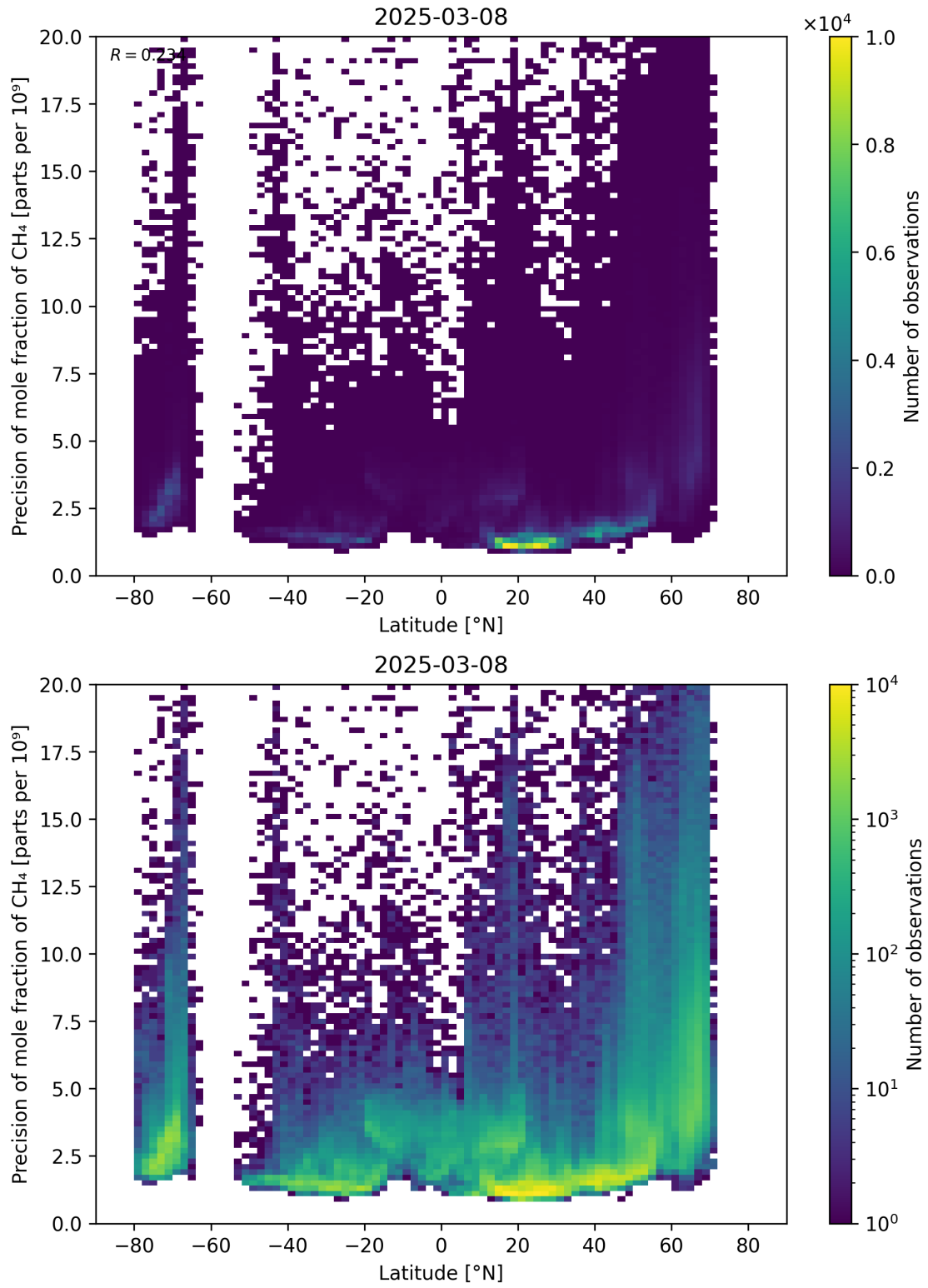
Figure 59: Scatter density plot of “Latitude” against “Precision of mole fraction of \text{CH}_4 ” for 2025-03-07 to 2025-03-09.
