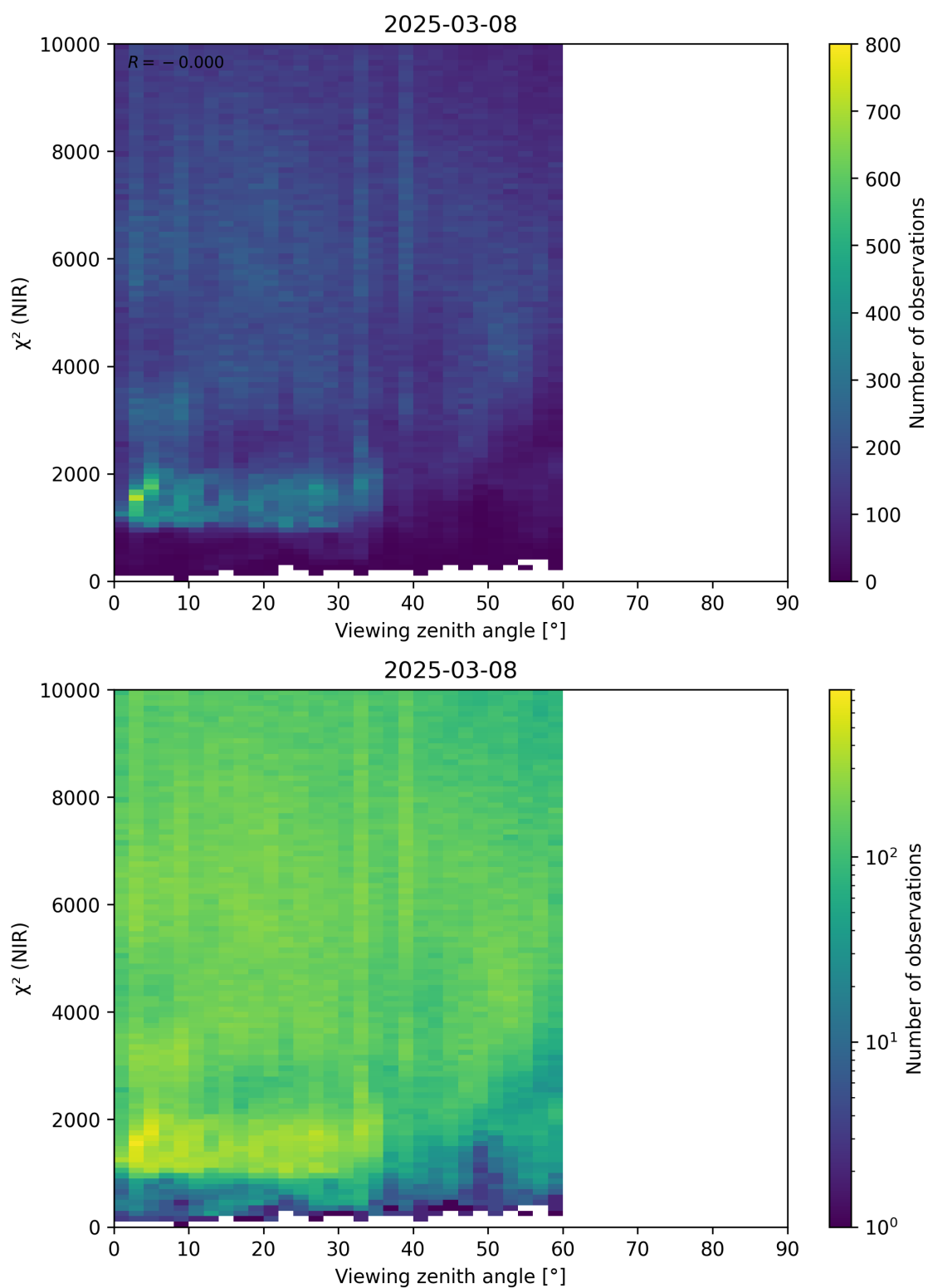
Figure 105: Scatter density plot of “Viewing zenith angle” against “ \chi^2 (NIR)” for 2025-03-07 to 2025-03-09.
