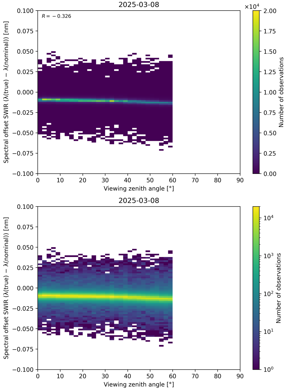
Figure 116: Scatter density plot of “Viewing zenith angle” against “Spectral offset SWIR ( \lambda_{\text{true}} - \lambda_{\text{nominal}} )” for 2025-03-07 to 2025-03-09.
