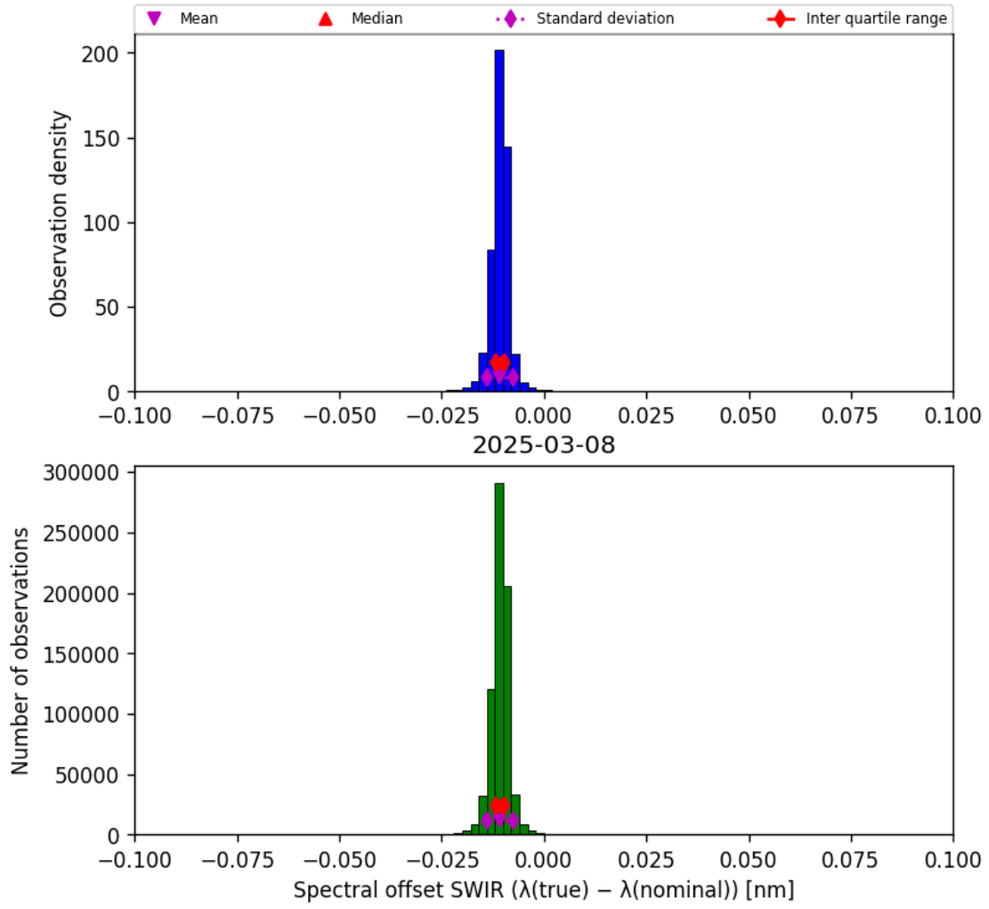
Figure 27: Histogram of “Spectral offset SWIR ( \lambda_{\text{true}} - \lambda_{\text{nominal}} )” for 2025-03-07 to 2025-03-09
