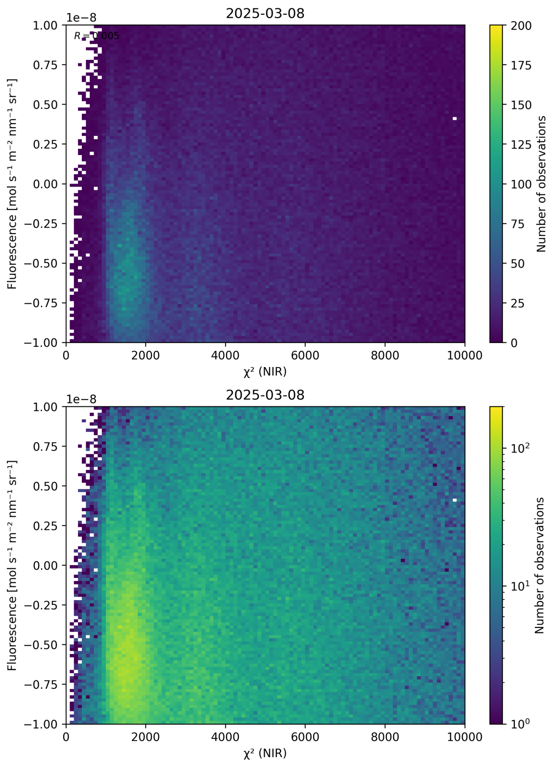
Figure 45: Scatter density plot of “ \chi^2 (NIR)” against “Fluorescence” for 2025-03-07 to 2025-03-09.
