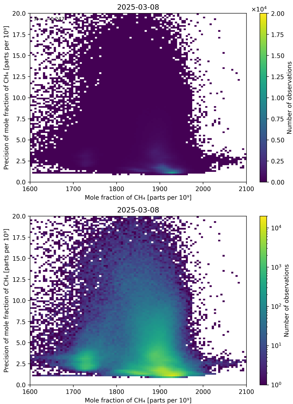
Figure 75: Scatter density plot of “Mole fraction of CH 4 ” against “Precision of mole fraction of CH 4 ” for 2025-03-07 to 2025-03-09.
