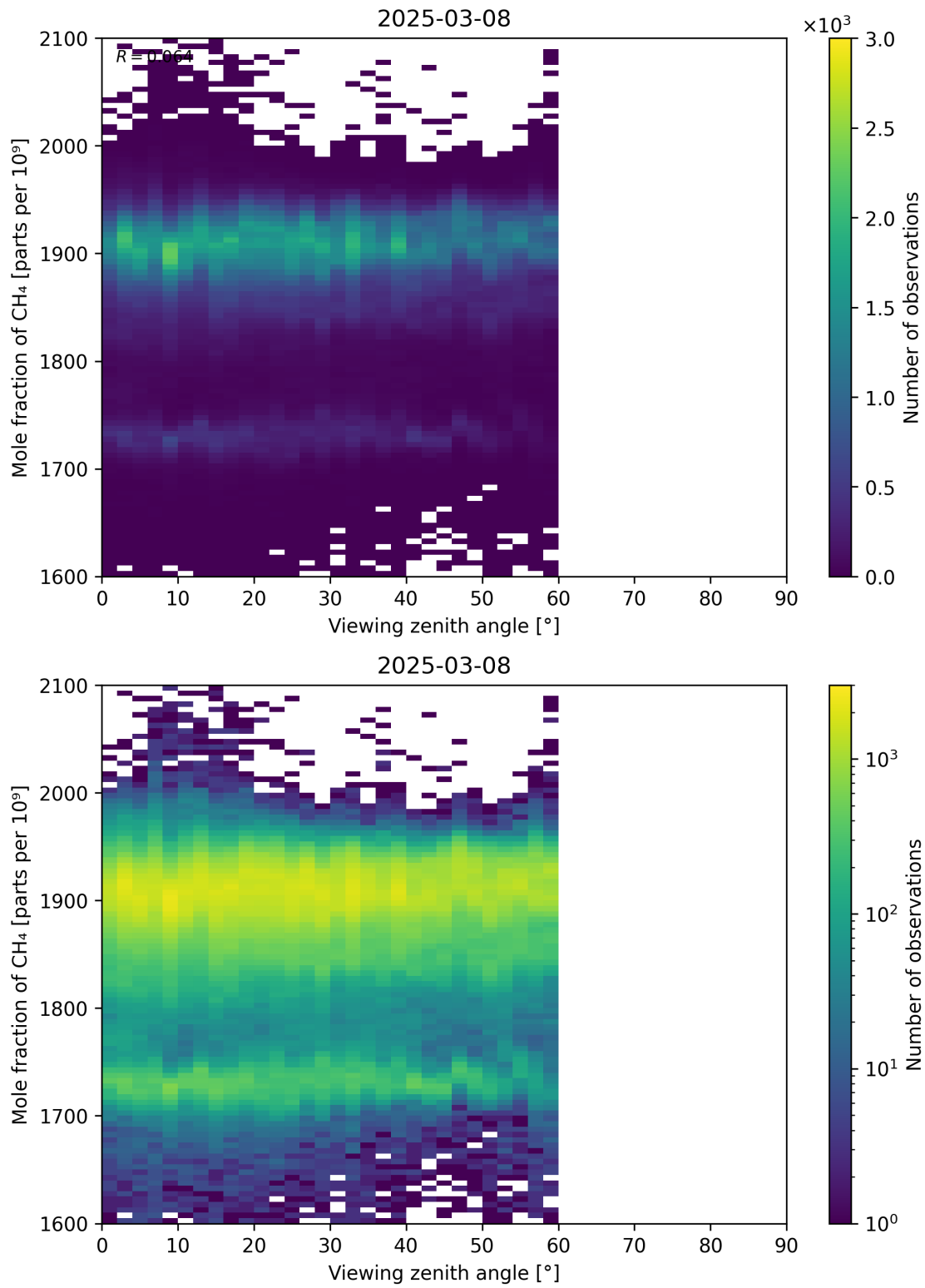
Figure 110: Scatter density plot of "Viewing zenith angle" against "Mole fraction of CH 4 " for 2025-03-07 to 2025-03-09.
