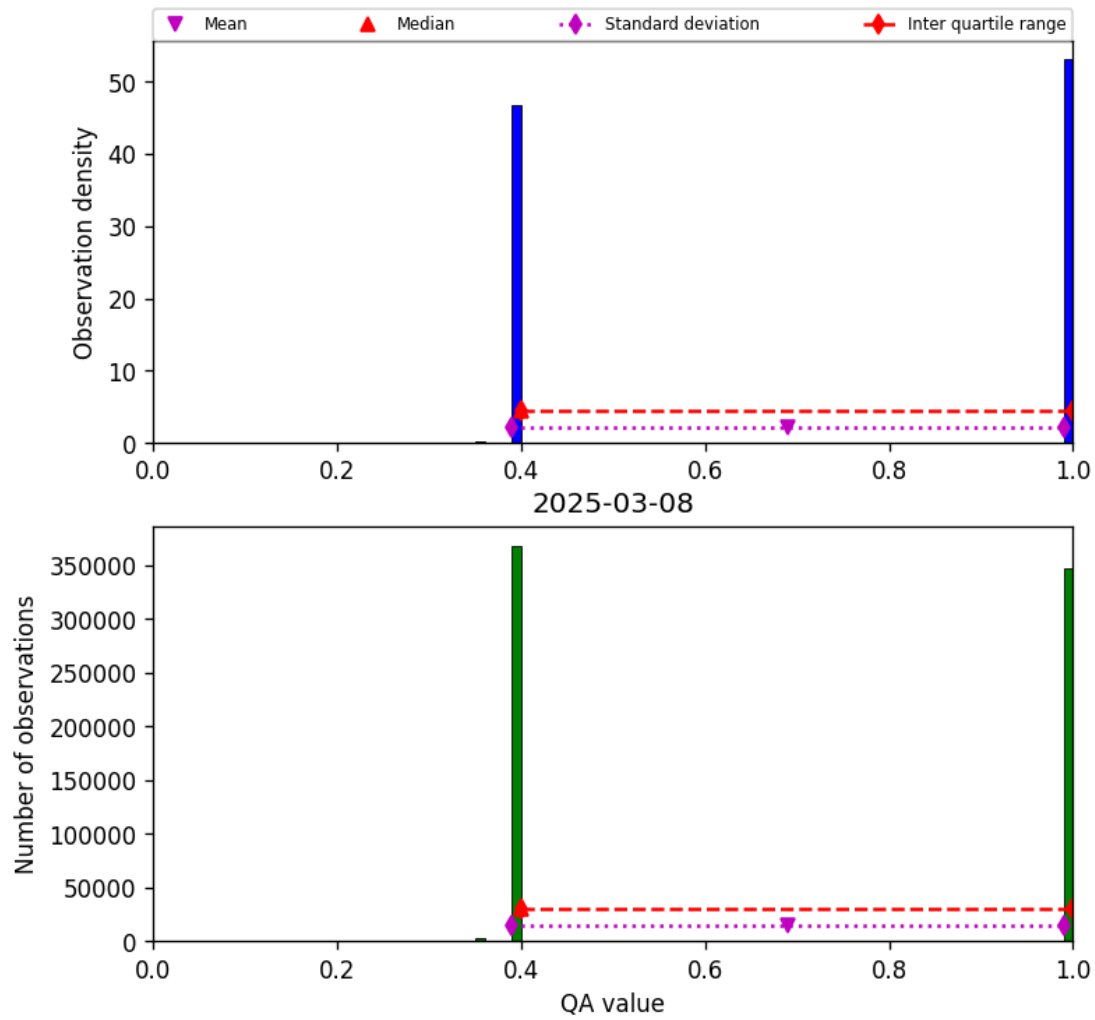
Figure 22: Histogram of “QA value” for 2025-03-07 to 2025-03-09
