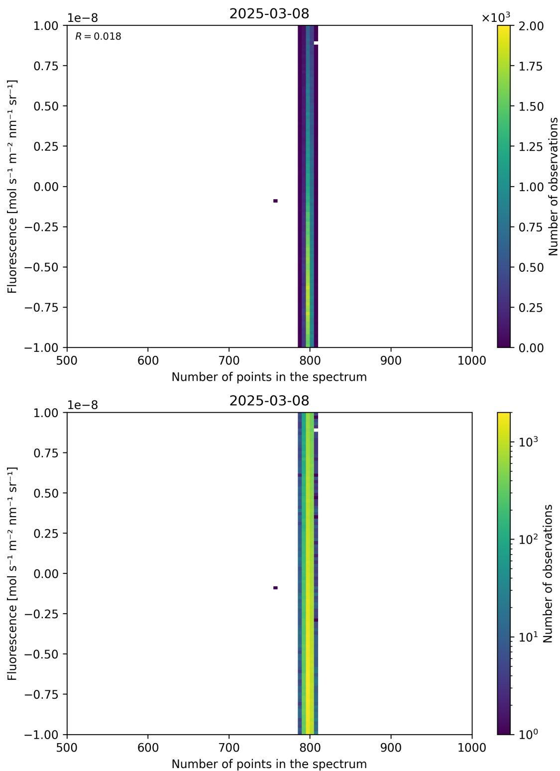
Figure 91: Scatter density plot of “Number of points in the spectrum” against “Fluorescence” for 2025-03-07 to 2025-03-09.
