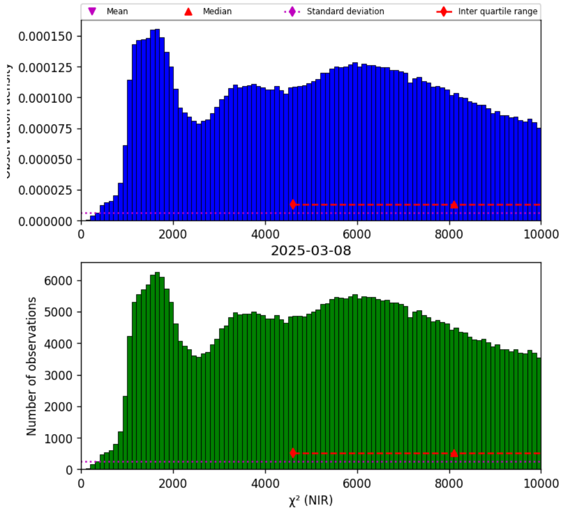
Figure 29: Histogram of “ \chi^2 (NIR)” for 2025-03-07 to 2025-03-09
