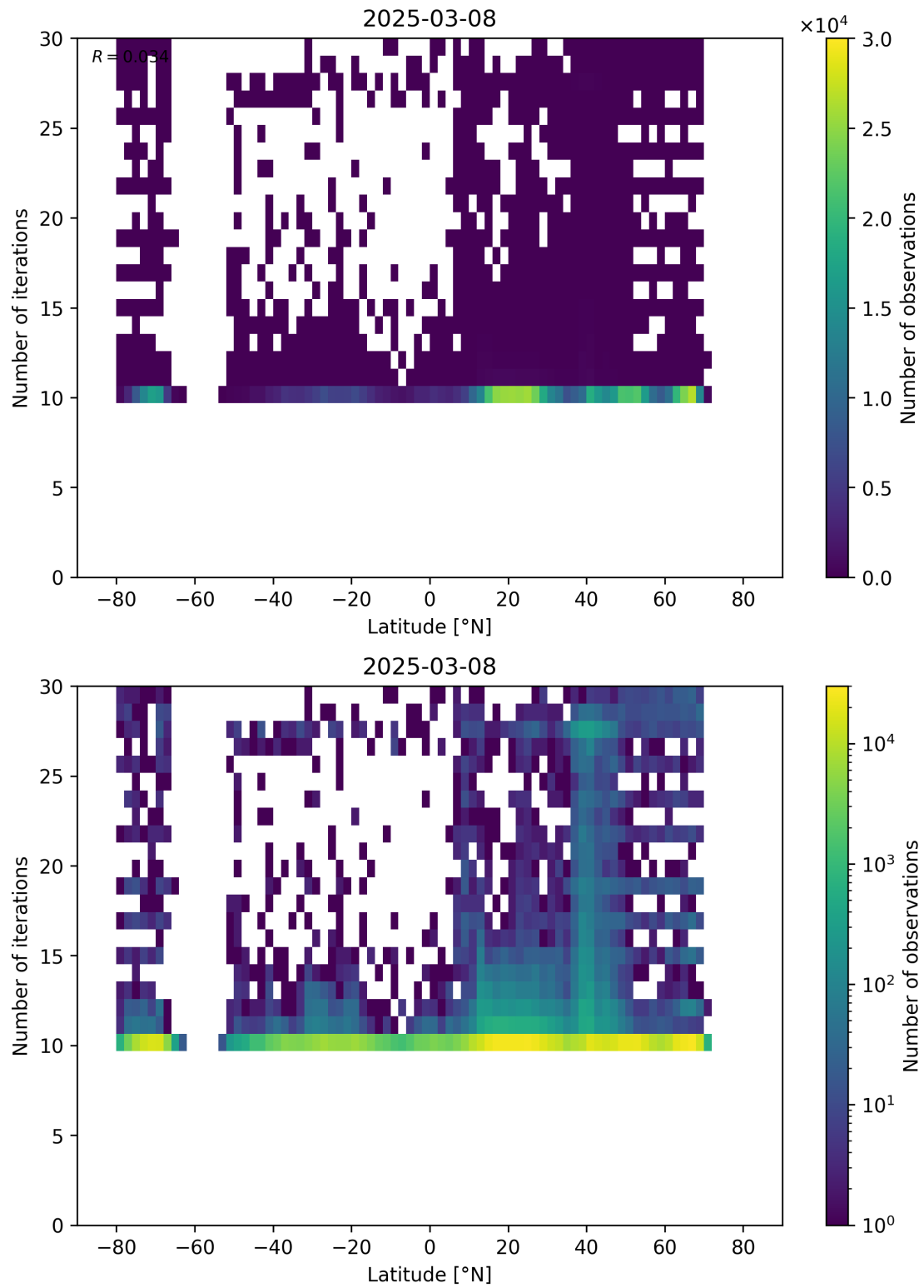
Figure 60: Scatter density plot of “Latitude” against “Number of iterations” for 2025-03-07 to 2025-03-09.
