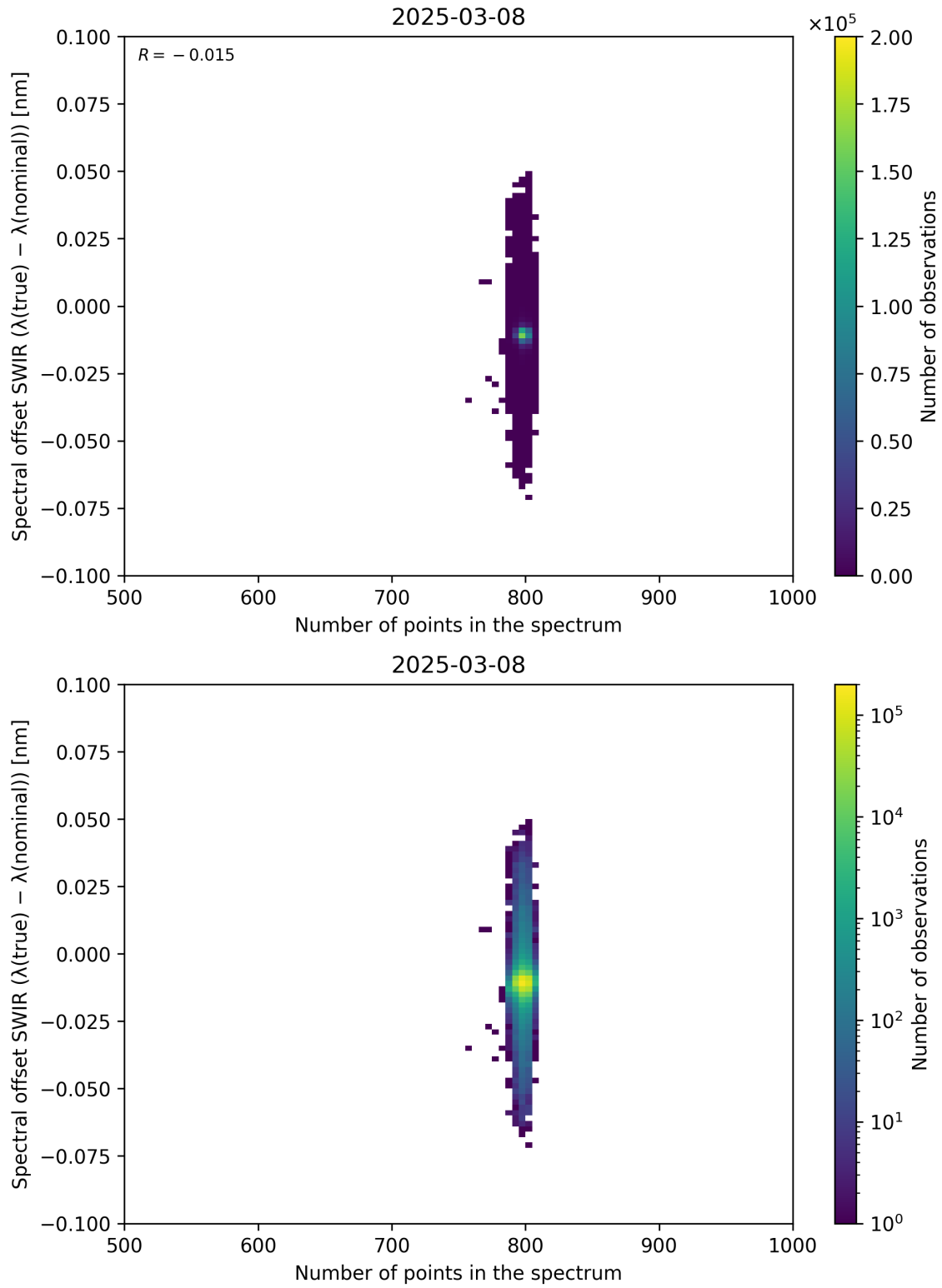
Figure 93: Scatter density plot of “Number of points in the spectrum” against “Spectral offset SWIR ( \lambda_{\text{true}} - \lambda_{\text{nominal}} )” for 2025-03-07 to 2025-03-09.
