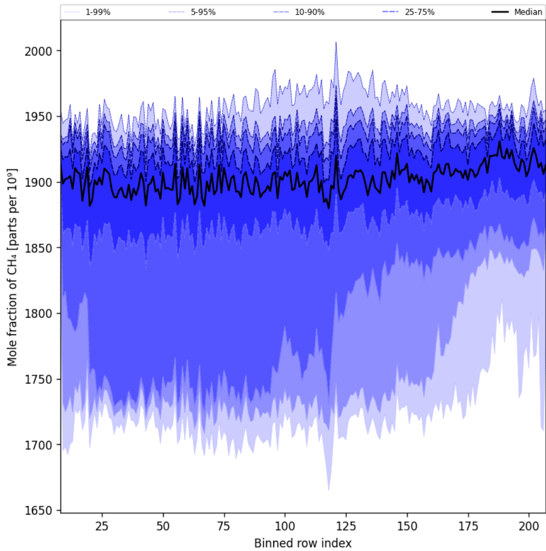
Figure 34: Along track statistics of “Mole fraction of CH 4 ” for 2025-03-07 to 2025-03-09
