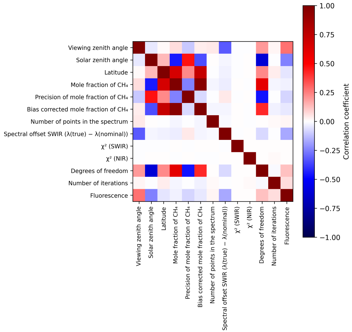
Figure 2: Map of correlation matrix for 2025-03-07 to 2025-03-09.
