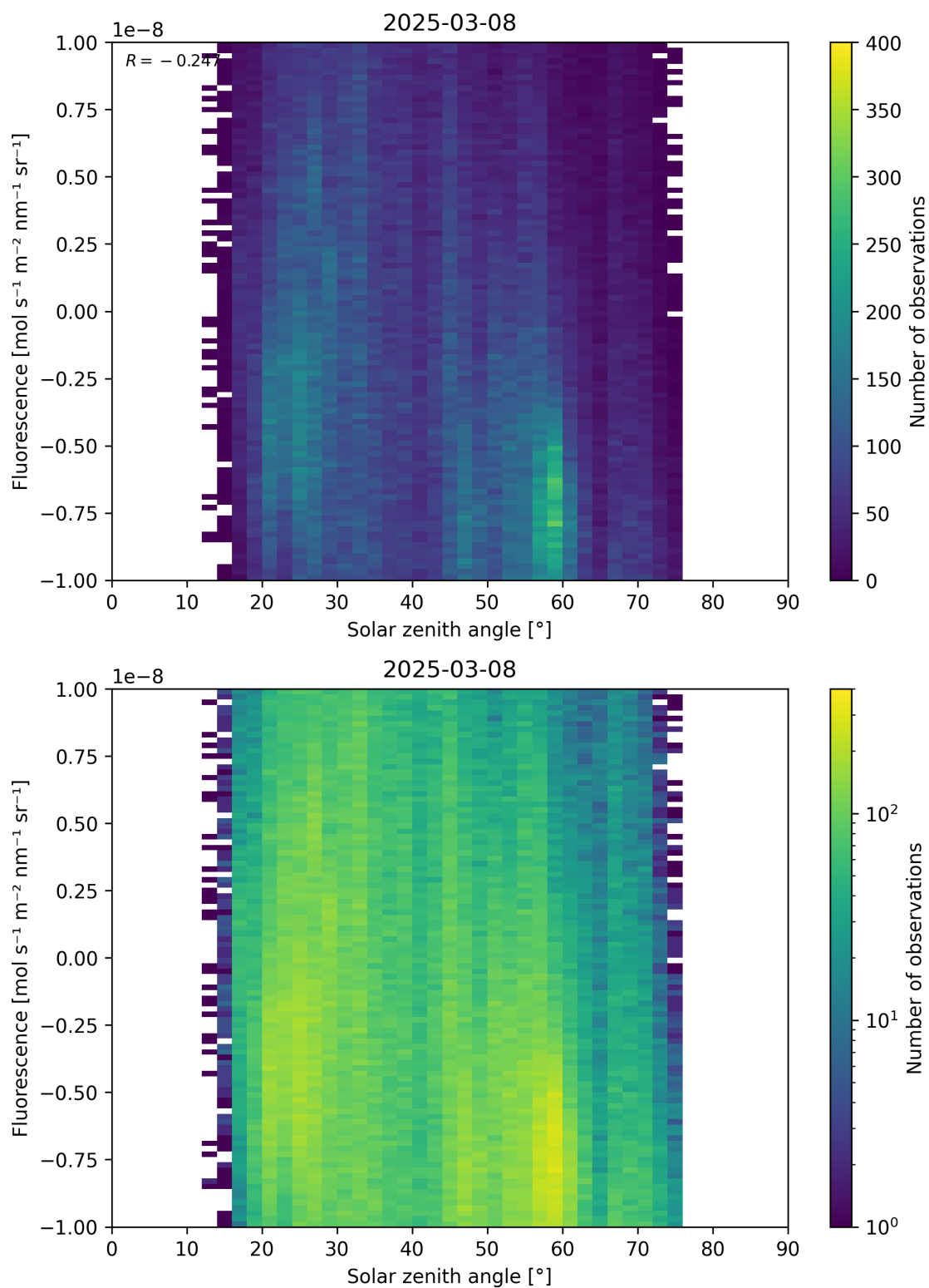
Figure 97: Scatter density plot of “Solar zenith angle” against “Fluorescence” for 2025-03-07 to 2025-03-09.
