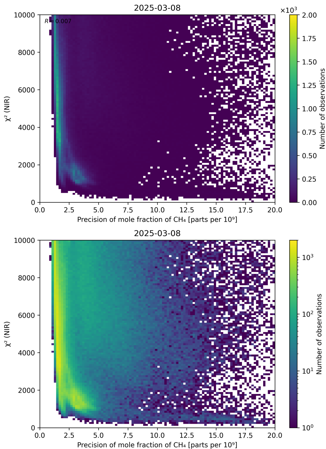
Figure 78: Scatter density plot of “Precision of mole fraction of CH 4 ” against “ \chi^2 (NIR)” for 2025-03-07 to 2025-03-09.
