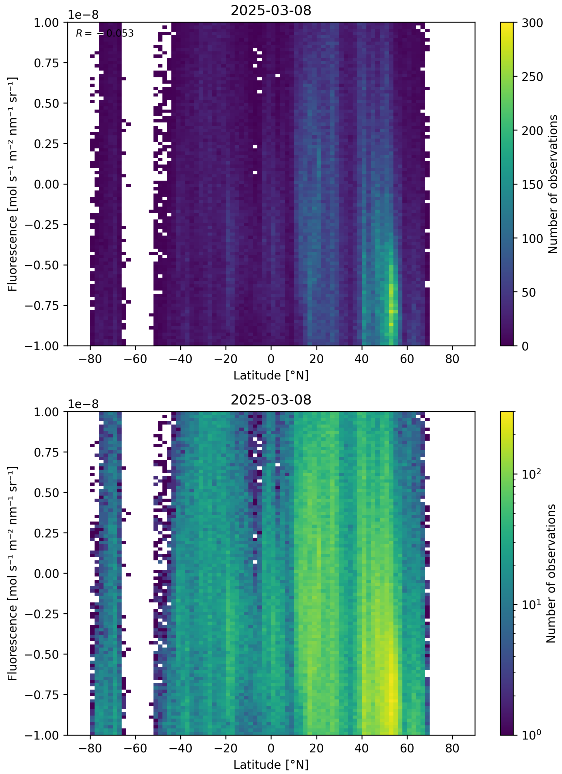
Figure 56: Scatter density plot of “Latitude” against “Fluorescence” for 2025-03-07 to 2025-03-09.
