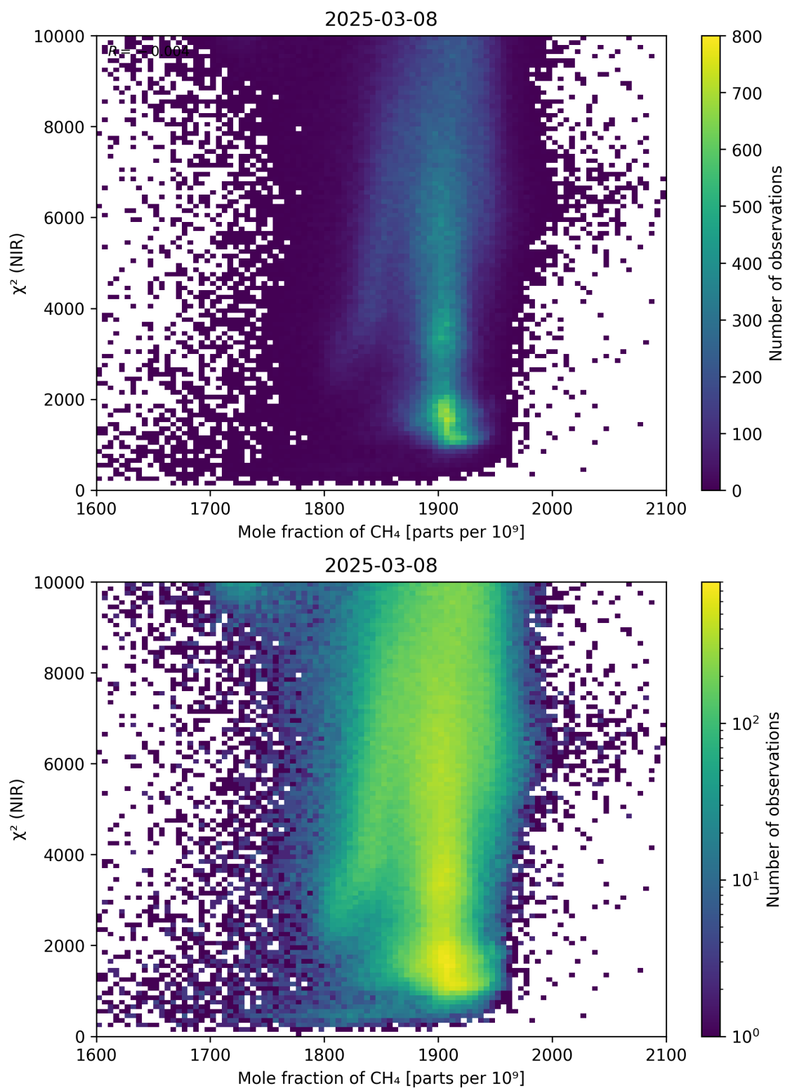
Figure 70: Scatter density plot of “Mole fraction of \text{CH}_4 ” against “ \chi^2 (NIR)” for 2025-03-07 to 2025-03-09.
