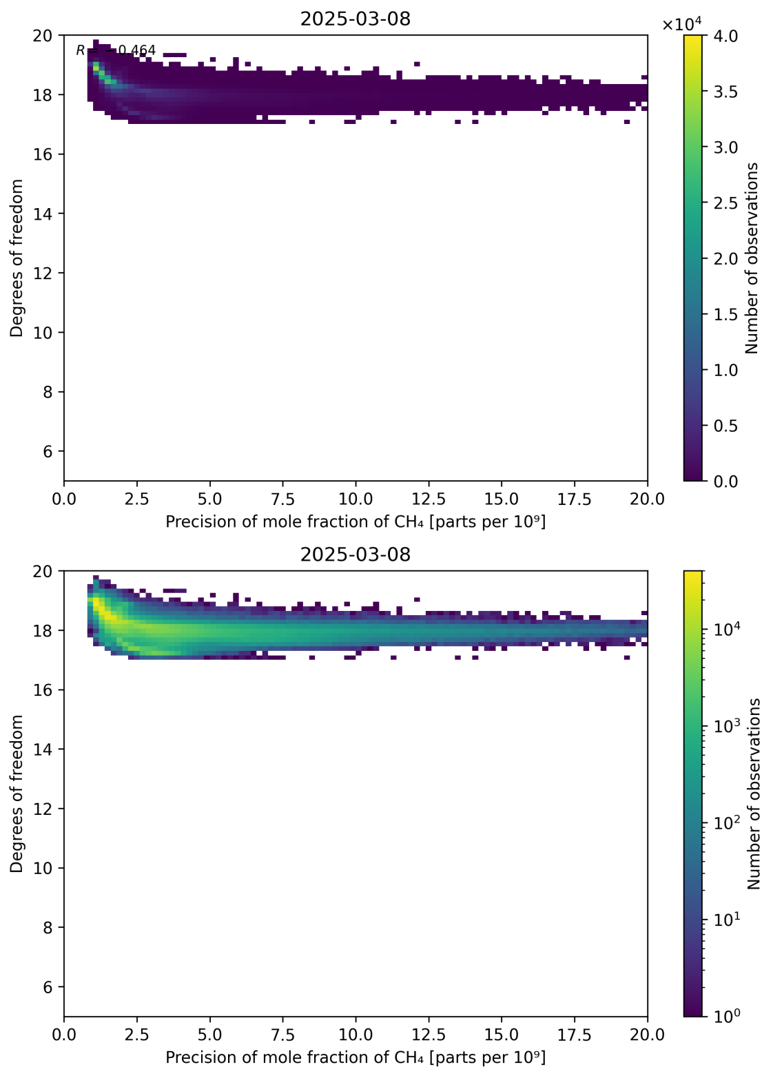
Figure 80: Scatter density plot of “Precision of mole fraction of CH 4 ” against “Degrees of freedom” for 2025-03-07 to 2025-03-09.
