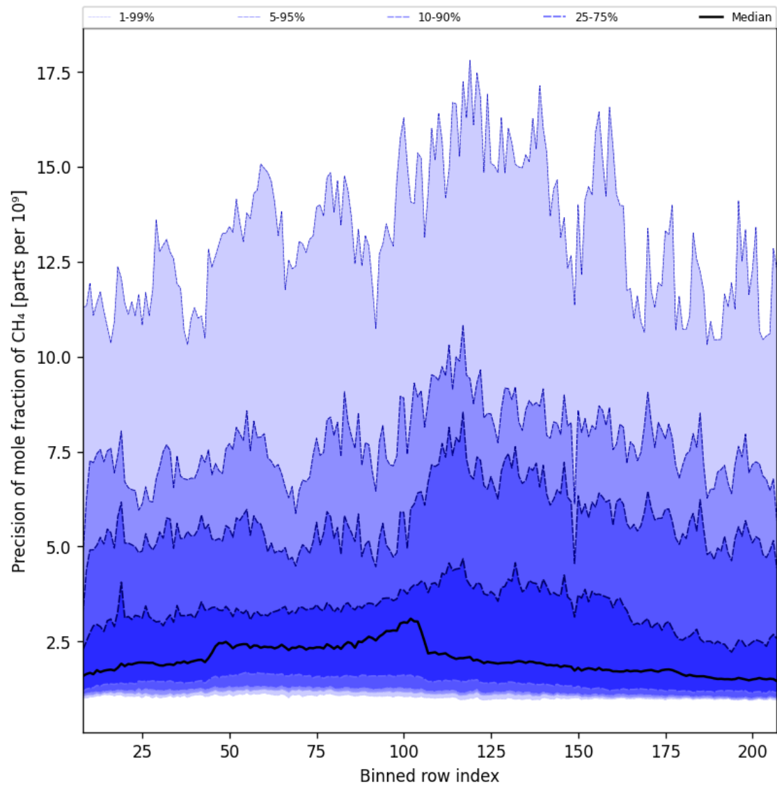
Figure 35: Along track statistics of “Precision of mole fraction of CH 4 ” for 2025-03-07 to 2025-03-09
