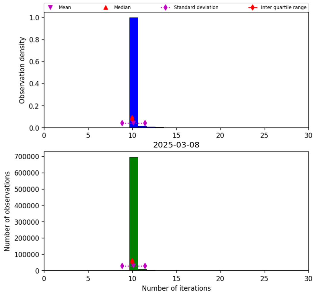
Figure 31: Histogram of “Number of iterations” for 2025-03-07 to 2025-03-09
