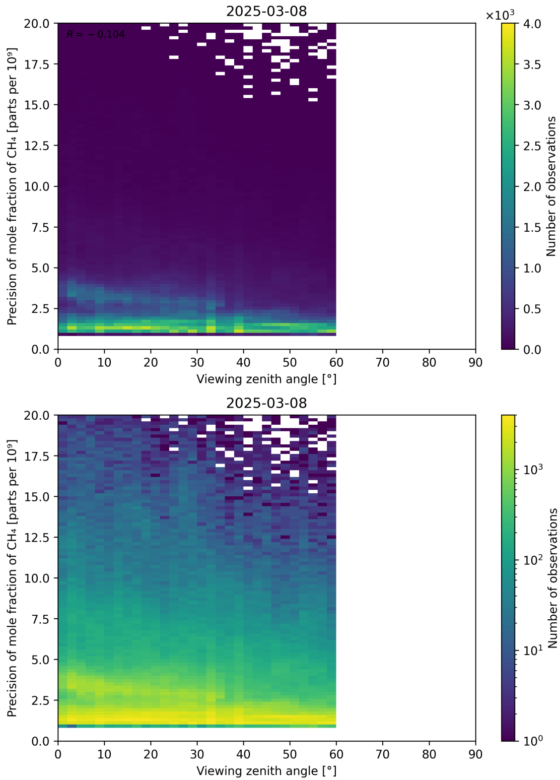
Figure 112: Scatter density plot of “Viewing zenith angle” against “Precision of mole fraction of CH 4 ” for 2025-03-07 to 2025-03-09.
