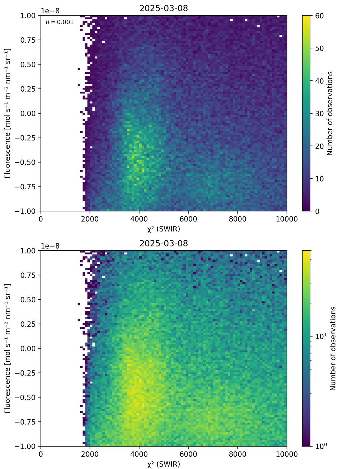
Figure 49: Scatter density plot of “ \chi^2 (SWIR)” against “Fluorescence” for 2025-03-07 to 2025-03-09.
