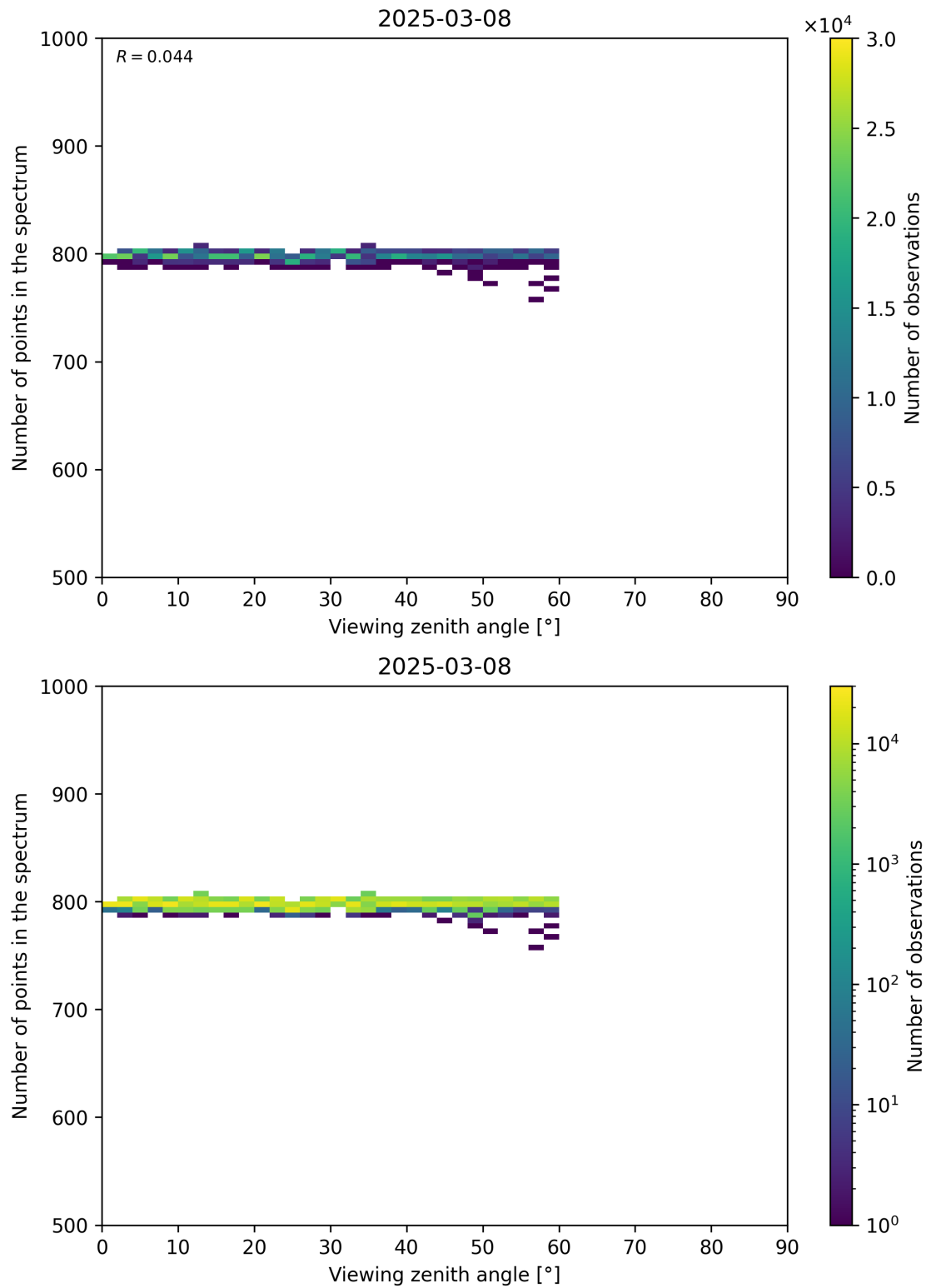
Figure 114: Scatter density plot of “Viewing zenith angle” against “Number of points in the spectrum” for 2025-03-07 to 2025-03-09.
