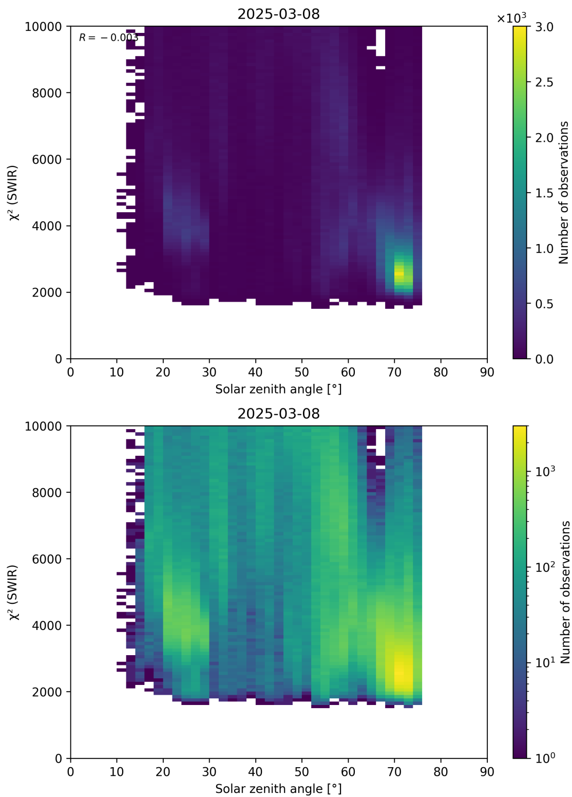
Figure 95: Scatter density plot of “Solar zenith angle” against “ \chi^2 (SWIR)” for 2025-03-07 to 2025-03-09.
