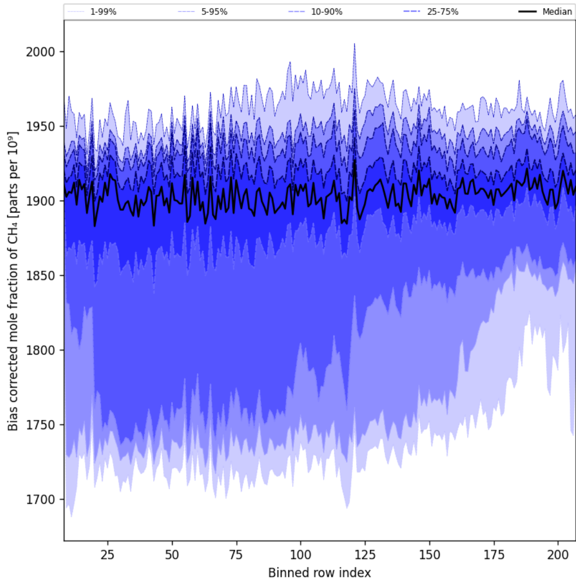
Figure 36: Along track statistics of “Bias corrected mole fraction of \text{CH}_4 ” for 2025-03-07 to 2025-03-09
