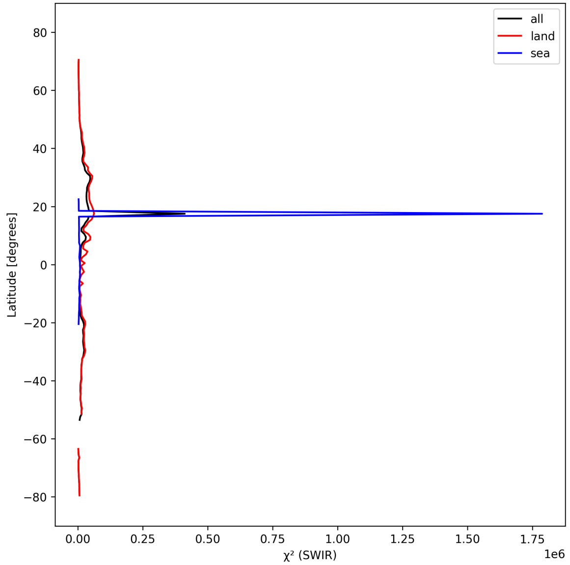
Figure 17: Zonal average of “ \chi^2 (SWIR)” for 2025-03-07 to 2025-03-09.
