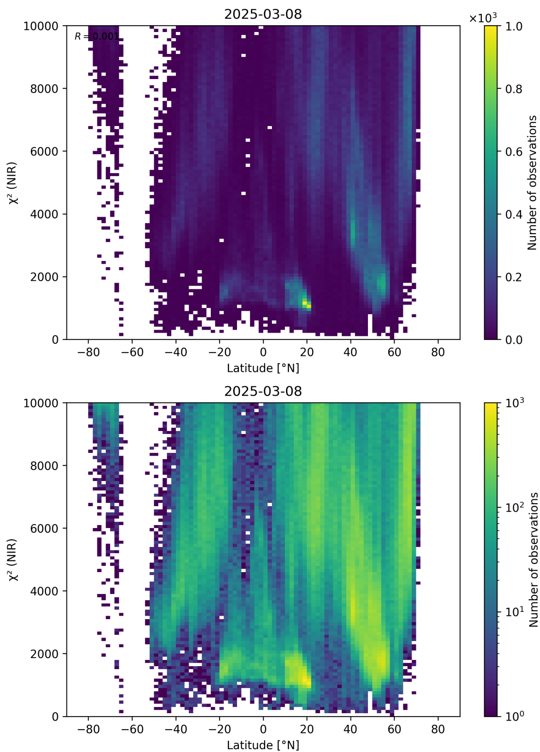
Figure 53: Scatter density plot of “Latitude” against “ \chi^2 (NIR)” for 2025-03-07 to 2025-03-09.
