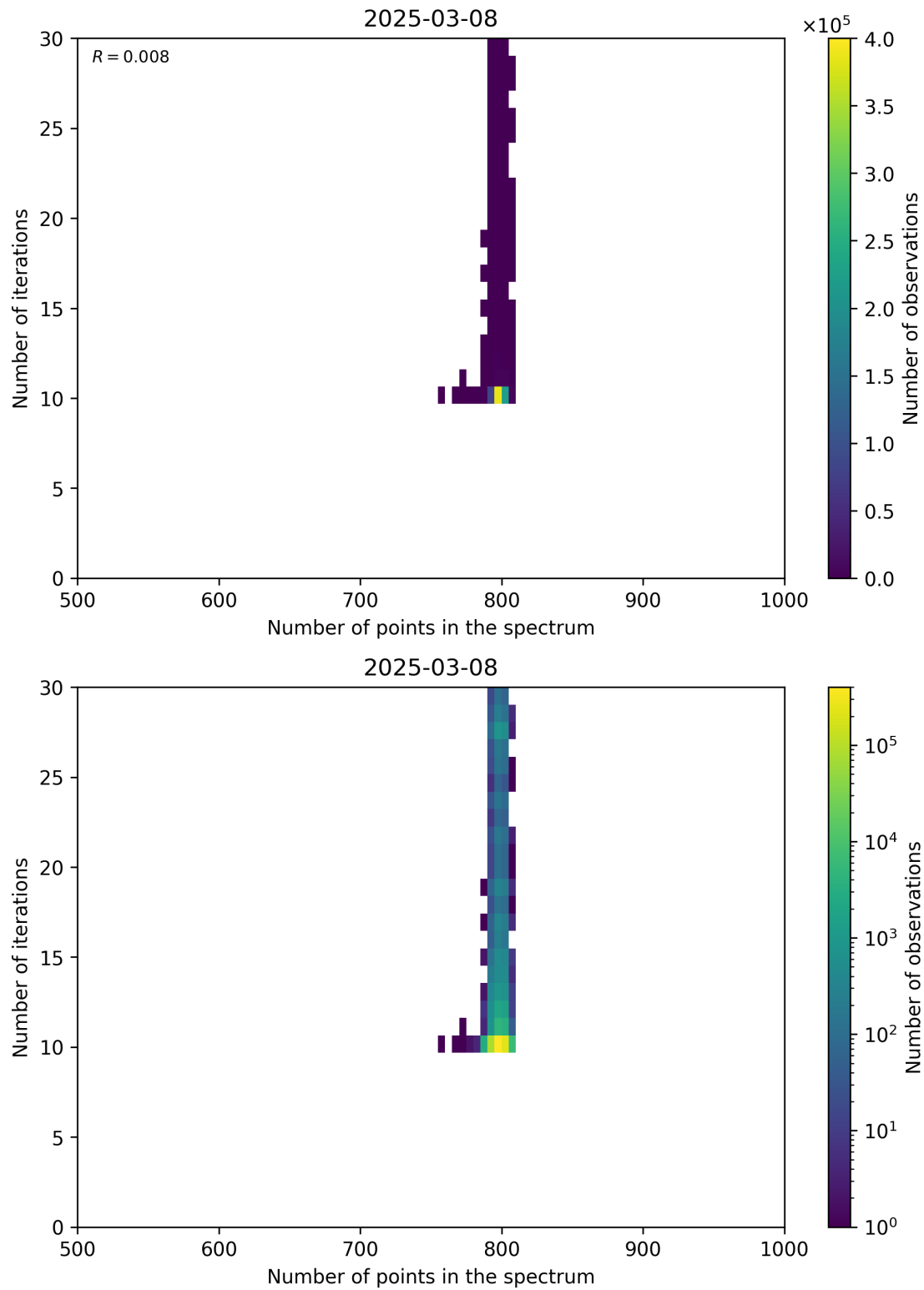
Figure 92: Scatter density plot of “Number of points in the spectrum” against “Number of iterations” for 2025-03-07 to 2025-03-09.
