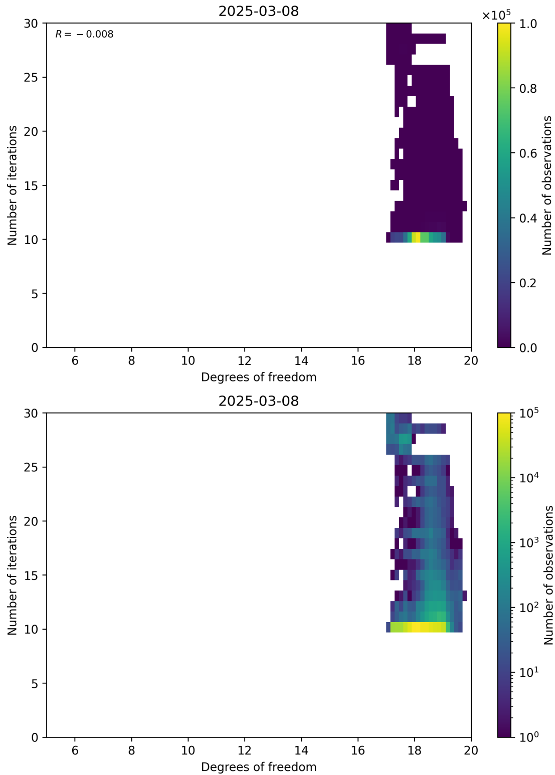
Figure 52: Scatter density plot of “Degrees of freedom” against “Number of iterations” for 2025-03-07 to 2025-03-09.
