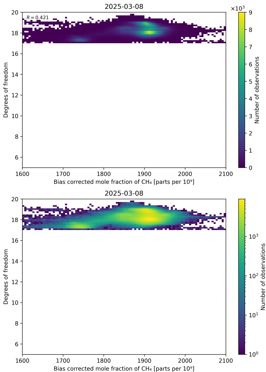
Figure 65: Scatter density plot of “Bias corrected mole fraction of CH 4 ” against “Degrees of freedom” for 2025-03-07 to 2025-03-09.
