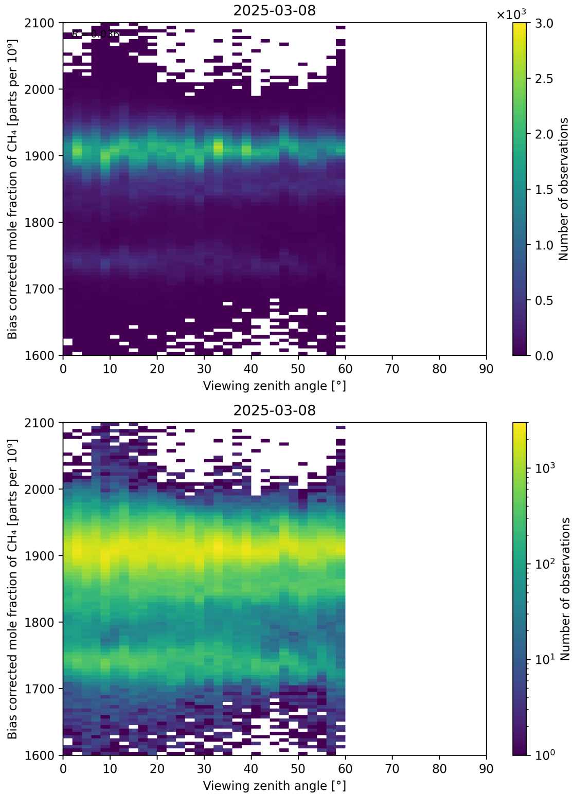
Figure 111: Scatter density plot of “Viewing zenith angle” against “Bias corrected mole fraction of CH 4 ” for 2025-03-07 to 2025-03-09.
