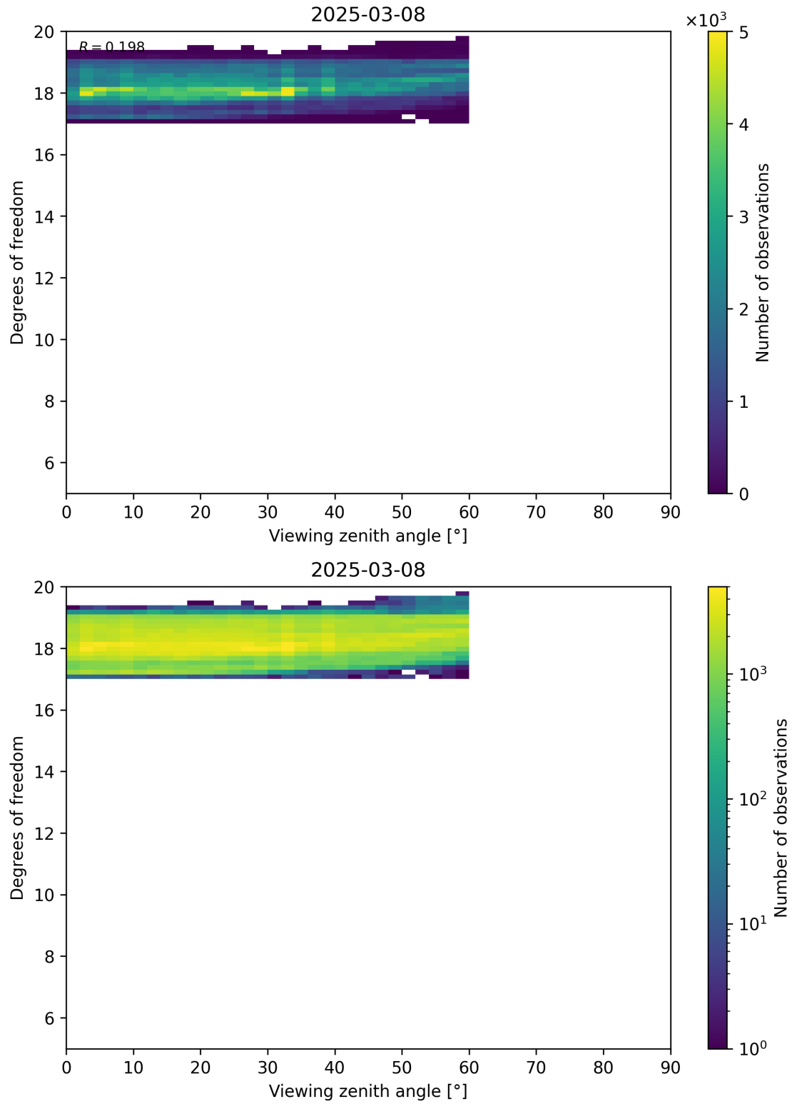
Figure 107: Scatter density plot of “Viewing zenith angle” against “Degrees of freedom” for 2025-03-07 to 2025-03-09.
