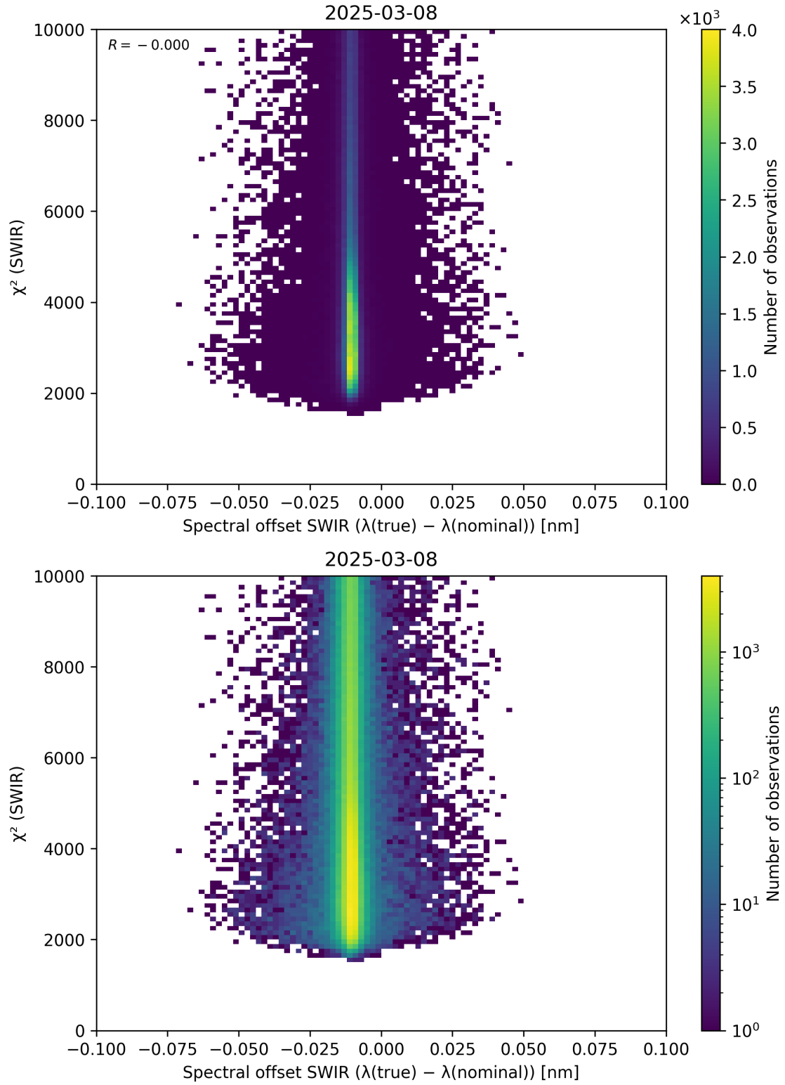
Figure 118: Scatter density plot of “Spectral offset SWIR ( \lambda_{\text{true}} - \lambda_{\text{nominal}} )” against “ \chi^2 (SWIR)” for 2025-03-07 to 2025-03-09.
