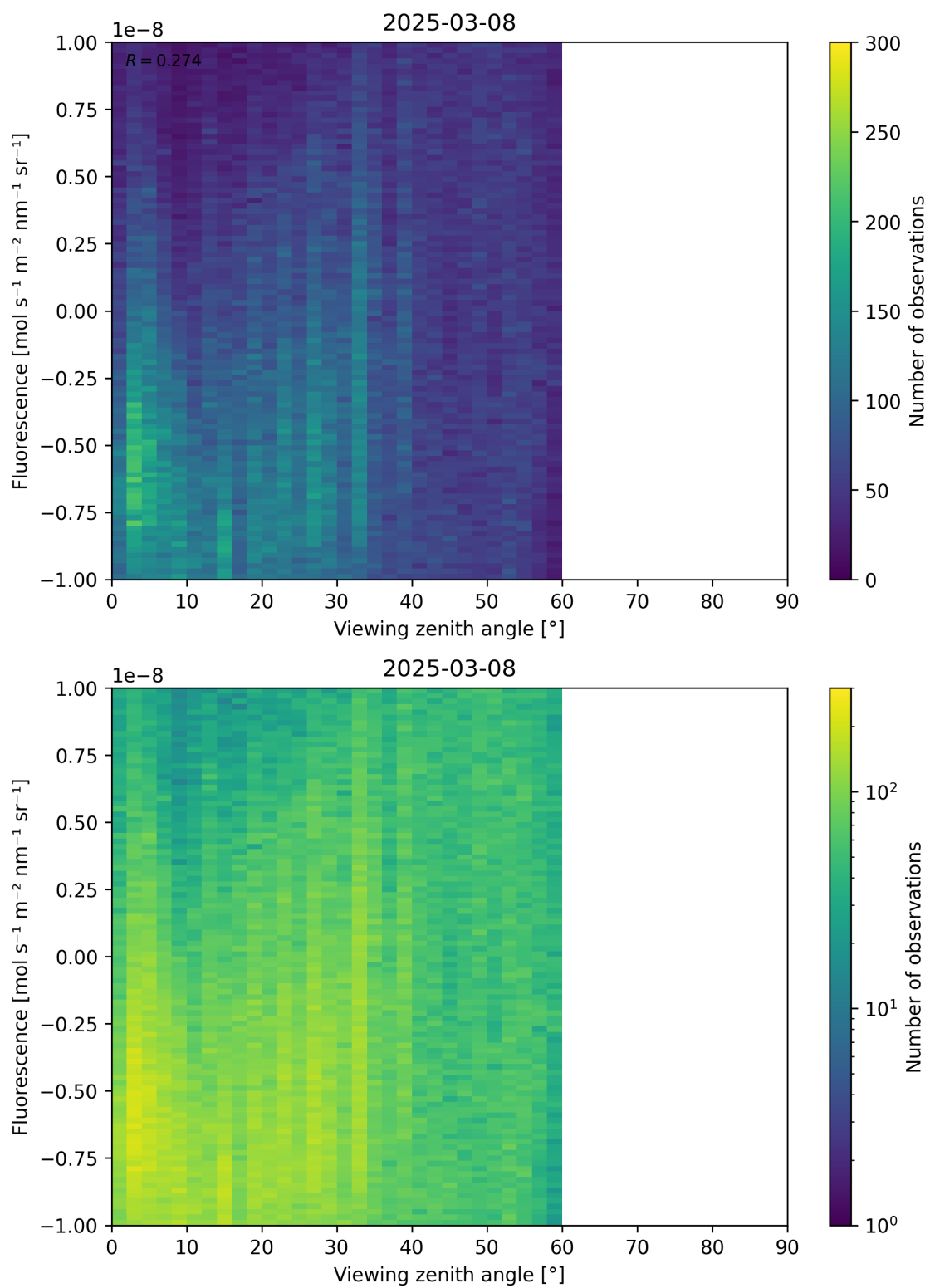
Figure 108: Scatter density plot of “Viewing zenith angle” against “Fluorescence” for 2025-03-07 to 2025-03-09.
