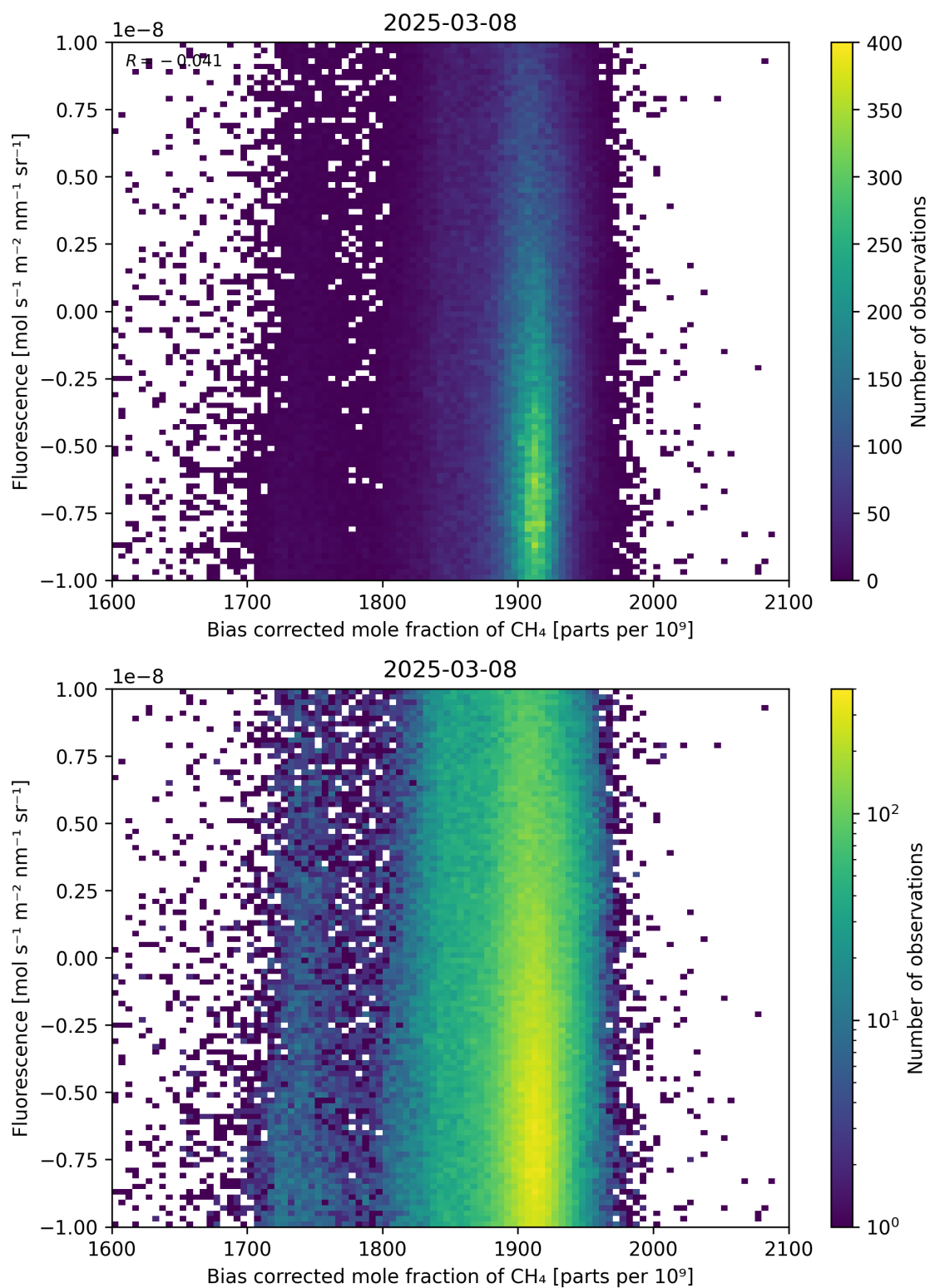
Figure 66: Scatter density plot of “Bias corrected mole fraction of \text{CH}_4 ” against “Fluorescence” for 2025-03-07 to 2025-03-09.
