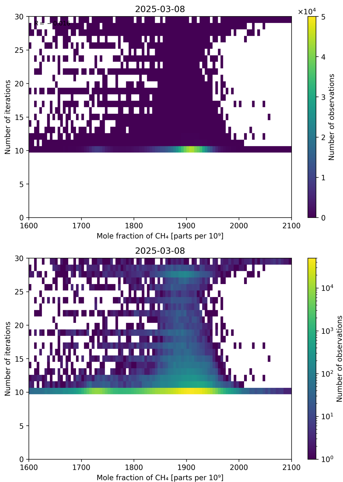
Figure 76: Scatter density plot of “Mole fraction of CH 4 ” against “Number of iterations” for 2025-03-07 to 2025-03-09.
