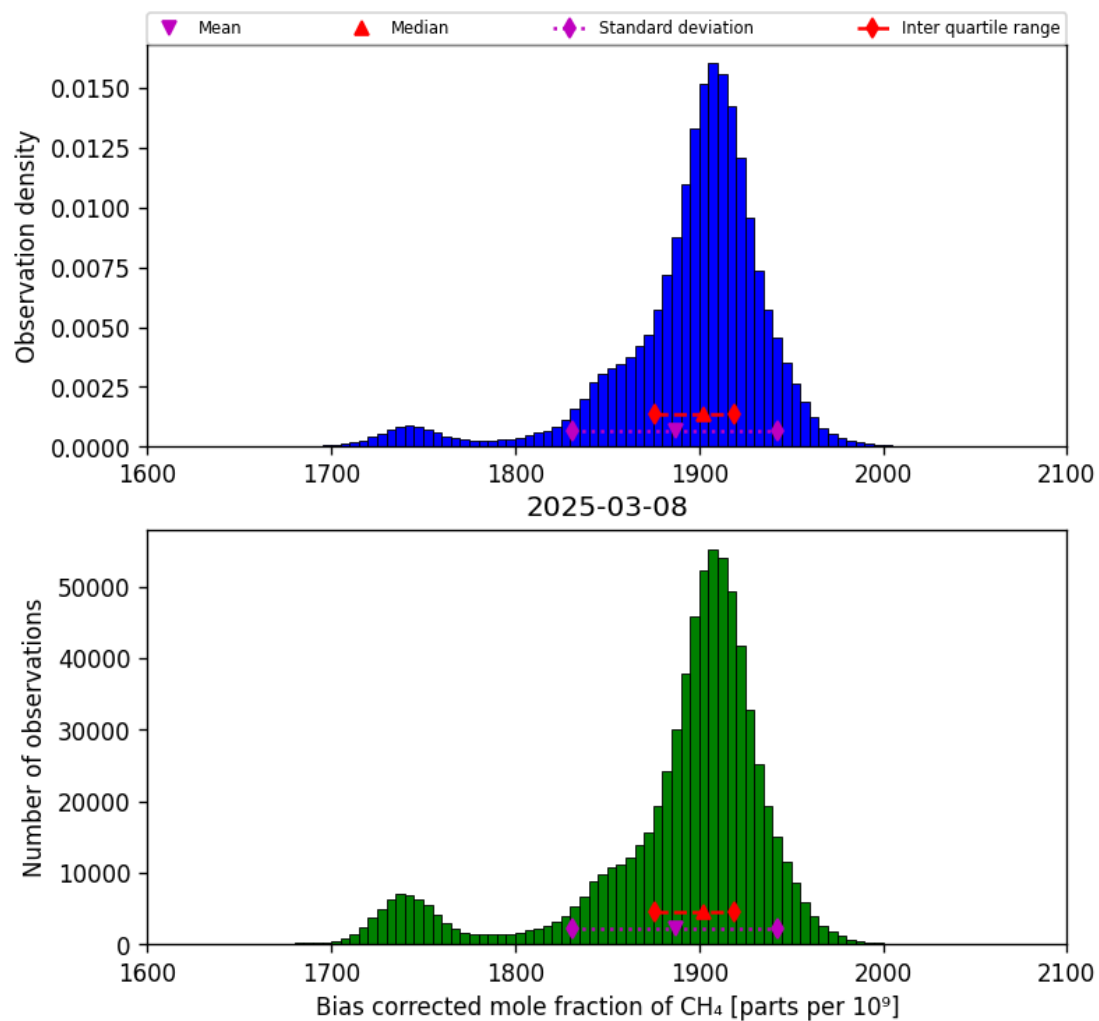
Figure 25: Histogram of “Bias corrected mole fraction of CH 4 ” for 2025-03-07 to 2025-03-09
