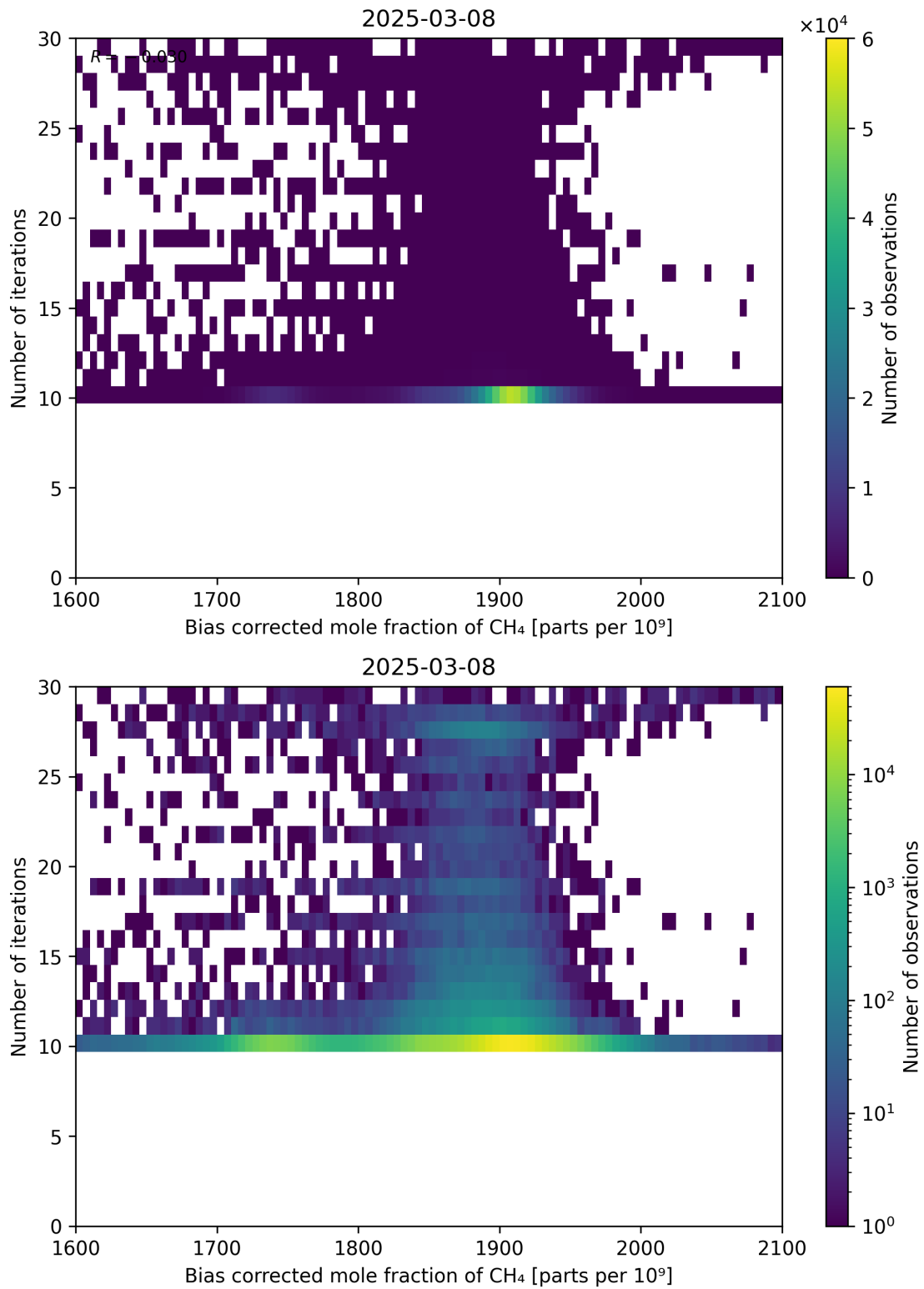
Figure 67: Scatter density plot of “Bias corrected mole fraction of \text{CH}_4 ” against “Number of iterations” for 2025-03-07 to 2025-03-09.
