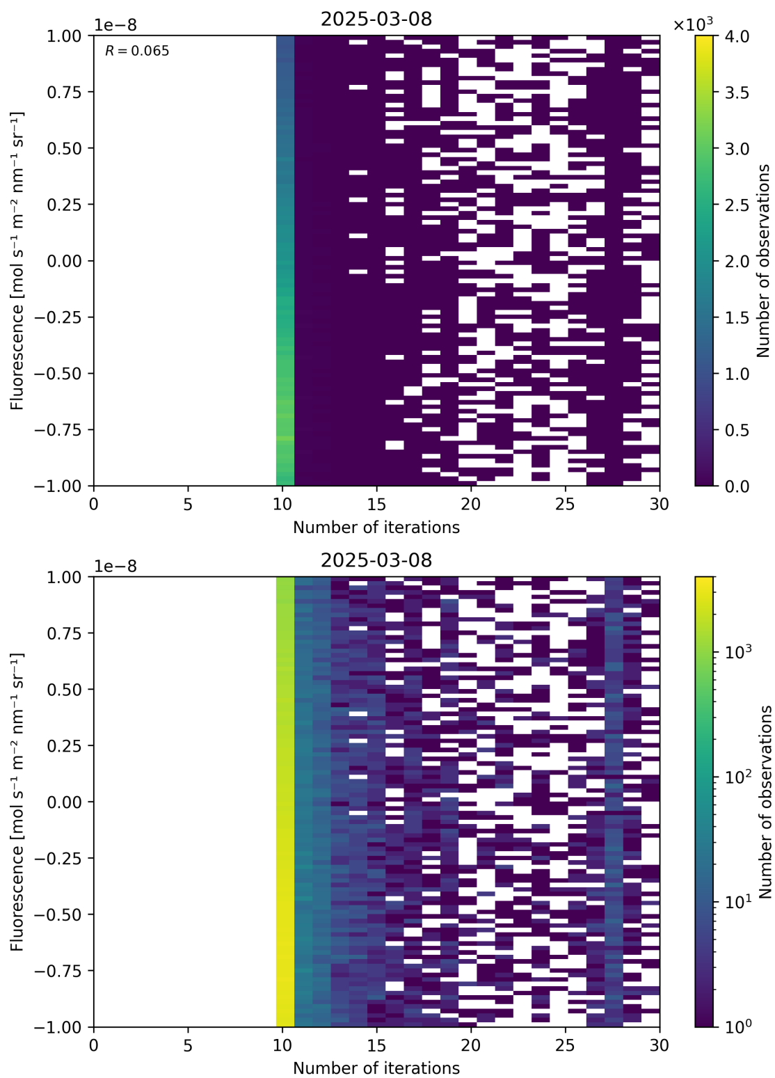
Figure 87: Scatter density plot of “Number of iterations” against “Fluorescence” for 2025-03-07 to 2025-03-09.
