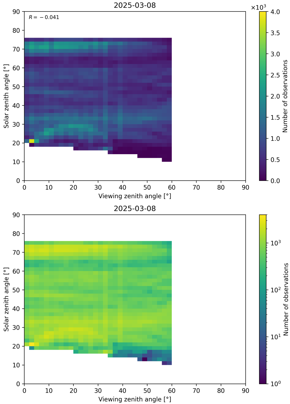
Figure 115: Scatter density plot of “Viewing zenith angle” against “Solar zenith angle” for 2025-03-07 to 2025-03-09.
