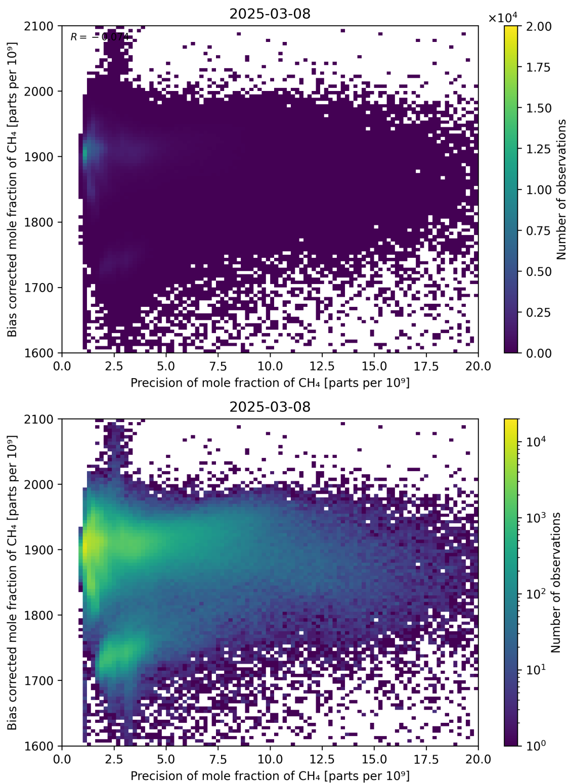
Figure 82: Scatter density plot of “Precision of mole fraction of CH 4 ” against “Bias corrected mole fraction of CH 4 ” for 2025-03-07 to 2025-03-09.
