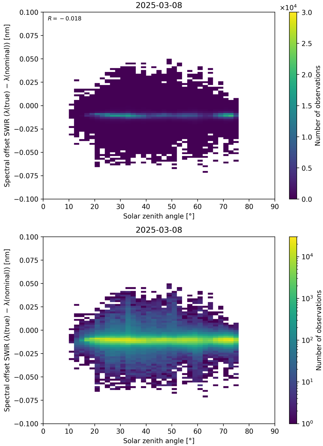
Figure 104: Scatter density plot of “Solar zenith angle” against “Spectral offset SWIR ( \lambda_{\text{true}} - \lambda_{\text{nominal}} )” for 2025-03-07 to 2025-03-09.
