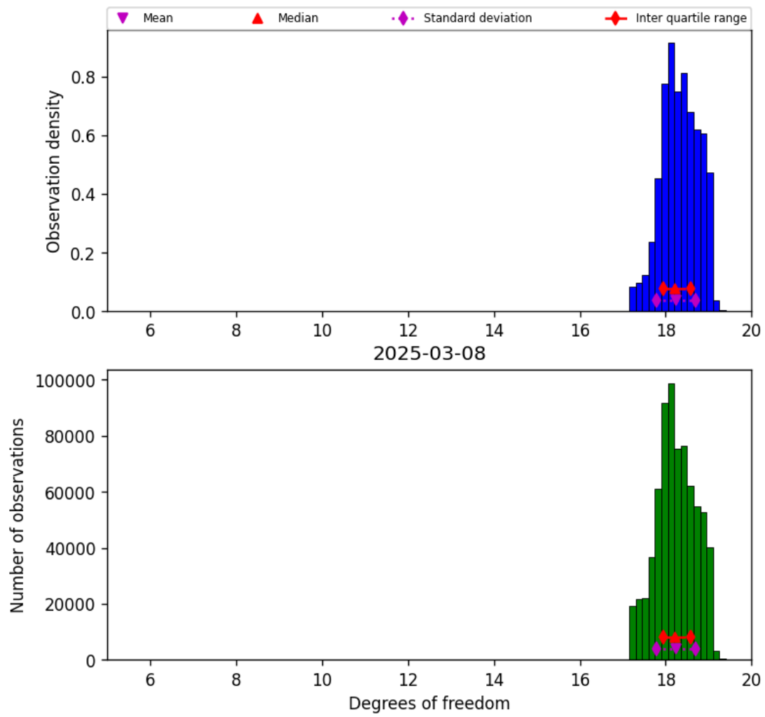
Figure 30: Histogram of “Degrees of freedom” for 2025-03-07 to 2025-03-09
