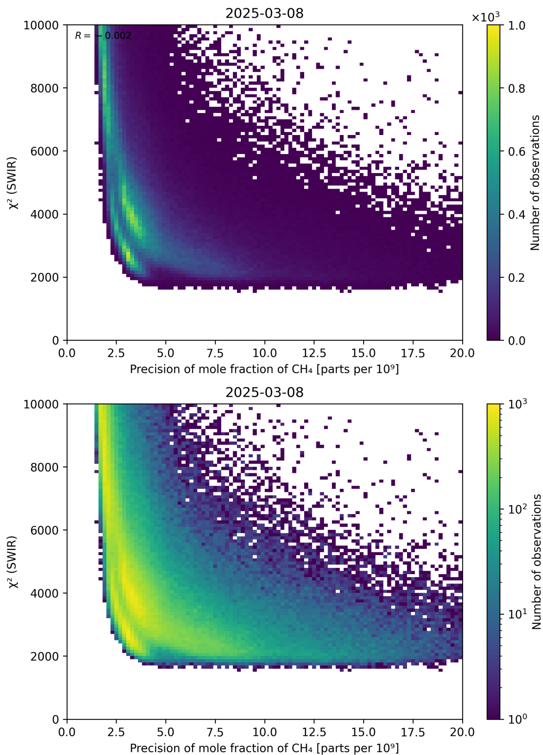
Figure 79: Scatter density plot of “Precision of mole fraction of \text{CH}_4 ” against “ \chi^2 (SWIR)” for 2025-03-07 to 2025-03-09.
