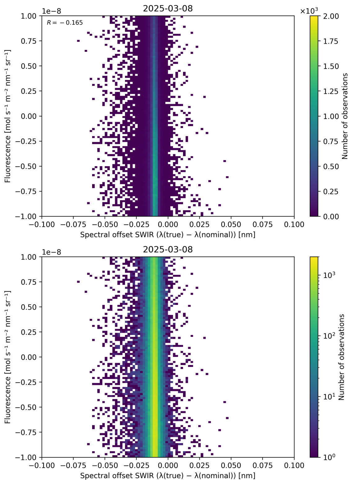
Figure 120: Scatter density plot of “Spectral offset SWIR ( \lambda_{\text{true}} - \lambda_{\text{nominal}} )” against “Fluorescence” for 2025-03-07 to 2025-03-09.
