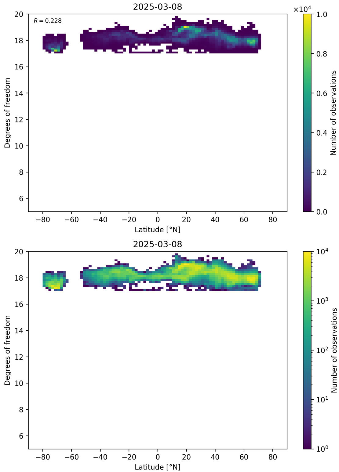
Figure 55: Scatter density plot of “Latitude” against “Degrees of freedom” for 2025-03-07 to 2025-03-09.
