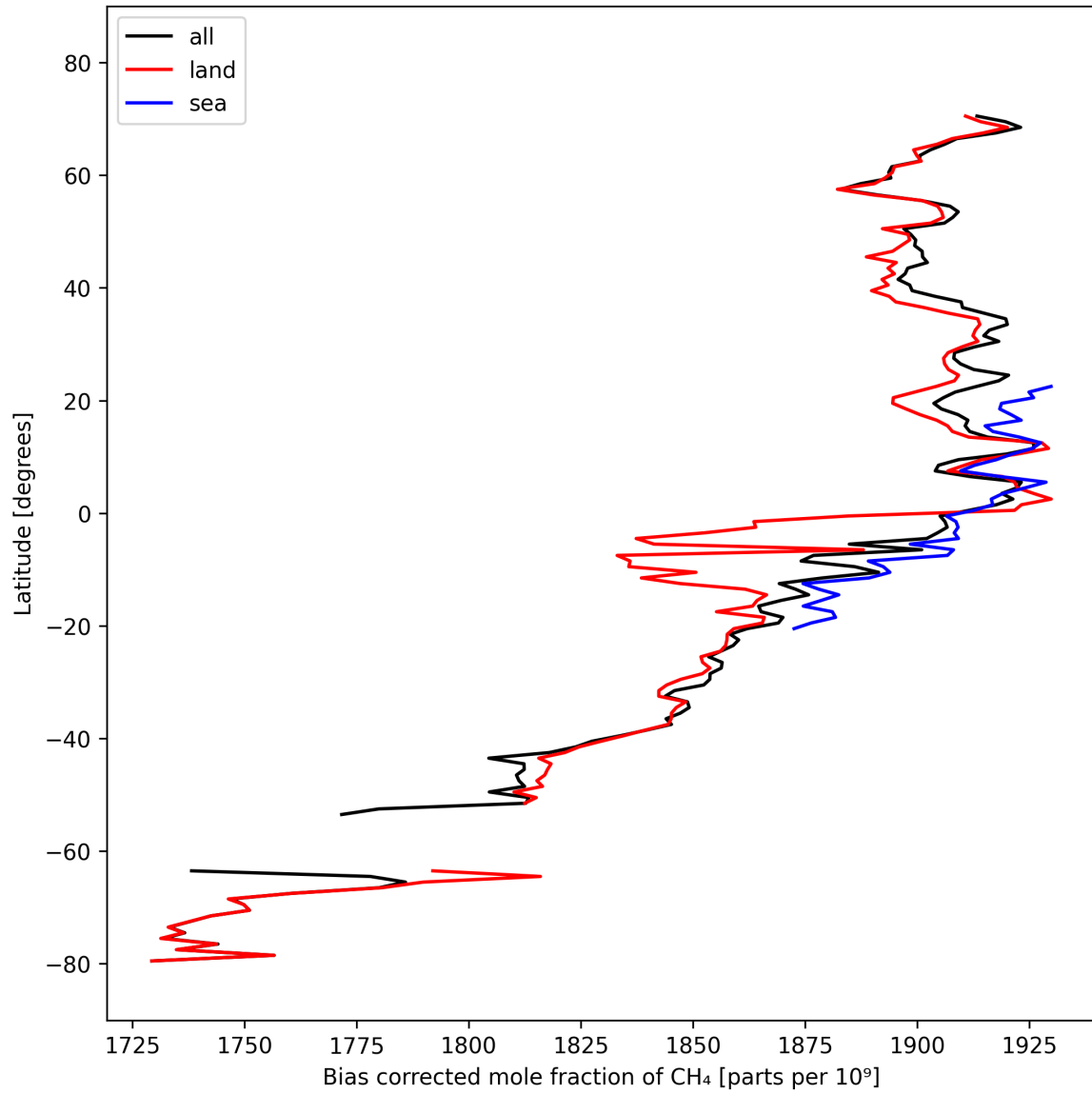
Figure 14: Zonal average of “Bias corrected mole fraction of CH 4 ” for 2025-03-07 to 2025-03-09.
