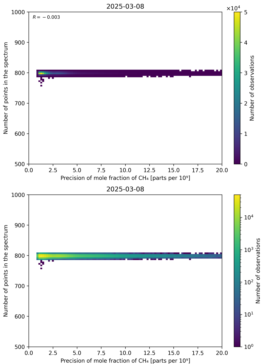
Figure 84: Scatter density plot of “Precision of mole fraction of CH 4 ” against “Number of points in the spectrum” for 2025-03-07 to 2025-03-09.
