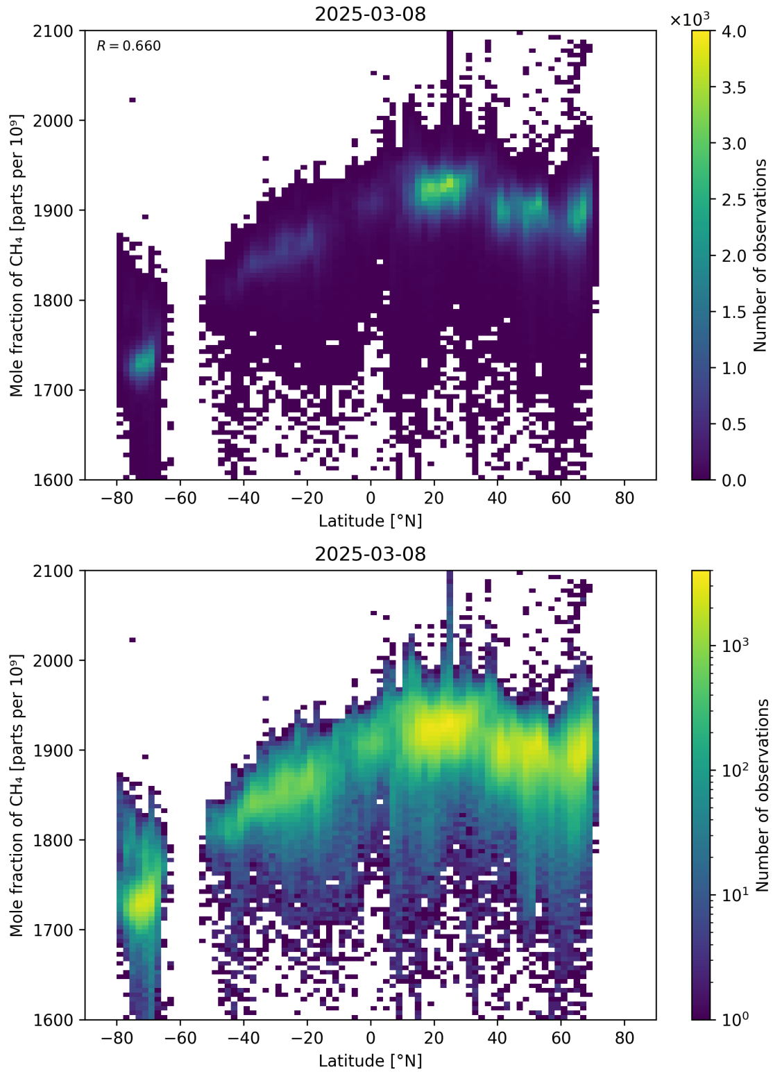
Figure 57: Scatter density plot of “Latitude” against “Mole fraction of CH 4 ” for 2025-03-07 to 2025-03-09.
