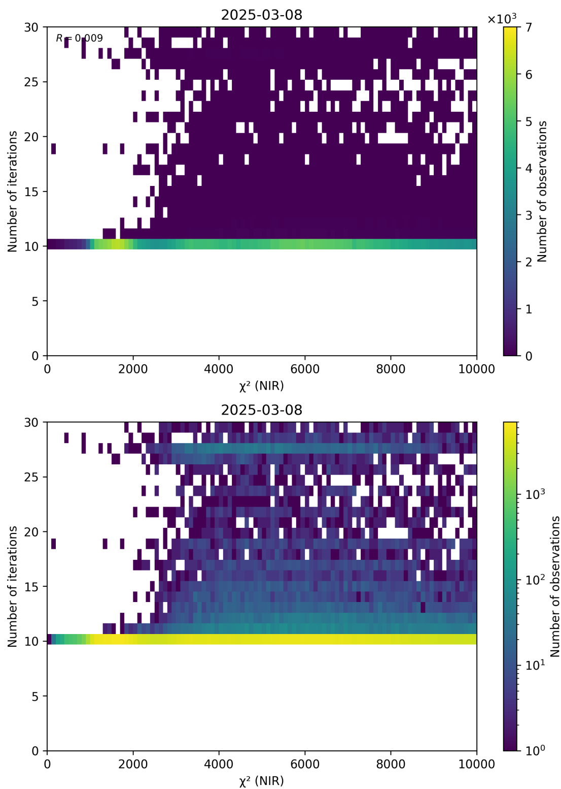
Figure 46: Scatter density plot of “ \chi^2 (NIR)” against “Number of iterations” for 2025-03-07 to 2025-03-09.
