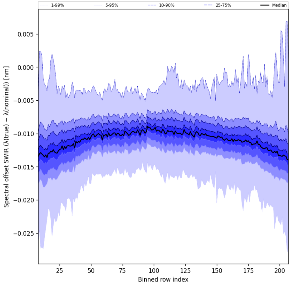
Figure 38: Along track statistics of “Spectral offset SWIR ( \lambda_{\text{true}} - \lambda_{\text{nominal}} )” for 2025-03-07 to 2025-03-09
