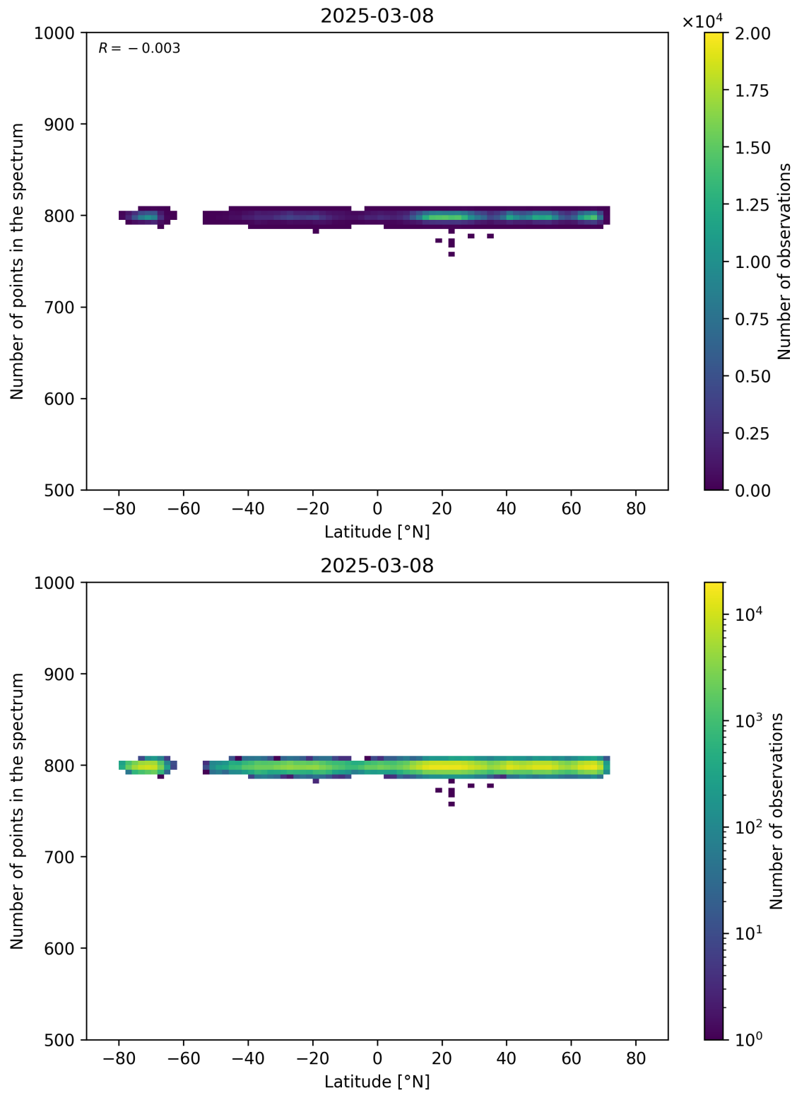
Figure 61: Scatter density plot of “Latitude” against “Number of points in the spectrum” for 2025-03-07 to 2025-03-09.
