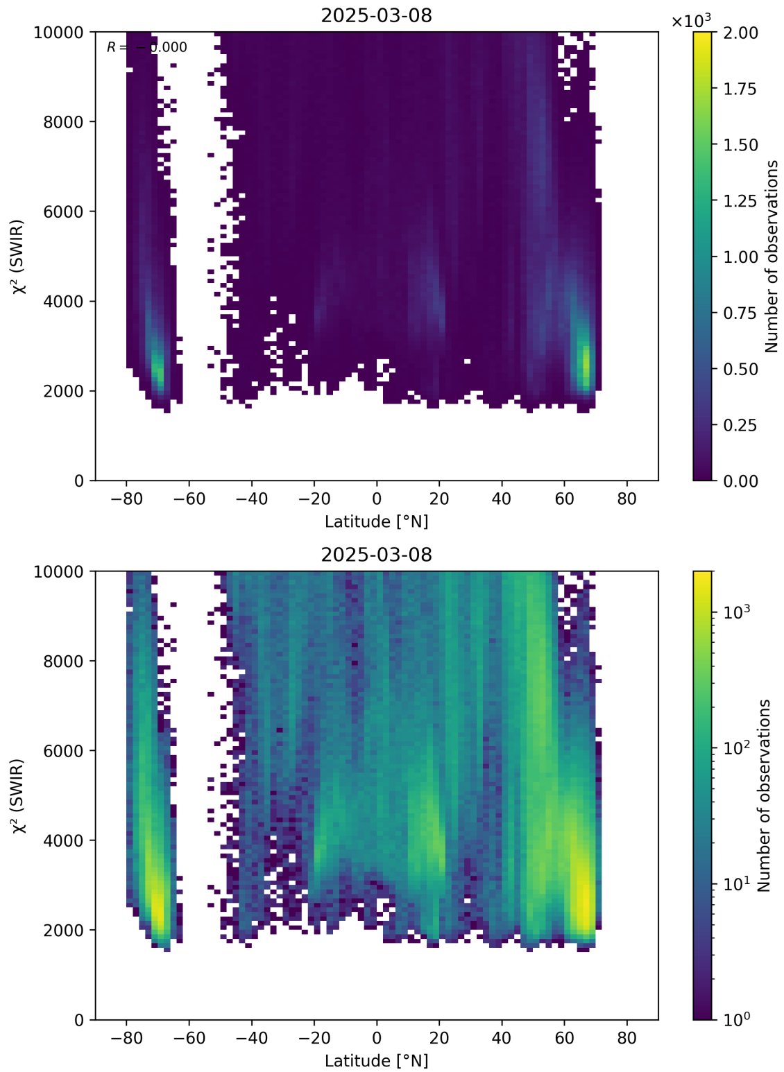
Figure 54: Scatter density plot of “Latitude” against “ \chi^2 (SWIR)” for 2025-03-07 to 2025-03-09.
