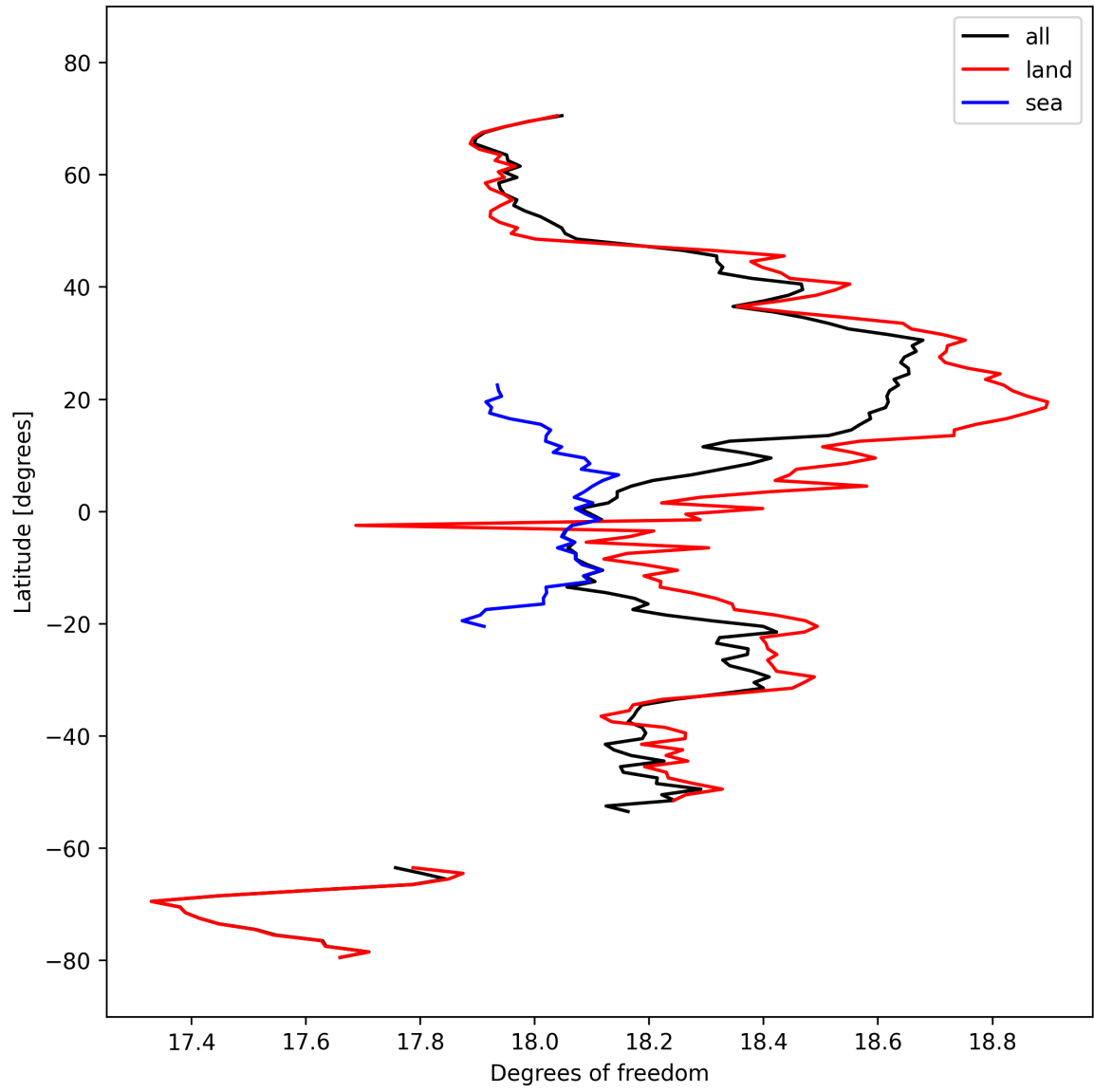
Figure 19: Zonal average of “Degrees of freedom” for 2025-03-07 to 2025-03-09.
