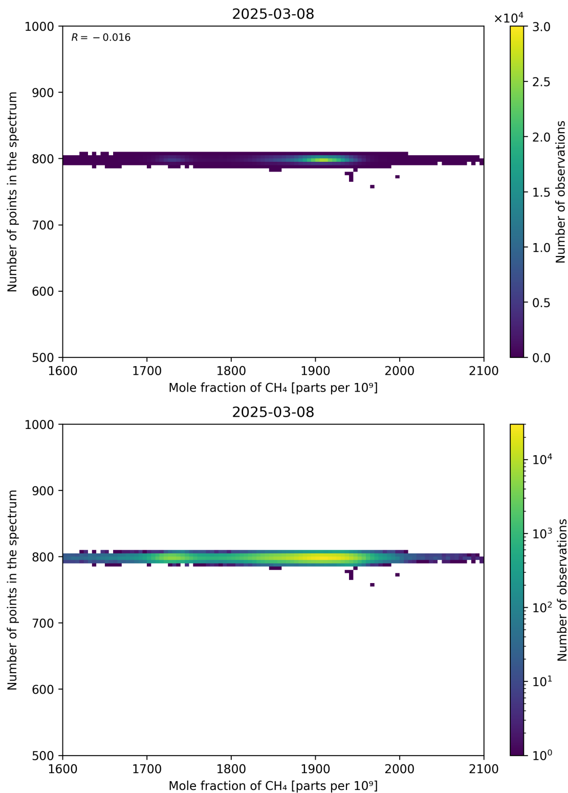
Figure 77: Scatter density plot of “Mole fraction of CH 4 ” against “Number of points in the spectrum” for 2025-03-07 to 2025-03-09.
