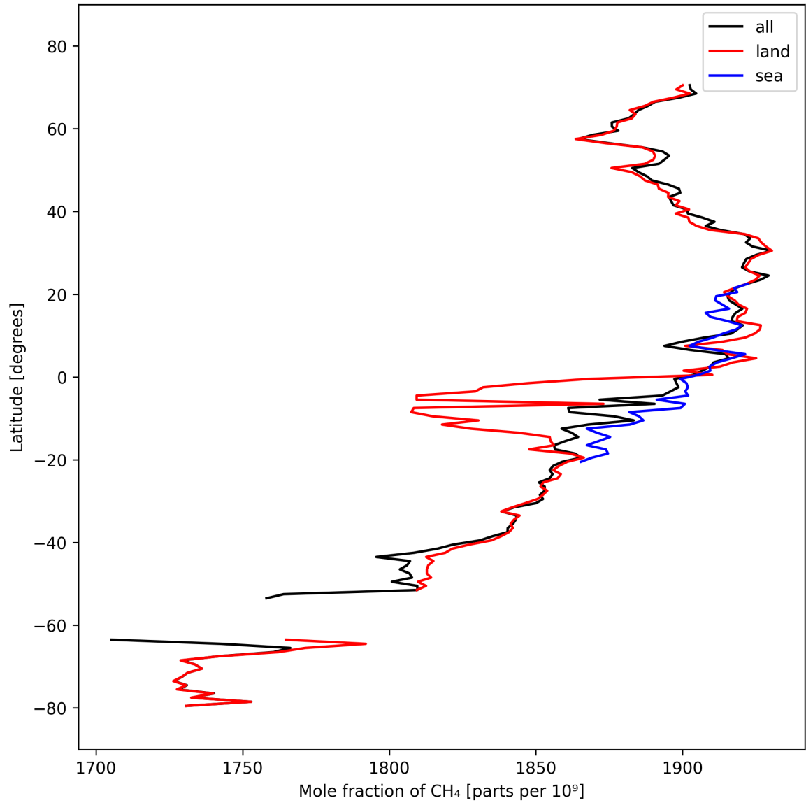
Figure 12: Zonal average of “Mole fraction of \text{CH}_4 ” for 2025-03-07 to 2025-03-09.
