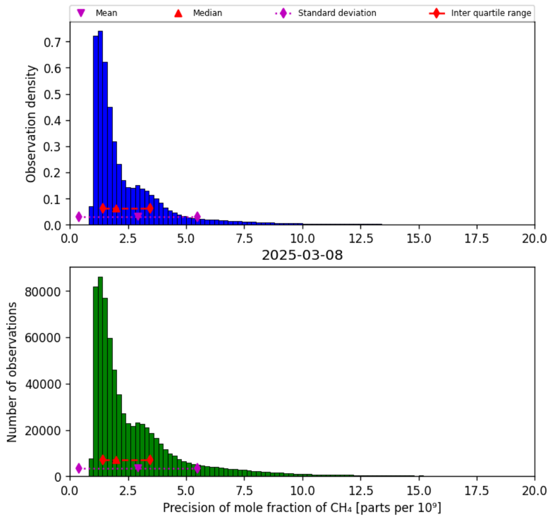
Figure 24: Histogram of “Precision of mole fraction of CH 4 ” for 2025-03-07 to 2025-03-09
