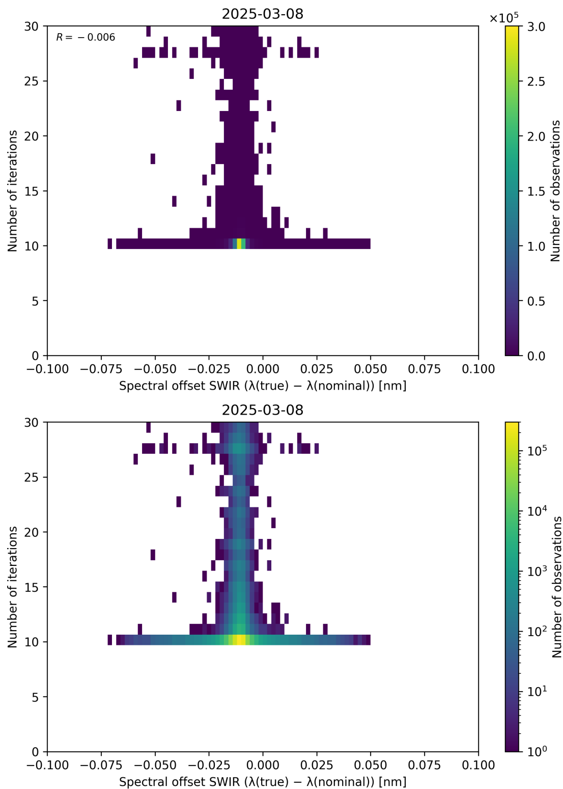
Figure 121: Scatter density plot of “Spectral offset SWIR ( \lambda_{\text{true}} - \lambda_{\text{nominal}} )” against “Number of iterations” for 2025-03-07 to 2025-03-09.
