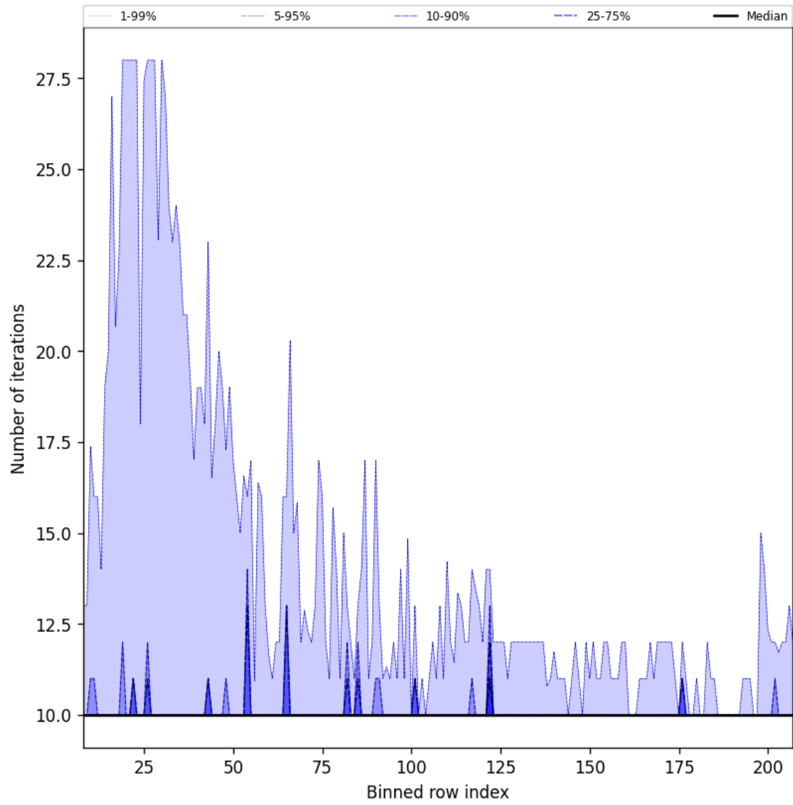
Figure 42: Along track statistics of “Number of iterations” for 2025-03-07 to 2025-03-09
