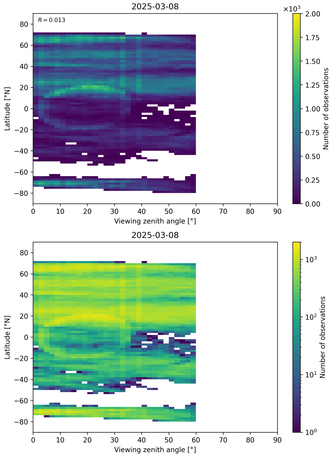
Figure 109: Scatter density plot of “Viewing zenith angle” against “Latitude” for 2025-03-07 to 2025-03-09.
