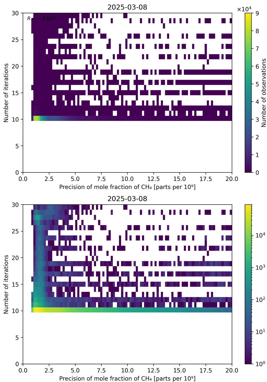
Figure 83: Scatter density plot of “Precision of mole fraction of CH 4 ” against “Number of iterations” for 2025-03-07 to 2025-03-09.
