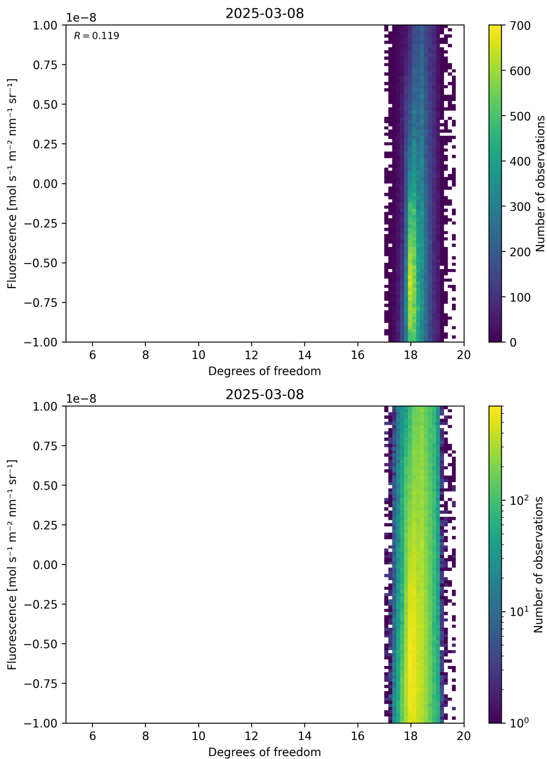
Figure 51: Scatter density plot of “Degrees of freedom” against “Fluorescence” for 2025-03-07 to 2025-03-09.
