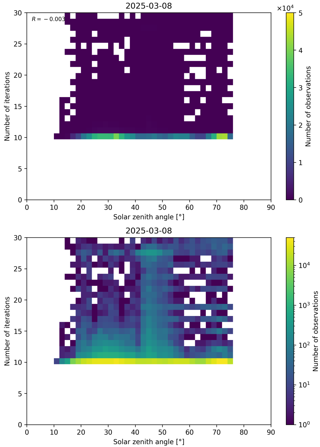
Figure 102: Scatter density plot of “Solar zenith angle” against “Number of iterations” for 2025-03-07 to 2025-03-09.
