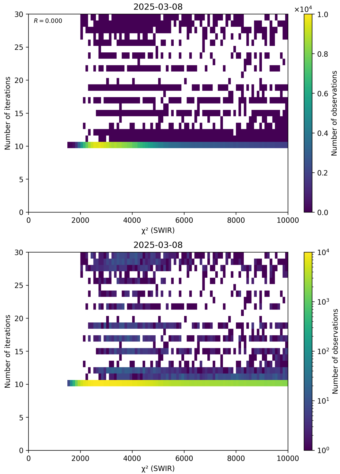
Figure 50: Scatter density plot of “ \chi^2 (SWIR)” against “Number of iterations” for 2025-03-07 to 2025-03-09.
