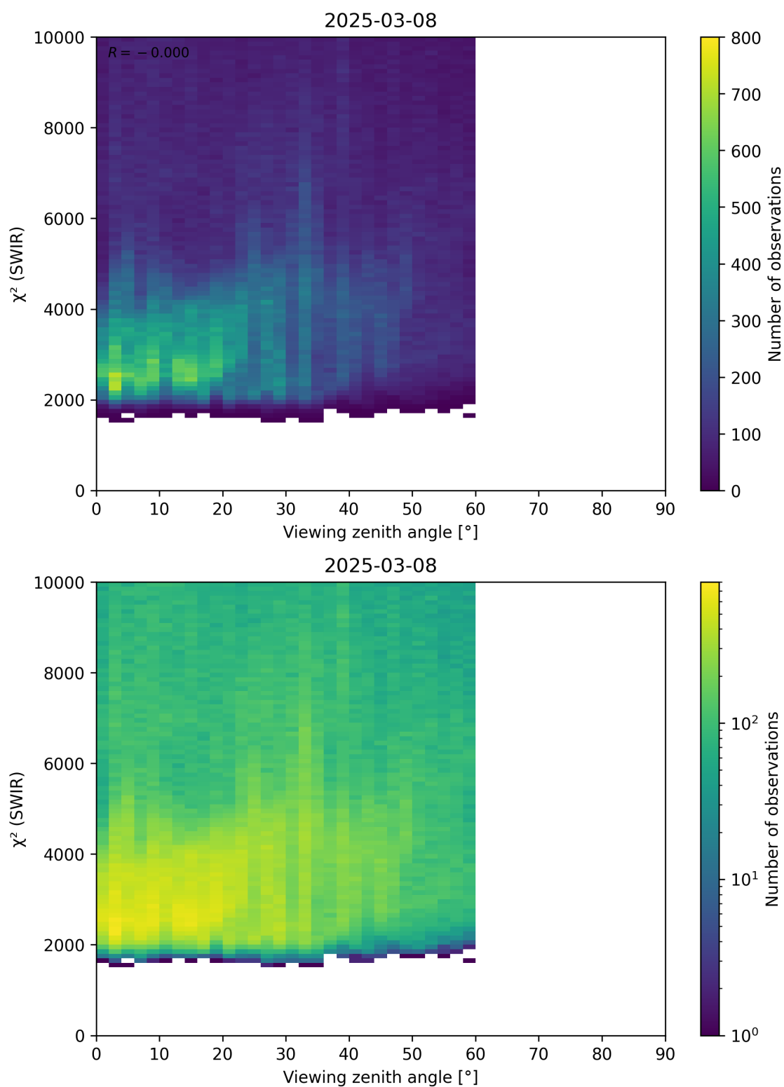
Figure 106: Scatter density plot of “Viewing zenith angle” against “ \chi^2 (SWIR)” for 2025-03-07 to 2025-03-09.
