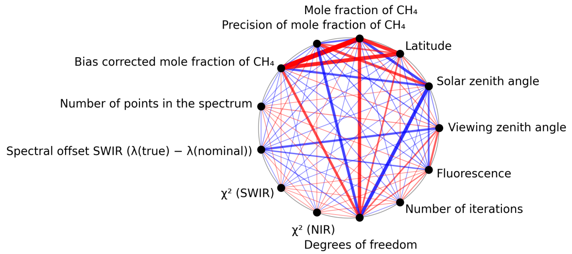
Figure 1: Map of correlation graph for 2025-03-07 to 2025-03-09.
