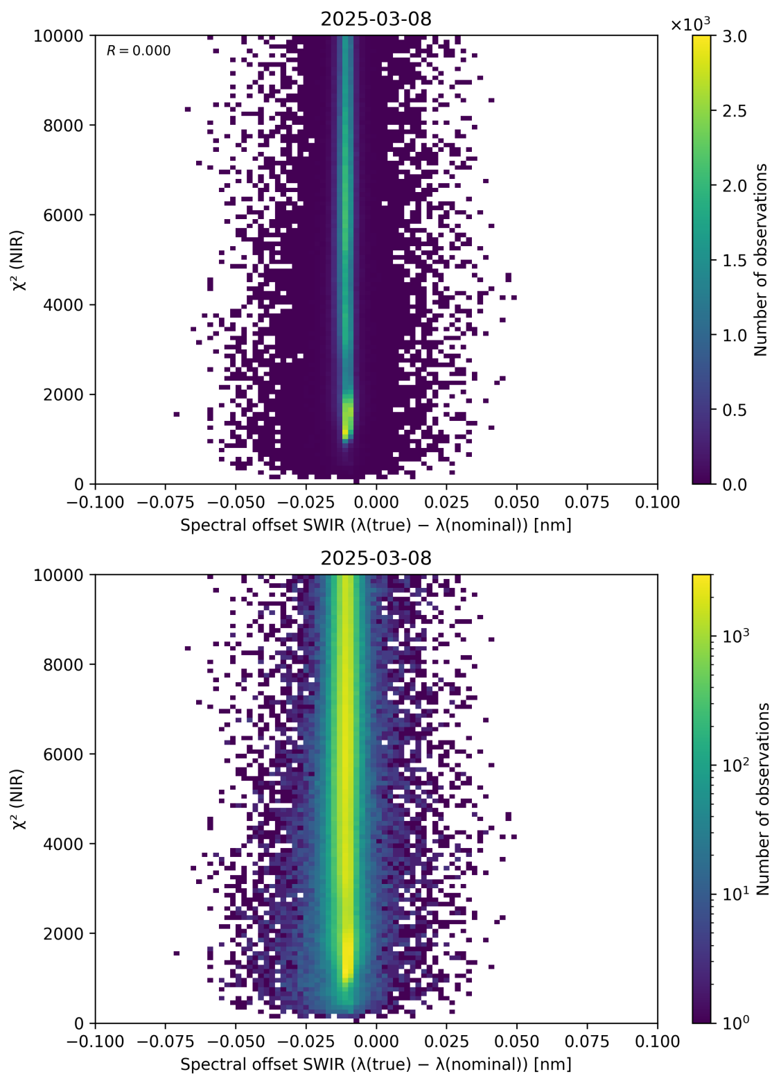
Figure 117: Scatter density plot of “Spectral offset SWIR ( \lambda_{\text{true}} - \lambda_{\text{nominal}} )” against “ \chi^2 (NIR)” for 2025-03-07 to 2025-03-09.
