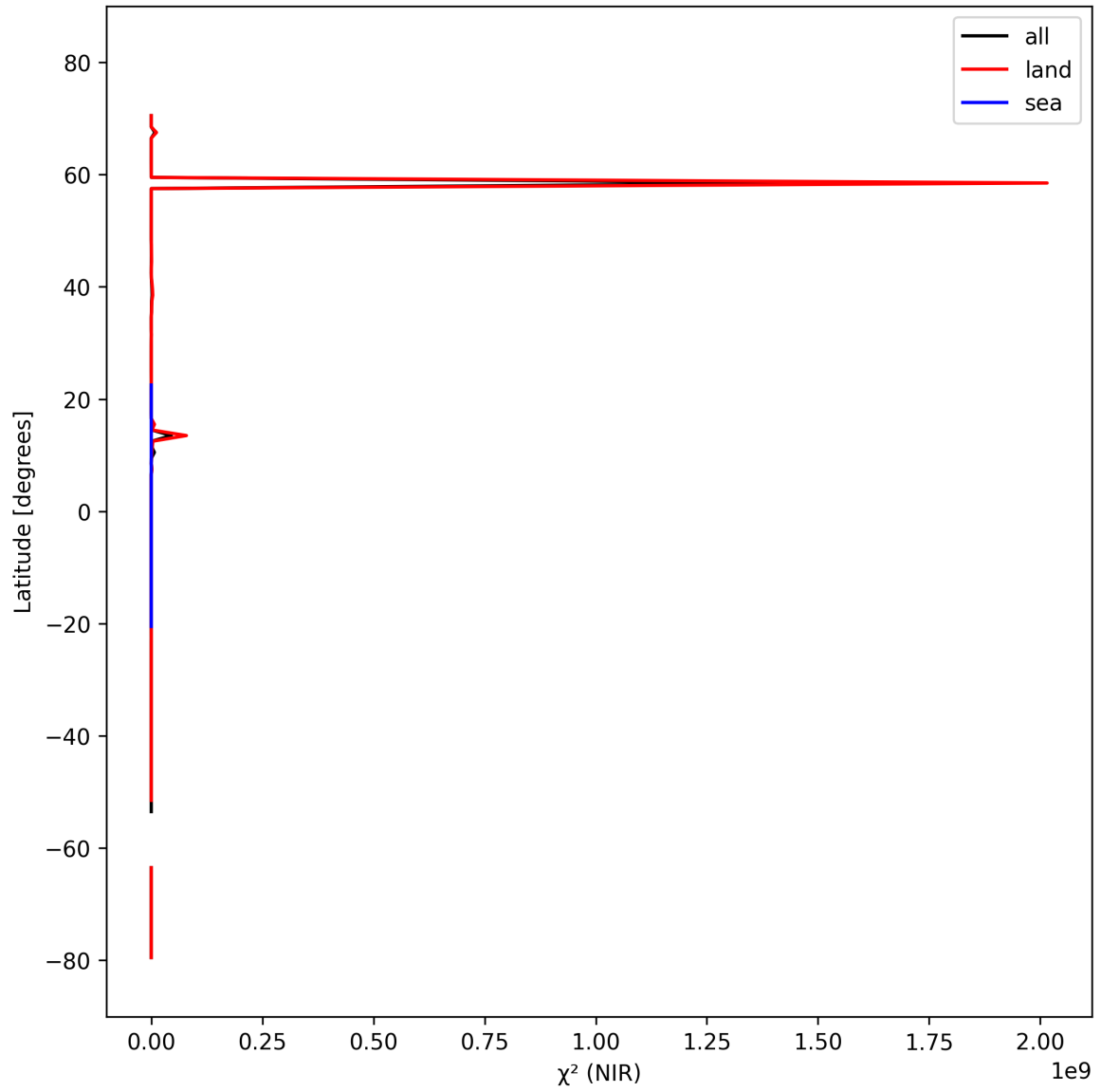
Figure 18: Zonal average of “ \chi^2 (NIR)” for 2025-03-07 to 2025-03-09.
