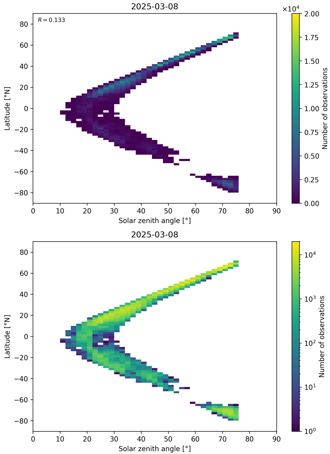
Figure 98: Scatter density plot of “Solar zenith angle” against “Latitude” for 2025-03-07 to 2025-03-09.
