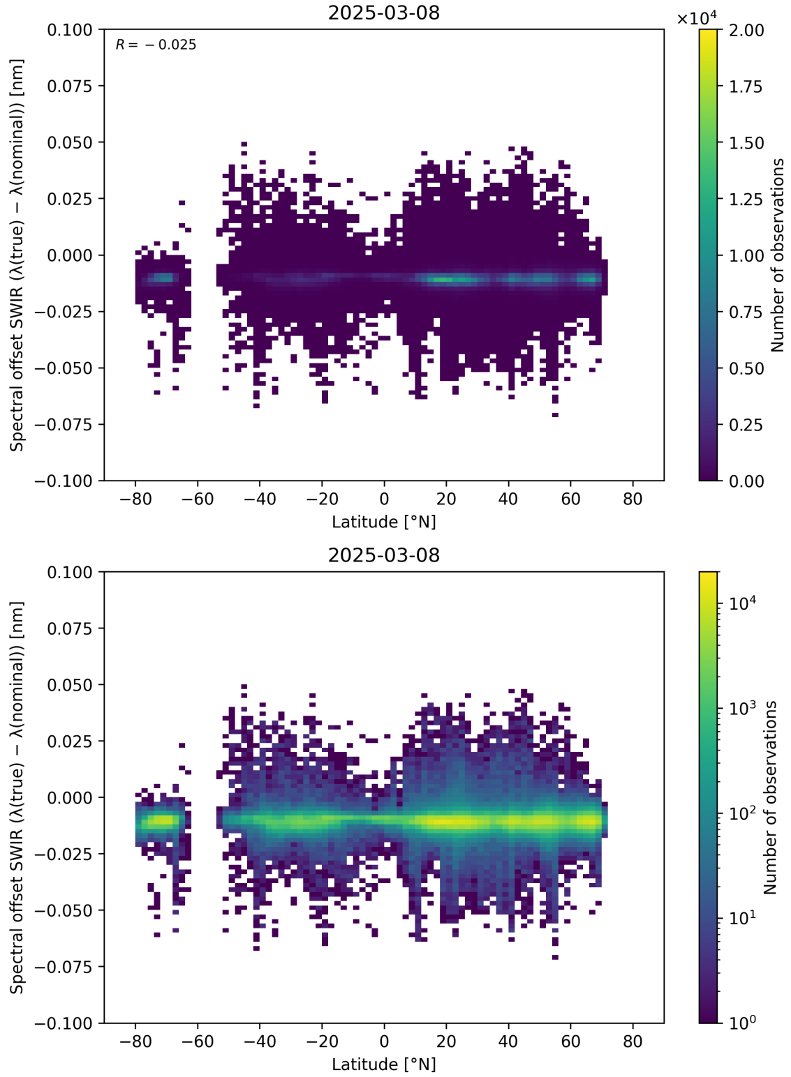
Figure 62: Scatter density plot of “Latitude” against “Spectral offset SWIR ( \lambda_{\text{true}} - \lambda_{\text{nominal}} )” for 2025-03-07 to 2025-03-09.
