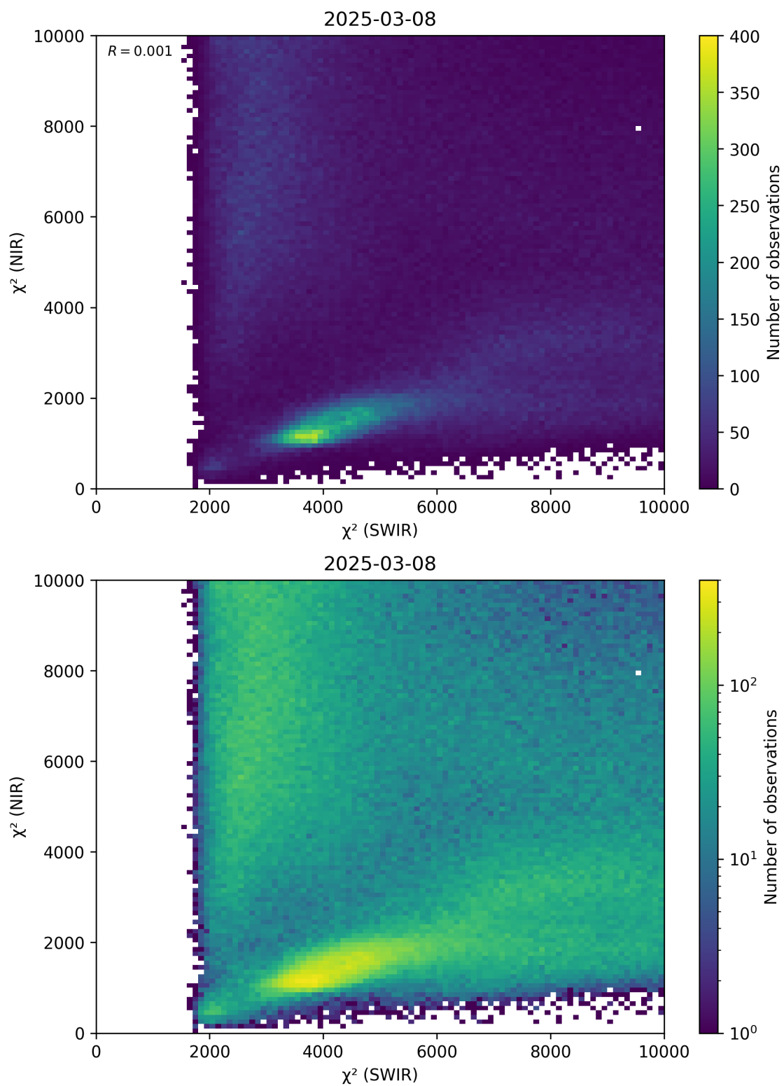
Figure 47: Scatter density plot of “ \chi^2 (SWIR)” against “ \chi^2 (NIR)” for 2025-03-07 to 2025-03-09.
