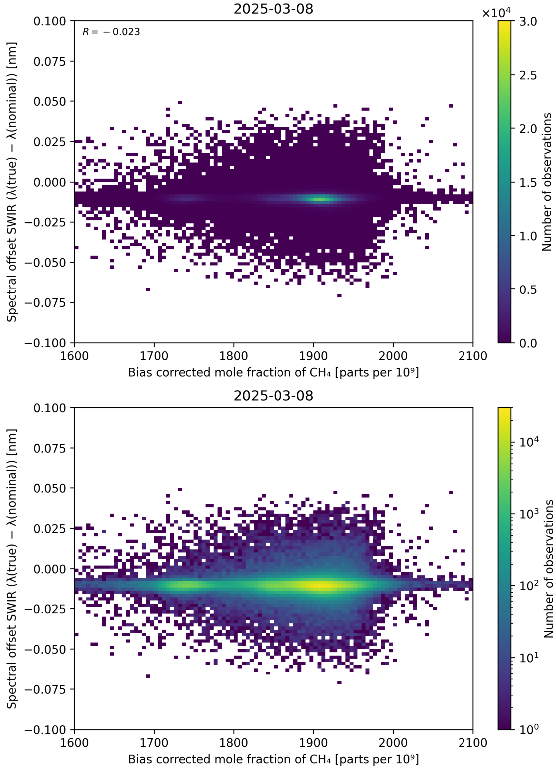
Figure 69: Scatter density plot of “Bias corrected mole fraction of CH 4 ” against “Spectral offset SWIR ( \lambda_{\text{true}} - \lambda_{\text{nominal}} )” for 2025-03-07 to 2025-03-09.
