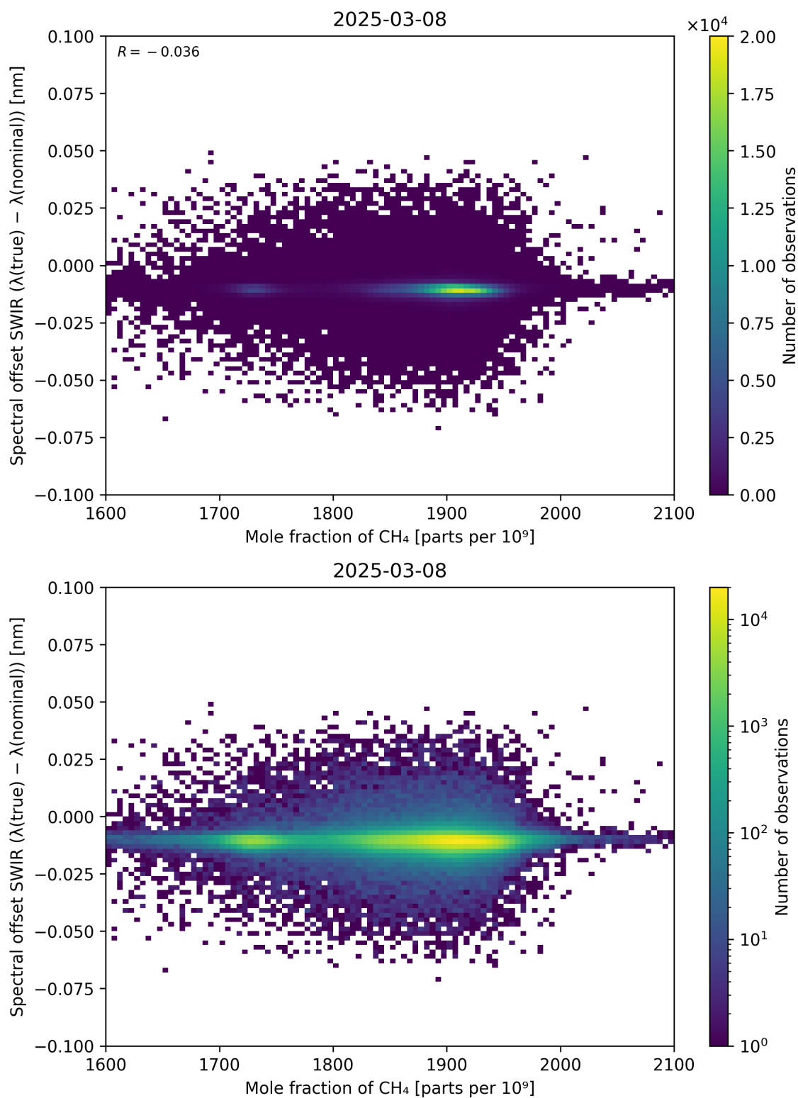
Figure 86: Scatter density plot of “Mole fraction of \text{CH}_4 ” against “Spectral offset SWIR ( \lambda_{\text{true}} - \lambda_{\text{nominal}} )” for 2025-03-07 to 2025-03-09.
