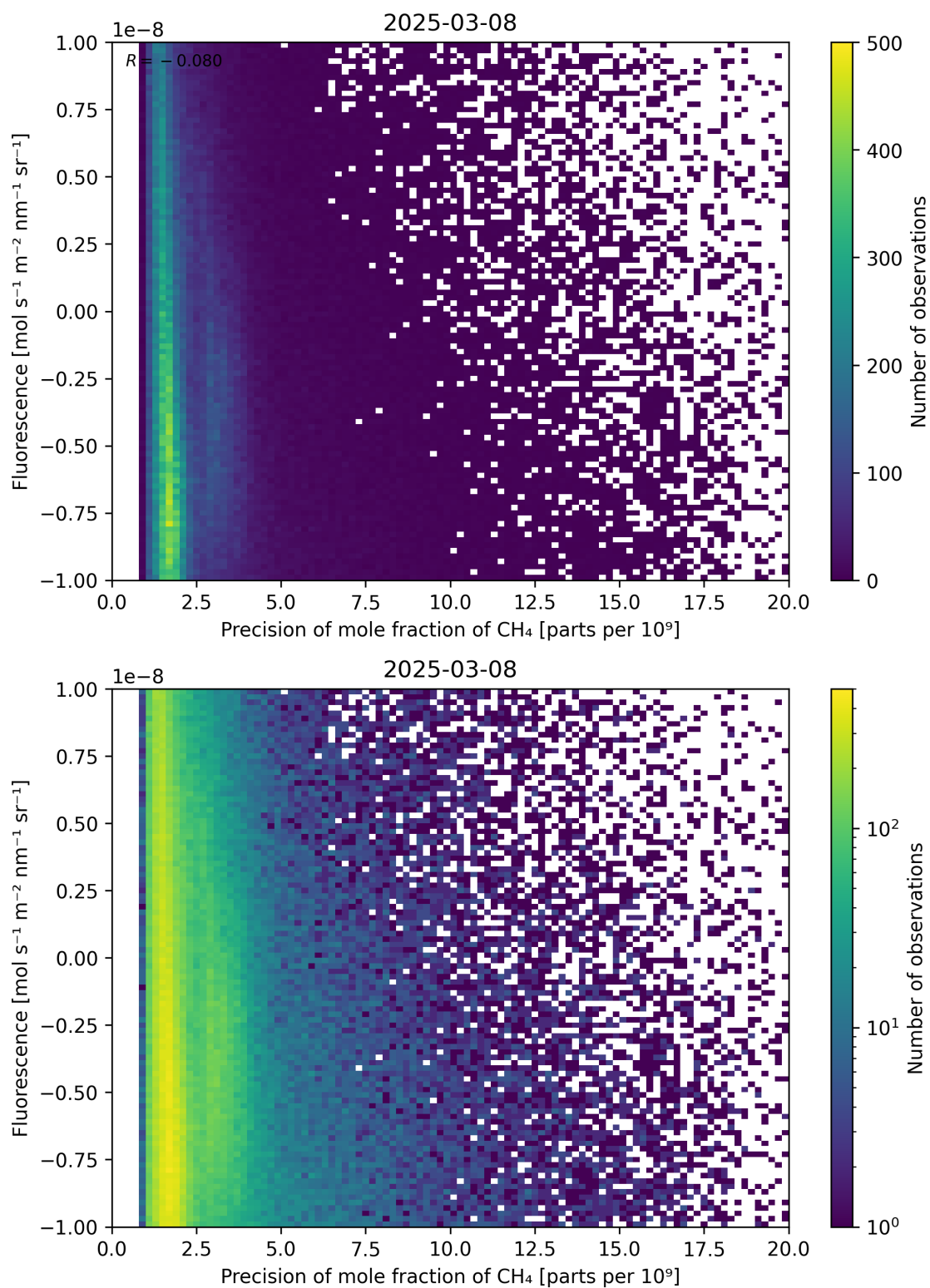
Figure 81: Scatter density plot of “Precision of mole fraction of CH 4 ” against “Fluorescence” for 2025-03-07 to 2025-03-09.
