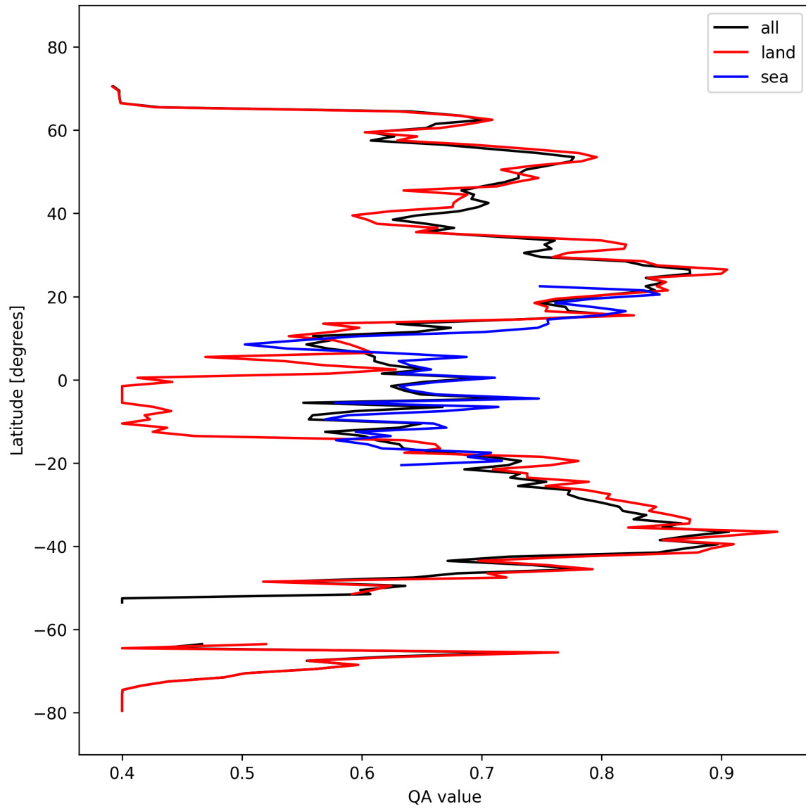
Figure 11: Zonal average of “QA value” for 2025-03-07 to 2025-03-09.
