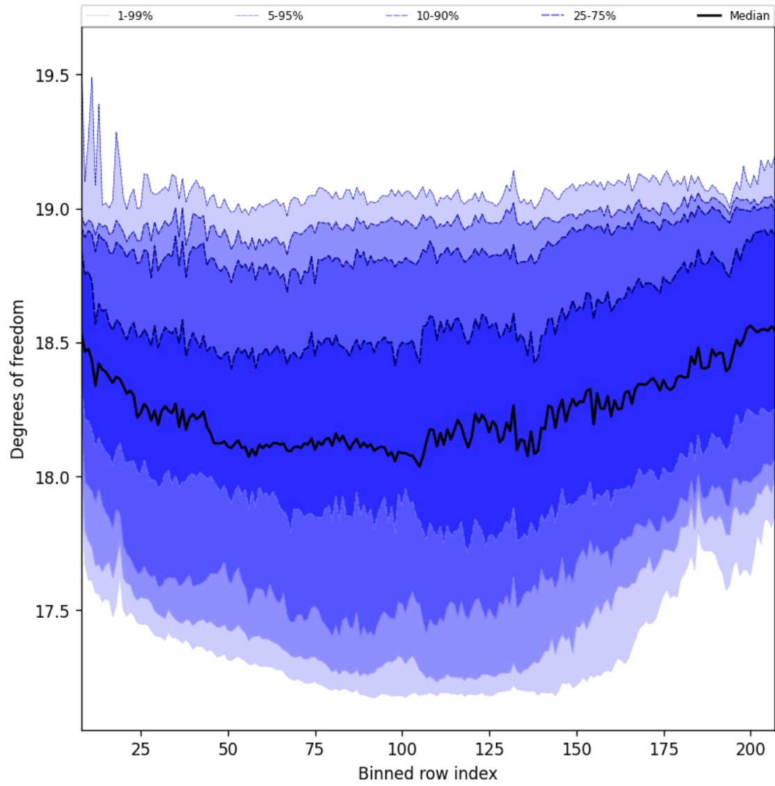
Figure 41: Along track statistics of “Degrees of freedom” for 2025-03-07 to 2025-03-09
