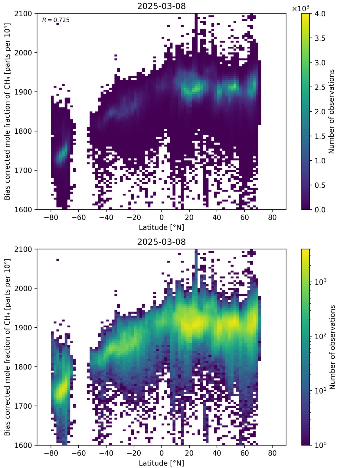
Figure 58: Scatter density plot of “Latitude” against “Bias corrected mole fraction of CH 4 ” for 2025-03-07 to 2025-03-09.
