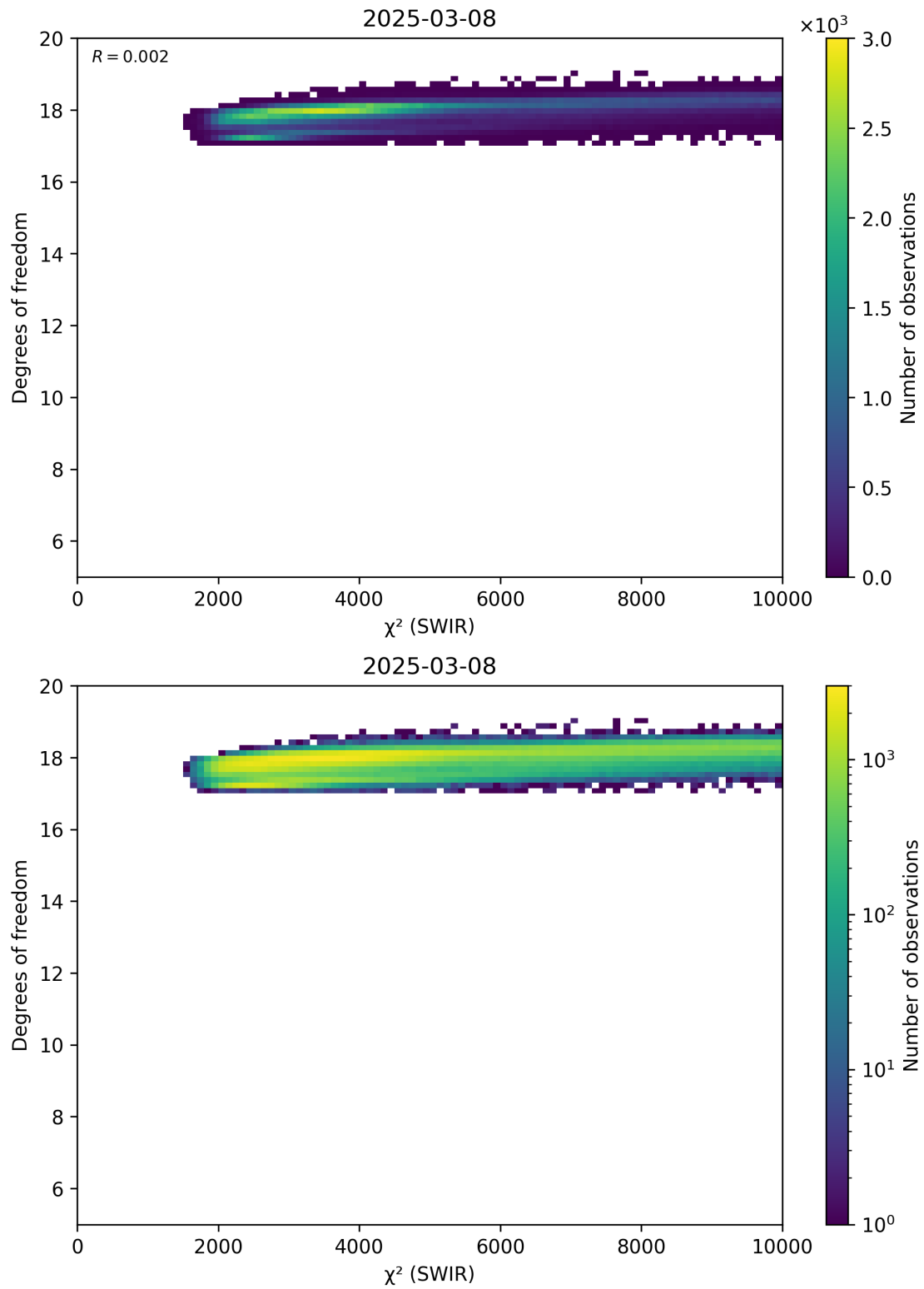
Figure 48: Scatter density plot of “ \chi^2 (SWIR)” against “Degrees of freedom” for 2025-03-07 to 2025-03-09.
