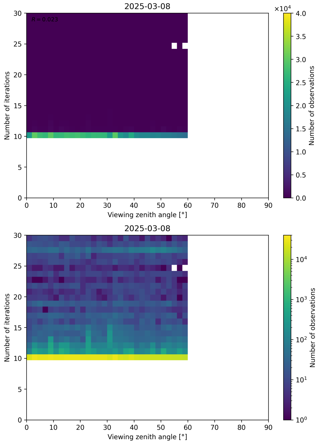
Figure 113: Scatter density plot of “Viewing zenith angle” against “Number of iterations” for 2025-03-07 to 2025-03-09.
