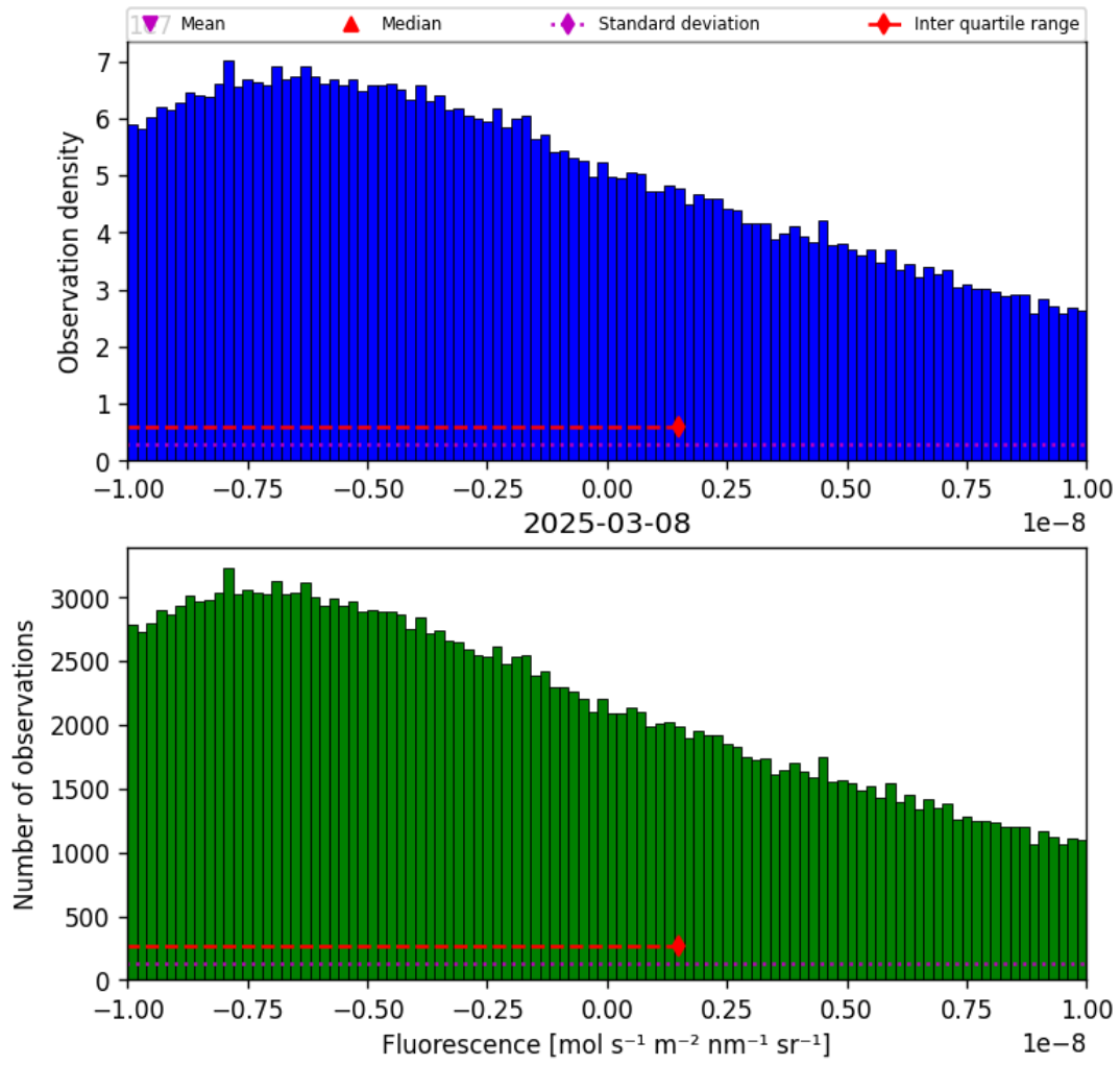
Figure 32: Histogram of “Fluorescence” for 2025-03-07 to 2025-03-09
