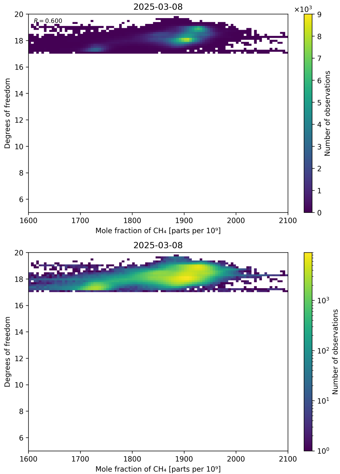
Figure 72: Scatter density plot of “Mole fraction of CH 4 ” against “Degrees of freedom” for 2025-03-07 to 2025-03-09.
