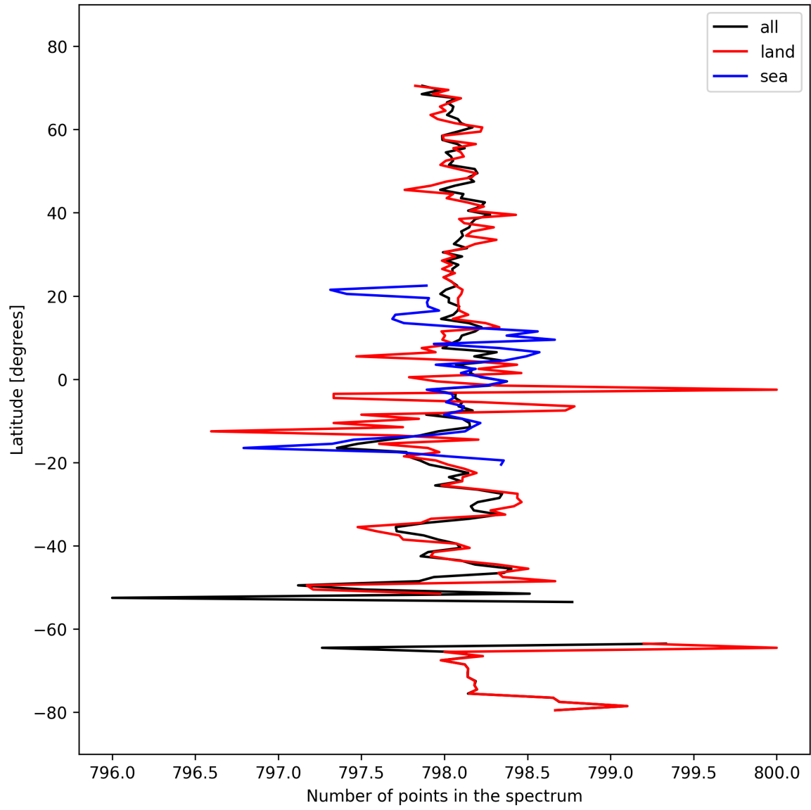
Figure 15: Zonal average of “Number of points in the spectrum” for 2025-03-07 to 2025-03-09.
