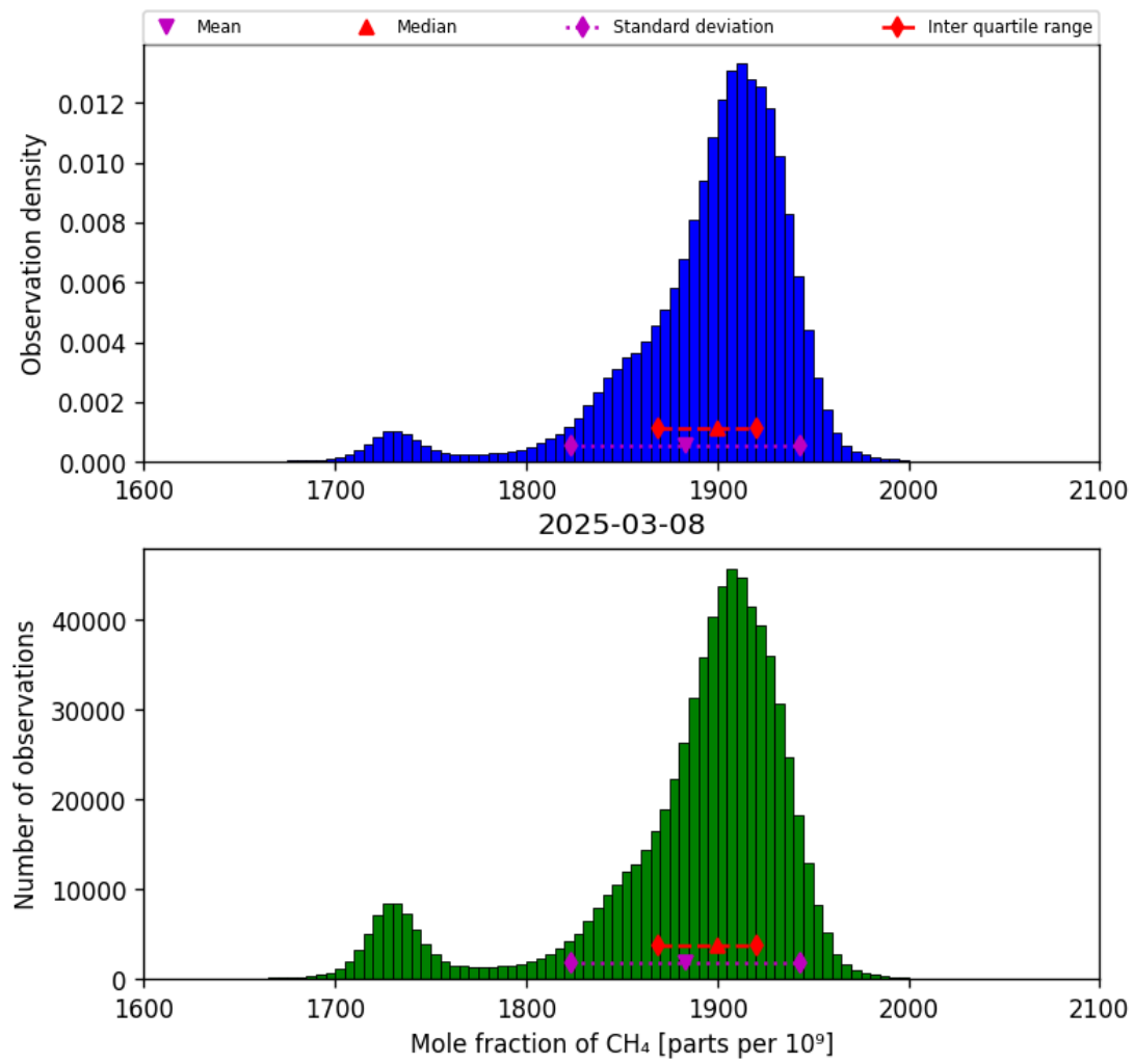
Figure 23: Histogram of “Mole fraction of CH 4 ” for 2025-03-07 to 2025-03-09
