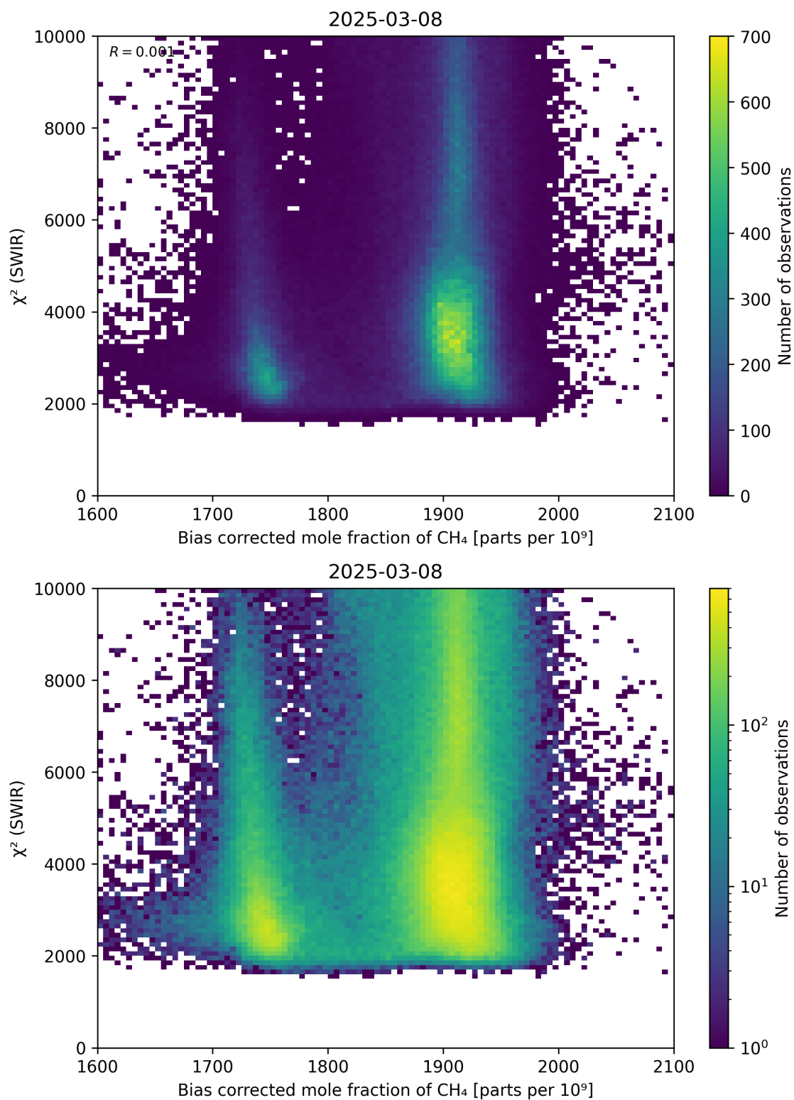
Figure 64: Scatter density plot of “Bias corrected mole fraction of CH 4 ” against “ \chi^2 (SWIR)” for 2025-03-07 to 2025-03-09.
