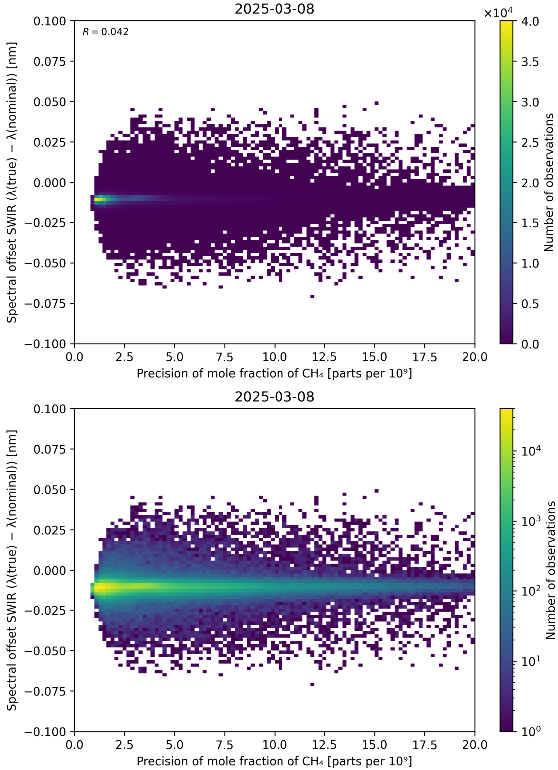
Figure 85: Scatter density plot of “Precision of mole fraction of CH 4 ” against “Spectral offset SWIR ( \lambda_{\text{true}} - \lambda_{\text{nominal}} )” for 2025-03-07 to 2025-03-09.
