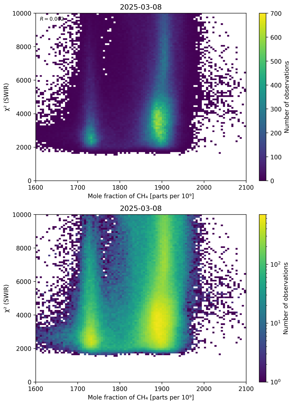
Figure 71: Scatter density plot of “Mole fraction of \text{CH}_4 ” against “ \chi^2 (SWIR)” for 2025-03-07 to 2025-03-09.
