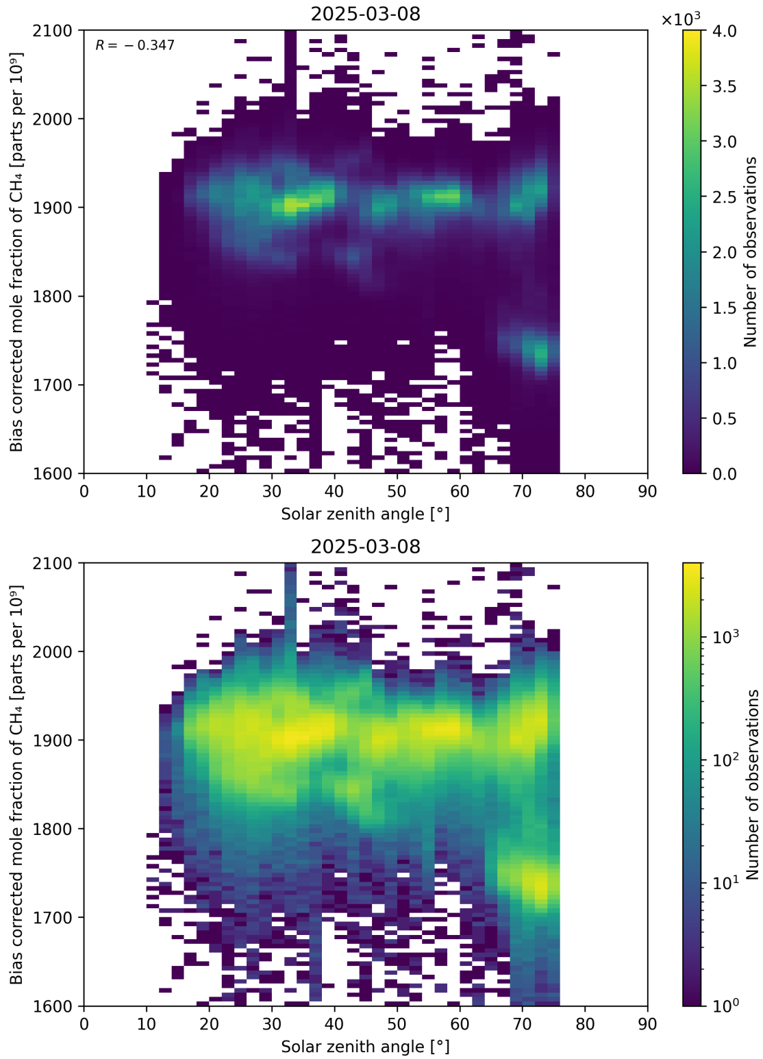
Figure 100: Scatter density plot of “Solar zenith angle” against “Bias corrected mole fraction of \text{CH}_4 ” for 2025-03-07 to 2025-03-09.
