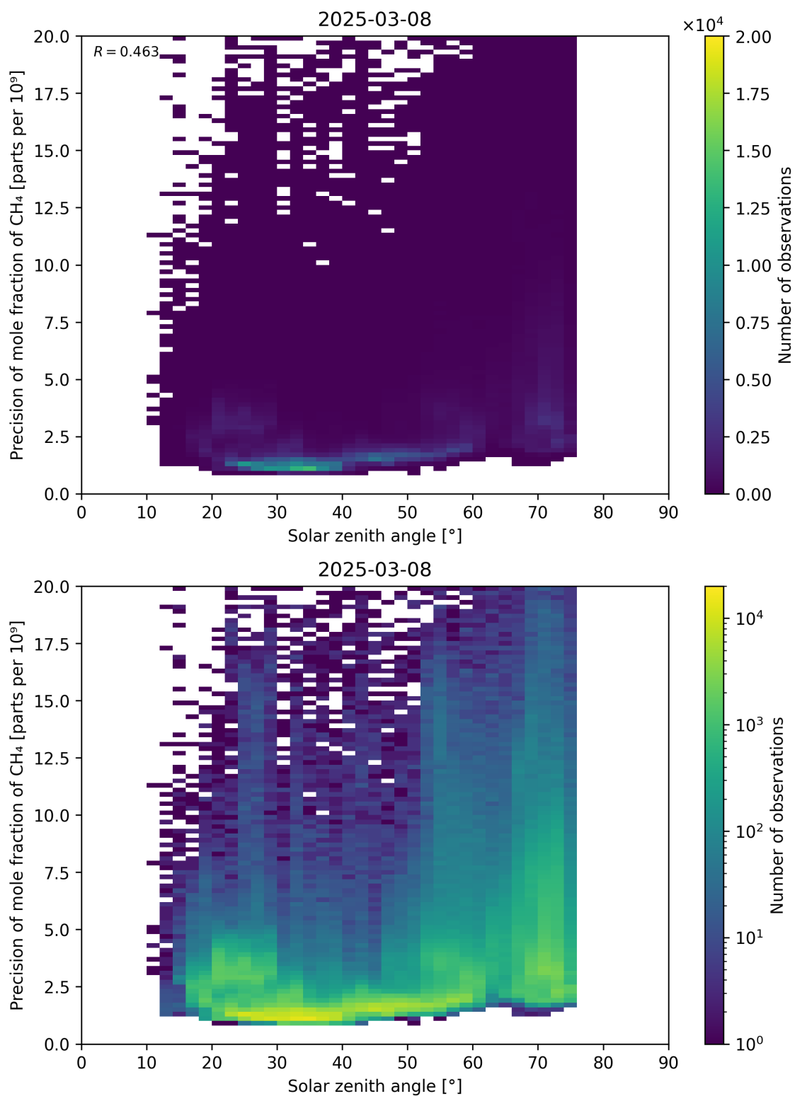
Figure 101: Scatter density plot of “Solar zenith angle” against “Precision of mole fraction of CH 4 ” for 2025-03-07 to 2025-03-09.
