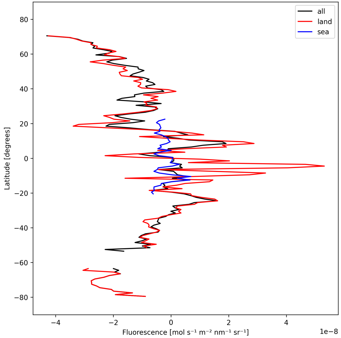
Figure 21: Zonal average of “Fluorescence” for 2025-03-07 to 2025-03-09.
