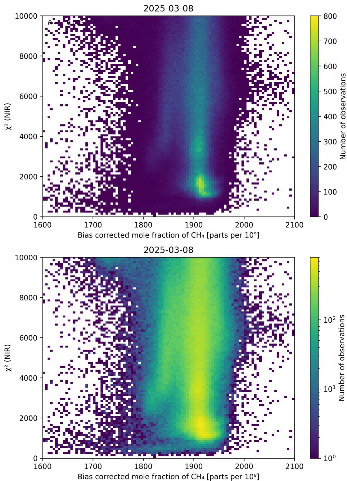
Figure 63: Scatter density plot of “Bias corrected mole fraction of CH 4 ” against “ \chi^2 (NIR)” for 2025-03-07 to 2025-03-09.
