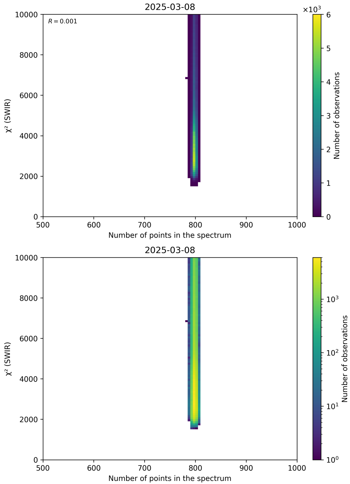
Figure 89: Scatter density plot of “Number of points in the spectrum” against “ \chi^2 (SWIR)” for 2025-03-07 to 2025-03-09.
