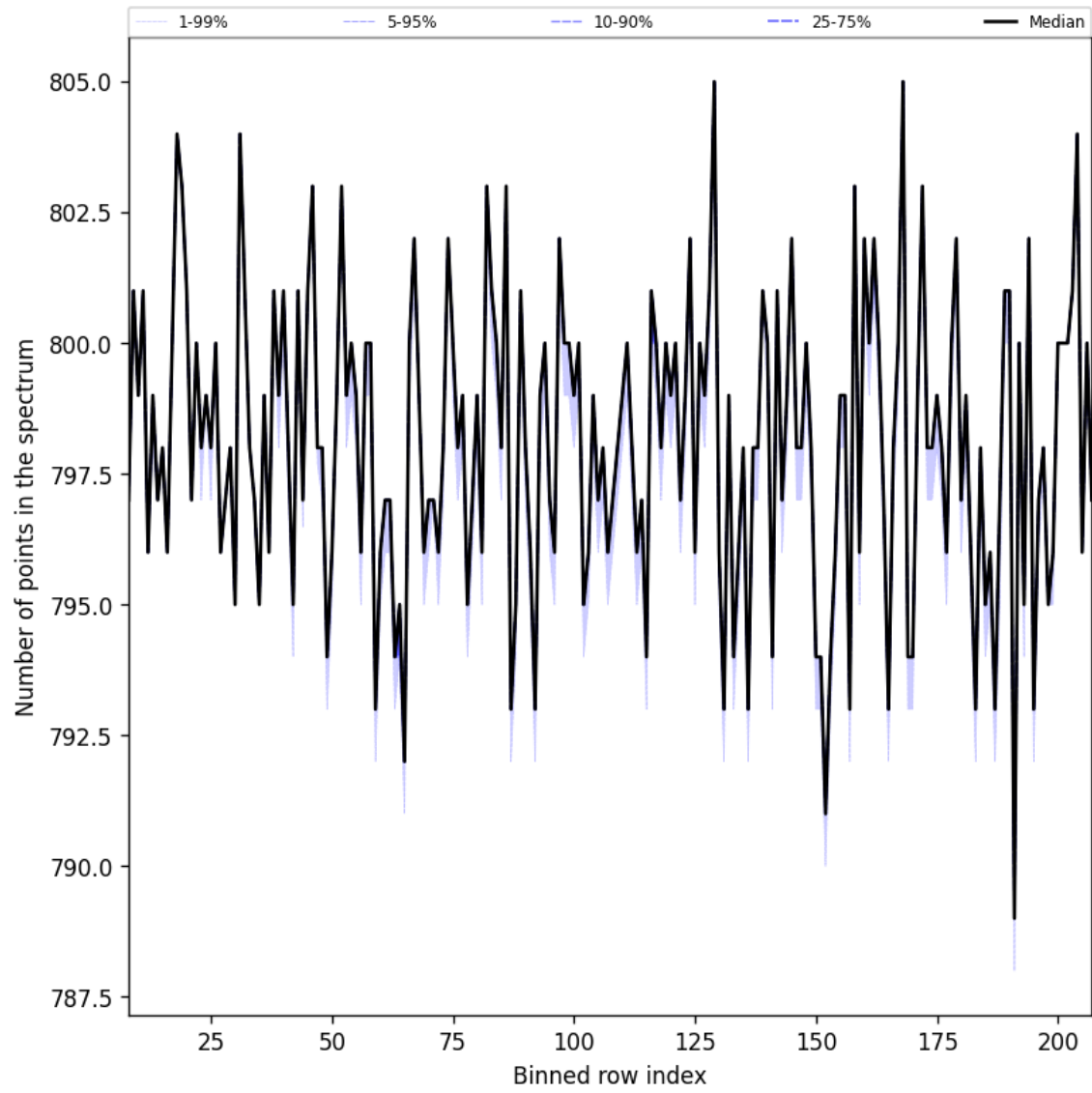
Figure 37: Along track statistics of “Number of points in the spectrum” for 2025-03-07 to 2025-03-09
