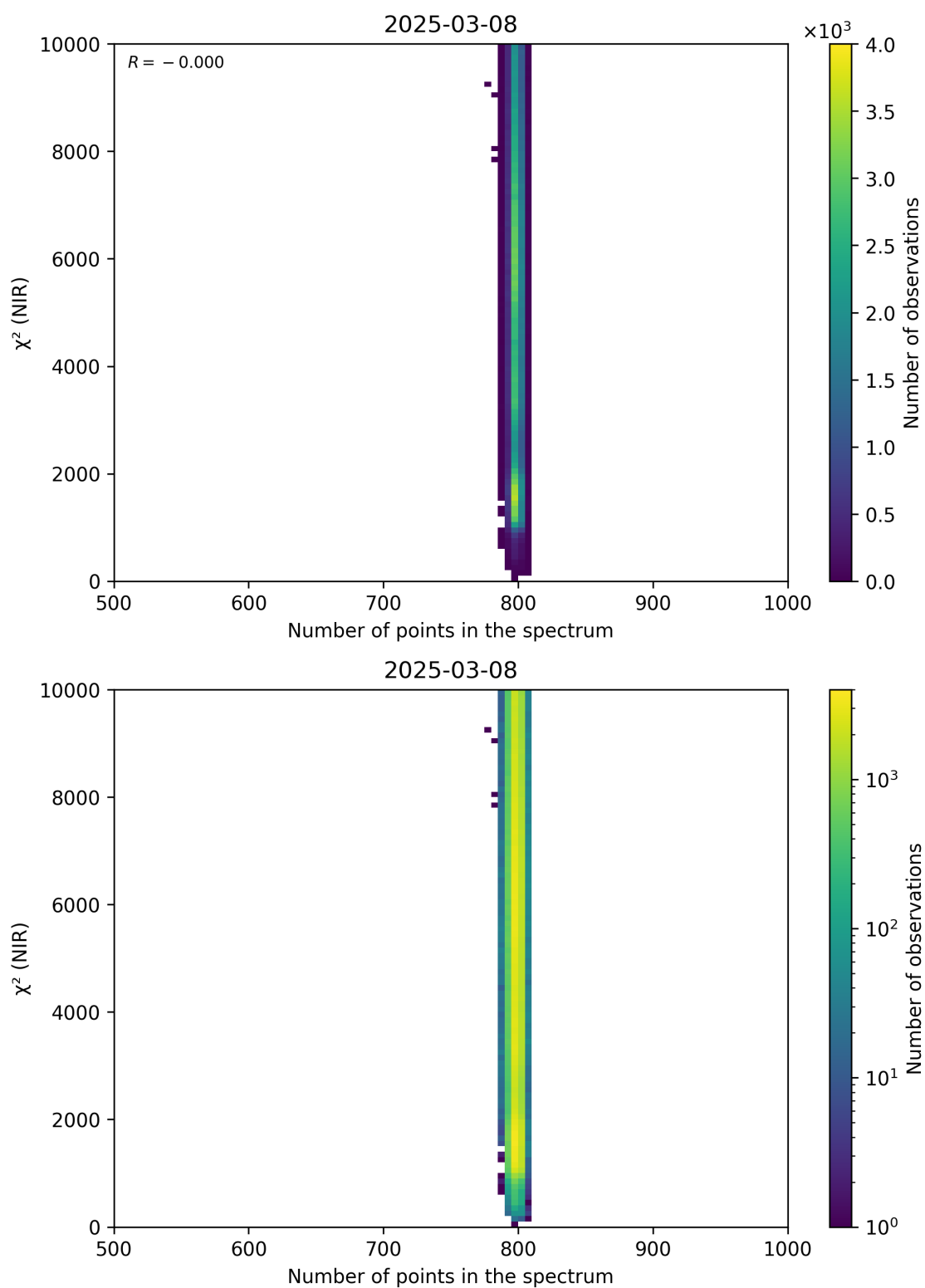
Figure 88: Scatter density plot of “Number of points in the spectrum” against “ \chi^2 (NIR)” for 2025-03-07 to 2025-03-09.
