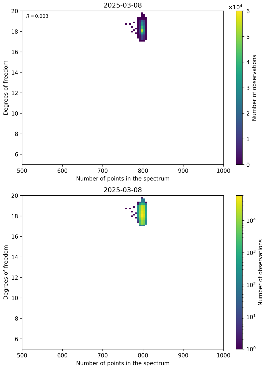
Figure 90: Scatter density plot of “Number of points in the spectrum” against “Degrees of freedom” for 2025-03-07 to 2025-03-09.
