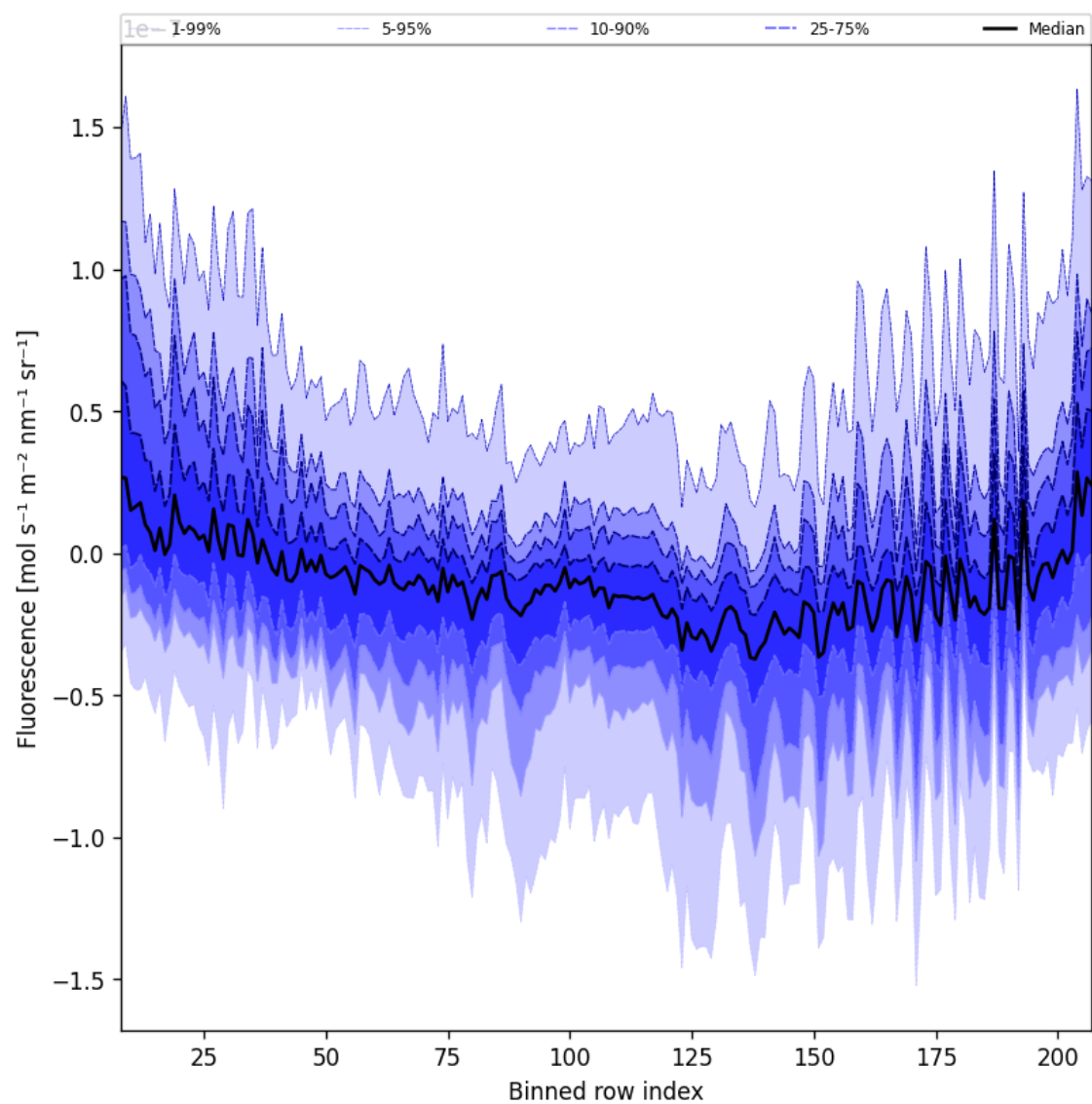
Figure 43: Along track statistics of “Fluorescence” for 2025-03-07 to 2025-03-09
