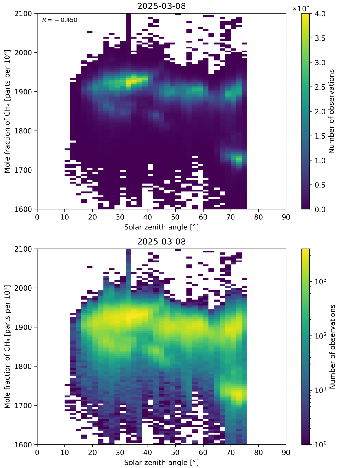
Figure 99: Scatter density plot of “Solar zenith angle” against “Mole fraction of CH 4 ” for 2025-03-07 to 2025-03-09.
