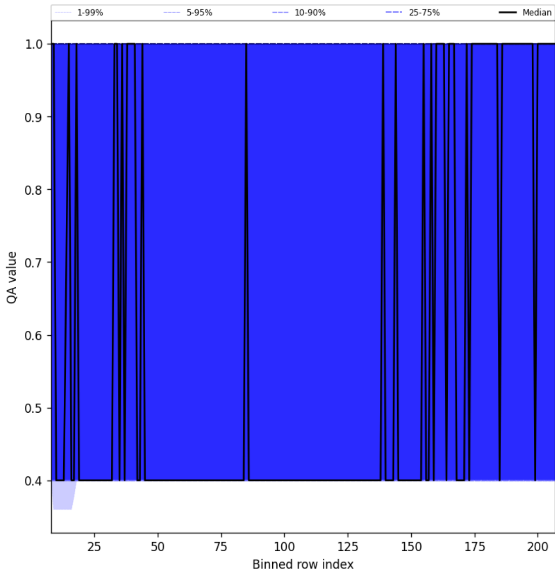
Figure 33: Along track statistics of “QA value” for 2025-03-07 to 2025-03-09
