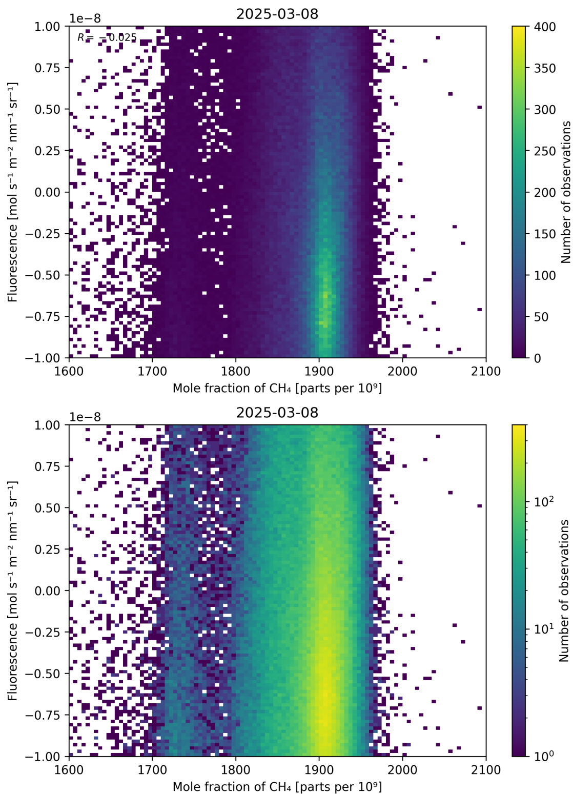
Figure 73: Scatter density plot of “Mole fraction of \text{CH}_4 ” against “Fluorescence” for 2025-03-07 to 2025-03-09.
