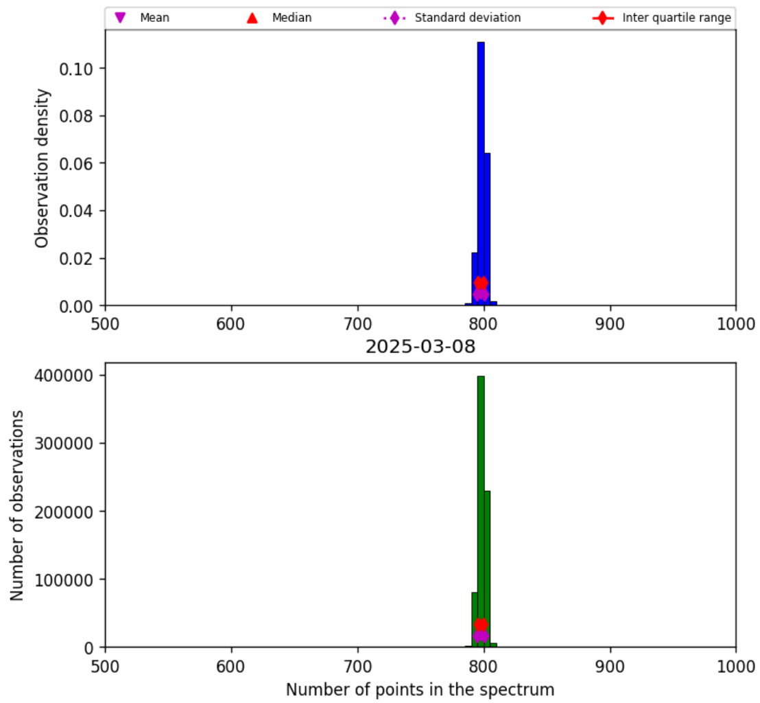
Figure 26: Histogram of “Number of points in the spectrum” for 2025-03-07 to 2025-03-09
