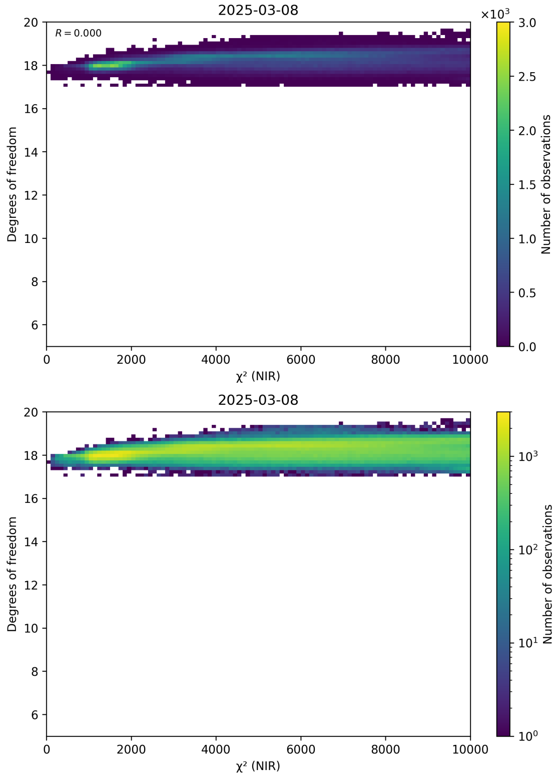
Figure 44: Scatter density plot of “ \chi^2 (NIR)” against “Degrees of freedom” for 2025-03-07 to 2025-03-09.
