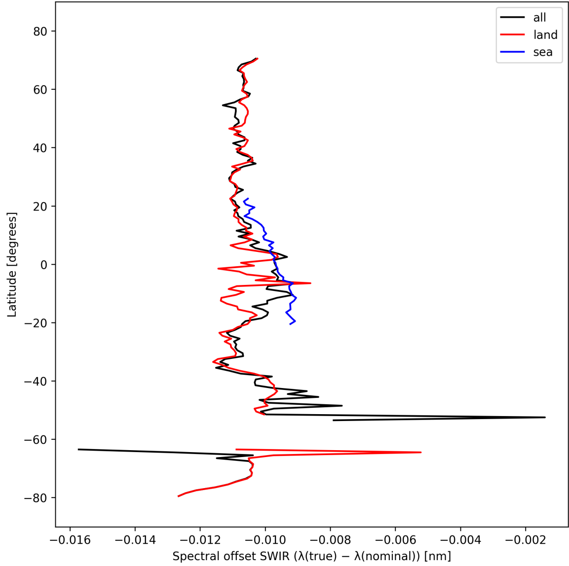
Figure 16: Zonal average of “Spectral offset SWIR ( \lambda_{\text{true}} - \lambda_{\text{nominal}} )” for 2025-03-07 to 2025-03-09.
