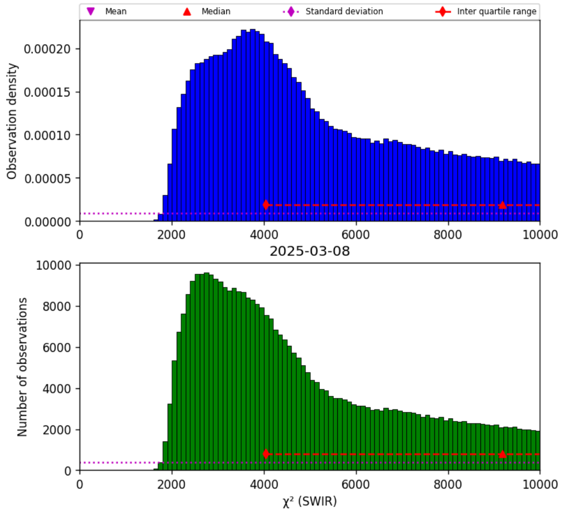
Figure 28: Histogram of " \chi^2 (SWIR)" for 2025-03-07 to 2025-03-09
