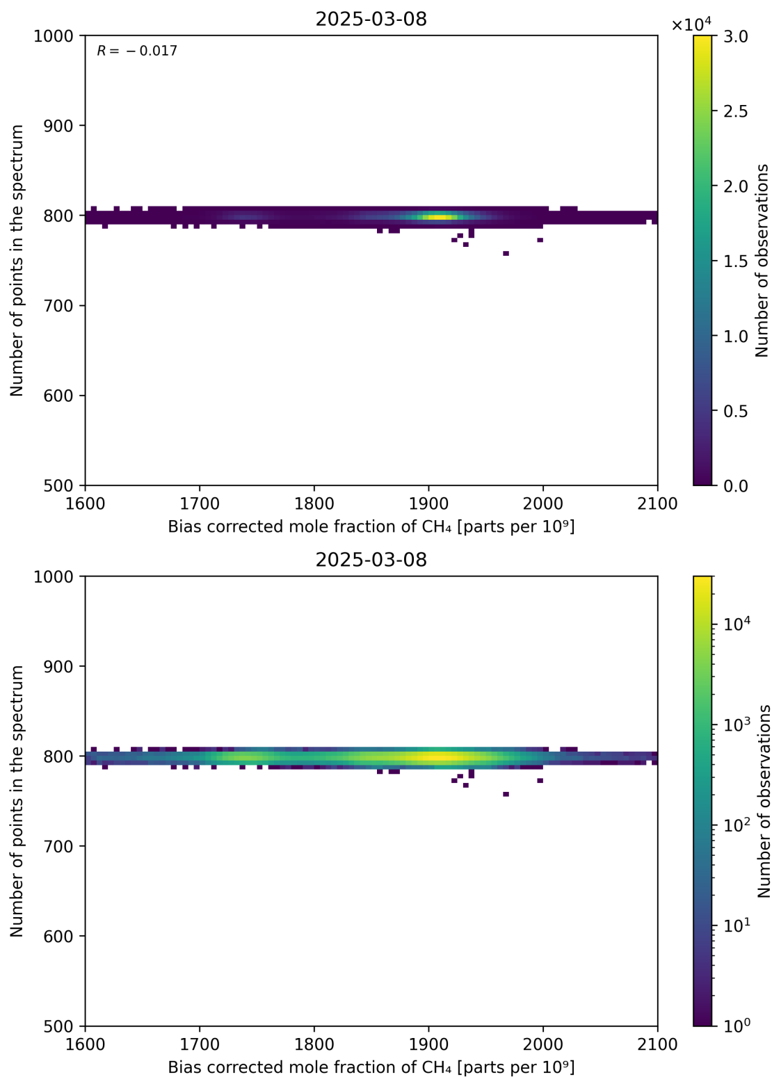
Figure 68: Scatter density plot of “Bias corrected mole fraction of CH 4 ” against “Number of points in the spectrum” for 2025-03-07 to 2025-03-09.
