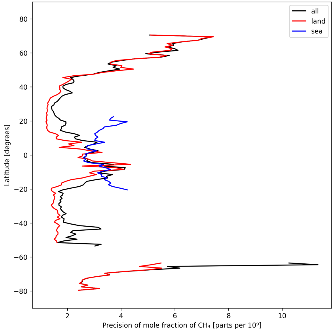
Figure 13: Zonal average of “Precision of mole fraction of CH 4 ” for 2025-03-07 to 2025-03-09.
