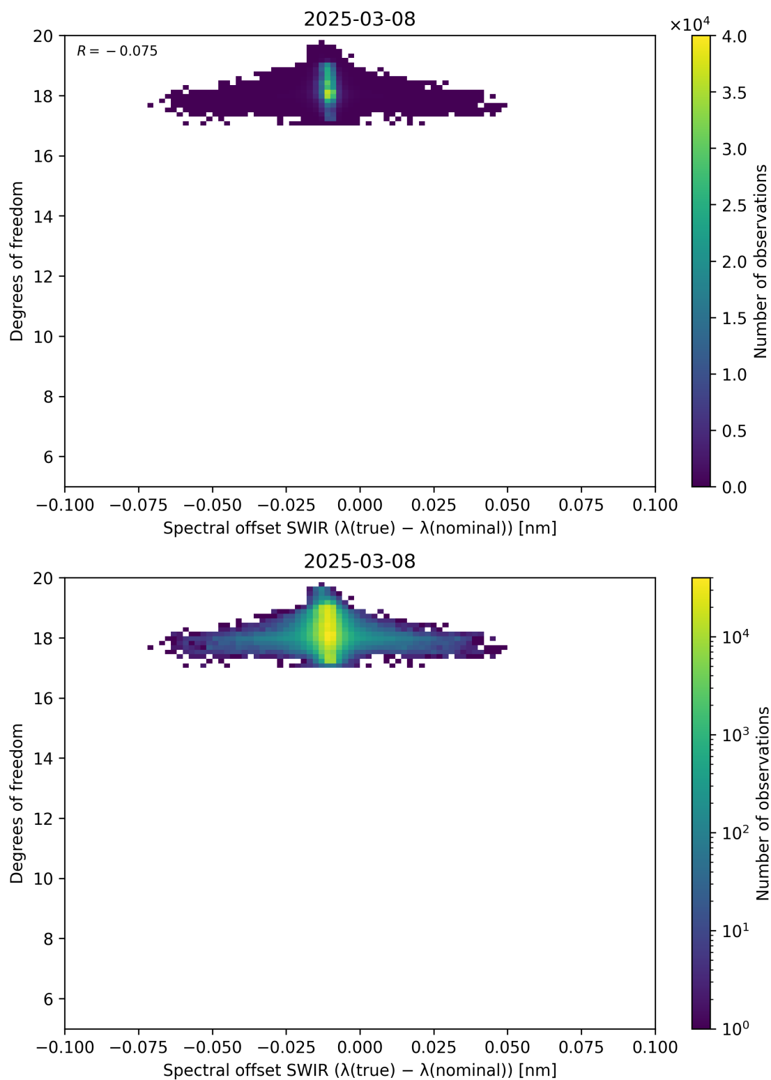
Figure 119: Scatter density plot of “Spectral offset SWIR ( \lambda_{\text{true}} - \lambda_{\text{nominal}} )” against “Degrees of freedom” for 2025-03-07 to 2025-03-09.
