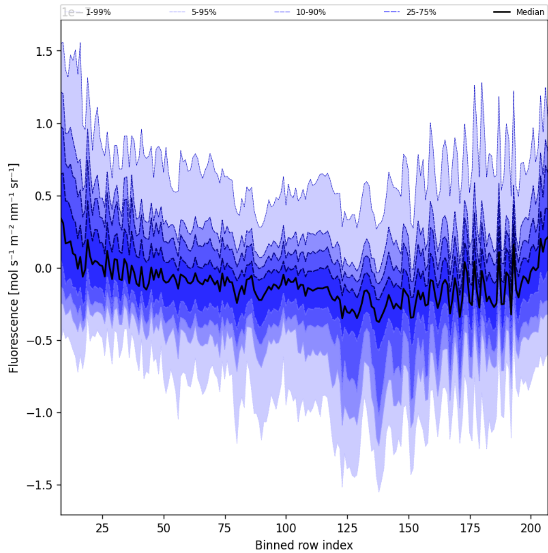
Figure 43: Along track statistics of “Fluorescence” for 2025-03-08 to 2025-03-10
