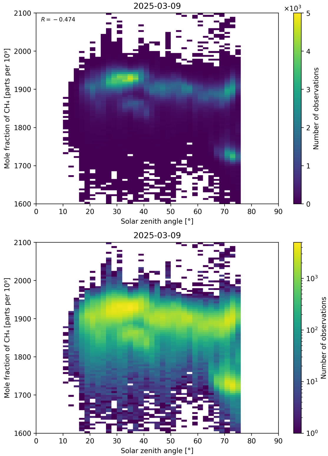
Figure 99: Scatter density plot of “Solar zenith angle” against “Mole fraction of CH 4 ” for 2025-03-08 to 2025-03-10.
