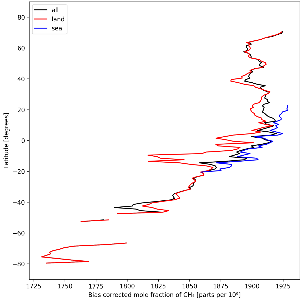
Figure 14: Zonal average of “Bias corrected mole fraction of CH 4 ” for 2025-03-08 to 2025-03-10.
