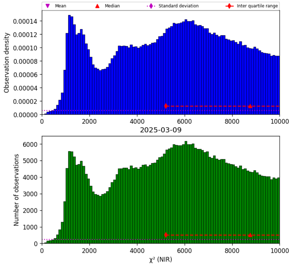
Figure 29: Histogram of " \chi^2 (NIR)" for 2025-03-08 to 2025-03-10
