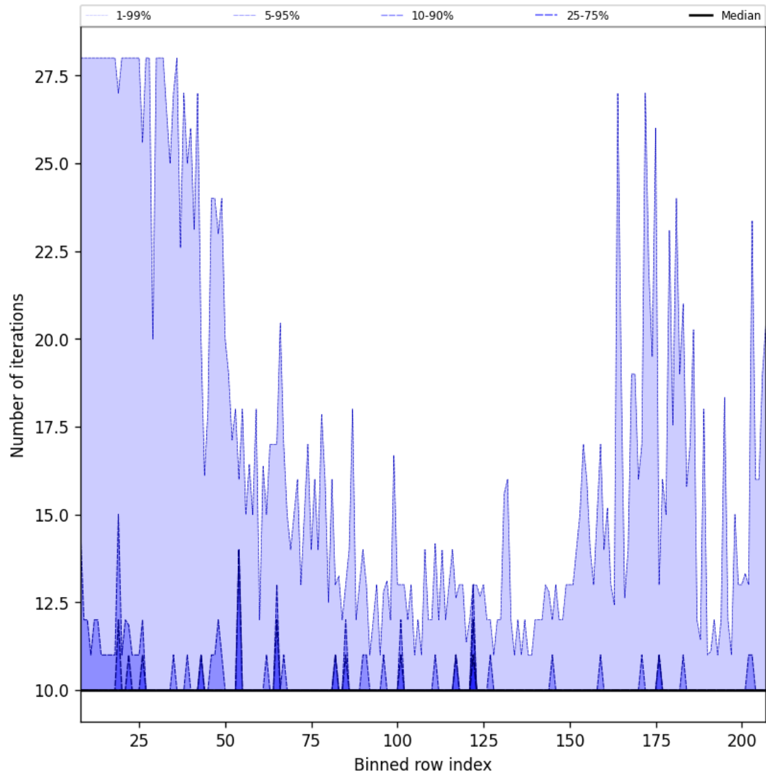
Figure 42: Along track statistics of “Number of iterations” for 2025-03-08 to 2025-03-10
