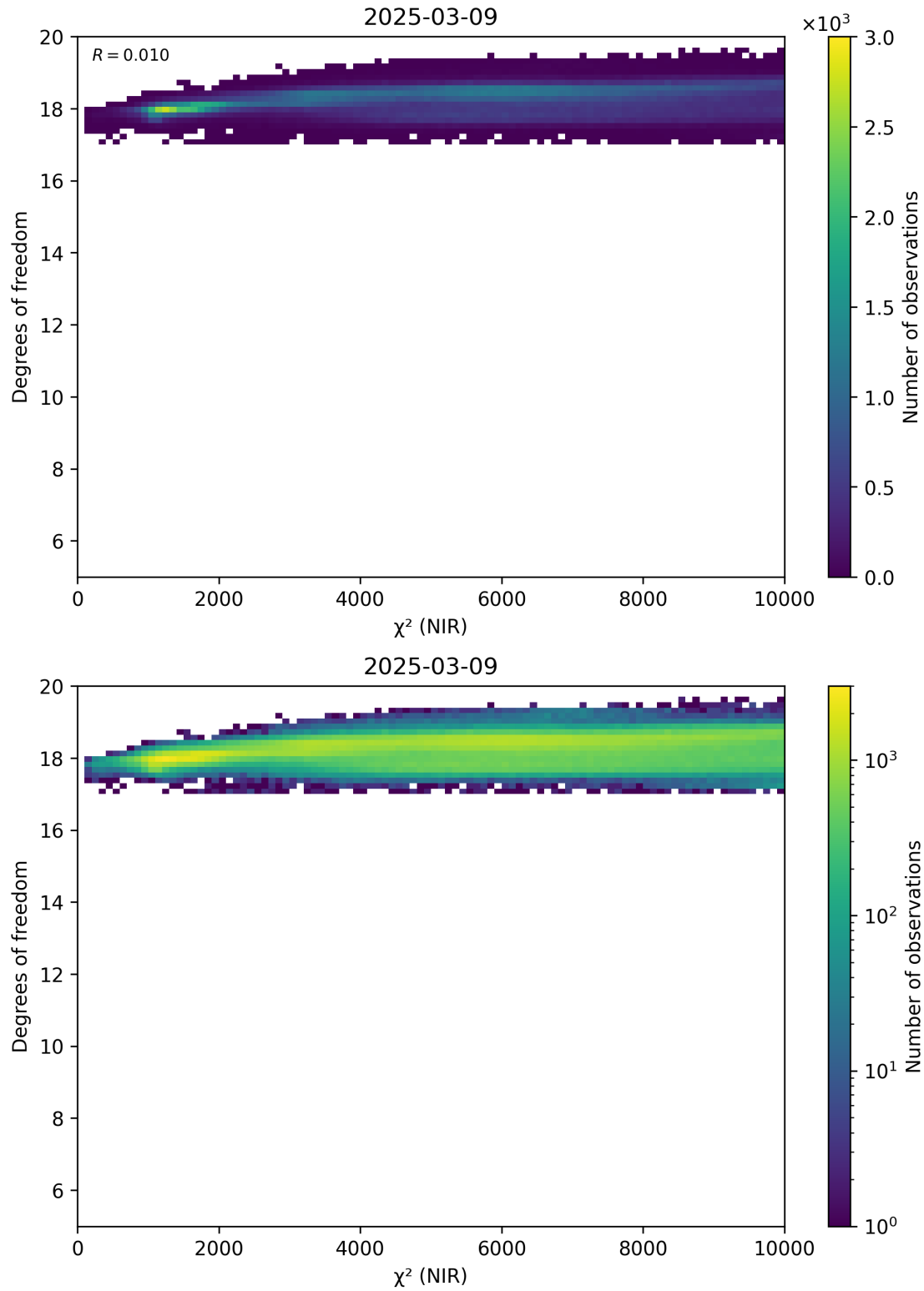
Figure 44: Scatter density plot of “ \chi^2 (NIR)” against “Degrees of freedom” for 2025-03-08 to 2025-03-10.
