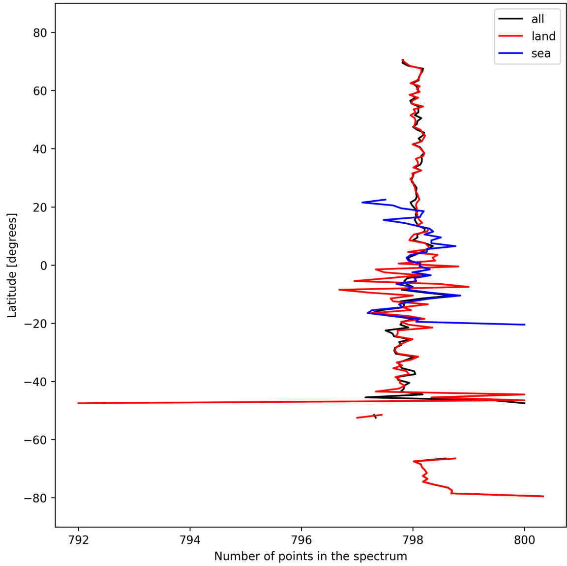
Figure 15: Zonal average of “Number of points in the spectrum” for 2025-03-08 to 2025-03-10.
