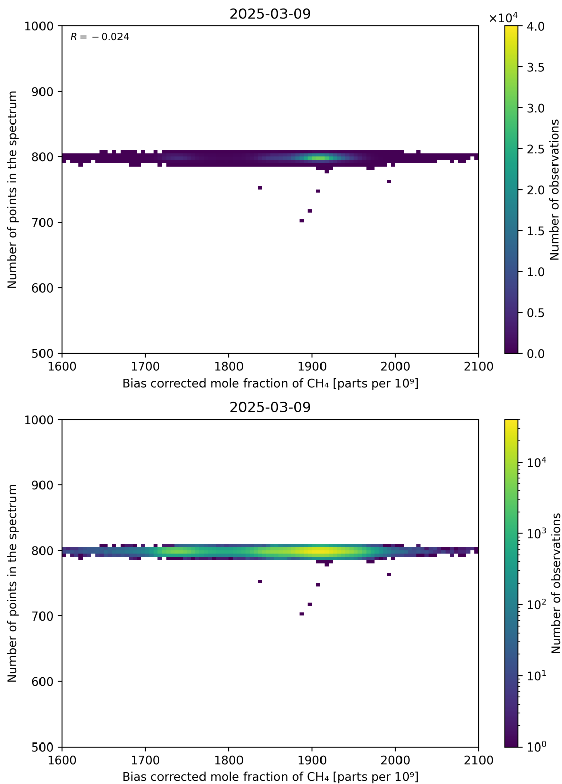
Figure 68: Scatter density plot of “Bias corrected mole fraction of CH 4 ” against “Number of points in the spectrum” for 2025-03-08 to 2025-03-10.
