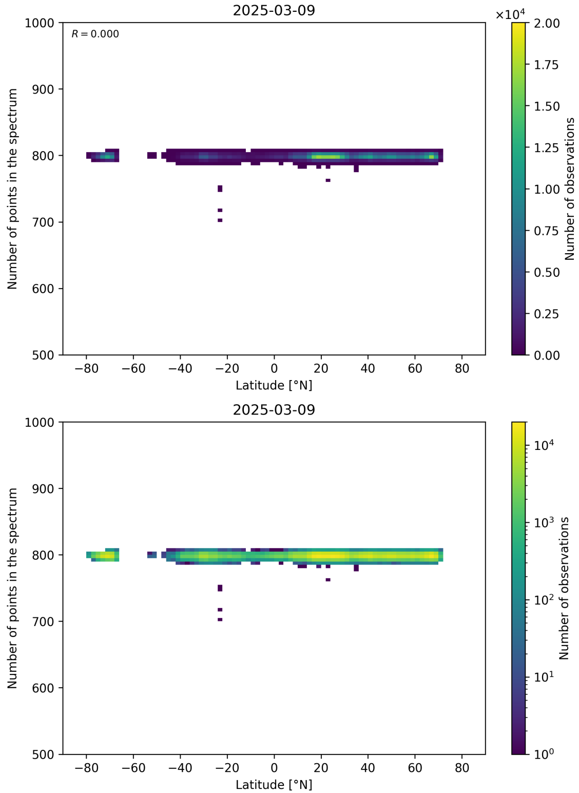
Figure 61: Scatter density plot of “Latitude” against “Number of points in the spectrum” for 2025-03-08 to 2025-03-10.
