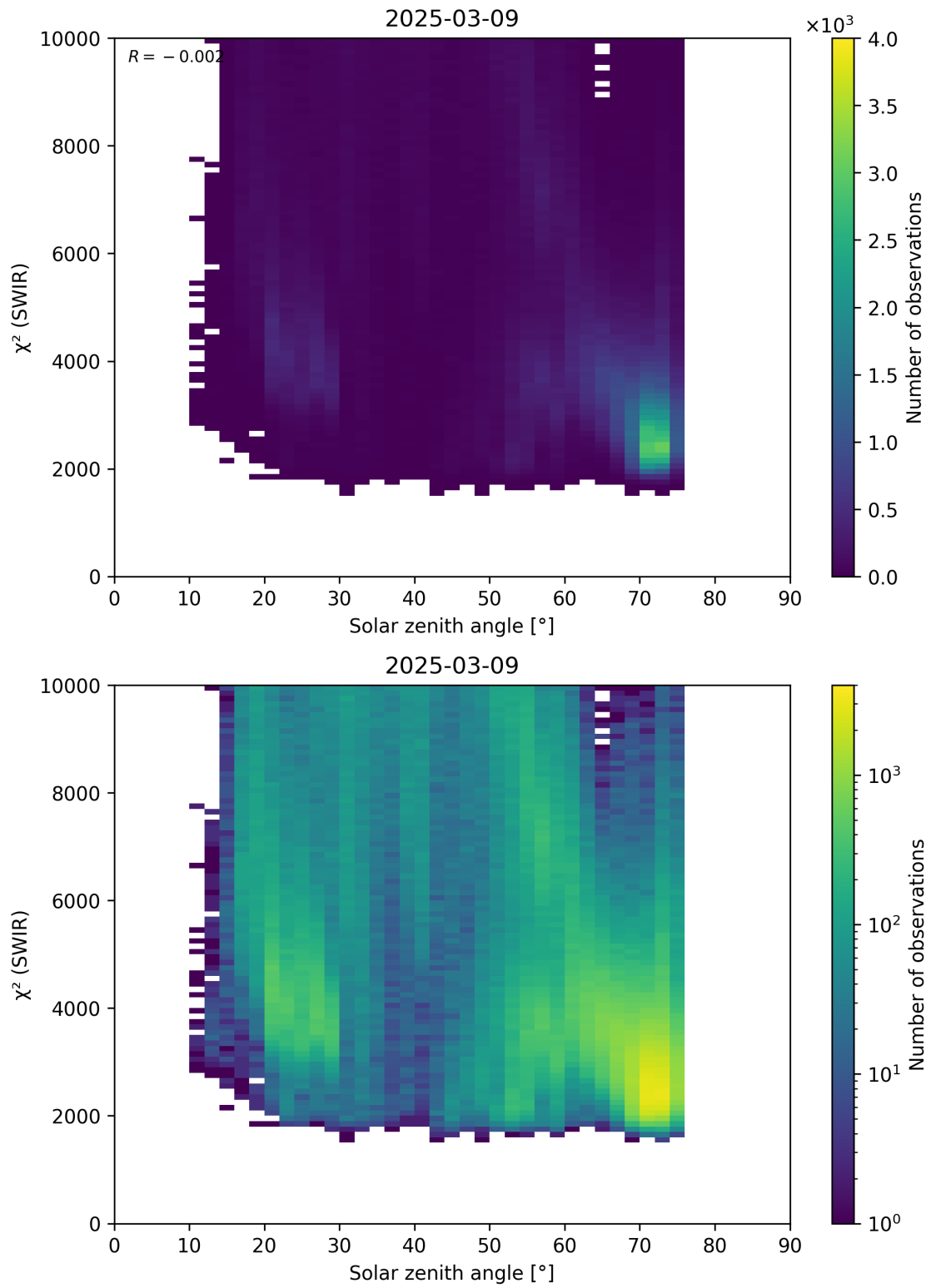
Figure 95: Scatter density plot of “Solar zenith angle” against “ \chi^2 (SWIR)” for 2025-03-08 to 2025-03-10.
