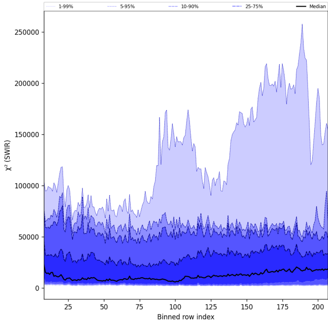
Figure 39: Along track statistics of " \chi^2 (SWIR)" for 2025-03-08 to 2025-03-10
