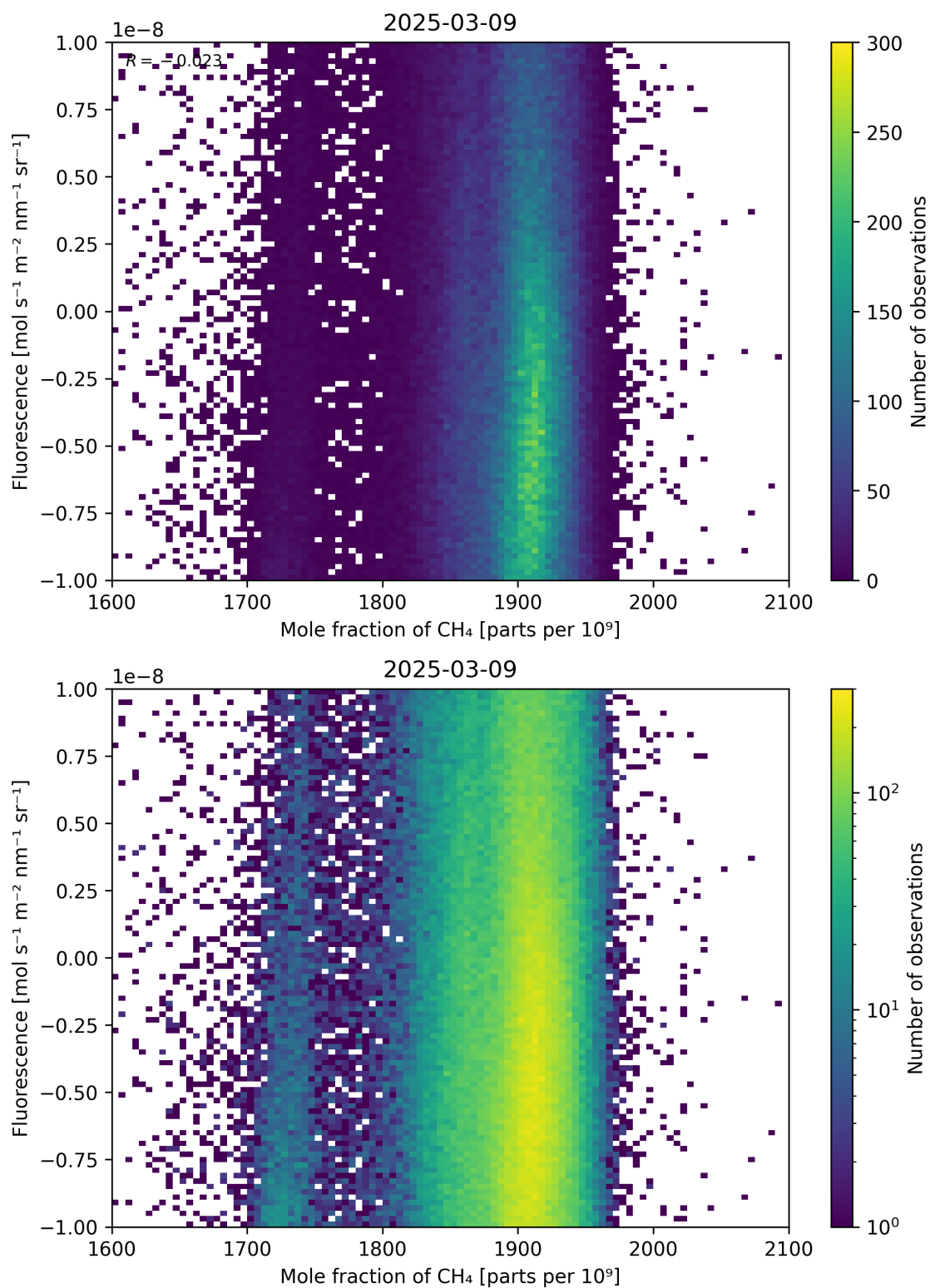
Figure 73: Scatter density plot of “Mole fraction of \text{CH}_4 ” against “Fluorescence” for 2025-03-08 to 2025-03-10.
