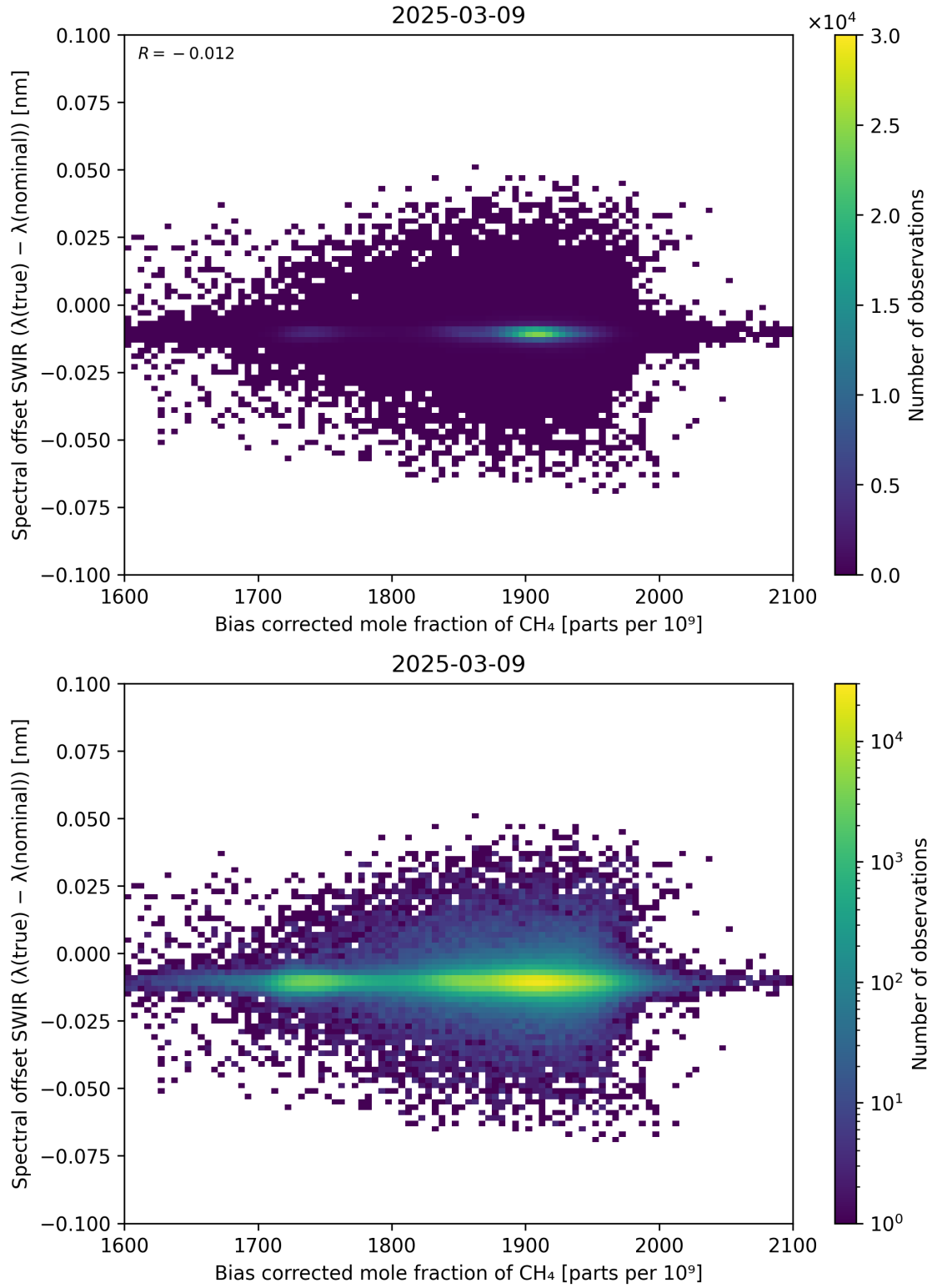
Figure 69: Scatter density plot of “Bias corrected mole fraction of \text{CH}_4 ” against “Spectral offset SWIR ( \lambda_{\text{true}} - \lambda_{\text{nominal}} )” for 2025-03-08 to 2025-03-10.
