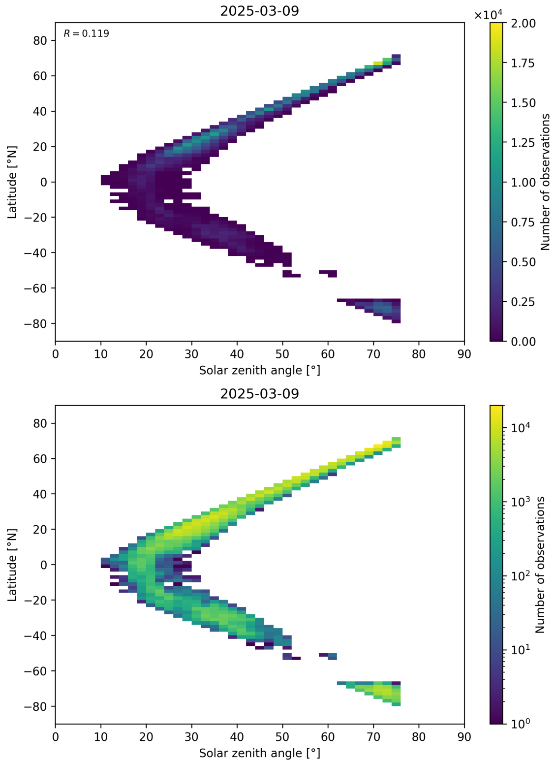
Figure 98: Scatter density plot of “Solar zenith angle” against “Latitude” for 2025-03-08 to 2025-03-10.
