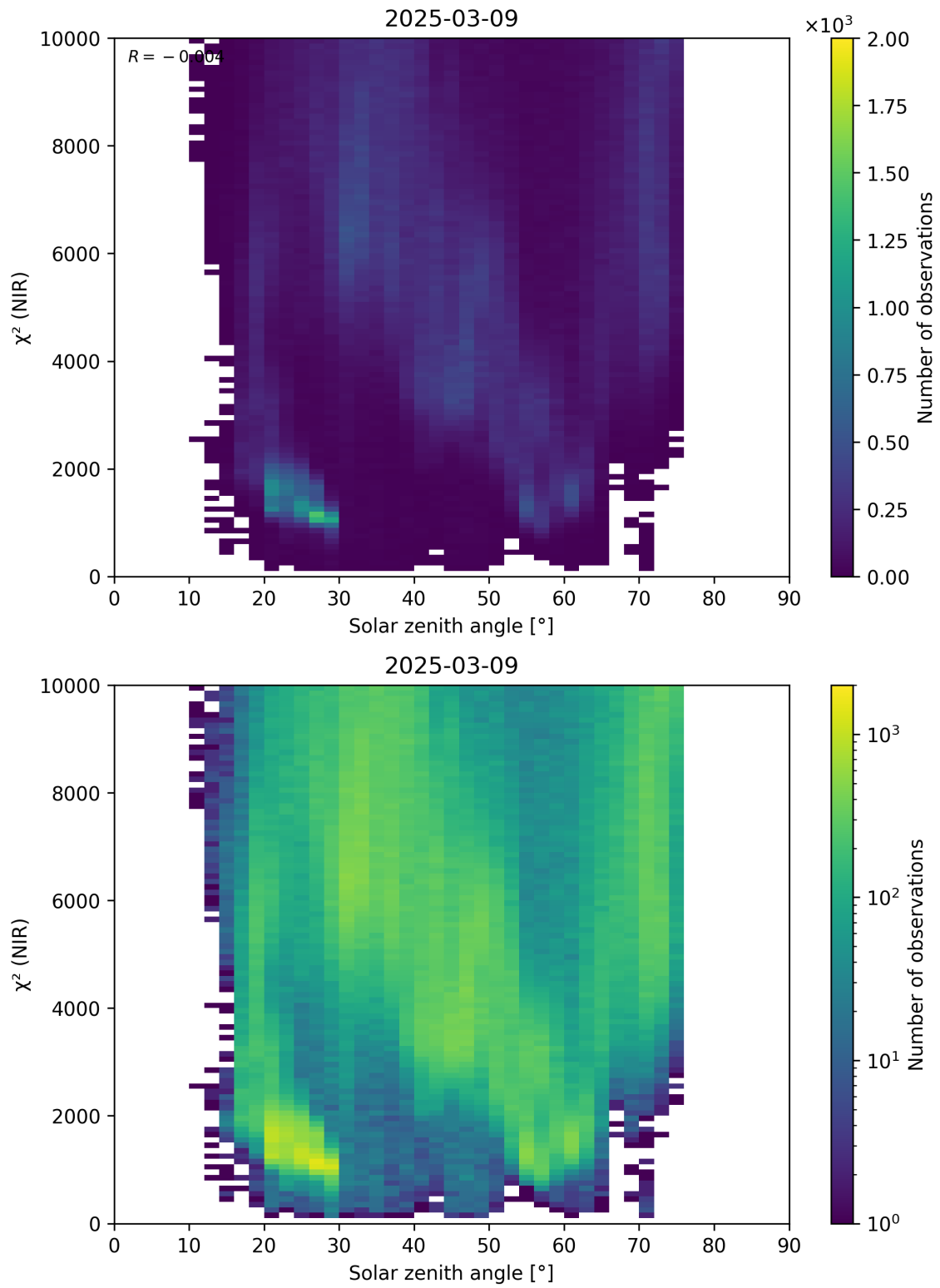
Figure 94: Scatter density plot of “Solar zenith angle” against “ \chi^2 (NIR)” for 2025-03-08 to 2025-03-10.
