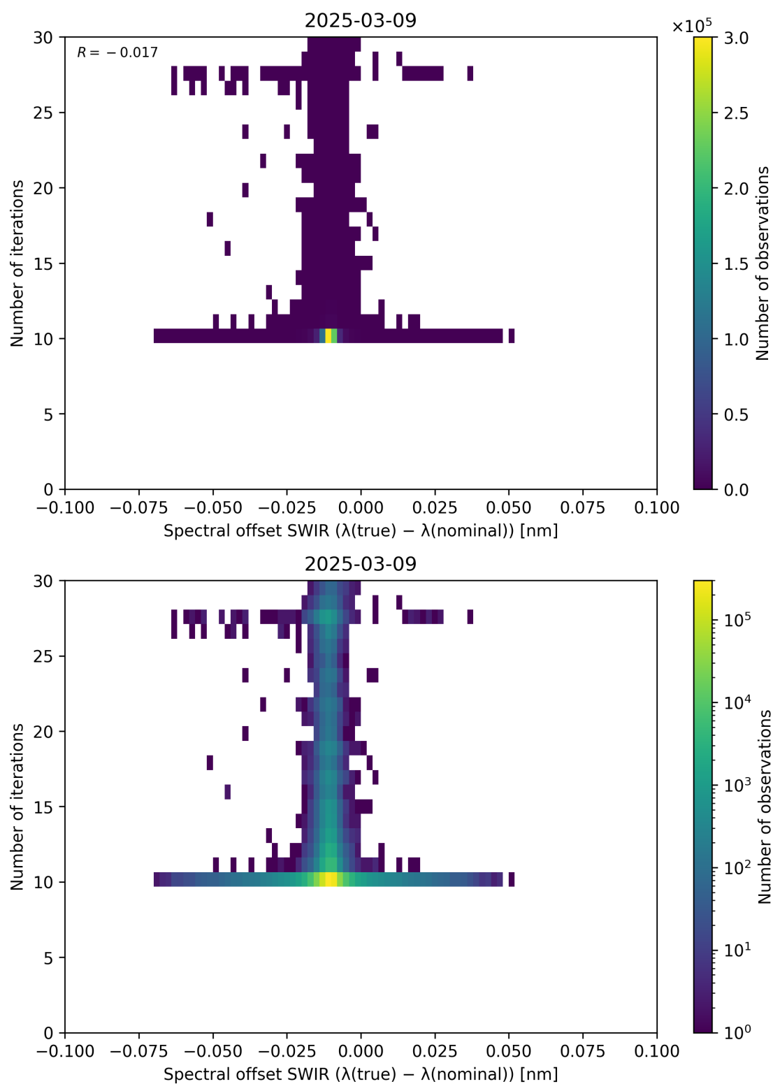
Figure 121: Scatter density plot of “Spectral offset SWIR ( \lambda_{\text{true}} - \lambda_{\text{nominal}} )” against “Number of iterations” for 2025-03-08 to 2025-03-10.
