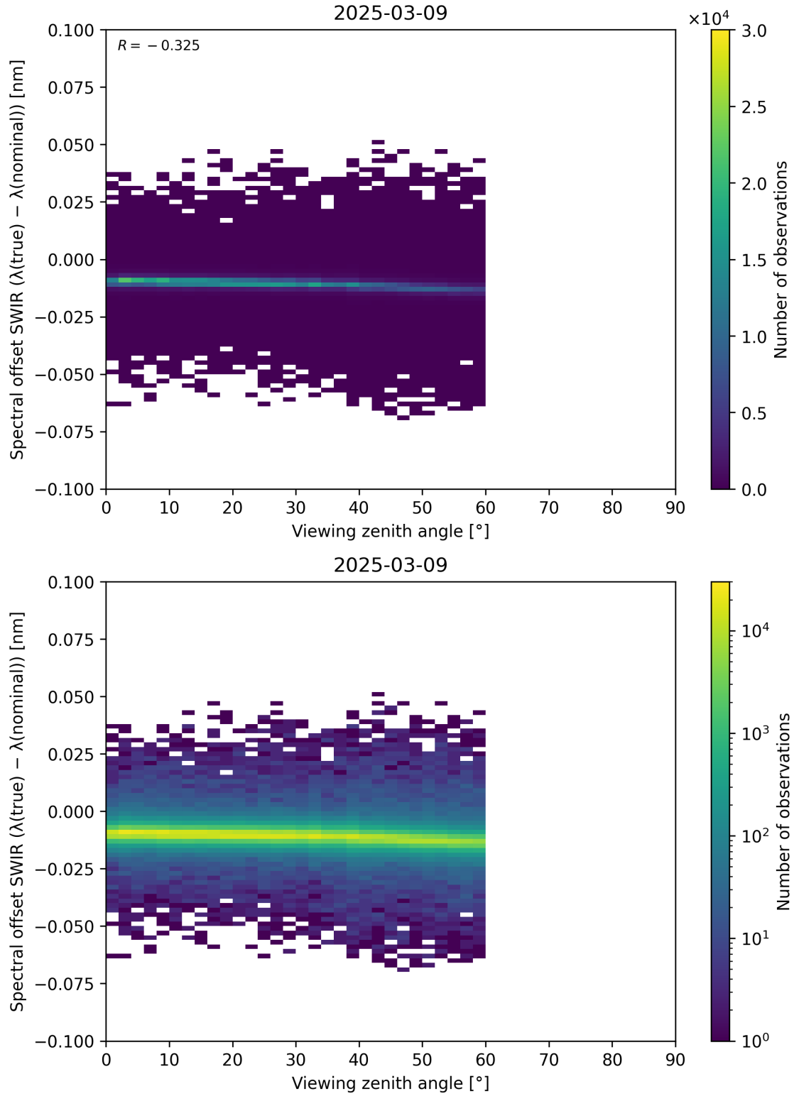
Figure 116: Scatter density plot of “Viewing zenith angle” against “Spectral offset SWIR ( \lambda_{\text{true}} - \lambda_{\text{nominal}} )” for 2025-03-08 to 2025-03-10.
