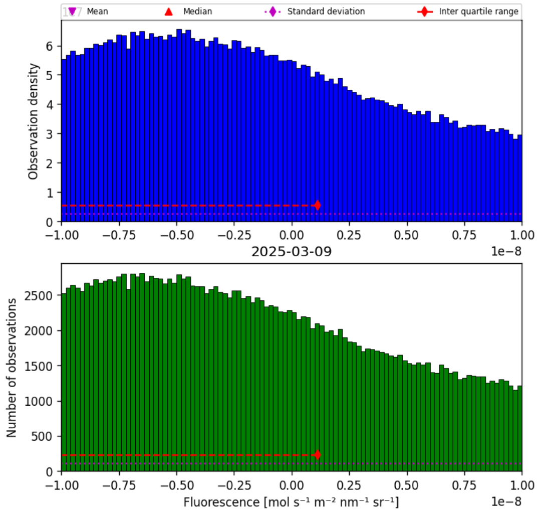
Figure 32: Histogram of “Fluorescence” for 2025-03-08 to 2025-03-10
