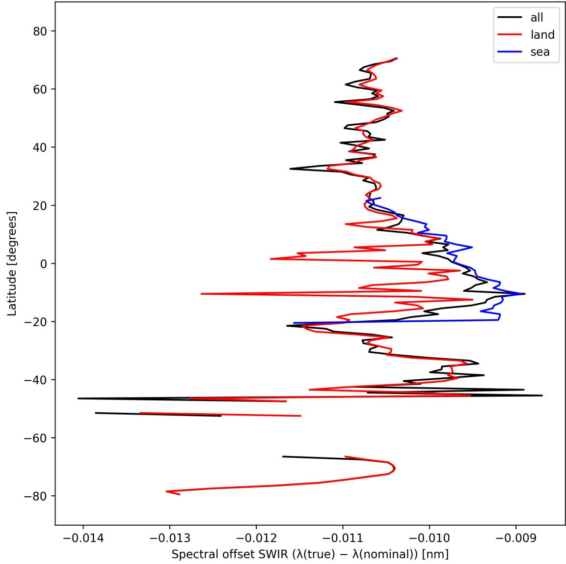
Figure 16: Zonal average of “Spectral offset SWIR ( \lambda_{\text{true}} - \lambda_{\text{nominal}} )” for 2025-03-08 to 2025-03-10.
