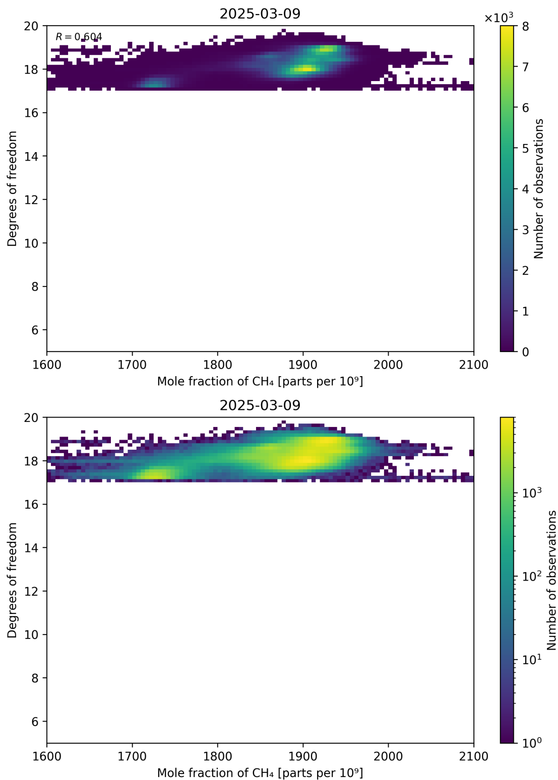
Figure 72: Scatter density plot of “Mole fraction of CH 4 ” against “Degrees of freedom” for 2025-03-08 to 2025-03-10.
