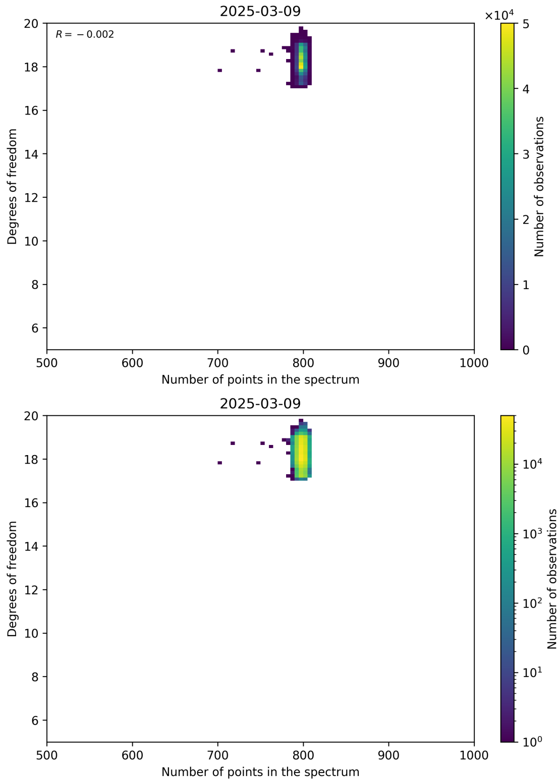
Figure 90: Scatter density plot of “Number of points in the spectrum” against “Degrees of freedom” for 2025-03-08 to 2025-03-10.
