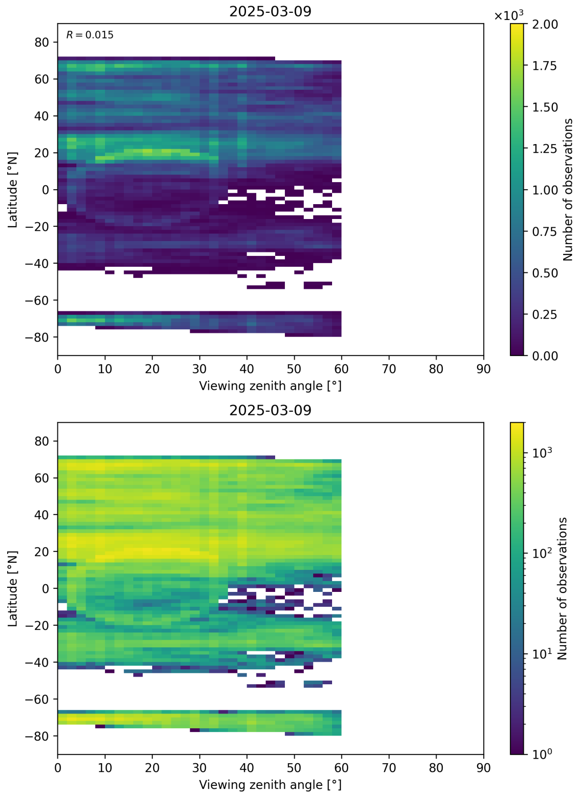
Figure 109: Scatter density plot of “Viewing zenith angle” against “Latitude” for 2025-03-08 to 2025-03-10.
