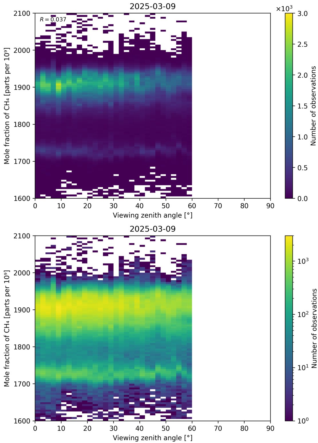
Figure 110: Scatter density plot of “Viewing zenith angle” against “Mole fraction of CH 4 ” for 2025-03-08 to 2025-03-10.
