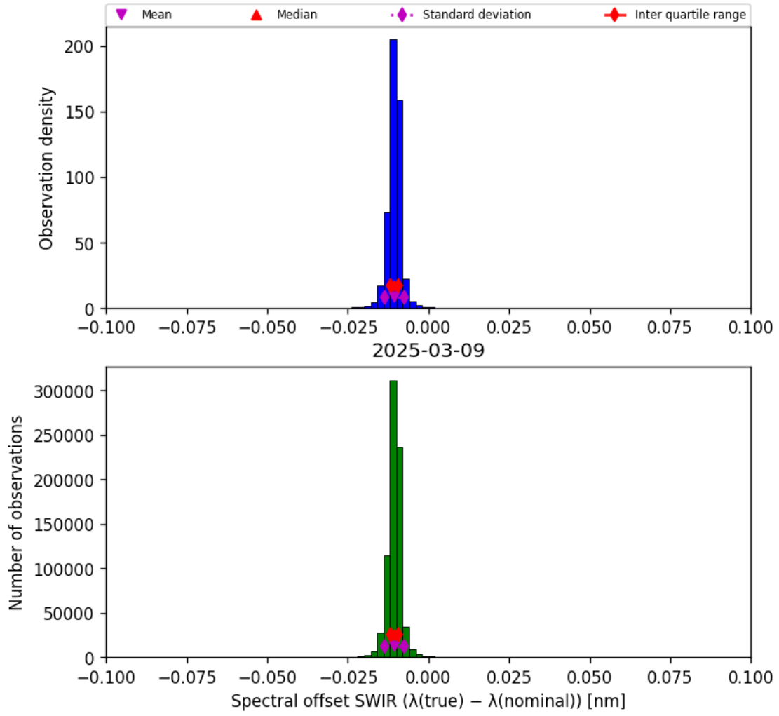
Figure 27: Histogram of “Spectral offset SWIR ( \lambda_{\text{true}} - \lambda_{\text{nominal}} )” for 2025-03-08 to 2025-03-10
