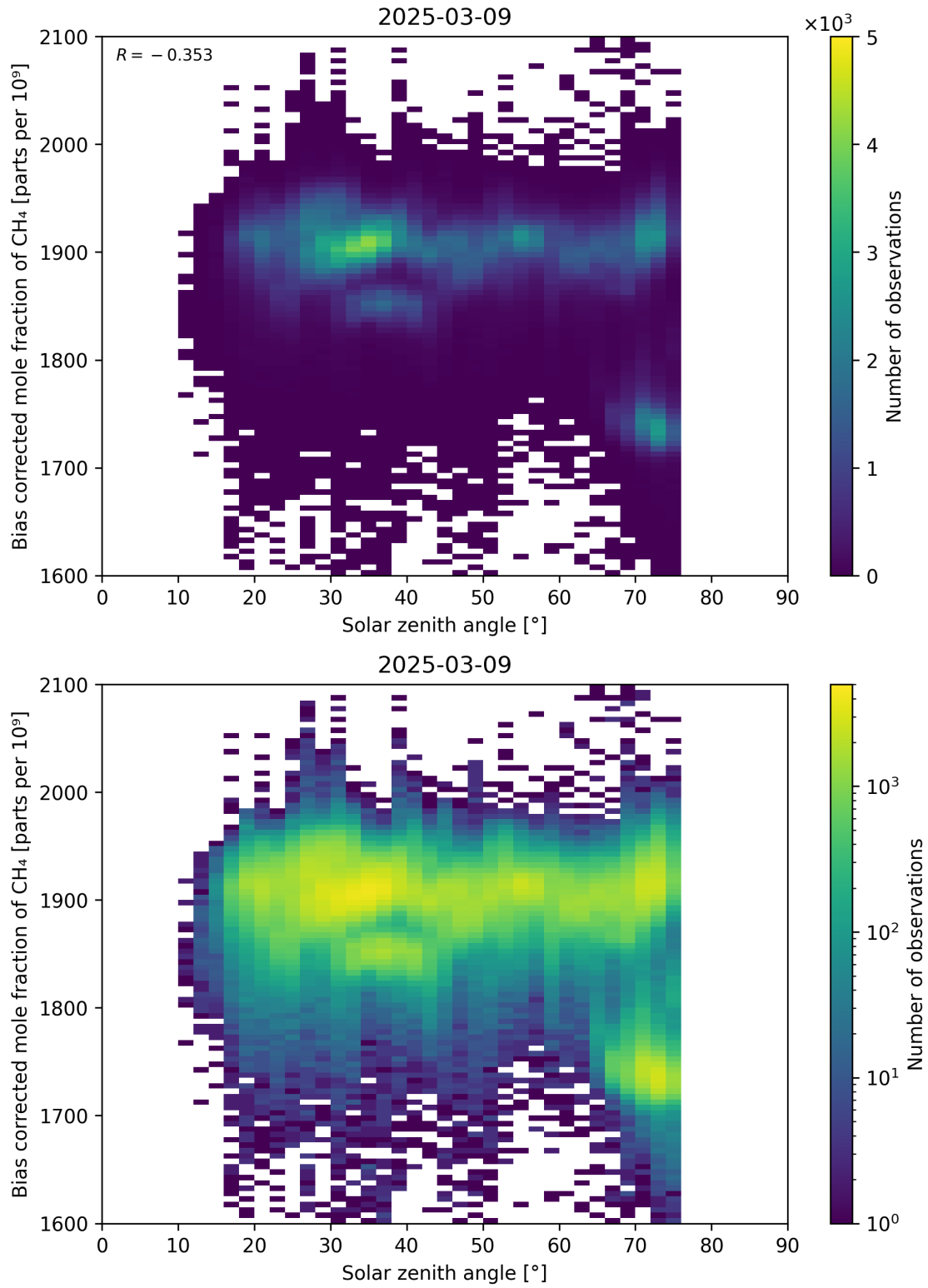
Figure 100: Scatter density plot of “Solar zenith angle” against “Bias corrected mole fraction of CH 4 ” for 2025-03-08 to 2025-03-10.
