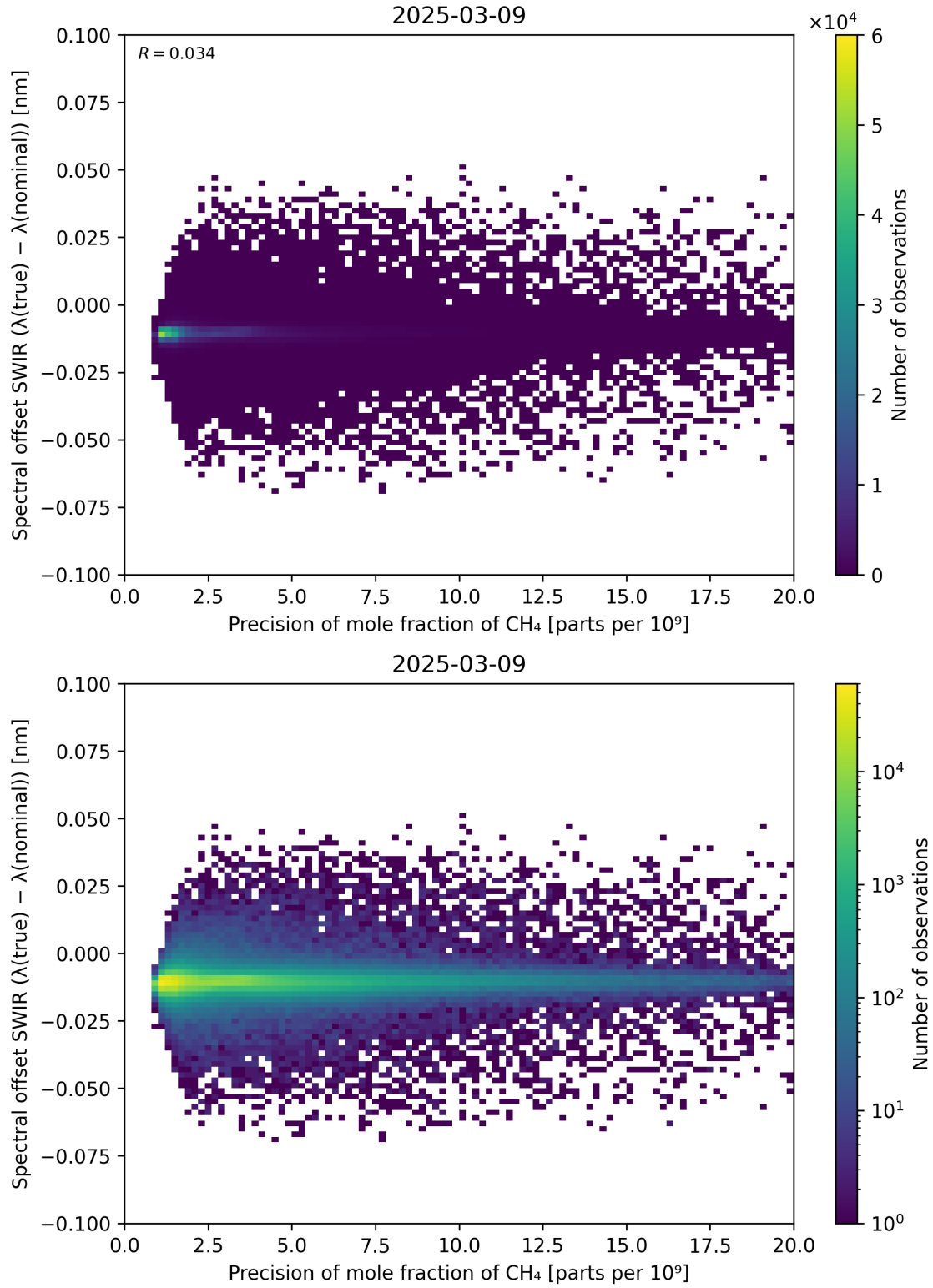
Figure 85: Scatter density plot of “Precision of mole fraction of \text{CH}_4 ” against “Spectral offset SWIR ( \lambda_{\text{true}} - \lambda_{\text{nominal}} )” for 2025-03-08 to 2025-03-10.
