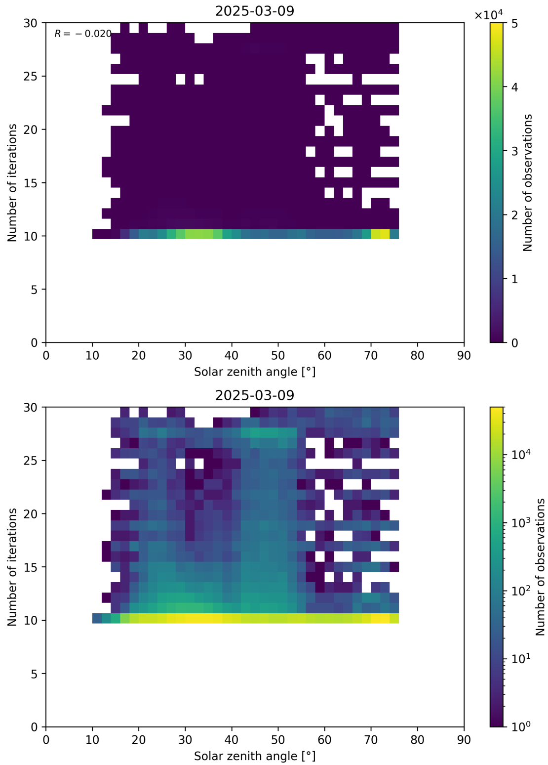
Figure 102: Scatter density plot of “Solar zenith angle” against “Number of iterations” for 2025-03-08 to 2025-03-10.
