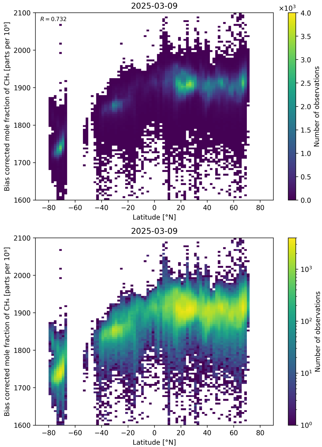
Figure 58: Scatter density plot of “Latitude” against “Bias corrected mole fraction of CH 4 ” for 2025-03-08 to 2025-03-10.
