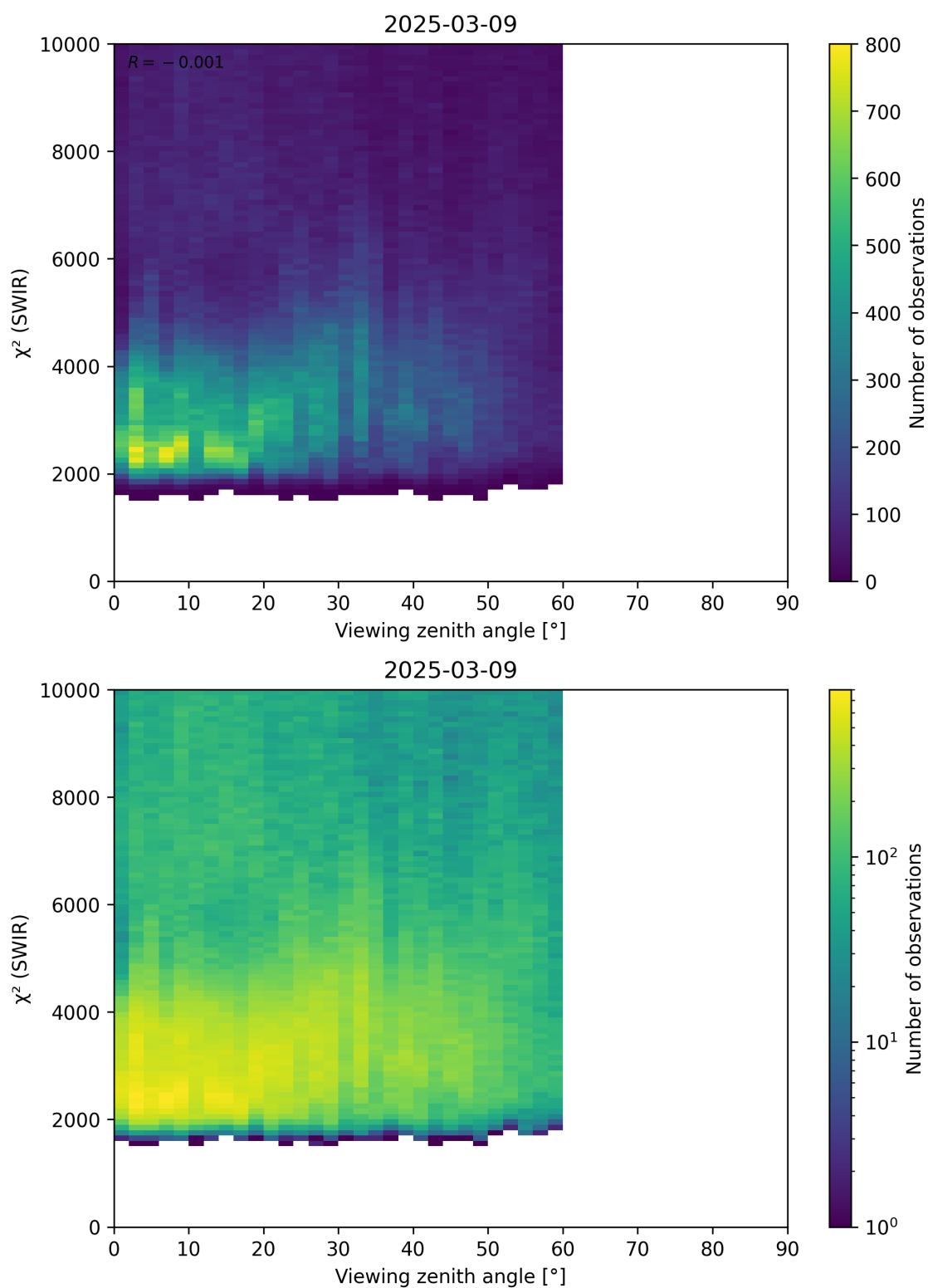
Figure 106: Scatter density plot of “Viewing zenith angle” against “ \chi^2 (SWIR)” for 2025-03-08 to 2025-03-10.
