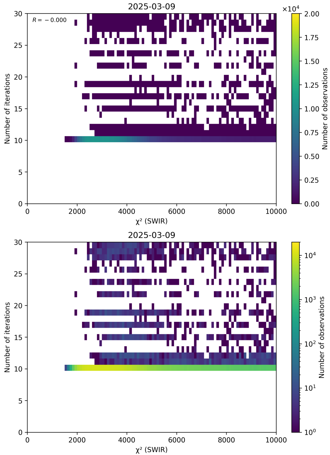
Figure 50: Scatter density plot of “ \chi^2 (SWIR)” against “Number of iterations” for 2025-03-08 to 2025-03-10.
