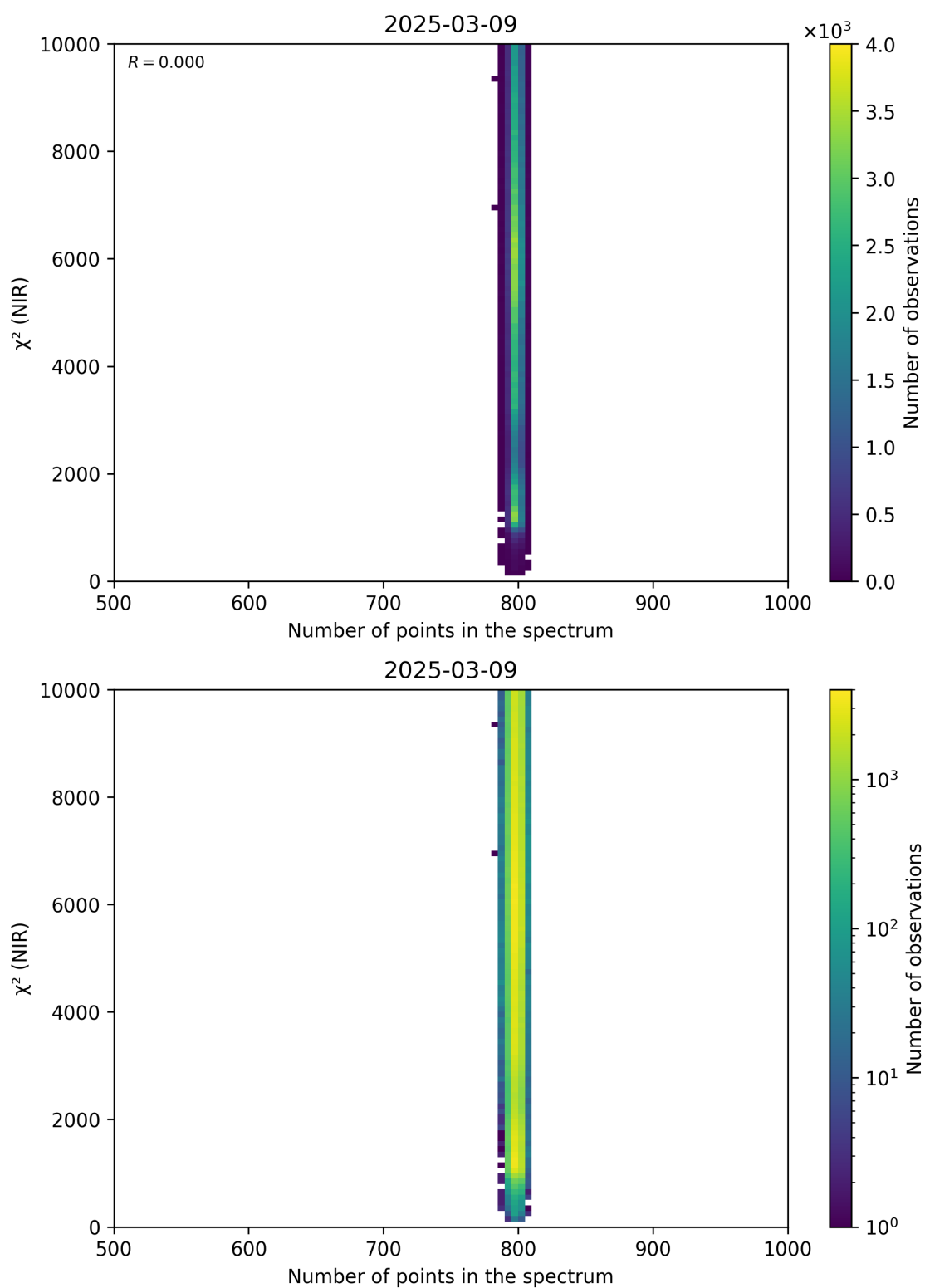
Figure 88: Scatter density plot of “Number of points in the spectrum” against “ \chi^2 (NIR)” for 2025-03-08 to 2025-03-10.
