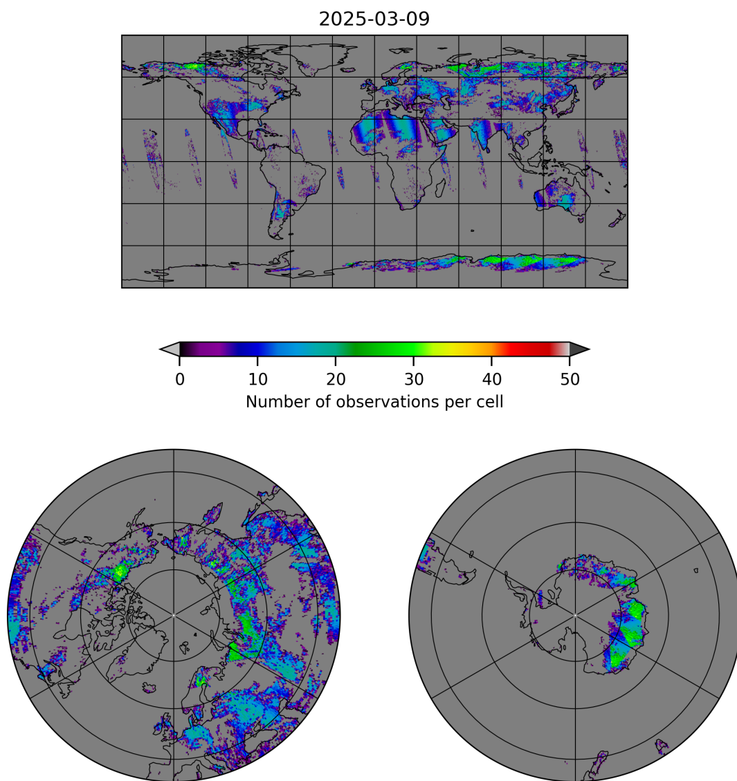
Figure 10: Map of the number of observations for 2025-03-08 to 2025-03-10
