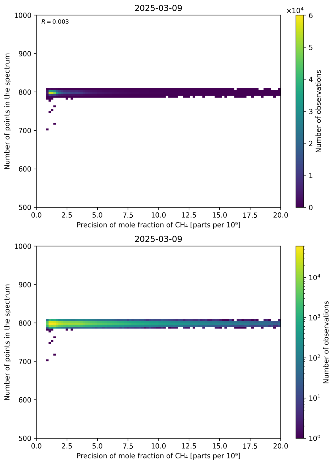
Figure 84: Scatter density plot of “Precision of mole fraction of CH 4 ” against “Number of points in the spectrum” for 2025-03-08 to 2025-03-10.
