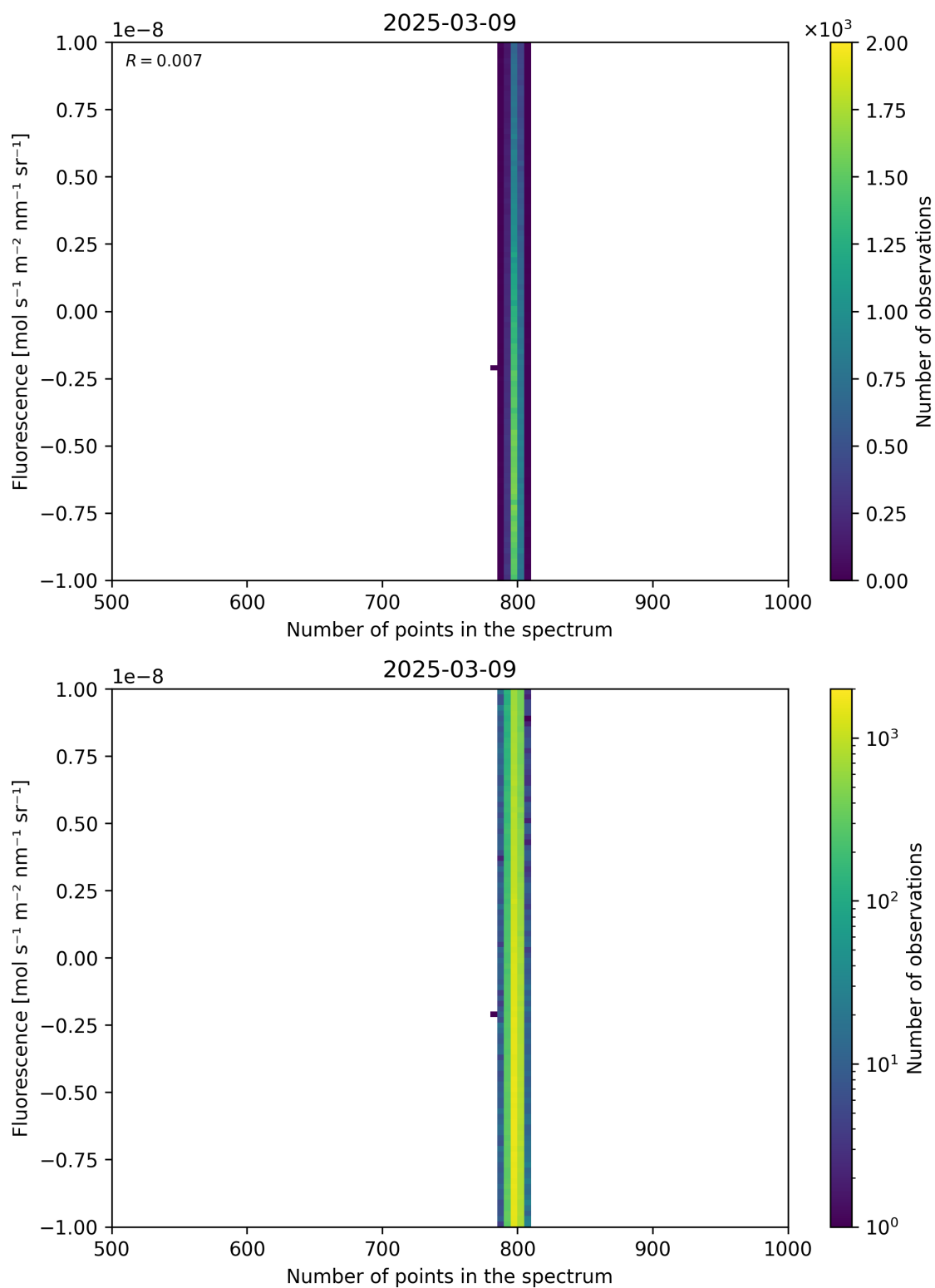
Figure 91: Scatter density plot of “Number of points in the spectrum” against “Fluorescence” for 2025-03-08 to 2025-03-10.
