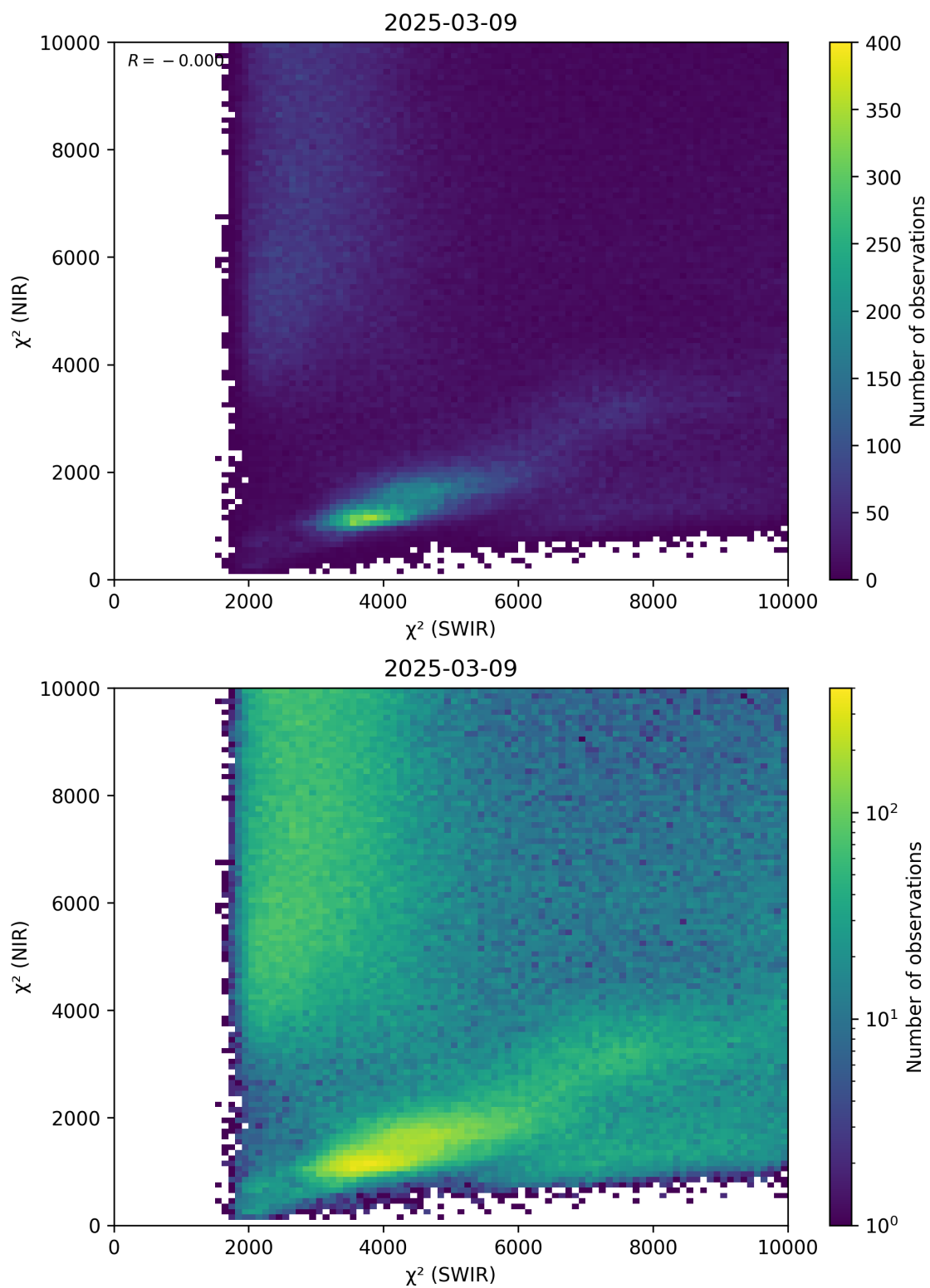
Figure 47: Scatter density plot of “ \chi^2 (SWIR)” against “ \chi^2 (NIR)” for 2025-03-08 to 2025-03-10.
