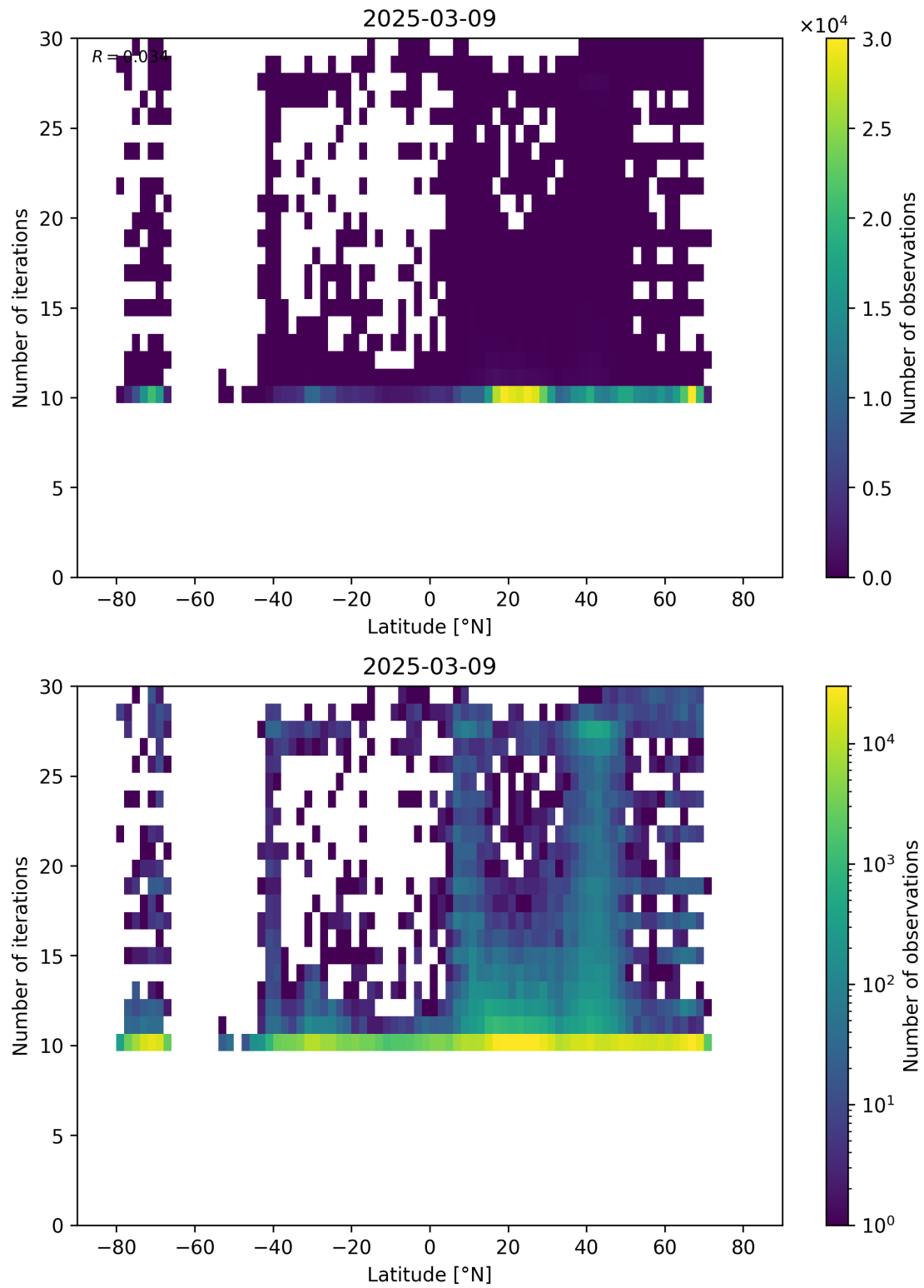
Figure 60: Scatter density plot of “Latitude” against “Number of iterations” for 2025-03-08 to 2025-03-10.
