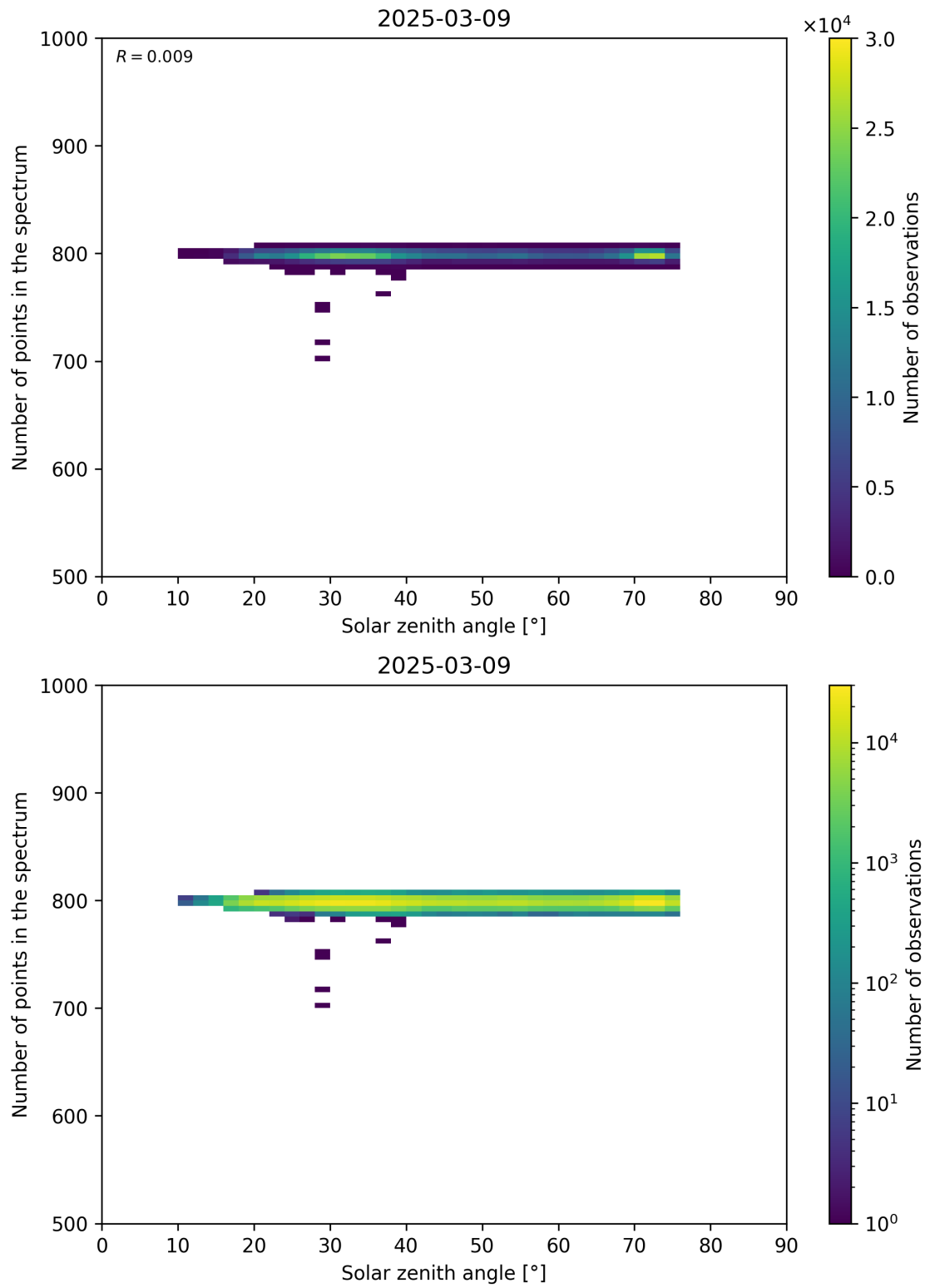
Figure 103: Scatter density plot of “Solar zenith angle” against “Number of points in the spectrum” for 2025-03-08 to 2025-03-10.
