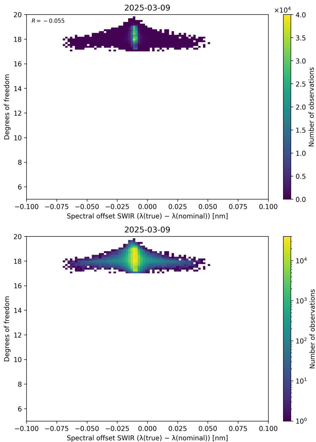
Figure 119: Scatter density plot of “Spectral offset SWIR ( \lambda_{\text{true}} - \lambda_{\text{nominal}} )” against “Degrees of freedom” for 2025-03-08 to 2025-03-10.
