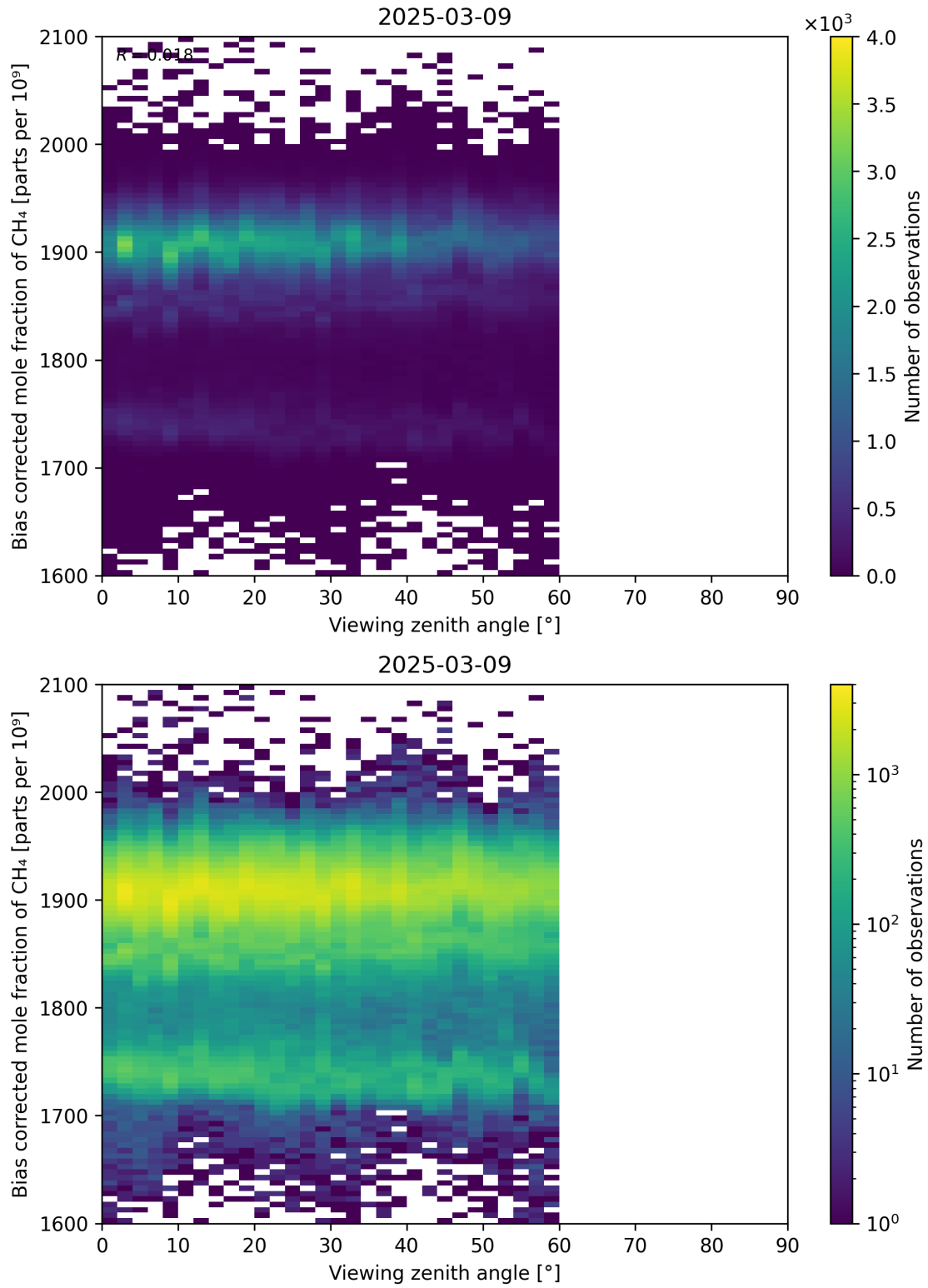
Figure 111: Scatter density plot of “Viewing zenith angle” against “Bias corrected mole fraction of CH 4 ” for 2025-03-08 to 2025-03-10.
