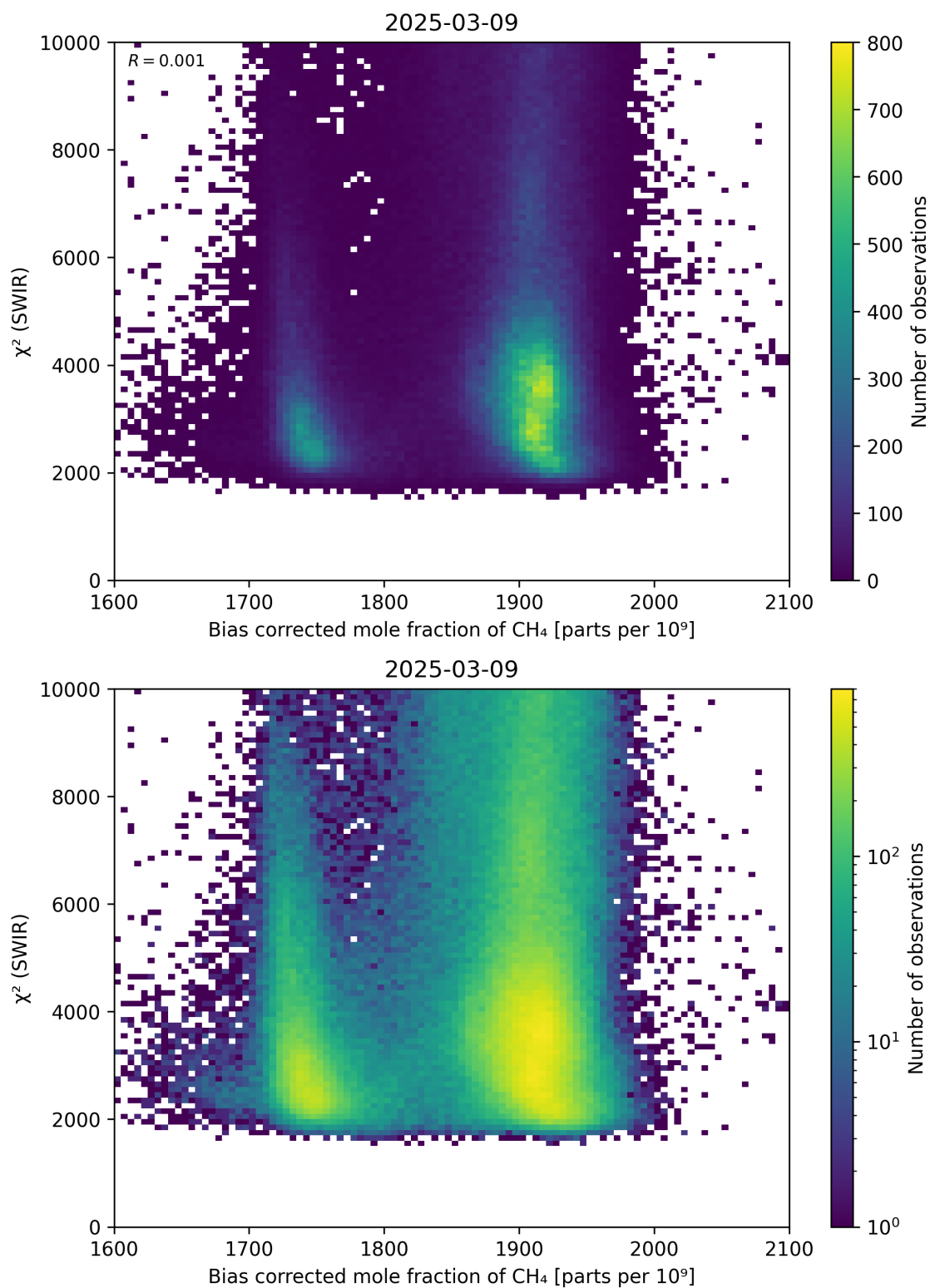
Figure 64: Scatter density plot of “Bias corrected mole fraction of \text{CH}_4 ” against “ \chi^2 (SWIR)” for 2025-03-08 to 2025-03-10.
