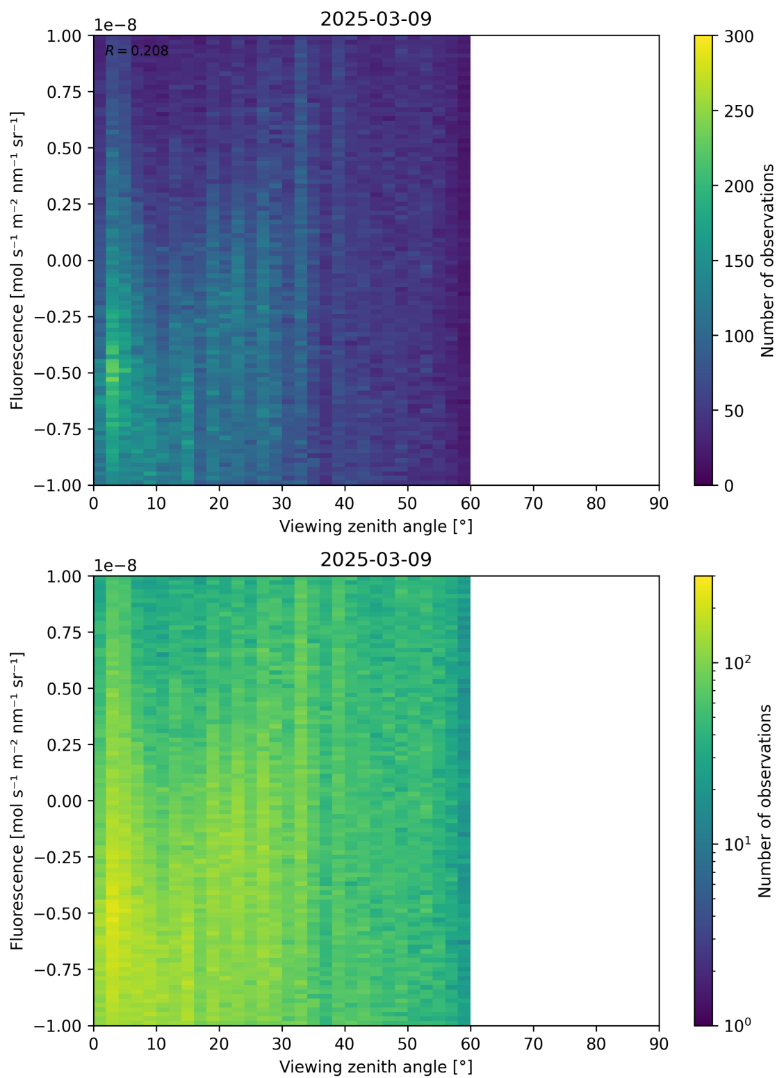
Figure 108: Scatter density plot of “Viewing zenith angle” against “Fluorescence” for 2025-03-08 to 2025-03-10.
