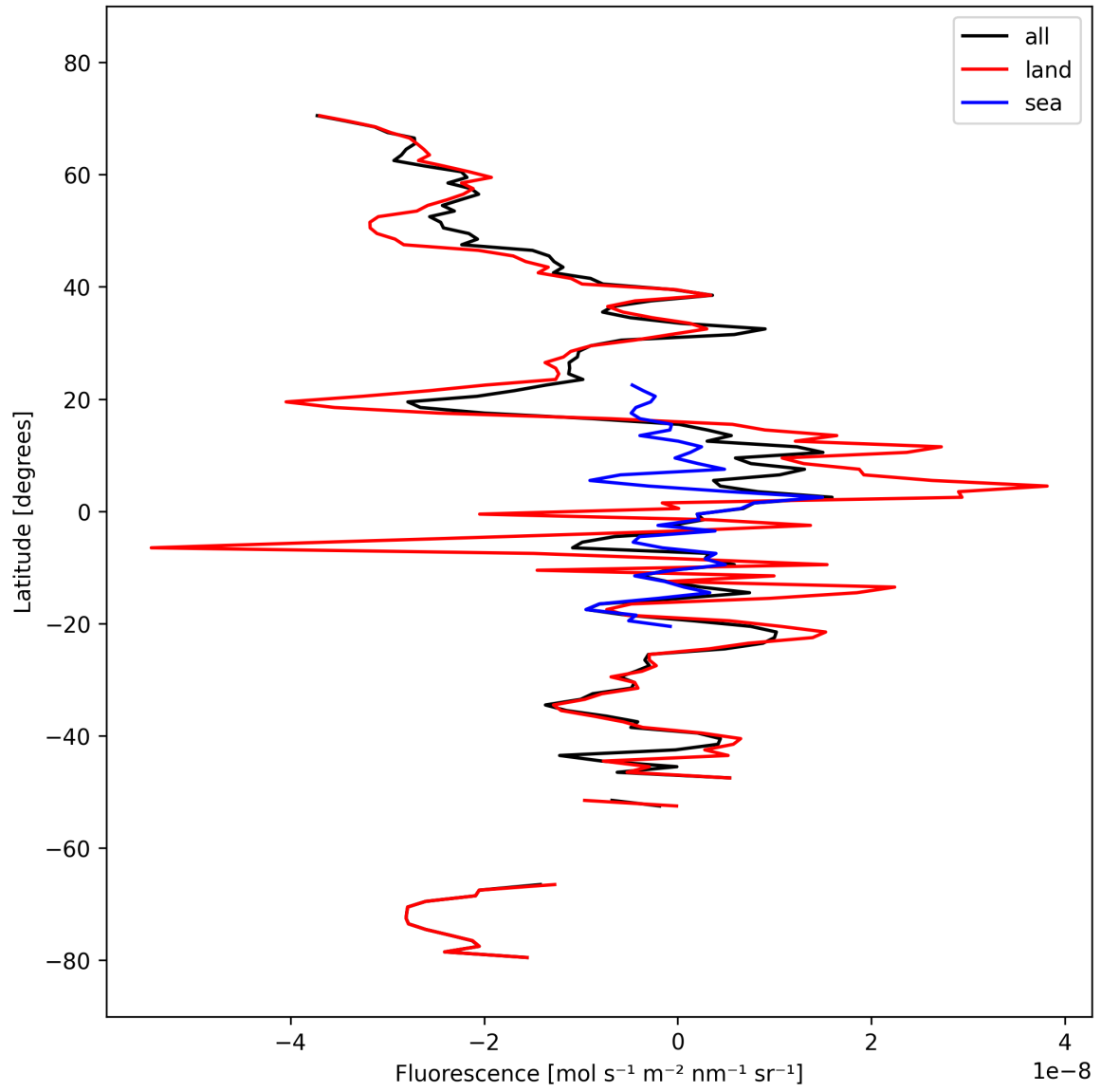
Figure 21: Zonal average of “Fluorescence” for 2025-03-08 to 2025-03-10.
