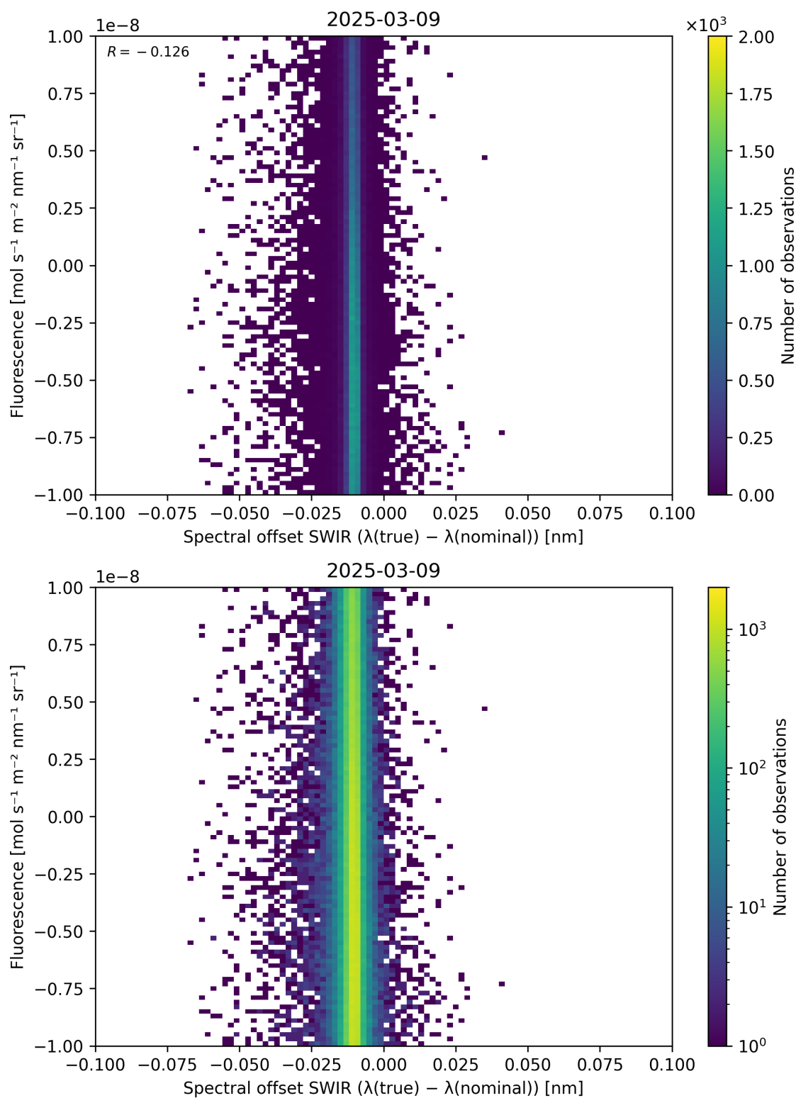
Figure 120: Scatter density plot of “Spectral offset SWIR ( \lambda_{\text{true}} - \lambda_{\text{nominal}} )” against “Fluorescence” for 2025-03-08 to 2025-03-10.
