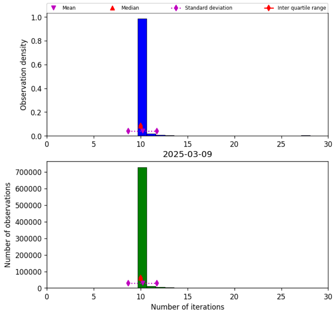
Figure 31: Histogram of “Number of iterations” for 2025-03-08 to 2025-03-10
