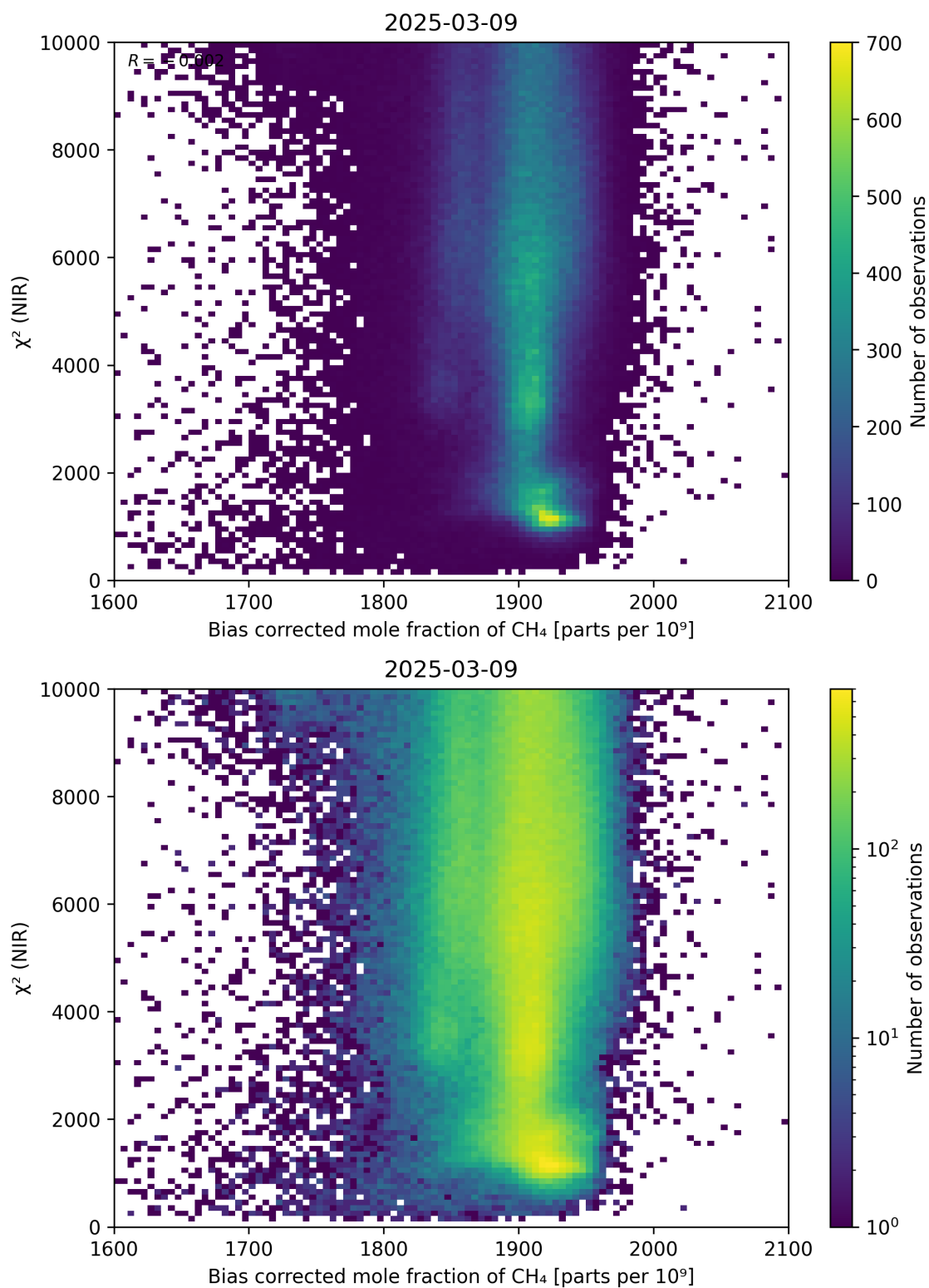
Figure 63: Scatter density plot of “Bias corrected mole fraction of \text{CH}_4 ” against “ \chi^2 (NIR)” for 2025-03-08 to 2025-03-10.
