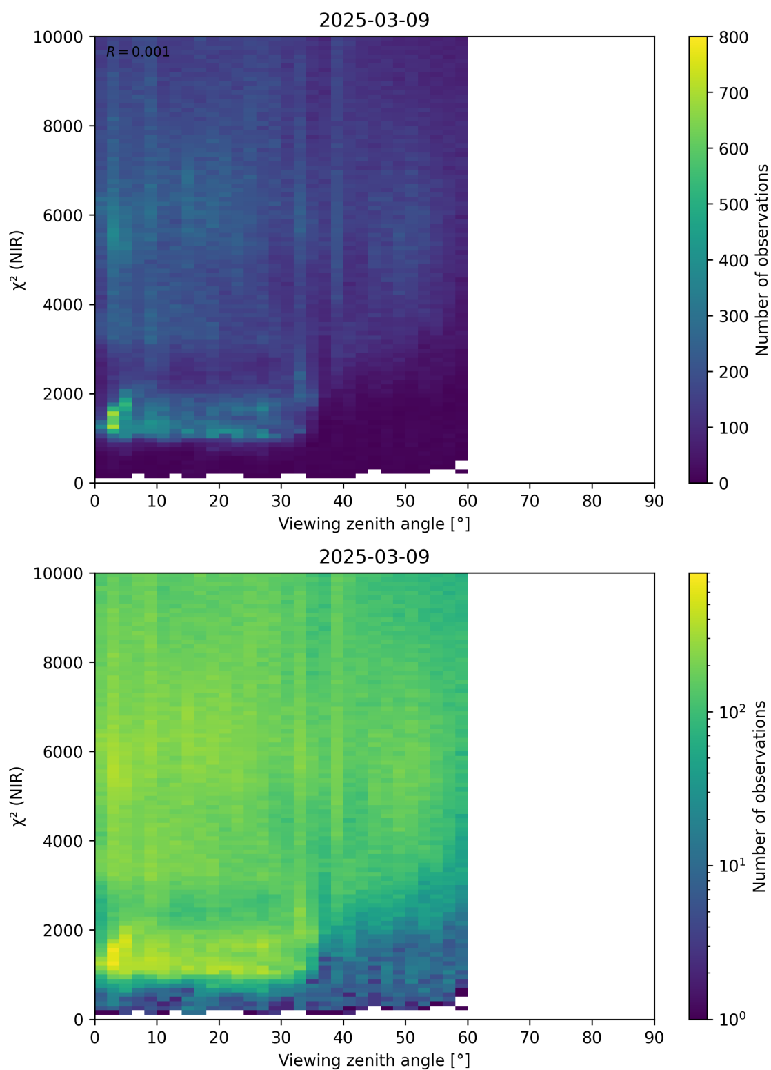
Figure 105: Scatter density plot of “Viewing zenith angle” against “ \chi^2 (NIR)” for 2025-03-08 to 2025-03-10.
