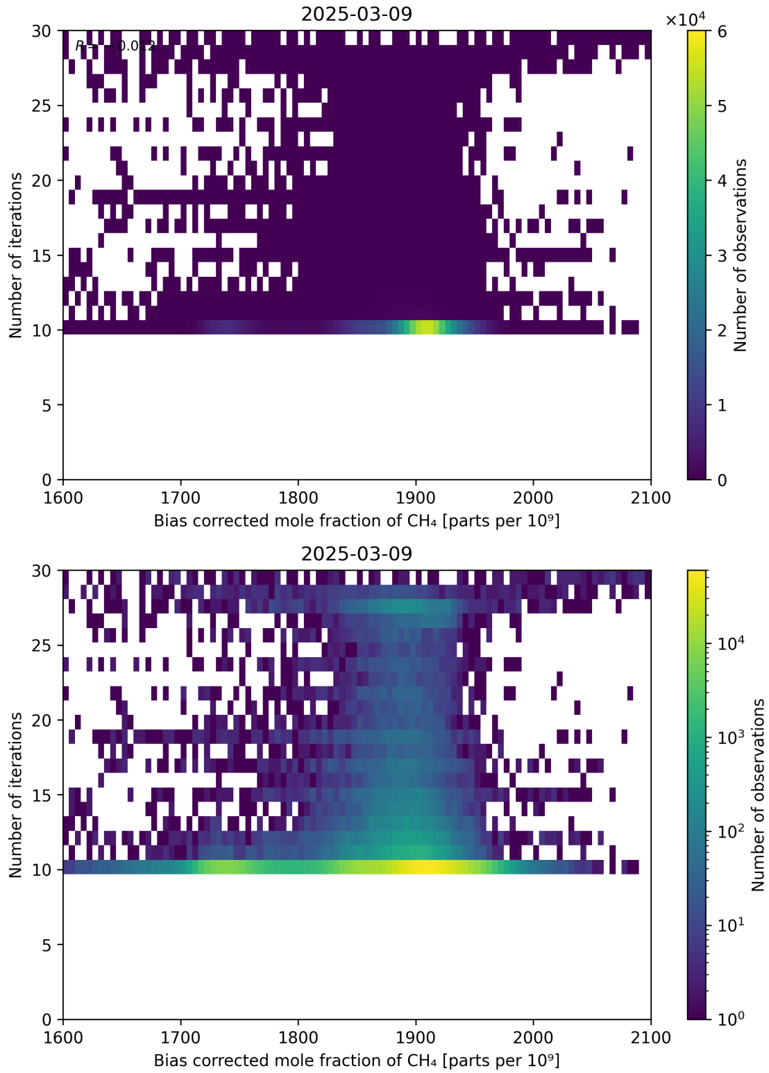
Figure 67: Scatter density plot of “Bias corrected mole fraction of \text{CH}_4 ” against “Number of iterations” for 2025-03-08 to 2025-03-10.
