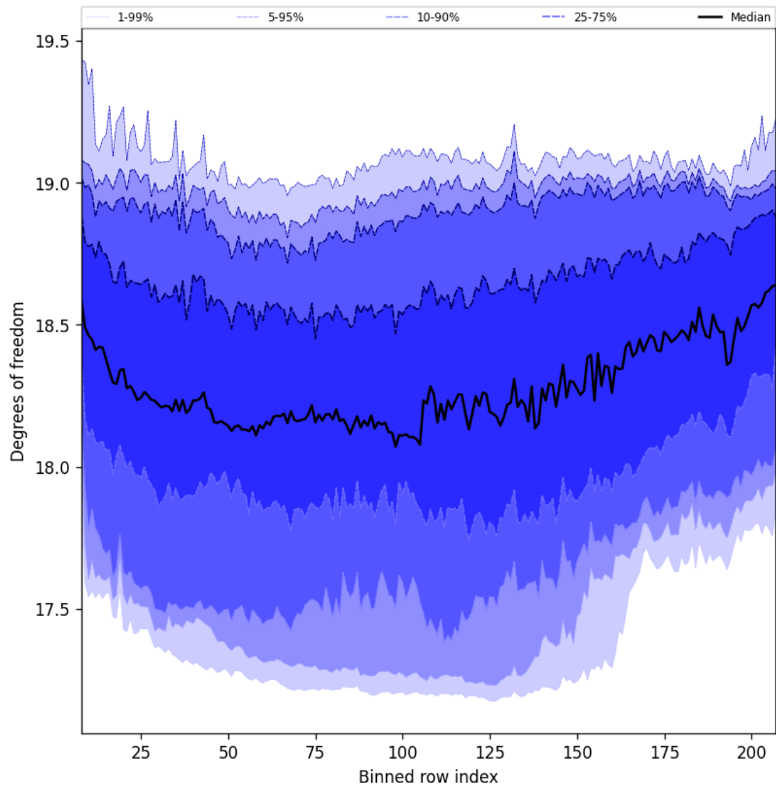
Figure 41: Along track statistics of “Degrees of freedom” for 2025-03-08 to 2025-03-10
