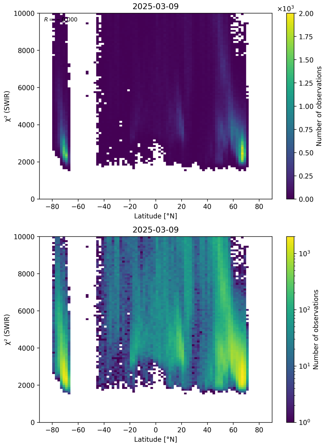
Figure 54: Scatter density plot of “Latitude” against “ \chi^2 (SWIR)” for 2025-03-08 to 2025-03-10.
