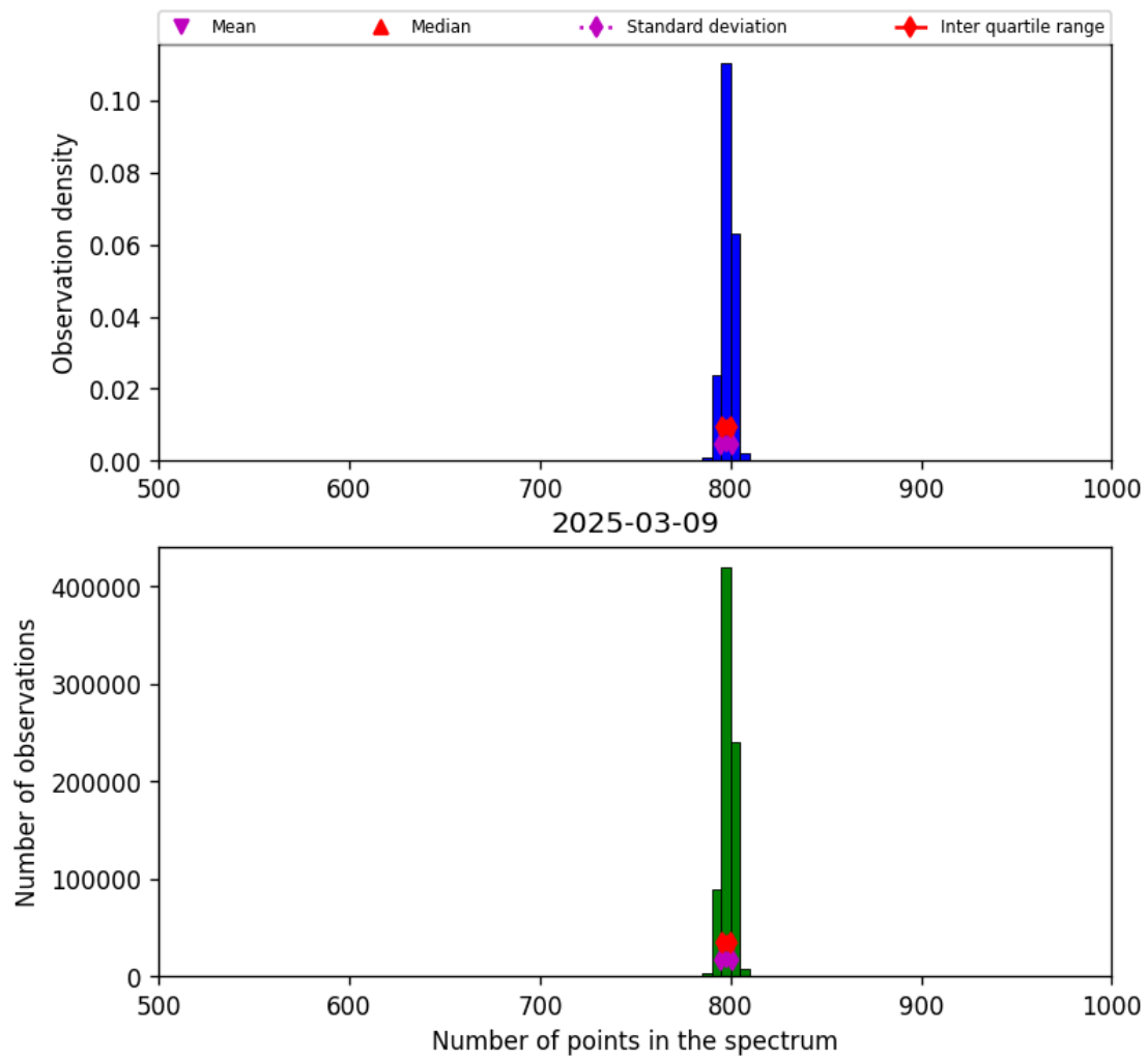
Figure 26: Histogram of “Number of points in the spectrum” for 2025-03-08 to 2025-03-10
