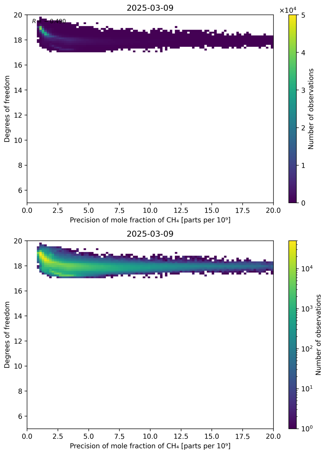
Figure 80: Scatter density plot of “Precision of mole fraction of CH 4 ” against “Degrees of freedom” for 2025-03-08 to 2025-03-10.
