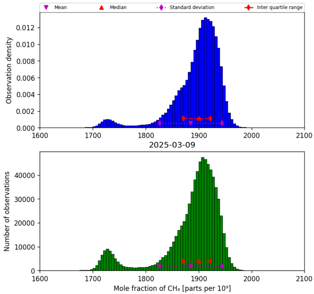
Figure 23: Histogram of “Mole fraction of CH 4 ” for 2025-03-08 to 2025-03-10
