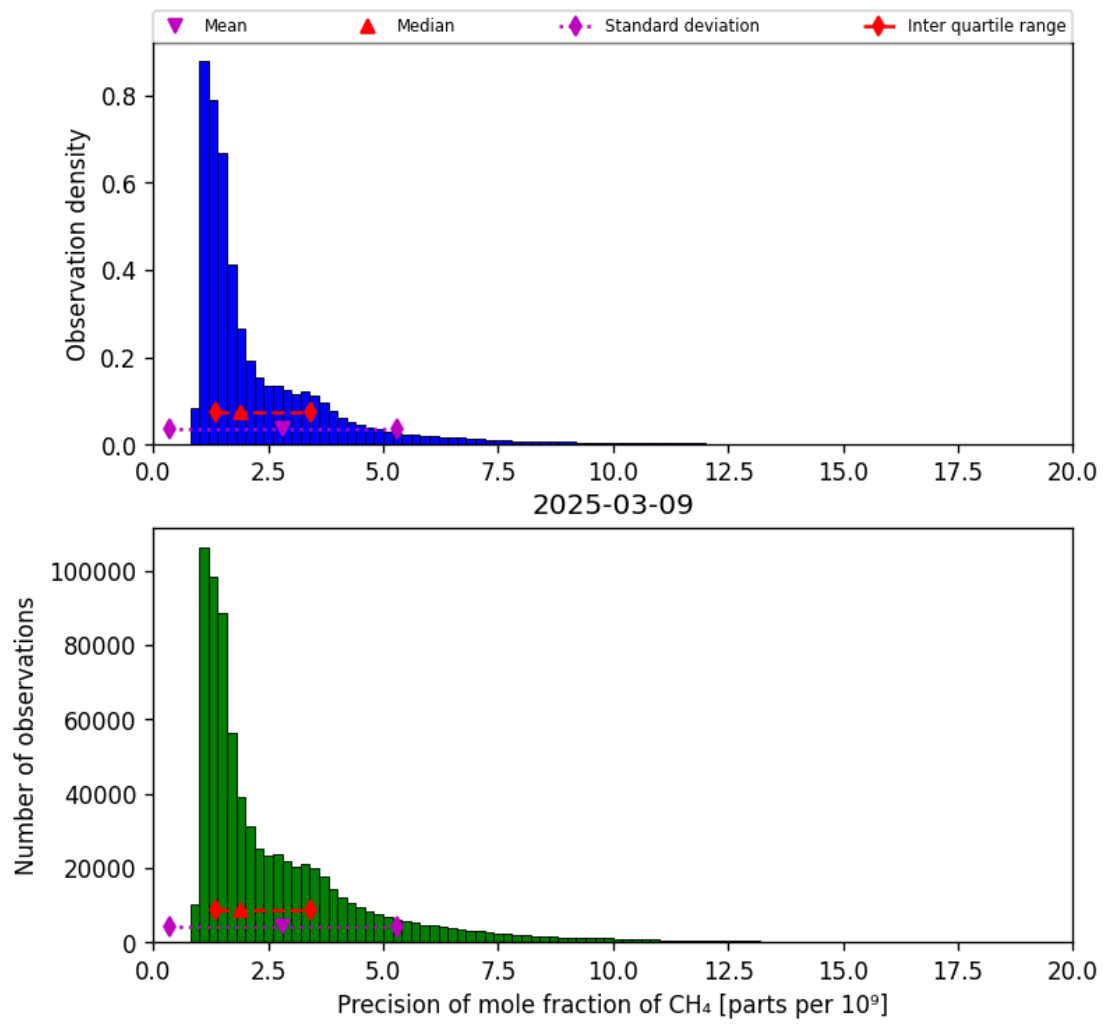
Figure 24: Histogram of “Precision of mole fraction of CH 4 ” for 2025-03-08 to 2025-03-10
