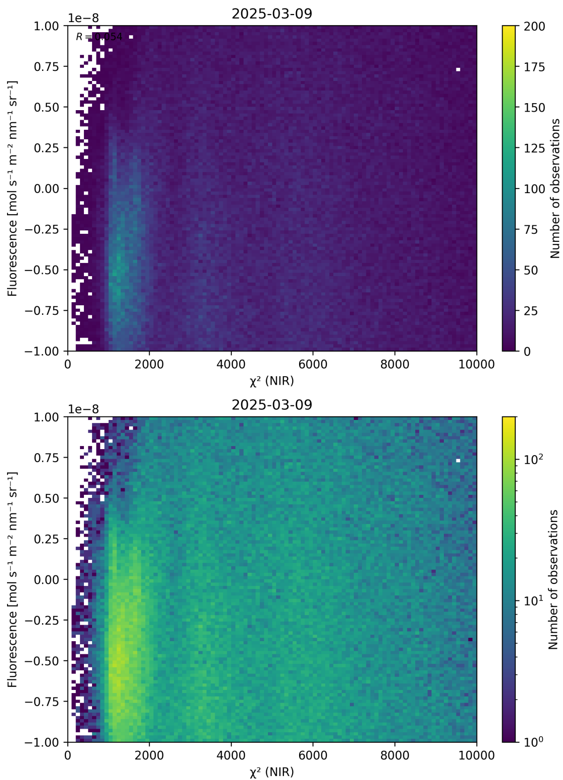
Figure 45: Scatter density plot of “ \chi^2 (NIR)” against “Fluorescence” for 2025-03-08 to 2025-03-10.
