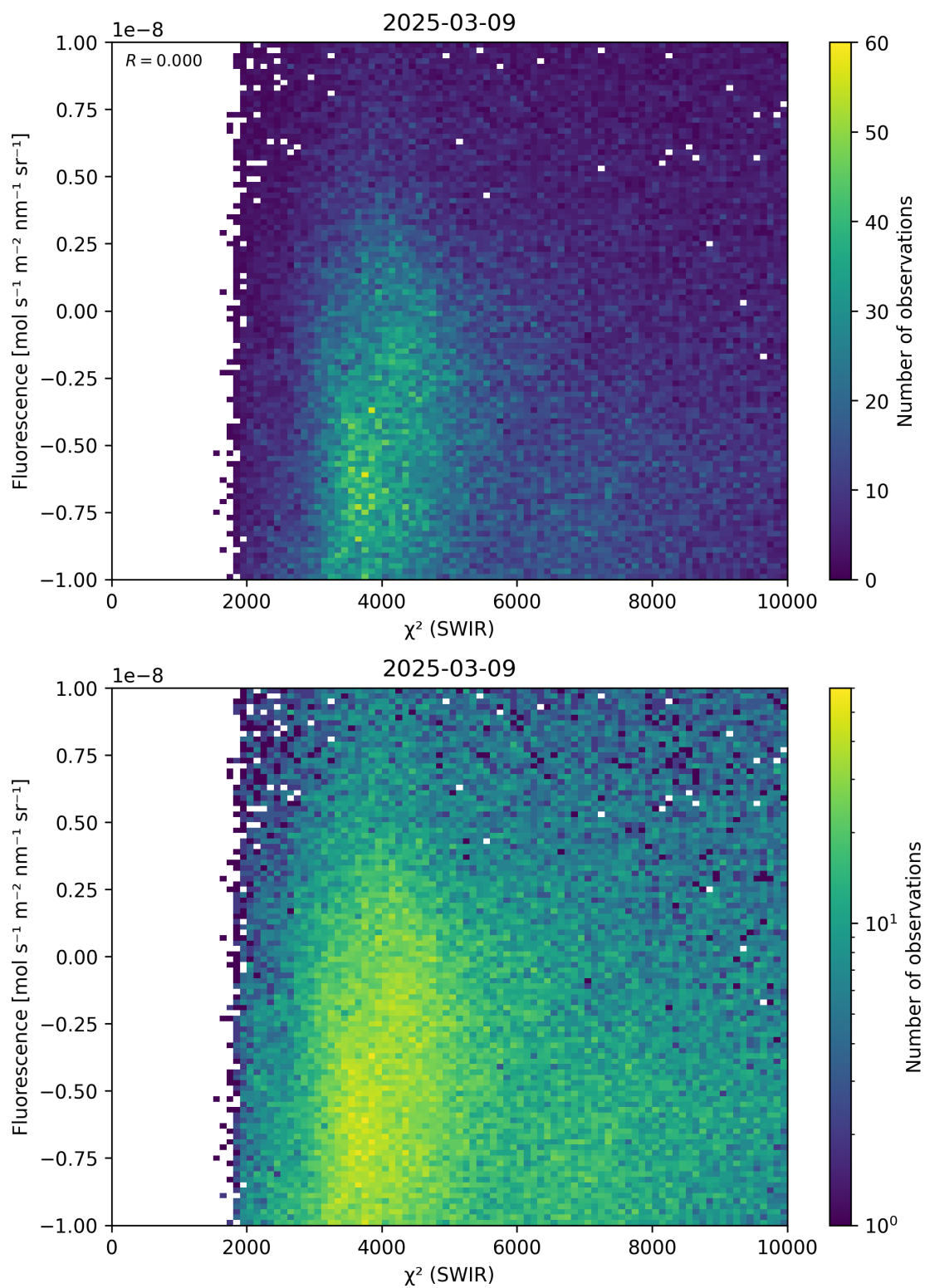
Figure 49: Scatter density plot of “ \chi^2 (SWIR)” against “Fluorescence” for 2025-03-08 to 2025-03-10.
