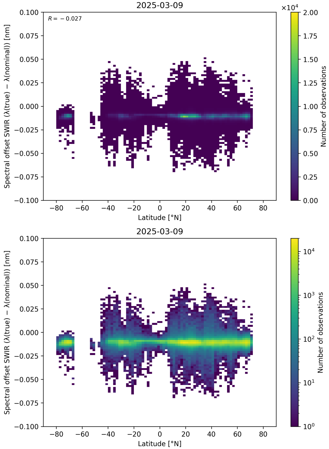
Figure 62: Scatter density plot of “Latitude” against “Spectral offset SWIR ( \lambda_{\text{true}} - \lambda_{\text{nominal}} )” for 2025-03-08 to 2025-03-10.
