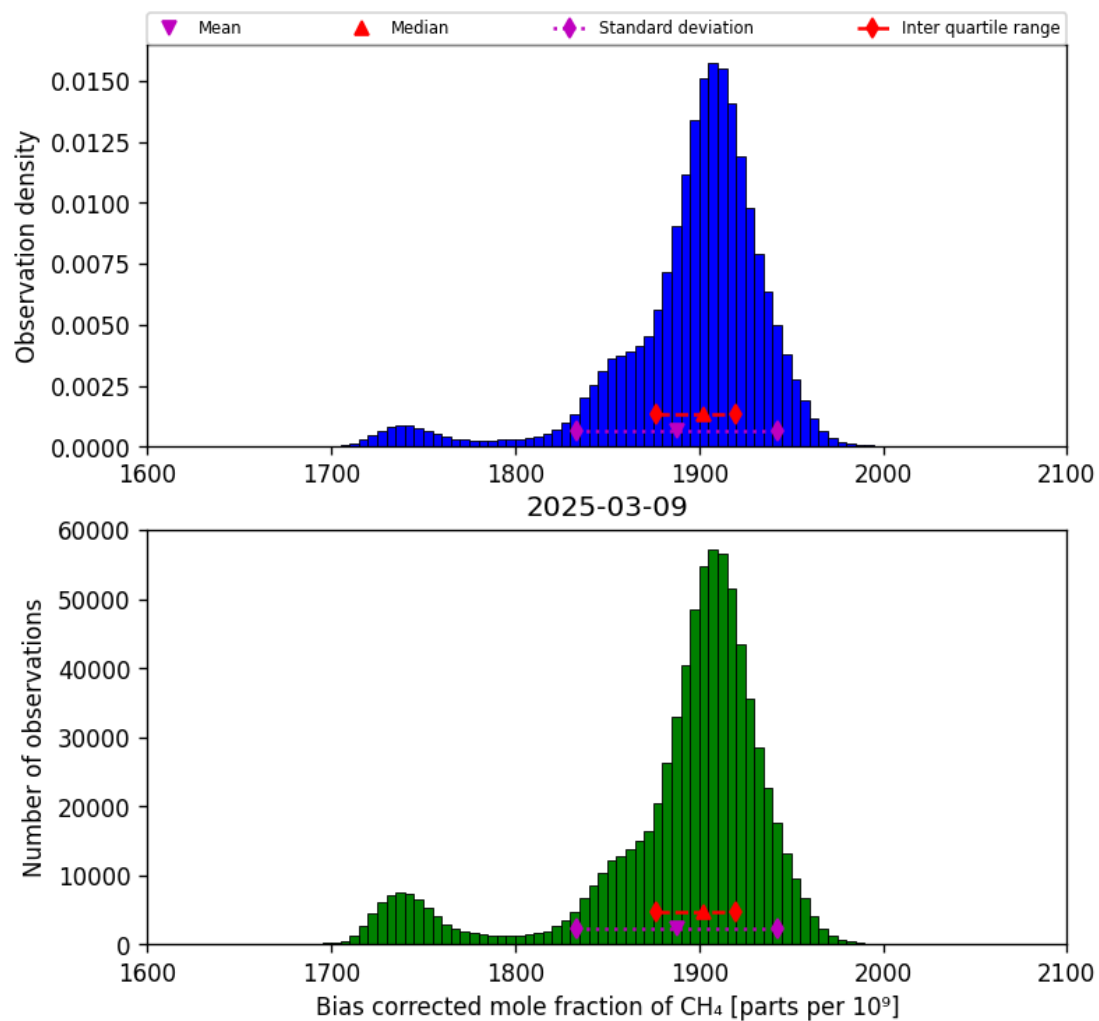
Figure 25: Histogram of “Bias corrected mole fraction of CH 4 ” for 2025-03-08 to 2025-03-10
