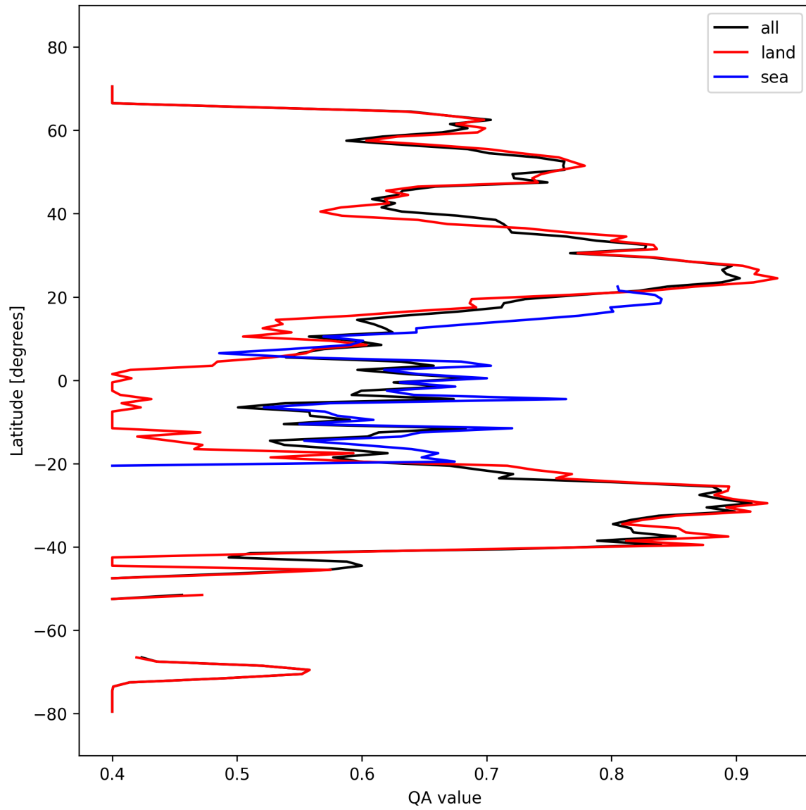
Figure 11: Zonal average of “QA value” for 2025-03-08 to 2025-03-10.
