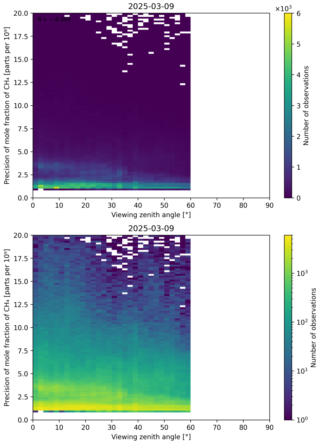
Figure 112: Scatter density plot of “Viewing zenith angle” against “Precision of mole fraction of CH 4 ” for 2025-03-08 to 2025-03-10.
