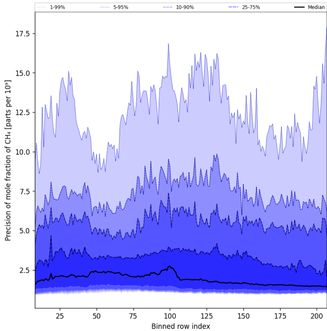
Figure 35: Along track statistics of “Precision of mole fraction of CH 4 ” for 2025-03-08 to 2025-03-10
