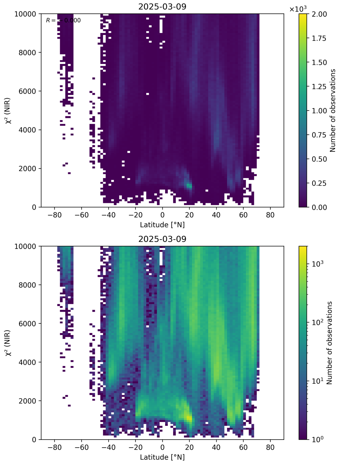
Figure 53: Scatter density plot of “Latitude” against “ \chi^2 (NIR)” for 2025-03-08 to 2025-03-10.
