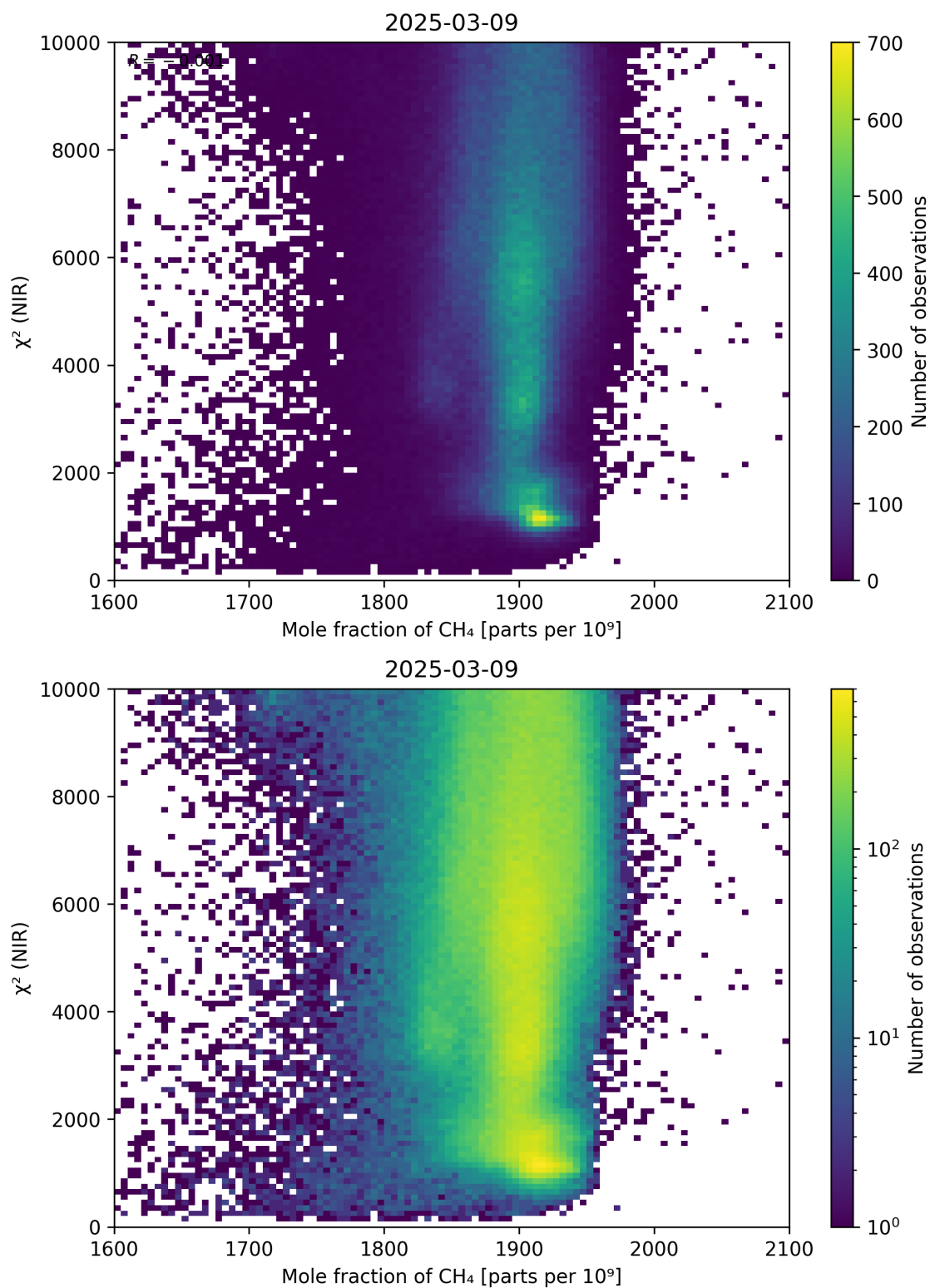
Figure 70: Scatter density plot of “Mole fraction of CH 4 ” against “ \chi^2 (NIR)” for 2025-03-08 to 2025-03-10.
