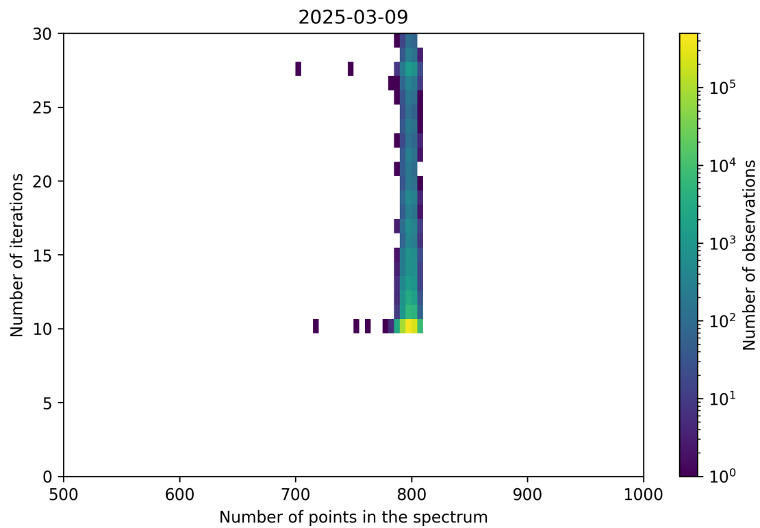
Figure 92: Scatter density plot of “Number of points in the spectrum” against “Number of iterations” for 2025-03-08 to 2025-03-10.
