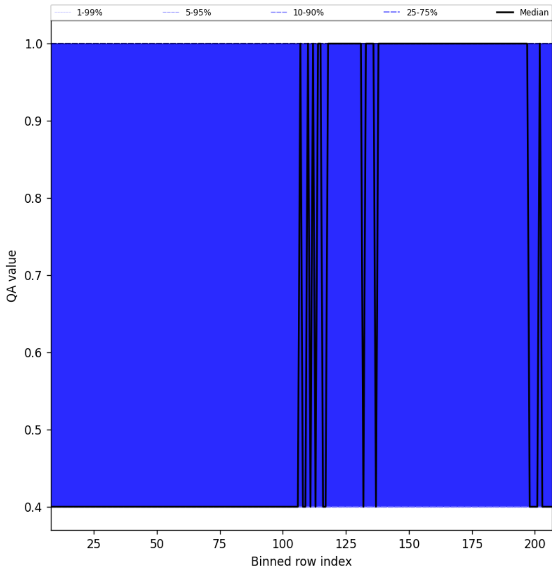
Figure 33: Along track statistics of “QA value” for 2025-03-08 to 2025-03-10
