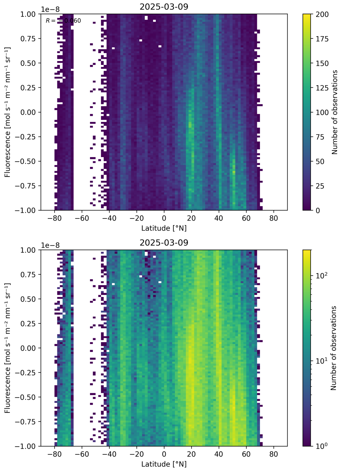
Figure 56: Scatter density plot of “Latitude” against “Fluorescence” for 2025-03-08 to 2025-03-10.
