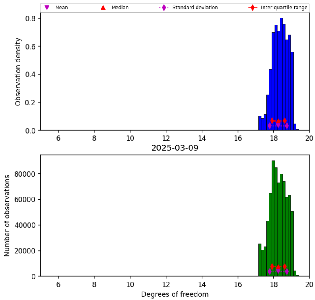
Figure 30: Histogram of “Degrees of freedom” for 2025-03-08 to 2025-03-10
