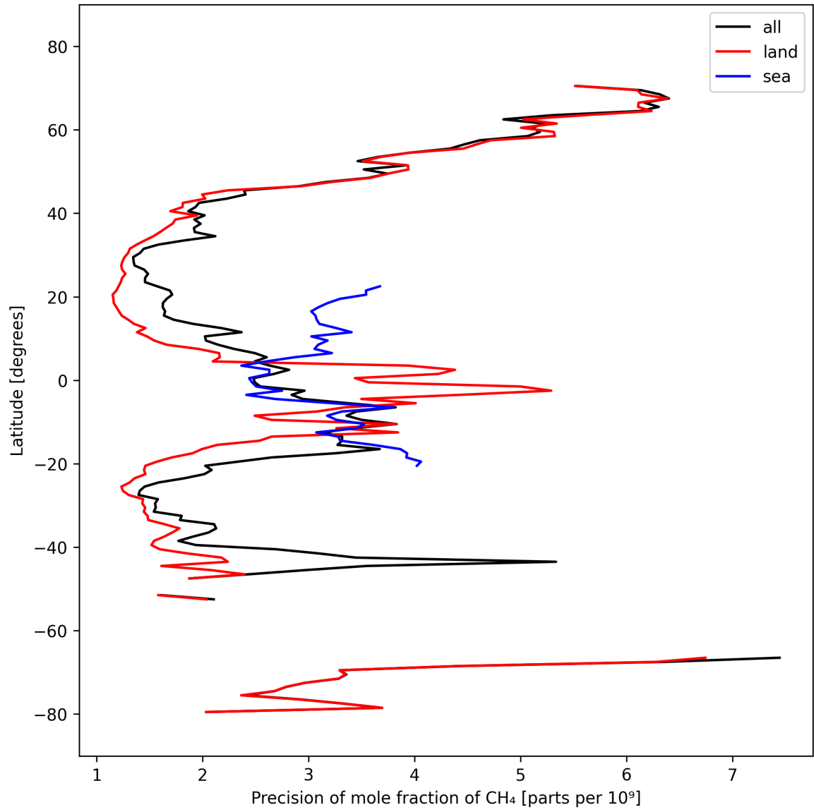
Figure 13: Zonal average of “Precision of mole fraction of CH 4 ” for 2025-03-08 to 2025-03-10.
