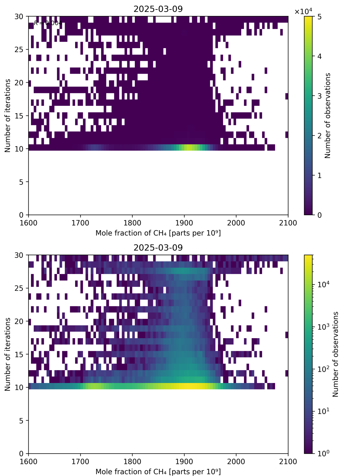
Figure 76: Scatter density plot of “Mole fraction of CH 4 ” against “Number of iterations” for 2025-03-08 to 2025-03-10.
