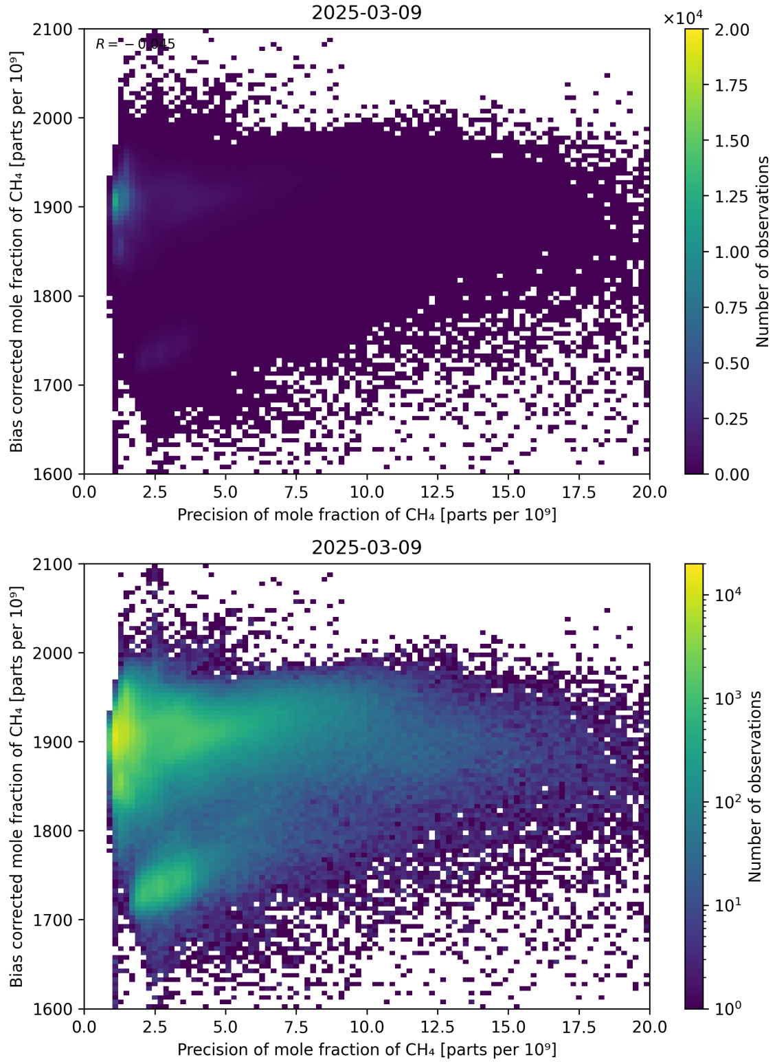
Figure 82: Scatter density plot of “Precision of mole fraction of CH 4 ” against “Bias corrected mole fraction of CH 4 ” for 2025-03-08 to 2025-03-10.
