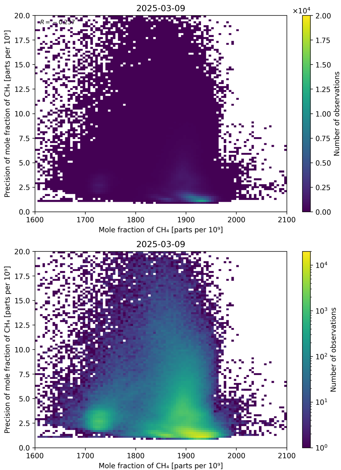
Figure 75: Scatter density plot of “Mole fraction of CH 4 ” against “Precision of mole fraction of CH 4 ” for 2025-03-08 to 2025-03-10.
