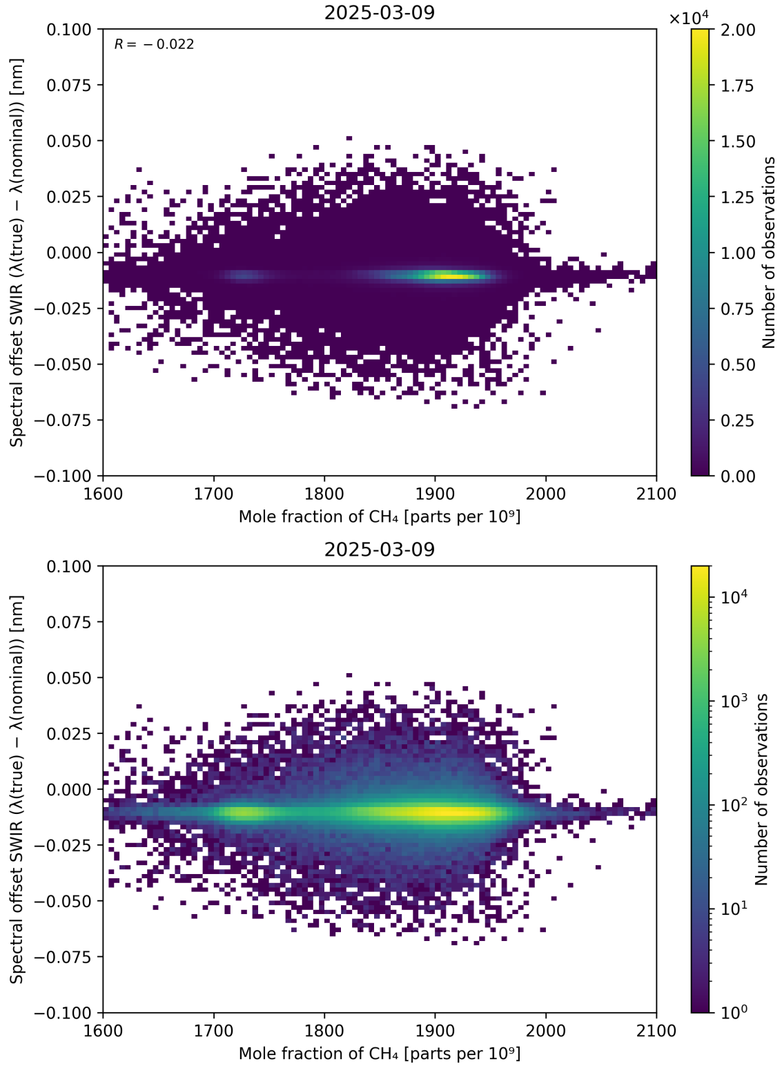
Figure 86: Scatter density plot of “Mole fraction of CH 4 ” against “Spectral offset SWIR ( \lambda_{\text{true}} - \lambda_{\text{nominal}} )” for 2025-03-08 to 2025-03-10.
