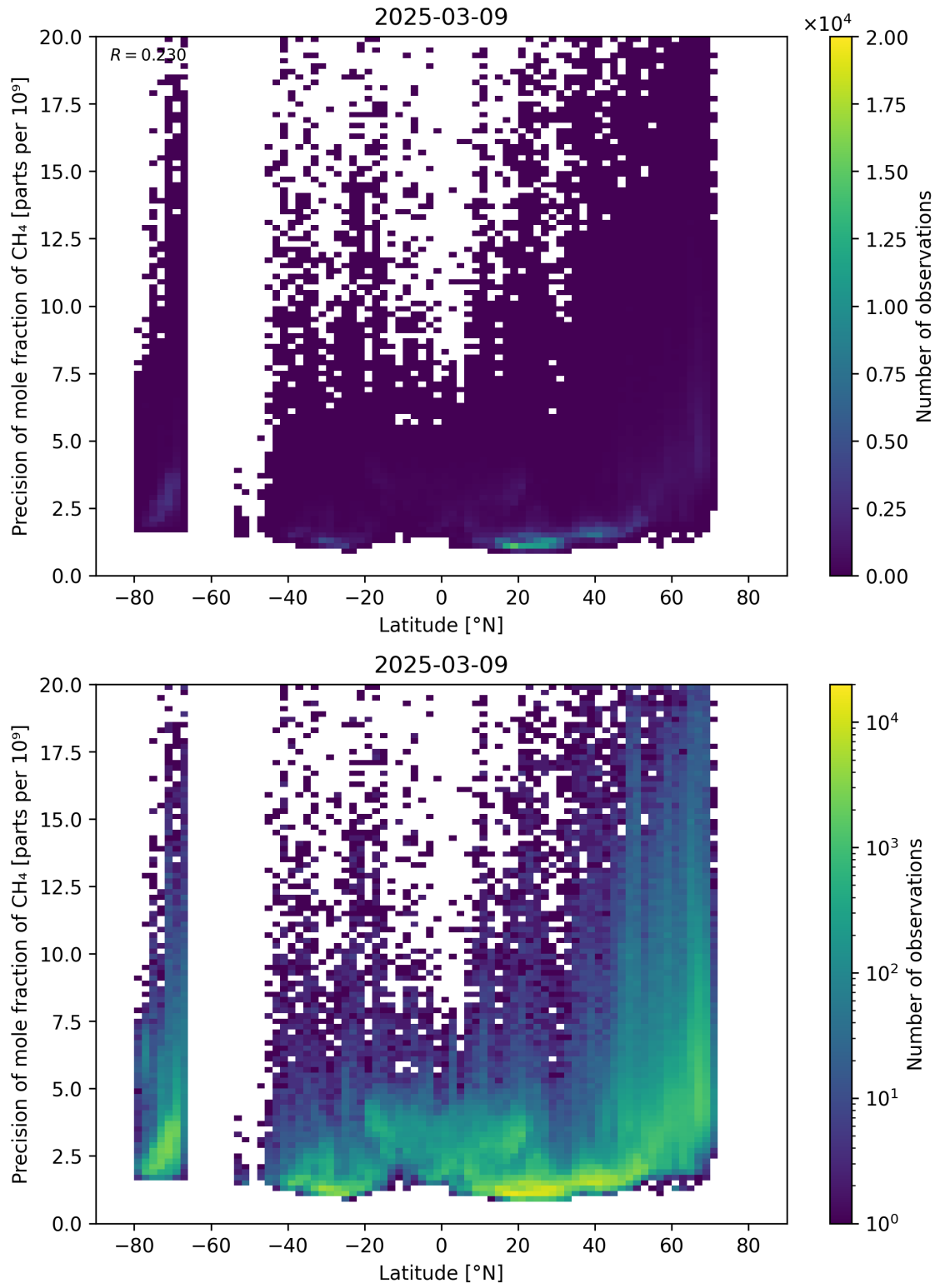
Figure 59: Scatter density plot of “Latitude” against “Precision of mole fraction of CH 4 ” for 2025-03-08 to 2025-03-10.
