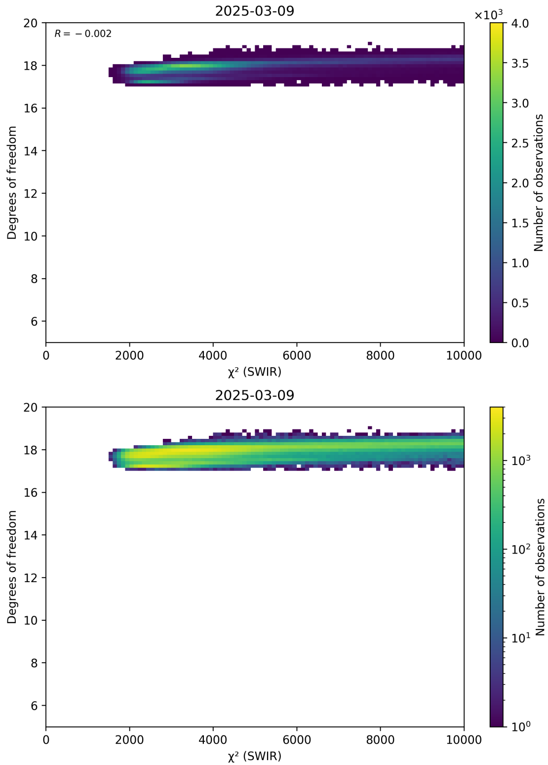
Figure 48: Scatter density plot of “ \chi^2 (SWIR)” against “Degrees of freedom” for 2025-03-08 to 2025-03-10.
