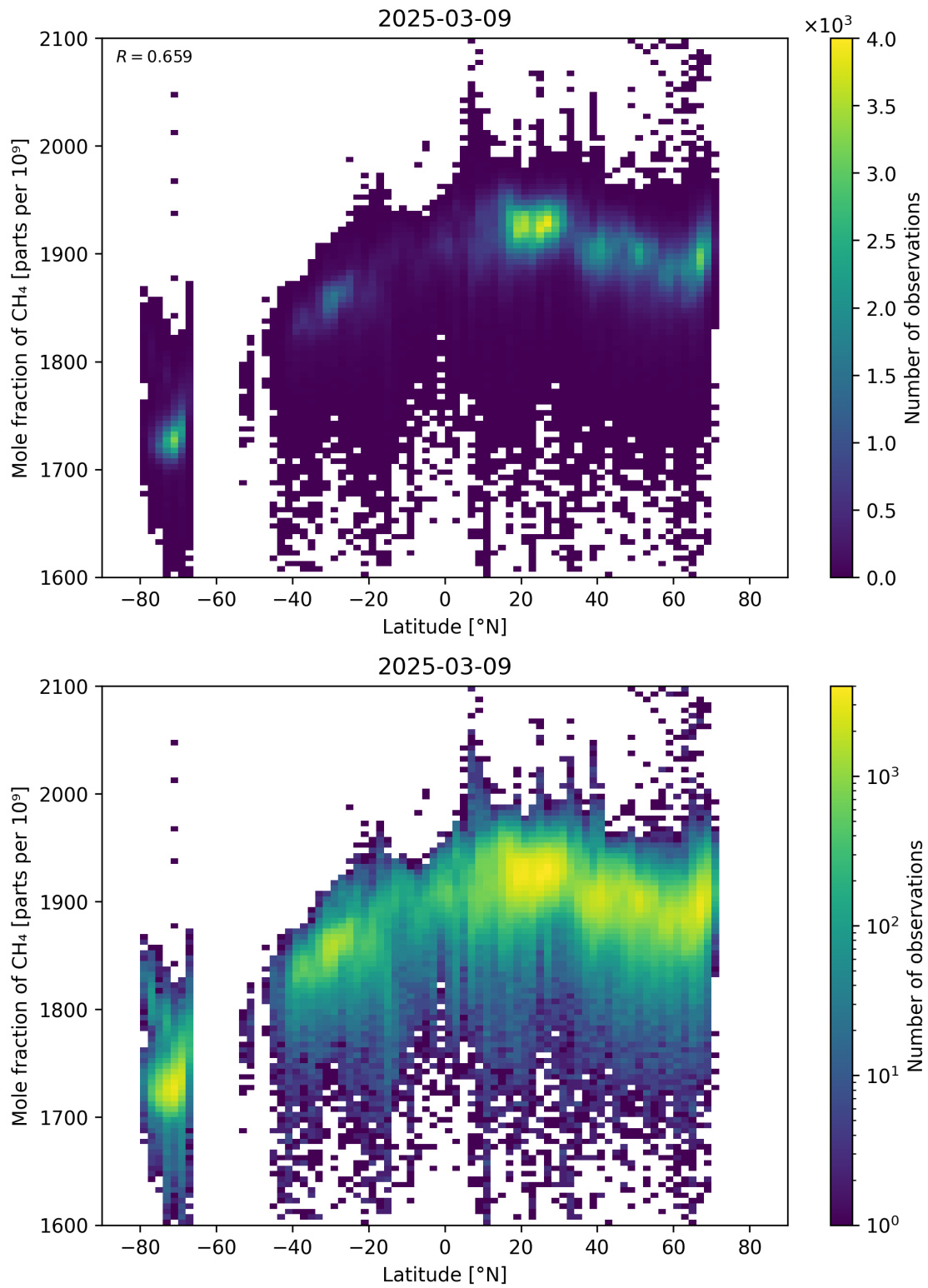
Figure 57: Scatter density plot of “Latitude” against “Mole fraction of CH 4 ” for 2025-03-08 to 2025-03-10.
