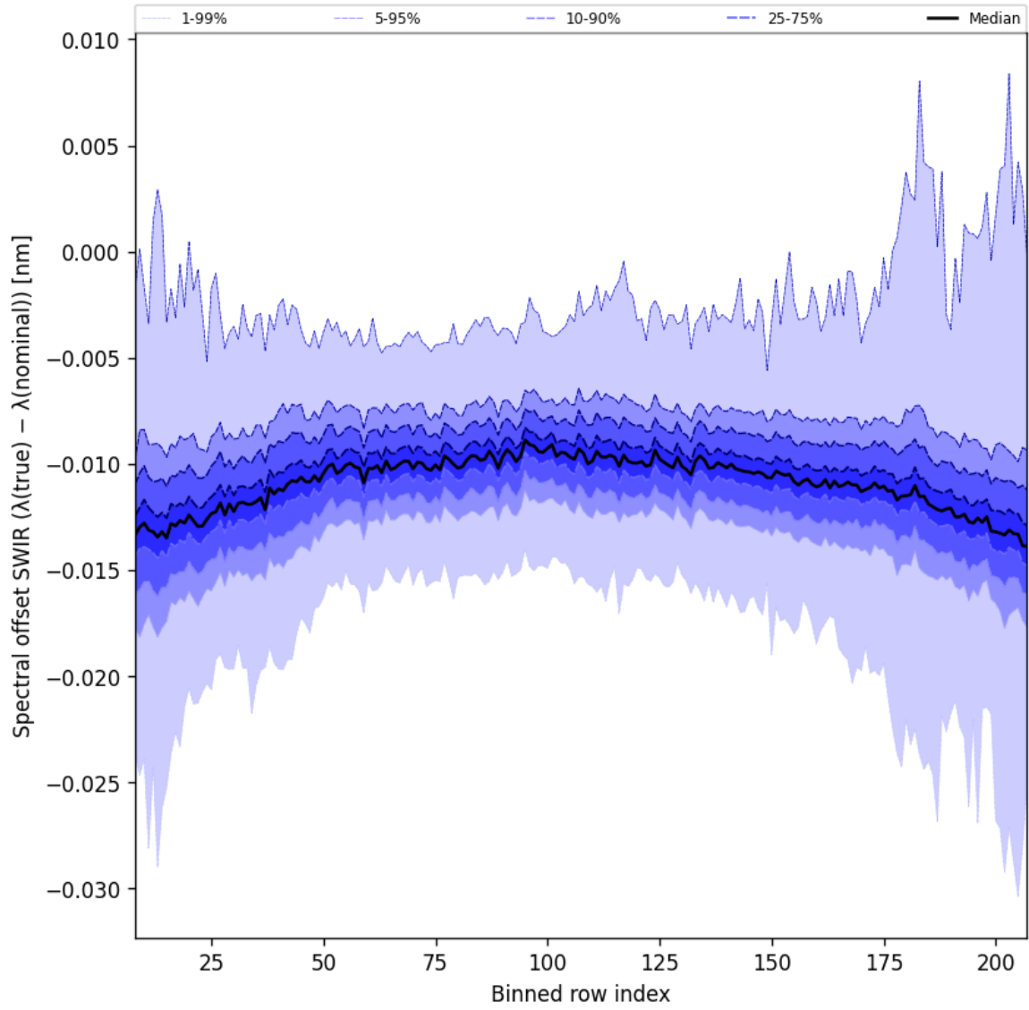
Figure 38: Along track statistics of “Spectral offset SWIR ( \lambda_{\text{true}} - \lambda_{\text{nominal}} )” for 2025-03-08 to 2025-03-10
