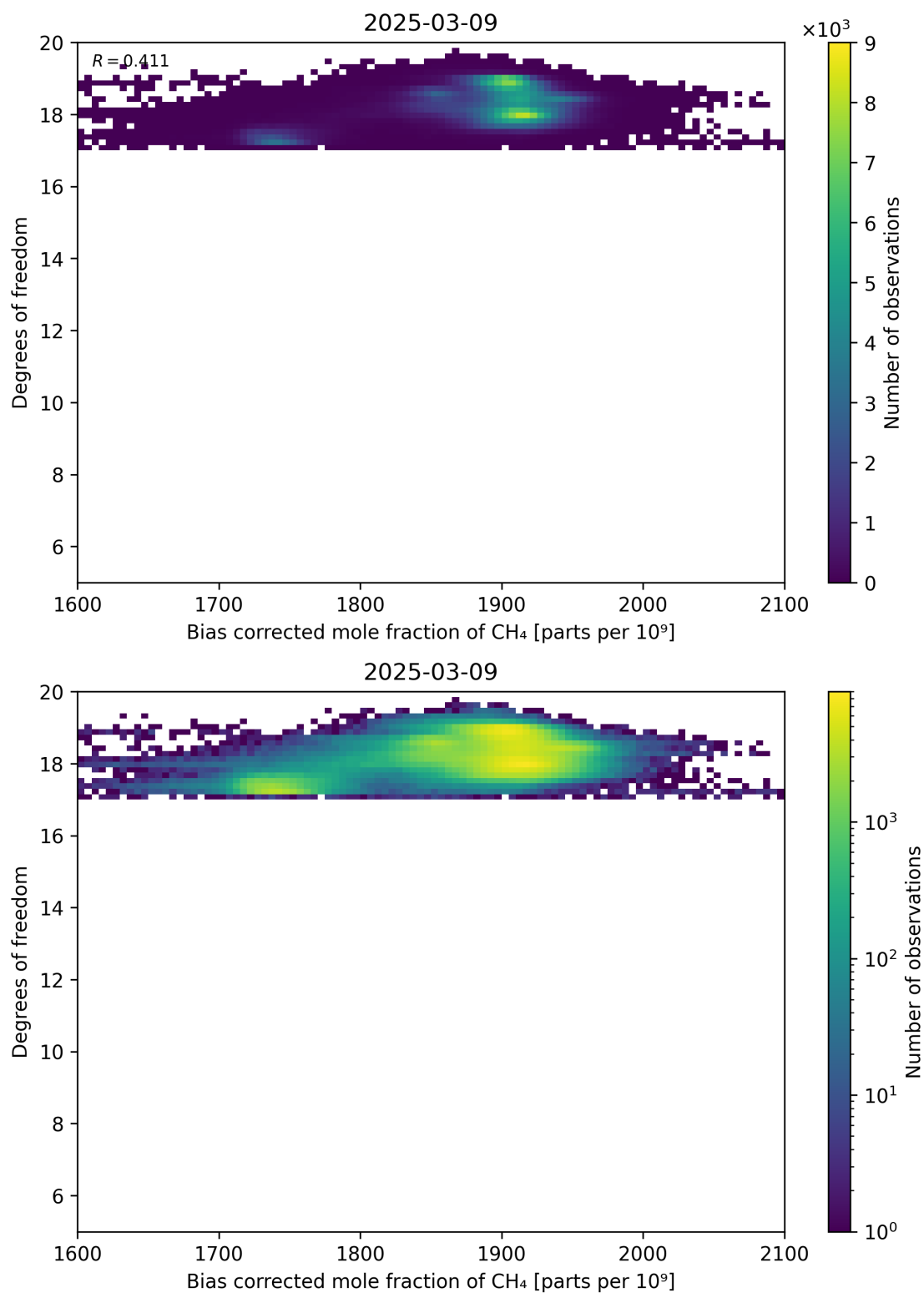
Figure 65: Scatter density plot of “Bias corrected mole fraction of CH 4 ” against “Degrees of freedom” for 2025-03-08 to 2025-03-10.
