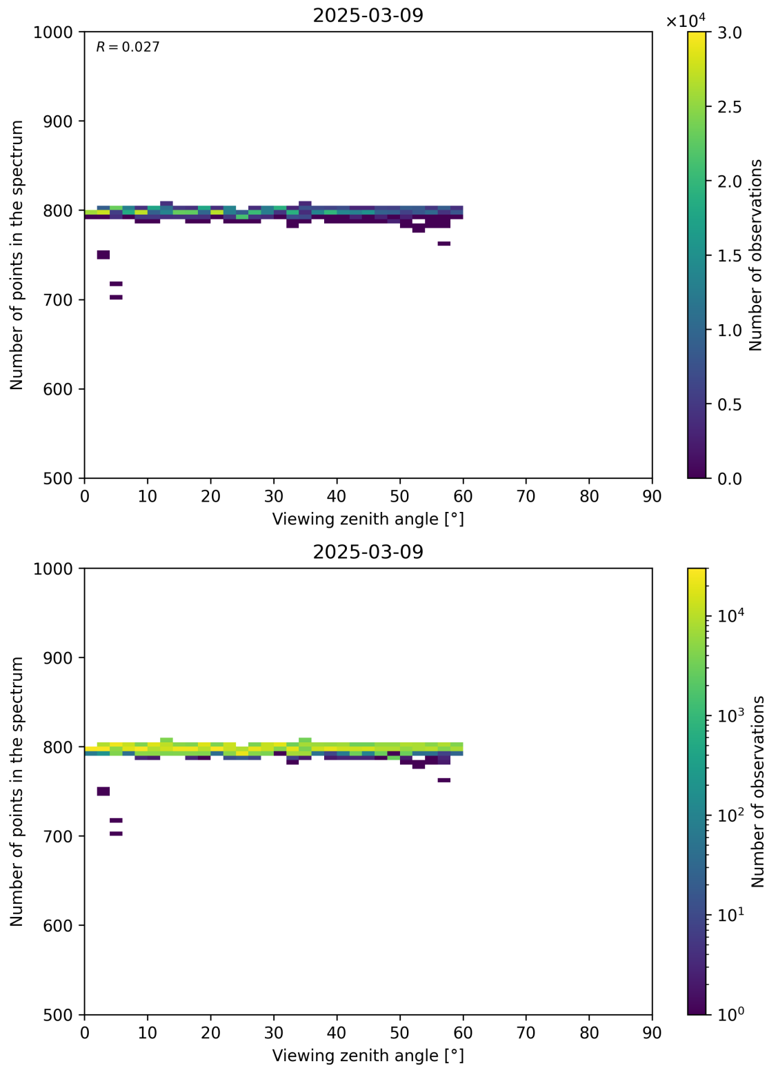
Figure 114: Scatter density plot of “Viewing zenith angle” against “Number of points in the spectrum” for 2025-03-08 to 2025-03-10.
