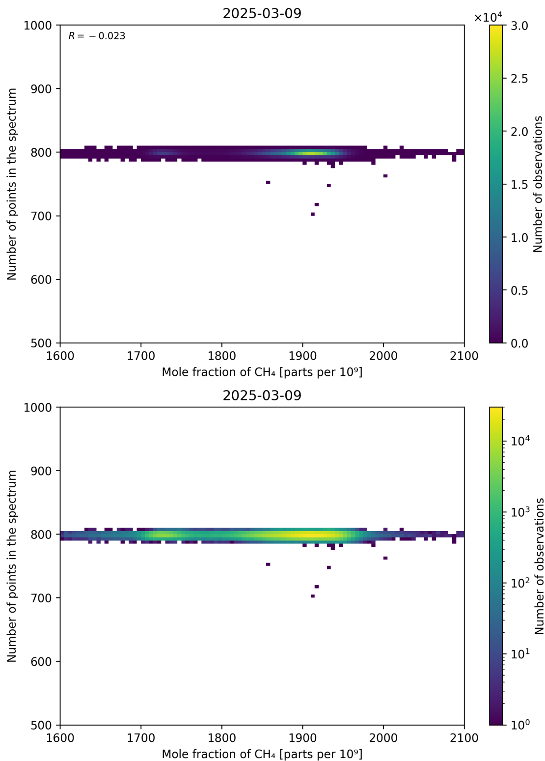
Figure 77: Scatter density plot of “Mole fraction of CH 4 ” against “Number of points in the spectrum” for 2025-03-08 to 2025-03-10.
