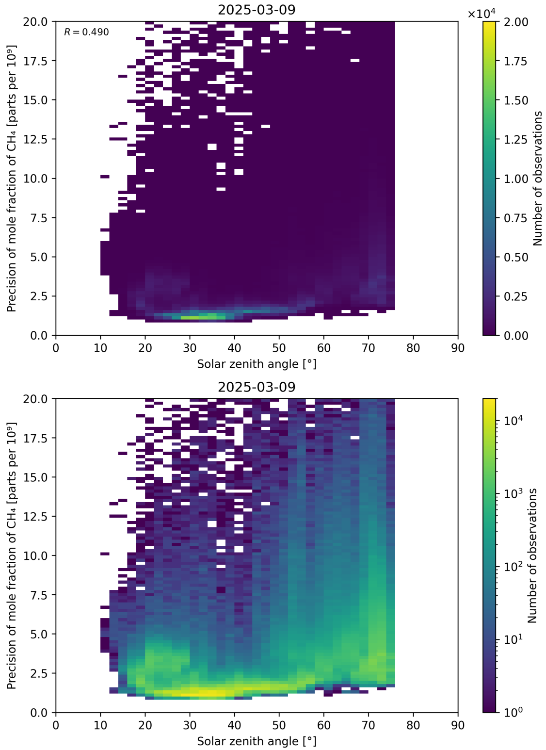
Figure 101: Scatter density plot of “Solar zenith angle” against “Precision of mole fraction of CH 4 ” for 2025-03-08 to 2025-03-10.
