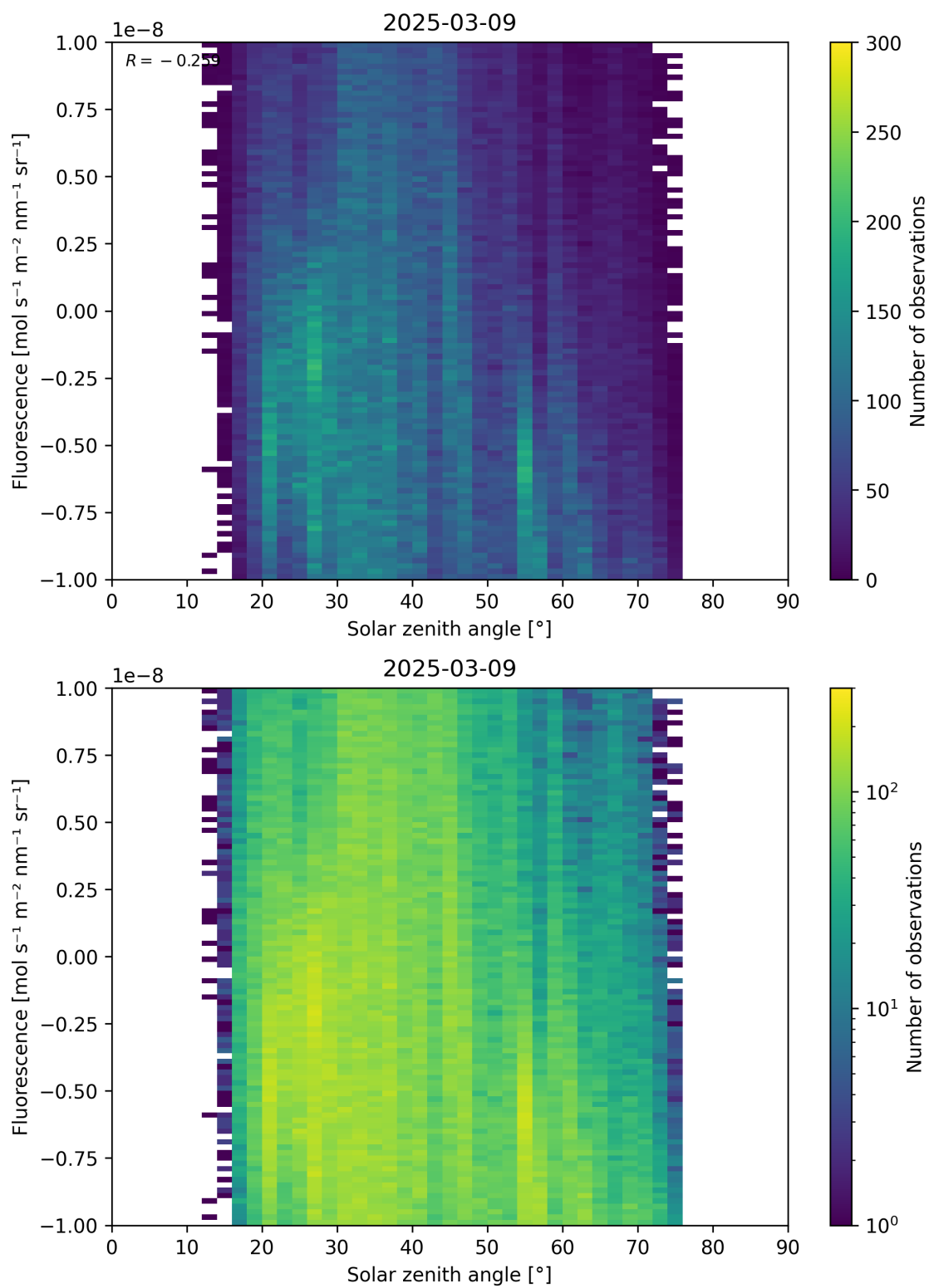
Figure 97: Scatter density plot of “Solar zenith angle” against “Fluorescence” for 2025-03-08 to 2025-03-10.
