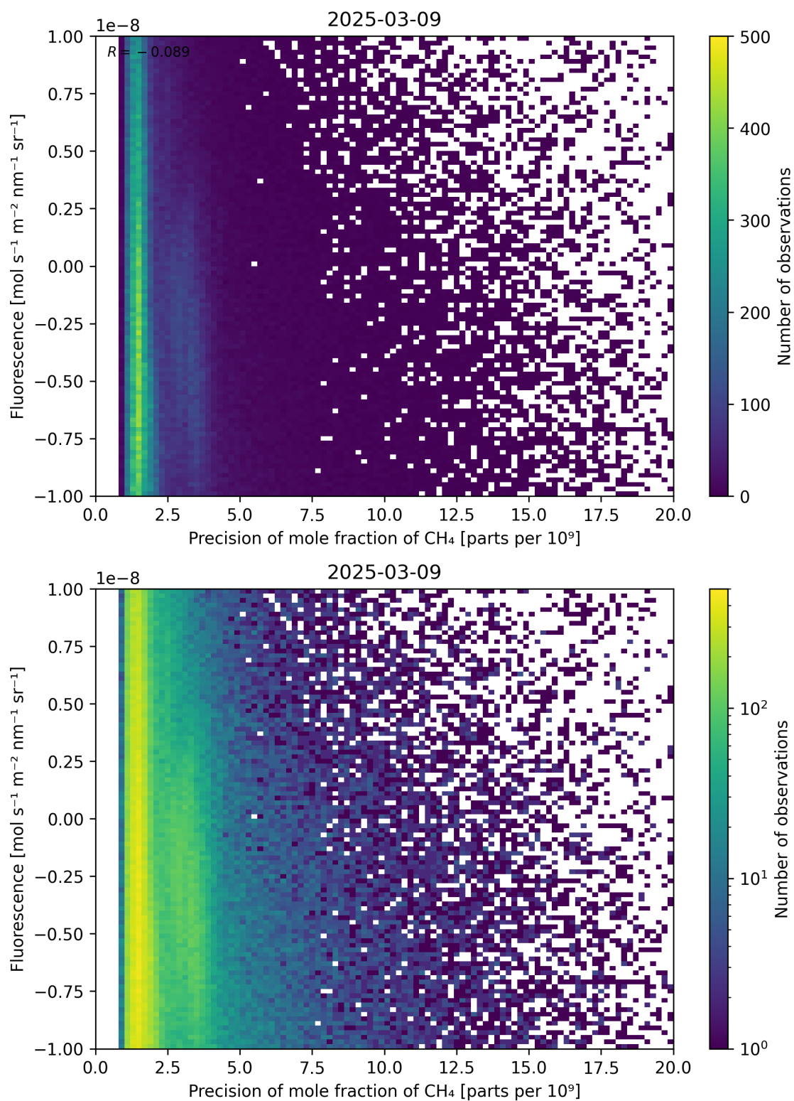
Figure 81: Scatter density plot of “Precision of mole fraction of \text{CH}_4 ” against “Fluorescence” for 2025-03-08 to 2025-03-10.
