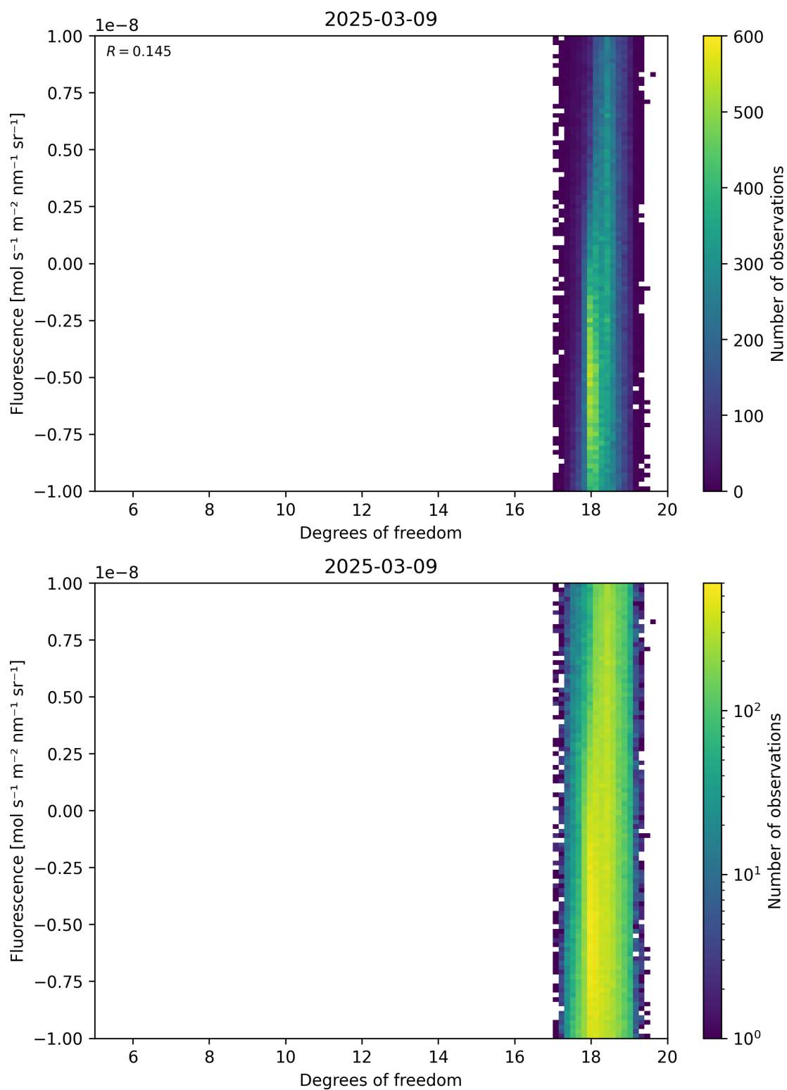
Figure 51: Scatter density plot of “Degrees of freedom” against “Fluorescence” for 2025-03-08 to 2025-03-10.
