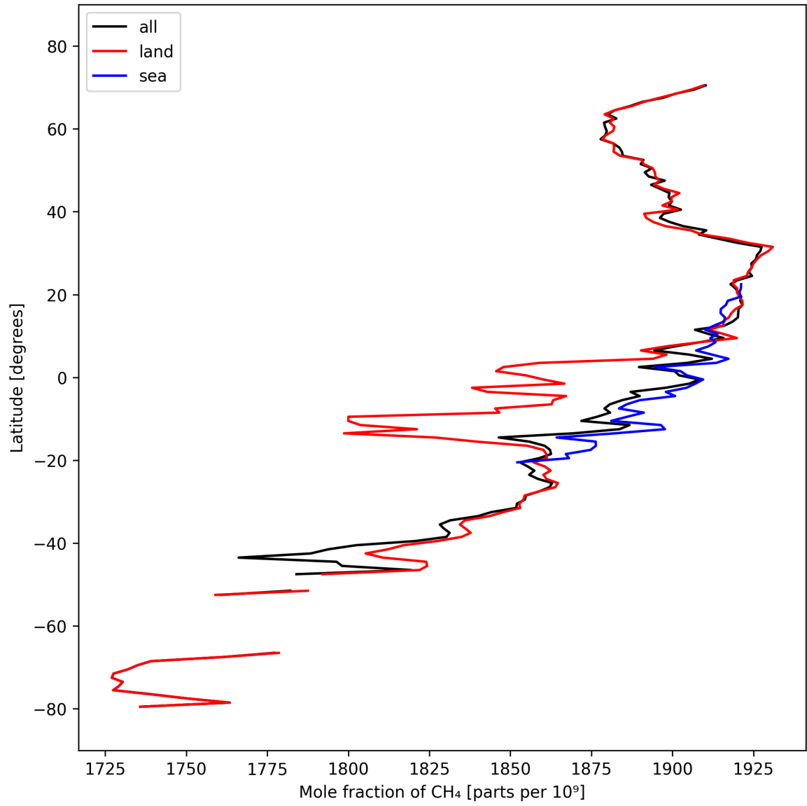
Figure 12: Zonal average of “Mole fraction of \text{CH}_4 ” for 2025-03-08 to 2025-03-10.
