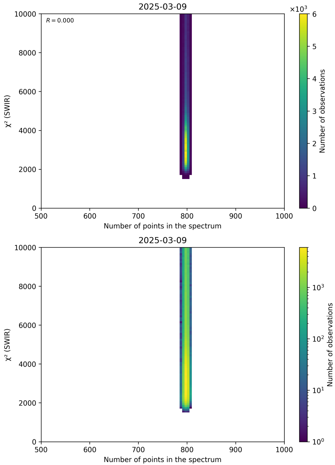
Figure 89: Scatter density plot of “Number of points in the spectrum” against “ \chi^2 (SWIR)” for 2025-03-08 to 2025-03-10.
