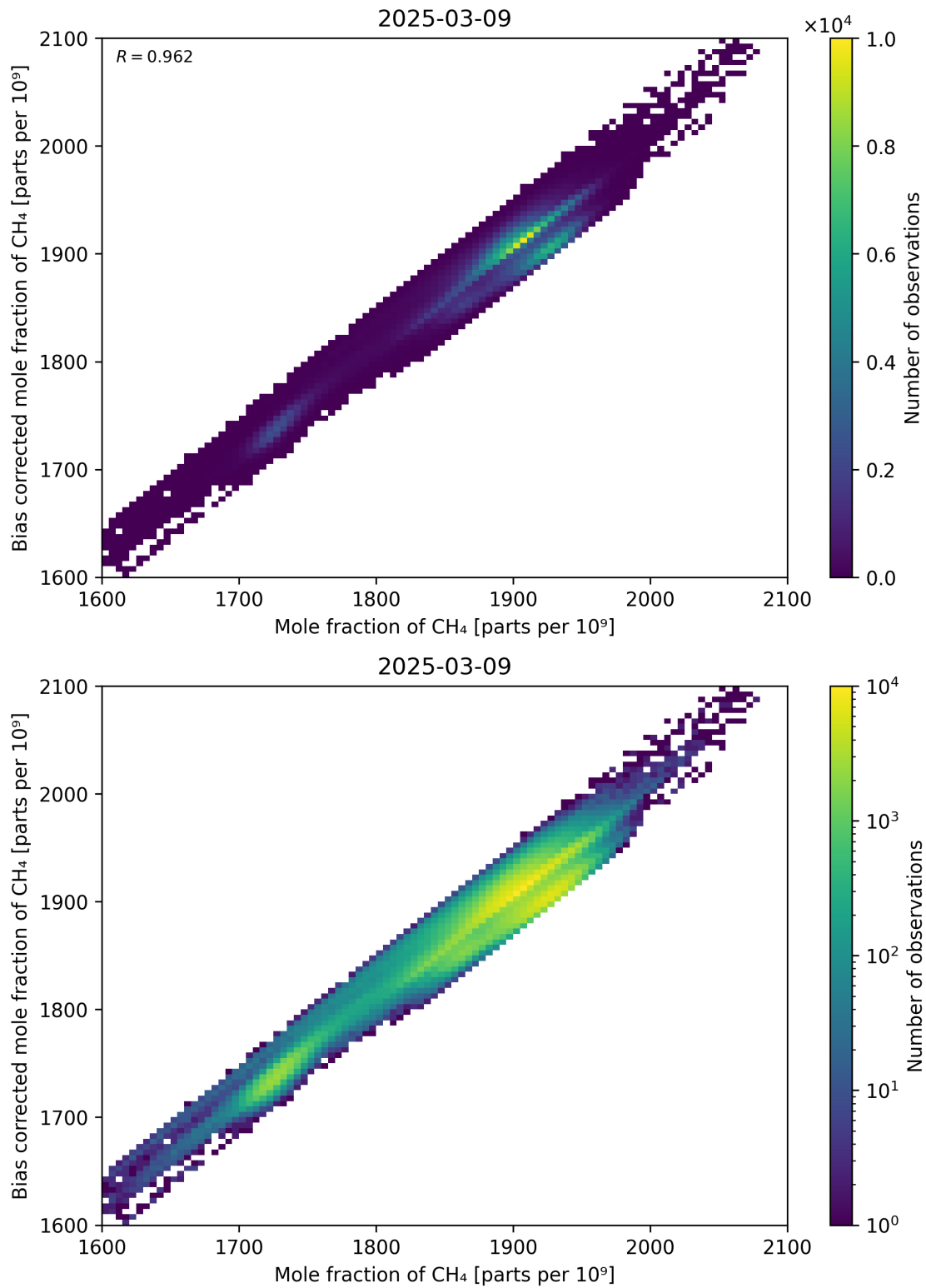
Figure 74: Scatter density plot of “Mole fraction of CH 4 ” against “Bias corrected mole fraction of CH 4 ” for 2025-03-08 to 2025-03-10.
