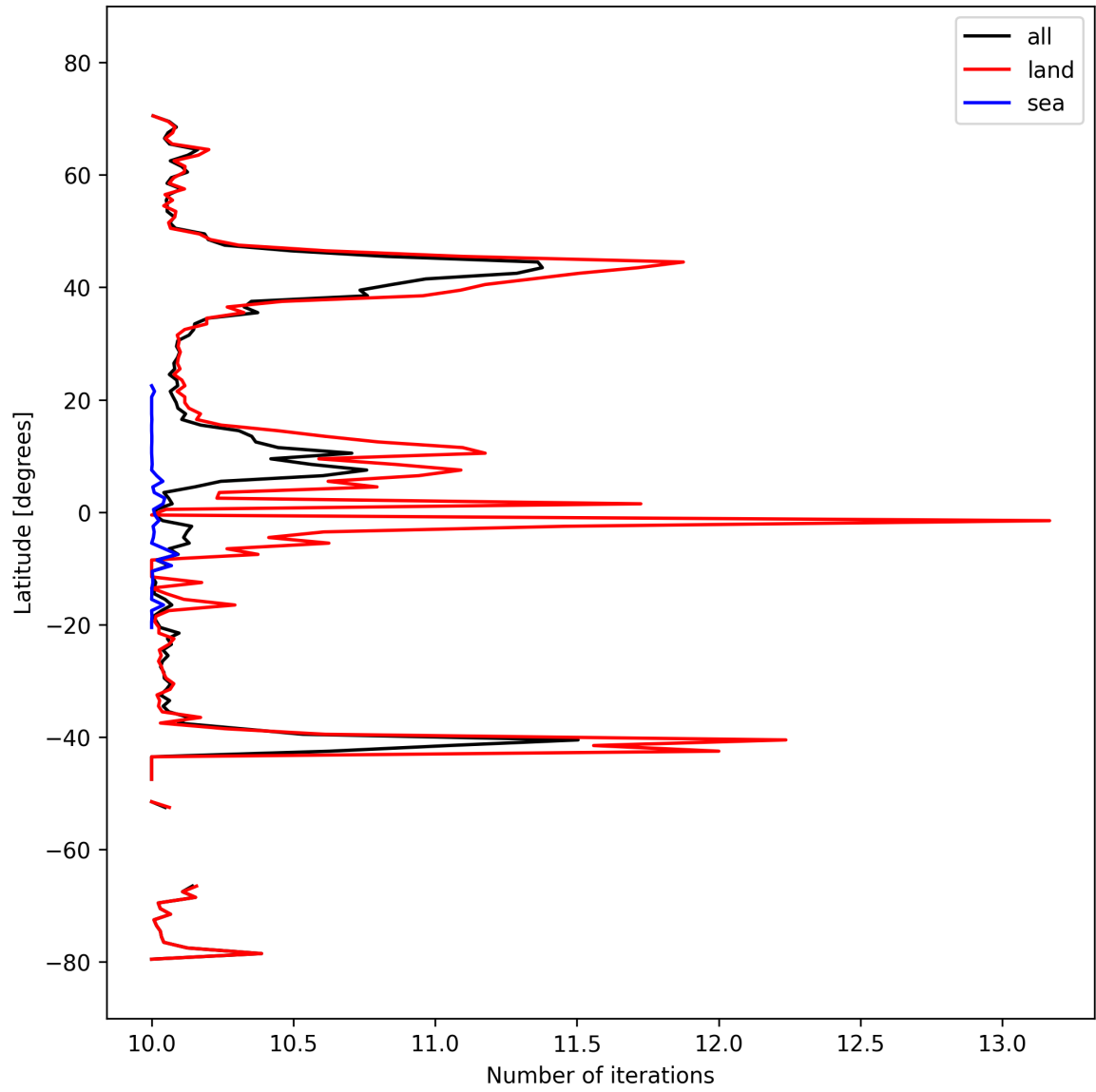
Figure 20: Zonal average of “Number of iterations” for 2025-03-08 to 2025-03-10.
