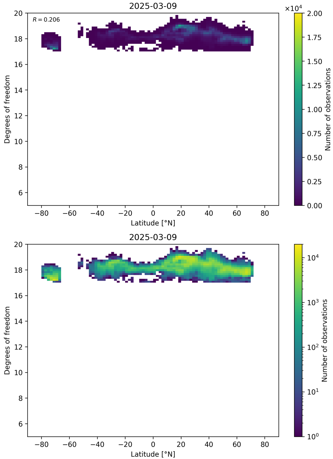
Figure 55: Scatter density plot of “Latitude” against “Degrees of freedom” for 2025-03-08 to 2025-03-10.
