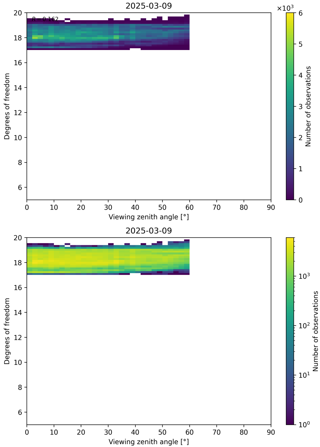
Figure 107: Scatter density plot of “Viewing zenith angle” against “Degrees of freedom” for 2025-03-08 to 2025-03-10.
