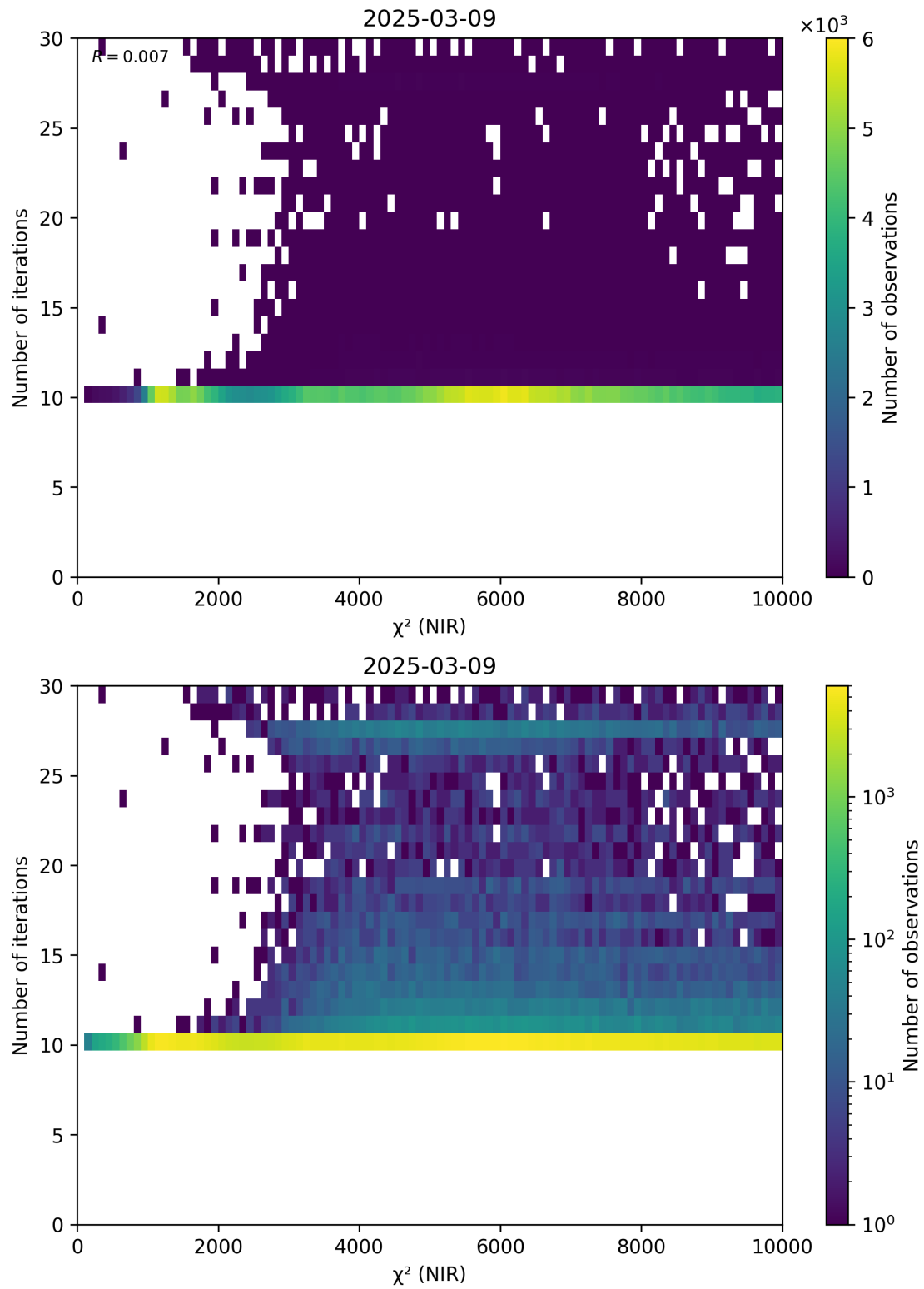
Figure 46: Scatter density plot of “ \chi^2 (NIR)” against “Number of iterations” for 2025-03-08 to 2025-03-10.
