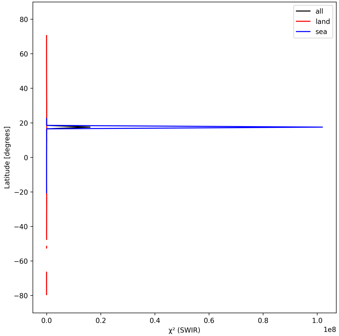
Figure 17: Zonal average of “ \chi^2 (SWIR)” for 2025-03-08 to 2025-03-10.
