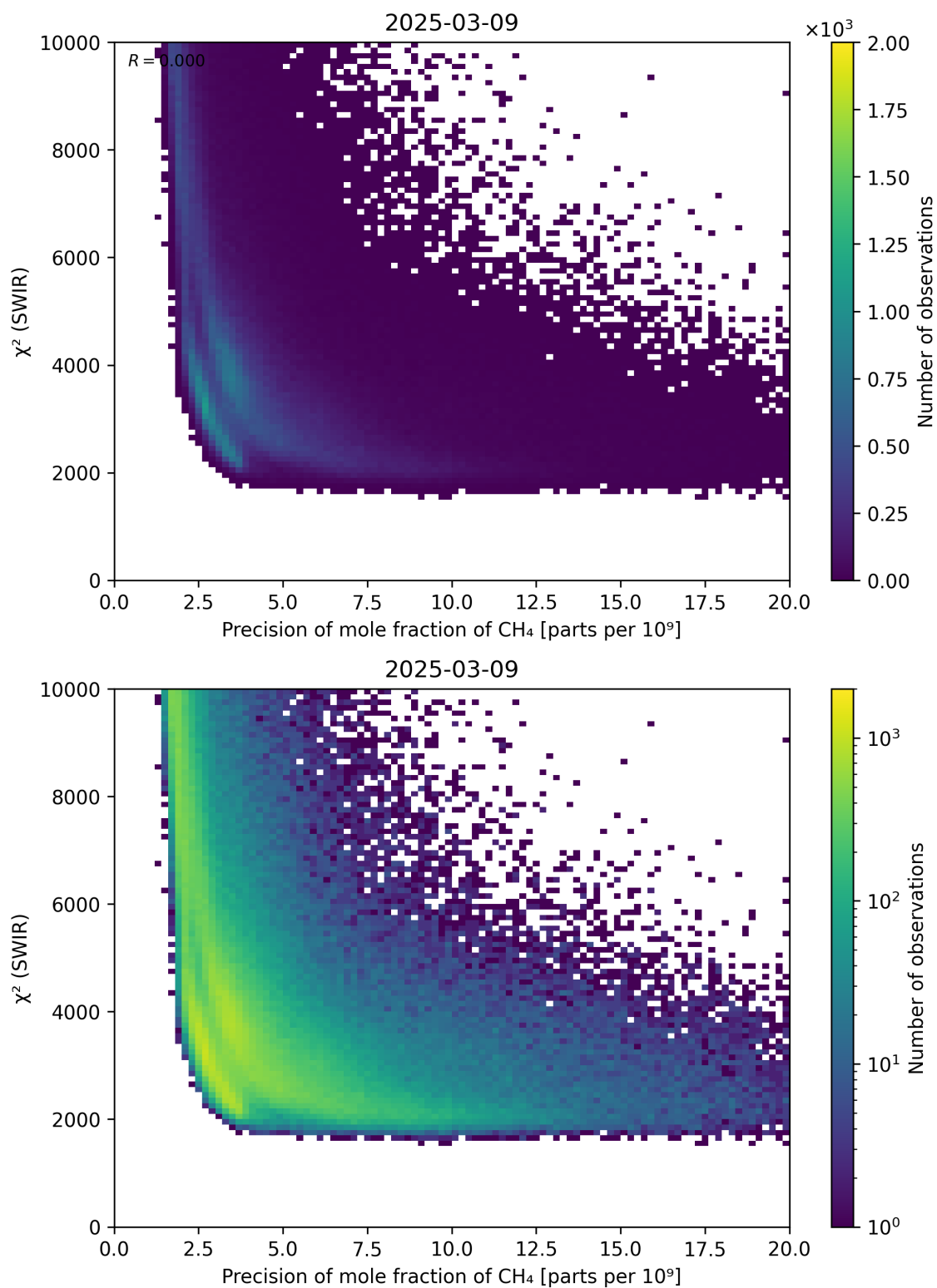
Figure 79: Scatter density plot of “Precision of mole fraction of \text{CH}_4 ” against “ \chi^2 (SWIR)” for 2025-03-08 to 2025-03-10.
