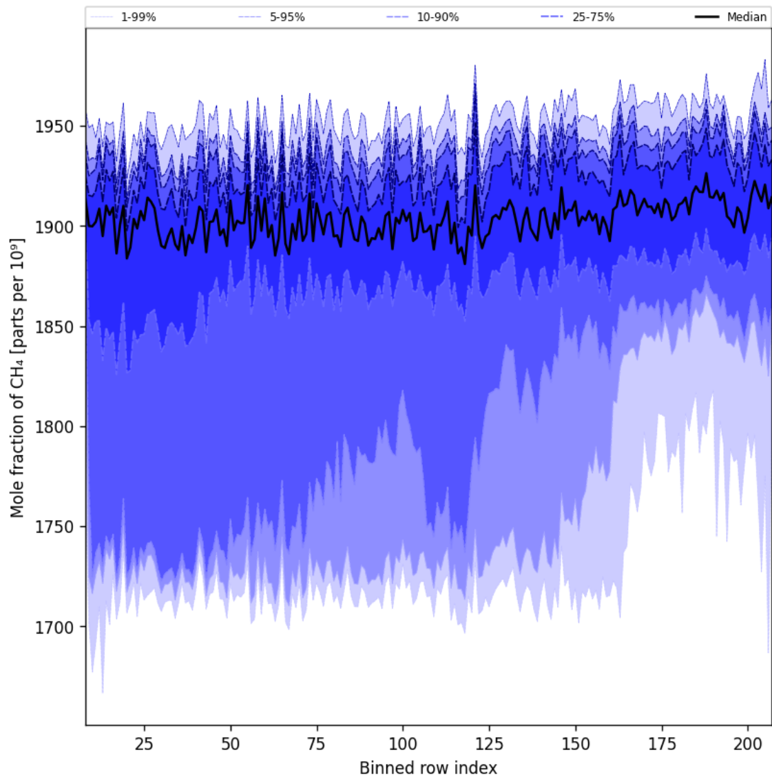
Figure 34: Along track statistics of “Mole fraction of CH 4 ” for 2025-03-08 to 2025-03-10
