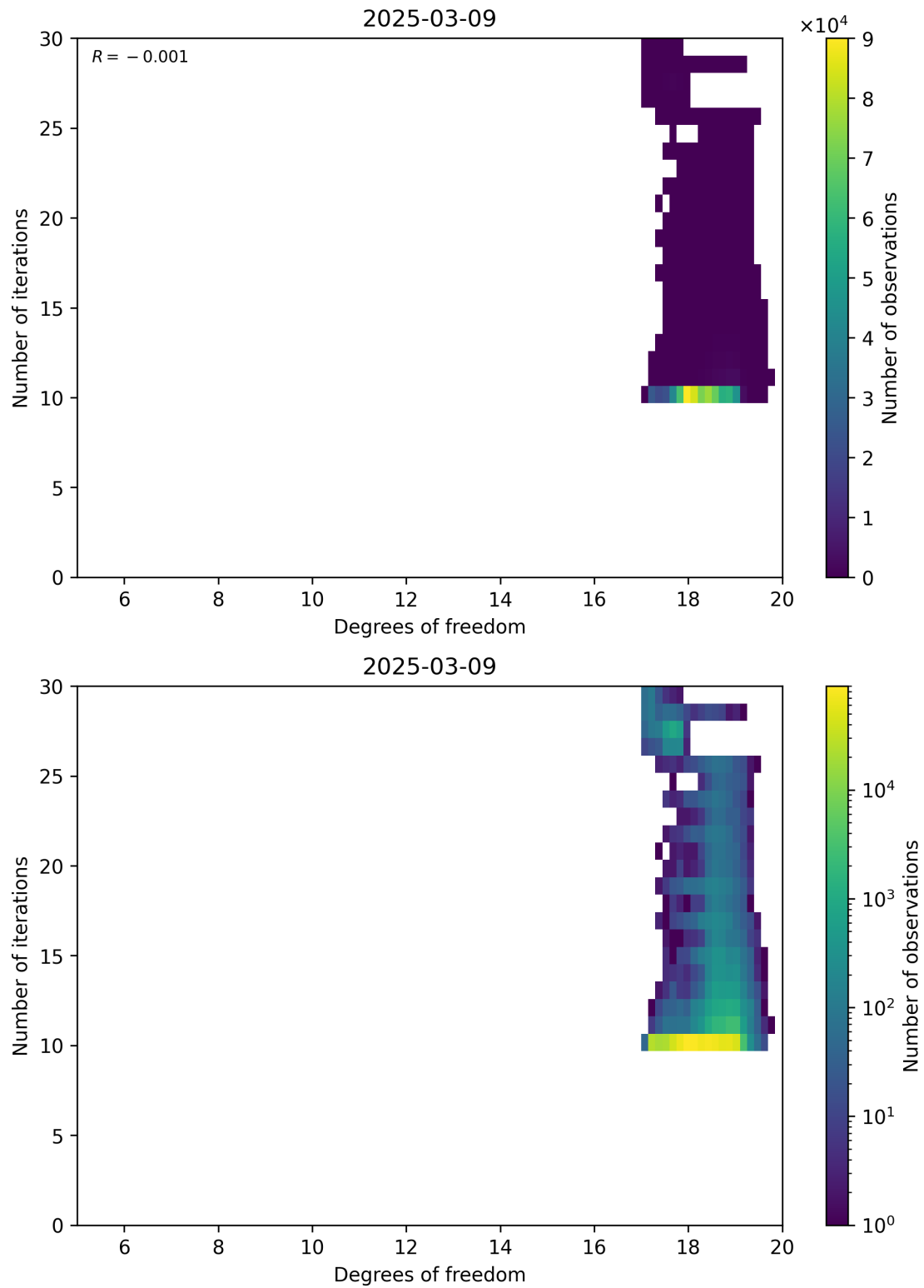
Figure 52: Scatter density plot of “Degrees of freedom” against “Number of iterations” for 2025-03-08 to 2025-03-10.
