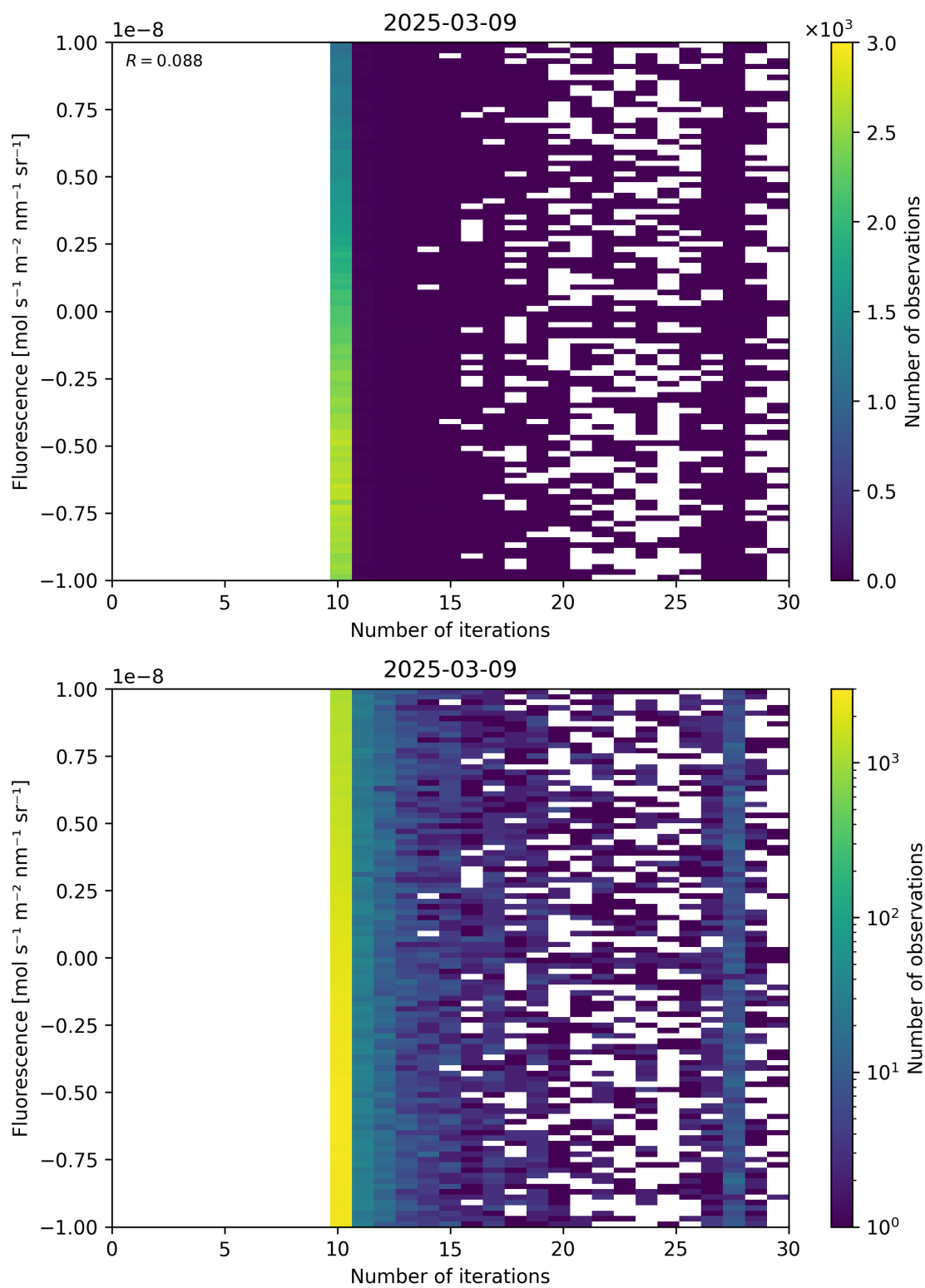
Figure 87: Scatter density plot of “Number of iterations” against “Fluorescence” for 2025-03-08 to 2025-03-10.
