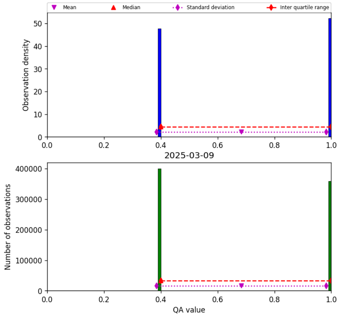
Figure 22: Histogram of “QA value” for 2025-03-08 to 2025-03-10
