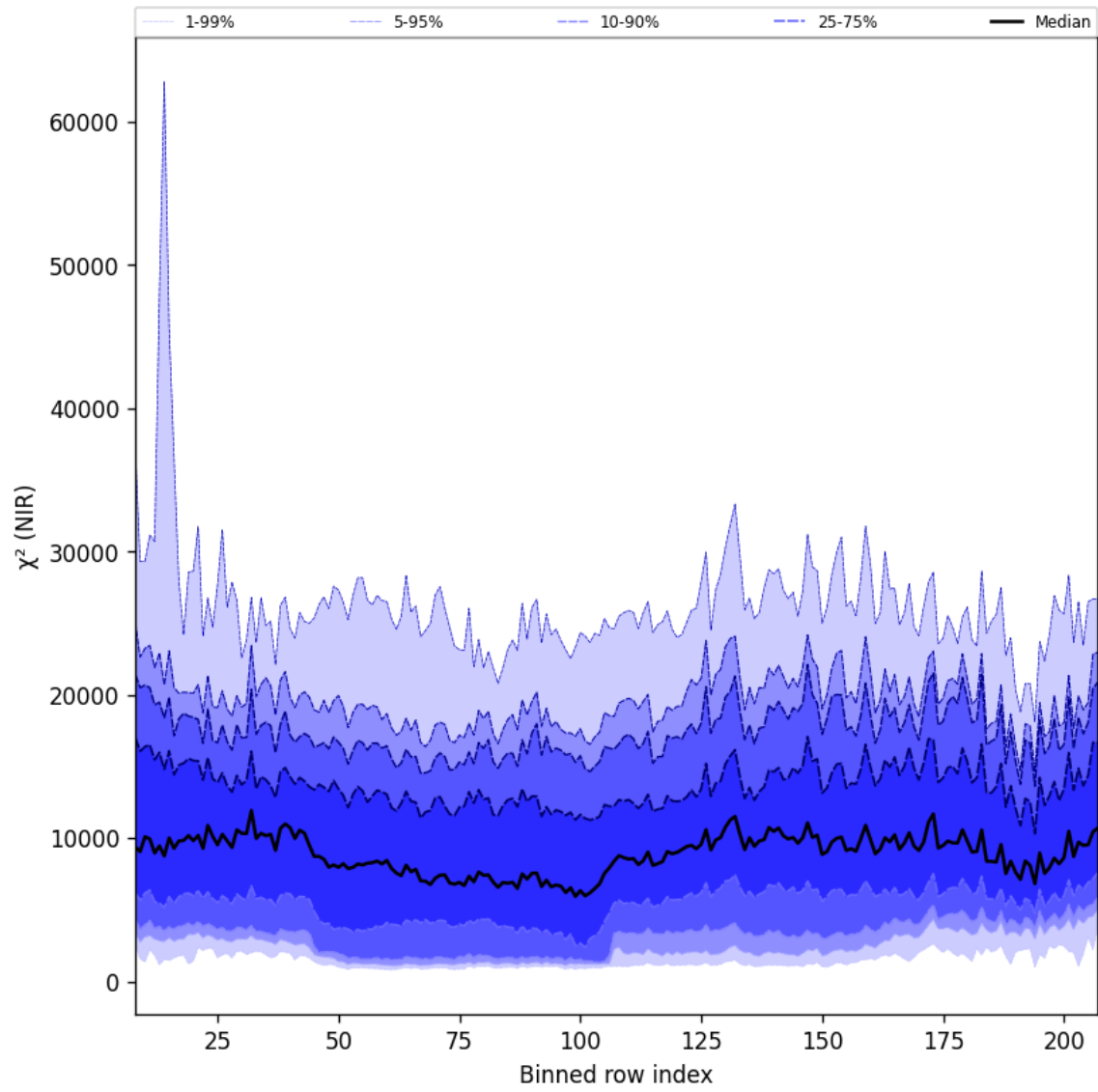
Figure 40: Along track statistics of “ \chi^2 (NIR)” for 2025-03-08 to 2025-03-10
