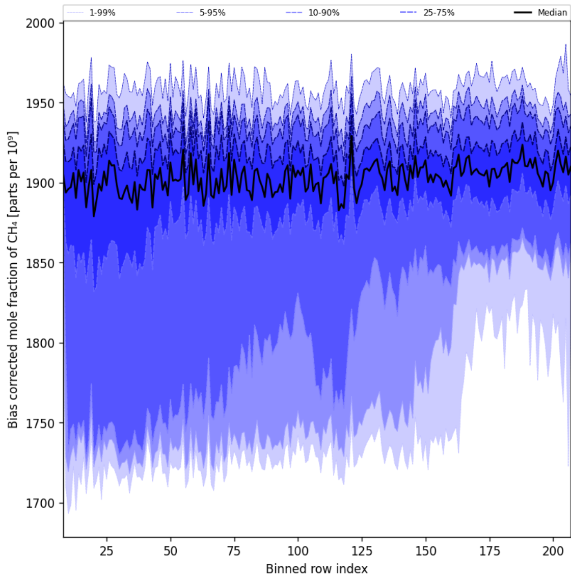
Figure 36: Along track statistics of “Bias corrected mole fraction of CH 4 ” for 2025-03-08 to 2025-03-10
