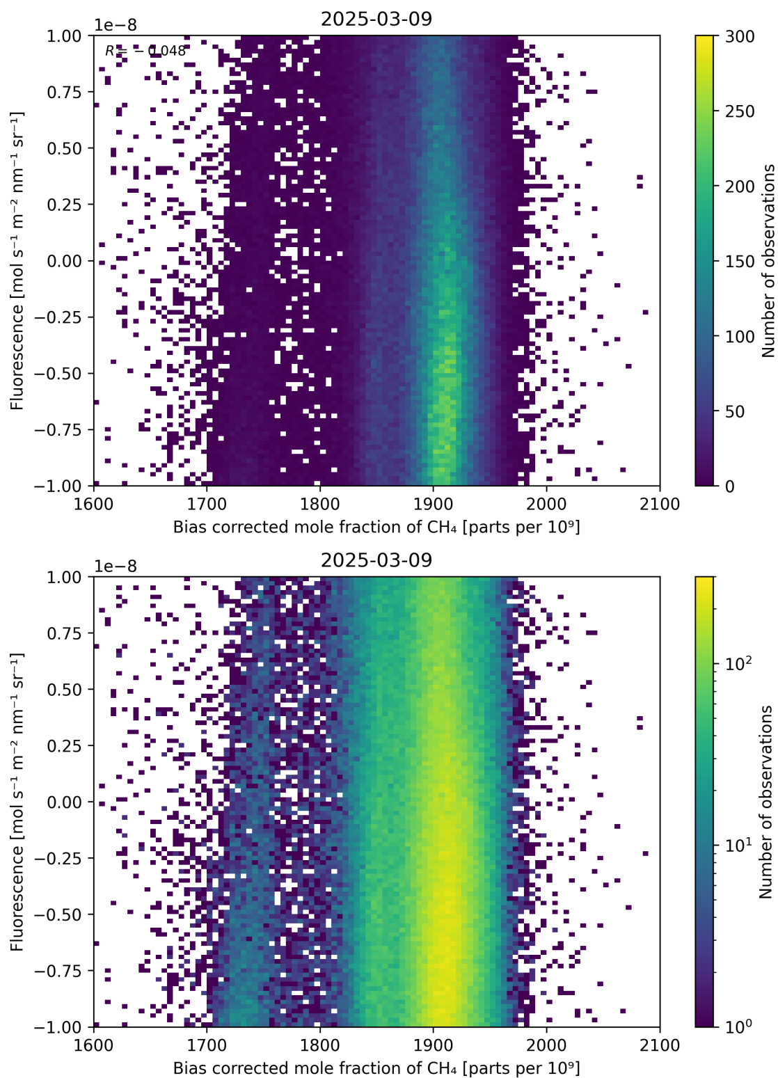
Figure 66: Scatter density plot of “Bias corrected mole fraction of \text{CH}_4 ” against “Fluorescence” for 2025-03-08 to 2025-03-10.
