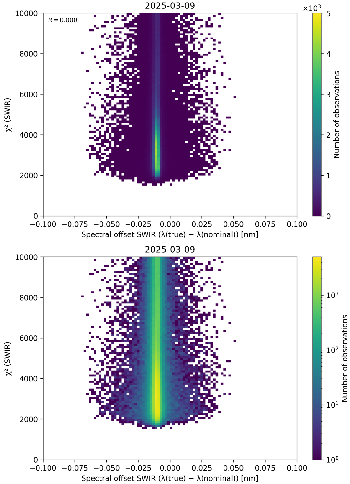
Figure 118: Scatter density plot of “Spectral offset SWIR ( \lambda_{\text{true}} - \lambda_{\text{nominal}} )” against “ \chi^2 (SWIR)” for 2025-03-08 to 2025-03-10.
