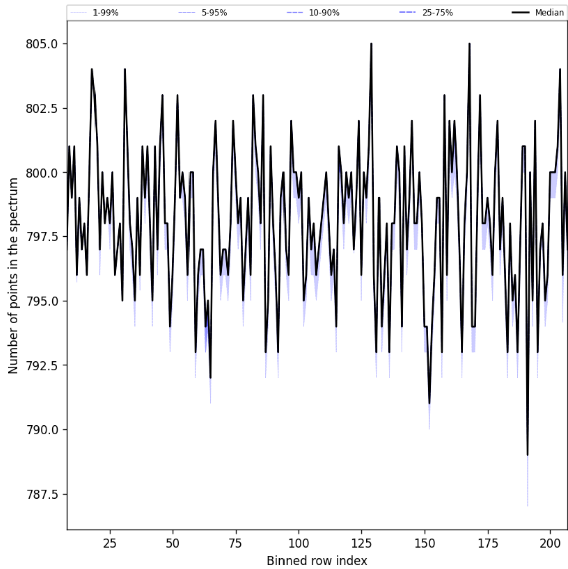
Figure 37: Along track statistics of “Number of points in the spectrum” for 2025-03-08 to 2025-03-10
