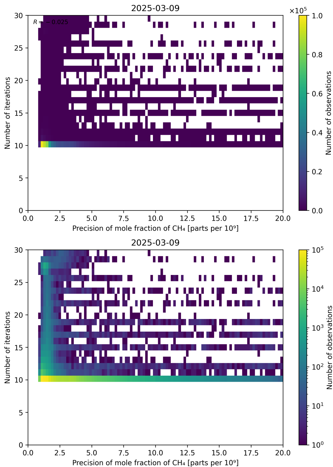
Figure 83: Scatter density plot of “Precision of mole fraction of CH 4 ” against “Number of iterations” for 2025-03-08 to 2025-03-10.
