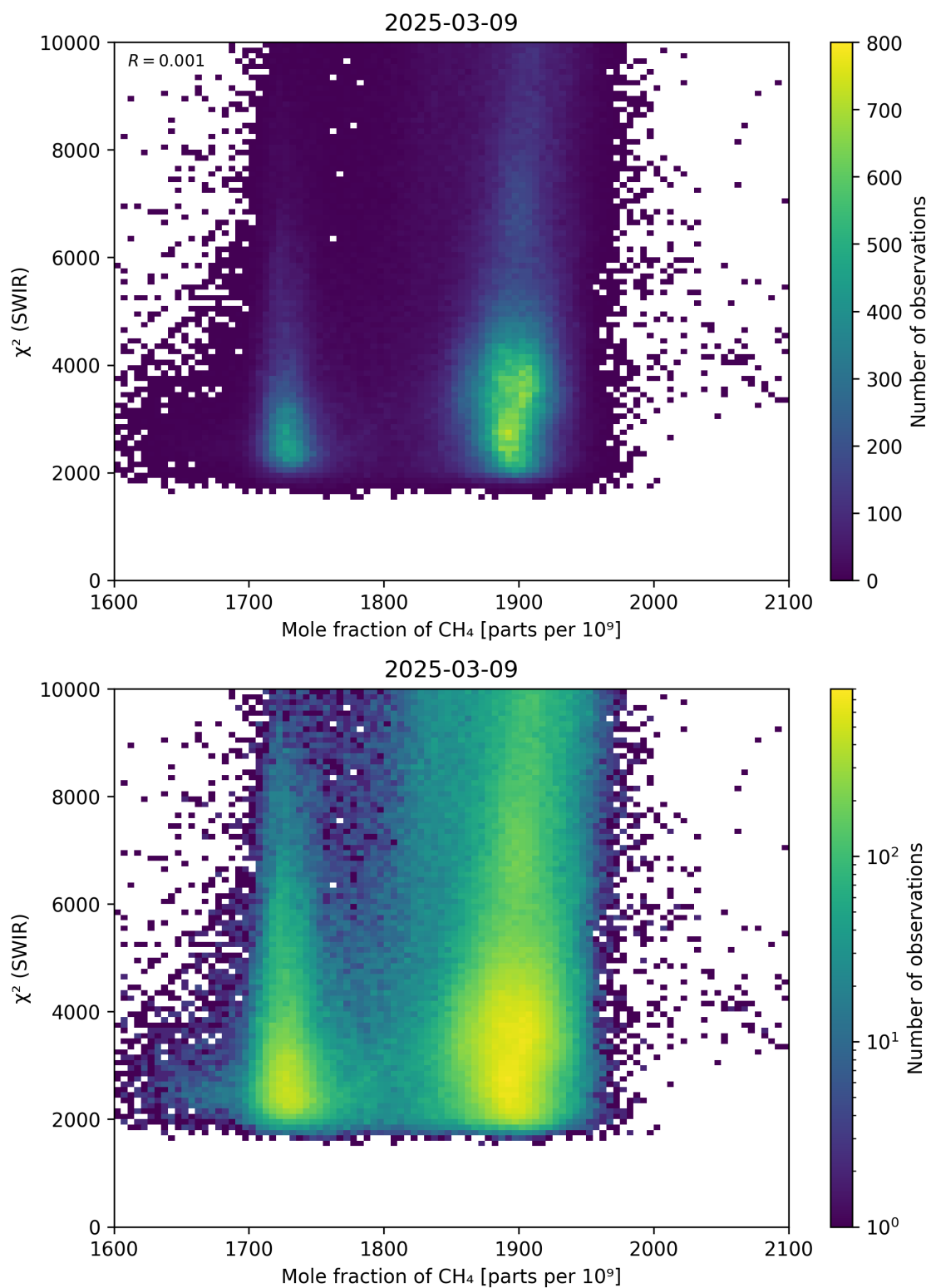
Figure 71: Scatter density plot of “Mole fraction of \text{CH}_4 ” against “ \chi^2 (SWIR)” for 2025-03-08 to 2025-03-10.
