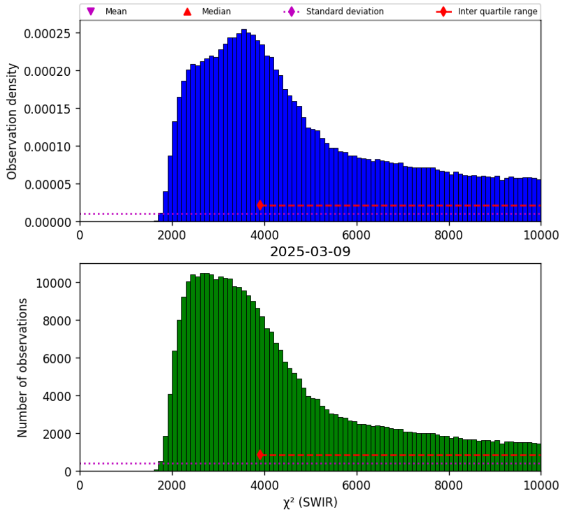
Figure 28: Histogram of " \chi^2 (SWIR)" for 2025-03-08 to 2025-03-10
