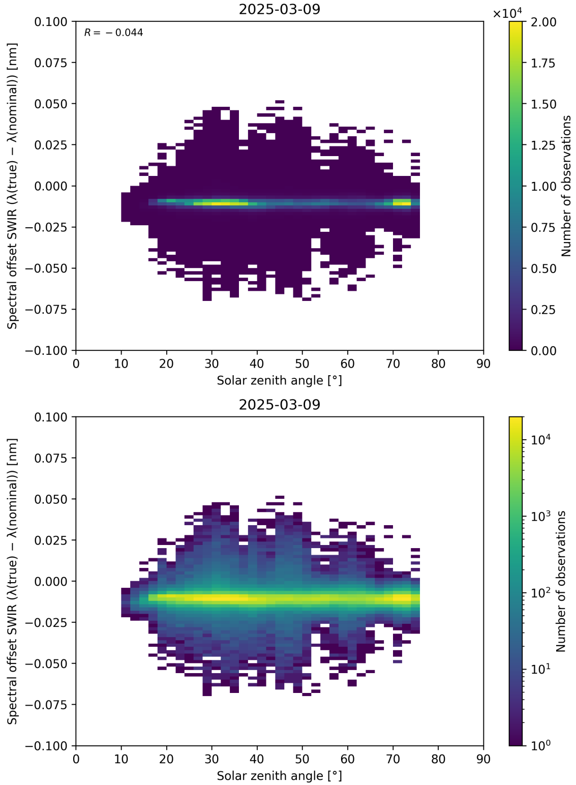
Figure 104: Scatter density plot of “Solar zenith angle” against “Spectral offset SWIR ( \lambda_{\text{true}} - \lambda_{\text{nominal}} )” for 2025-03-08 to 2025-03-10.
