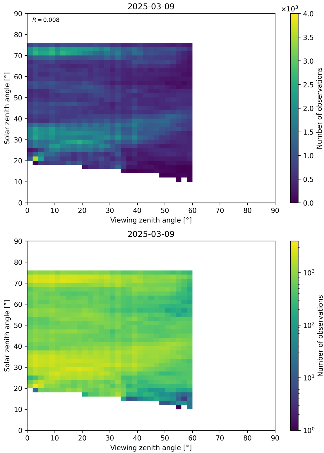
Figure 115: Scatter density plot of “Viewing zenith angle” against “Solar zenith angle” for 2025-03-08 to 2025-03-10.
