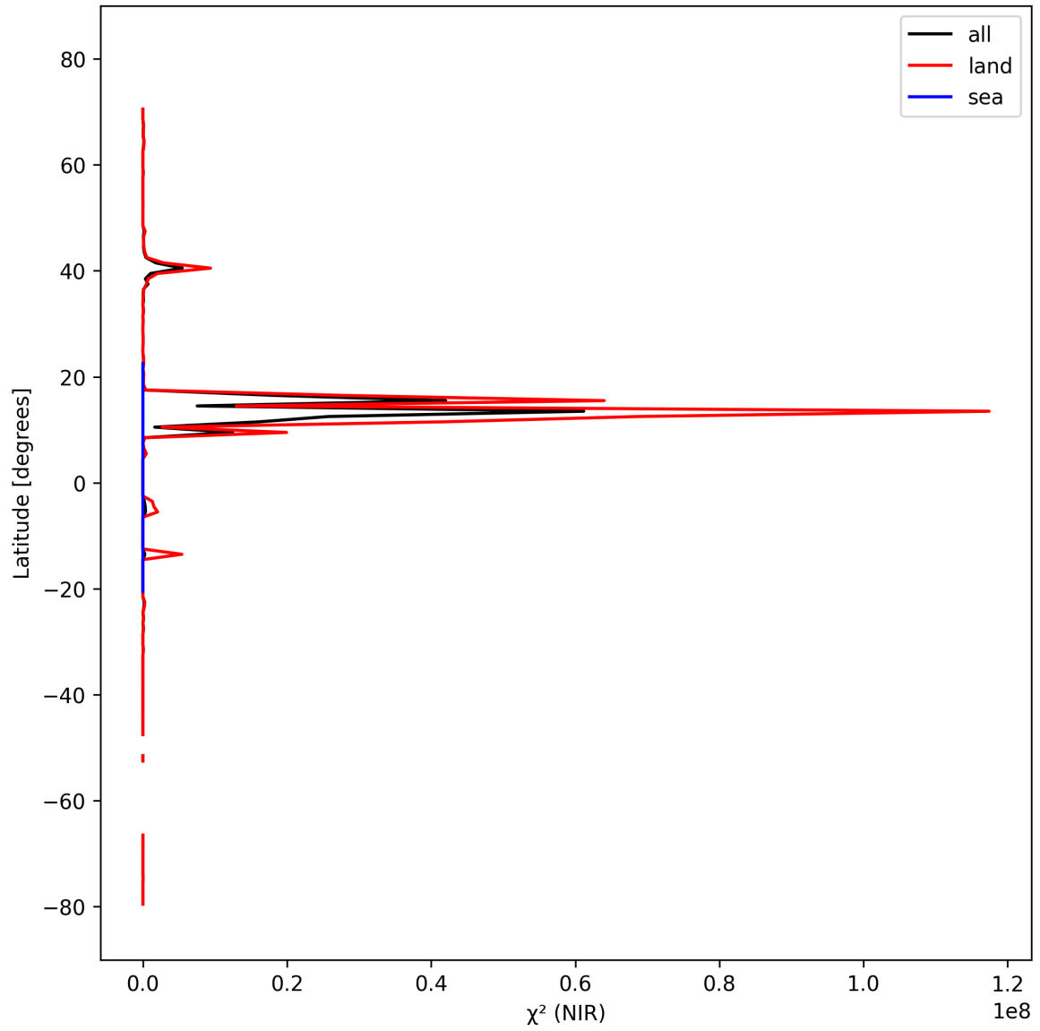
Figure 18: Zonal average of “ \chi^2 (NIR)” for 2025-03-08 to 2025-03-10.
