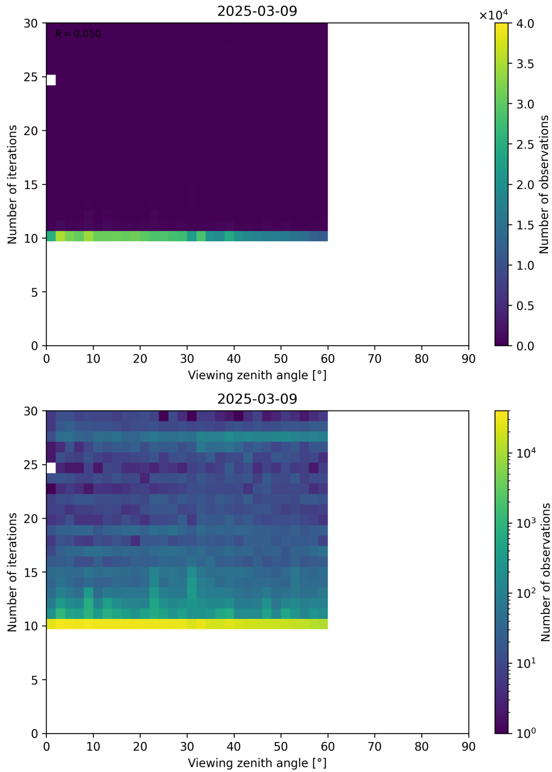
Figure 113: Scatter density plot of “Viewing zenith angle” against “Number of iterations” for 2025-03-08 to 2025-03-10.
