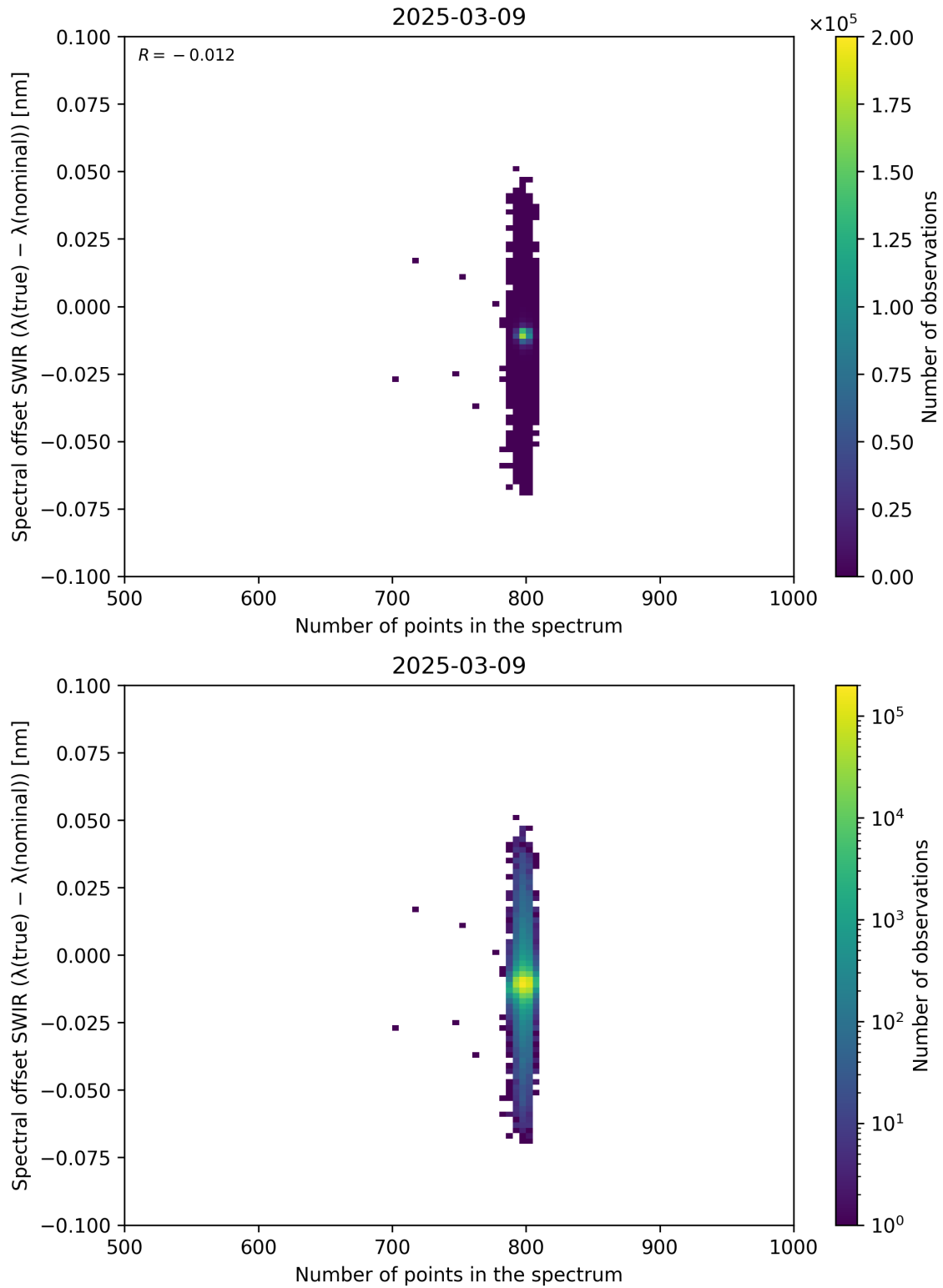
Figure 93: Scatter density plot of “Number of points in the spectrum” against “Spectral offset SWIR ( \lambda_{\text{true}} - \lambda_{\text{nominal}} )” for 2025-03-08 to 2025-03-10.
