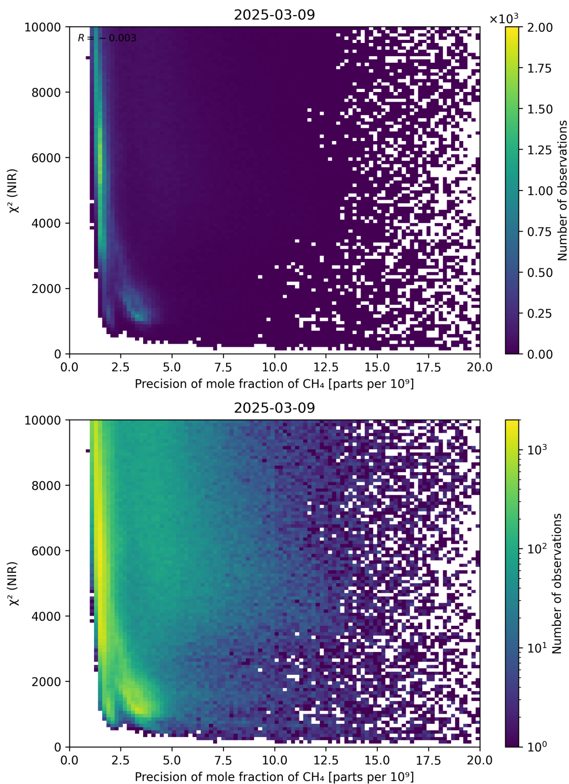
Figure 78: Scatter density plot of “Precision of mole fraction of CH 4 ” against “ \chi^2 (NIR)” for 2025-03-08 to 2025-03-10.
