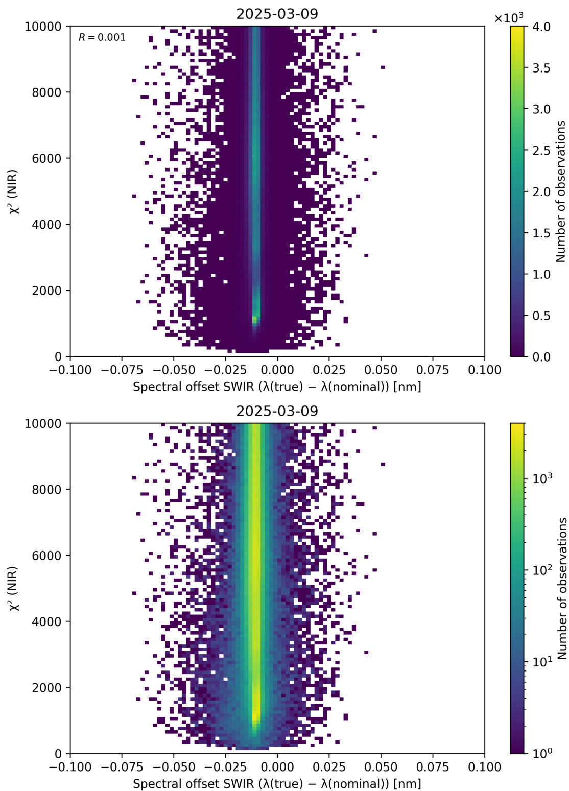
Figure 117: Scatter density plot of “Spectral offset SWIR ( \lambda_{\text{true}} - \lambda_{\text{nominal}} )” against “ \chi^2 (NIR)” for 2025-03-08 to 2025-03-10.
