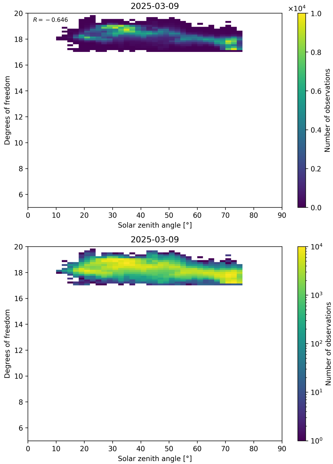
Figure 96: Scatter density plot of “Solar zenith angle” against “Degrees of freedom” for 2025-03-08 to 2025-03-10.
