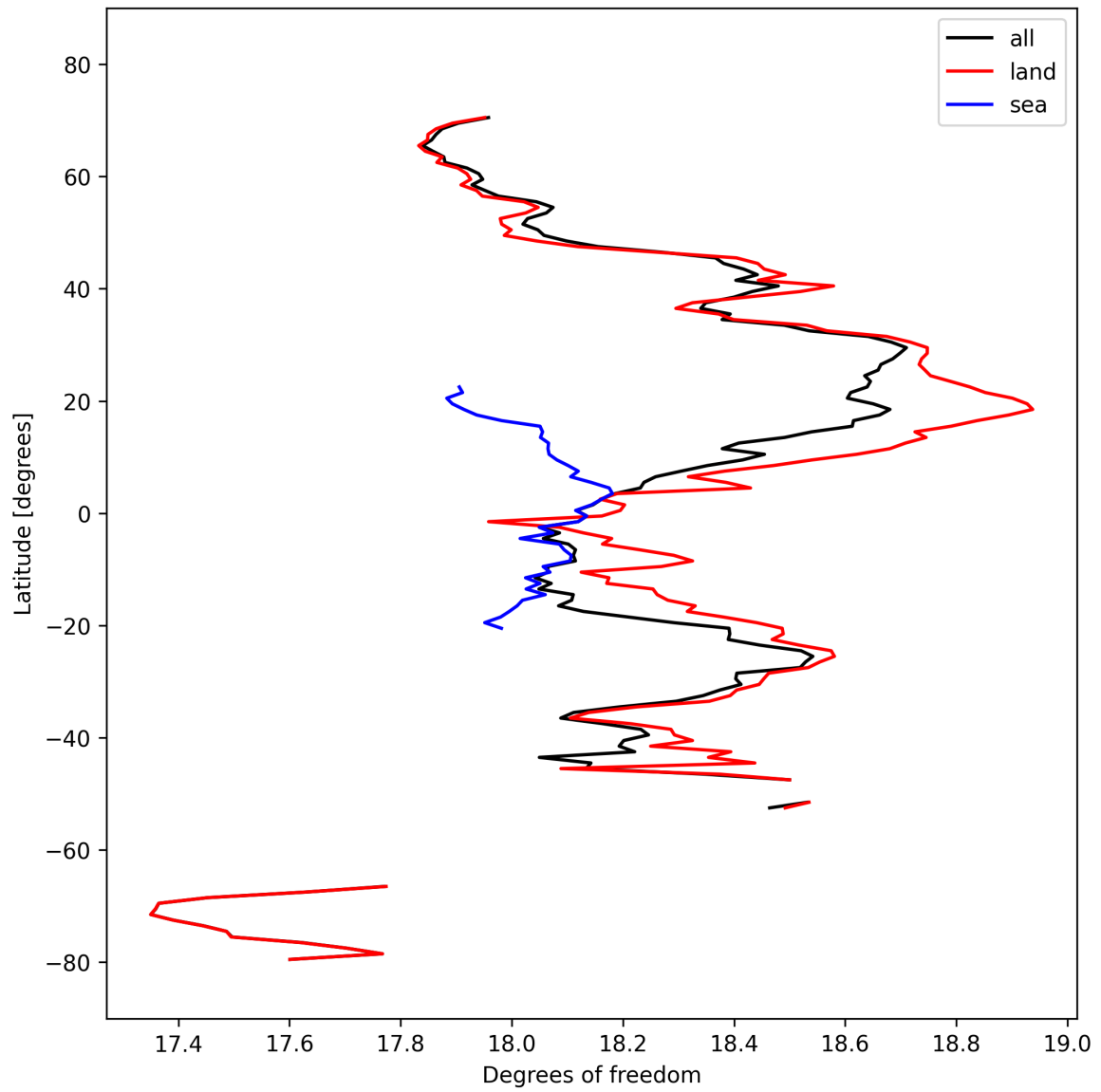
Figure 19: Zonal average of “Degrees of freedom” for 2025-03-08 to 2025-03-10.
