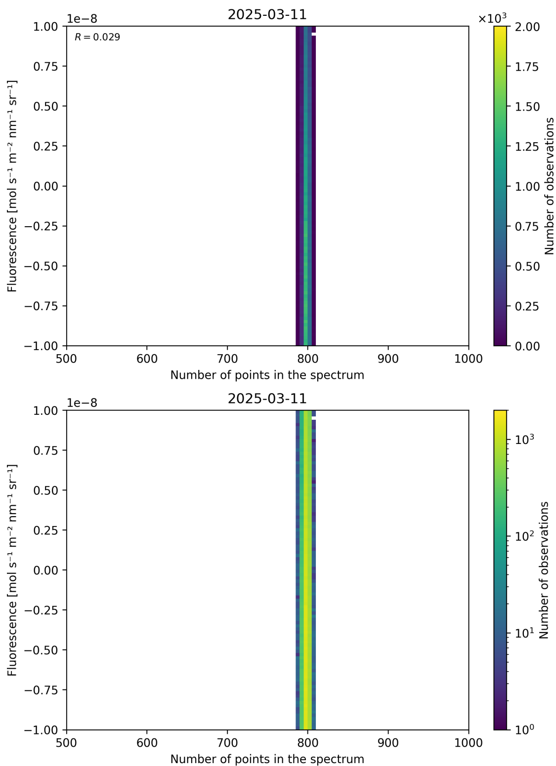
Figure 91: Scatter density plot of “Number of points in the spectrum” against “Fluorescence” for 2025-03-10 to 2025-03-12.
