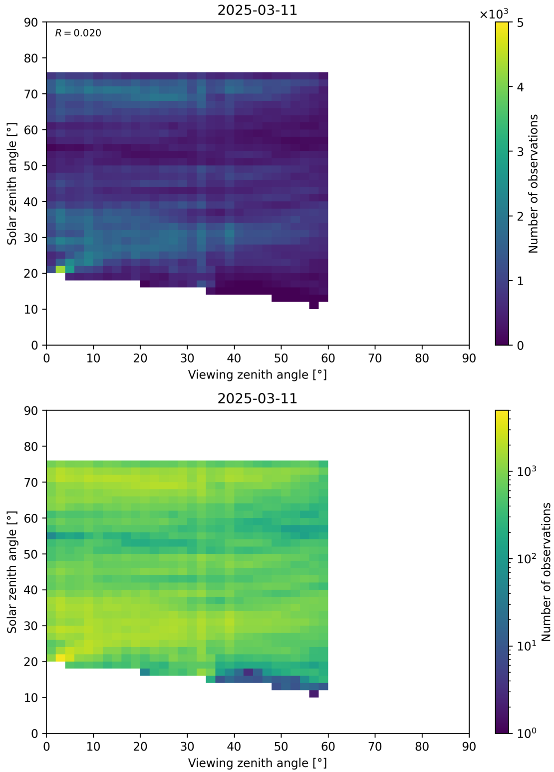
Figure 115: Scatter density plot of “Viewing zenith angle” against “Solar zenith angle” for 2025-03-10 to 2025-03-12.
