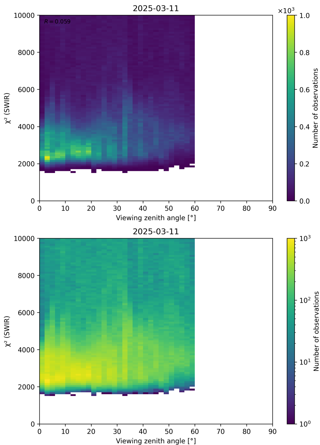
Figure 106: Scatter density plot of “Viewing zenith angle” against “ \chi^2 (SWIR)” for 2025-03-10 to 2025-03-12.
