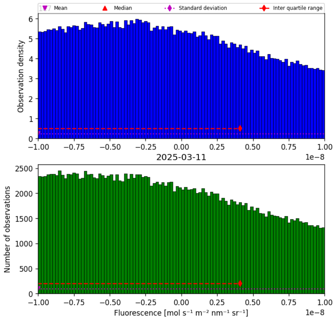
Figure 32: Histogram of “Fluorescence” for 2025-03-10 to 2025-03-12
