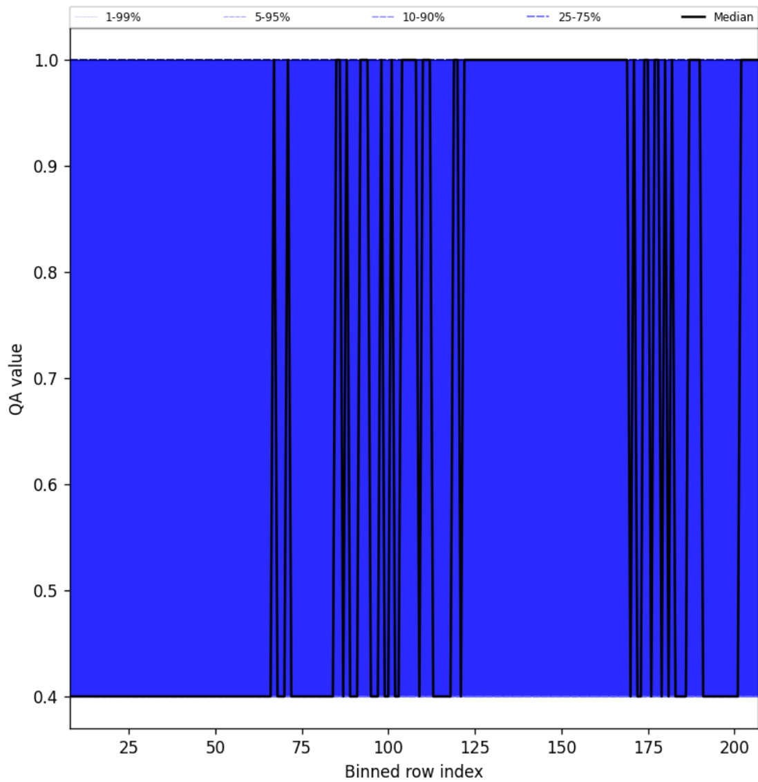
Figure 33: Along track statistics of “QA value” for 2025-03-10 to 2025-03-12
