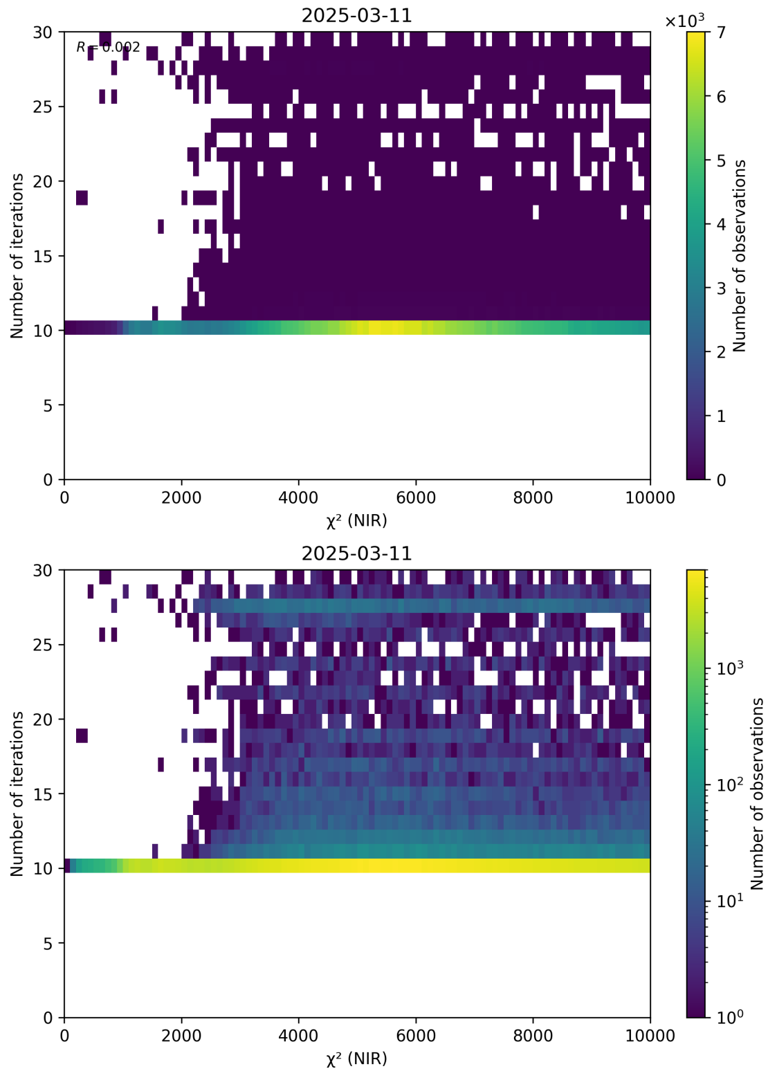
Figure 46: Scatter density plot of “ \chi^2 (NIR)” against “Number of iterations” for 2025-03-10 to 2025-03-12.
