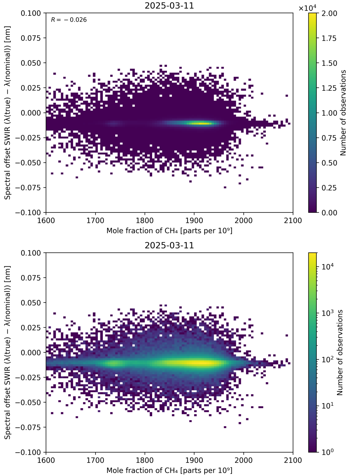
Figure 86: Scatter density plot of “Mole fraction of CH 4 ” against “Spectral offset SWIR ( \lambda_{\text{true}} - \lambda_{\text{nominal}} )” for 2025-03-10 to 2025-03-12.
