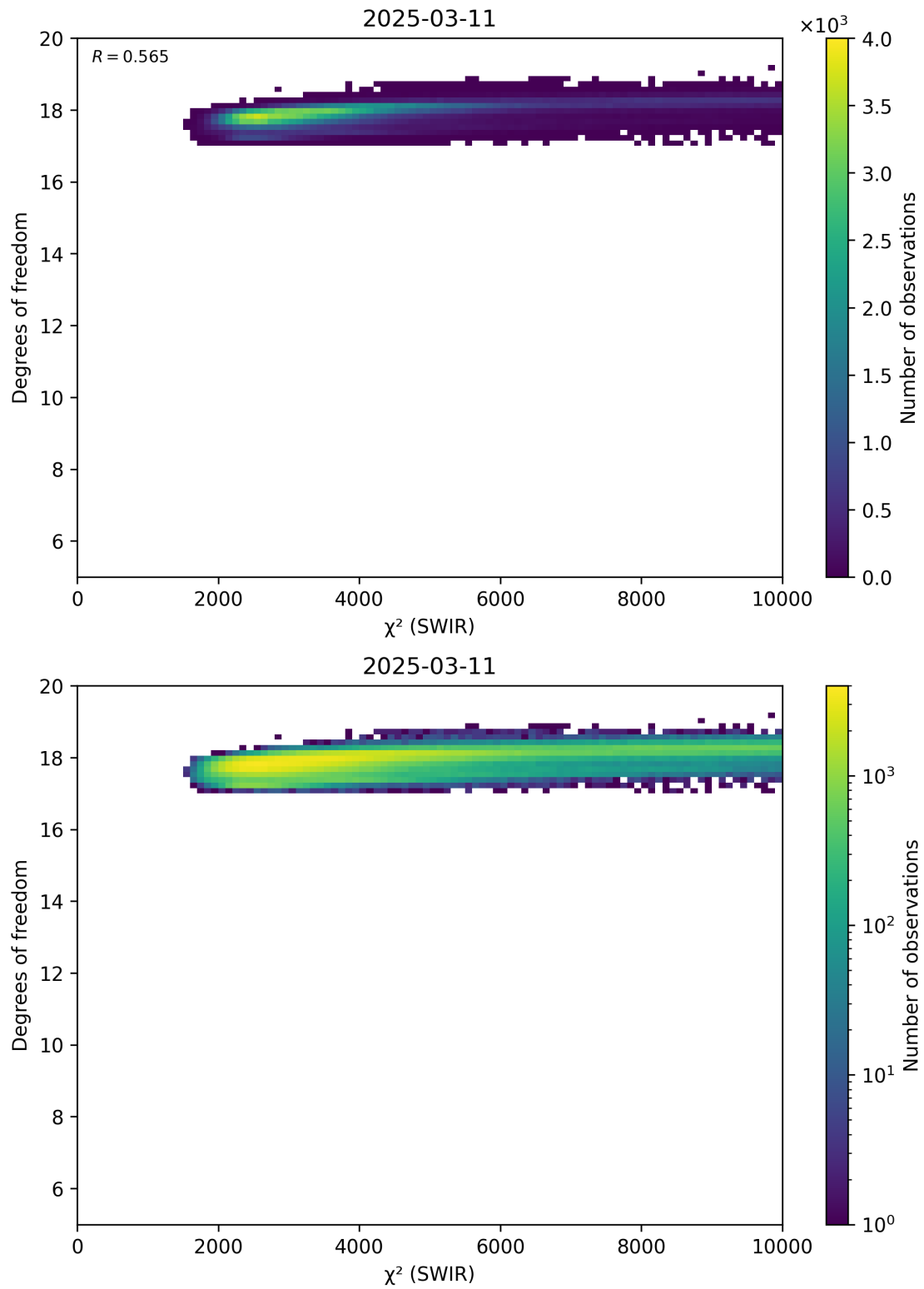
Figure 48: Scatter density plot of " \chi^2 (SWIR)" against "Degrees of freedom" for 2025-03-10 to 2025-03-12.
