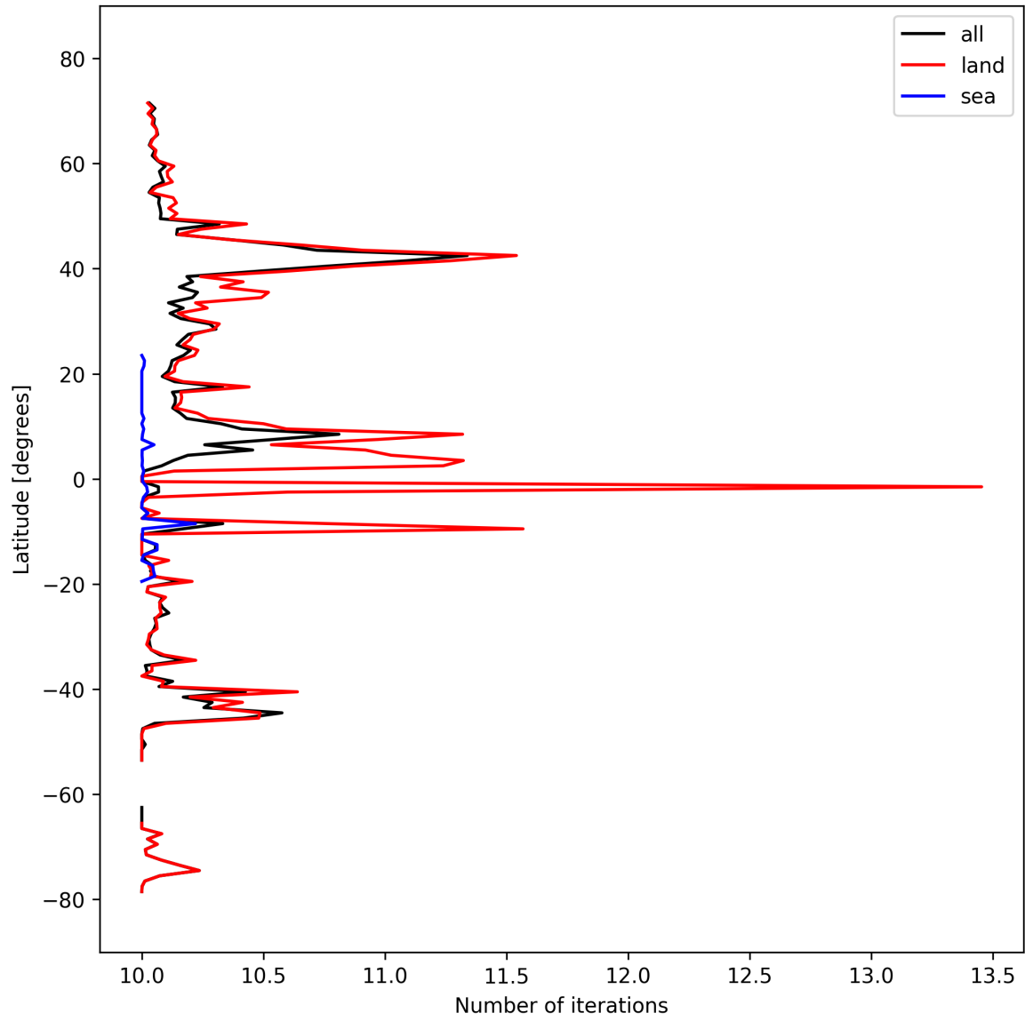
Figure 20: Zonal average of “Number of iterations” for 2025-03-10 to 2025-03-12.
