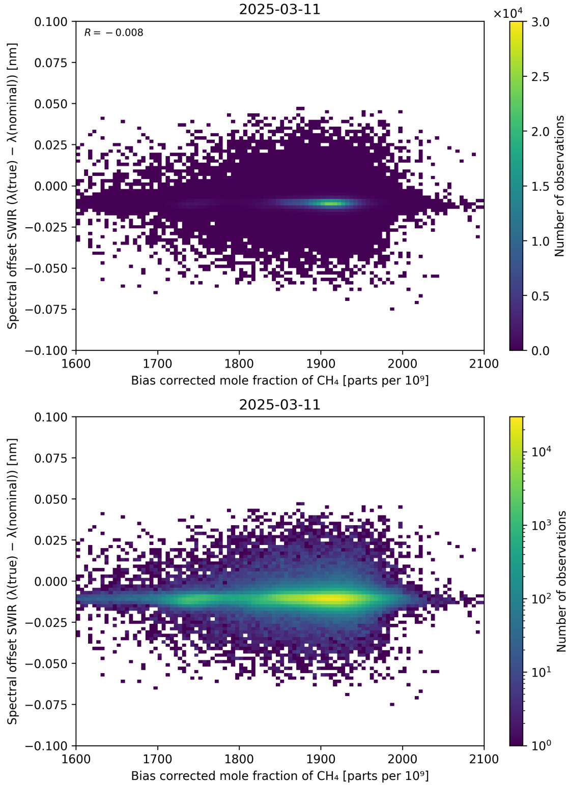
Figure 69: Scatter density plot of “Bias corrected mole fraction of \text{CH}_4 ” against “Spectral offset SWIR ( \lambda_{\text{true}} - \lambda_{\text{nominal}} )” for 2025-03-10 to 2025-03-12.
