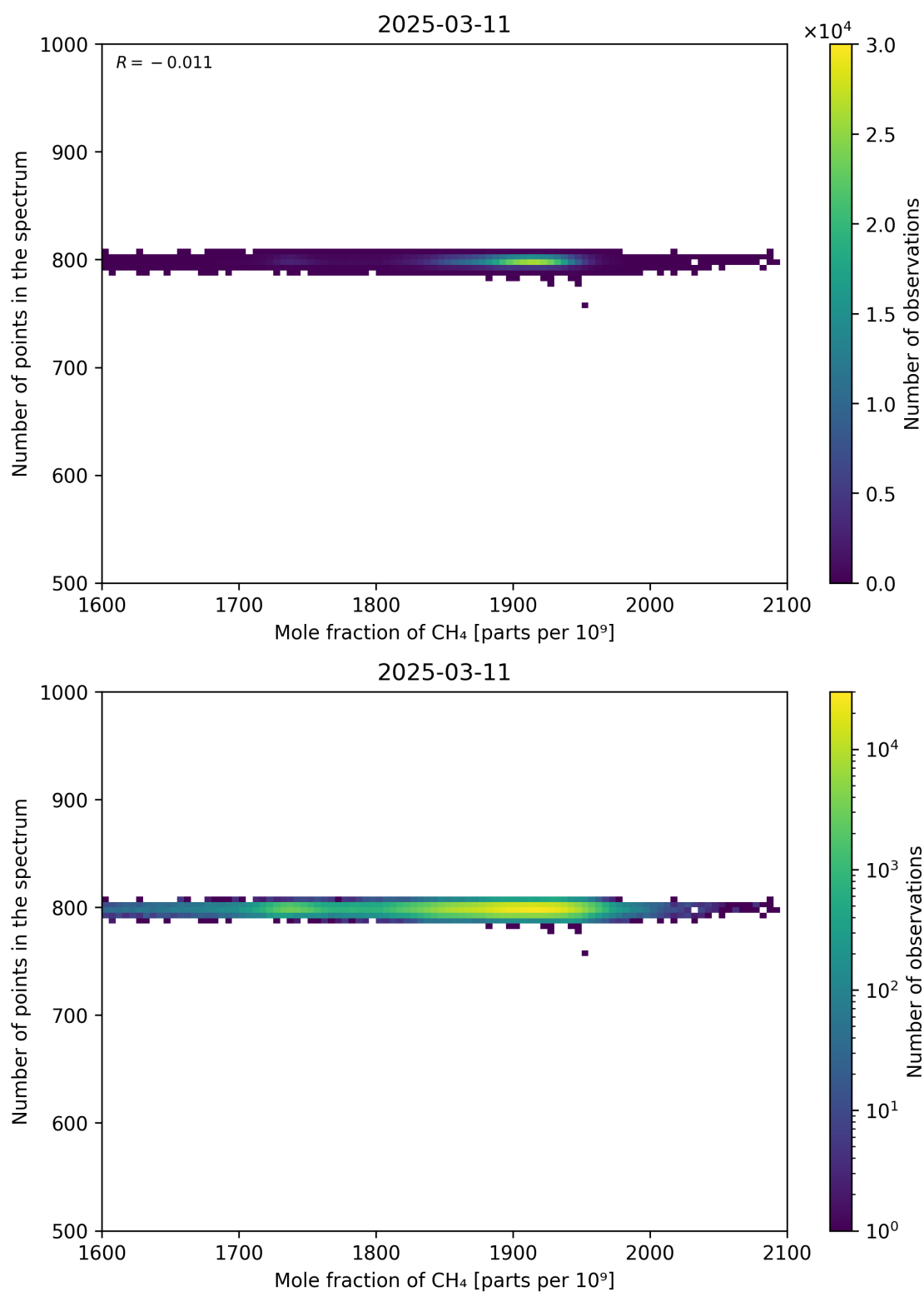
Figure 77: Scatter density plot of “Mole fraction of CH 4 ” against “Number of points in the spectrum” for 2025-03-10 to 2025-03-12.
