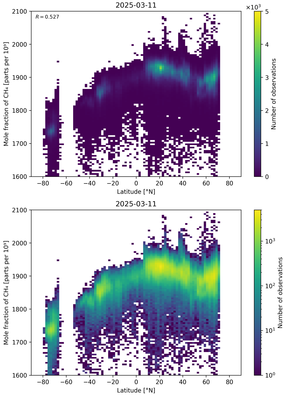
Figure 57: Scatter density plot of “Latitude” against “Mole fraction of CH 4 ” for 2025-03-10 to 2025-03-12.
