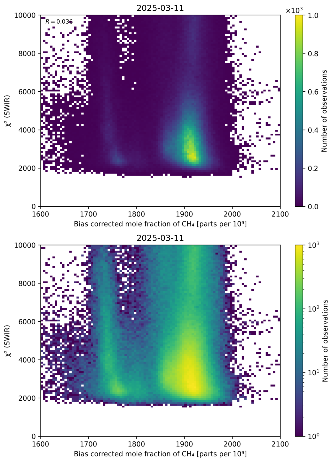
Figure 64: Scatter density plot of “Bias corrected mole fraction of \text{CH}_4 ” against “ \chi^2 (SWIR)” for 2025-03-10 to 2025-03-12.
