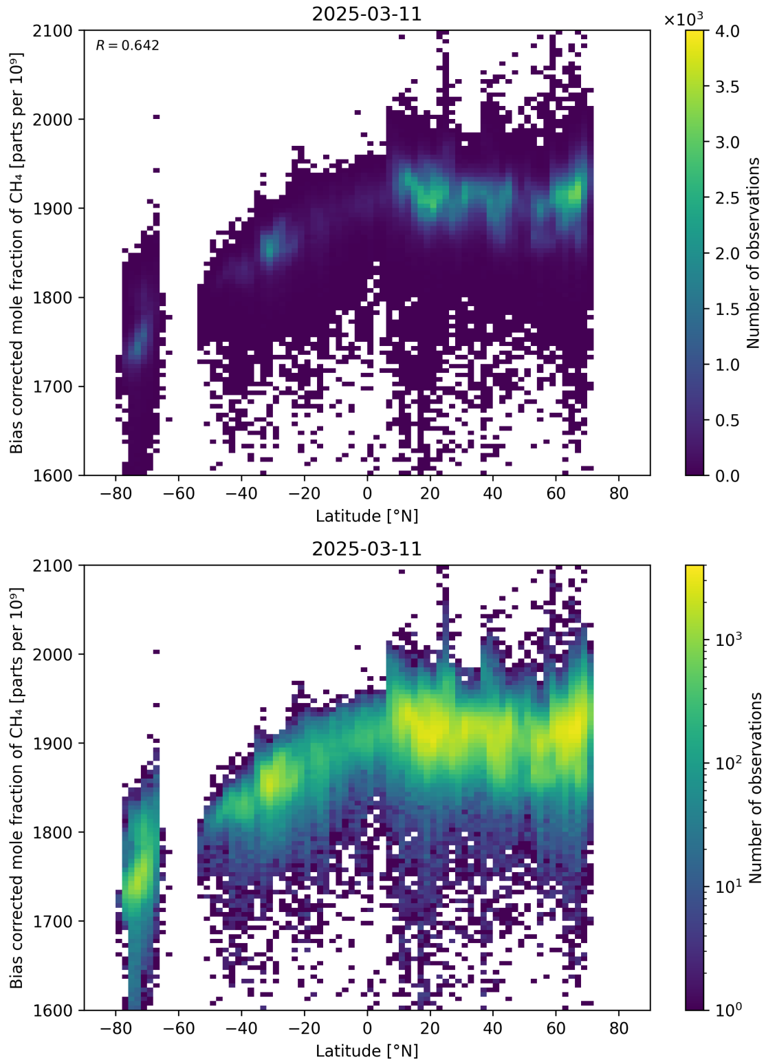
Figure 58: Scatter density plot of “Latitude” against “Bias corrected mole fraction of CH 4 ” for 2025-03-10 to 2025-03-12.
