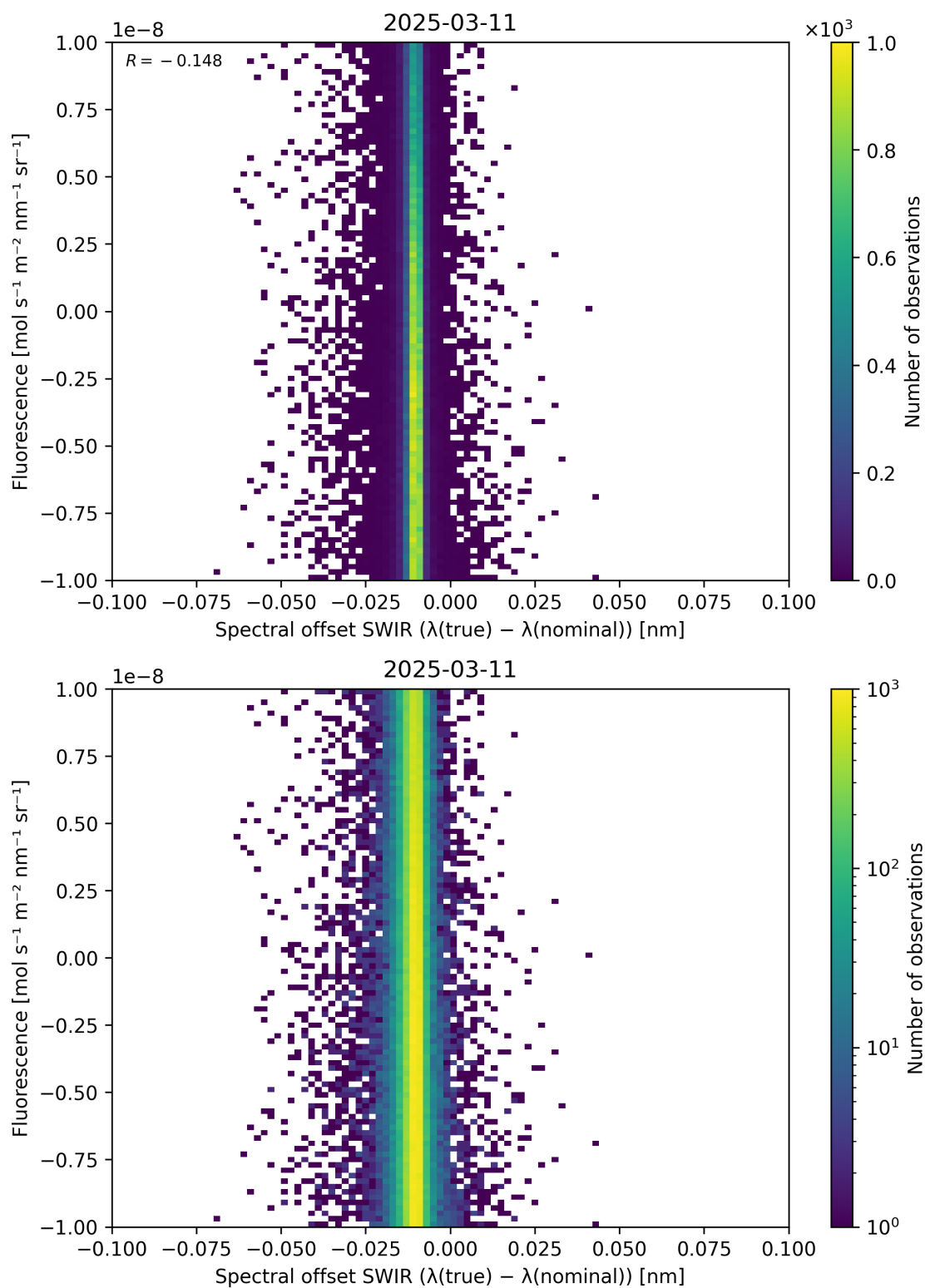
Figure 120: Scatter density plot of “Spectral offset SWIR ( \lambda_{\text{true}} - \lambda_{\text{nominal}} )” against “Fluorescence” for 2025-03-10 to 2025-03-12.
