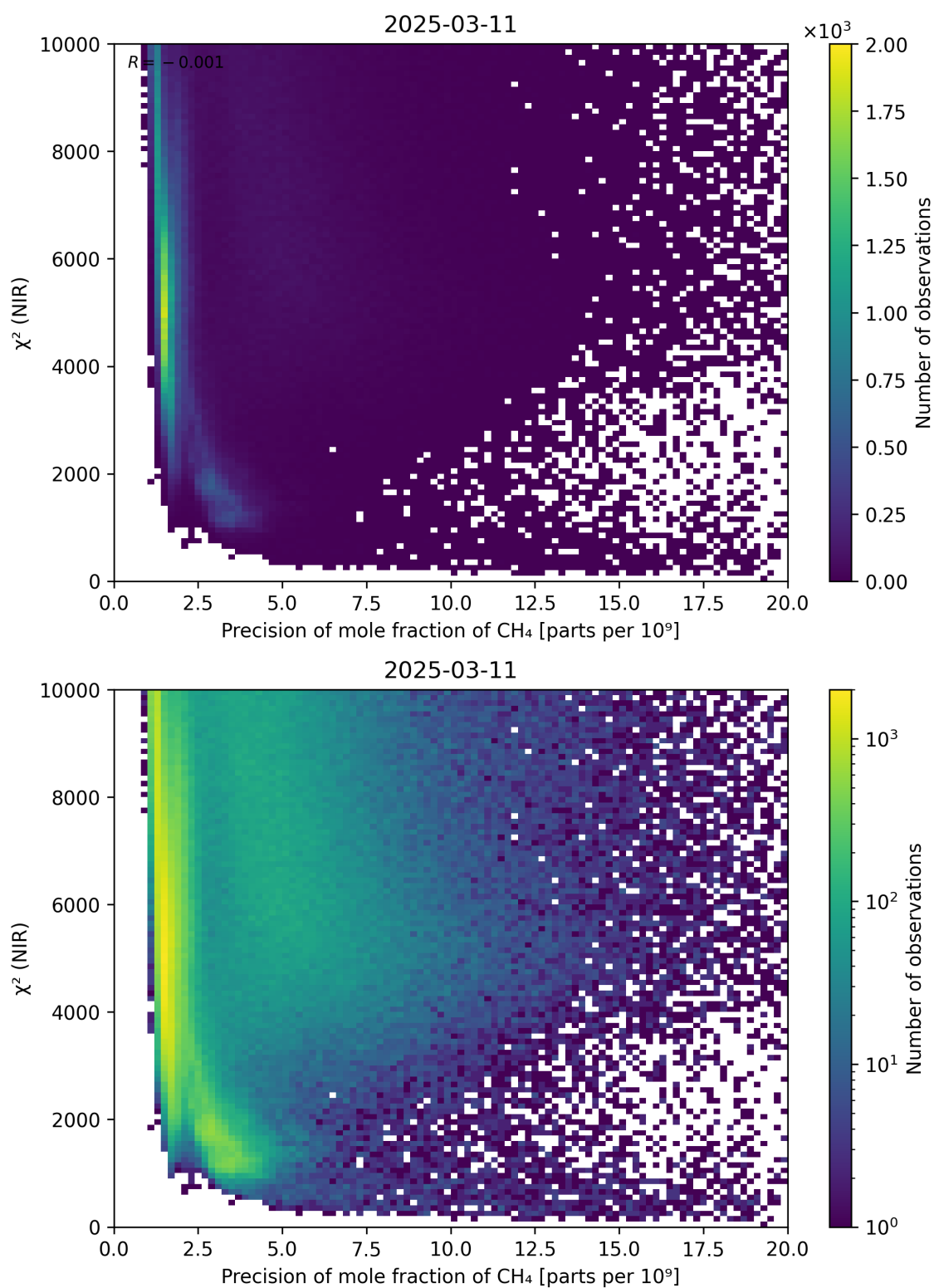
Figure 78: Scatter density plot of “Precision of mole fraction of CH 4 ” against “ \chi^2 (NIR)” for 2025-03-10 to 2025-03-12.
