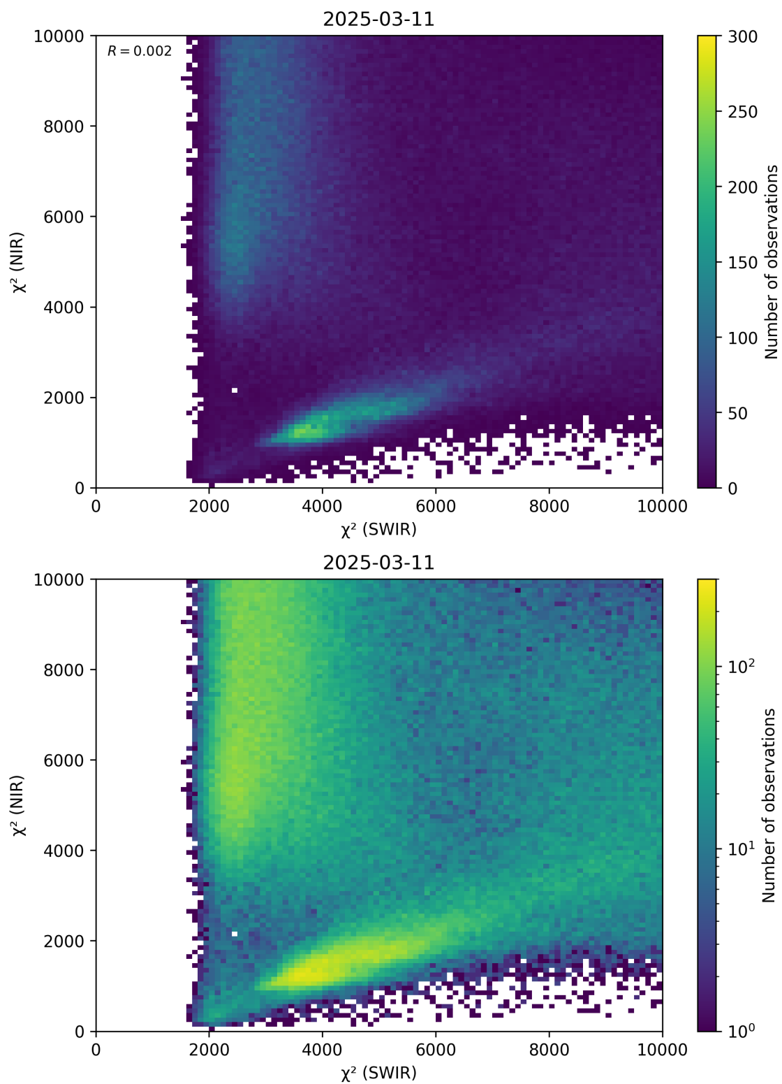
Figure 47: Scatter density plot of “ \chi^2 (SWIR)” against “ \chi^2 (NIR)” for 2025-03-10 to 2025-03-12.
