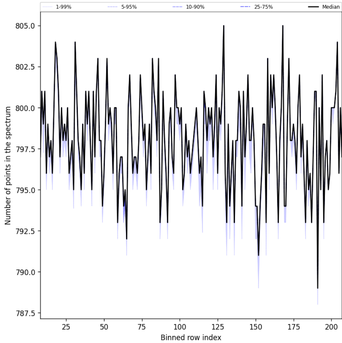
Figure 37: Along track statistics of “Number of points in the spectrum” for 2025-03-10 to 2025-03-12
