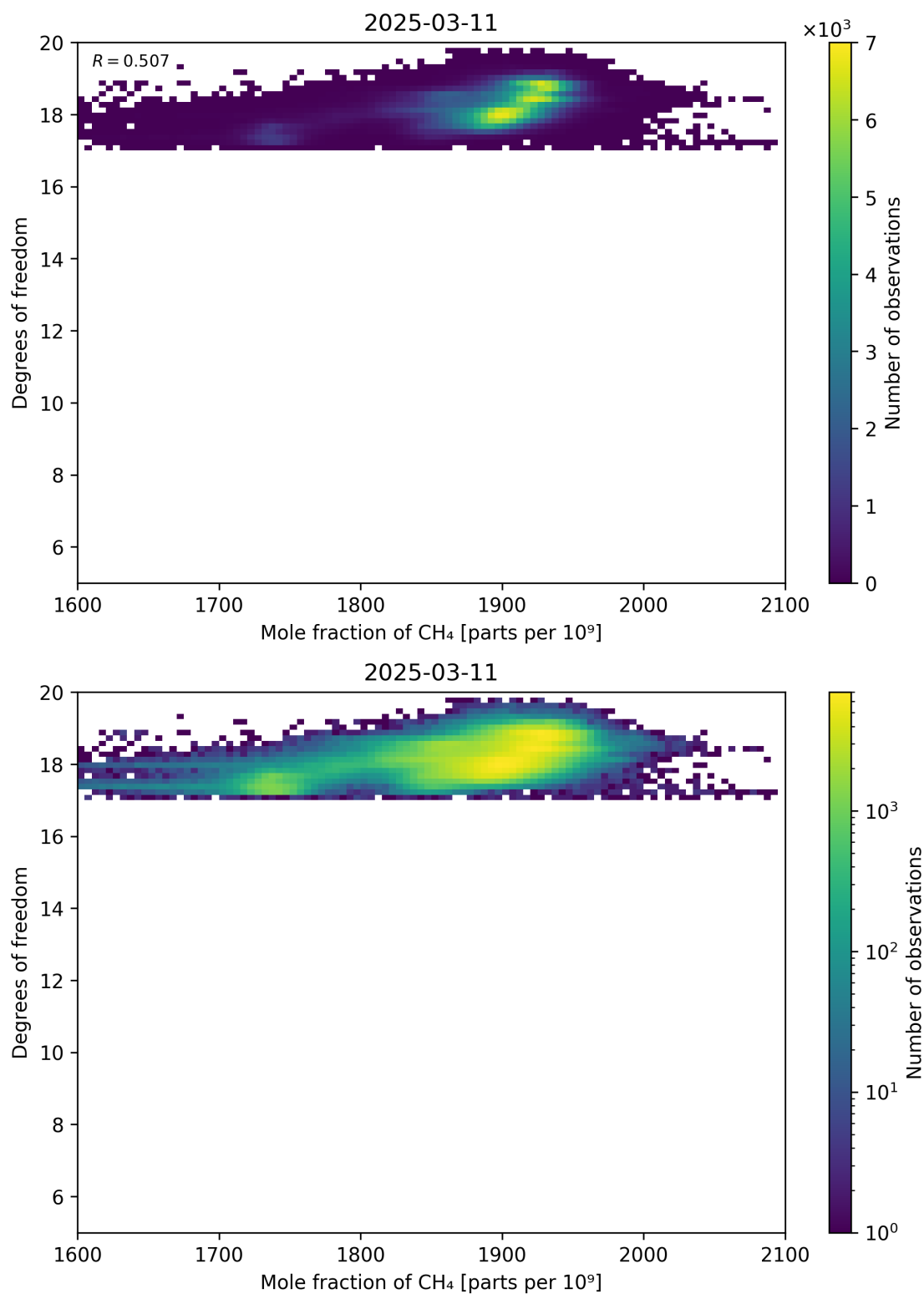
Figure 72: Scatter density plot of “Mole fraction of CH 4 ” against “Degrees of freedom” for 2025-03-10 to 2025-03-12.
