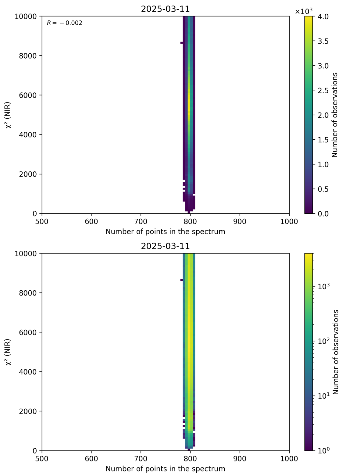
Figure 88: Scatter density plot of “Number of points in the spectrum” against “ \chi^2 (NIR)” for 2025-03-10 to 2025-03-12.
