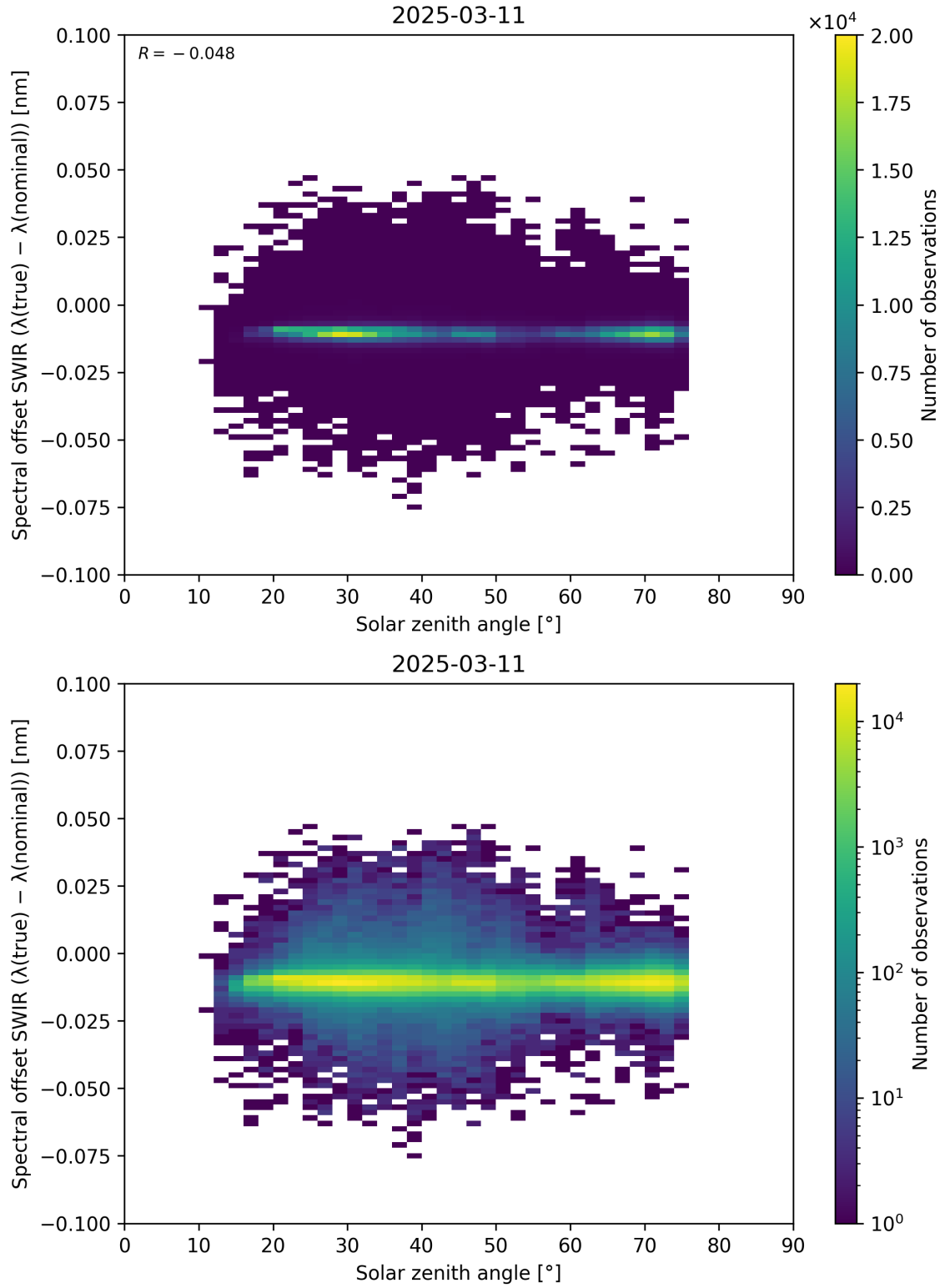
Figure 104: Scatter density plot of “Solar zenith angle” against “Spectral offset SWIR ( \lambda_{\text{true}} - \lambda_{\text{nominal}} )” for 2025-03-10 to 2025-03-12.
