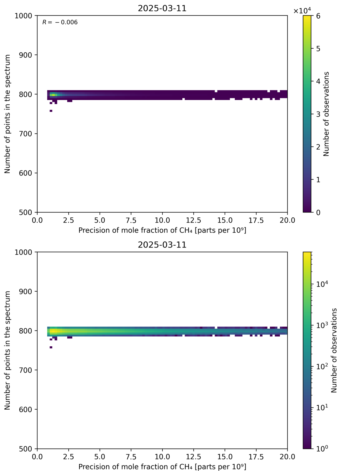
Figure 84: Scatter density plot of “Precision of mole fraction of CH 4 ” against “Number of points in the spectrum” for 2025-03-10 to 2025-03-12.
