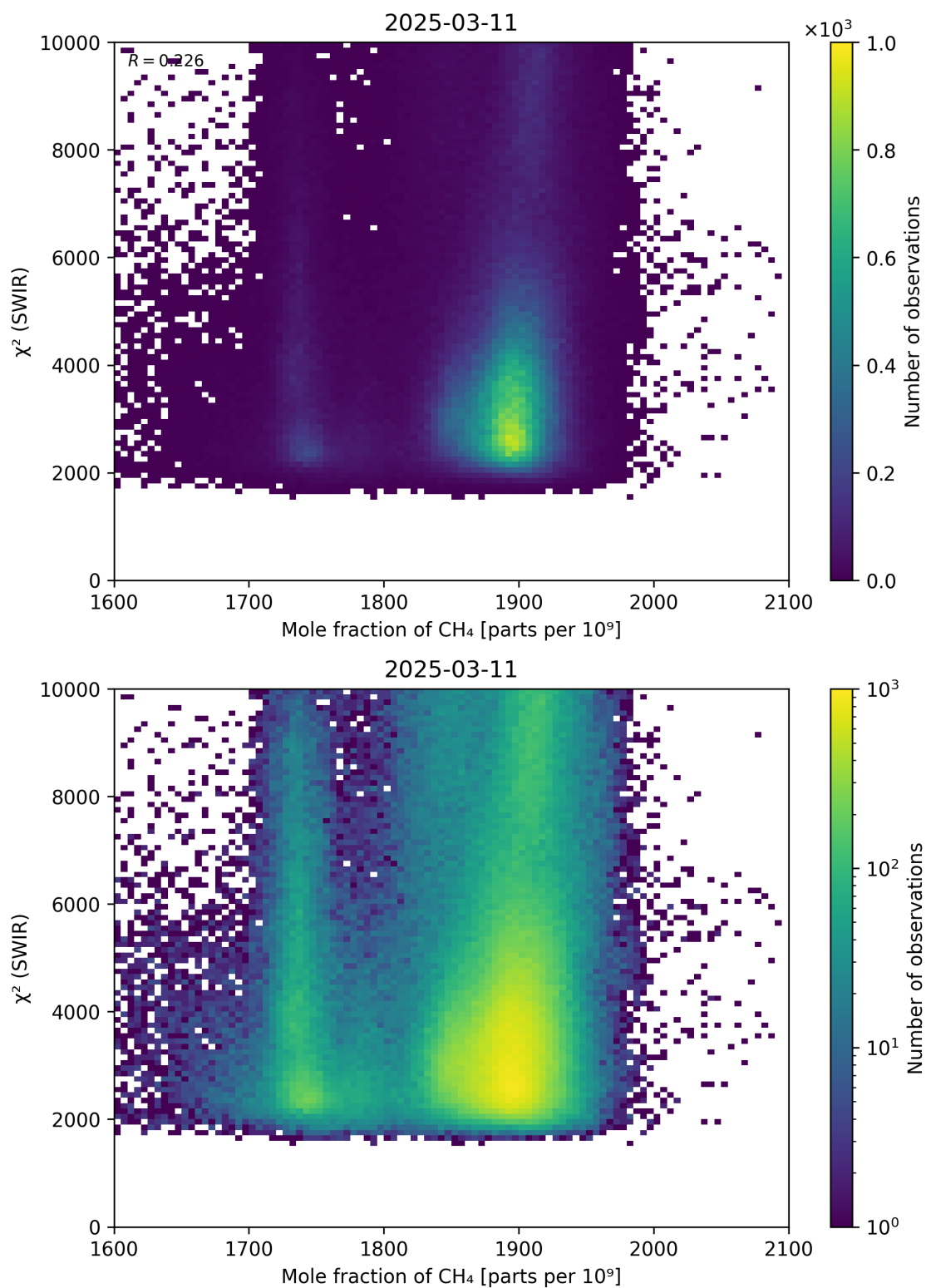
Figure 71: Scatter density plot of “Mole fraction of \text{CH}_4 ” against “ \chi^2 (SWIR)” for 2025-03-10 to 2025-03-12.
