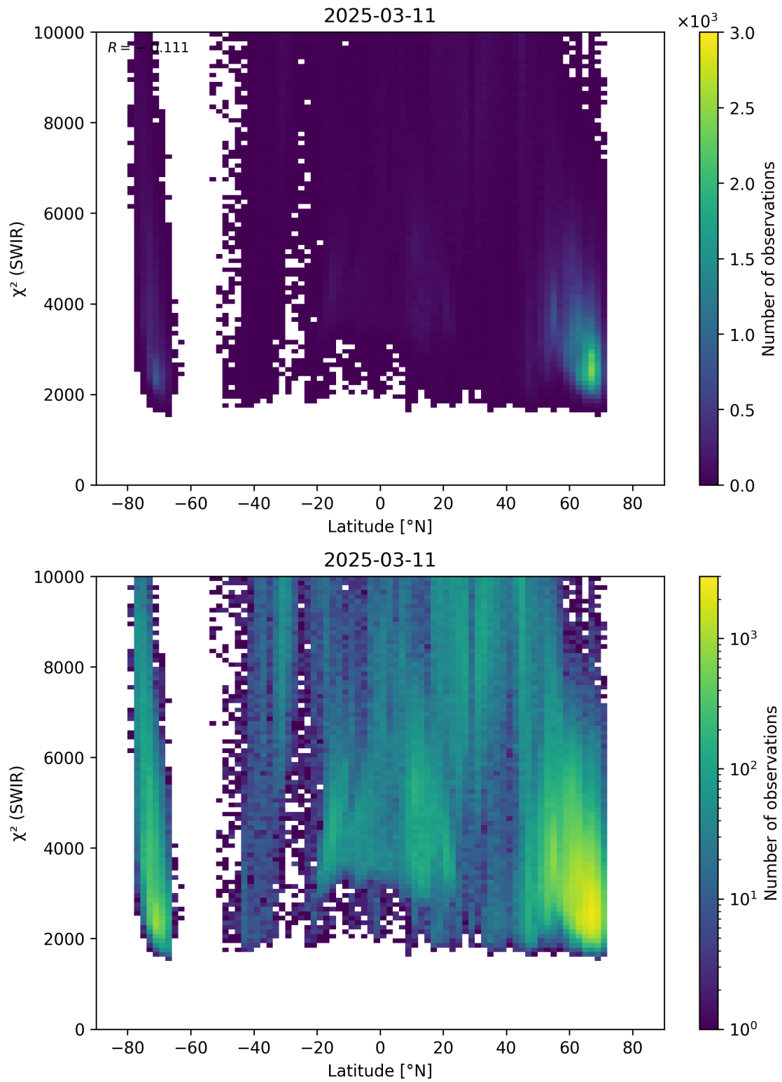
Figure 54: Scatter density plot of “Latitude” against “ \chi^2 (SWIR)” for 2025-03-10 to 2025-03-12.
