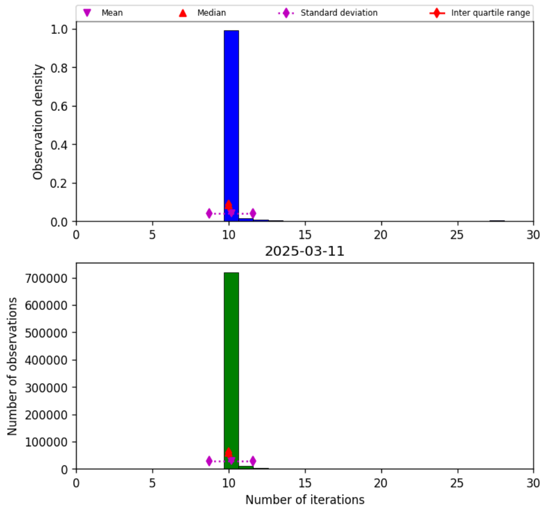
Figure 31: Histogram of “Number of iterations” for 2025-03-10 to 2025-03-12
