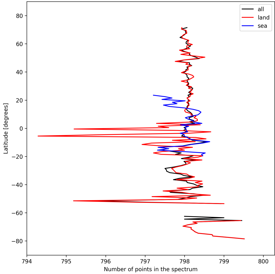
Figure 15: Zonal average of “Number of points in the spectrum” for 2025-03-10 to 2025-03-12.
