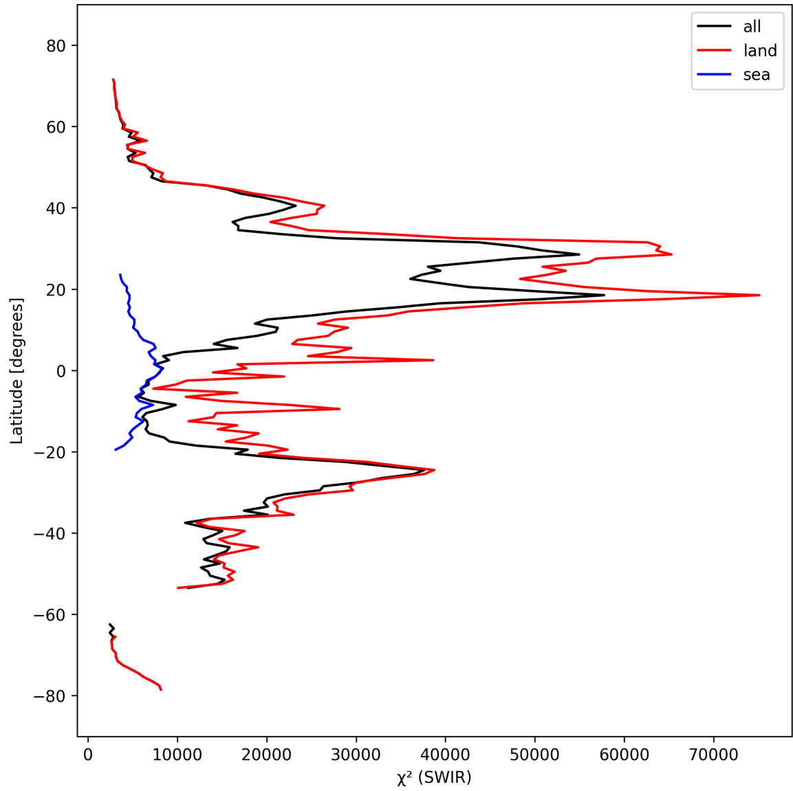
Figure 17: Zonal average of “ \chi^2 (SWIR)” for 2025-03-10 to 2025-03-12.
