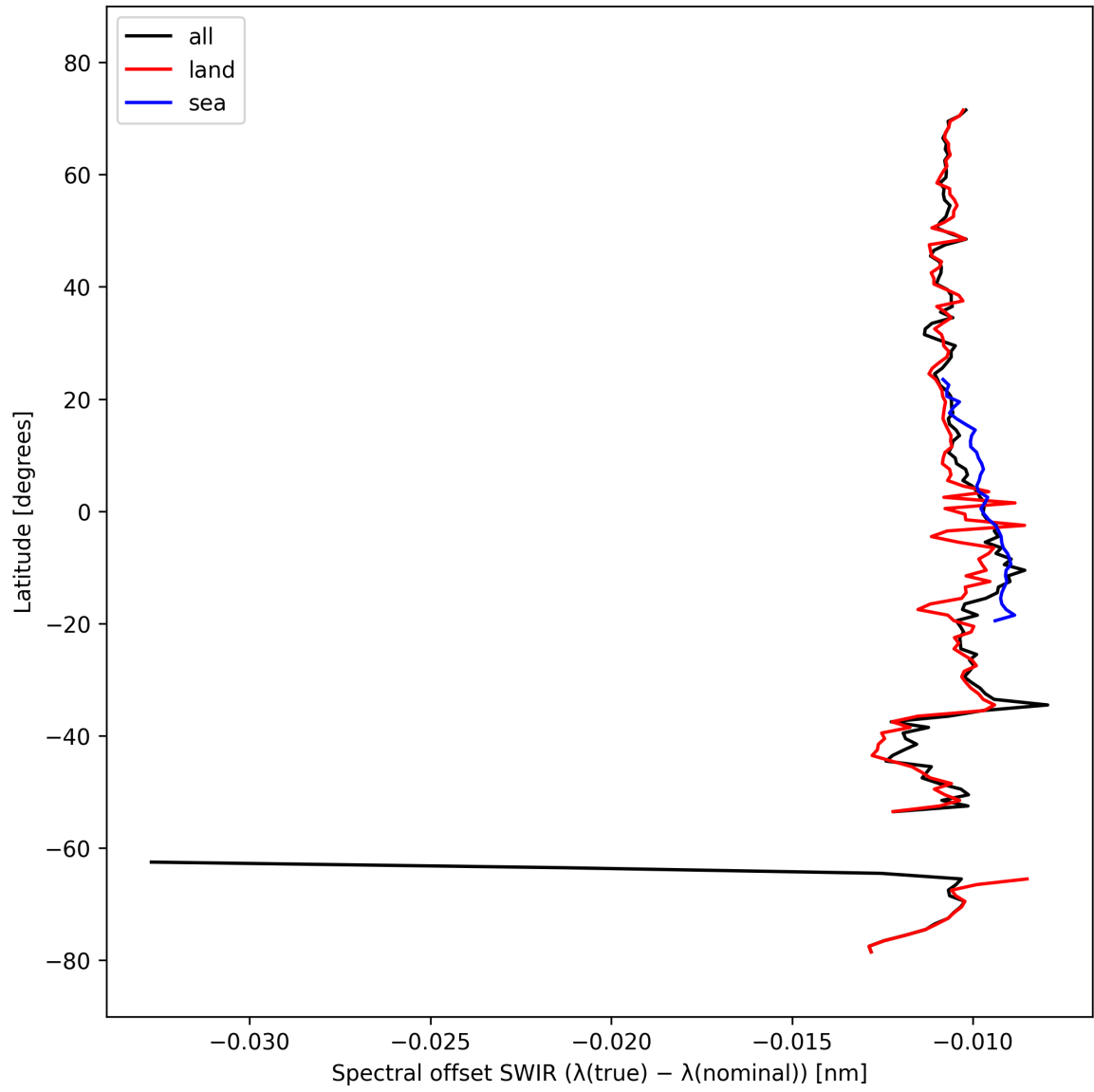
Figure 16: Zonal average of “Spectral offset SWIR ( \lambda_{\text{true}} - \lambda_{\text{nominal}} )” for 2025-03-10 to 2025-03-12.
