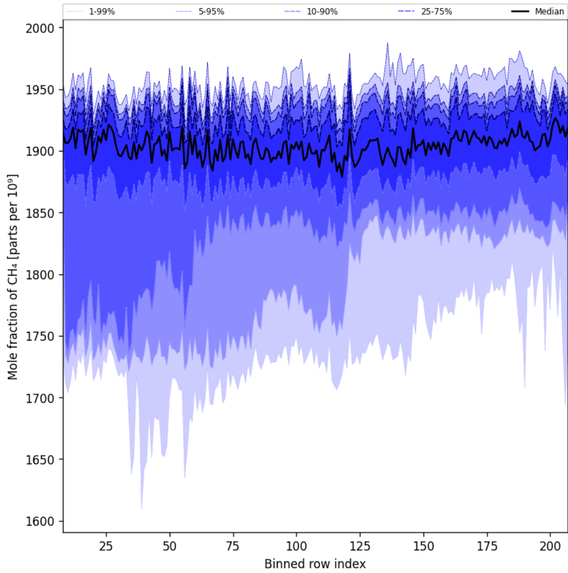
Figure 34: Along track statistics of “Mole fraction of CH 4 ” for 2025-03-10 to 2025-03-12
