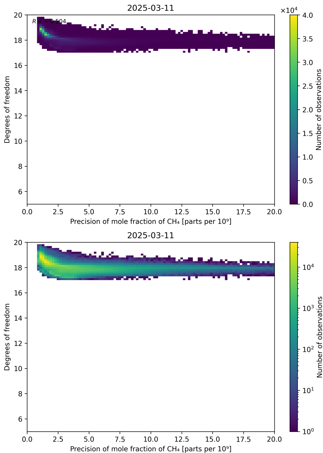
Figure 80: Scatter density plot of “Precision of mole fraction of CH 4 ” against “Degrees of freedom” for 2025-03-10 to 2025-03-12.
