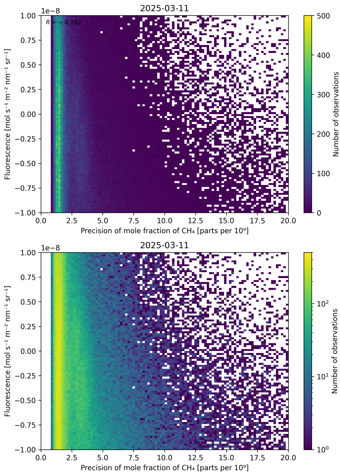
Figure 81: Scatter density plot of “Precision of mole fraction of CH 4 ” against “Fluorescence” for 2025-03-10 to 2025-03-12.
