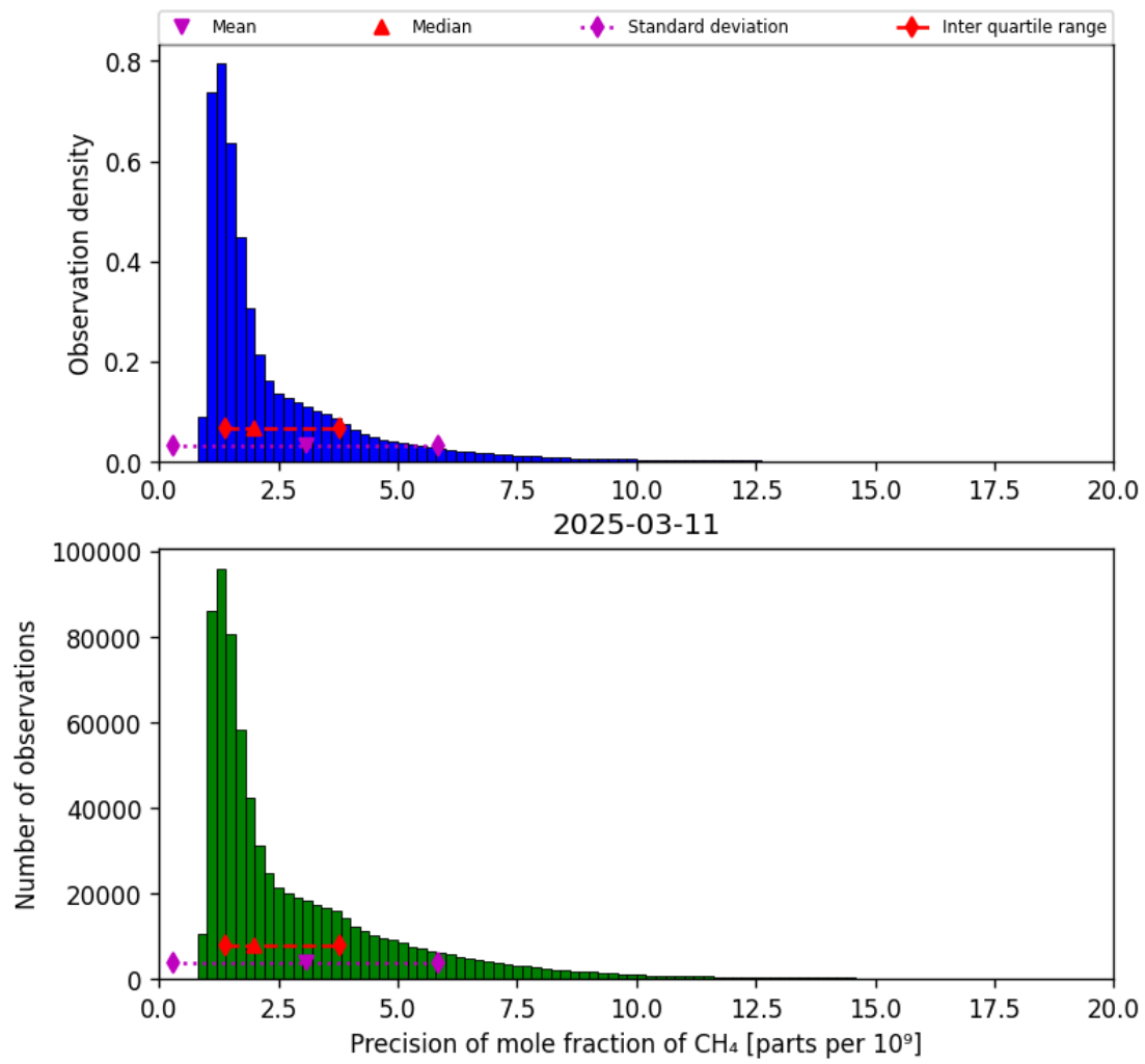
Figure 24: Histogram of “Precision of mole fraction of CH 4 ” for 2025-03-10 to 2025-03-12
