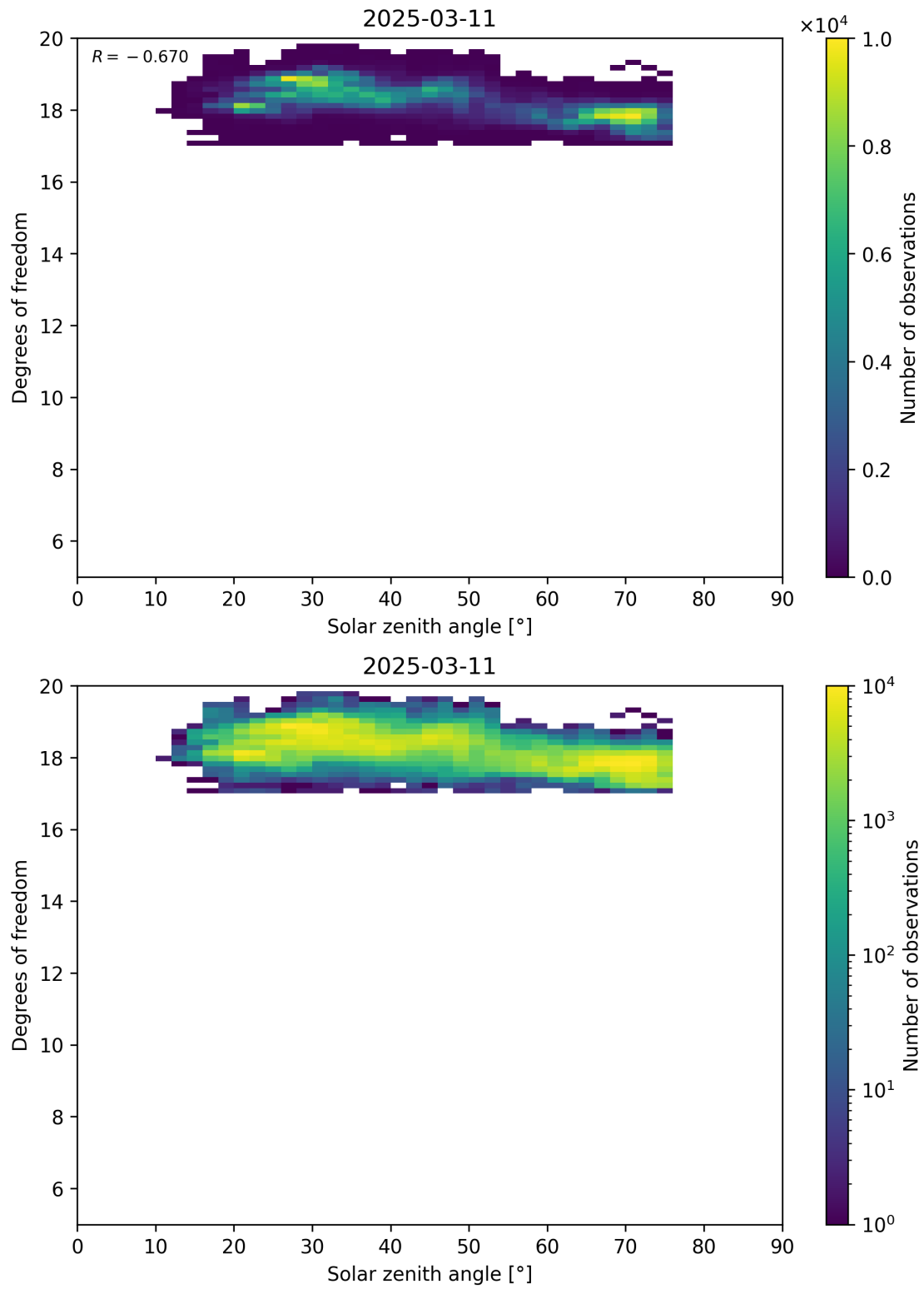
Figure 96: Scatter density plot of “Solar zenith angle” against “Degrees of freedom” for 2025-03-10 to 2025-03-12.
