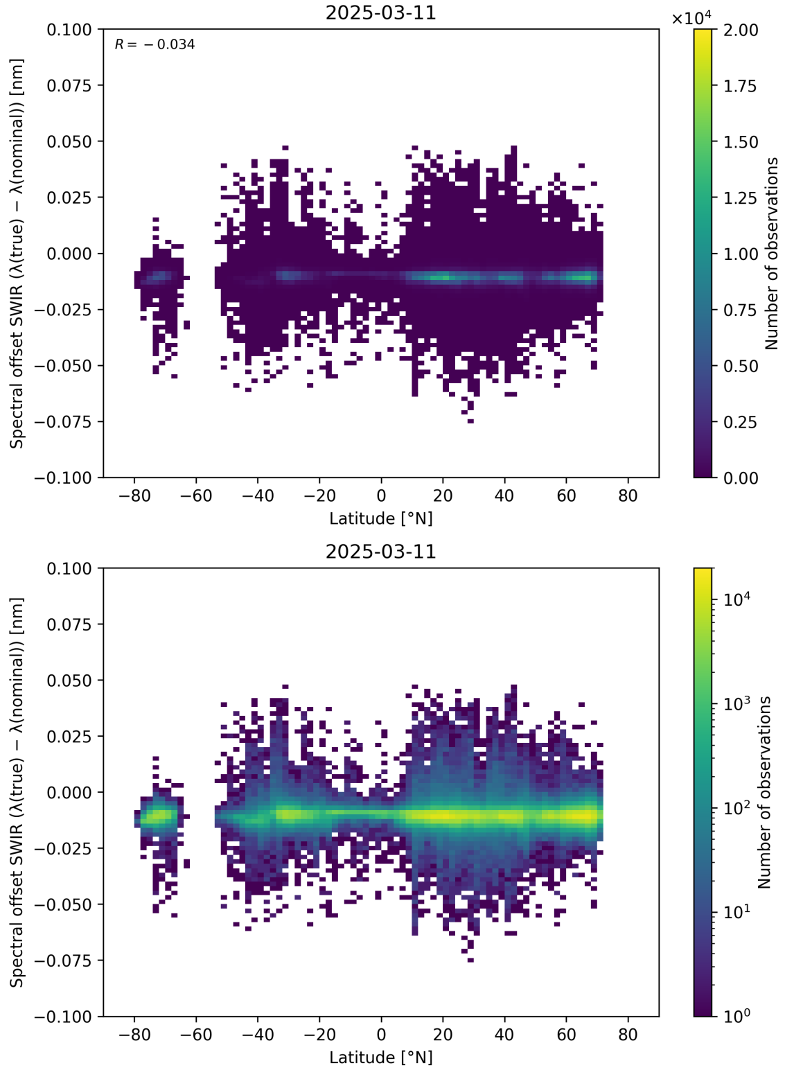
Figure 62: Scatter density plot of “Latitude” against “Spectral offset SWIR ( \lambda_{\text{true}} - \lambda_{\text{nominal}} )” for 2025-03-10 to 2025-03-12.
