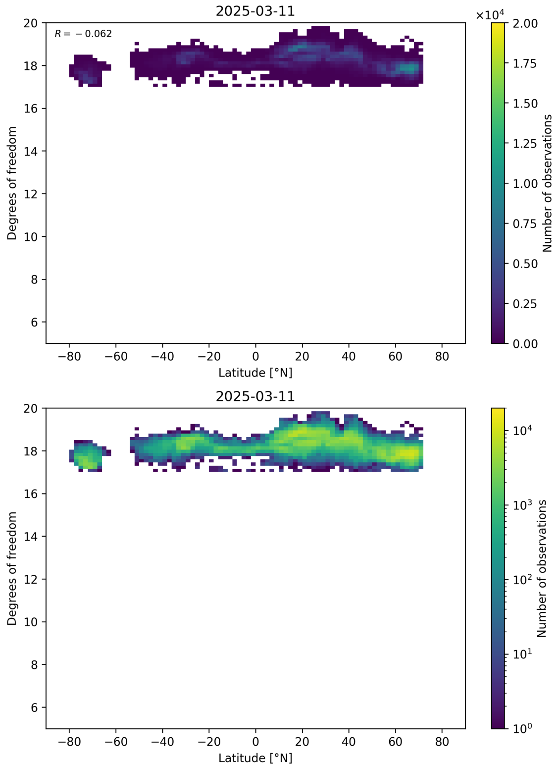
Figure 55: Scatter density plot of “Latitude” against “Degrees of freedom” for 2025-03-10 to 2025-03-12.
