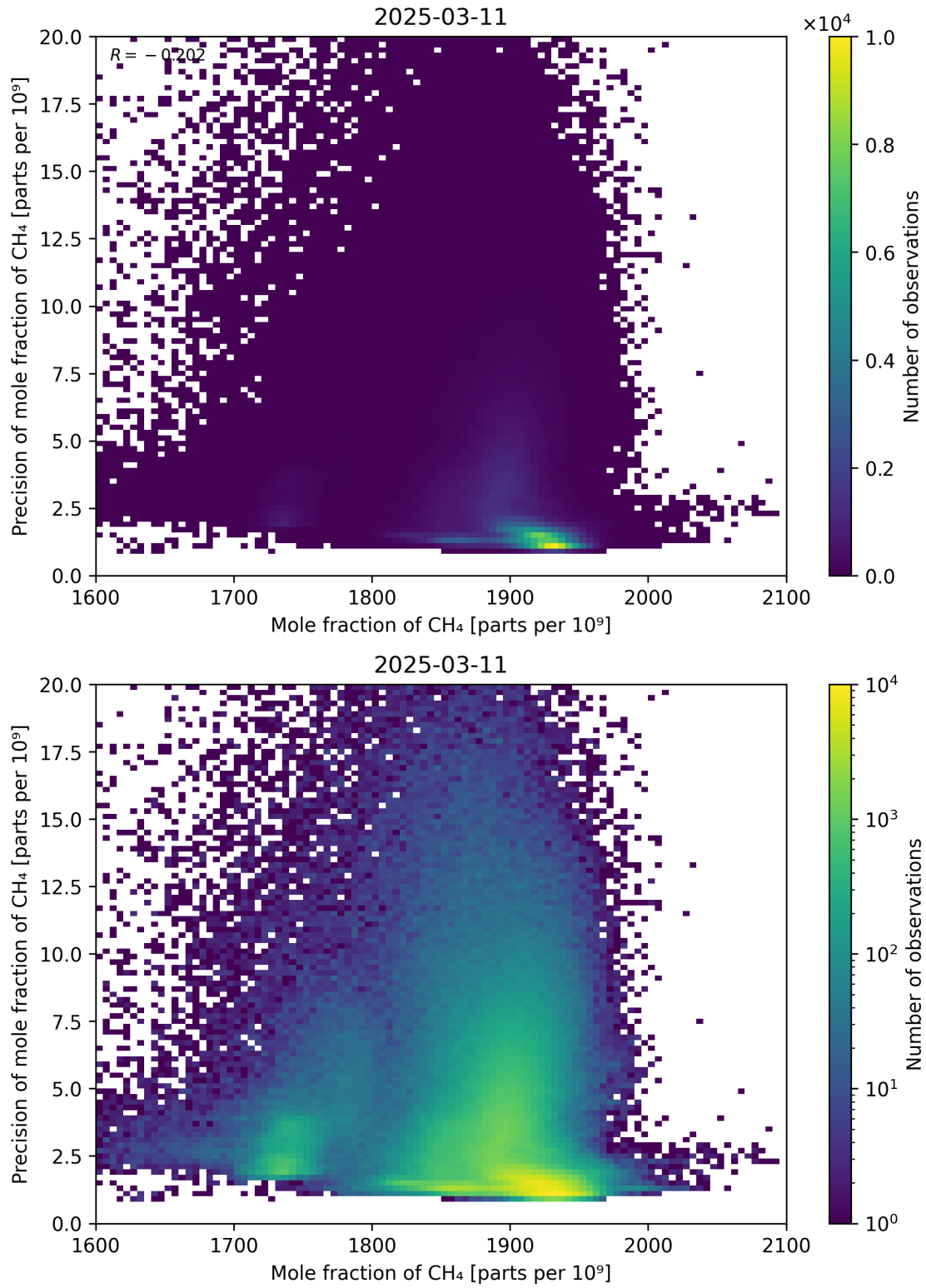
Figure 75: Scatter density plot of “Mole fraction of CH 4 ” against “Precision of mole fraction of CH 4 ” for 2025-03-10 to 2025-03-12.
