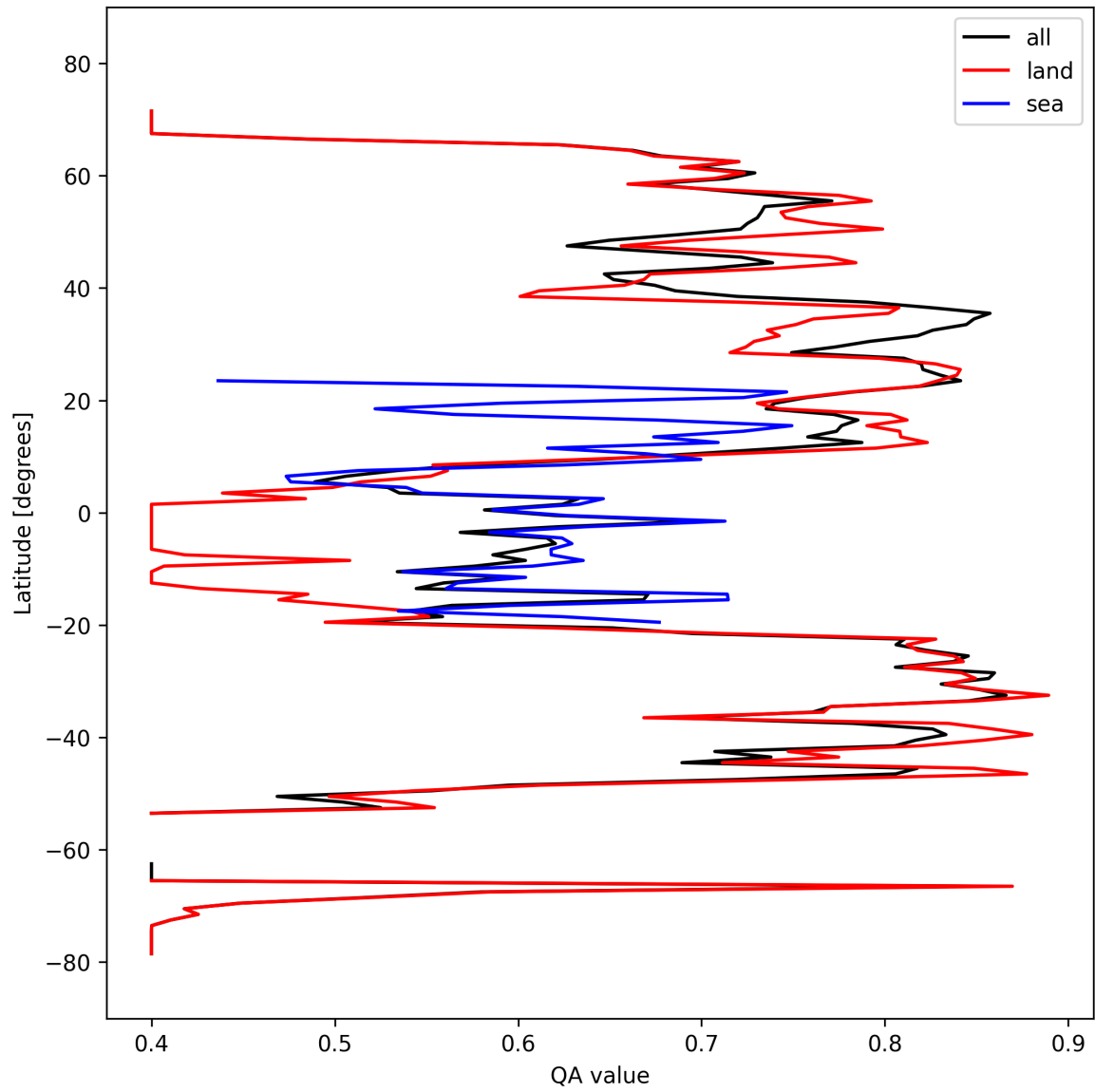
Figure 11: Zonal average of “QA value” for 2025-03-10 to 2025-03-12.
