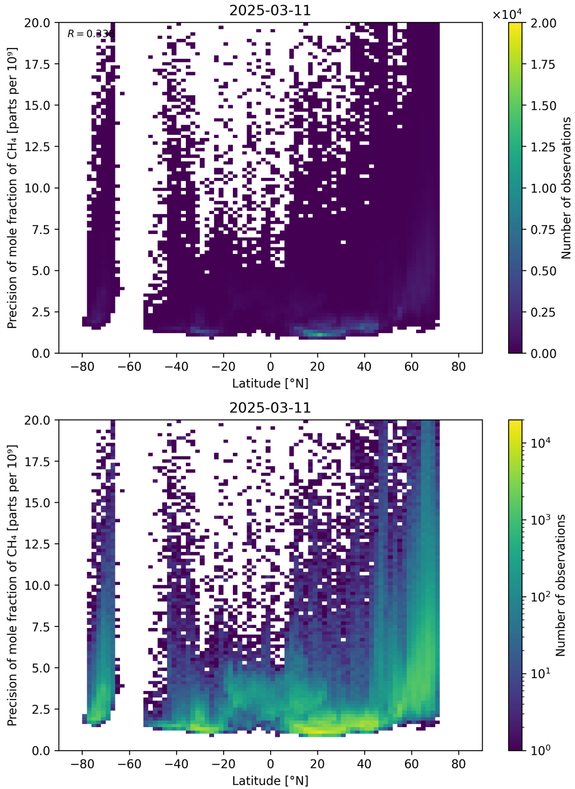
Figure 59: Scatter density plot of “Latitude” against “Precision of mole fraction of CH 4 ” for 2025-03-10 to 2025-03-12.
