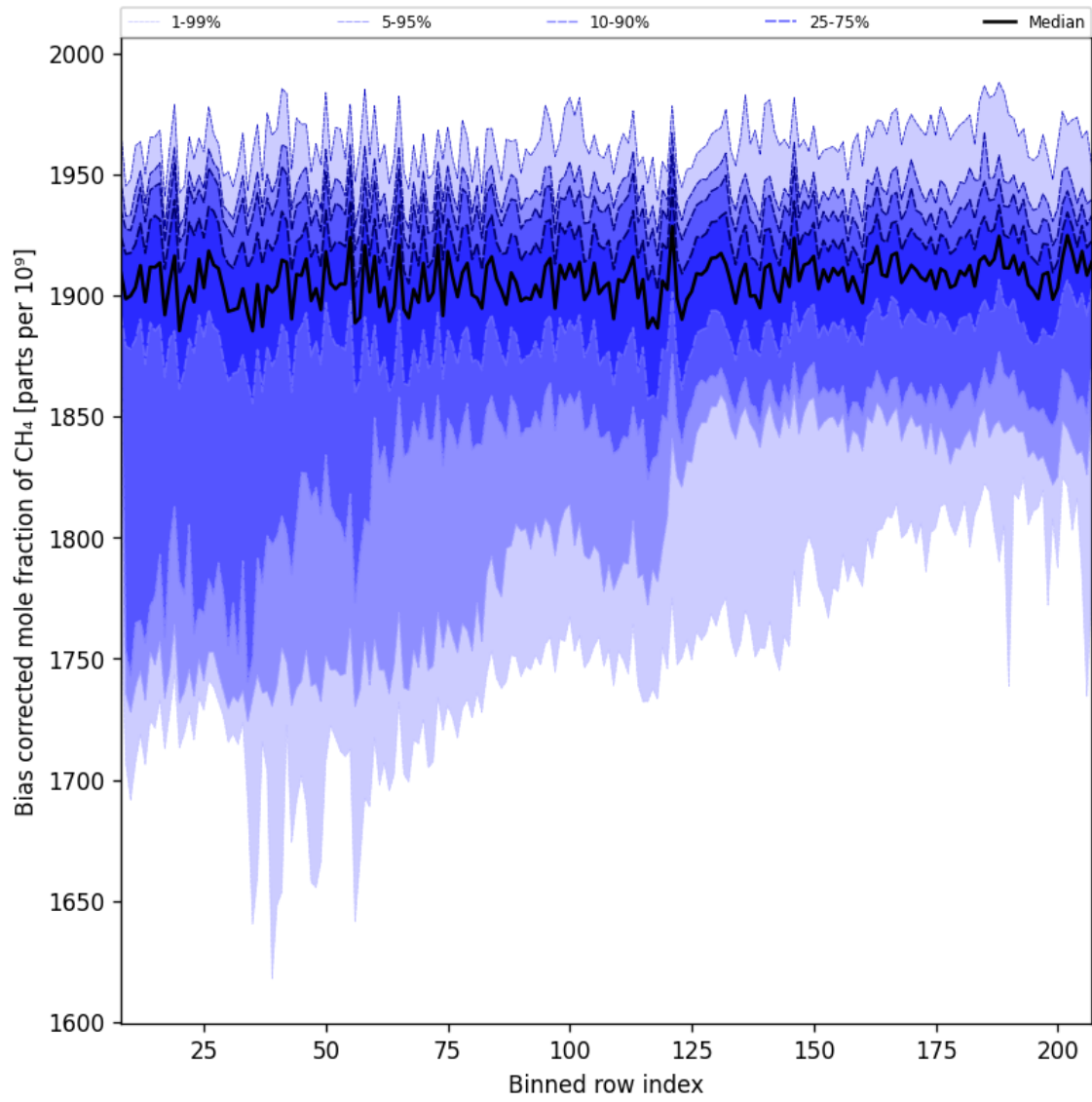
Figure 36: Along track statistics of “Bias corrected mole fraction of CH 4 ” for 2025-03-10 to 2025-03-12
