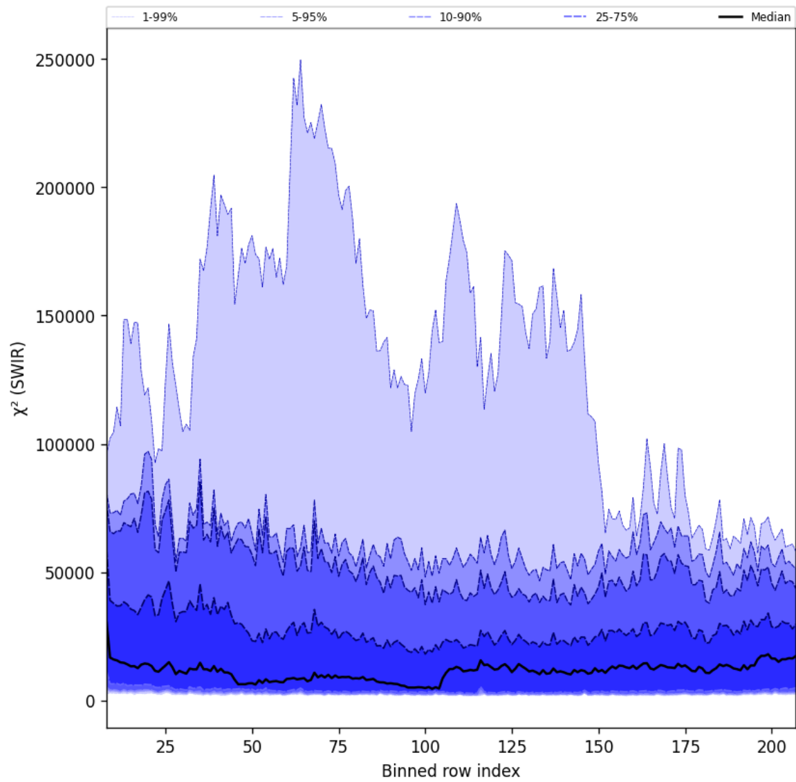
Figure 39: Along track statistics of “ \chi^2 (SWIR)” for 2025-03-10 to 2025-03-12
