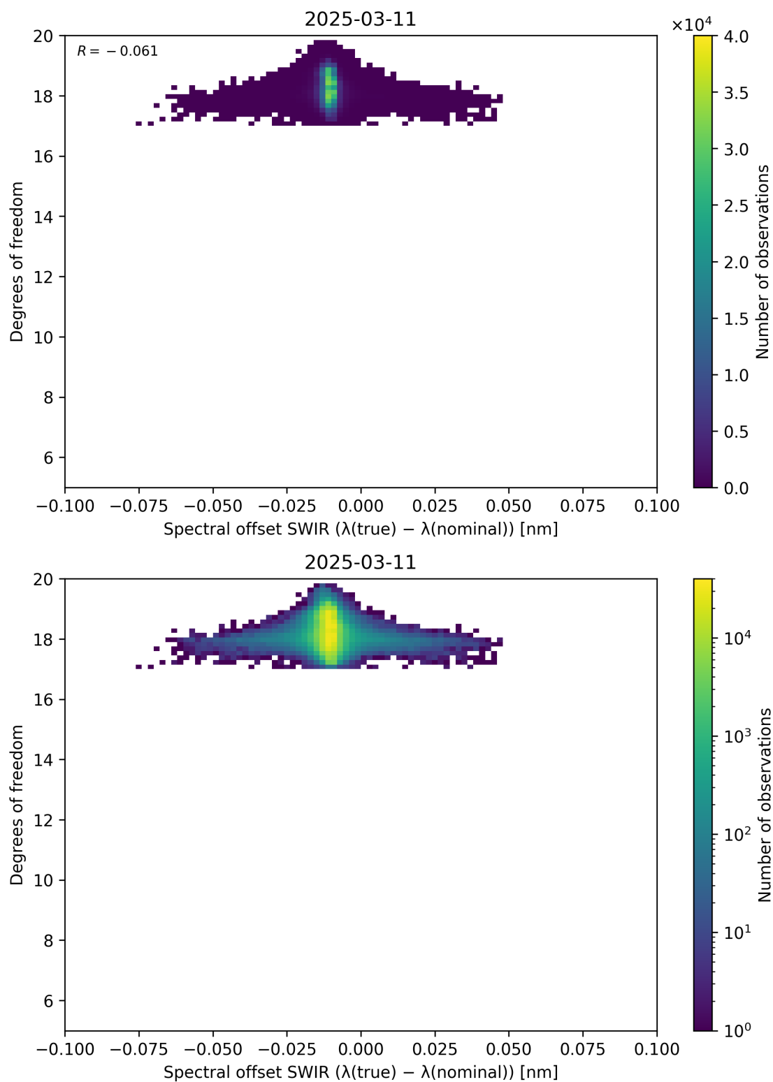
Figure 119: Scatter density plot of “Spectral offset SWIR ( \lambda_{\text{true}} - \lambda_{\text{nominal}} )” against “Degrees of freedom” for 2025-03-10 to 2025-03-12.
