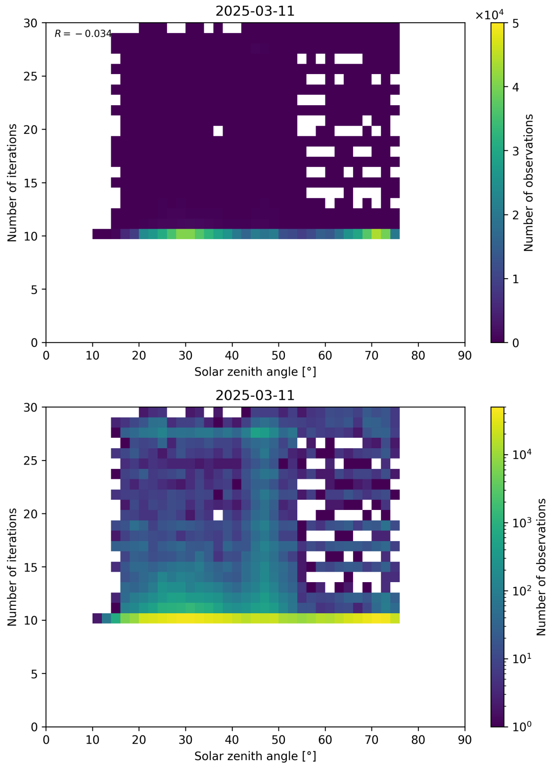
Figure 102: Scatter density plot of “Solar zenith angle” against “Number of iterations” for 2025-03-10 to 2025-03-12.
