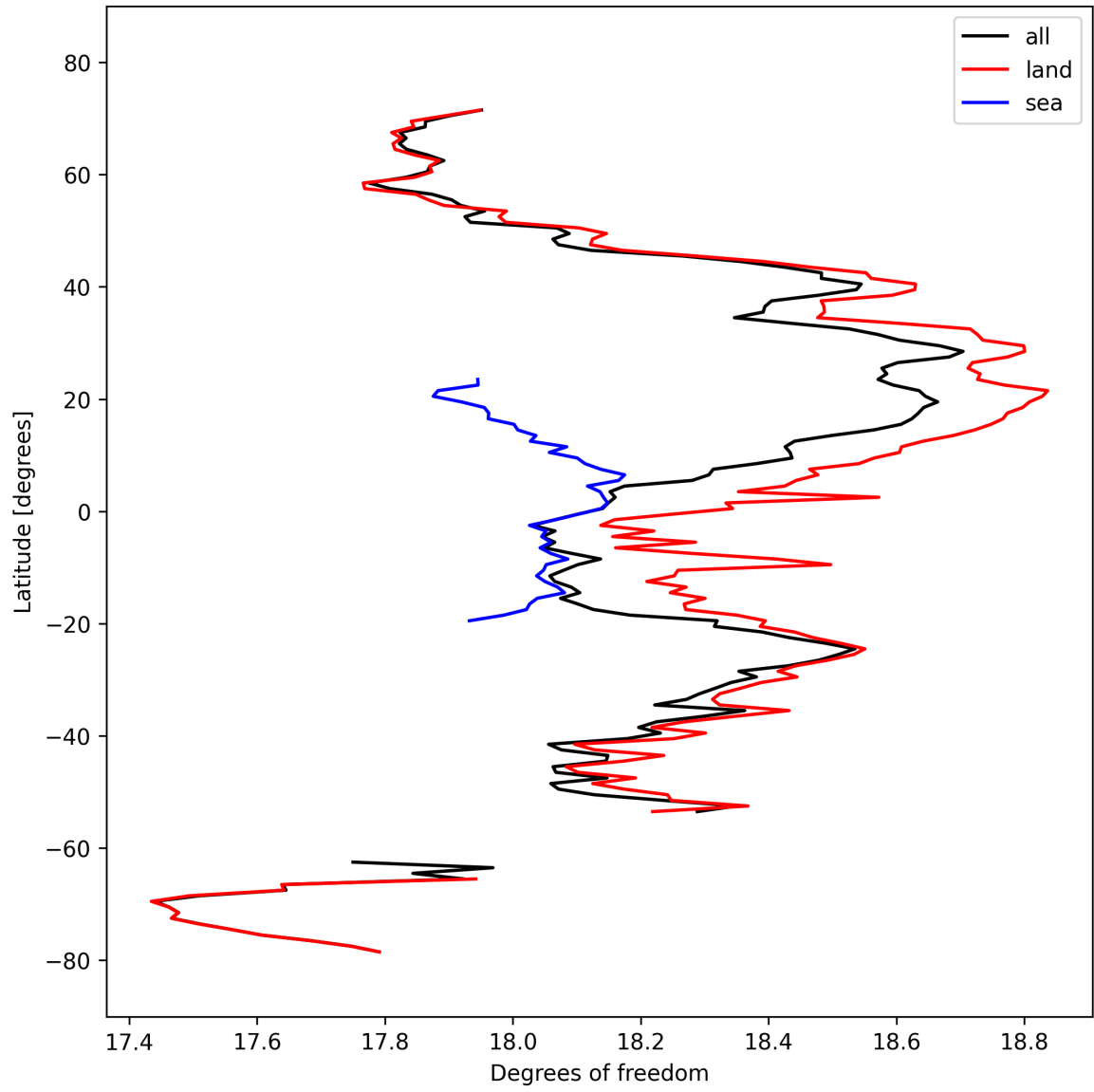
Figure 19: Zonal average of “Degrees of freedom” for 2025-03-10 to 2025-03-12.
