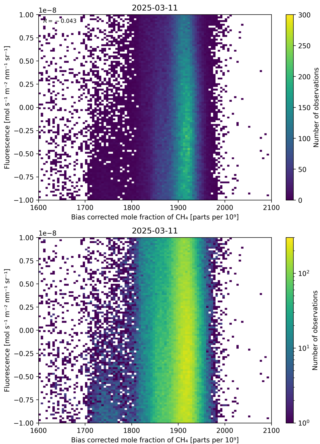
Figure 66: Scatter density plot of “Bias corrected mole fraction of \text{CH}_4 ” against “Fluorescence” for 2025-03-10 to 2025-03-12.
