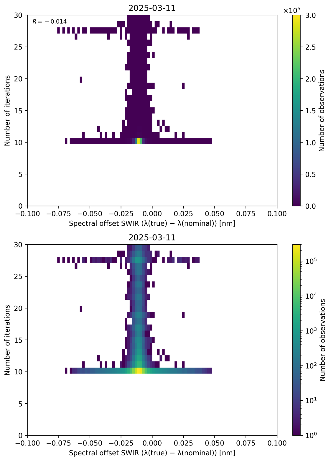
Figure 121: Scatter density plot of “Spectral offset SWIR ( \lambda_{\text{true}} - \lambda_{\text{nominal}} )” against “Number of iterations” for 2025-03-10 to 2025-03-12.
