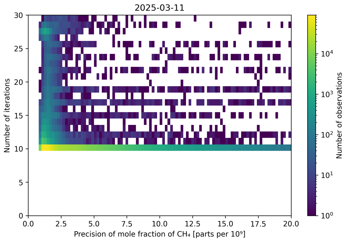
Figure 83: Scatter density plot of “Precision of mole fraction of CH 4 ” against “Number of iterations” for 2025-03-10 to 2025-03-12.
