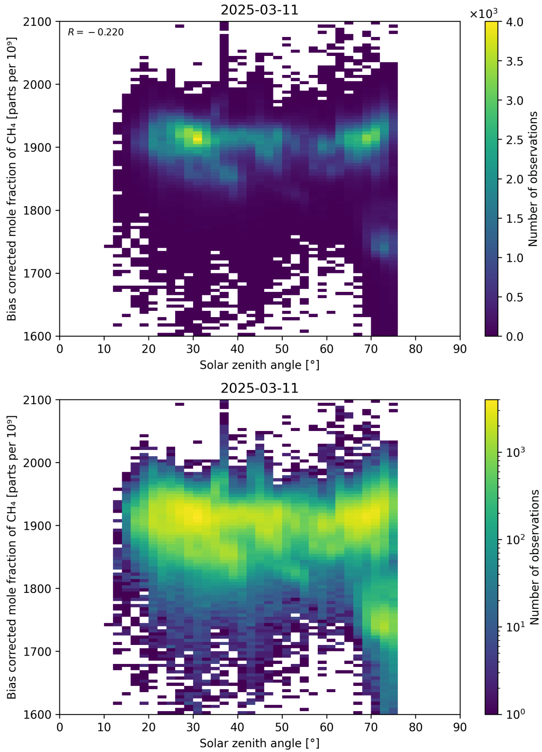
Figure 100: Scatter density plot of “Solar zenith angle” against “Bias corrected mole fraction of CH 4 ” for 2025-03-10 to 2025-03-12.
