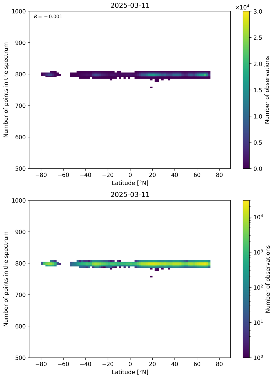
Figure 61: Scatter density plot of “Latitude” against “Number of points in the spectrum” for 2025-03-10 to 2025-03-12.
