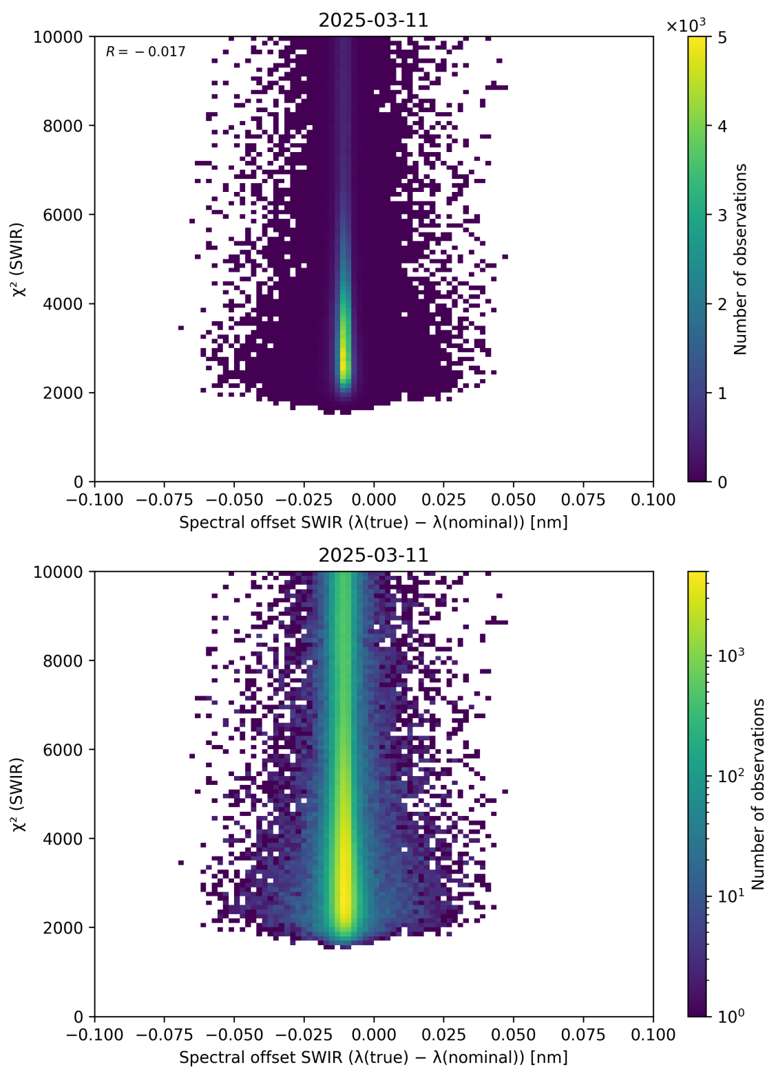
Figure 118: Scatter density plot of “Spectral offset SWIR ( \lambda_{\text{true}} - \lambda_{\text{nominal}} )” against “ \chi^2 (SWIR)” for 2025-03-10 to 2025-03-12.
