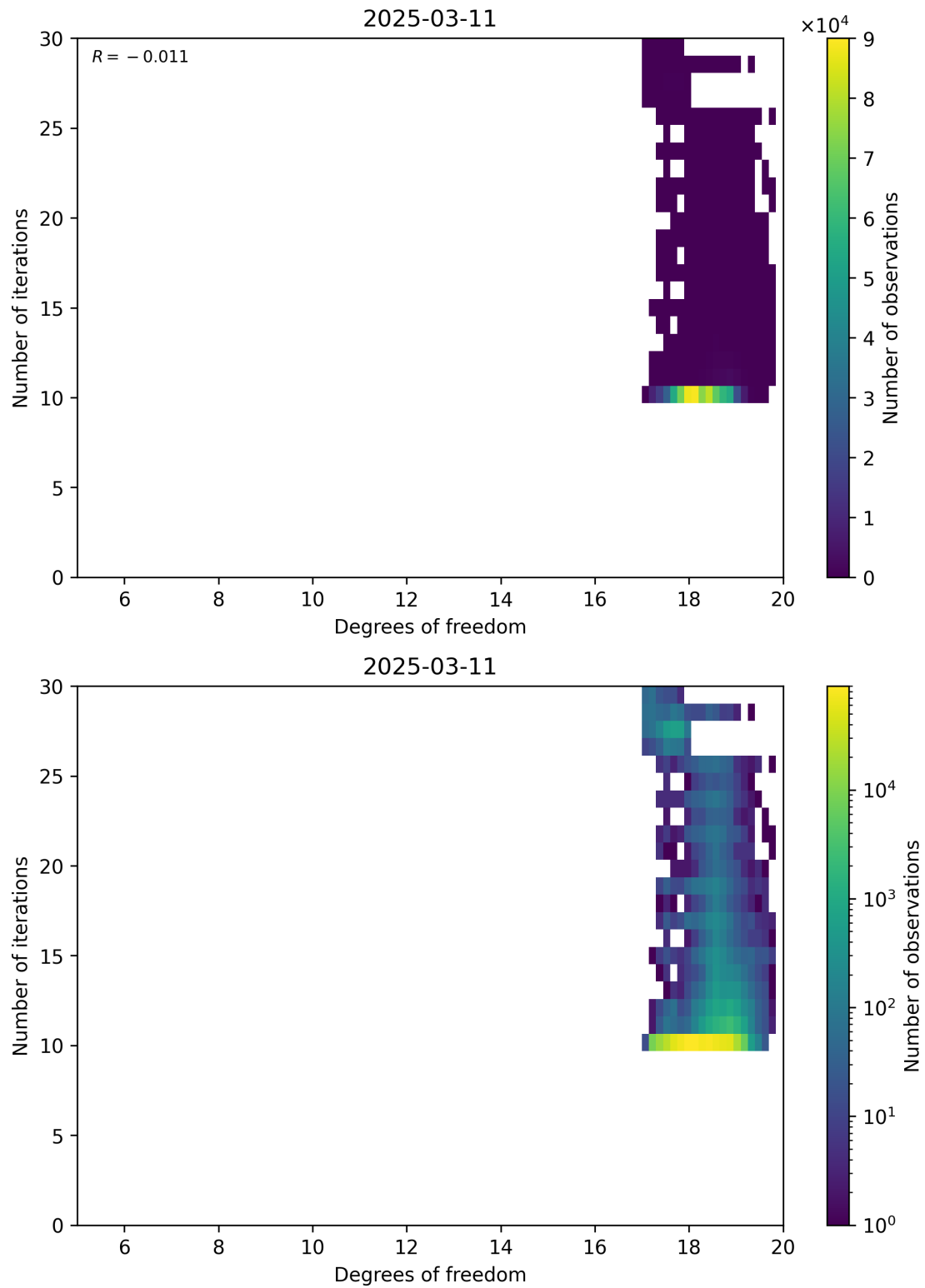
Figure 52: Scatter density plot of “Degrees of freedom” against “Number of iterations” for 2025-03-10 to 2025-03-12.
