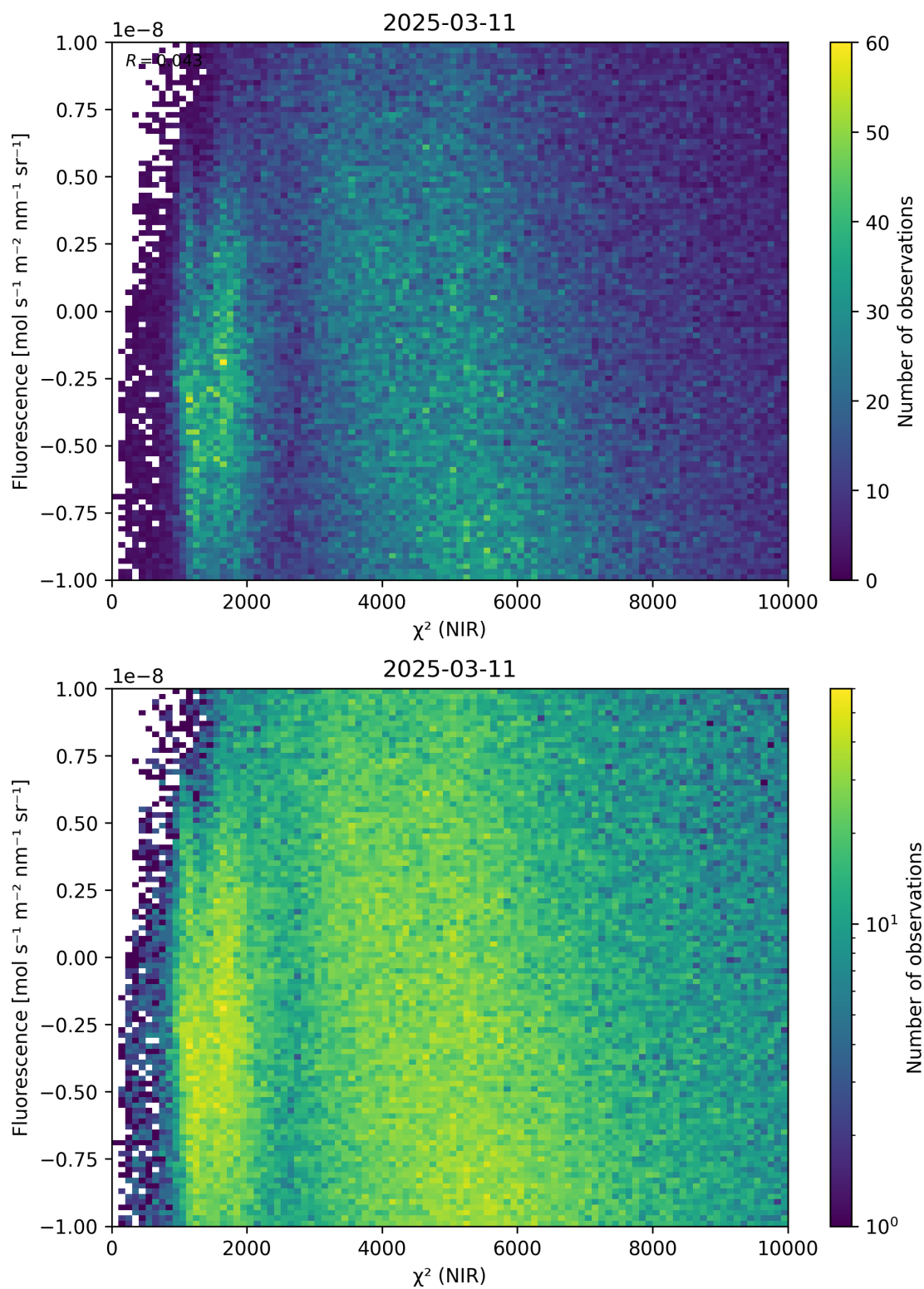
Figure 45: Scatter density plot of “ \chi^2 (NIR)” against “Fluorescence” for 2025-03-10 to 2025-03-12.
