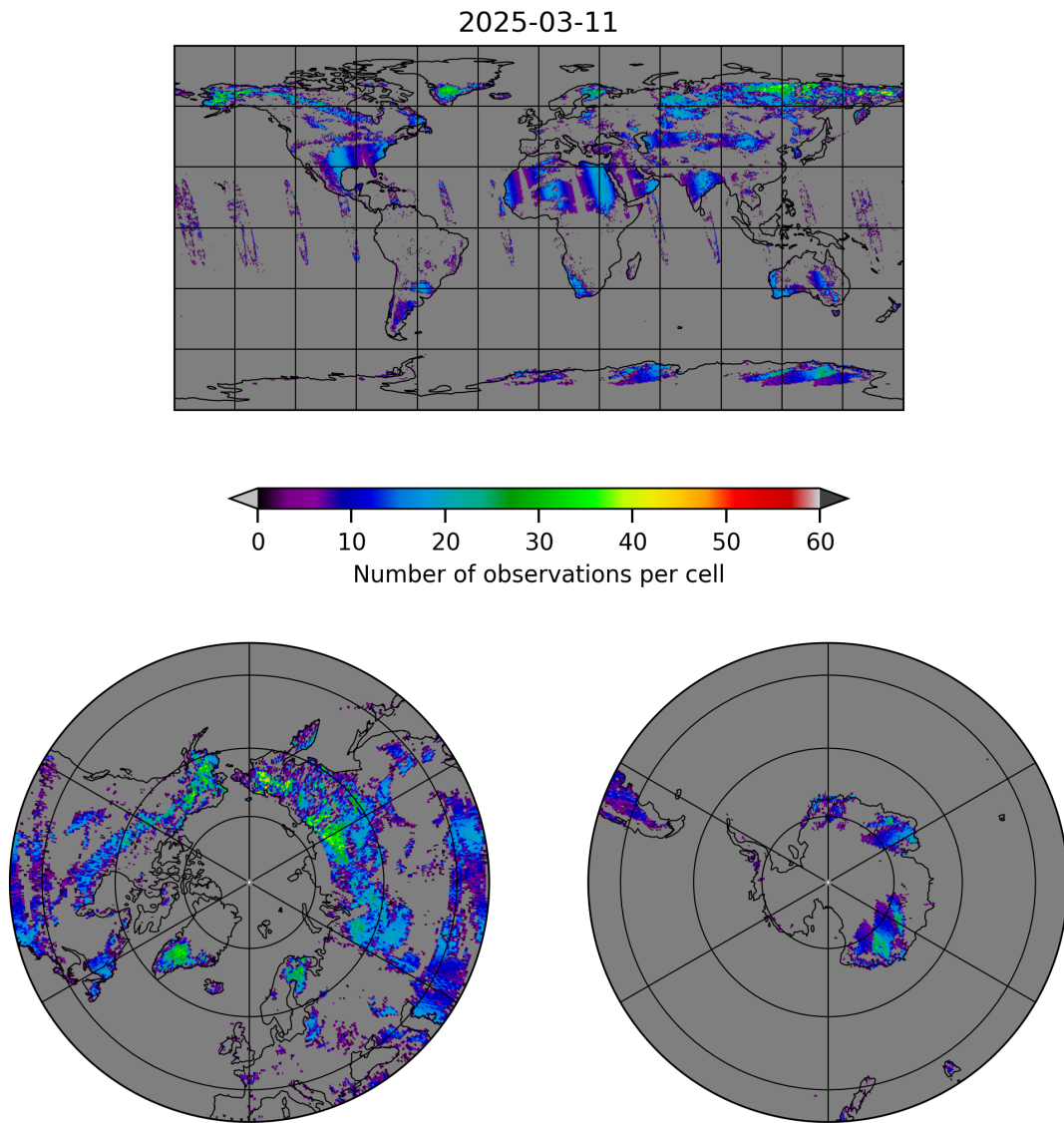
Figure 10: Map of the number of observations for 2025-03-10 to 2025-03-12
