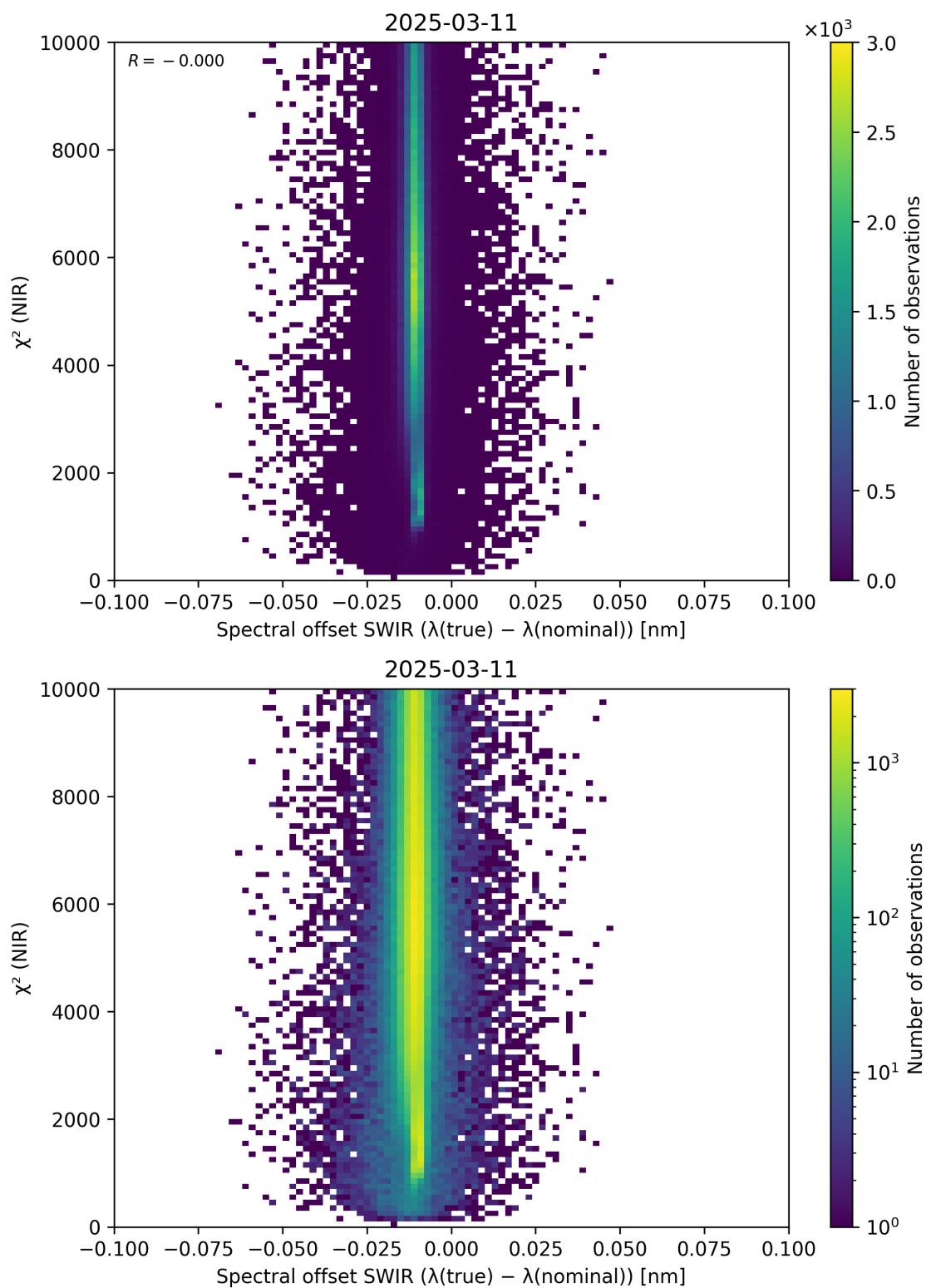
Figure 117: Scatter density plot of “Spectral offset SWIR ( \lambda_{\text{true}} - \lambda_{\text{nominal}} )” against “ \chi^2 (NIR)” for 2025-03-10 to 2025-03-12.
