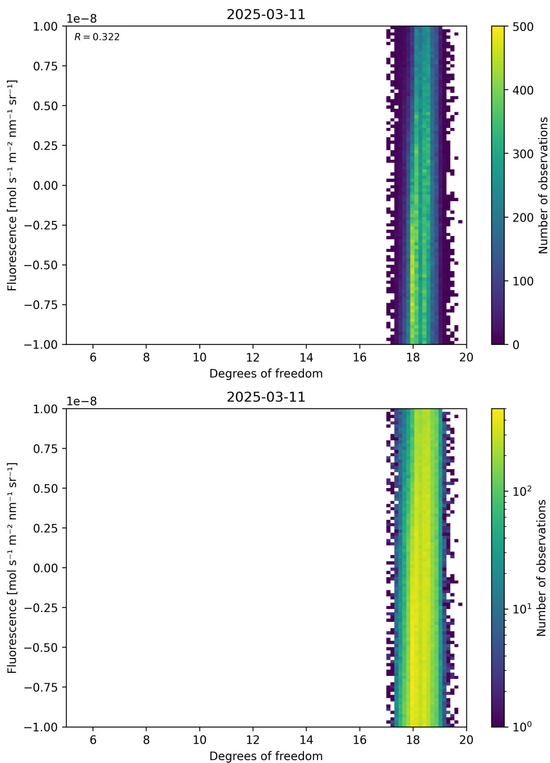
Figure 51: Scatter density plot of “Degrees of freedom” against “Fluorescence” for 2025-03-10 to 2025-03-12.
