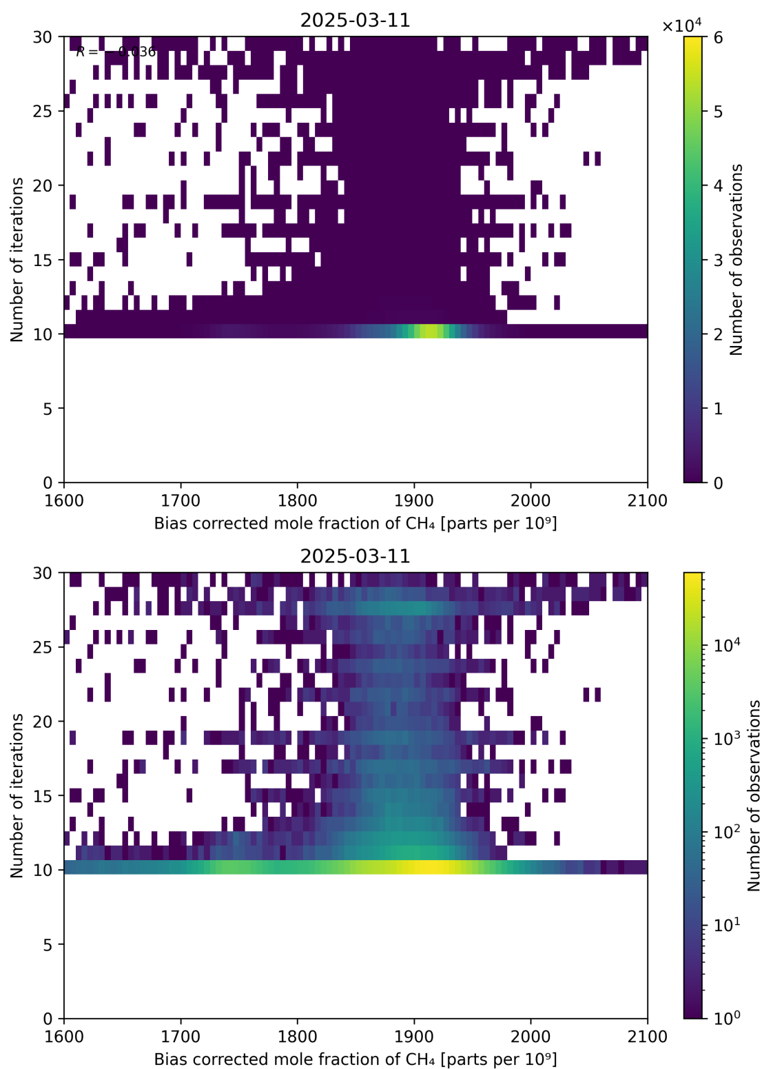
Figure 67: Scatter density plot of “Bias corrected mole fraction of CH 4 ” against “Number of iterations” for 2025-03-10 to 2025-03-12.
