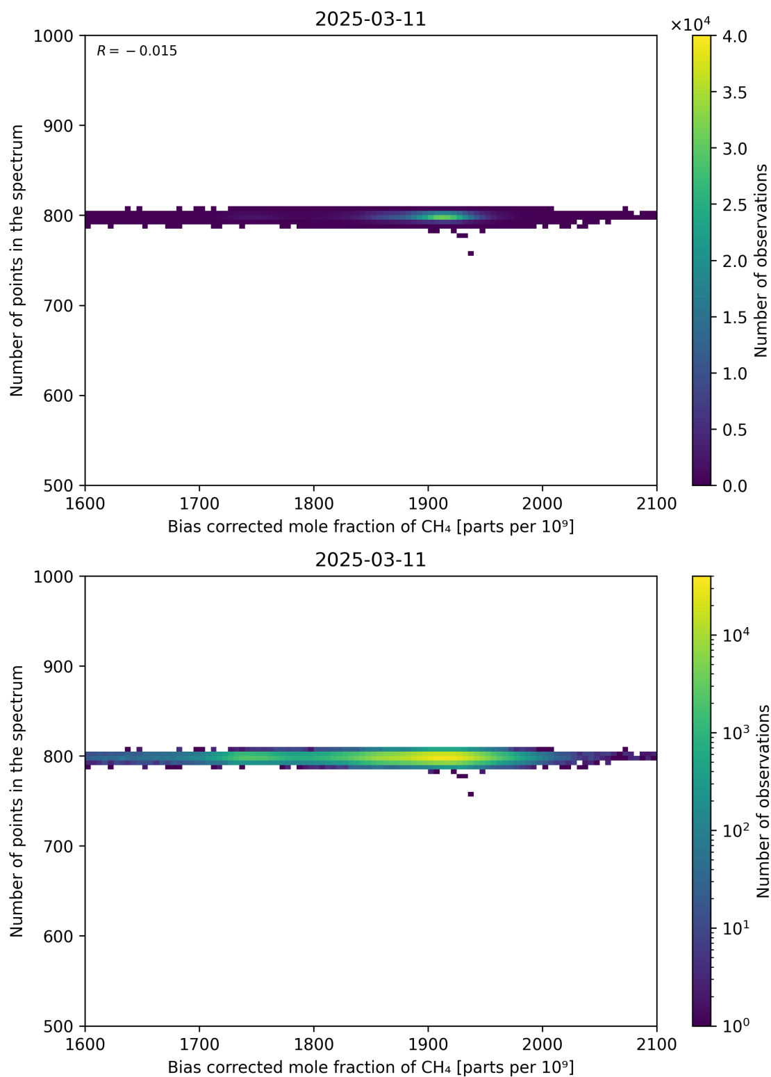
Figure 68: Scatter density plot of “Bias corrected mole fraction of CH 4 ” against “Number of points in the spectrum” for 2025-03-10 to 2025-03-12.
