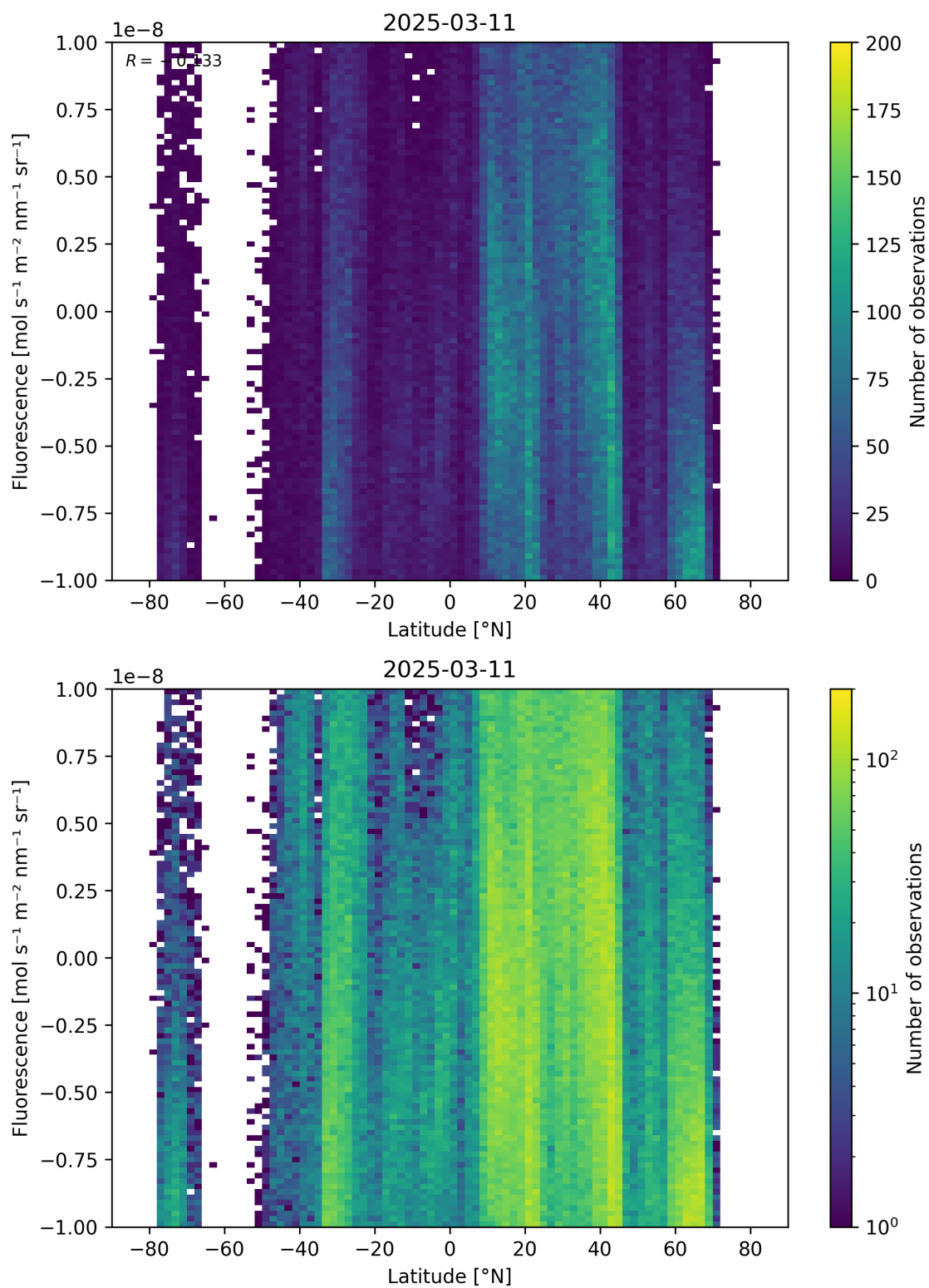
Figure 56: Scatter density plot of “Latitude” against “Fluorescence” for 2025-03-10 to 2025-03-12.
