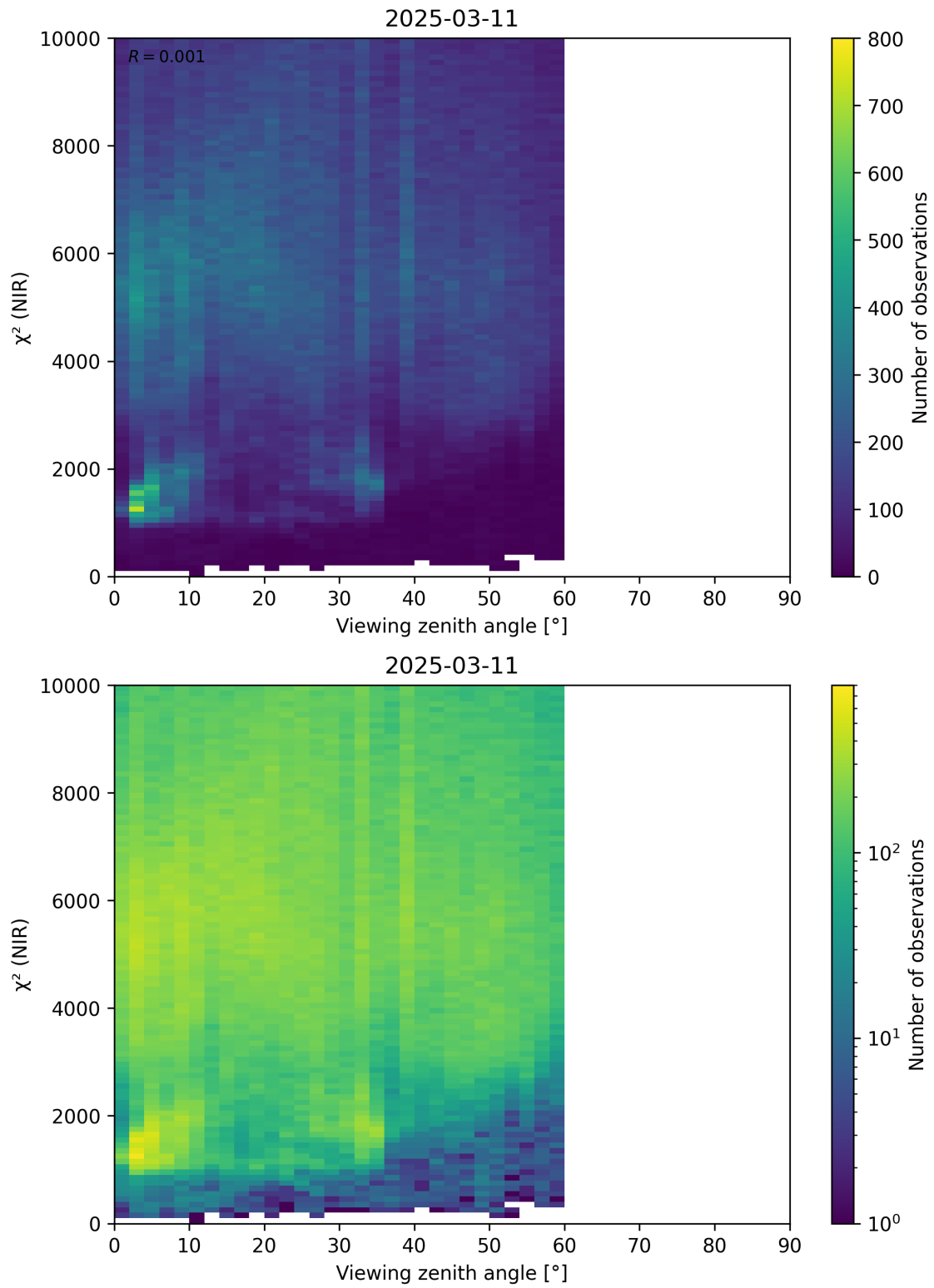
Figure 105: Scatter density plot of “Viewing zenith angle” against “ \chi^2 (NIR)” for 2025-03-10 to 2025-03-12.
