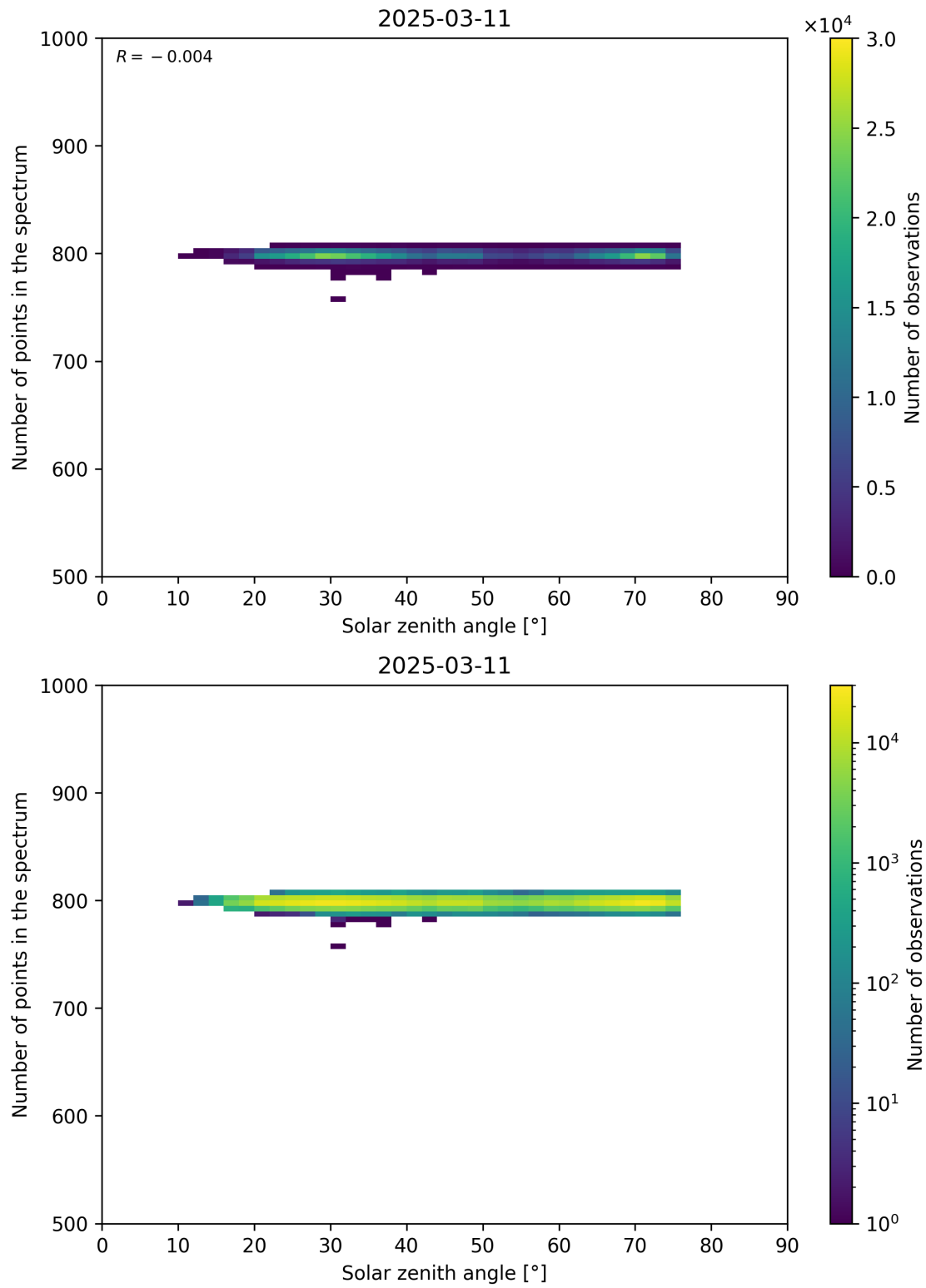
Figure 103: Scatter density plot of “Solar zenith angle” against “Number of points in the spectrum” for 2025-03-10 to 2025-03-12.
