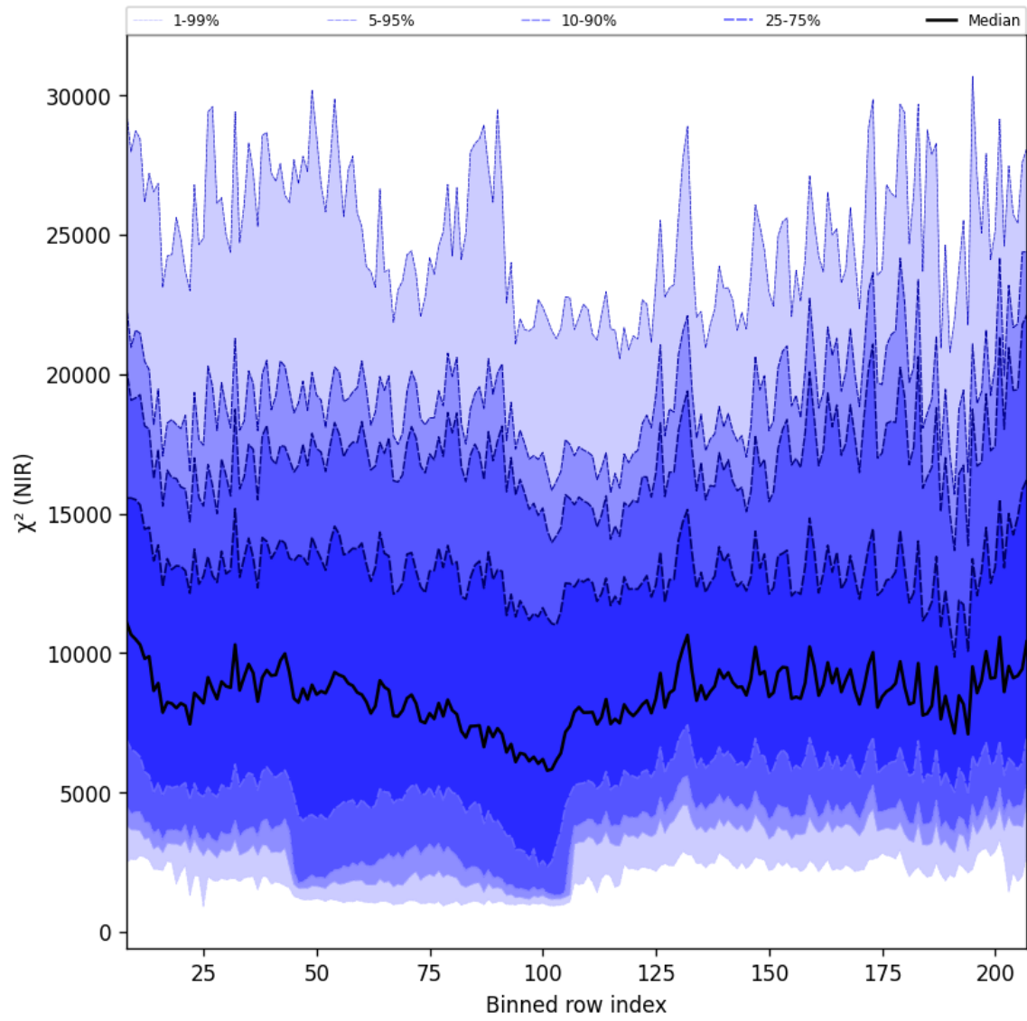
Figure 40: Along track statistics of “ \chi^2 (NIR)” for 2025-03-10 to 2025-03-12
