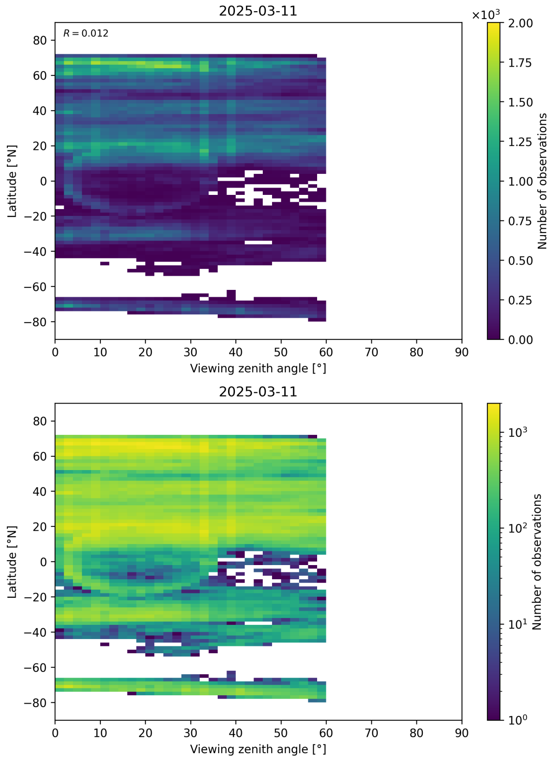
Figure 109: Scatter density plot of “Viewing zenith angle” against “Latitude” for 2025-03-10 to 2025-03-12.
