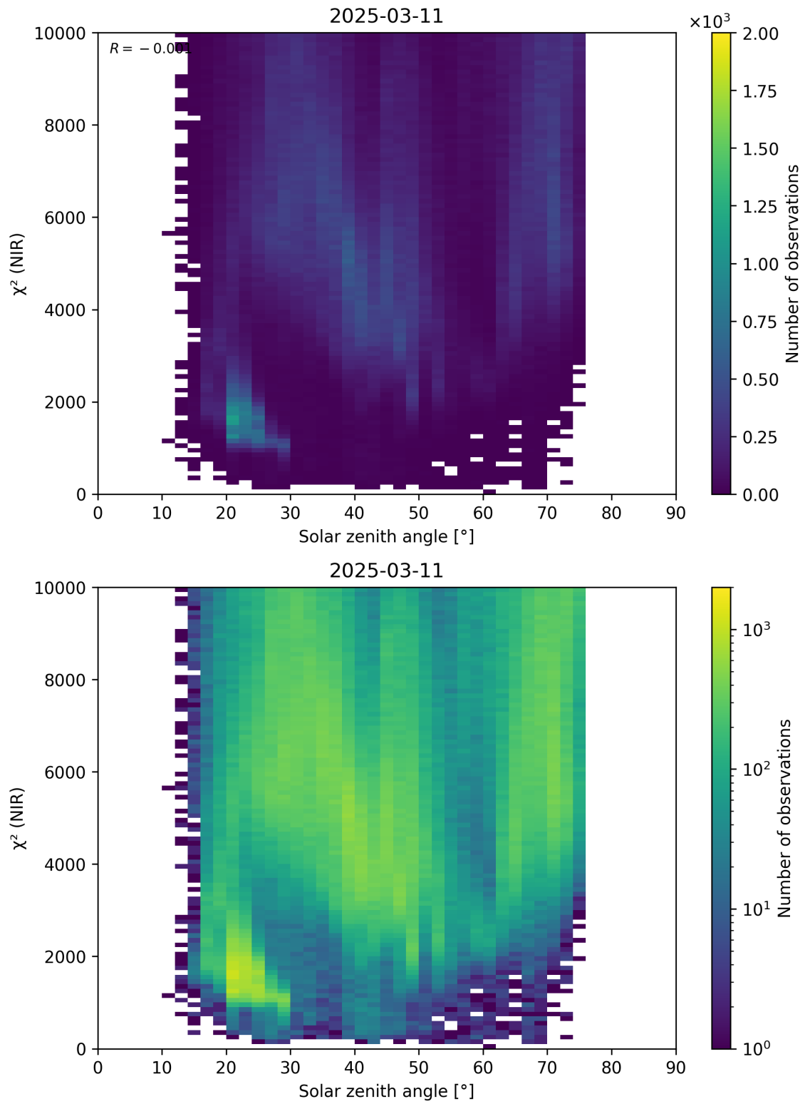
Figure 94: Scatter density plot of “Solar zenith angle” against “ \chi^2 (NIR)” for 2025-03-10 to 2025-03-12.
