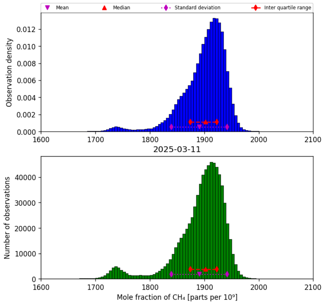
Figure 23: Histogram of “Mole fraction of CH 4 ” for 2025-03-10 to 2025-03-12
