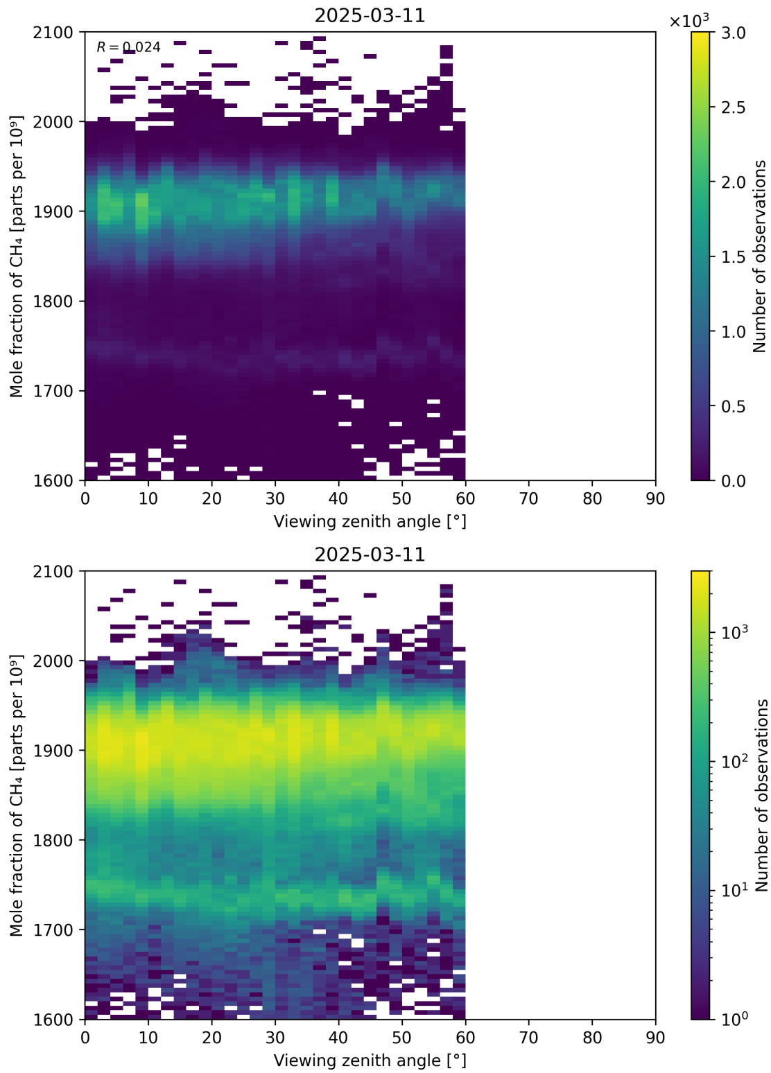
Figure 110: Scatter density plot of “Viewing zenith angle” against “Mole fraction of CH 4 ” for 2025-03-10 to 2025-03-12.
