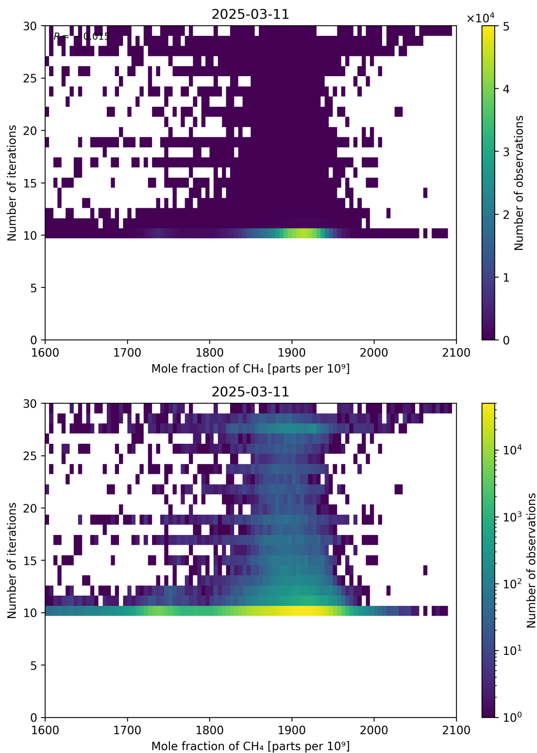
Figure 76: Scatter density plot of “Mole fraction of CH 4 ” against “Number of iterations” for 2025-03-10 to 2025-03-12.
