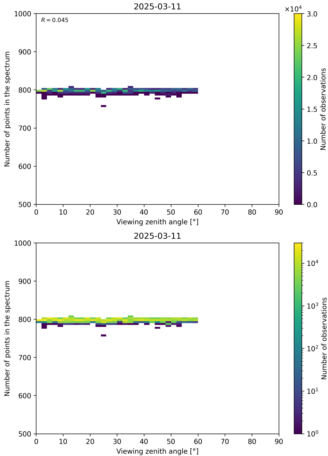
Figure 114: Scatter density plot of “Viewing zenith angle” against “Number of points in the spectrum” for 2025-03-10 to 2025-03-12.
