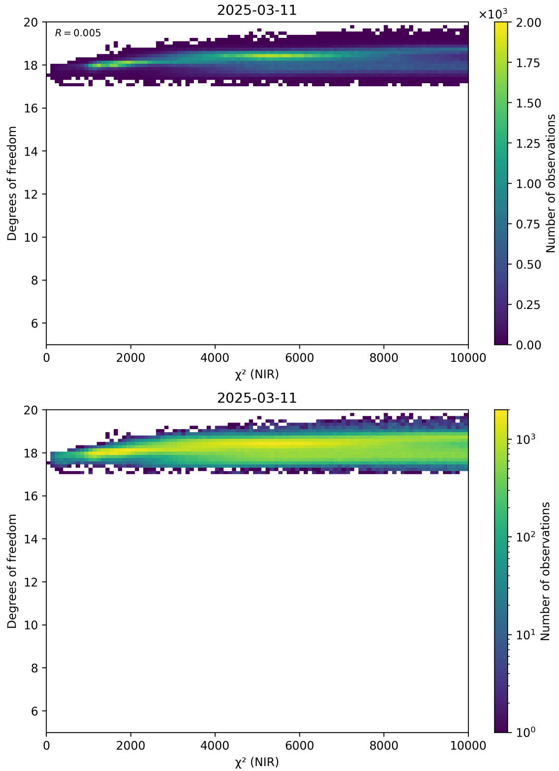
Figure 44: Scatter density plot of “ \chi^2 (NIR)” against “Degrees of freedom” for 2025-03-10 to 2025-03-12.
