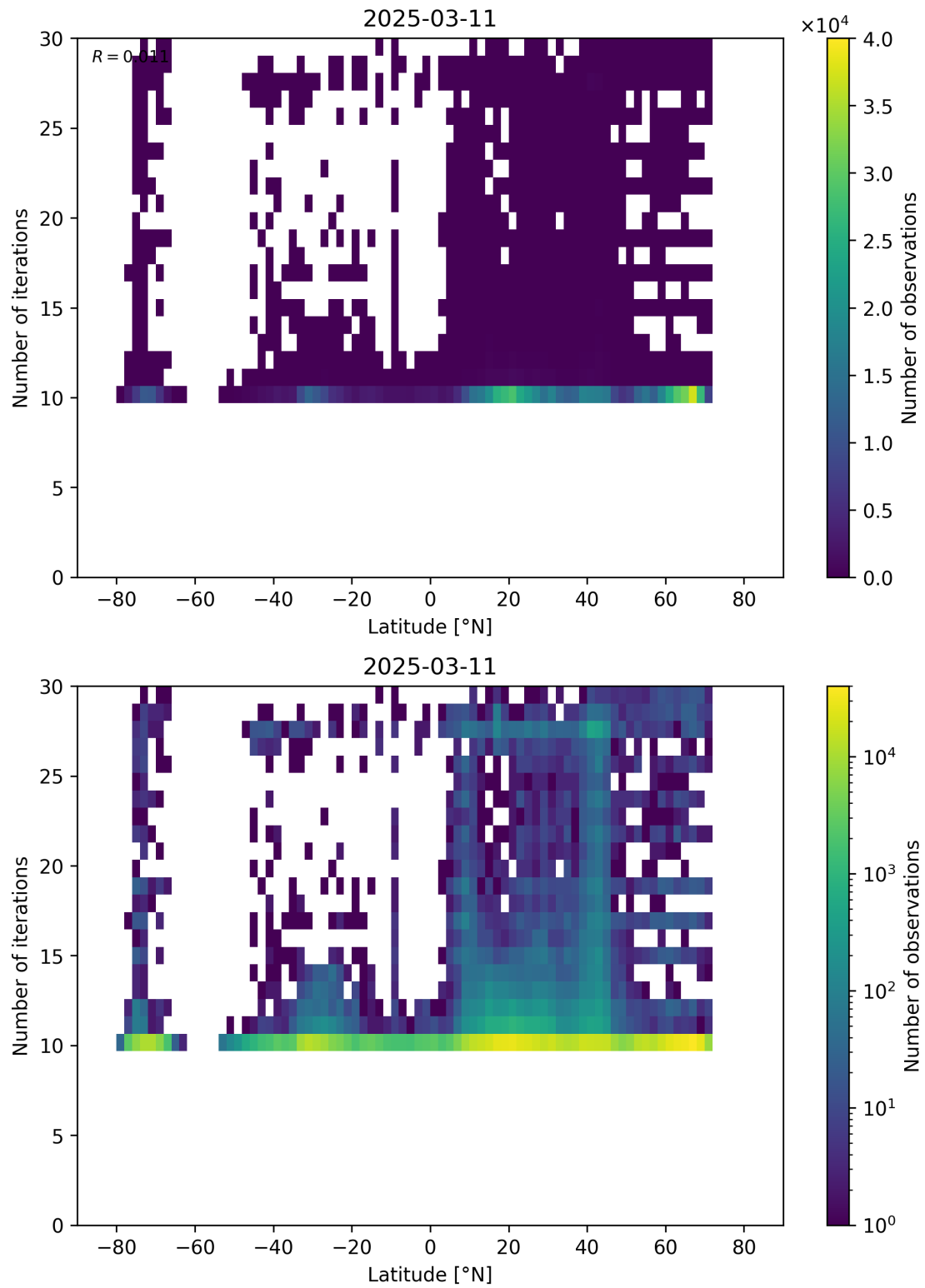
Figure 60: Scatter density plot of “Latitude” against “Number of iterations” for 2025-03-10 to 2025-03-12.
