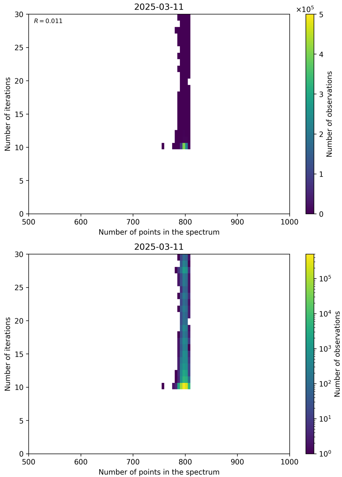
Figure 92: Scatter density plot of “Number of points in the spectrum” against “Number of iterations” for 2025-03-10 to 2025-03-12.
