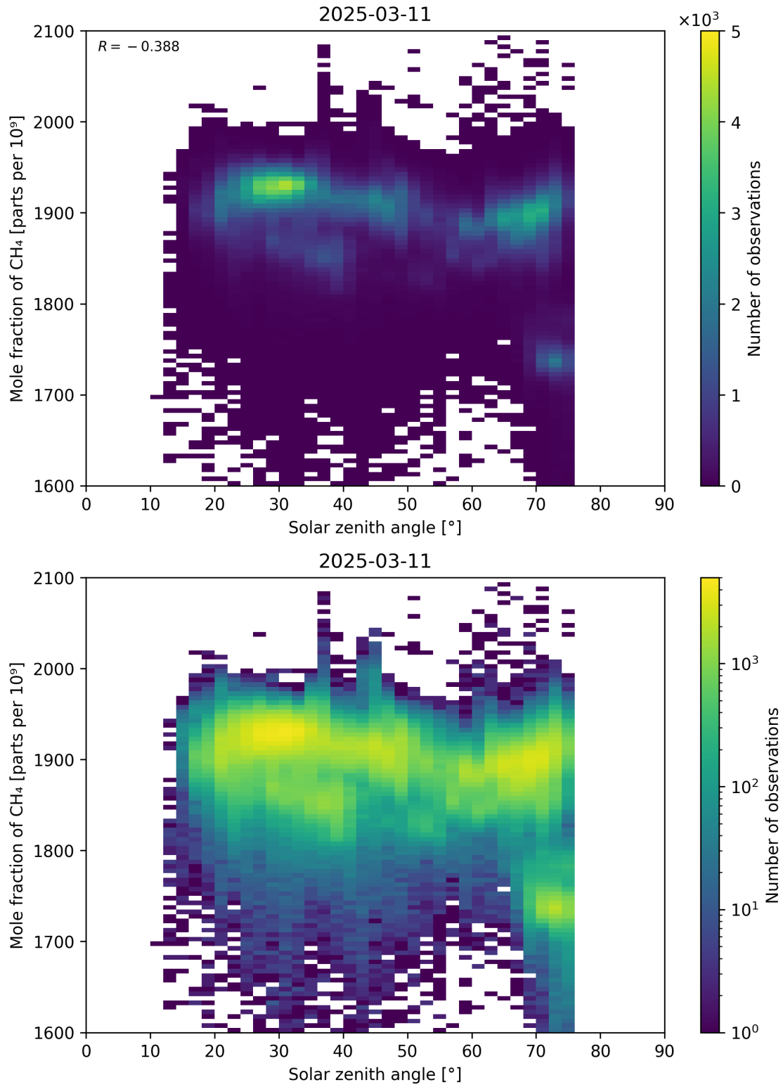
Figure 99: Scatter density plot of “Solar zenith angle” against “Mole fraction of CH 4 ” for 2025-03-10 to 2025-03-12.
