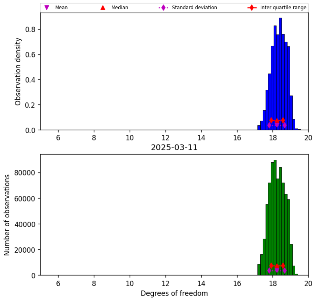
Figure 30: Histogram of “Degrees of freedom” for 2025-03-10 to 2025-03-12
