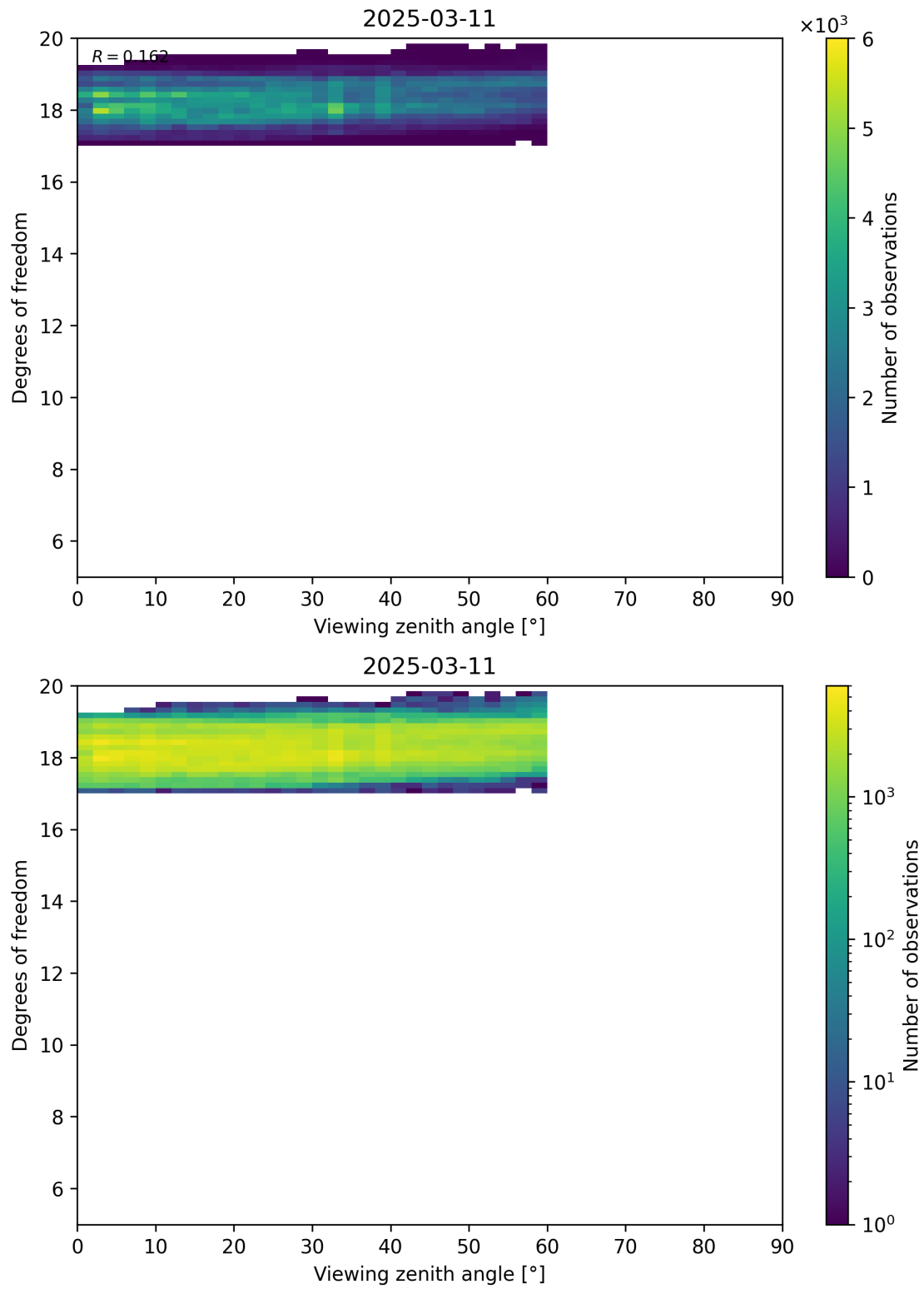
Figure 107: Scatter density plot of “Viewing zenith angle” against “Degrees of freedom” for 2025-03-10 to 2025-03-12.
