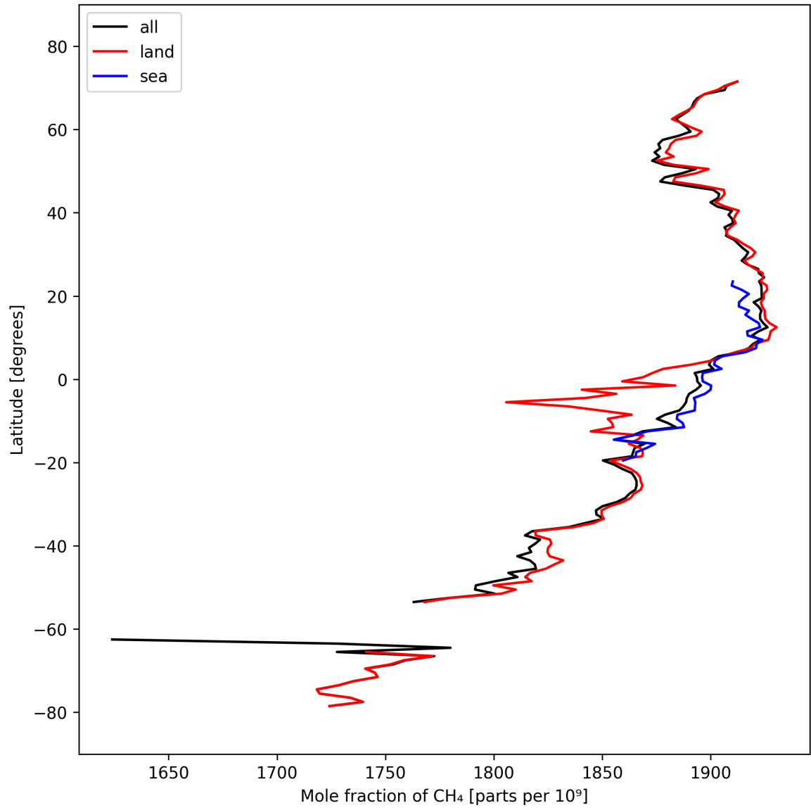
Figure 12: Zonal average of “Mole fraction of \text{CH}_4 ” for 2025-03-10 to 2025-03-12.
