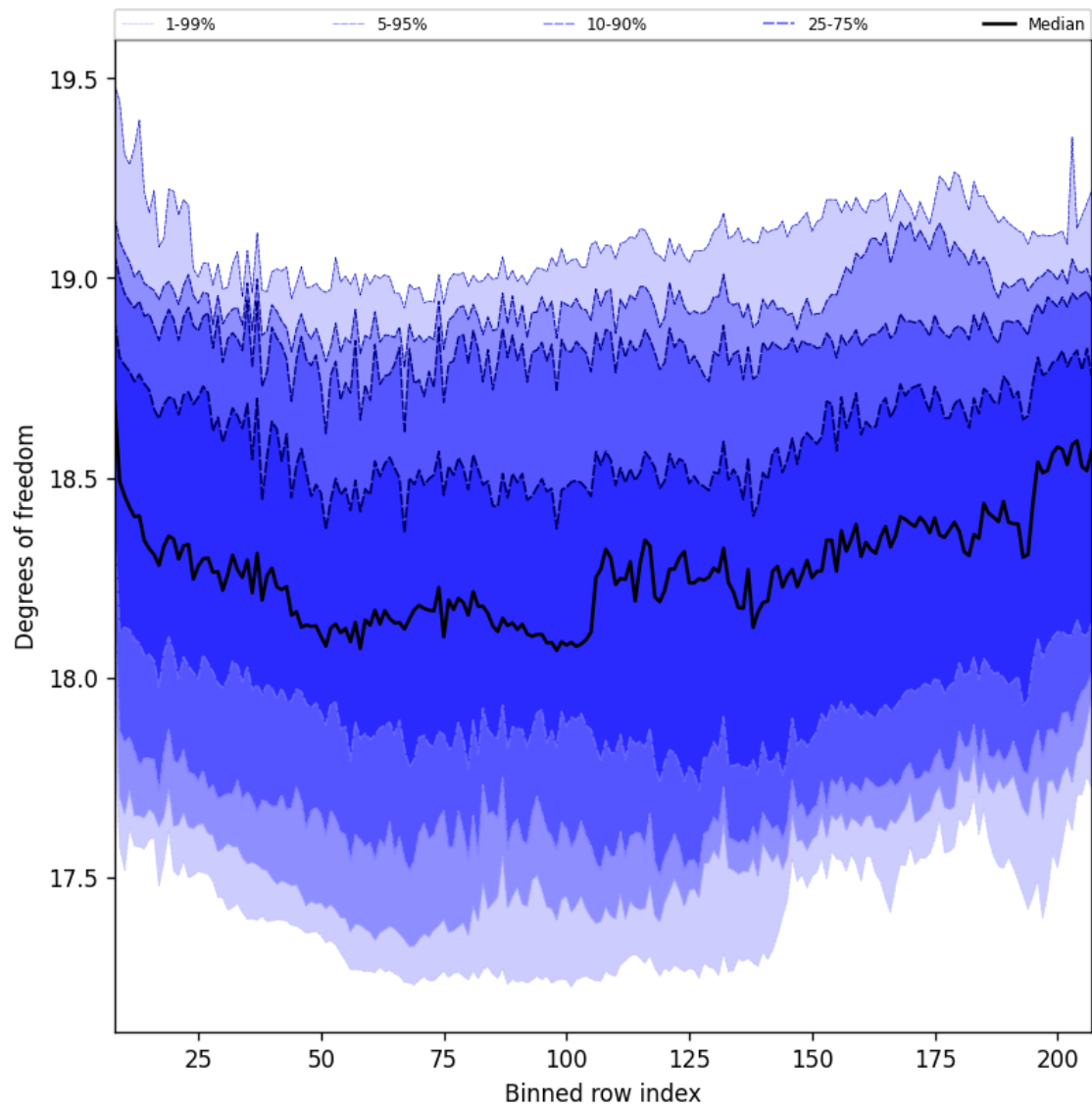
Figure 41: Along track statistics of “Degrees of freedom” for 2025-03-10 to 2025-03-12
