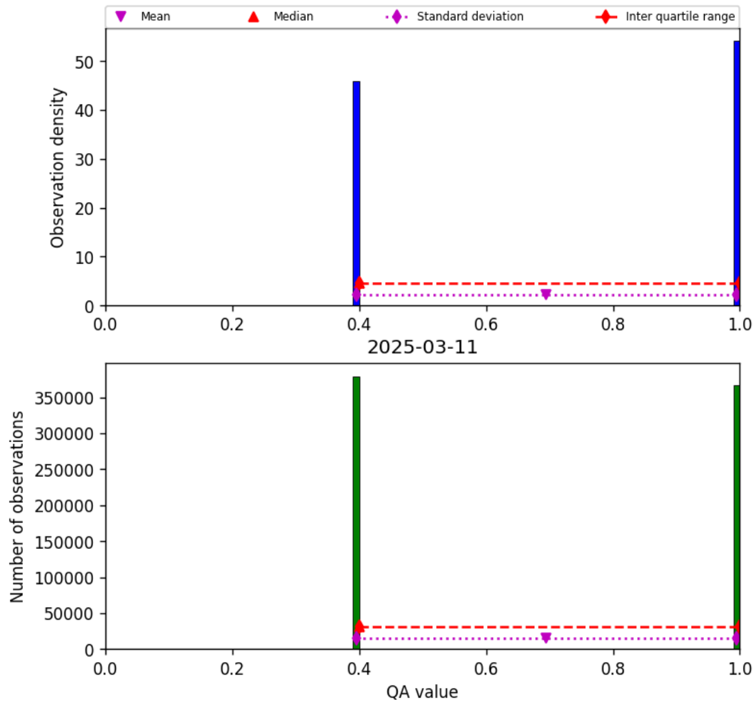
Figure 22: Histogram of “QA value” for 2025-03-10 to 2025-03-12
