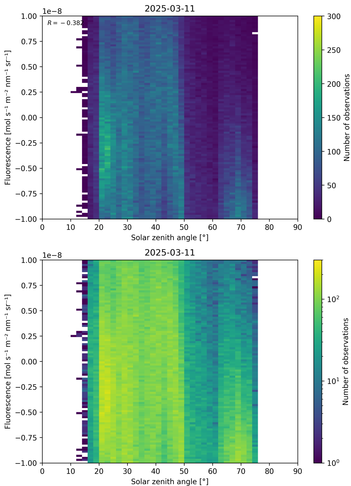
Figure 97: Scatter density plot of “Solar zenith angle” against “Fluorescence” for 2025-03-10 to 2025-03-12.
