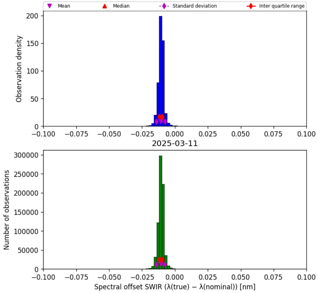
Figure 27: Histogram of “Spectral offset SWIR ( \lambda_{\text{true}} - \lambda_{\text{nominal}} )” for 2025-03-10 to 2025-03-12
