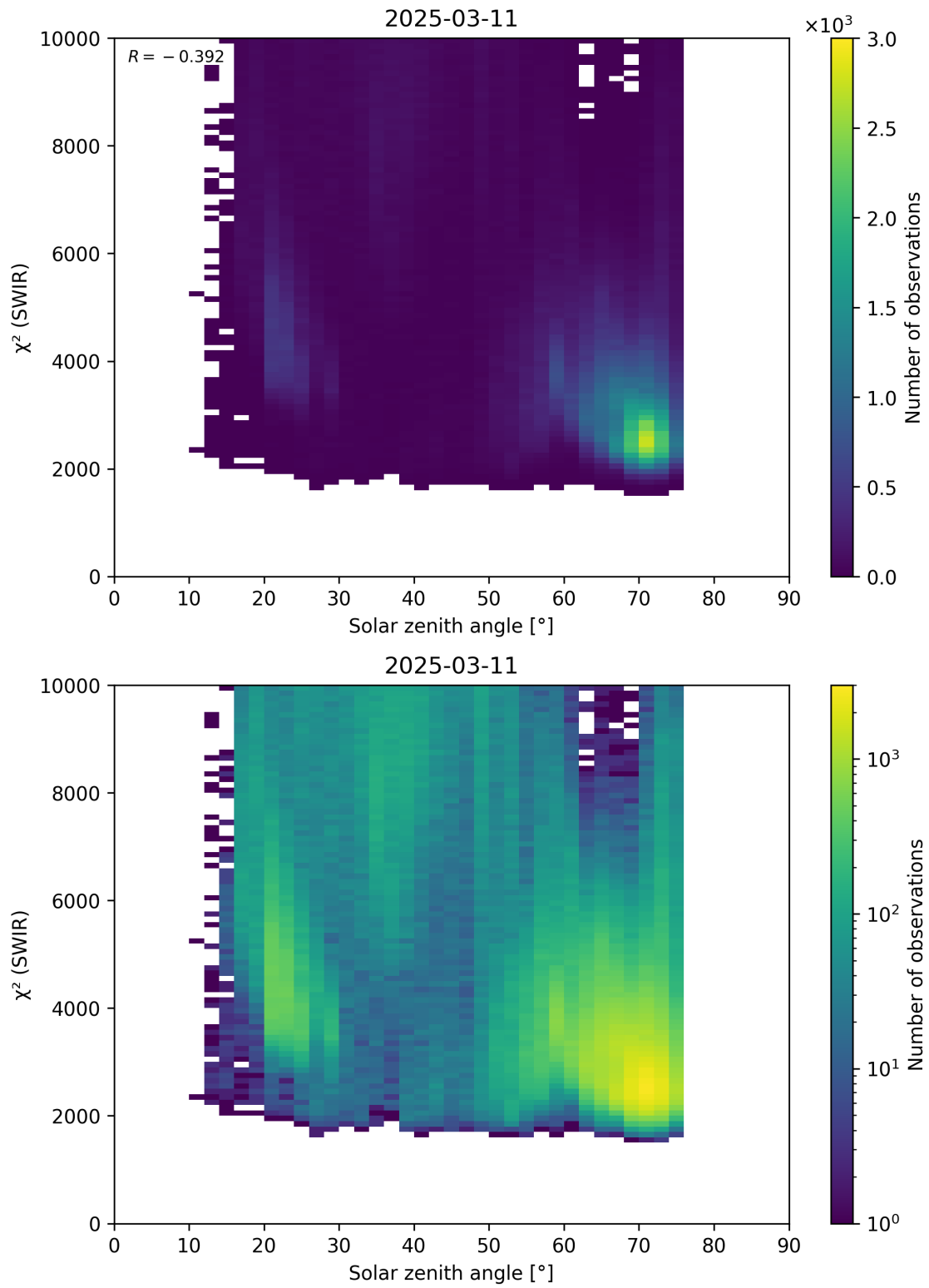
Figure 95: Scatter density plot of “Solar zenith angle” against “ \chi^2 (SWIR)” for 2025-03-10 to 2025-03-12.
