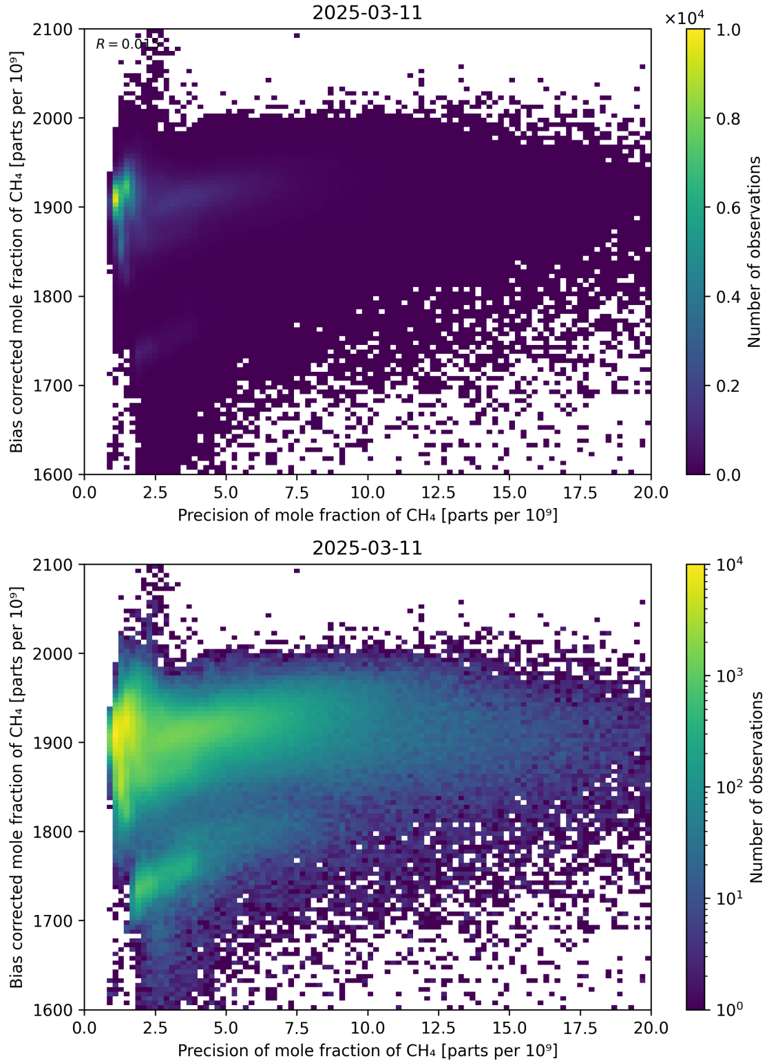
Figure 82: Scatter density plot of “Precision of mole fraction of \text{CH}_4 ” against “Bias corrected mole fraction of \text{CH}_4 ” for 2025-03-10 to 2025-03-12.
