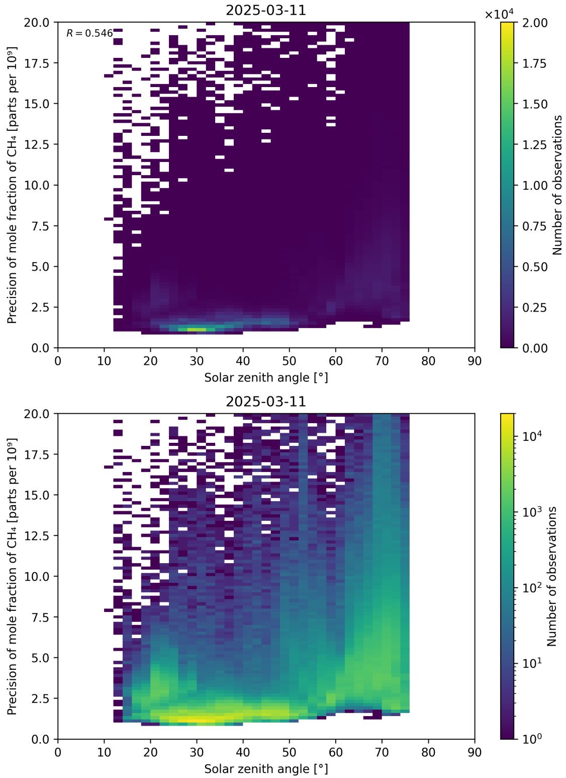
Figure 101: Scatter density plot of “Solar zenith angle” against “Precision of mole fraction of \text{CH}_4 ” for 2025-03-10 to 2025-03-12.
