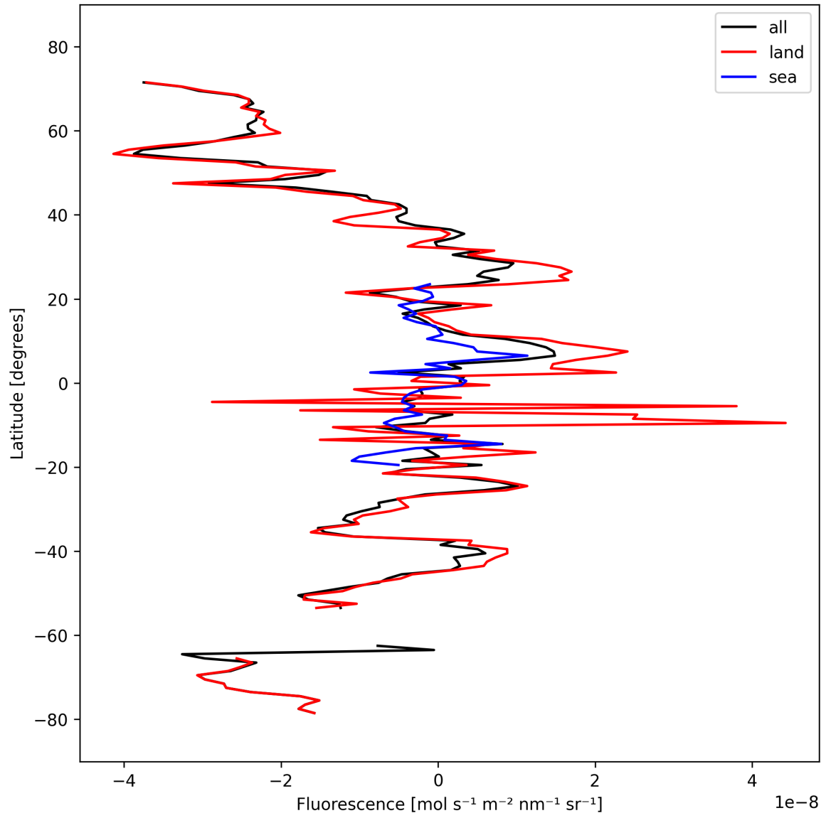
Figure 21: Zonal average of “Fluorescence” for 2025-03-10 to 2025-03-12.
