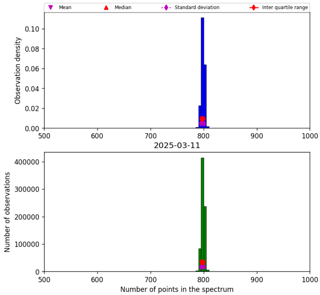
Figure 26: Histogram of “Number of points in the spectrum” for 2025-03-10 to 2025-03-12
