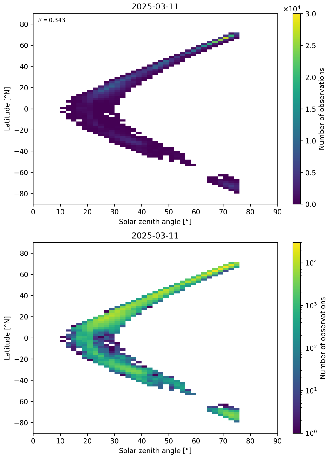
Figure 98: Scatter density plot of “Solar zenith angle” against “Latitude” for 2025-03-10 to 2025-03-12.
