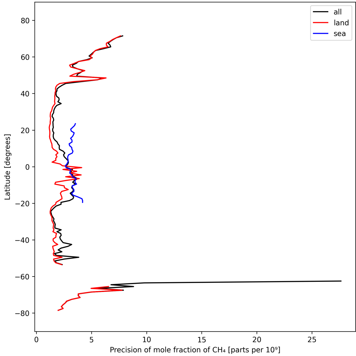
Figure 13: Zonal average of “Precision of mole fraction of CH 4 ” for 2025-03-10 to 2025-03-12.
