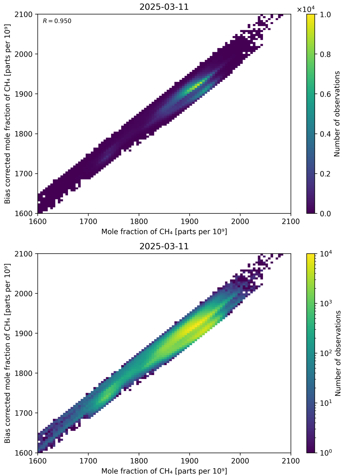
Figure 74: Scatter density plot of “Mole fraction of CH 4 ” against “Bias corrected mole fraction of CH 4 ” for 2025-03-10 to 2025-03-12.
