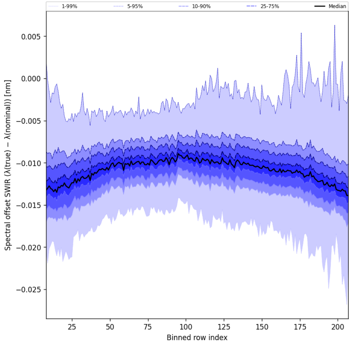
Figure 38: Along track statistics of “Spectral offset SWIR ( \lambda_{\text{true}} - \lambda_{\text{nominal}} )” for 2025-03-10 to 2025-03-12
