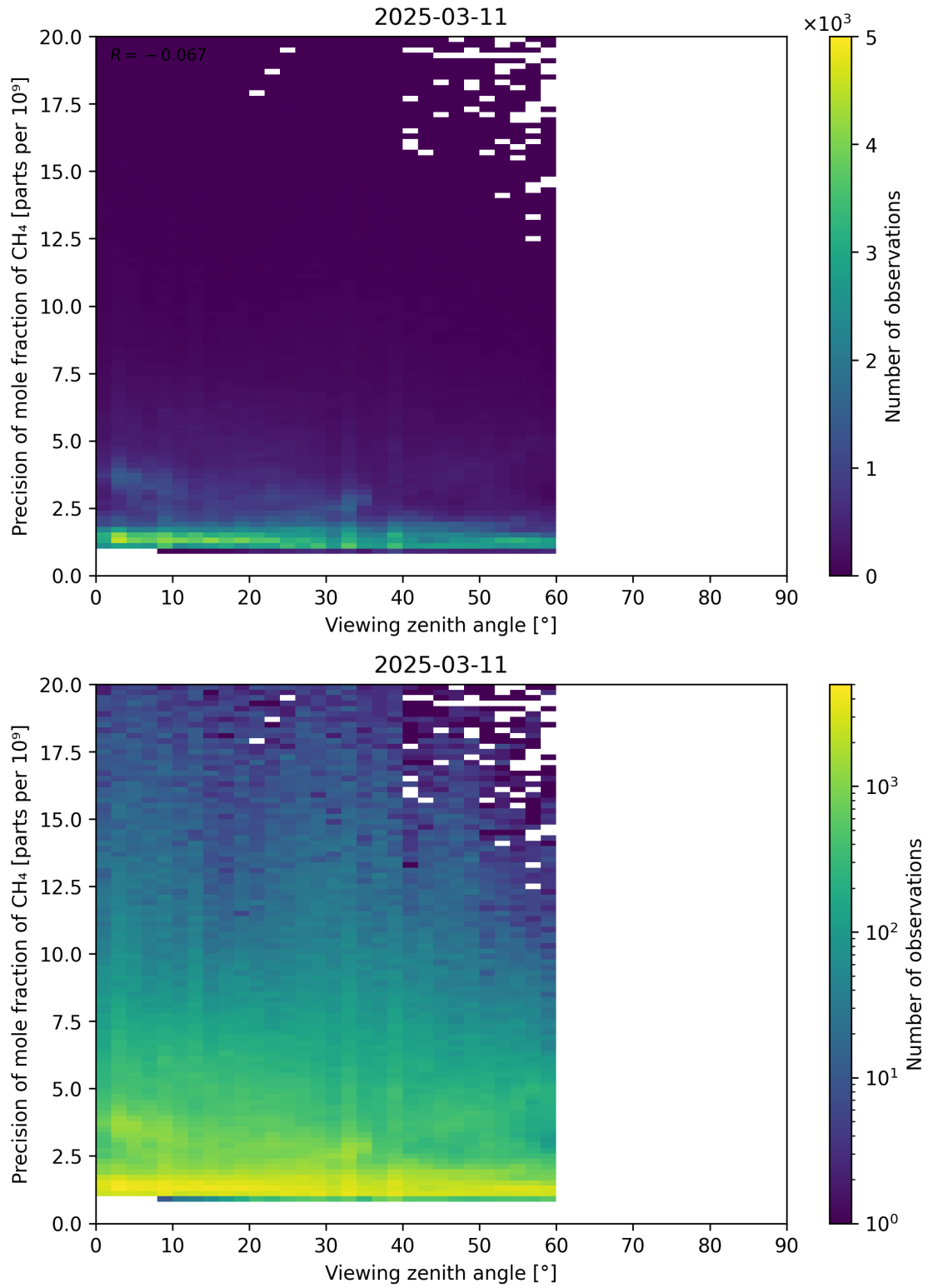
Figure 112: Scatter density plot of “Viewing zenith angle” against “Precision of mole fraction of CH 4 ” for 2025-03-10 to 2025-03-12.
