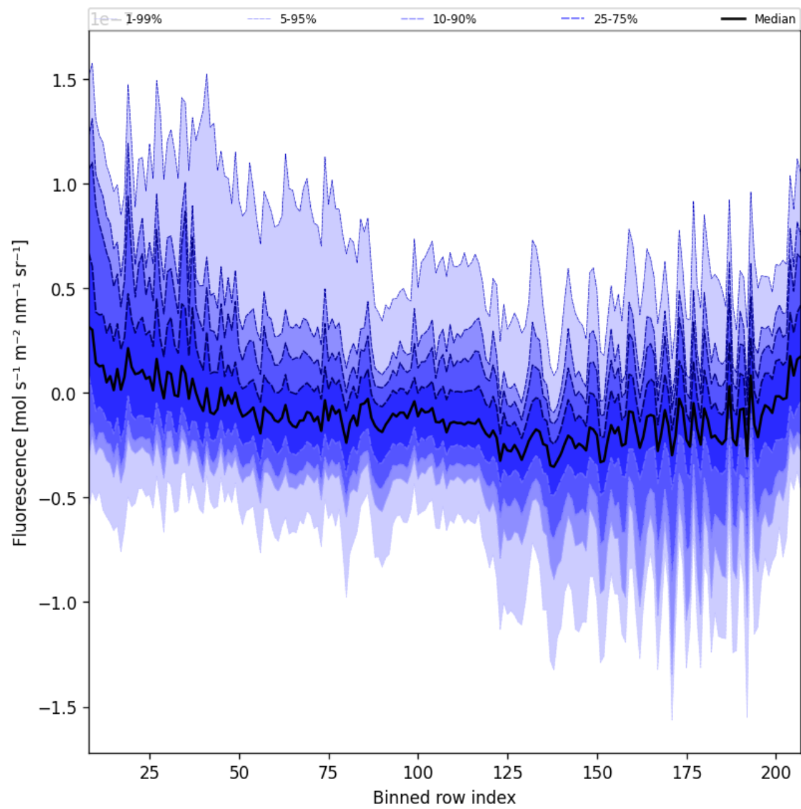
Figure 43: Along track statistics of "Fluorescence" for 2025-03-10 to 2025-03-12
