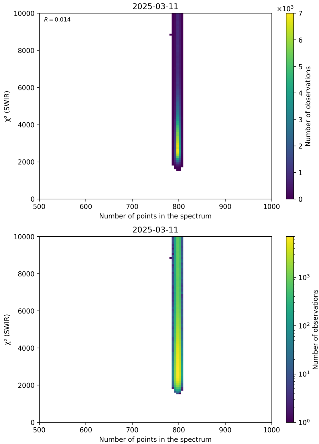
Figure 89: Scatter density plot of “Number of points in the spectrum” against “ \chi^2 (SWIR)” for 2025-03-10 to 2025-03-12.
