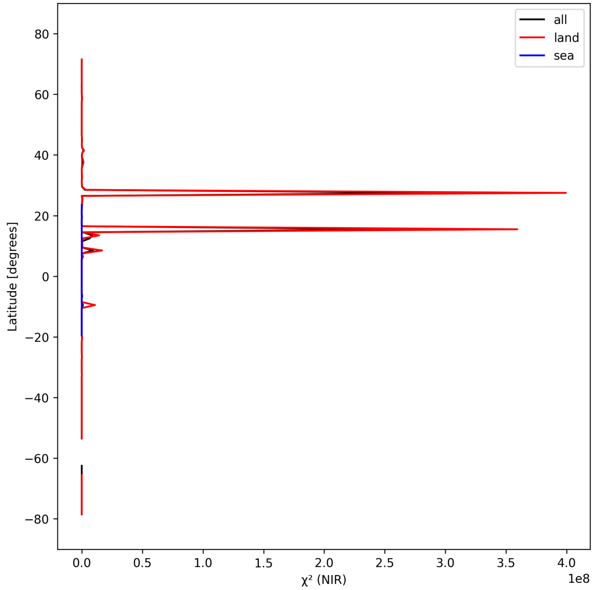
Figure 18: Zonal average of “ \chi^2 (NIR)” for 2025-03-10 to 2025-03-12.
