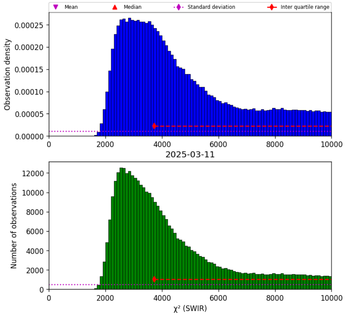
Figure 28: Histogram of " \chi^2 (SWIR)" for 2025-03-10 to 2025-03-12
