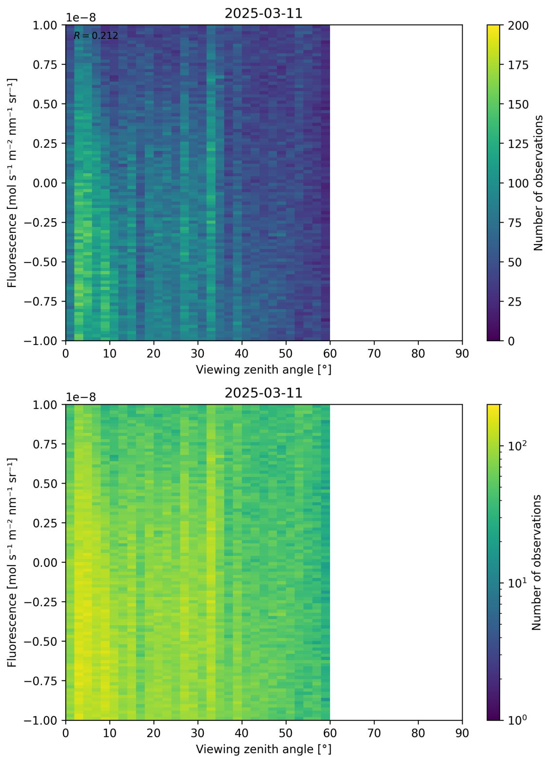
Figure 108: Scatter density plot of “Viewing zenith angle” against “Fluorescence” for 2025-03-10 to 2025-03-12.
