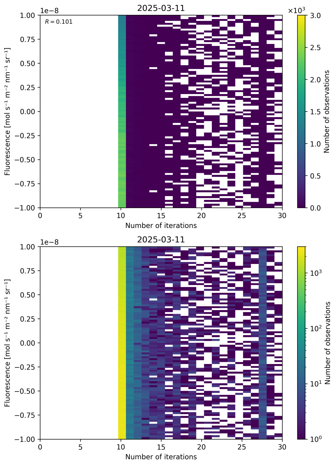
Figure 87: Scatter density plot of “Number of iterations” against “Fluorescence” for 2025-03-10 to 2025-03-12.
