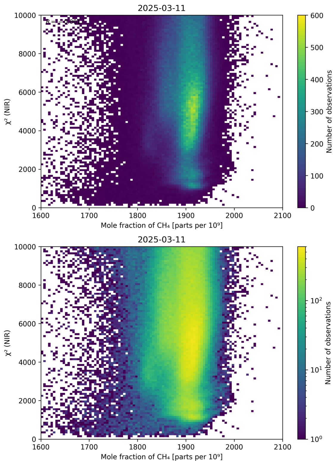
Figure 70: Scatter density plot of “Mole fraction of CH 4 ” against “ \chi^2 (NIR)” for 2025-03-10 to 2025-03-12.
