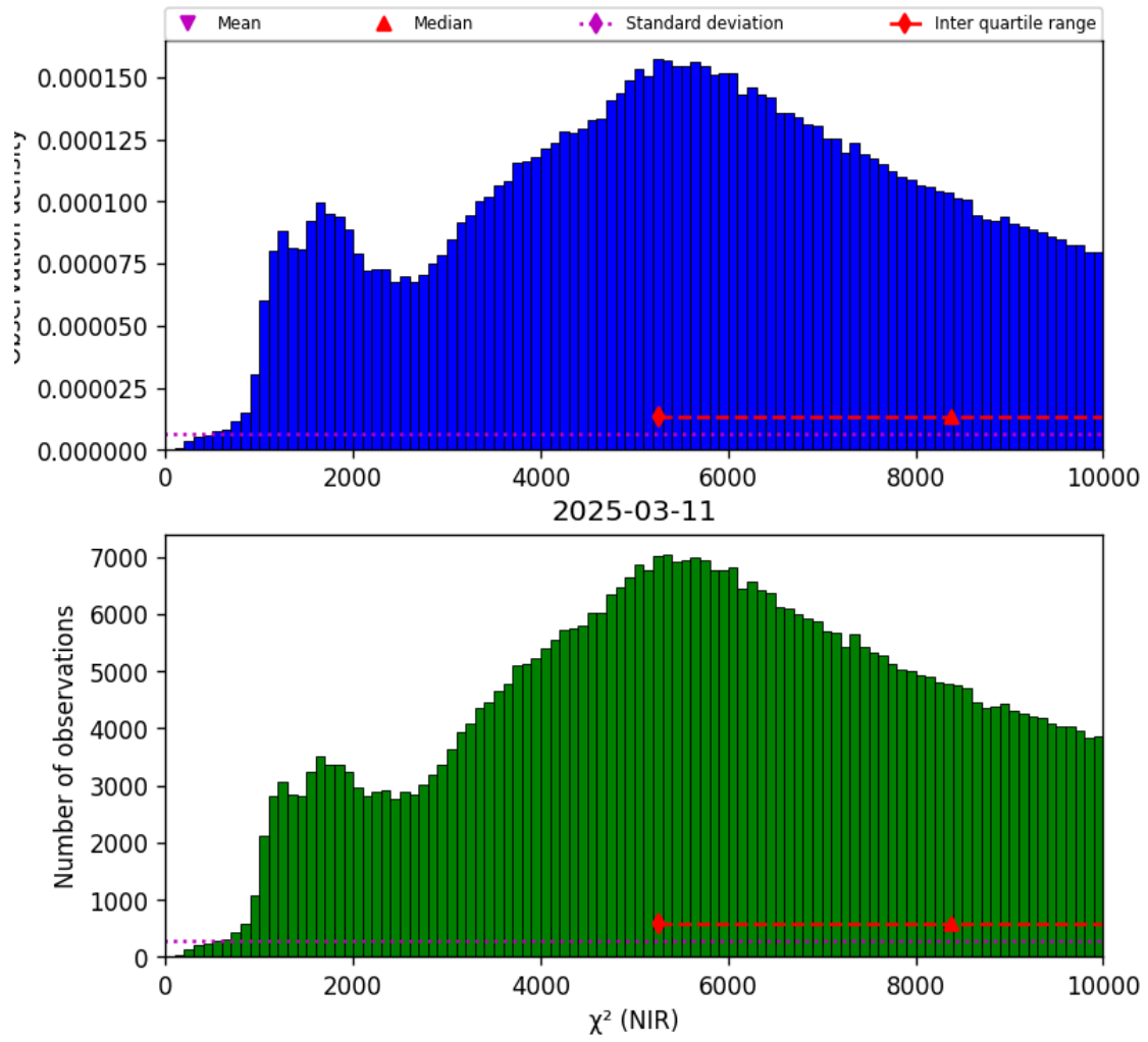
Figure 29: Histogram of “ \chi^2 (NIR)” for 2025-03-10 to 2025-03-12
