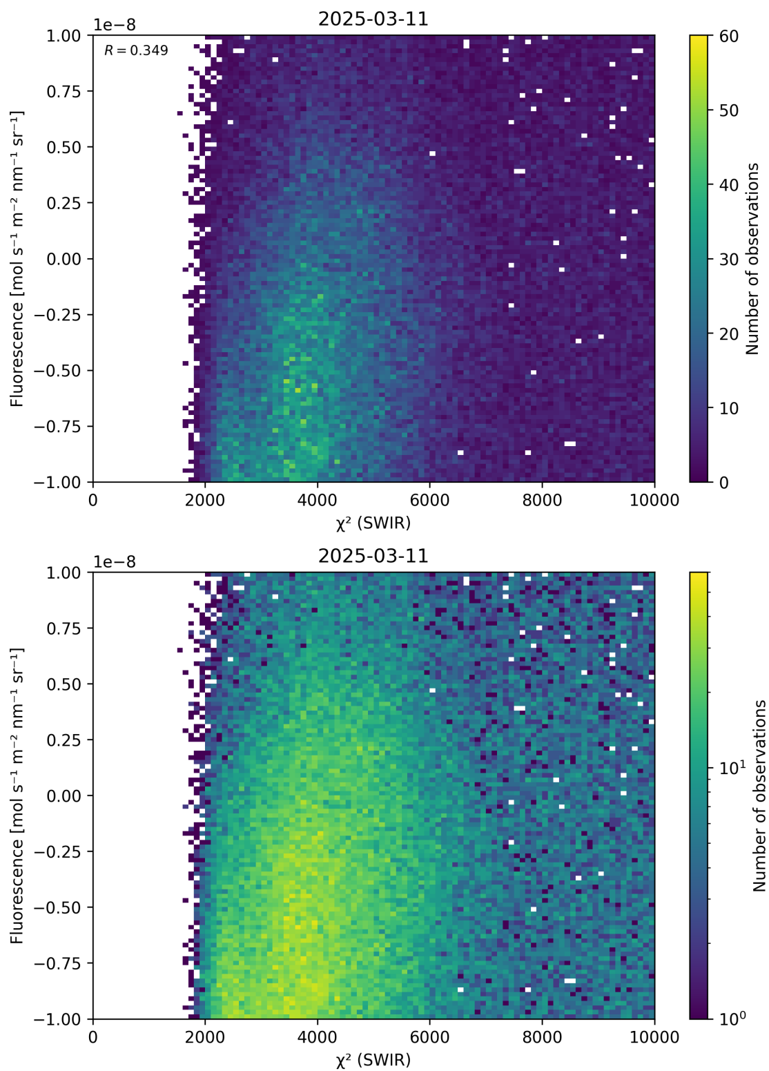
Figure 49: Scatter density plot of “ \chi^2 (SWIR)” against “Fluorescence” for 2025-03-10 to 2025-03-12.
