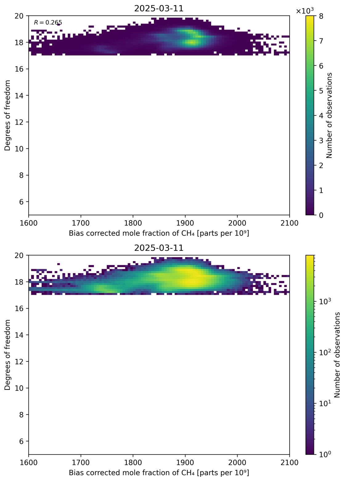
Figure 65: Scatter density plot of “Bias corrected mole fraction of CH 4 ” against “Degrees of freedom” for 2025-03-10 to 2025-03-12.
