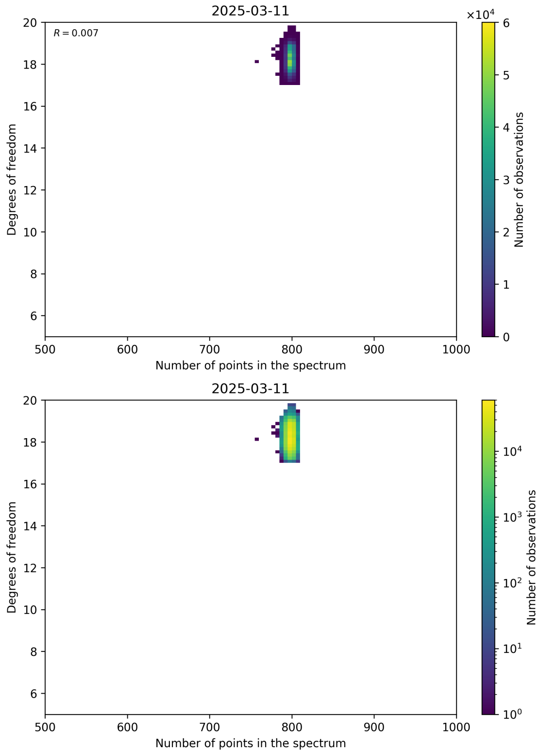
Figure 90: Scatter density plot of “Number of points in the spectrum” against “Degrees of freedom” for 2025-03-10 to 2025-03-12.
