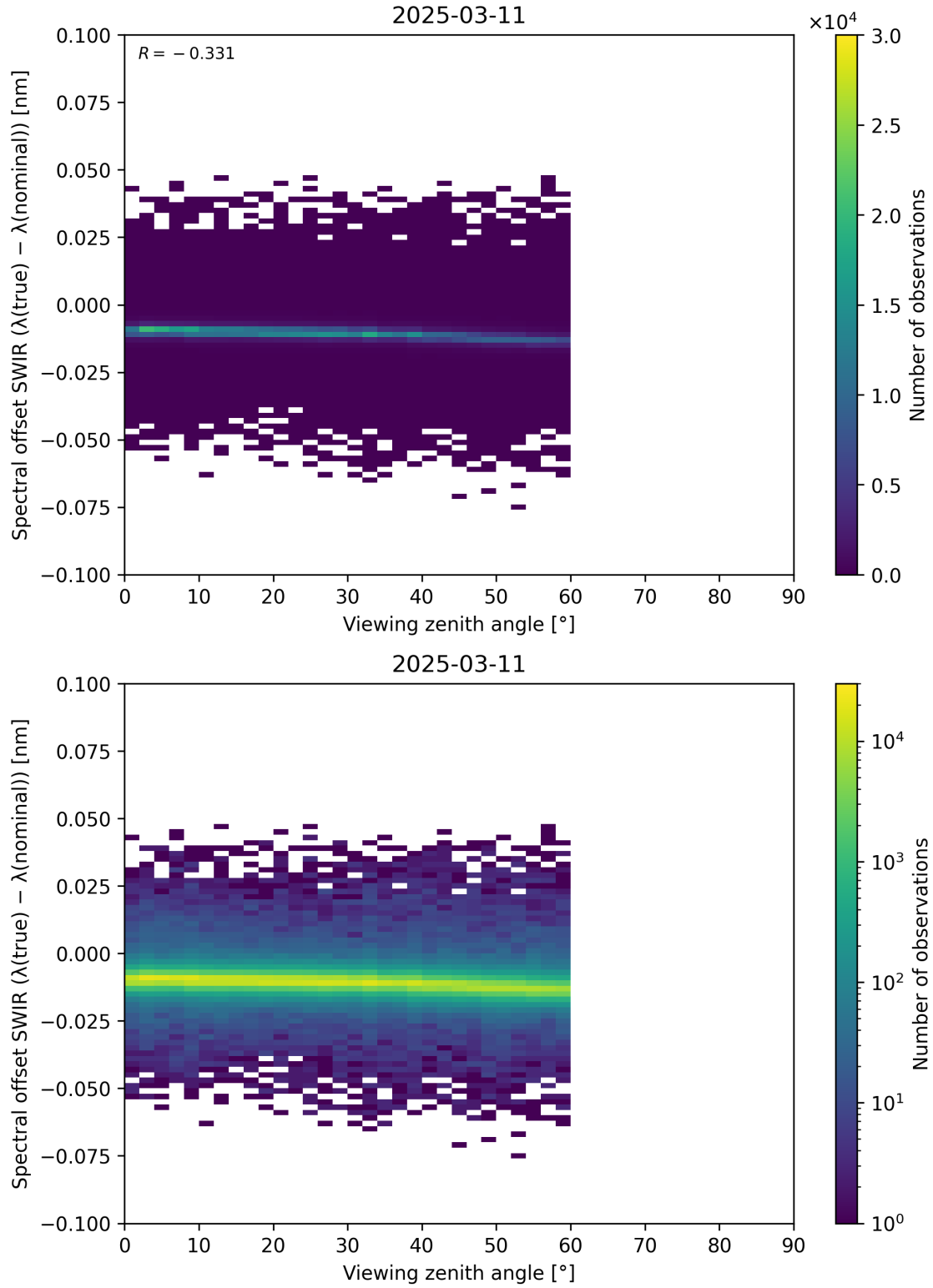
Figure 116: Scatter density plot of “Viewing zenith angle” against “Spectral offset SWIR ( \lambda_{\text{true}} - \lambda_{\text{nominal}} )” for 2025-03-10 to 2025-03-12.
