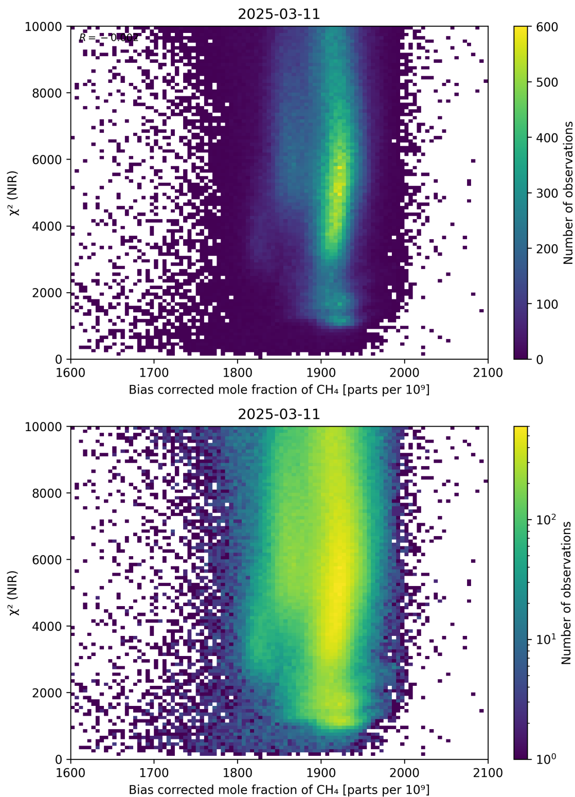
Figure 63: Scatter density plot of “Bias corrected mole fraction of CH 4 ” against “ \chi^2 (NIR)” for 2025-03-10 to 2025-03-12.
