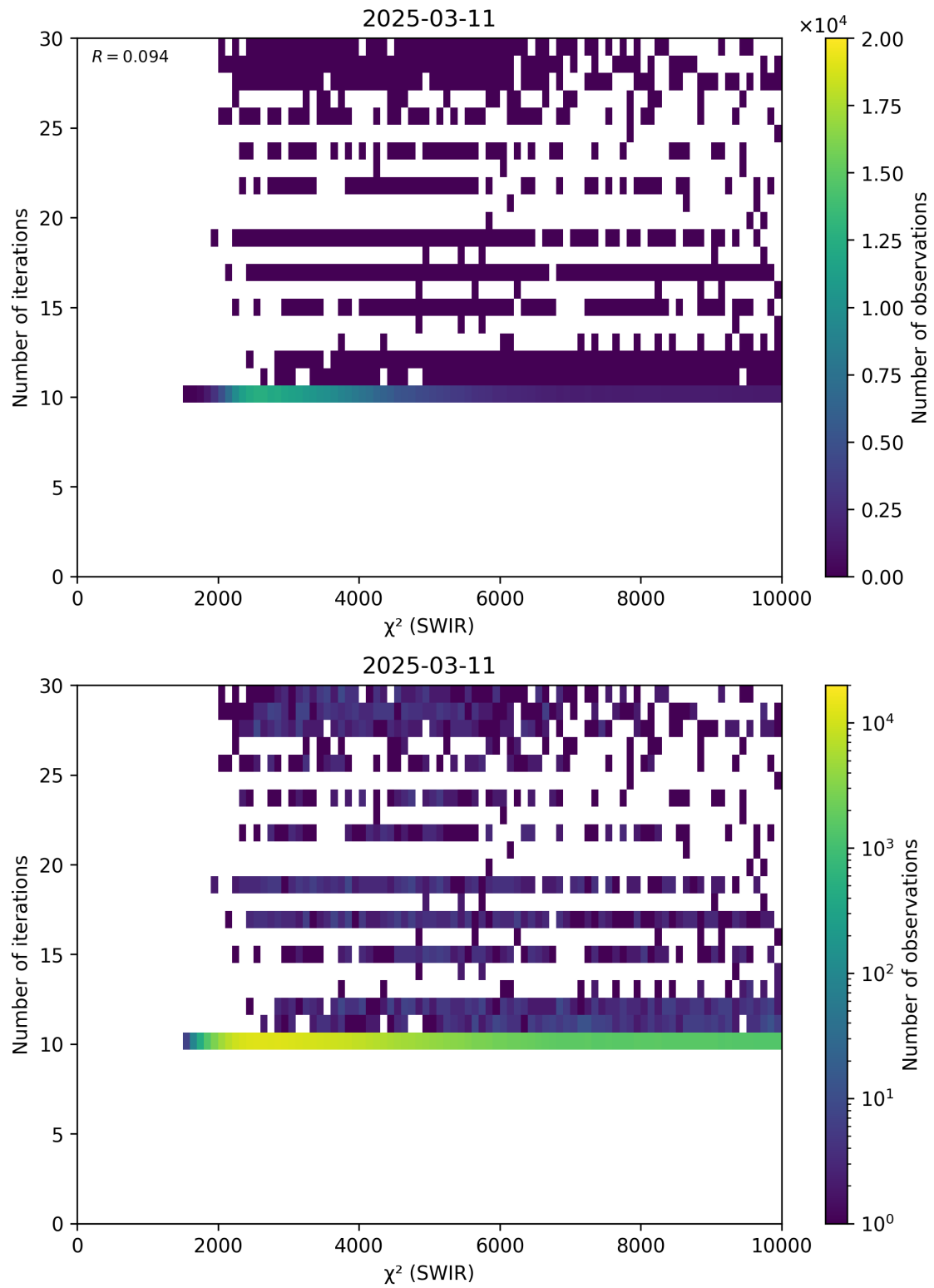
Figure 50: Scatter density plot of “ \chi^2 (SWIR)” against “Number of iterations” for 2025-03-10 to 2025-03-12.
