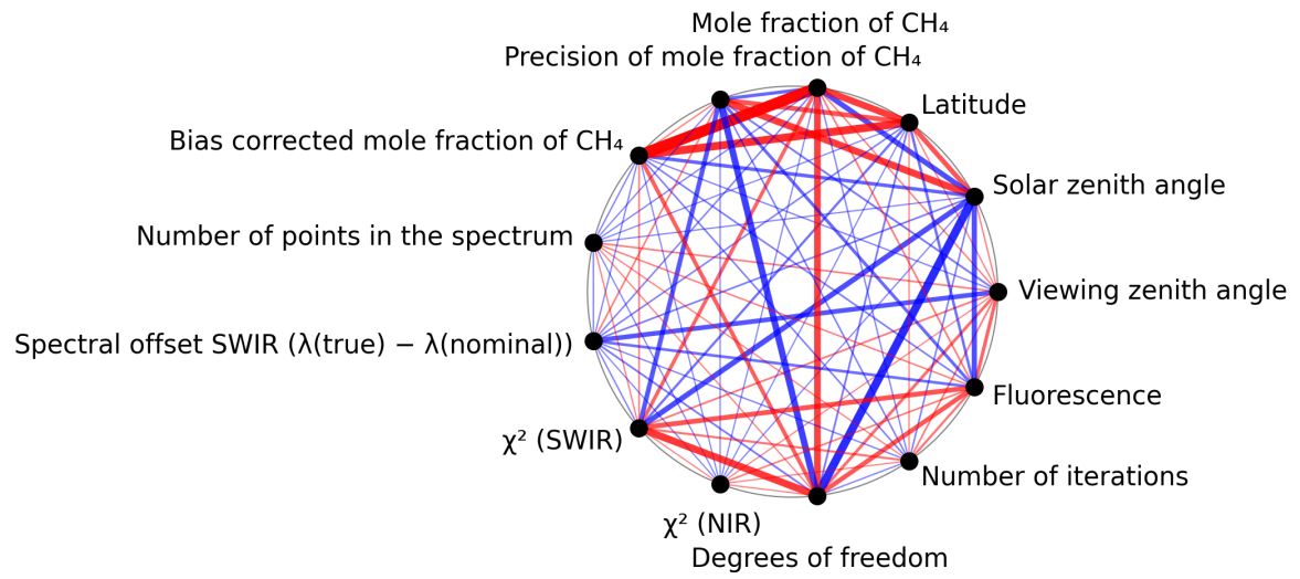
Figure 1: Map of correlation graph for 2025-03-10 to 2025-03-12.
