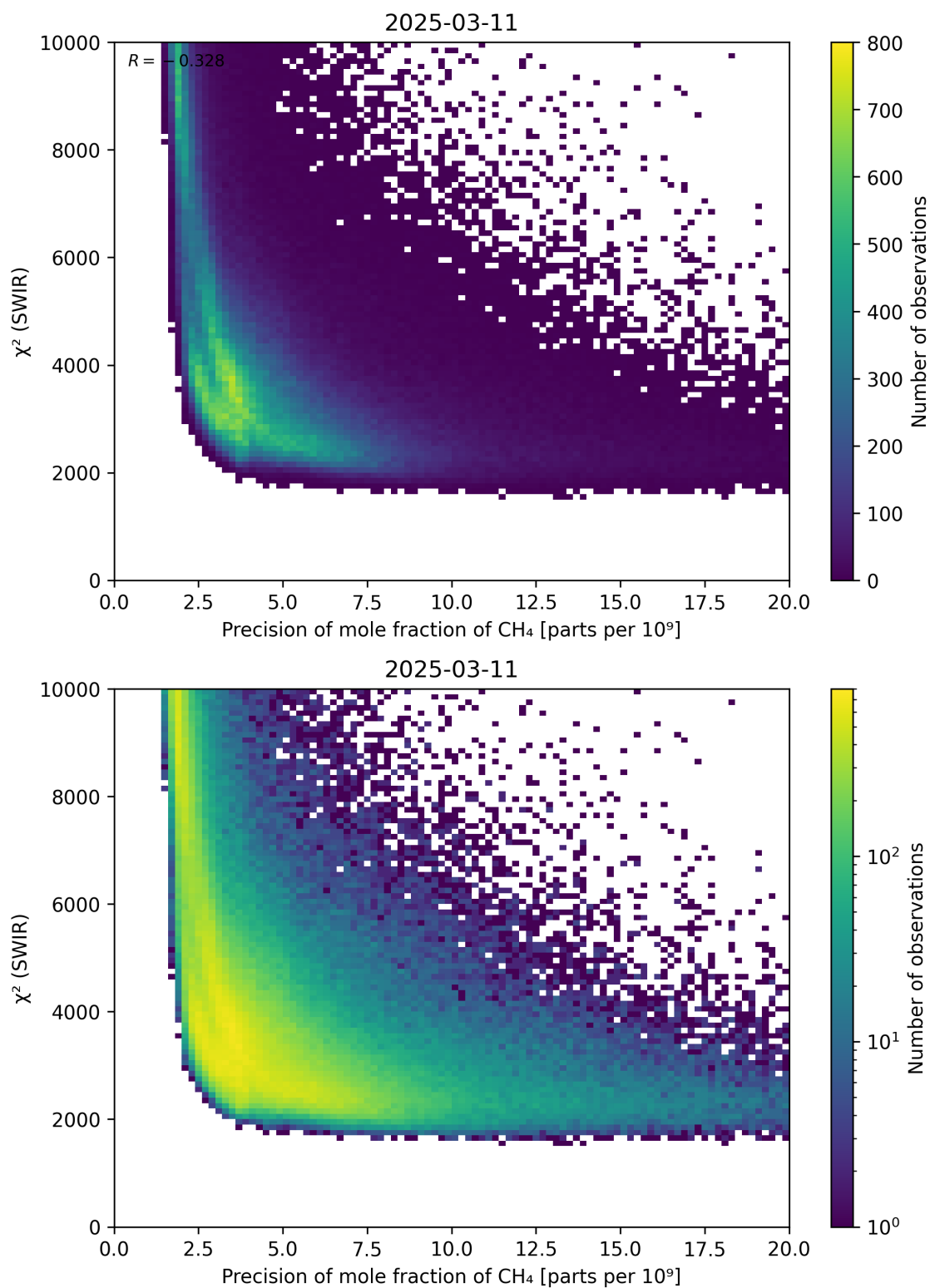
Figure 79: Scatter density plot of “Precision of mole fraction of \text{CH}_4 ” against “ \chi^2 (SWIR)” for 2025-03-10 to 2025-03-12.
