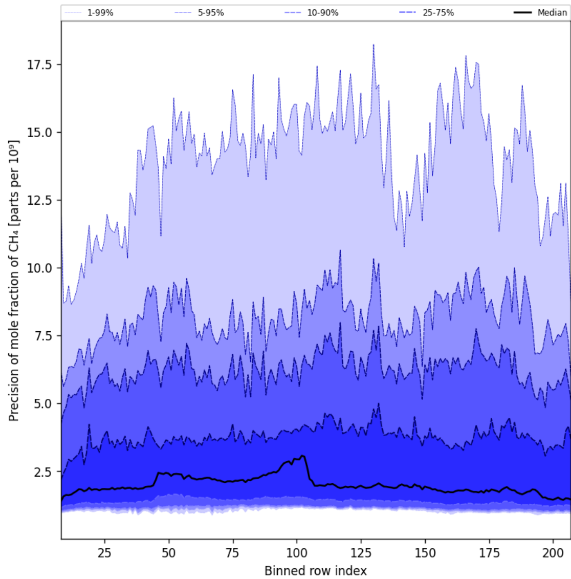
Figure 35: Along track statistics of “Precision of mole fraction of CH 4 ” for 2025-03-10 to 2025-03-12
