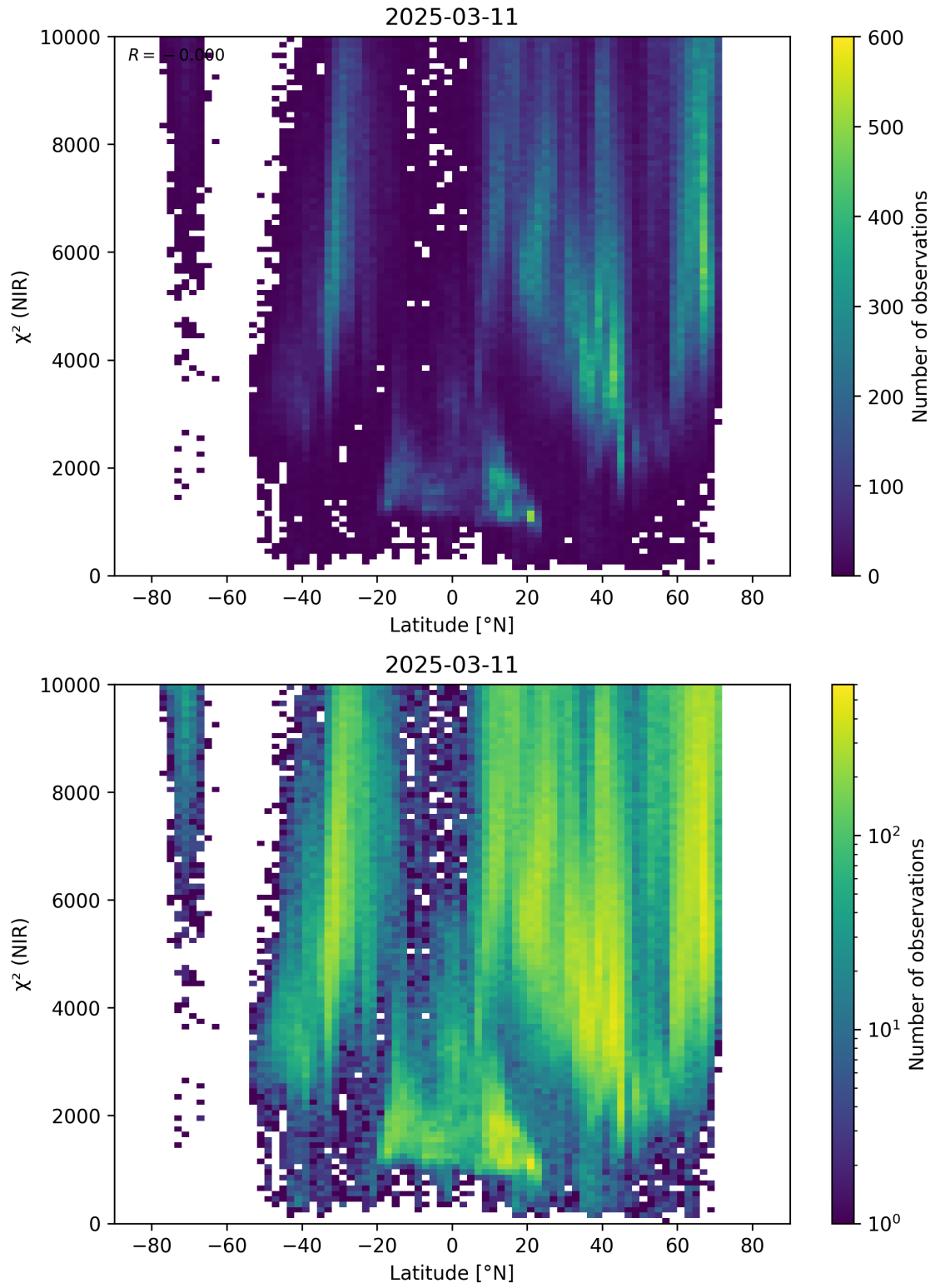
Figure 53: Scatter density plot of “Latitude” against “ \chi^2 (NIR)” for 2025-03-10 to 2025-03-12.
