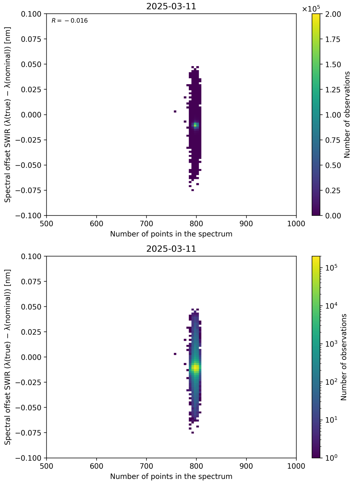
Figure 93: Scatter density plot of “Number of points in the spectrum” against “Spectral offset SWIR ( \lambda_{\text{true}} - \lambda_{\text{nominal}} )” for 2025-03-10 to 2025-03-12.
