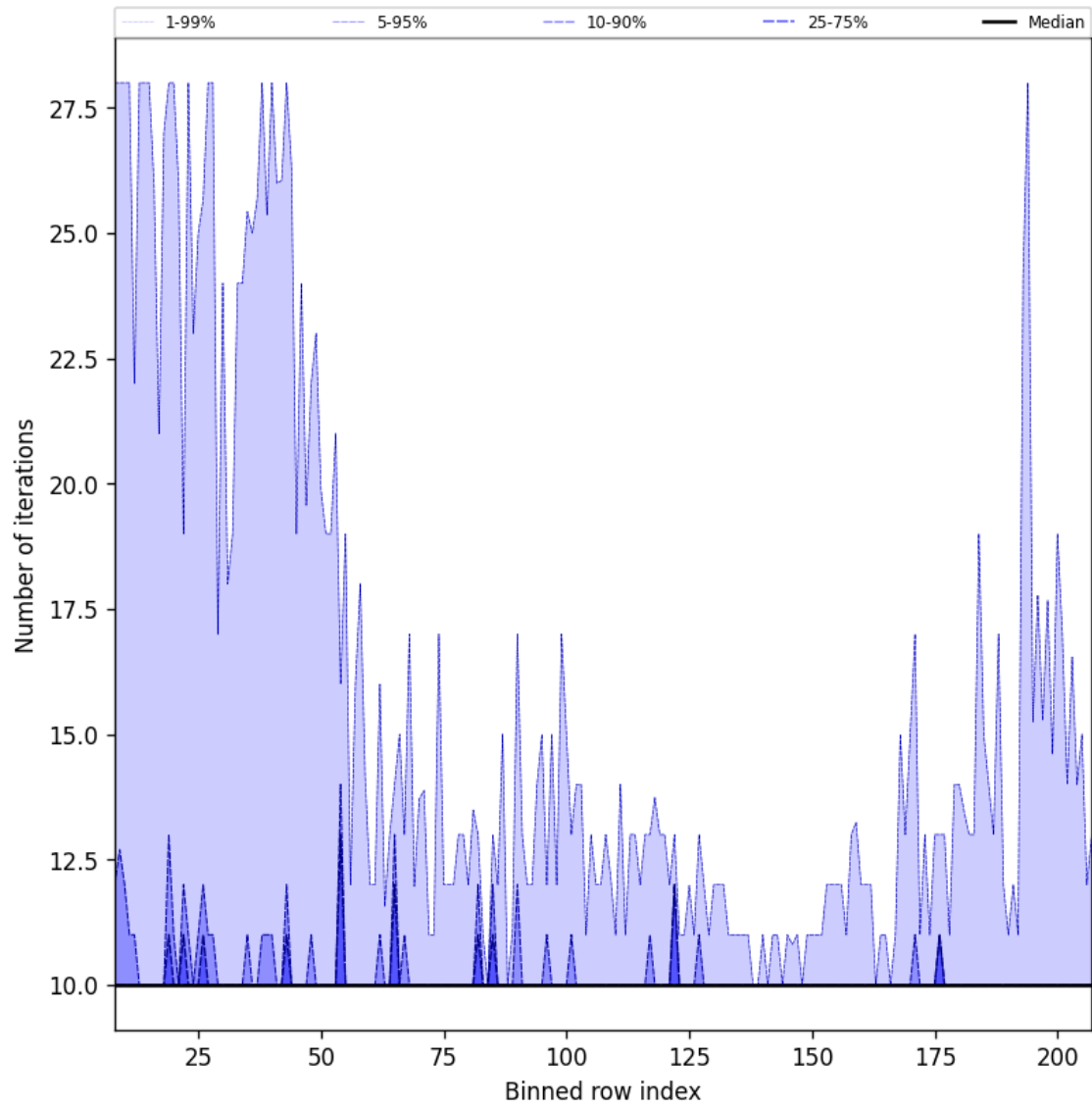
Figure 42: Along track statistics of “Number of iterations” for 2025-03-10 to 2025-03-12
