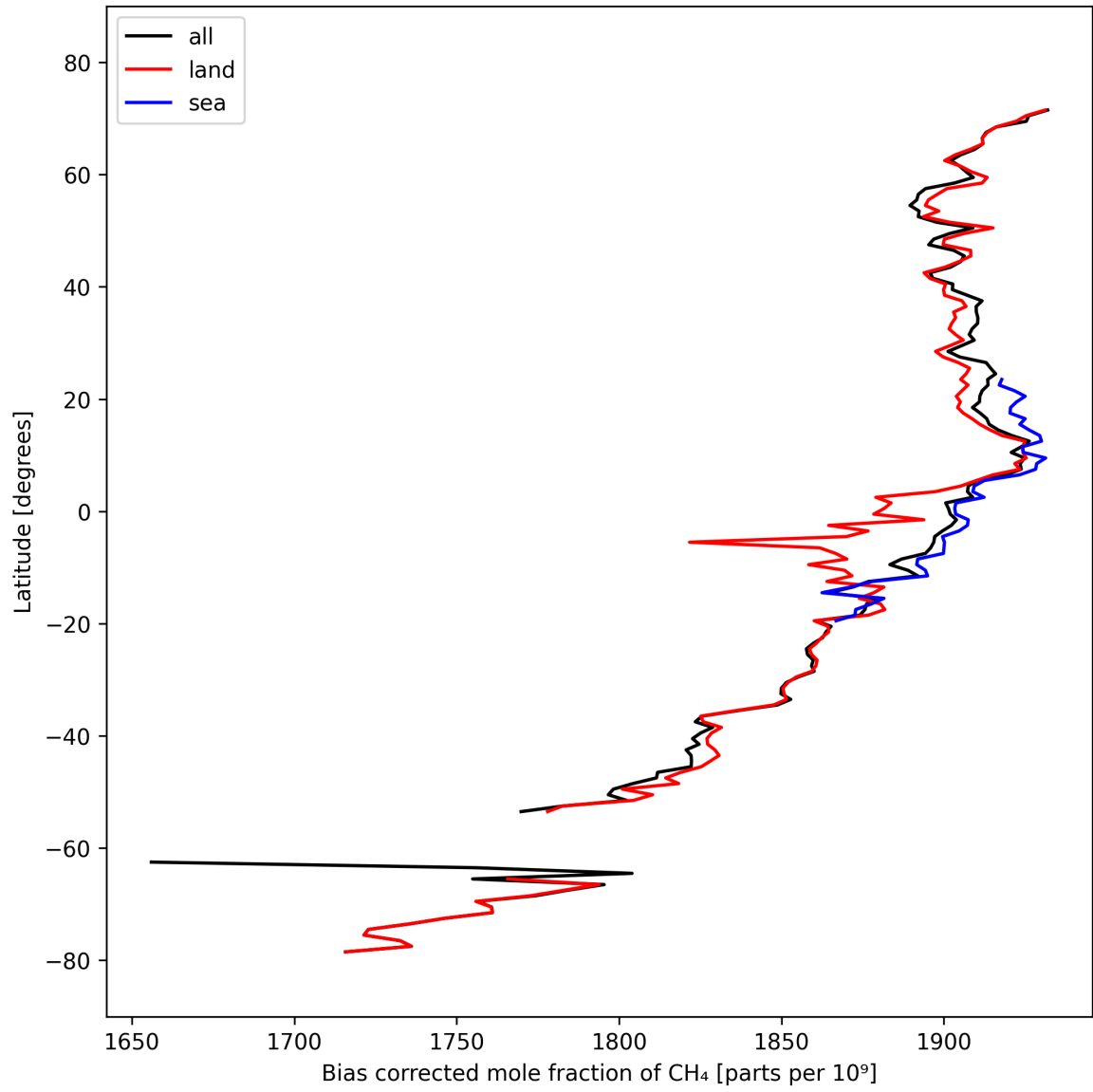
Figure 14: Zonal average of “Bias corrected mole fraction of CH 4 ” for 2025-03-10 to 2025-03-12.
