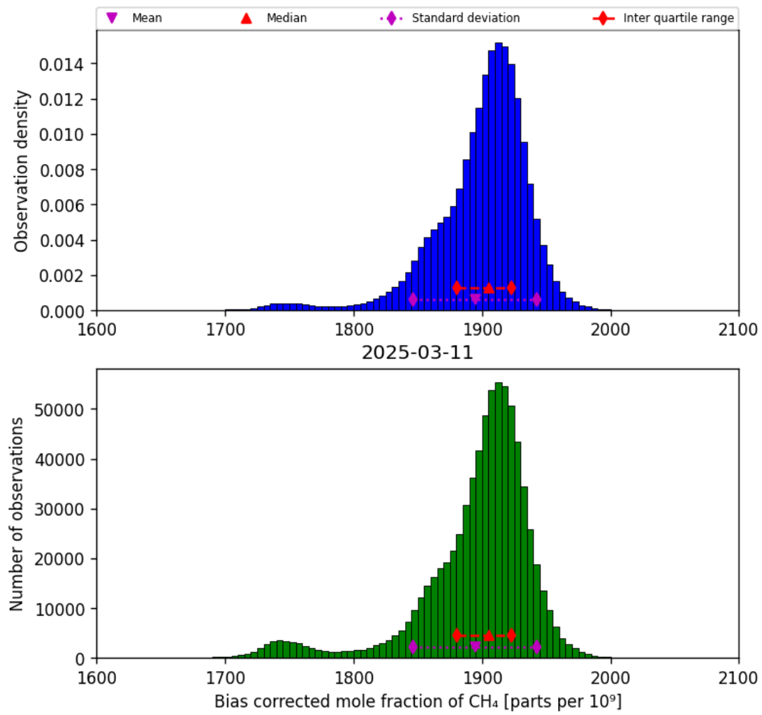
Figure 25: Histogram of “Bias corrected mole fraction of CH 4 ” for 2025-03-10 to 2025-03-12
