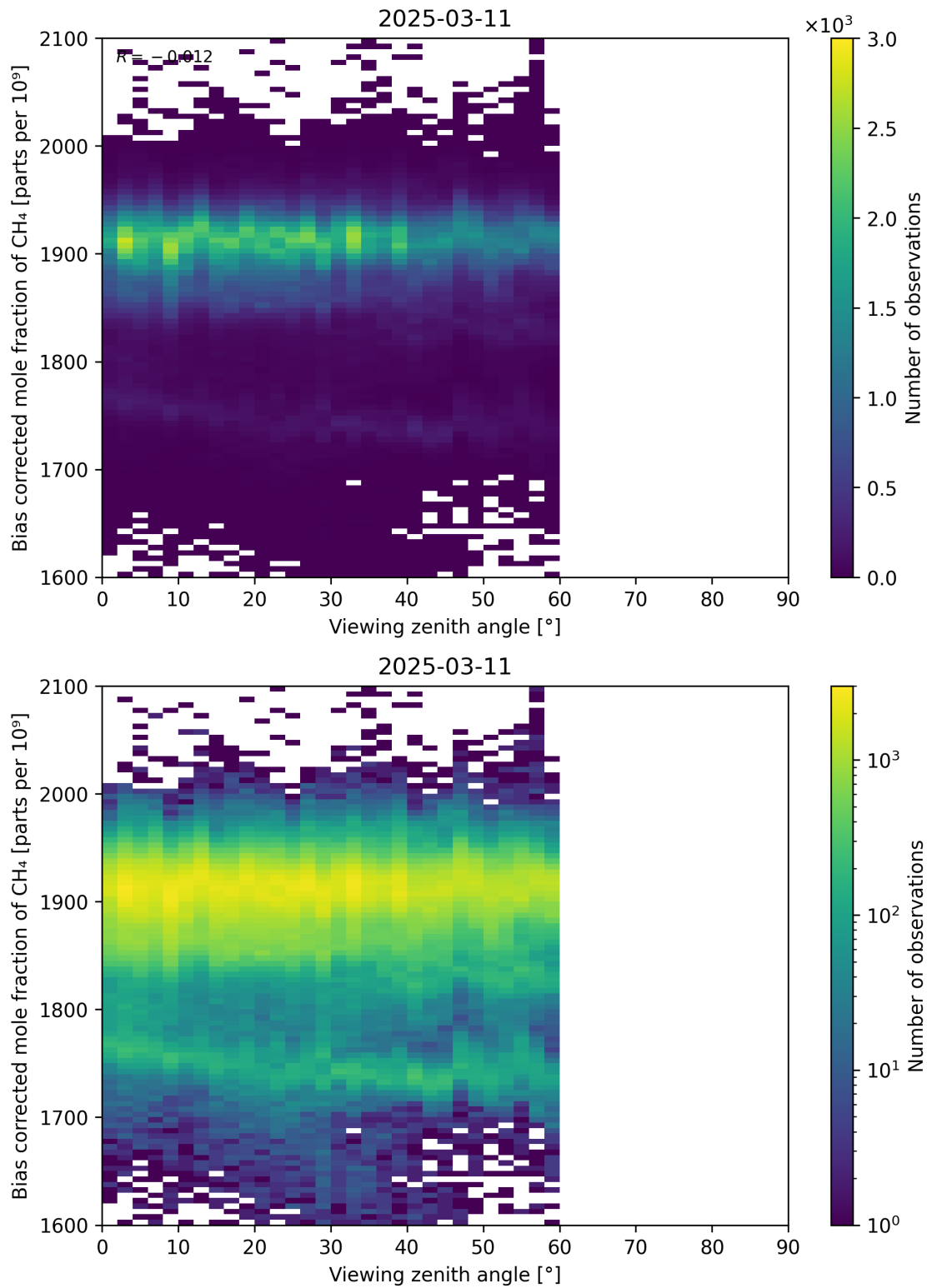
Figure 111: Scatter density plot of “Viewing zenith angle” against “Bias corrected mole fraction of CH 4 ” for 2025-03-10 to 2025-03-12.
