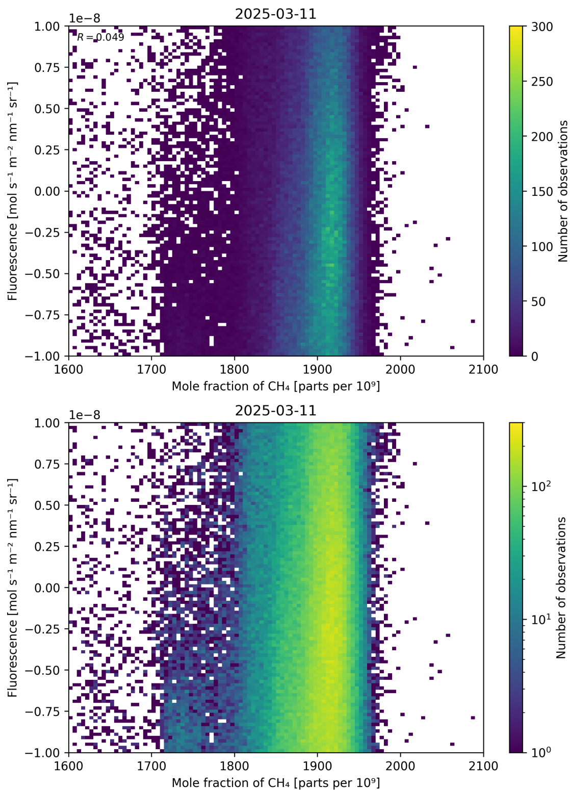
Figure 73: Scatter density plot of “Mole fraction of \text{CH}_4 ” against “Fluorescence” for 2025-03-10 to 2025-03-12.
