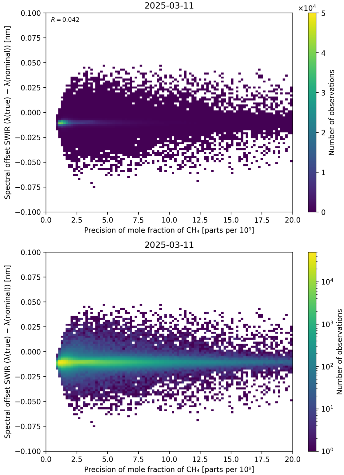
Figure 85: Scatter density plot of “Precision of mole fraction of CH 4 ” against “Spectral offset SWIR ( \lambda_{\text{true}} - \lambda_{\text{nominal}} )” for 2025-03-10 to 2025-03-12.
