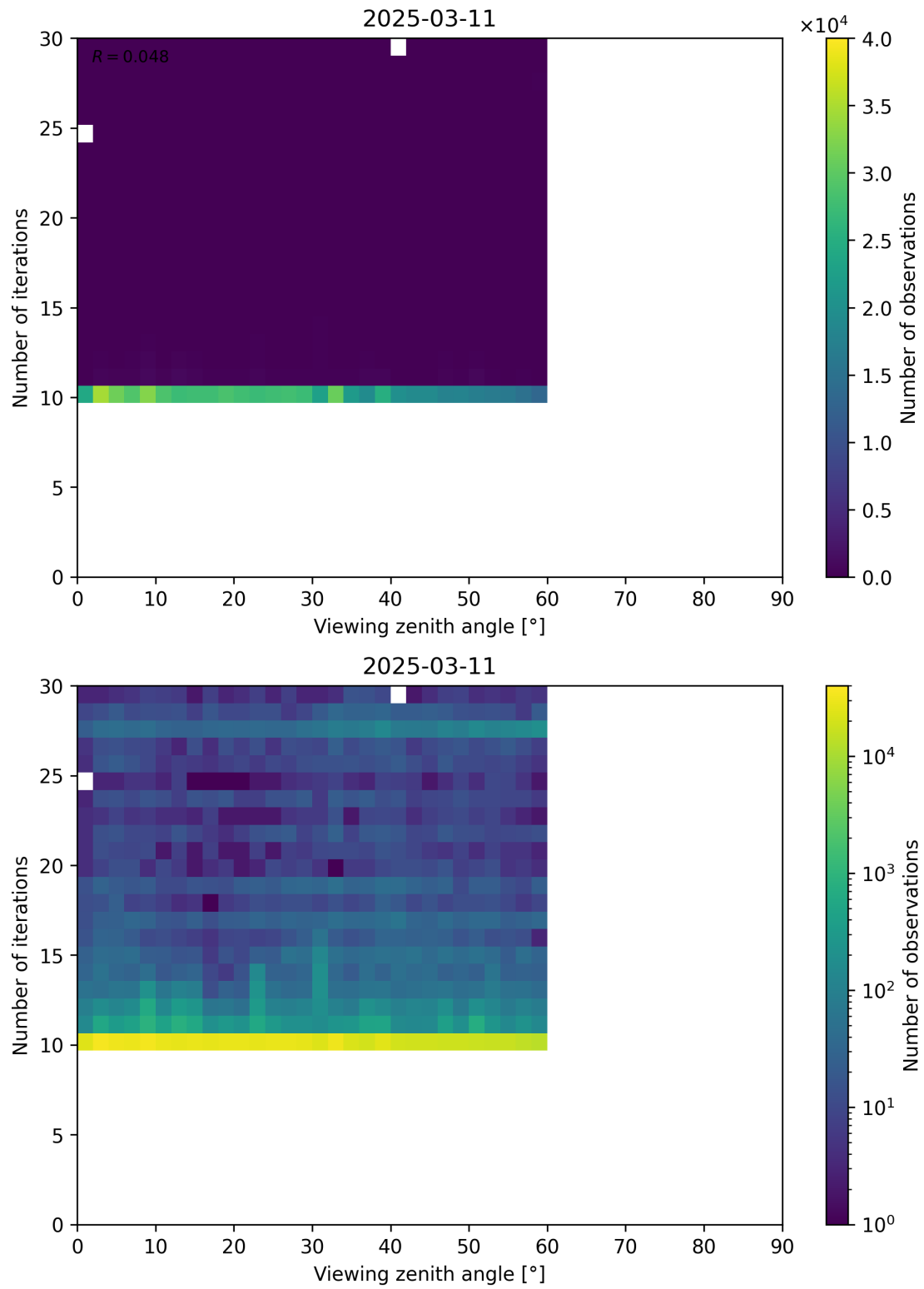
Figure 113: Scatter density plot of “Viewing zenith angle” against “Number of iterations” for 2025-03-10 to 2025-03-12.
