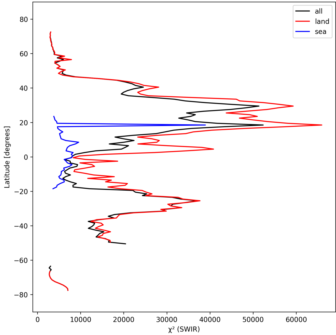
Figure 17: Zonal average of “ \chi^2 (SWIR)” for 2025-03-12 to 2025-03-13.
