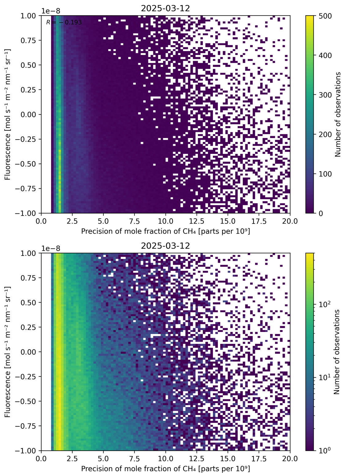
Figure 81: Scatter density plot of “Precision of mole fraction of CH 4 ” against “Fluorescence” for 2025-03-12 to 2025-03-13.
