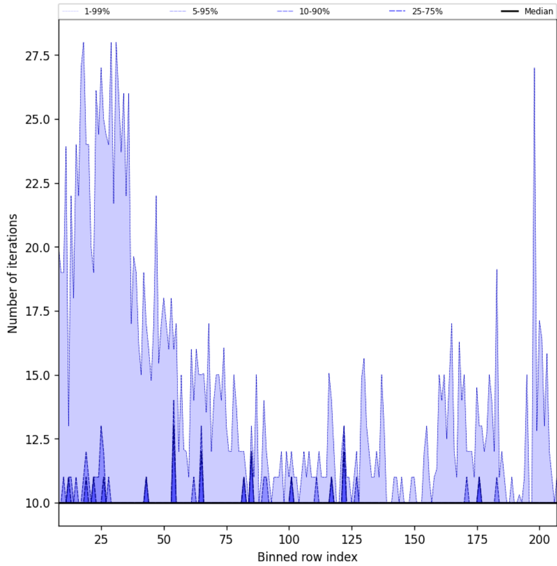
Figure 42: Along track statistics of “Number of iterations” for 2025-03-12 to 2025-03-13
