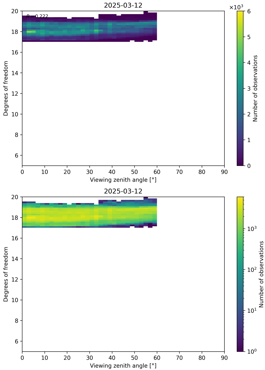
Figure 107: Scatter density plot of “Viewing zenith angle” against “Degrees of freedom” for 2025-03-12 to 2025-03-13.
