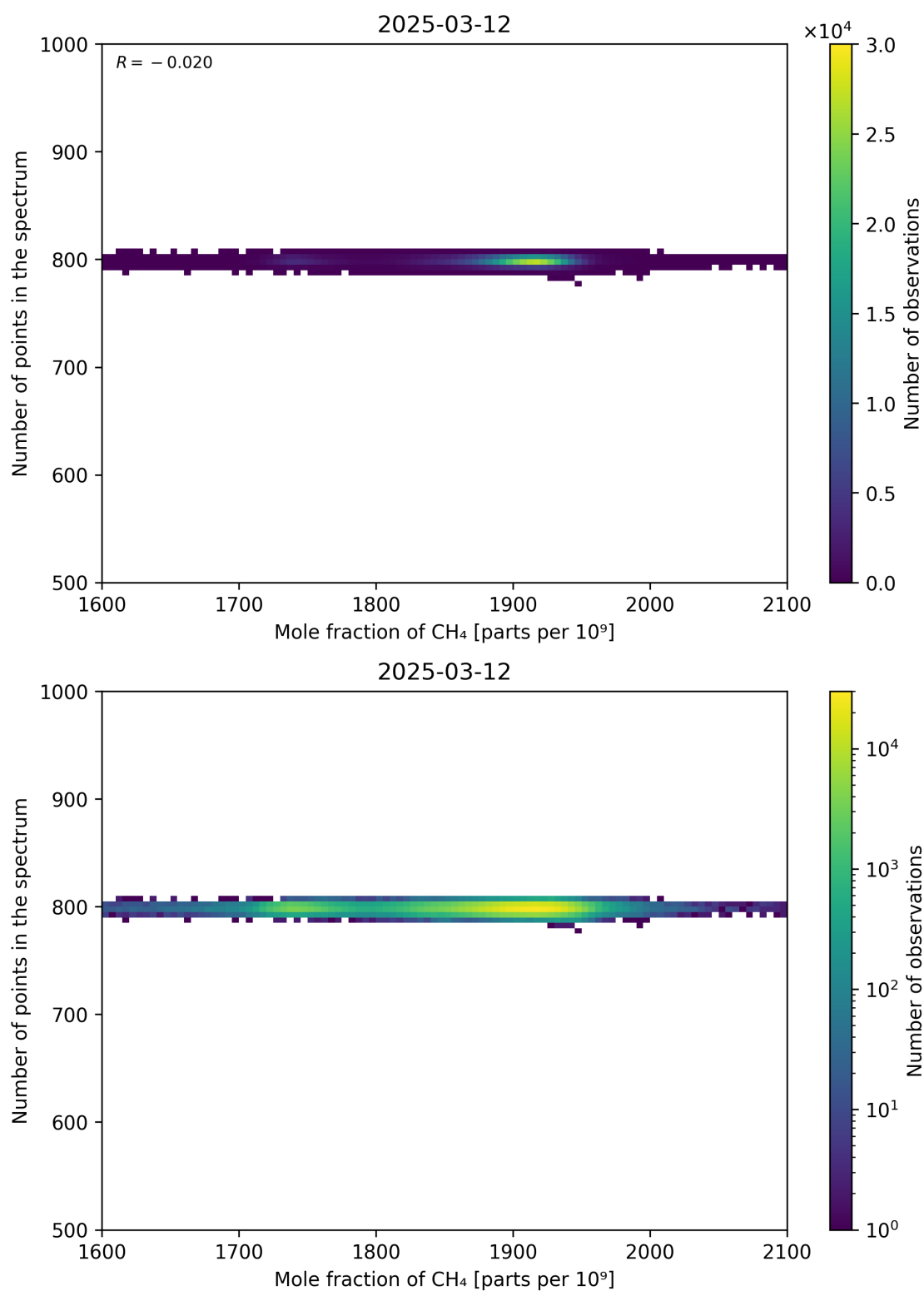
Figure 77: Scatter density plot of “Mole fraction of CH 4 ” against “Number of points in the spectrum” for 2025-03-12 to 2025-03-13.
