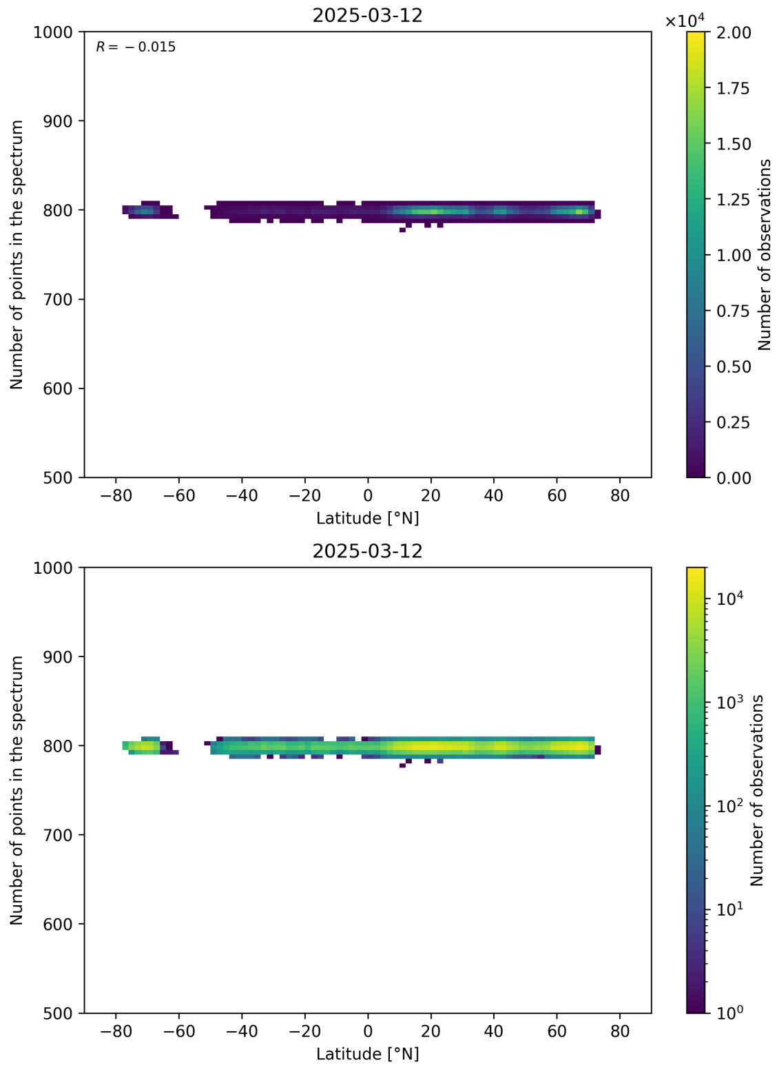
Figure 61: Scatter density plot of “Latitude” against “Number of points in the spectrum” for 2025-03-12 to 2025-03-13.
