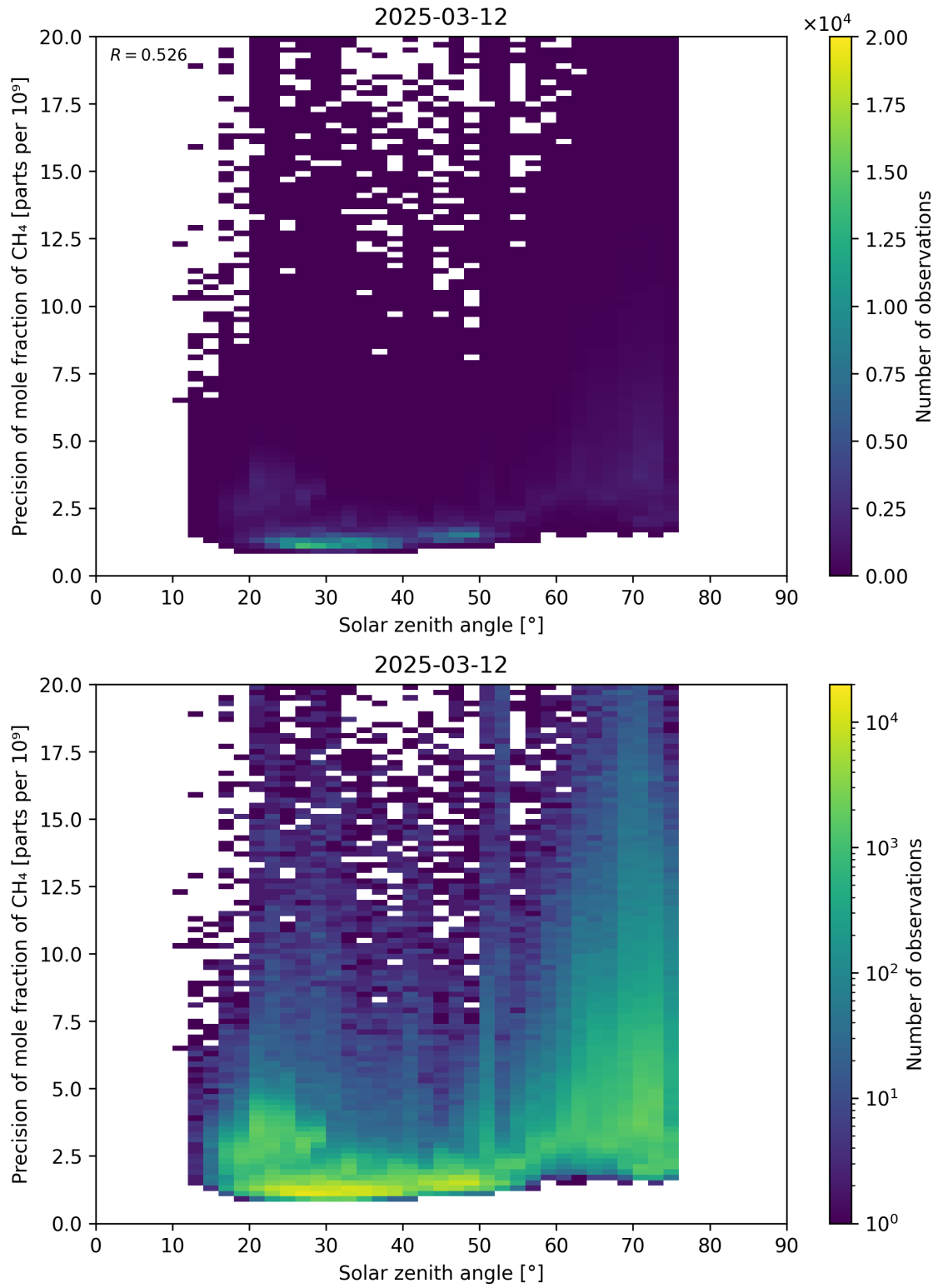
Figure 101: Scatter density plot of “Solar zenith angle” against “Precision of mole fraction of \text{CH}_4 ” for 2025-03-12 to 2025-03-13.
