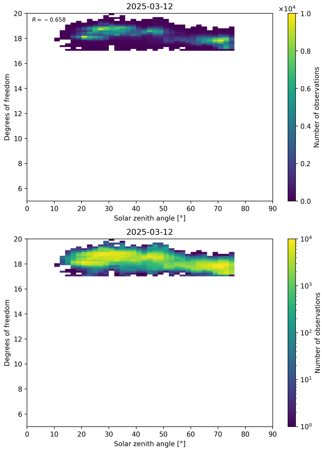
Figure 96: Scatter density plot of “Solar zenith angle” against “Degrees of freedom” for 2025-03-12 to 2025-03-13.
