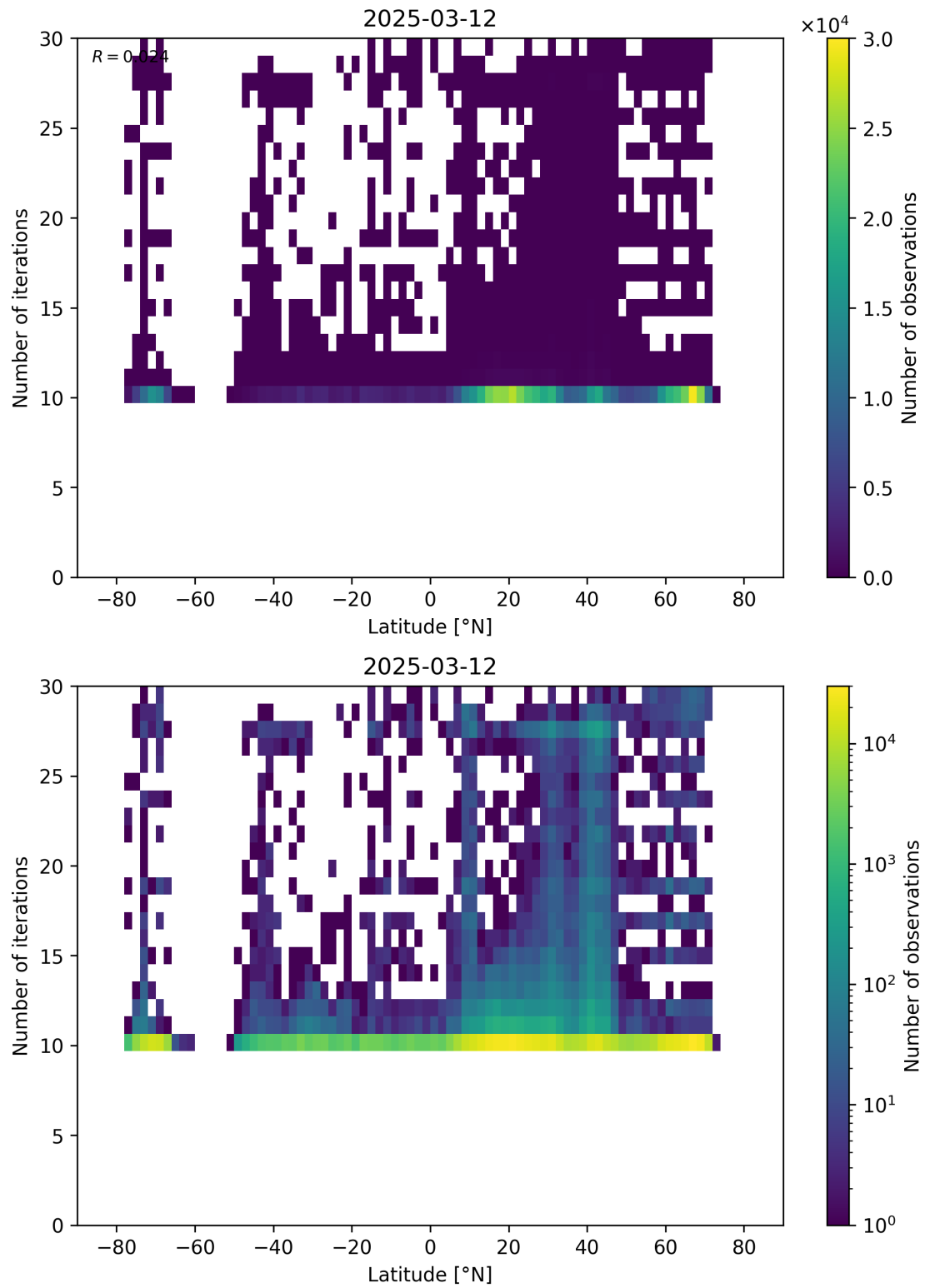
Figure 60: Scatter density plot of “Latitude” against “Number of iterations” for 2025-03-12 to 2025-03-13.
