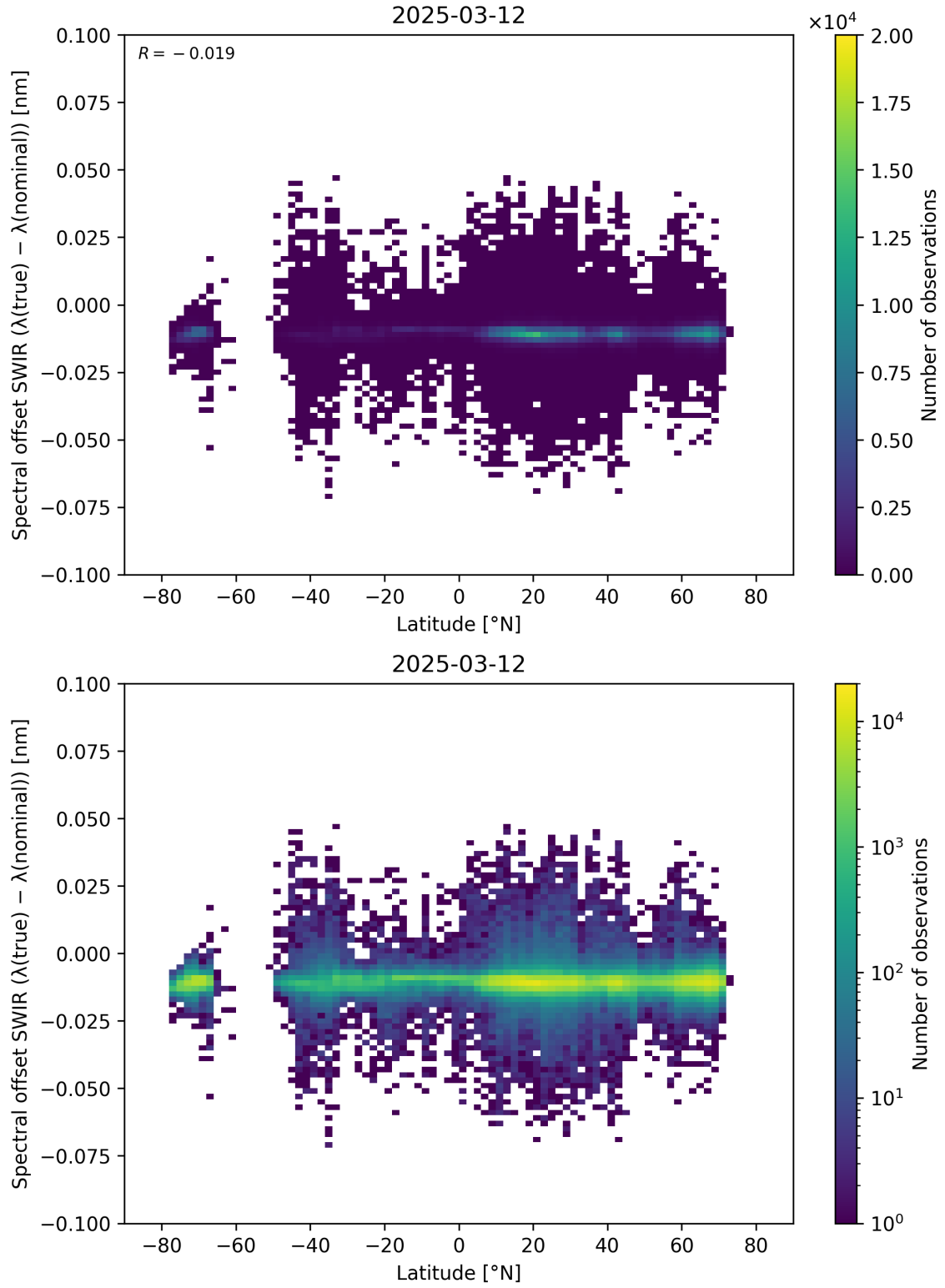
Figure 62: Scatter density plot of “Latitude” against “Spectral offset SWIR ( \lambda_{\text{true}} - \lambda_{\text{nominal}} )” for 2025-03-12 to 2025-03-13.
