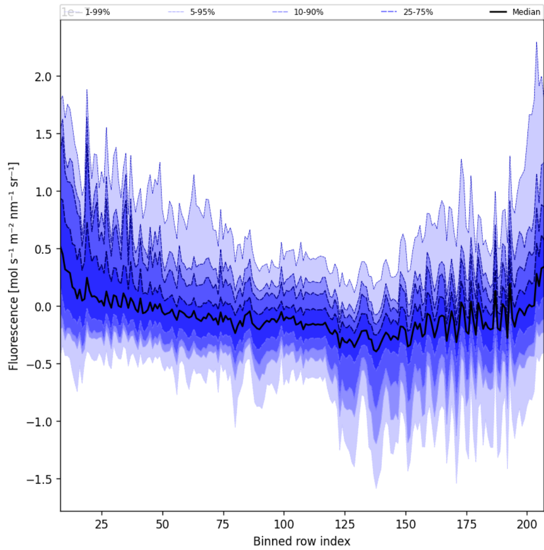
Figure 43: Along track statistics of “Fluorescence” for 2025-03-12 to 2025-03-13
