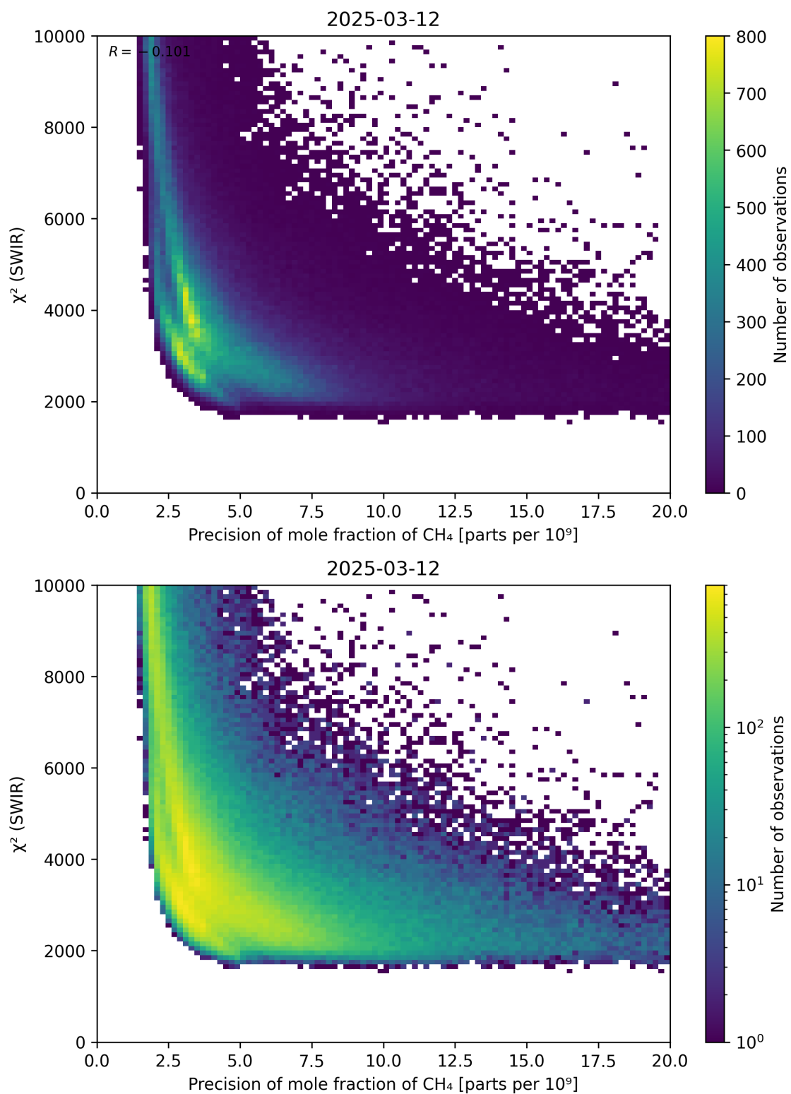
Figure 79: Scatter density plot of “Precision of mole fraction of \text{CH}_4 ” against “ \chi^2 (SWIR)” for 2025-03-12 to 2025-03-13.
