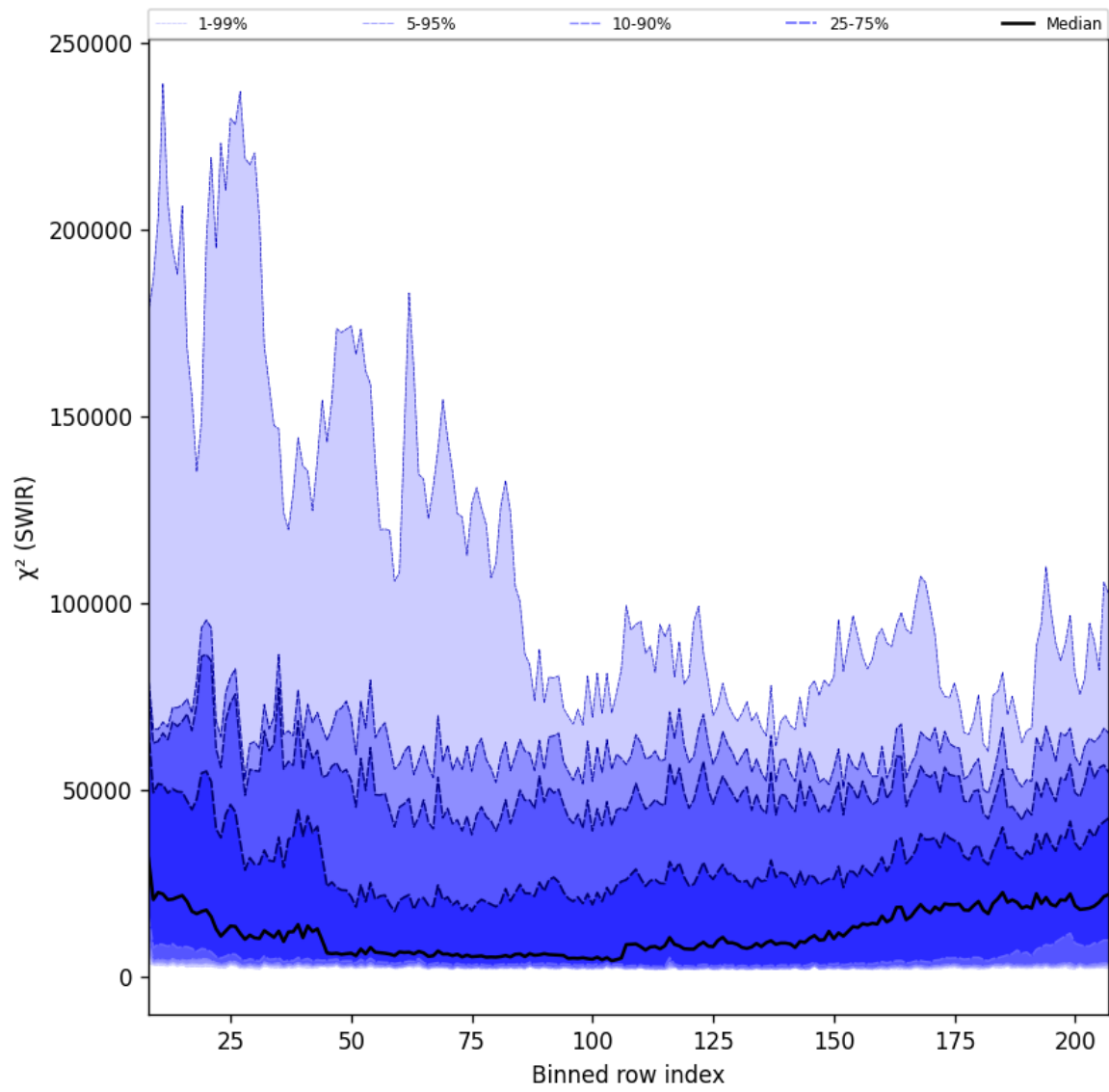
Figure 39: Along track statistics of “ \chi^2 (SWIR)” for 2025-03-12 to 2025-03-13
