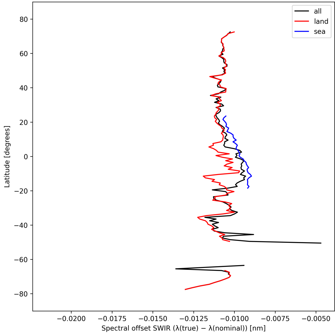
Figure 16: Zonal average of “Spectral offset SWIR ( \lambda_{\text{true}} - \lambda_{\text{nominal}} )” for 2025-03-12 to 2025-03-13.
