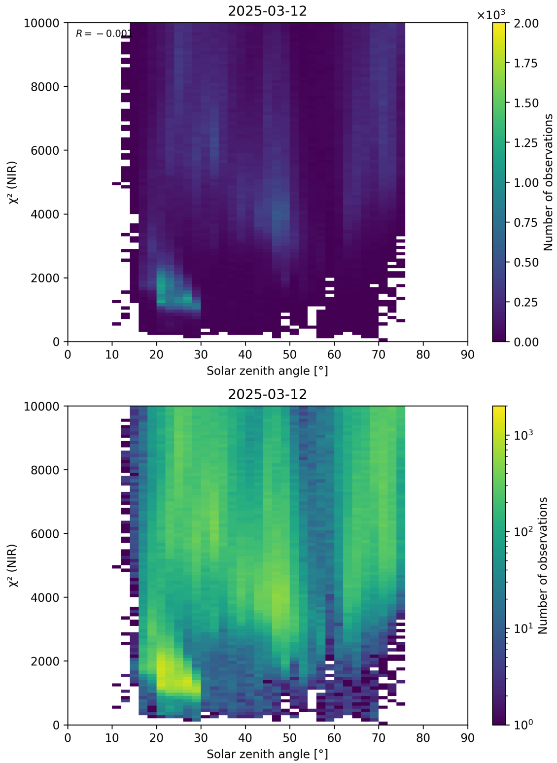
Figure 94: Scatter density plot of “Solar zenith angle” against “ \chi^2 (NIR)” for 2025-03-12 to 2025-03-13.
