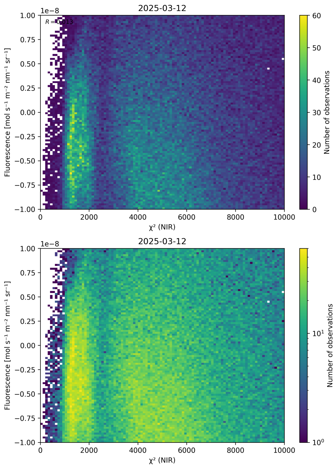
Figure 45: Scatter density plot of “ \chi^2 (NIR)” against “Fluorescence” for 2025-03-12 to 2025-03-13.
