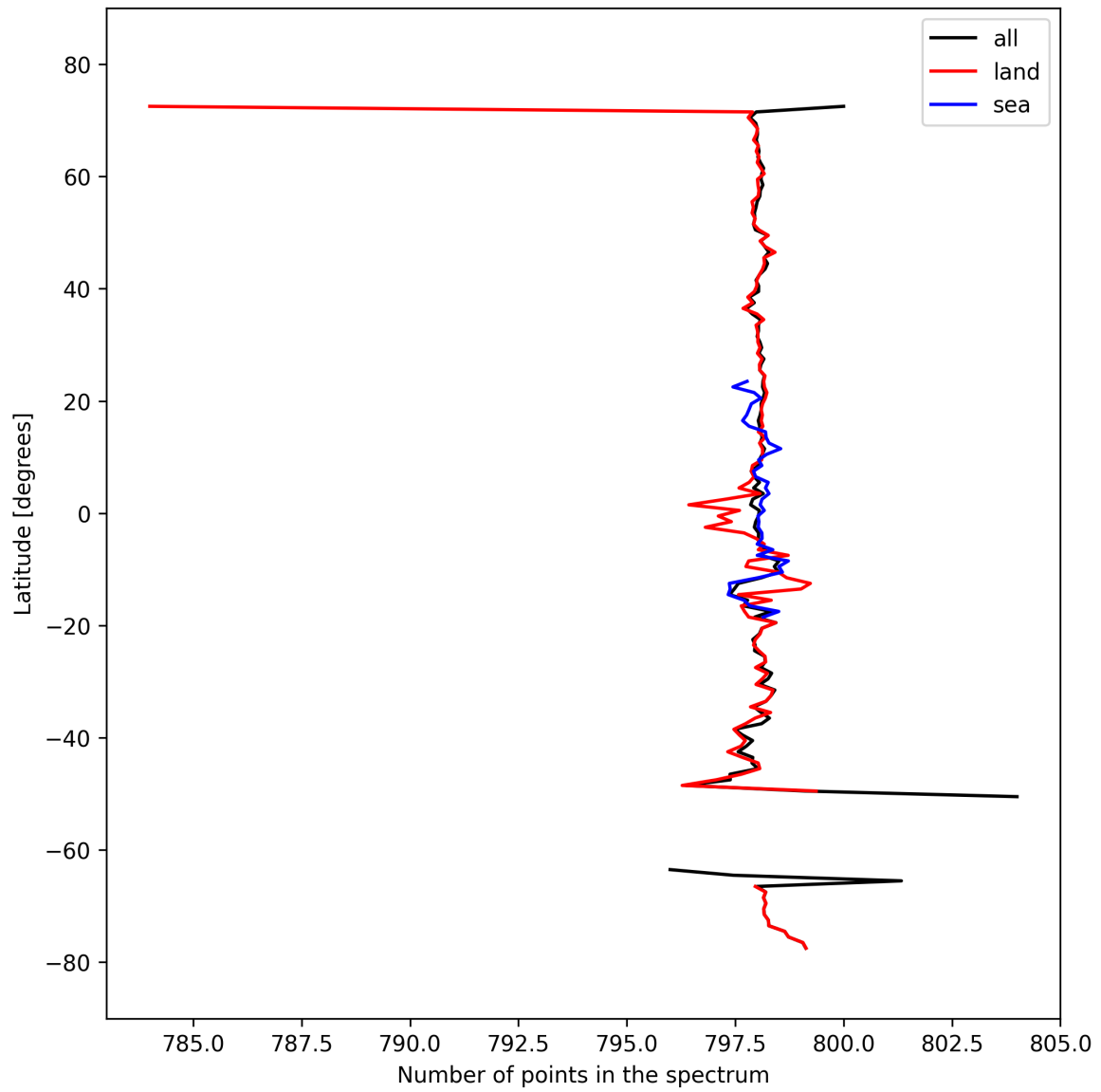
Figure 15: Zonal average of “Number of points in the spectrum” for 2025-03-12 to 2025-03-13.
