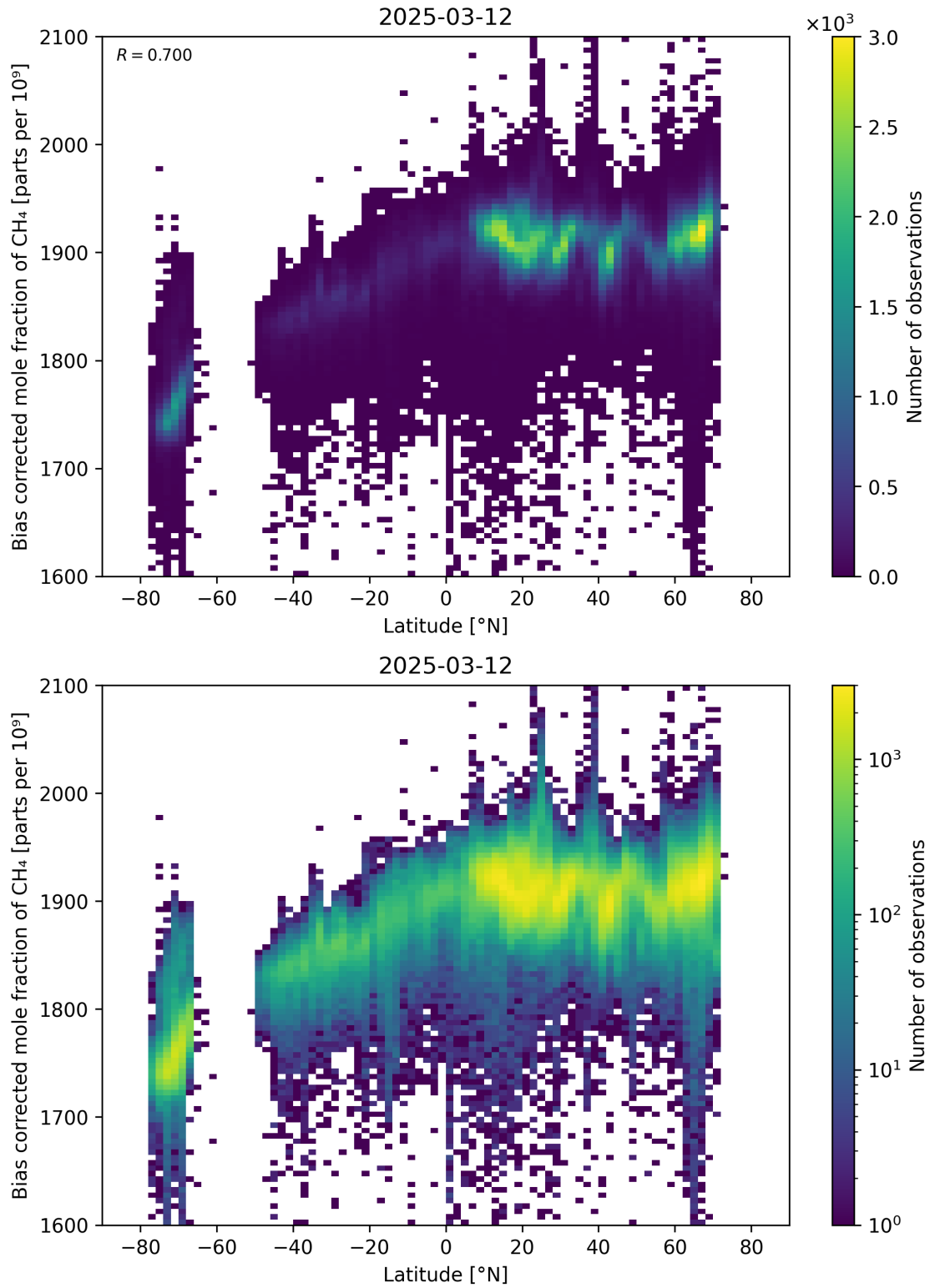
Figure 58: Scatter density plot of “Latitude” against “Bias corrected mole fraction of CH 4 ” for 2025-03-12 to 2025-03-13.
