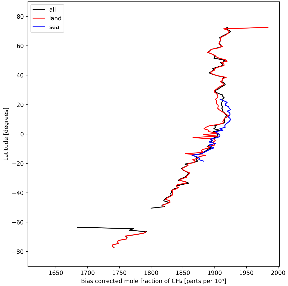
Figure 14: Zonal average of “Bias corrected mole fraction of CH 4 ” for 2025-03-12 to 2025-03-13.
