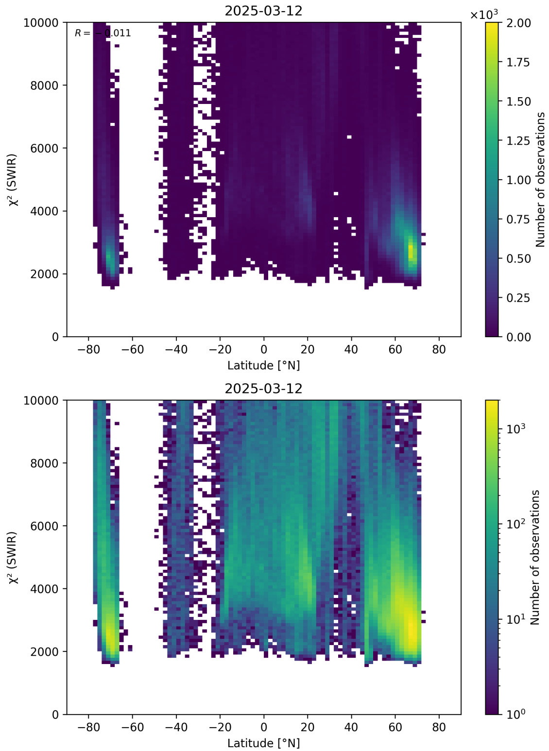
Figure 54: Scatter density plot of “Latitude” against “ \chi^2 (SWIR)” for 2025-03-12 to 2025-03-13.
