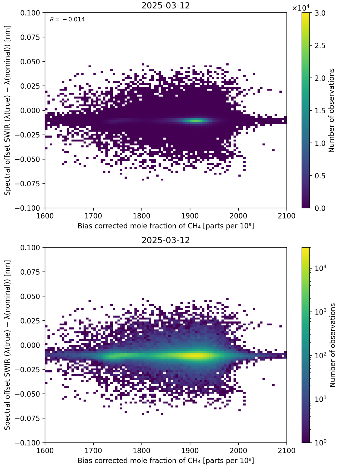
Figure 69: Scatter density plot of “Bias corrected mole fraction of \text{CH}_4 ” against “Spectral offset SWIR ( \lambda_{\text{true}} - \lambda_{\text{nominal}} )” for 2025-03-12 to 2025-03-13.
