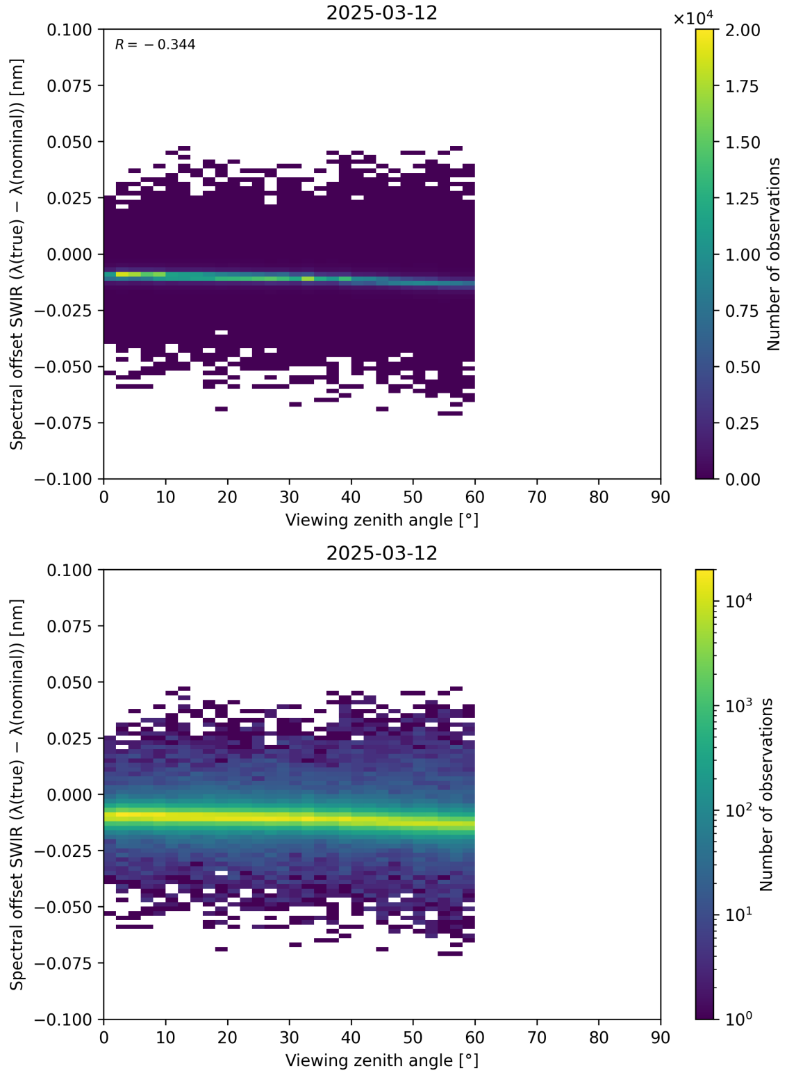
Figure 116: Scatter density plot of “Viewing zenith angle” against “Spectral offset SWIR ( \lambda_{\text{true}} - \lambda_{\text{nominal}} )” for 2025-03-12 to 2025-03-13.
