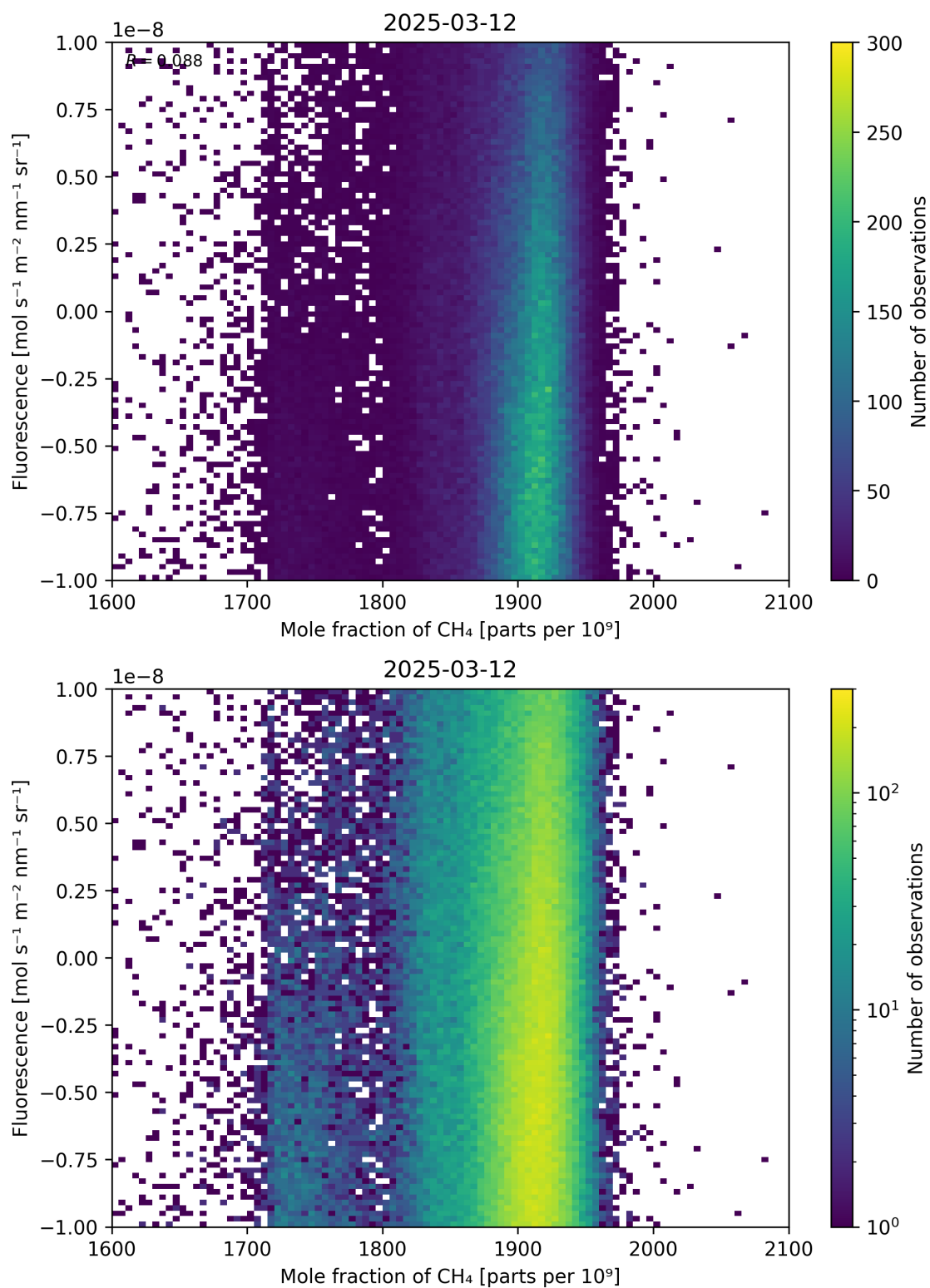
Figure 73: Scatter density plot of “Mole fraction of CH 4 ” against “Fluorescence” for 2025-03-12 to 2025-03-13.
