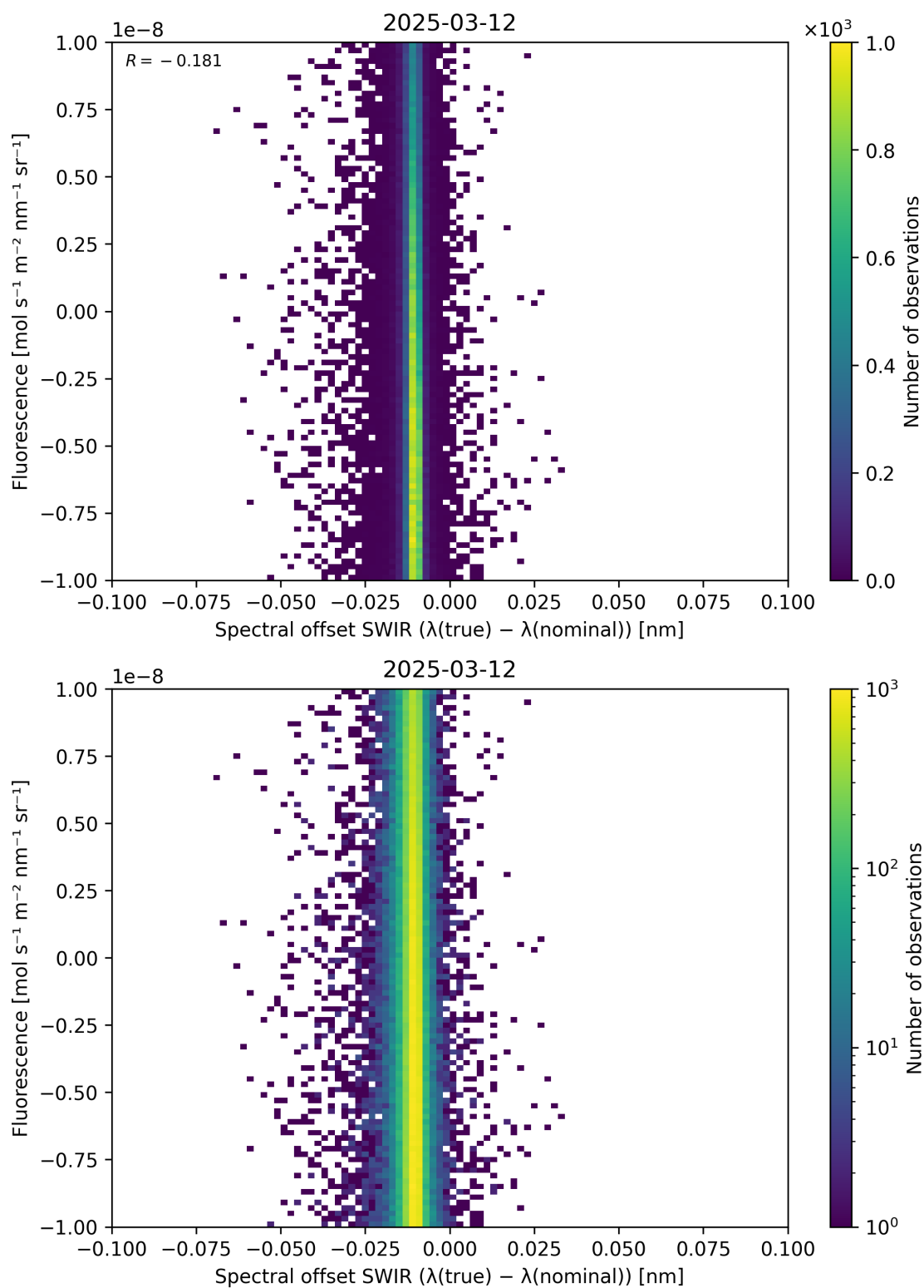
Figure 120: Scatter density plot of “Spectral offset SWIR ( \lambda_{\text{true}} - \lambda_{\text{nominal}} )” against “Fluorescence” for 2025-03-12 to 2025-03-13.
