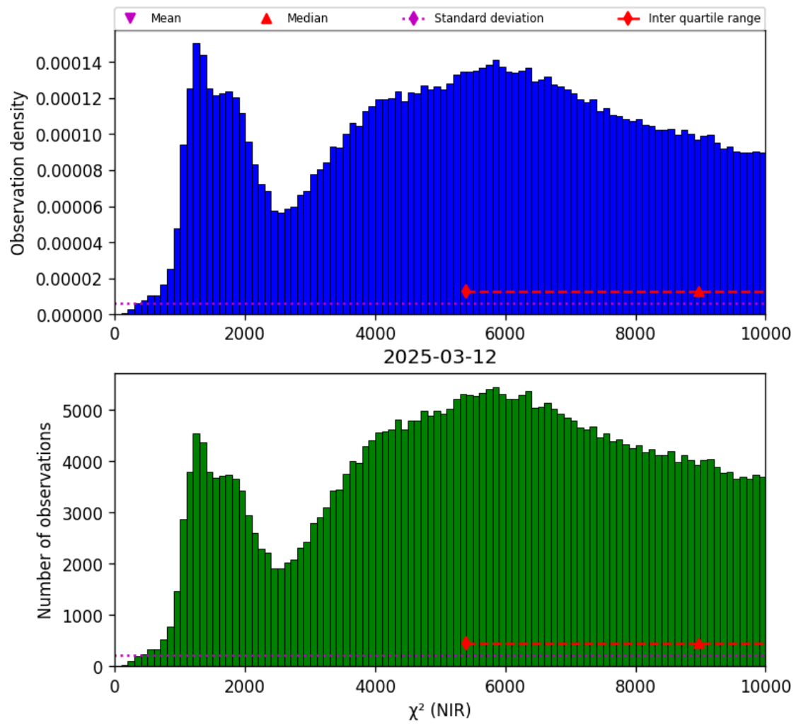
Figure 29: Histogram of “ \chi^2 (NIR)” for 2025-03-12 to 2025-03-13
