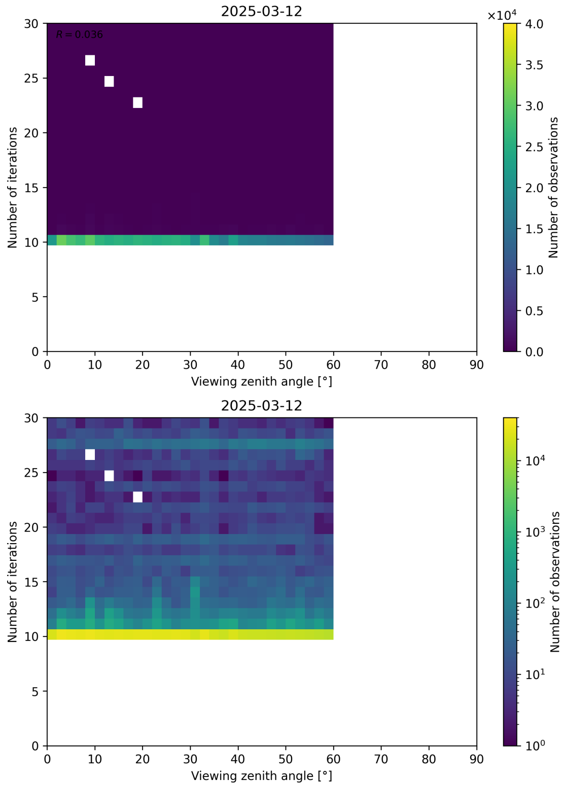
Figure 113: Scatter density plot of “Viewing zenith angle” against “Number of iterations” for 2025-03-12 to 2025-03-13.
