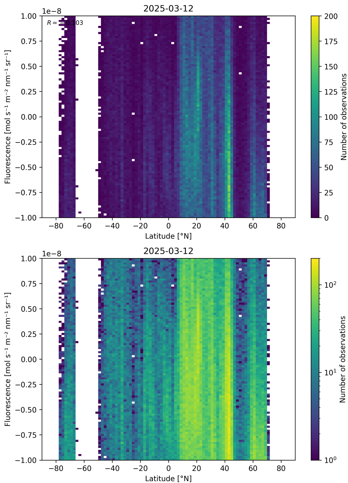
Figure 56: Scatter density plot of “Latitude” against “Fluorescence” for 2025-03-12 to 2025-03-13.
