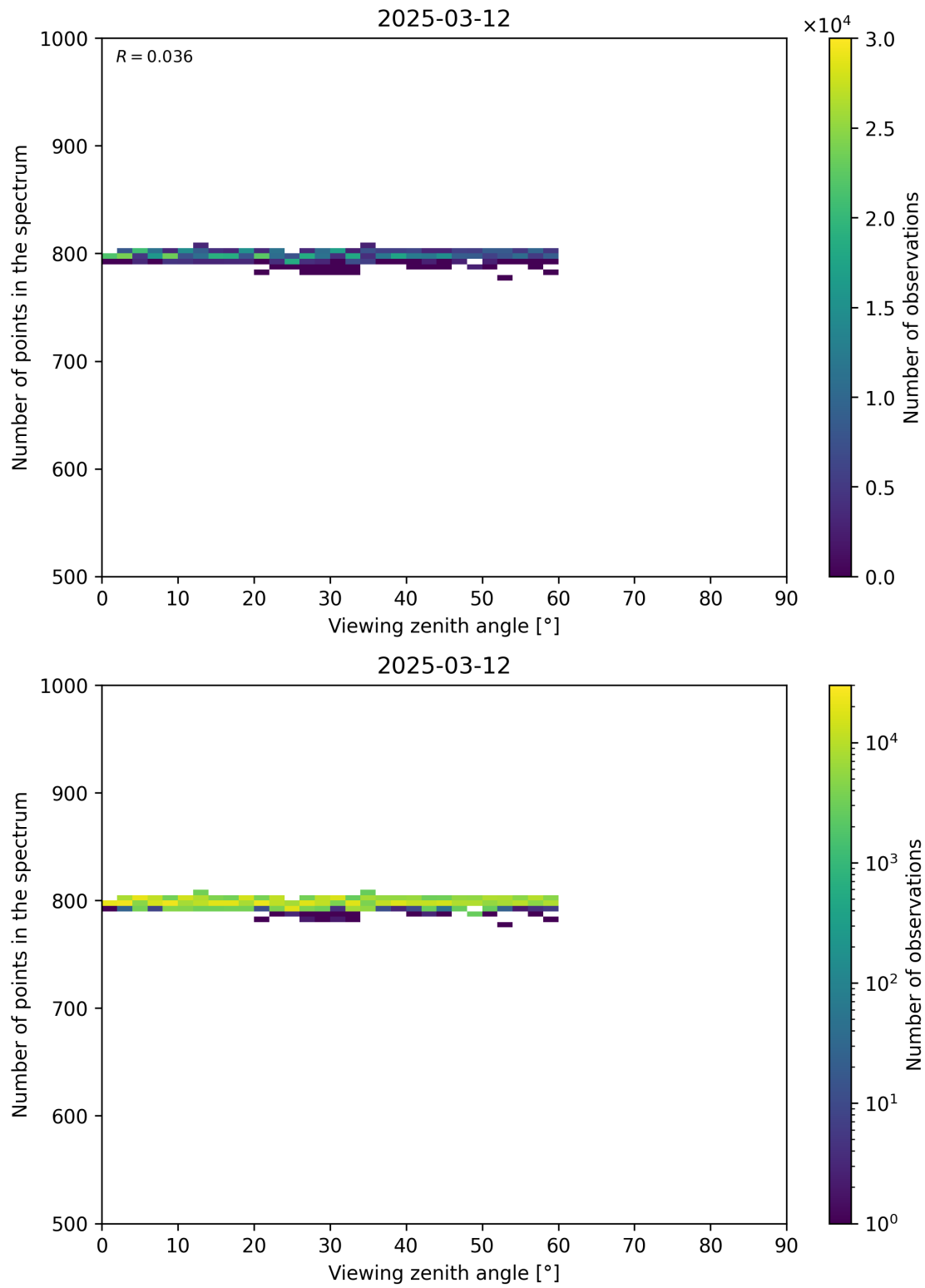
Figure 114: Scatter density plot of “Viewing zenith angle” against “Number of points in the spectrum” for 2025-03-12 to 2025-03-13.
