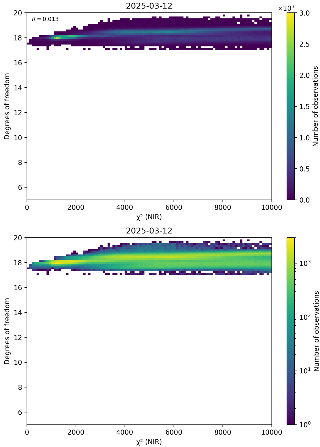
Figure 44: Scatter density plot of “ \chi^2 (NIR)” against “Degrees of freedom” for 2025-03-12 to 2025-03-13.
