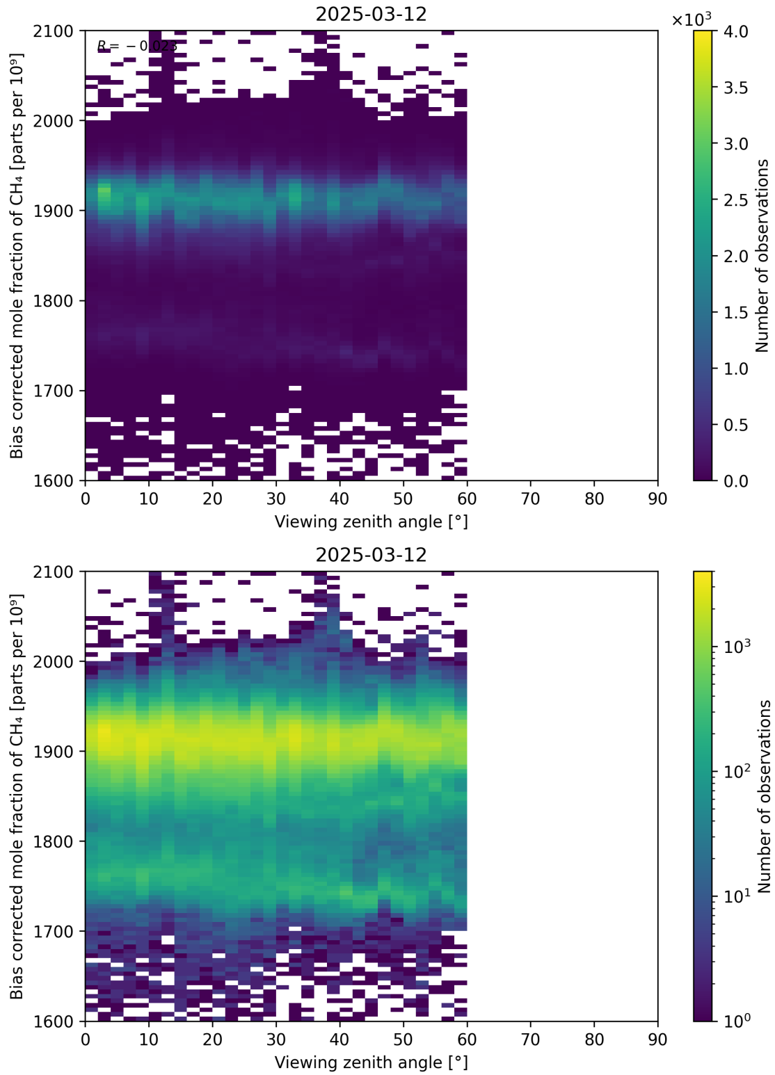
Figure 111: Scatter density plot of “Viewing zenith angle” against “Bias corrected mole fraction of CH 4 ” for 2025-03-12 to 2025-03-13.
