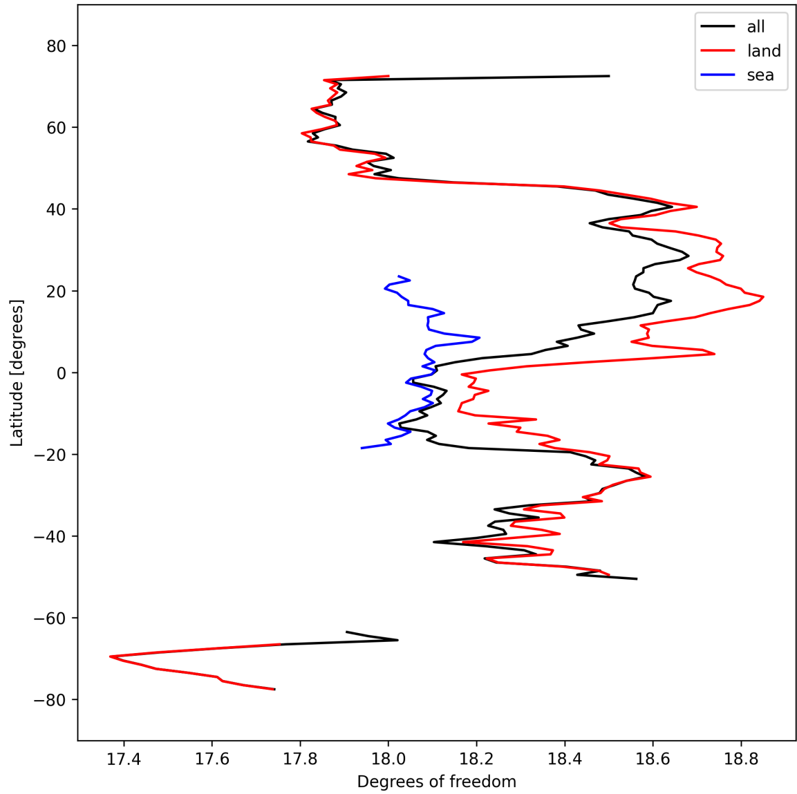
Figure 19: Zonal average of “Degrees of freedom” for 2025-03-12 to 2025-03-13.
