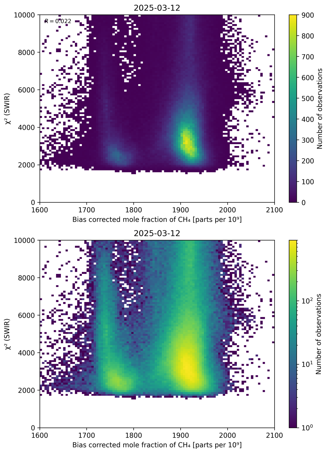
Figure 64: Scatter density plot of “Bias corrected mole fraction of \text{CH}_4 ” against “ \chi^2 (SWIR)” for 2025-03-12 to 2025-03-13.
