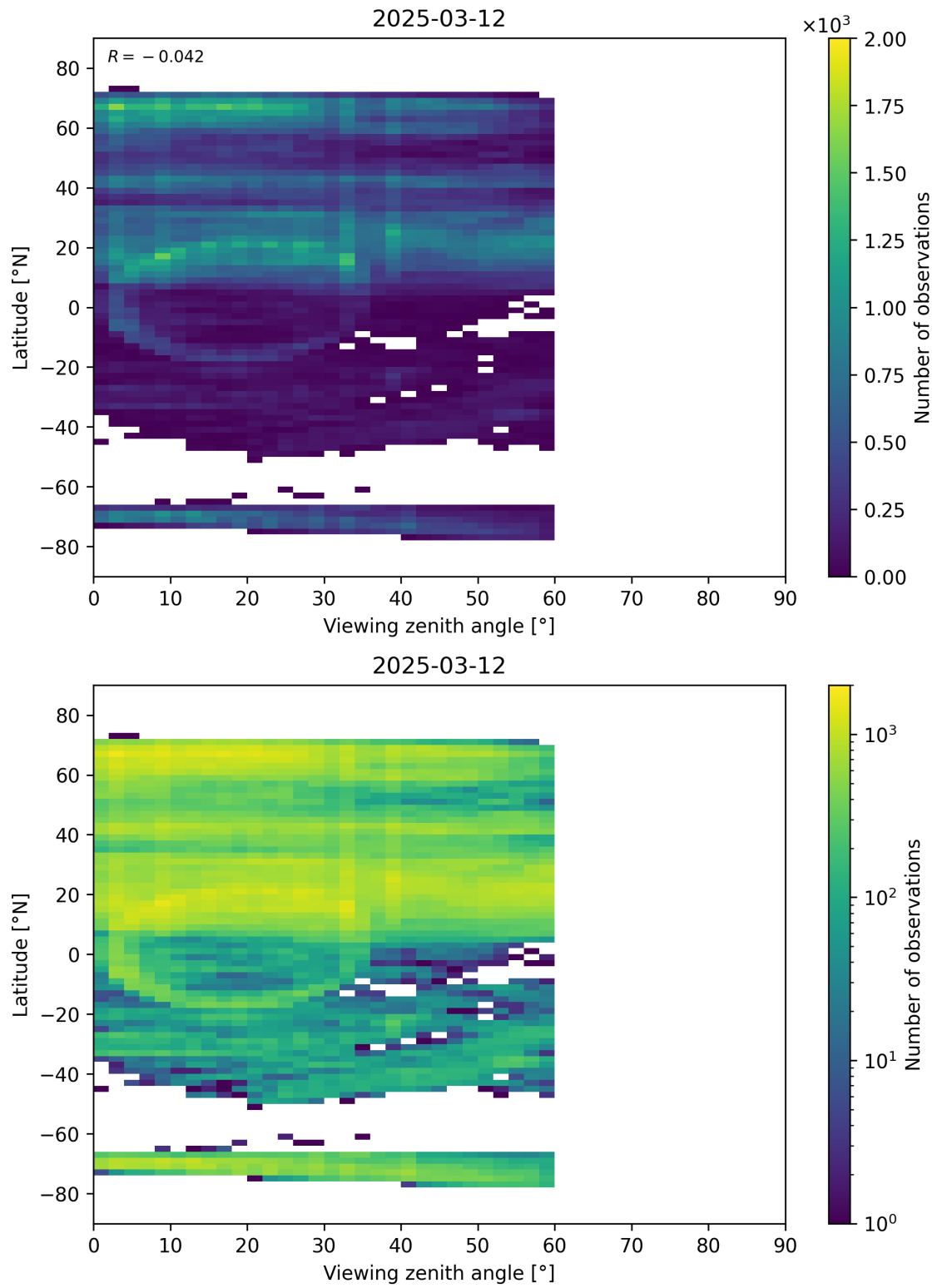
Figure 109: Scatter density plot of “Viewing zenith angle” against “Latitude” for 2025-03-12 to 2025-03-13.
