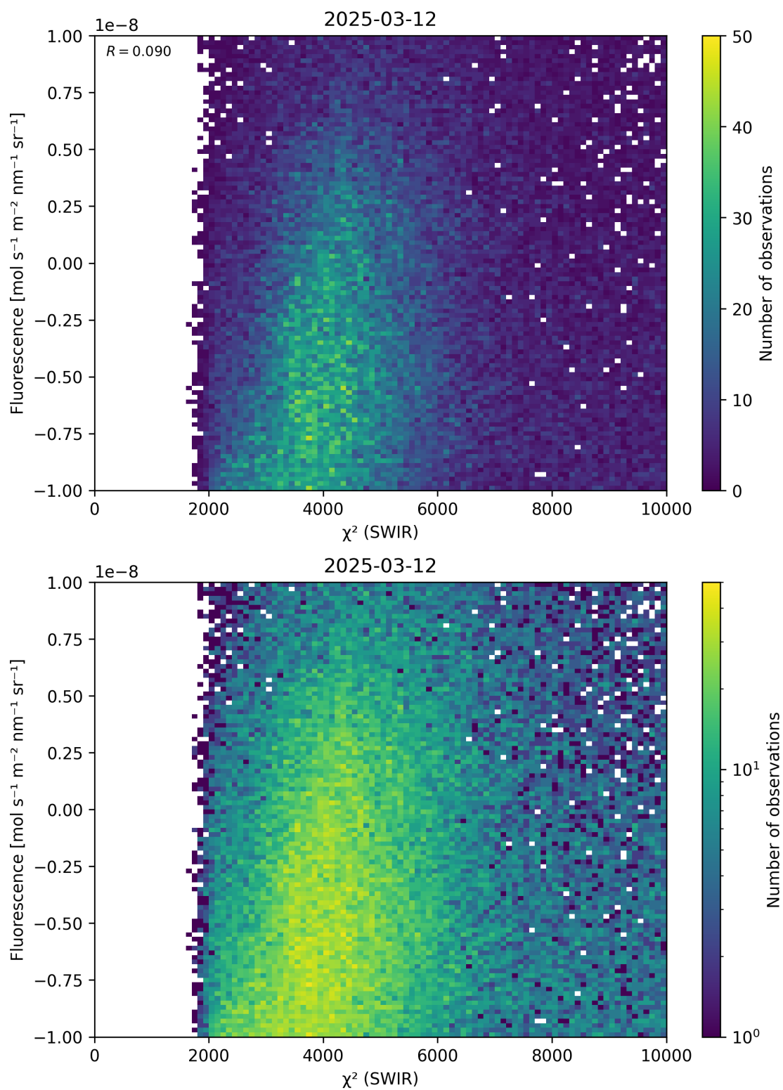
Figure 49: Scatter density plot of “ \chi^2 (SWIR)” against “Fluorescence” for 2025-03-12 to 2025-03-13.
