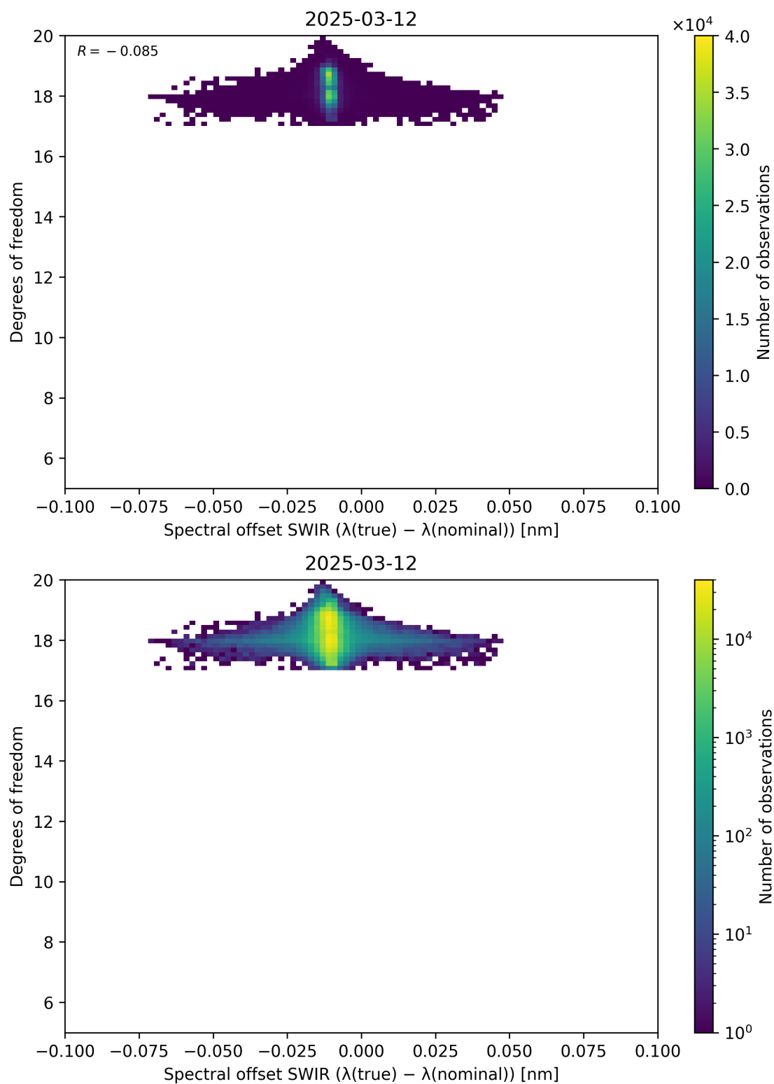
Figure 119: Scatter density plot of “Spectral offset SWIR ( \lambda_{\text{true}} - \lambda_{\text{nominal}} )” against “Degrees of freedom” for 2025-03-12 to 2025-03-13.
