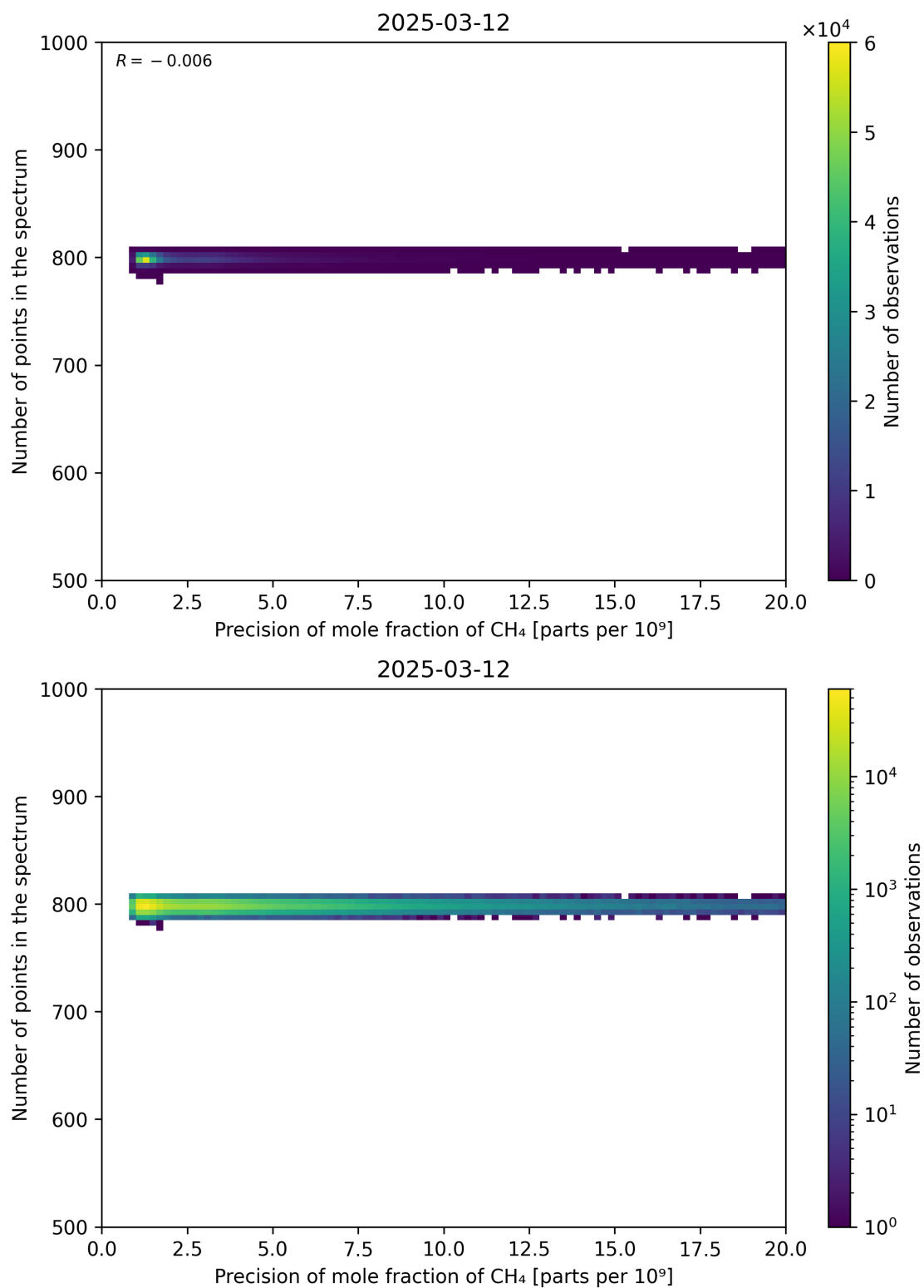
Figure 84: Scatter density plot of “Precision of mole fraction of CH 4 ” against “Number of points in the spectrum” for 2025-03-12 to 2025-03-13.
