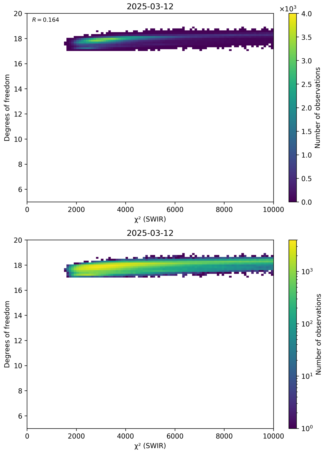
Figure 48: Scatter density plot of " \chi^2 (SWIR)" against "Degrees of freedom" for 2025-03-12 to 2025-03-13.
