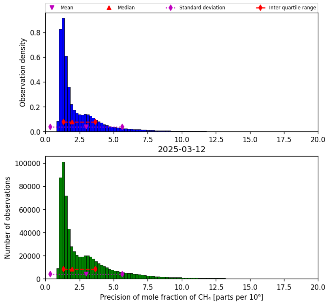
Figure 24: Histogram of “Precision of mole fraction of CH 4 ” for 2025-03-12 to 2025-03-13
