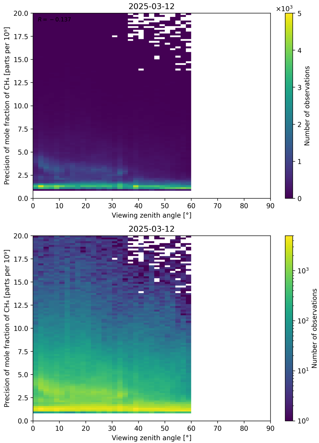
Figure 112: Scatter density plot of “Viewing zenith angle” against “Precision of mole fraction of CH 4 ” for 2025-03-12 to 2025-03-13.
