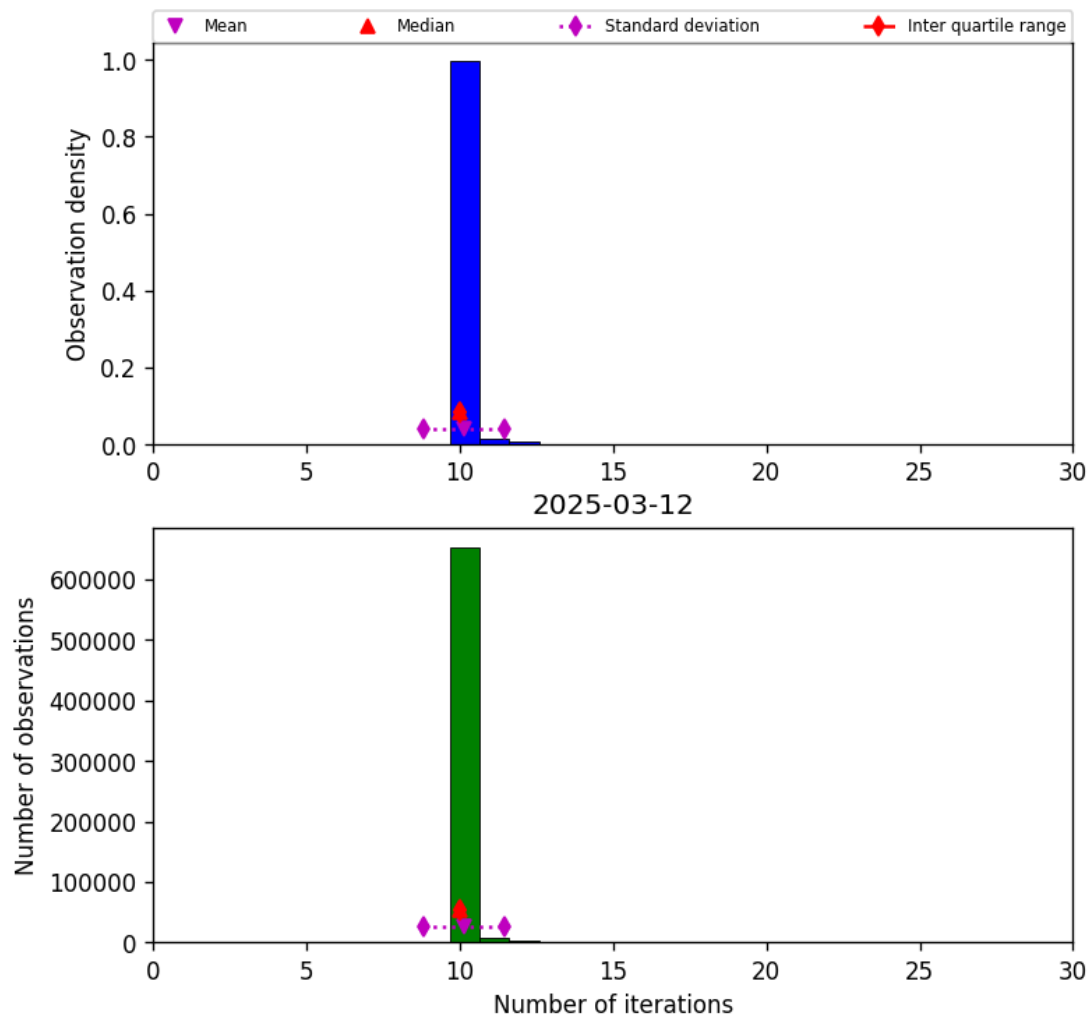
Figure 31: Histogram of “Number of iterations” for 2025-03-12 to 2025-03-13
