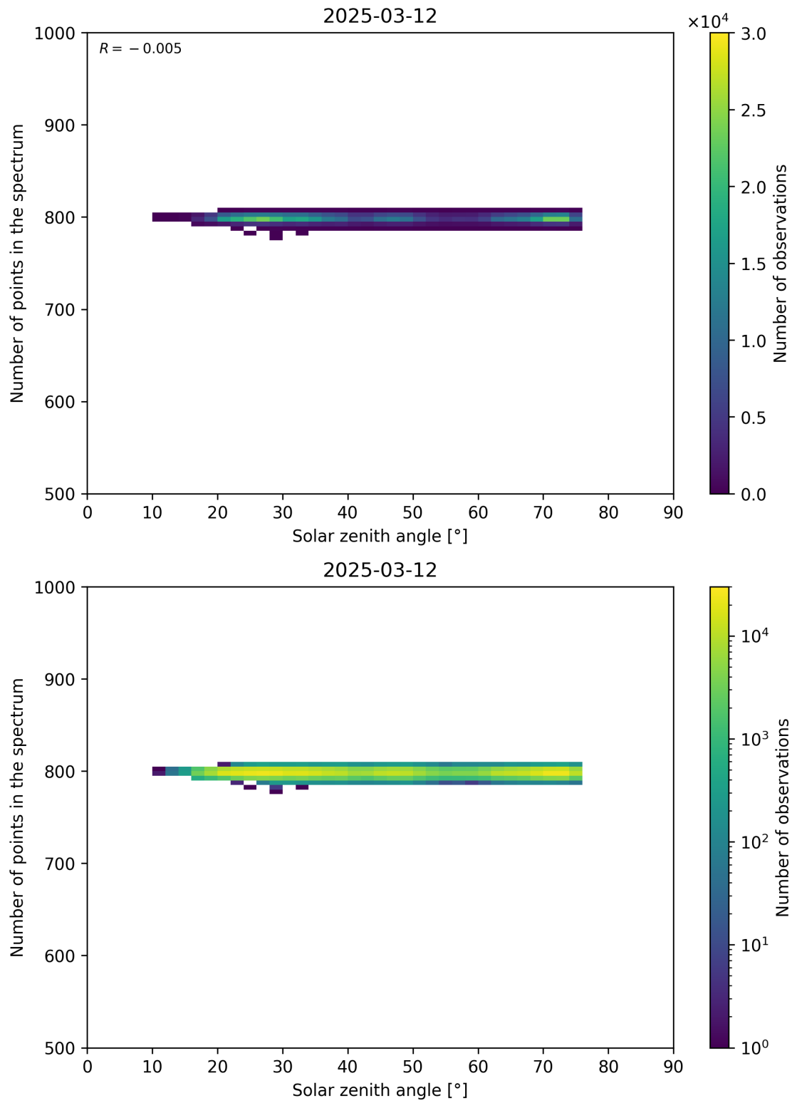
Figure 103: Scatter density plot of “Solar zenith angle” against “Number of points in the spectrum” for 2025-03-12 to 2025-03-13.
