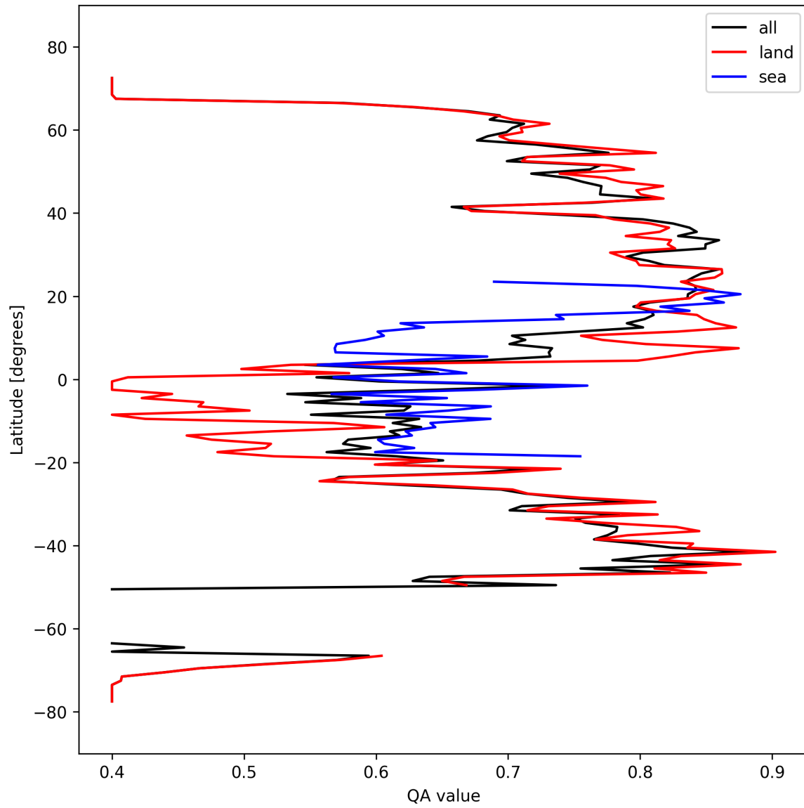
Figure 11: Zonal average of “QA value” for 2025-03-12 to 2025-03-13.
