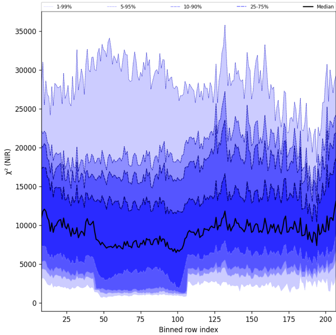
Figure 40: Along track statistics of “ \chi^2 (NIR)” for 2025-03-12 to 2025-03-13
