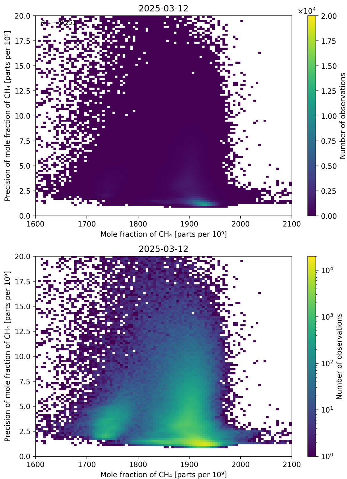
Figure 75: Scatter density plot of “Mole fraction of CH 4 ” against “Precision of mole fraction of CH 4 ” for 2025-03-12 to 2025-03-13.
