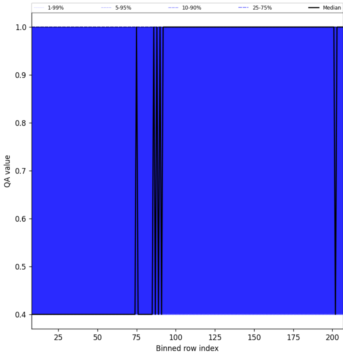
Figure 33: Along track statistics of “QA value” for 2025-03-12 to 2025-03-13
