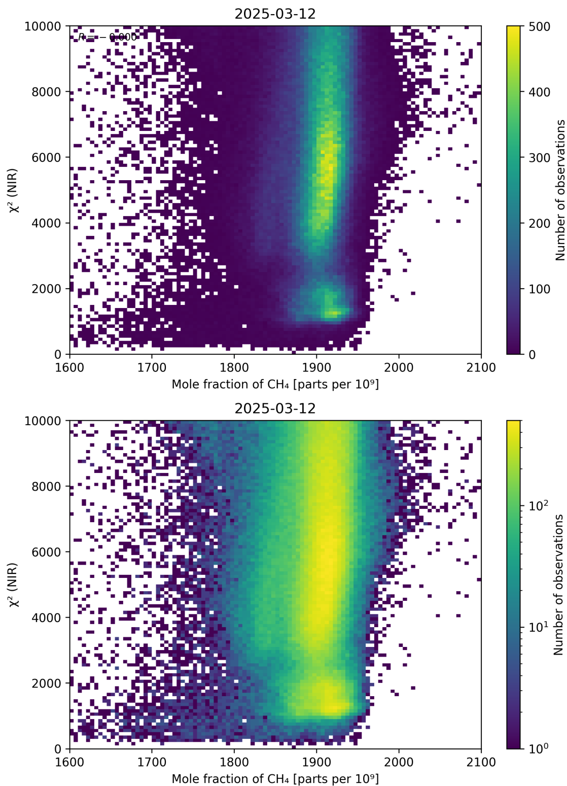
Figure 70: Scatter density plot of “Mole fraction of \text{CH}_4 ” against “ \chi^2 (NIR)” for 2025-03-12 to 2025-03-13.
