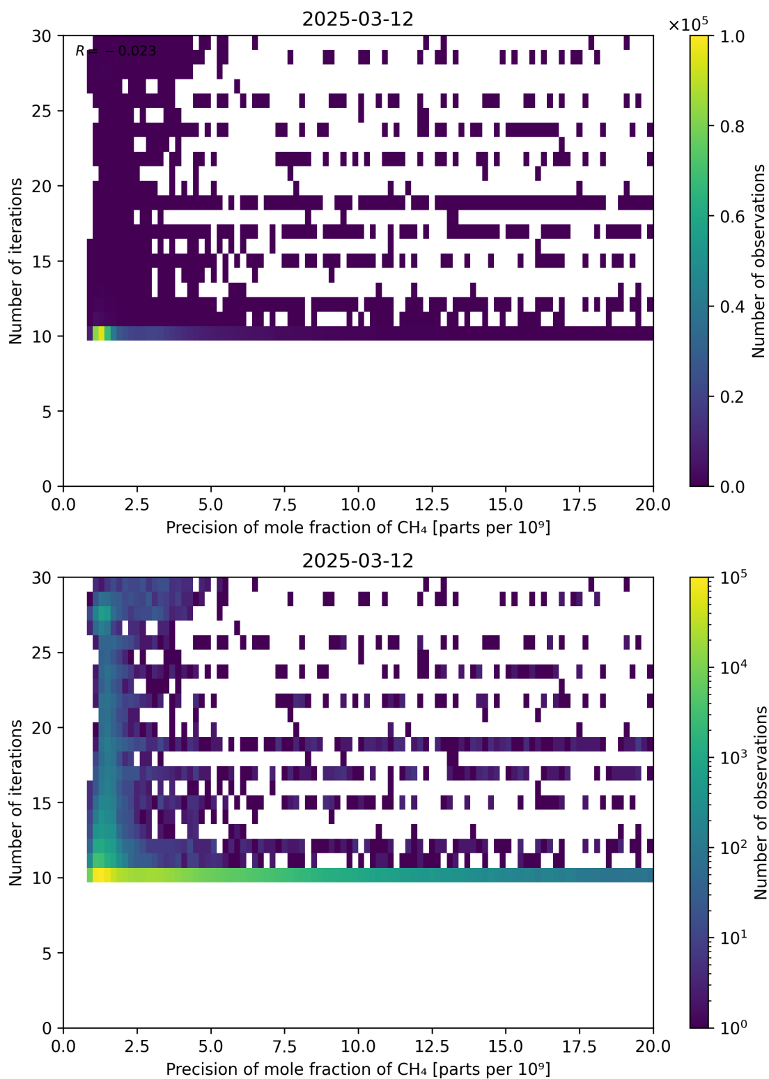
Figure 83: Scatter density plot of “Precision of mole fraction of CH 4 ” against “Number of iterations” for 2025-03-12 to 2025-03-13.
