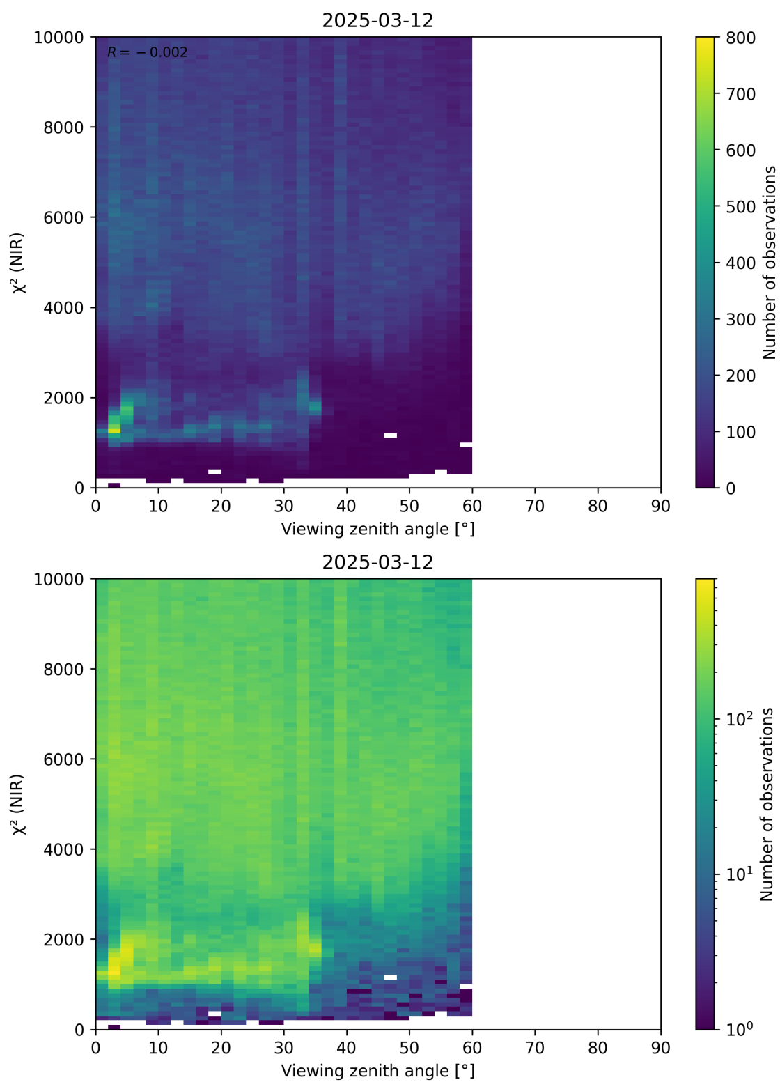
Figure 105: Scatter density plot of “Viewing zenith angle” against “ \chi^2 (NIR)” for 2025-03-12 to 2025-03-13.
