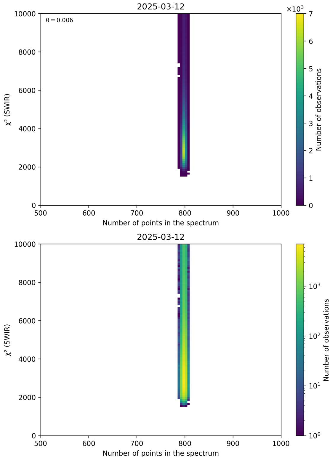
Figure 89: Scatter density plot of “Number of points in the spectrum” against “ \chi^2 (SWIR)” for 2025-03-12 to 2025-03-13.
