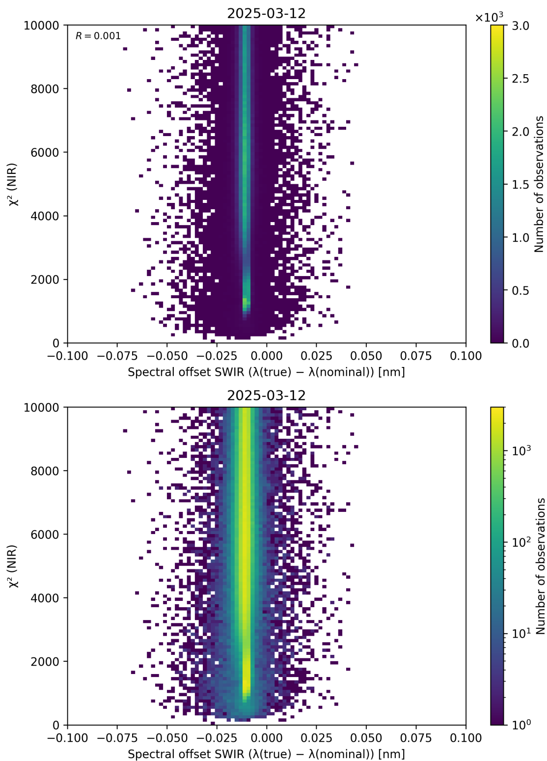
Figure 117: Scatter density plot of “Spectral offset SWIR ( \lambda_{\text{true}} - \lambda_{\text{nominal}} )” against “ \chi^2 (NIR)” for 2025-03-12 to 2025-03-13.
