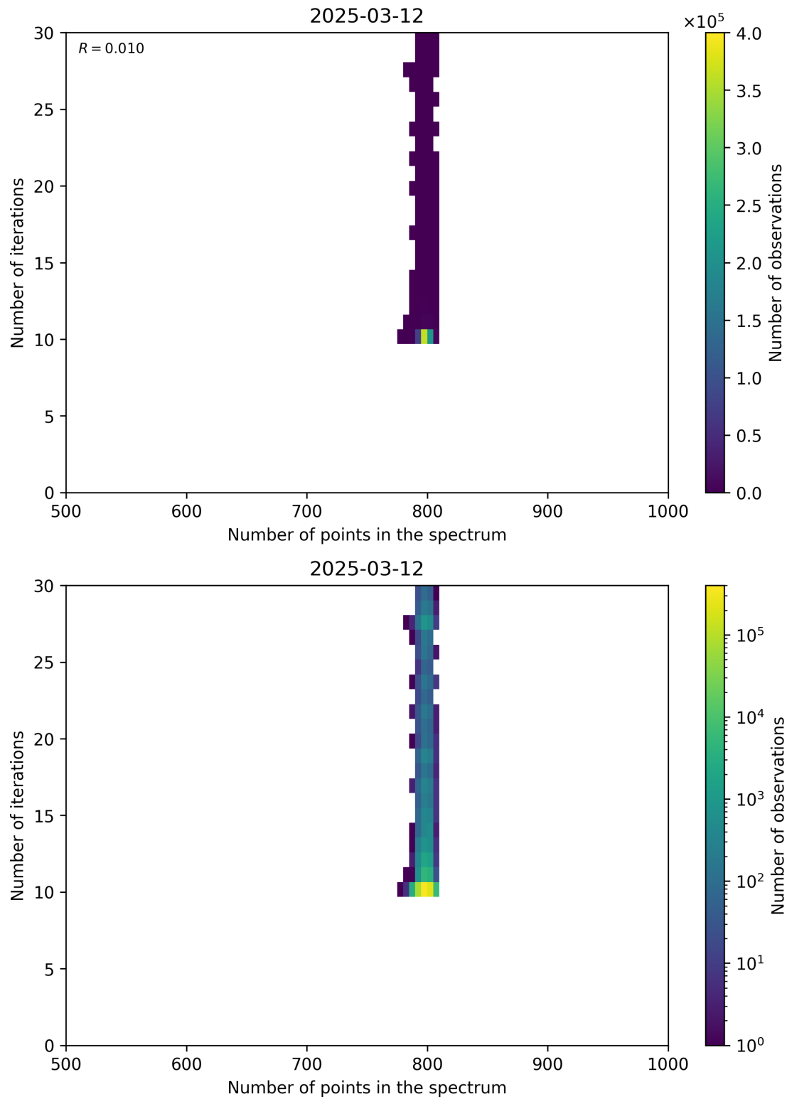
Figure 92: Scatter density plot of “Number of points in the spectrum” against “Number of iterations” for 2025-03-12 to 2025-03-13.
