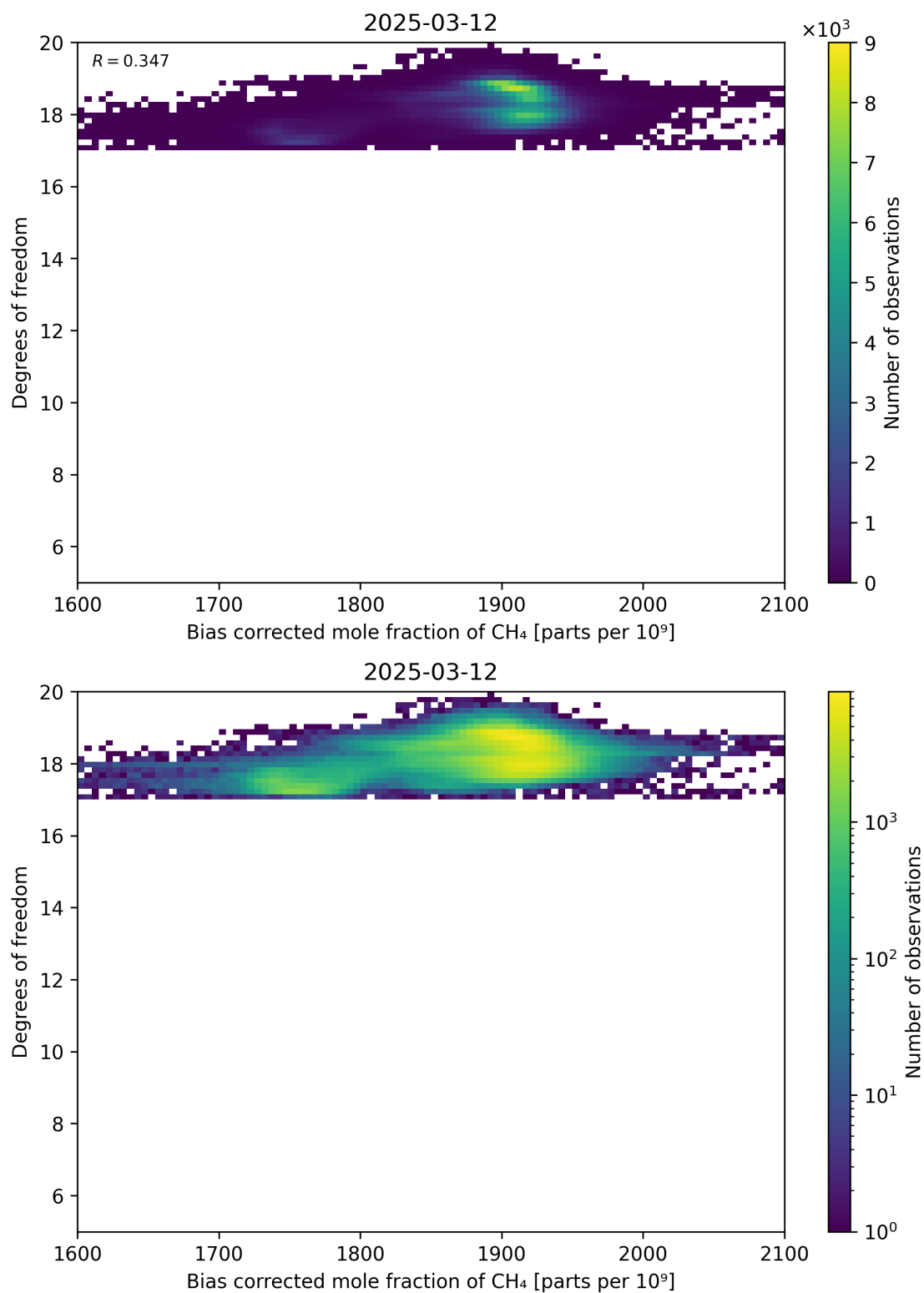
Figure 65: Scatter density plot of “Bias corrected mole fraction of CH 4 ” against “Degrees of freedom” for 2025-03-12 to 2025-03-13.
