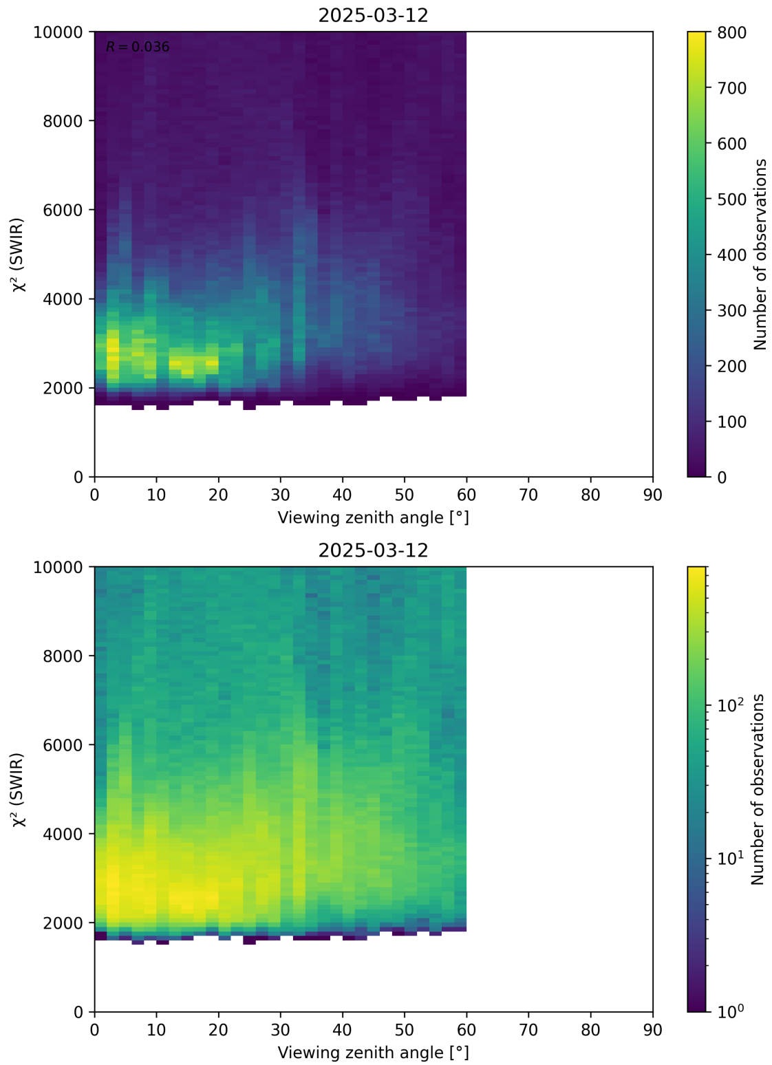
Figure 106: Scatter density plot of “Viewing zenith angle” against “ \chi^2 (SWIR)” for 2025-03-12 to 2025-03-13.
