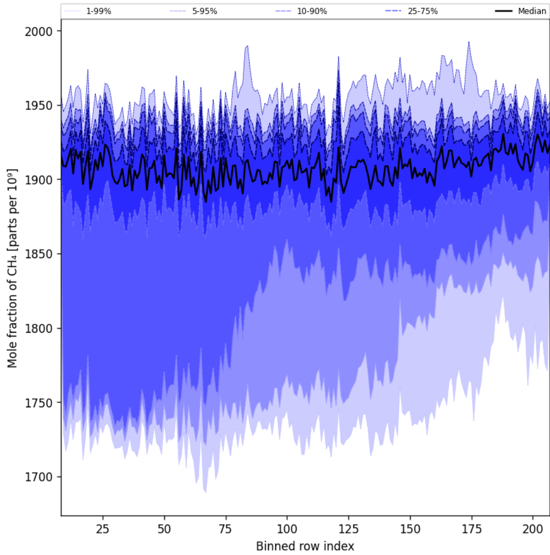
Figure 34: Along track statistics of “Mole fraction of CH 4 ” for 2025-03-12 to 2025-03-13
