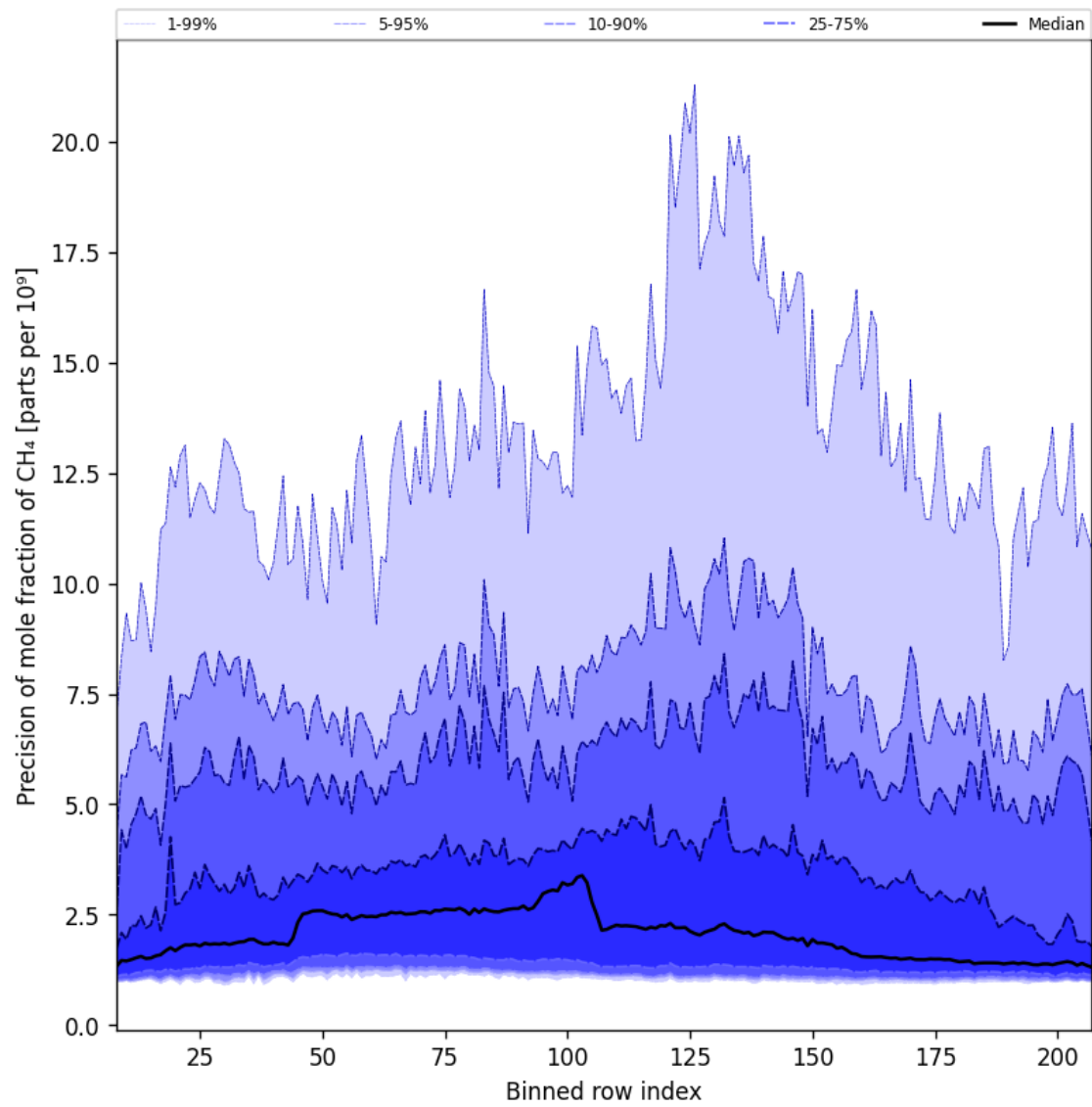
Figure 35: Along track statistics of “Precision of mole fraction of CH 4 ” for 2025-03-12 to 2025-03-13
