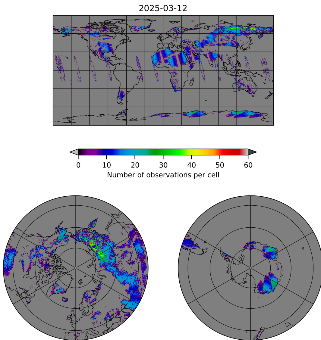
Figure 10: Map of the number of observations for 2025-03-12 to 2025-03-13
