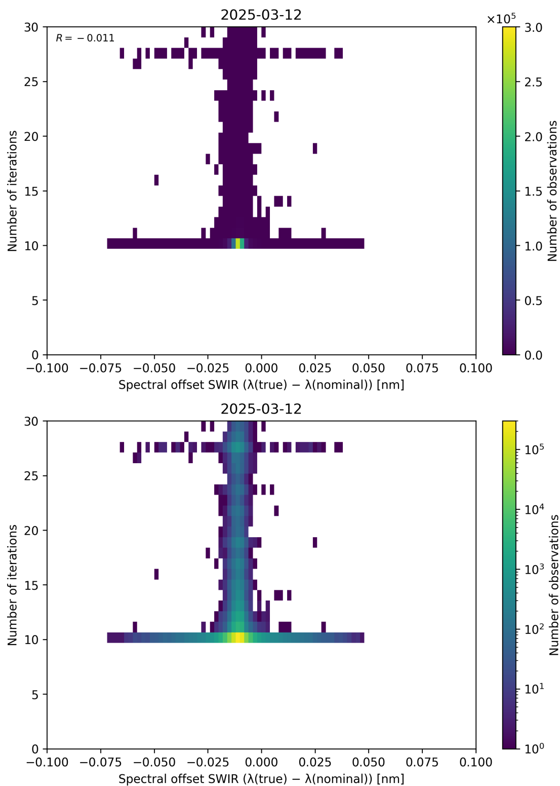
Figure 121: Scatter density plot of “Spectral offset SWIR ( \lambda_{\text{true}} - \lambda_{\text{nominal}} )” against “Number of iterations” for 2025-03-12 to 2025-03-13.
