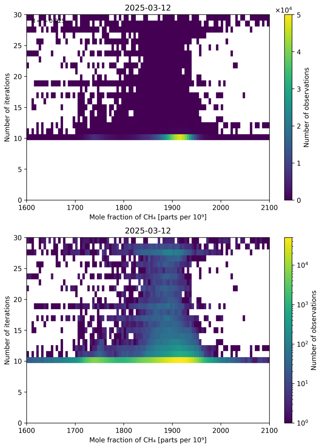
Figure 76: Scatter density plot of “Mole fraction of CH 4 ” against “Number of iterations” for 2025-03-12 to 2025-03-13.
