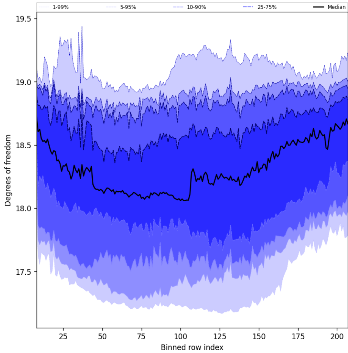
Figure 41: Along track statistics of “Degrees of freedom” for 2025-03-12 to 2025-03-13
