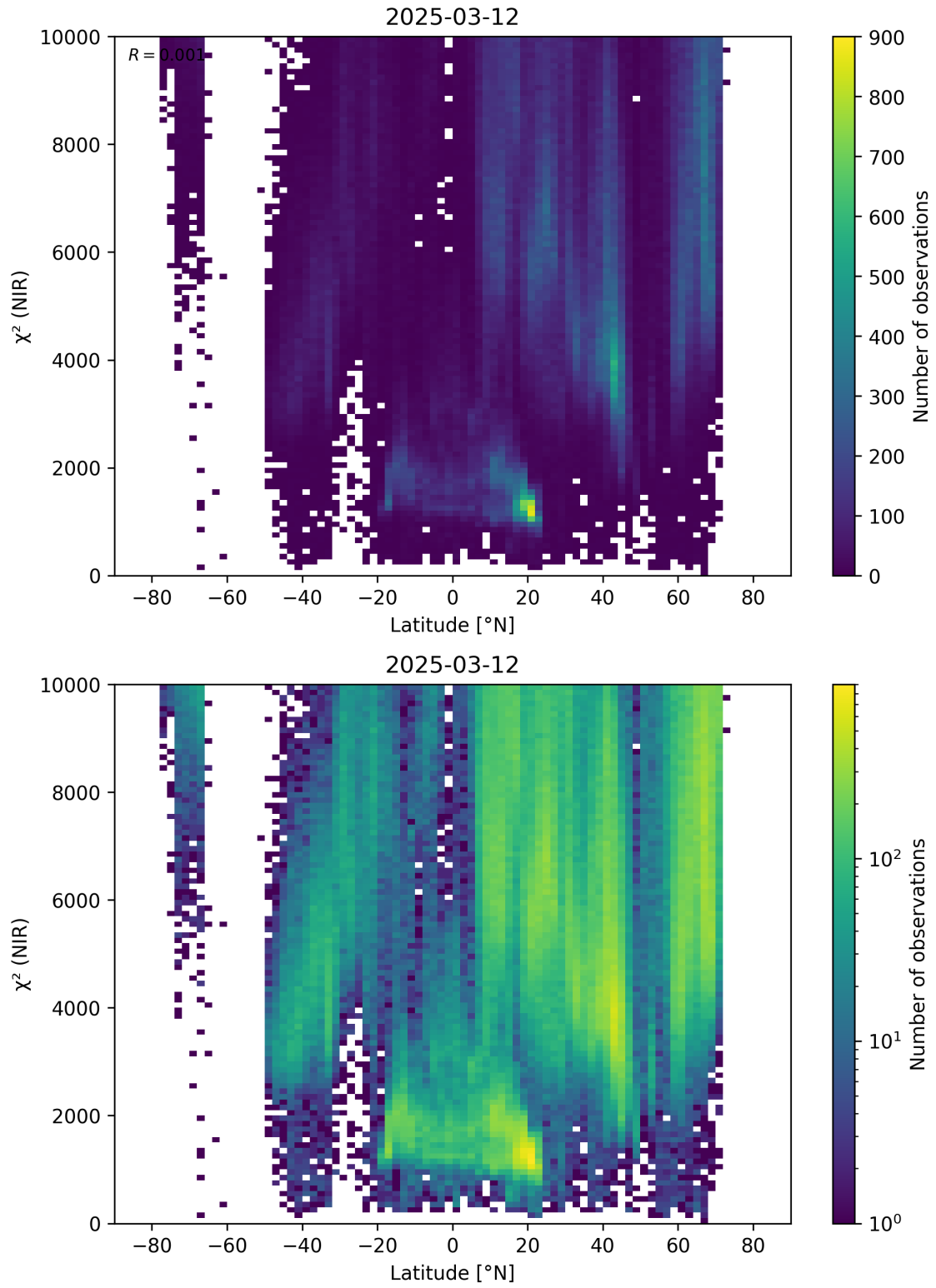
Figure 53: Scatter density plot of “Latitude” against “ \chi^2 (NIR)” for 2025-03-12 to 2025-03-13.
