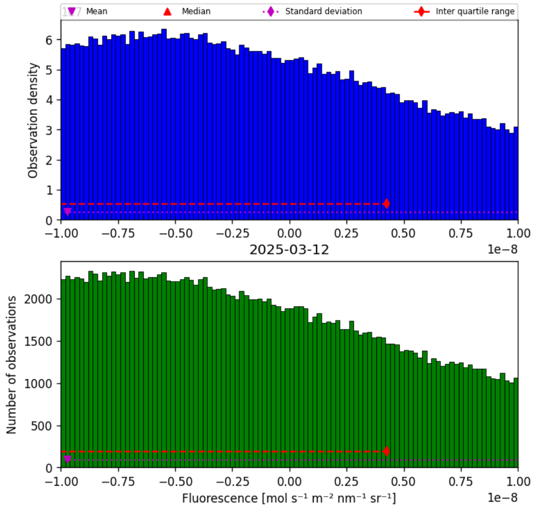
Figure 32: Histogram of “Fluorescence” for 2025-03-12 to 2025-03-13
