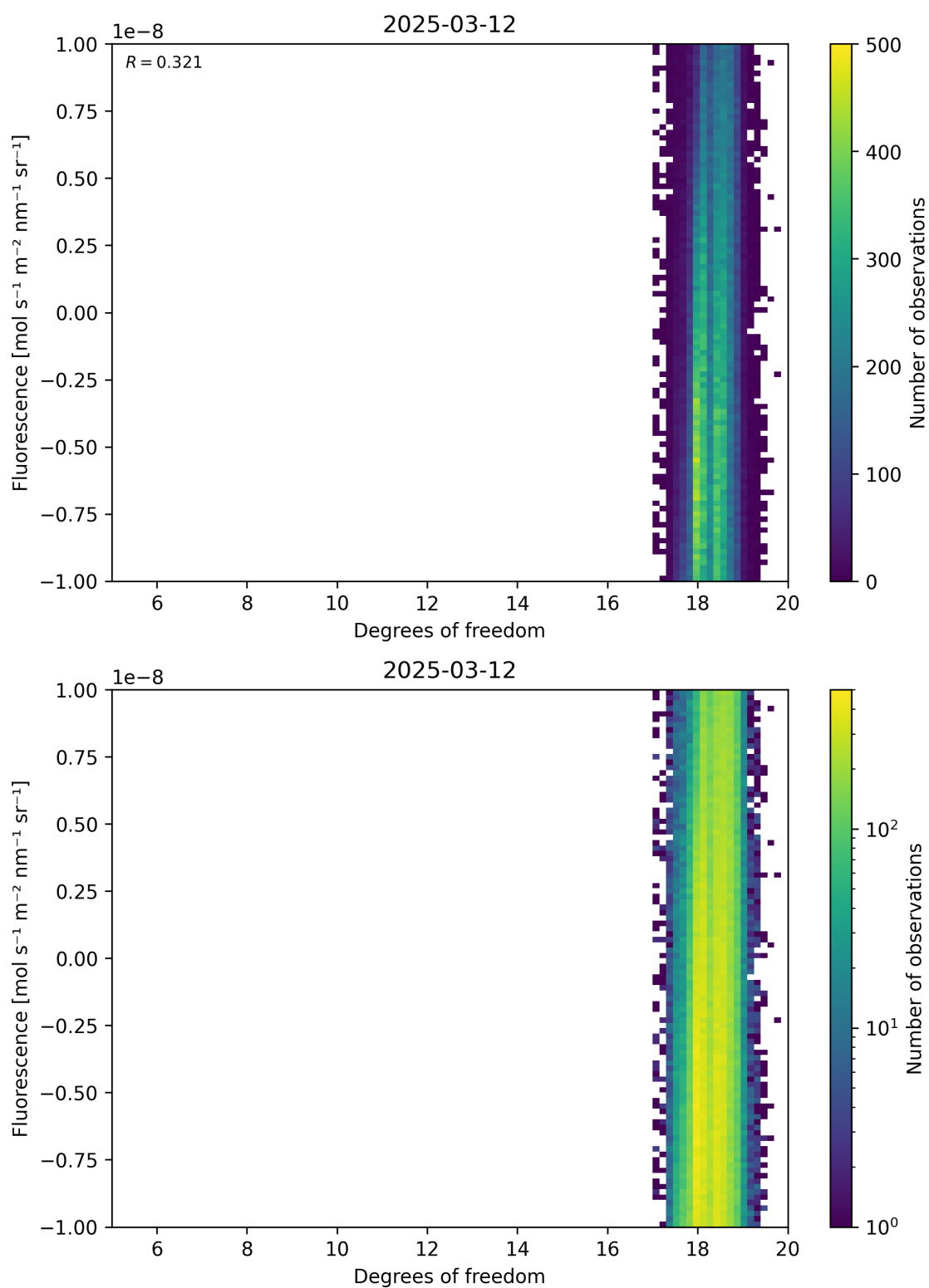
Figure 51: Scatter density plot of “Degrees of freedom” against “Fluorescence” for 2025-03-12 to 2025-03-13.
