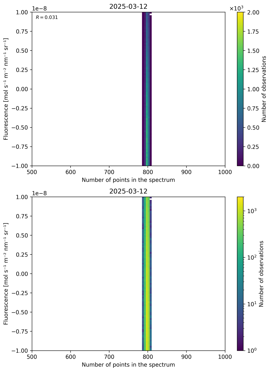
Figure 91: Scatter density plot of “Number of points in the spectrum” against “Fluorescence” for 2025-03-12 to 2025-03-13.
