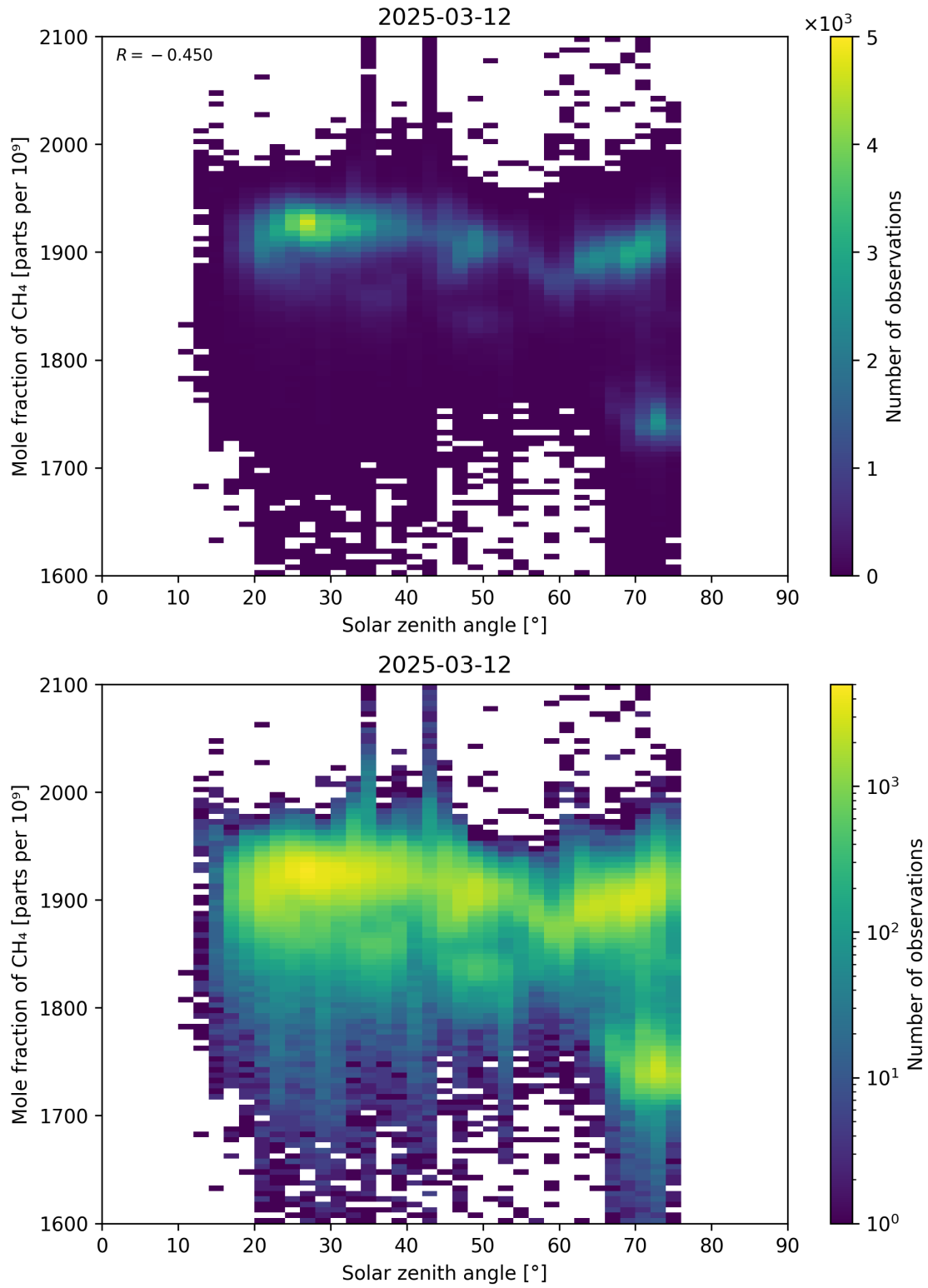
Figure 99: Scatter density plot of “Solar zenith angle” against “Mole fraction of CH 4 ” for 2025-03-12 to 2025-03-13.
