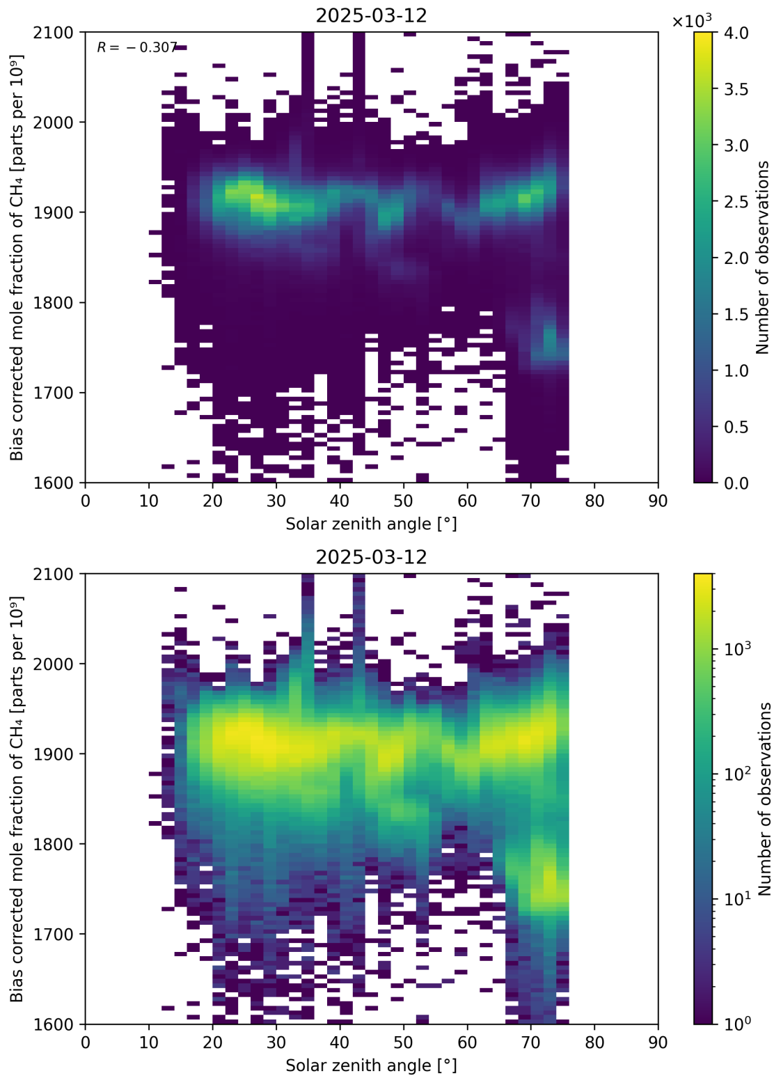
Figure 100: Scatter density plot of “Solar zenith angle” against “Bias corrected mole fraction of CH 4 ” for 2025-03-12 to 2025-03-13.
