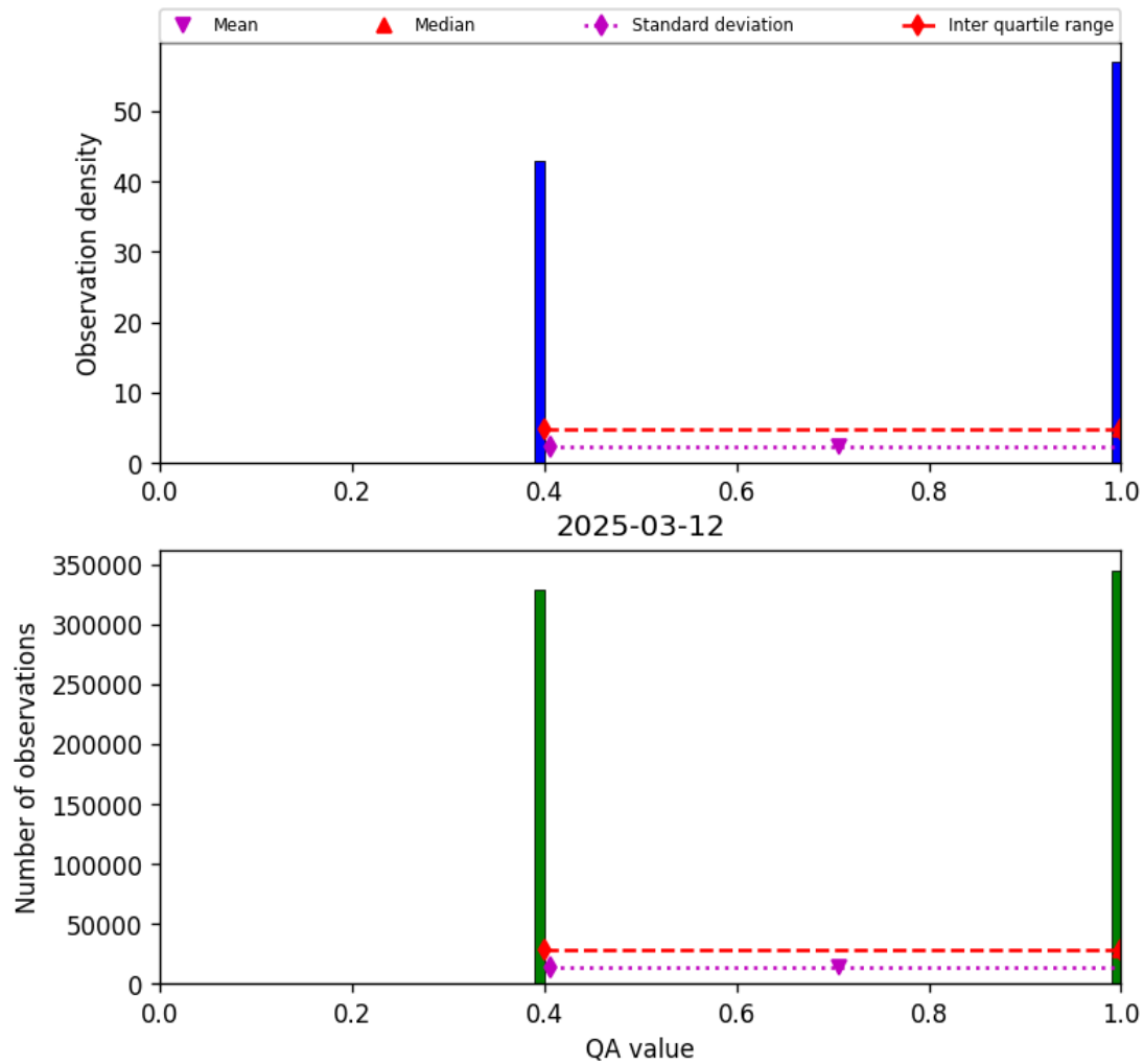
Figure 22: Histogram of “QA value” for 2025-03-12 to 2025-03-13
