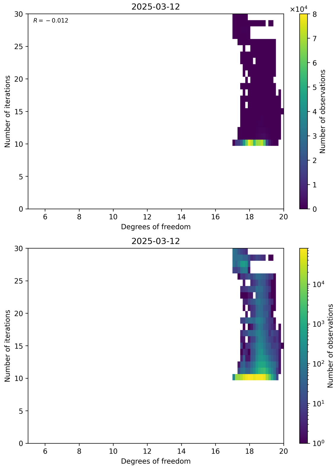
Figure 52: Scatter density plot of “Degrees of freedom” against “Number of iterations” for 2025-03-12 to 2025-03-13.
