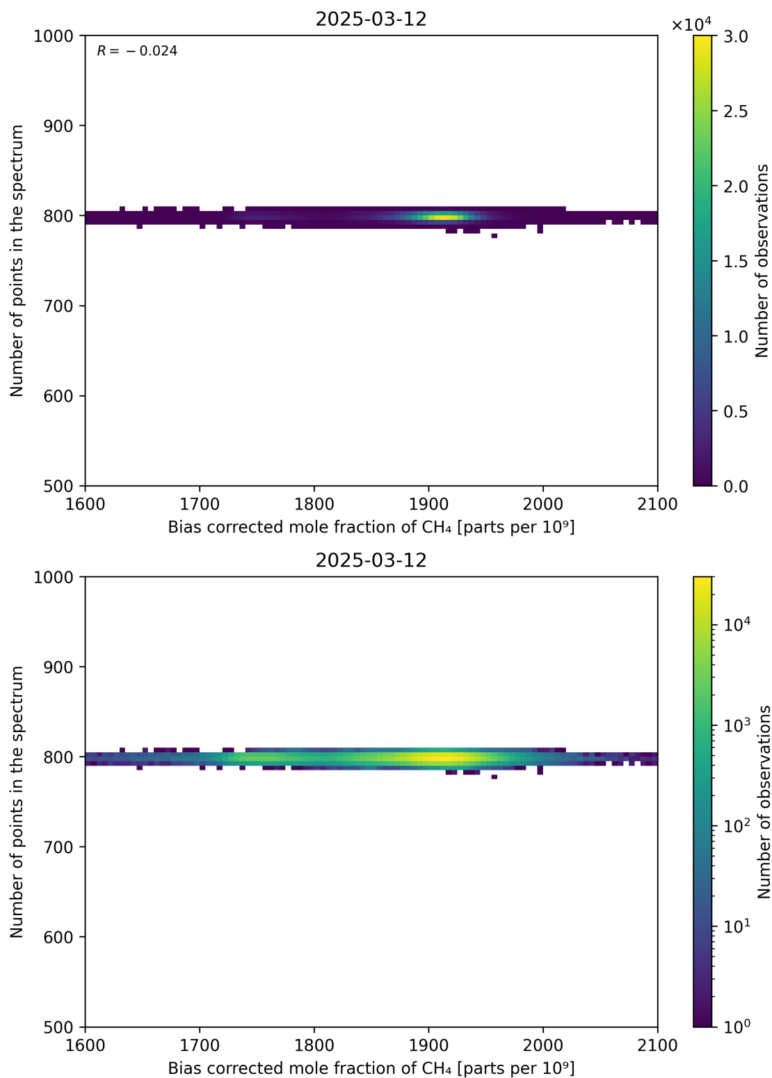
Figure 68: Scatter density plot of “Bias corrected mole fraction of CH 4 ” against “Number of points in the spectrum” for 2025-03-12 to 2025-03-13.
