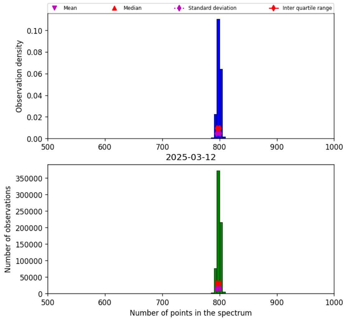
Figure 26: Histogram of “Number of points in the spectrum” for 2025-03-12 to 2025-03-13
