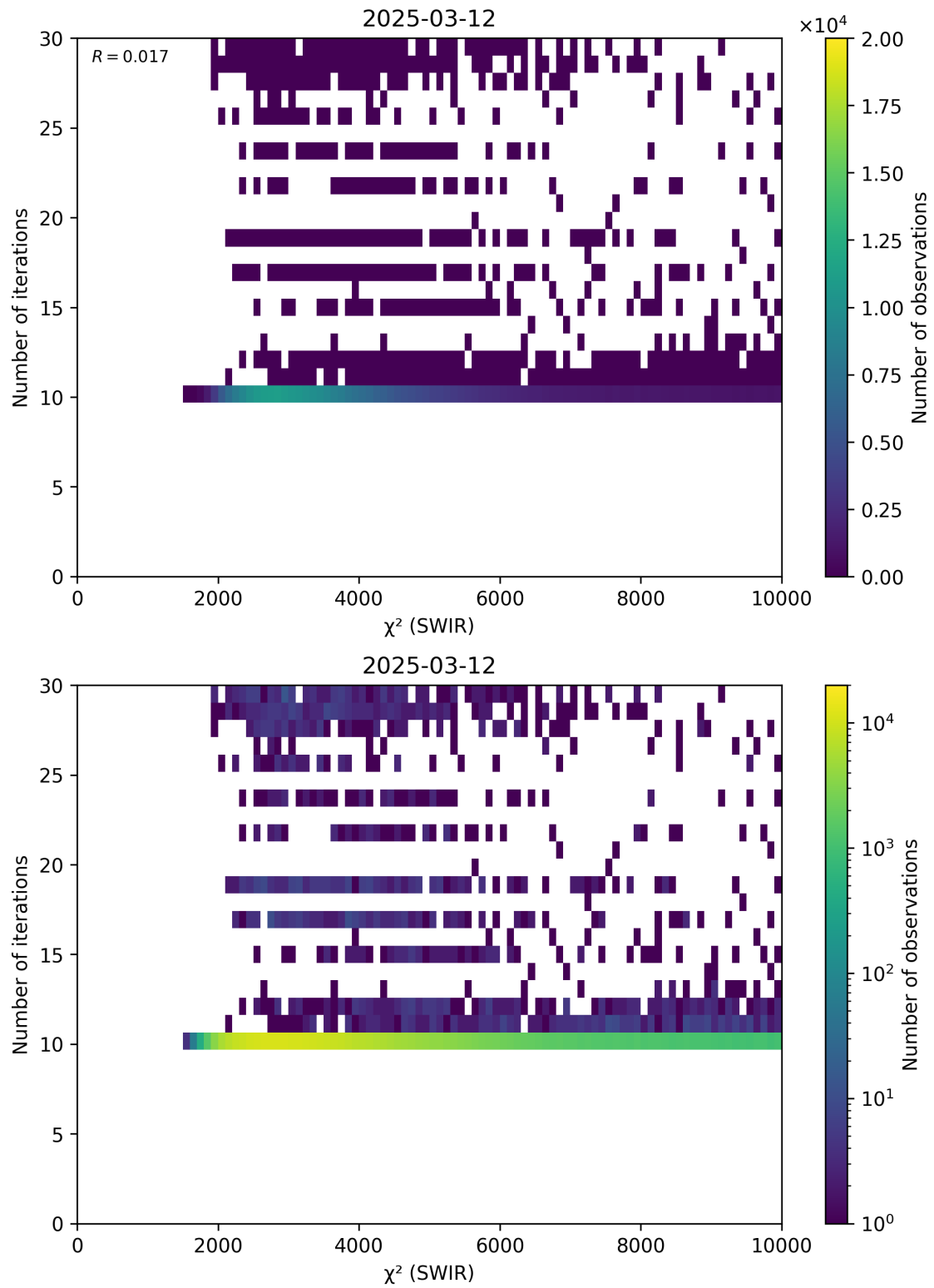
Figure 50: Scatter density plot of “ \chi^2 (SWIR)” against “Number of iterations” for 2025-03-12 to 2025-03-13.
