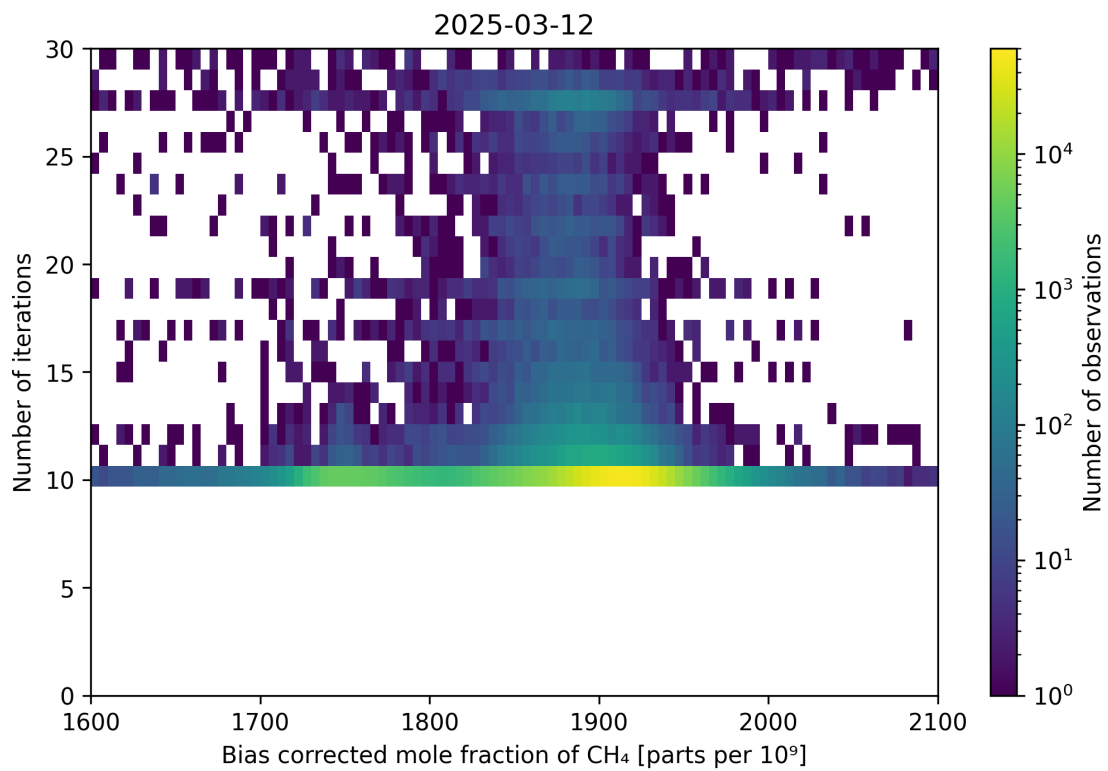
Figure 67: Scatter density plot of “Bias corrected mole fraction of CH 4 ” against “Number of iterations” for 2025-03-12 to 2025-03-13.
