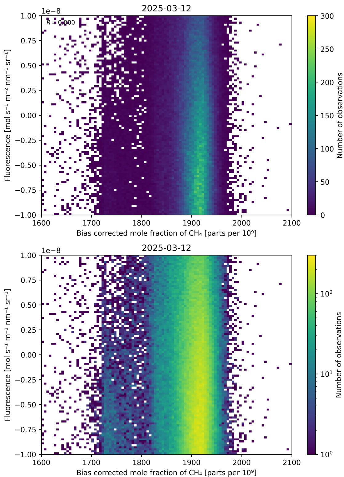
Figure 66: Scatter density plot of “Bias corrected mole fraction of \text{CH}_4 ” against “Fluorescence” for 2025-03-12 to 2025-03-13.
