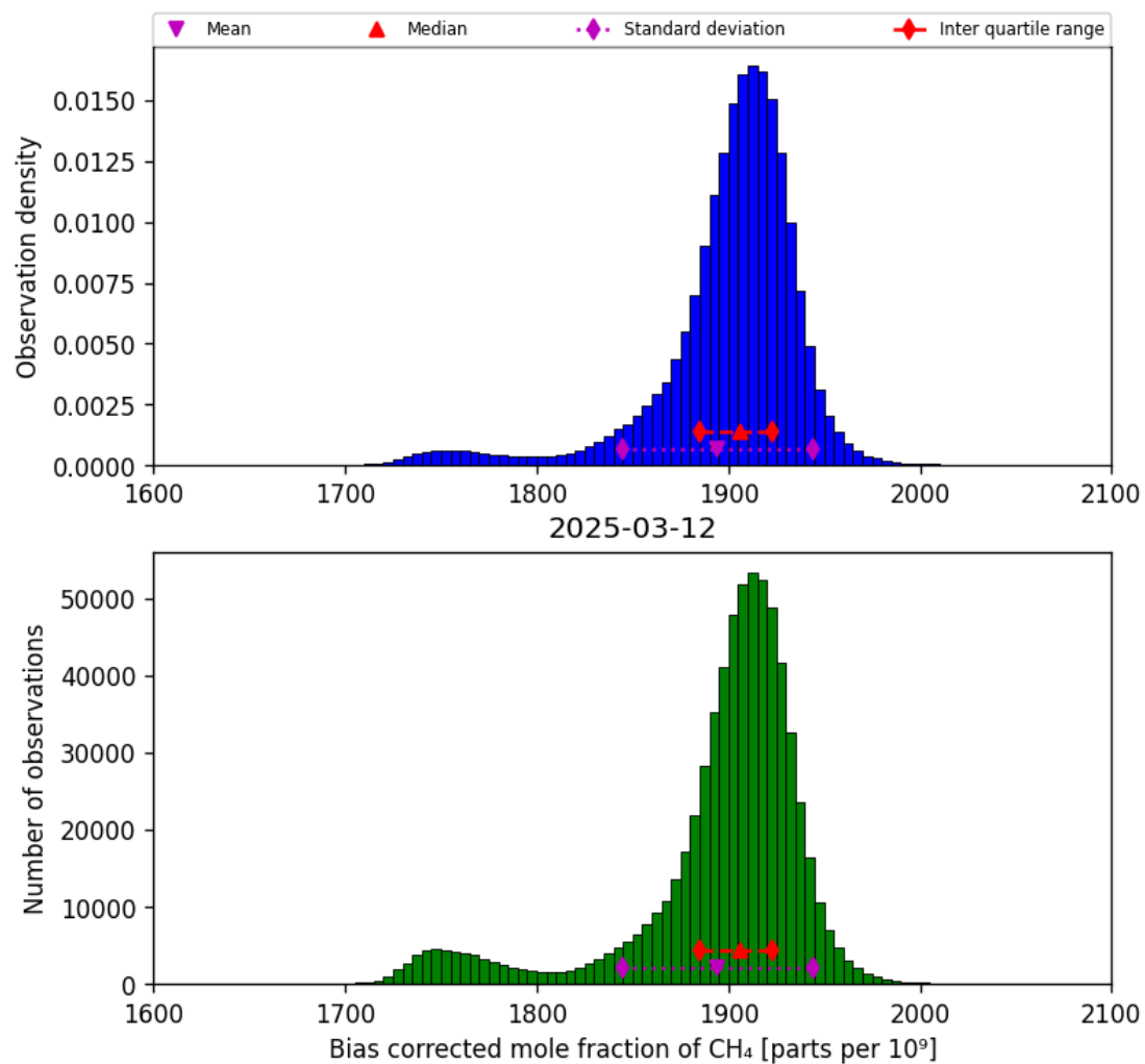
Figure 25: Histogram of “Bias corrected mole fraction of CH 4 ” for 2025-03-12 to 2025-03-13
