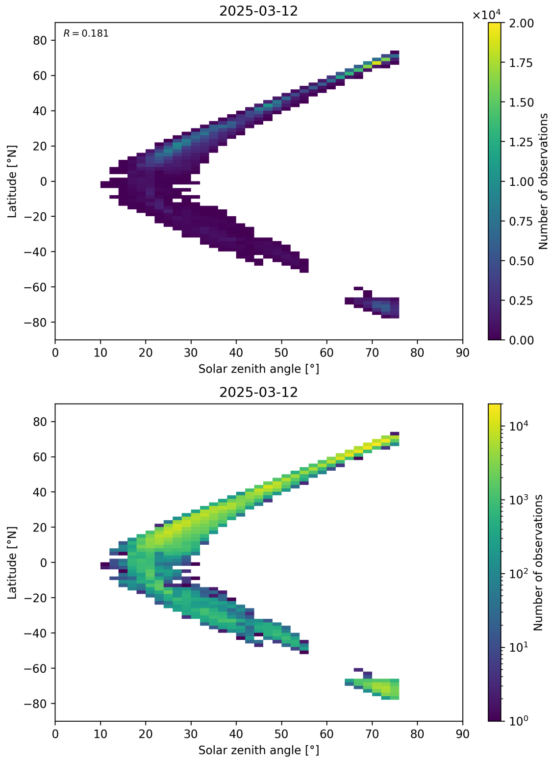
Figure 98: Scatter density plot of “Solar zenith angle” against “Latitude” for 2025-03-12 to 2025-03-13.
