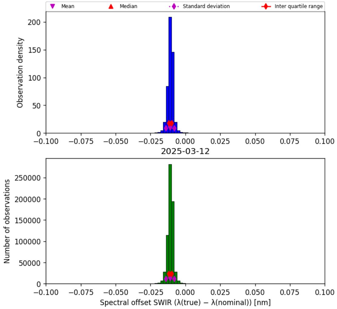
Figure 27: Histogram of “Spectral offset SWIR ( \lambda_{\text{true}} - \lambda_{\text{nominal}} )” for 2025-03-12 to 2025-03-13
