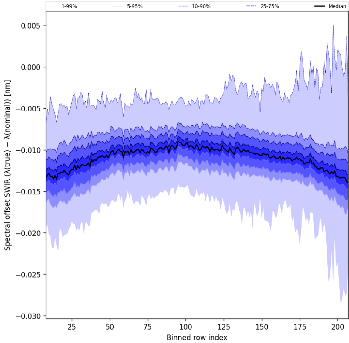
Figure 38: Along track statistics of “Spectral offset SWIR ( \lambda_{\text{true}} - \lambda_{\text{nominal}} )” for 2025-03-12 to 2025-03-13
