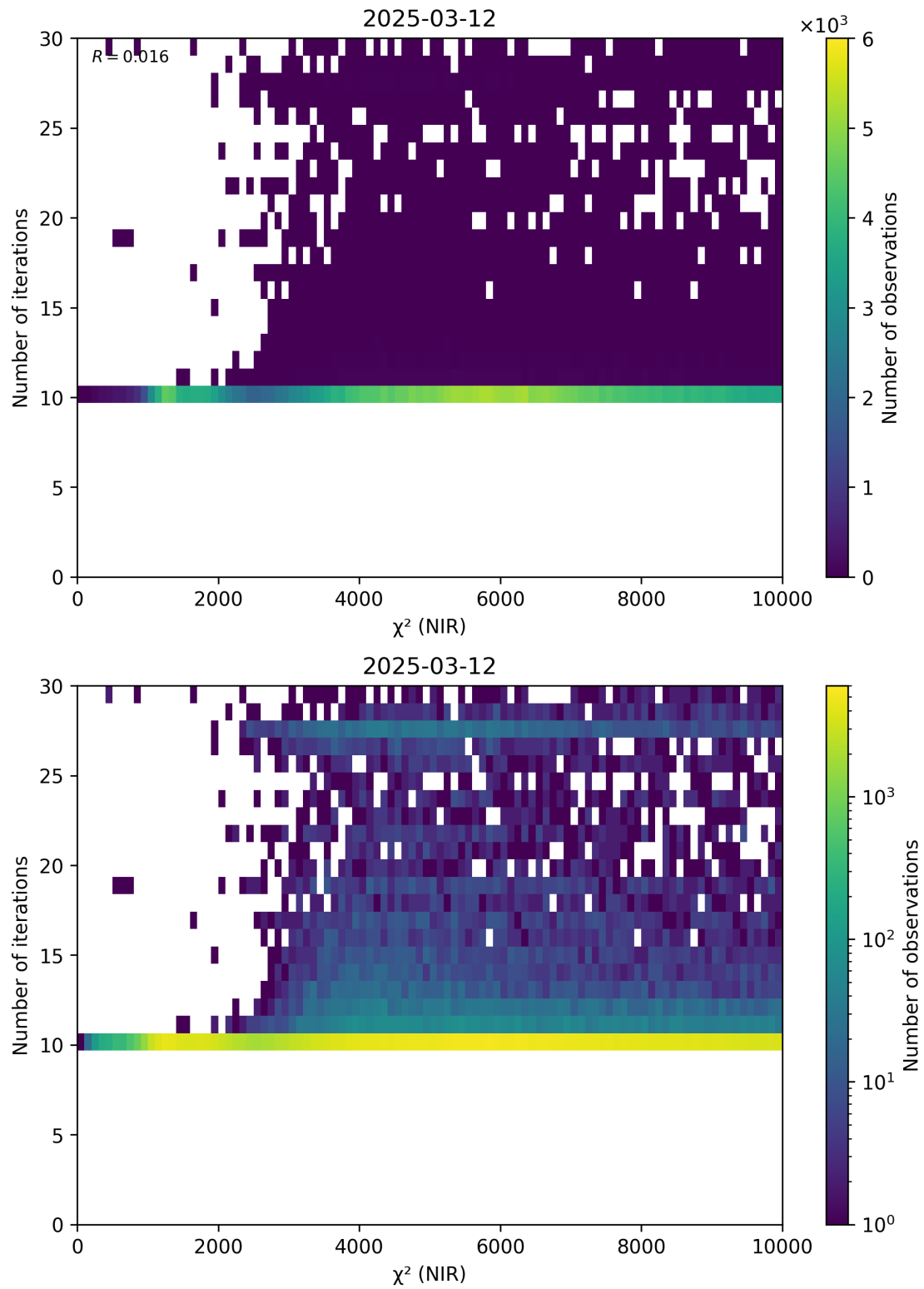
Figure 46: Scatter density plot of “ \chi^2 (NIR)” against “Number of iterations” for 2025-03-12 to 2025-03-13.
