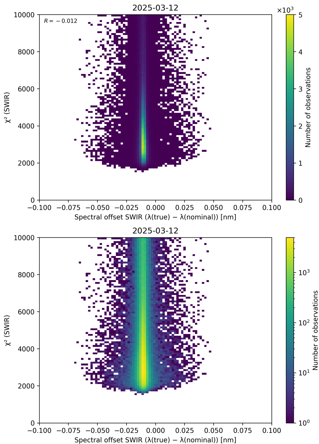
Figure 118: Scatter density plot of “Spectral offset SWIR ( \lambda_{\text{true}} - \lambda_{\text{nominal}} )” against “ \chi^2 (SWIR)” for 2025-03-12 to 2025-03-13.
