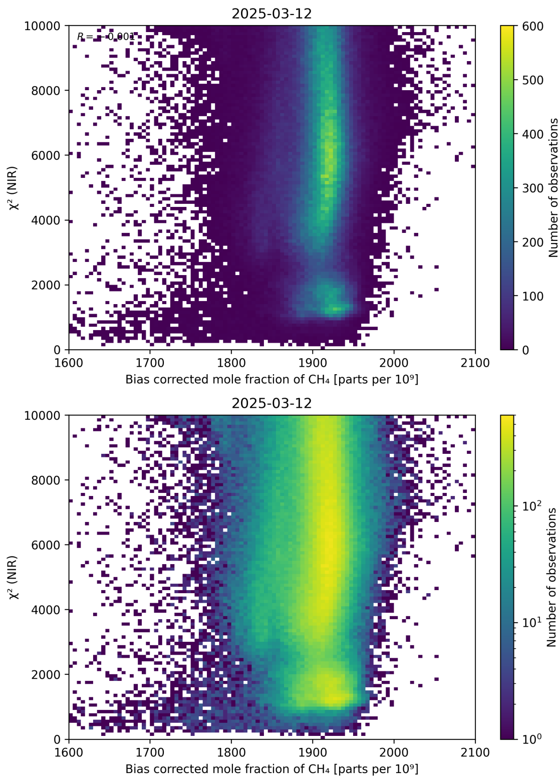
Figure 63: Scatter density plot of “Bias corrected mole fraction of \text{CH}_4 ” against “ \chi^2 (NIR)” for 2025-03-12 to 2025-03-13.
