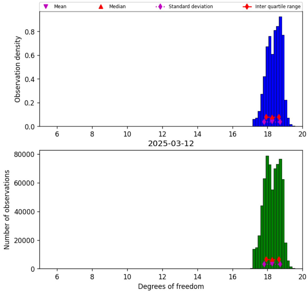
Figure 30: Histogram of “Degrees of freedom” for 2025-03-12 to 2025-03-13
