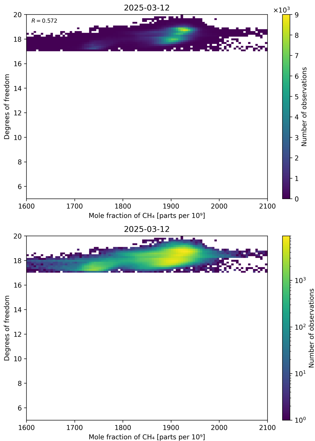
Figure 72: Scatter density plot of “Mole fraction of CH 4 ” against “Degrees of freedom” for 2025-03-12 to 2025-03-13.
