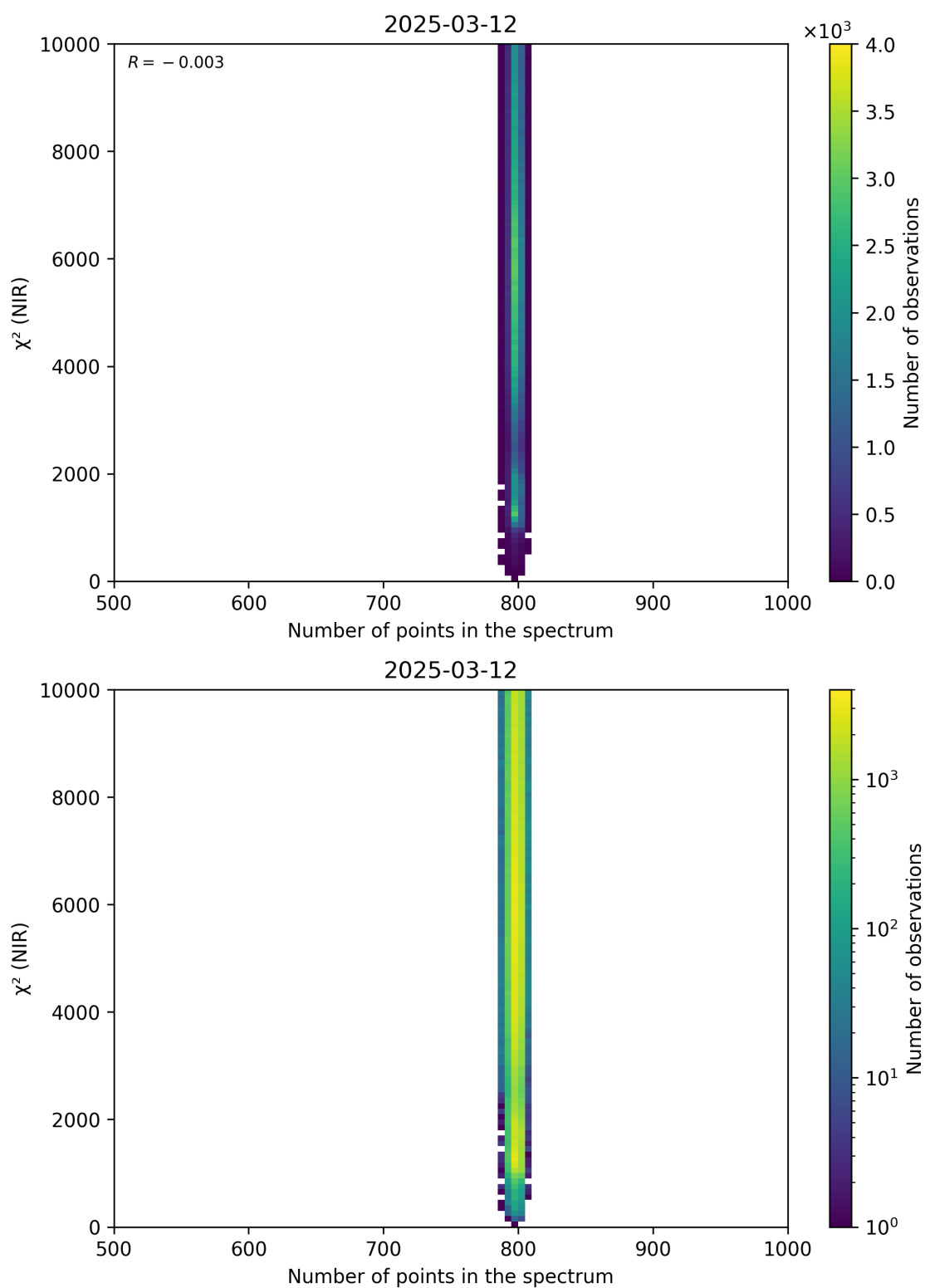
Figure 88: Scatter density plot of “Number of points in the spectrum” against “ \chi^2 (NIR)” for 2025-03-12 to 2025-03-13.
