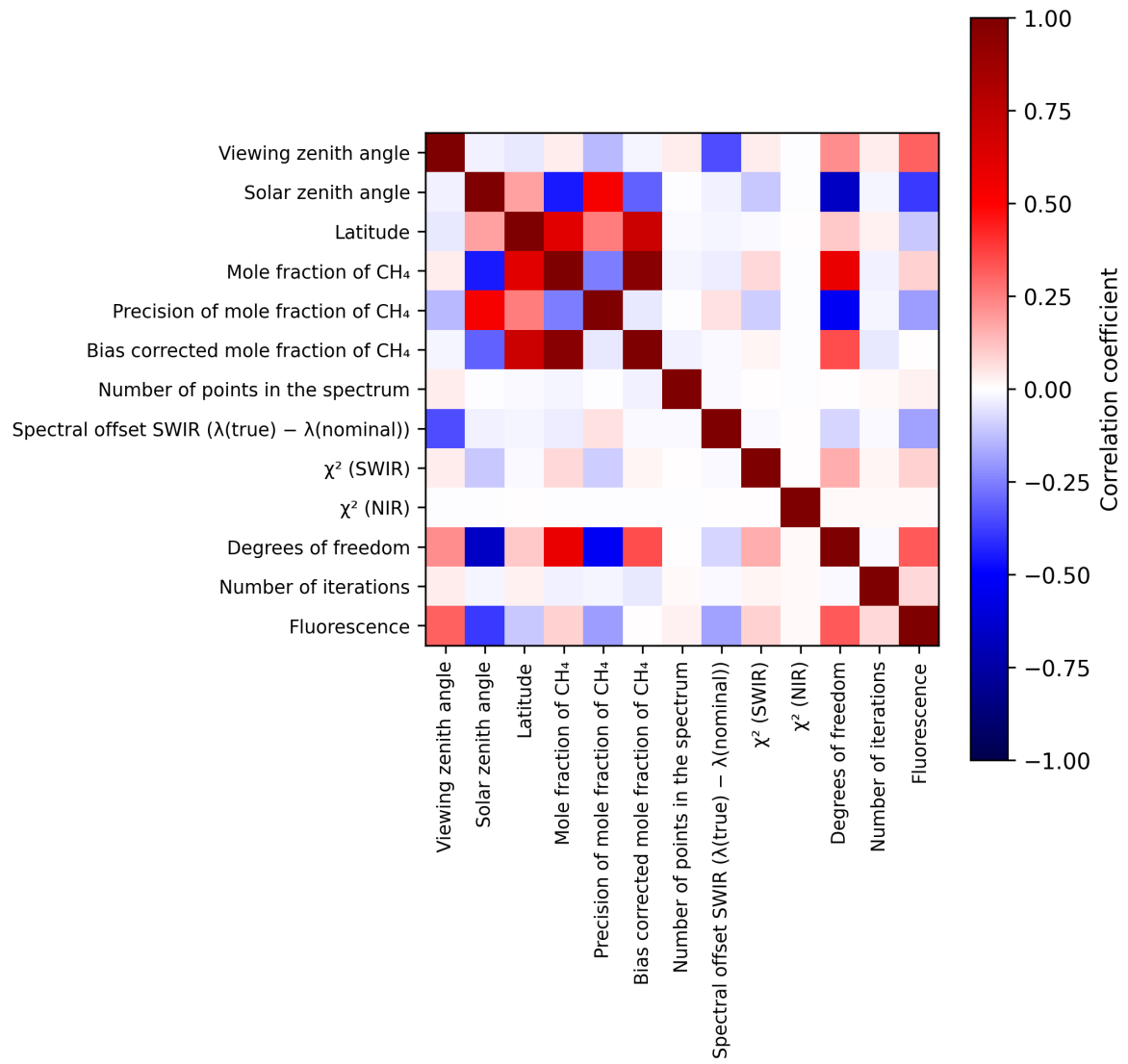
Figure 2: Map of correlation matrix for 2025-03-12 to 2025-03-13.
