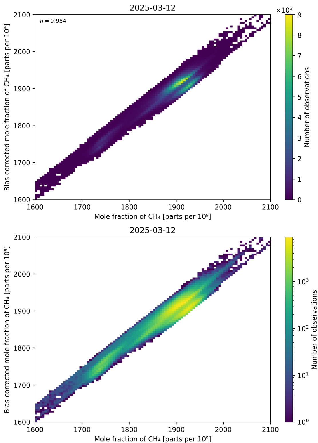
Figure 74: Scatter density plot of “Mole fraction of CH 4 ” against “Bias corrected mole fraction of CH 4 ” for 2025-03-12 to 2025-03-13.
