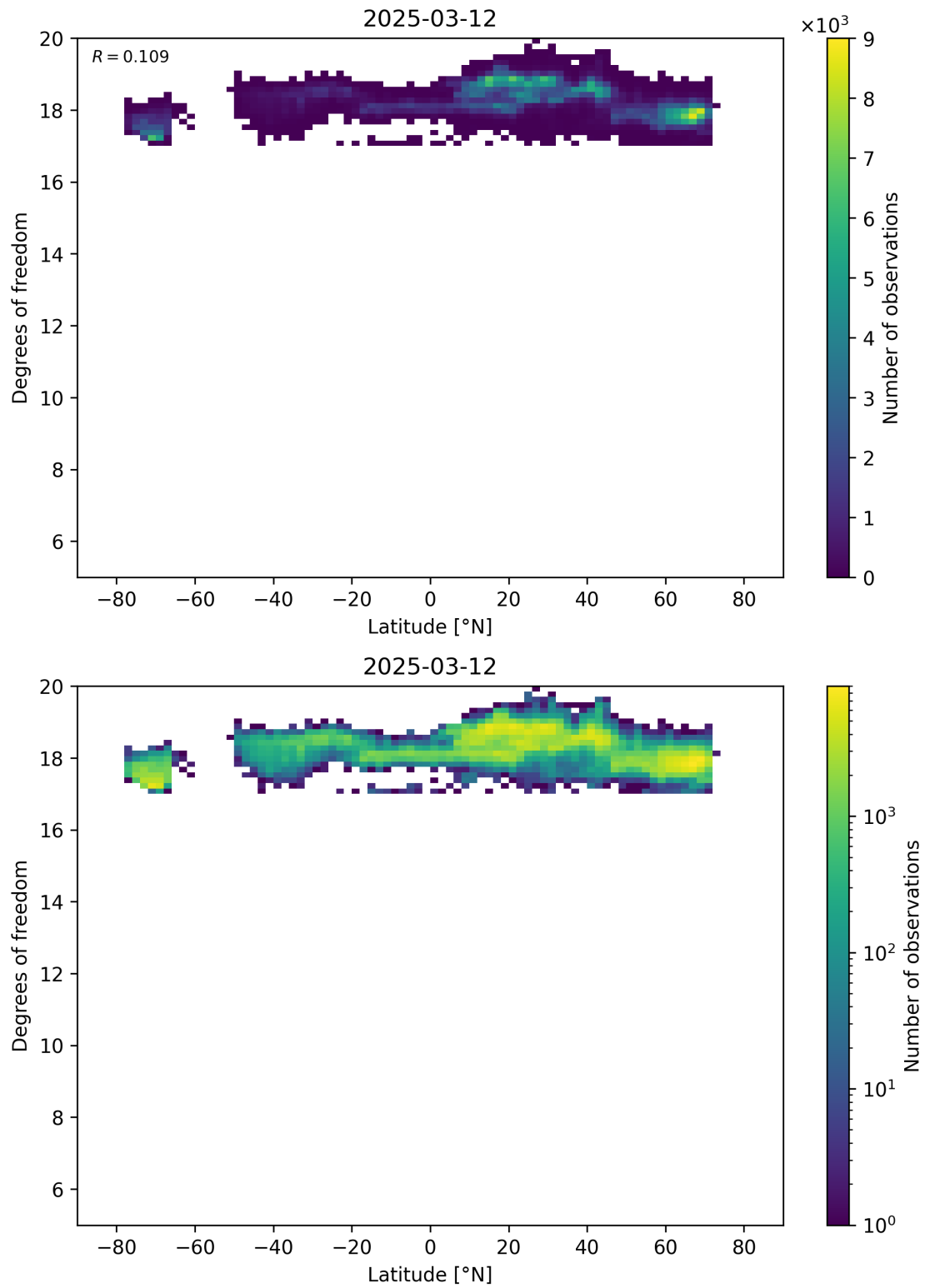
Figure 55: Scatter density plot of “Latitude” against “Degrees of freedom” for 2025-03-12 to 2025-03-13.
