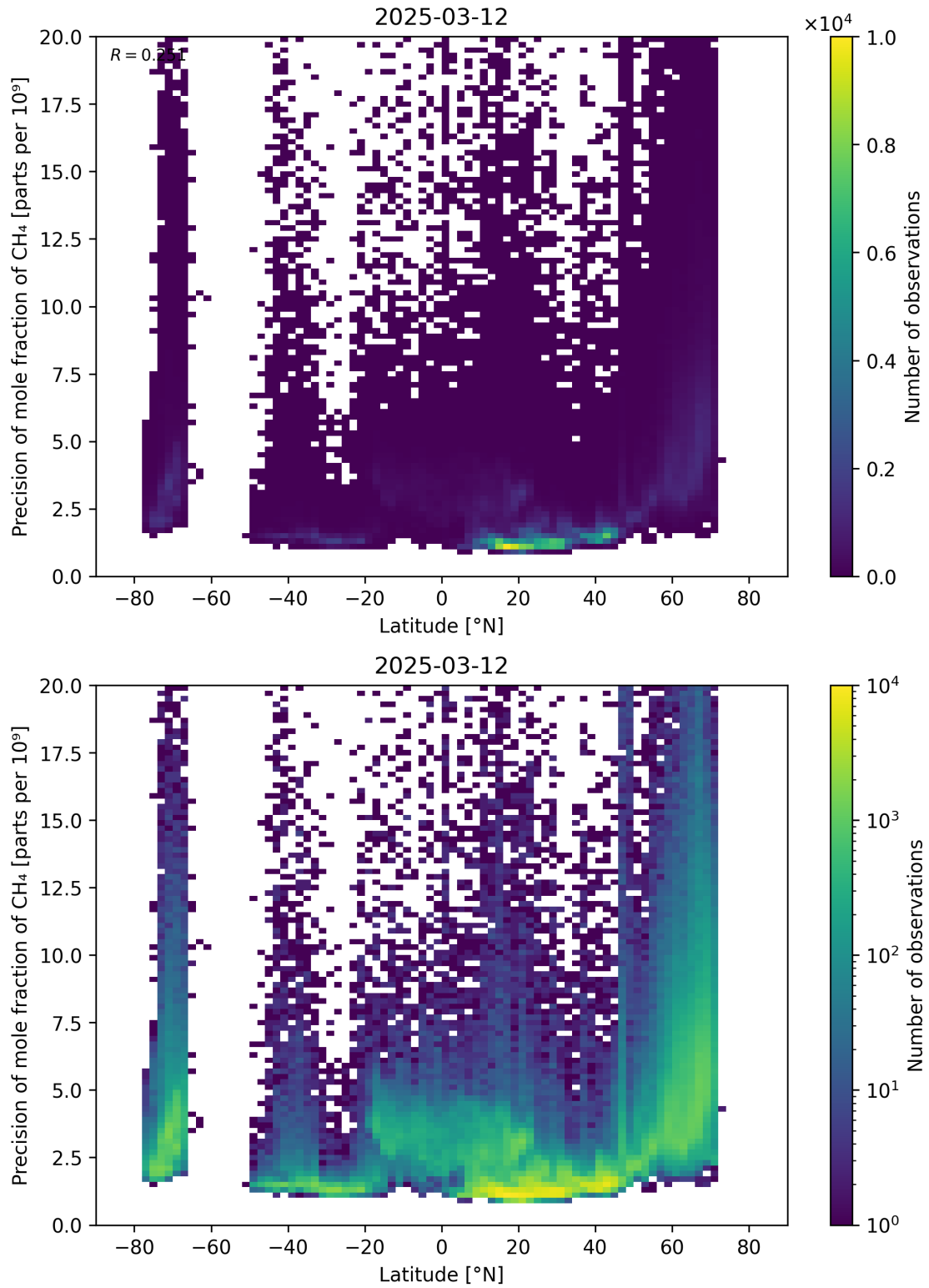
Figure 59: Scatter density plot of “Latitude” against “Precision of mole fraction of CH 4 ” for 2025-03-12 to 2025-03-13.
