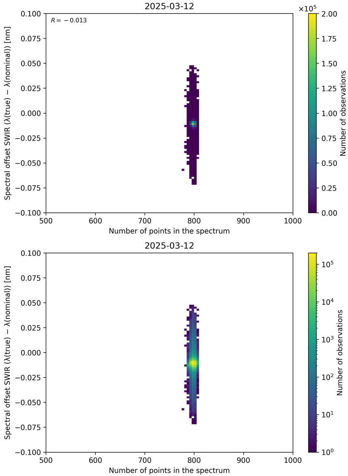
Figure 93: Scatter density plot of “Number of points in the spectrum” against “Spectral offset SWIR ( \lambda_{\text{true}} - \lambda_{\text{nominal}} )” for 2025-03-12 to 2025-03-13.
