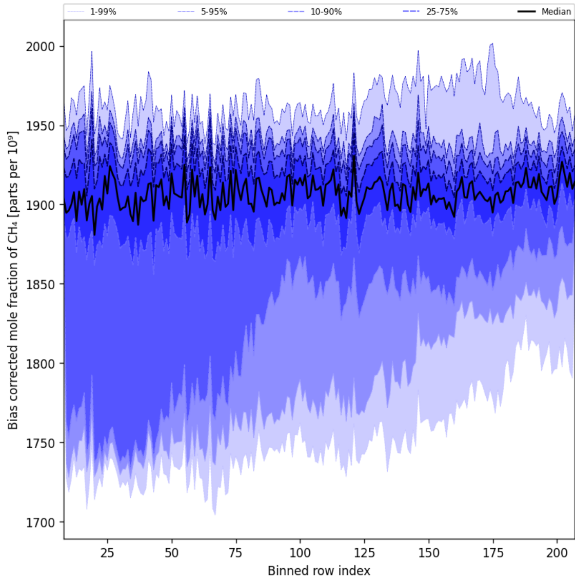
Figure 36: Along track statistics of “Bias corrected mole fraction of CH 4 ” for 2025-03-12 to 2025-03-13
