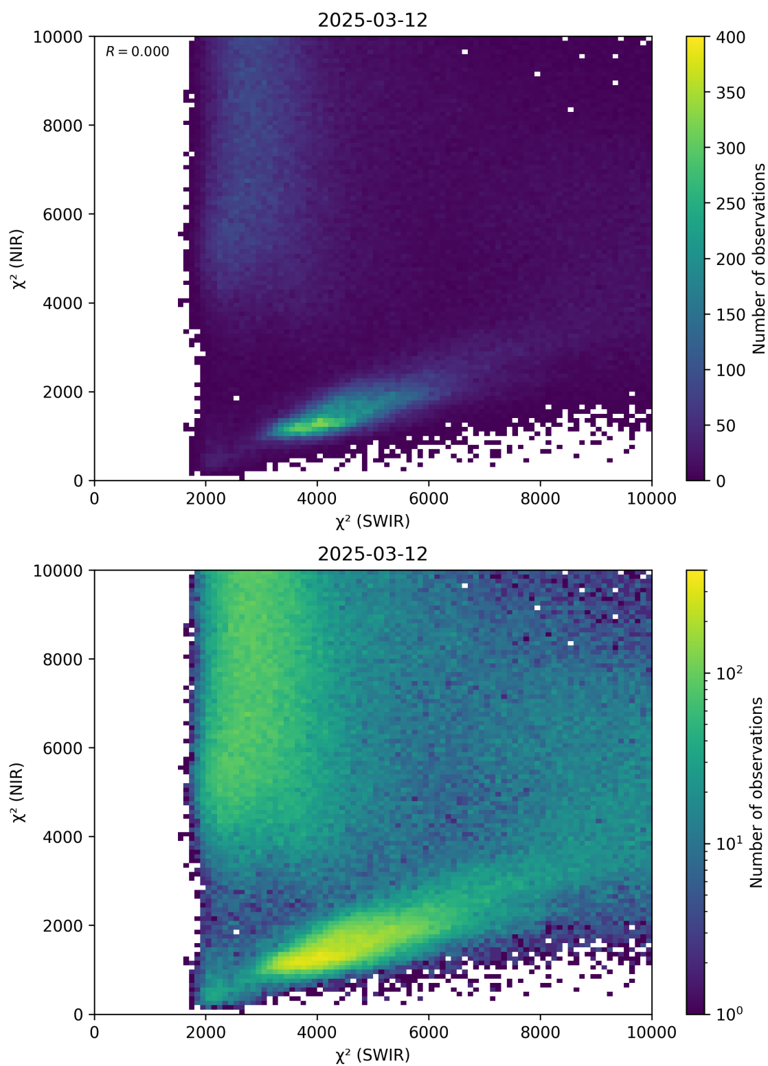
Figure 47: Scatter density plot of “ \chi^2 (SWIR)” against “ \chi^2 (NIR)” for 2025-03-12 to 2025-03-13.
