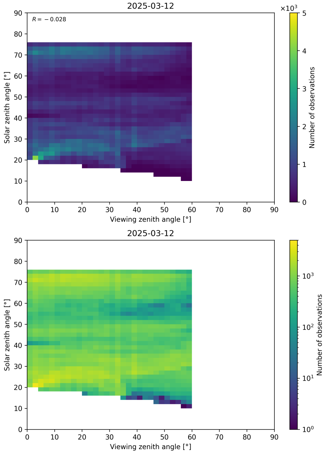
Figure 115: Scatter density plot of “Viewing zenith angle” against “Solar zenith angle” for 2025-03-12 to 2025-03-13.
