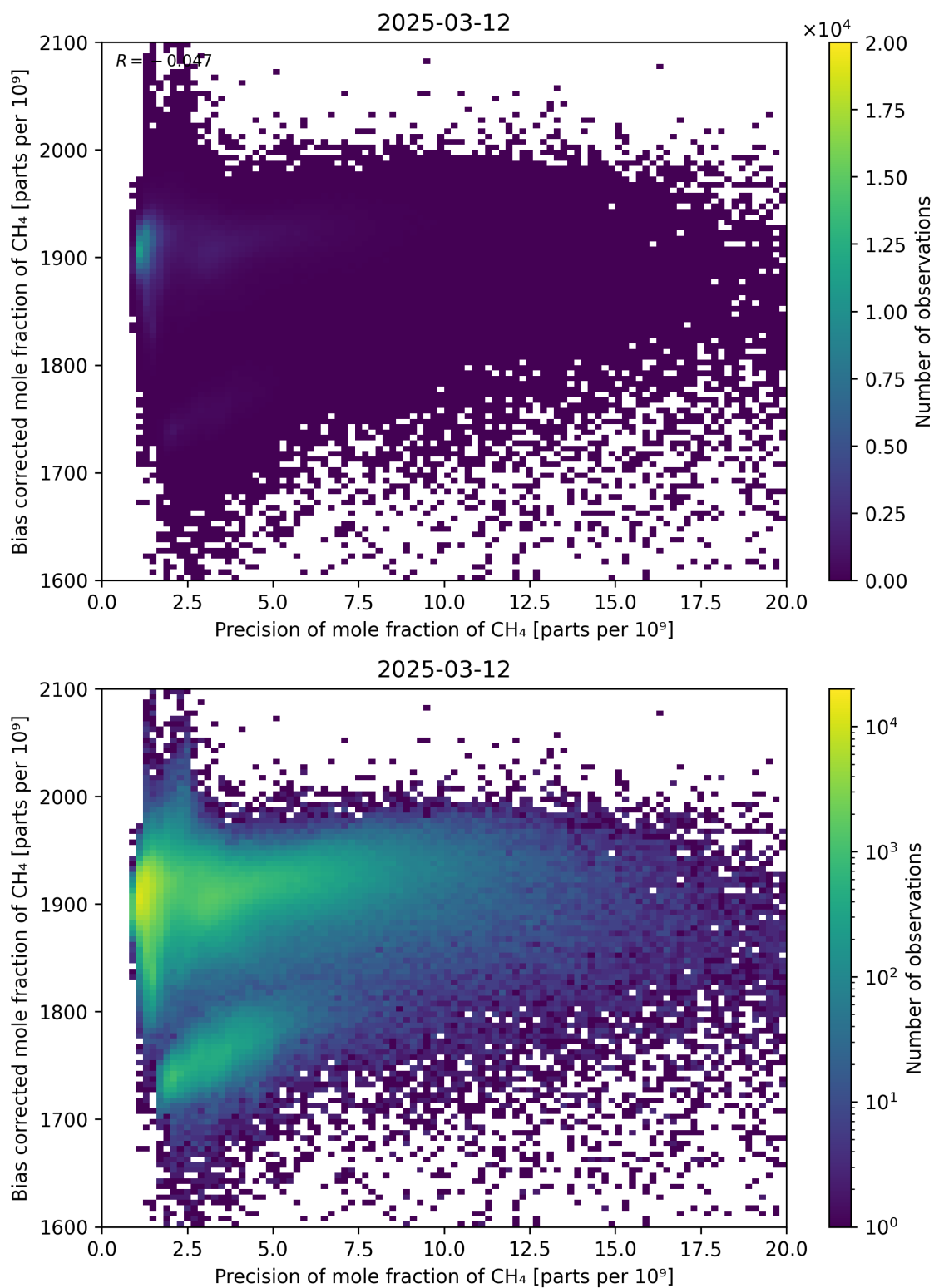
Figure 82: Scatter density plot of “Precision of mole fraction of CH 4 ” against “Bias corrected mole fraction of CH 4 ” for 2025-03-12 to 2025-03-13.
