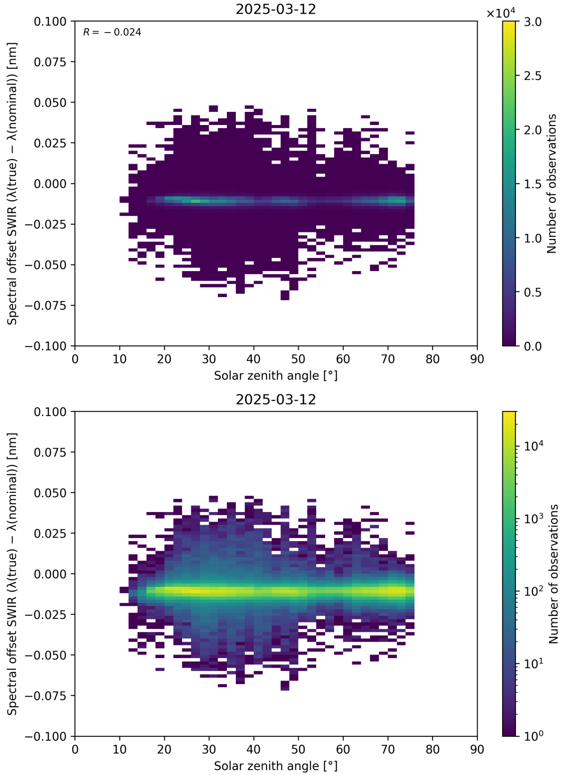
Figure 104: Scatter density plot of “Solar zenith angle” against “Spectral offset SWIR ( \lambda_{\text{true}} - \lambda_{\text{nominal}} )” for 2025-03-12 to 2025-03-13.
