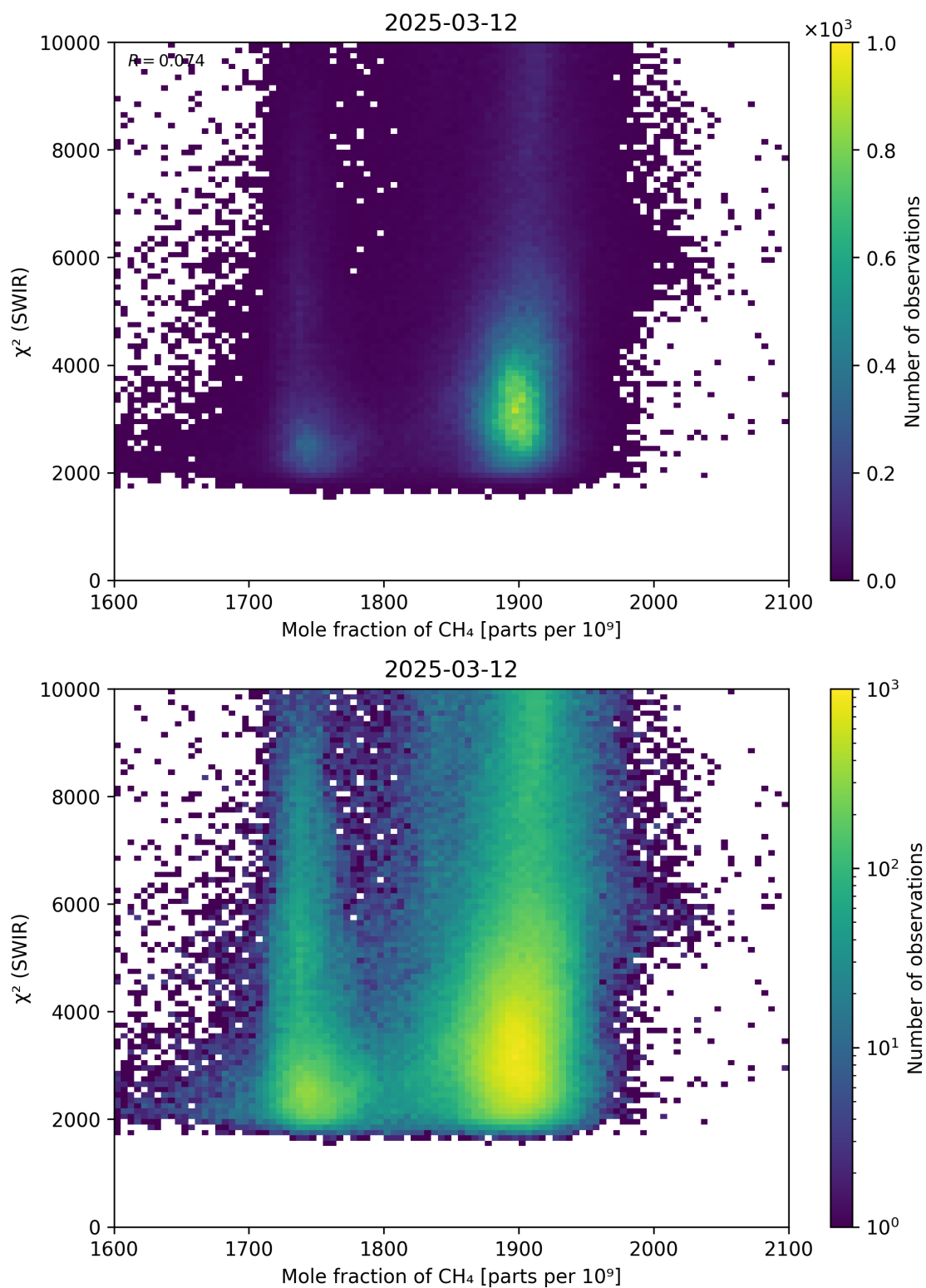
Figure 71: Scatter density plot of “Mole fraction of \text{CH}_4 ” against “ \chi^2 (SWIR)” for 2025-03-12 to 2025-03-13.
