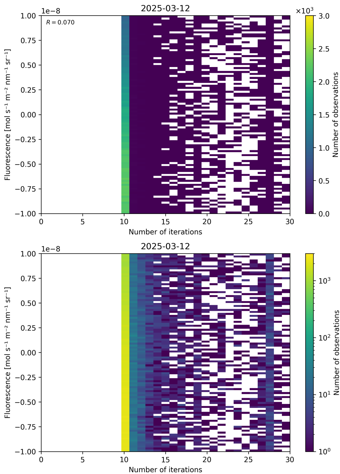
Figure 87: Scatter density plot of “Number of iterations” against “Fluorescence” for 2025-03-12 to 2025-03-13.
