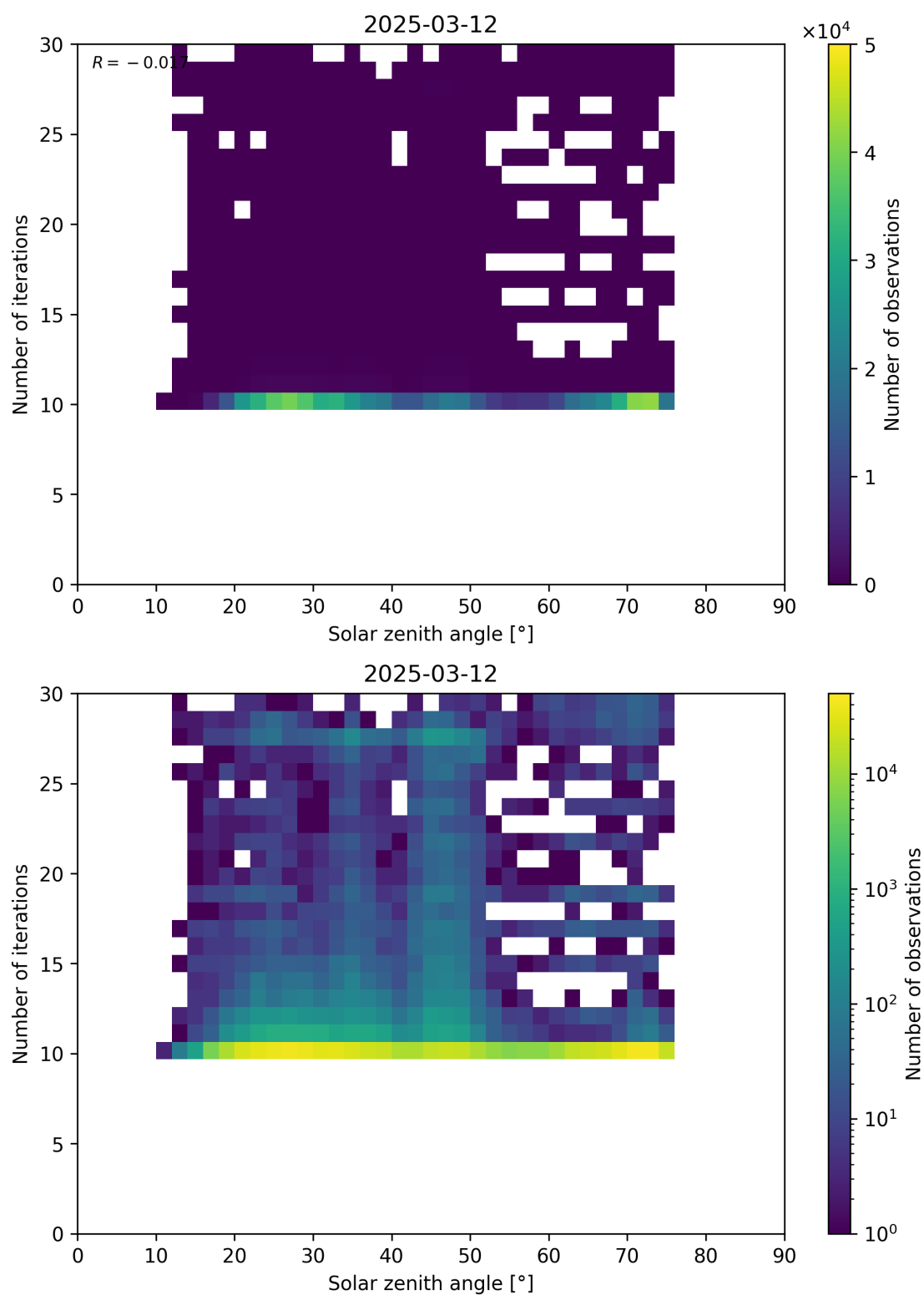
Figure 102: Scatter density plot of “Solar zenith angle” against “Number of iterations” for 2025-03-12 to 2025-03-13.
