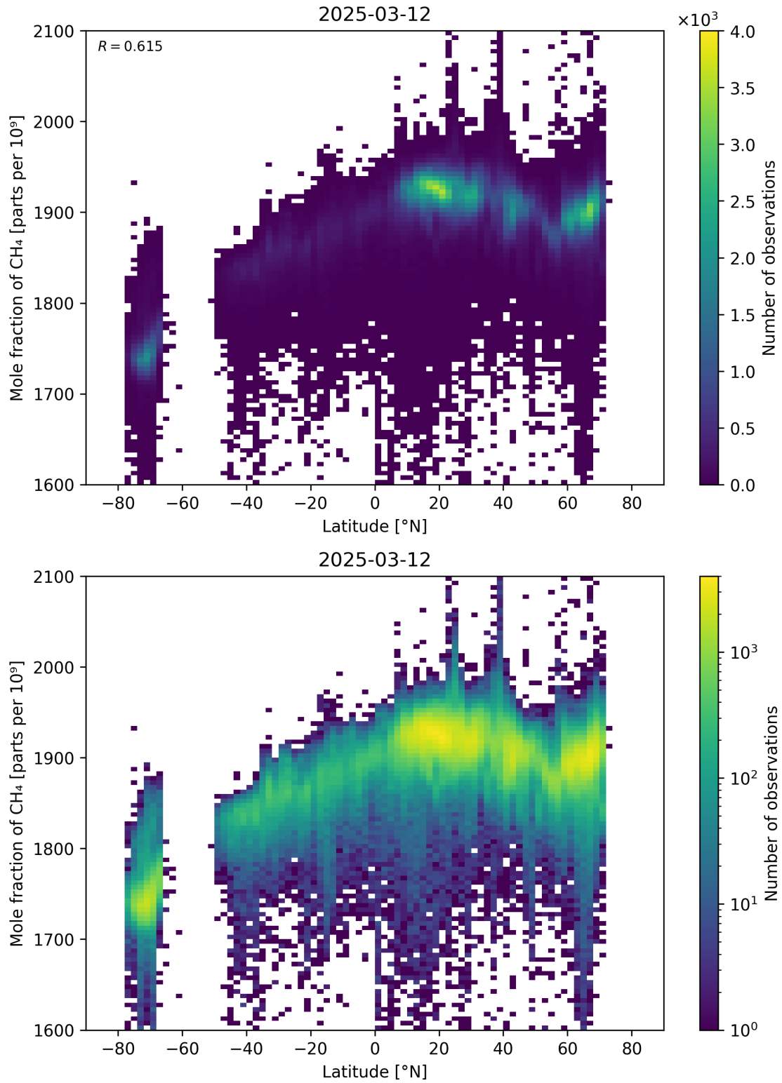
Figure 57: Scatter density plot of “Latitude” against “Mole fraction of CH 4 ” for 2025-03-12 to 2025-03-13.
