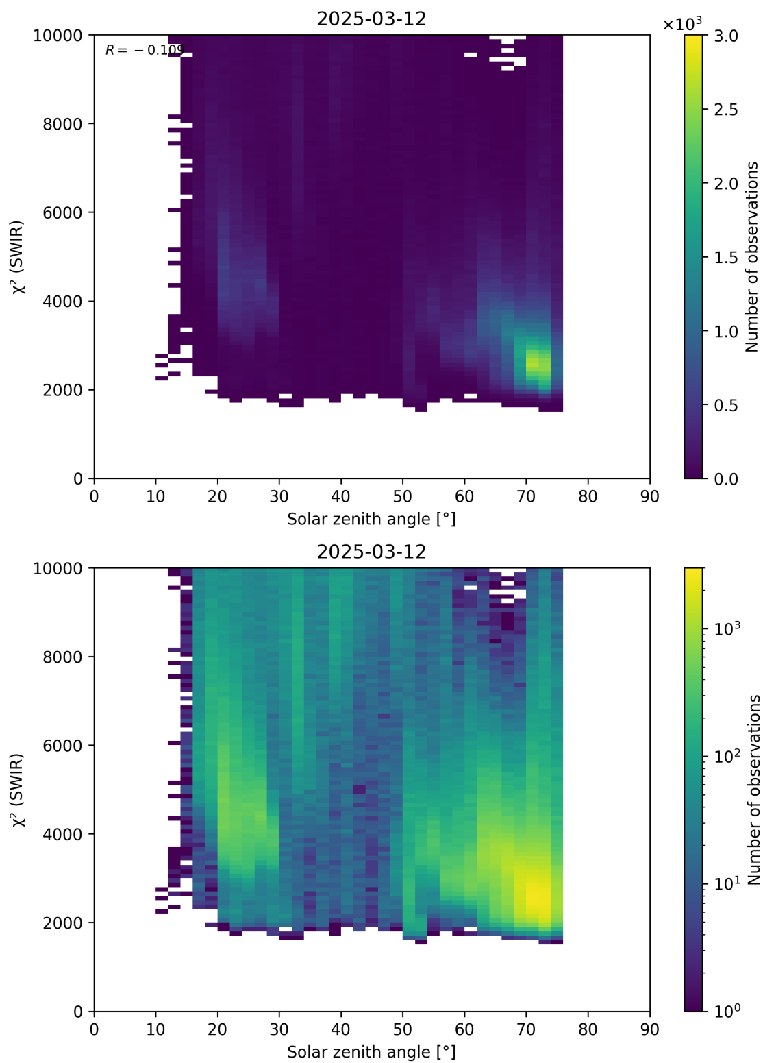
Figure 95: Scatter density plot of “Solar zenith angle” against “ \chi^2 (SWIR)” for 2025-03-12 to 2025-03-13.
