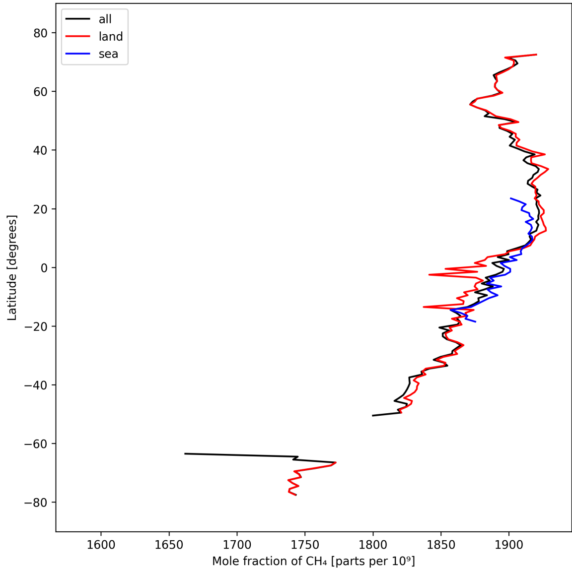
Figure 12: Zonal average of “Mole fraction of \text{CH}_4 ” for 2025-03-12 to 2025-03-13.
