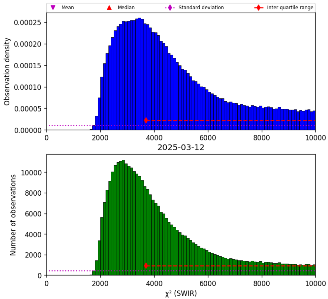
Figure 28: Histogram of “ \chi^2 (SWIR)” for 2025-03-12 to 2025-03-13
