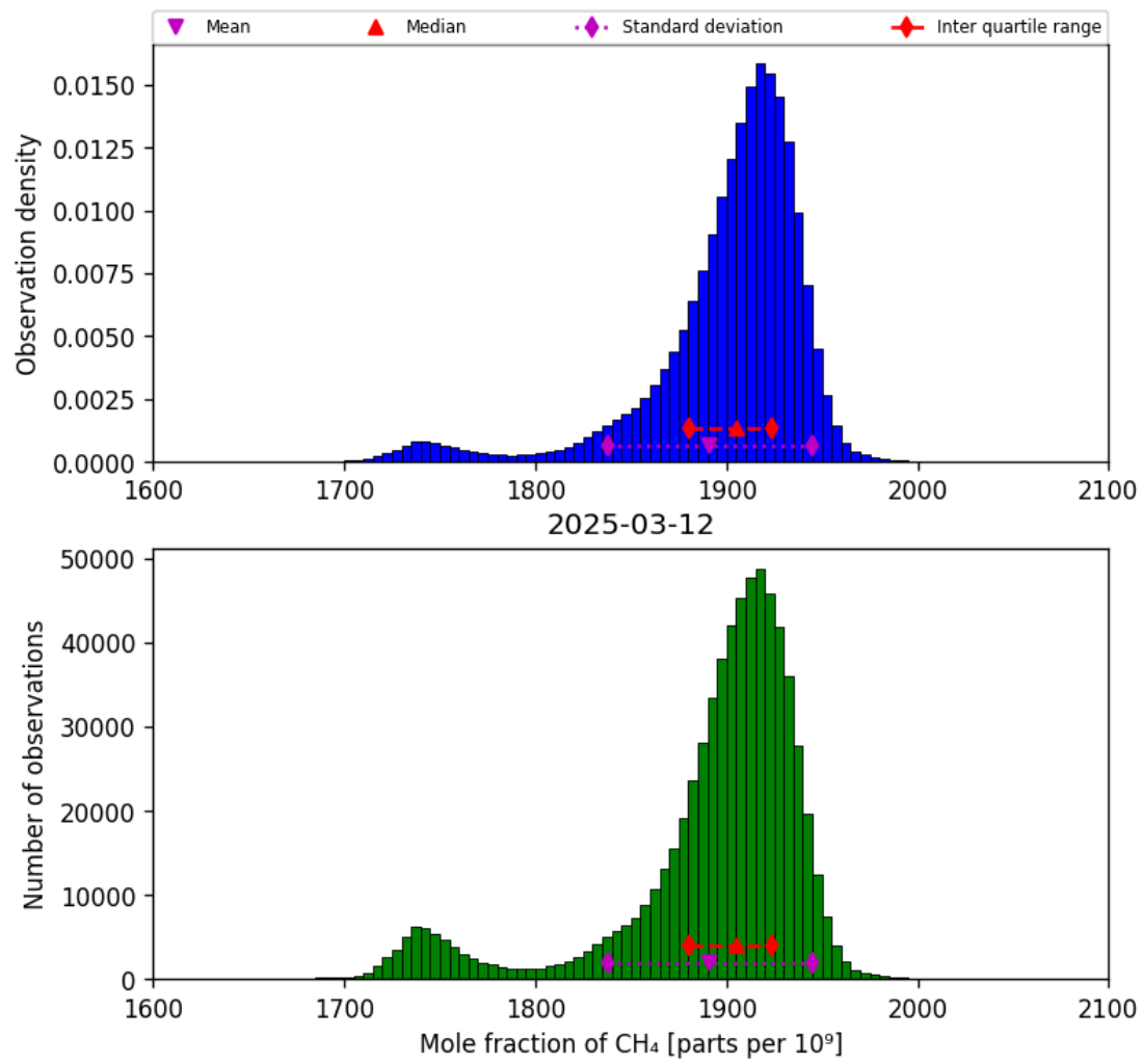
Figure 23: Histogram of “Mole fraction of CH 4 ” for 2025-03-12 to 2025-03-13
