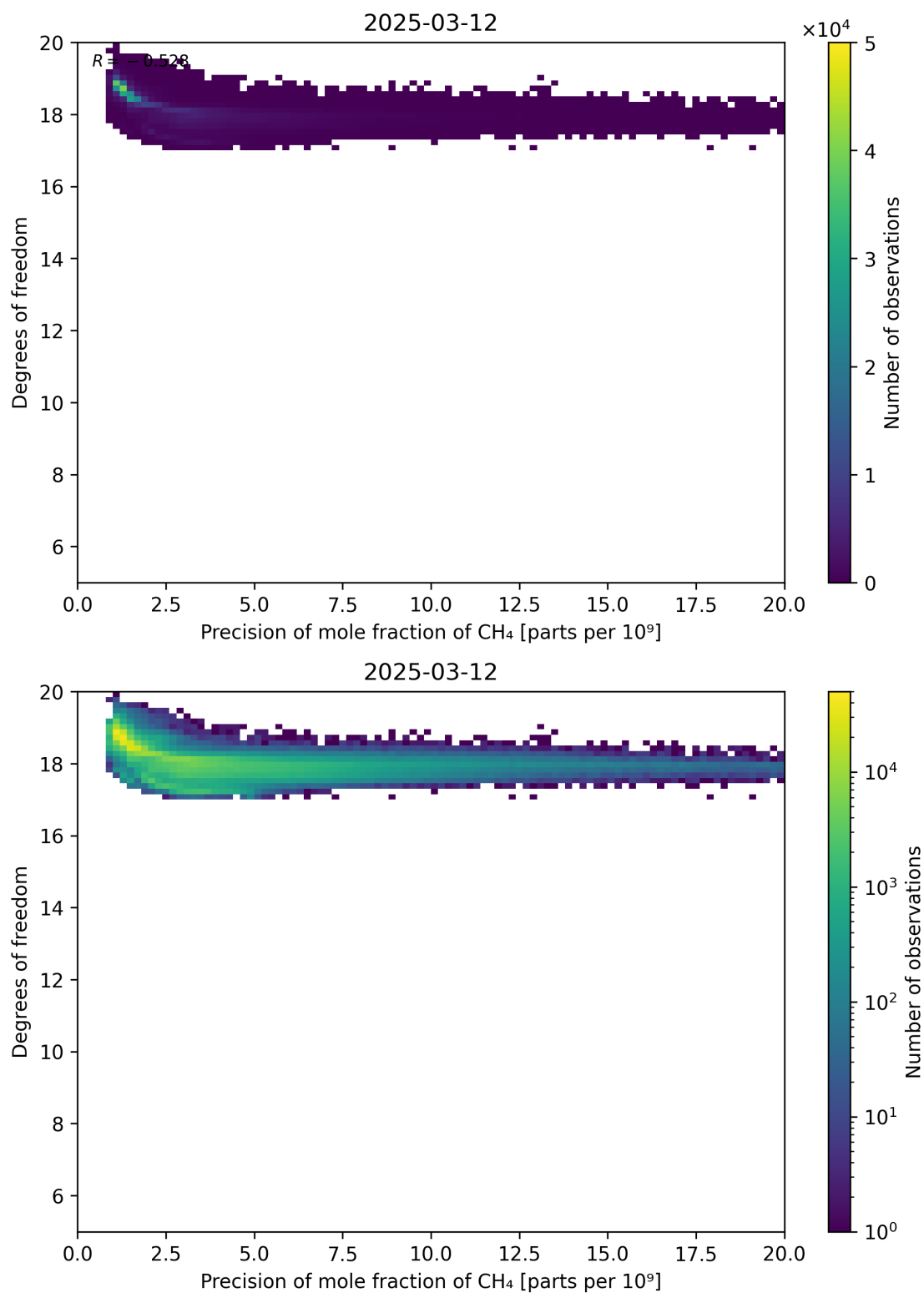
Figure 80: Scatter density plot of “Precision of mole fraction of CH 4 ” against “Degrees of freedom” for 2025-03-12 to 2025-03-13.
