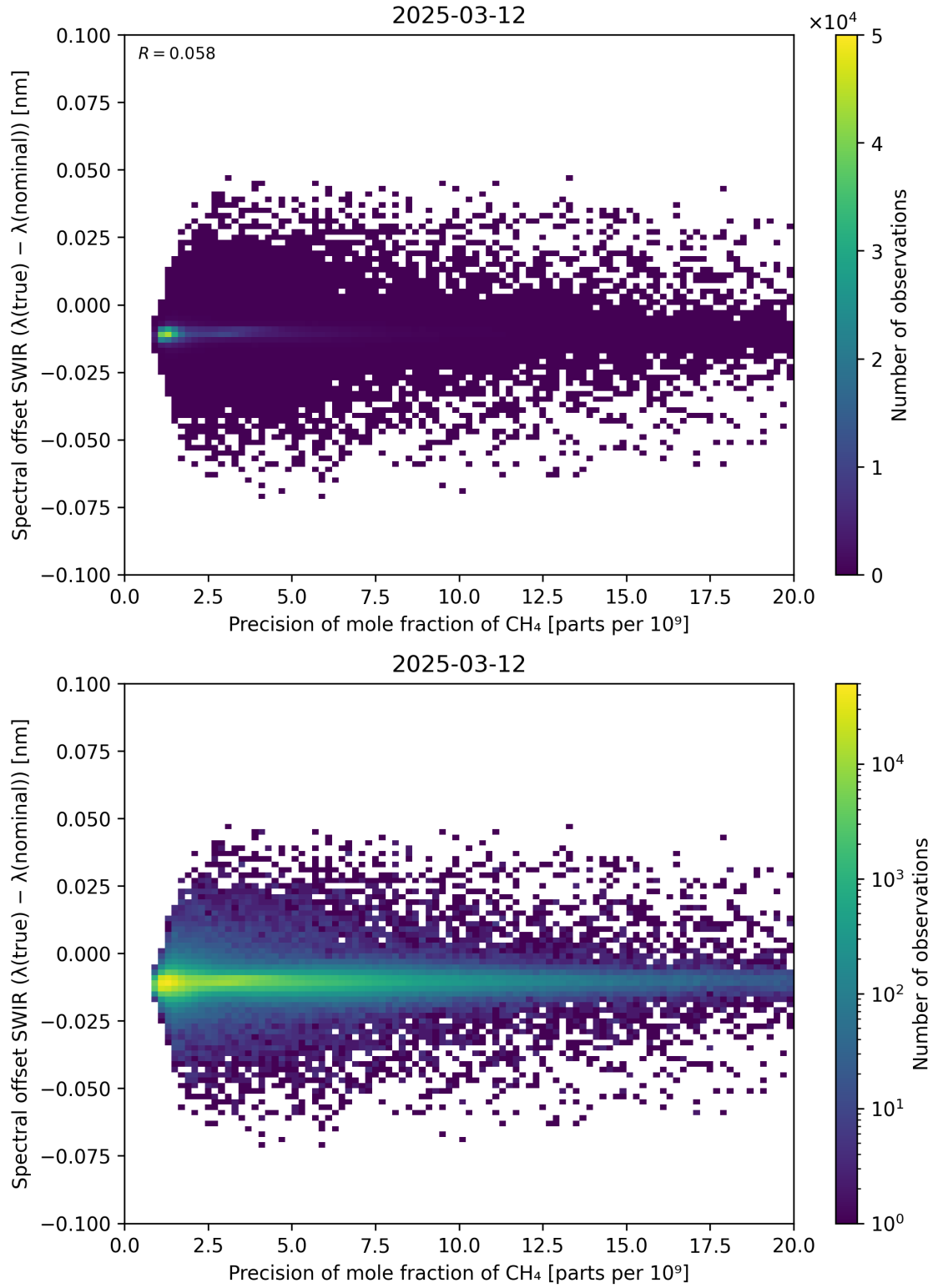
Figure 85: Scatter density plot of “Precision of mole fraction of \text{CH}_4 ” against “Spectral offset SWIR ( \lambda_{\text{true}} - \lambda_{\text{nominal}} )” for 2025-03-12 to 2025-03-13.
