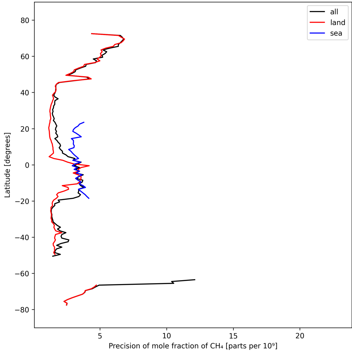
Figure 13: Zonal average of “Precision of mole fraction of CH 4 ” for 2025-03-12 to 2025-03-13.
