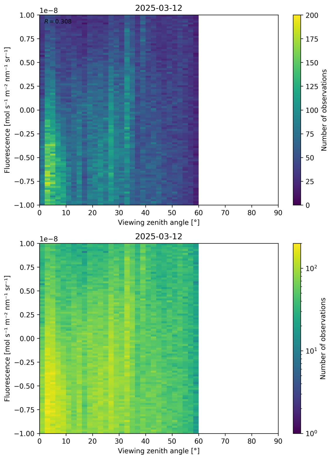
Figure 108: Scatter density plot of “Viewing zenith angle” against “Fluorescence” for 2025-03-12 to 2025-03-13.
