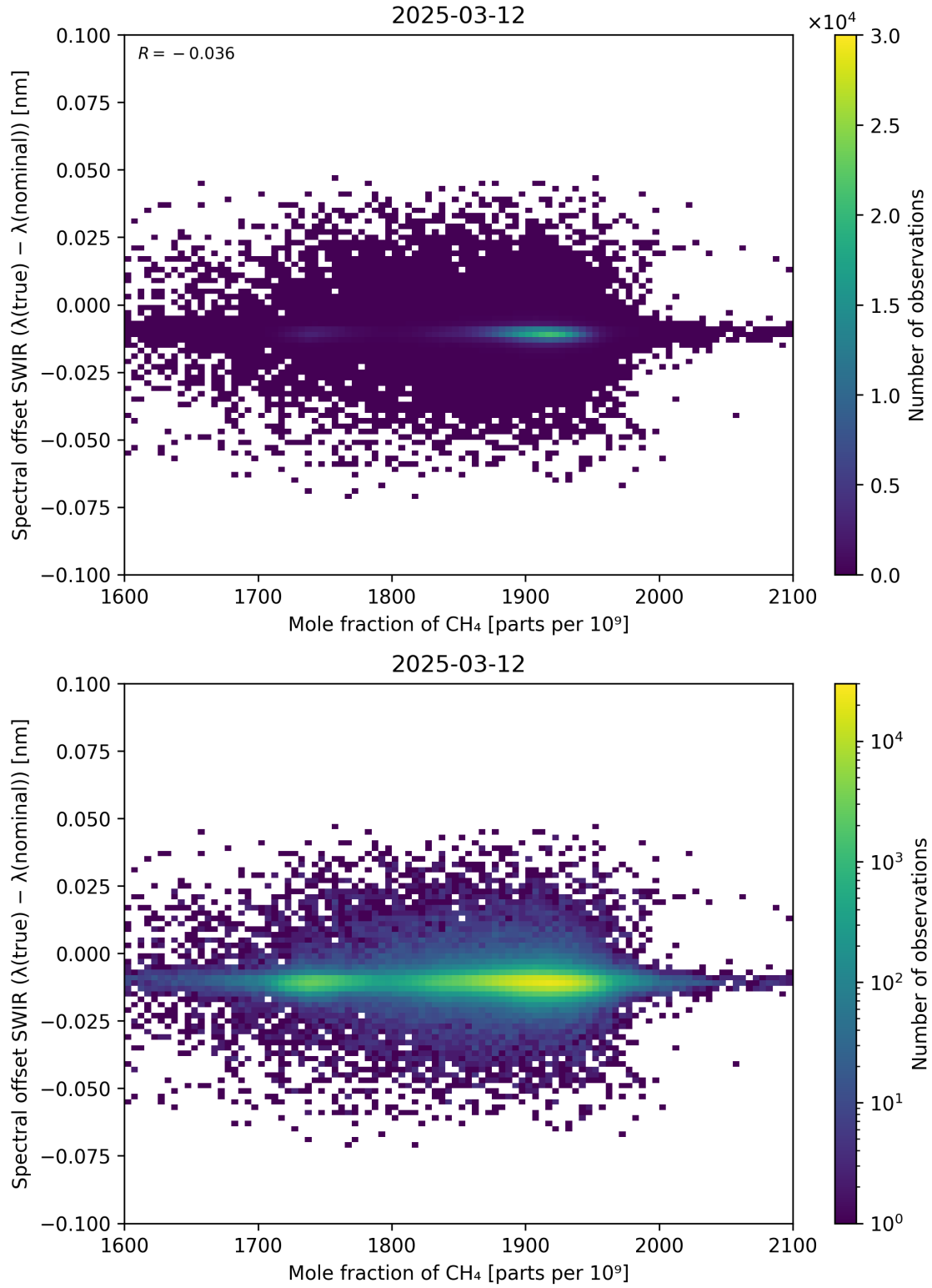
Figure 86: Scatter density plot of “Mole fraction of \text{CH}_4 ” against “Spectral offset SWIR ( \lambda_{\text{true}} - \lambda_{\text{nominal}} )” for 2025-03-12 to 2025-03-13.
