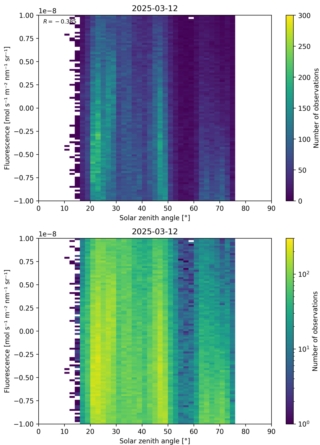
Figure 97: Scatter density plot of “Solar zenith angle” against “Fluorescence” for 2025-03-12 to 2025-03-13.
