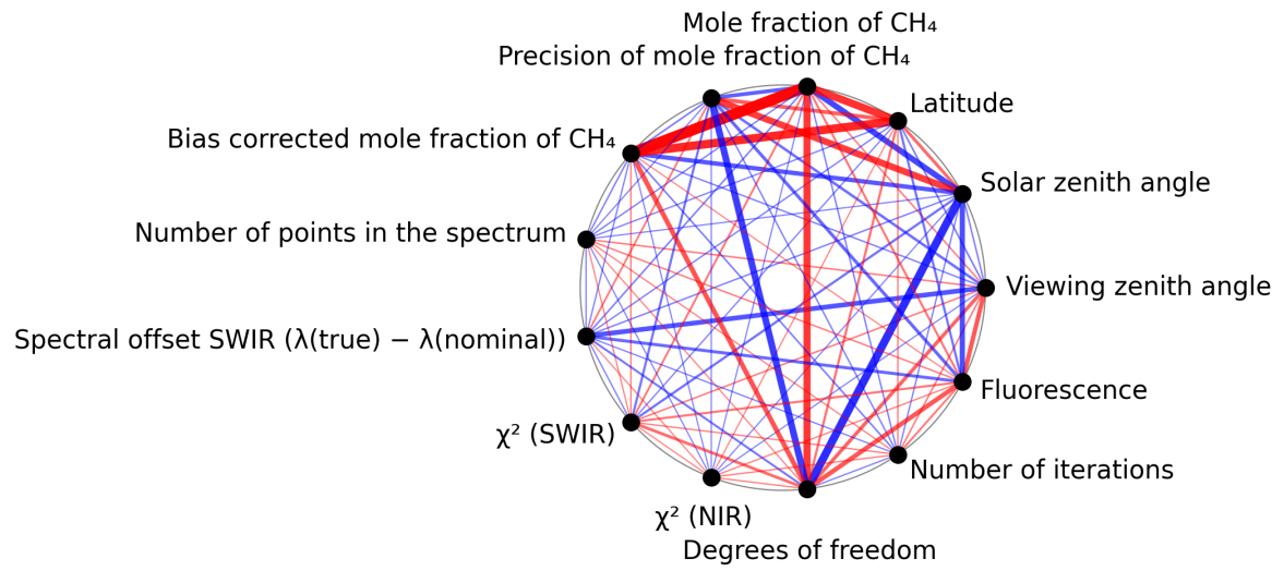
Figure 1: Map of correlation graph for 2025-03-12 to 2025-03-13.
