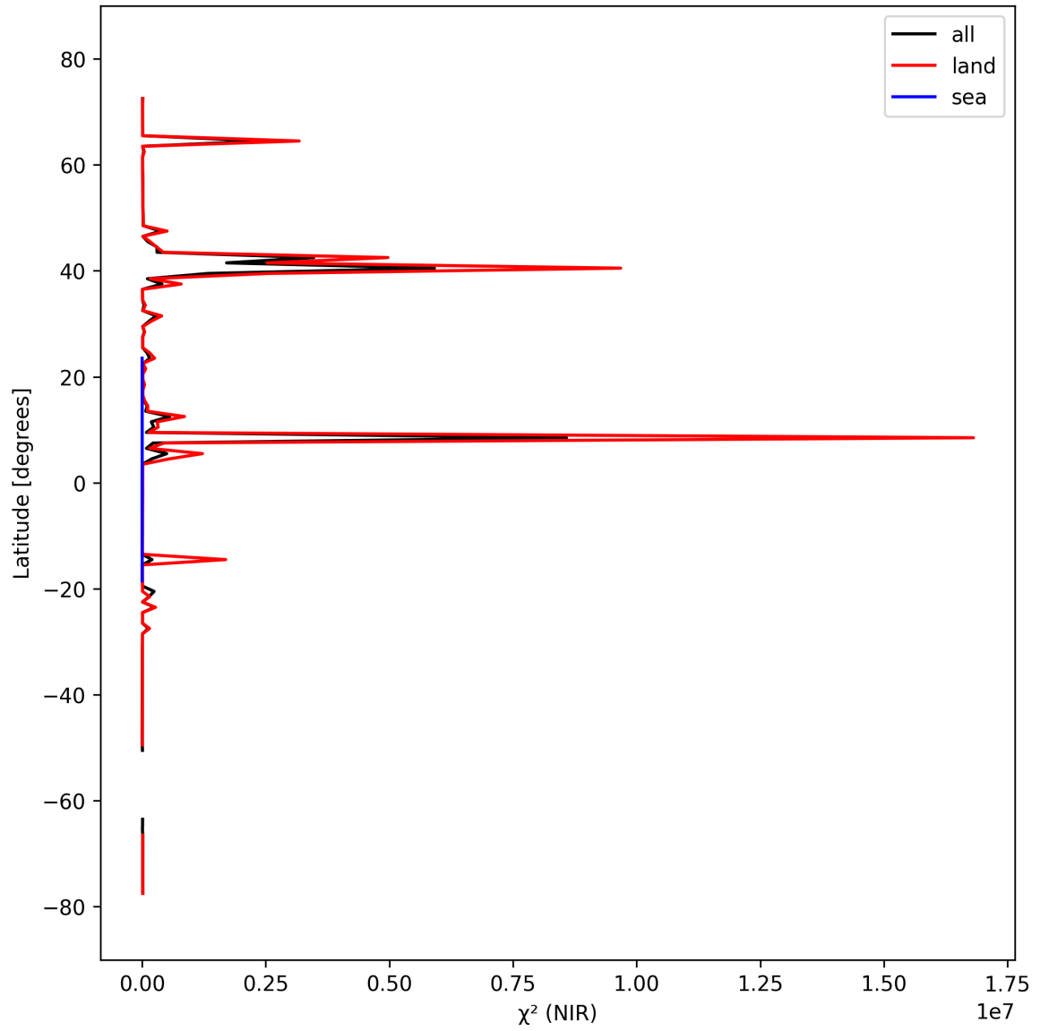
Figure 18: Zonal average of “ \chi^2 (NIR)” for 2025-03-12 to 2025-03-13.
