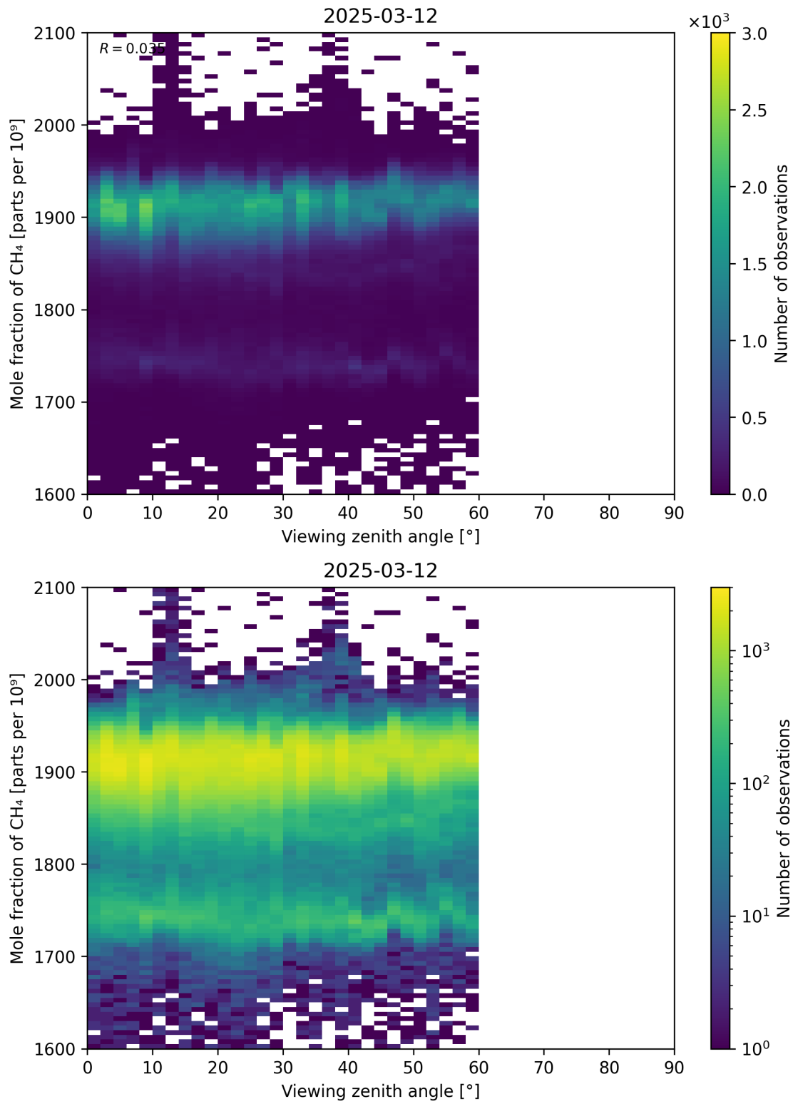
Figure 110: Scatter density plot of “Viewing zenith angle” against “Mole fraction of CH 4 ” for 2025-03-12 to 2025-03-13.
