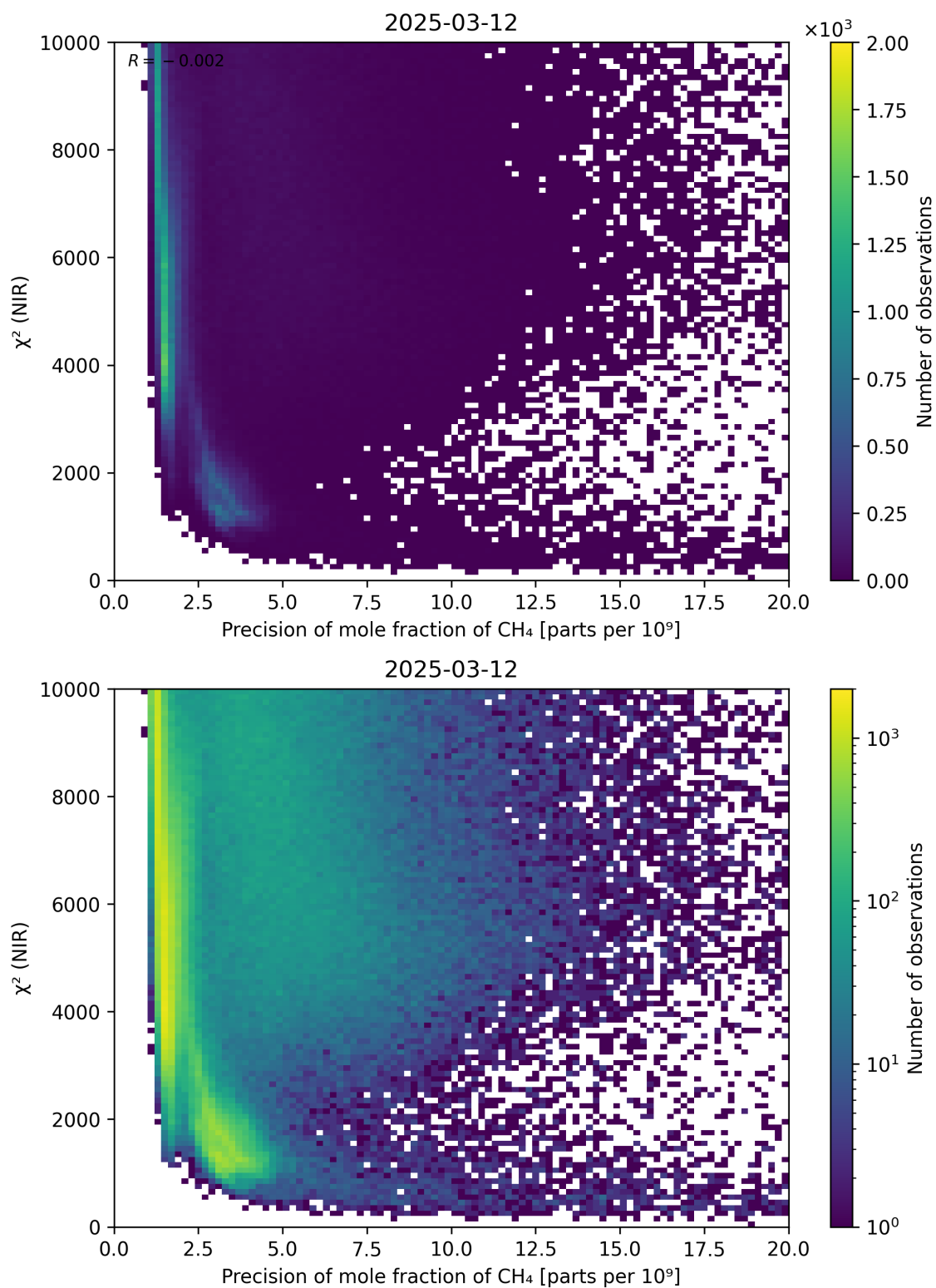
Figure 78: Scatter density plot of “Precision of mole fraction of CH 4 ” against “ \chi^2 (NIR)” for 2025-03-12 to 2025-03-13.
