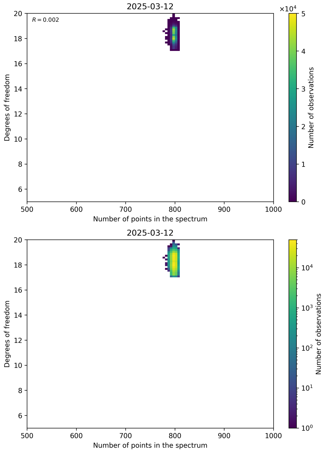
Figure 90: Scatter density plot of “Number of points in the spectrum” against “Degrees of freedom” for 2025-03-12 to 2025-03-13.
