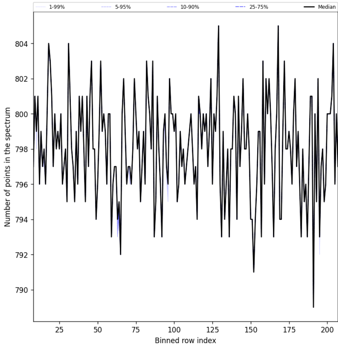
Figure 37: Along track statistics of “Number of points in the spectrum” for 2025-03-12 to 2025-03-13
