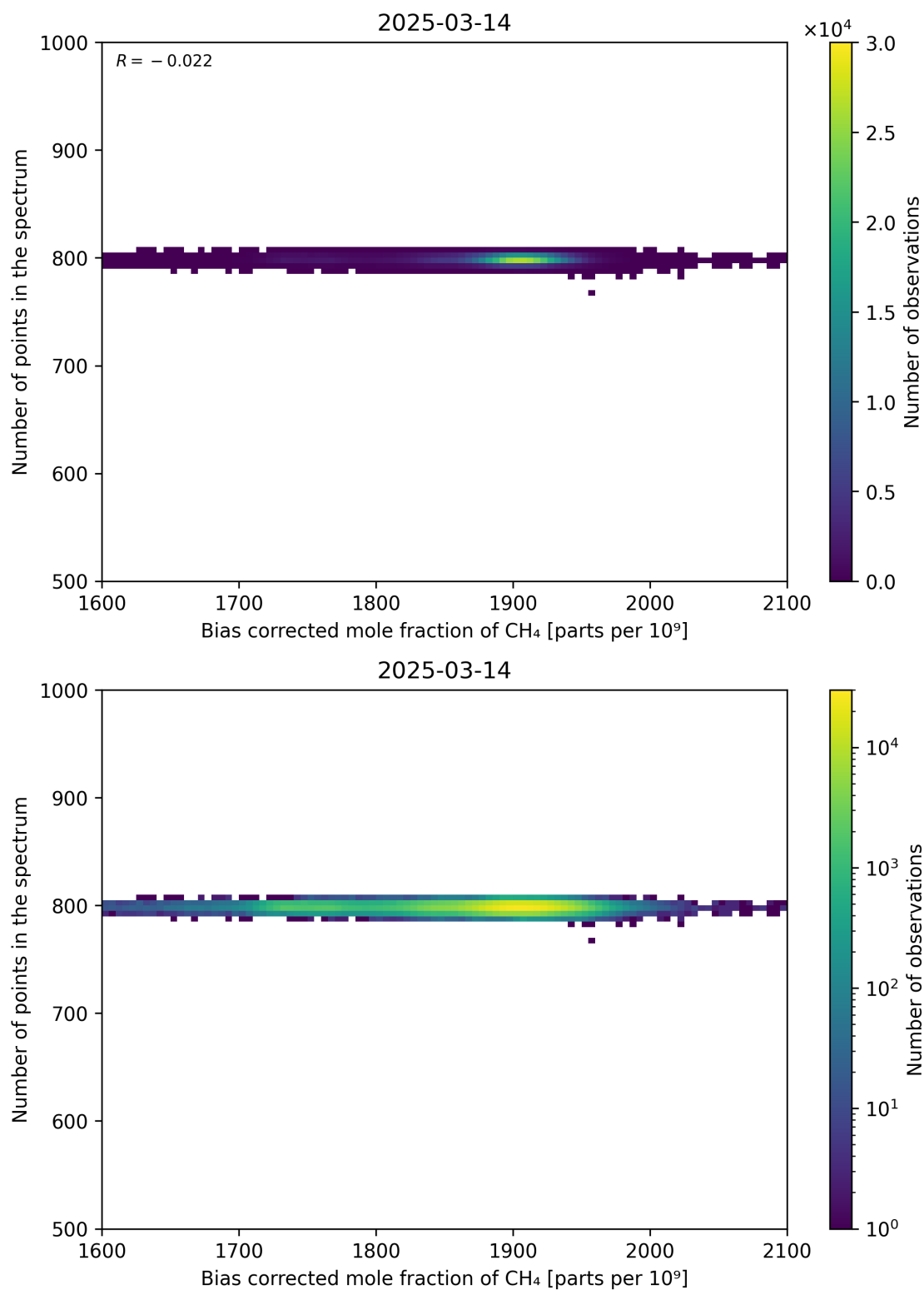
Figure 68: Scatter density plot of “Bias corrected mole fraction of CH 4 ” against “Number of points in the spectrum” for 2025-03-13 to 2025-03-15.
