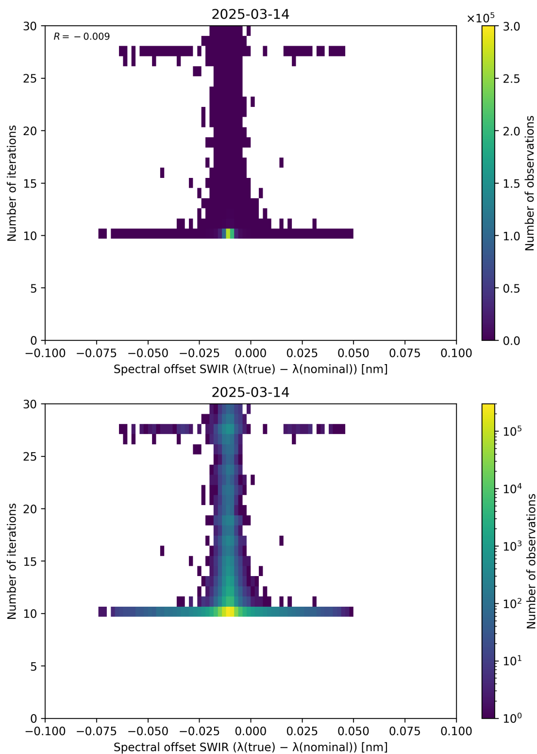
Figure 121: Scatter density plot of “Spectral offset SWIR ( \lambda_{\text{true}} - \lambda_{\text{nominal}} )” against “Number of iterations” for 2025-03-13 to 2025-03-15.
