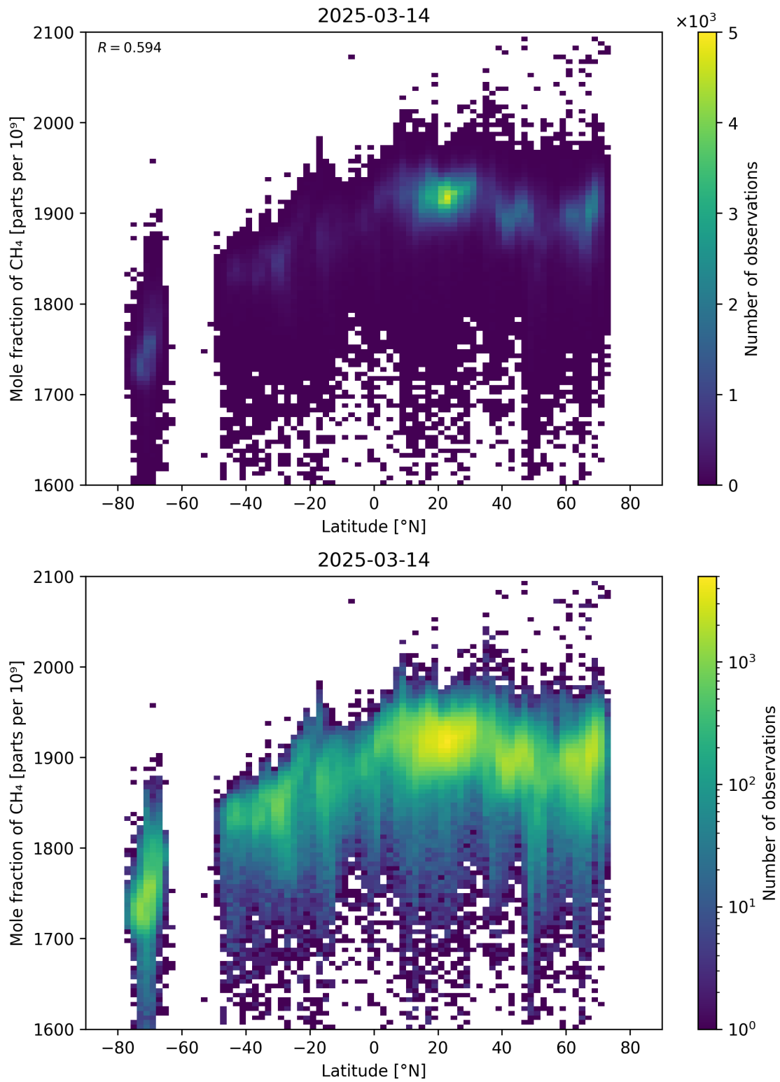
Figure 57: Scatter density plot of “Latitude” against “Mole fraction of CH 4 ” for 2025-03-13 to 2025-03-15.
