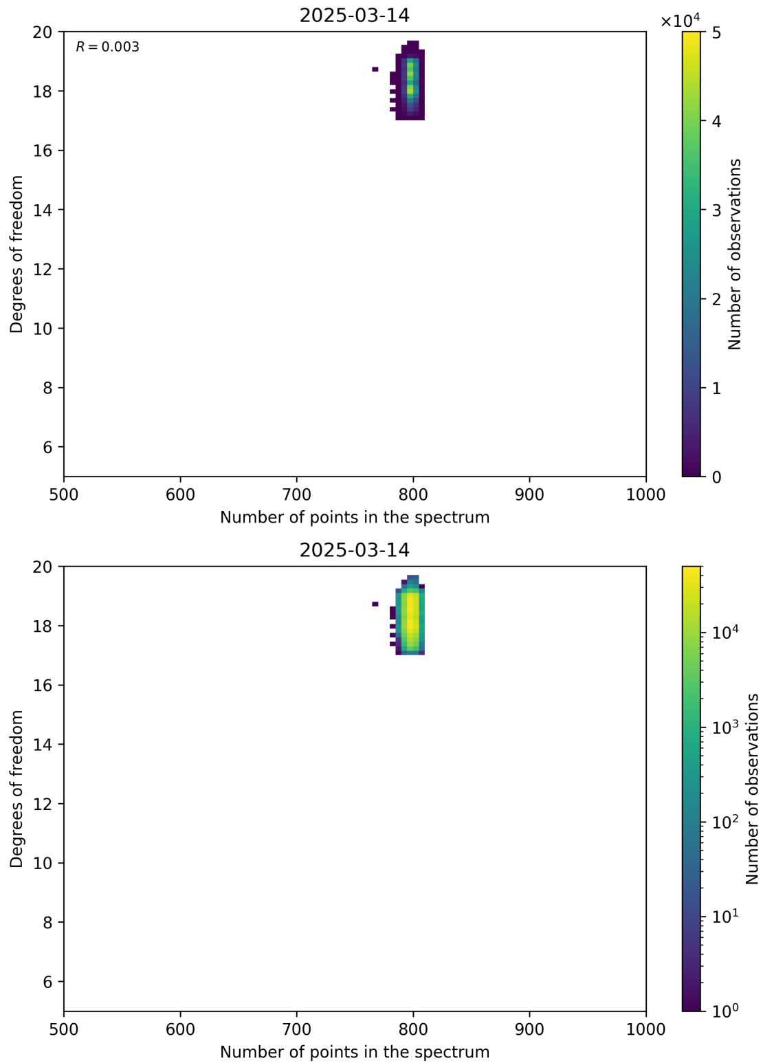
Figure 90: Scatter density plot of “Number of points in the spectrum” against “Degrees of freedom” for 2025-03-13 to 2025-03-15.
