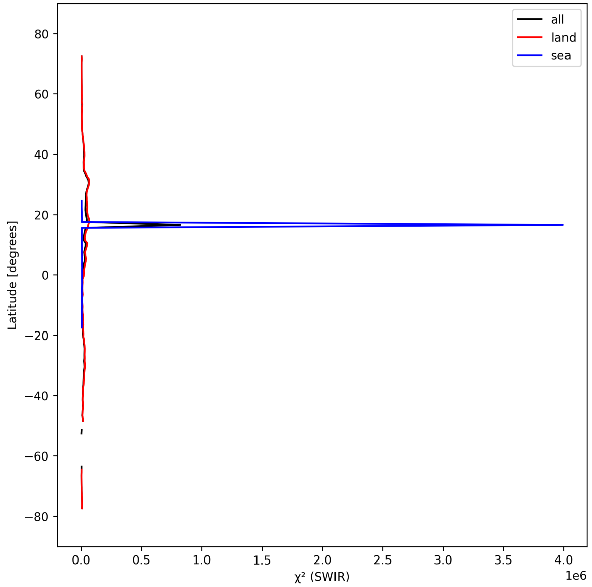
Figure 17: Zonal average of “ \chi^2 (SWIR)” for 2025-03-13 to 2025-03-15.
