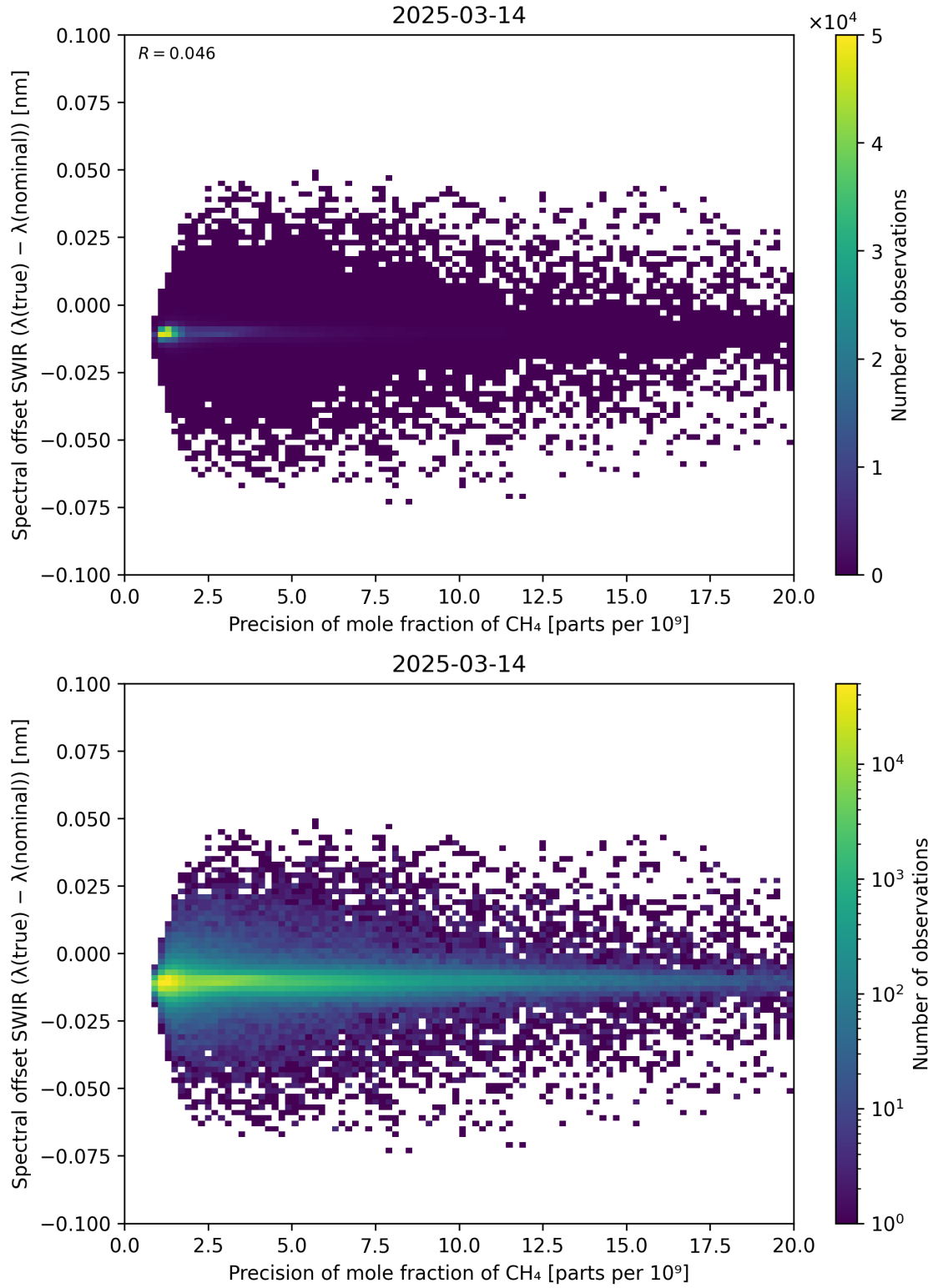
Figure 85: Scatter density plot of “Precision of mole fraction of CH 4 ” against “Spectral offset SWIR ( \lambda_{\text{true}} - \lambda_{\text{nominal}} )” for 2025-03-13 to 2025-03-15.
