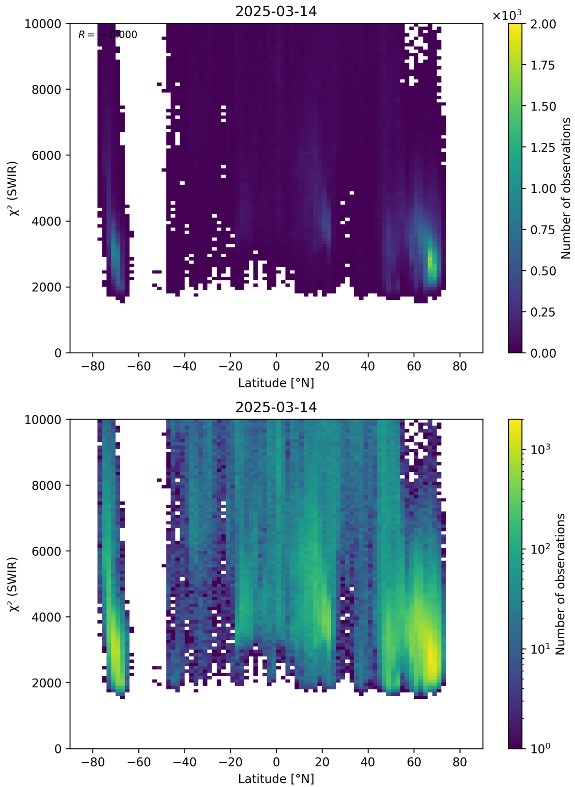
Figure 54: Scatter density plot of “Latitude” against “ \chi^2 (SWIR)” for 2025-03-13 to 2025-03-15.
