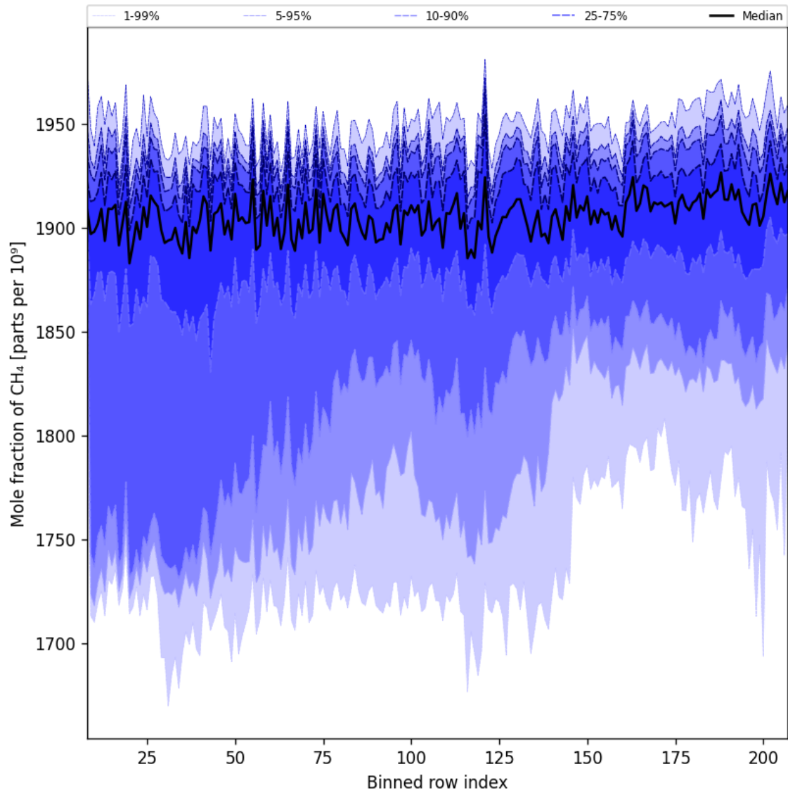
Figure 34: Along track statistics of “Mole fraction of CH 4 ” for 2025-03-13 to 2025-03-15
