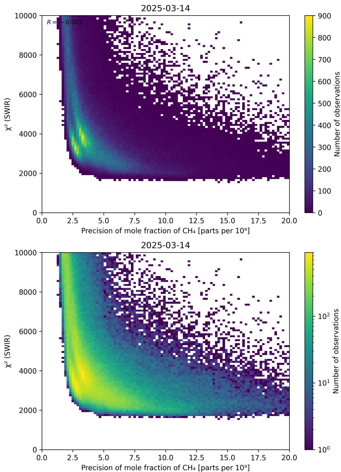
Figure 79: Scatter density plot of “Precision of mole fraction of CH 4 ” against “ \chi^2 (SWIR)” for 2025-03-13 to 2025-03-15.
