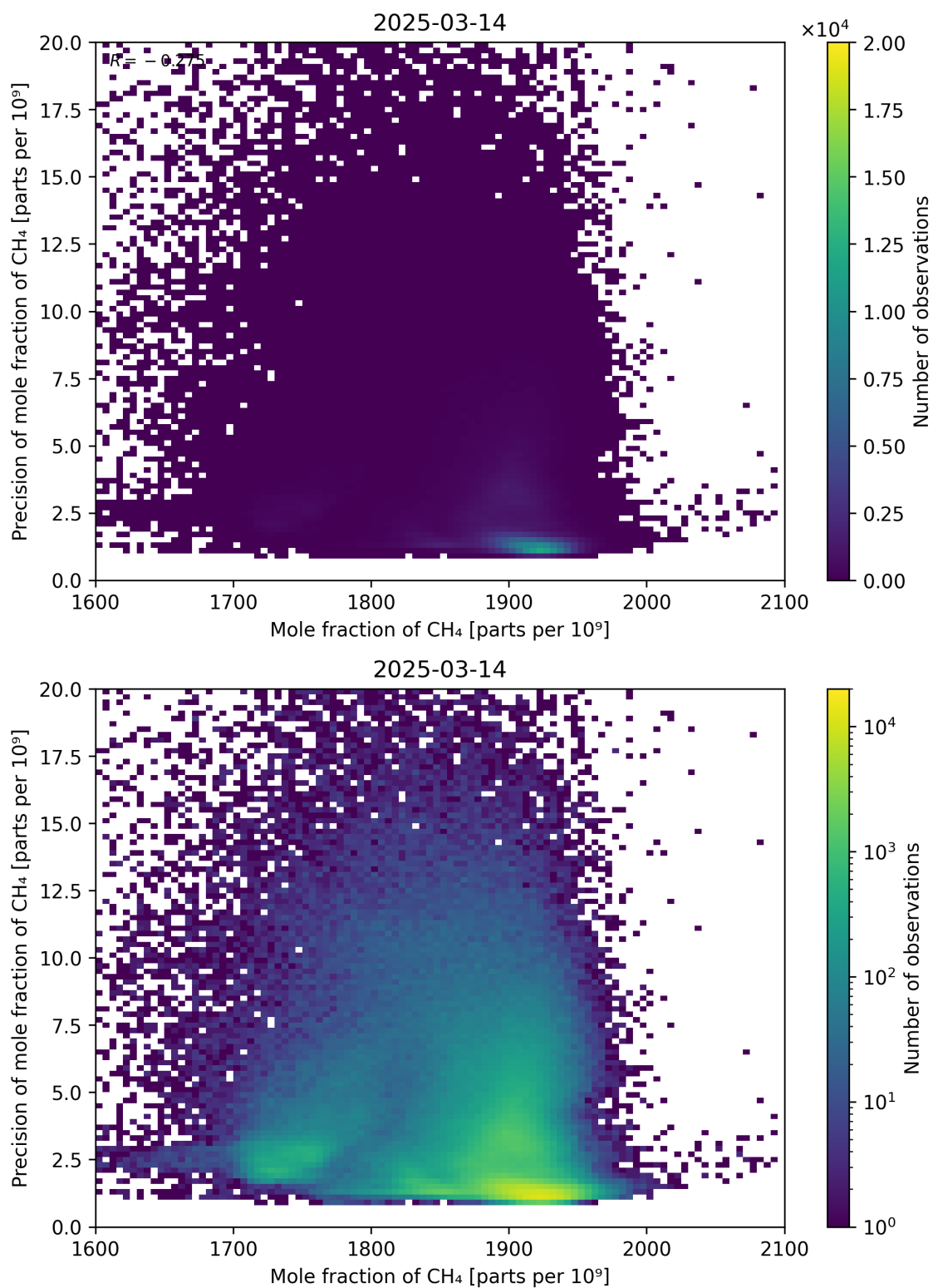
Figure 75: Scatter density plot of “Mole fraction of CH 4 ” against “Precision of mole fraction of CH 4 ” for 2025-03-13 to 2025-03-15.
