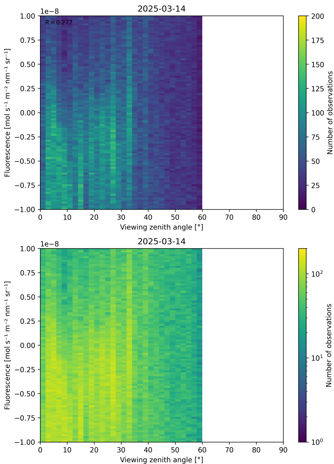
Figure 108: Scatter density plot of “Viewing zenith angle” against “Fluorescence” for 2025-03-13 to 2025-03-15.
