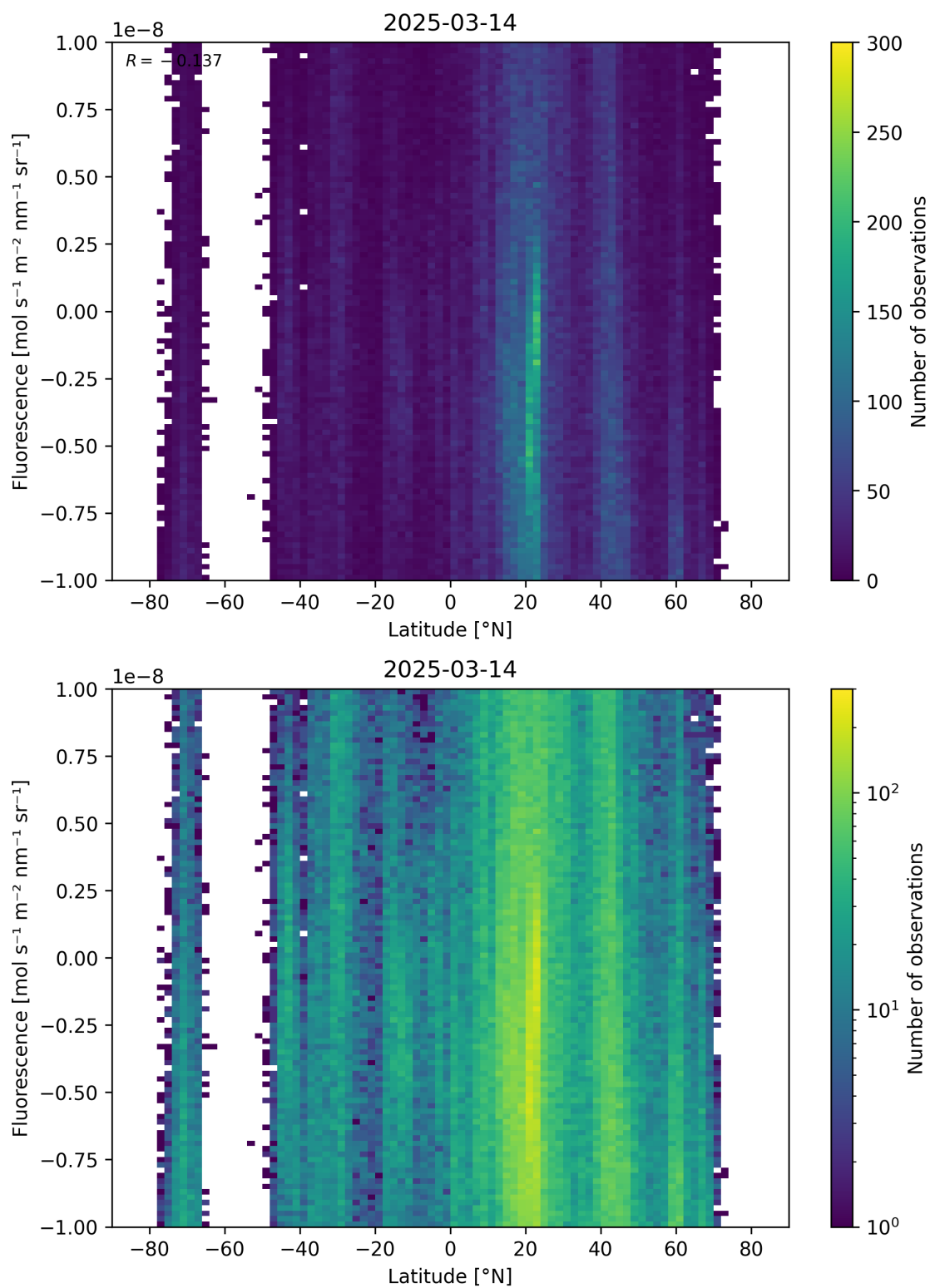
Figure 56: Scatter density plot of “Latitude” against “Fluorescence” for 2025-03-13 to 2025-03-15.
