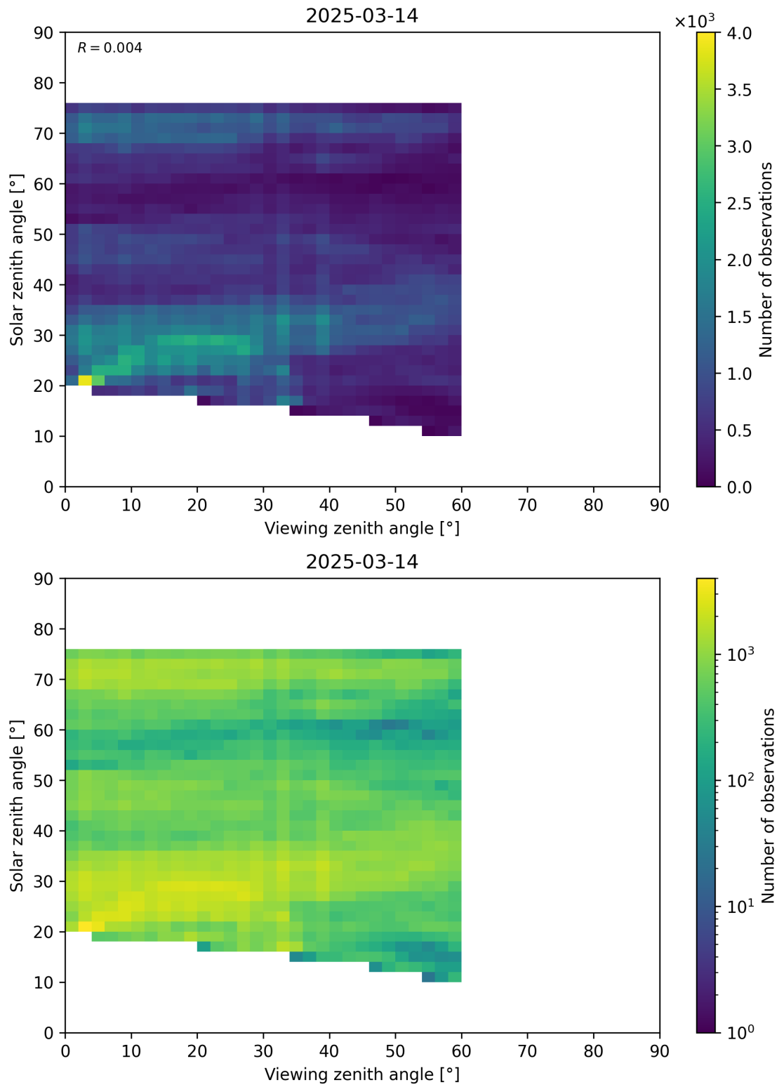
Figure 115: Scatter density plot of “Viewing zenith angle” against “Solar zenith angle” for 2025-03-13 to 2025-03-15.
