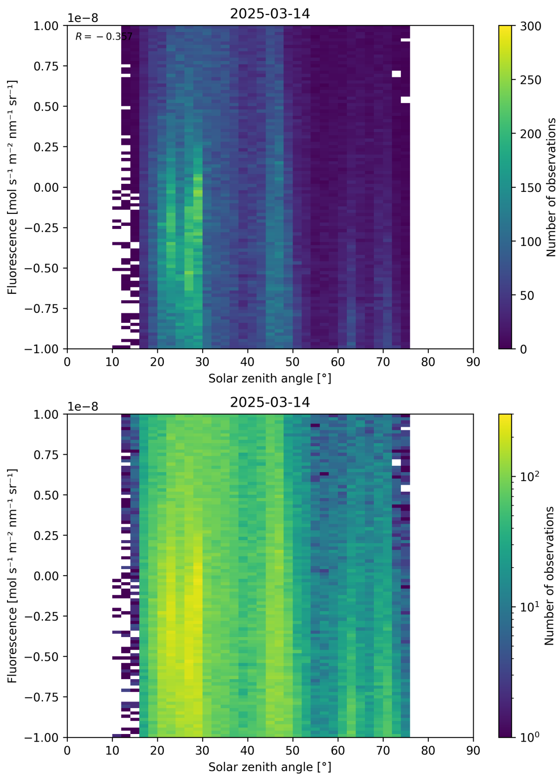
Figure 97: Scatter density plot of “Solar zenith angle” against “Fluorescence” for 2025-03-13 to 2025-03-15.
