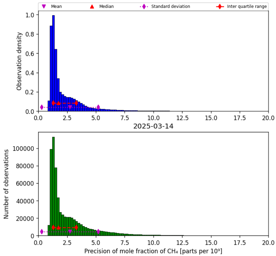
Figure 24: Histogram of “Precision of mole fraction of CH 4 ” for 2025-03-13 to 2025-03-15
