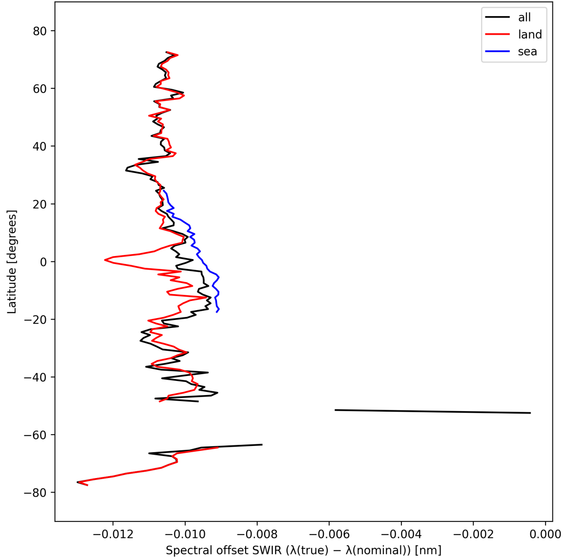
Figure 16: Zonal average of “Spectral offset SWIR ( \lambda_{\text{true}} - \lambda_{\text{nominal}} )” for 2025-03-13 to 2025-03-15.
