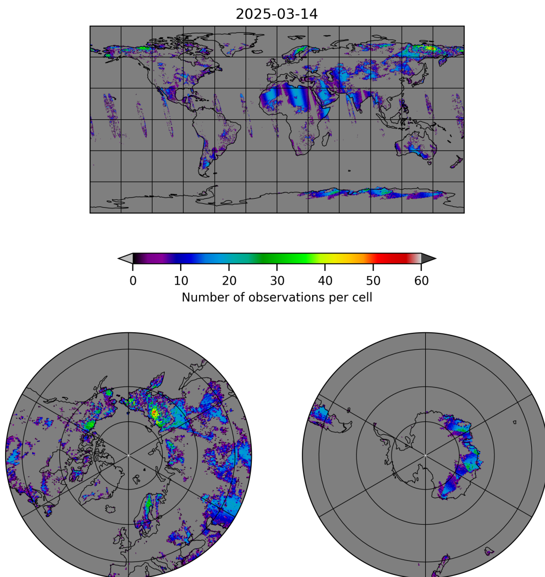
Figure 10: Map of the number of observations for 2025-03-13 to 2025-03-15
