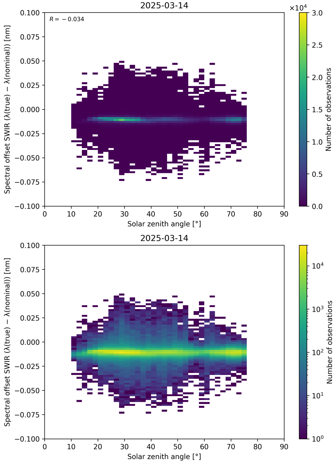
Figure 104: Scatter density plot of “Solar zenith angle” against “Spectral offset SWIR ( \lambda_{\text{true}} - \lambda_{\text{nominal}} )” for 2025-03-13 to 2025-03-15.
