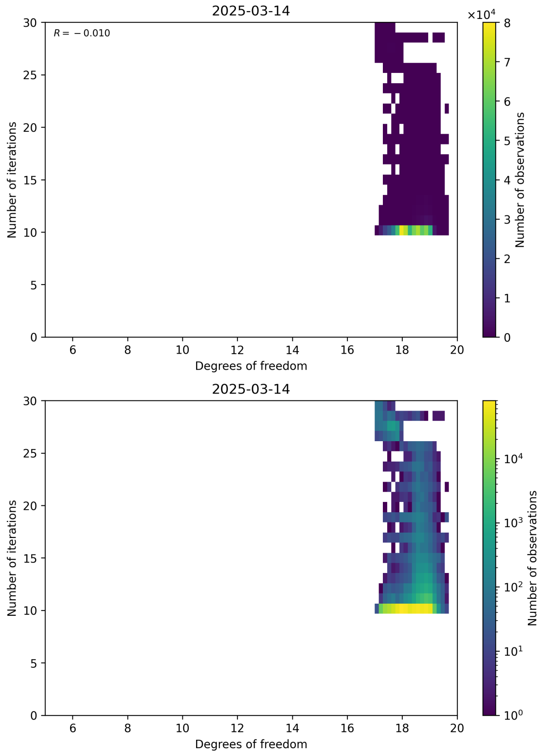
Figure 52: Scatter density plot of “Degrees of freedom” against “Number of iterations” for 2025-03-13 to 2025-03-15.
