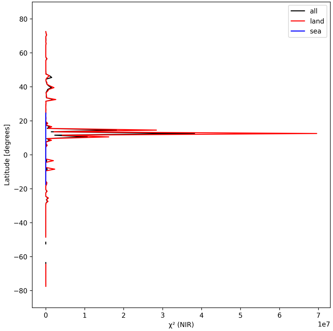
Figure 18: Zonal average of “ \chi^2 (NIR)” for 2025-03-13 to 2025-03-15.
