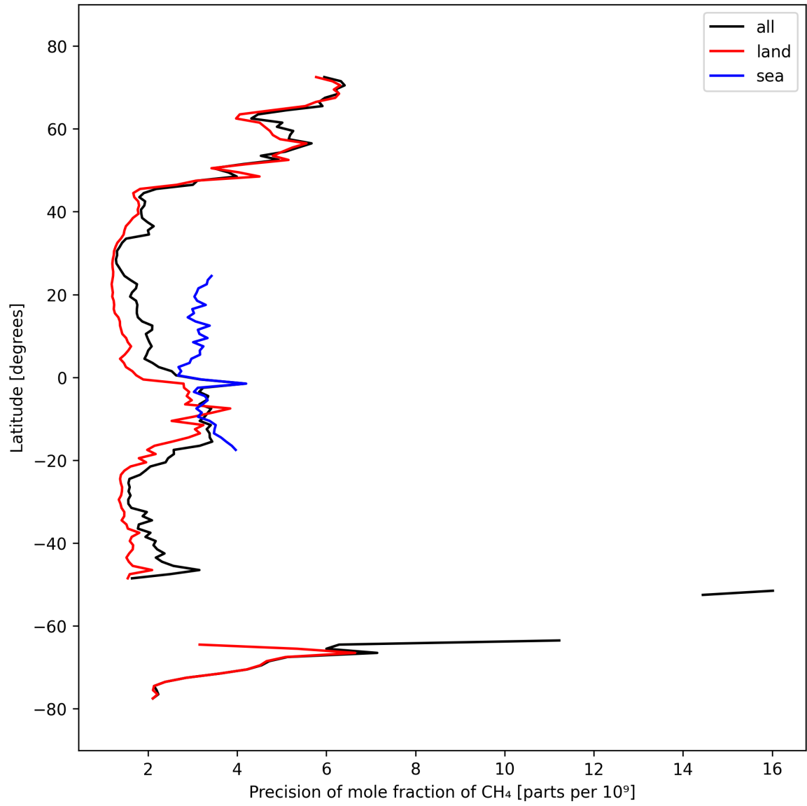
Figure 13: Zonal average of “Precision of mole fraction of CH 4 ” for 2025-03-13 to 2025-03-15.
