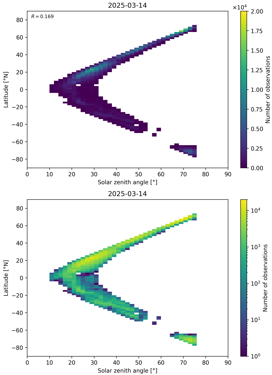
Figure 98: Scatter density plot of “Solar zenith angle” against “Latitude” for 2025-03-13 to 2025-03-15.
