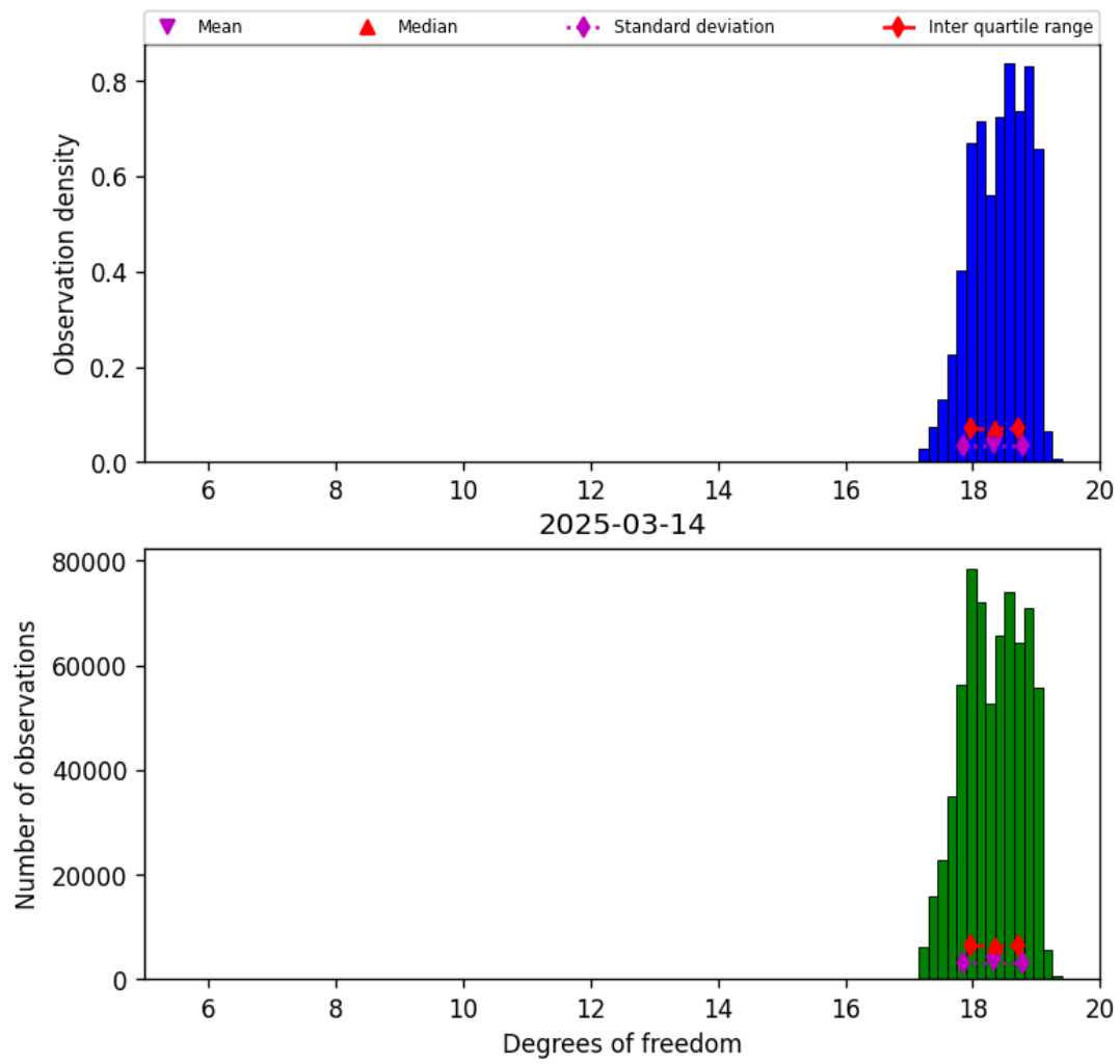
Figure 30: Histogram of “Degrees of freedom” for 2025-03-13 to 2025-03-15
