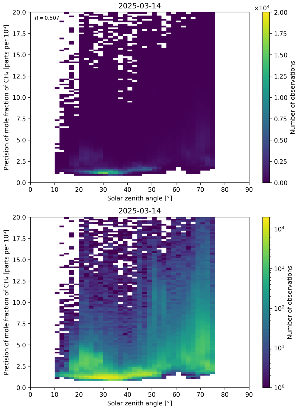
Figure 101: Scatter density plot of “Solar zenith angle” against “Precision of mole fraction of CH 4 ” for 2025-03-13 to 2025-03-15.
