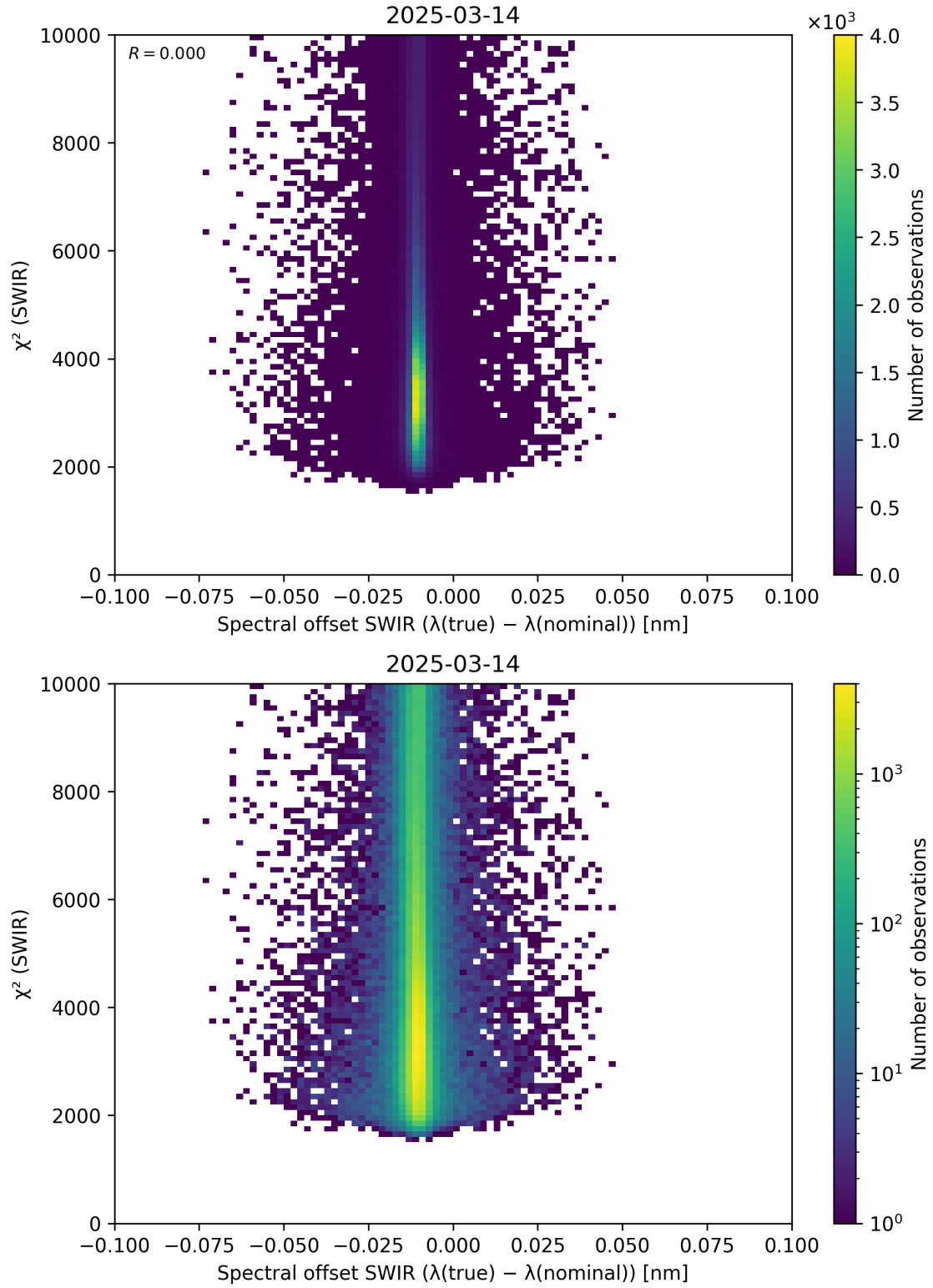
Figure 118: Scatter density plot of “Spectral offset SWIR ( \lambda_{\text{true}} - \lambda_{\text{nominal}} )” against “ \chi^2 (SWIR)” for 2025-03-13 to 2025-03-15.
