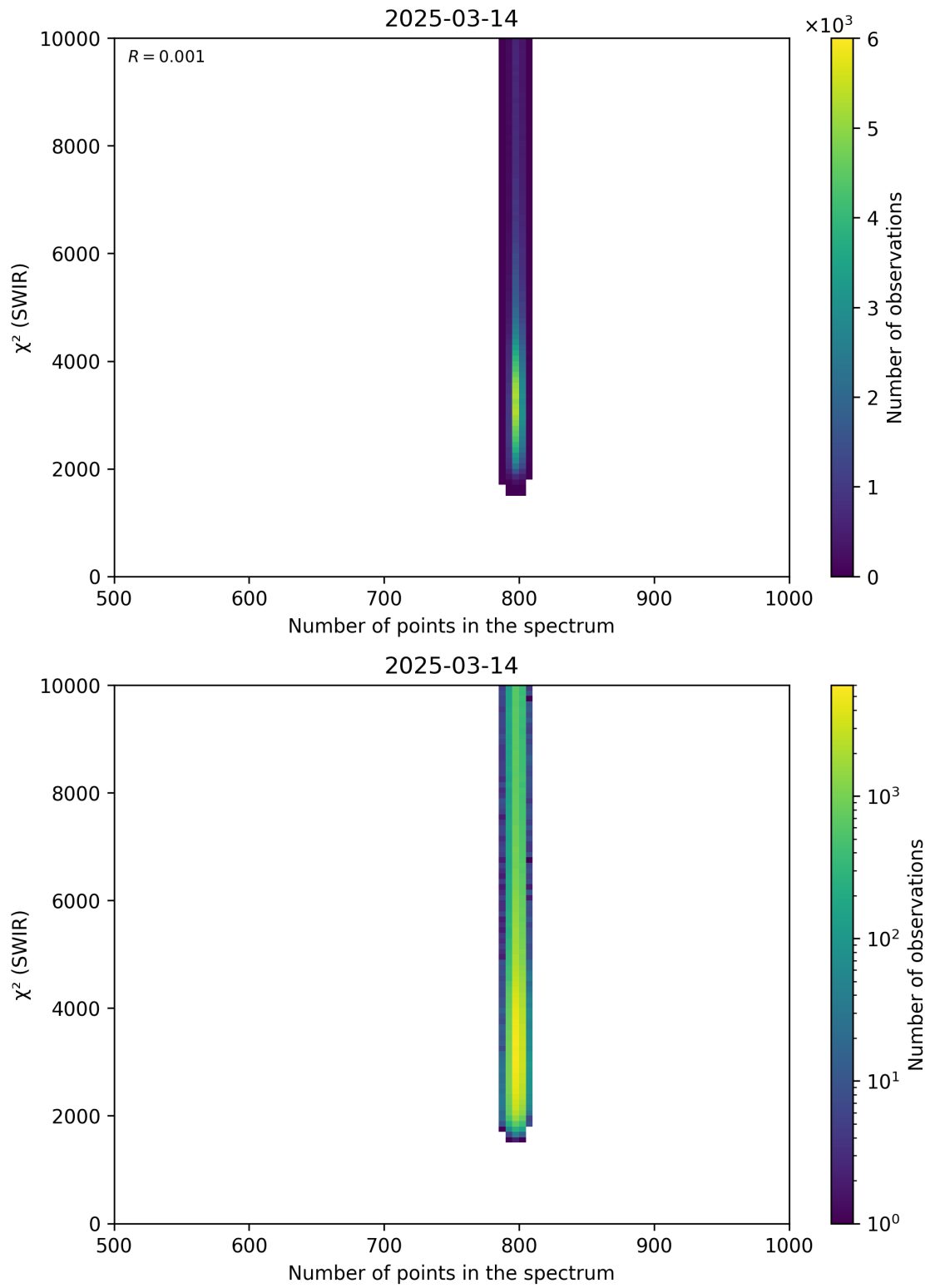
Figure 89: Scatter density plot of “Number of points in the spectrum” against “ \chi^2 (SWIR)” for 2025-03-13 to 2025-03-15.
