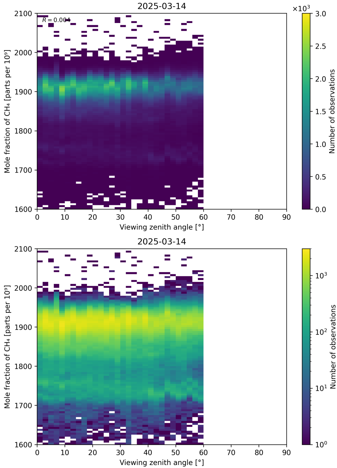
Figure 110: Scatter density plot of “Viewing zenith angle” against “Mole fraction of CH 4 ” for 2025-03-13 to 2025-03-15.
