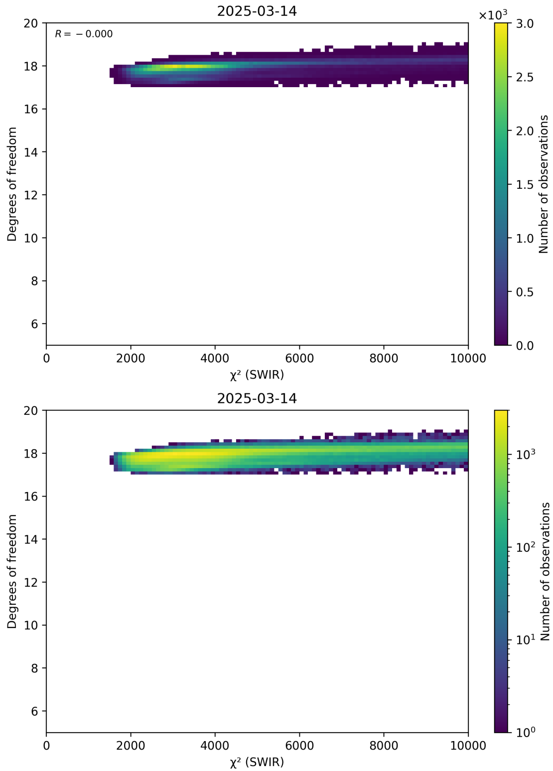
Figure 48: Scatter density plot of “ \chi^2 (SWIR)” against “Degrees of freedom” for 2025-03-13 to 2025-03-15.
