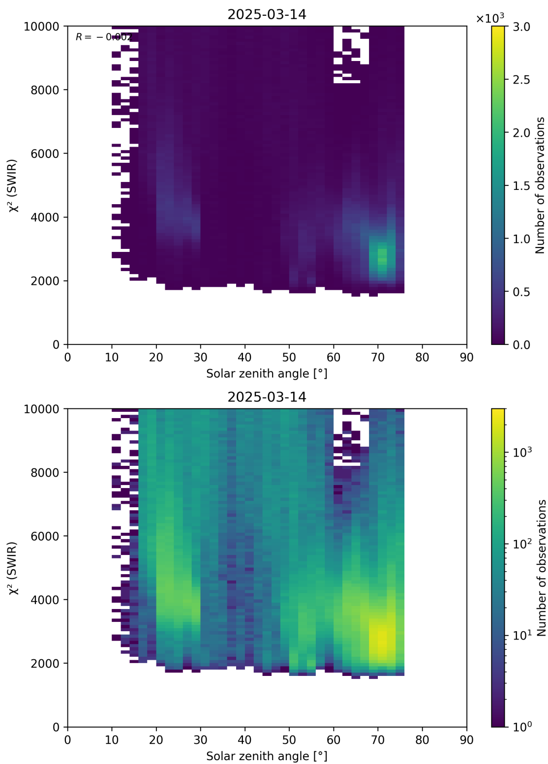
Figure 95: Scatter density plot of “Solar zenith angle” against “ \chi^2 (SWIR)” for 2025-03-13 to 2025-03-15.
