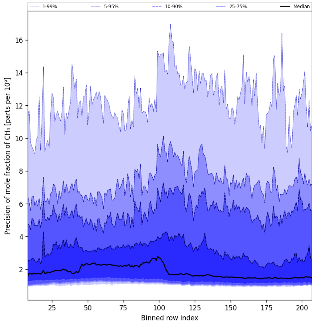
Figure 35: Along track statistics of “Precision of mole fraction of CH 4 ” for 2025-03-13 to 2025-03-15
