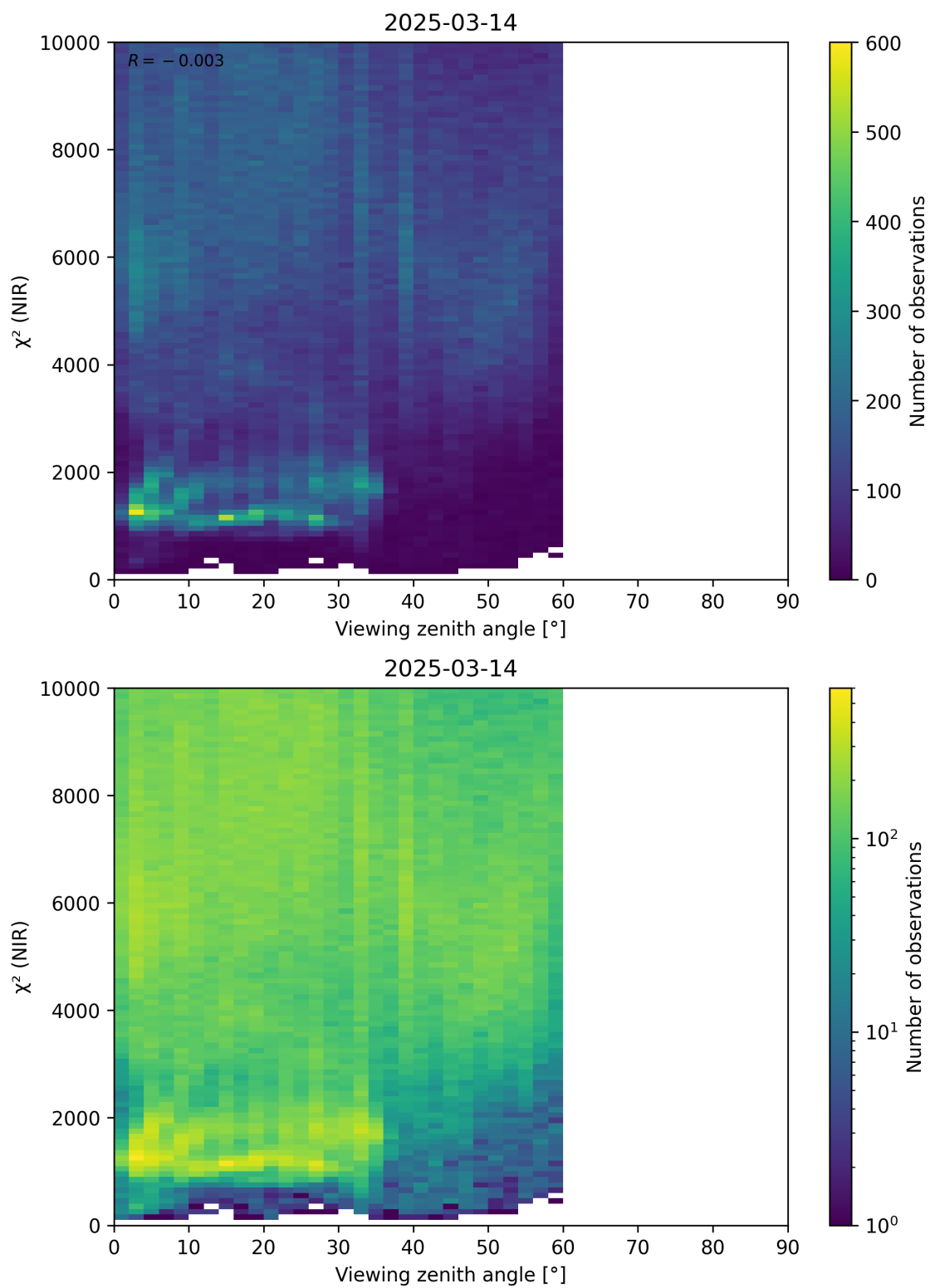
Figure 105: Scatter density plot of “Viewing zenith angle” against “ \chi^2 (NIR)” for 2025-03-13 to 2025-03-15.
