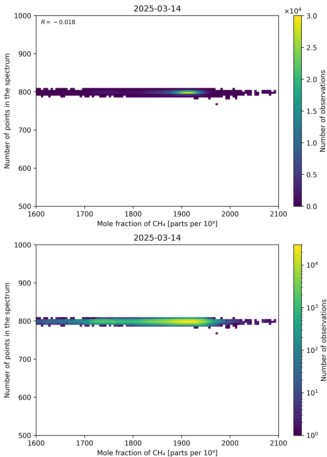
Figure 77: Scatter density plot of “Mole fraction of CH 4 ” against “Number of points in the spectrum” for 2025-03-13 to 2025-03-15.
