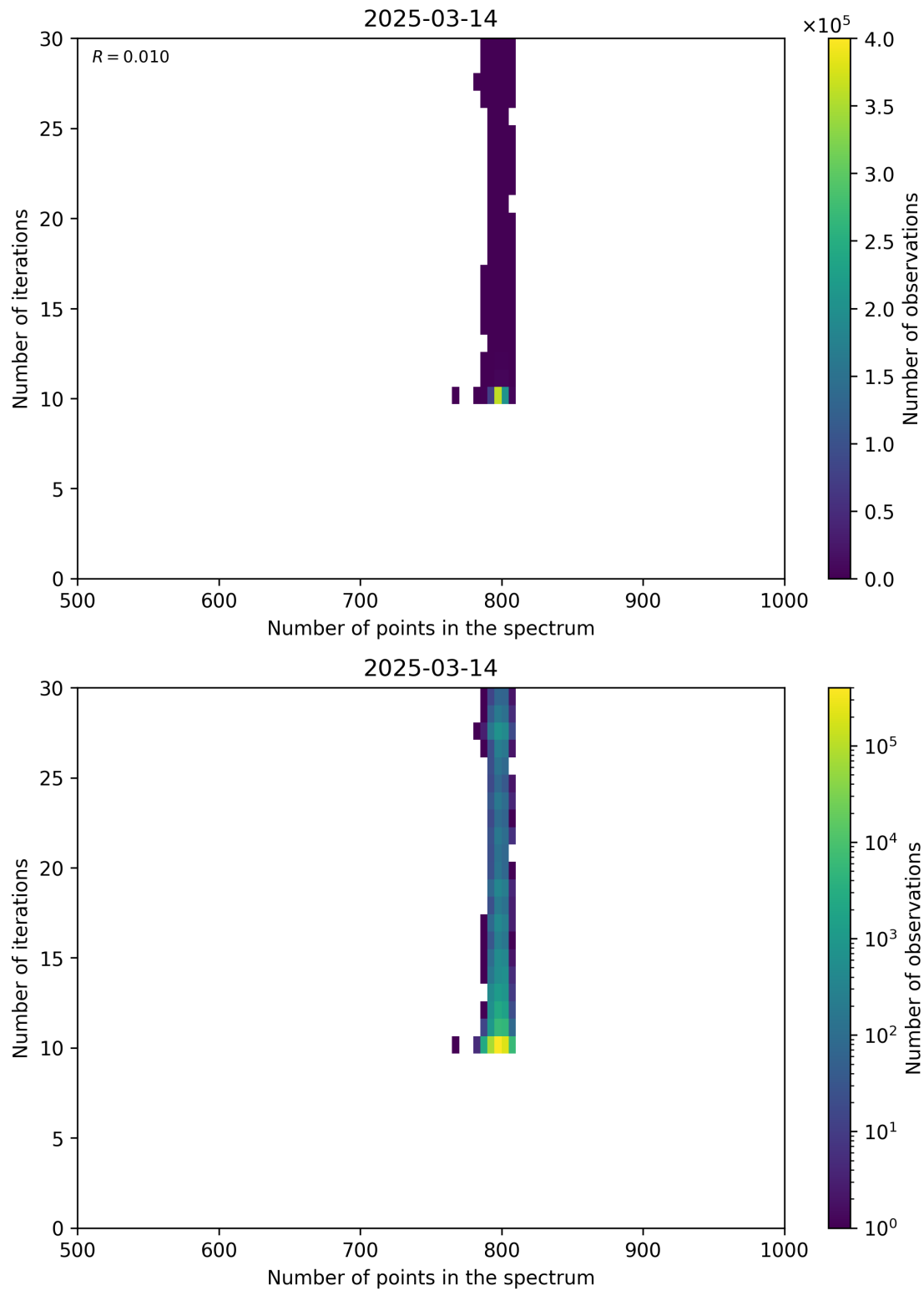
Figure 92: Scatter density plot of “Number of points in the spectrum” against “Number of iterations” for 2025-03-13 to 2025-03-15.
