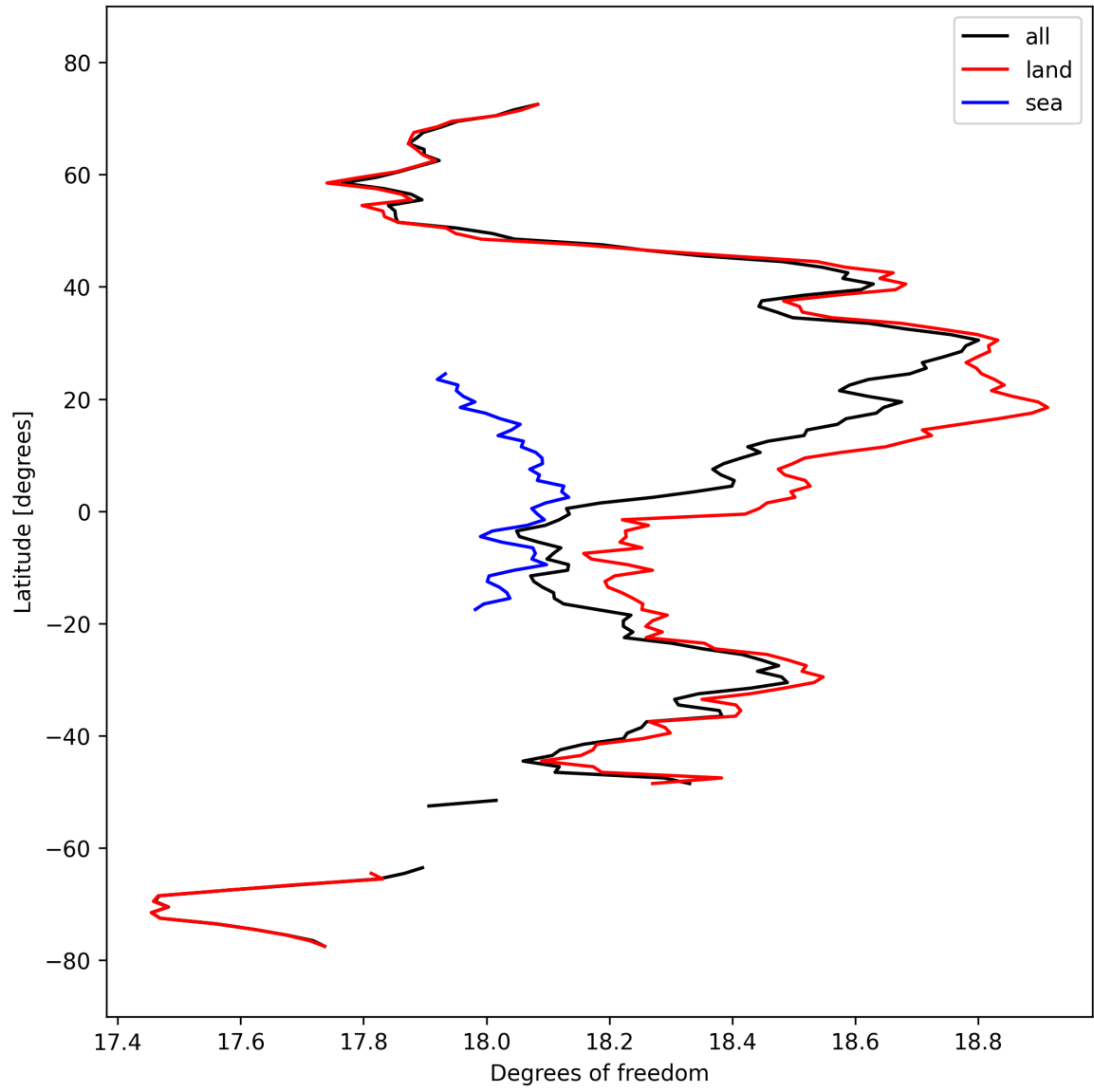
Figure 19: Zonal average of “Degrees of freedom” for 2025-03-13 to 2025-03-15.
