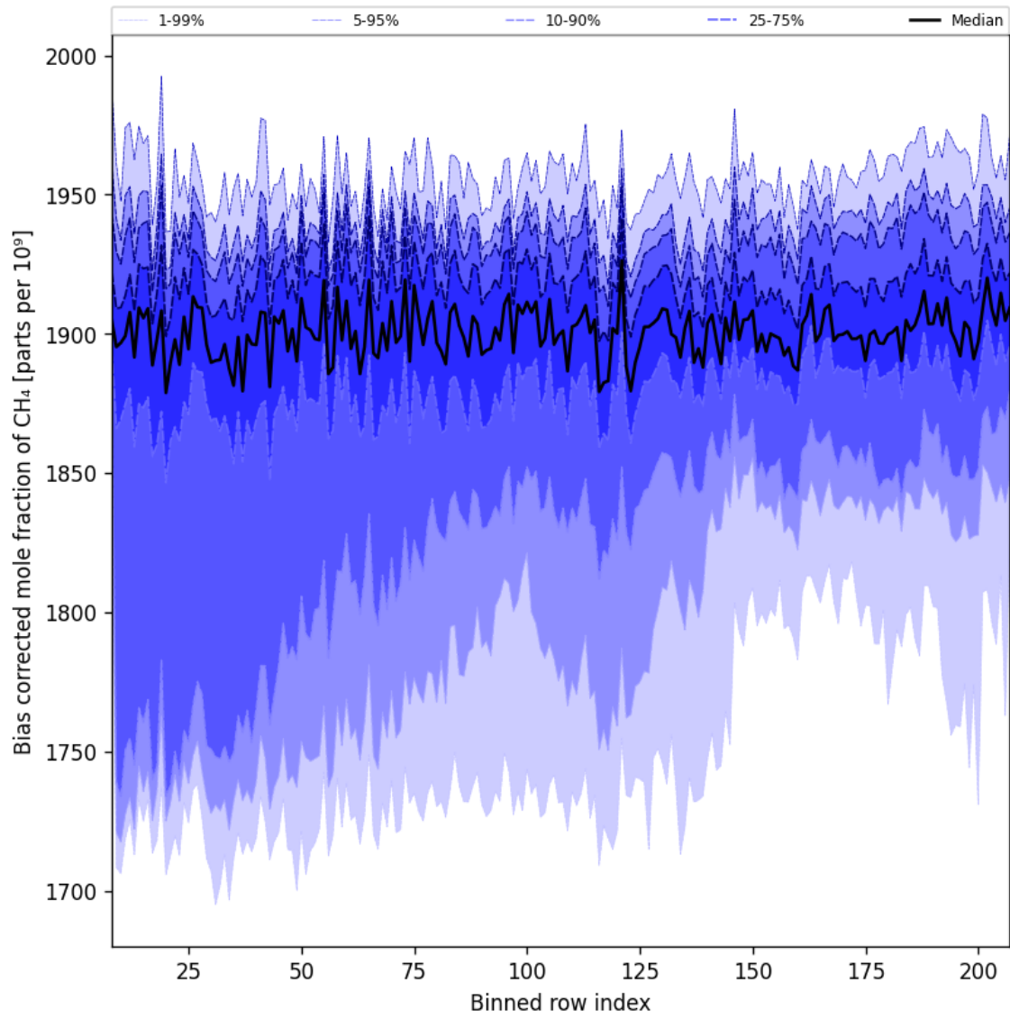
Figure 36: Along track statistics of “Bias corrected mole fraction of CH 4 ” for 2025-03-13 to 2025-03-15
