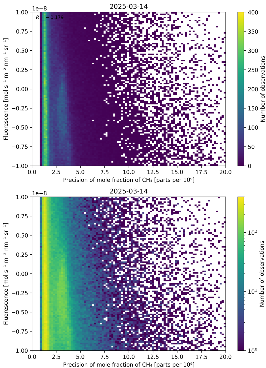
Figure 81: Scatter density plot of “Precision of mole fraction of CH 4 ” against “Fluorescence” for 2025-03-13 to 2025-03-15.
