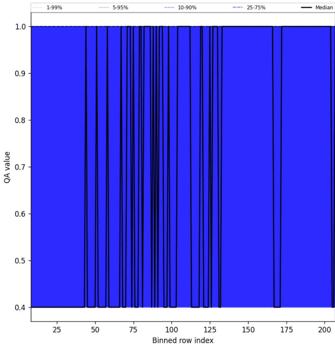
Figure 33: Along track statistics of “QA value” for 2025-03-13 to 2025-03-15
