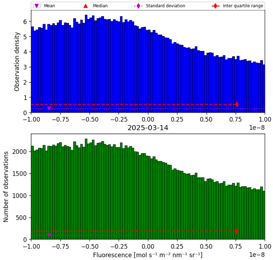
Figure 32: Histogram of “Fluorescence” for 2025-03-13 to 2025-03-15
