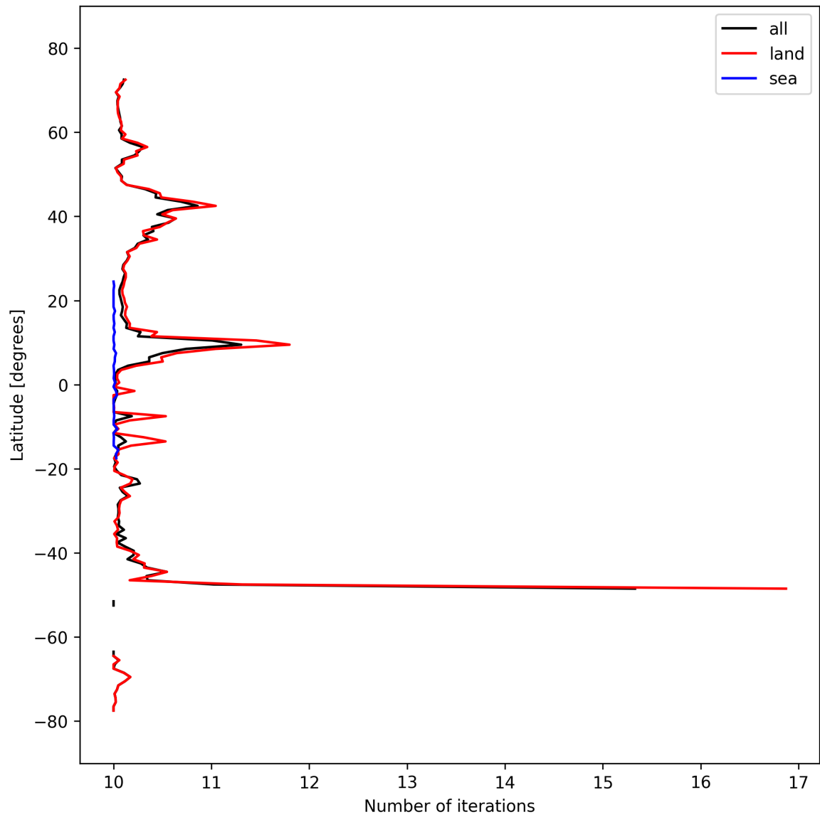
Figure 20: Zonal average of “Number of iterations” for 2025-03-13 to 2025-03-15.
