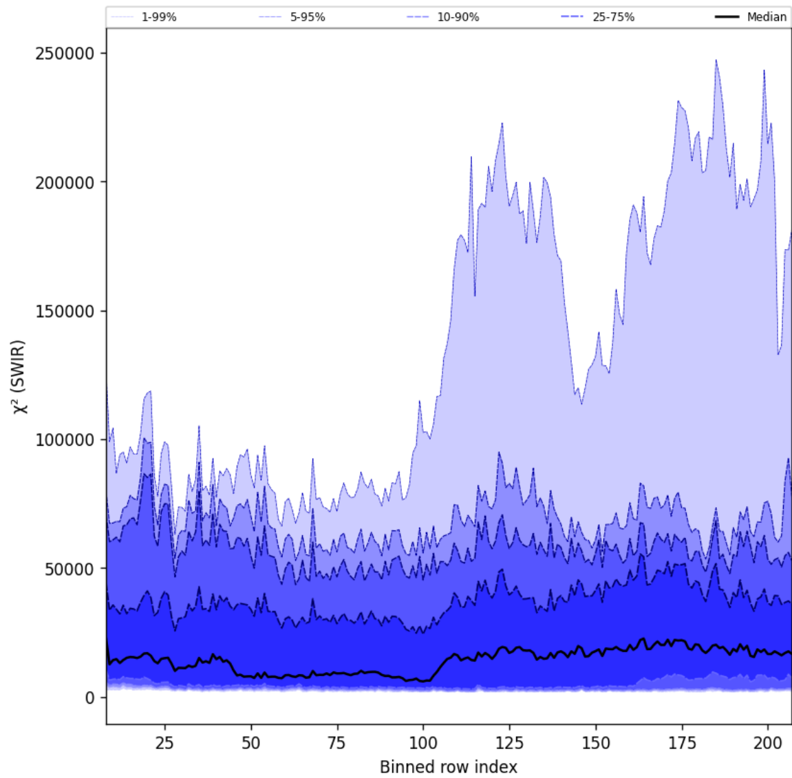
Figure 39: Along track statistics of “ \chi^2 (SWIR)” for 2025-03-13 to 2025-03-15
