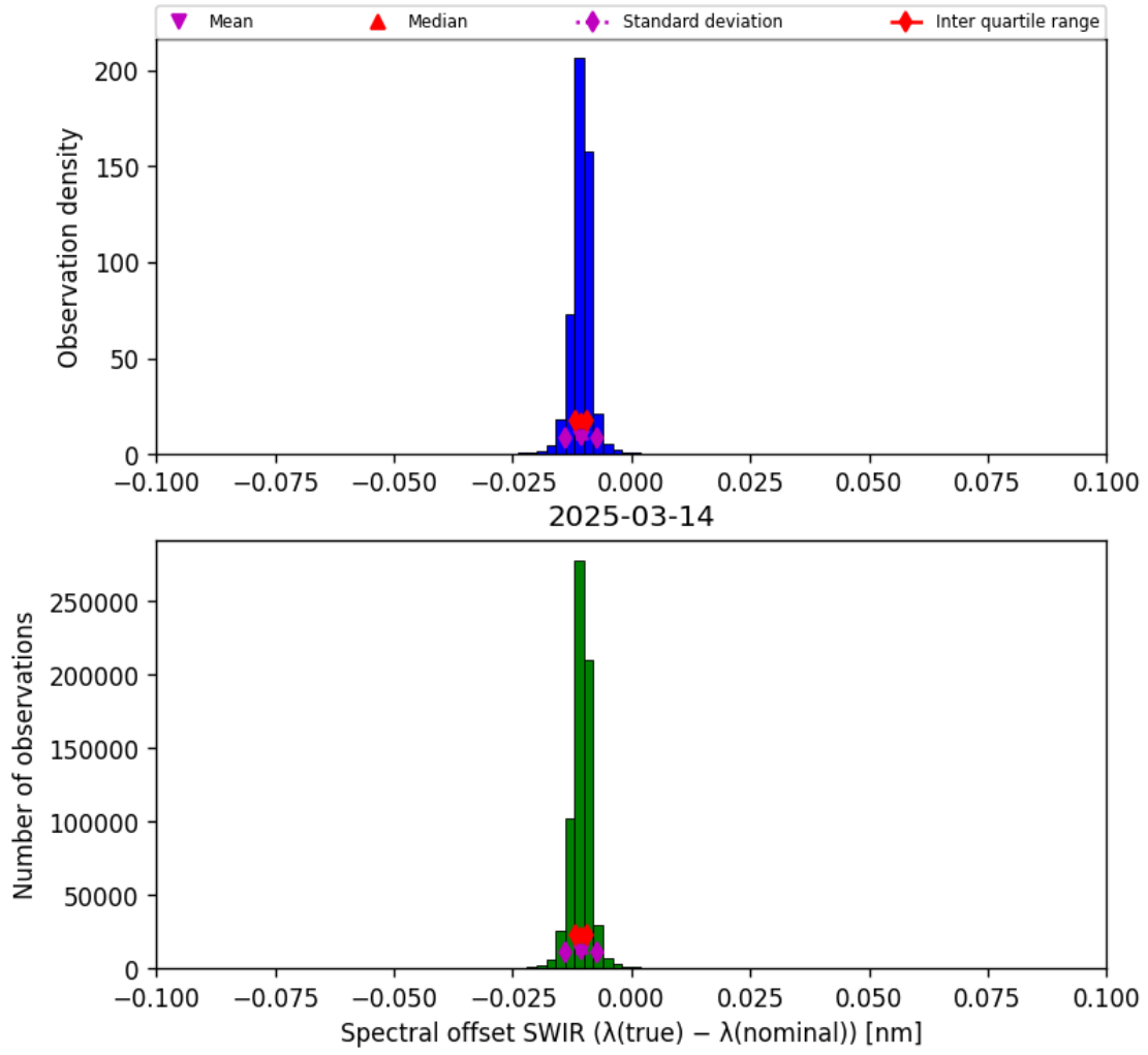
Figure 27: Histogram of “Spectral offset SWIR ( \lambda_{\text{true}} - \lambda_{\text{nominal}} )” for 2025-03-13 to 2025-03-15
