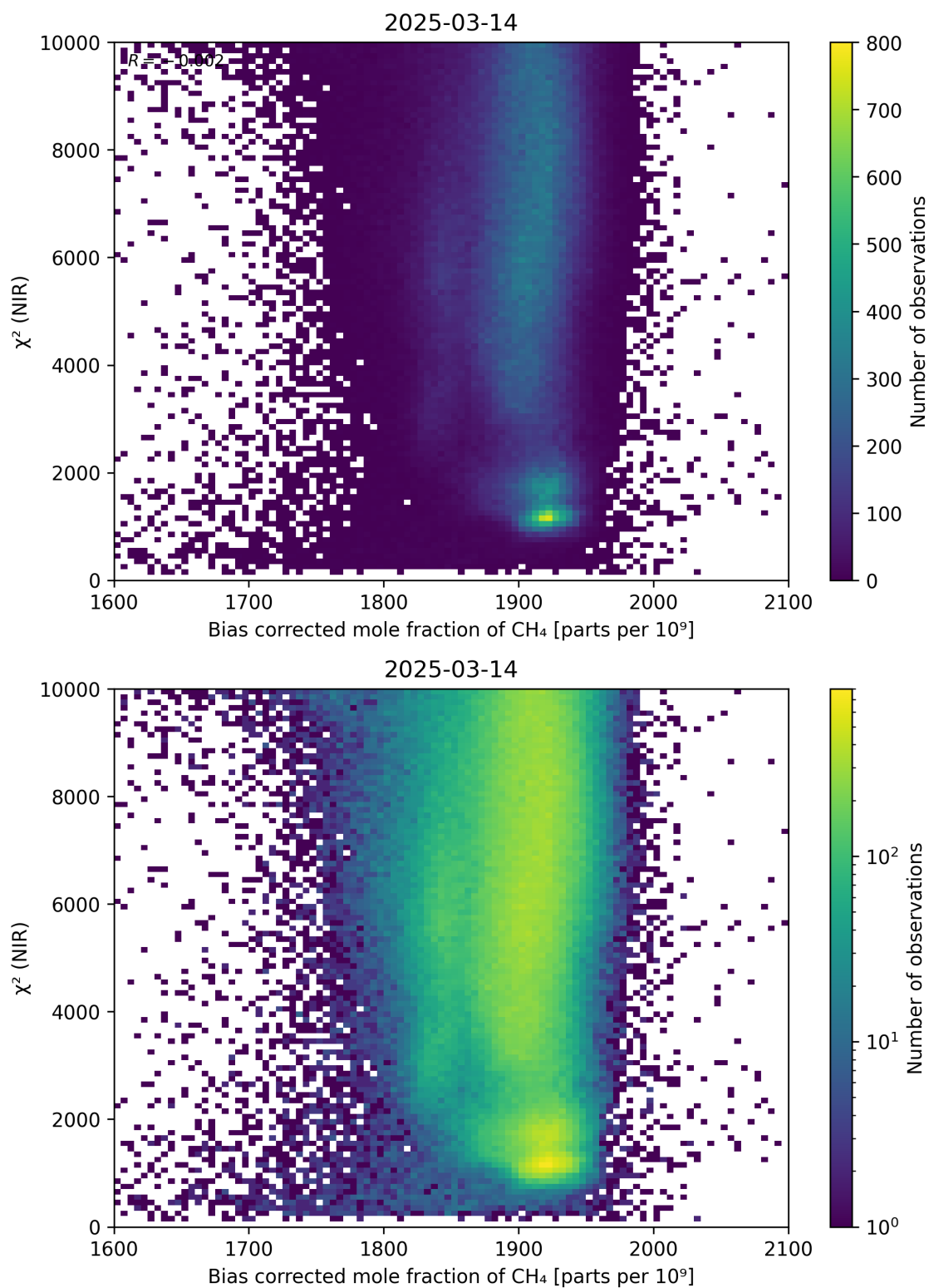
Figure 63: Scatter density plot of “Bias corrected mole fraction of \text{CH}_4 ” against “ \chi^2 (NIR)” for 2025-03-13 to 2025-03-15.
