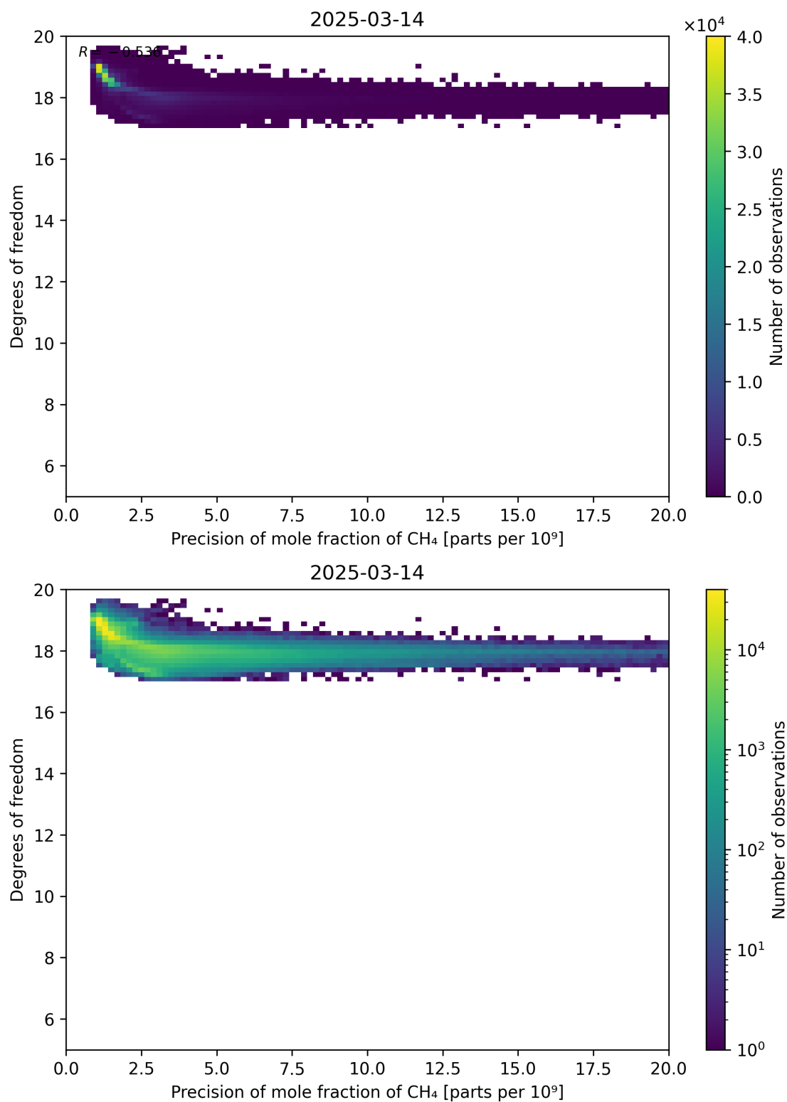
Figure 80: Scatter density plot of “Precision of mole fraction of CH 4 ” against “Degrees of freedom” for 2025-03-13 to 2025-03-15.
