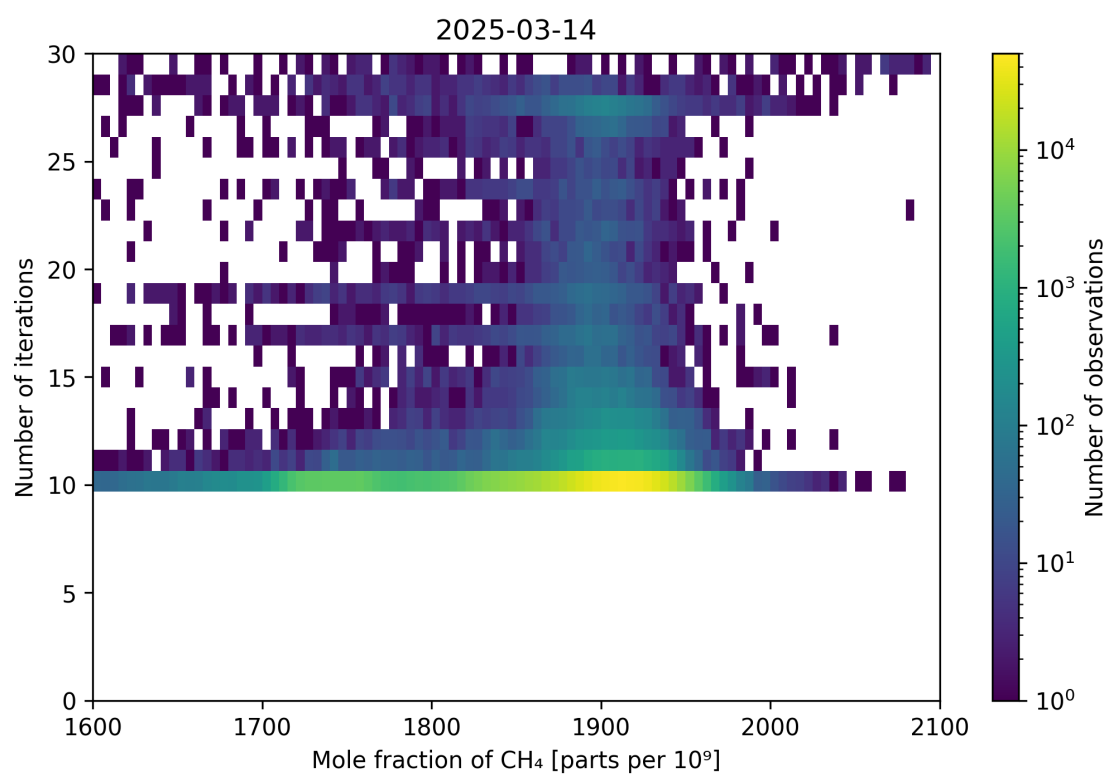
Figure 76: Scatter density plot of “Mole fraction of CH 4 ” against “Number of iterations” for 2025-03-13 to 2025-03-15.
