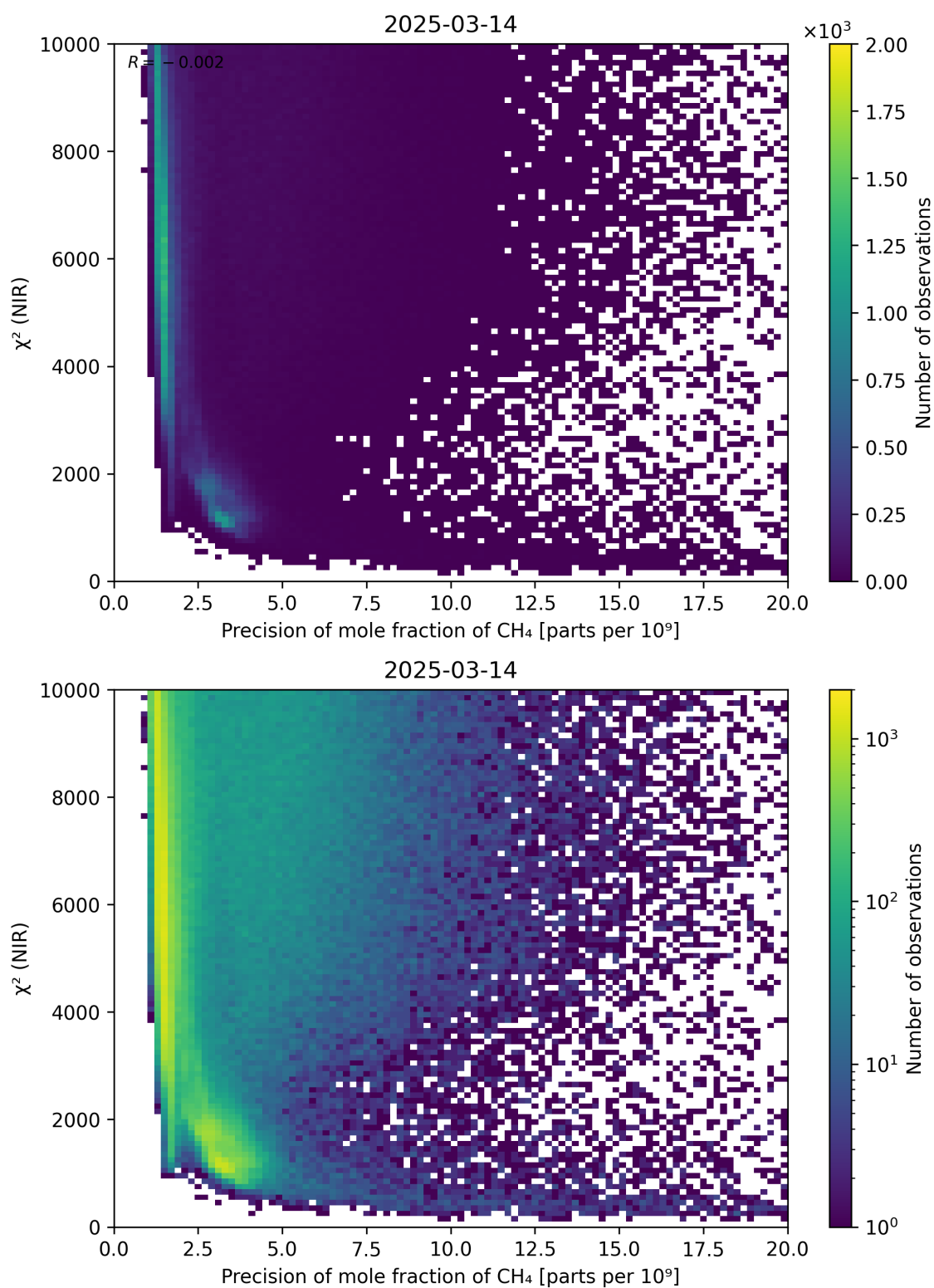
Figure 78: Scatter density plot of “Precision of mole fraction of \text{CH}_4 ” against “ \chi^2 (NIR)” for 2025-03-13 to 2025-03-15.
