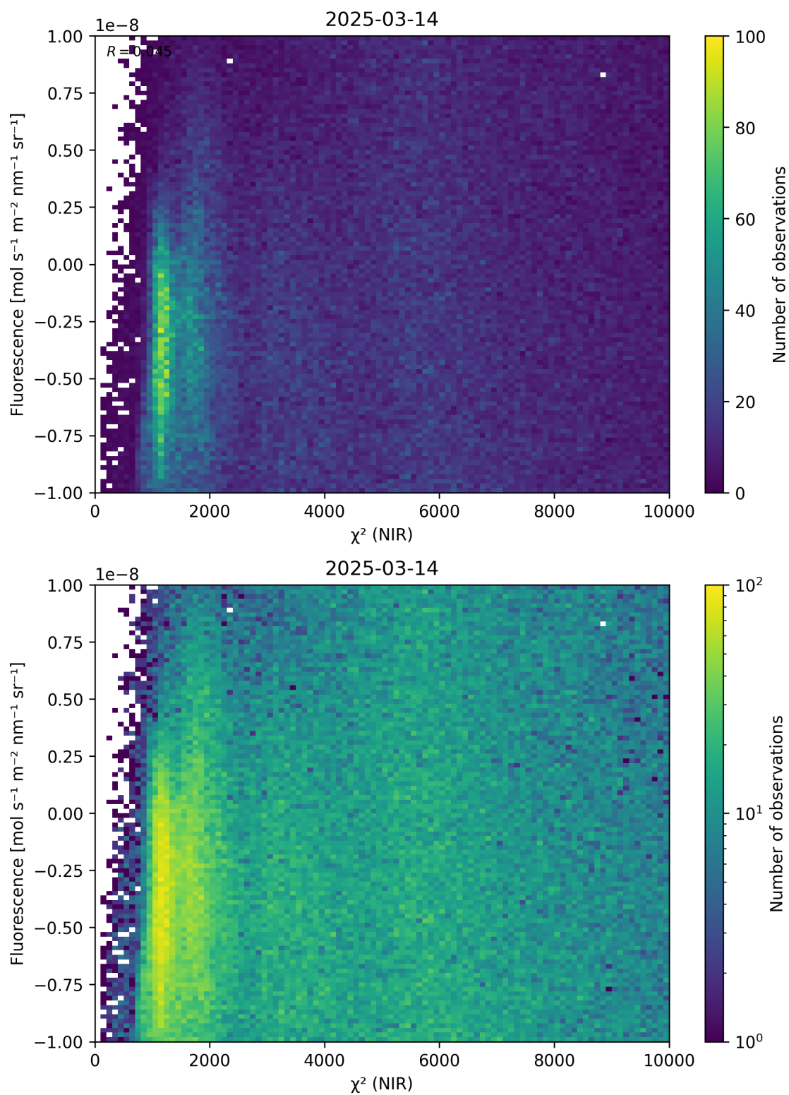
Figure 45: Scatter density plot of “ \chi^2 (NIR)” against “Fluorescence” for 2025-03-13 to 2025-03-15.
