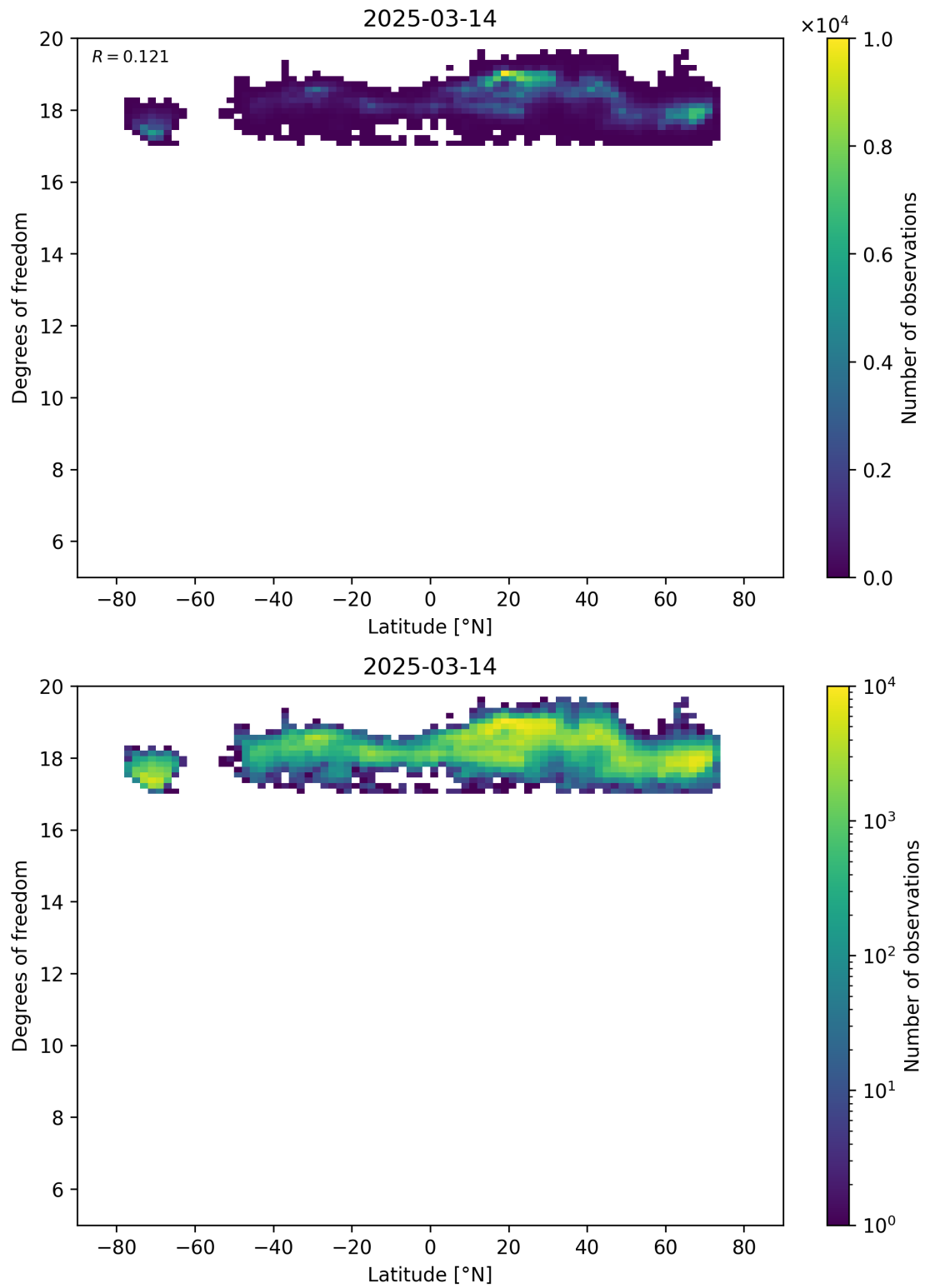
Figure 55: Scatter density plot of “Latitude” against “Degrees of freedom” for 2025-03-13 to 2025-03-15.
