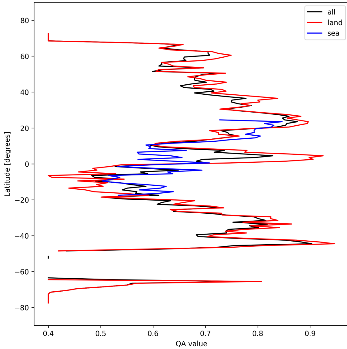
Figure 11: Zonal average of “QA value” for 2025-03-13 to 2025-03-15.
