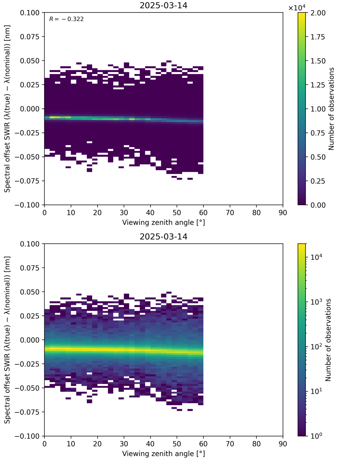
Figure 116: Scatter density plot of “Viewing zenith angle” against “Spectral offset SWIR ( \lambda_{\text{true}} - \lambda_{\text{nominal}} )” for 2025-03-13 to 2025-03-15.
