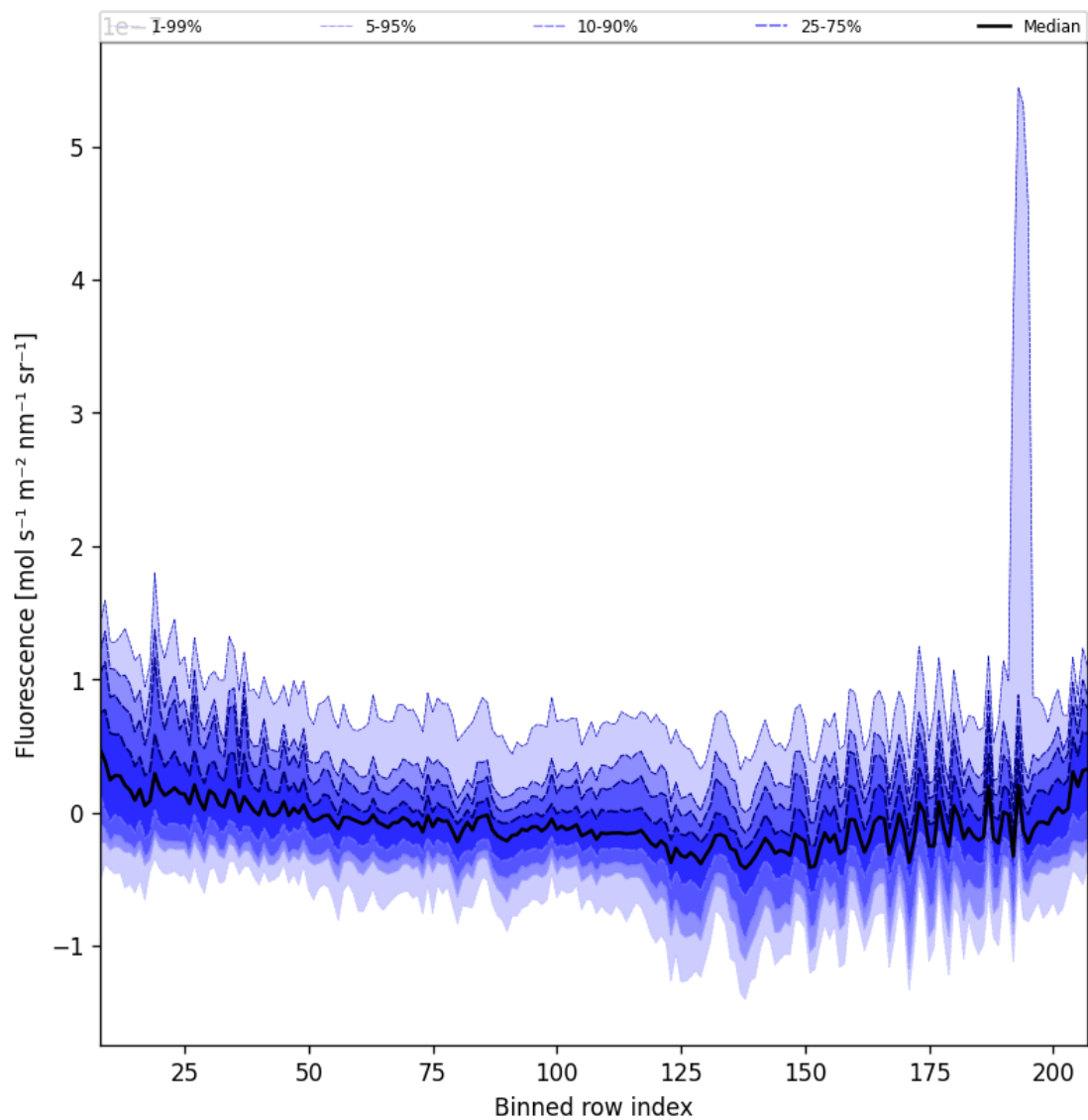
Figure 43: Along track statistics of “Fluorescence” for 2025-03-13 to 2025-03-15
