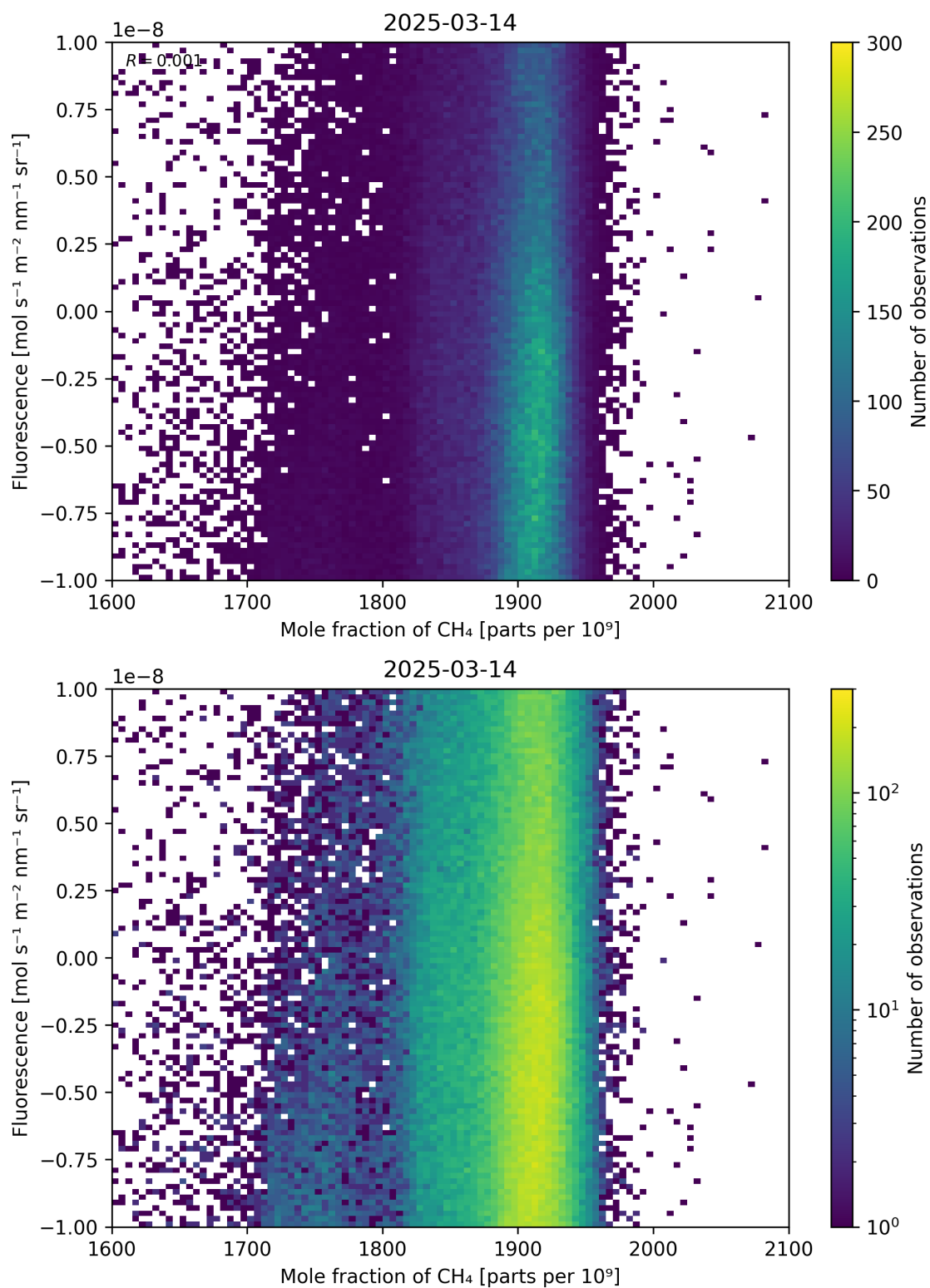
Figure 73: Scatter density plot of “Mole fraction of \text{CH}_4 ” against “Fluorescence” for 2025-03-13 to 2025-03-15.
