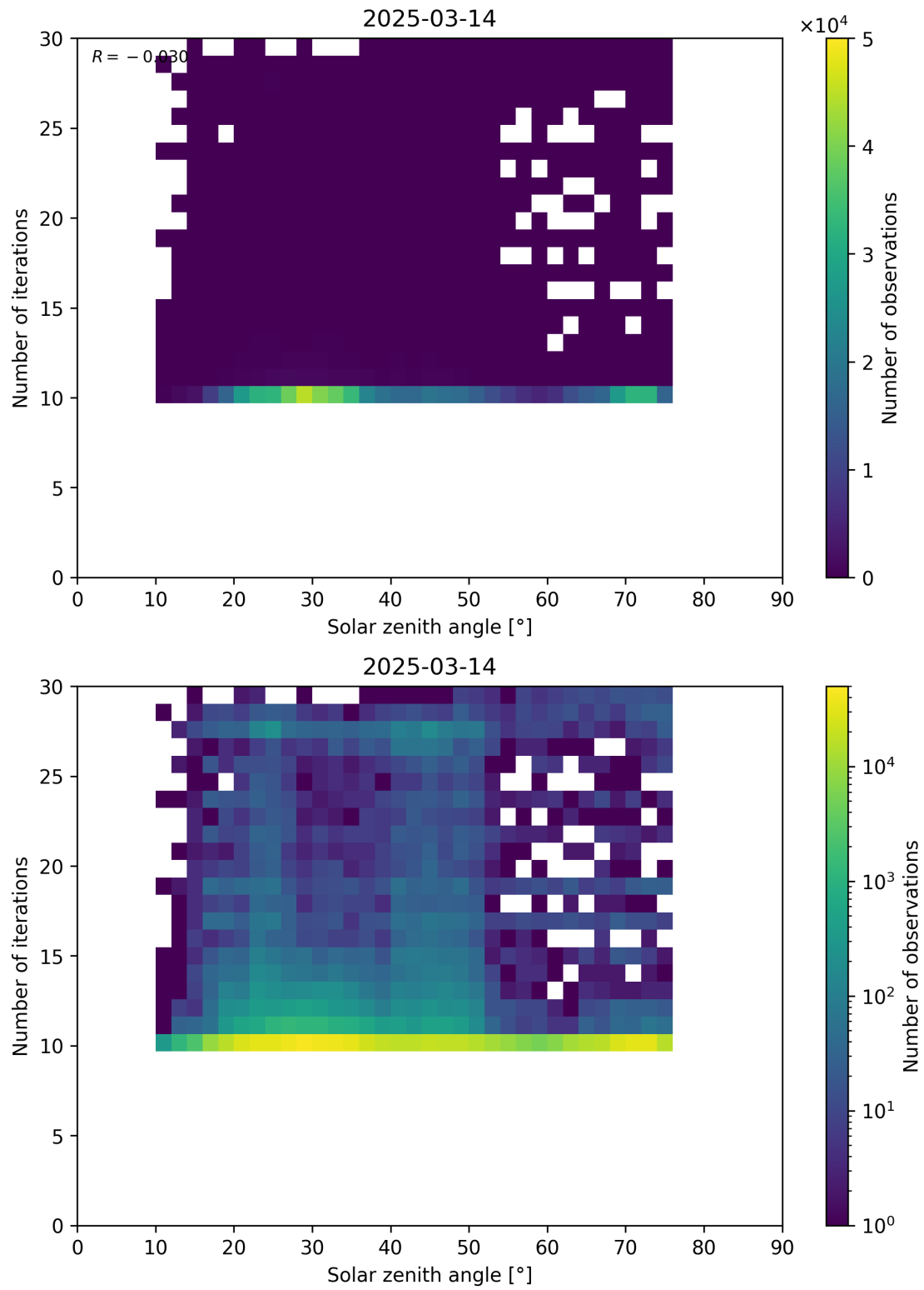
Figure 102: Scatter density plot of “Solar zenith angle” against “Number of iterations” for 2025-03-13 to 2025-03-15.
