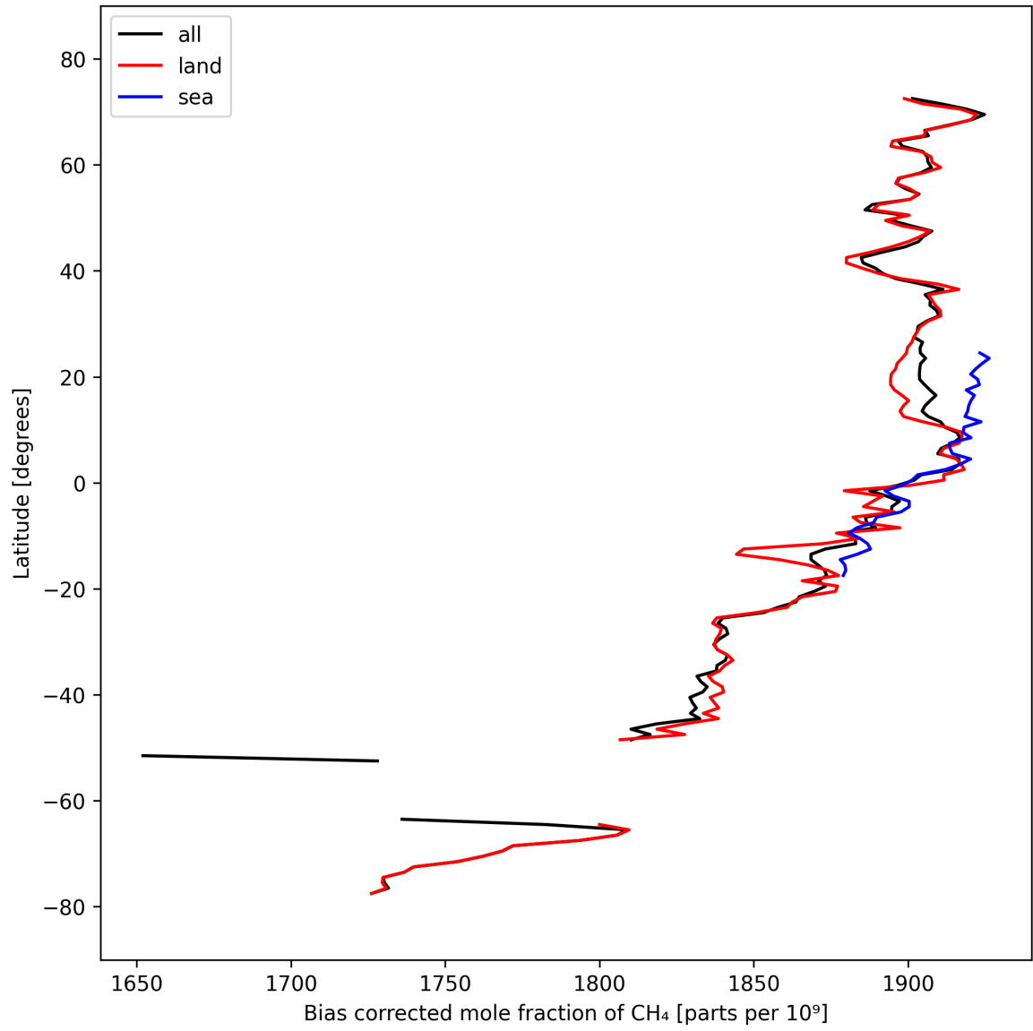
Figure 14: Zonal average of “Bias corrected mole fraction of CH 4 ” for 2025-03-13 to 2025-03-15.
