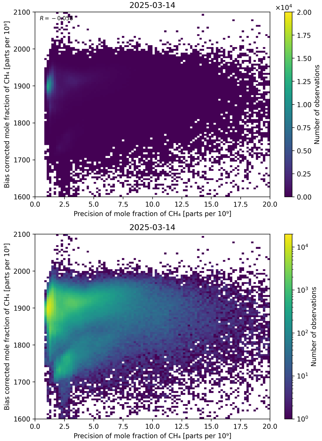
Figure 82: Scatter density plot of “Precision of mole fraction of CH 4 ” against “Bias corrected mole fraction of CH 4 ” for 2025-03-13 to 2025-03-15.
