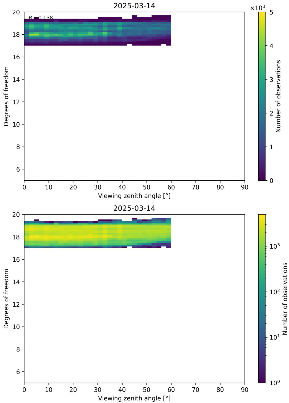
Figure 107: Scatter density plot of “Viewing zenith angle” against “Degrees of freedom” for 2025-03-13 to 2025-03-15.
