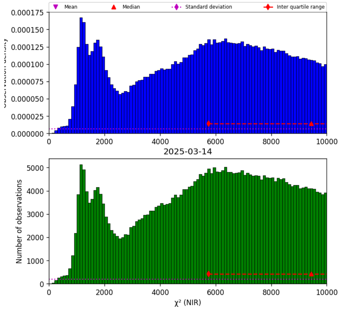
Figure 29: Histogram of “ \chi^2 (NIR)” for 2025-03-13 to 2025-03-15
