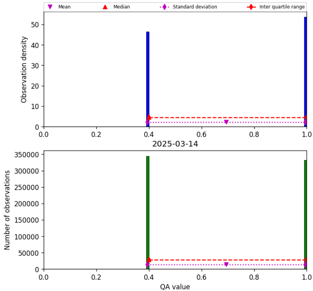
Figure 22: Histogram of “QA value” for 2025-03-13 to 2025-03-15
