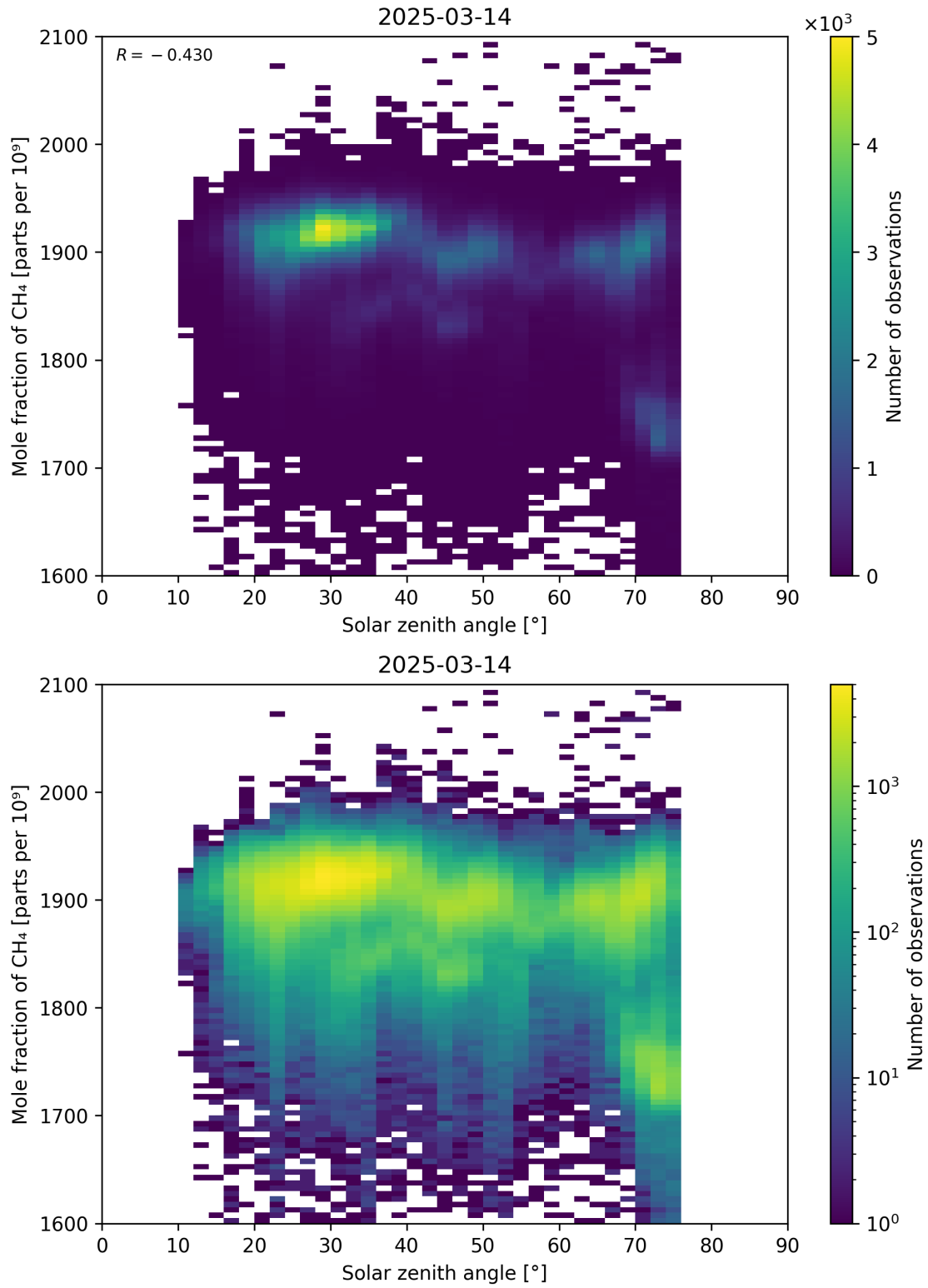
Figure 99: Scatter density plot of “Solar zenith angle” against “Mole fraction of CH 4 ” for 2025-03-13 to 2025-03-15.
