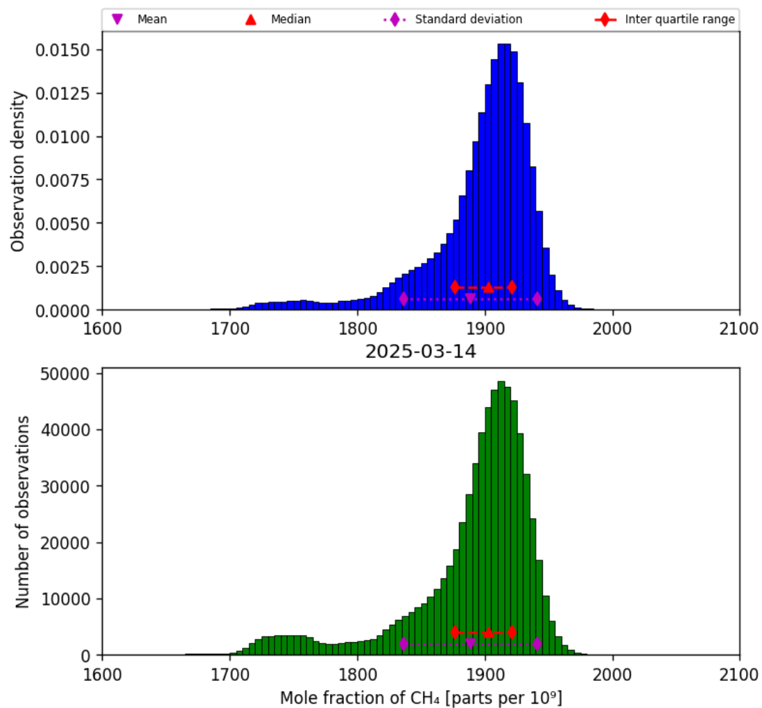
Figure 23: Histogram of “Mole fraction of CH 4 ” for 2025-03-13 to 2025-03-15
