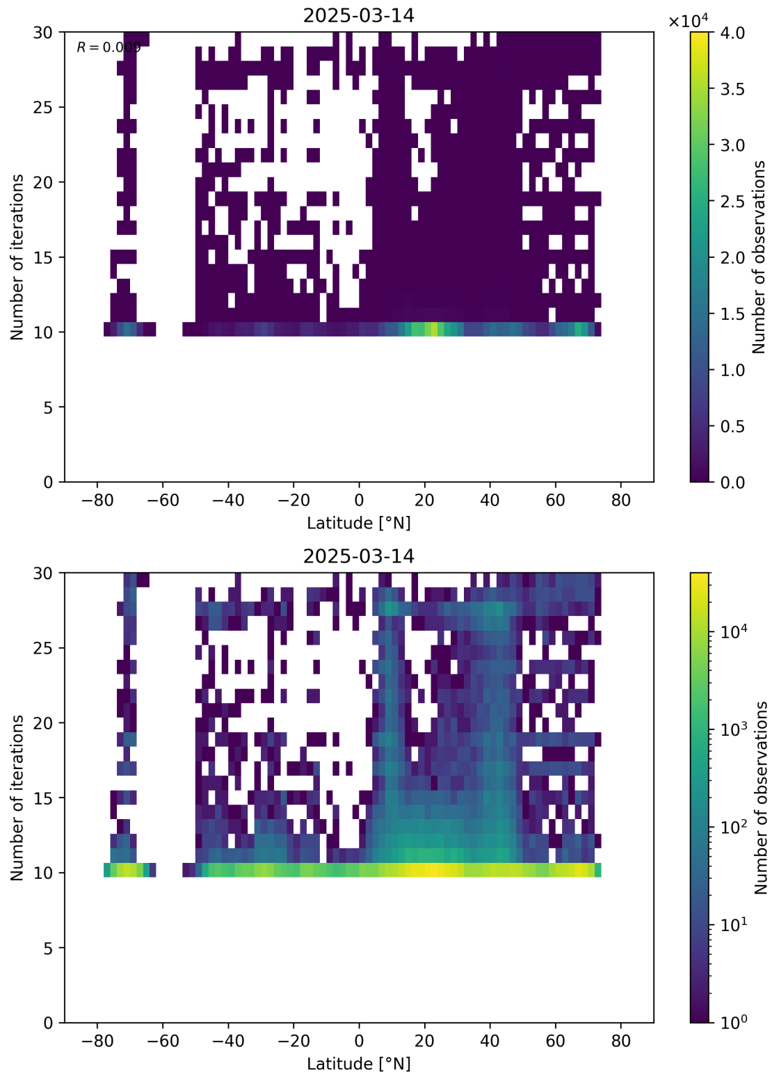
Figure 60: Scatter density plot of “Latitude” against “Number of iterations” for 2025-03-13 to 2025-03-15.
