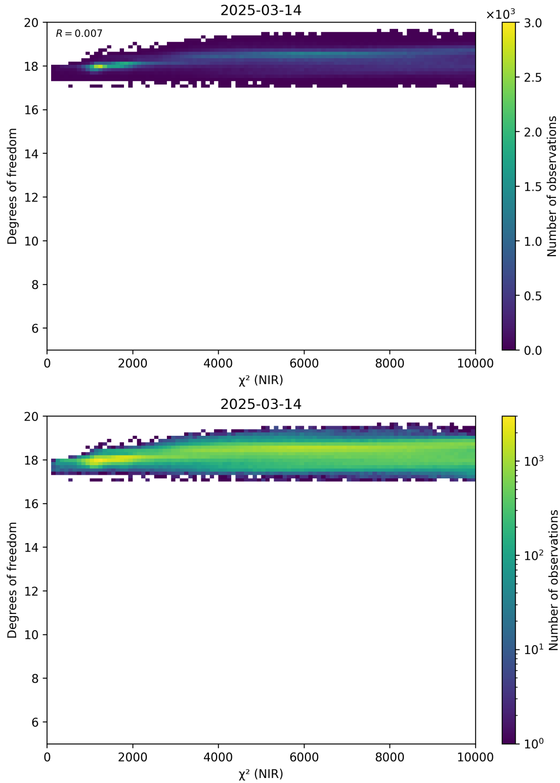
Figure 44: Scatter density plot of “ \chi^2 (NIR)” against “Degrees of freedom” for 2025-03-13 to 2025-03-15.
