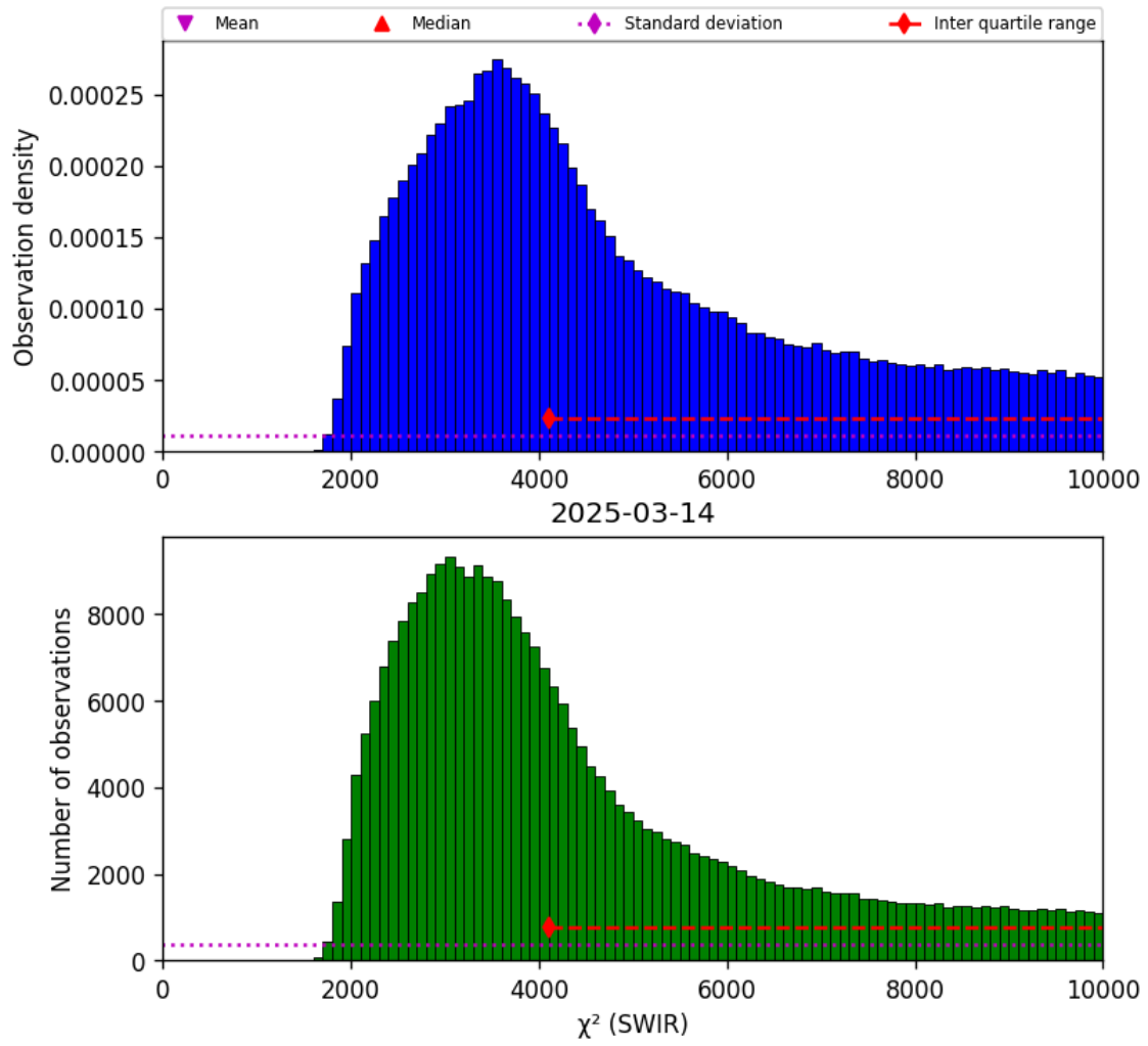
Figure 28: Histogram of " \chi^2 (SWIR)" for 2025-03-13 to 2025-03-15
