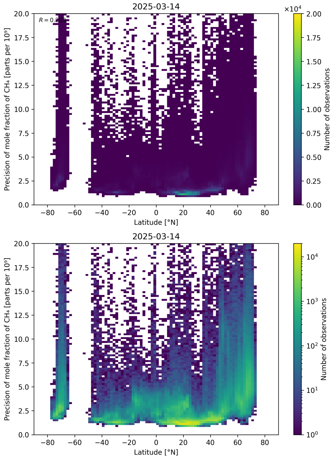
Figure 59: Scatter density plot of “Latitude” against “Precision of mole fraction of CH 4 ” for 2025-03-13 to 2025-03-15.
