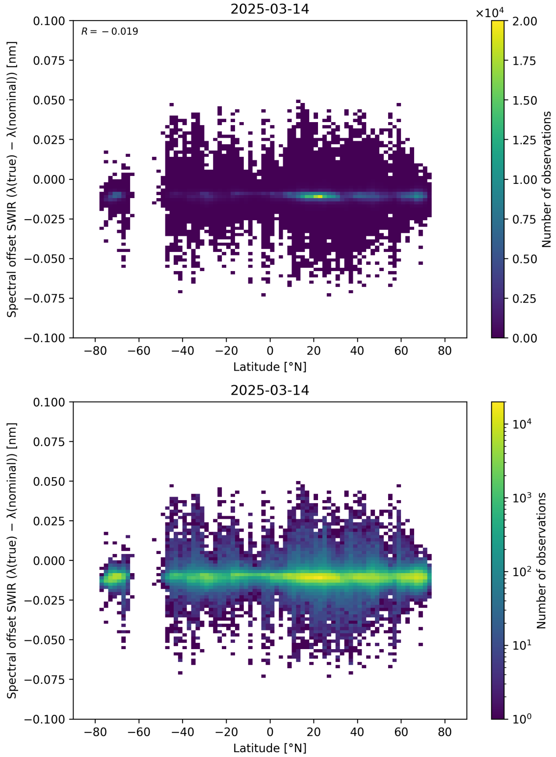
Figure 62: Scatter density plot of “Latitude” against “Spectral offset SWIR ( \lambda_{\text{true}} - \lambda_{\text{nominal}} )” for 2025-03-13 to 2025-03-15.
