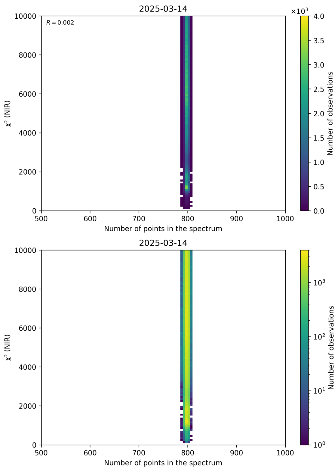
Figure 88: Scatter density plot of “Number of points in the spectrum” against “ \chi^2 (NIR)” for 2025-03-13 to 2025-03-15.
