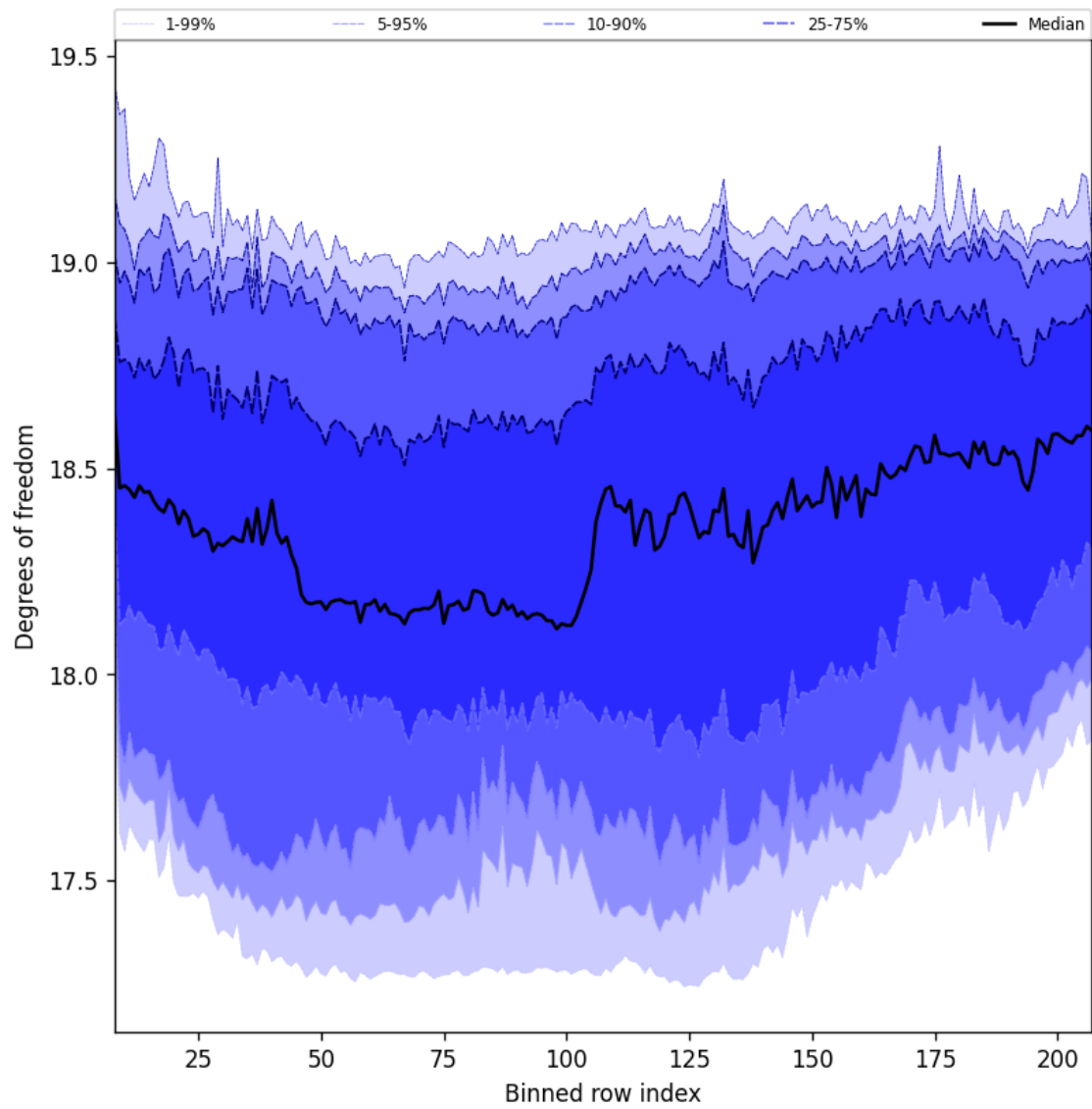
Figure 41: Along track statistics of “Degrees of freedom” for 2025-03-13 to 2025-03-15
