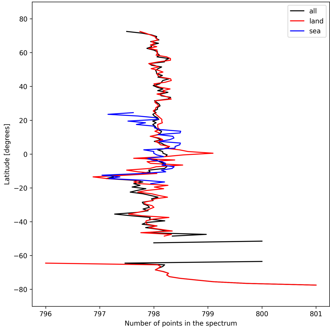
Figure 15: Zonal average of “Number of points in the spectrum” for 2025-03-13 to 2025-03-15.
