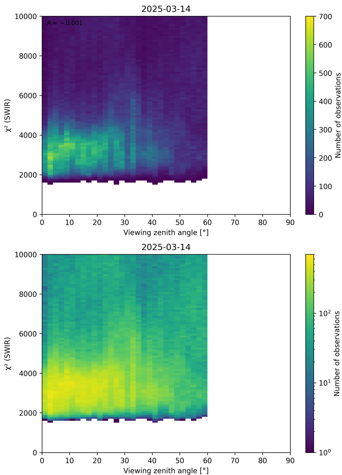
Figure 106: Scatter density plot of “Viewing zenith angle” against “ \chi^2 (SWIR)” for 2025-03-13 to 2025-03-15.
