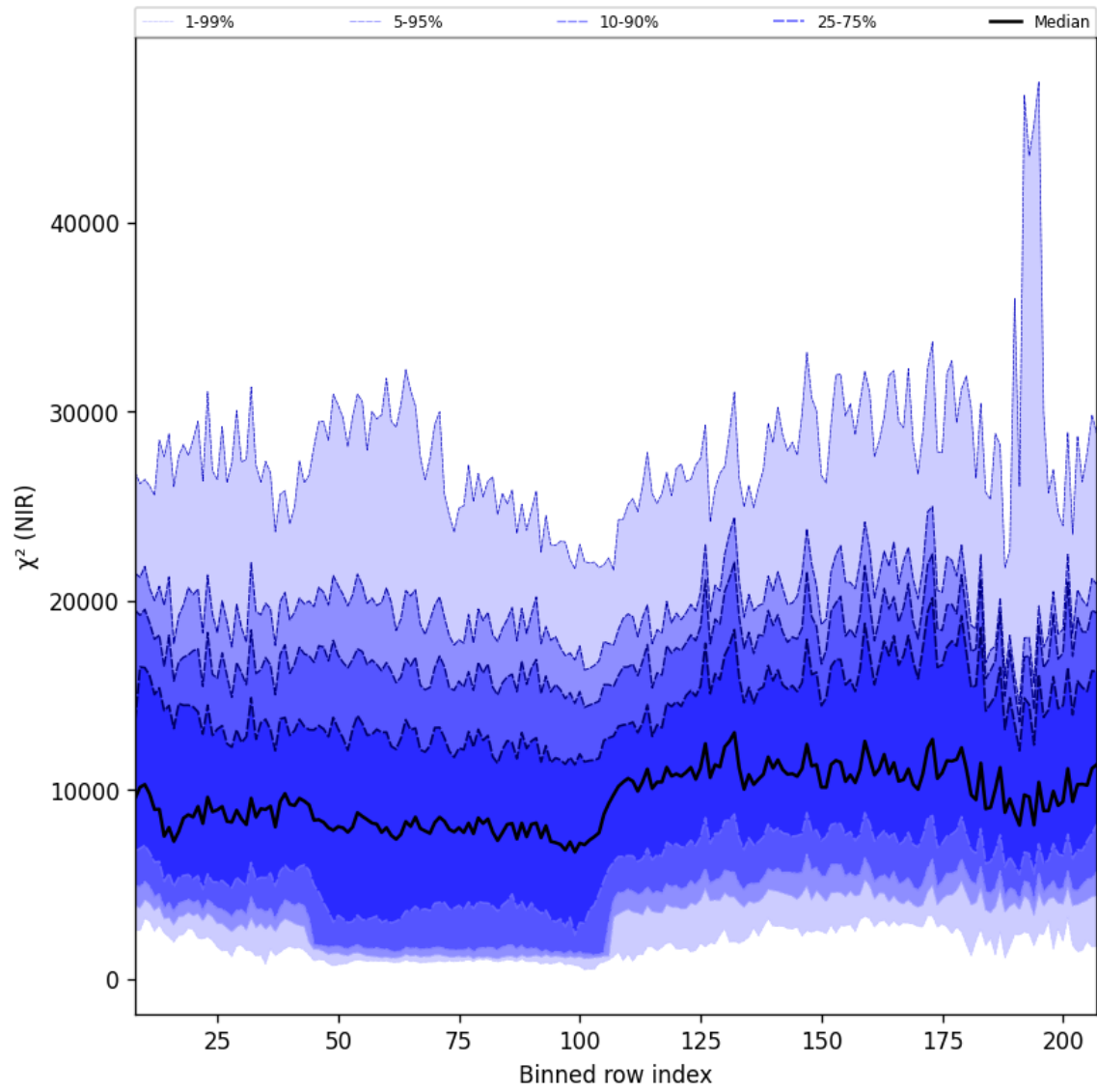
Figure 40: Along track statistics of “ \chi^2 (NIR)” for 2025-03-13 to 2025-03-15
