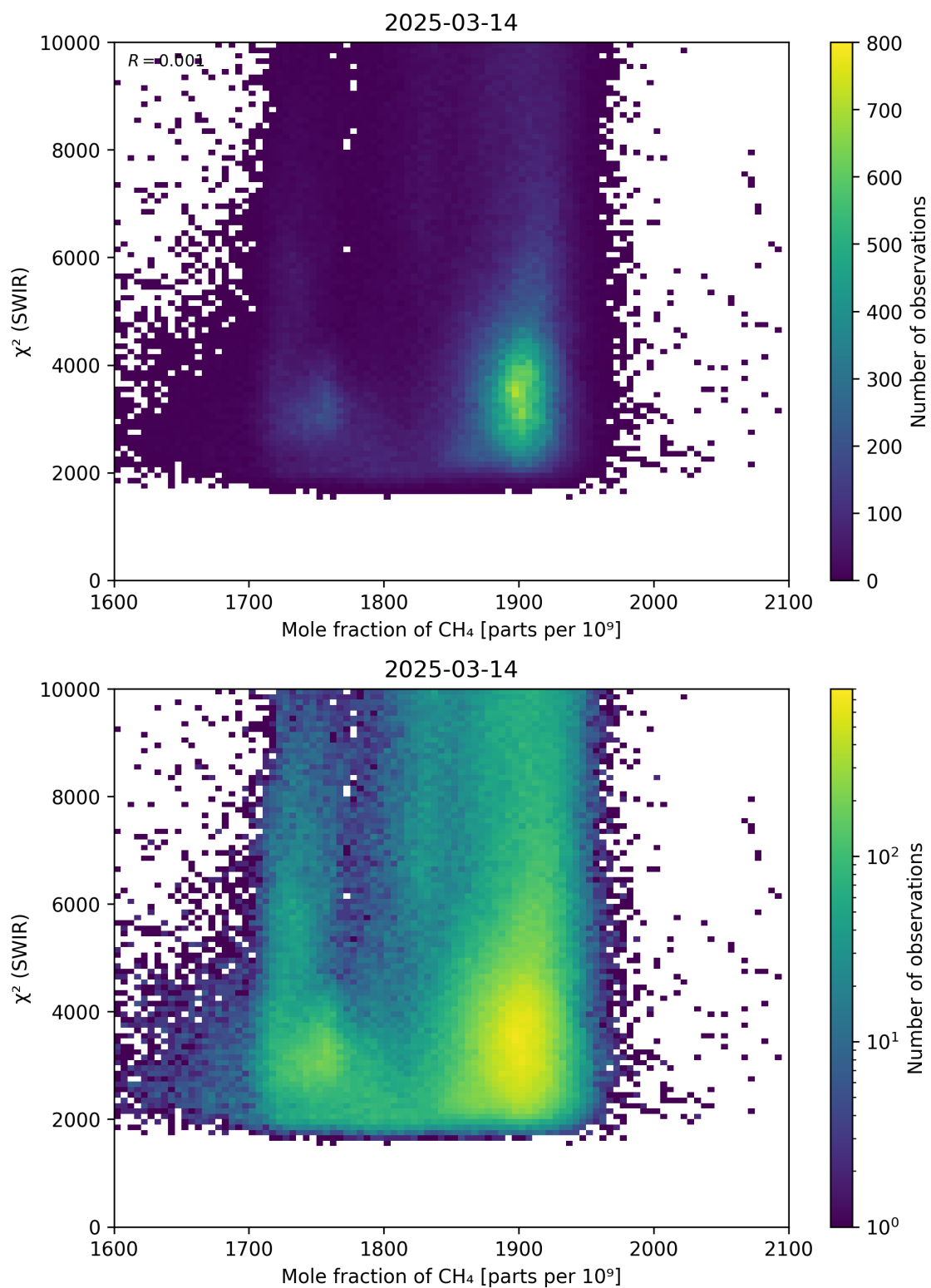
Figure 71: Scatter density plot of “Mole fraction of \text{CH}_4 ” against “ \chi^2 (SWIR)” for 2025-03-13 to 2025-03-15.
