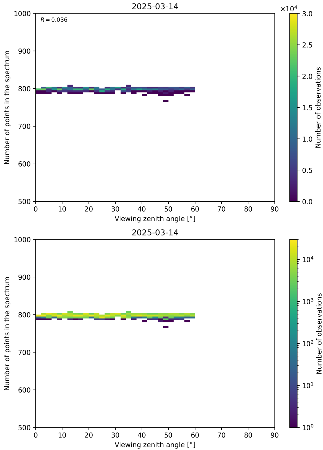
Figure 114: Scatter density plot of “Viewing zenith angle” against “Number of points in the spectrum” for 2025-03-13 to 2025-03-15.
