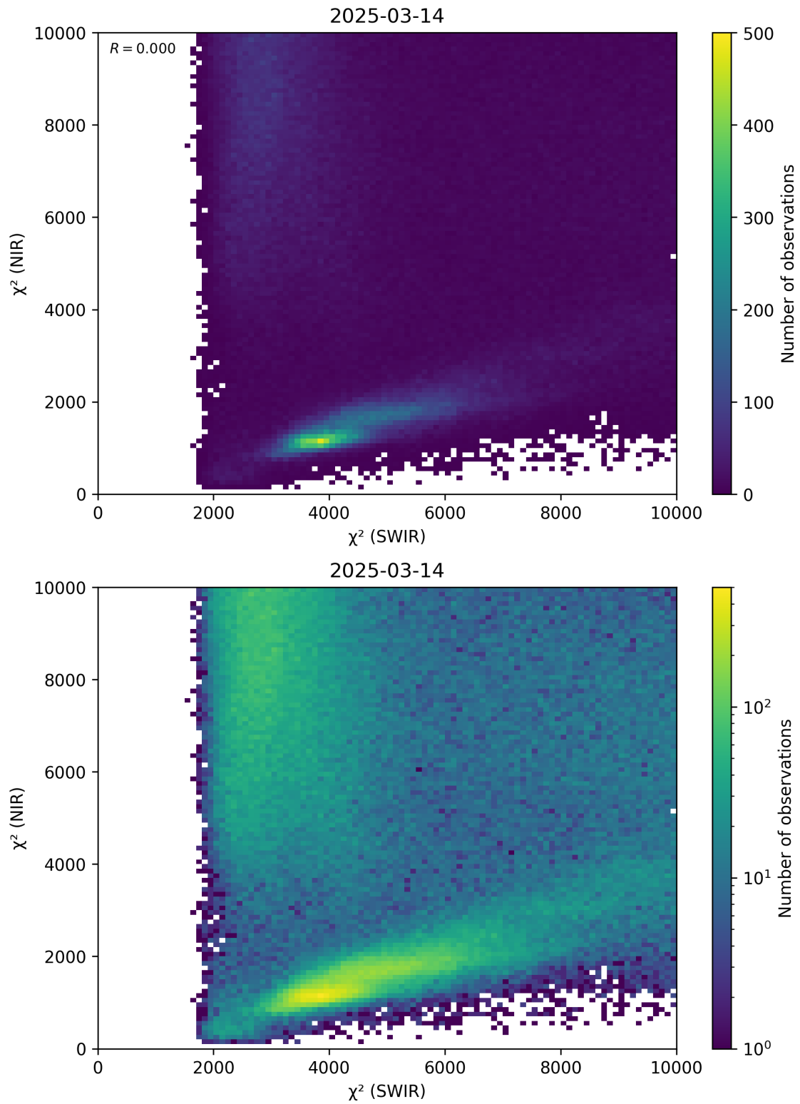
Figure 47: Scatter density plot of “ \chi^2 (SWIR)” against “ \chi^2 (NIR)” for 2025-03-13 to 2025-03-15.
