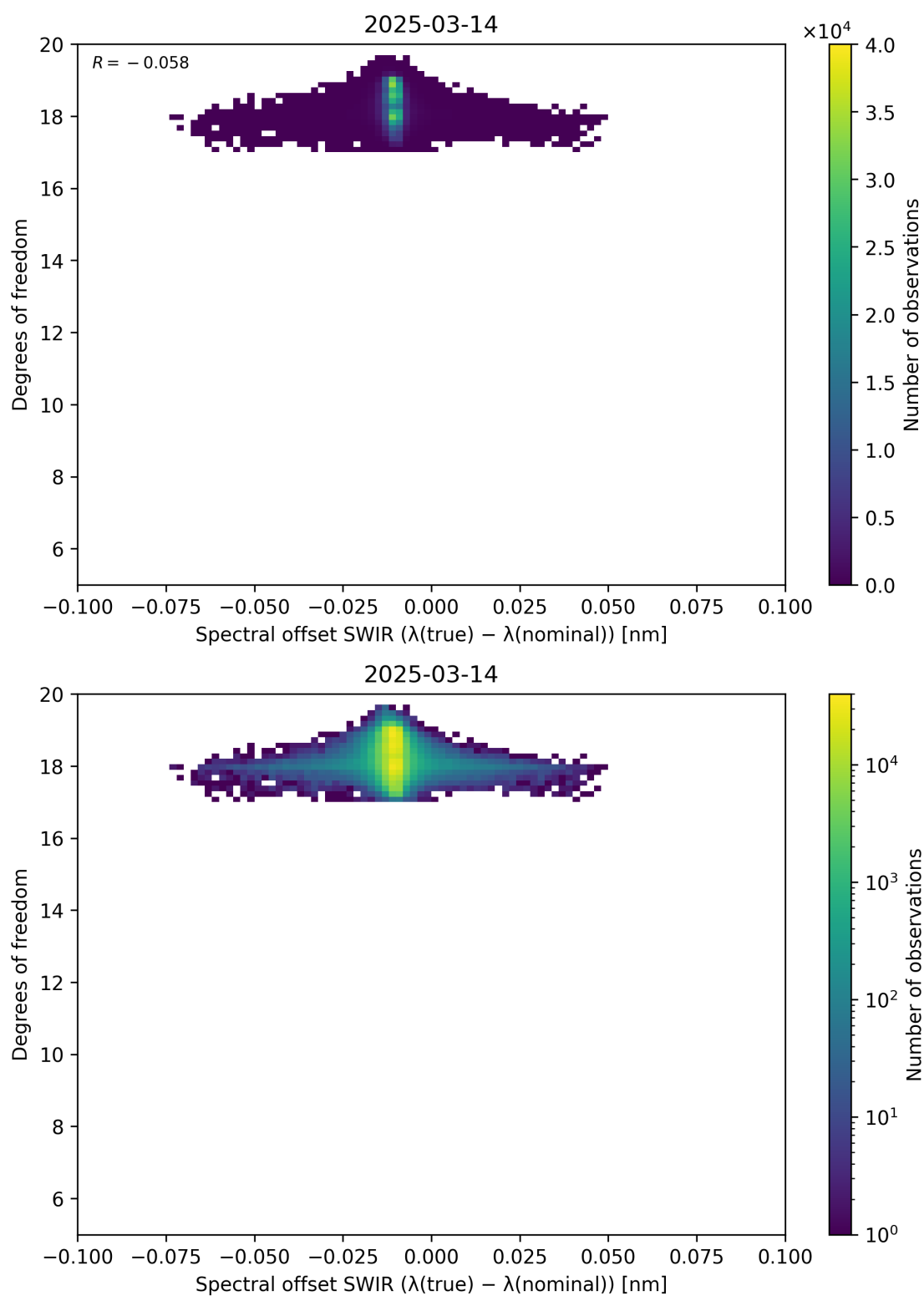
Figure 119: Scatter density plot of “Spectral offset SWIR ( \lambda_{\text{true}} - \lambda_{\text{nominal}} )” against “Degrees of freedom” for 2025-03-13 to 2025-03-15.
