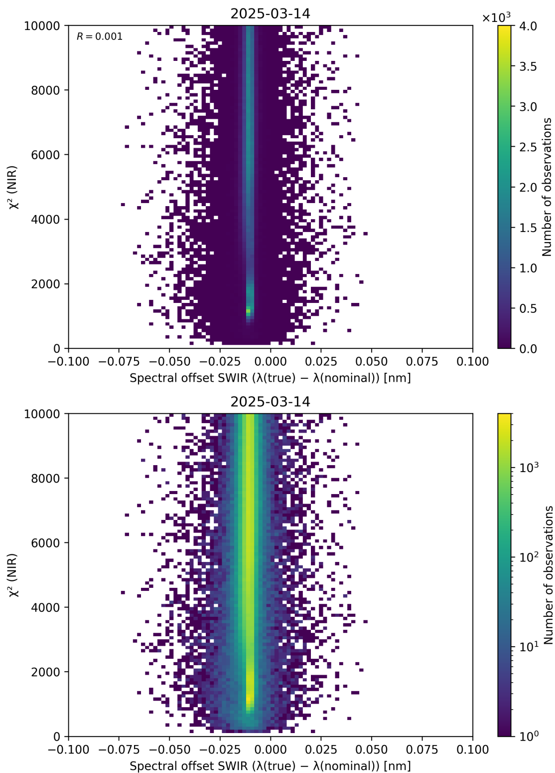
Figure 117: Scatter density plot of “Spectral offset SWIR ( \lambda_{\text{true}} - \lambda_{\text{nominal}} )” against “ \chi^2 (NIR)” for 2025-03-13 to 2025-03-15.
