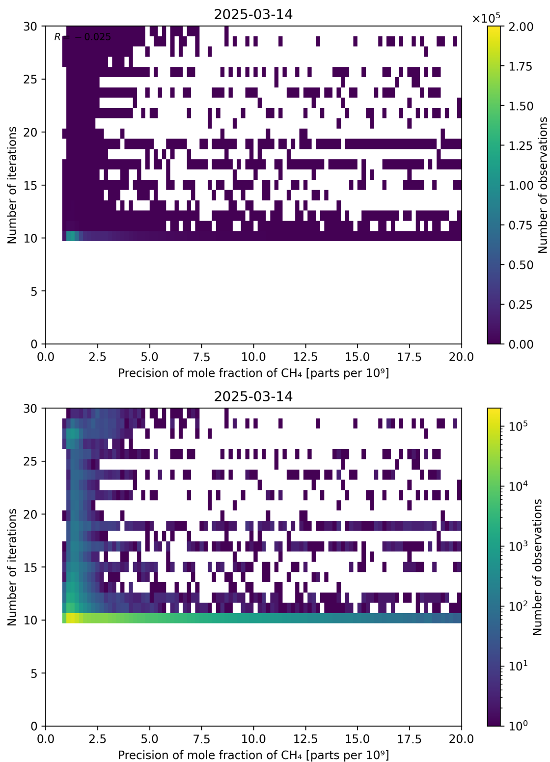
Figure 83: Scatter density plot of “Precision of mole fraction of CH 4 ” against “Number of iterations” for 2025-03-13 to 2025-03-15.
