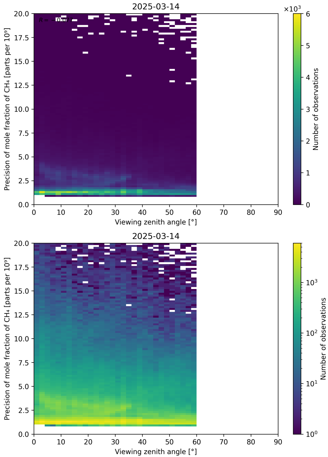
Figure 112: Scatter density plot of “Viewing zenith angle” against “Precision of mole fraction of CH 4 ” for 2025-03-13 to 2025-03-15.
