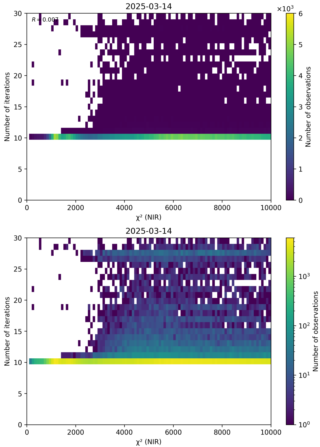
Figure 46: Scatter density plot of “ \chi^2 (NIR)” against “Number of iterations” for 2025-03-13 to 2025-03-15.
