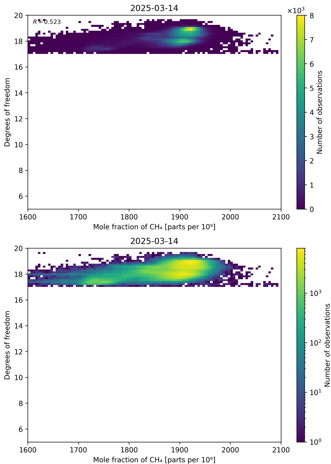
Figure 72: Scatter density plot of “Mole fraction of CH 4 ” against “Degrees of freedom” for 2025-03-13 to 2025-03-15.
