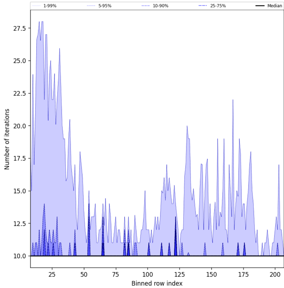
Figure 42: Along track statistics of “Number of iterations” for 2025-03-13 to 2025-03-15
