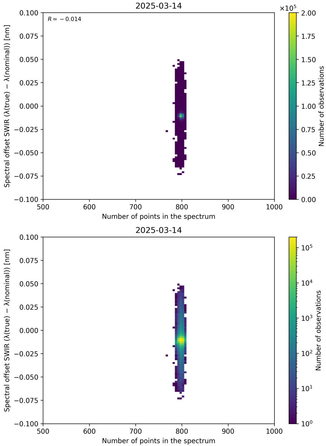
Figure 93: Scatter density plot of “Number of points in the spectrum” against “Spectral offset SWIR ( \lambda_{\text{true}} - \lambda_{\text{nominal}} )” for 2025-03-13 to 2025-03-15.
