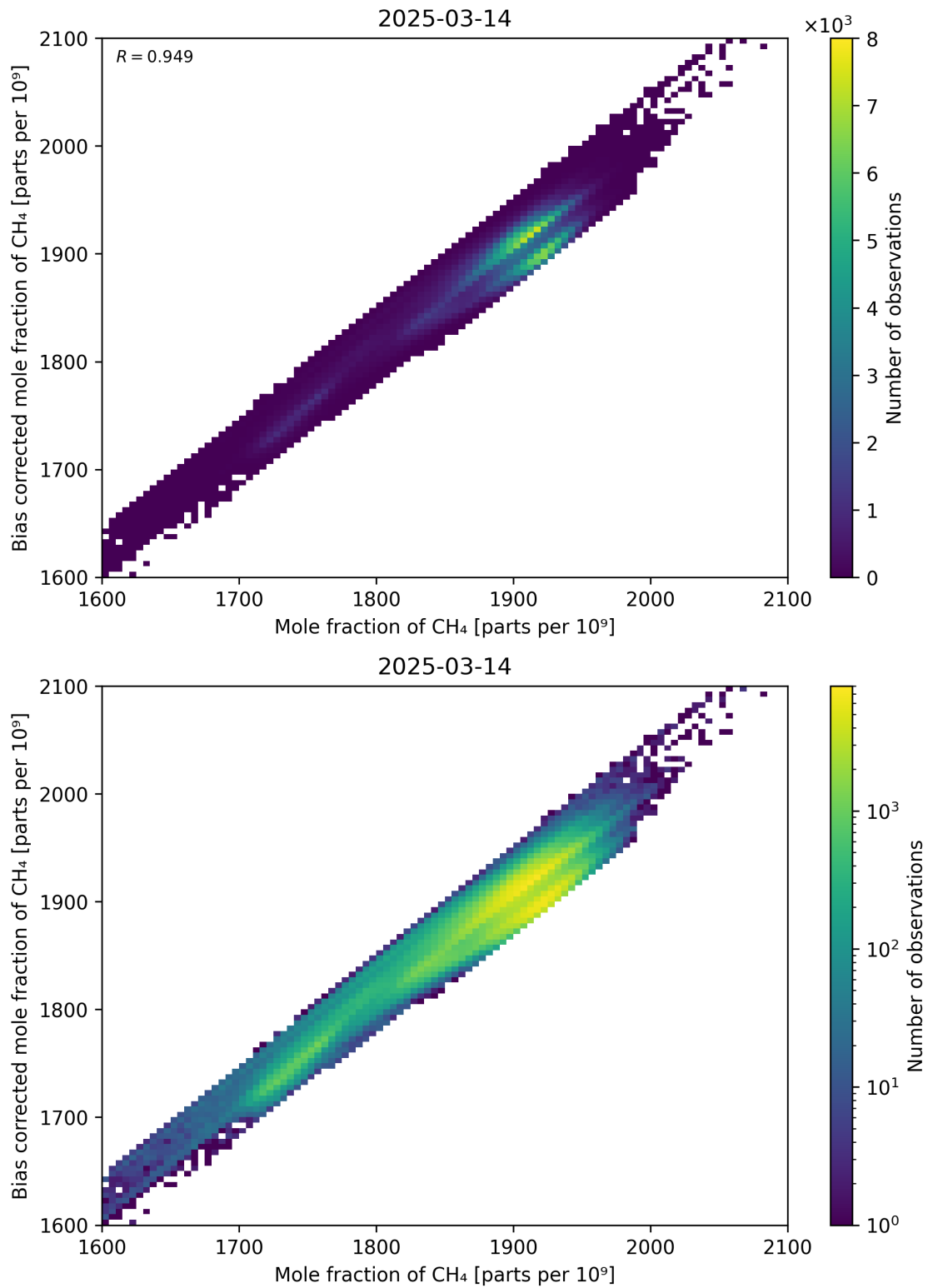
Figure 74: Scatter density plot of “Mole fraction of CH 4 ” against “Bias corrected mole fraction of CH 4 ” for 2025-03-13 to 2025-03-15.
