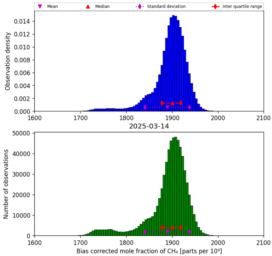
Figure 25: Histogram of “Bias corrected mole fraction of CH 4 ” for 2025-03-13 to 2025-03-15
