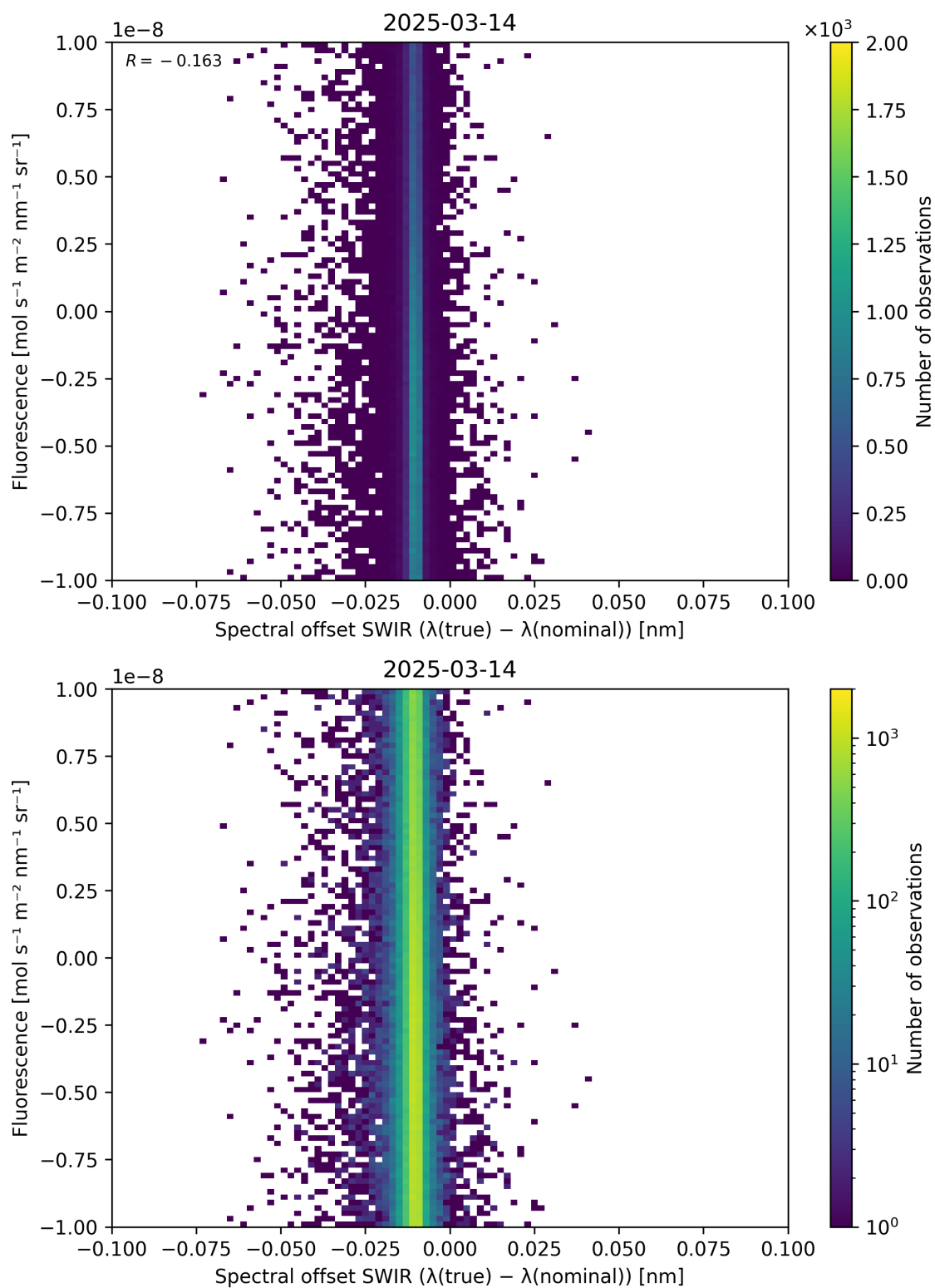
Figure 120: Scatter density plot of “Spectral offset SWIR ( \lambda_{\text{true}} - \lambda_{\text{nominal}} )” against “Fluorescence” for 2025-03-13 to 2025-03-15.
