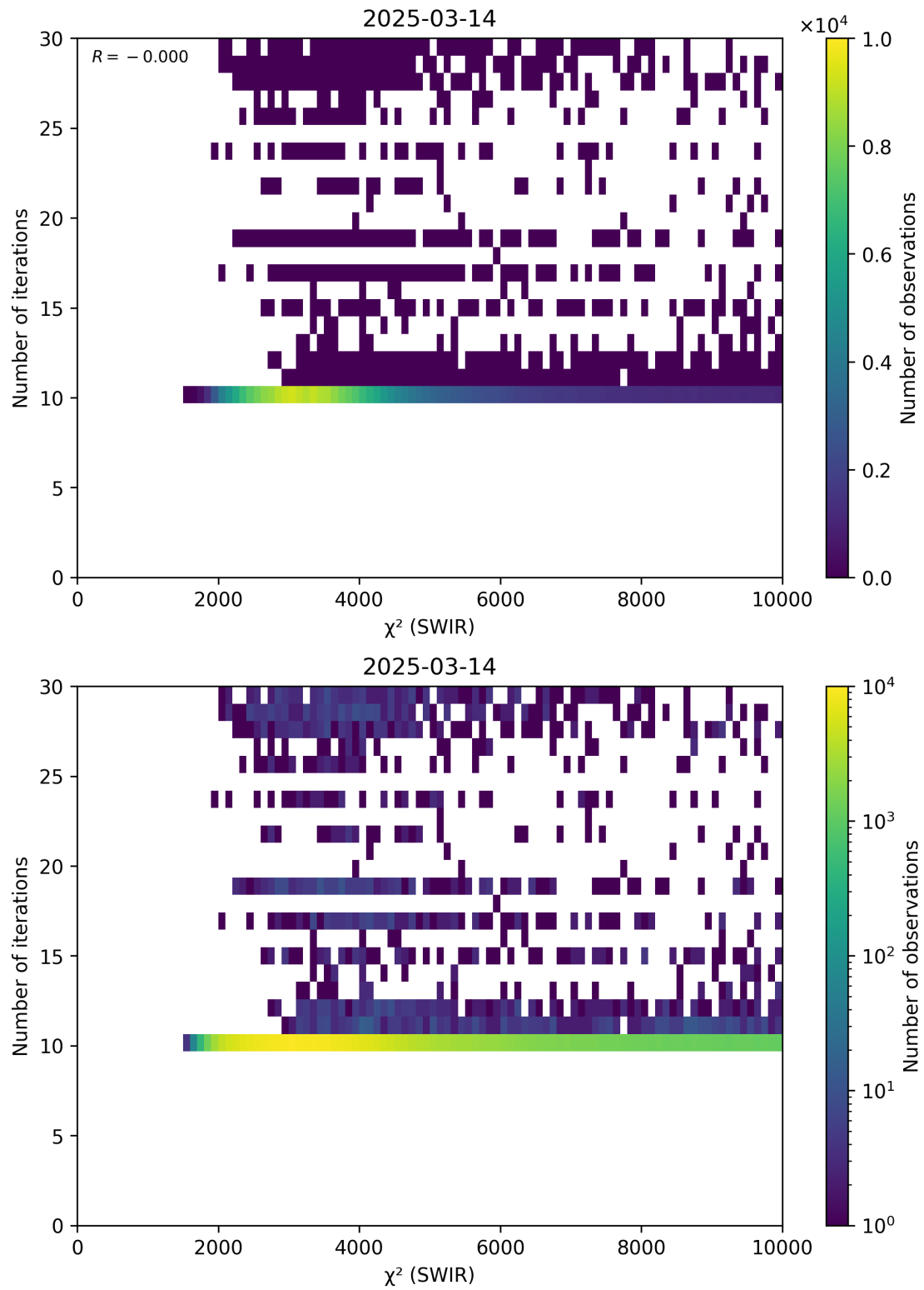
Figure 50: Scatter density plot of “ \chi^2 (SWIR)” against “Number of iterations” for 2025-03-13 to 2025-03-15.
