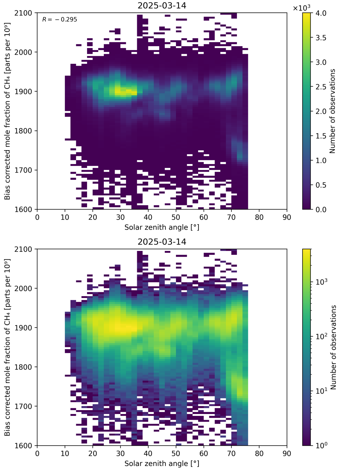
Figure 100: Scatter density plot of “Solar zenith angle” against “Bias corrected mole fraction of CH 4 ” for 2025-03-13 to 2025-03-15.
