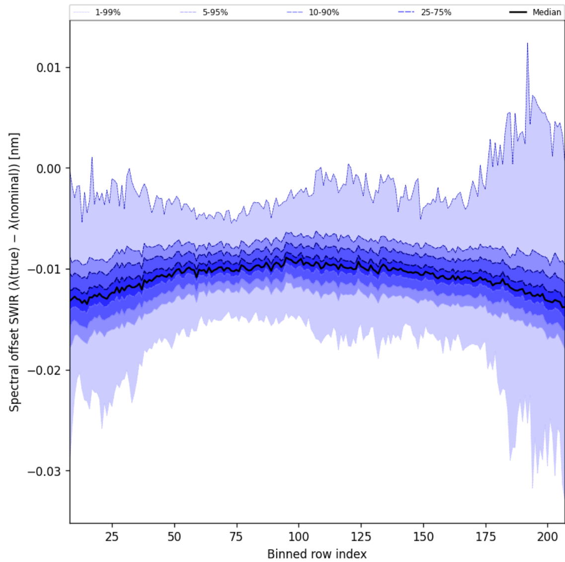
Figure 38: Along track statistics of “Spectral offset SWIR ( \lambda_{\text{true}} - \lambda_{\text{nominal}} )” for 2025-03-13 to 2025-03-15
