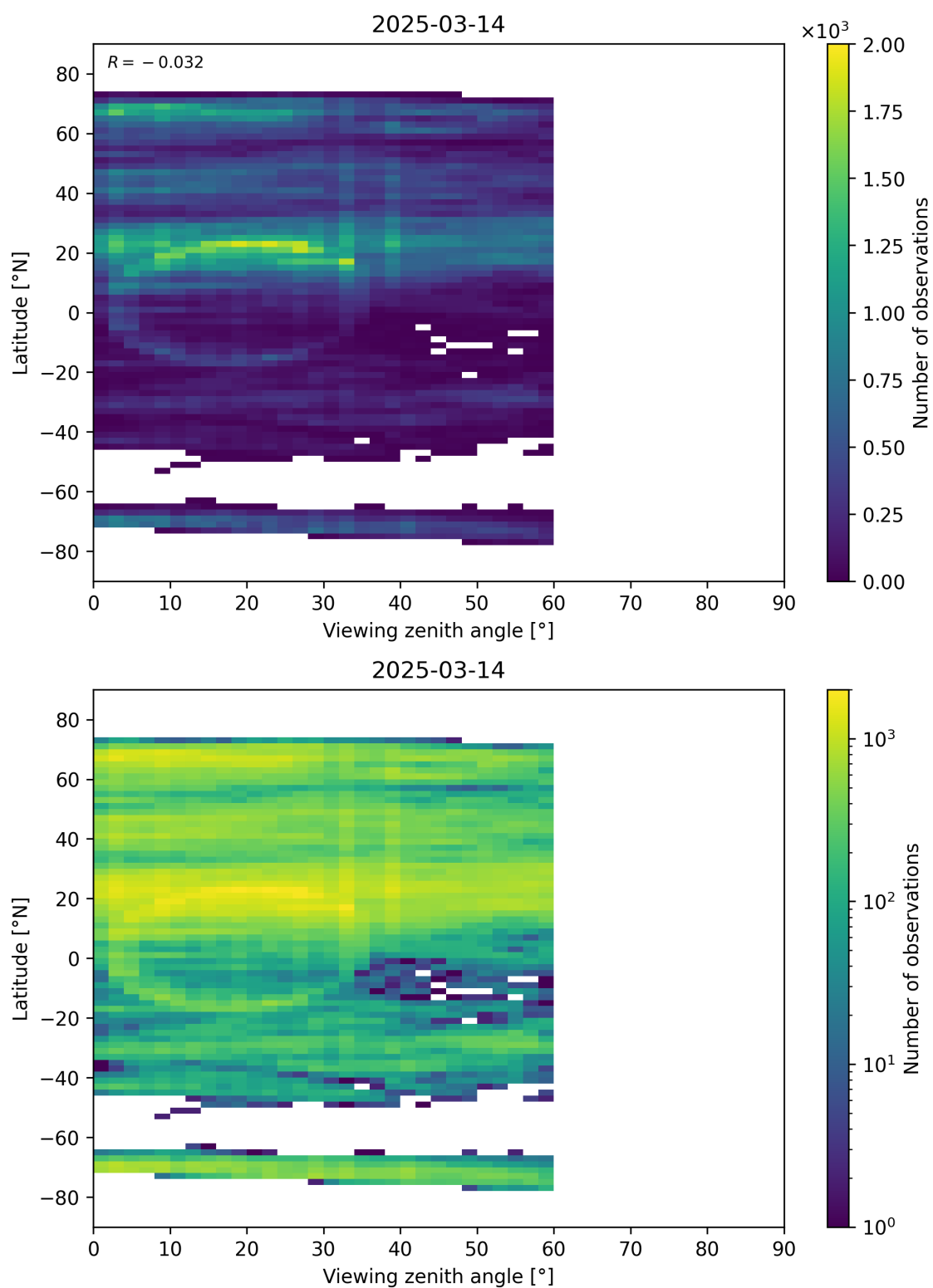
Figure 109: Scatter density plot of “Viewing zenith angle” against “Latitude” for 2025-03-13 to 2025-03-15.
