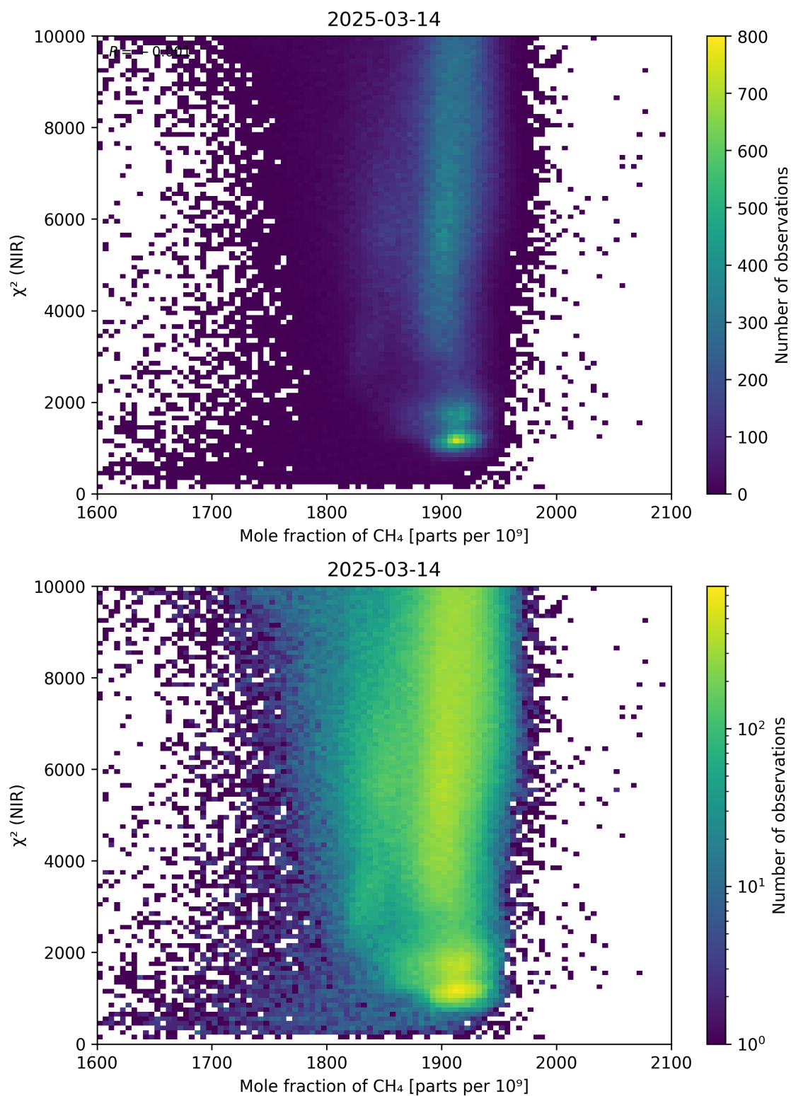
Figure 70: Scatter density plot of “Mole fraction of CH 4 ” against “ \chi^2 (NIR)” for 2025-03-13 to 2025-03-15.
