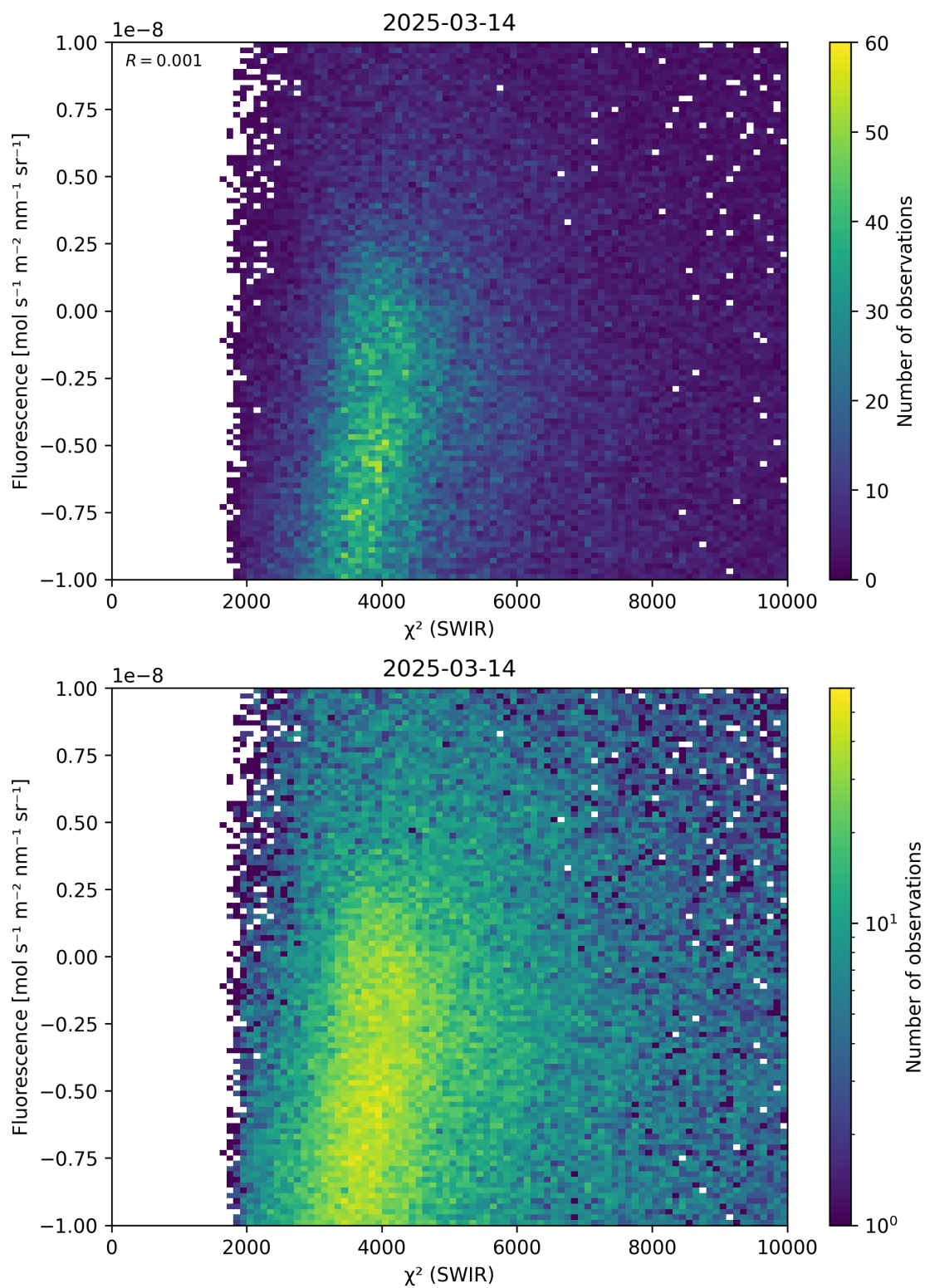
Figure 49: Scatter density plot of “ \chi^2 (SWIR)” against “Fluorescence” for 2025-03-13 to 2025-03-15.
