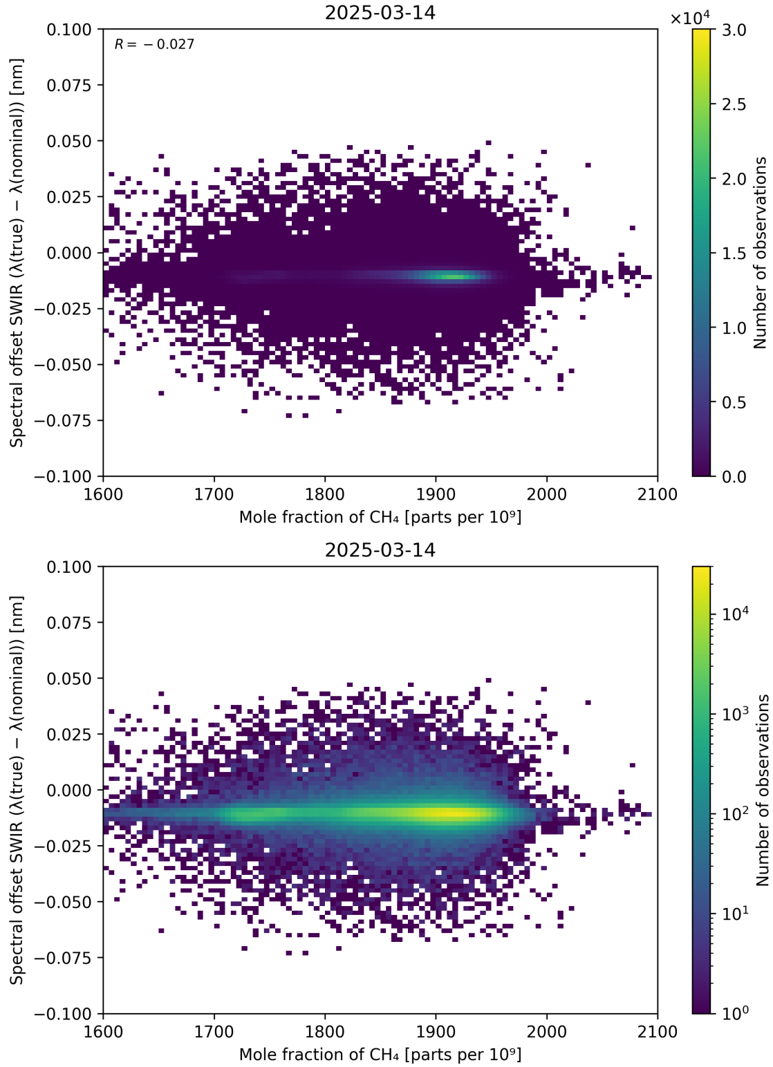
Figure 86: Scatter density plot of “Mole fraction of CH 4 ” against “Spectral offset SWIR ( \lambda_{\text{true}} - \lambda_{\text{nominal}} )” for 2025-03-13 to 2025-03-15.
