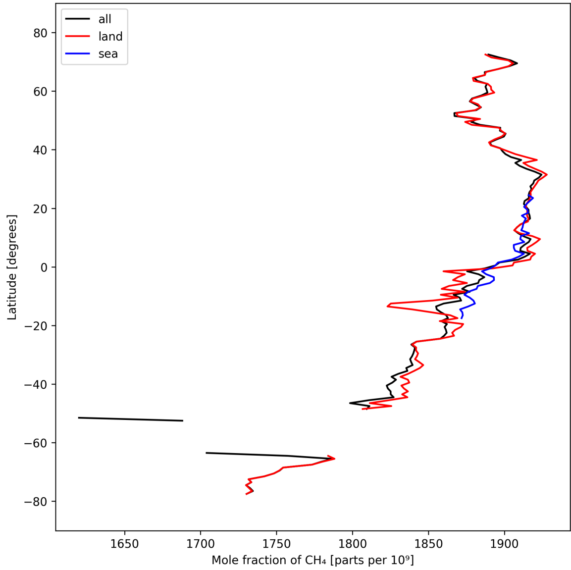
Figure 12: Zonal average of “Mole fraction of CH 4 ” for 2025-03-13 to 2025-03-15.
