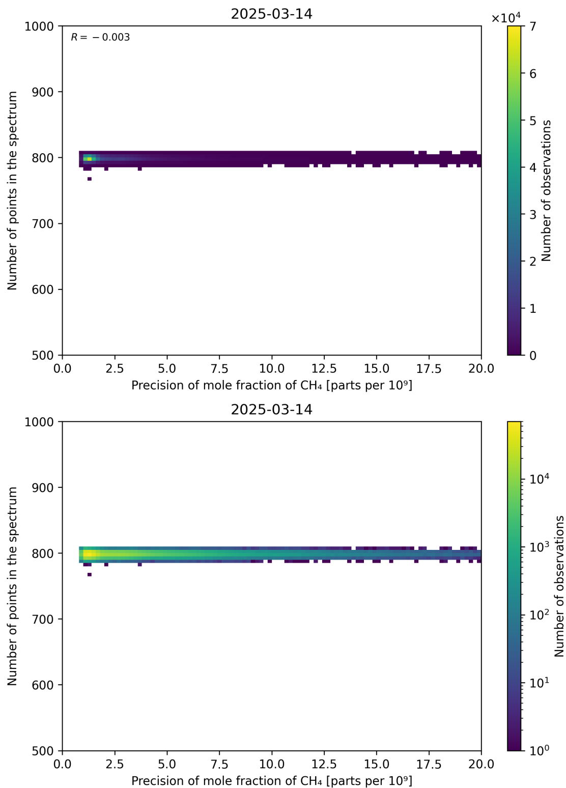
Figure 84: Scatter density plot of “Precision of mole fraction of CH 4 ” against “Number of points in the spectrum” for 2025-03-13 to 2025-03-15.
