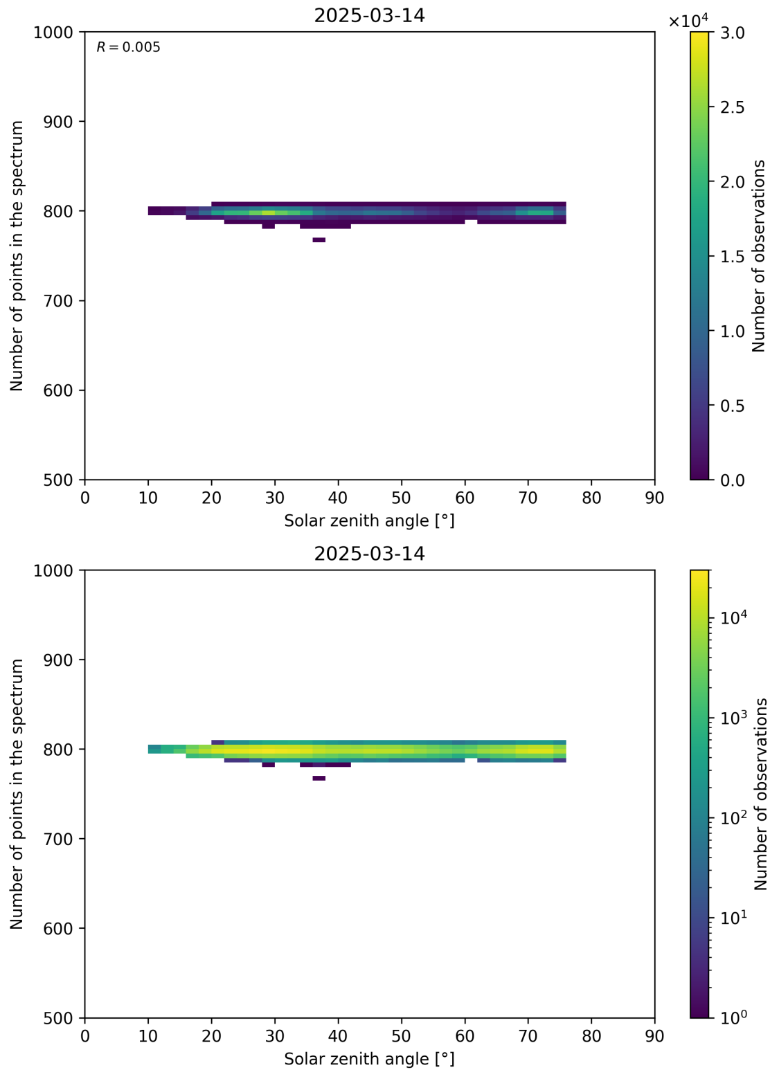
Figure 103: Scatter density plot of “Solar zenith angle” against “Number of points in the spectrum” for 2025-03-13 to 2025-03-15.
