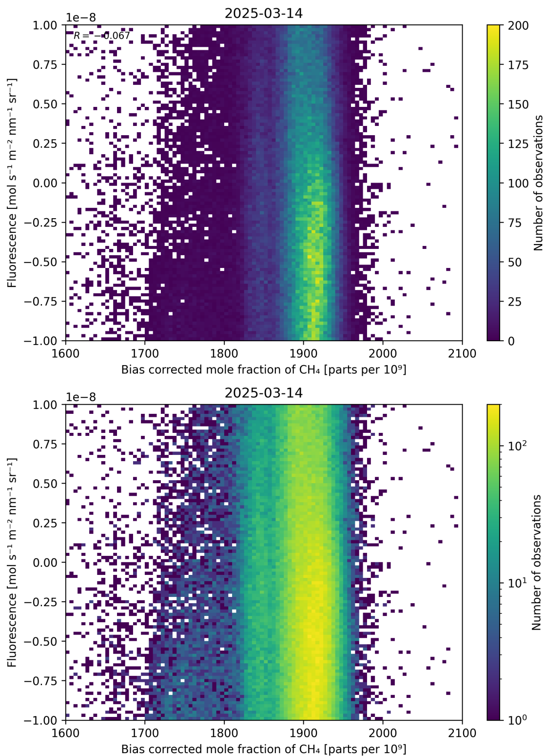
Figure 66: Scatter density plot of “Bias corrected mole fraction of \text{CH}_4 ” against “Fluorescence” for 2025-03-13 to 2025-03-15.
