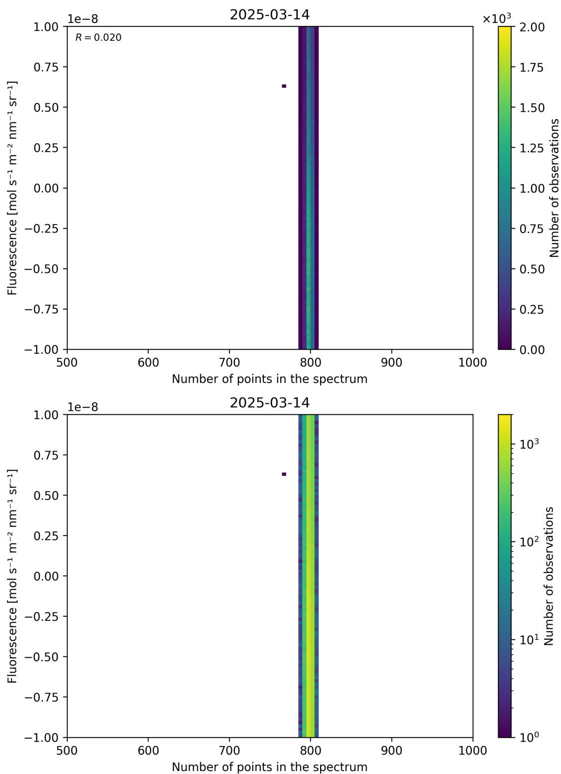
Figure 91: Scatter density plot of “Number of points in the spectrum” against “Fluorescence” for 2025-03-13 to 2025-03-15.
