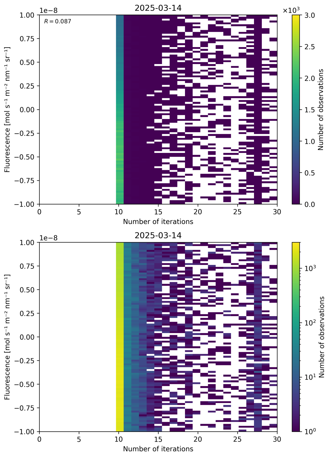
Figure 87: Scatter density plot of “Number of iterations” against “Fluorescence” for 2025-03-13 to 2025-03-15.
