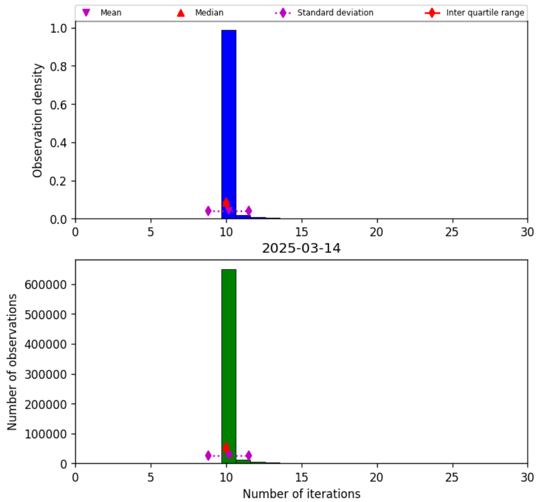
Figure 31: Histogram of "Number of iterations" for 2025-03-13 to 2025-03-15
