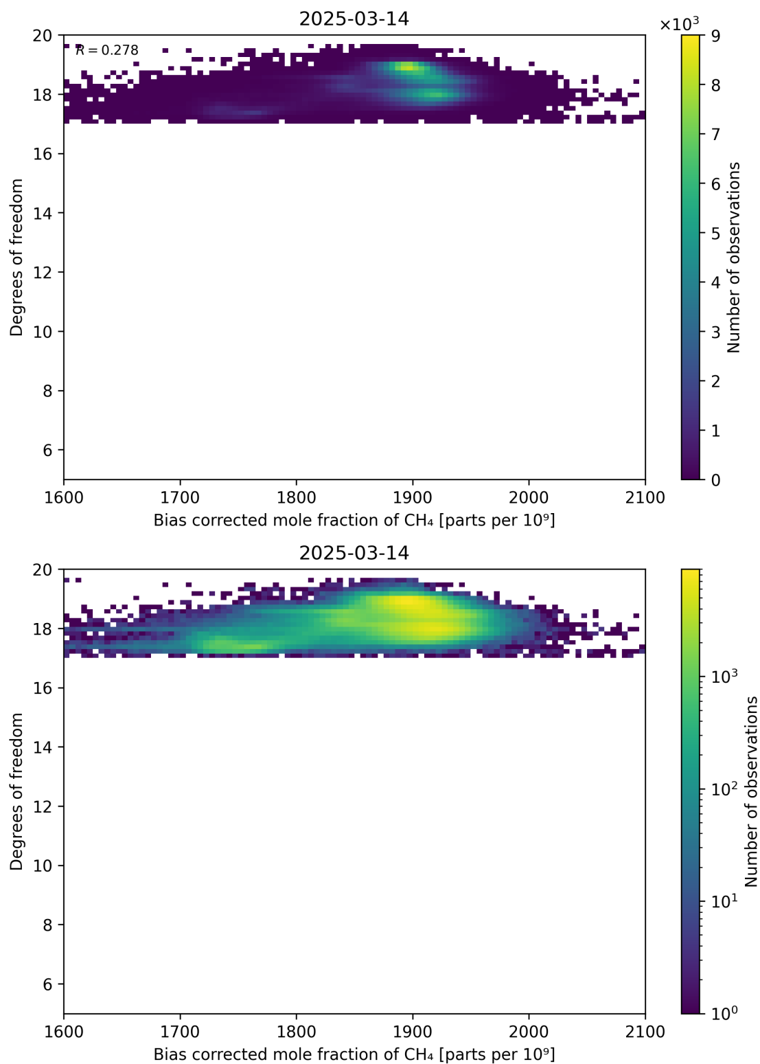
Figure 65: Scatter density plot of “Bias corrected mole fraction of CH 4 ” against “Degrees of freedom” for 2025-03-13 to 2025-03-15.
