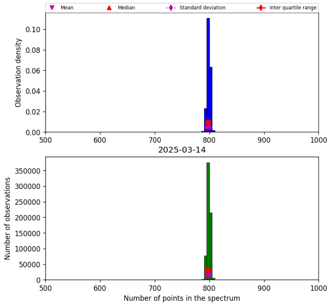
Figure 26: Histogram of “Number of points in the spectrum” for 2025-03-13 to 2025-03-15
