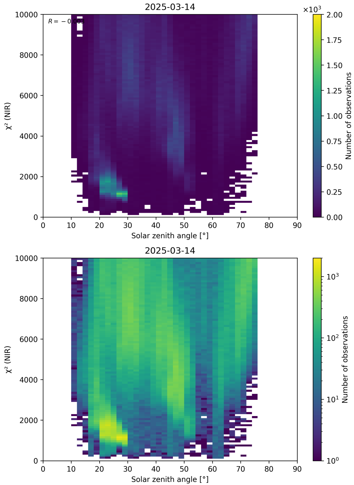
Figure 94: Scatter density plot of “Solar zenith angle” against “ \chi^2 (NIR)” for 2025-03-13 to 2025-03-15.
