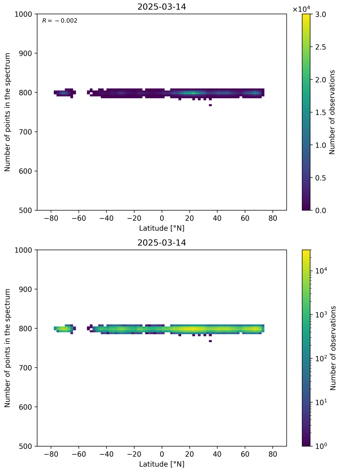
Figure 61: Scatter density plot of “Latitude” against “Number of points in the spectrum” for 2025-03-13 to 2025-03-15.
