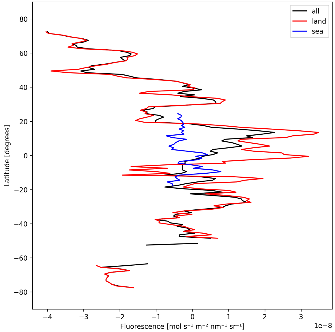
Figure 21: Zonal average of “Fluorescence” for 2025-03-13 to 2025-03-15.
