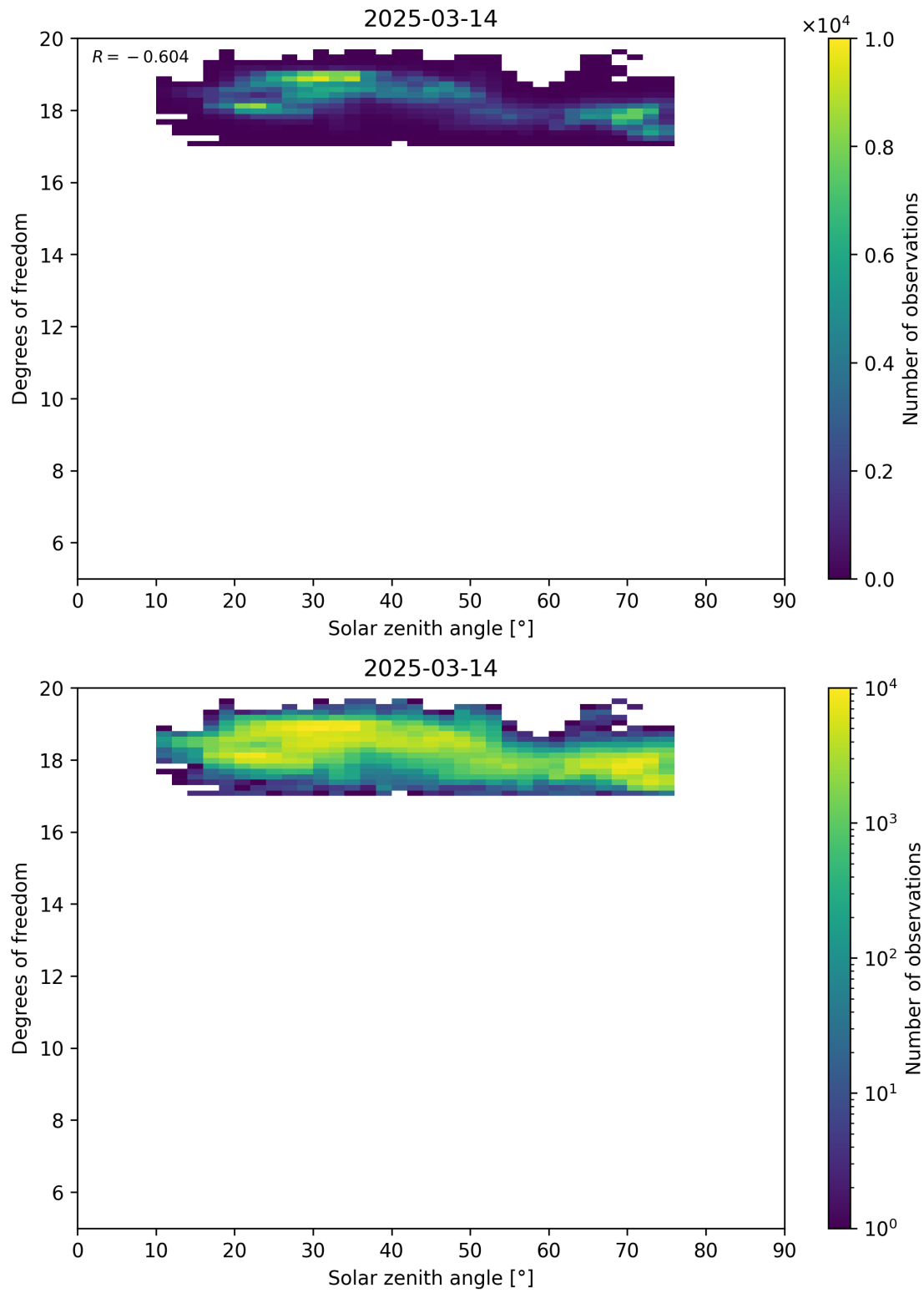
Figure 96: Scatter density plot of “Solar zenith angle” against “Degrees of freedom” for 2025-03-13 to 2025-03-15.
