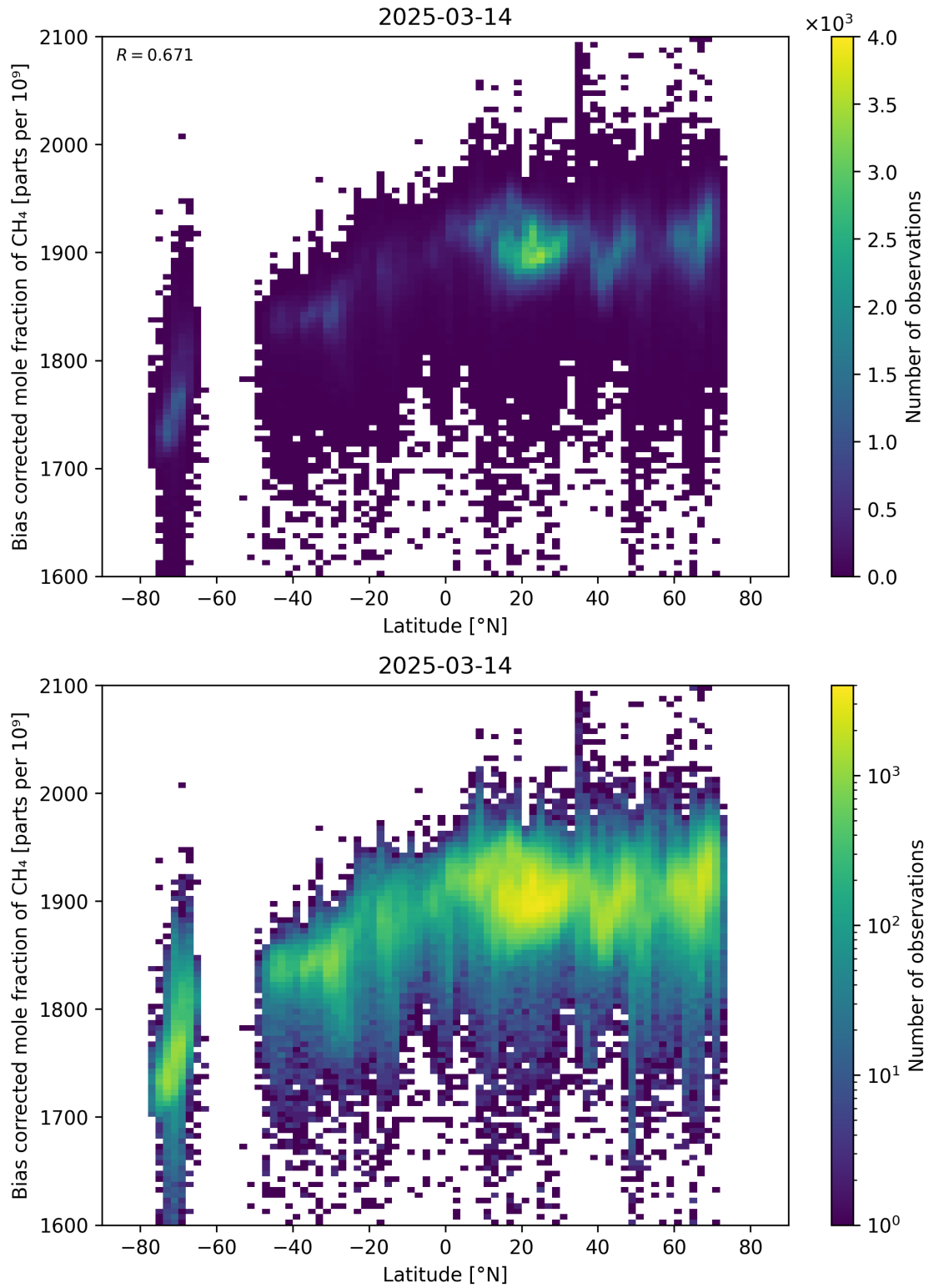
Figure 58: Scatter density plot of “Latitude” against “Bias corrected mole fraction of CH 4 ” for 2025-03-13 to 2025-03-15.
