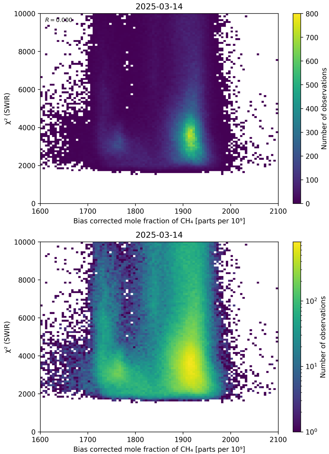
Figure 64: Scatter density plot of “Bias corrected mole fraction of \text{CH}_4 ” against “ \chi^2 (SWIR)” for 2025-03-13 to 2025-03-15.
