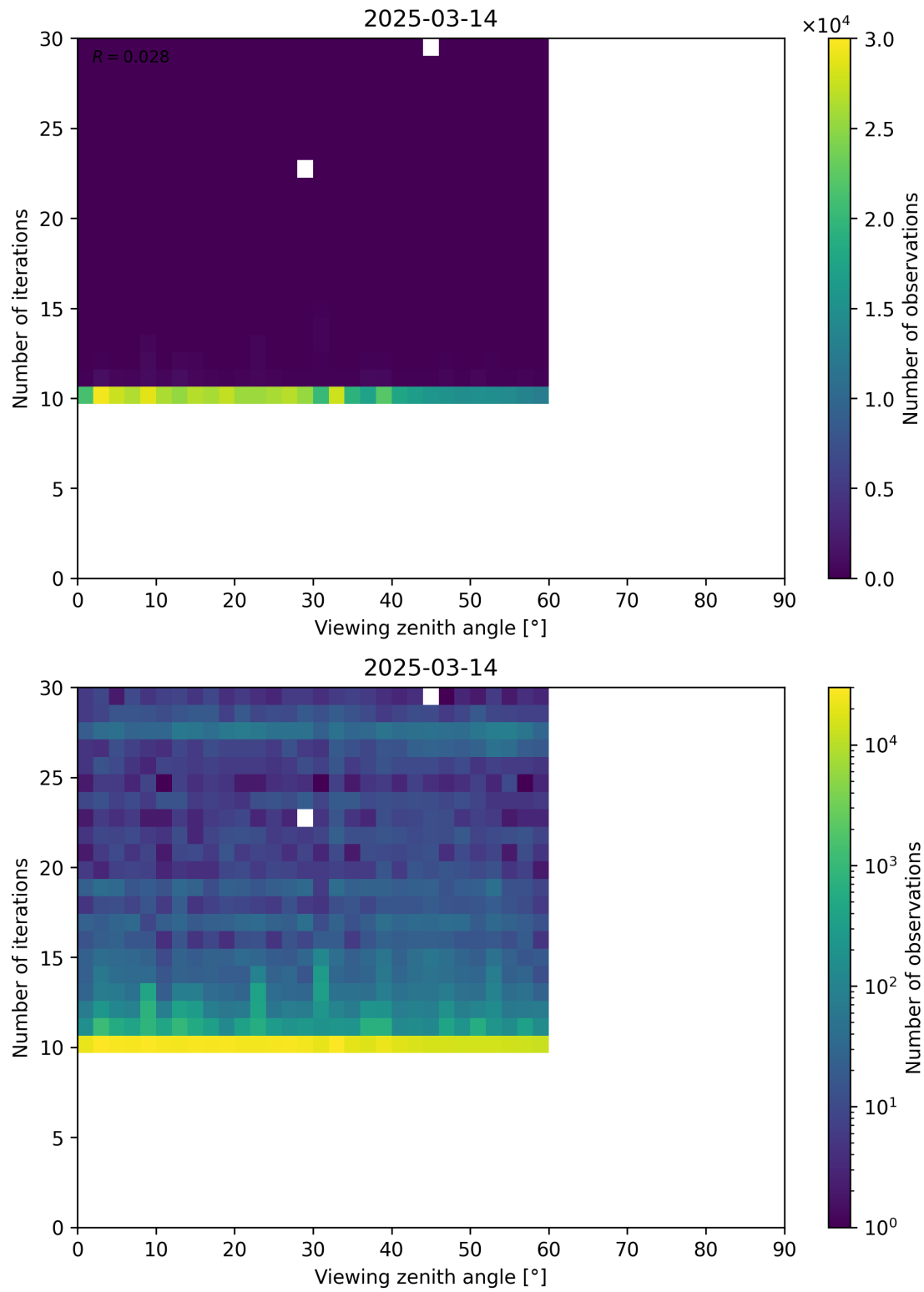
Figure 113: Scatter density plot of “Viewing zenith angle” against “Number of iterations” for 2025-03-13 to 2025-03-15.
