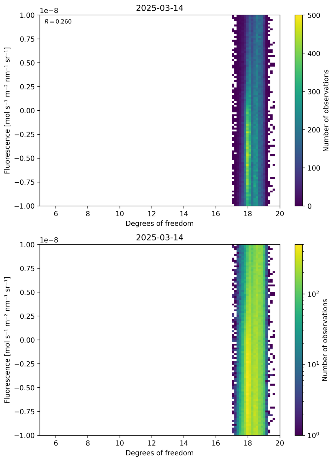
Figure 51: Scatter density plot of “Degrees of freedom” against “Fluorescence” for 2025-03-13 to 2025-03-15.
