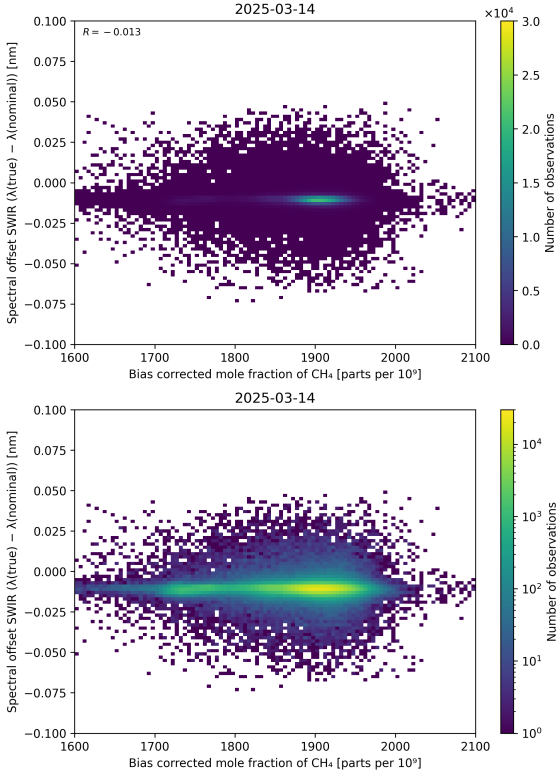
Figure 69: Scatter density plot of “Bias corrected mole fraction of \text{CH}_4 ” against “Spectral offset SWIR ( \lambda_{\text{true}} - \lambda_{\text{nominal}} )” for 2025-03-13 to 2025-03-15.
