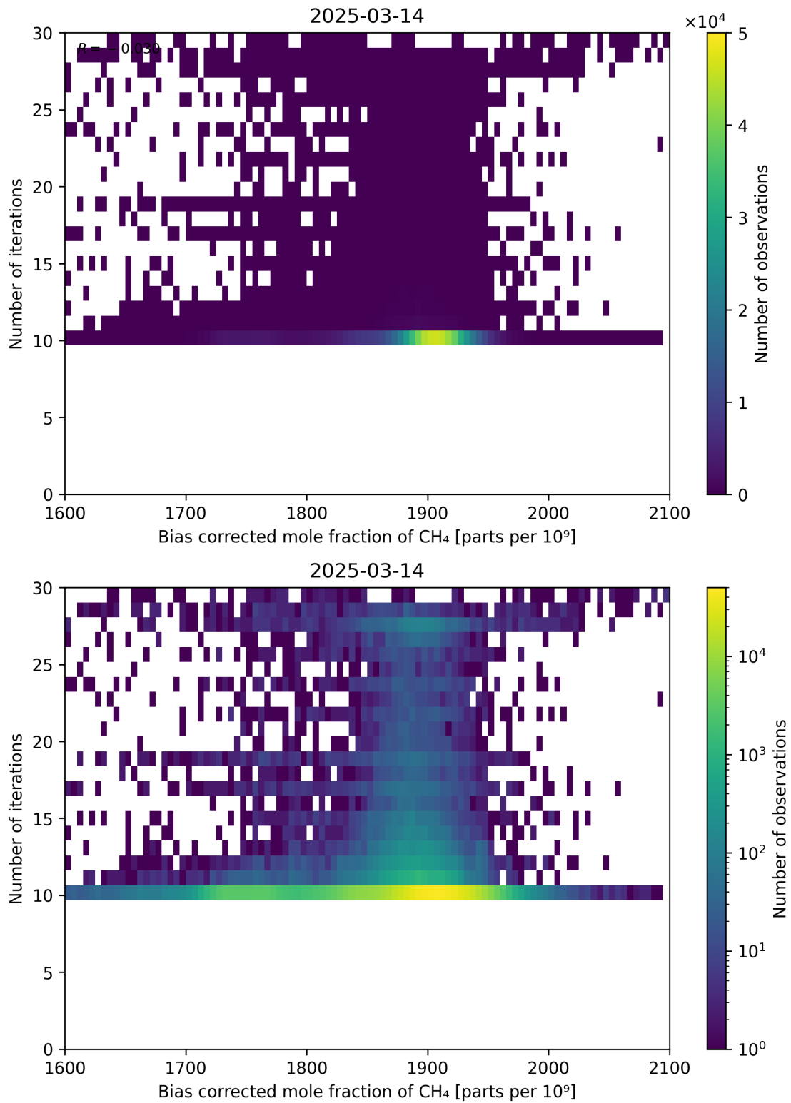
Figure 67: Scatter density plot of “Bias corrected mole fraction of CH 4 ” against “Number of iterations” for 2025-03-13 to 2025-03-15.
