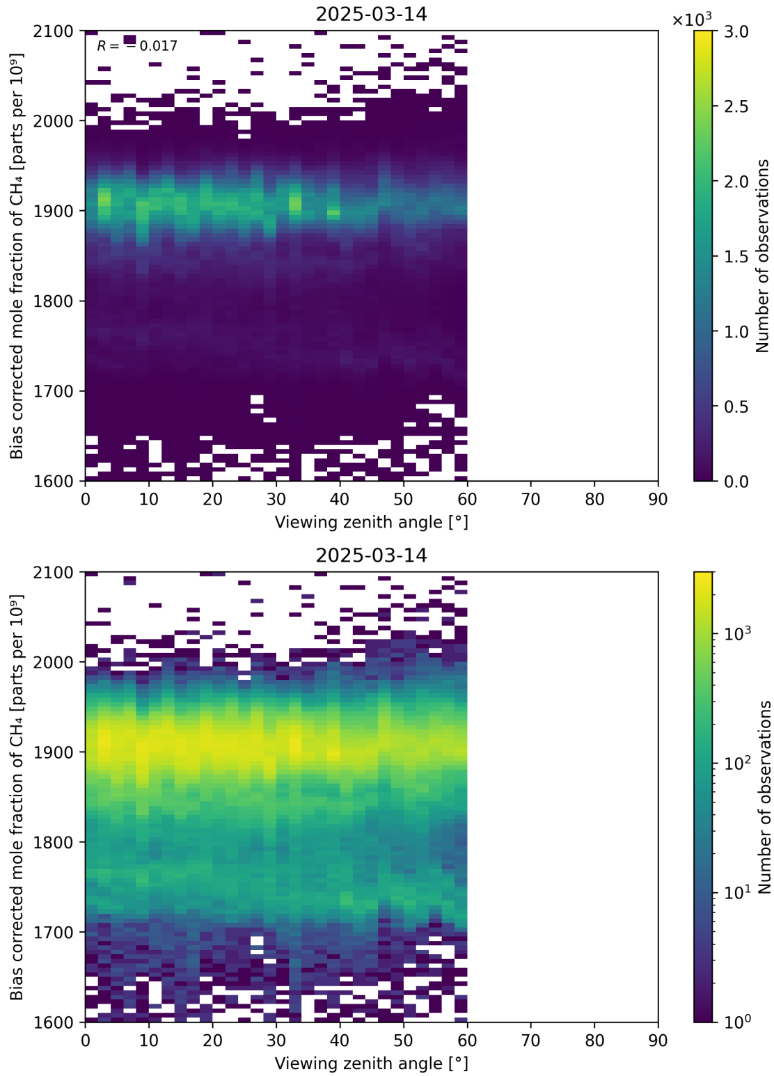
Figure 111: Scatter density plot of “Viewing zenith angle” against “Bias corrected mole fraction of CH 4 ” for 2025-03-13 to 2025-03-15.
