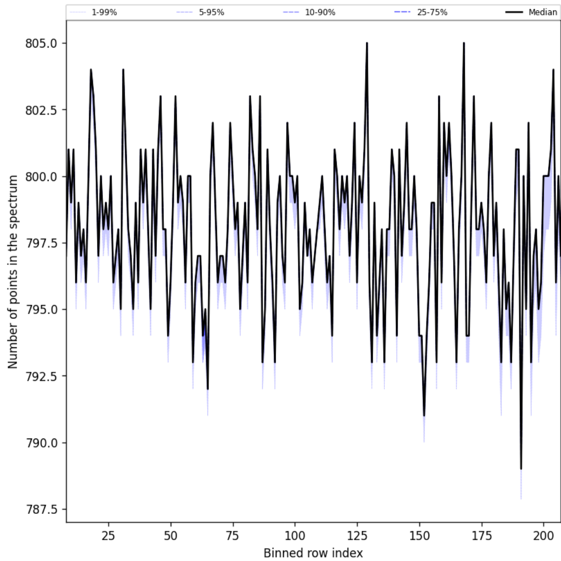
Figure 37: Along track statistics of “Number of points in the spectrum” for 2025-03-13 to 2025-03-15
