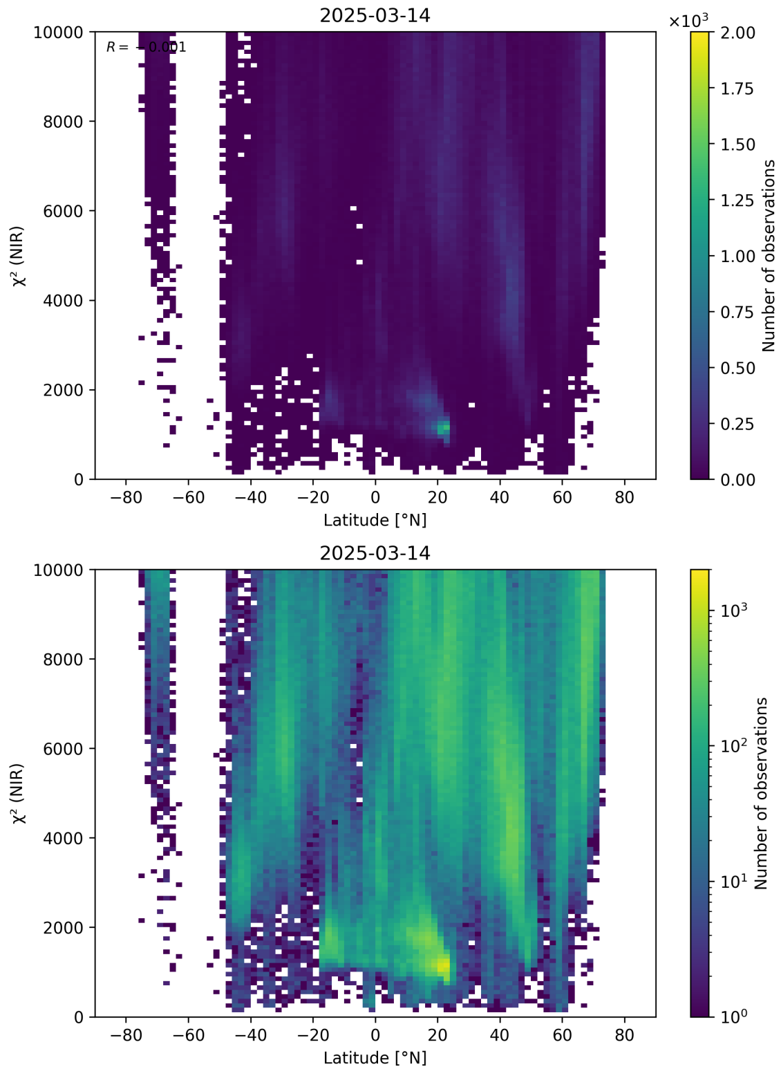
Figure 53: Scatter density plot of “Latitude” against “ \chi^2 (NIR)” for 2025-03-13 to 2025-03-15.
