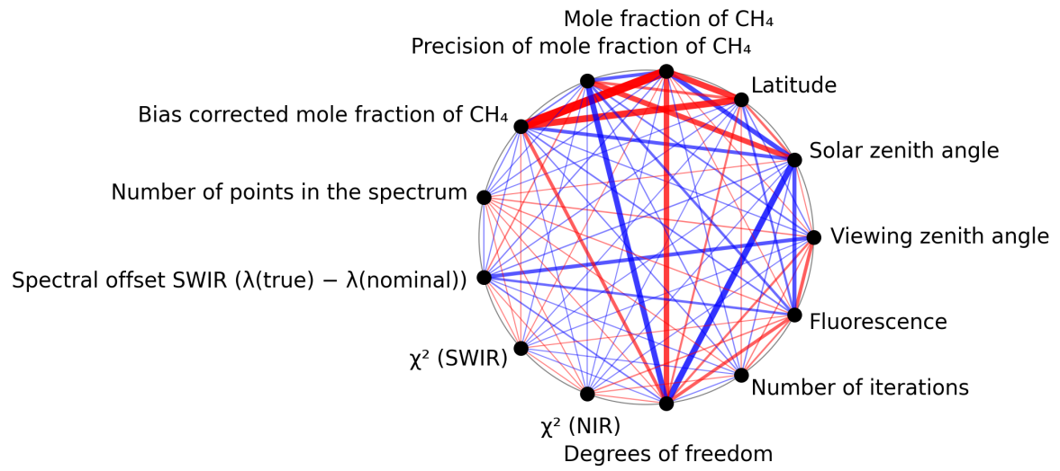
Figure 1: Map of correlation graph for 2025-03-13 to 2025-03-15.
