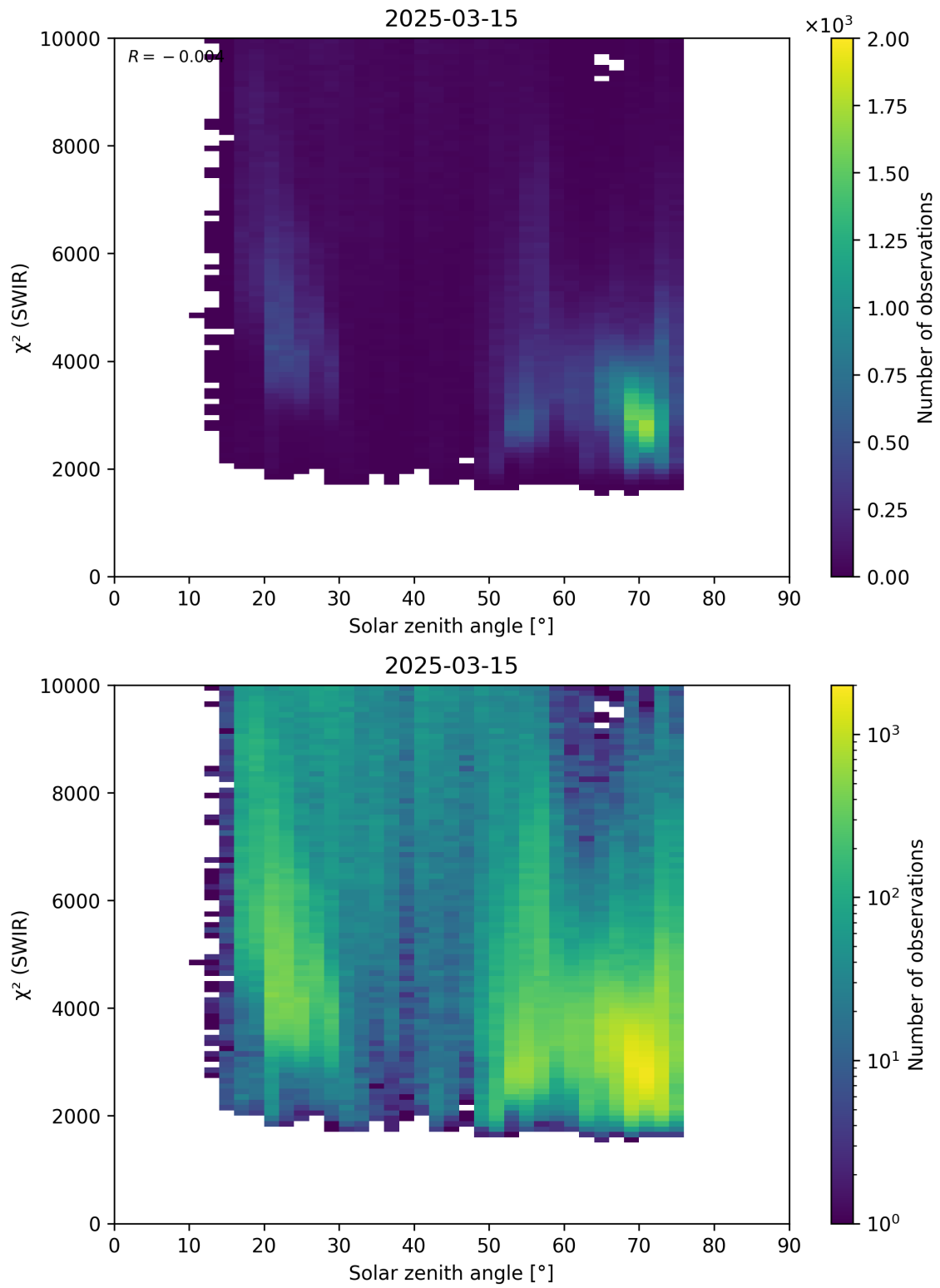
Figure 95: Scatter density plot of “Solar zenith angle” against “ \chi^2 (SWIR)” for 2025-03-14 to 2025-03-16.
