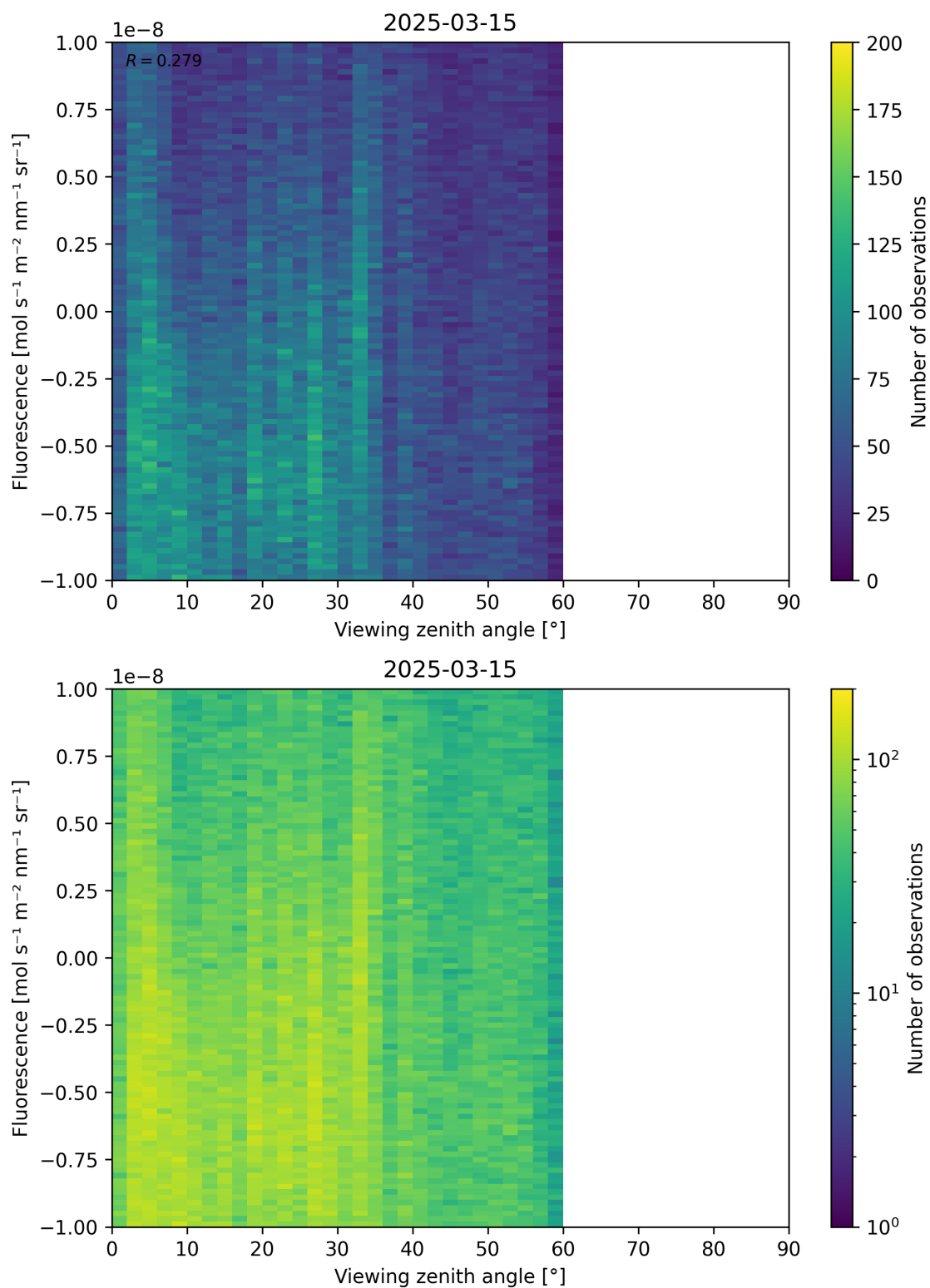
Figure 108: Scatter density plot of “Viewing zenith angle” against “Fluorescence” for 2025-03-14 to 2025-03-16.
