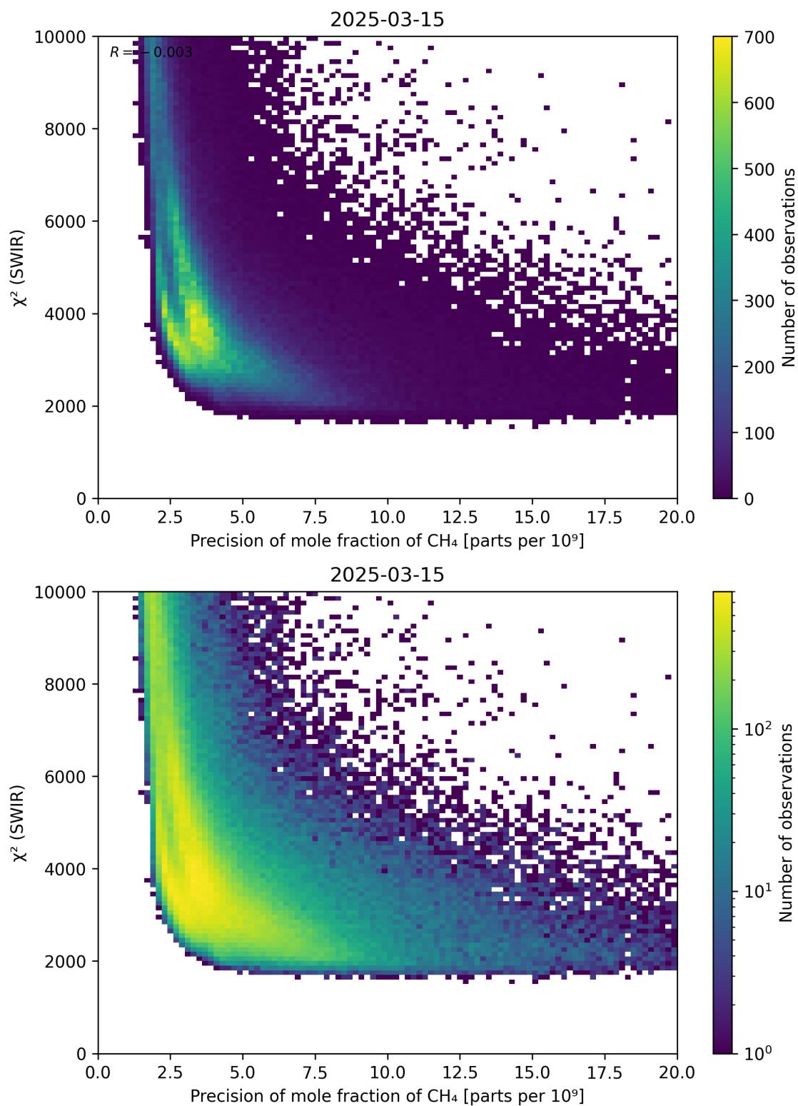
Figure 79: Scatter density plot of “Precision of mole fraction of CH 4 ” against “ \chi^2 (SWIR)” for 2025-03-14 to 2025-03-16.
