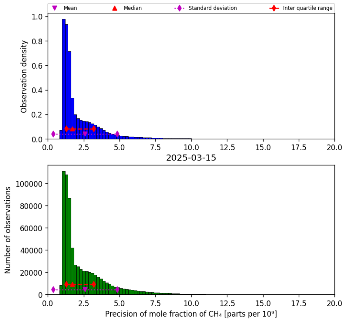
Figure 24: Histogram of “Precision of mole fraction of CH 4 ” for 2025-03-14 to 2025-03-16
