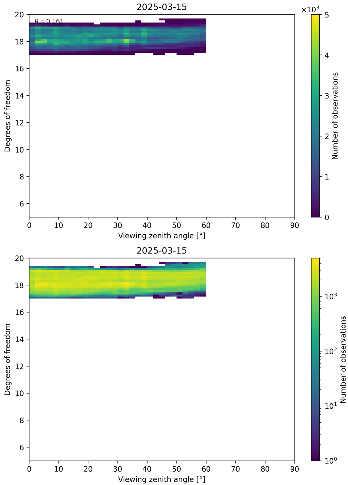
Figure 107: Scatter density plot of “Viewing zenith angle” against “Degrees of freedom” for 2025-03-14 to 2025-03-16.
