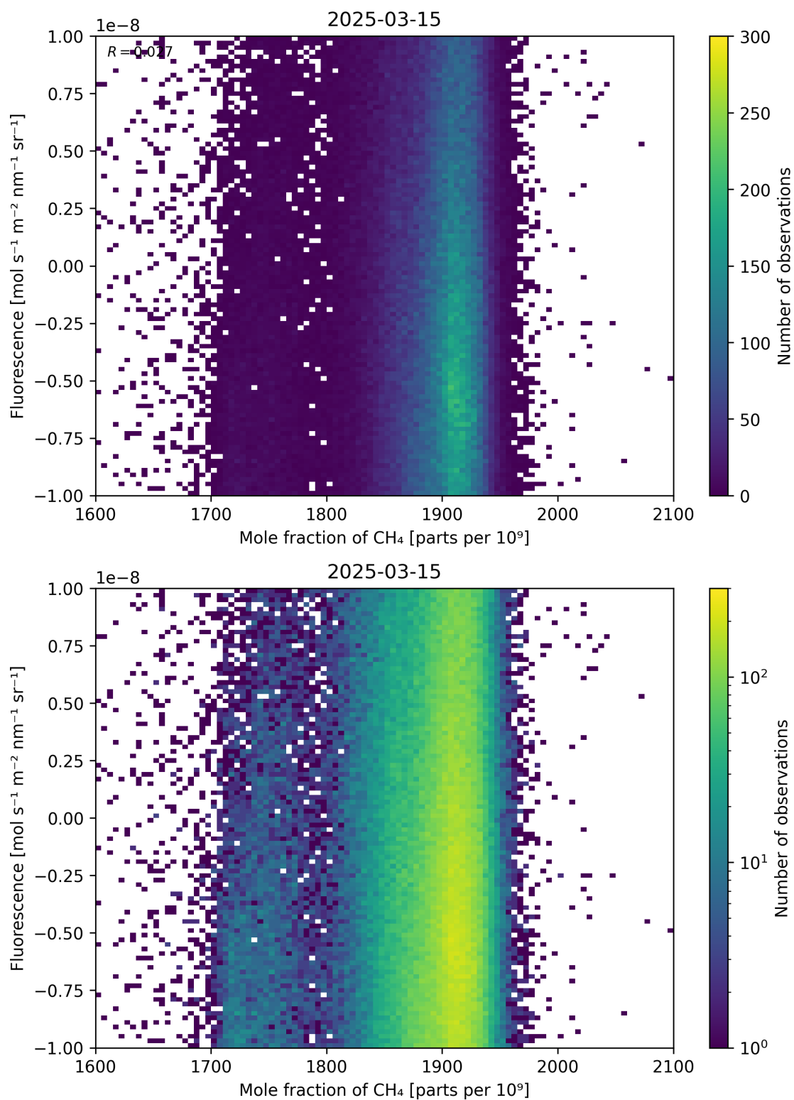
Figure 73: Scatter density plot of “Mole fraction of \text{CH}_4 ” against “Fluorescence” for 2025-03-14 to 2025-03-16.
