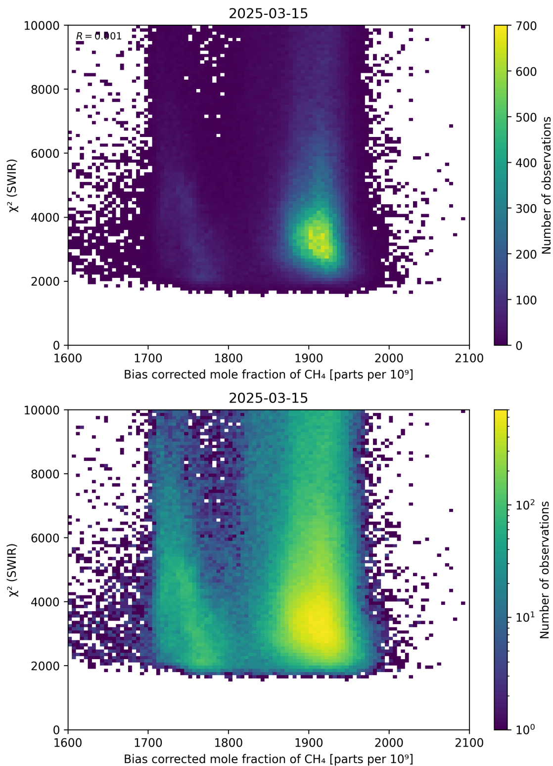
Figure 64: Scatter density plot of “Bias corrected mole fraction of \text{CH}_4 ” against “ \chi^2 (SWIR)” for 2025-03-14 to 2025-03-16.
