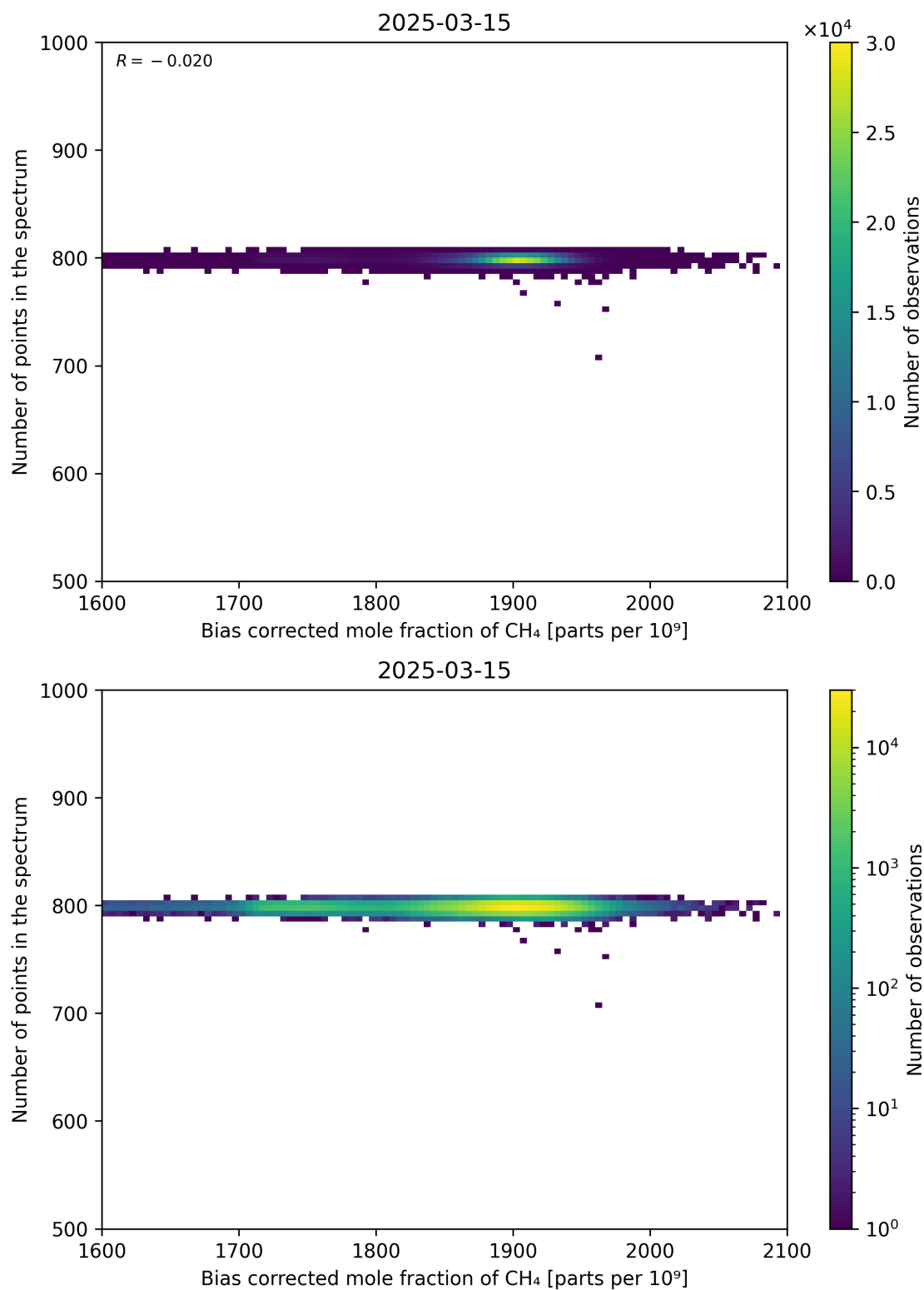
Figure 68: Scatter density plot of “Bias corrected mole fraction of CH 4 ” against “Number of points in the spectrum” for 2025-03-14 to 2025-03-16.
