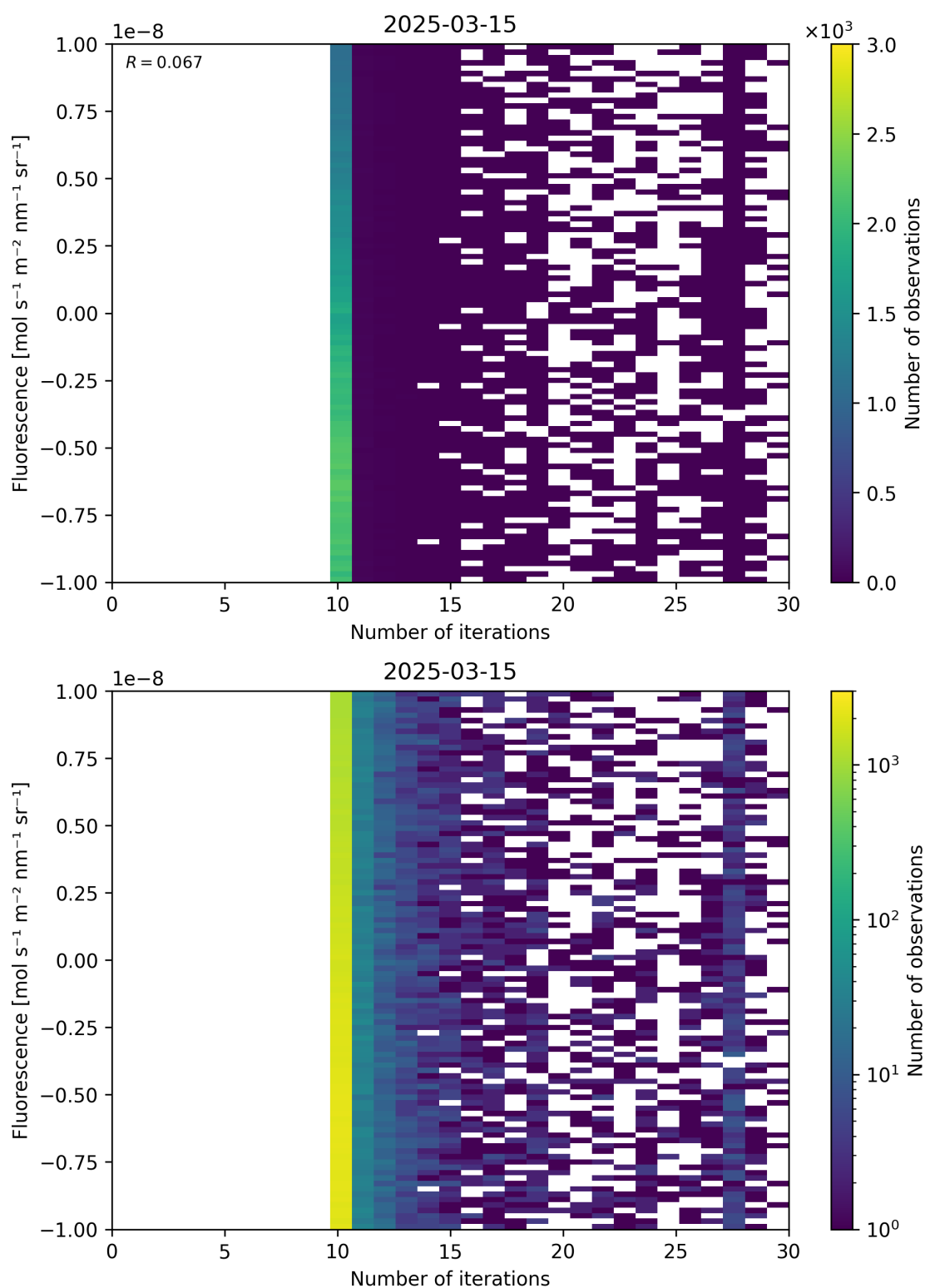
Figure 87: Scatter density plot of “Number of iterations” against “Fluorescence” for 2025-03-14 to 2025-03-16.
