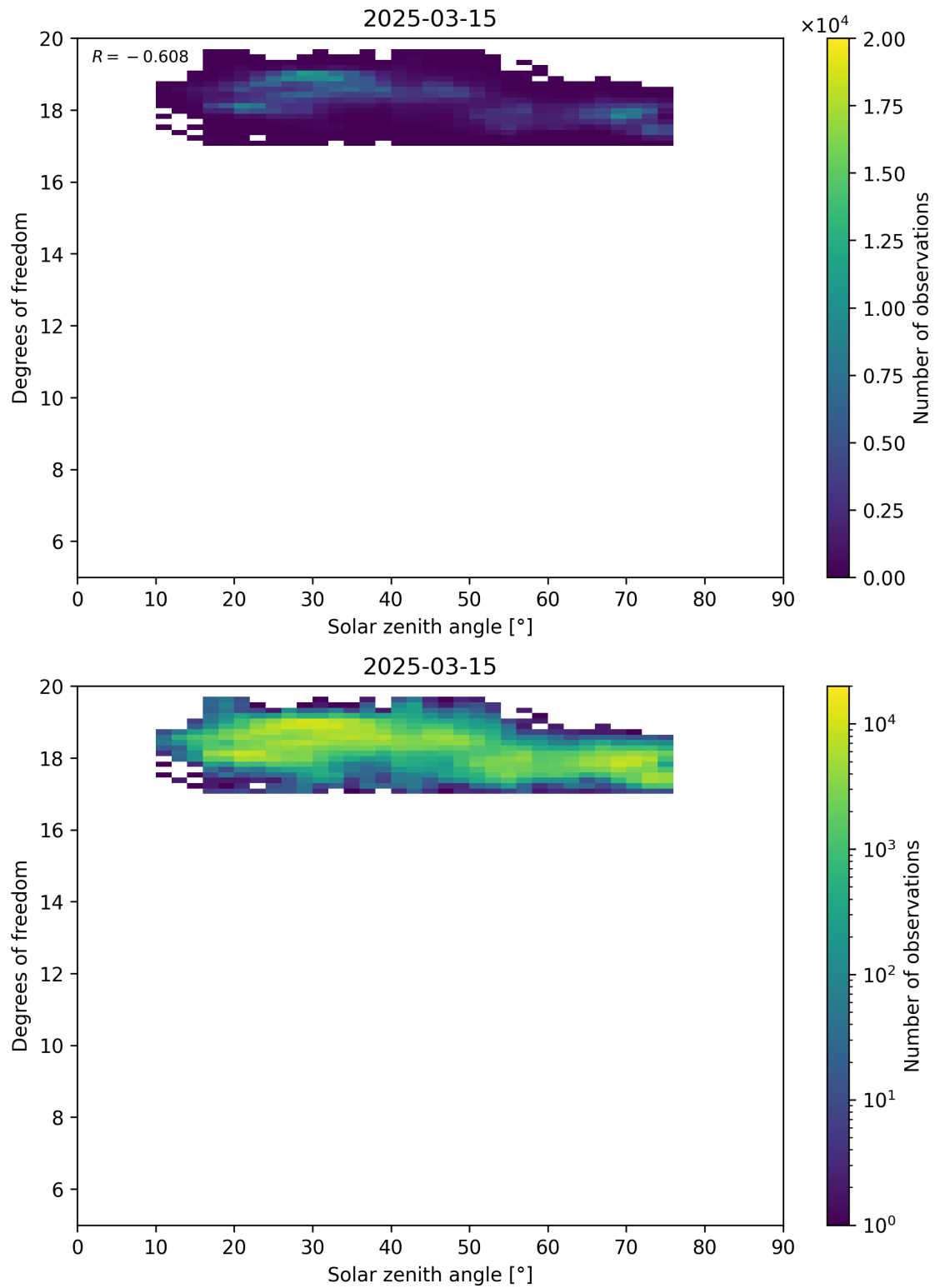
Figure 96: Scatter density plot of “Solar zenith angle” against “Degrees of freedom” for 2025-03-14 to 2025-03-16.
