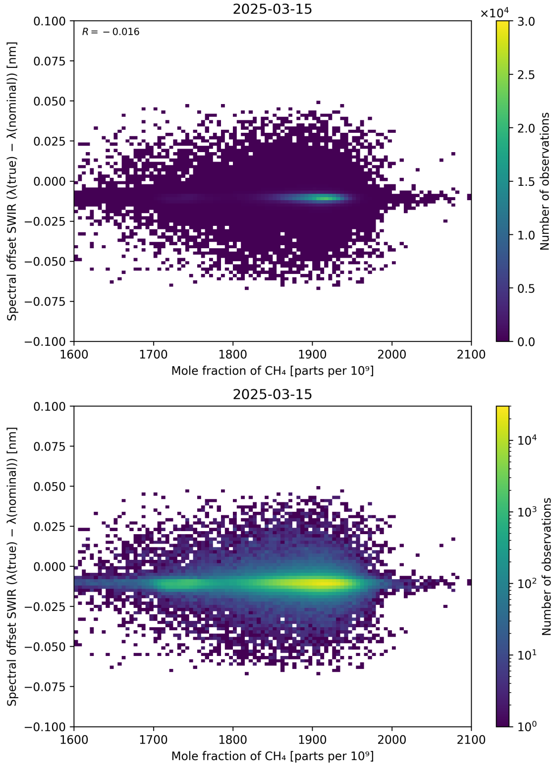
Figure 86: Scatter density plot of “Mole fraction of CH 4 ” against “Spectral offset SWIR ( \lambda_{\text{true}} - \lambda_{\text{nominal}} )” for 2025-03-14 to 2025-03-16.
