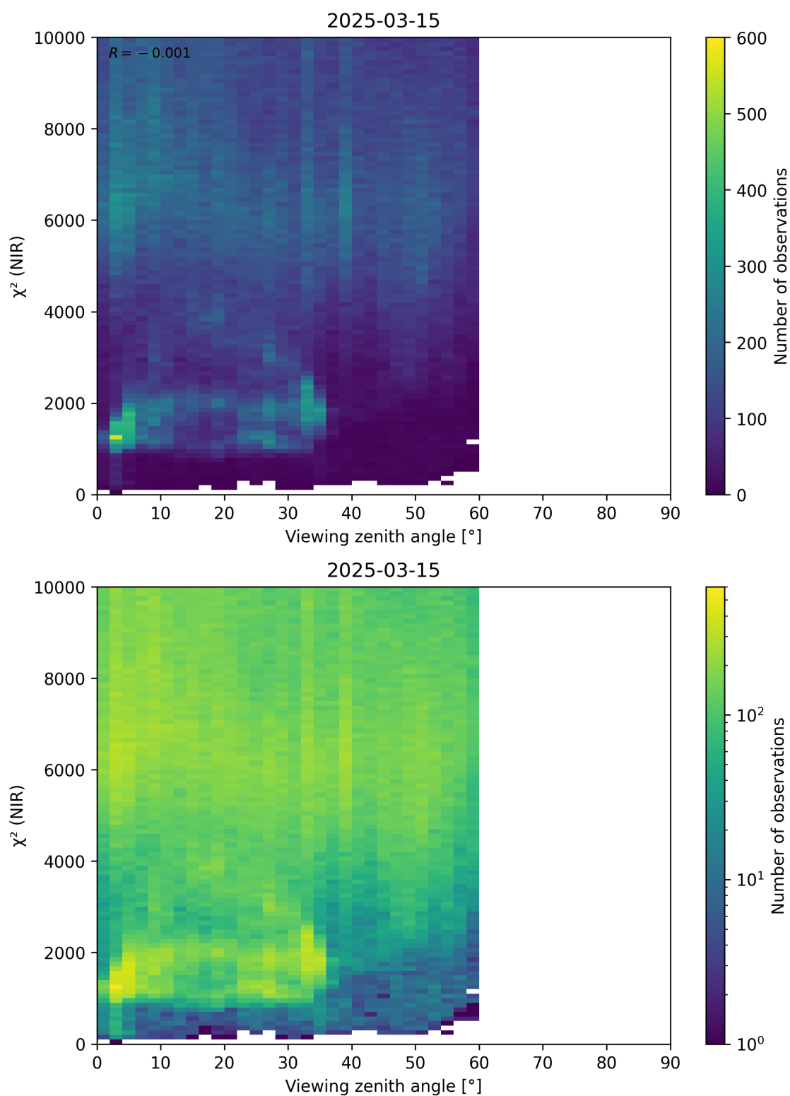
Figure 105: Scatter density plot of “Viewing zenith angle” against “ \chi^2 (NIR)” for 2025-03-14 to 2025-03-16.
