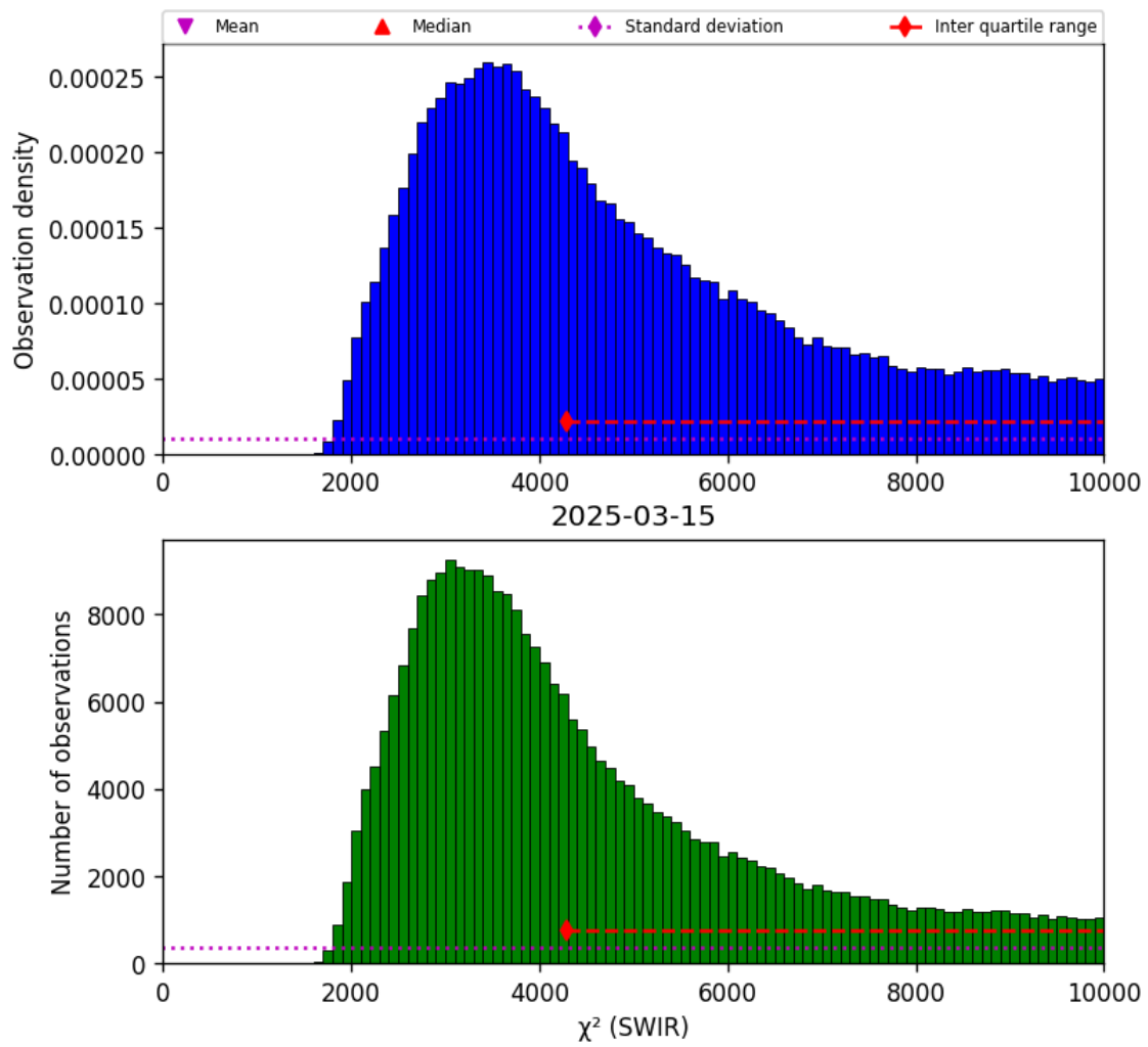
Figure 28: Histogram of “ \chi^2 (SWIR)” for 2025-03-14 to 2025-03-16
