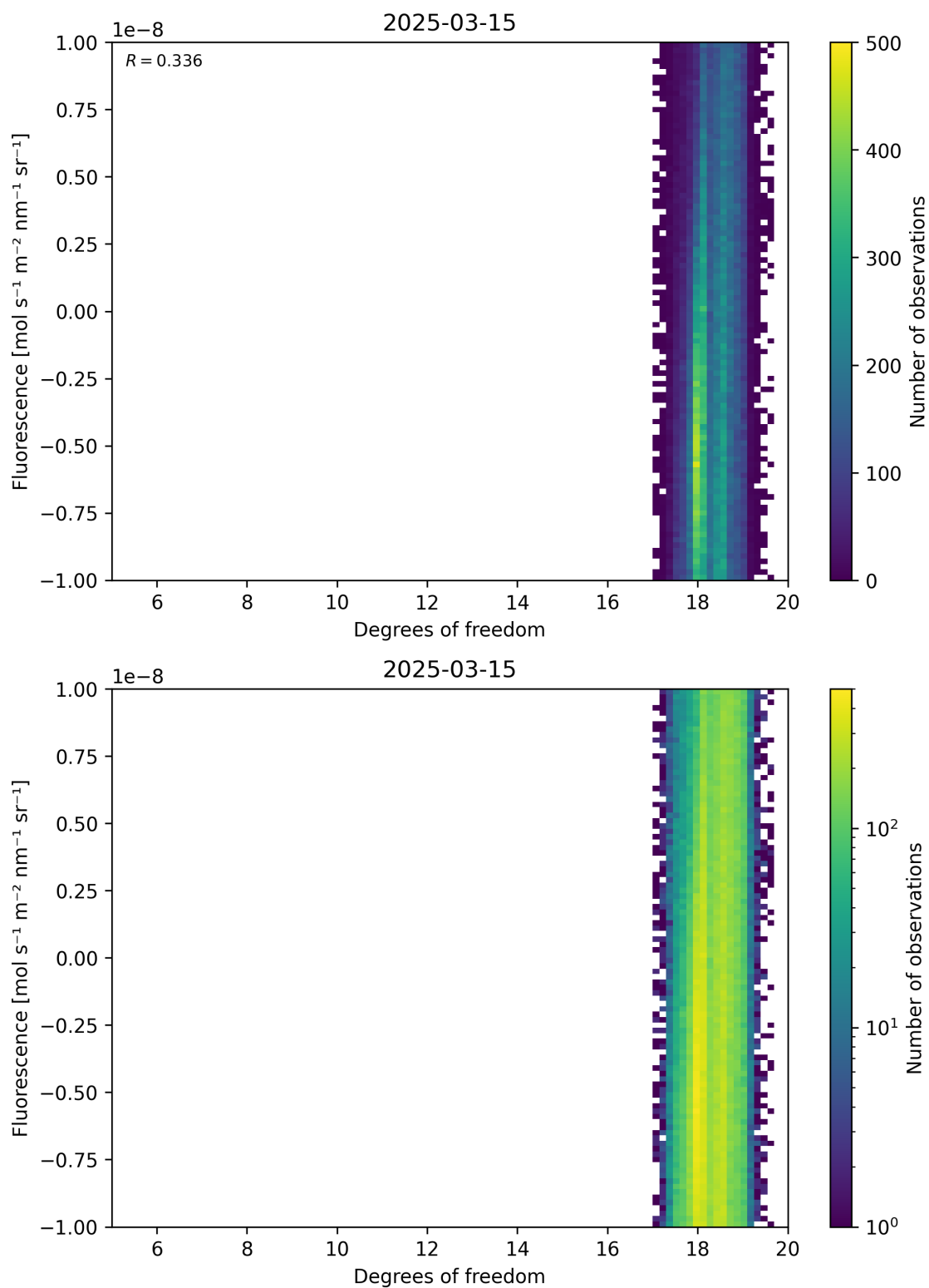
Figure 51: Scatter density plot of “Degrees of freedom” against “Fluorescence” for 2025-03-14 to 2025-03-16.
