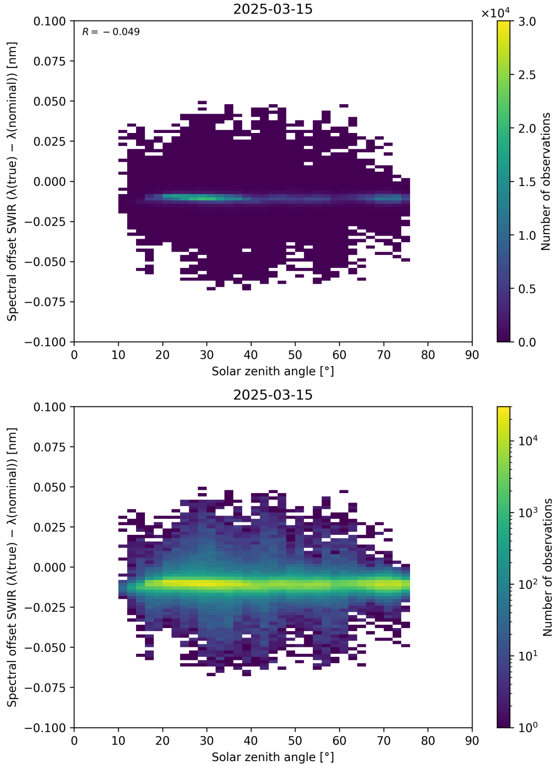
Figure 104: Scatter density plot of “Solar zenith angle” against “Spectral offset SWIR ( \lambda_{\text{true}} - \lambda_{\text{nominal}} )” for 2025-03-14 to 2025-03-16.
