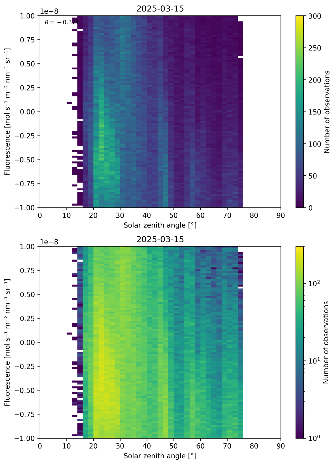
Figure 97: Scatter density plot of “Solar zenith angle” against “Fluorescence” for 2025-03-14 to 2025-03-16.
