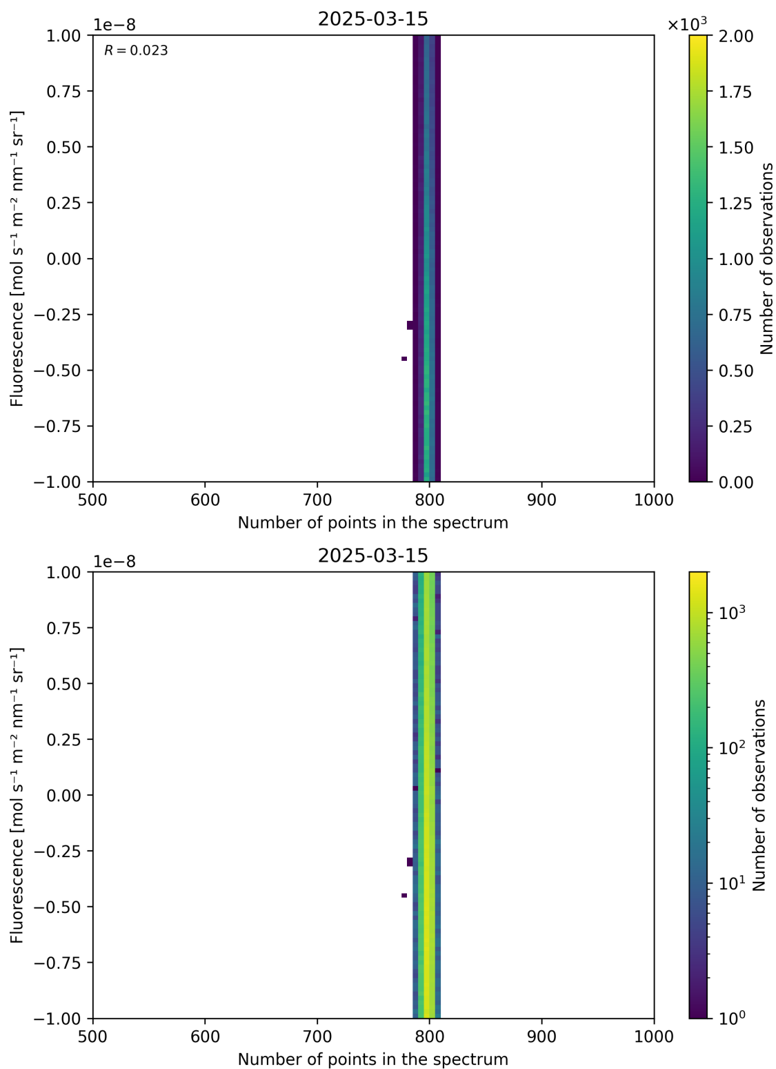
Figure 91: Scatter density plot of “Number of points in the spectrum” against “Fluorescence” for 2025-03-14 to 2025-03-16.
