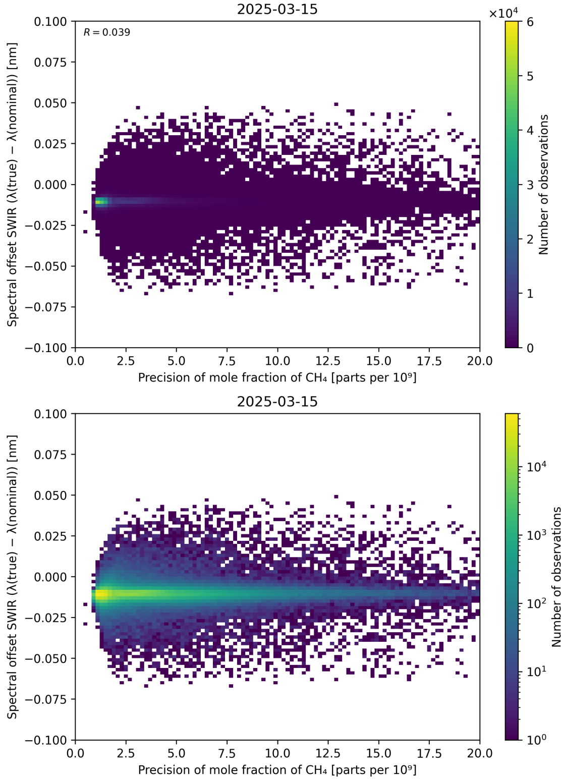
Figure 85: Scatter density plot of “Precision of mole fraction of \text{CH}_4 ” against “Spectral offset SWIR ( \lambda_{\text{true}} - \lambda_{\text{nominal}} )” for 2025-03-14 to 2025-03-16.
