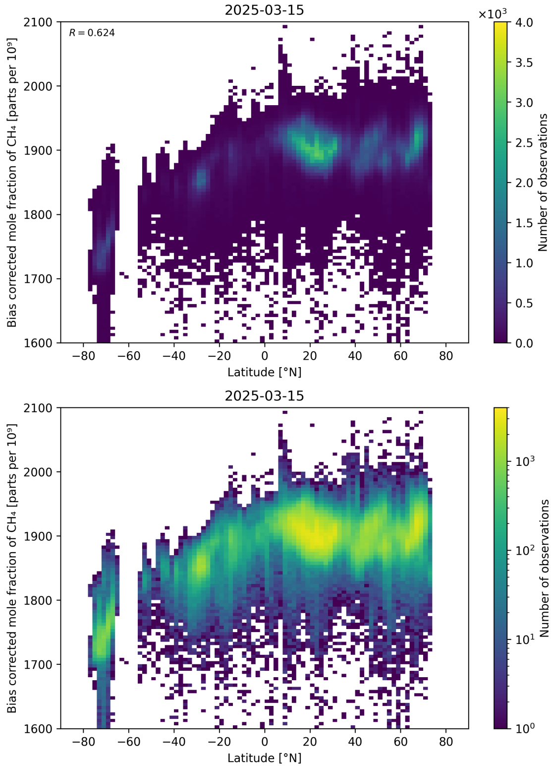
Figure 58: Scatter density plot of “Latitude” against “Bias corrected mole fraction of CH 4 ” for 2025-03-14 to 2025-03-16.
