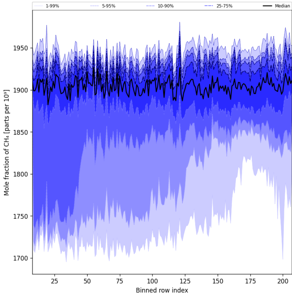
Figure 34: Along track statistics of “Mole fraction of CH 4 ” for 2025-03-14 to 2025-03-16
