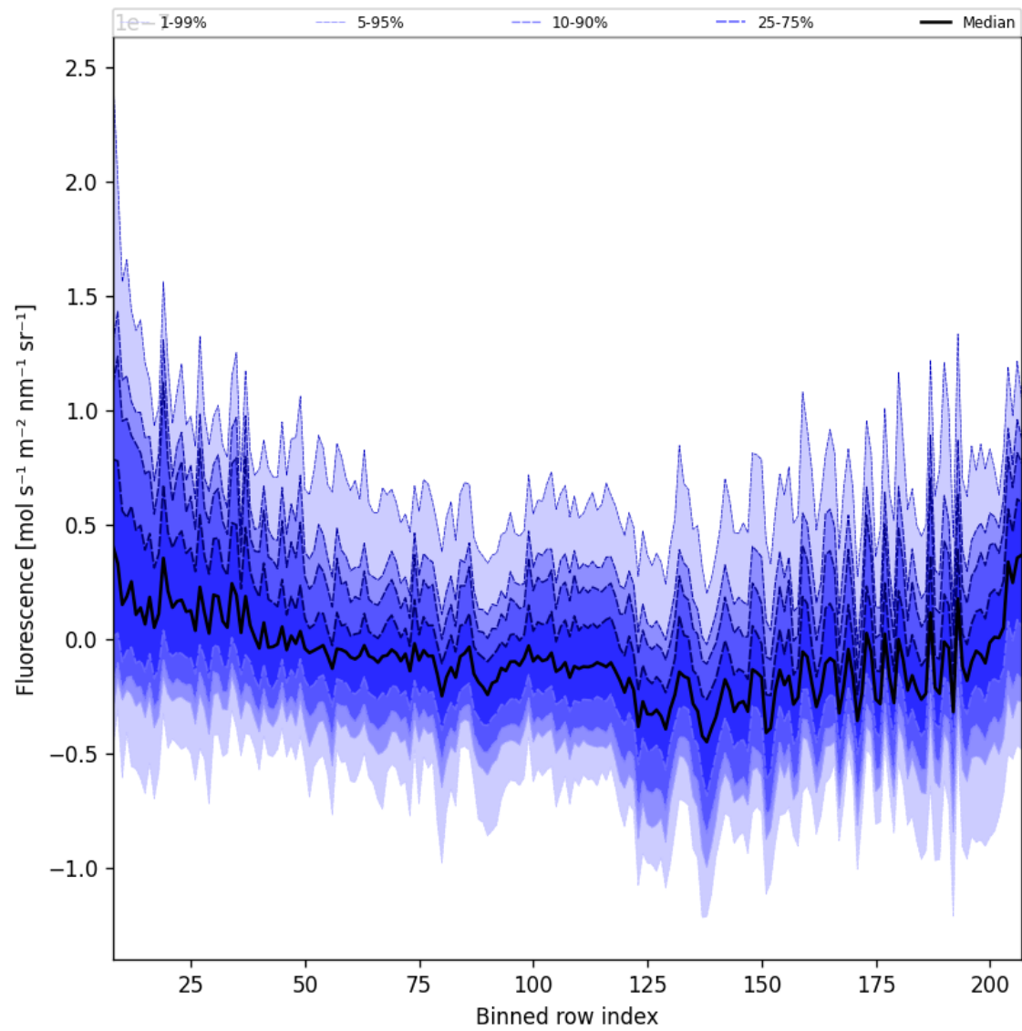
Figure 43: Along track statistics of “Fluorescence” for 2025-03-14 to 2025-03-16
