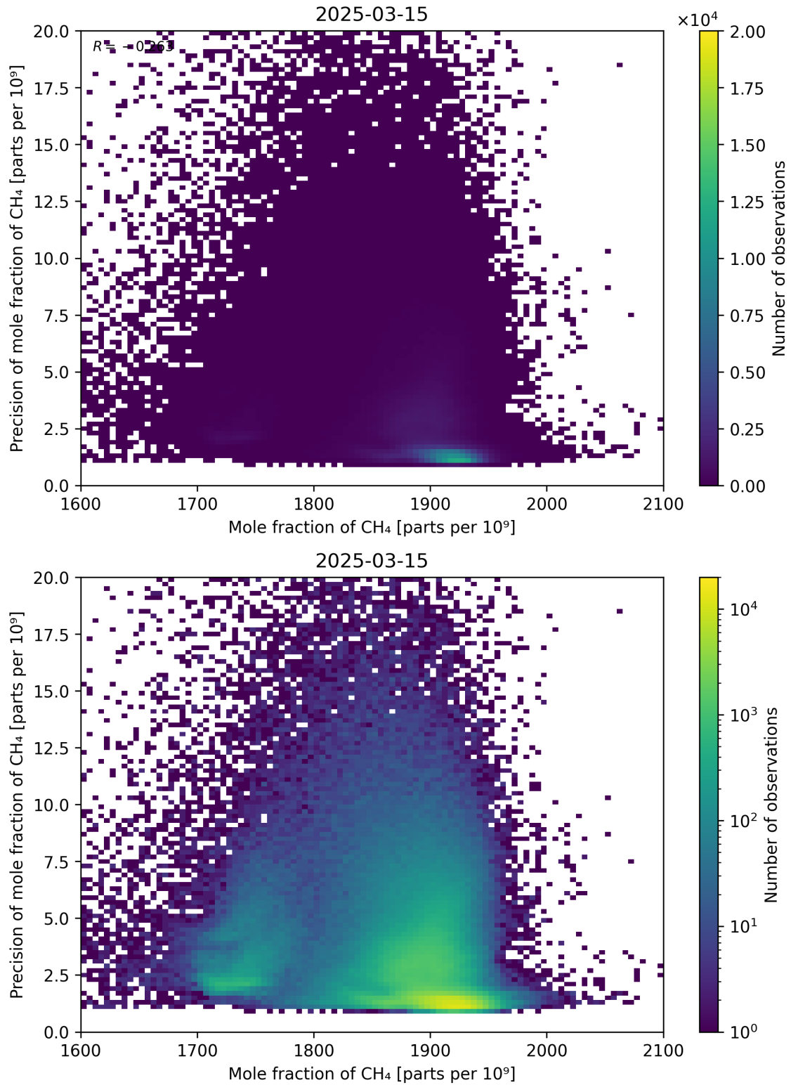
Figure 75: Scatter density plot of “Mole fraction of CH 4 ” against “Precision of mole fraction of CH 4 ” for 2025-03-14 to 2025-03-16.
