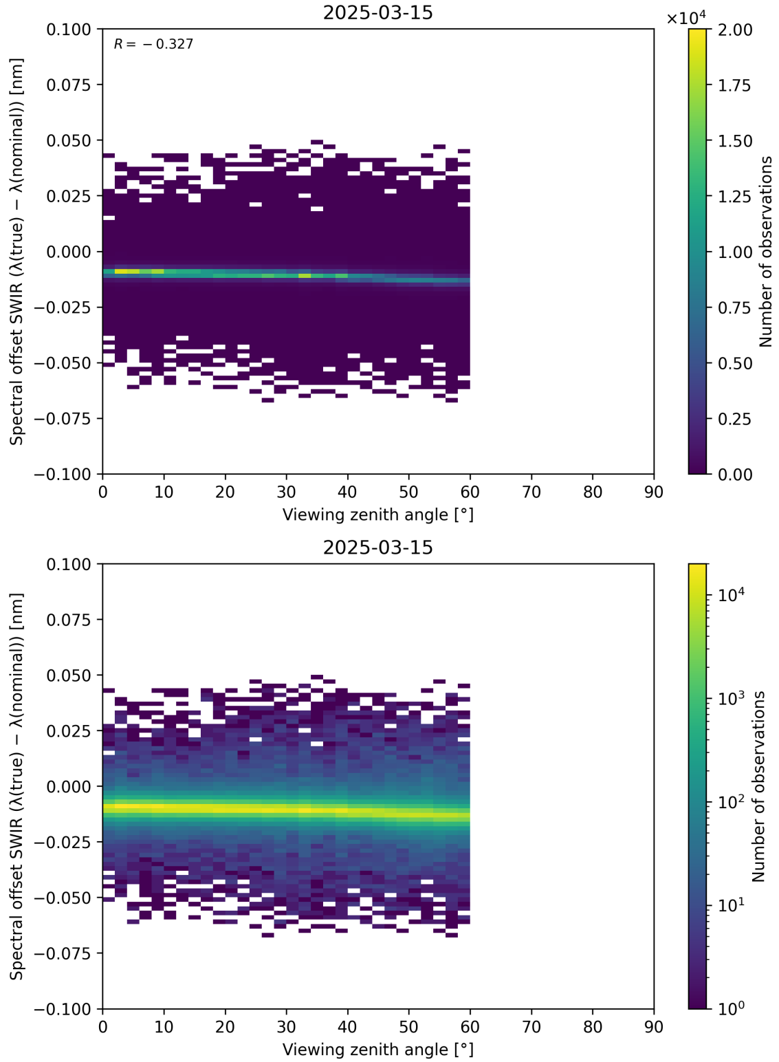
Figure 116: Scatter density plot of “Viewing zenith angle” against “Spectral offset SWIR ( \lambda_{\text{true}} - \lambda_{\text{nominal}} )” for 2025-03-14 to 2025-03-16.
