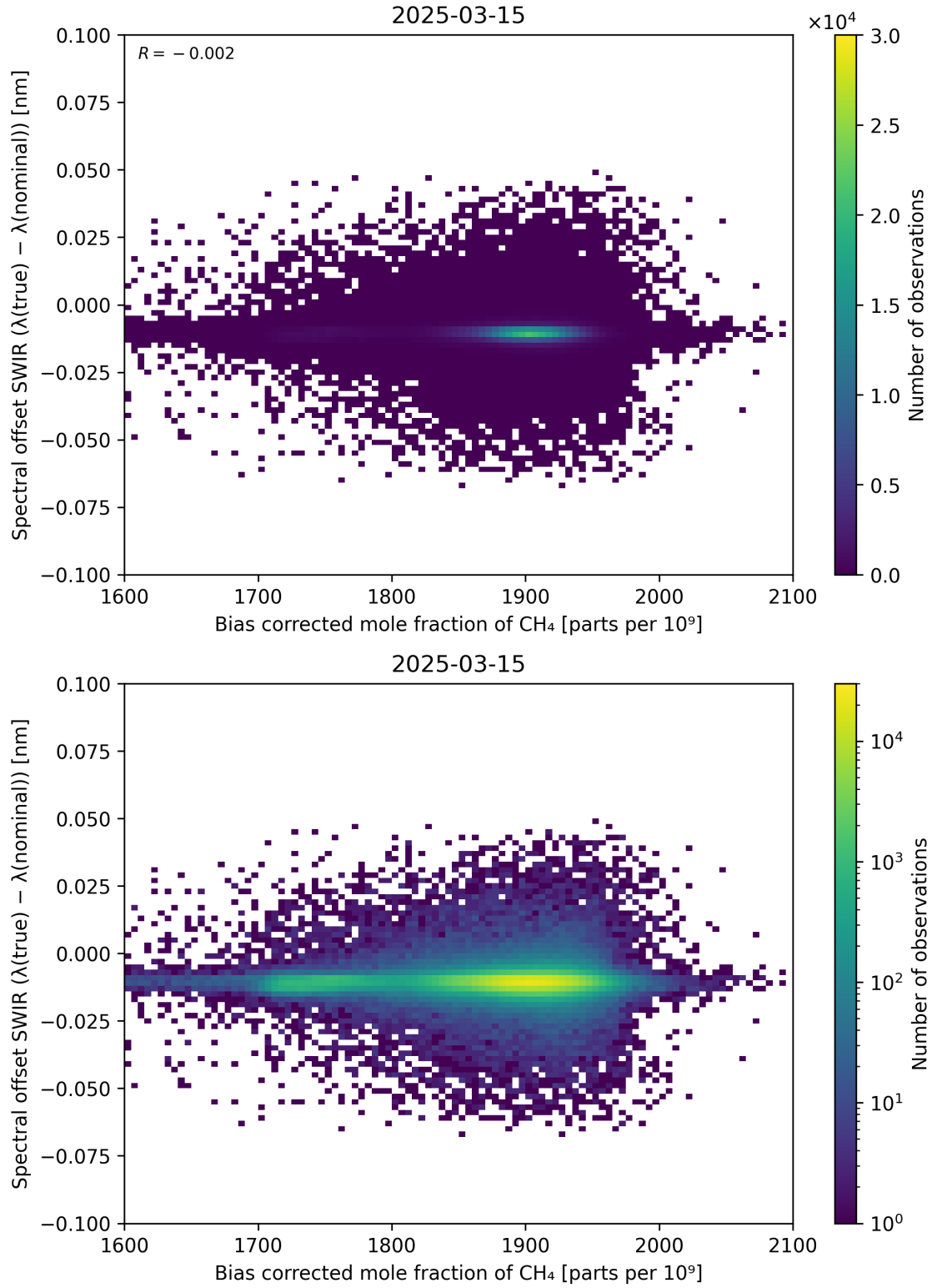
Figure 69: Scatter density plot of “Bias corrected mole fraction of \text{CH}_4 ” against “Spectral offset SWIR ( \lambda_{\text{true}} - \lambda_{\text{nominal}} )” for 2025-03-14 to 2025-03-16.
