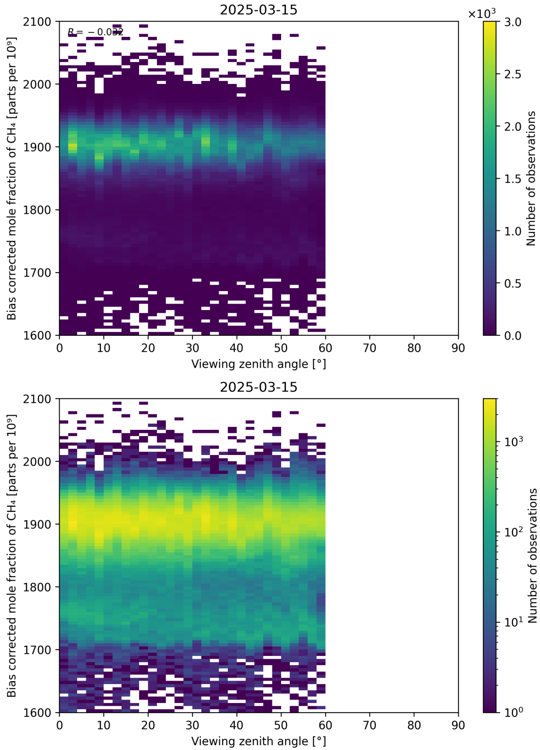
Figure 111: Scatter density plot of “Viewing zenith angle” against “Bias corrected mole fraction of CH 4 ” for 2025-03-14 to 2025-03-16.
