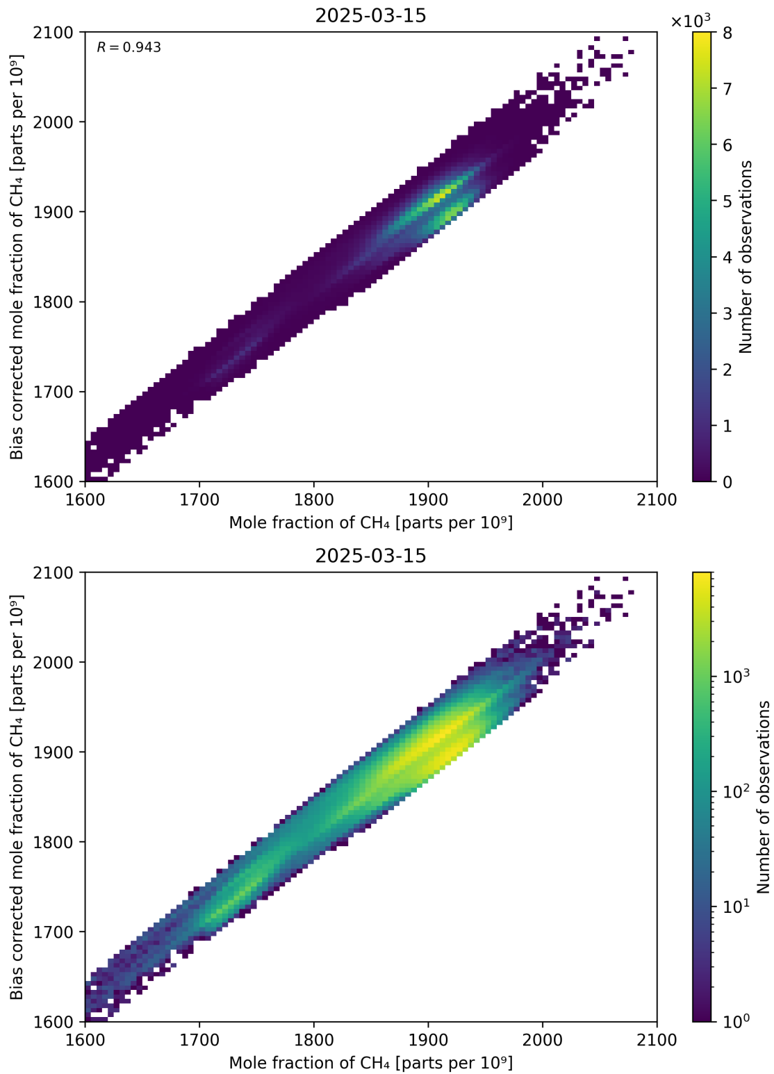
Figure 74: Scatter density plot of “Mole fraction of CH 4 ” against “Bias corrected mole fraction of CH 4 ” for 2025-03-14 to 2025-03-16.
