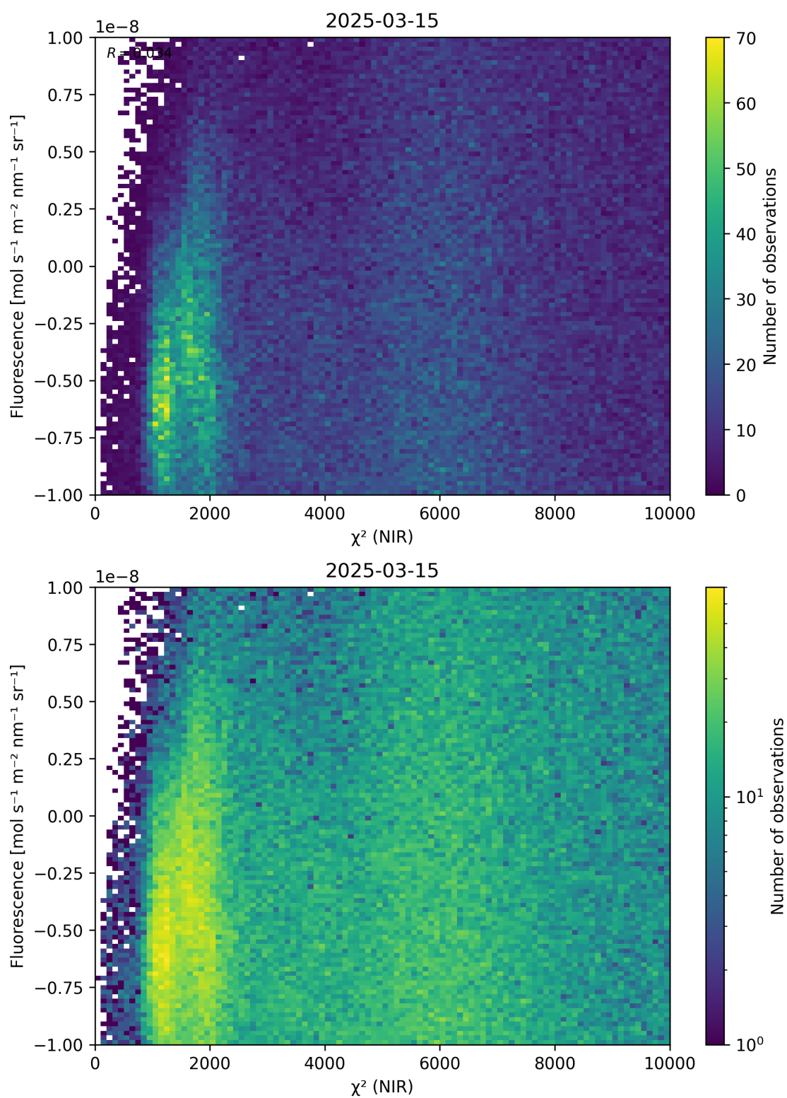
Figure 45: Scatter density plot of “ \chi^2 (NIR)” against “Fluorescence” for 2025-03-14 to 2025-03-16.
