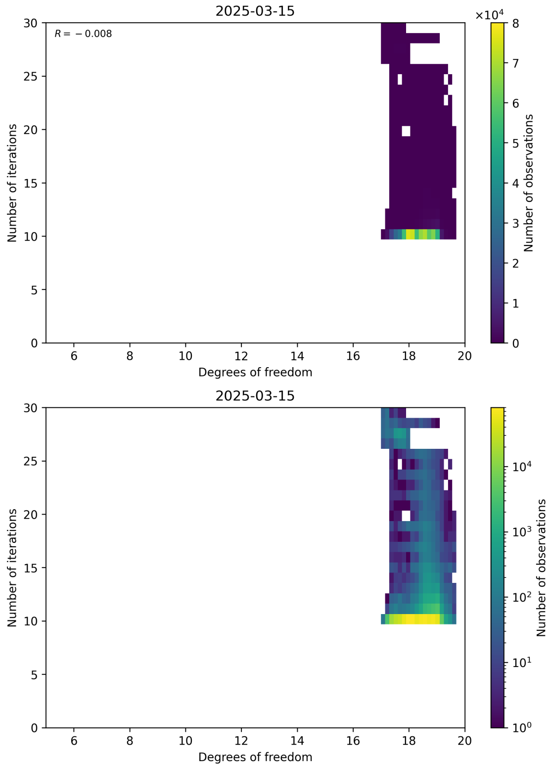
Figure 52: Scatter density plot of “Degrees of freedom” against “Number of iterations” for 2025-03-14 to 2025-03-16.
