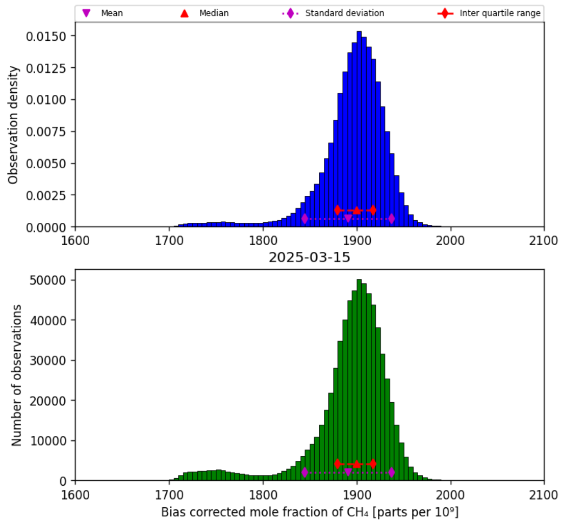
Figure 25: Histogram of “Bias corrected mole fraction of CH 4 ” for 2025-03-14 to 2025-03-16
