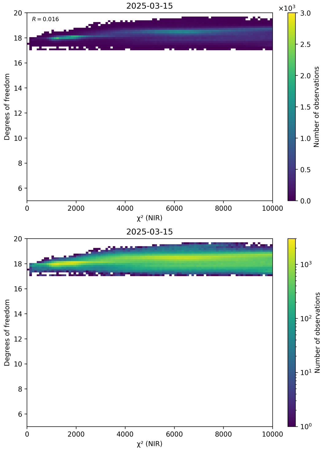
Figure 44: Scatter density plot of “ \chi^2 (NIR)” against “Degrees of freedom” for 2025-03-14 to 2025-03-16.
