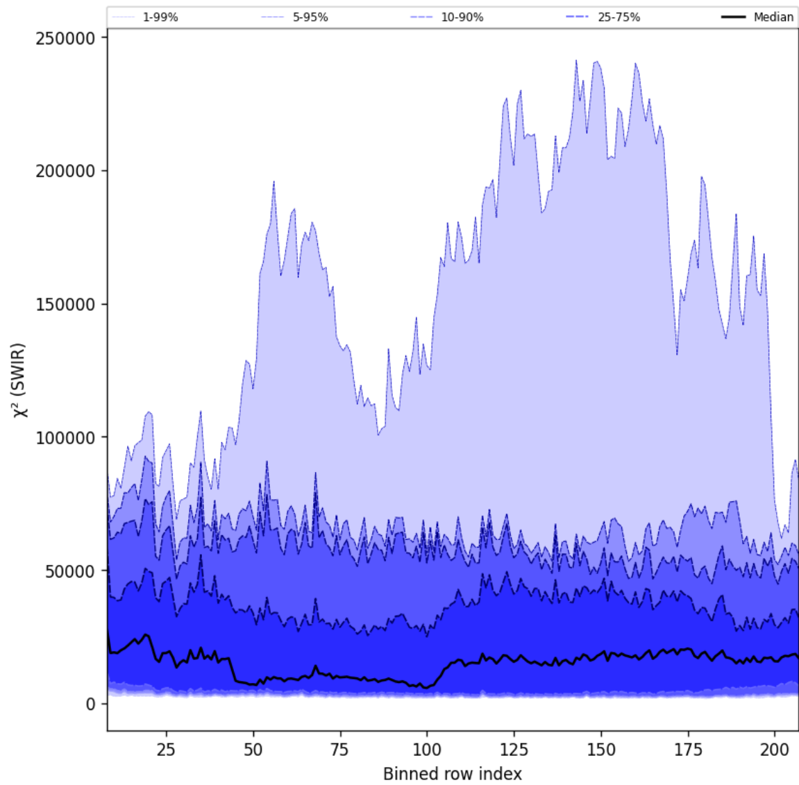
Figure 39: Along track statistics of “ \chi^2 (SWIR)” for 2025-03-14 to 2025-03-16
