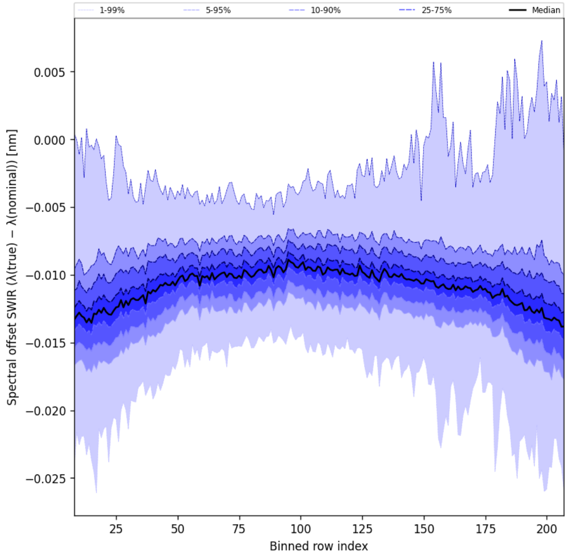
Figure 38: Along track statistics of “Spectral offset SWIR ( \lambda_{\text{true}} - \lambda_{\text{nominal}} )” for 2025-03-14 to 2025-03-16
