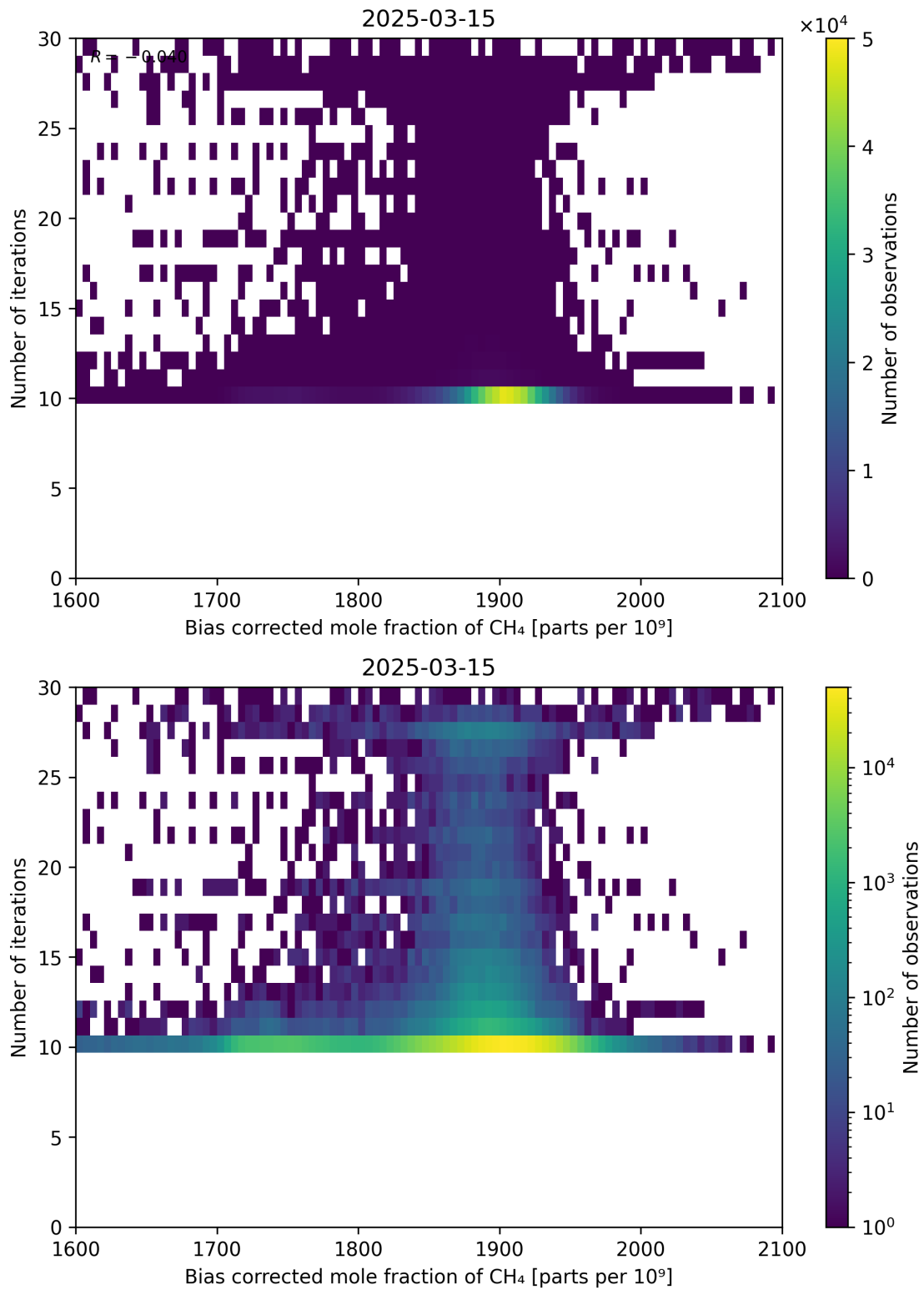
Figure 67: Scatter density plot of “Bias corrected mole fraction of \text{CH}_4 ” against “Number of iterations” for 2025-03-14 to 2025-03-16.
