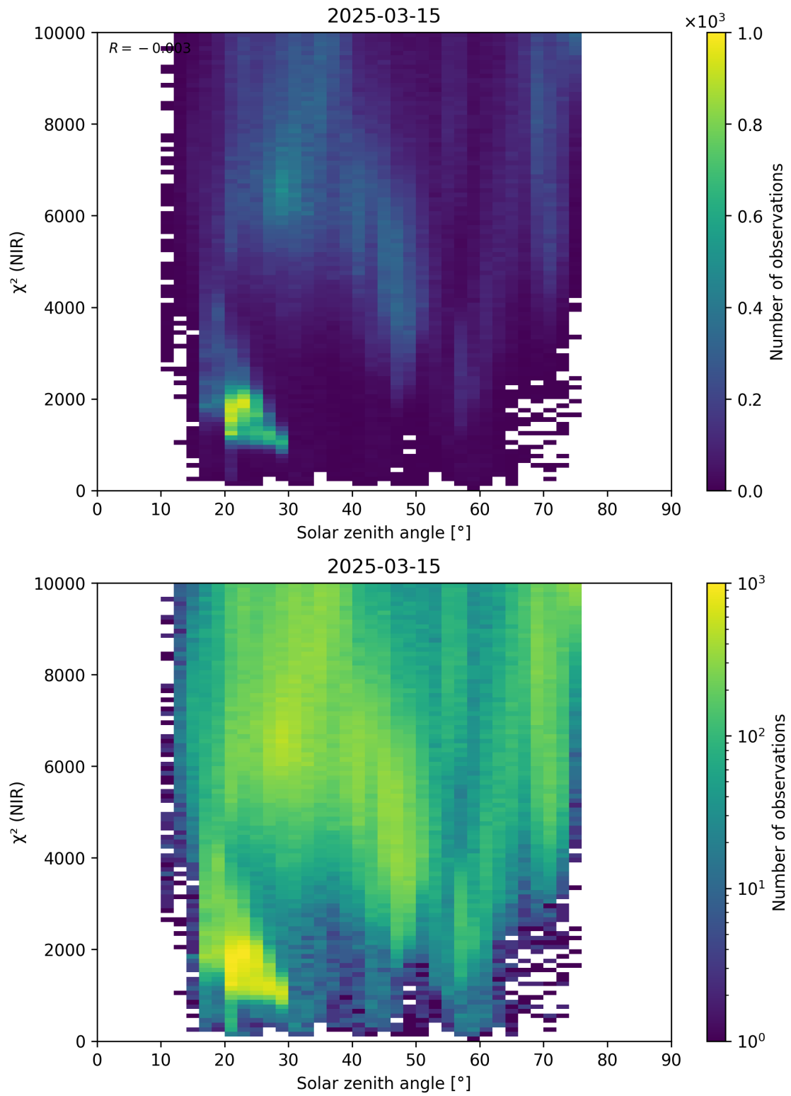
Figure 94: Scatter density plot of “Solar zenith angle” against “ \chi^2 (NIR)” for 2025-03-14 to 2025-03-16.
