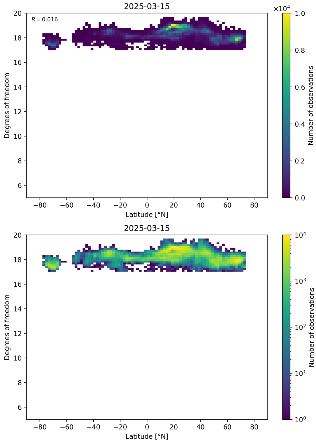
Figure 55: Scatter density plot of “Latitude” against “Degrees of freedom” for 2025-03-14 to 2025-03-16.
