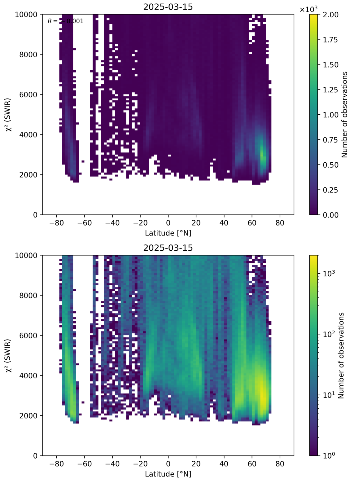
Figure 54: Scatter density plot of “Latitude” against “ \chi^2 (SWIR)” for 2025-03-14 to 2025-03-16.
