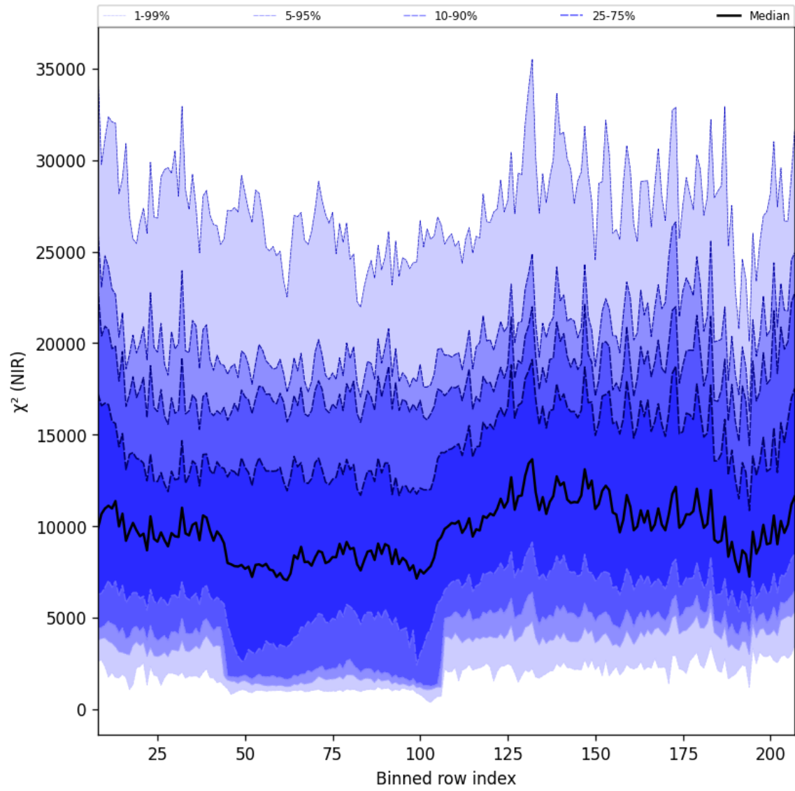
Figure 40: Along track statistics of “ \chi^2 (NIR)” for 2025-03-14 to 2025-03-16
