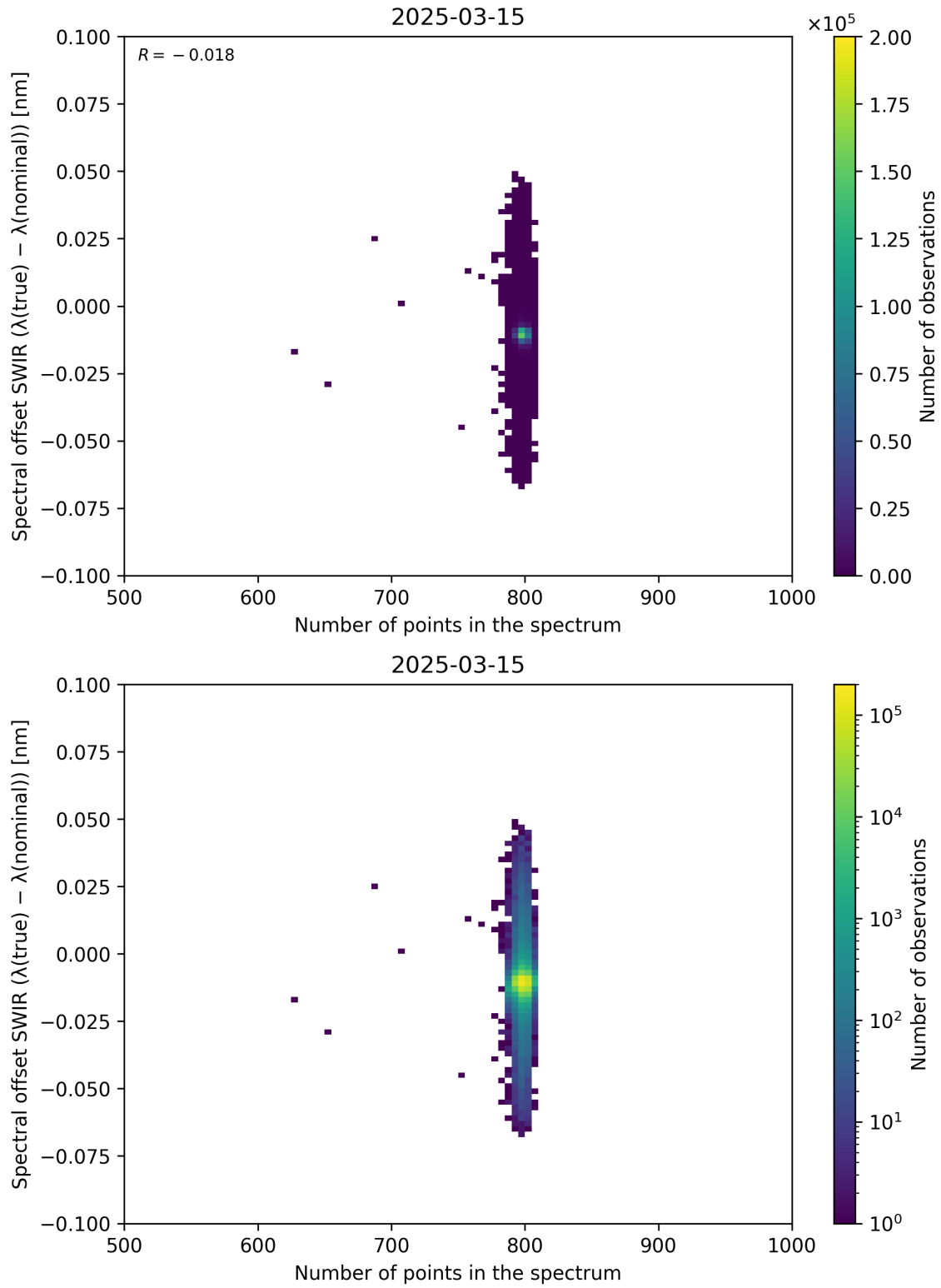
Figure 93: Scatter density plot of “Number of points in the spectrum” against “Spectral offset SWIR ( \lambda_{\text{true}} - \lambda_{\text{nominal}} )” for 2025-03-14 to 2025-03-16.
