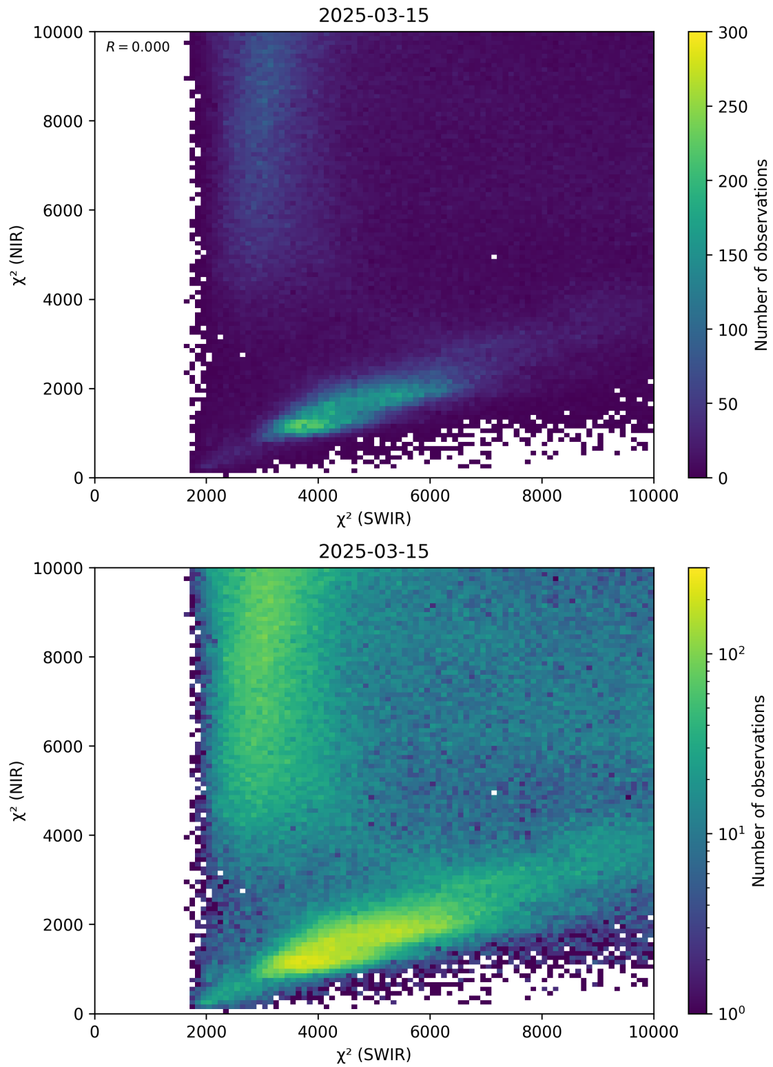
Figure 47: Scatter density plot of “ \chi^2 (SWIR)” against “ \chi^2 (NIR)” for 2025-03-14 to 2025-03-16.
