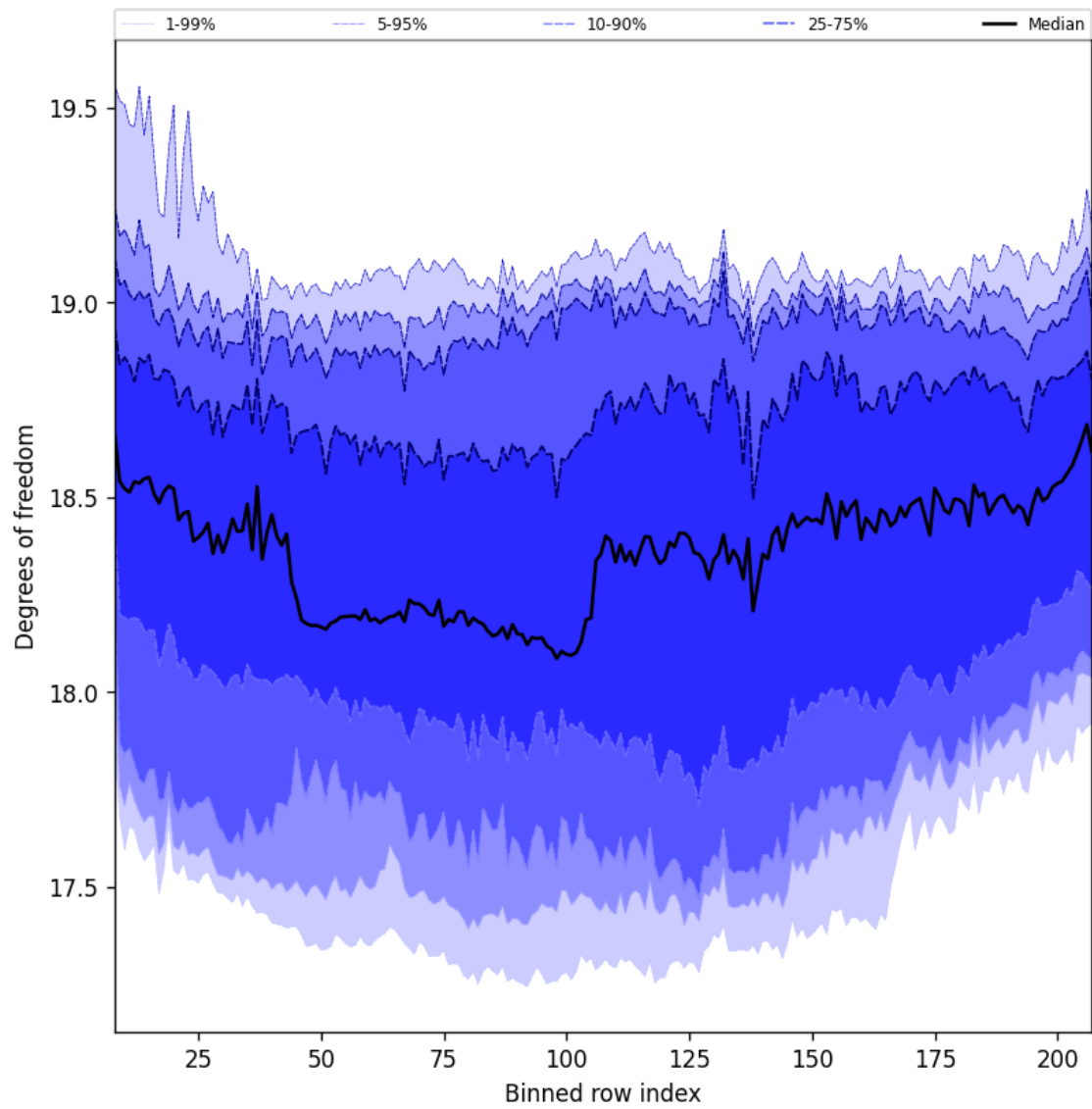
Figure 41: Along track statistics of “Degrees of freedom” for 2025-03-14 to 2025-03-16
