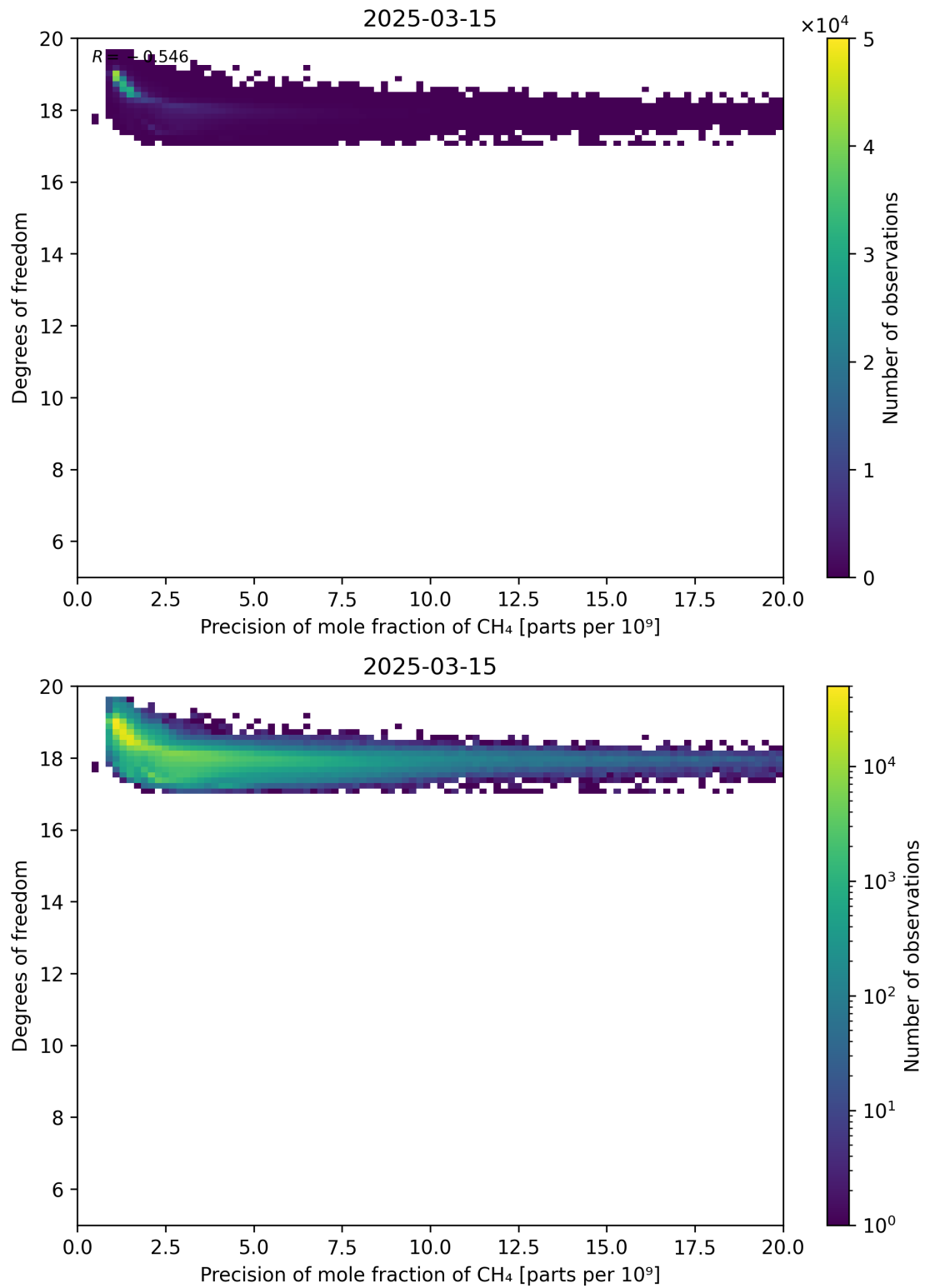
Figure 80: Scatter density plot of “Precision of mole fraction of CH 4 ” against “Degrees of freedom” for 2025-03-14 to 2025-03-16.
