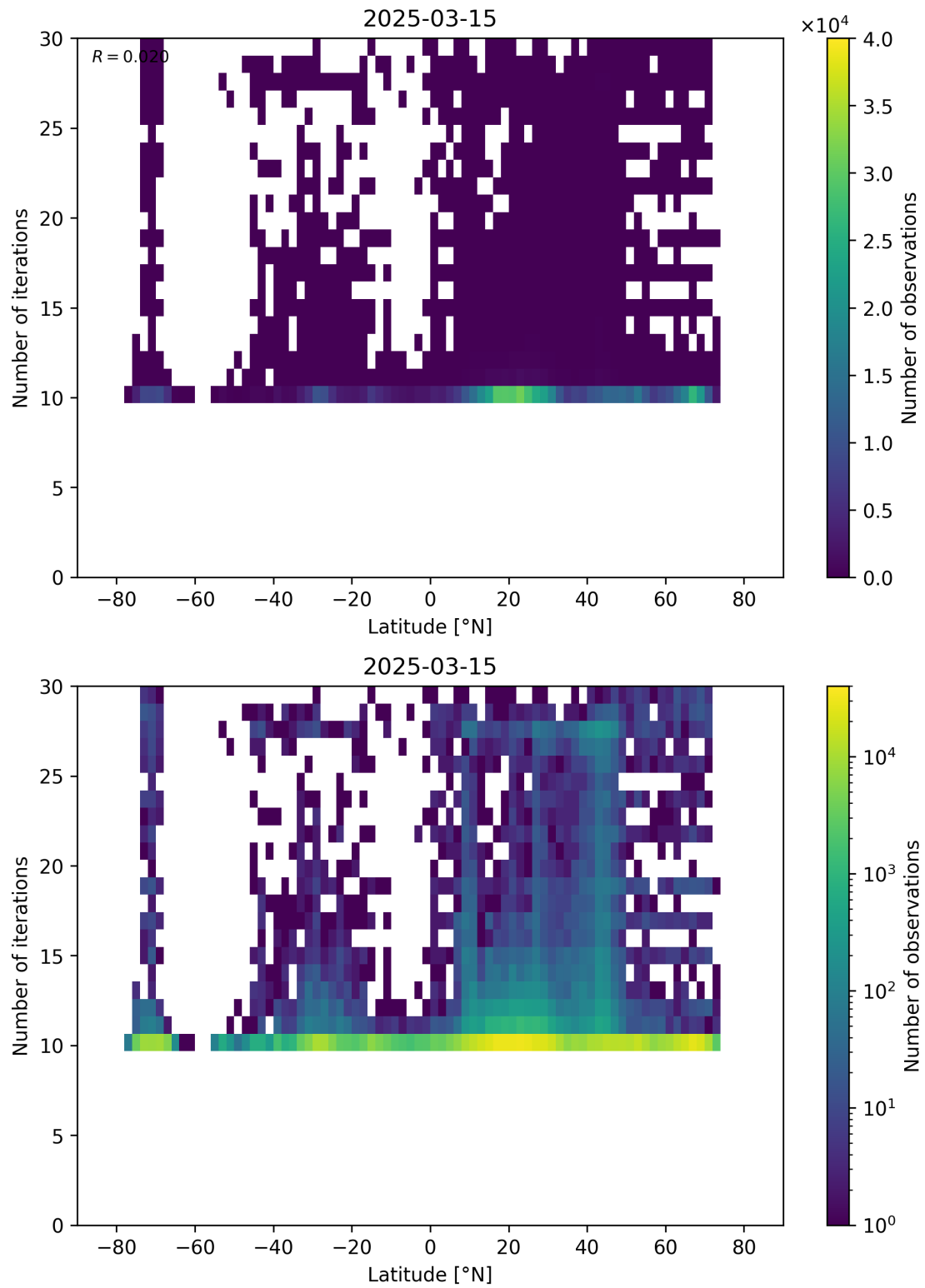
Figure 60: Scatter density plot of “Latitude” against “Number of iterations” for 2025-03-14 to 2025-03-16.
