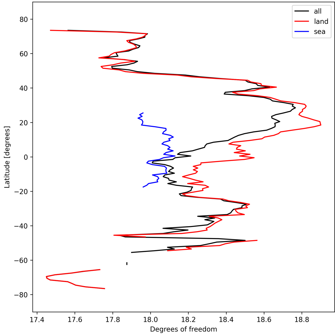
Figure 19: Zonal average of “Degrees of freedom” for 2025-03-14 to 2025-03-16.
