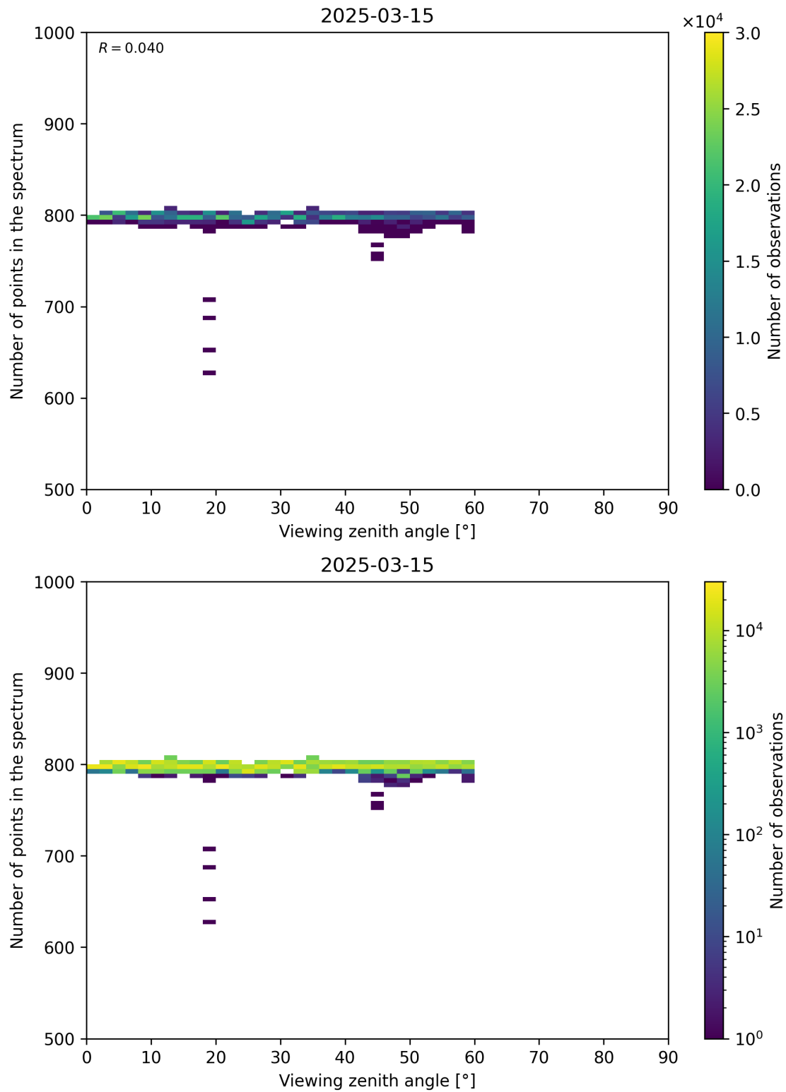
Figure 114: Scatter density plot of “Viewing zenith angle” against “Number of points in the spectrum” for 2025-03-14 to 2025-03-16.
