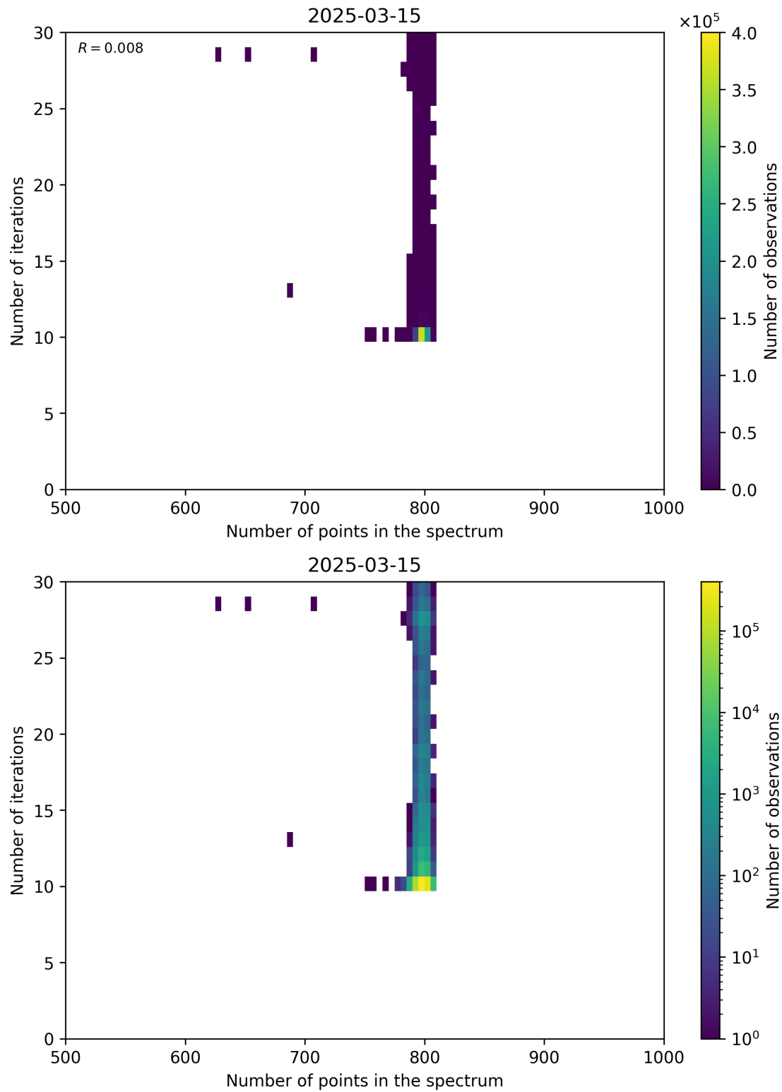
Figure 92: Scatter density plot of “Number of points in the spectrum” against “Number of iterations” for 2025-03-14 to 2025-03-16.
