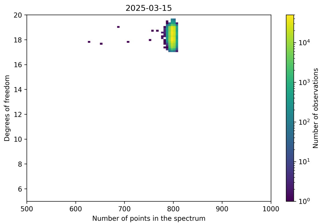
Figure 90: Scatter density plot of “Number of points in the spectrum” against “Degrees of freedom” for 2025-03-14 to 2025-03-16.
