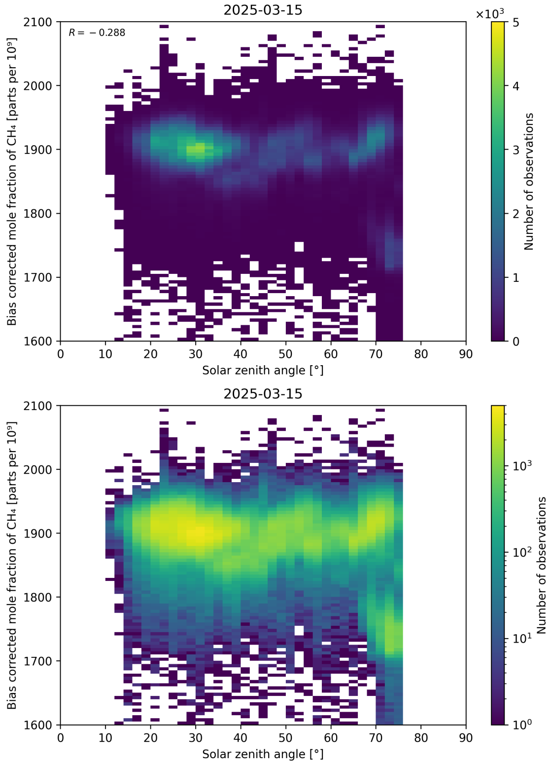
Figure 100: Scatter density plot of “Solar zenith angle” against “Bias corrected mole fraction of CH 4 ” for 2025-03-14 to 2025-03-16.
