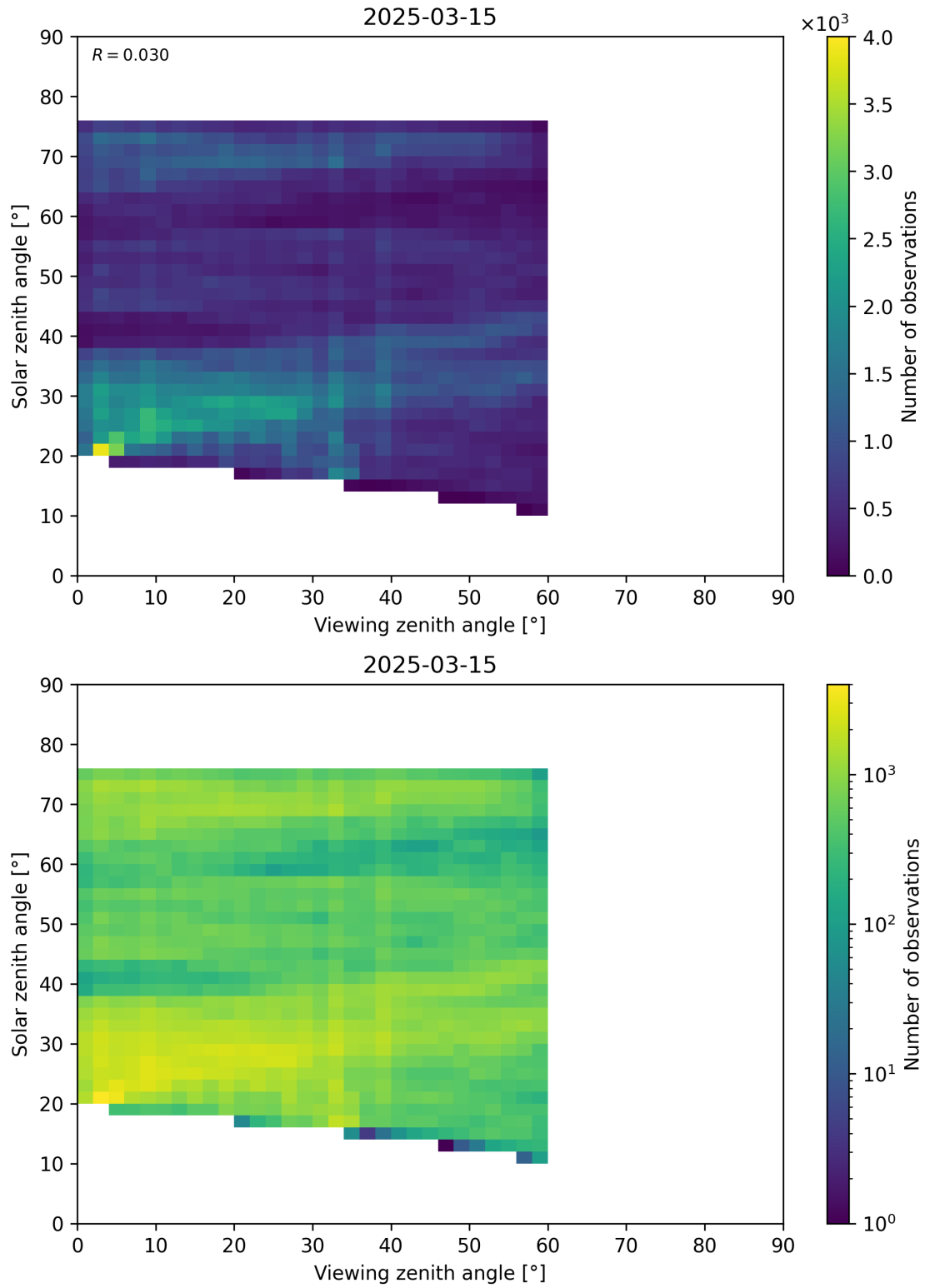
Figure 115: Scatter density plot of “Viewing zenith angle” against “Solar zenith angle” for 2025-03-14 to 2025-03-16.
