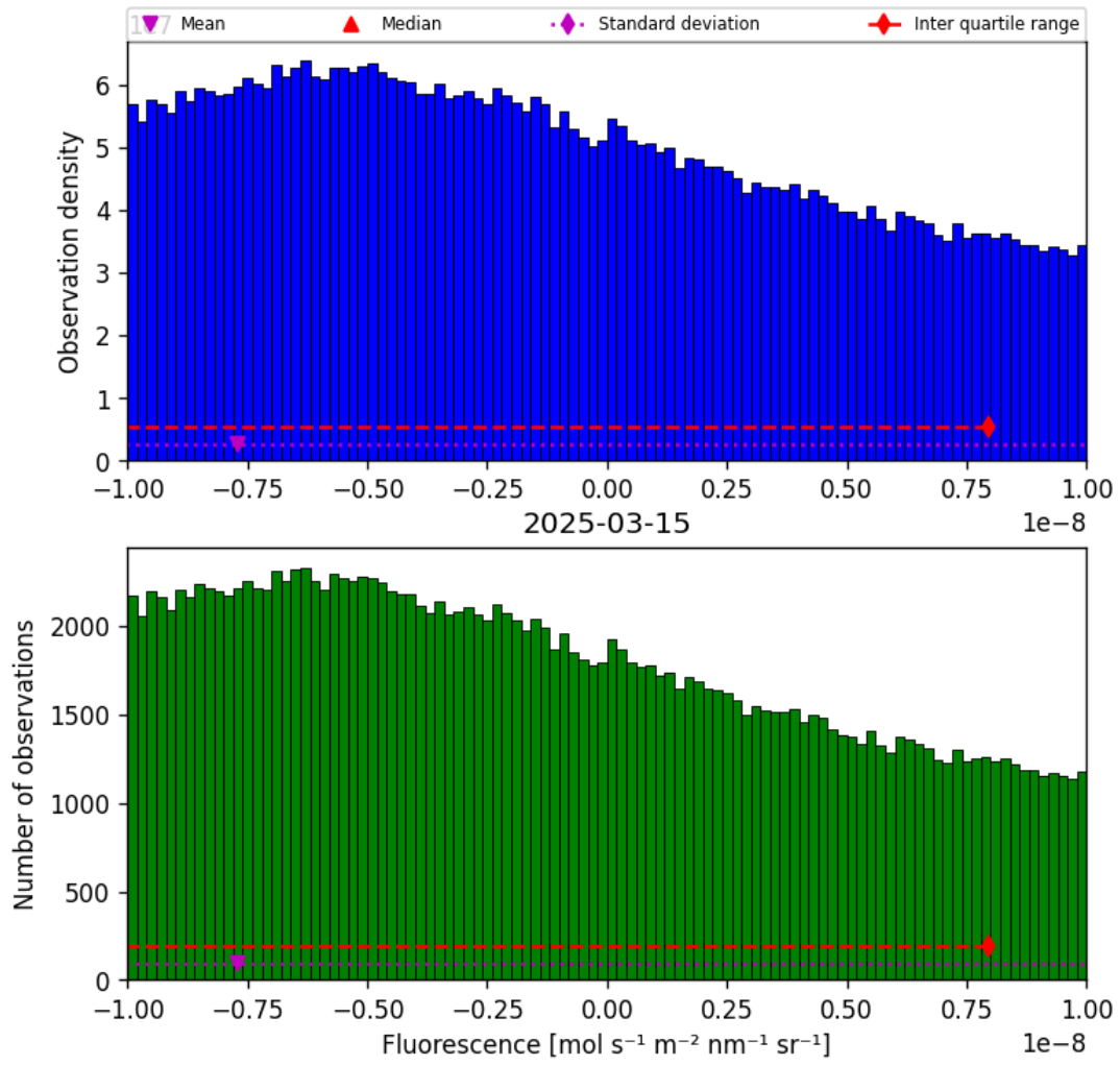
Figure 32: Histogram of “Fluorescence” for 2025-03-14 to 2025-03-16
