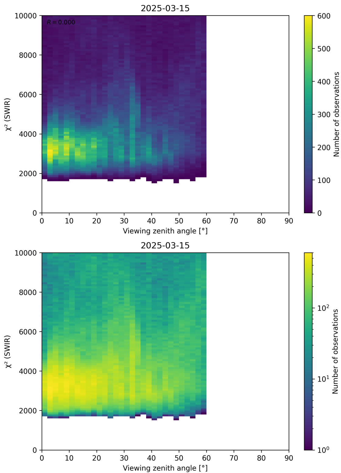
Figure 106: Scatter density plot of “Viewing zenith angle” against “ \chi^2 (SWIR)” for 2025-03-14 to 2025-03-16.
