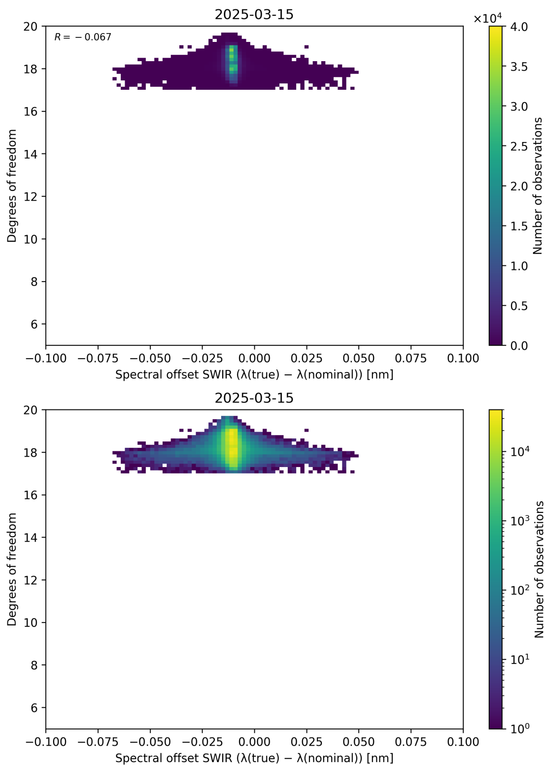
Figure 119: Scatter density plot of “Spectral offset SWIR ( \lambda_{\text{true}} - \lambda_{\text{nominal}} )” against “Degrees of freedom” for 2025-03-14 to 2025-03-16.
