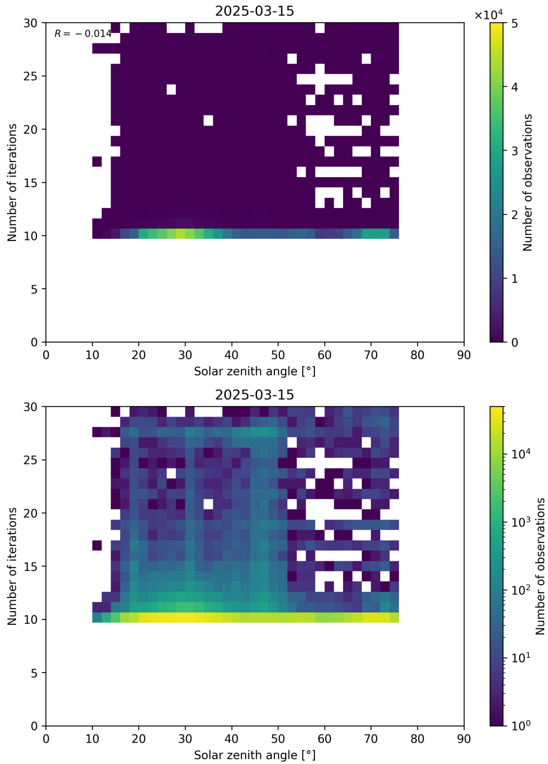
Figure 102: Scatter density plot of “Solar zenith angle” against “Number of iterations” for 2025-03-14 to 2025-03-16.
