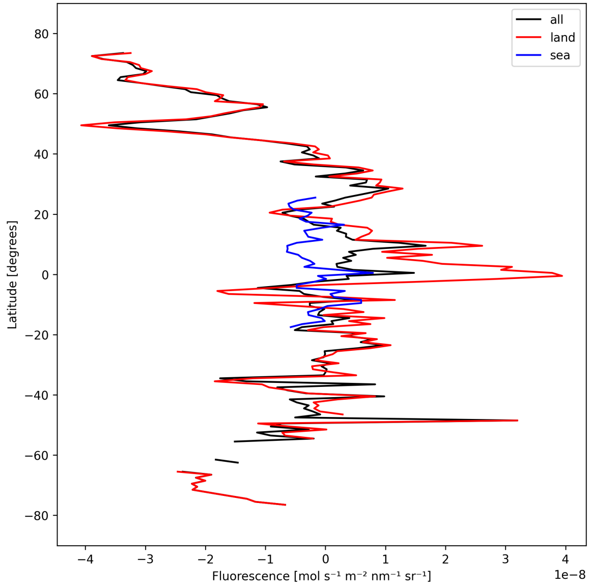
Figure 21: Zonal average of “Fluorescence” for 2025-03-14 to 2025-03-16.
