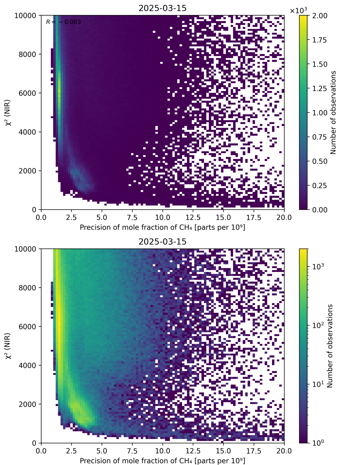
Figure 78: Scatter density plot of “Precision of mole fraction of CH 4 ” against “ \chi^2 (NIR)” for 2025-03-14 to 2025-03-16.
