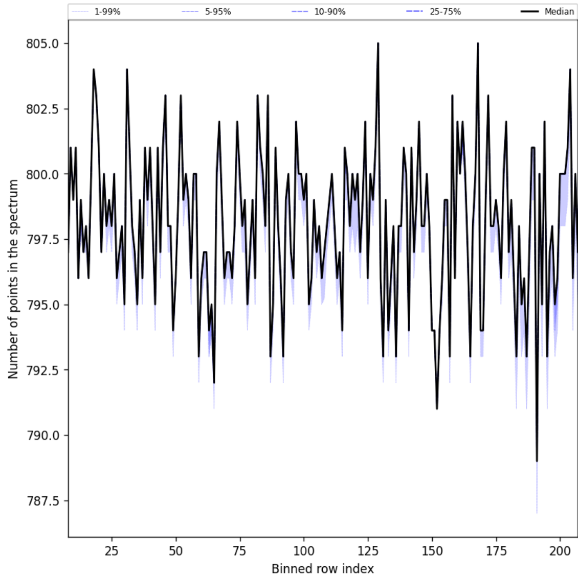
Figure 37: Along track statistics of “Number of points in the spectrum” for 2025-03-14 to 2025-03-16
