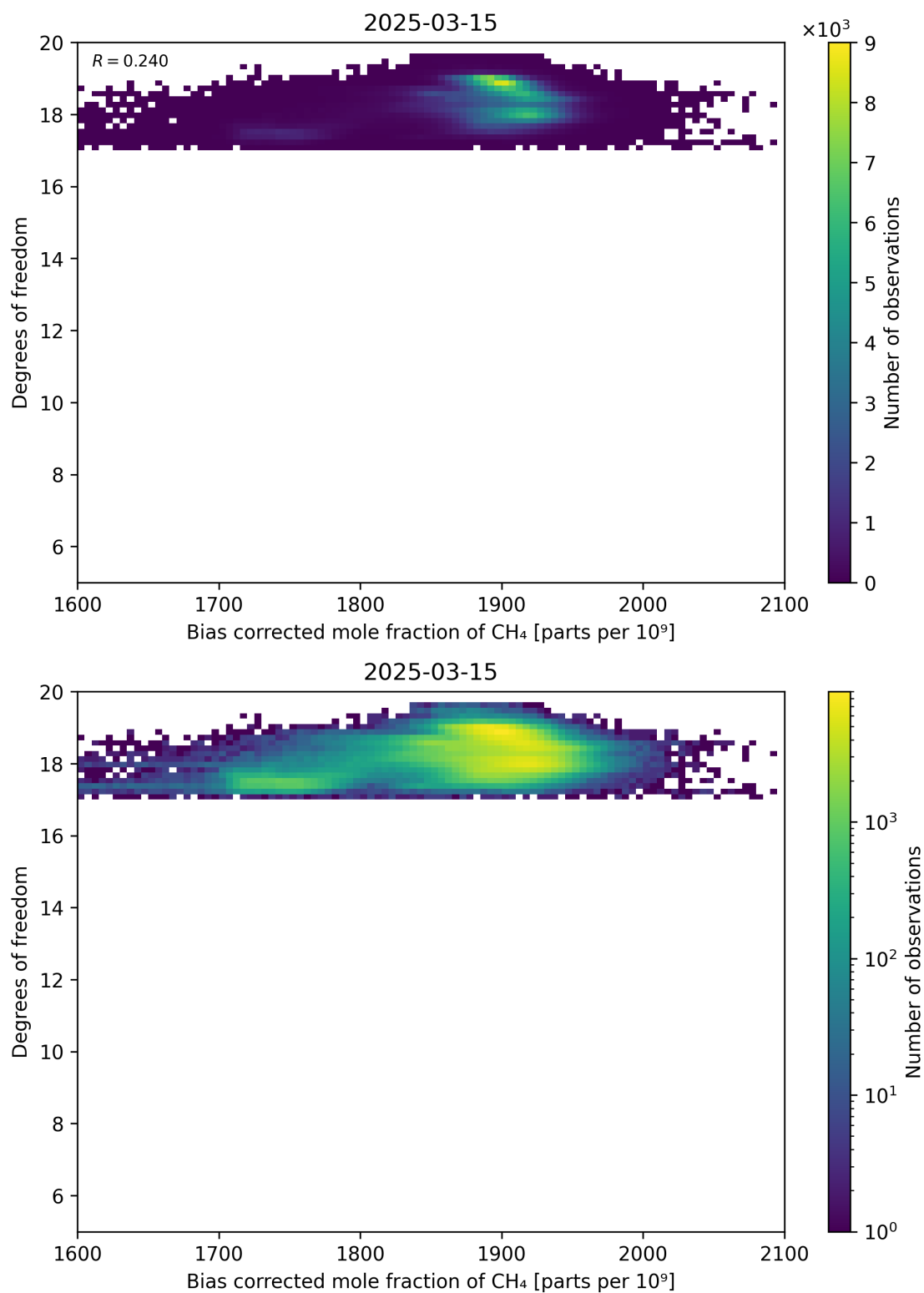
Figure 65: Scatter density plot of “Bias corrected mole fraction of CH 4 ” against “Degrees of freedom” for 2025-03-14 to 2025-03-16.
