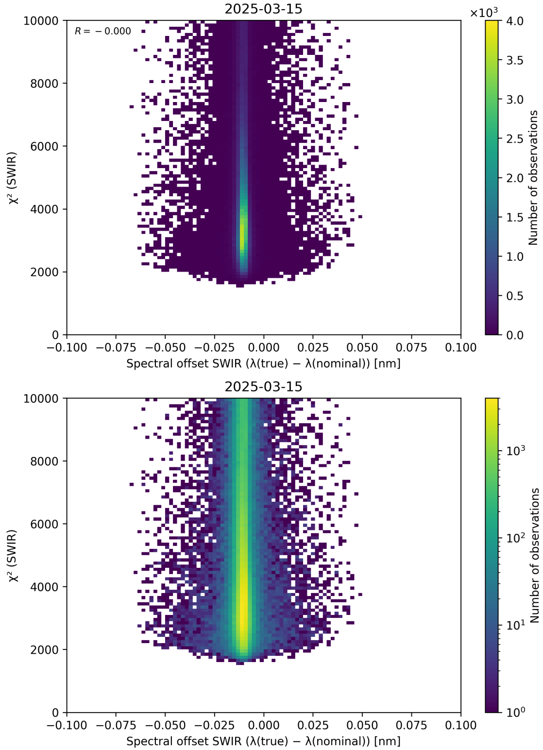
Figure 118: Scatter density plot of “Spectral offset SWIR ( \lambda_{\text{true}} - \lambda_{\text{nominal}} )” against “ \chi^2 (SWIR)” for 2025-03-14 to 2025-03-16.
