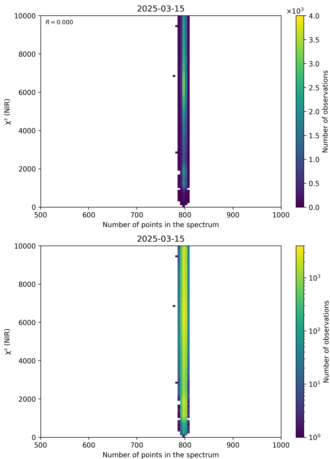
Figure 88: Scatter density plot of “Number of points in the spectrum” against “ \chi^2 (NIR)” for 2025-03-14 to 2025-03-16.
