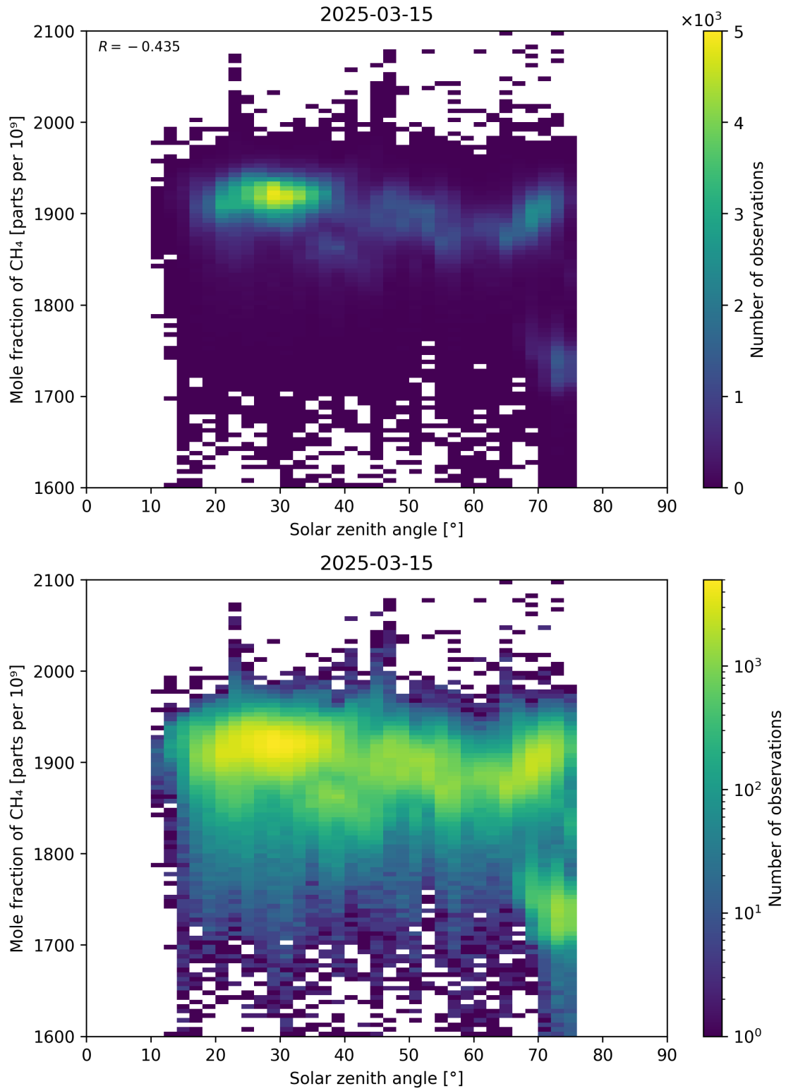
Figure 99: Scatter density plot of “Solar zenith angle” against “Mole fraction of CH 4 ” for 2025-03-14 to 2025-03-16.
