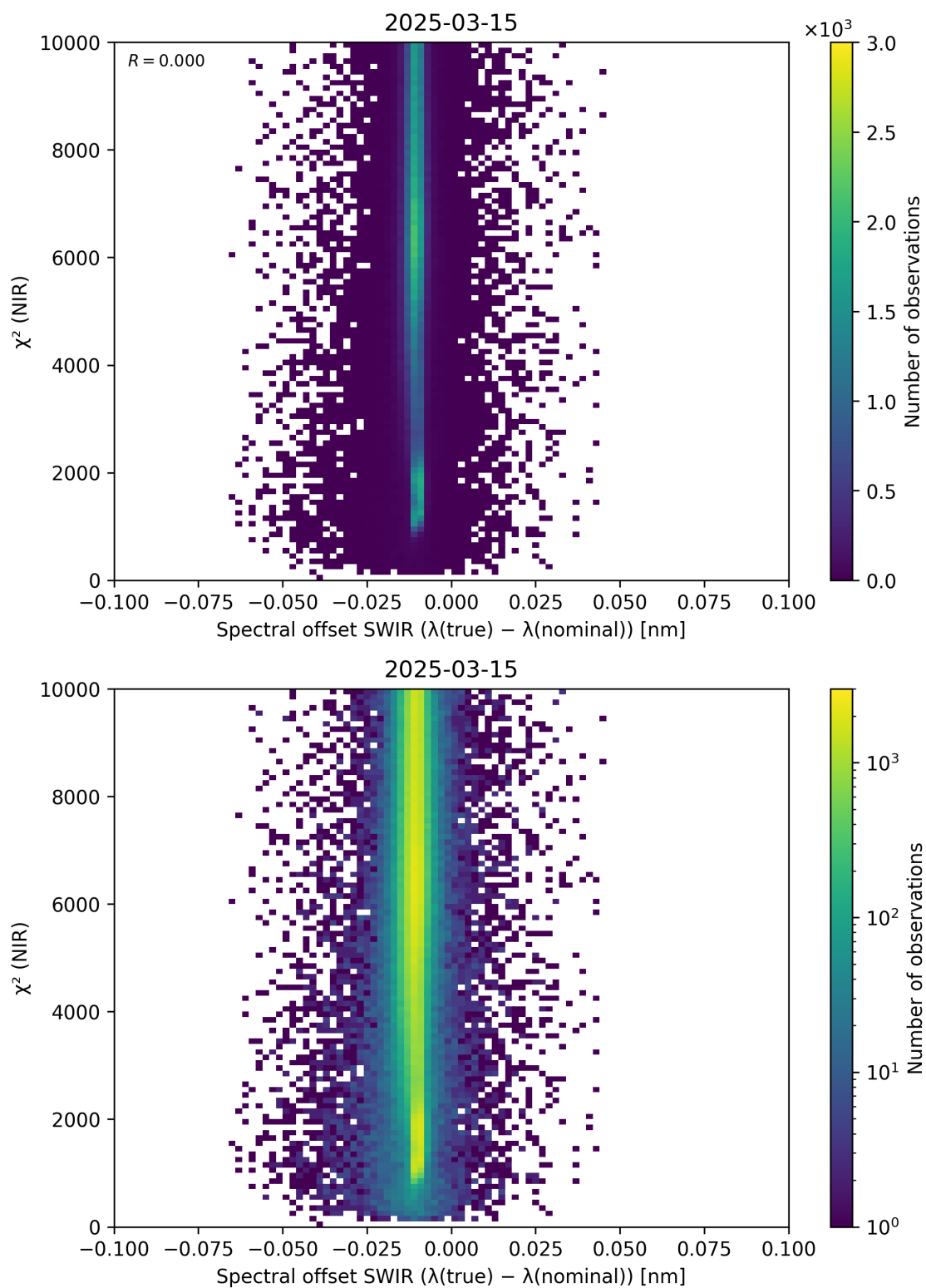
Figure 117: Scatter density plot of “Spectral offset SWIR ( \lambda_{\text{true}} - \lambda_{\text{nominal}} )” against “ \chi^2 (NIR)” for 2025-03-14 to 2025-03-16.
