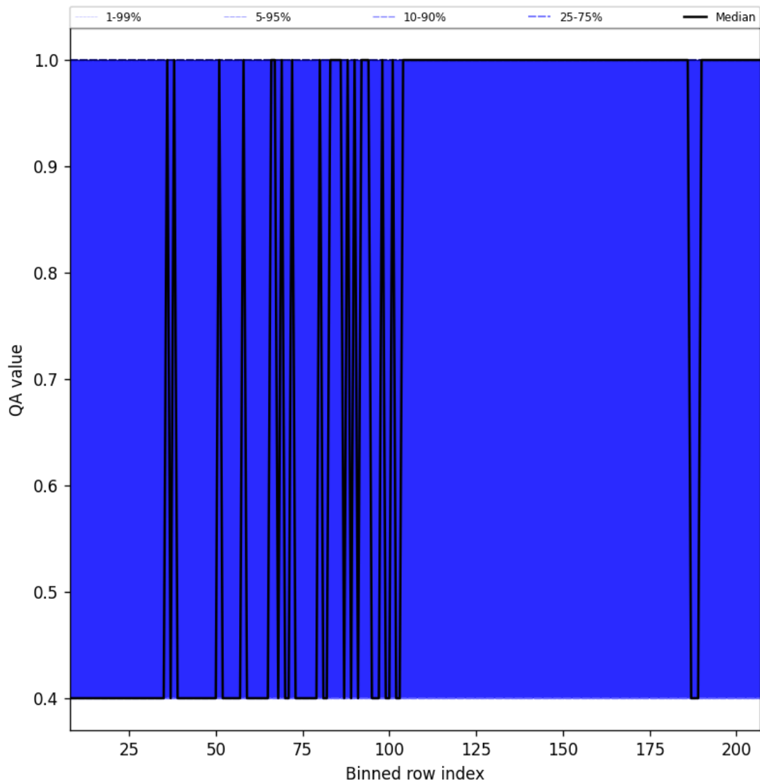
Figure 33: Along track statistics of “QA value” for 2025-03-14 to 2025-03-16
