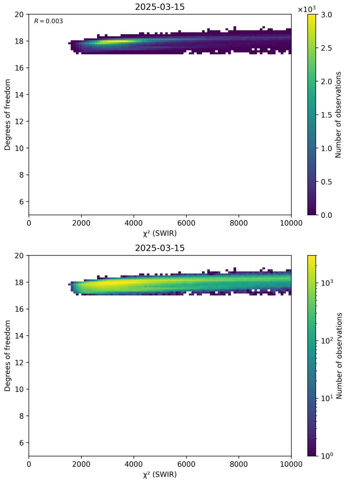
Figure 48: Scatter density plot of “ \chi^2 (SWIR)” against “Degrees of freedom” for 2025-03-14 to 2025-03-16.
