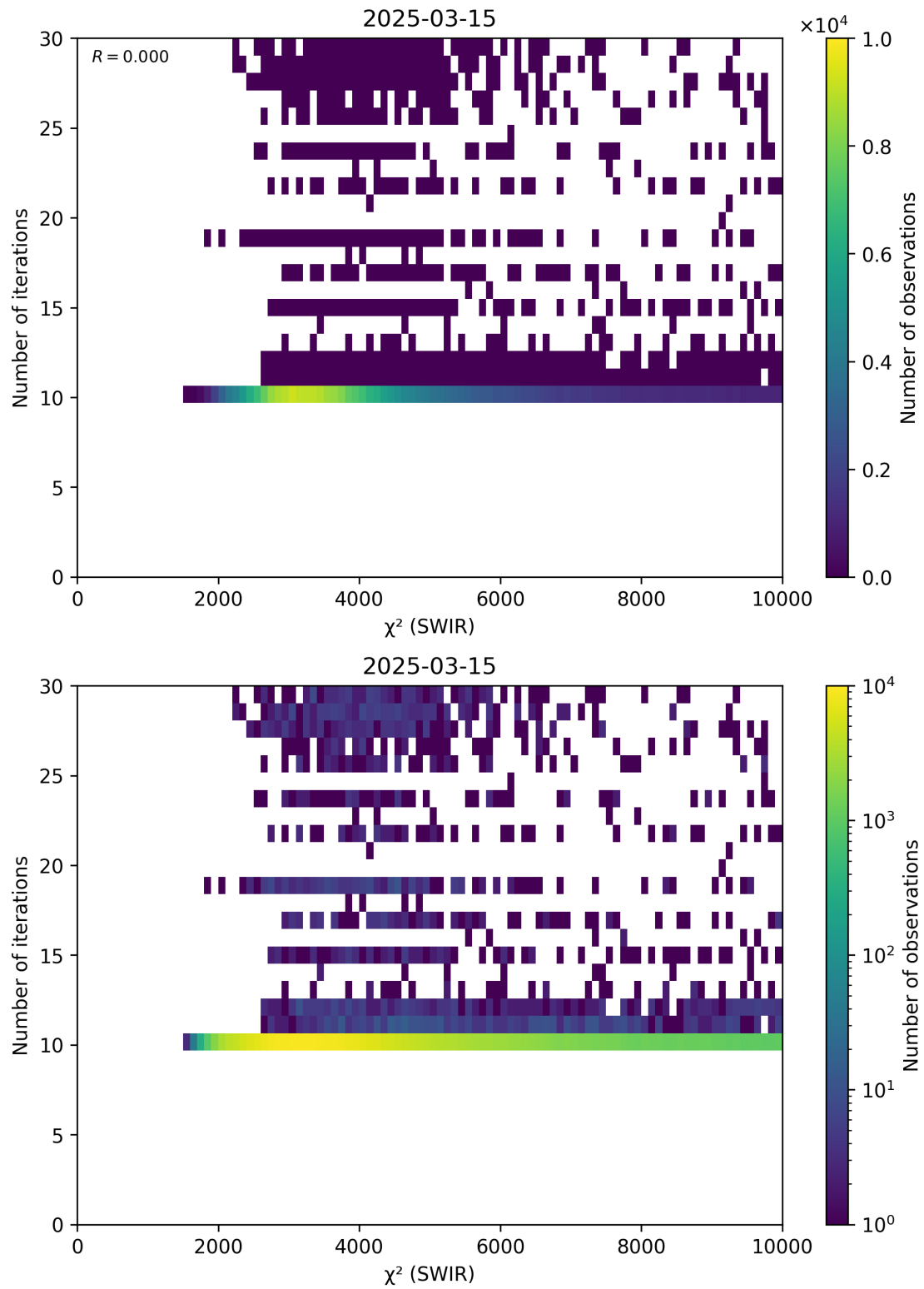
Figure 50: Scatter density plot of “ \chi^2 (SWIR)” against “Number of iterations” for 2025-03-14 to 2025-03-16.
