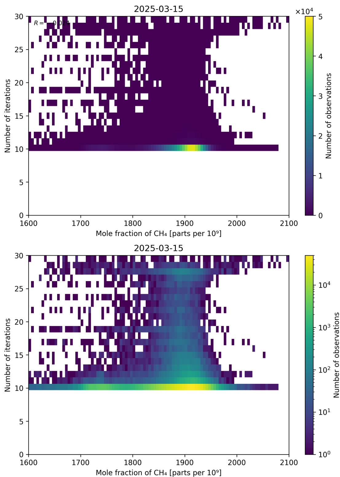
Figure 76: Scatter density plot of “Mole fraction of CH 4 ” against “Number of iterations” for 2025-03-14 to 2025-03-16.
