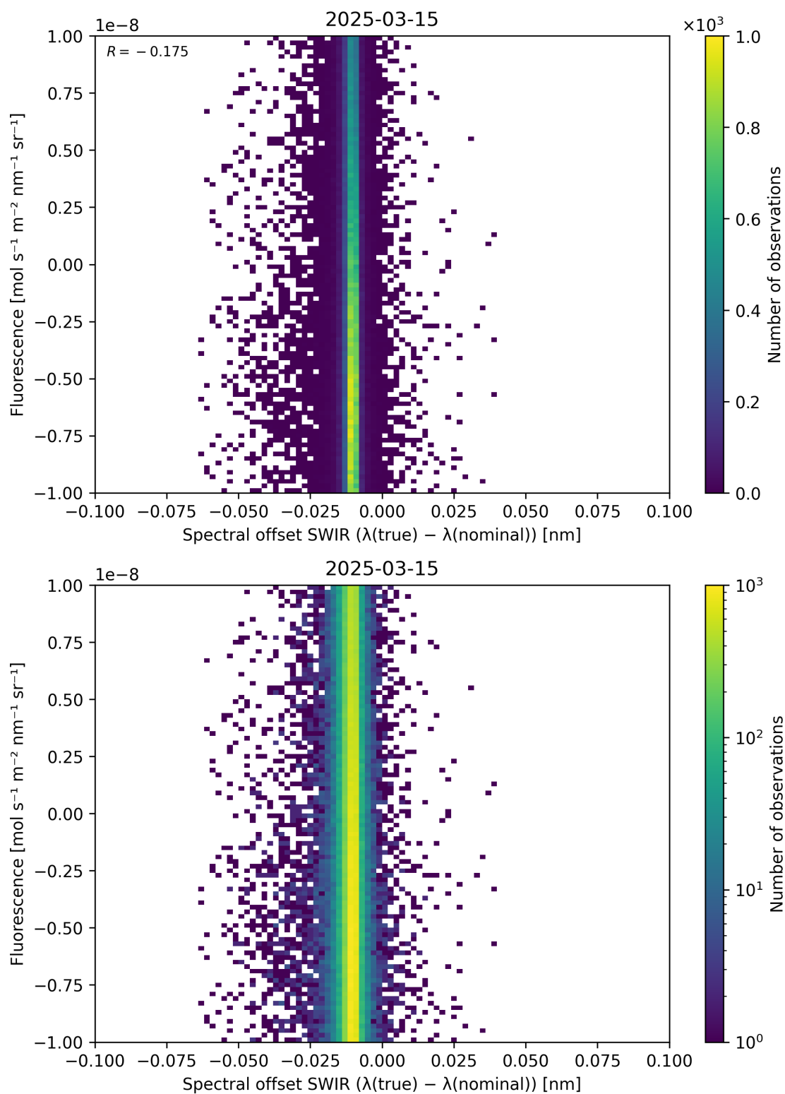
Figure 120: Scatter density plot of “Spectral offset SWIR ( \lambda_{\text{true}} - \lambda_{\text{nominal}} )” against “Fluorescence” for 2025-03-14 to 2025-03-16.
