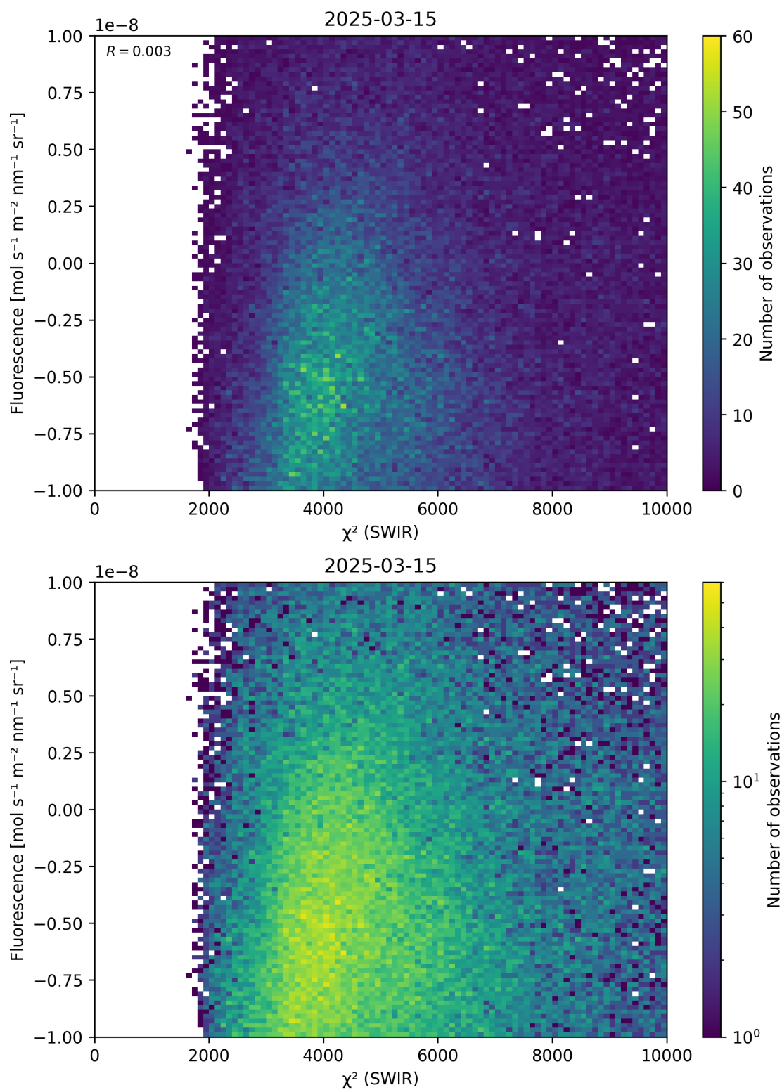
Figure 49: Scatter density plot of “ \chi^2 (SWIR)” against “Fluorescence” for 2025-03-14 to 2025-03-16.
