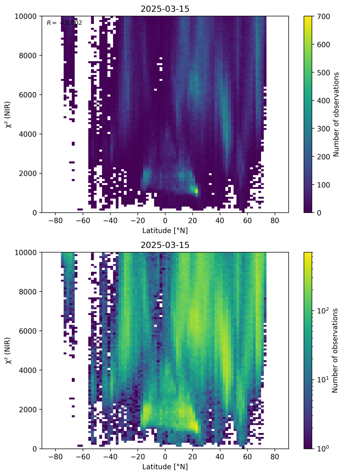
Figure 53: Scatter density plot of “Latitude” against “ \chi^2 (NIR)” for 2025-03-14 to 2025-03-16.
