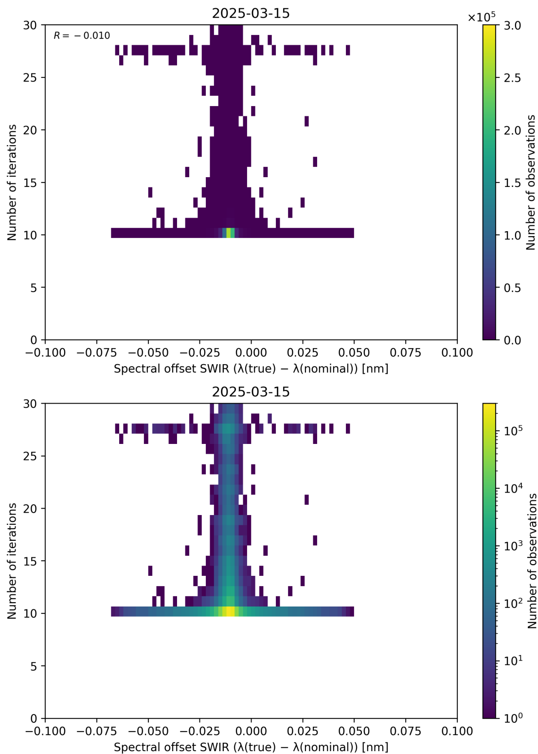
Figure 121: Scatter density plot of “Spectral offset SWIR ( \lambda_{\text{true}} - \lambda_{\text{nominal}} )” against “Number of iterations” for 2025-03-14 to 2025-03-16.
