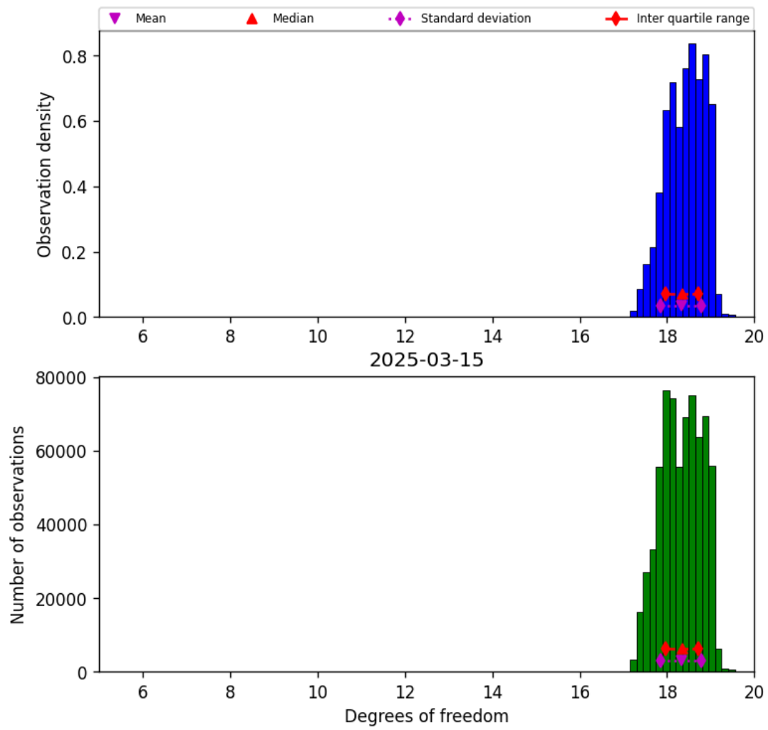
Figure 30: Histogram of “Degrees of freedom” for 2025-03-14 to 2025-03-16
