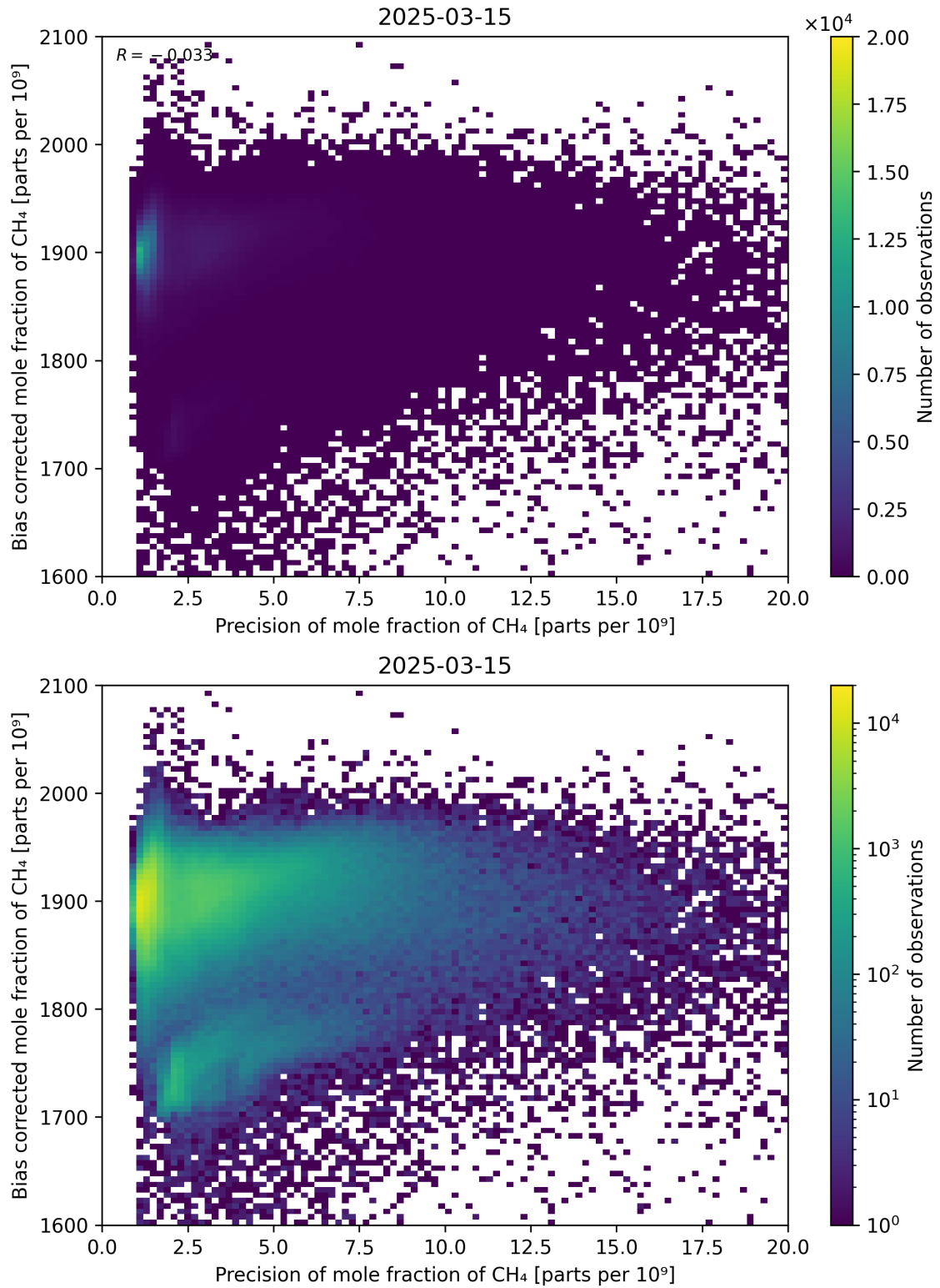
Figure 82: Scatter density plot of “Precision of mole fraction of CH 4 ” against “Bias corrected mole fraction of CH 4 ” for 2025-03-14 to 2025-03-16.
