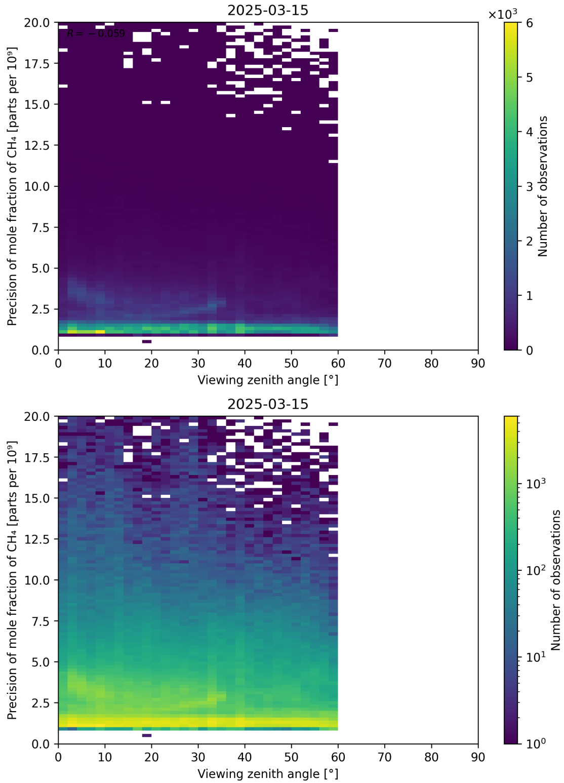
Figure 112: Scatter density plot of “Viewing zenith angle” against “Precision of mole fraction of CH 4 ” for 2025-03-14 to 2025-03-16.
