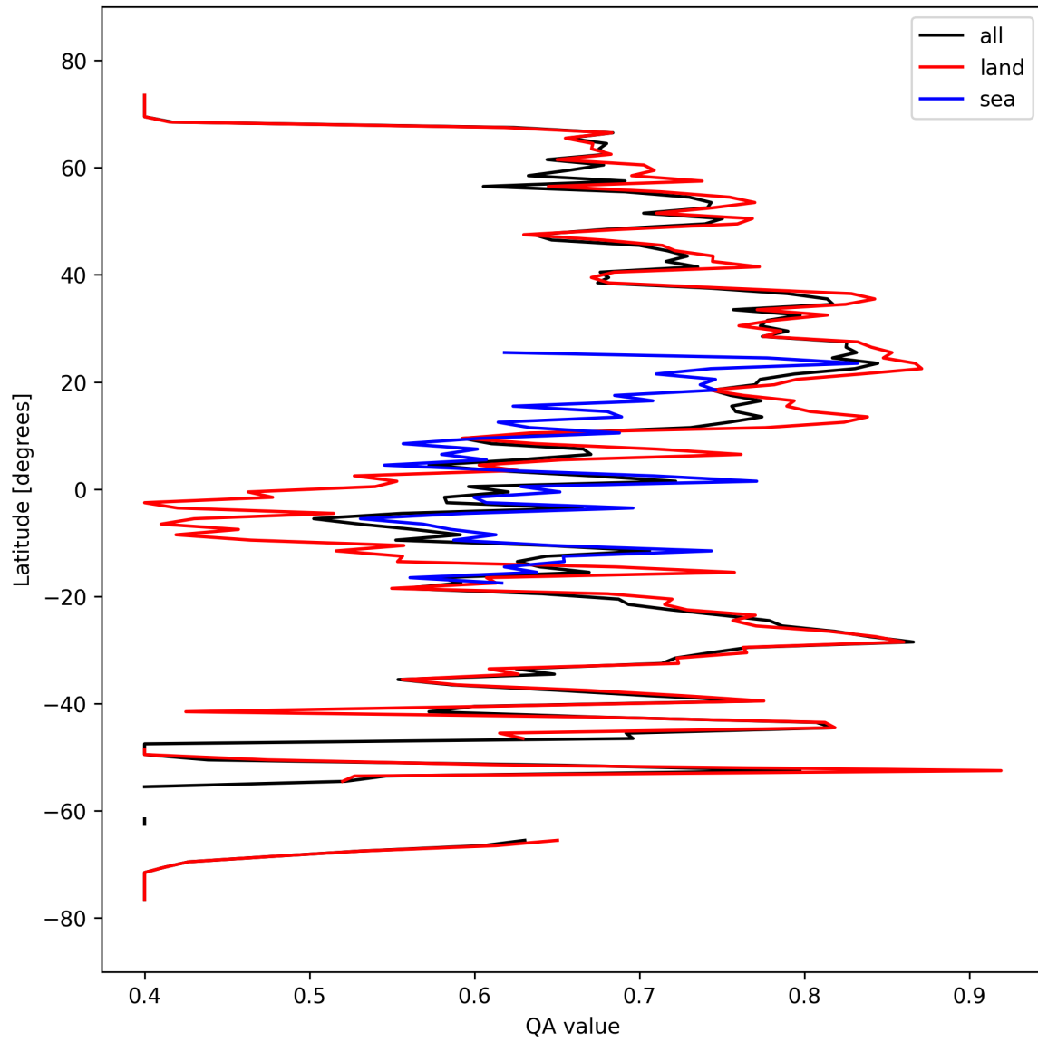
Figure 11: Zonal average of “QA value” for 2025-03-14 to 2025-03-16.
