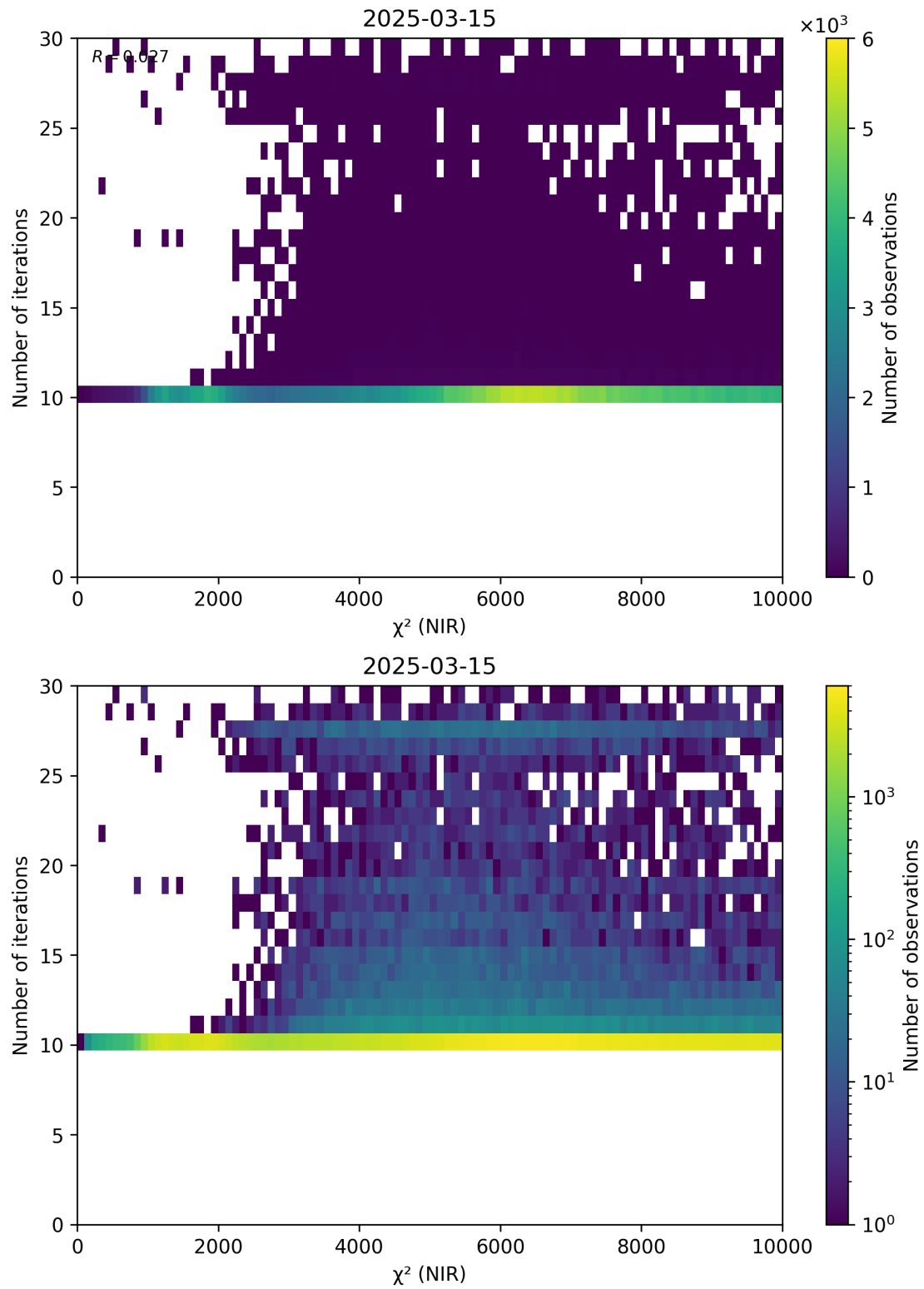
Figure 46: Scatter density plot of “ \chi^2 (NIR)” against “Number of iterations” for 2025-03-14 to 2025-03-16.
