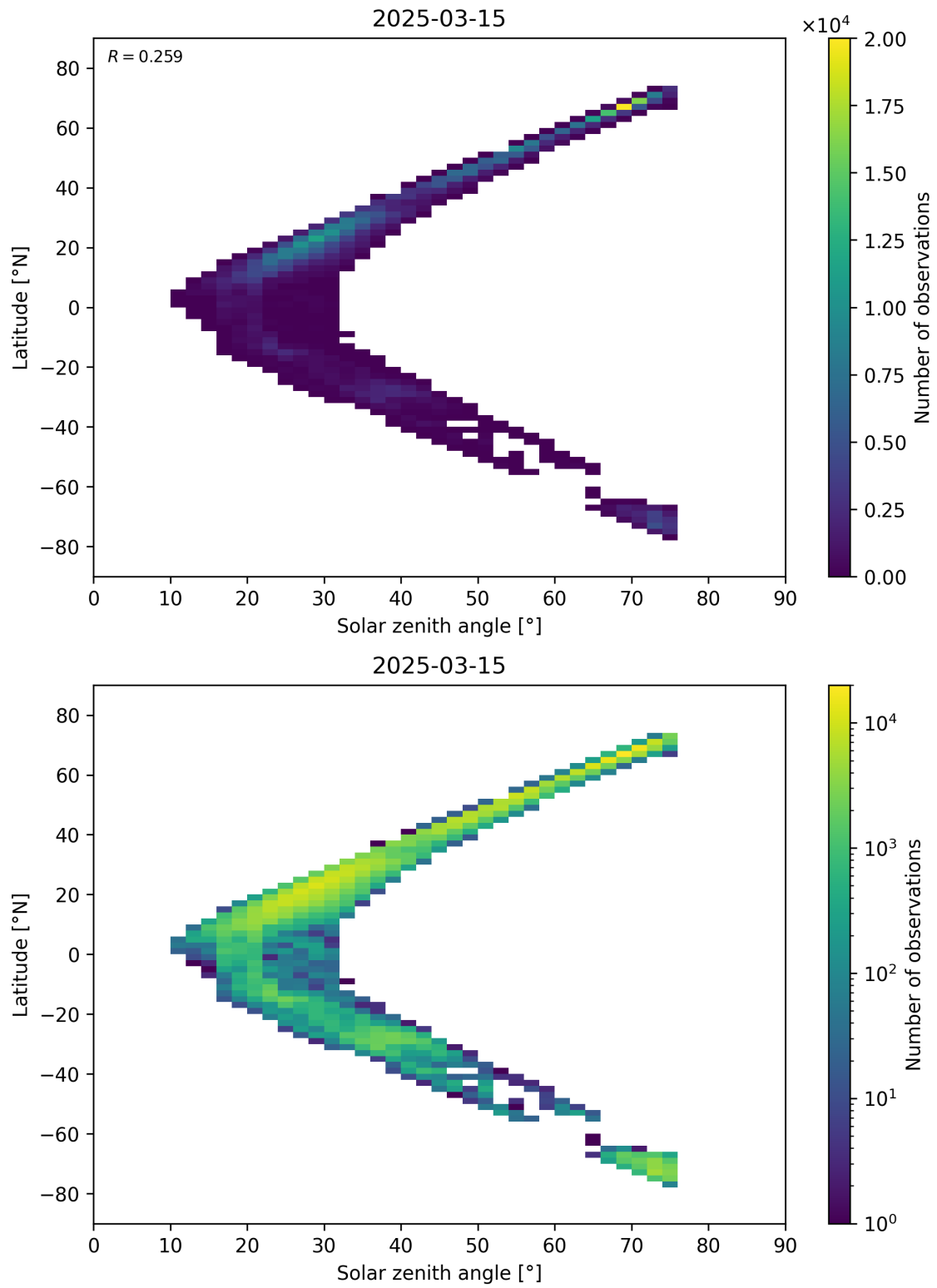
Figure 98: Scatter density plot of “Solar zenith angle” against “Latitude” for 2025-03-14 to 2025-03-16.
