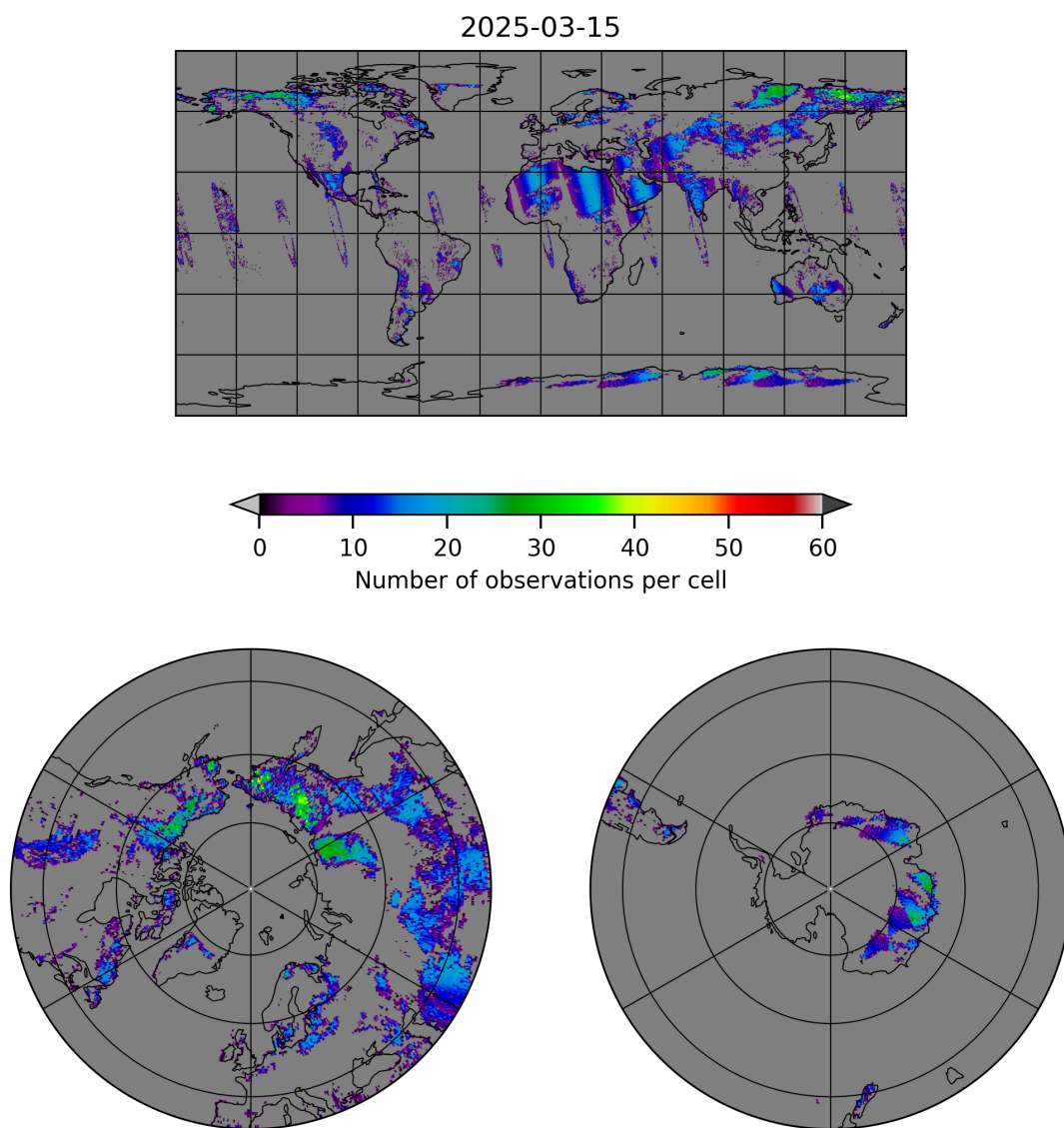
Figure 10: Map of the number of observations for 2025-03-14 to 2025-03-16
