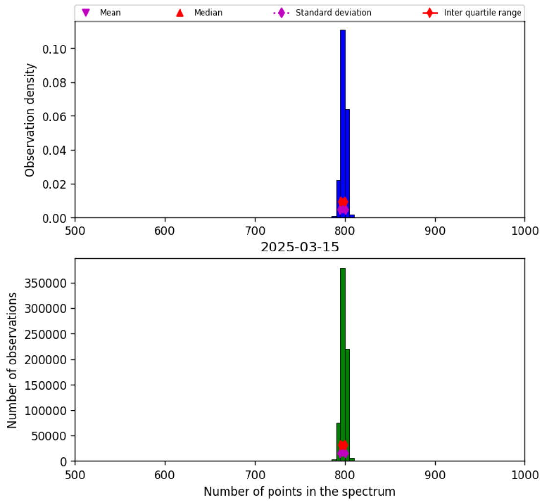
Figure 26: Histogram of “Number of points in the spectrum” for 2025-03-14 to 2025-03-16
