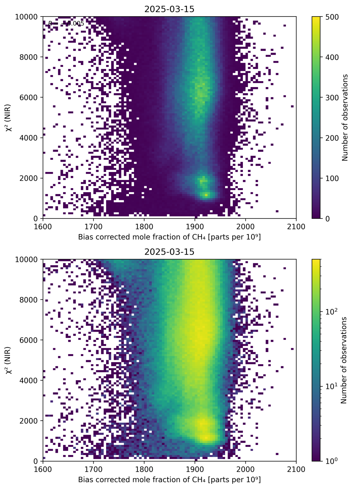
Figure 63: Scatter density plot of “Bias corrected mole fraction of \text{CH}_4 ” against “ \chi^2 (NIR)” for 2025-03-14 to 2025-03-16.
