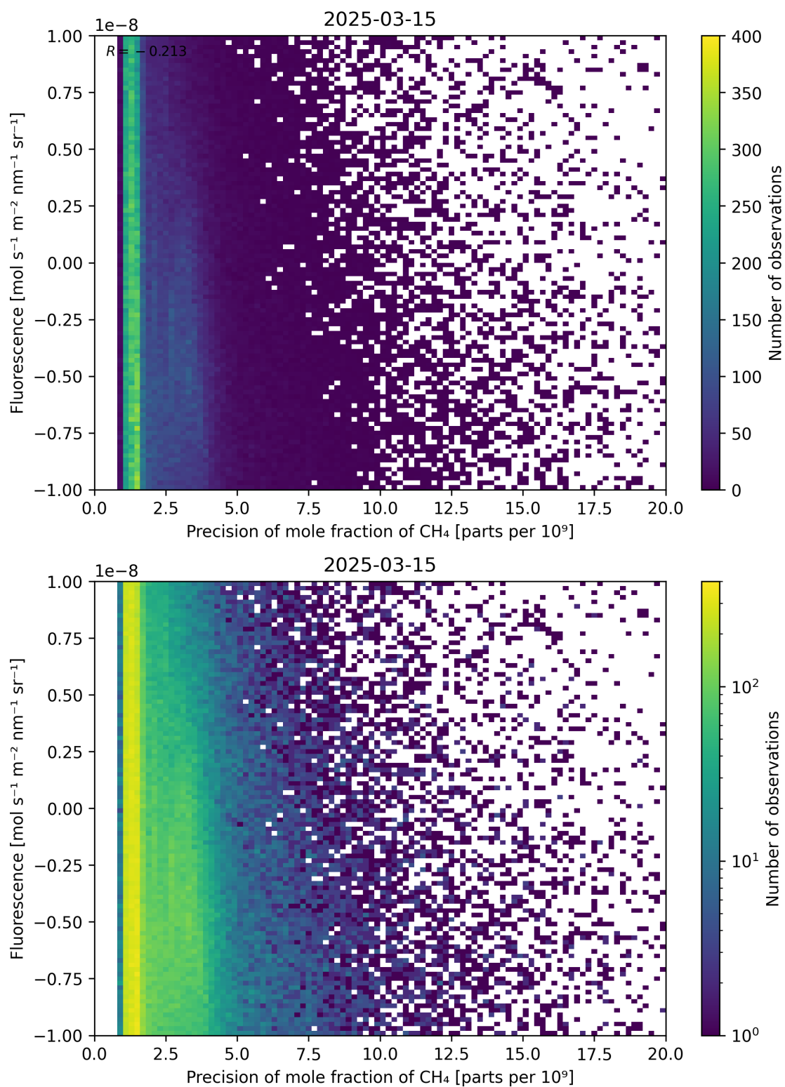
Figure 81: Scatter density plot of “Precision of mole fraction of CH 4 ” against “Fluorescence” for 2025-03-14 to 2025-03-16.
