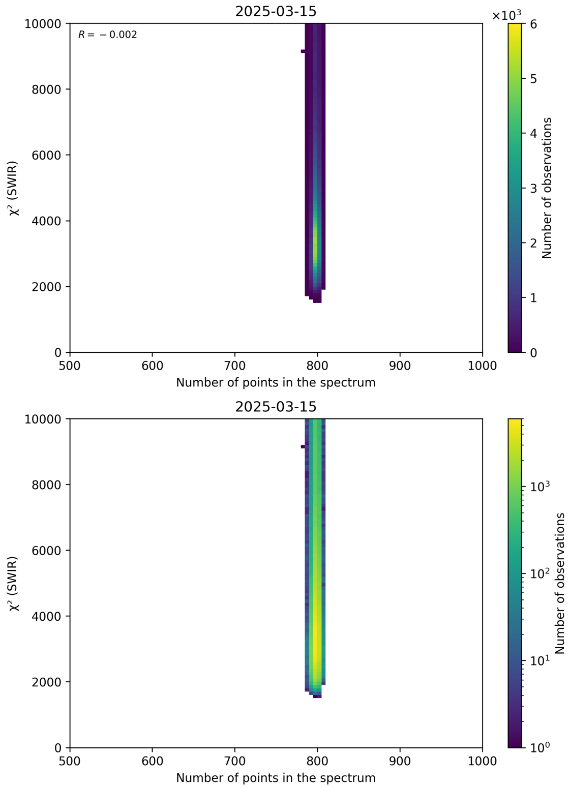
Figure 89: Scatter density plot of “Number of points in the spectrum” against “ \chi^2 (SWIR)” for 2025-03-14 to 2025-03-16.
