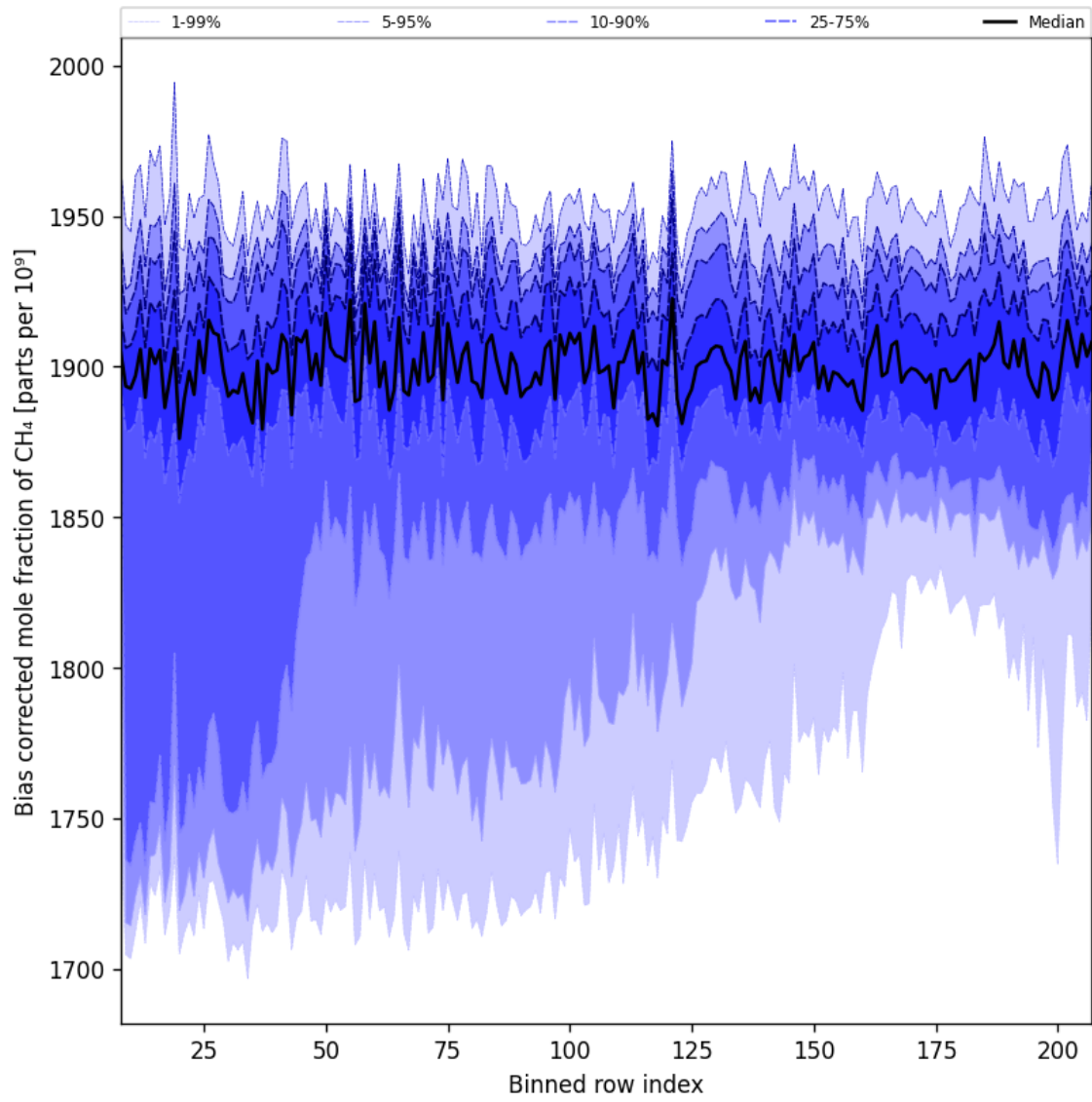
Figure 36: Along track statistics of “Bias corrected mole fraction of CH 4 ” for 2025-03-14 to 2025-03-16
