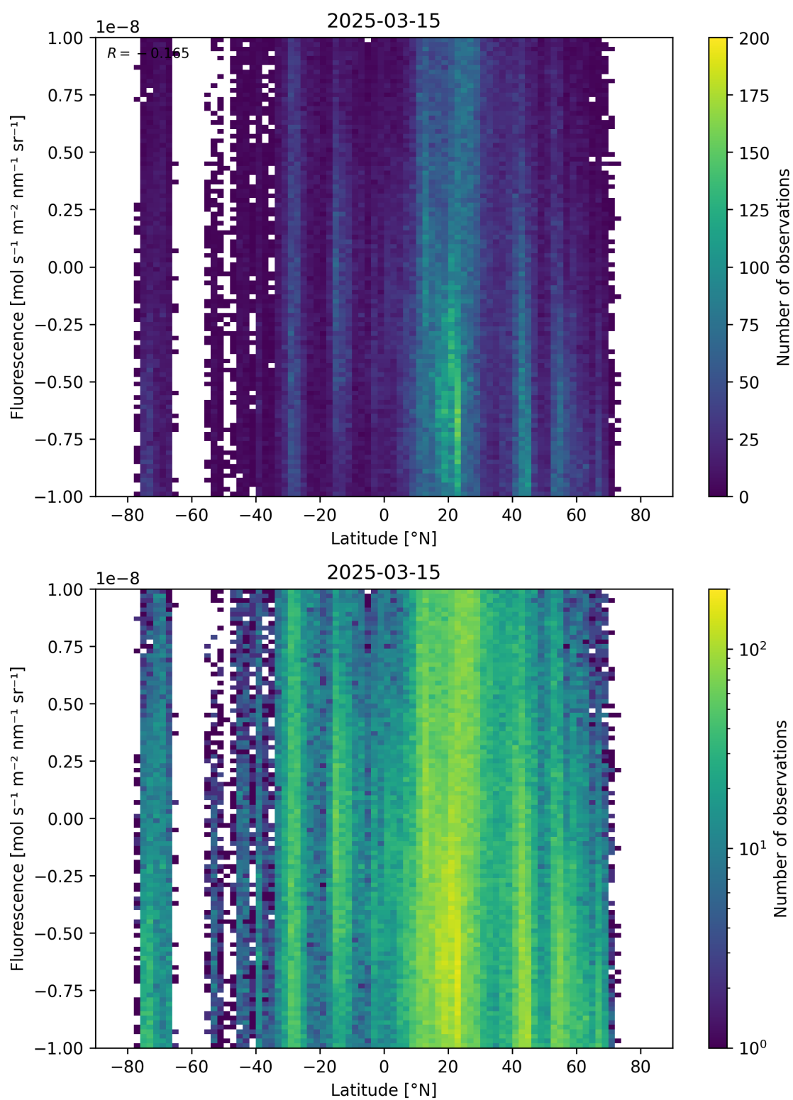
Figure 56: Scatter density plot of “Latitude” against “Fluorescence” for 2025-03-14 to 2025-03-16.
