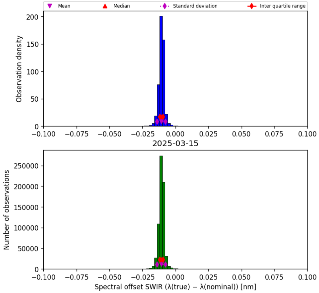
Figure 27: Histogram of “Spectral offset SWIR ( \lambda_{\text{true}} - \lambda_{\text{nominal}} )” for 2025-03-14 to 2025-03-16
