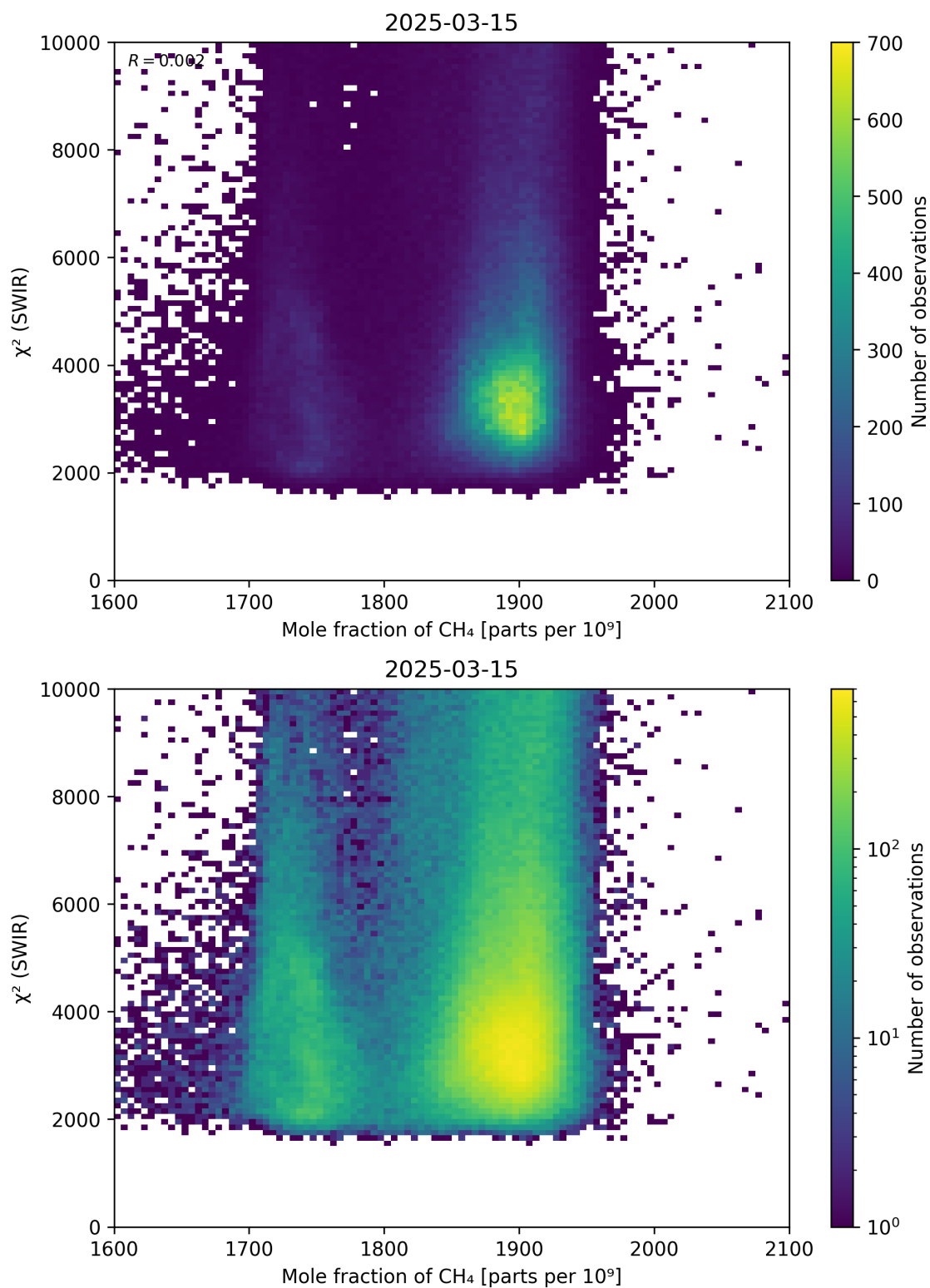
Figure 71: Scatter density plot of “Mole fraction of \text{CH}_4 ” against “ \chi^2 (SWIR)” for 2025-03-14 to 2025-03-16.
