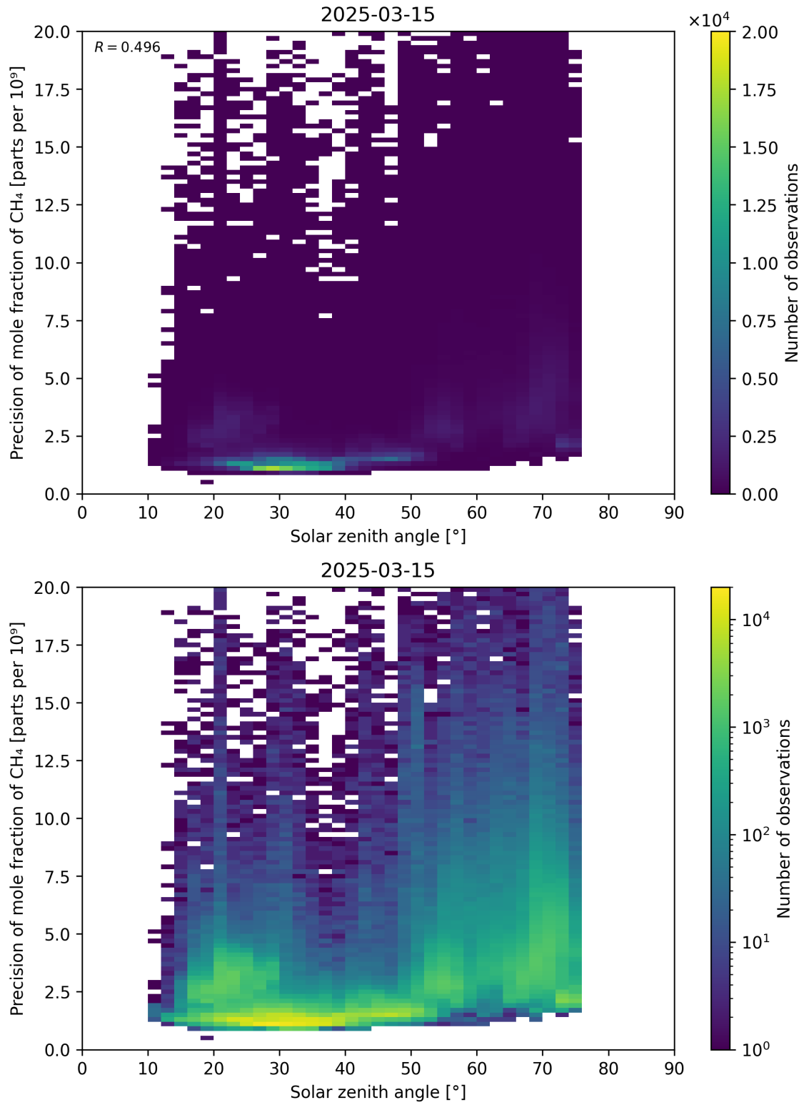
Figure 101: Scatter density plot of “Solar zenith angle” against “Precision of mole fraction of \text{CH}_4 ” for 2025-03-14 to 2025-03-16.
