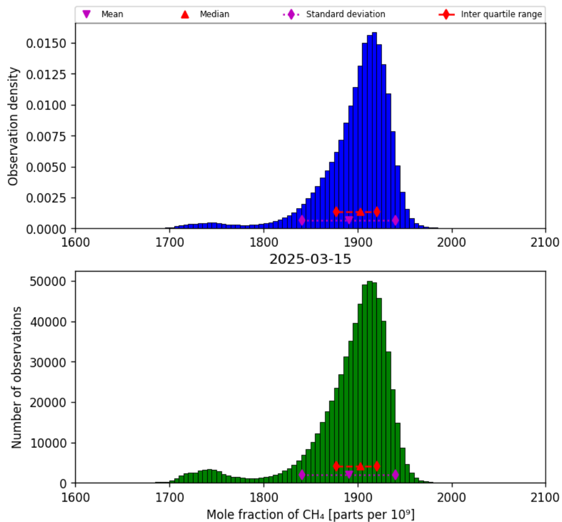
Figure 23: Histogram of "Mole fraction of CH 4 " for 2025-03-14 to 2025-03-16
