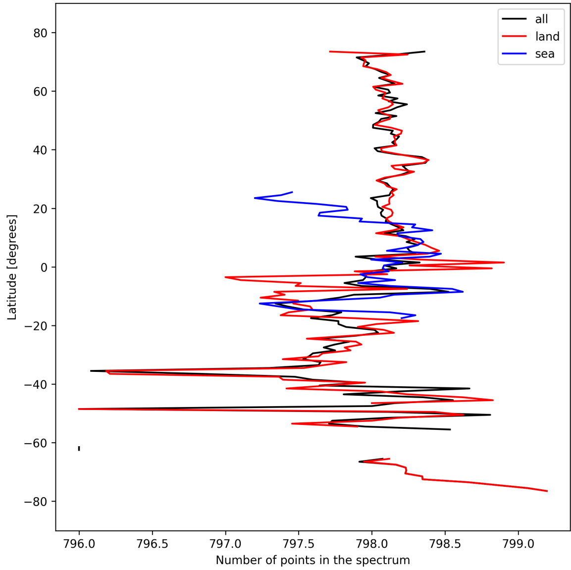
Figure 15: Zonal average of “Number of points in the spectrum” for 2025-03-14 to 2025-03-16.
