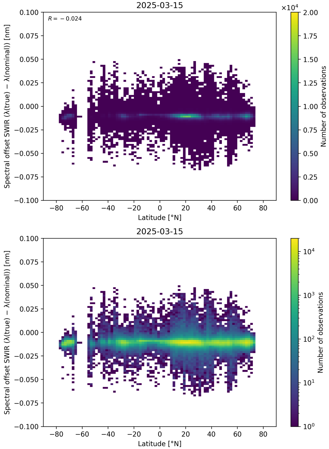
Figure 62: Scatter density plot of “Latitude” against “Spectral offset SWIR ( \lambda_{\text{true}} - \lambda_{\text{nominal}} )” for 2025-03-14 to 2025-03-16.
