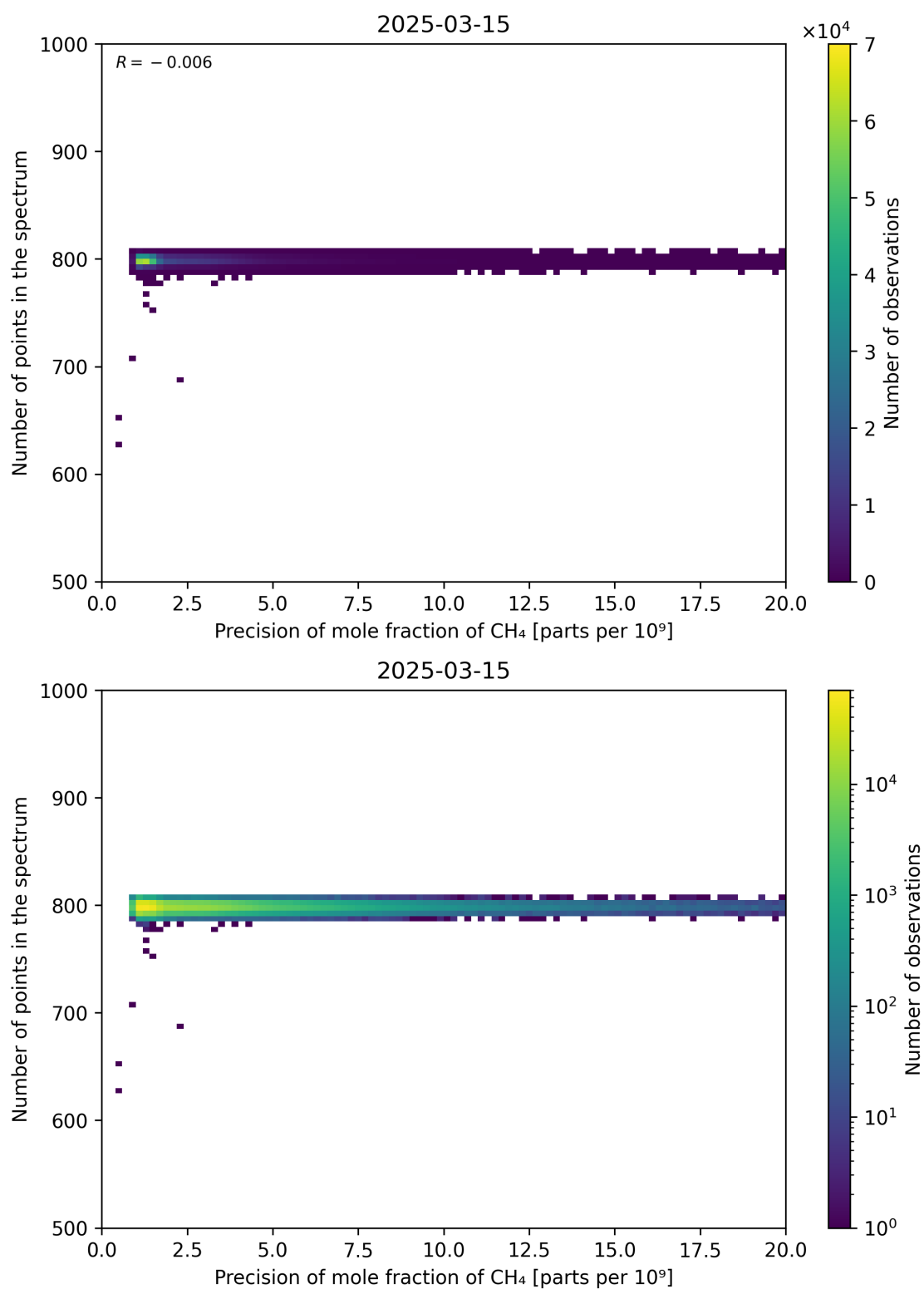
Figure 84: Scatter density plot of “Precision of mole fraction of CH 4 ” against “Number of points in the spectrum” for 2025-03-14 to 2025-03-16.
