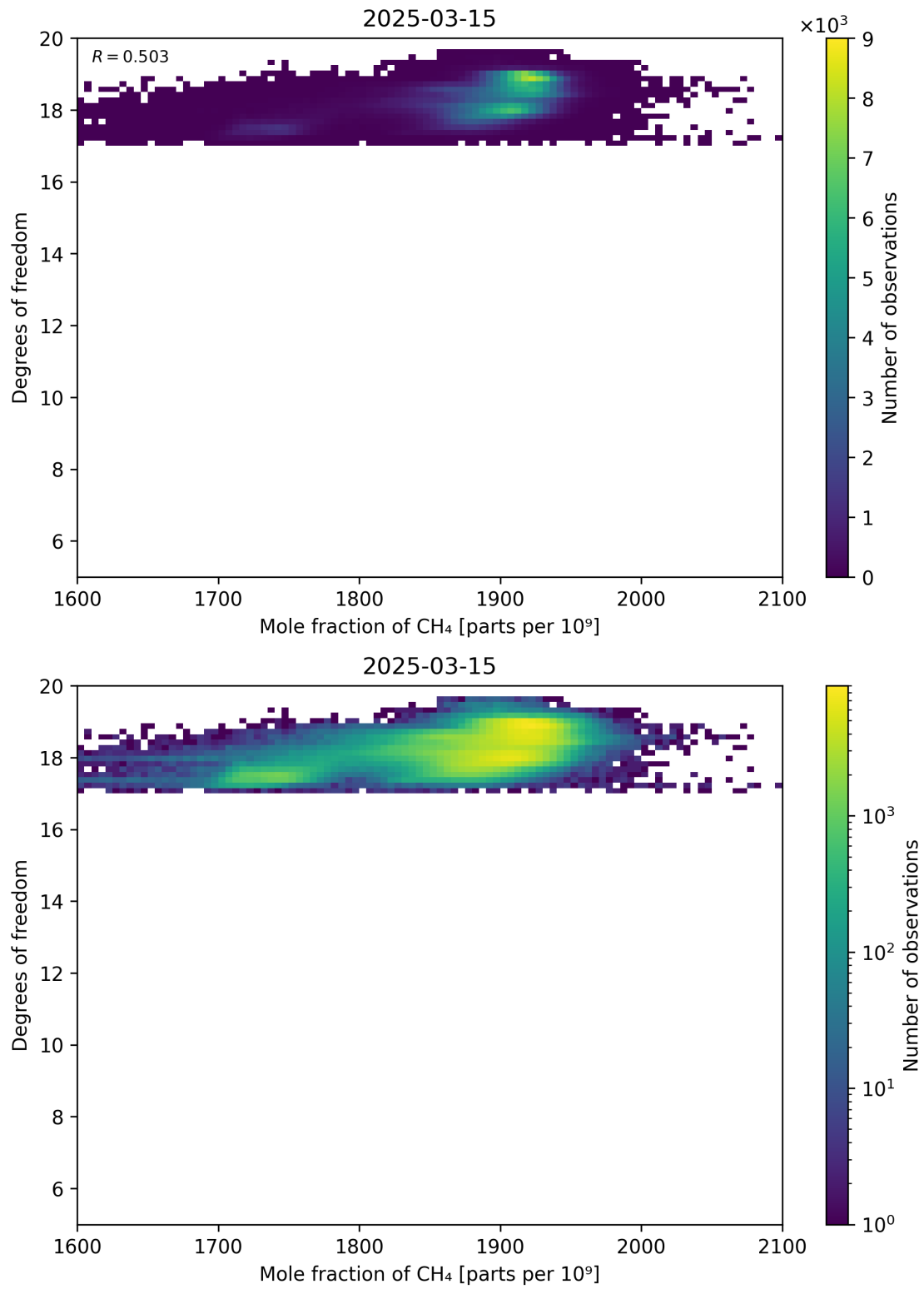
Figure 72: Scatter density plot of “Mole fraction of CH 4 ” against “Degrees of freedom” for 2025-03-14 to 2025-03-16.
