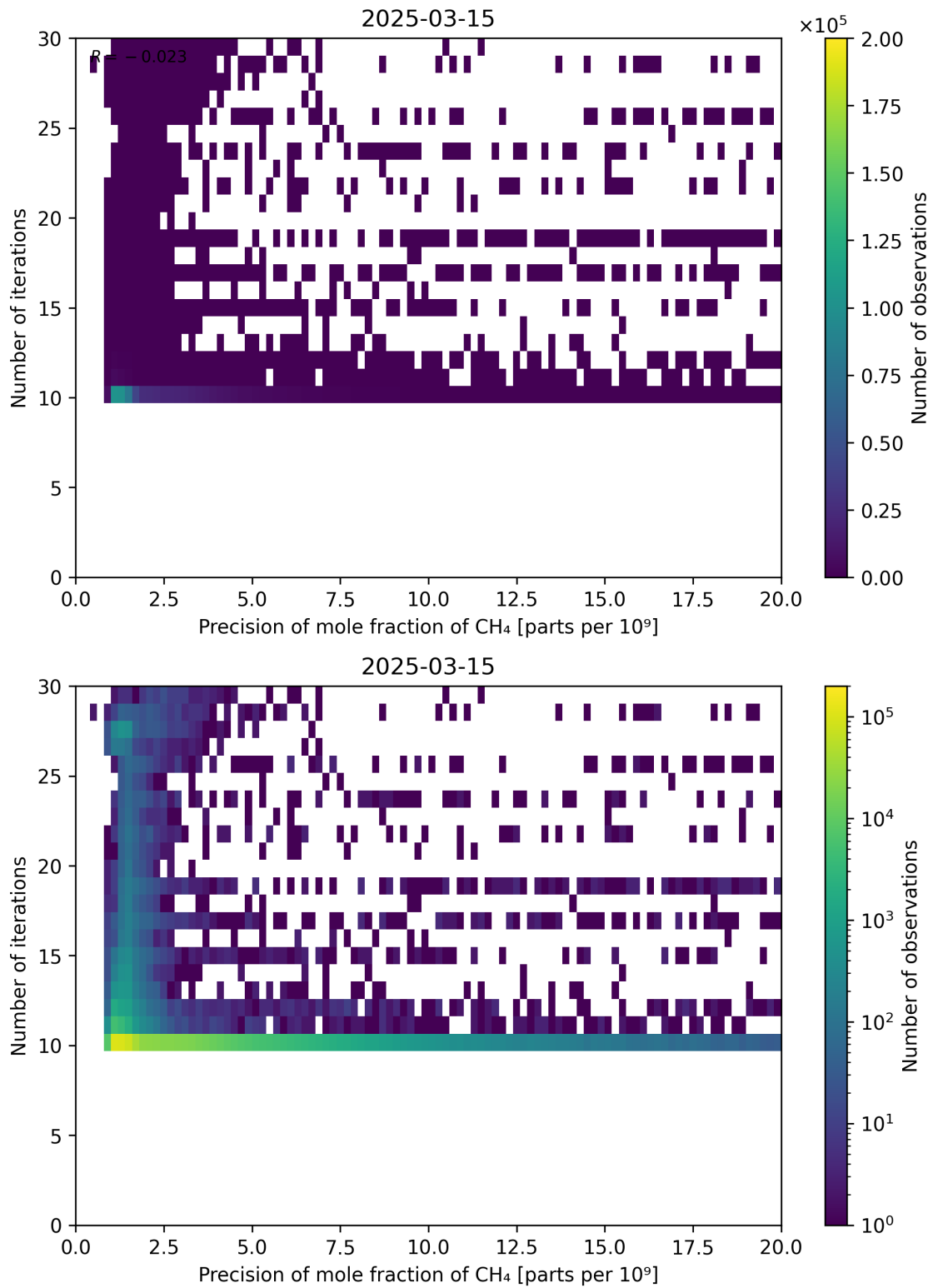
Figure 83: Scatter density plot of “Precision of mole fraction of CH 4 ” against “Number of iterations” for 2025-03-14 to 2025-03-16.
