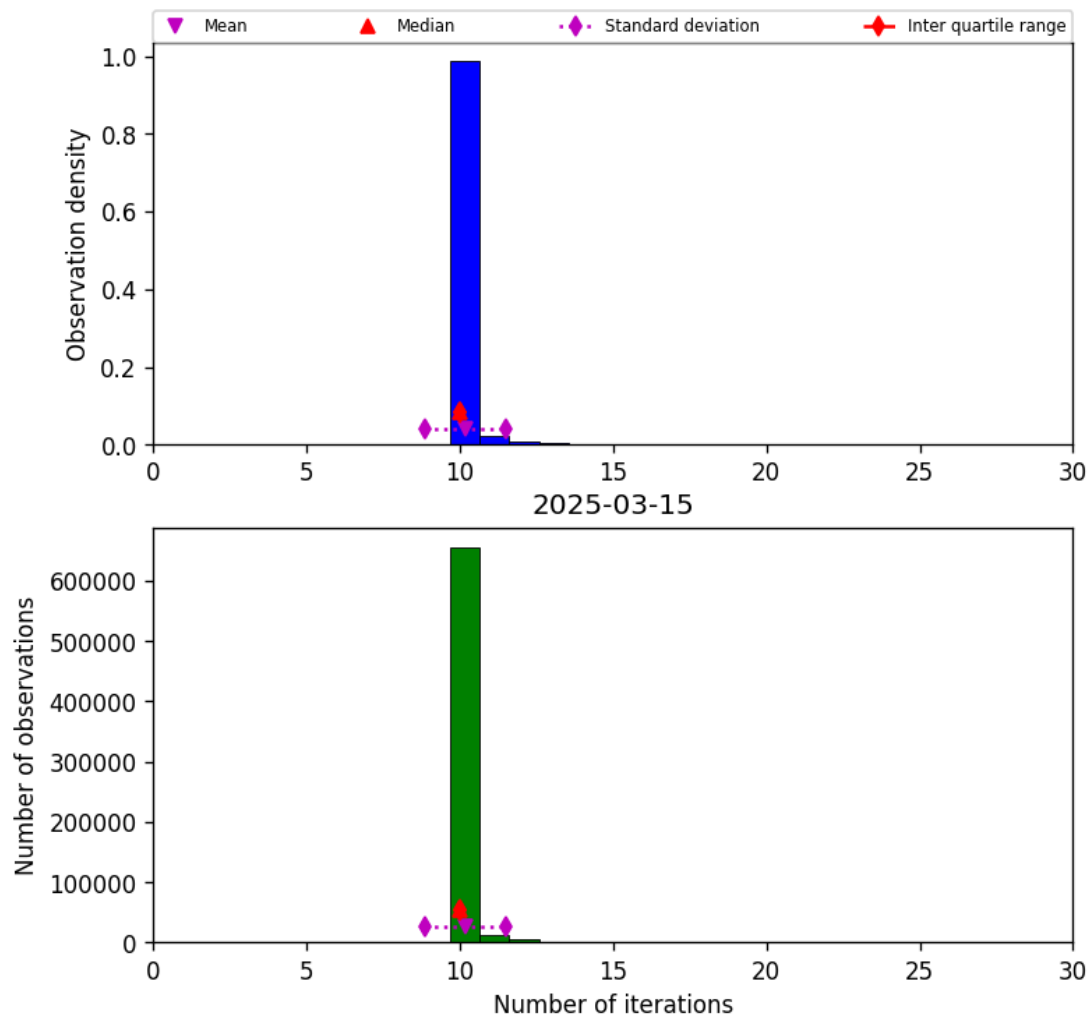
Figure 31: Histogram of “Number of iterations” for 2025-03-14 to 2025-03-16
