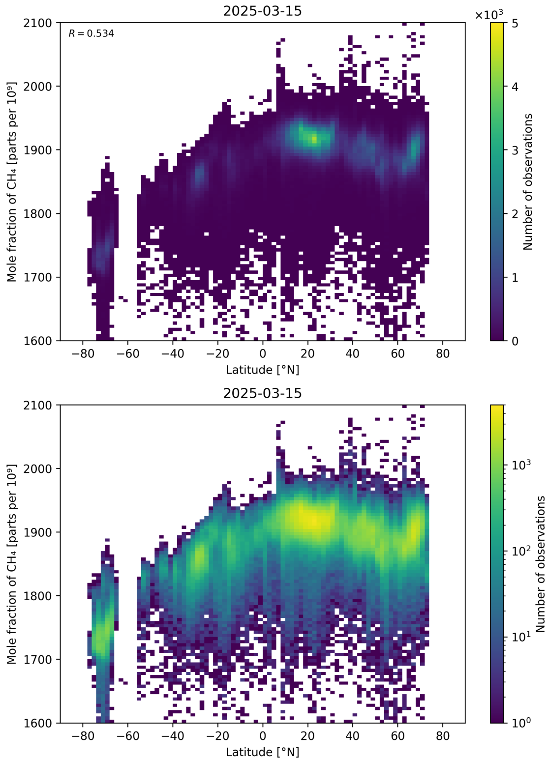
Figure 57: Scatter density plot of “Latitude” against “Mole fraction of \text{CH}_4 ” for 2025-03-14 to 2025-03-16.
