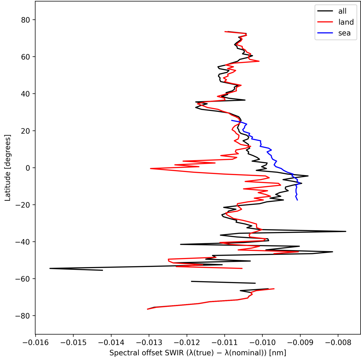
Figure 16: Zonal average of “Spectral offset SWIR ( \lambda_{\text{true}} - \lambda_{\text{nominal}} )” for 2025-03-14 to 2025-03-16.
