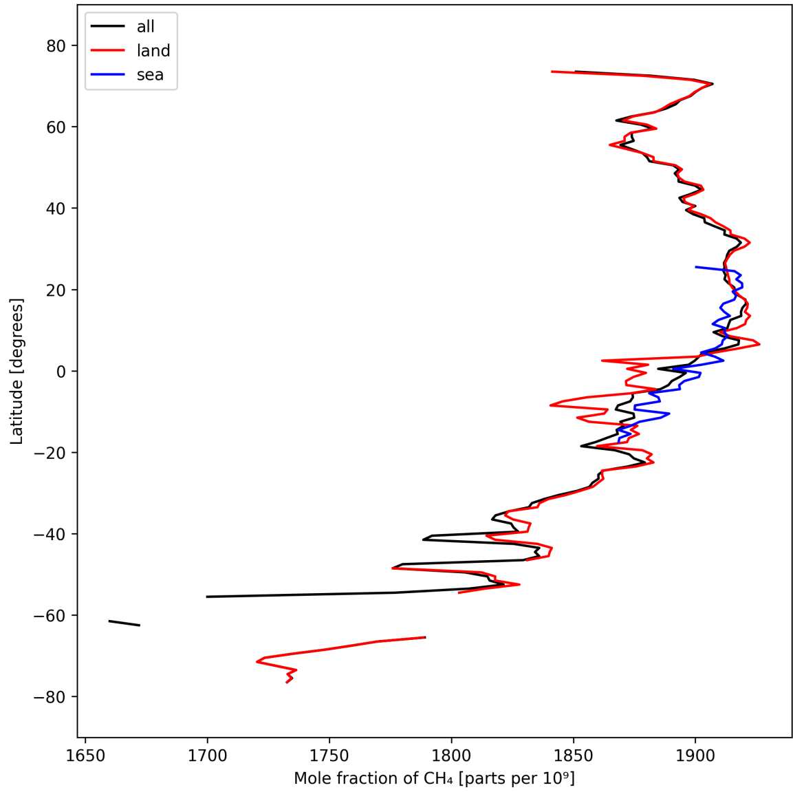
Figure 12: Zonal average of “Mole fraction of \text{CH}_4 ” for 2025-03-14 to 2025-03-16.
