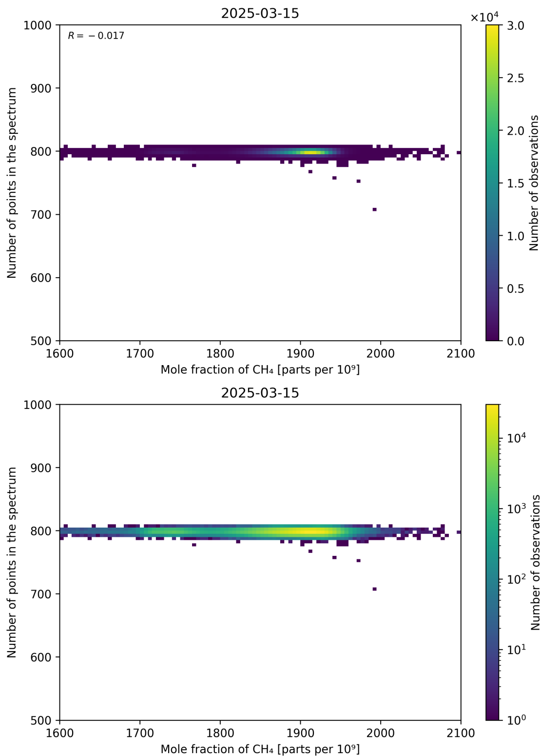
Figure 77: Scatter density plot of “Mole fraction of CH 4 ” against “Number of points in the spectrum” for 2025-03-14 to 2025-03-16.
