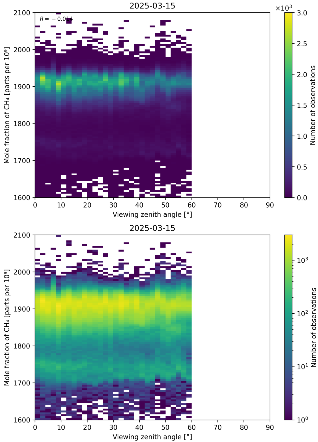
Figure 110: Scatter density plot of “Viewing zenith angle” against “Mole fraction of CH 4 ” for 2025-03-14 to 2025-03-16.
