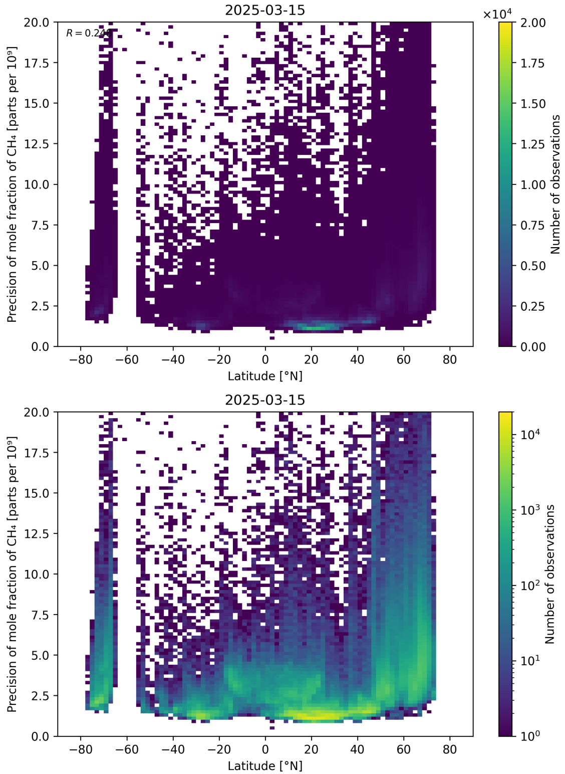
Figure 59: Scatter density plot of “Latitude” against “Precision of mole fraction of CH 4 ” for 2025-03-14 to 2025-03-16.
