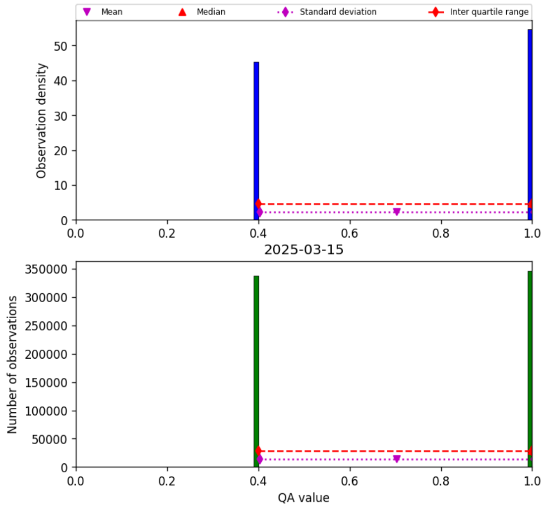
Figure 22: Histogram of “QA value” for 2025-03-14 to 2025-03-16
