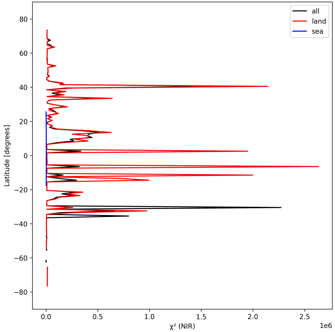
Figure 18: Zonal average of “ \chi^2 (NIR)” for 2025-03-14 to 2025-03-16.
