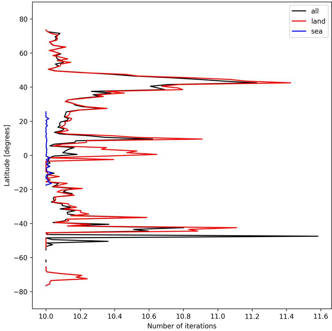
Figure 20: Zonal average of “Number of iterations” for 2025-03-14 to 2025-03-16.
