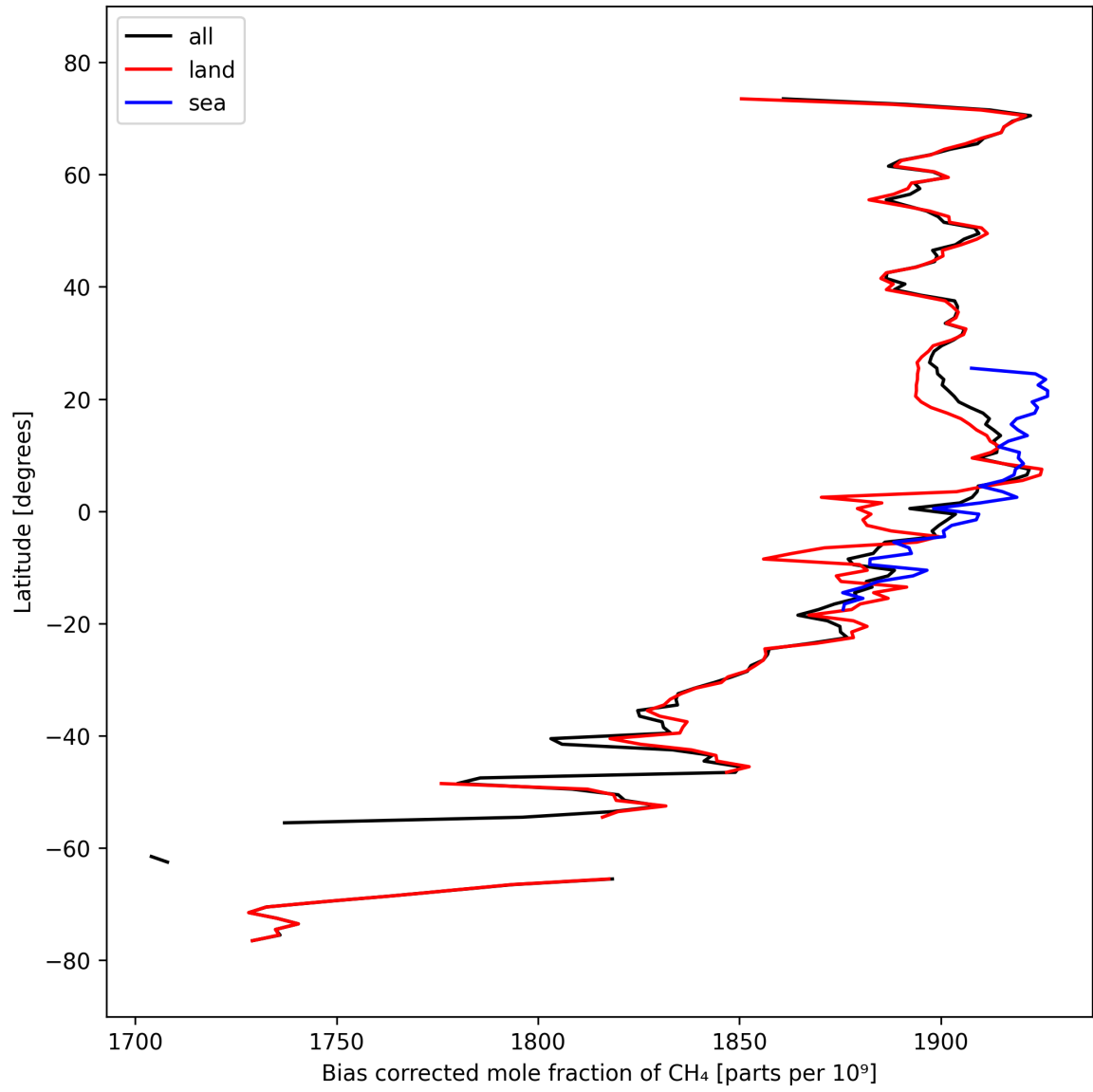
Figure 14: Zonal average of “Bias corrected mole fraction of CH 4 ” for 2025-03-14 to 2025-03-16.
