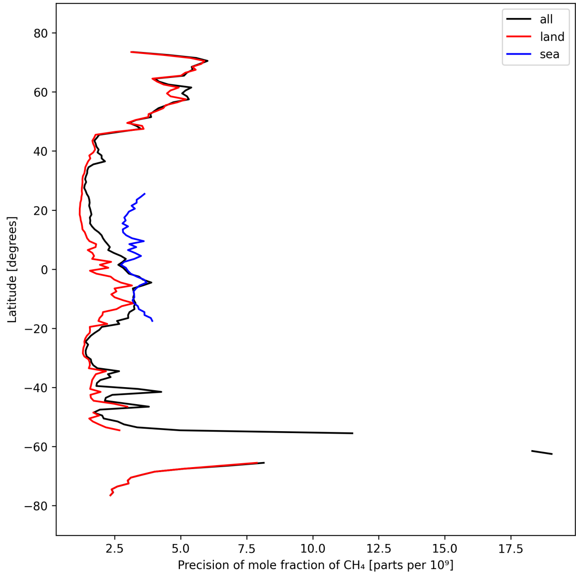
Figure 13: Zonal average of “Precision of mole fraction of CH 4 ” for 2025-03-14 to 2025-03-16.
