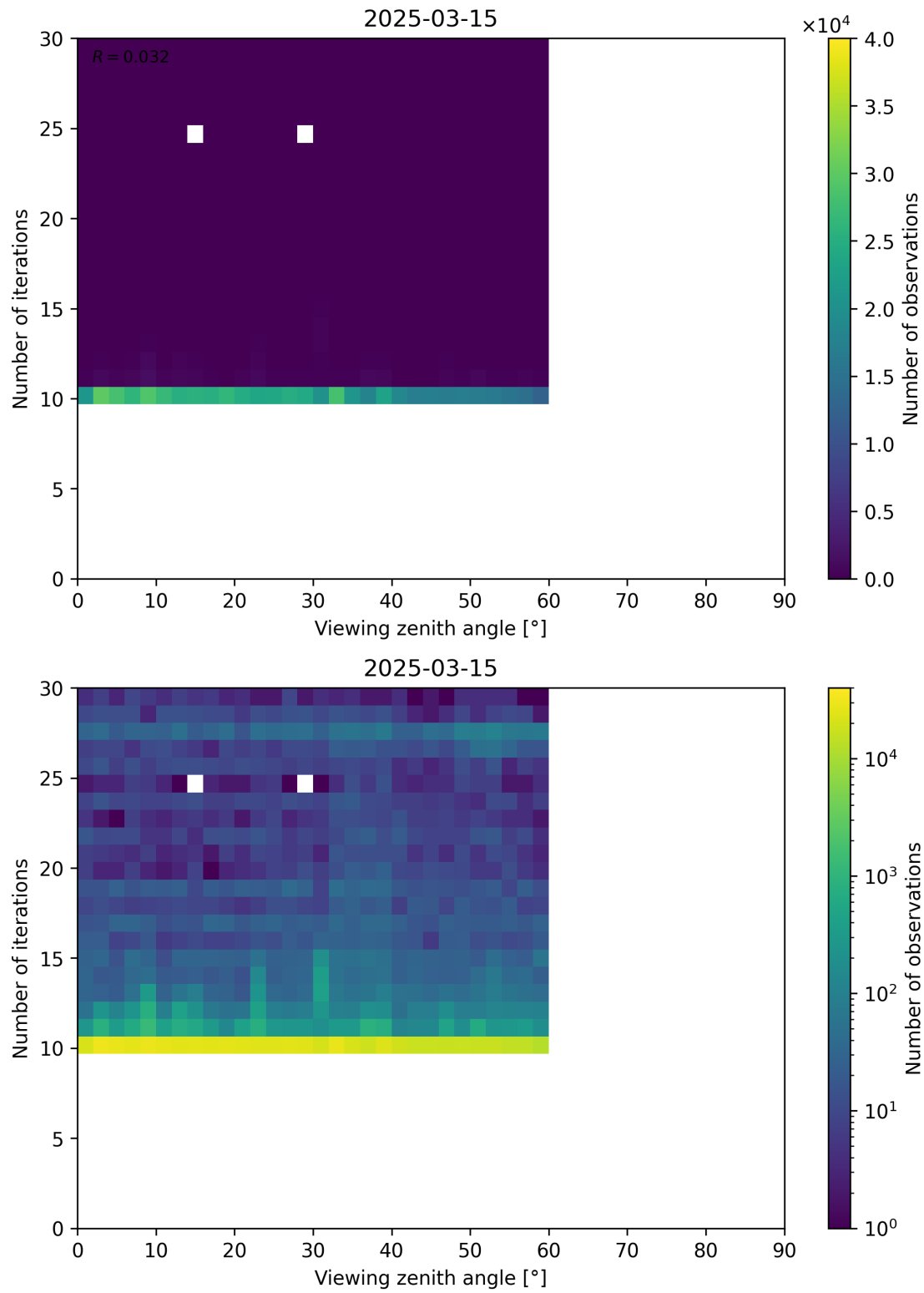
Figure 113: Scatter density plot of “Viewing zenith angle” against “Number of iterations” for 2025-03-14 to 2025-03-16.
