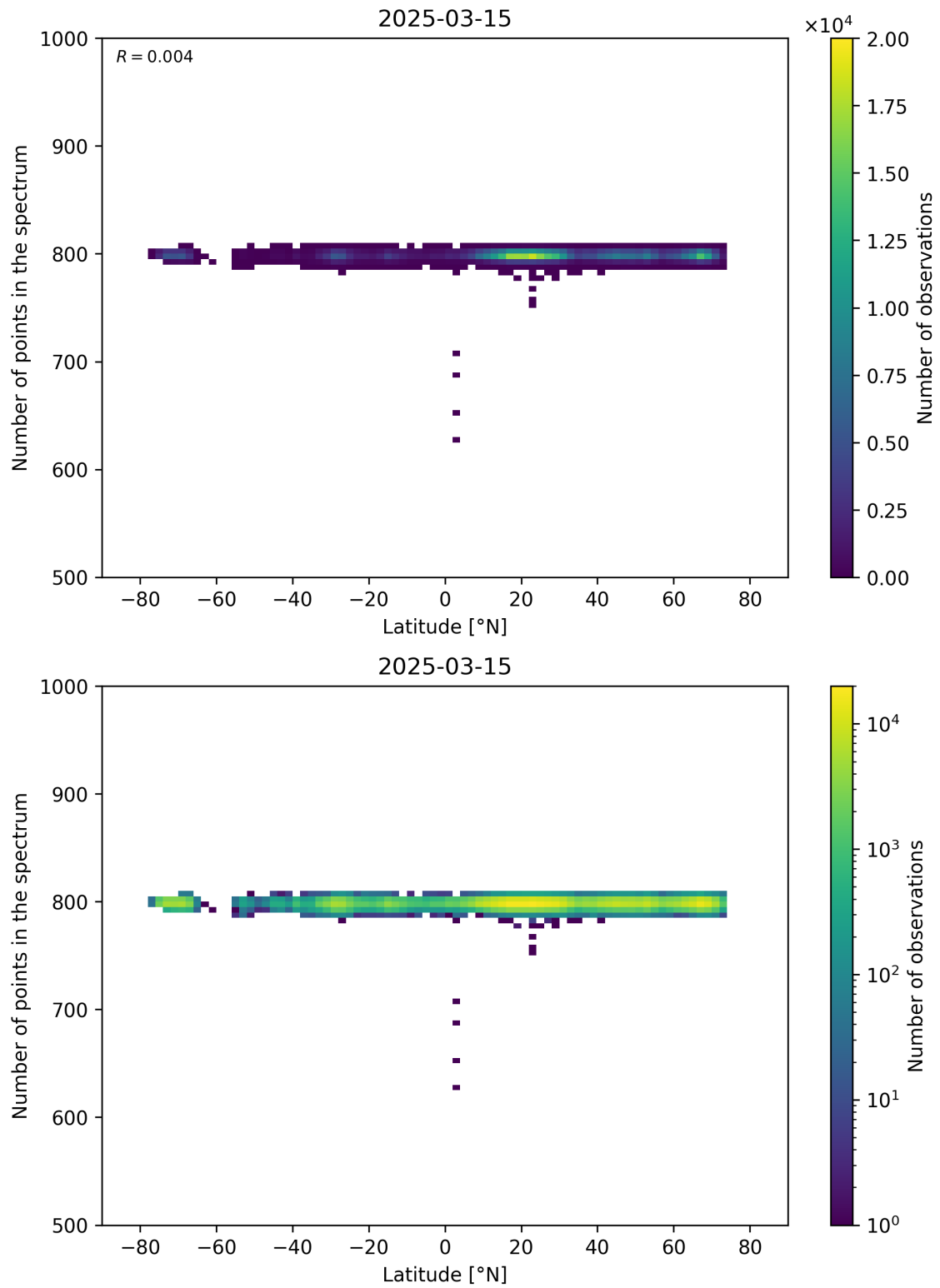
Figure 61: Scatter density plot of “Latitude” against “Number of points in the spectrum” for 2025-03-14 to 2025-03-16.
