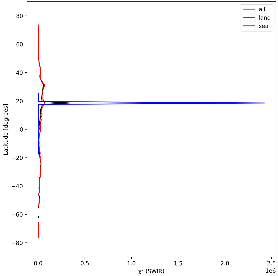
Figure 17: Zonal average of “ \chi^2 (SWIR)” for 2025-03-14 to 2025-03-16.
