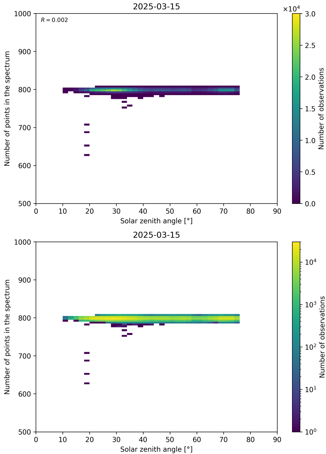
Figure 103: Scatter density plot of “Solar zenith angle” against “Number of points in the spectrum” for 2025-03-14 to 2025-03-16.
