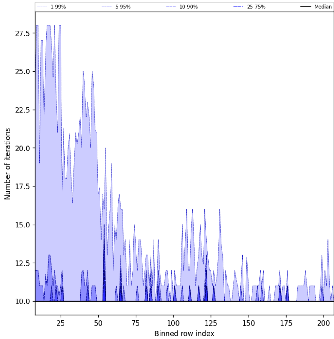
Figure 42: Along track statistics of “Number of iterations” for 2025-03-14 to 2025-03-16
