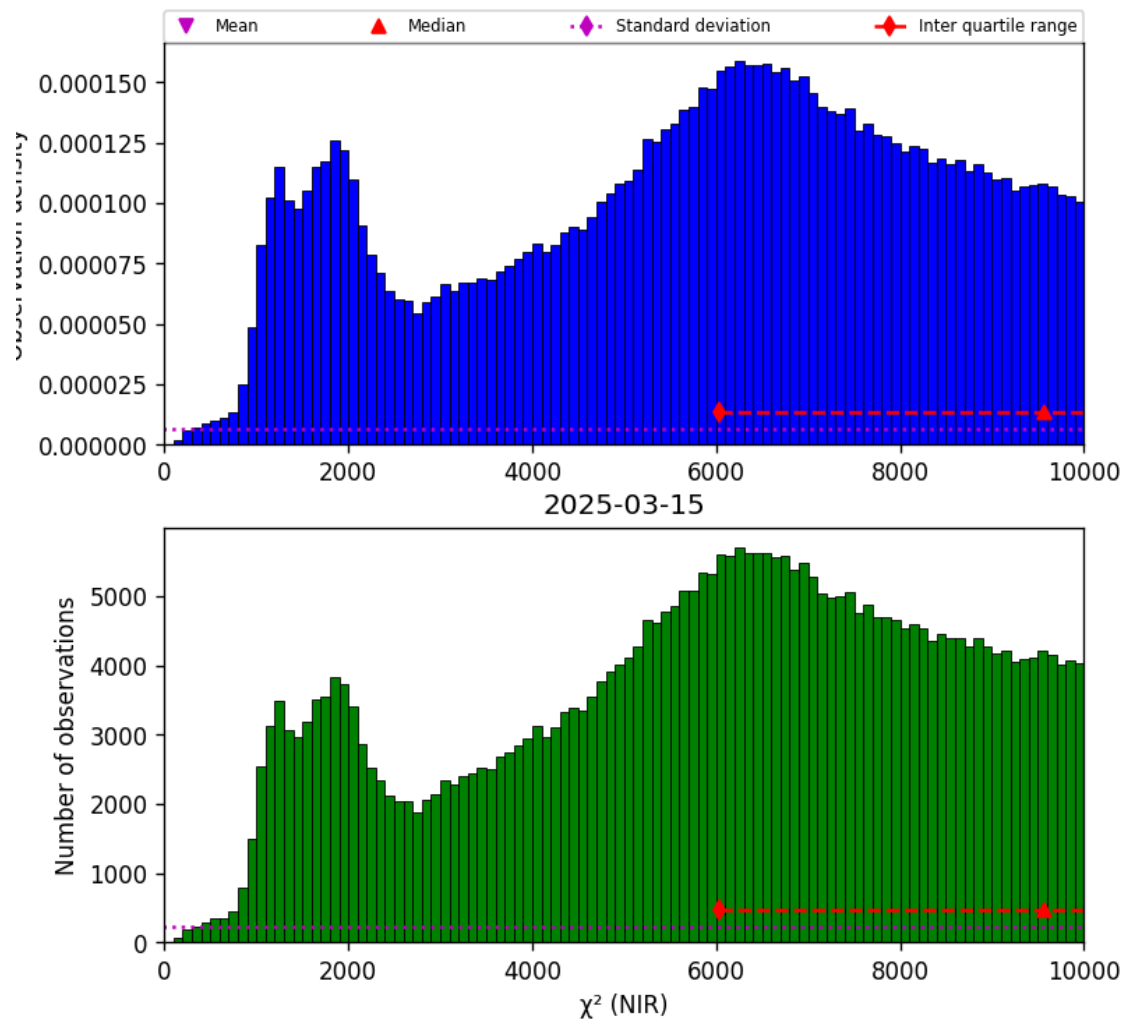
Figure 29: Histogram of “ \chi^2 (NIR)” for 2025-03-14 to 2025-03-16
