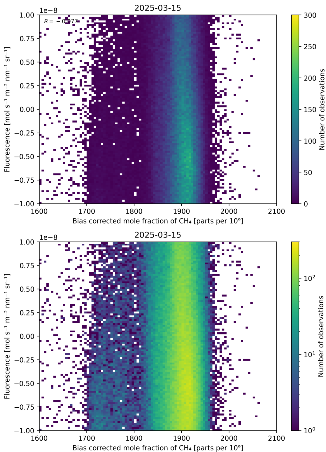
Figure 66: Scatter density plot of “Bias corrected mole fraction of \text{CH}_4 ” against “Fluorescence” for 2025-03-14 to 2025-03-16.
