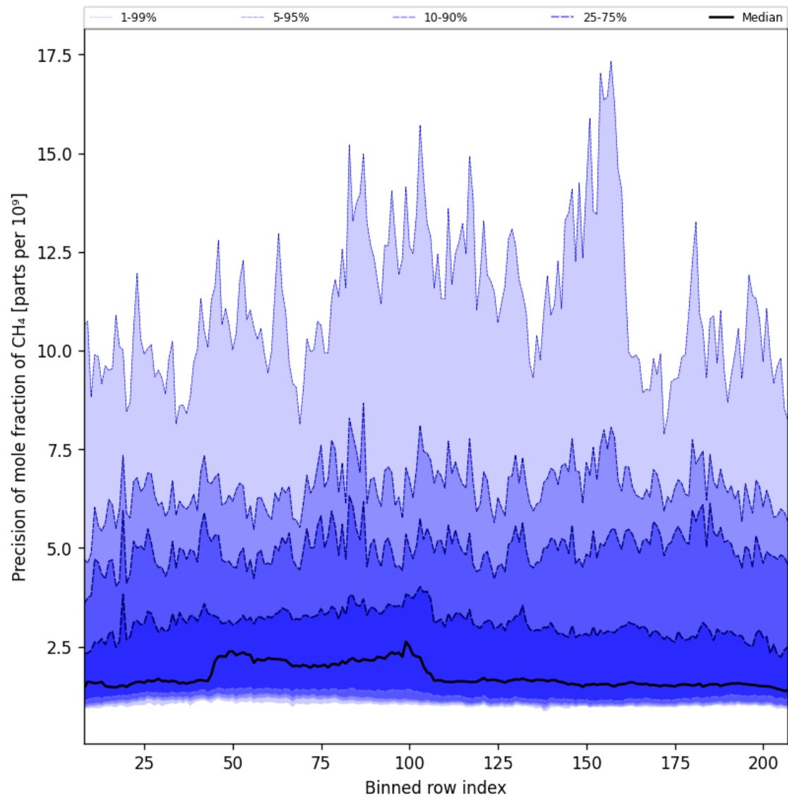
Figure 35: Along track statistics of “Precision of mole fraction of CH 4 ” for 2025-03-14 to 2025-03-16
