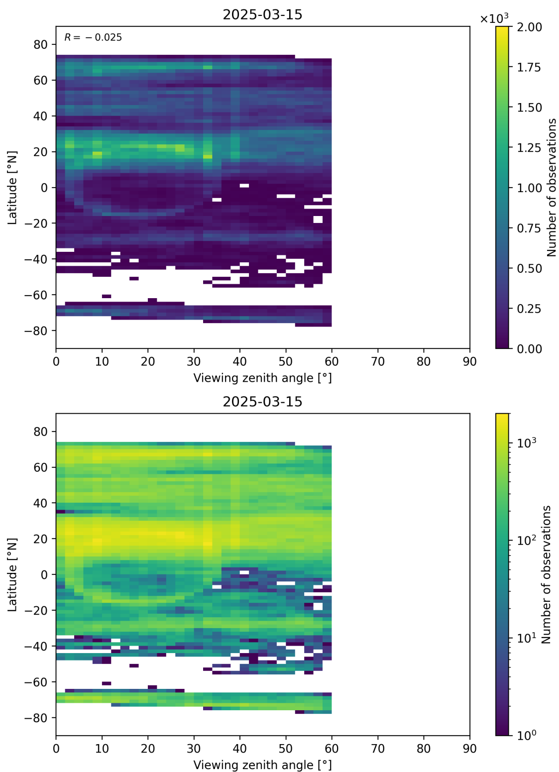
Figure 109: Scatter density plot of “Viewing zenith angle” against “Latitude” for 2025-03-14 to 2025-03-16.
