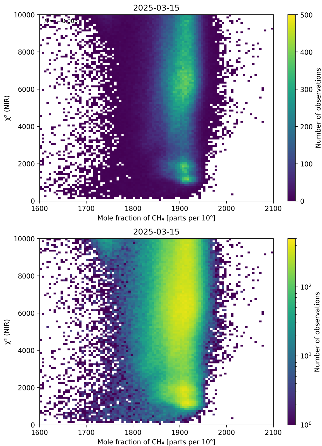
Figure 70: Scatter density plot of “Mole fraction of \text{CH}_4 ” against “ \chi^2 (NIR)” for 2025-03-14 to 2025-03-16.
