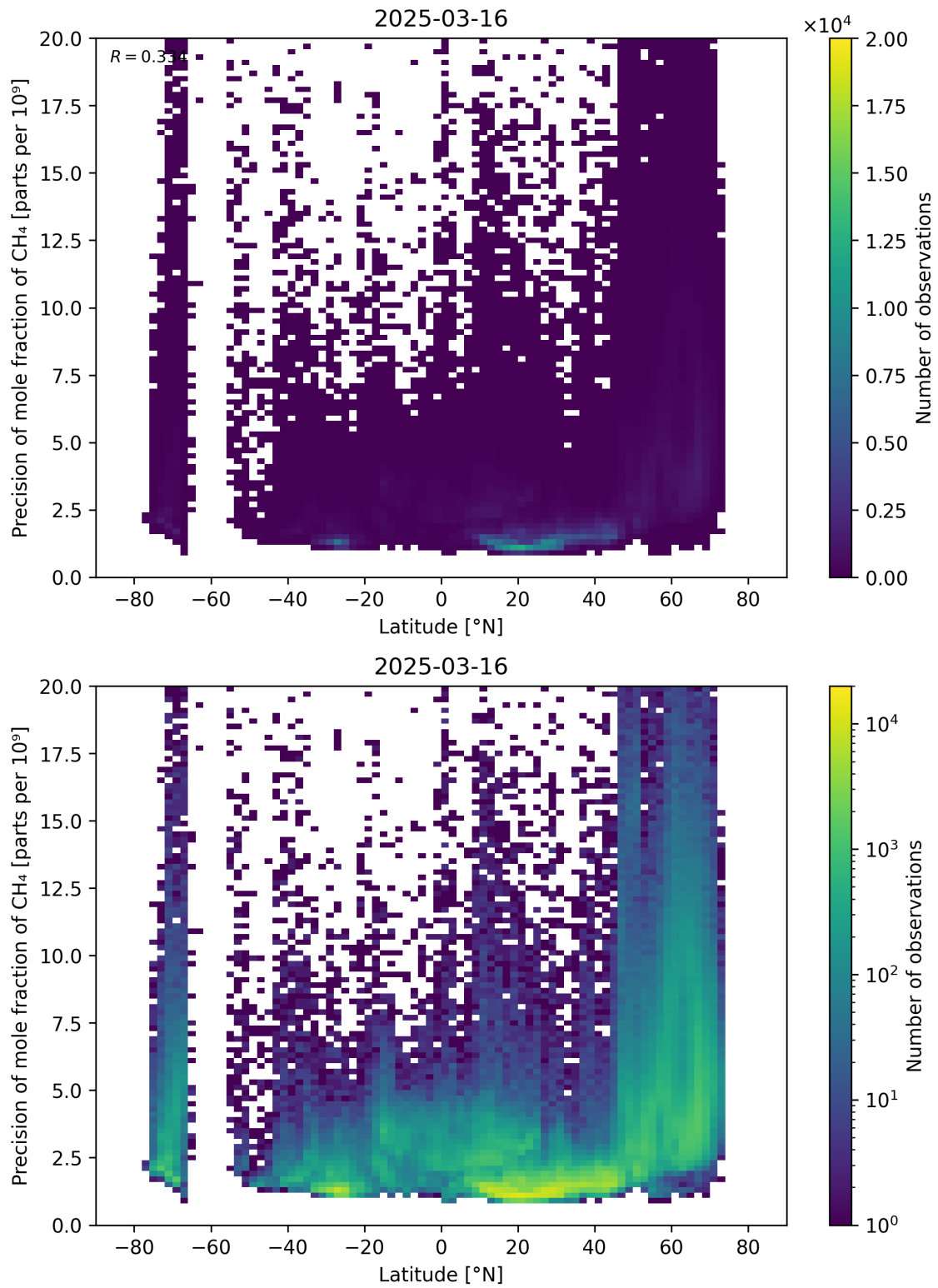
Figure 59: Scatter density plot of “Latitude” against “Precision of mole fraction of CH 4 ” for 2025-03-15 to 2025-03-17.
