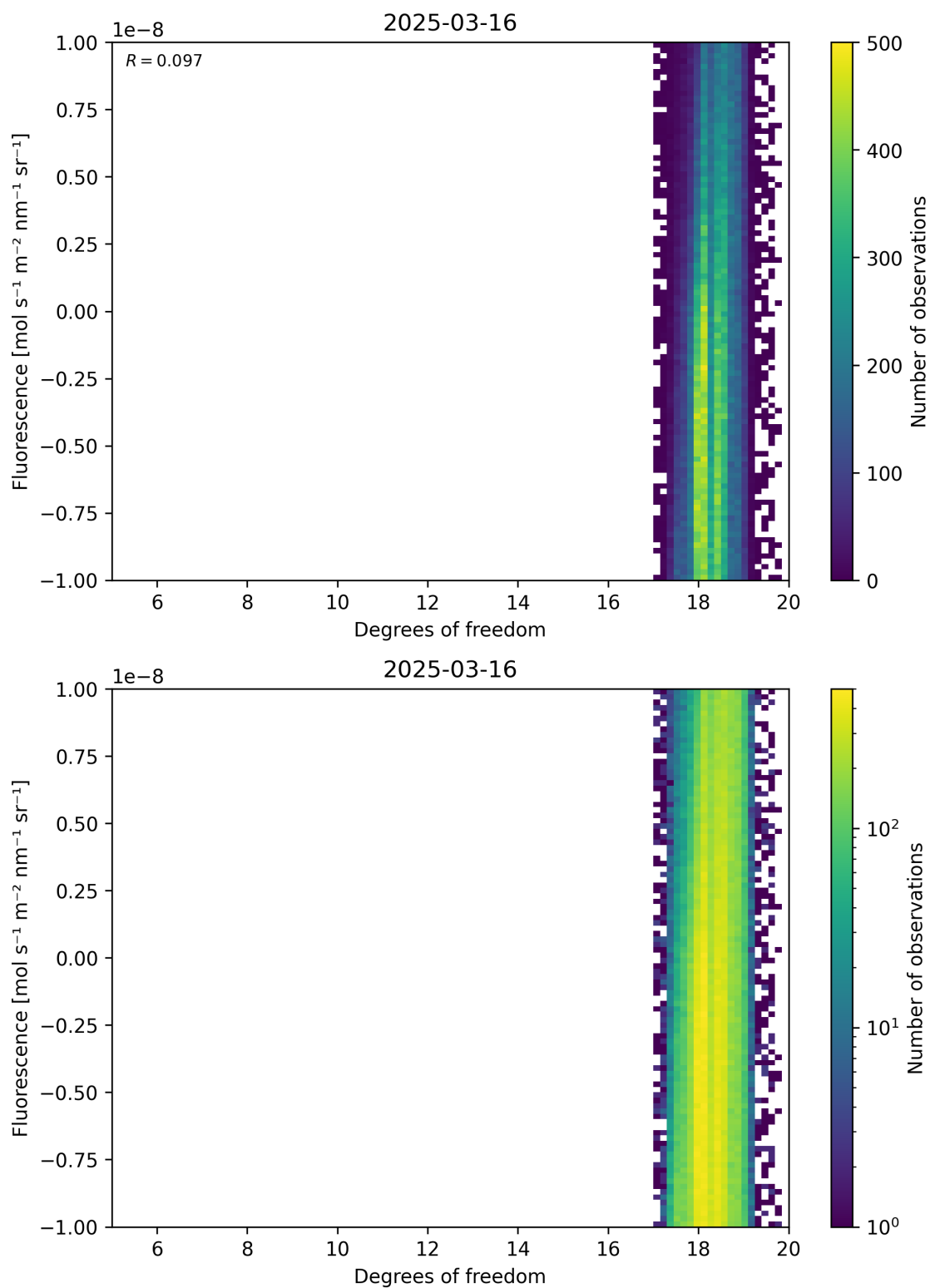
Figure 51: Scatter density plot of “Degrees of freedom” against “Fluorescence” for 2025-03-15 to 2025-03-17.
