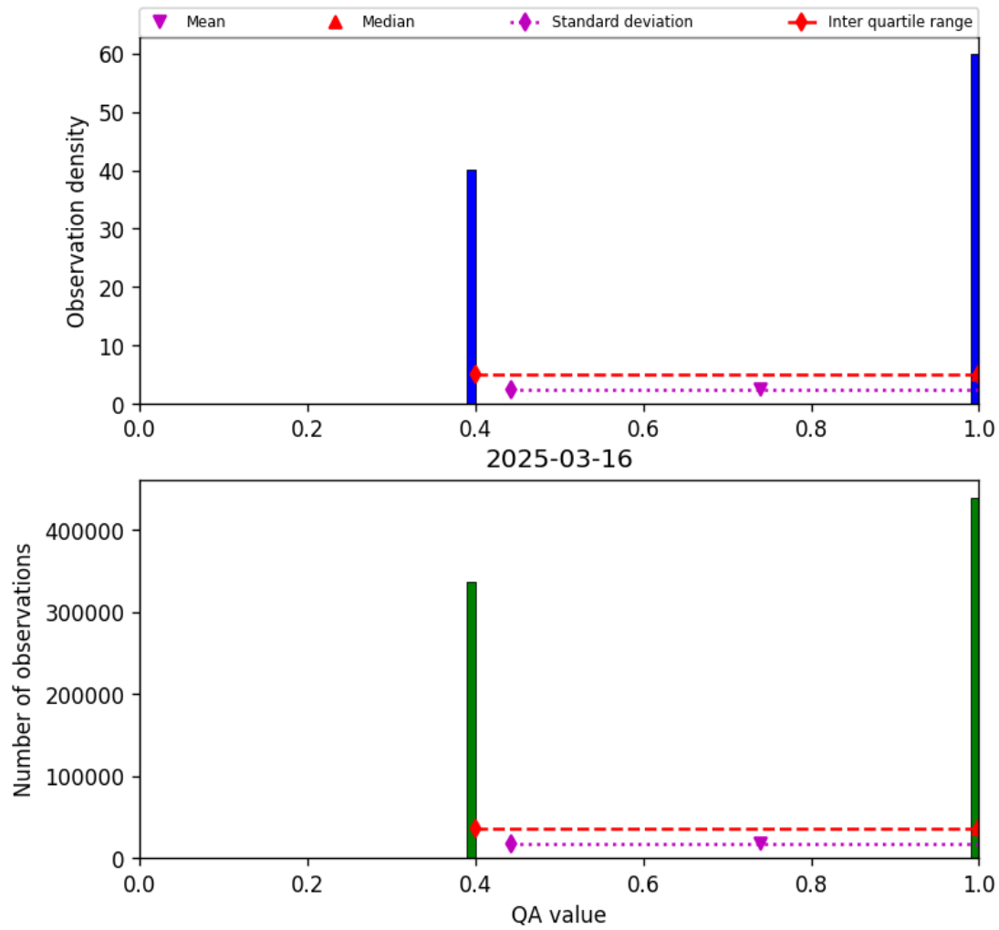
Figure 22: Histogram of “QA value” for 2025-03-15 to 2025-03-17
