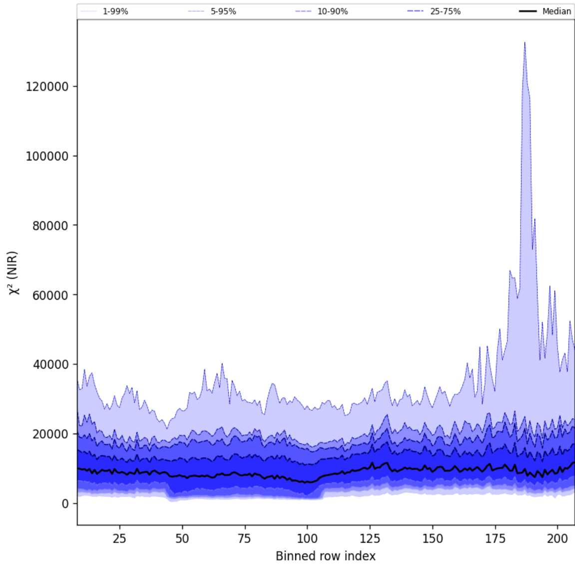
Figure 40: Along track statistics of “ \chi^2 (NIR)” for 2025-03-15 to 2025-03-17
