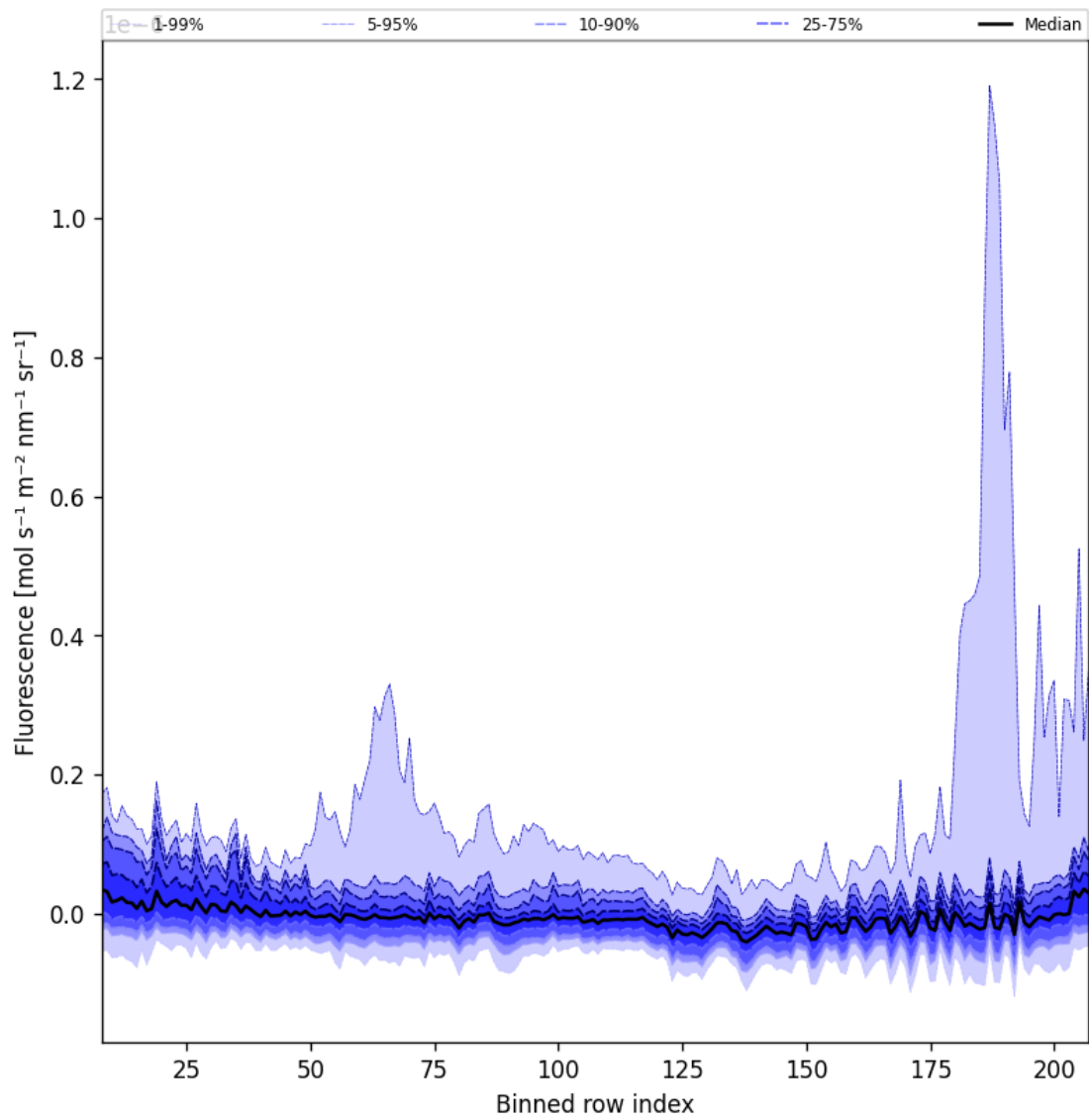
Figure 43: Along track statistics of “Fluorescence” for 2025-03-15 to 2025-03-17
