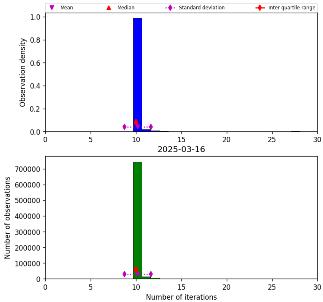
Figure 31: Histogram of “Number of iterations” for 2025-03-15 to 2025-03-17
