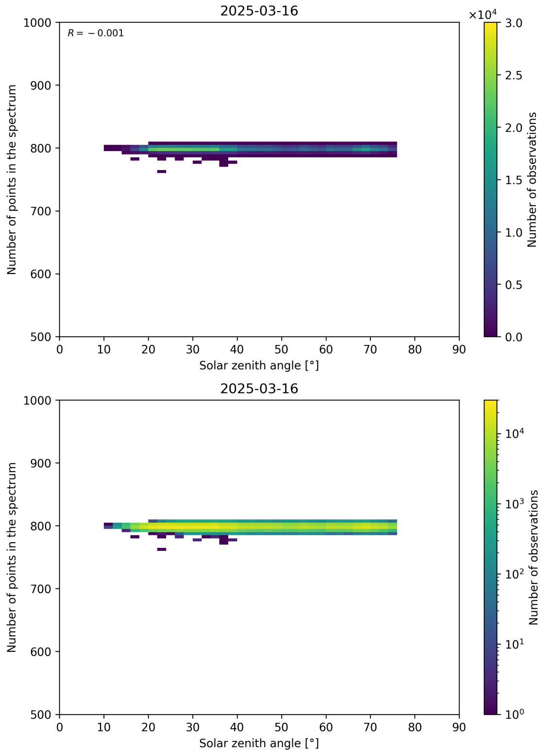
Figure 103: Scatter density plot of “Solar zenith angle” against “Number of points in the spectrum” for 2025-03-15 to 2025-03-17.
