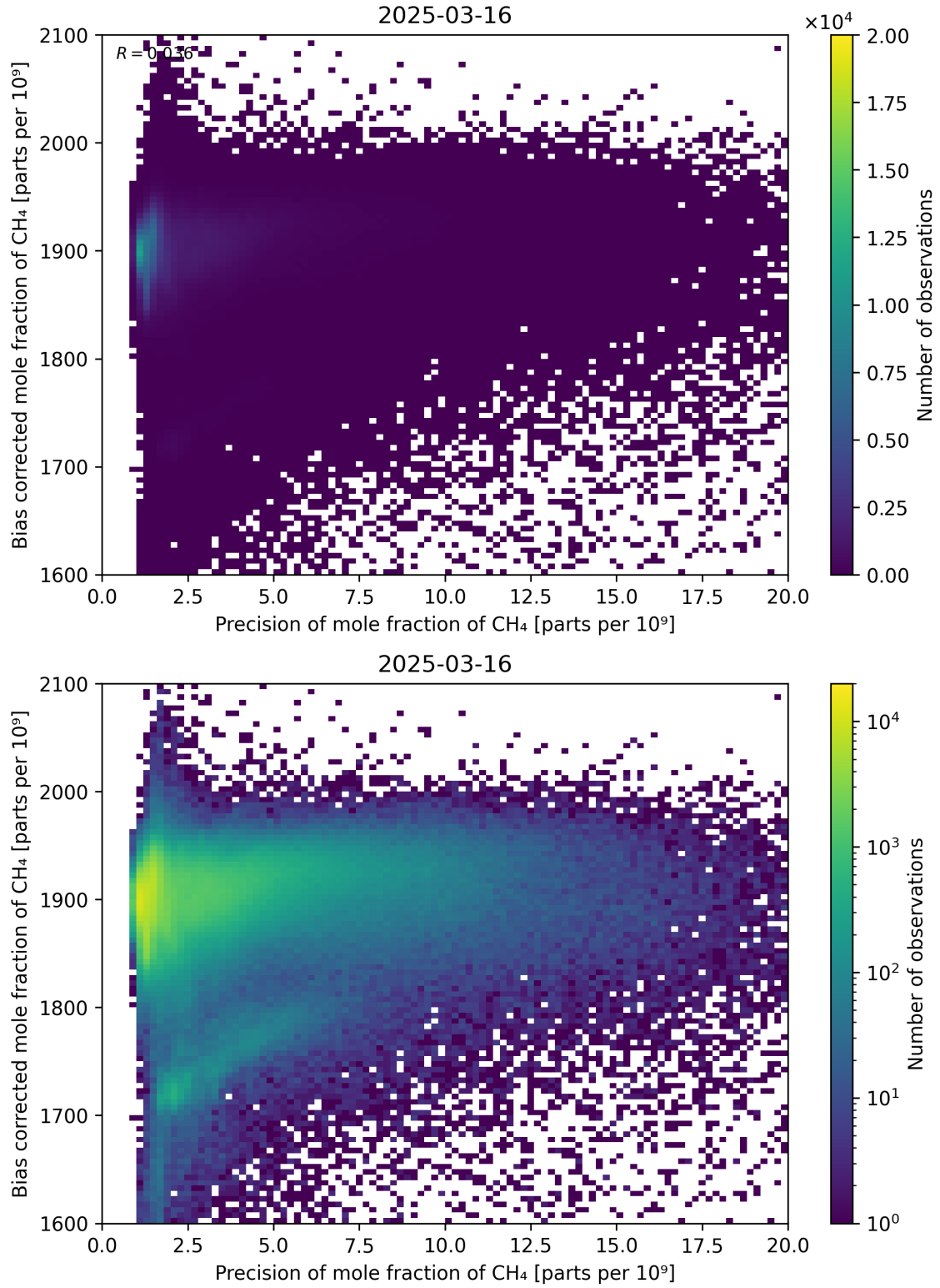
Figure 82: Scatter density plot of “Precision of mole fraction of CH 4 ” against “Bias corrected mole fraction of CH 4 ” for 2025-03-15 to 2025-03-17.
