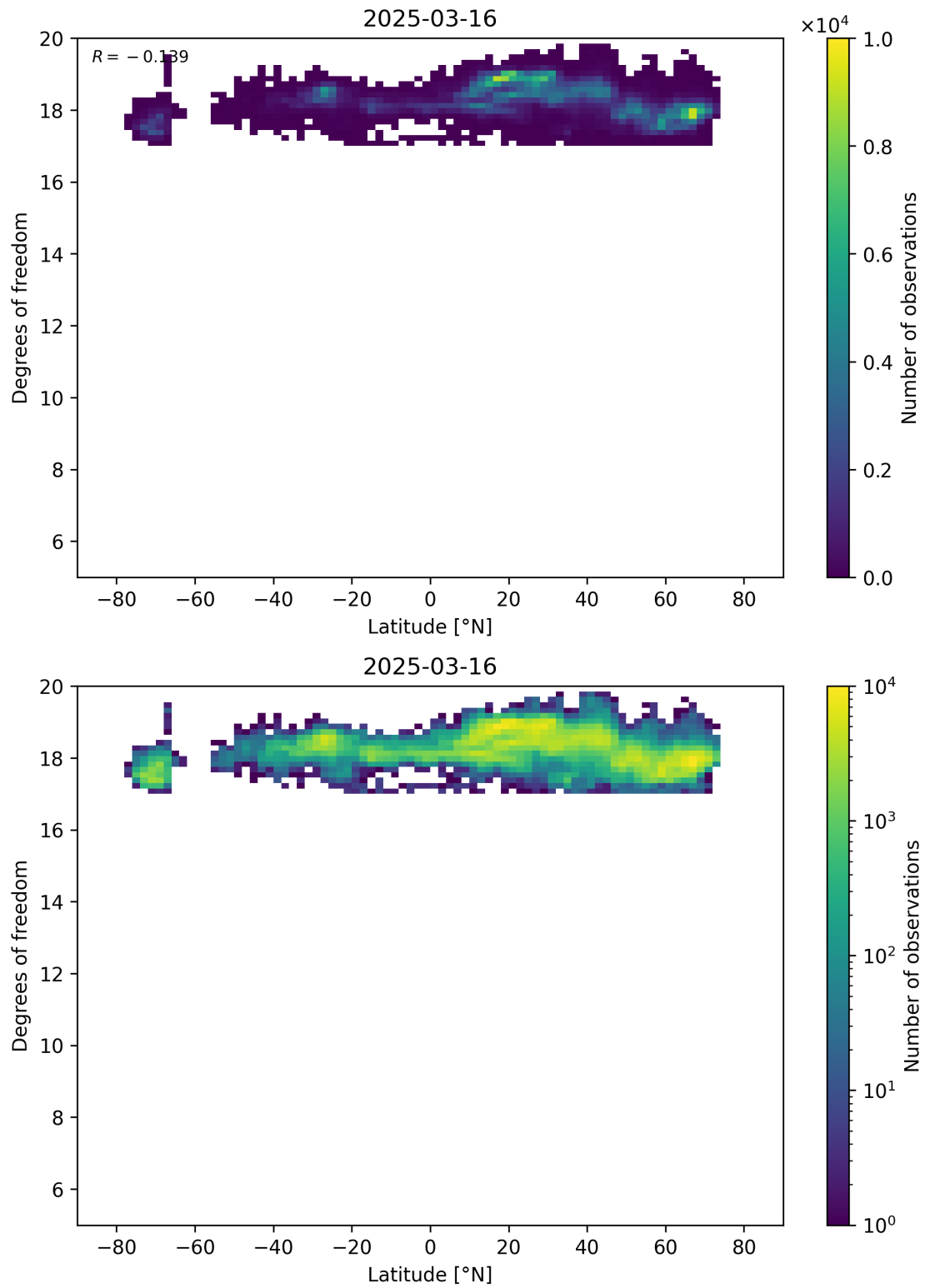
Figure 55: Scatter density plot of “Latitude” against “Degrees of freedom” for 2025-03-15 to 2025-03-17.
