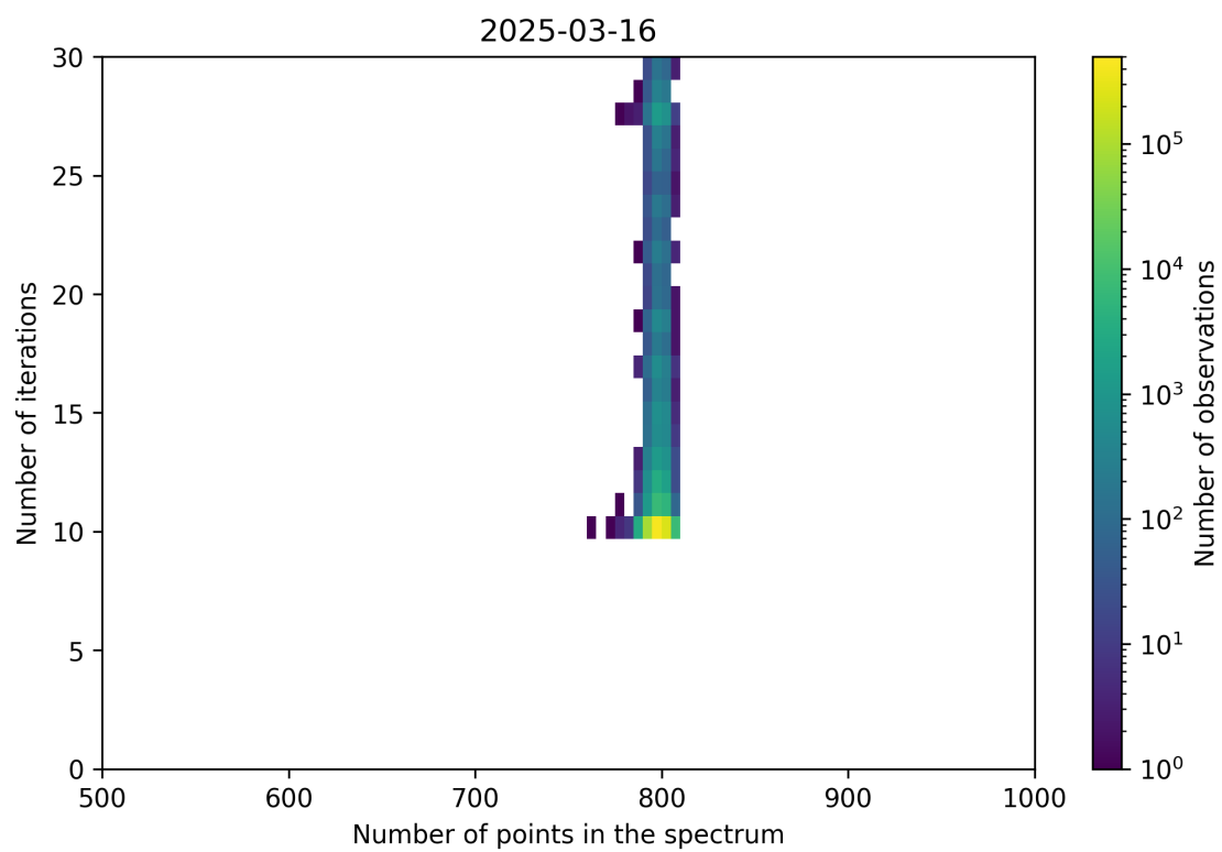
Figure 92: Scatter density plot of “Number of points in the spectrum” against “Number of iterations” for 2025-03-15 to 2025-03-17.
