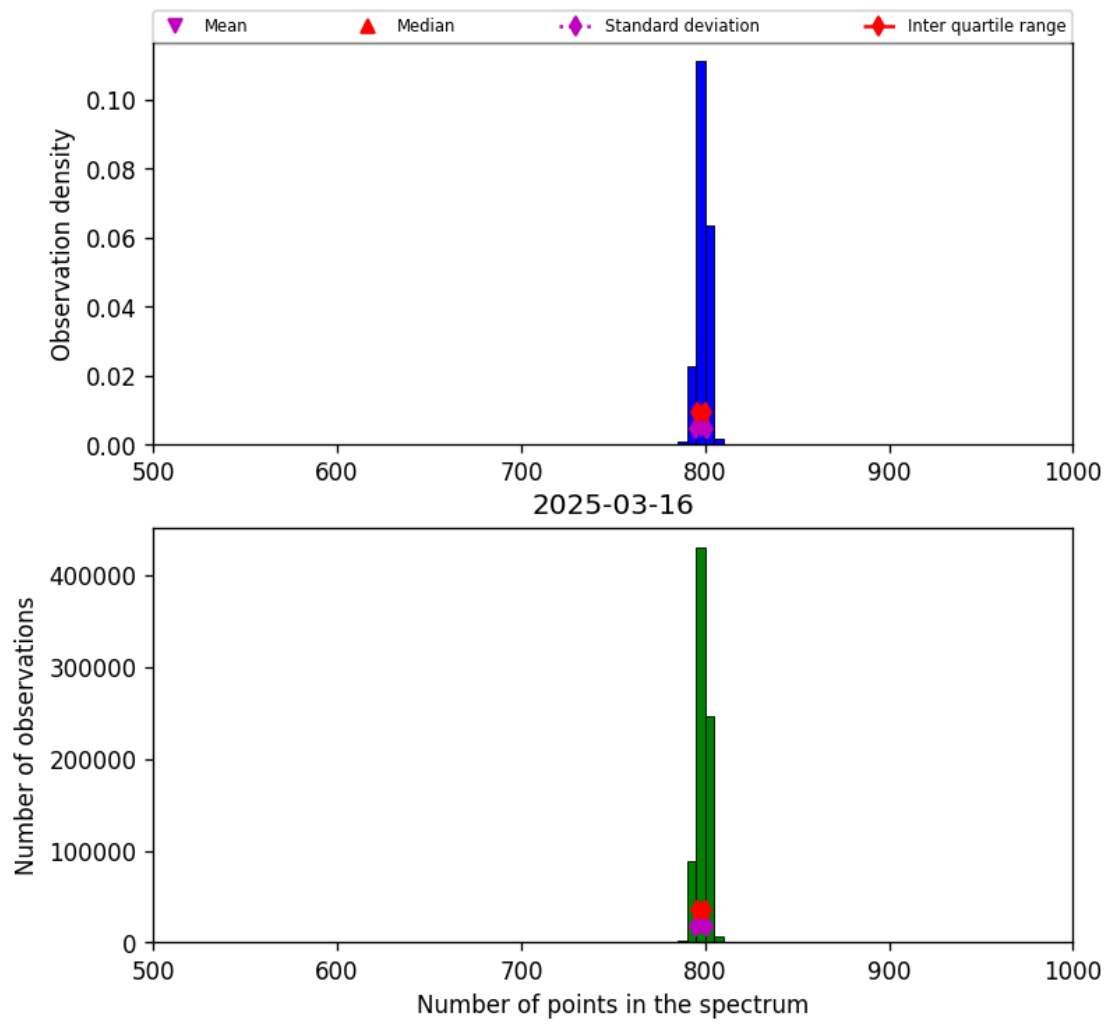
Figure 26: Histogram of “Number of points in the spectrum” for 2025-03-15 to 2025-03-17
