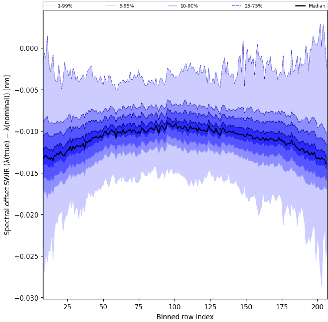
Figure 38: Along track statistics of “Spectral offset SWIR ( \lambda_{\text{true}} - \lambda_{\text{nominal}} )” for 2025-03-15 to 2025-03-17
