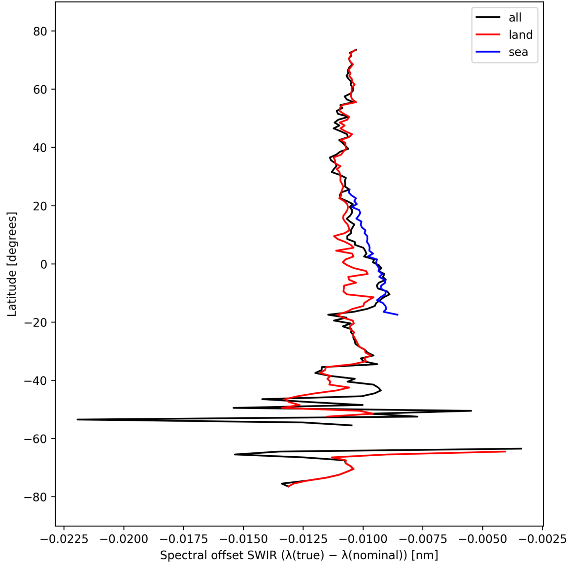
Figure 16: Zonal average of “Spectral offset SWIR ( \lambda_{\text{true}} - \lambda_{\text{nominal}} )” for 2025-03-15 to 2025-03-17.
