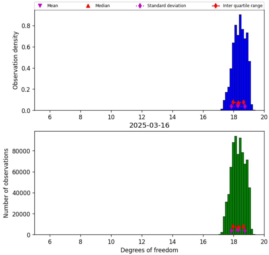
Figure 30: Histogram of “Degrees of freedom” for 2025-03-15 to 2025-03-17
