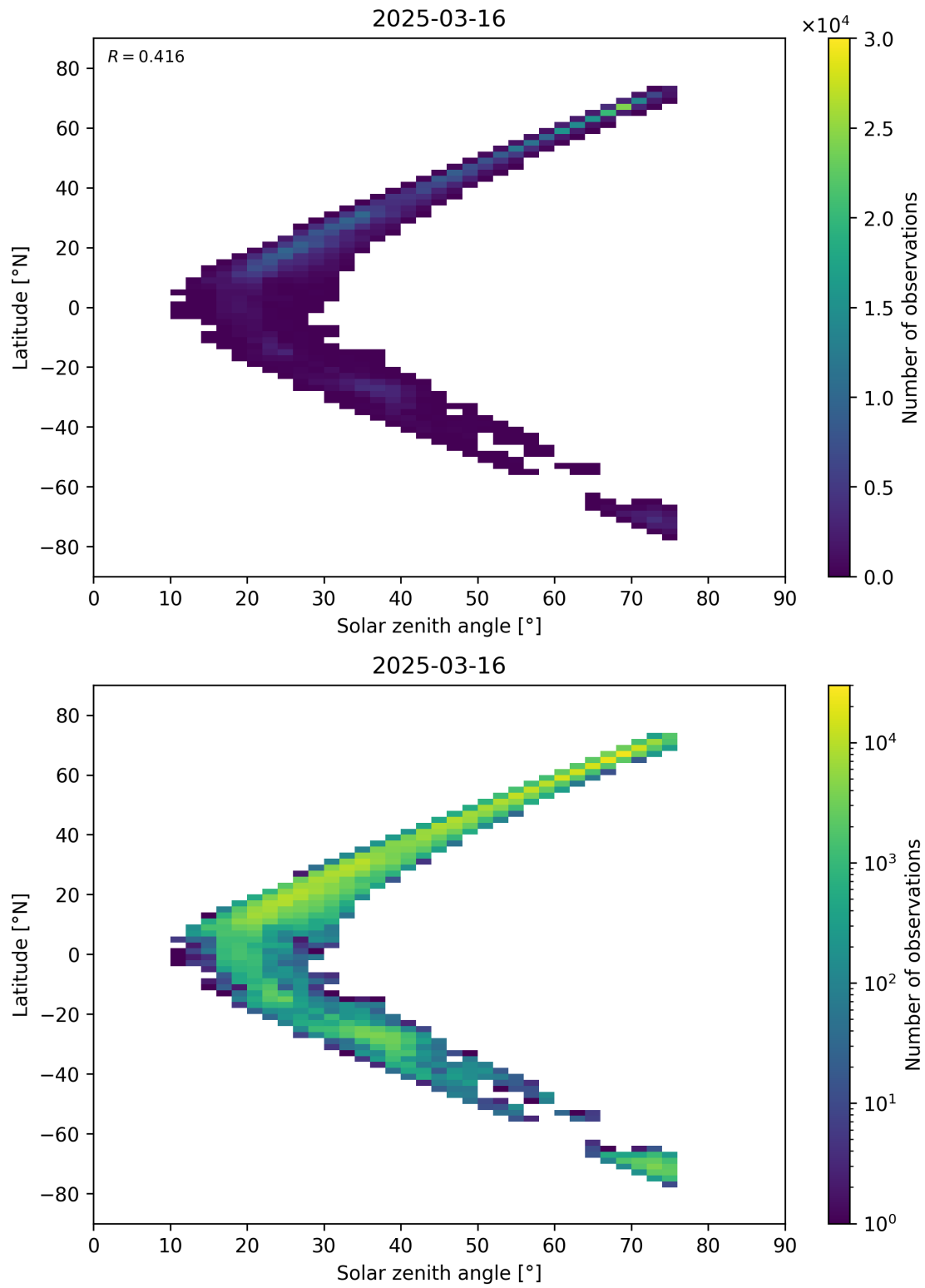
Figure 98: Scatter density plot of “Solar zenith angle” against “Latitude” for 2025-03-15 to 2025-03-17.
