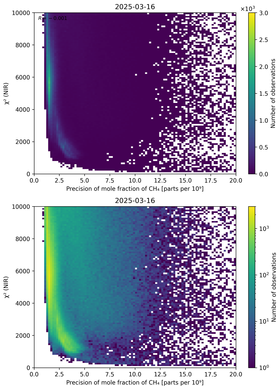
Figure 78: Scatter density plot of “Precision of mole fraction of CH 4 ” against “ \chi^2 (NIR)” for 2025-03-15 to 2025-03-17.
