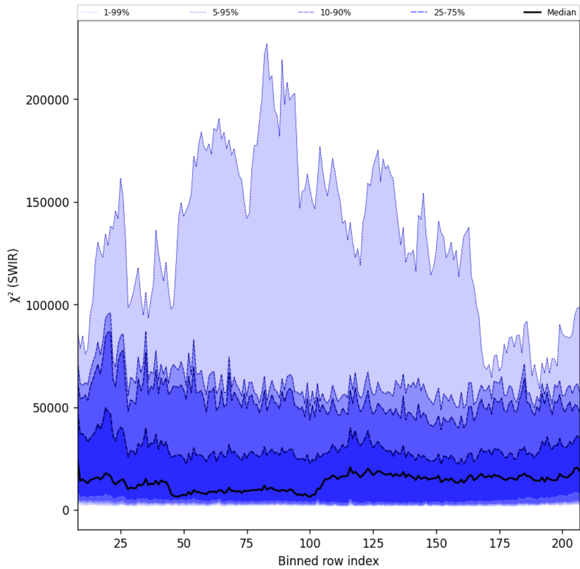
Figure 39: Along track statistics of “ \chi^2 (SWIR)” for 2025-03-15 to 2025-03-17
