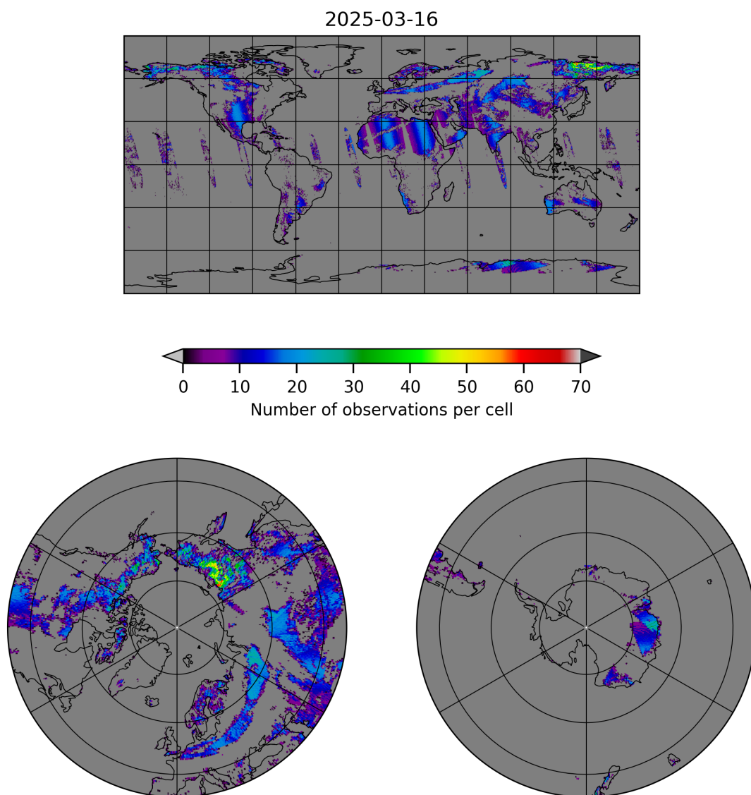
Figure 10: Map of the number of observations for 2025-03-15 to 2025-03-17
