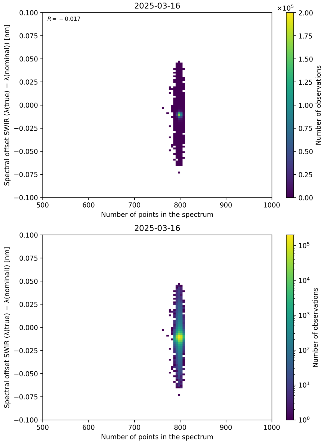
Figure 93: Scatter density plot of “Number of points in the spectrum” against “Spectral offset SWIR ( \lambda_{\text{true}} - \lambda_{\text{nominal}} )” for 2025-03-15 to 2025-03-17.
