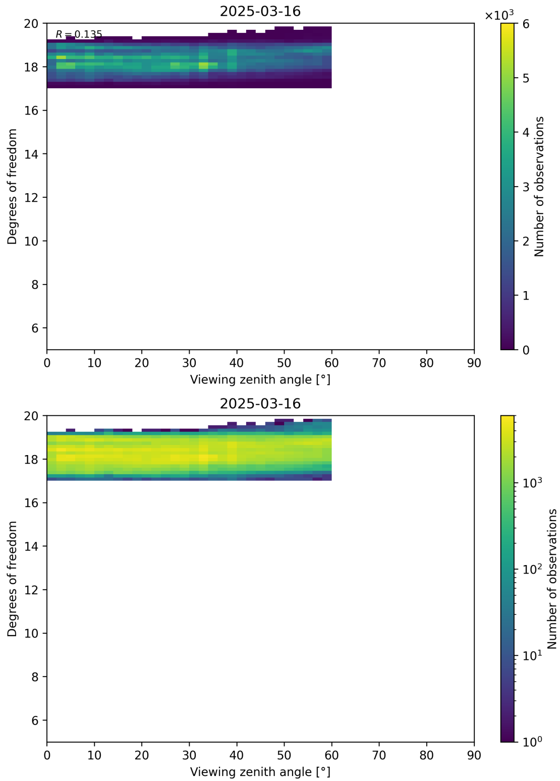
Figure 107: Scatter density plot of “Viewing zenith angle” against “Degrees of freedom” for 2025-03-15 to 2025-03-17.
