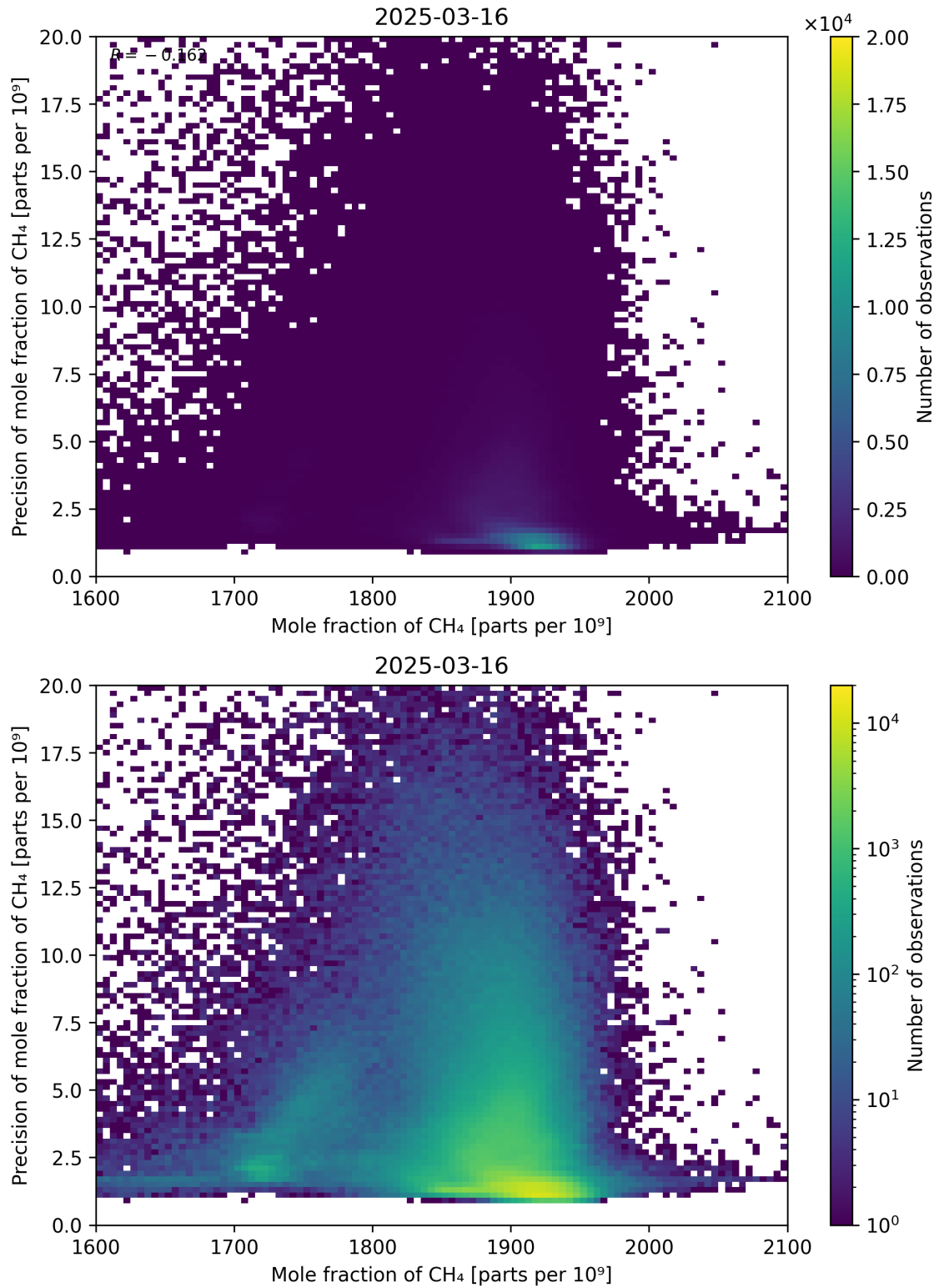
Figure 75: Scatter density plot of “Mole fraction of CH 4 ” against “Precision of mole fraction of CH 4 ” for 2025-03-15 to 2025-03-17.
