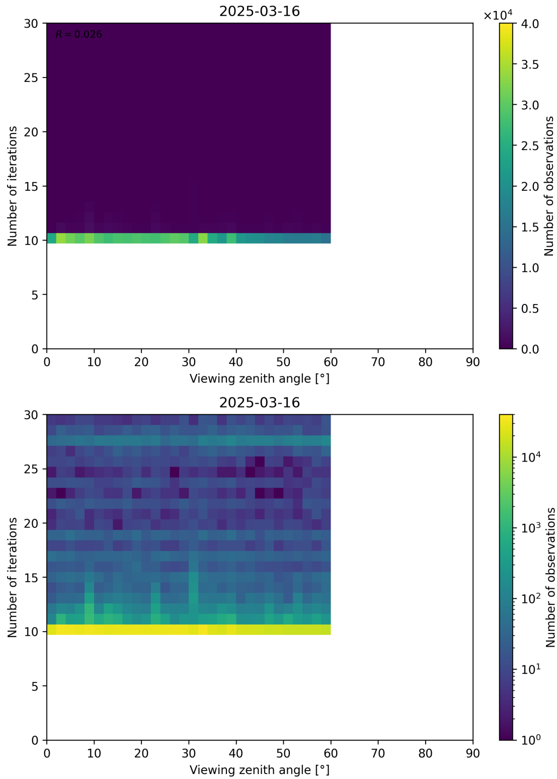
Figure 113: Scatter density plot of “Viewing zenith angle” against “Number of iterations” for 2025-03-15 to 2025-03-17.
