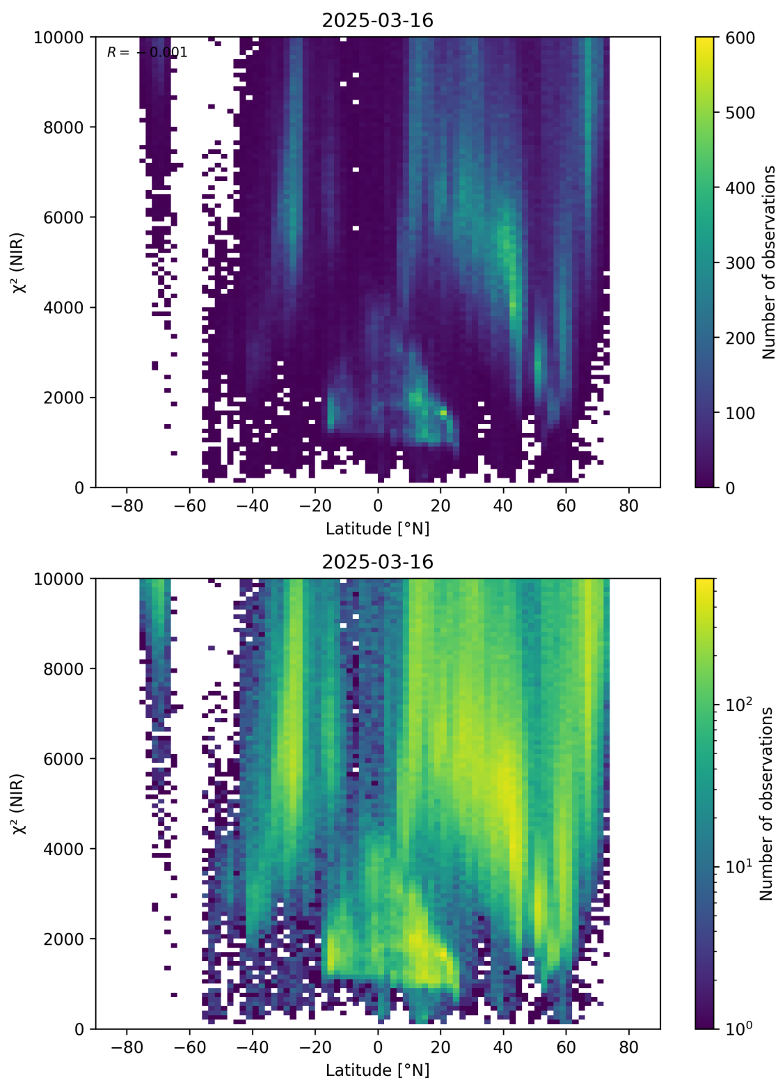
Figure 53: Scatter density plot of “Latitude” against “ \chi^2 (NIR)” for 2025-03-15 to 2025-03-17.
