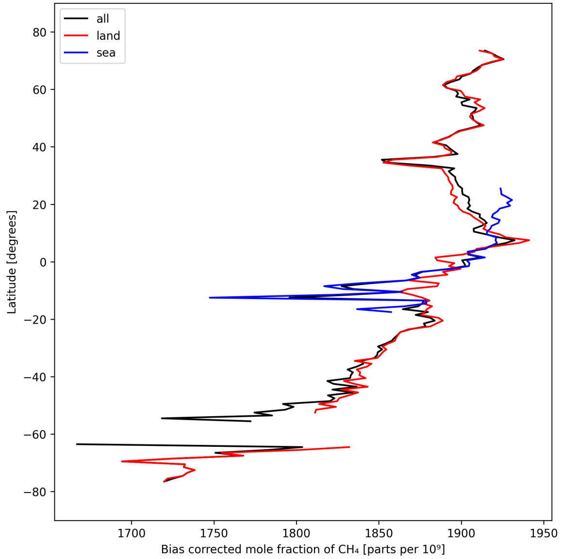
Figure 14: Zonal average of “Bias corrected mole fraction of CH 4 ” for 2025-03-15 to 2025-03-17.
