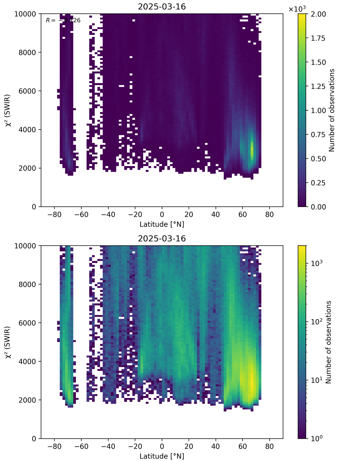
Figure 54: Scatter density plot of “Latitude” against “ \chi^2 (SWIR)” for 2025-03-15 to 2025-03-17.
