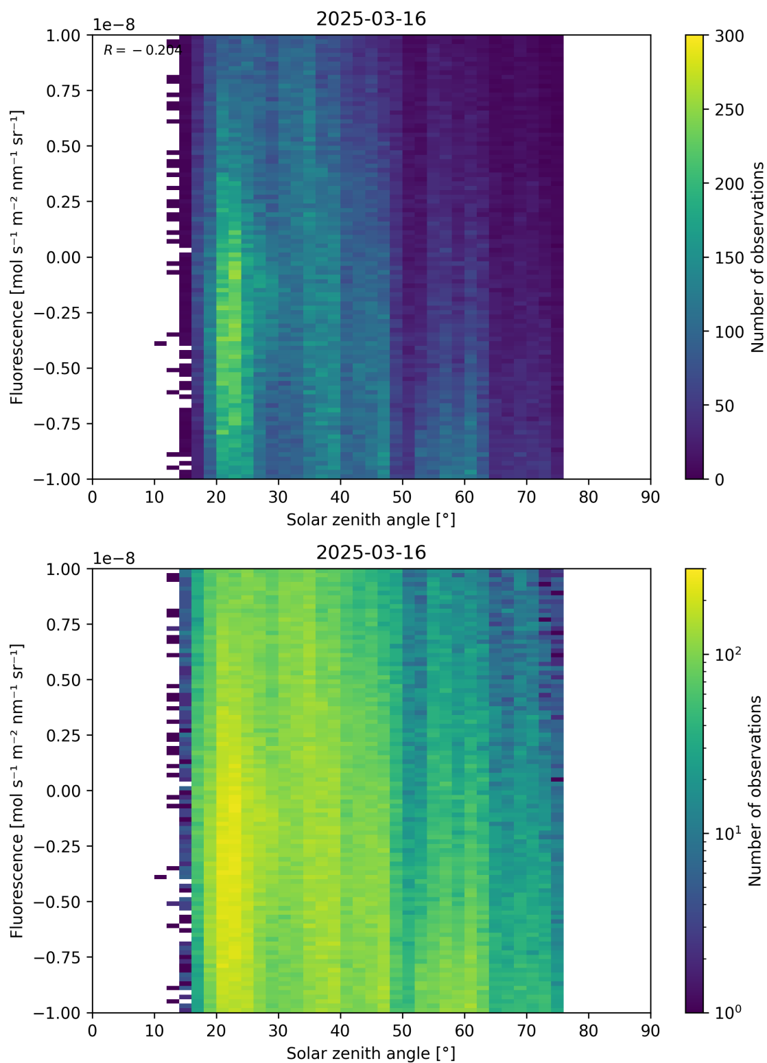
Figure 97: Scatter density plot of “Solar zenith angle” against “Fluorescence” for 2025-03-15 to 2025-03-17.
