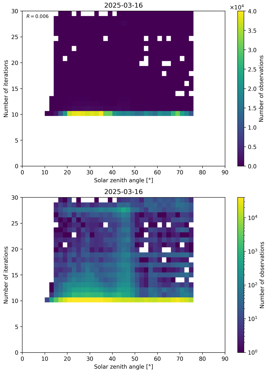
Figure 102: Scatter density plot of “Solar zenith angle” against “Number of iterations” for 2025-03-15 to 2025-03-17.
