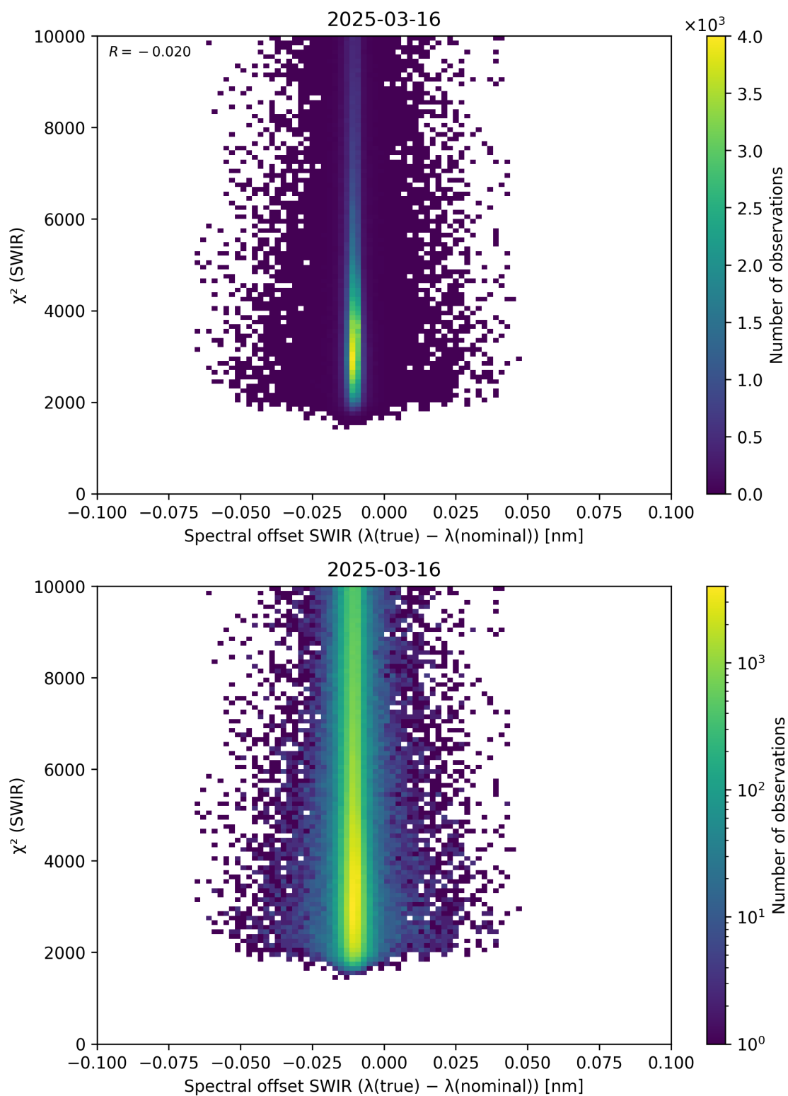
Figure 118: Scatter density plot of “Spectral offset SWIR ( \lambda_{\text{true}} - \lambda_{\text{nominal}} )” against “ \chi^2 (SWIR)” for 2025-03-15 to 2025-03-17.
