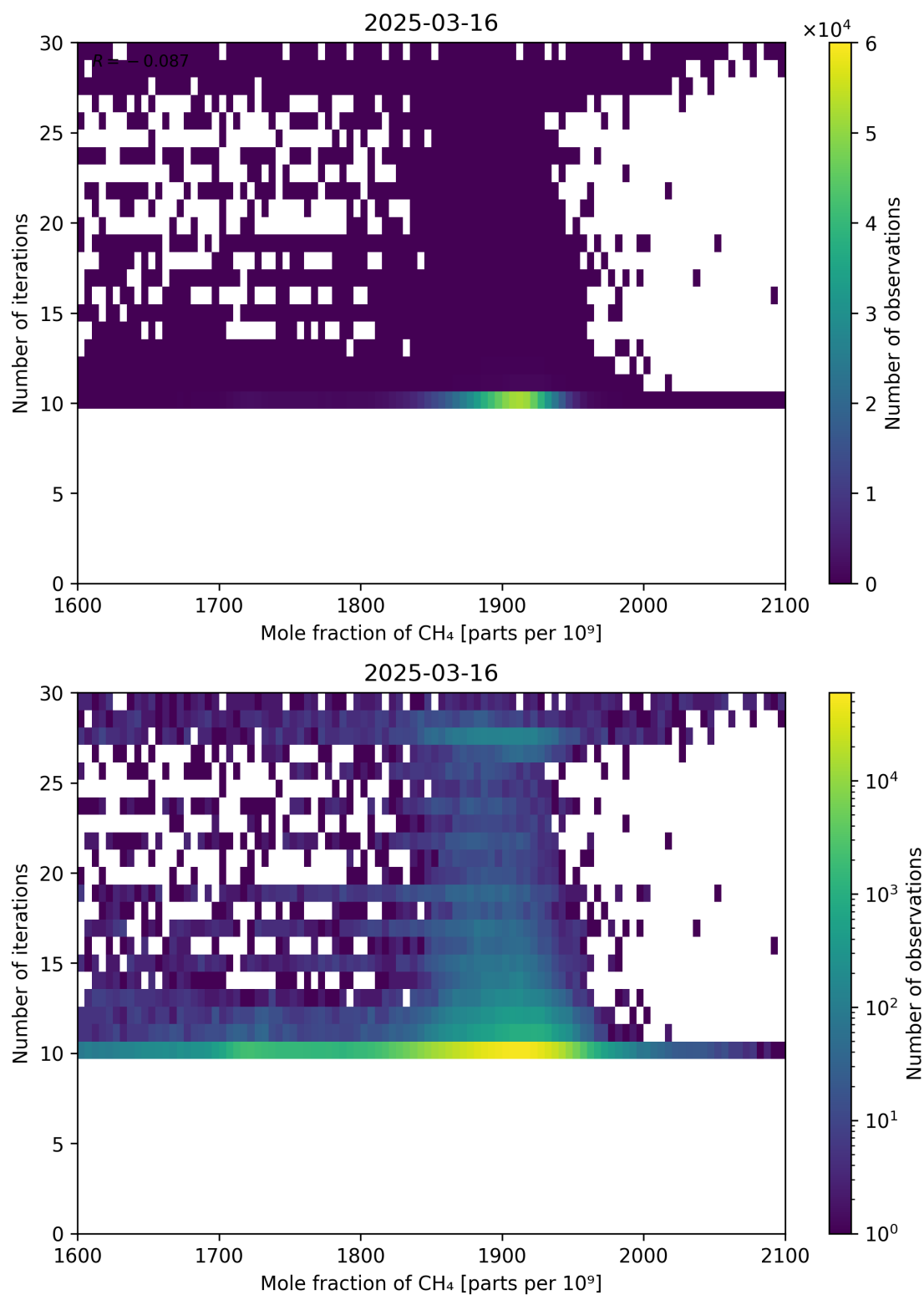
Figure 76: Scatter density plot of “Mole fraction of CH 4 ” against “Number of iterations” for 2025-03-15 to 2025-03-17.
