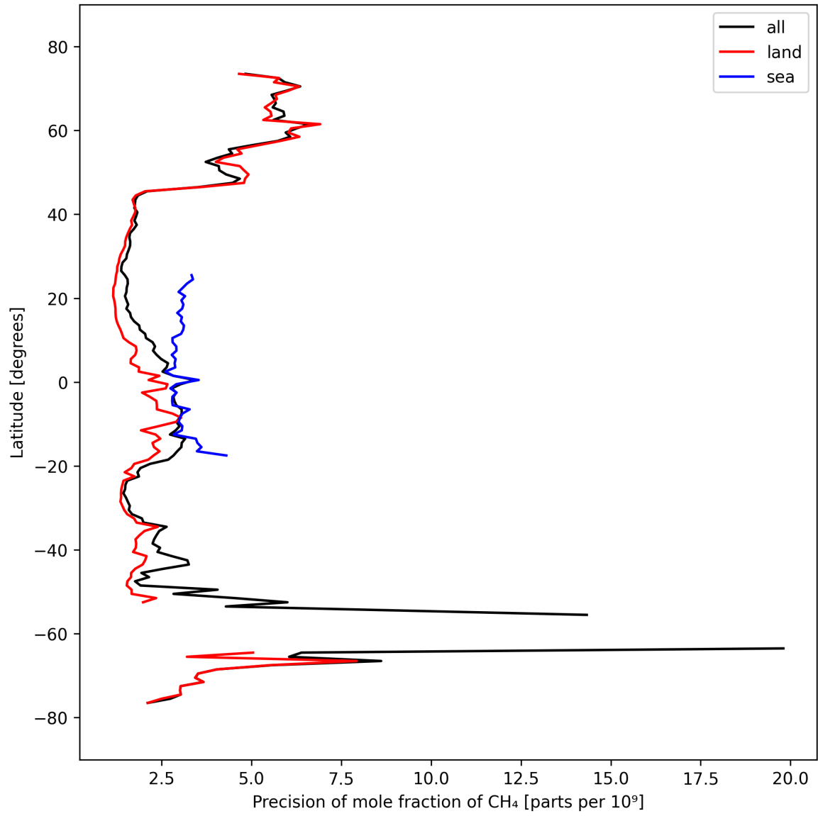
Figure 13: Zonal average of “Precision of mole fraction of CH 4 ” for 2025-03-15 to 2025-03-17.
