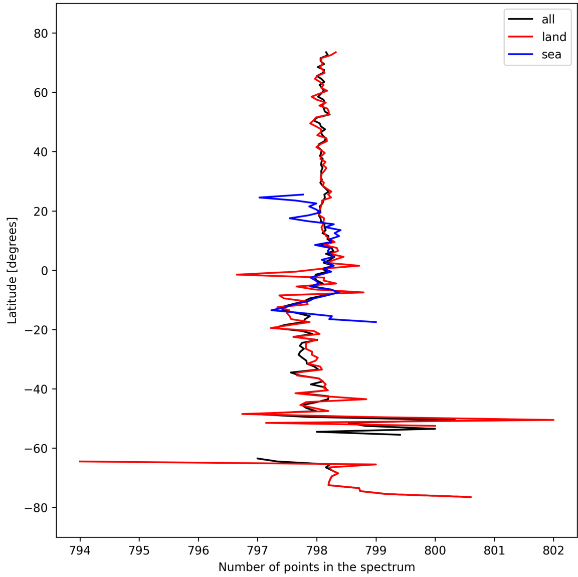
Figure 15: Zonal average of “Number of points in the spectrum” for 2025-03-15 to 2025-03-17.
