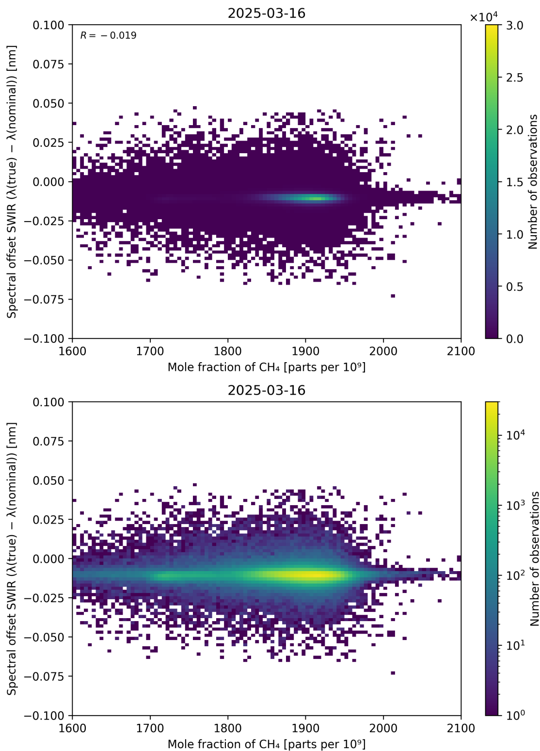
Figure 86: Scatter density plot of “Mole fraction of CH 4 ” against “Spectral offset SWIR ( \lambda_{\text{true}} - \lambda_{\text{nominal}} )” for 2025-03-15 to 2025-03-17.
