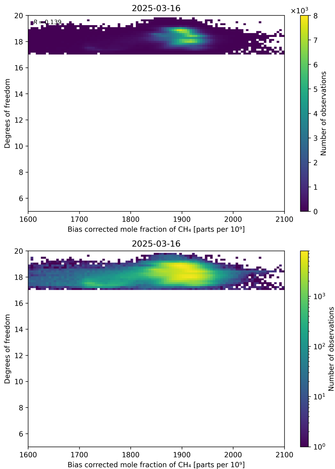
Figure 65: Scatter density plot of “Bias corrected mole fraction of CH 4 ” against “Degrees of freedom” for 2025-03-15 to 2025-03-17.
