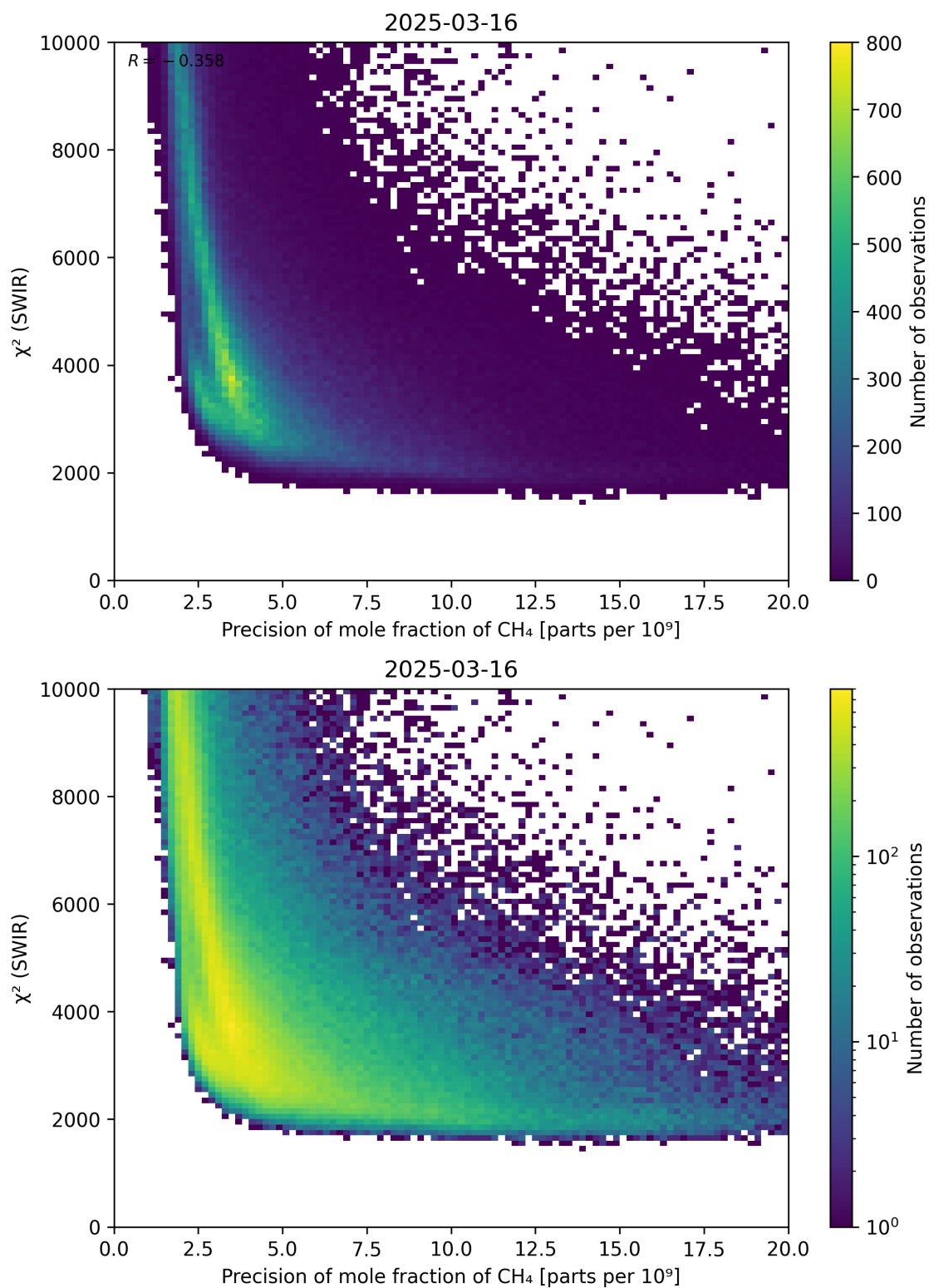
Figure 79: Scatter density plot of “Precision of mole fraction of \text{CH}_4 ” against “ \chi^2 (SWIR)” for 2025-03-15 to 2025-03-17.
