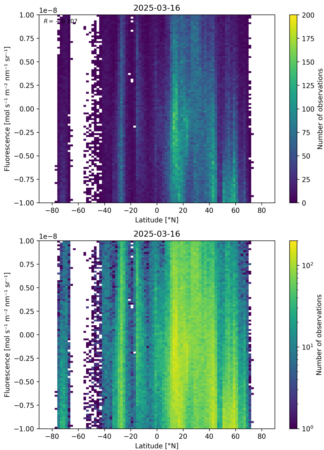
Figure 56: Scatter density plot of “Latitude” against “Fluorescence” for 2025-03-15 to 2025-03-17.
