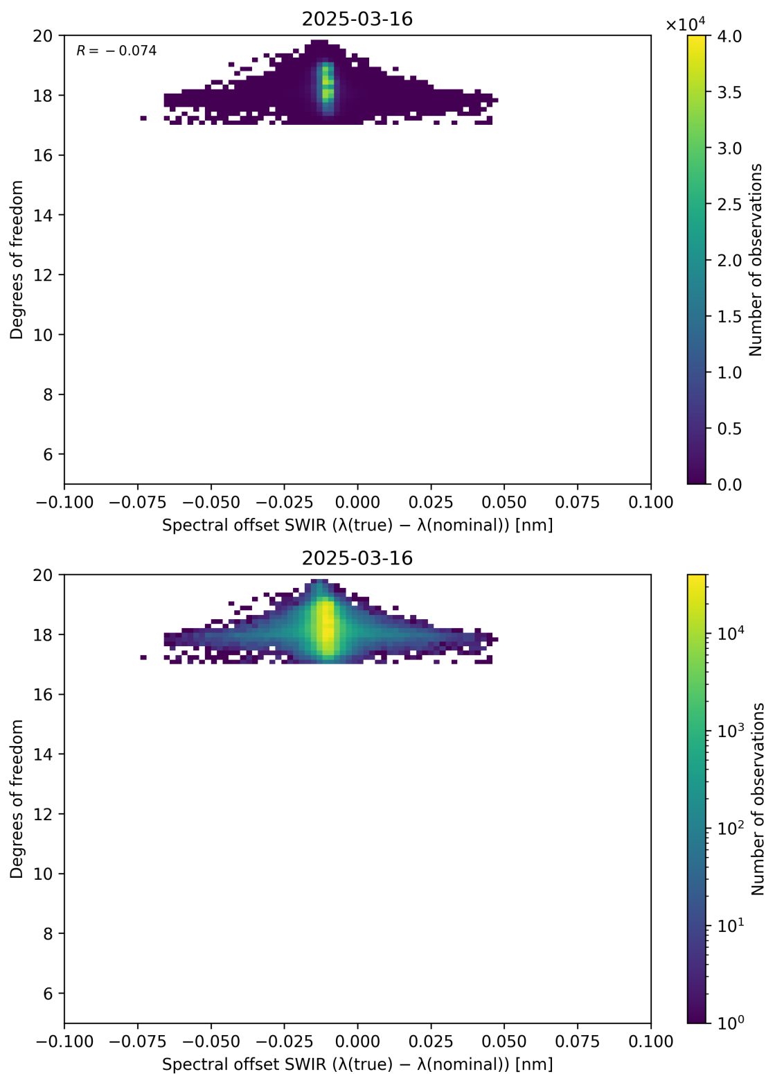
Figure 119: Scatter density plot of “Spectral offset SWIR ( \lambda_{\text{true}} - \lambda_{\text{nominal}} )” against “Degrees of freedom” for 2025-03-15 to 2025-03-17.
