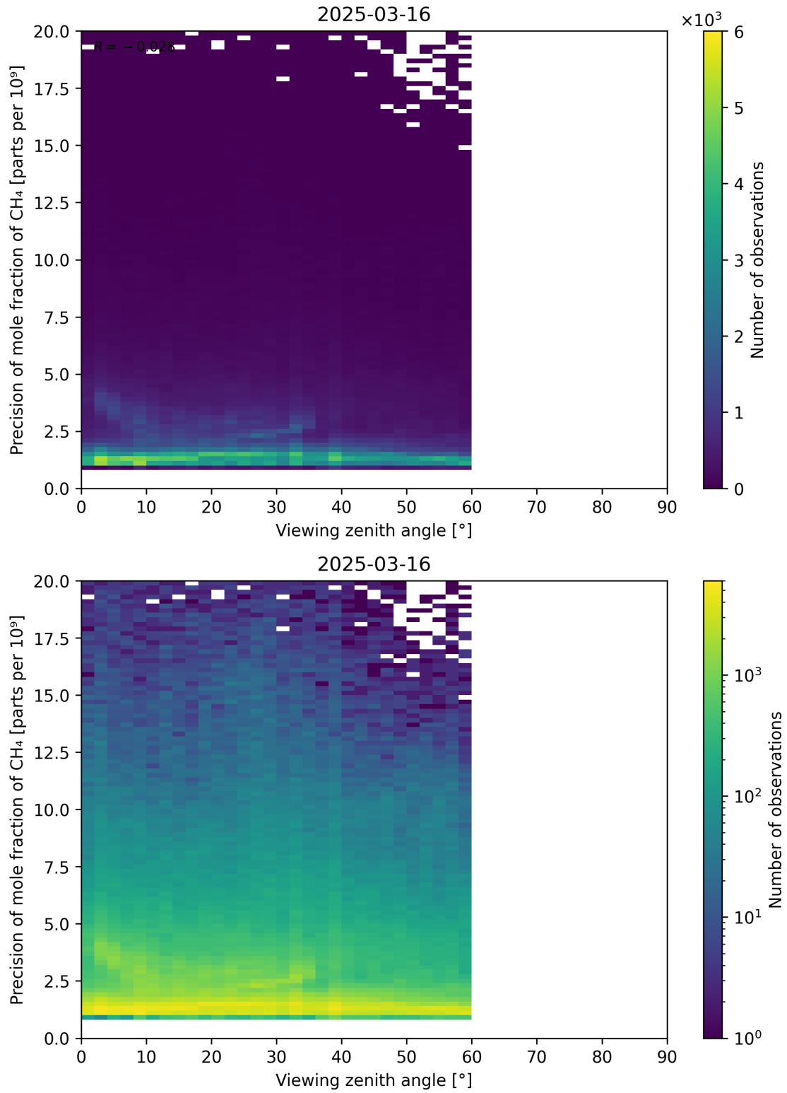
Figure 112: Scatter density plot of “Viewing zenith angle” against “Precision of mole fraction of CH 4 ” for 2025-03-15 to 2025-03-17.
