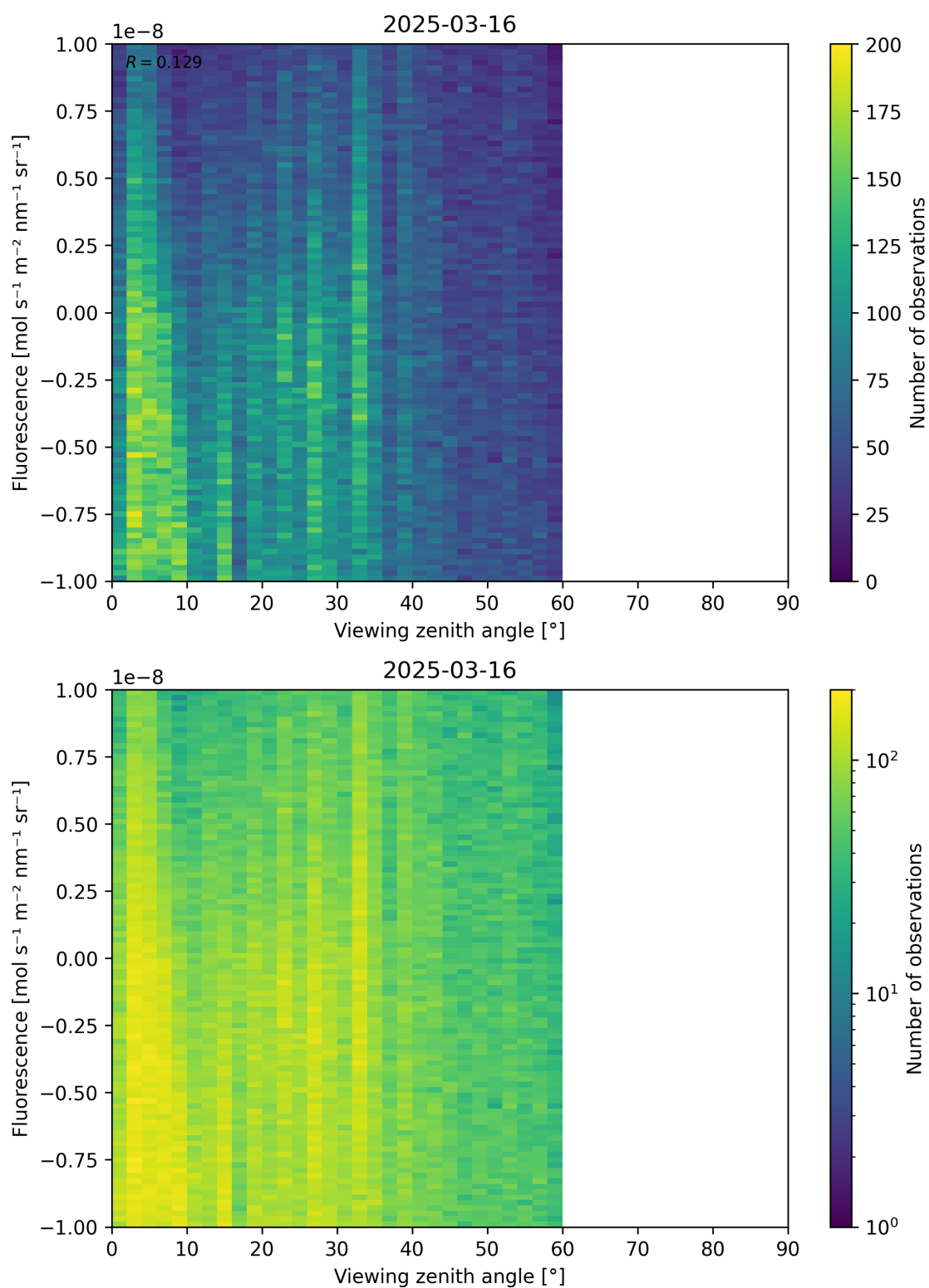
Figure 108: Scatter density plot of “Viewing zenith angle” against “Fluorescence” for 2025-03-15 to 2025-03-17.
