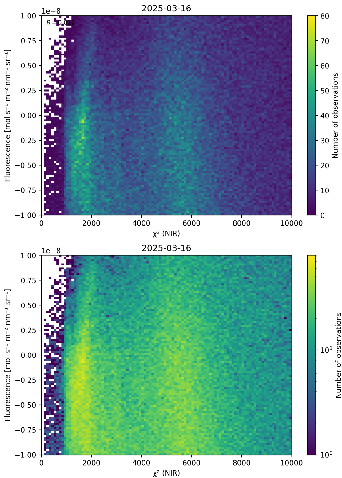
Figure 45: Scatter density plot of “ \chi^2 (NIR)” against “Fluorescence” for 2025-03-15 to 2025-03-17.
