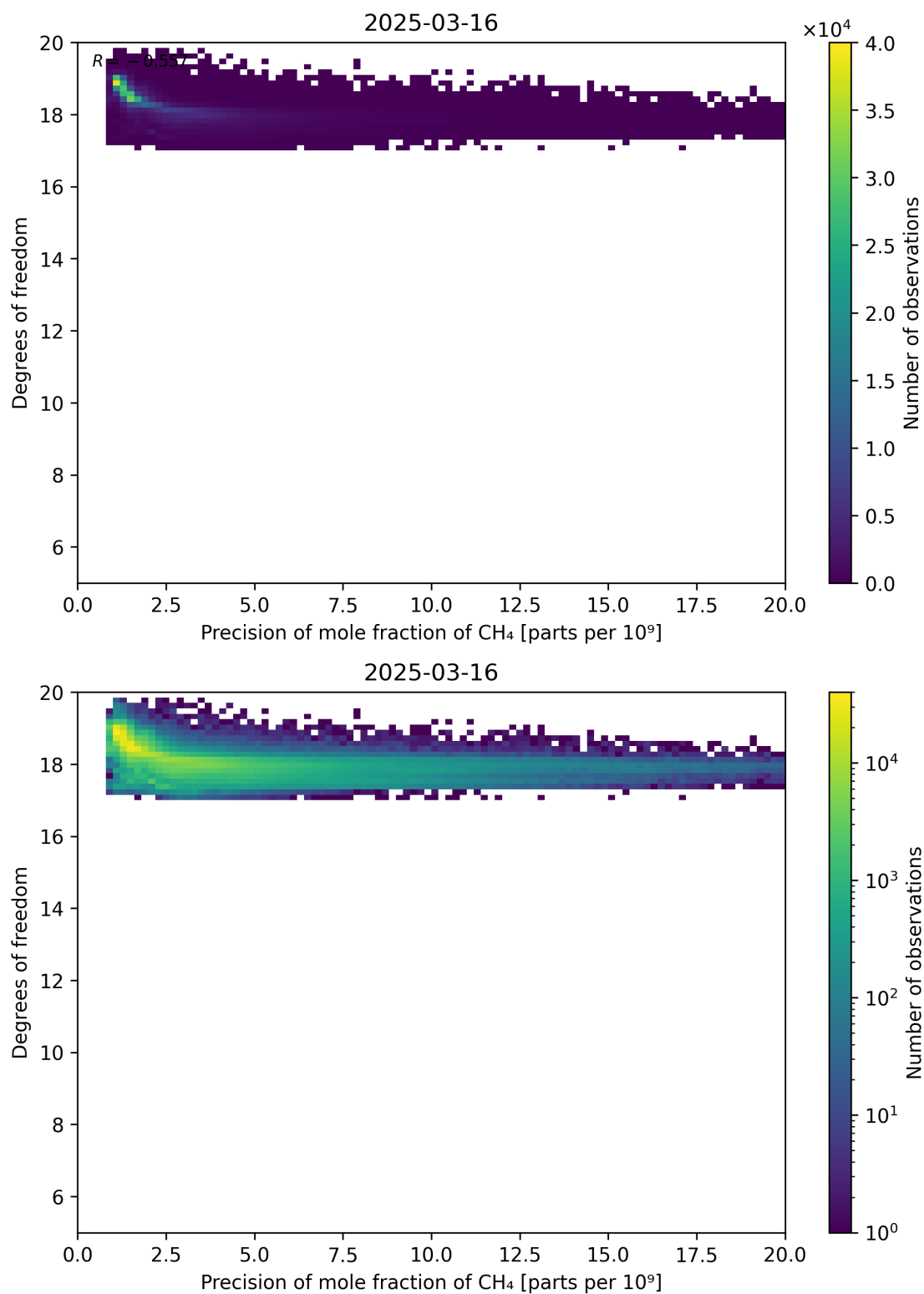
Figure 80: Scatter density plot of “Precision of mole fraction of CH 4 ” against “Degrees of freedom” for 2025-03-15 to 2025-03-17.
