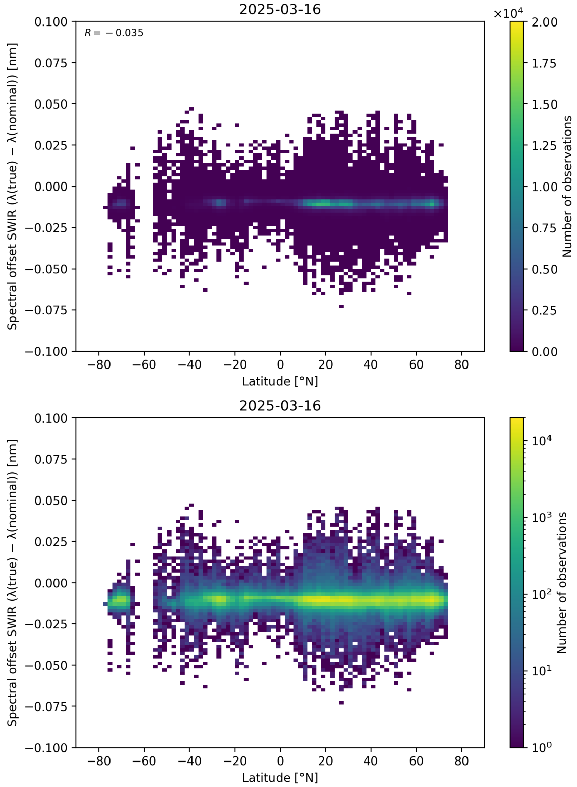
Figure 62: Scatter density plot of “Latitude” against “Spectral offset SWIR ( \lambda_{\text{true}} - \lambda_{\text{nominal}} )” for 2025-03-15 to 2025-03-17.
