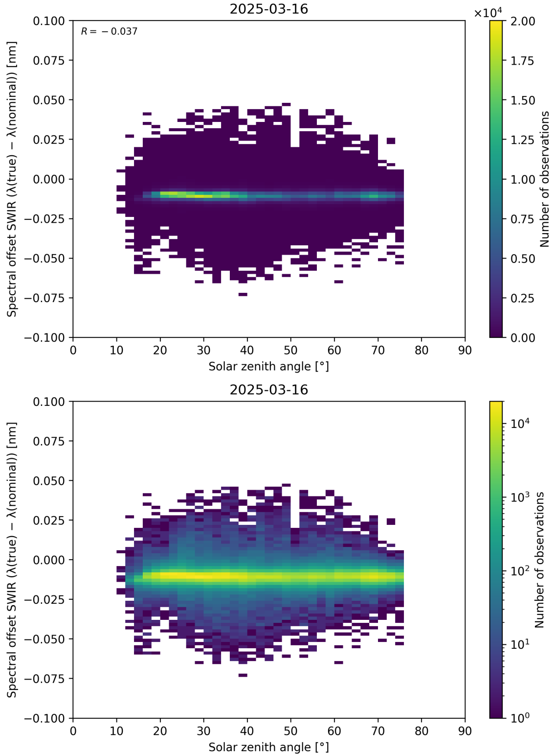
Figure 104: Scatter density plot of “Solar zenith angle” against “Spectral offset SWIR ( \lambda_{\text{true}} - \lambda_{\text{nominal}} )” for 2025-03-15 to 2025-03-17.
