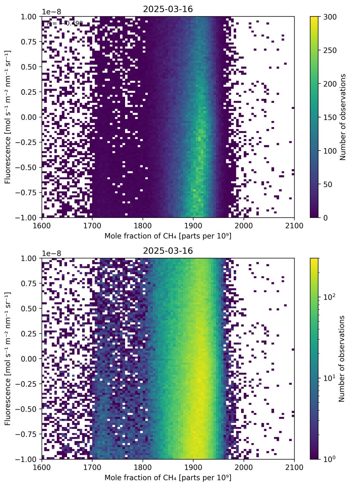
Figure 73: Scatter density plot of “Mole fraction of \text{CH}_4 ” against “Fluorescence” for 2025-03-15 to 2025-03-17.
