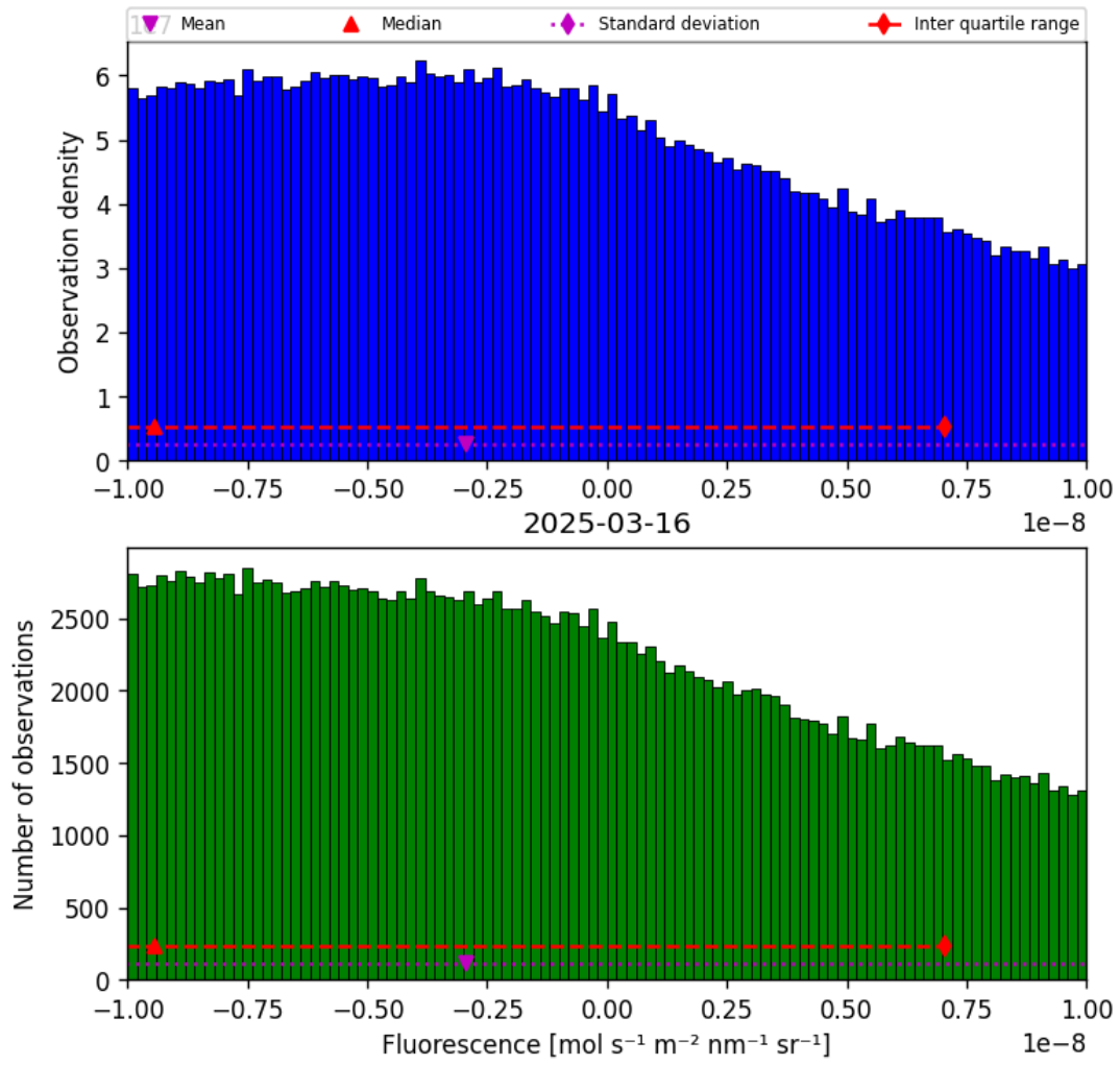
Figure 32: Histogram of “Fluorescence” for 2025-03-15 to 2025-03-17
