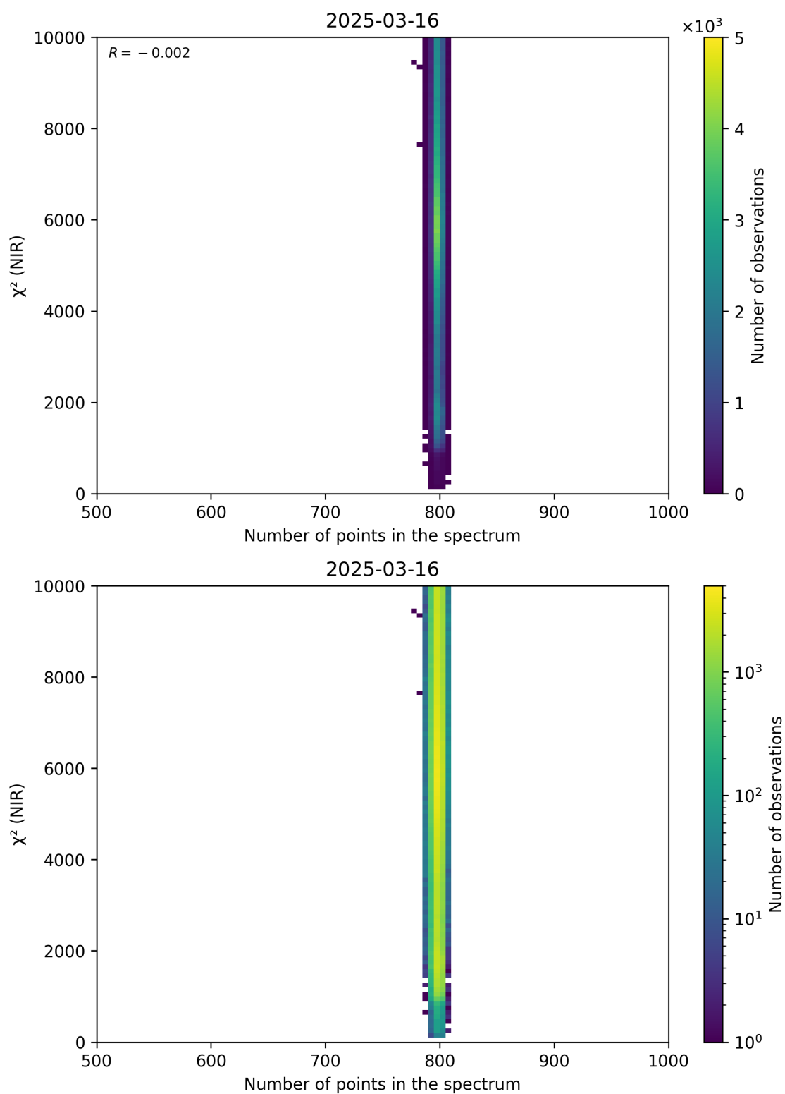
Figure 88: Scatter density plot of “Number of points in the spectrum” against “ \chi^2 (NIR)” for 2025-03-15 to 2025-03-17.
