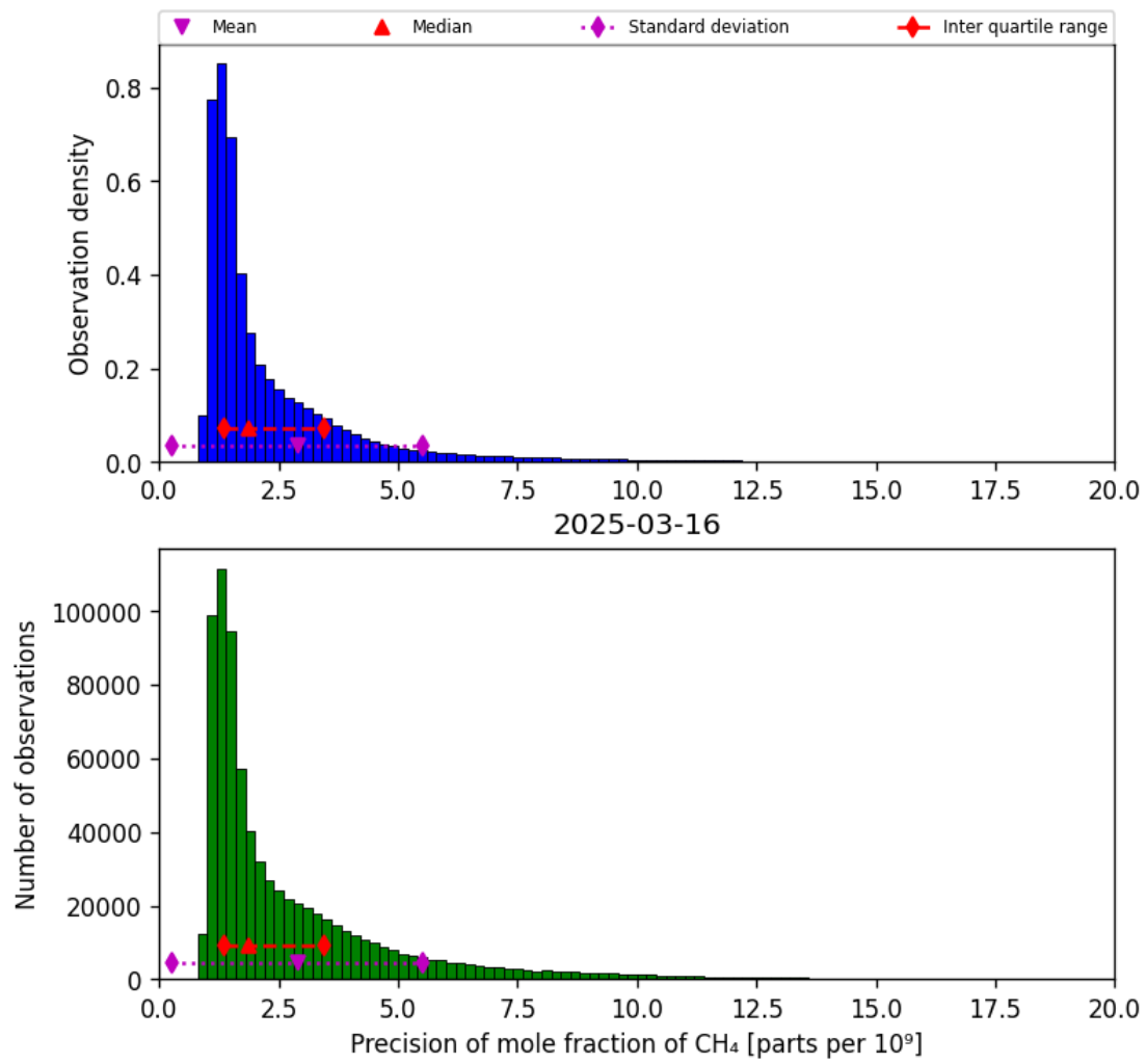
Figure 24: Histogram of “Precision of mole fraction of CH 4 ” for 2025-03-15 to 2025-03-17
