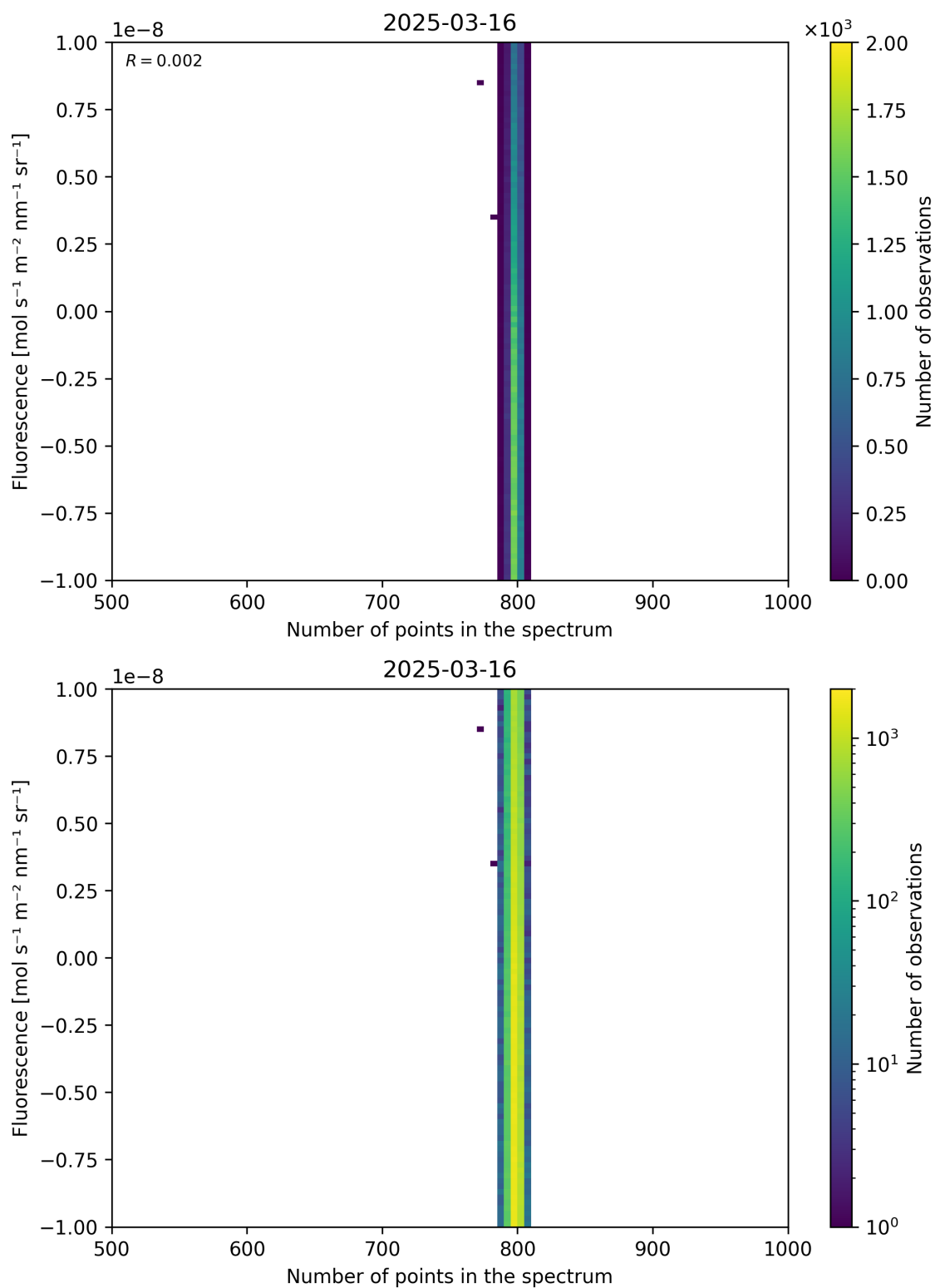
Figure 91: Scatter density plot of “Number of points in the spectrum” against “Fluorescence” for 2025-03-15 to 2025-03-17.
