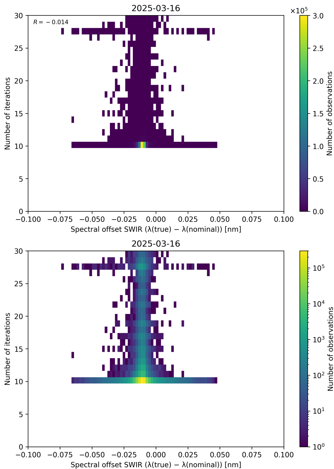
Figure 121: Scatter density plot of “Spectral offset SWIR ( \lambda_{\text{true}} - \lambda_{\text{nominal}} )” against “Number of iterations” for 2025-03-15 to 2025-03-17.
