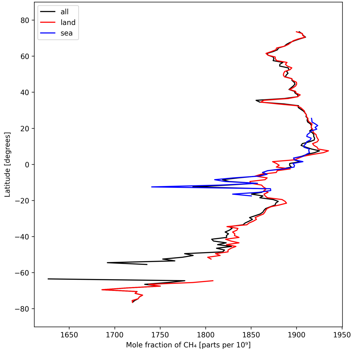
Figure 12: Zonal average of “Mole fraction of \text{CH}_4 ” for 2025-03-15 to 2025-03-17.
