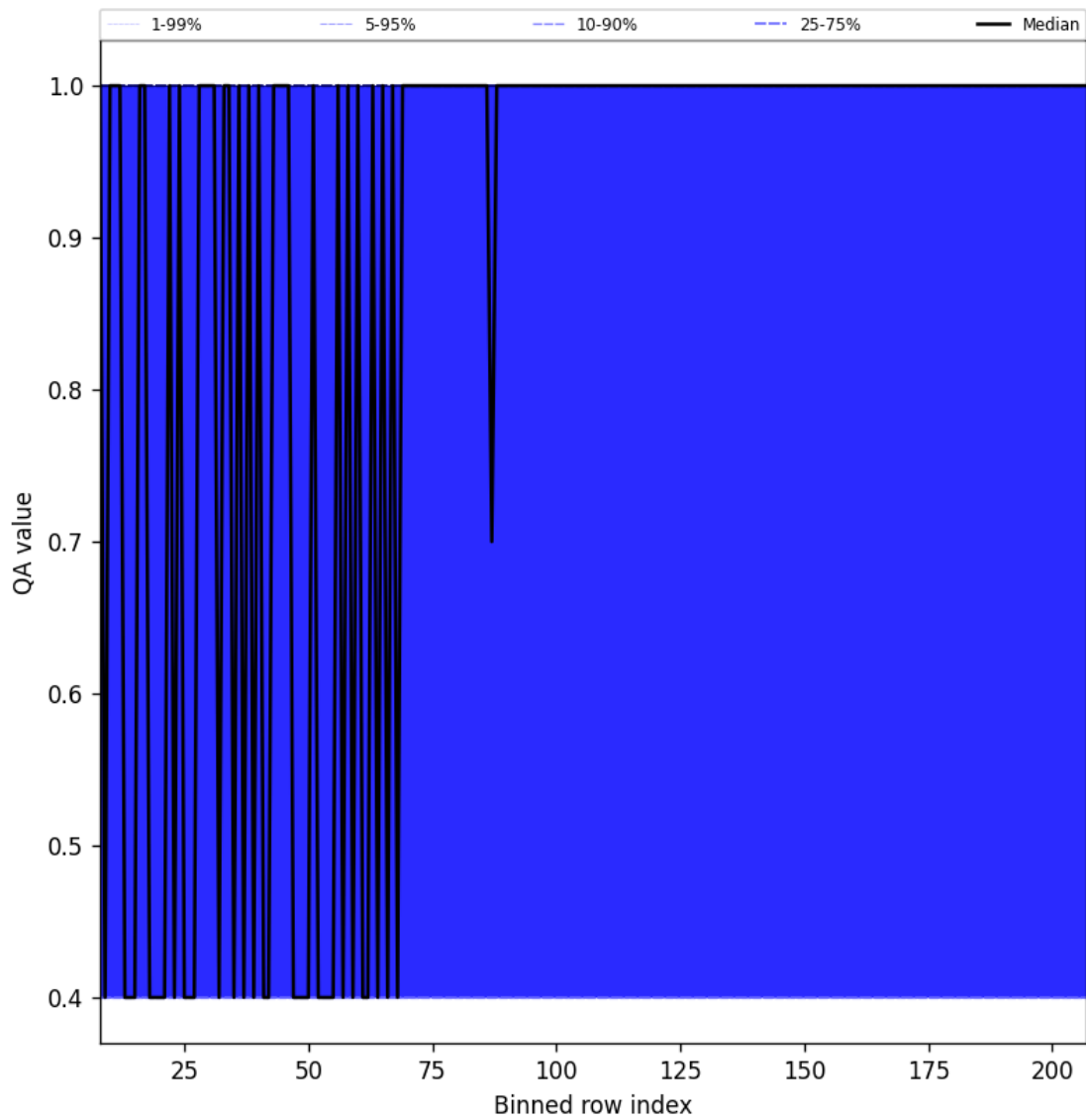
Figure 33: Along track statistics of “QA value” for 2025-03-15 to 2025-03-17
