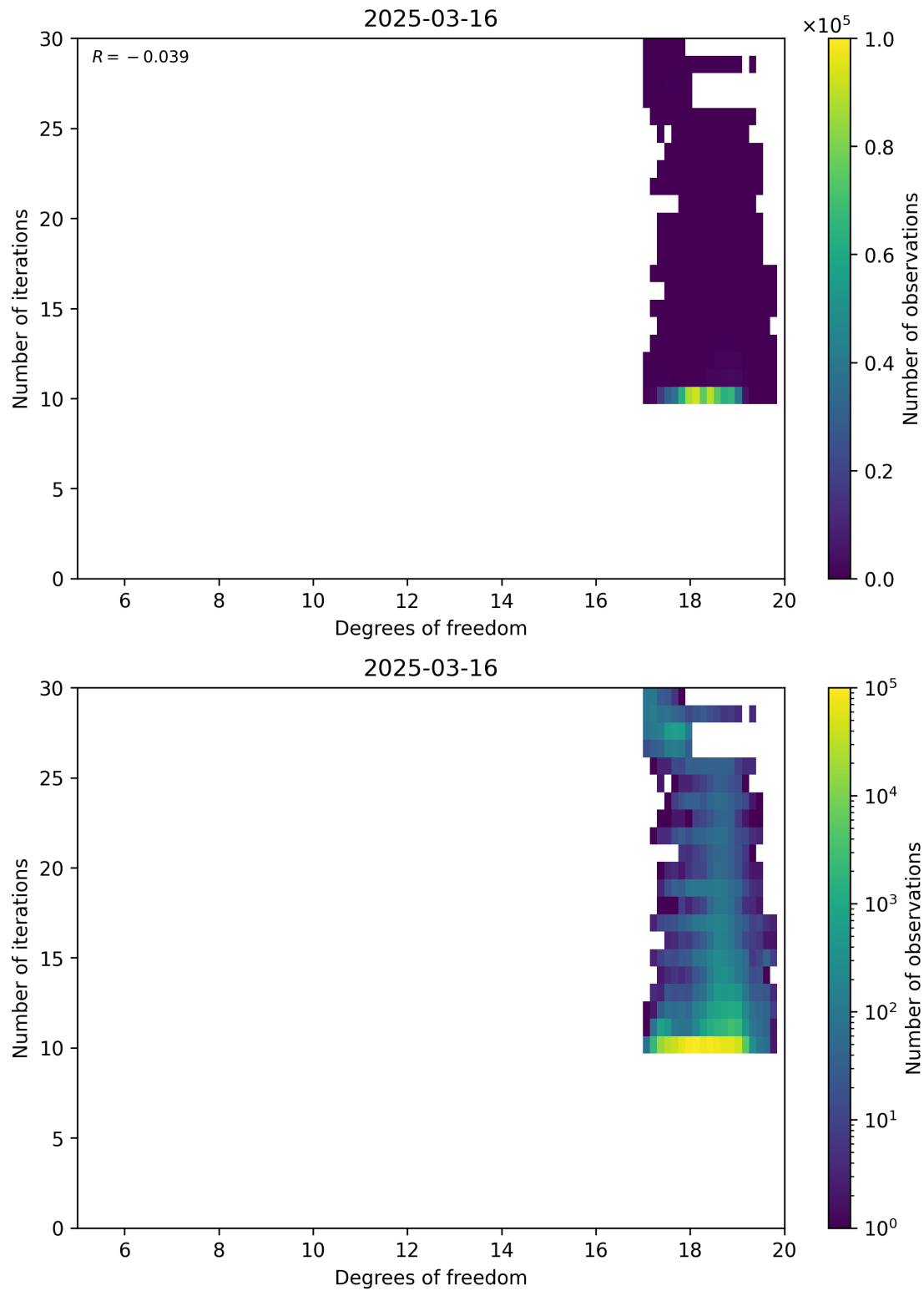
Figure 52: Scatter density plot of “Degrees of freedom” against “Number of iterations” for 2025-03-15 to 2025-03-17.
