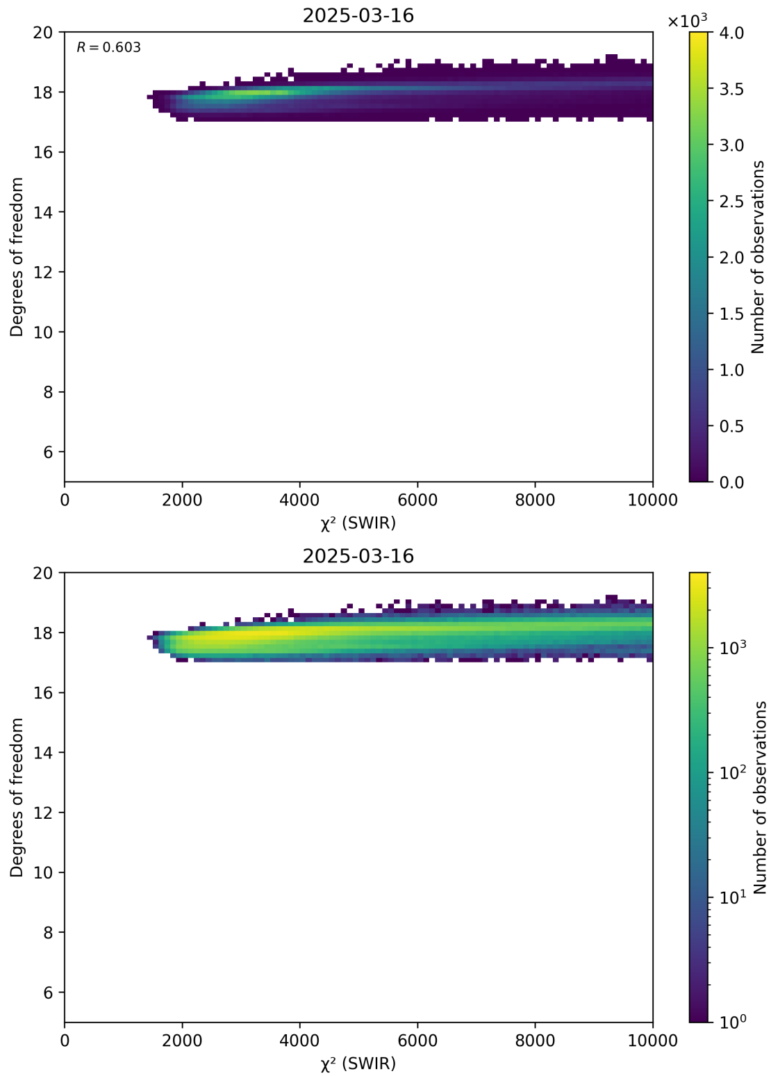
Figure 48: Scatter density plot of “ \chi^2 (SWIR)” against “Degrees of freedom” for 2025-03-15 to 2025-03-17.
