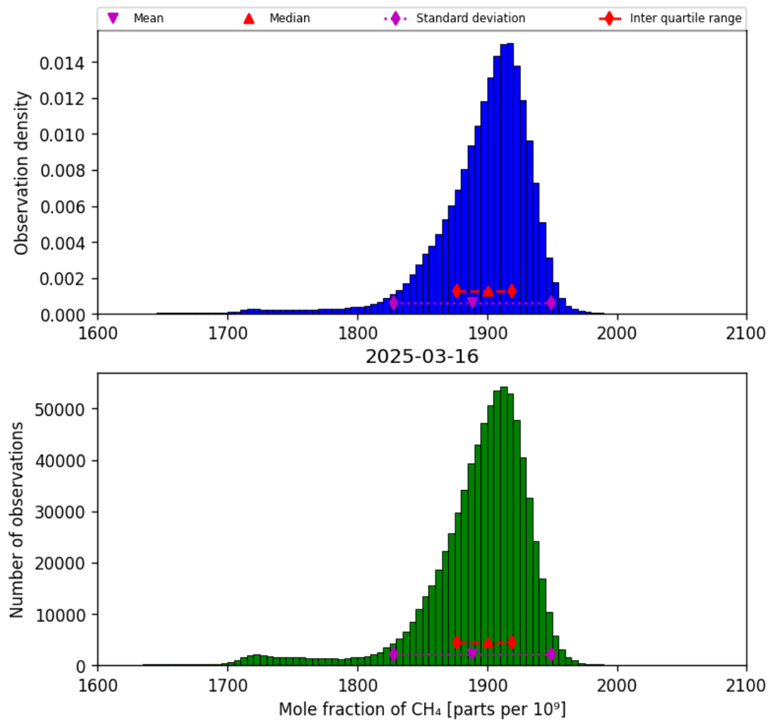
Figure 23: Histogram of “Mole fraction of CH 4 ” for 2025-03-15 to 2025-03-17
