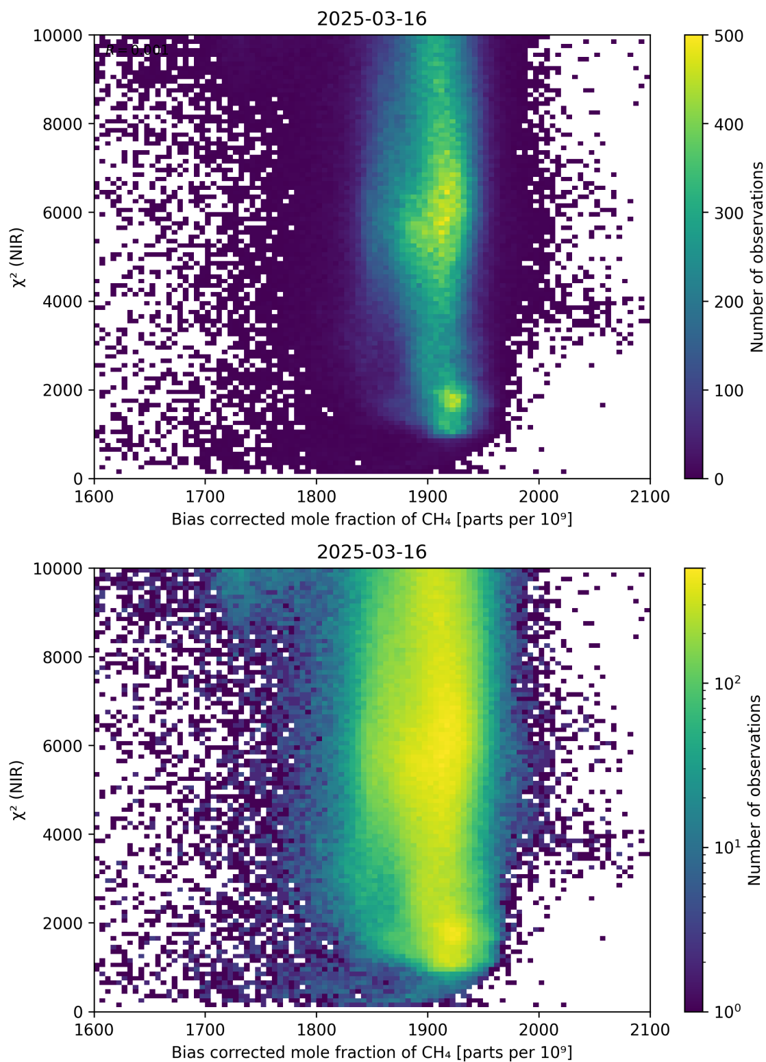
Figure 63: Scatter density plot of “Bias corrected mole fraction of CH 4 ” against “ \chi^2 (NIR)” for 2025-03-15 to 2025-03-17.
