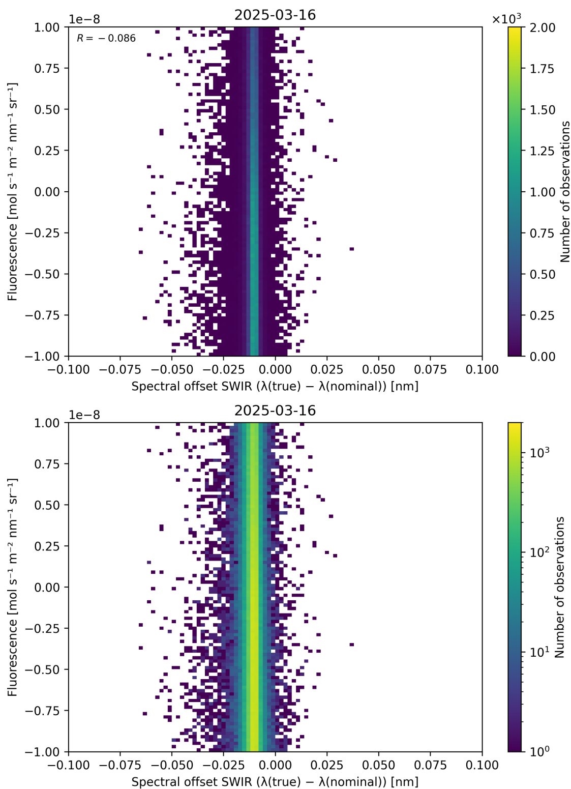
Figure 120: Scatter density plot of “Spectral offset SWIR ( \lambda_{\text{true}} - \lambda_{\text{nominal}} )” against “Fluorescence” for 2025-03-15 to 2025-03-17.
