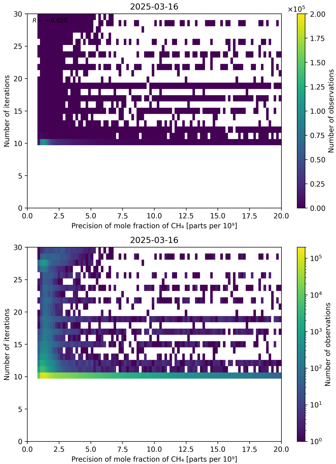
Figure 83: Scatter density plot of “Precision of mole fraction of CH 4 ” against “Number of iterations” for 2025-03-15 to 2025-03-17.
