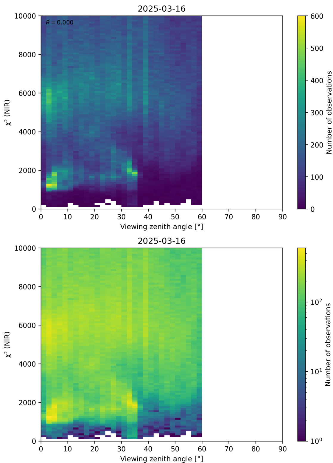
Figure 105: Scatter density plot of “Viewing zenith angle” against “ \chi^2 (NIR)” for 2025-03-15 to 2025-03-17.
