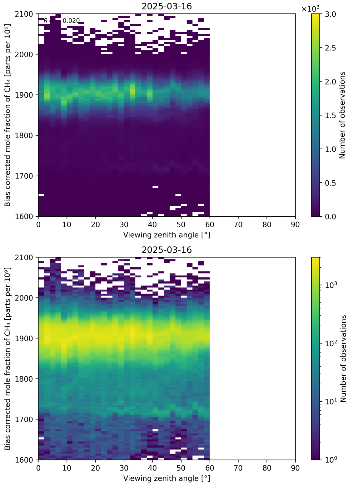
Figure 111: Scatter density plot of “Viewing zenith angle” against “Bias corrected mole fraction of CH 4 ” for 2025-03-15 to 2025-03-17.
