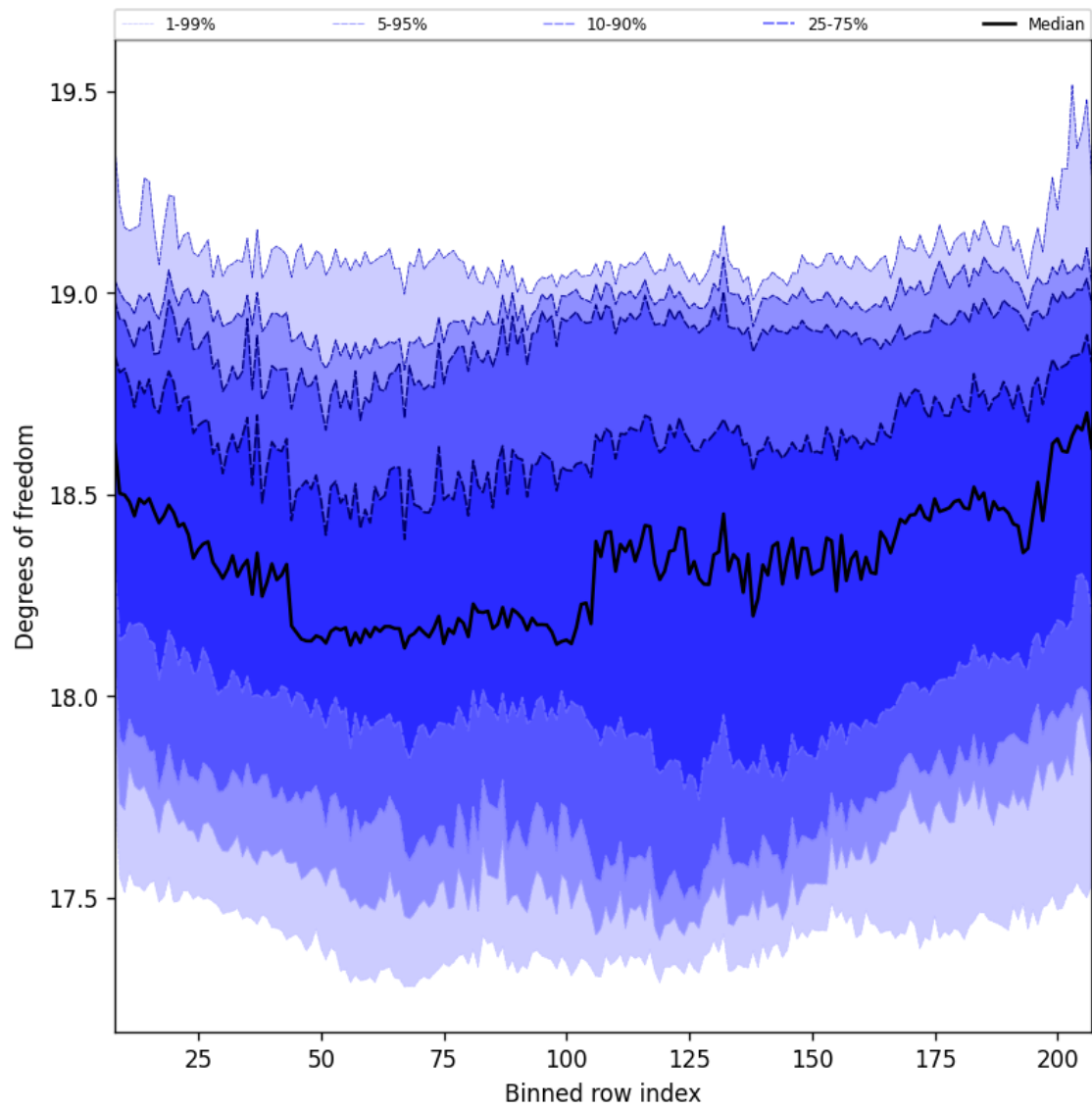
Figure 41: Along track statistics of “Degrees of freedom” for 2025-03-15 to 2025-03-17
