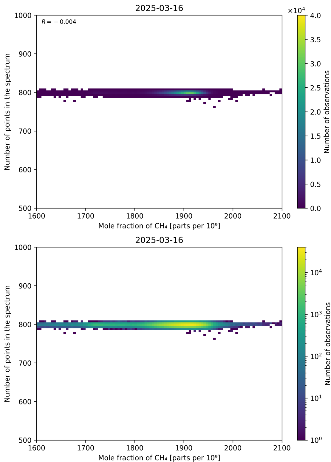
Figure 77: Scatter density plot of “Mole fraction of CH 4 ” against “Number of points in the spectrum” for 2025-03-15 to 2025-03-17.
