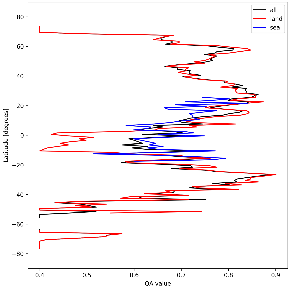
Figure 11: Zonal average of “QA value” for 2025-03-15 to 2025-03-17.
