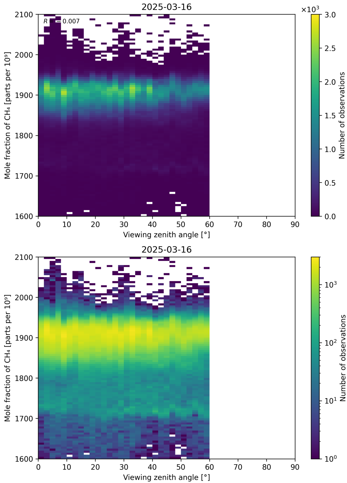
Figure 110: Scatter density plot of “Viewing zenith angle” against “Mole fraction of CH 4 ” for 2025-03-15 to 2025-03-17.
