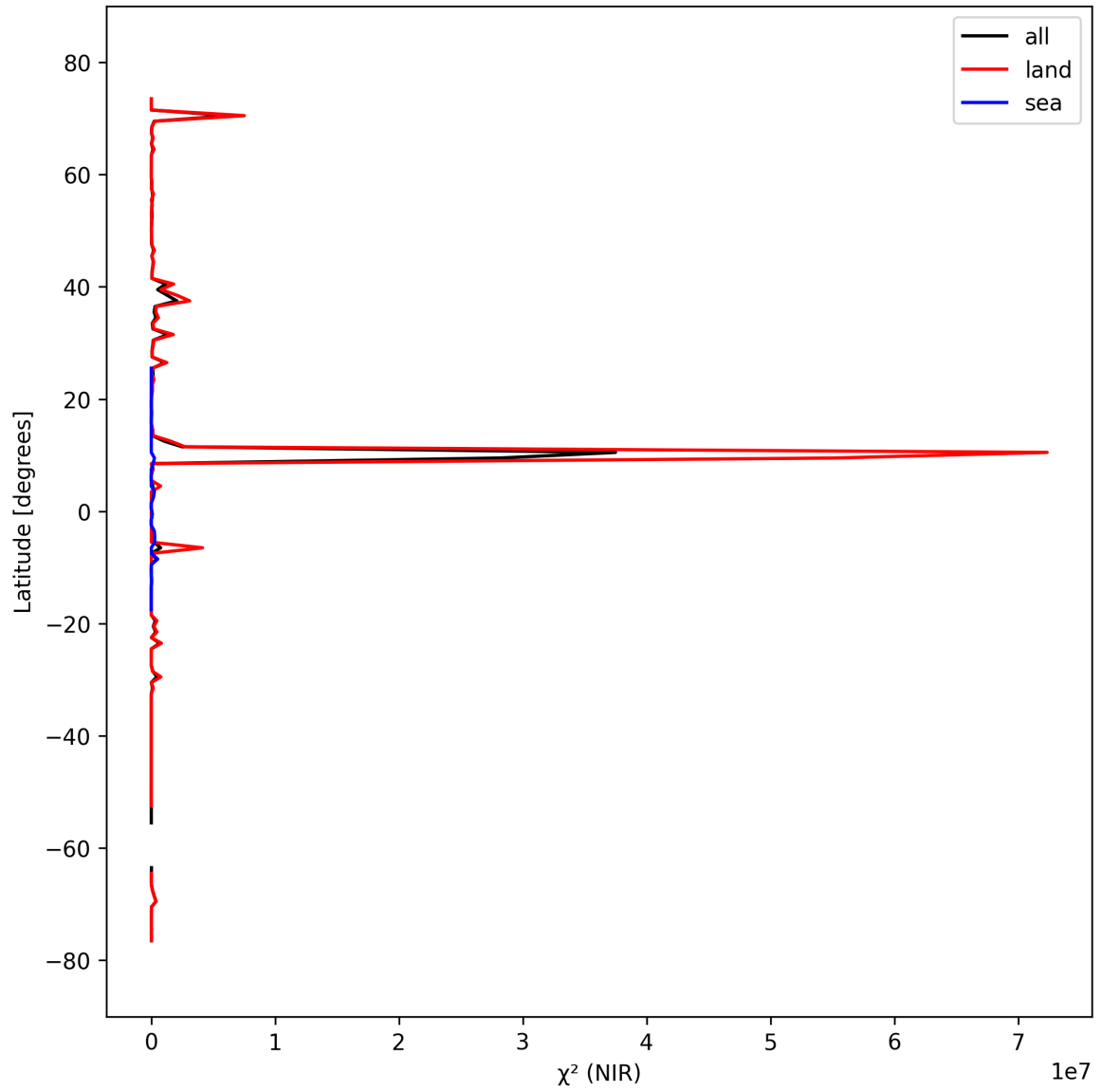
Figure 18: Zonal average of “ \chi^2 (NIR)” for 2025-03-15 to 2025-03-17.
