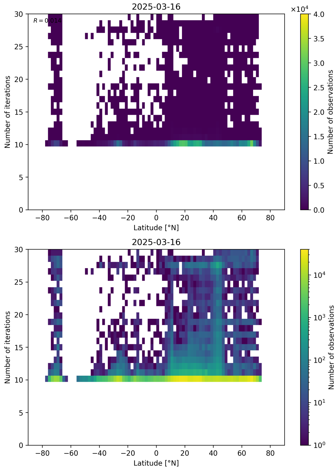
Figure 60: Scatter density plot of “Latitude” against “Number of iterations” for 2025-03-15 to 2025-03-17.
