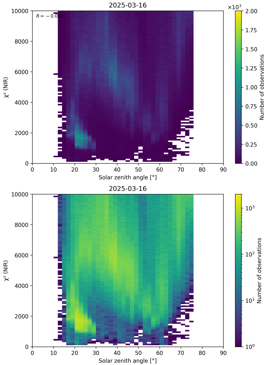
Figure 94: Scatter density plot of “Solar zenith angle” against “ \chi^2 (NIR)” for 2025-03-15 to 2025-03-17.
