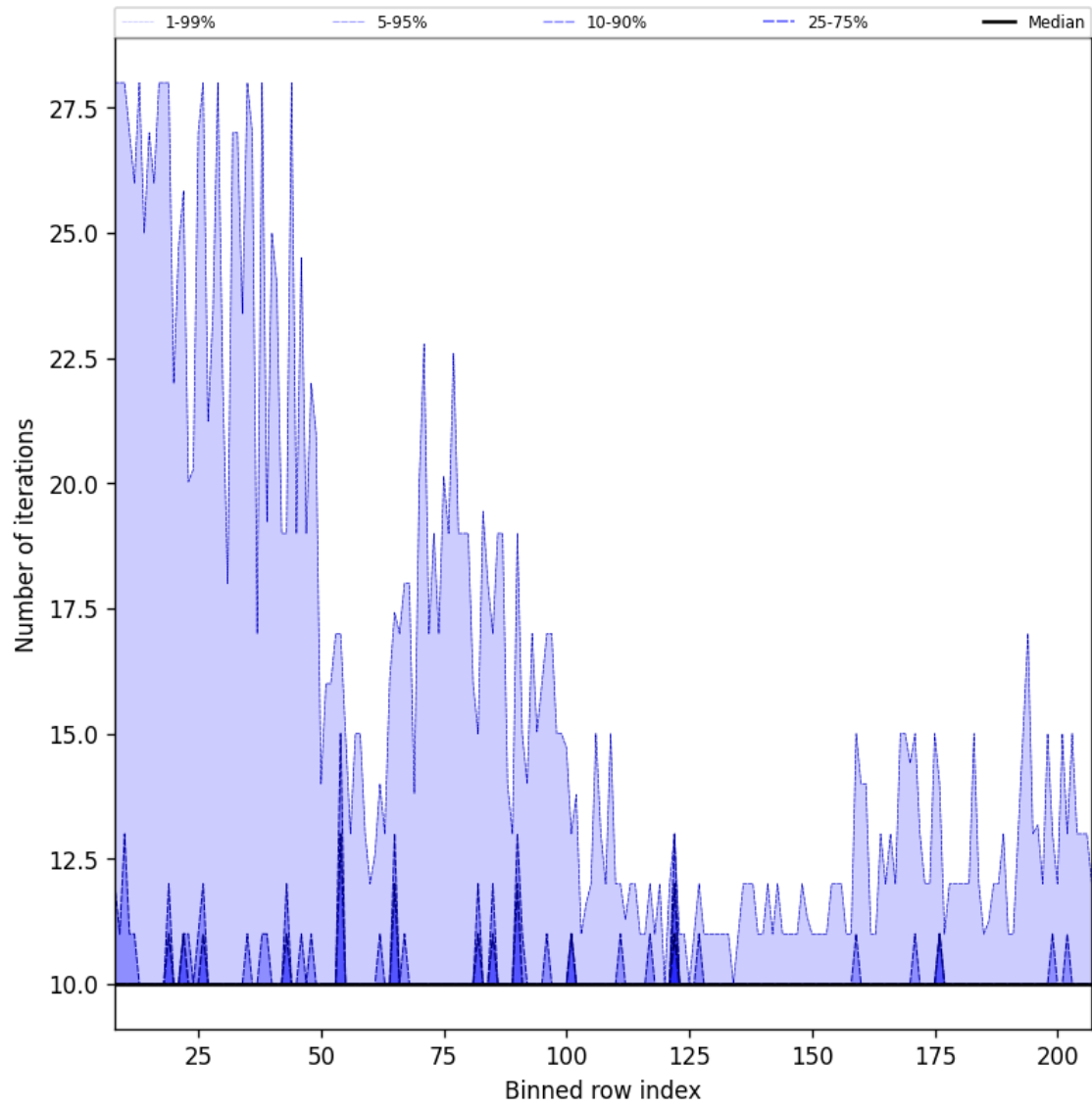
Figure 42: Along track statistics of “Number of iterations” for 2025-03-15 to 2025-03-17
