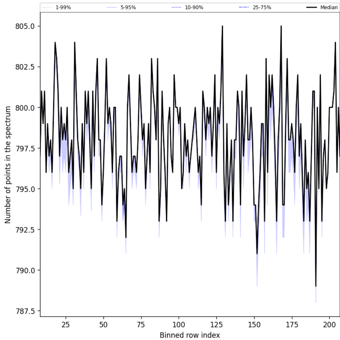
Figure 37: Along track statistics of “Number of points in the spectrum” for 2025-03-15 to 2025-03-17
