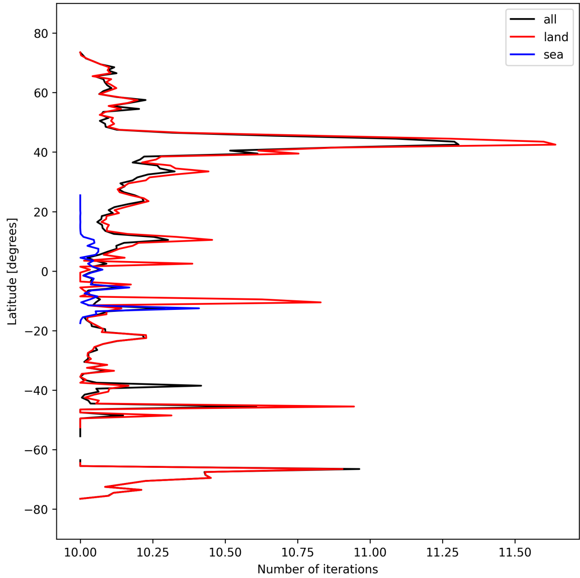
Figure 20: Zonal average of “Number of iterations” for 2025-03-15 to 2025-03-17.
