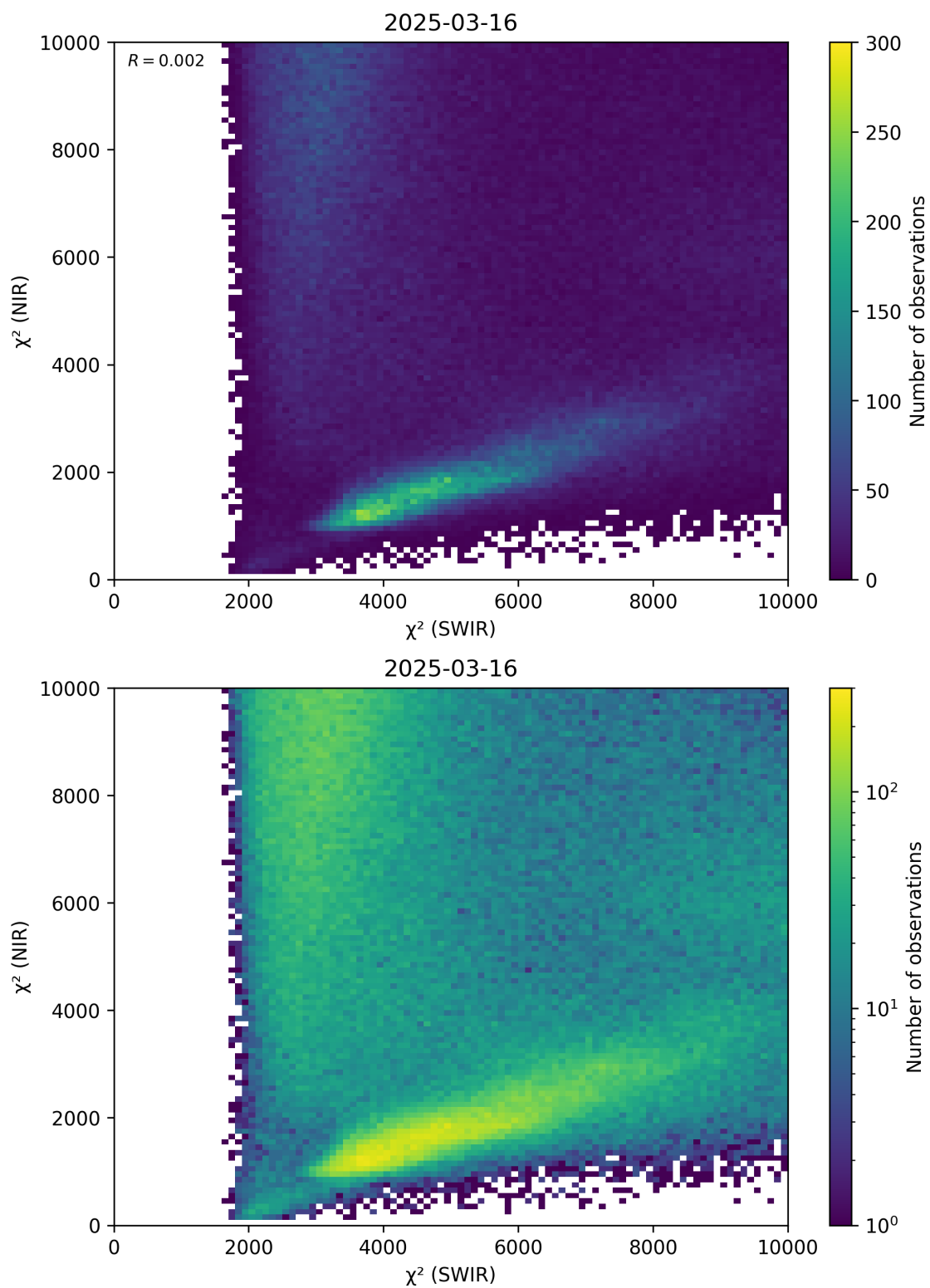
Figure 47: Scatter density plot of “ \chi^2 (SWIR)” against “ \chi^2 (NIR)” for 2025-03-15 to 2025-03-17.
