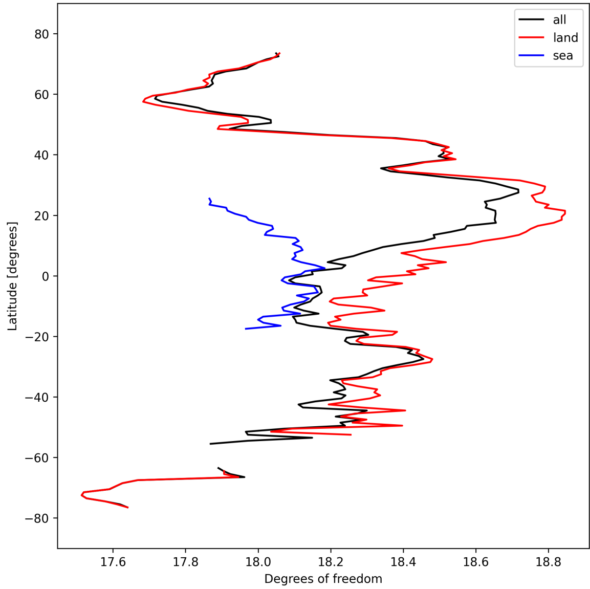
Figure 19: Zonal average of “Degrees of freedom” for 2025-03-15 to 2025-03-17.
