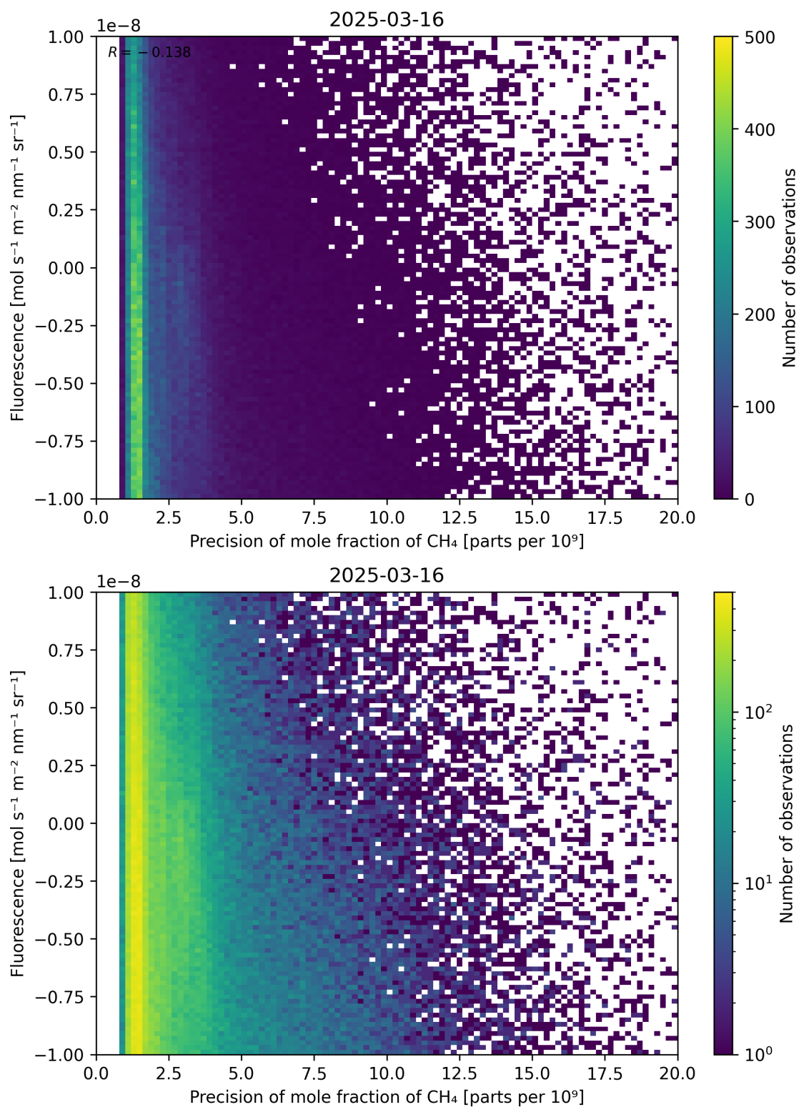
Figure 81: Scatter density plot of “Precision of mole fraction of CH 4 ” against “Fluorescence” for 2025-03-15 to 2025-03-17.
