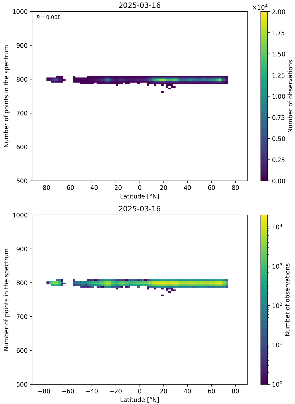
Figure 61: Scatter density plot of “Latitude” against “Number of points in the spectrum” for 2025-03-15 to 2025-03-17.
