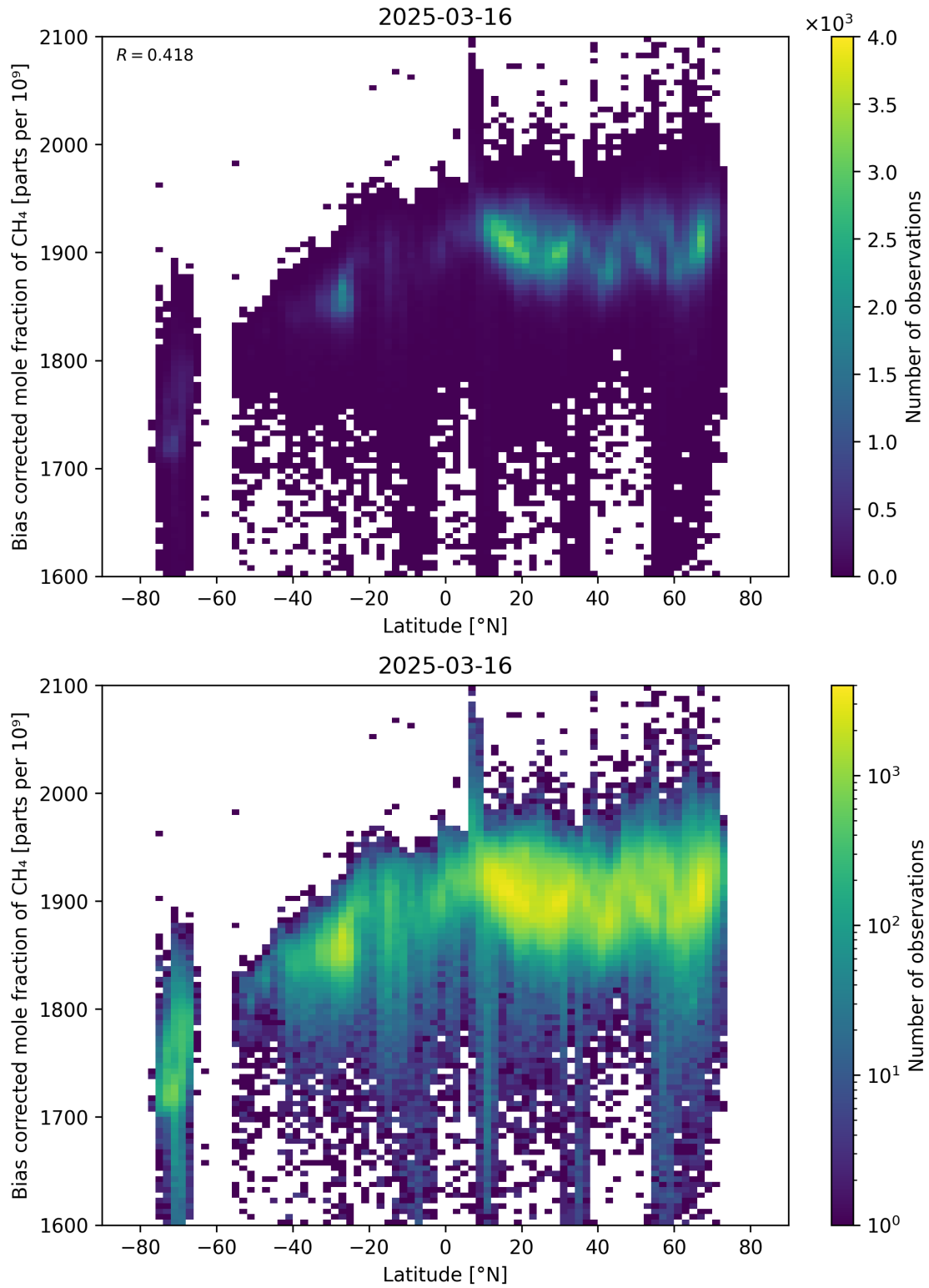
Figure 58: Scatter density plot of “Latitude” against “Bias corrected mole fraction of CH 4 ” for 2025-03-15 to 2025-03-17.
