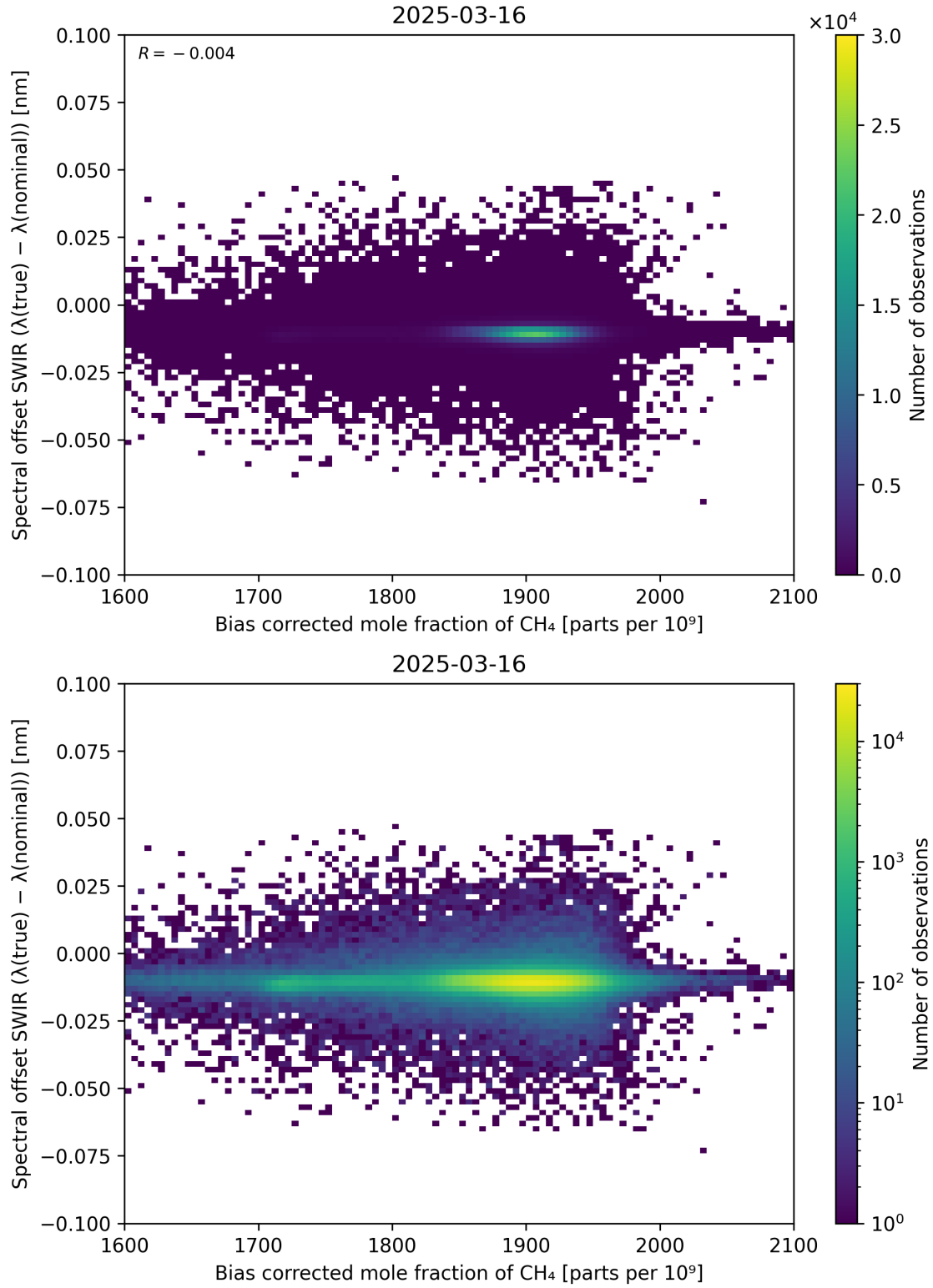
Figure 69: Scatter density plot of “Bias corrected mole fraction of \text{CH}_4 ” against “Spectral offset SWIR ( \lambda_{\text{true}} - \lambda_{\text{nominal}} )” for 2025-03-15 to 2025-03-17.
