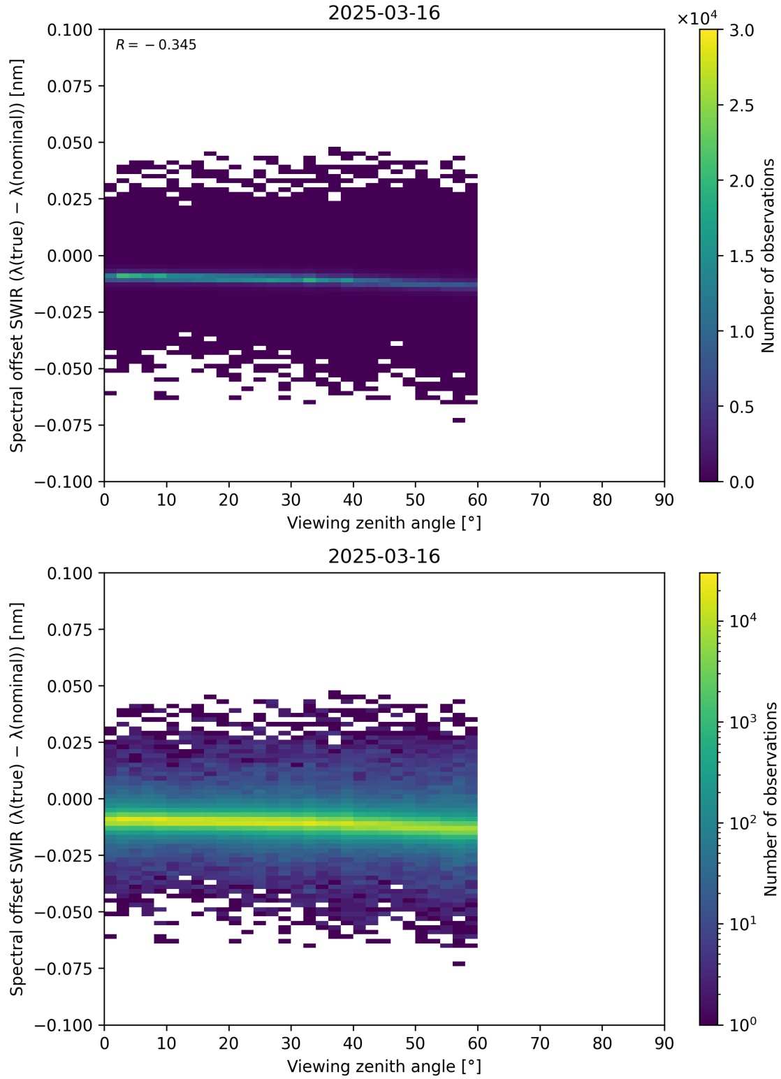
Figure 116: Scatter density plot of “Viewing zenith angle” against “Spectral offset SWIR ( \lambda_{\text{true}} - \lambda_{\text{nominal}} )” for 2025-03-15 to 2025-03-17.
