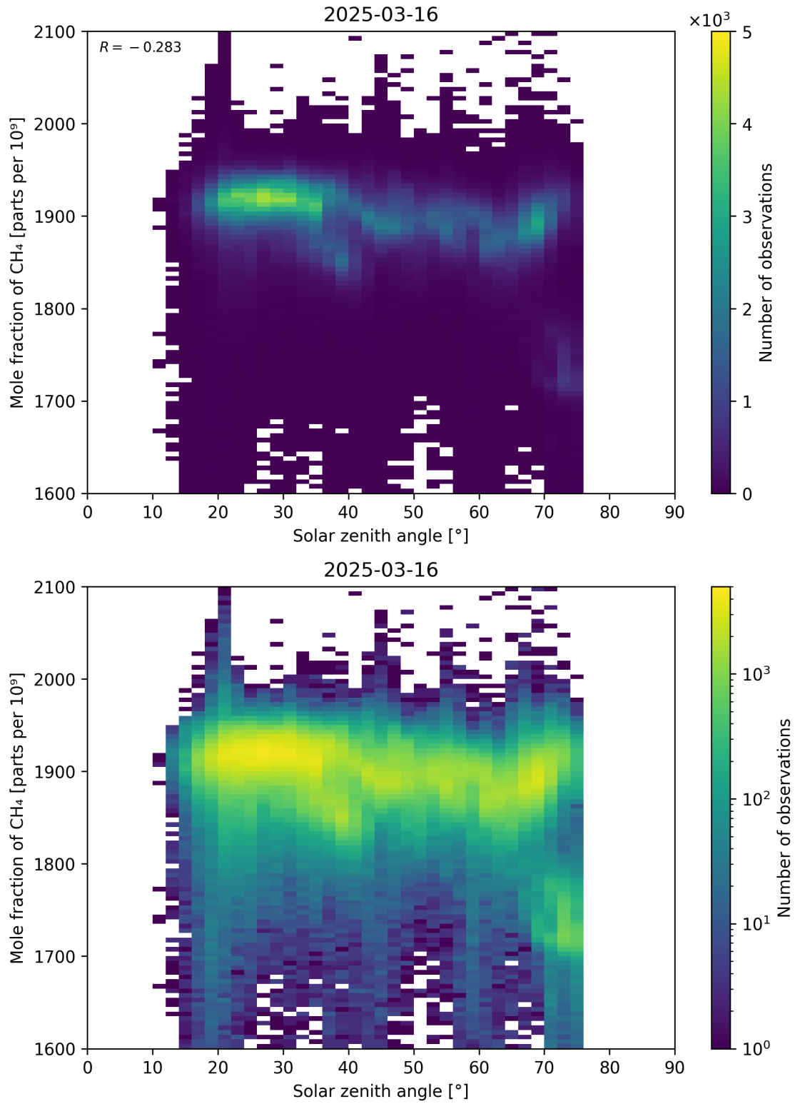
Figure 99: Scatter density plot of “Solar zenith angle” against “Mole fraction of CH 4 ” for 2025-03-15 to 2025-03-17.
