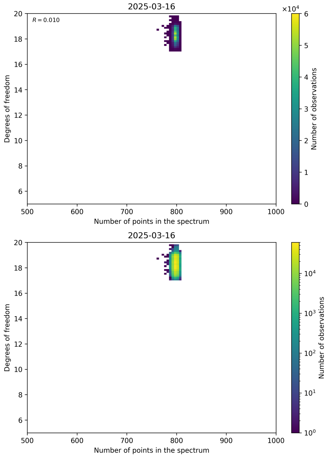
Figure 90: Scatter density plot of “Number of points in the spectrum” against “Degrees of freedom” for 2025-03-15 to 2025-03-17.
