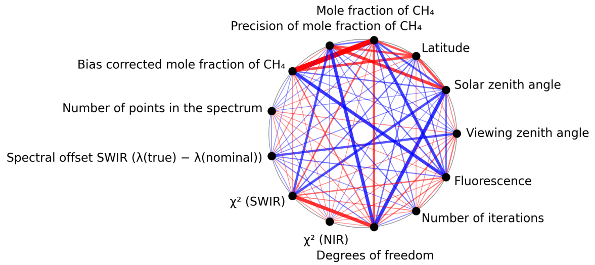
Figure 1: Map of correlation graph for 2025-03-15 to 2025-03-17.
