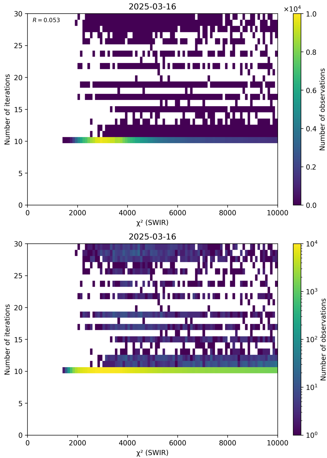
Figure 50: Scatter density plot of “ \chi^2 (SWIR)” against “Number of iterations” for 2025-03-15 to 2025-03-17.
