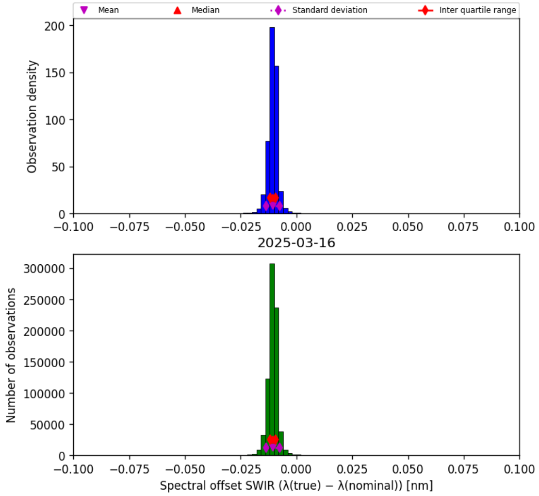
Figure 27: Histogram of “Spectral offset SWIR ( \lambda_{\text{true}} - \lambda_{\text{nominal}} )” for 2025-03-15 to 2025-03-17
