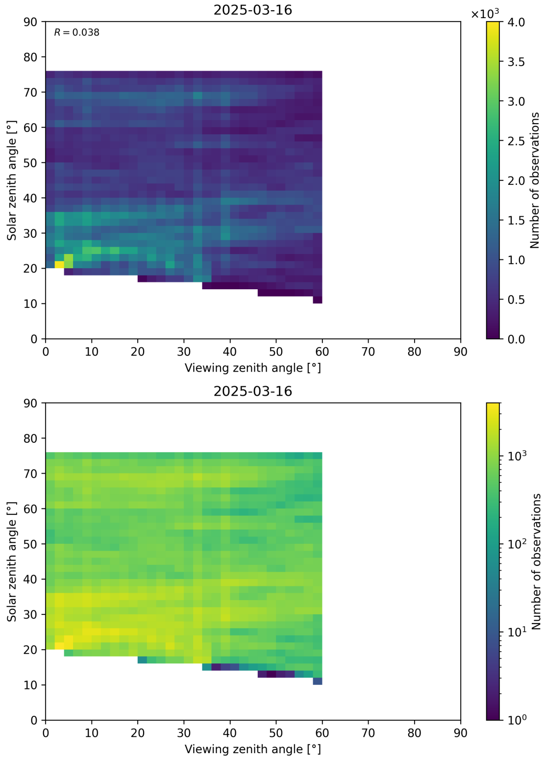
Figure 115: Scatter density plot of “Viewing zenith angle” against “Solar zenith angle” for 2025-03-15 to 2025-03-17.
