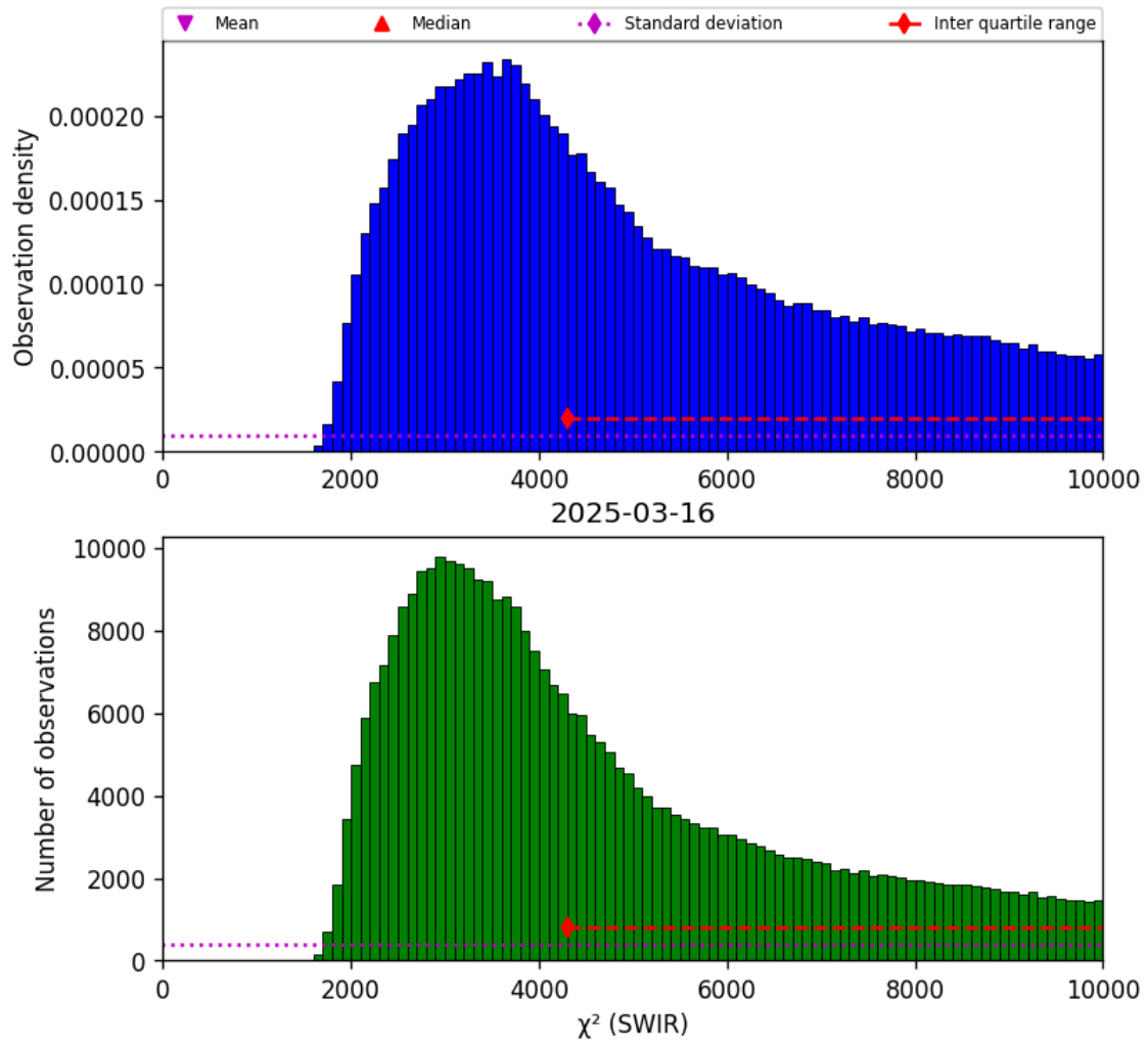
Figure 28: Histogram of " \chi^2 (SWIR)" for 2025-03-15 to 2025-03-17
