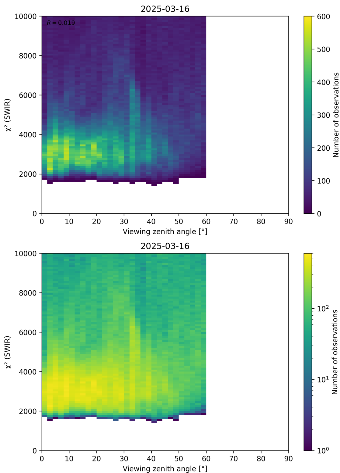
Figure 106: Scatter density plot of “Viewing zenith angle” against “ \chi^2 (SWIR)” for 2025-03-15 to 2025-03-17.
