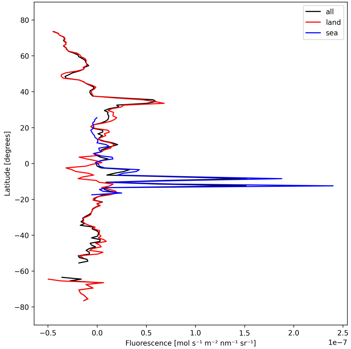
Figure 21: Zonal average of “Fluorescence” for 2025-03-15 to 2025-03-17.
