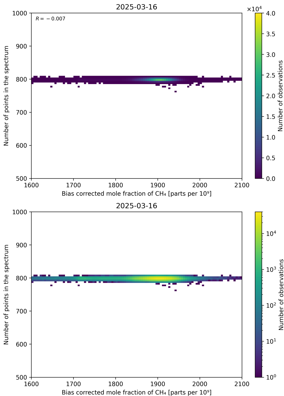
Figure 68: Scatter density plot of “Bias corrected mole fraction of CH 4 ” against “Number of points in the spectrum” for 2025-03-15 to 2025-03-17.
