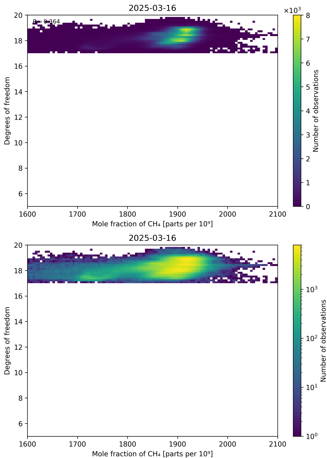
Figure 72: Scatter density plot of “Mole fraction of CH 4 ” against “Degrees of freedom” for 2025-03-15 to 2025-03-17.
