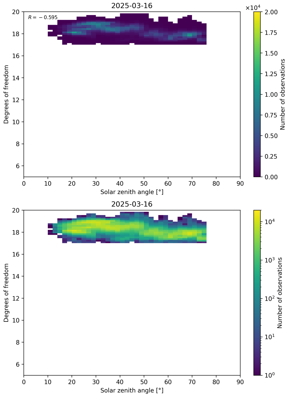
Figure 96: Scatter density plot of “Solar zenith angle” against “Degrees of freedom” for 2025-03-15 to 2025-03-17.
