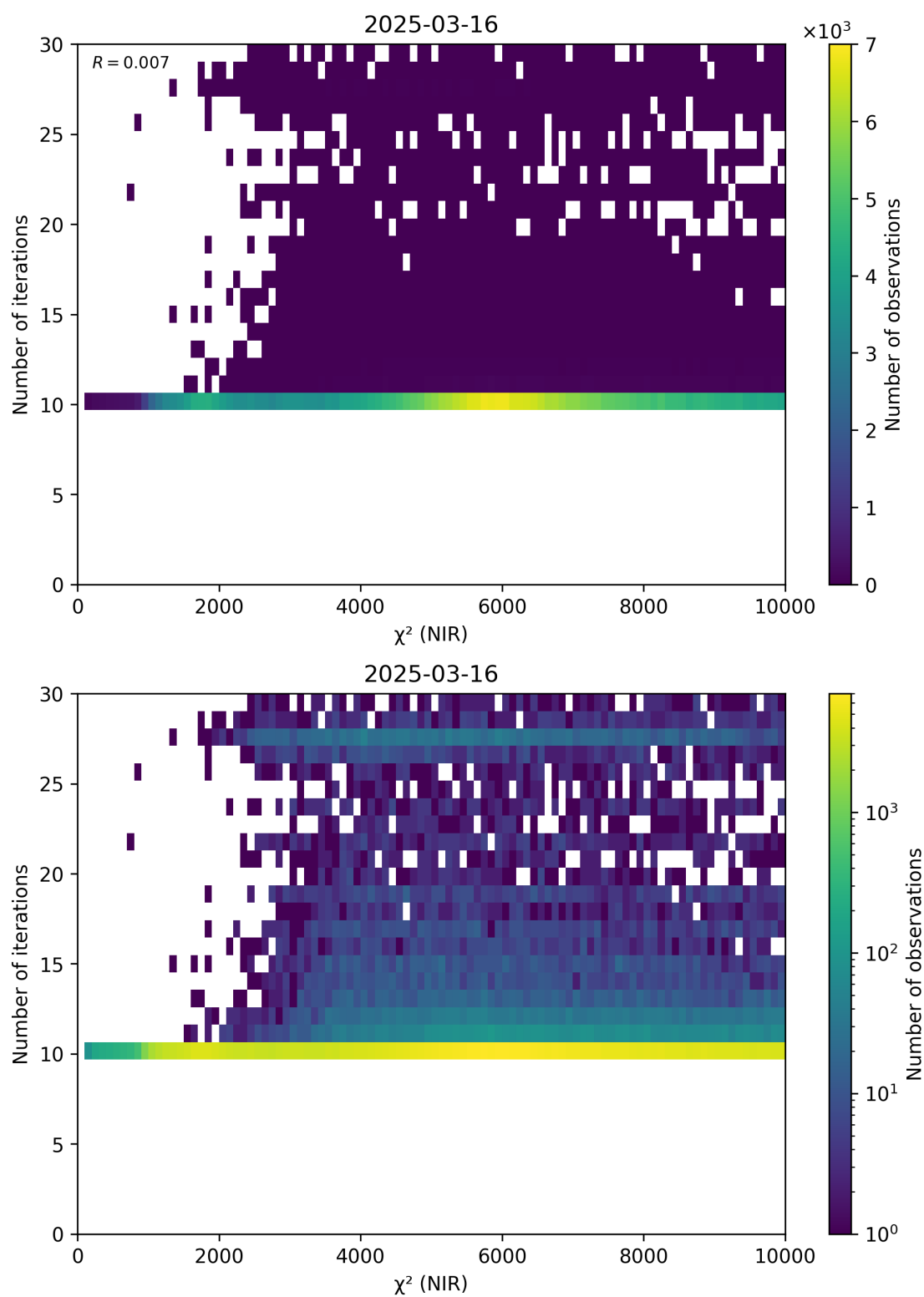
Figure 46: Scatter density plot of “ \chi^2 (NIR)” against “Number of iterations” for 2025-03-15 to 2025-03-17.
