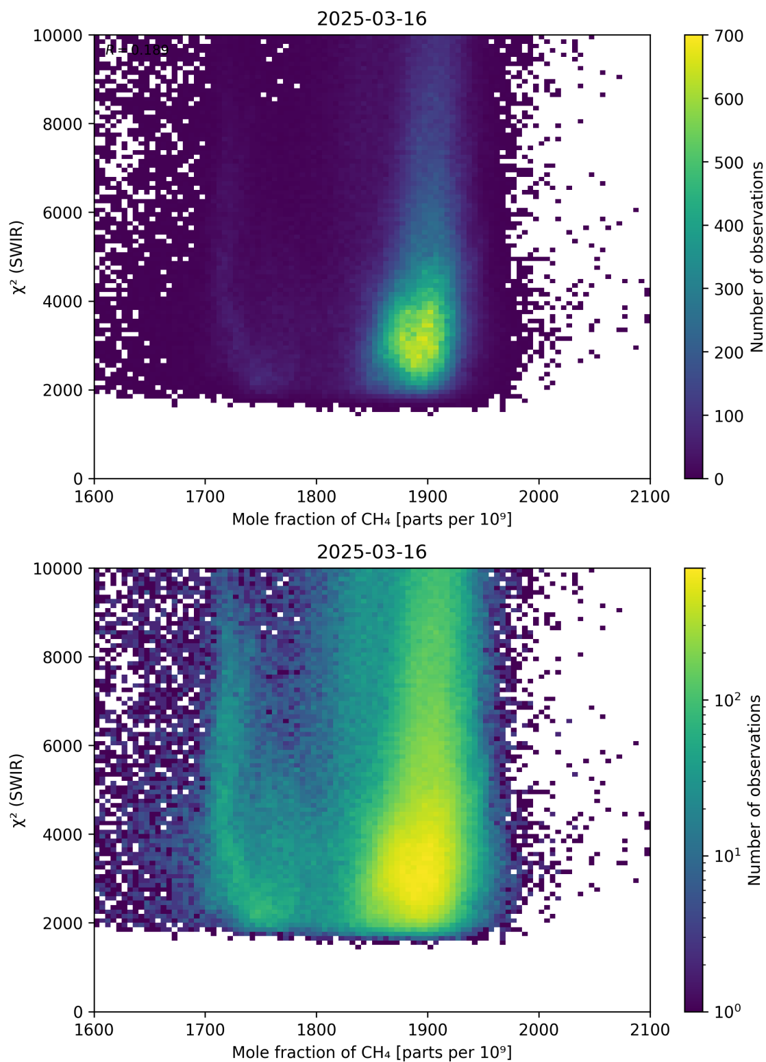
Figure 71: Scatter density plot of “Mole fraction of CH 4 ” against “ \chi^2 (SWIR)” for 2025-03-15 to 2025-03-17.
