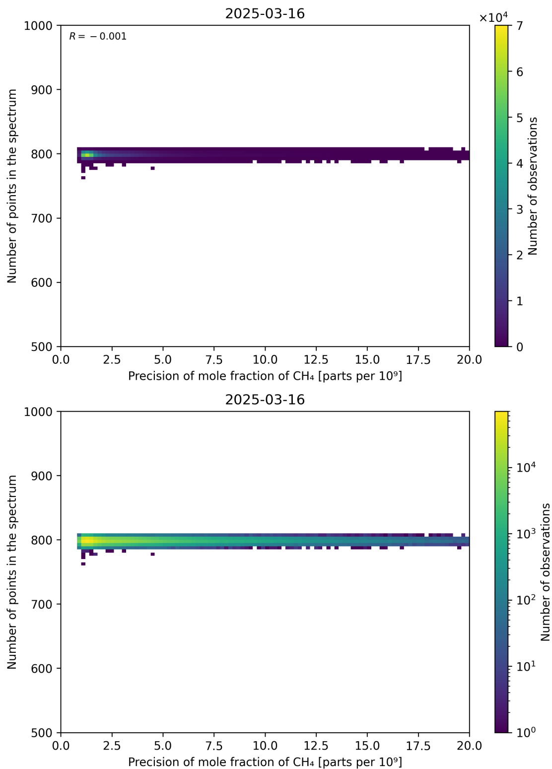
Figure 84: Scatter density plot of “Precision of mole fraction of CH 4 ” against “Number of points in the spectrum” for 2025-03-15 to 2025-03-17.
