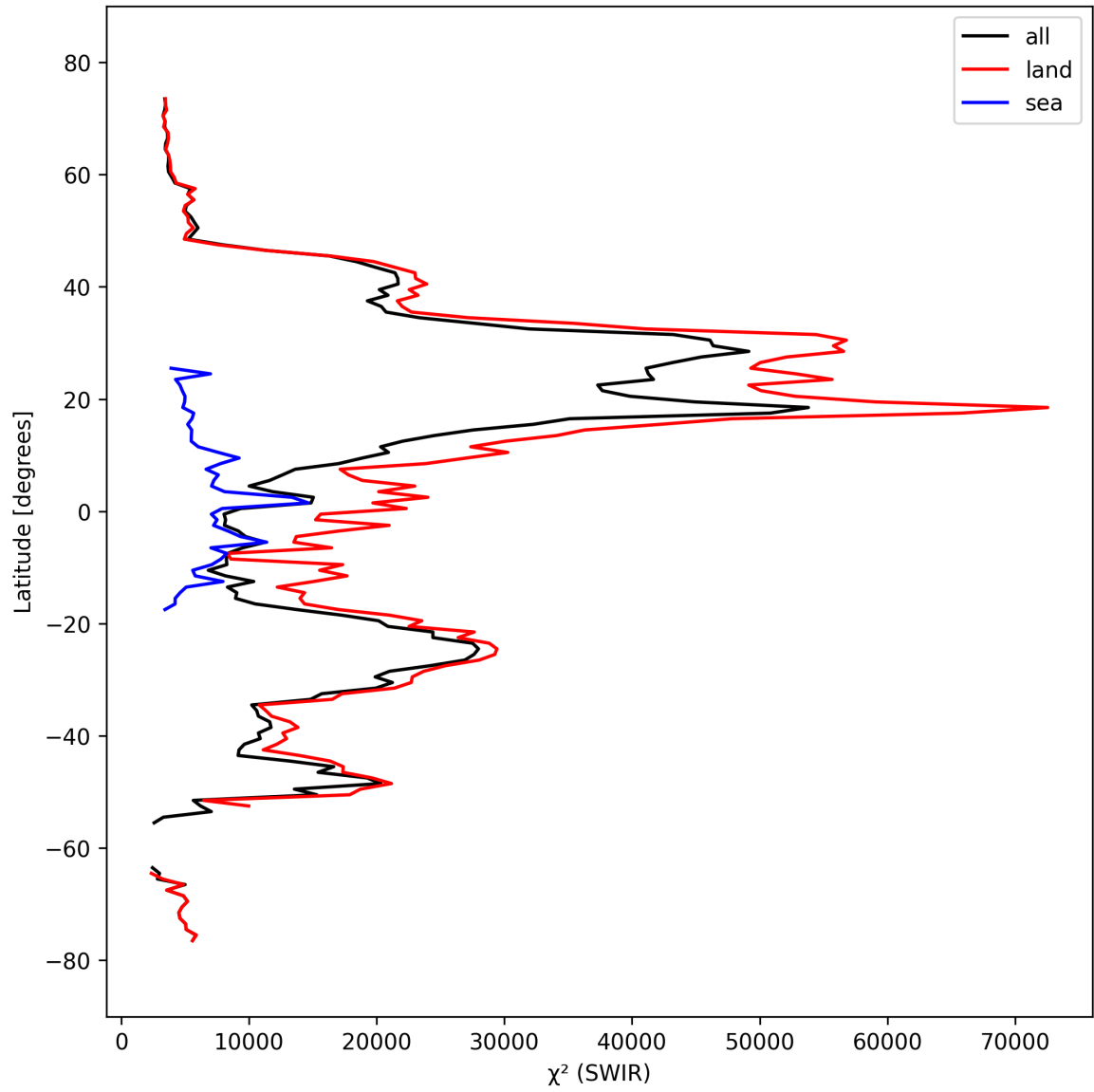
Figure 17: Zonal average of “ \chi^2 (SWIR)” for 2025-03-15 to 2025-03-17.
