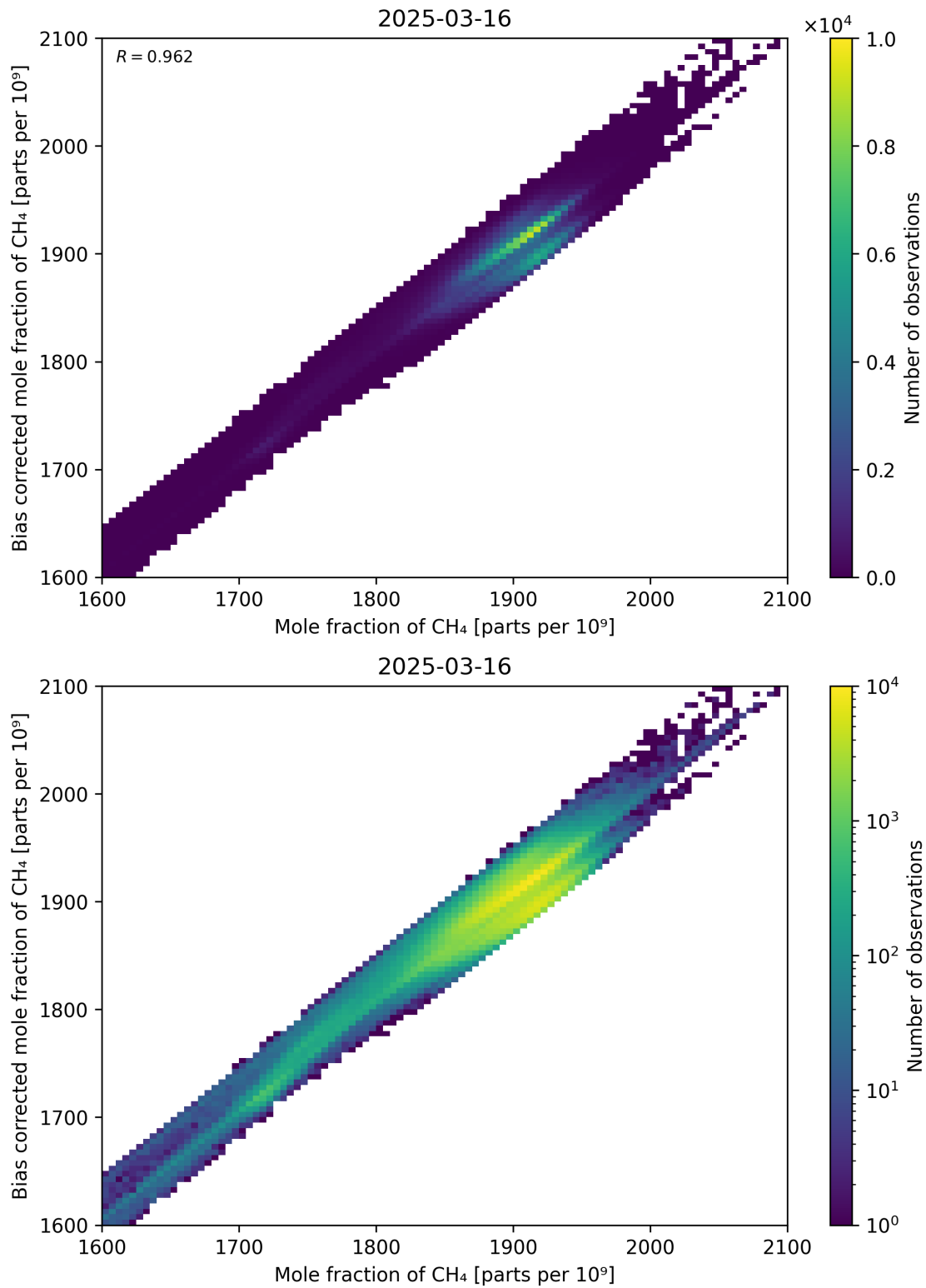
Figure 74: Scatter density plot of “Mole fraction of CH 4 ” against “Bias corrected mole fraction of CH 4 ” for 2025-03-15 to 2025-03-17.
