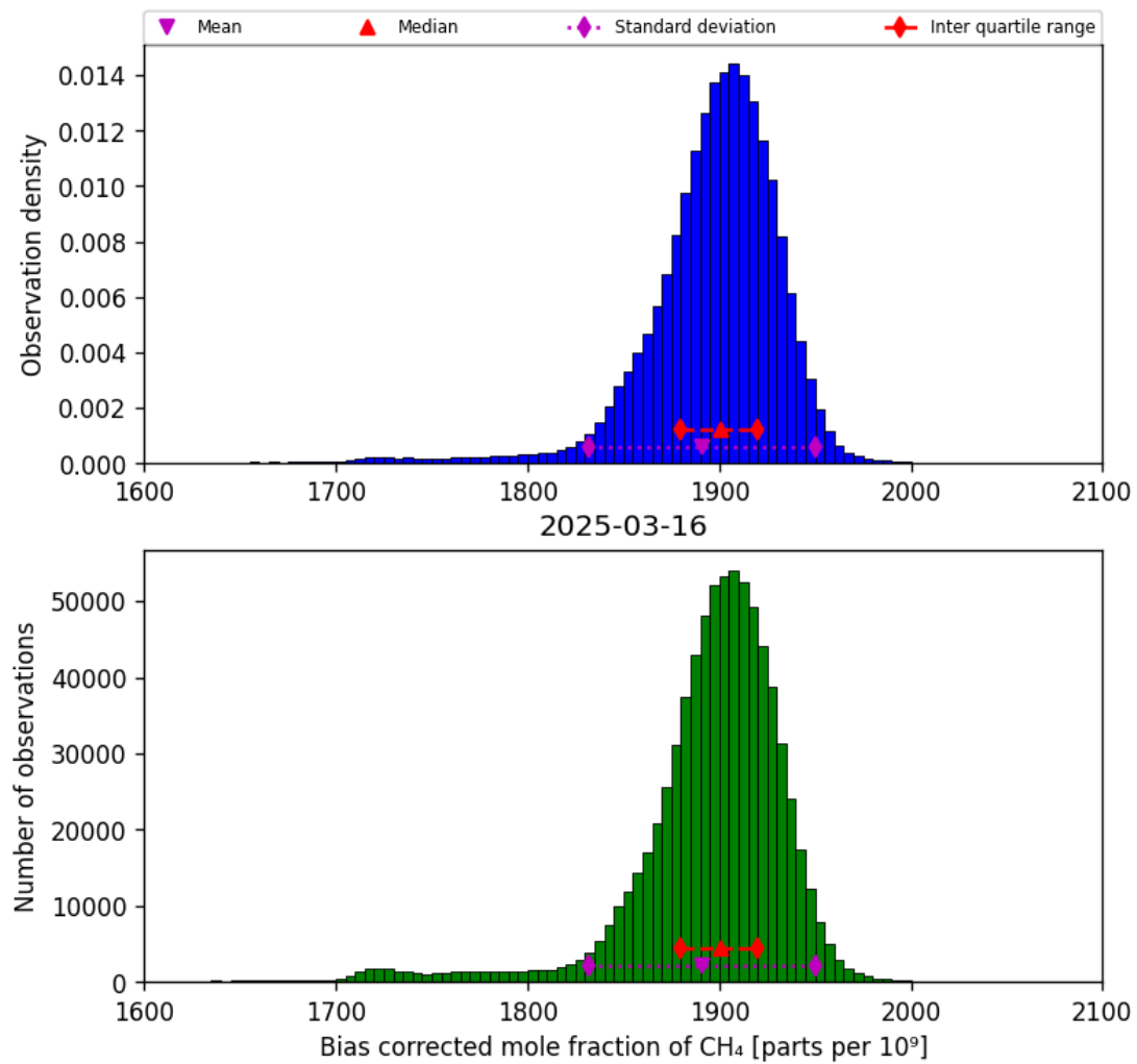
Figure 25: Histogram of “Bias corrected mole fraction of CH 4 ” for 2025-03-15 to 2025-03-17
