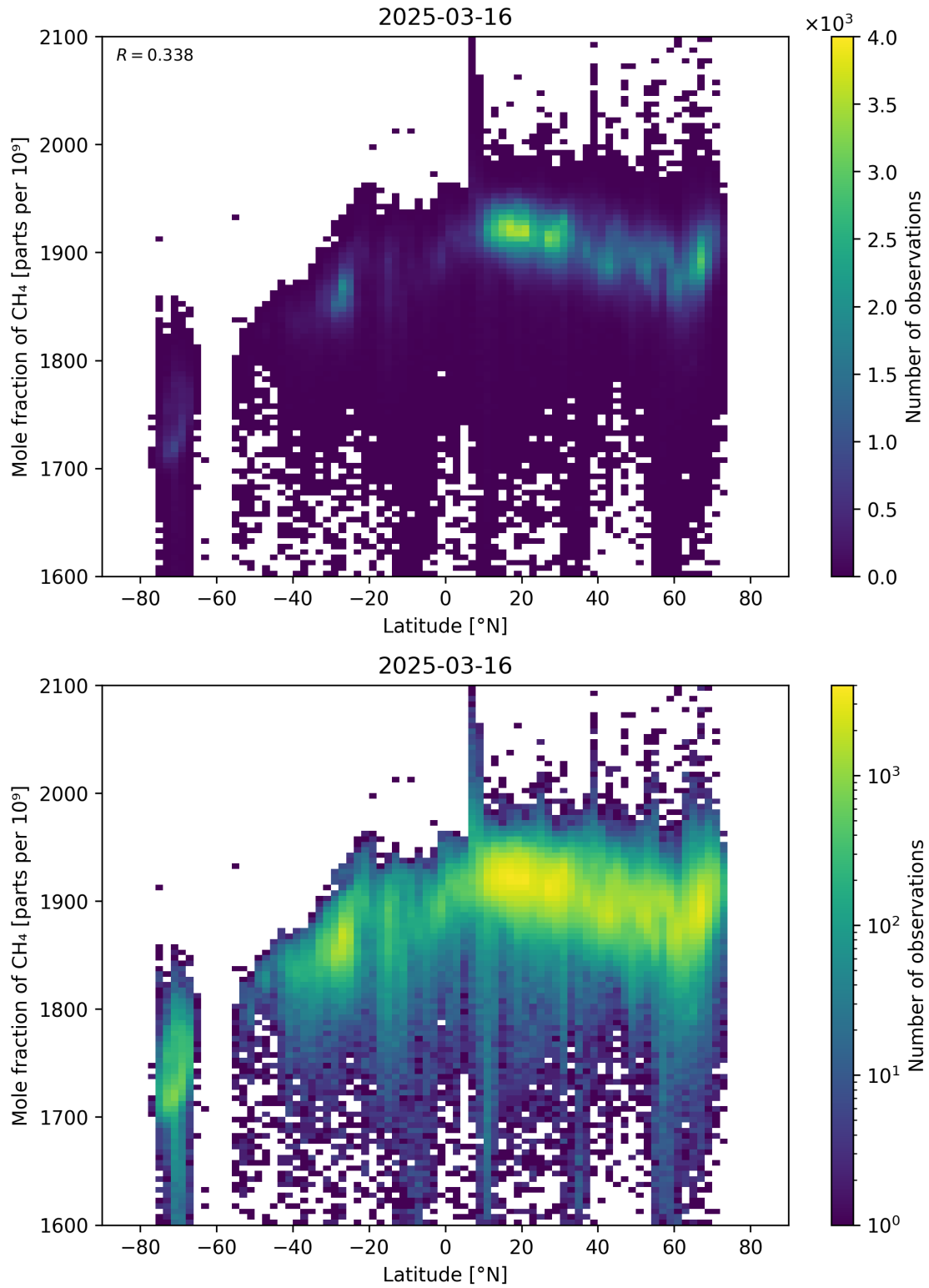
Figure 57: Scatter density plot of “Latitude” against “Mole fraction of CH 4 ” for 2025-03-15 to 2025-03-17.
