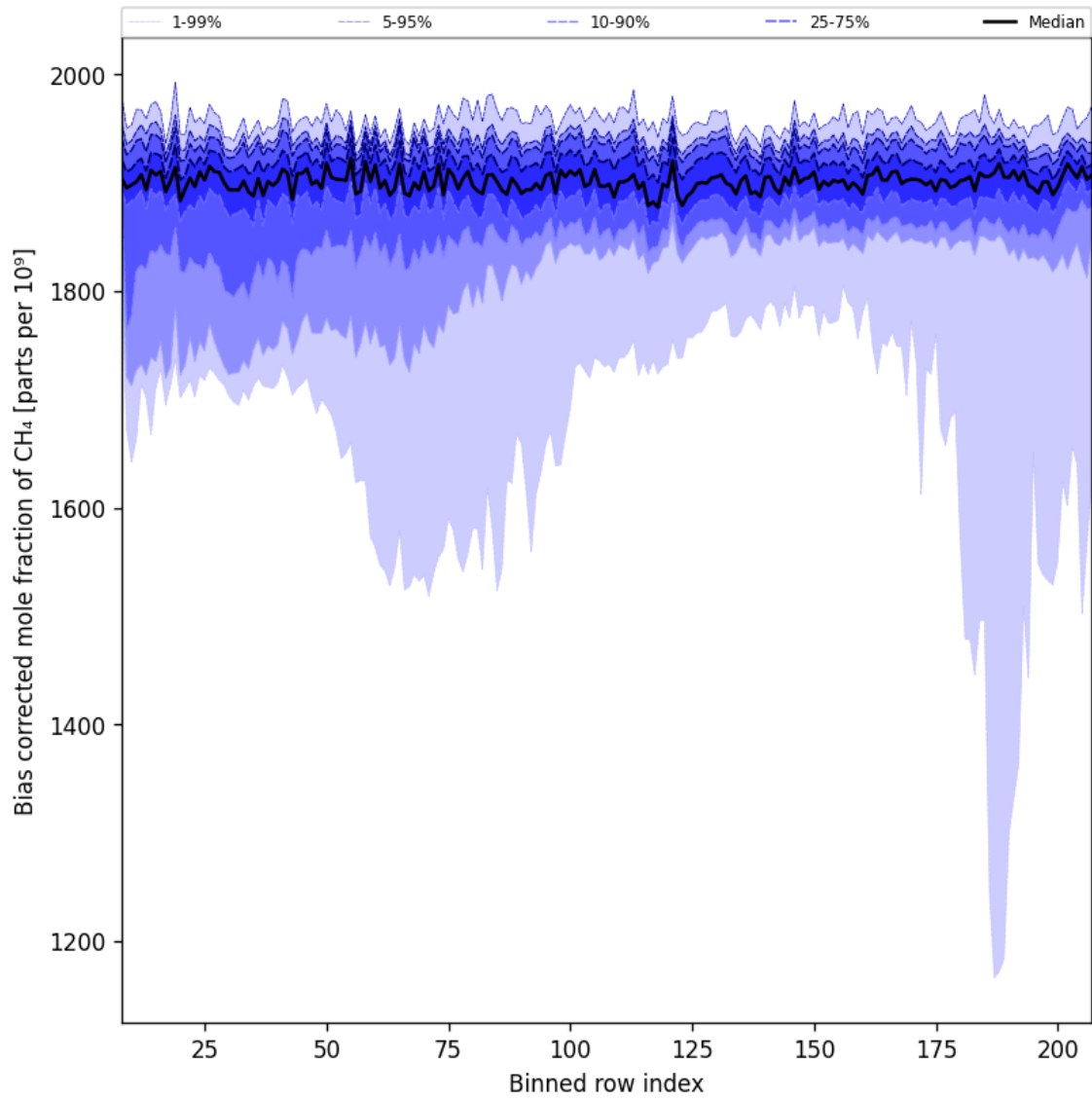
Figure 36: Along track statistics of “Bias corrected mole fraction of CH 4 ” for 2025-03-15 to 2025-03-17
