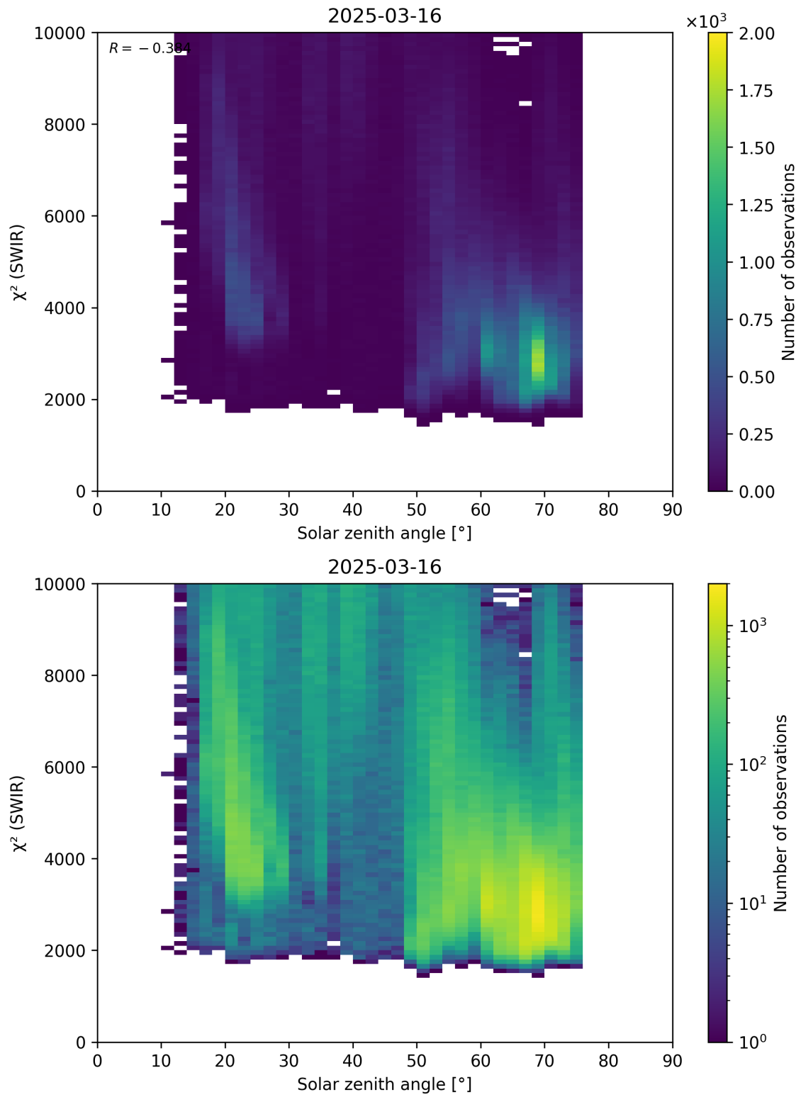
Figure 95: Scatter density plot of “Solar zenith angle” against “ \chi^2 (SWIR)” for 2025-03-15 to 2025-03-17.
