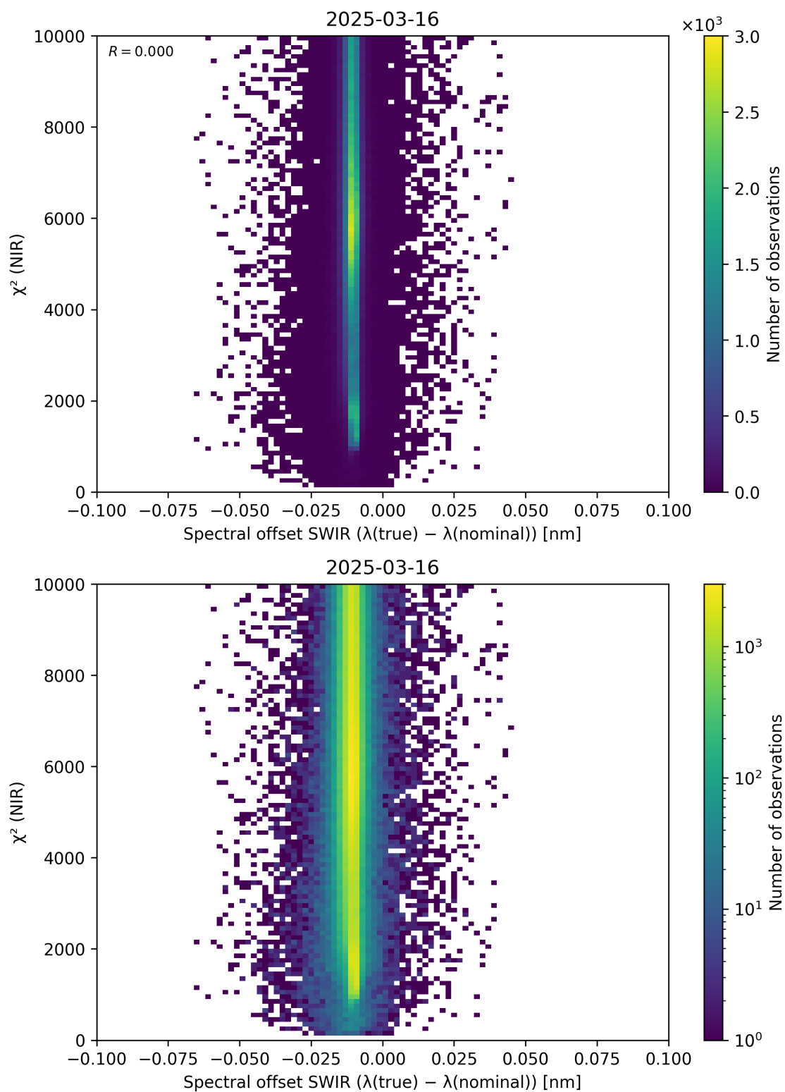
Figure 117: Scatter density plot of “Spectral offset SWIR ( \lambda_{\text{true}} - \lambda_{\text{nominal}} )” against “ \chi^2 (NIR)” for 2025-03-15 to 2025-03-17.
