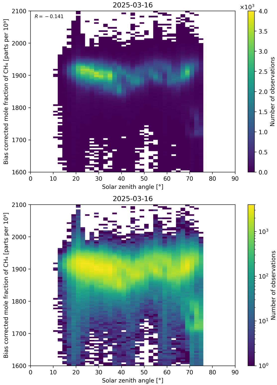
Figure 100: Scatter density plot of “Solar zenith angle” against “Bias corrected mole fraction of \text{CH}_4 ” for 2025-03-15 to 2025-03-17.
