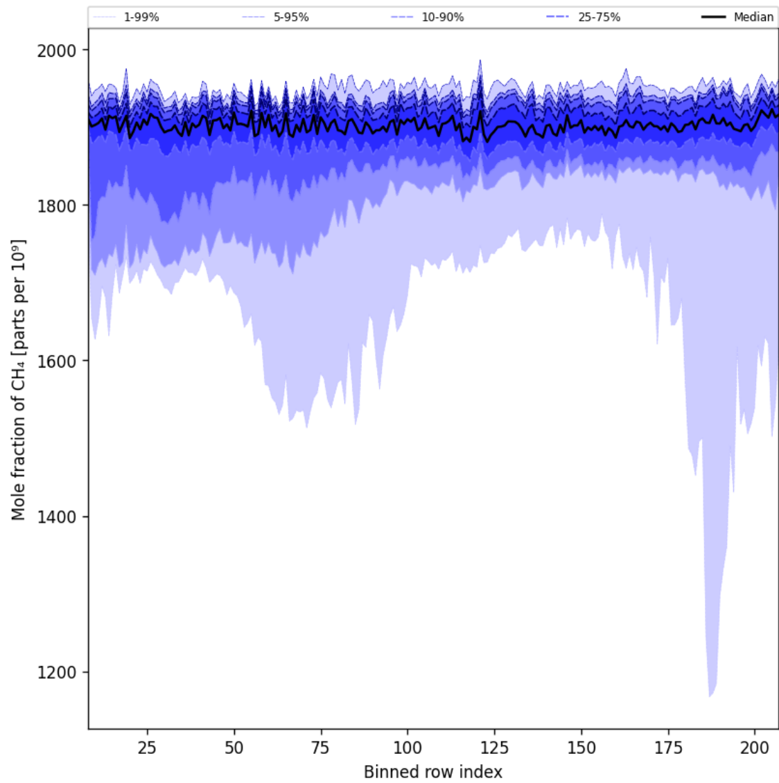
Figure 34: Along track statistics of “Mole fraction of CH 4 ” for 2025-03-15 to 2025-03-17
