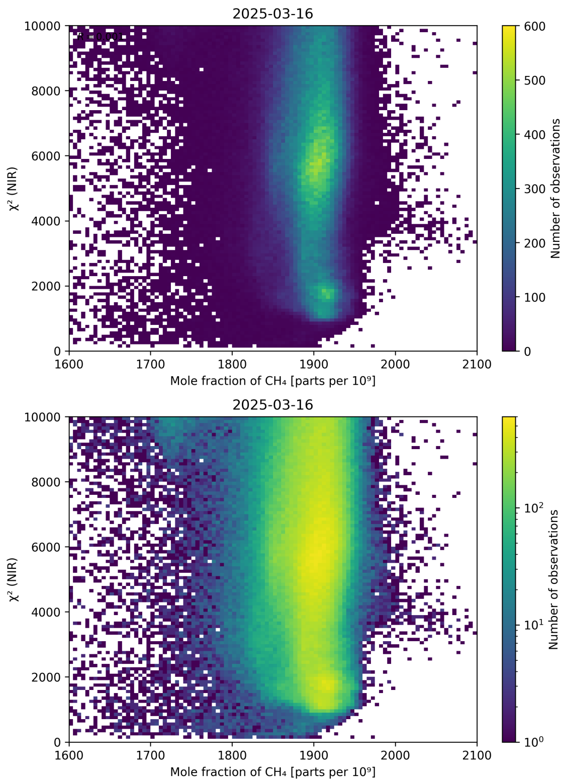
Figure 70: Scatter density plot of “Mole fraction of \text{CH}_4 ” against “ \chi^2 (NIR)” for 2025-03-15 to 2025-03-17.
