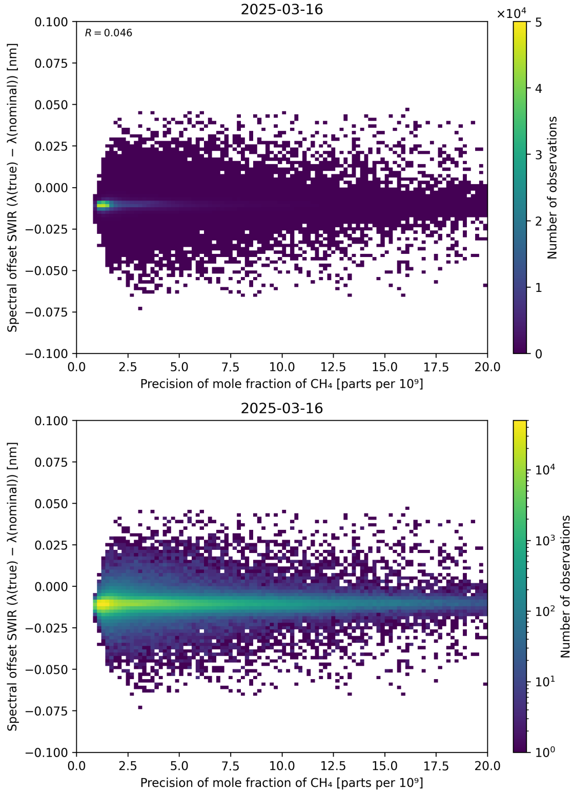
Figure 85: Scatter density plot of “Precision of mole fraction of CH 4 ” against “Spectral offset SWIR ( \lambda_{\text{true}} - \lambda_{\text{nominal}} )” for 2025-03-15 to 2025-03-17.
