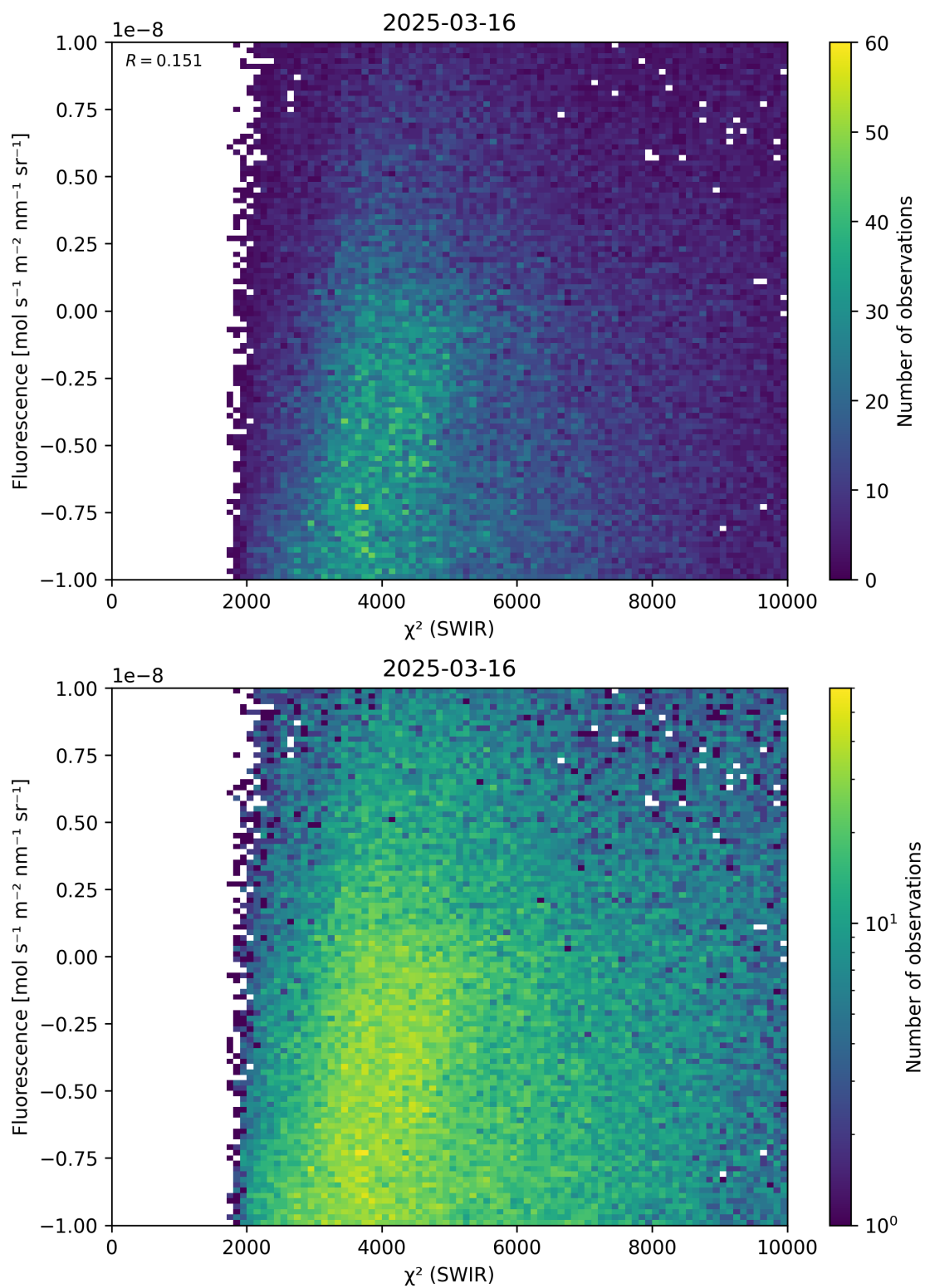
Figure 49: Scatter density plot of “ \chi^2 (SWIR)” against “Fluorescence” for 2025-03-15 to 2025-03-17.
