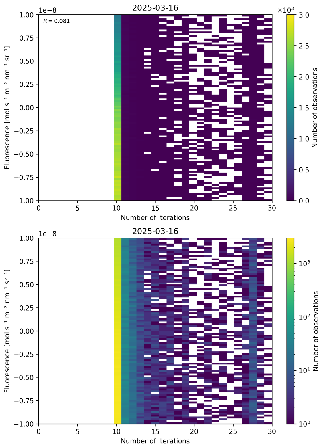
Figure 87: Scatter density plot of "Number of iterations" against "Fluorescence" for 2025-03-15 to 2025-03-17.
