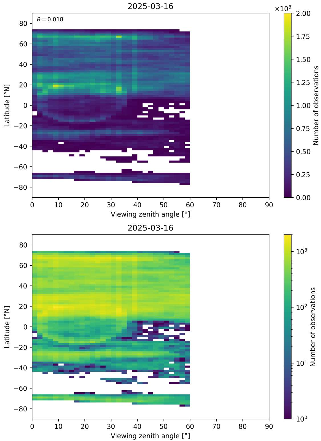
Figure 109: Scatter density plot of “Viewing zenith angle” against “Latitude” for 2025-03-15 to 2025-03-17.
