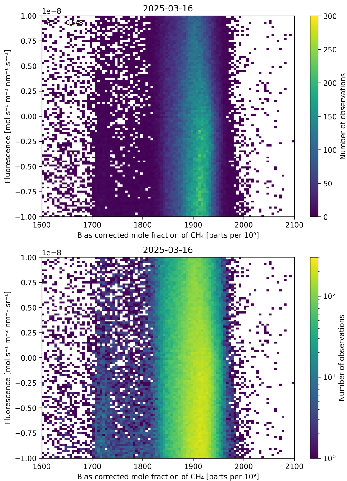
Figure 66: Scatter density plot of “Bias corrected mole fraction of CH 4 ” against “Fluorescence” for 2025-03-15 to 2025-03-17.
