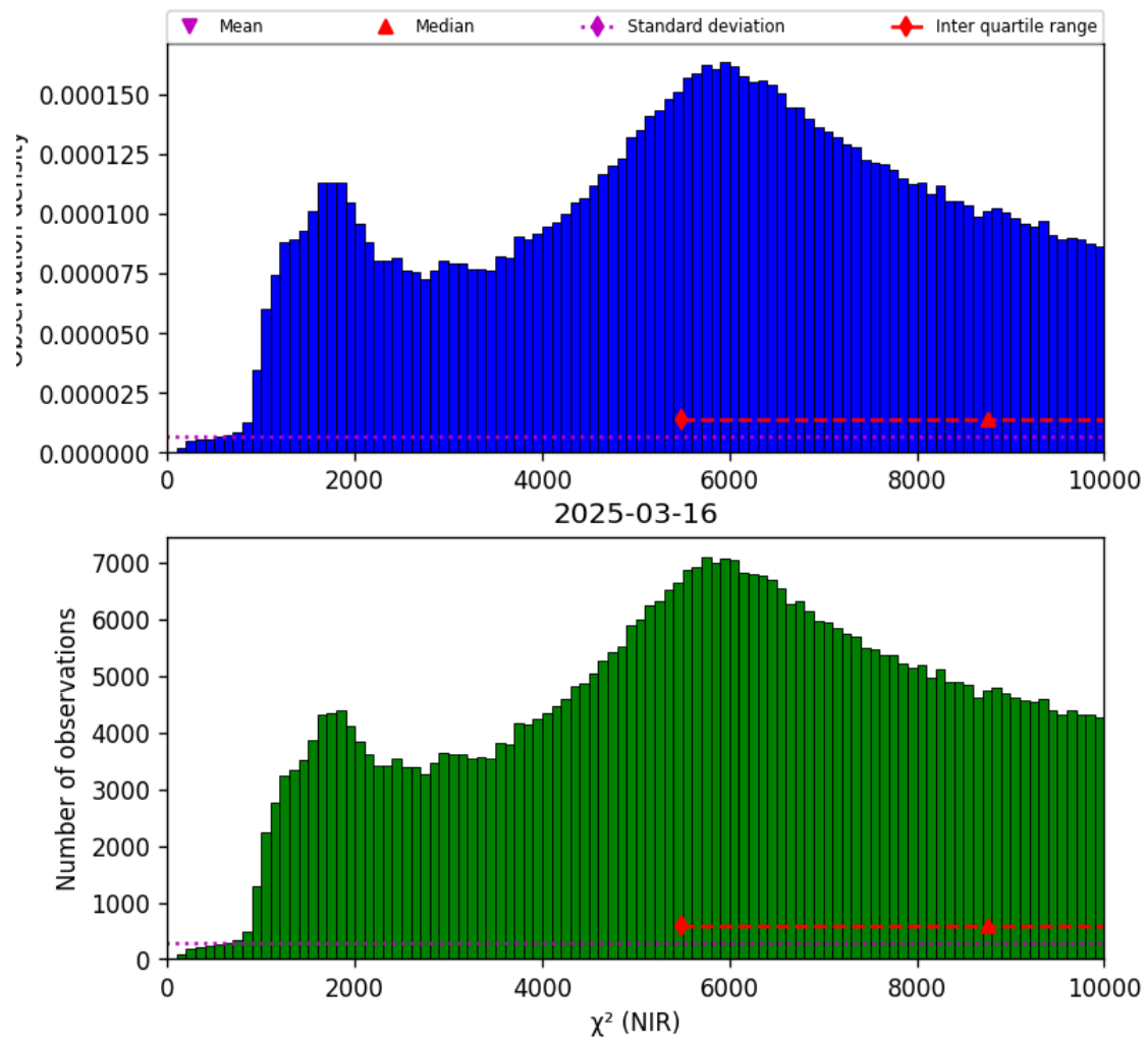
Figure 29: Histogram of “ \chi^2 (NIR)” for 2025-03-15 to 2025-03-17
