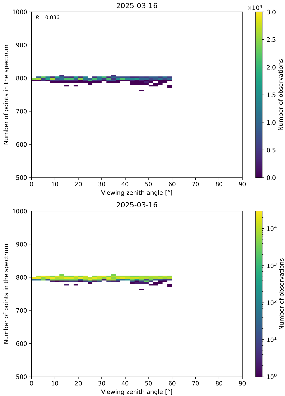
Figure 114: Scatter density plot of “Viewing zenith angle” against “Number of points in the spectrum” for 2025-03-15 to 2025-03-17.
