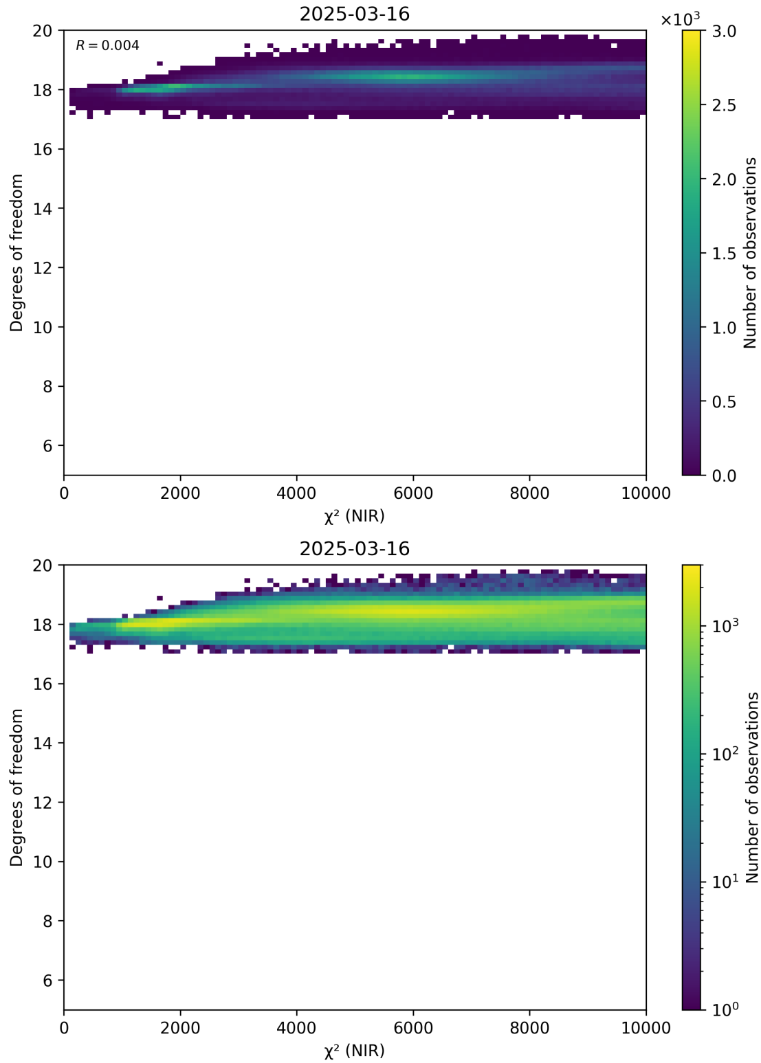
Figure 44: Scatter density plot of “ \chi^2 (NIR)” against “Degrees of freedom” for 2025-03-15 to 2025-03-17.
