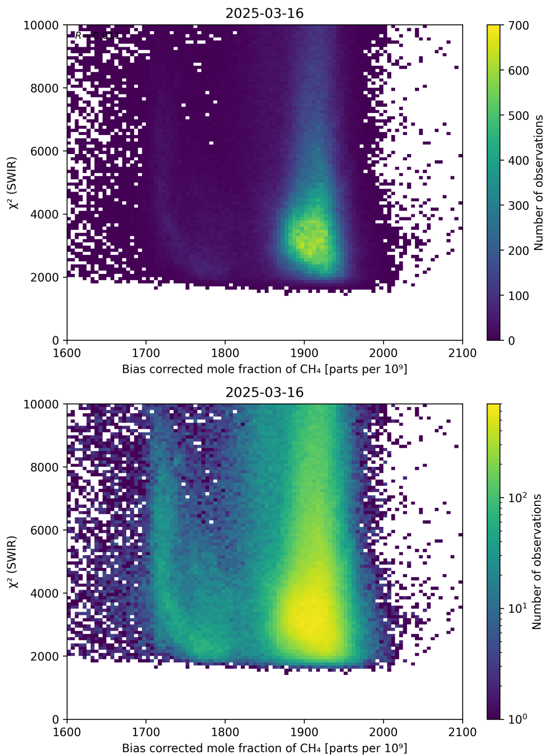
Figure 64: Scatter density plot of “Bias corrected mole fraction of \text{CH}_4 ” against “ \chi^2 (SWIR)” for 2025-03-15 to 2025-03-17.
