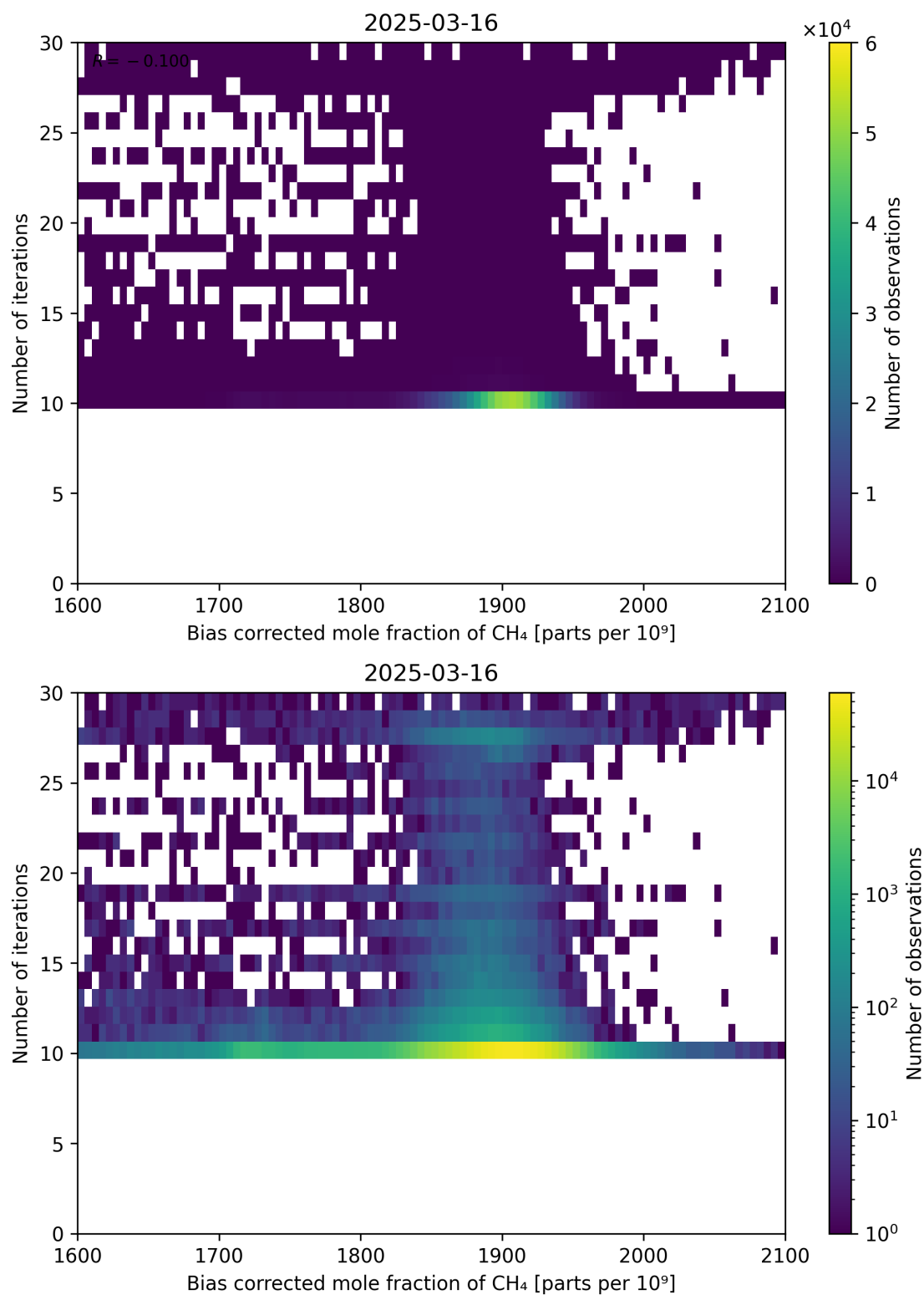
Figure 67: Scatter density plot of “Bias corrected mole fraction of \text{CH}_4 ” against “Number of iterations” for 2025-03-15 to 2025-03-17.
