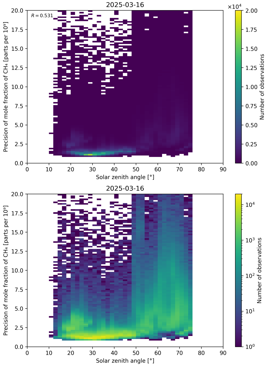
Figure 101: Scatter density plot of “Solar zenith angle” against “Precision of mole fraction of CH 4 ” for 2025-03-15 to 2025-03-17.
