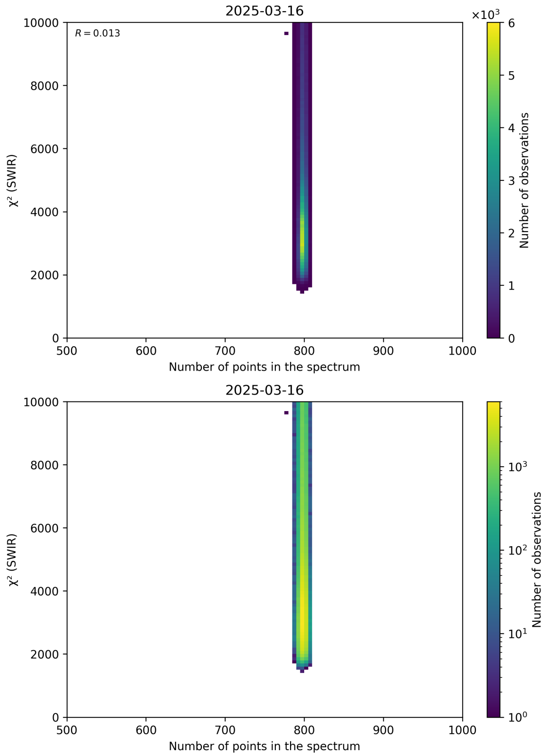
Figure 89: Scatter density plot of “Number of points in the spectrum” against “ \chi^2 (SWIR)” for 2025-03-15 to 2025-03-17.
