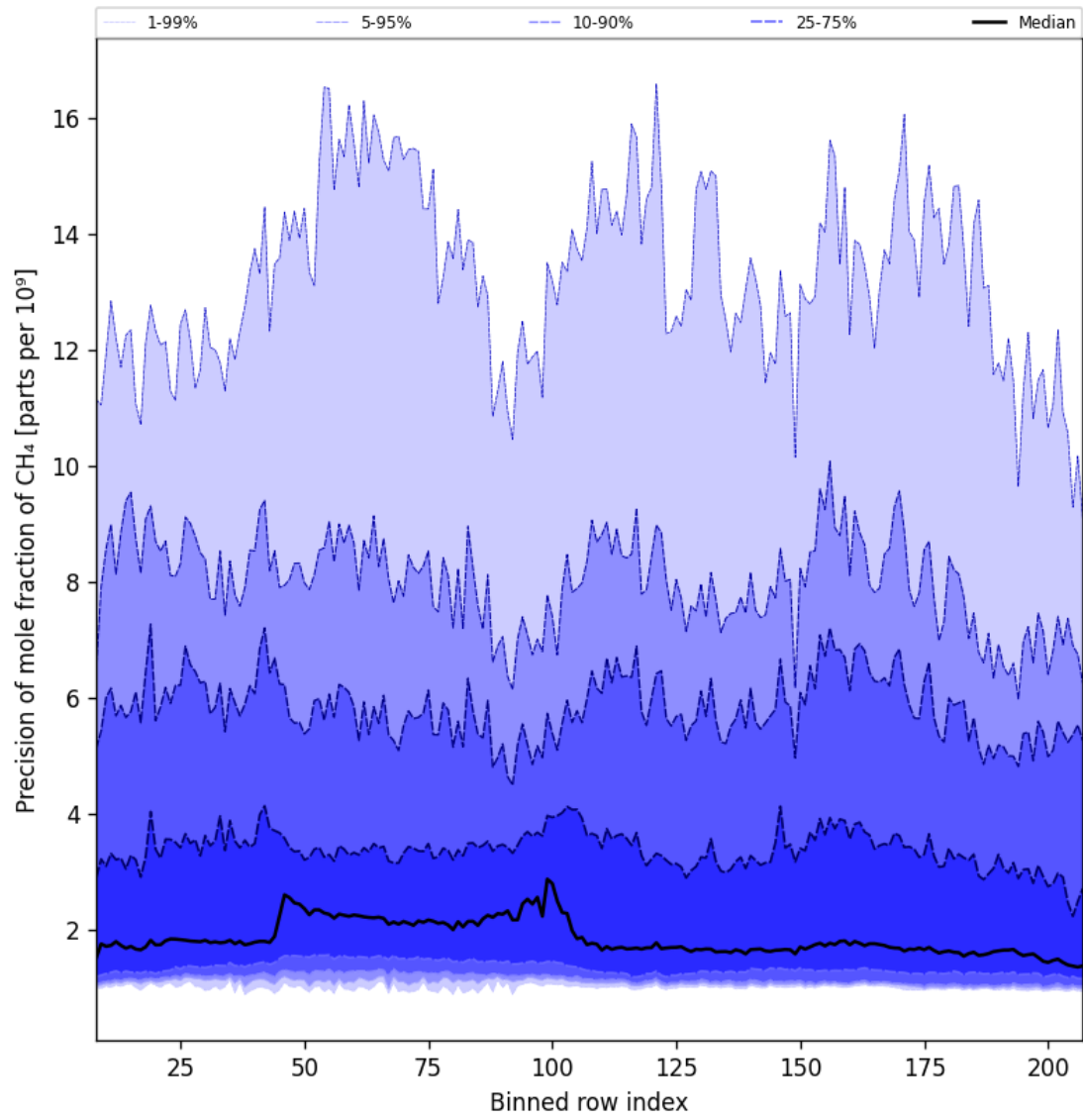
Figure 35: Along track statistics of “Precision of mole fraction of CH 4 ” for 2025-03-15 to 2025-03-17
