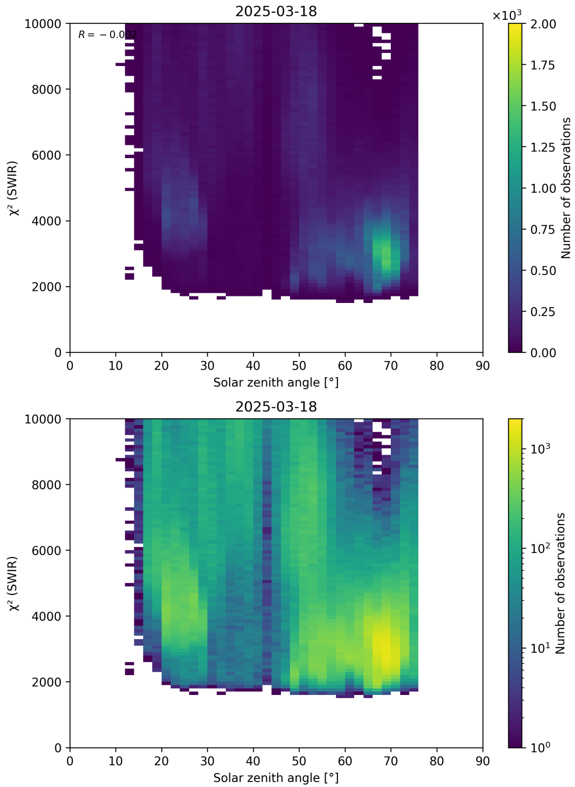
Figure 95: Scatter density plot of “Solar zenith angle” against “ \chi^2 (SWIR)” for 2025-03-17 to 2025-03-19.
