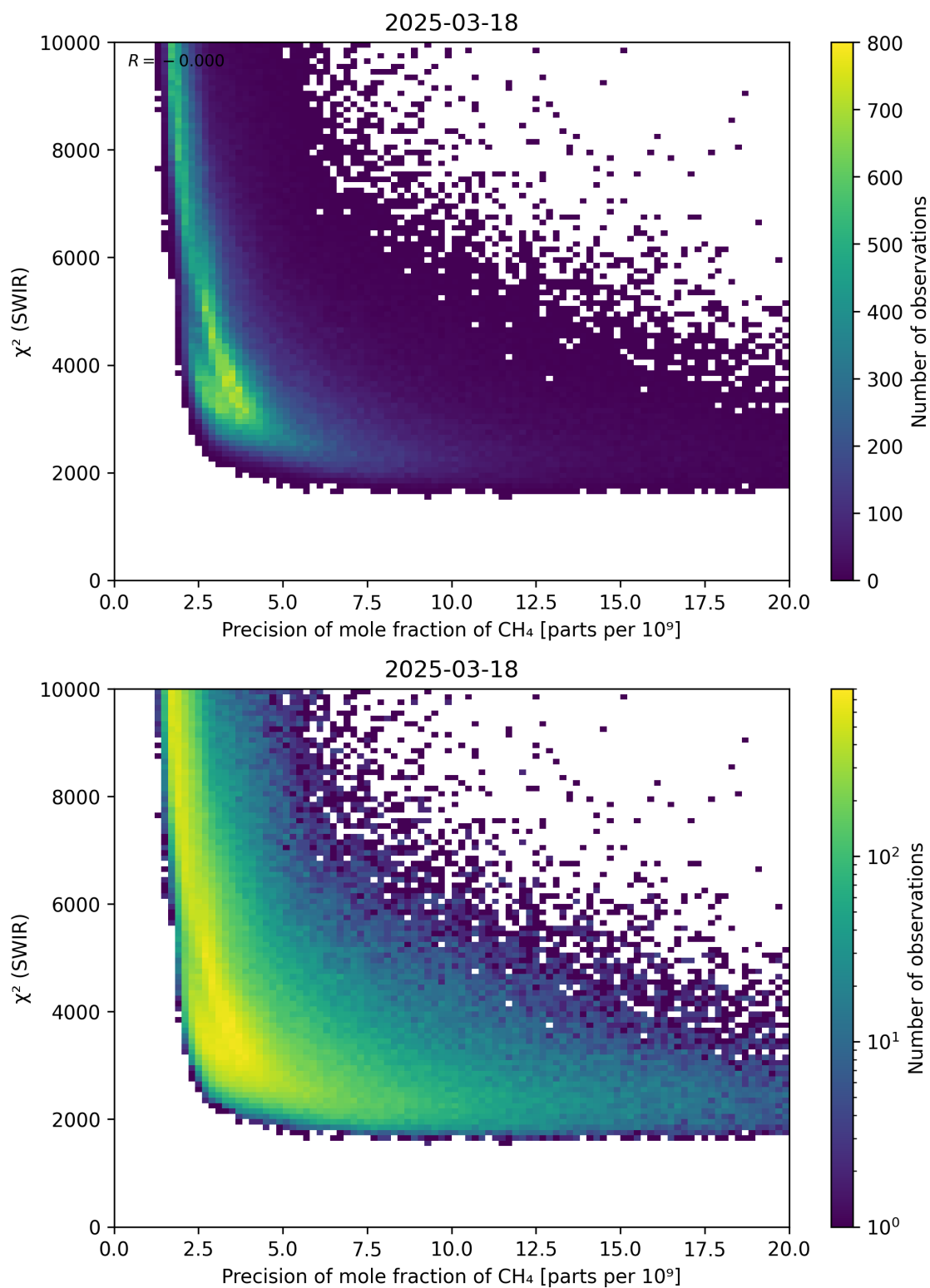
Figure 79: Scatter density plot of “Precision of mole fraction of \text{CH}_4 ” against “ \chi^2 (SWIR)” for 2025-03-17 to 2025-03-19.
