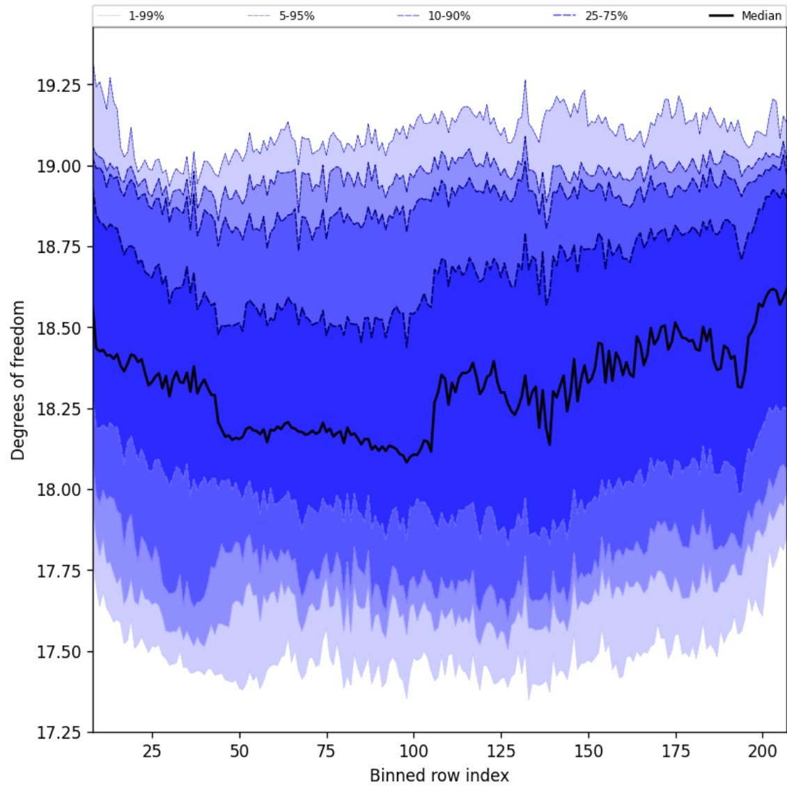
Figure 41: Along track statistics of “Degrees of freedom” for 2025-03-17 to 2025-03-19
