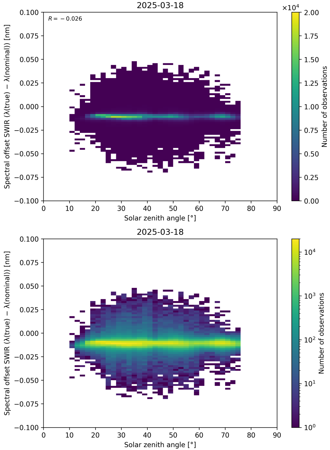
Figure 104: Scatter density plot of “Solar zenith angle” against “Spectral offset SWIR ( \lambda_{\text{true}} - \lambda_{\text{nominal}} )” for 2025-03-17 to 2025-03-19.
