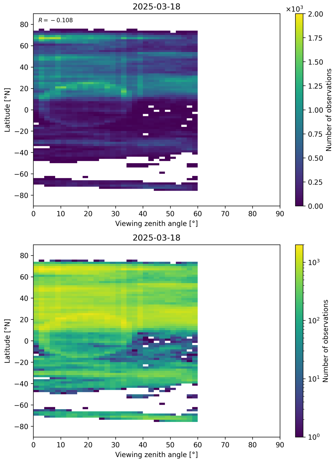
Figure 109: Scatter density plot of “Viewing zenith angle” against “Latitude” for 2025-03-17 to 2025-03-19.
