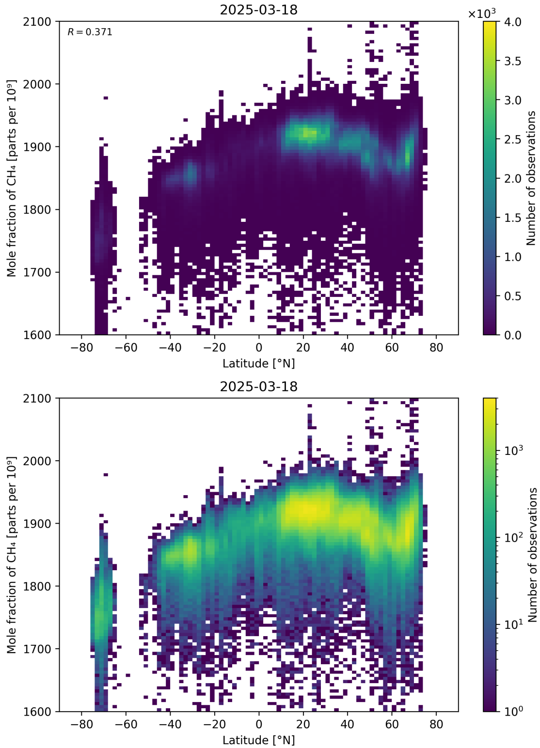
Figure 57: Scatter density plot of “Latitude” against “Mole fraction of CH 4 ” for 2025-03-17 to 2025-03-19.
