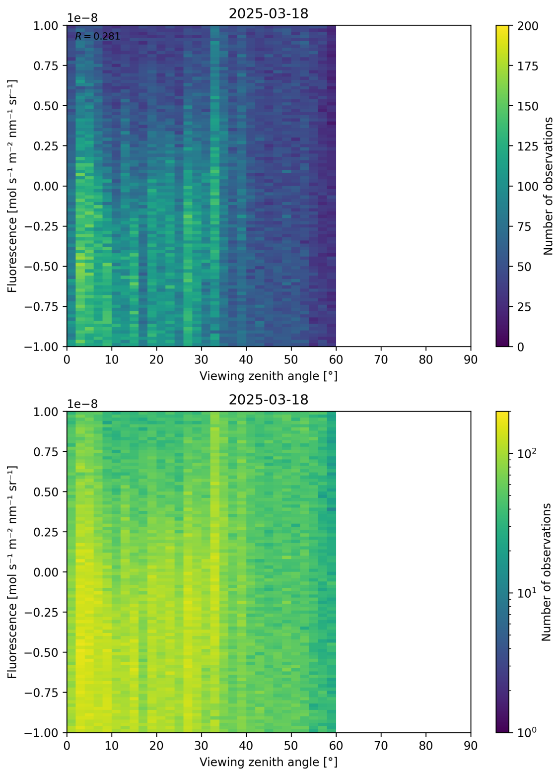
Figure 108: Scatter density plot of “Viewing zenith angle” against “Fluorescence” for 2025-03-17 to 2025-03-19.
