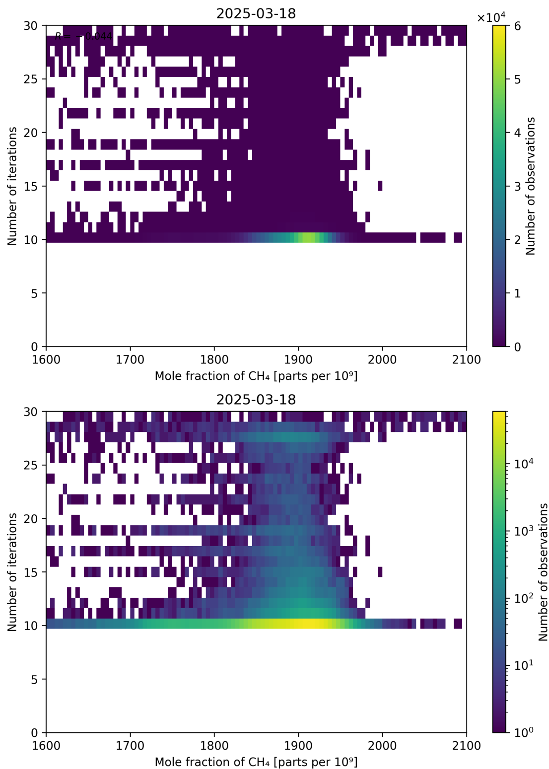
Figure 76: Scatter density plot of “Mole fraction of CH 4 ” against “Number of iterations” for 2025-03-17 to 2025-03-19.
