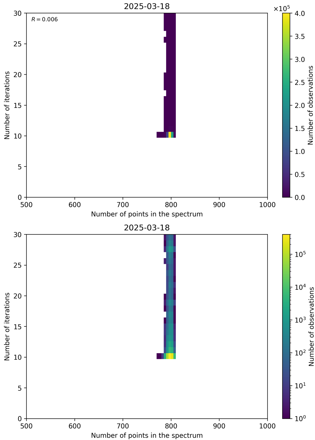
Figure 92: Scatter density plot of “Number of points in the spectrum” against “Number of iterations” for 2025-03-17 to 2025-03-19.
