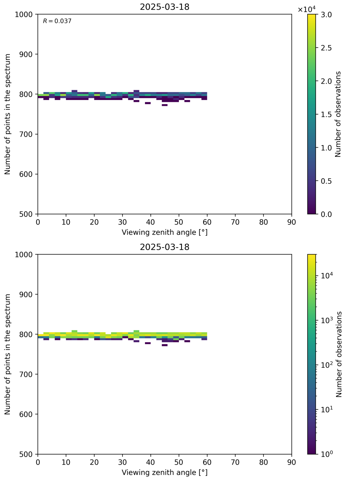
Figure 114: Scatter density plot of “Viewing zenith angle” against “Number of points in the spectrum” for 2025-03-17 to 2025-03-19.
