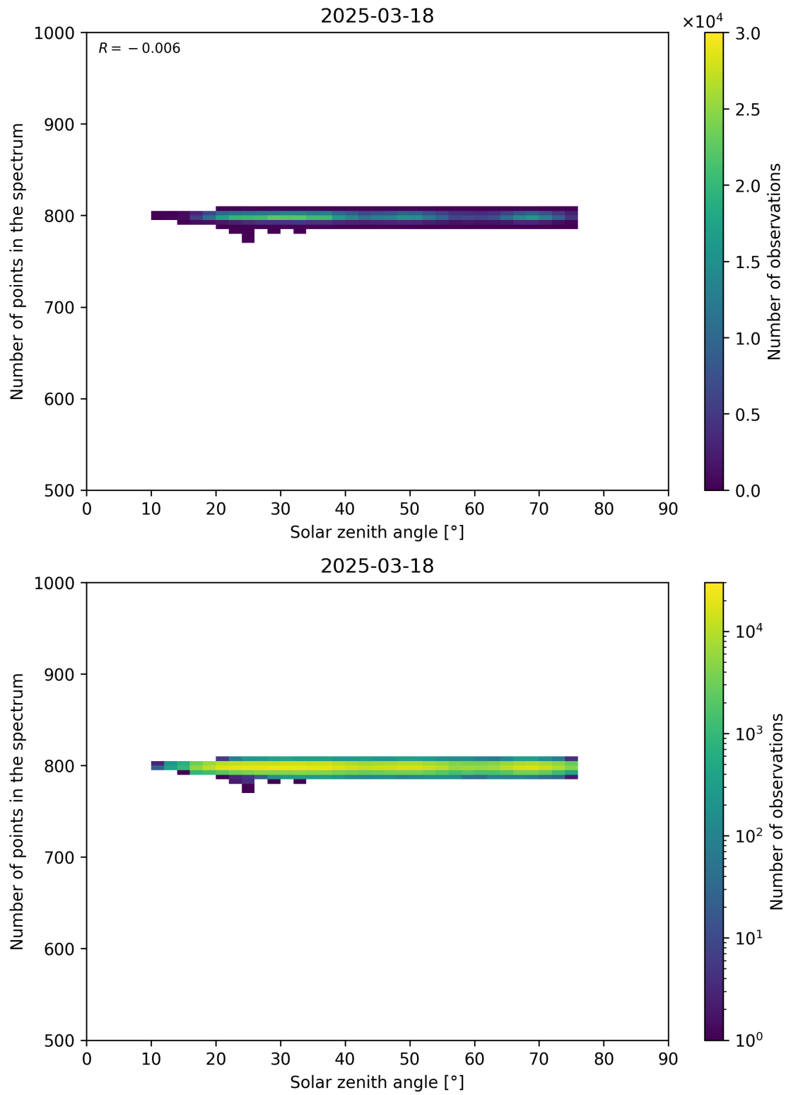
Figure 103: Scatter density plot of “Solar zenith angle” against “Number of points in the spectrum” for 2025-03-17 to 2025-03-19.
