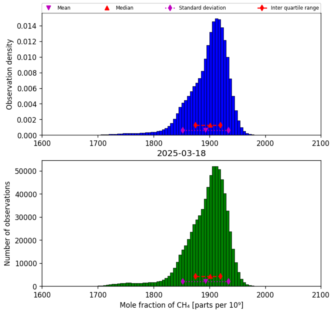
Figure 23: Histogram of “Mole fraction of CH 4 ” for 2025-03-17 to 2025-03-19
