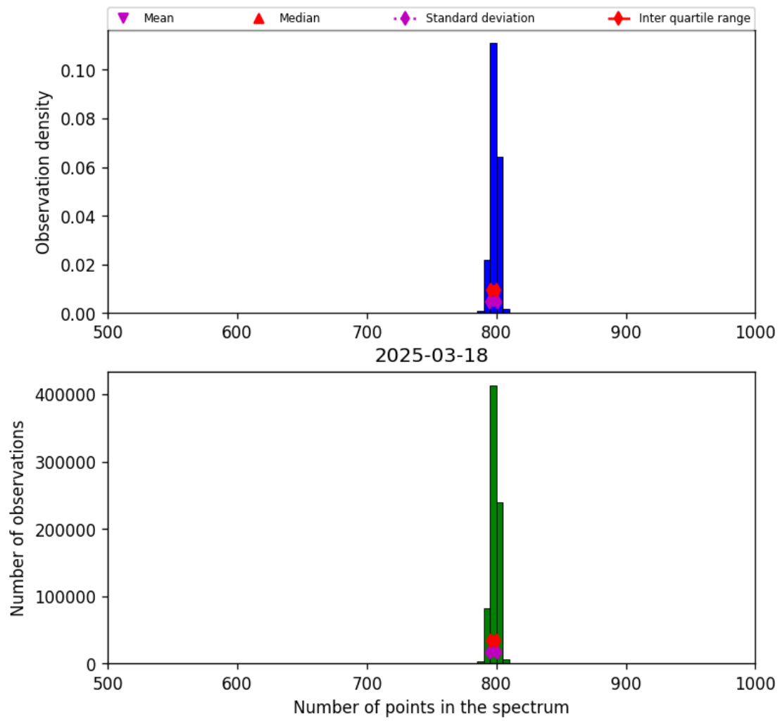
Figure 26: Histogram of “Number of points in the spectrum” for 2025-03-17 to 2025-03-19
