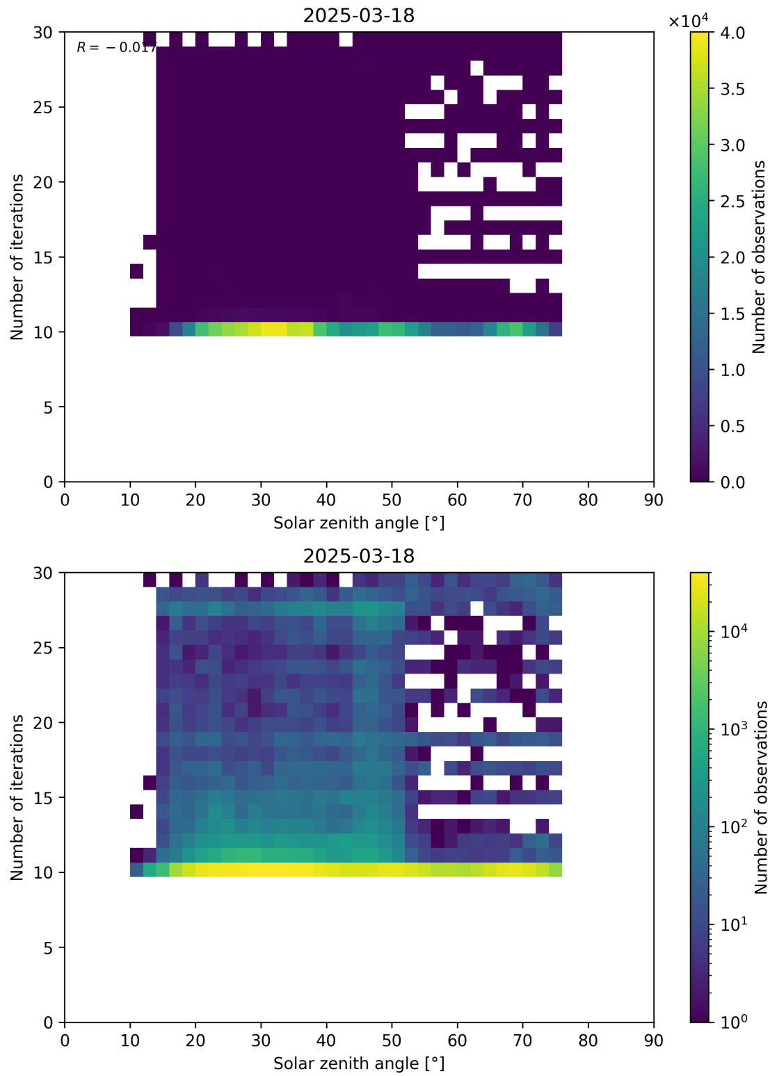
Figure 102: Scatter density plot of “Solar zenith angle” against “Number of iterations” for 2025-03-17 to 2025-03-19.
