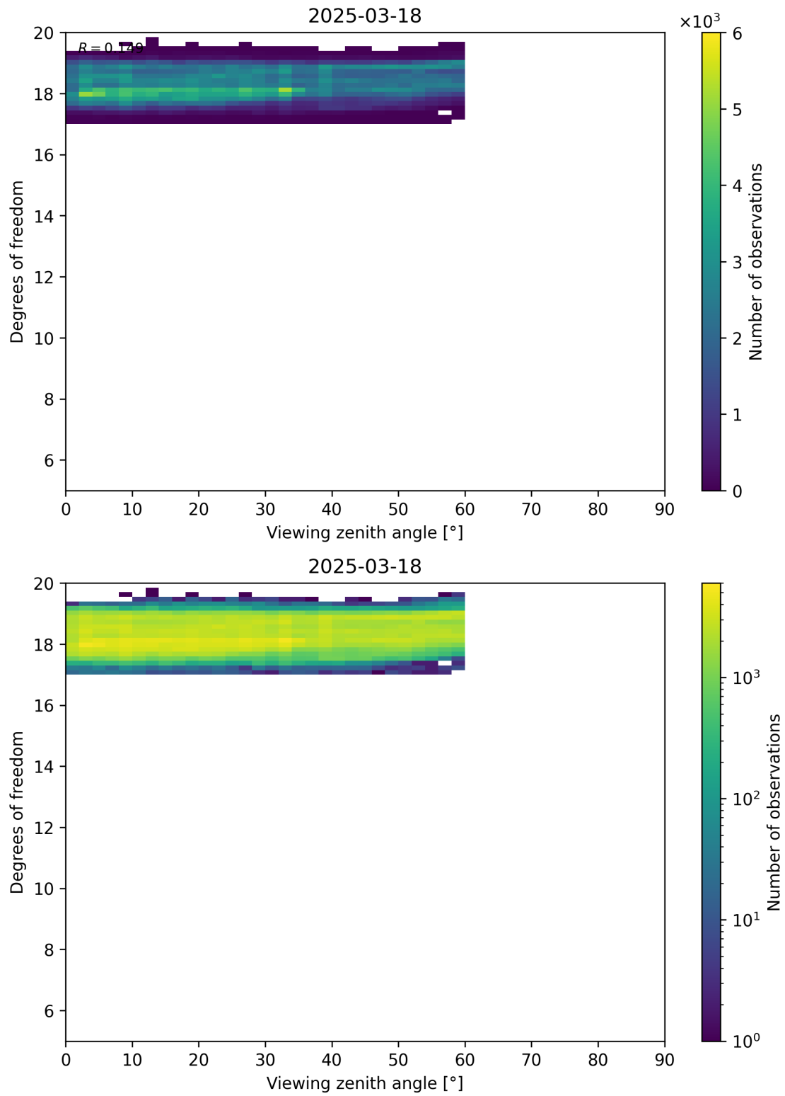
Figure 107: Scatter density plot of “Viewing zenith angle” against “Degrees of freedom” for 2025-03-17 to 2025-03-19.
