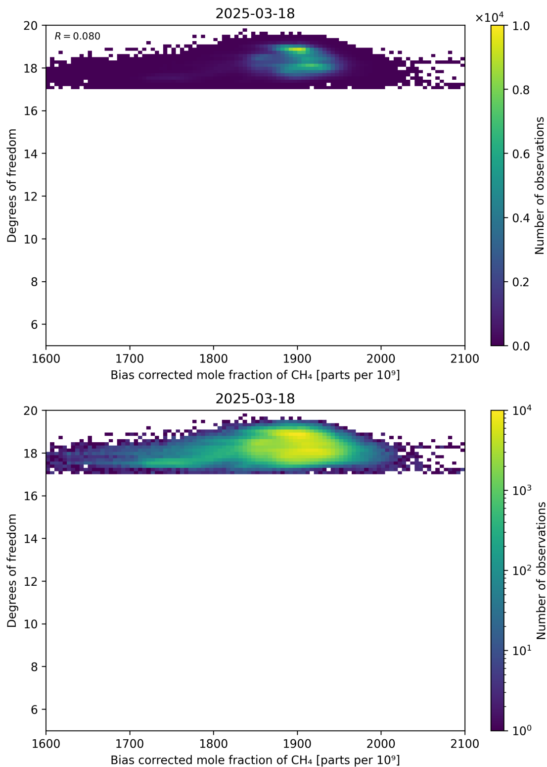
Figure 65: Scatter density plot of “Bias corrected mole fraction of CH 4 ” against “Degrees of freedom” for 2025-03-17 to 2025-03-19.
