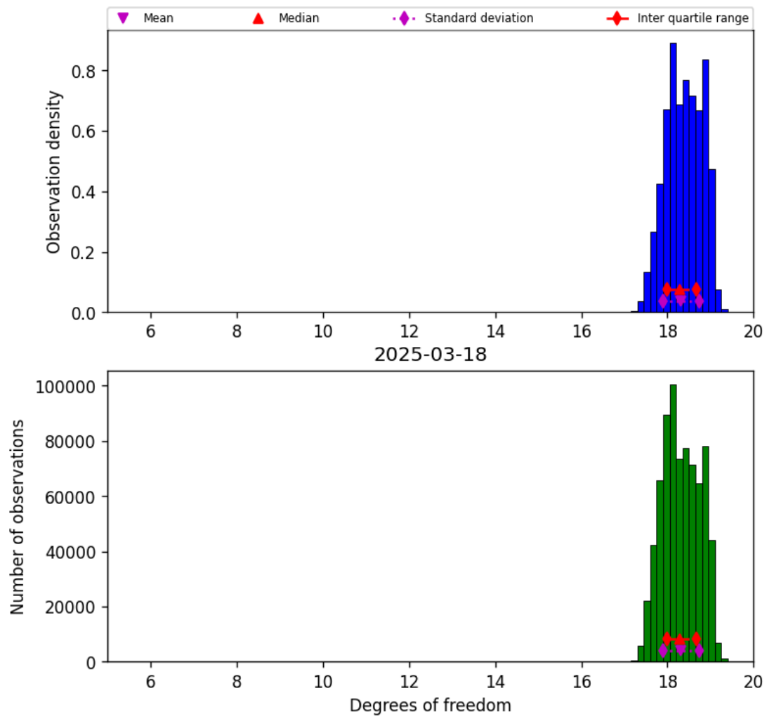
Figure 30: Histogram of “Degrees of freedom” for 2025-03-17 to 2025-03-19
