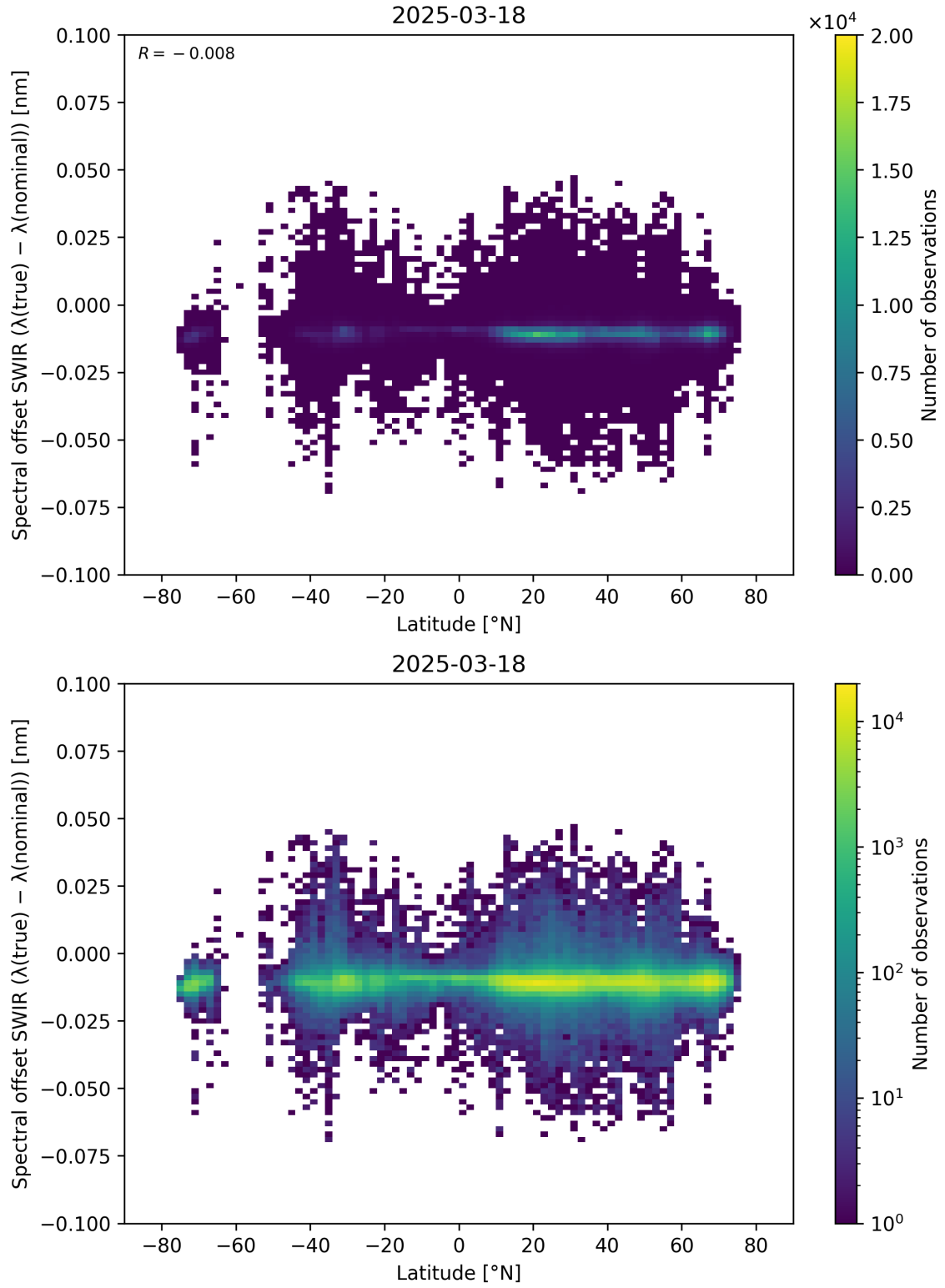
Figure 62: Scatter density plot of “Latitude” against “Spectral offset SWIR ( \lambda_{\text{true}} - \lambda_{\text{nominal}} )” for 2025-03-17 to 2025-03-19.
