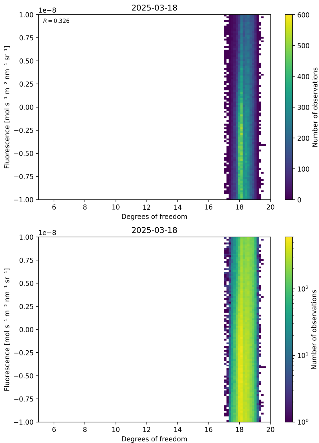
Figure 51: Scatter density plot of “Degrees of freedom” against “Fluorescence” for 2025-03-17 to 2025-03-19.
