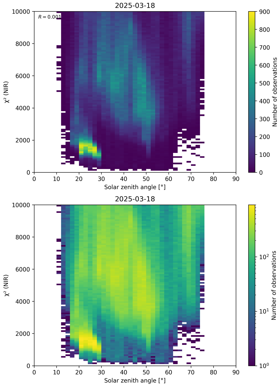
Figure 94: Scatter density plot of “Solar zenith angle” against “ \chi^2 (NIR)” for 2025-03-17 to 2025-03-19.
