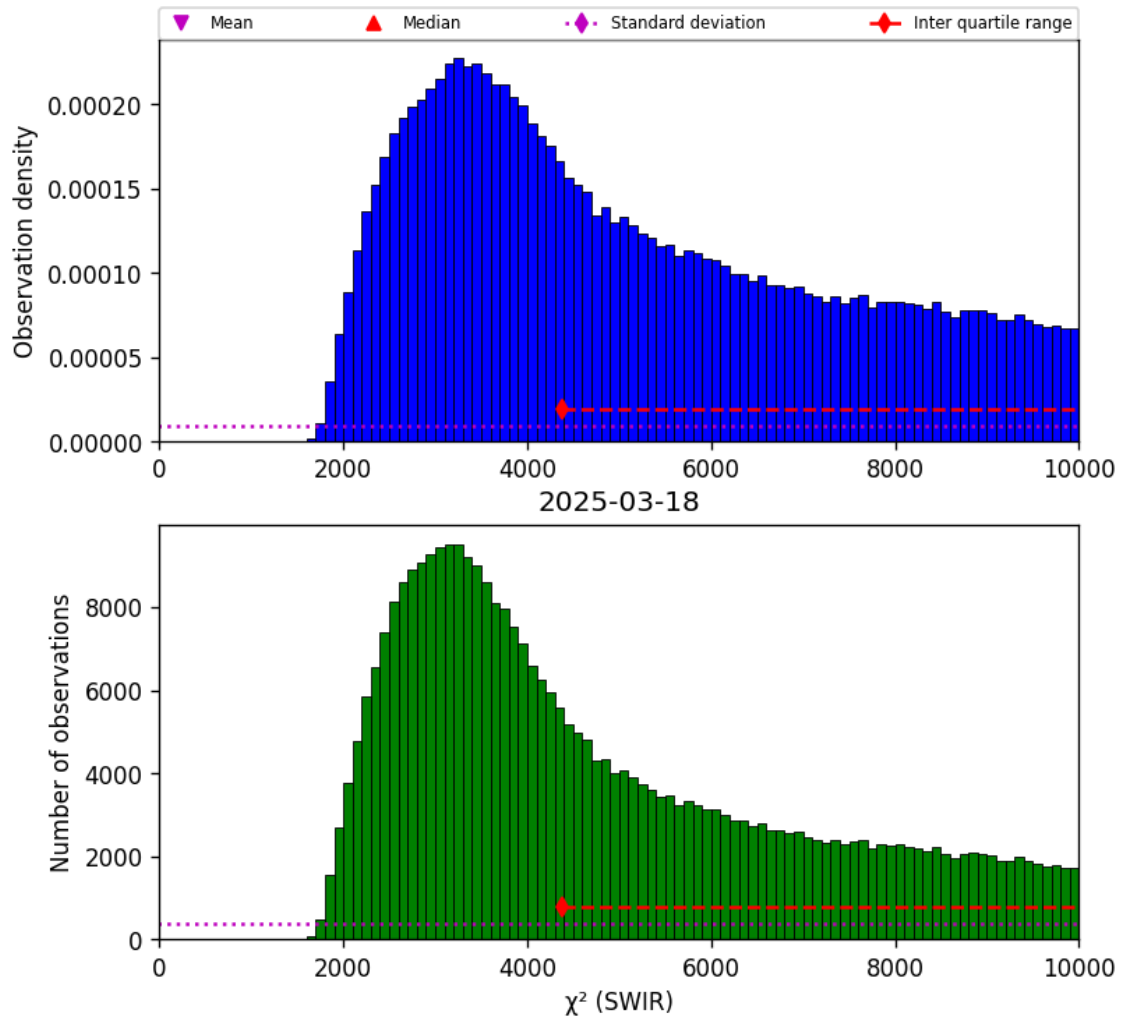
Figure 28: Histogram of " \chi^2 (SWIR)" for 2025-03-17 to 2025-03-19
