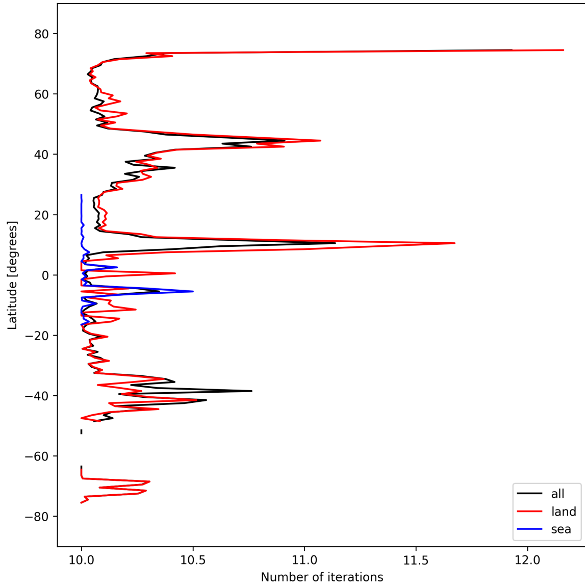
Figure 20: Zonal average of “Number of iterations” for 2025-03-17 to 2025-03-19.
