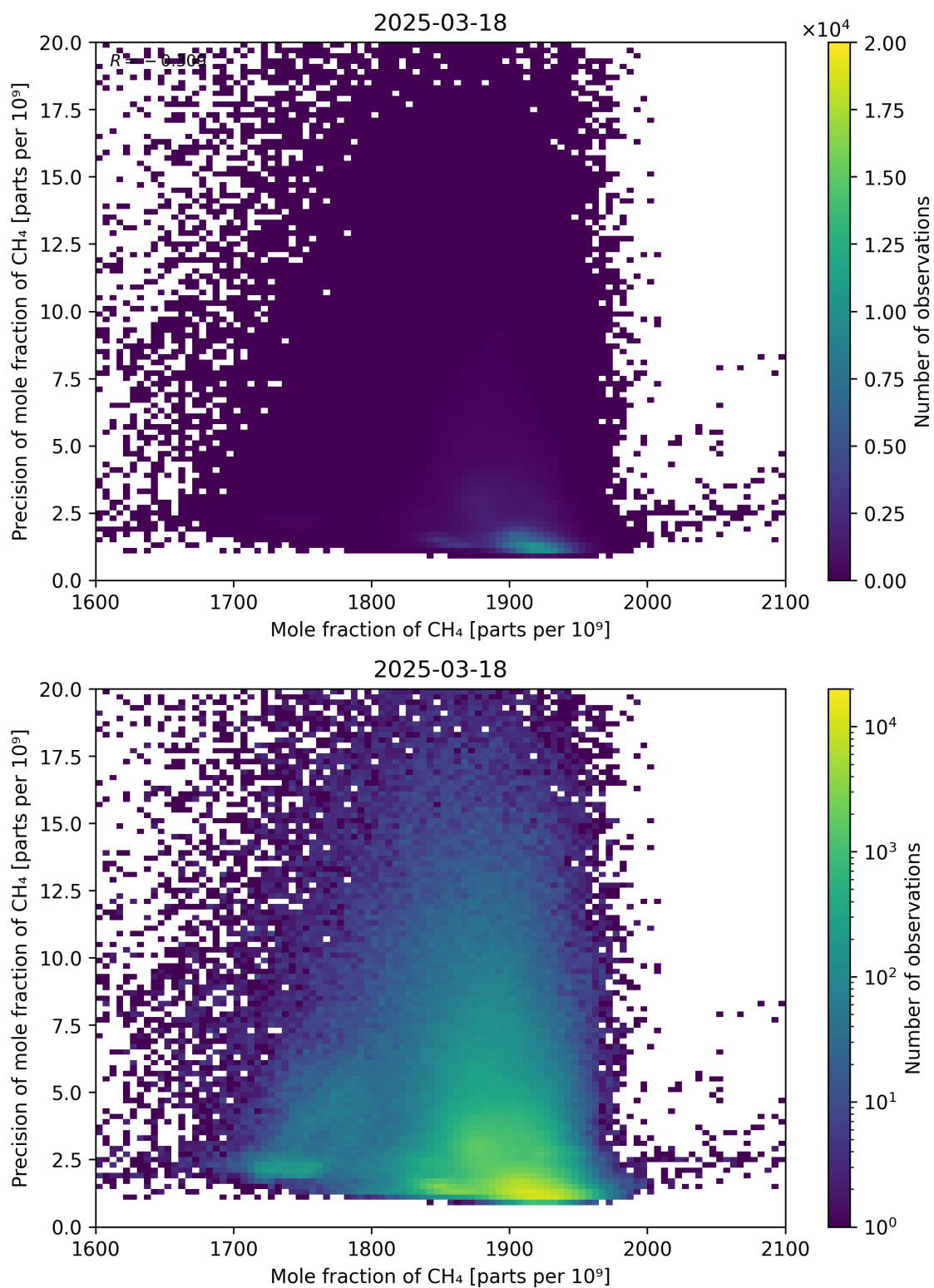
Figure 75: Scatter density plot of “Mole fraction of CH 4 ” against “Precision of mole fraction of CH 4 ” for 2025-03-17 to 2025-03-19.
