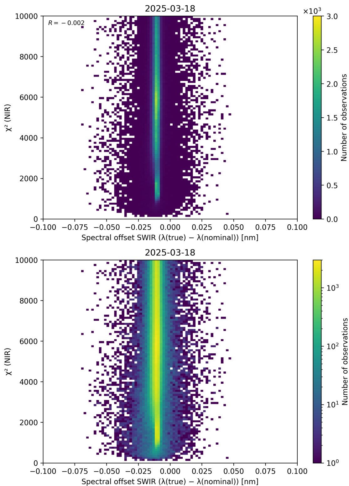
Figure 117: Scatter density plot of “Spectral offset SWIR ( \lambda_{\text{true}} - \lambda_{\text{nominal}} )” against “ \chi^2 (NIR)” for 2025-03-17 to 2025-03-19.
