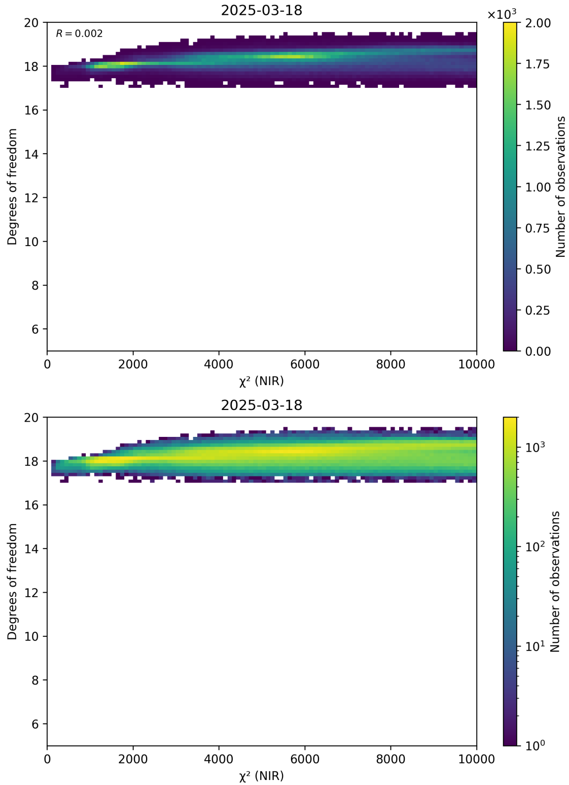
Figure 44: Scatter density plot of “ \chi^2 (NIR)” against “Degrees of freedom” for 2025-03-17 to 2025-03-19.
