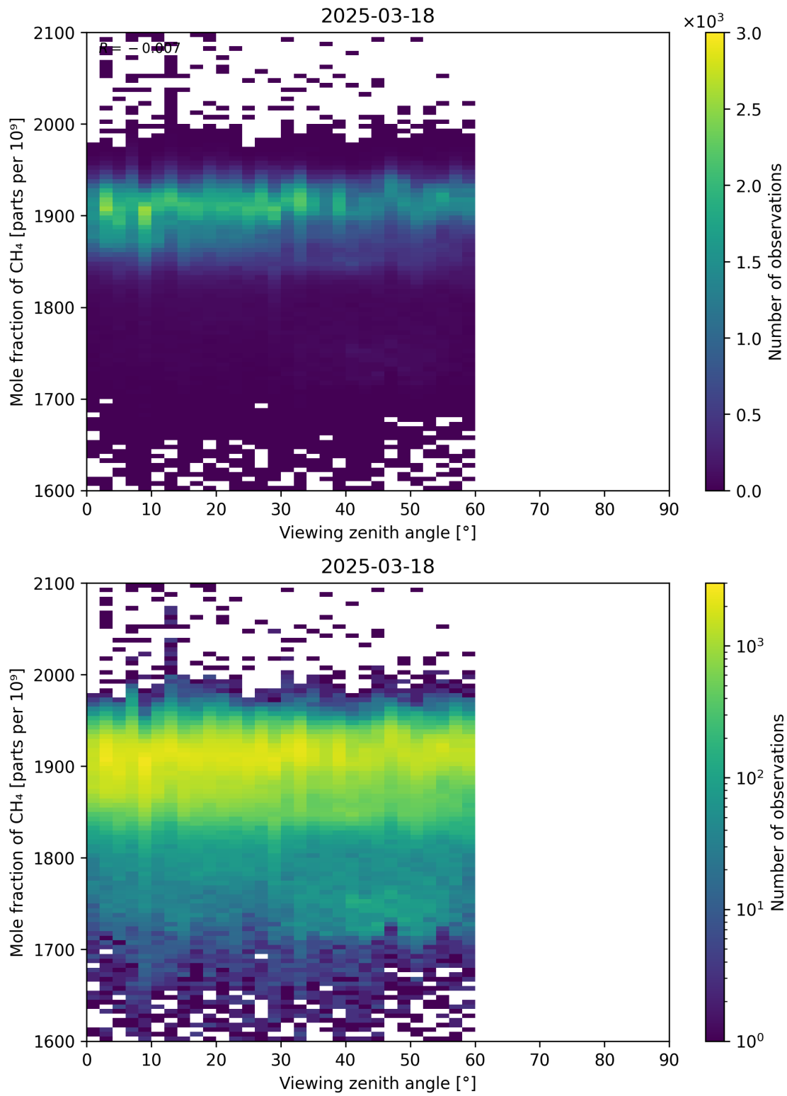
Figure 110: Scatter density plot of “Viewing zenith angle” against “Mole fraction of CH 4 ” for 2025-03-17 to 2025-03-19.
