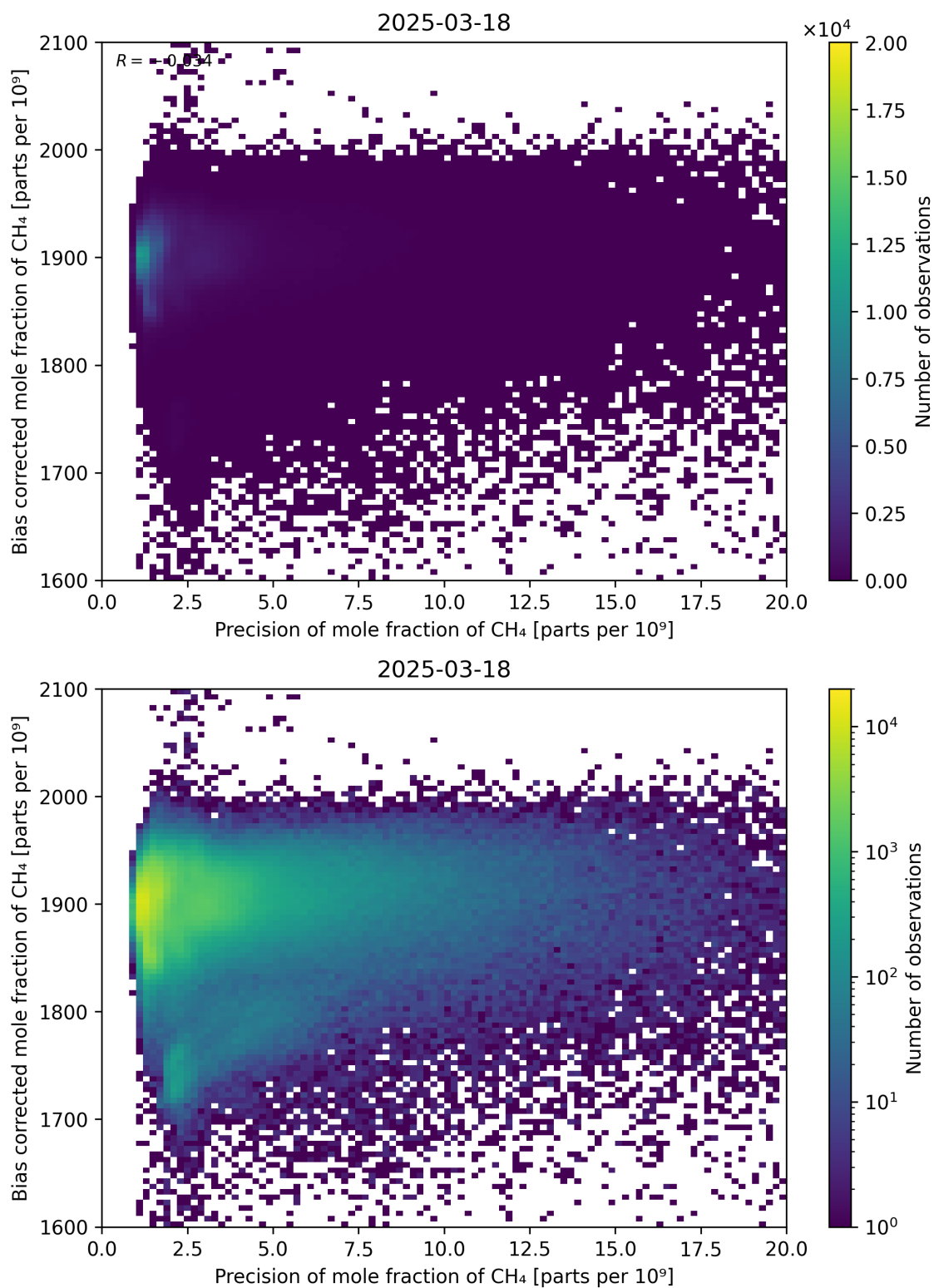
Figure 82: Scatter density plot of “Precision of mole fraction of CH 4 ” against “Bias corrected mole fraction of CH 4 ” for 2025-03-17 to 2025-03-19.
