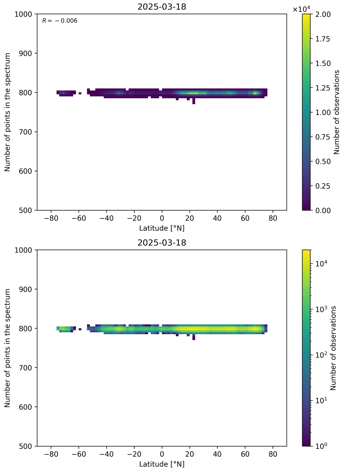
Figure 61: Scatter density plot of “Latitude” against “Number of points in the spectrum” for 2025-03-17 to 2025-03-19.
