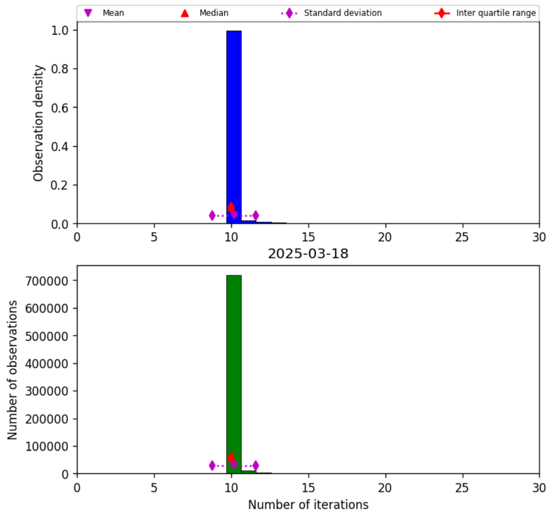
Figure 31: Histogram of “Number of iterations” for 2025-03-17 to 2025-03-19
