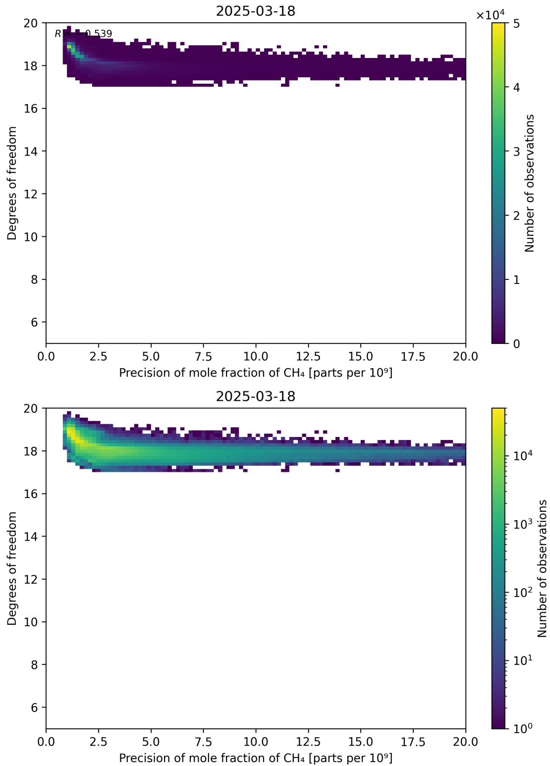
Figure 80: Scatter density plot of “Precision of mole fraction of CH 4 ” against “Degrees of freedom” for 2025-03-17 to 2025-03-19.
