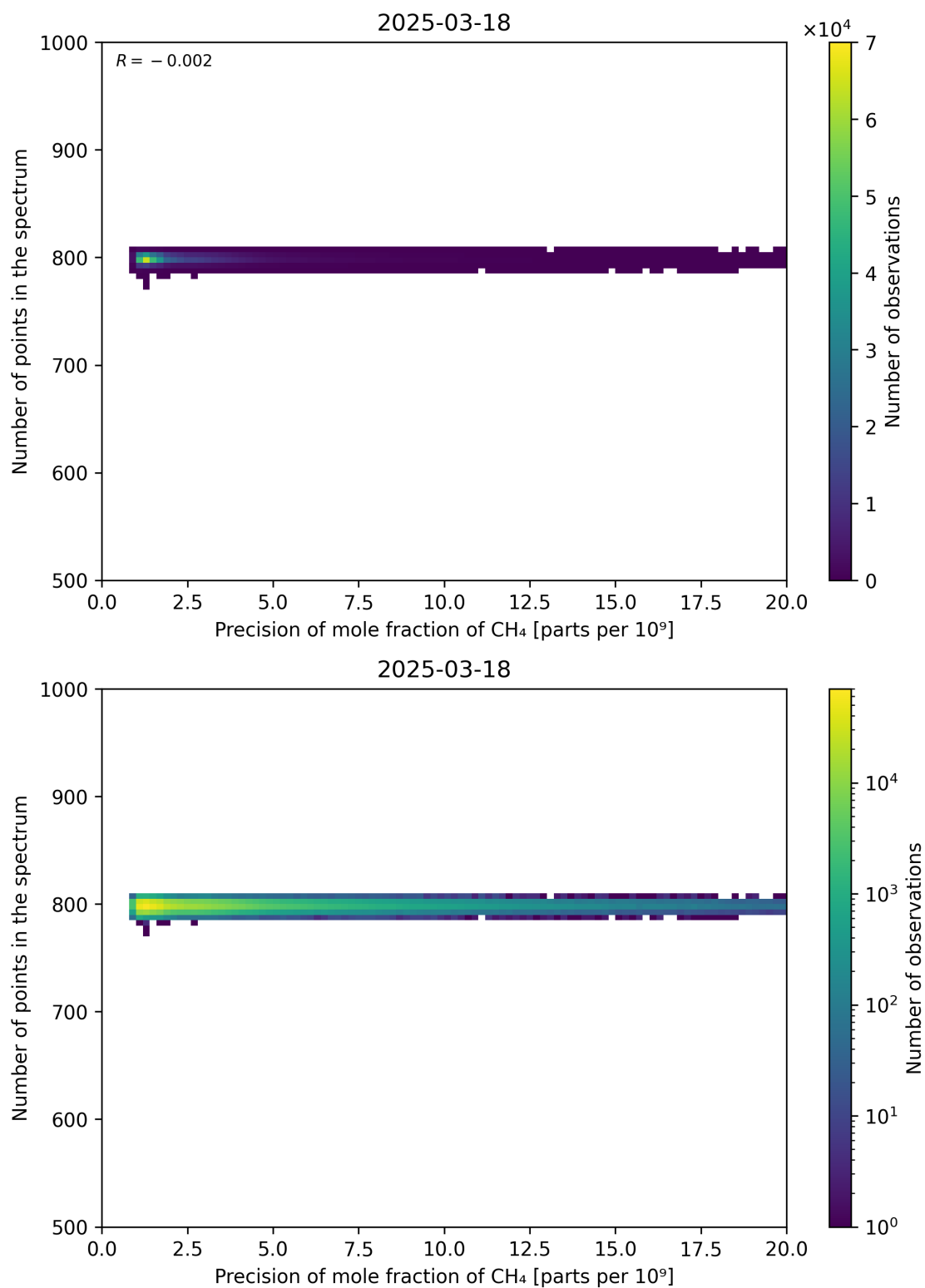
Figure 84: Scatter density plot of “Precision of mole fraction of CH 4 ” against “Number of points in the spectrum” for 2025-03-17 to 2025-03-19.
