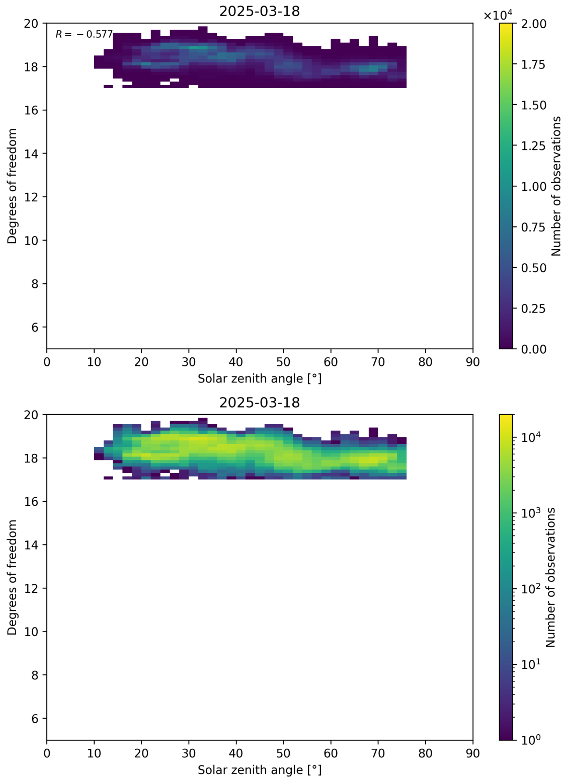
Figure 96: Scatter density plot of “Solar zenith angle” against “Degrees of freedom” for 2025-03-17 to 2025-03-19.
