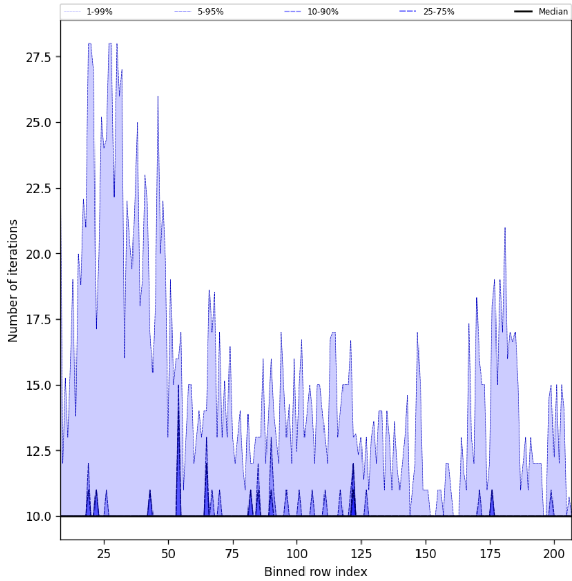
Figure 42: Along track statistics of “Number of iterations” for 2025-03-17 to 2025-03-19
