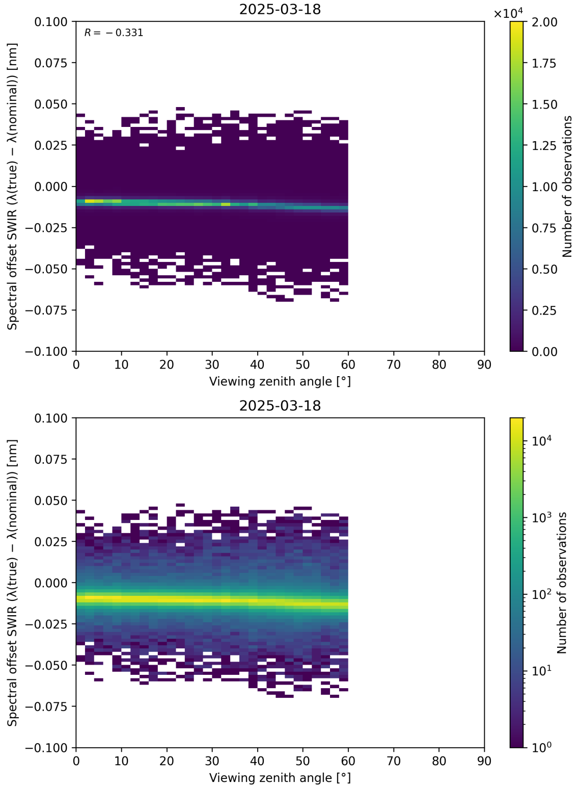
Figure 116: Scatter density plot of “Viewing zenith angle” against “Spectral offset SWIR ( \lambda_{\text{true}} - \lambda_{\text{nominal}} )” for 2025-03-17 to 2025-03-19.
