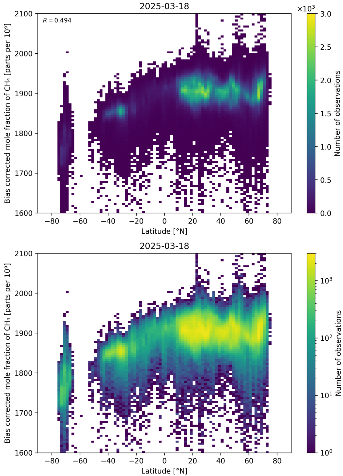
Figure 58: Scatter density plot of “Latitude” against “Bias corrected mole fraction of \text{CH}_4 ” for 2025-03-17 to 2025-03-19.
