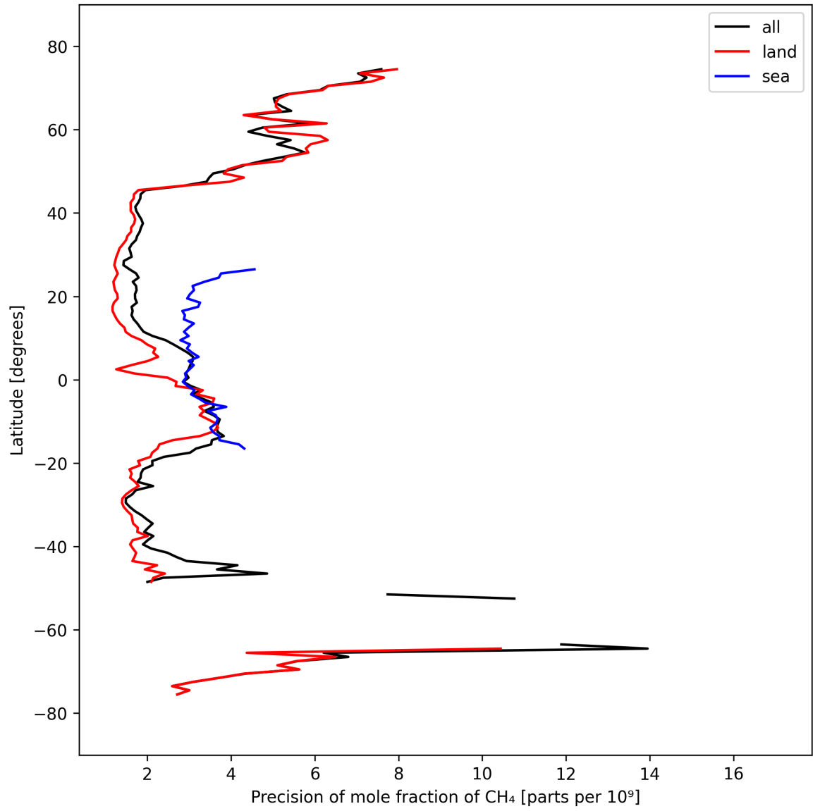
Figure 13: Zonal average of “Precision of mole fraction of CH 4 ” for 2025-03-17 to 2025-03-19.
