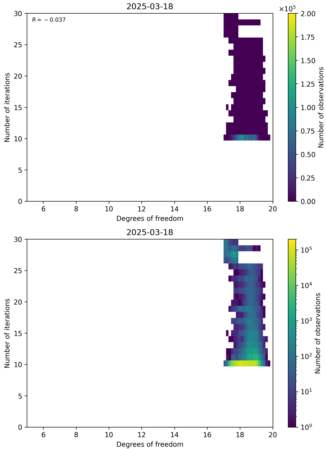
Figure 52: Scatter density plot of “Degrees of freedom” against “Number of iterations” for 2025-03-17 to 2025-03-19.
