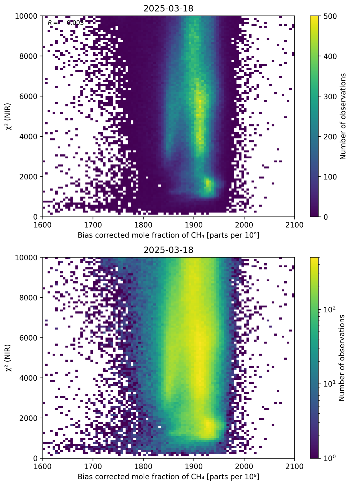
Figure 63: Scatter density plot of “Bias corrected mole fraction of \text{CH}_4 ” against “ \chi^2 (NIR)” for 2025-03-17 to 2025-03-19.
