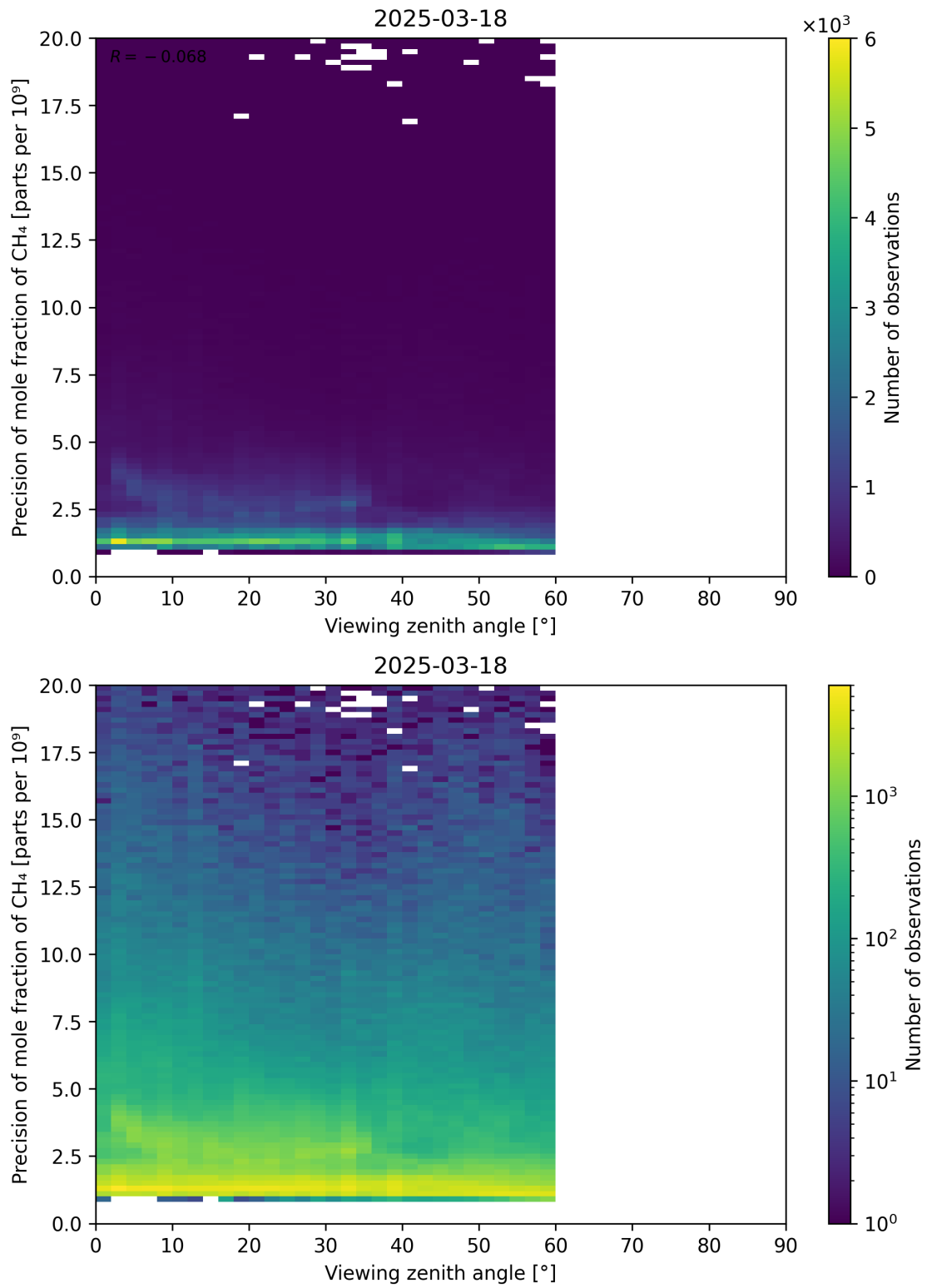
Figure 112: Scatter density plot of “Viewing zenith angle” against “Precision of mole fraction of CH 4 ” for 2025-03-17 to 2025-03-19.
