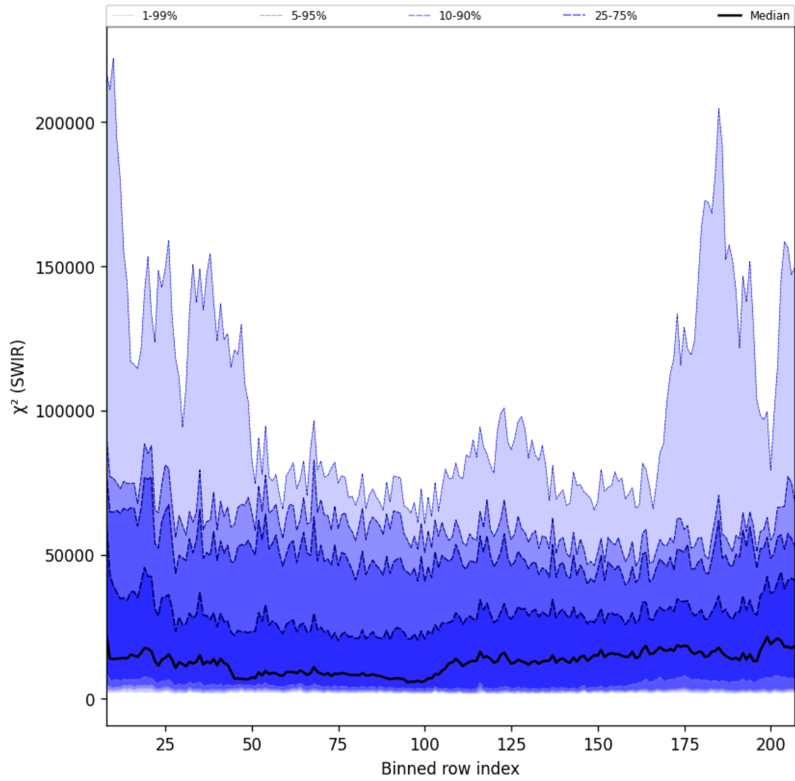
Figure 39: Along track statistics of “ \chi^2 (SWIR)” for 2025-03-17 to 2025-03-19
