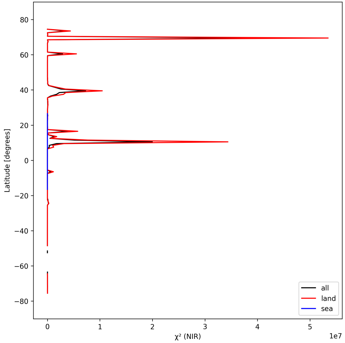
Figure 18: Zonal average of “ \chi^2 (NIR)” for 2025-03-17 to 2025-03-19.
