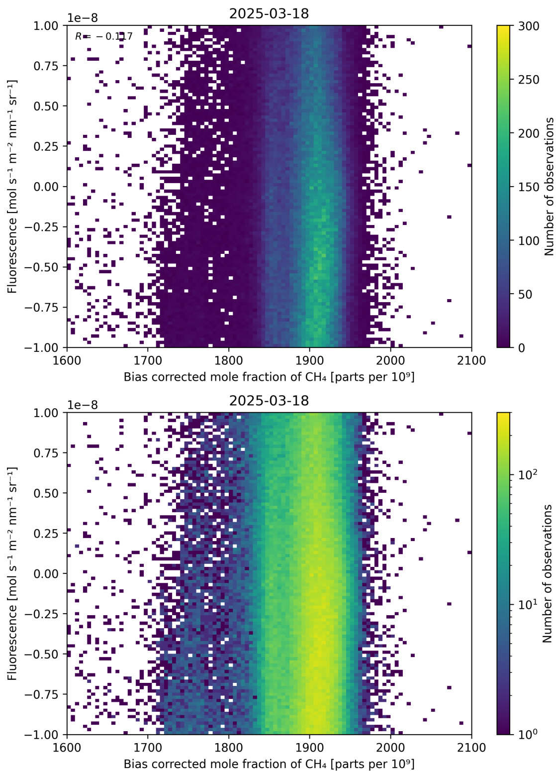
Figure 66: Scatter density plot of “Bias corrected mole fraction of \text{CH}_4 ” against “Fluorescence” for 2025-03-17 to 2025-03-19.
