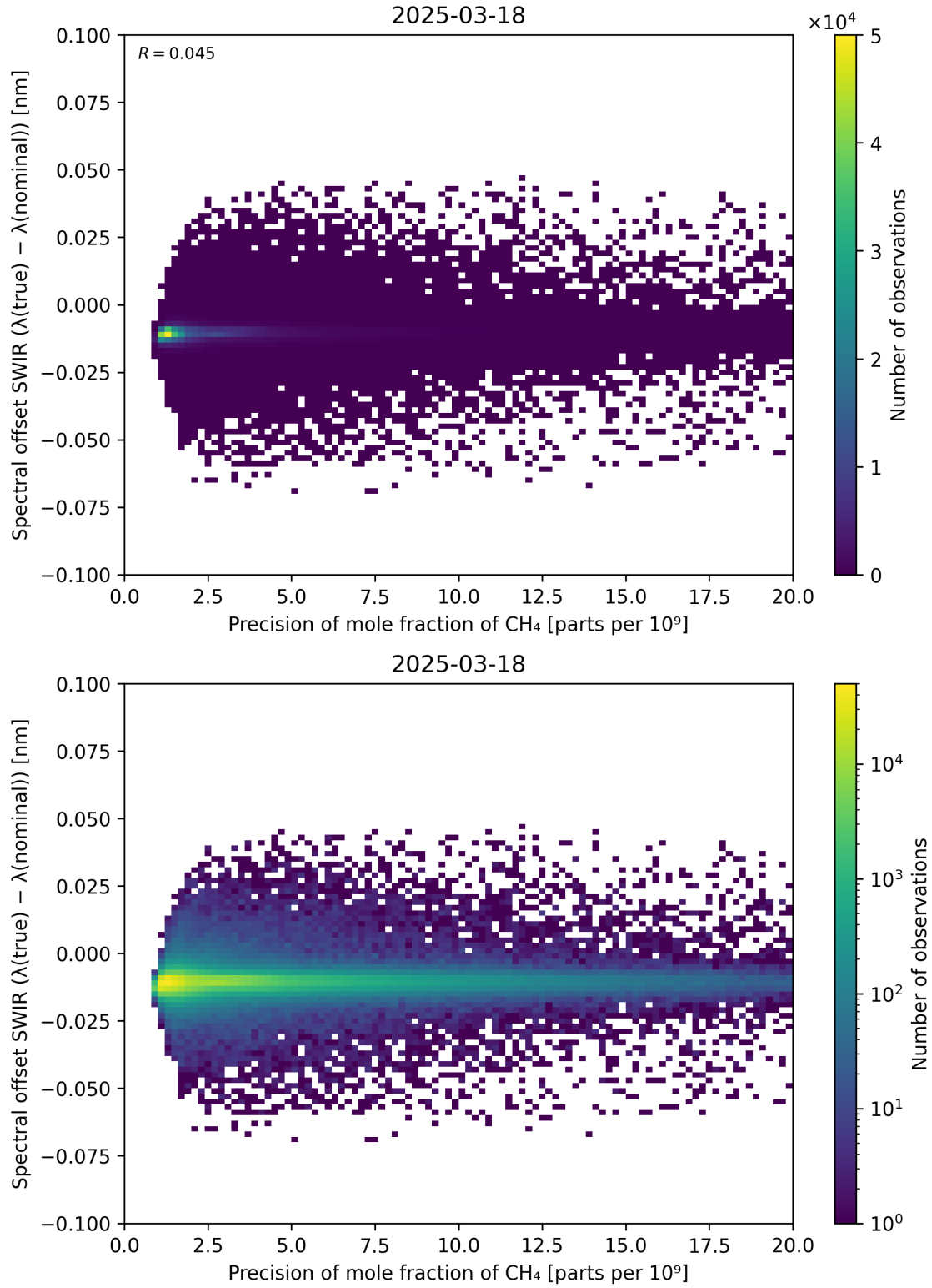
Figure 85: Scatter density plot of “Precision of mole fraction of CH 4 ” against “Spectral offset SWIR ( \lambda_{\text{true}} - \lambda_{\text{nominal}} )” for 2025-03-17 to 2025-03-19.
