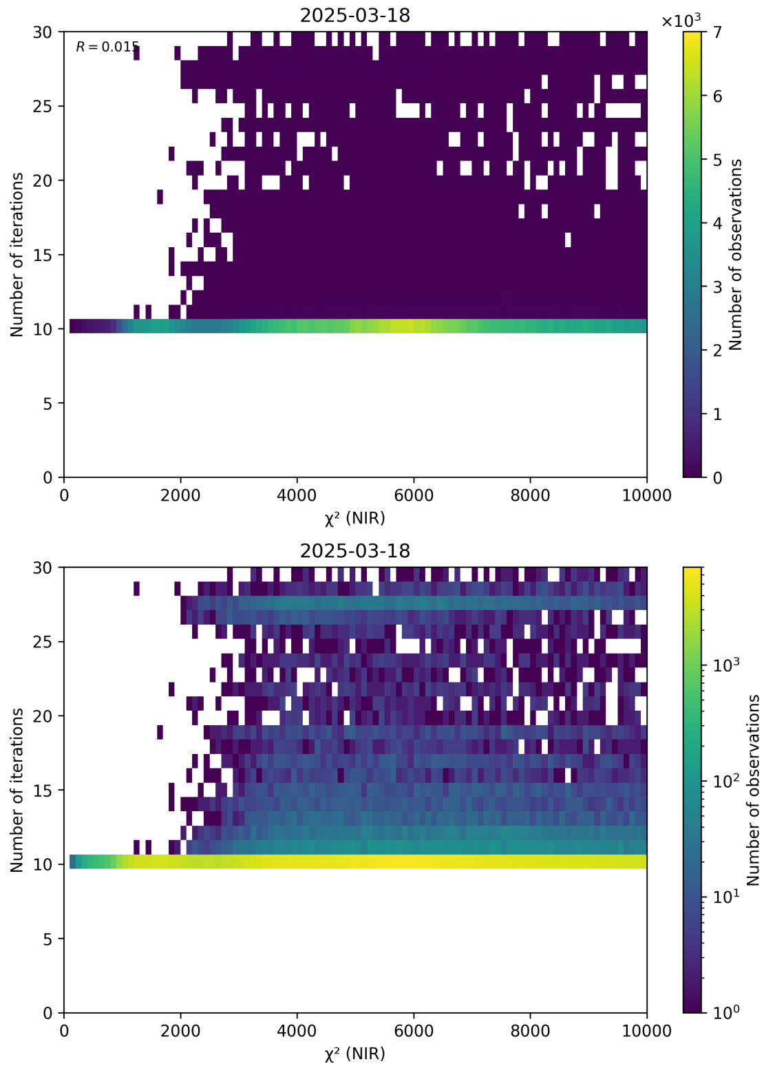
Figure 46: Scatter density plot of “ \chi^2 (NIR)” against “Number of iterations” for 2025-03-17 to 2025-03-19.
