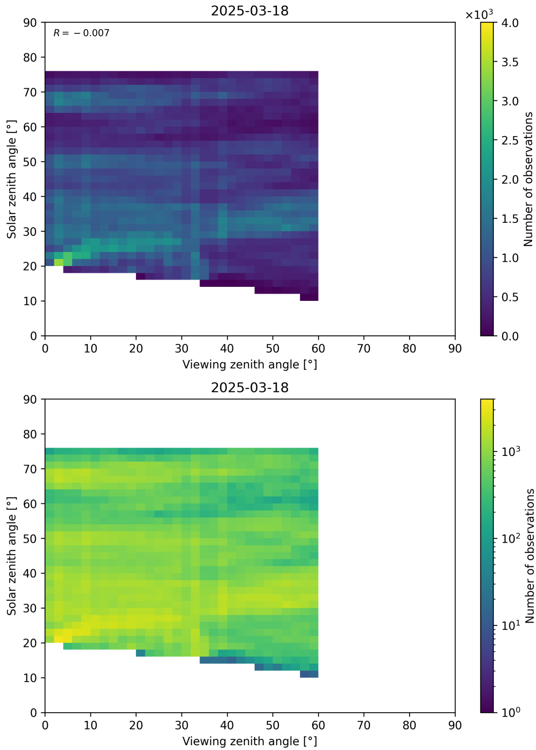
Figure 115: Scatter density plot of “Viewing zenith angle” against “Solar zenith angle” for 2025-03-17 to 2025-03-19.
