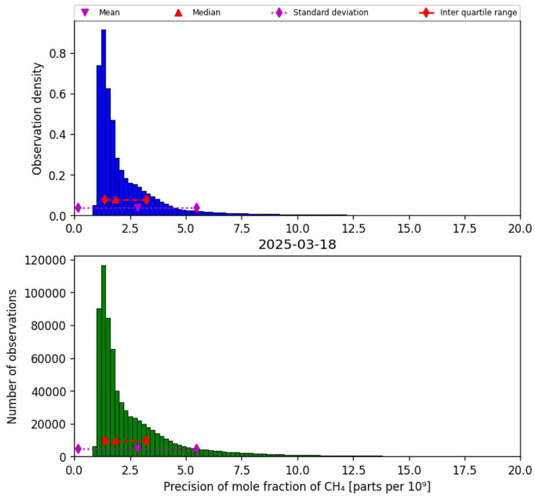
Figure 24: Histogram of “Precision of mole fraction of CH 4 ” for 2025-03-17 to 2025-03-19
