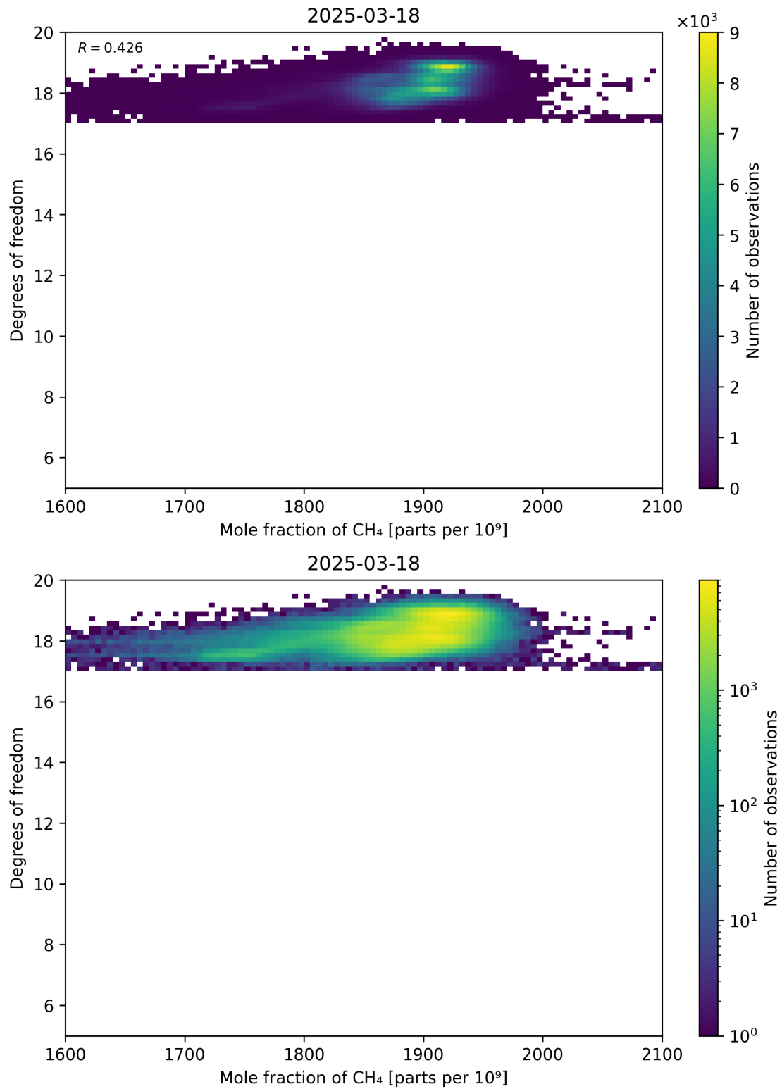
Figure 72: Scatter density plot of “Mole fraction of CH 4 ” against “Degrees of freedom” for 2025-03-17 to 2025-03-19.
