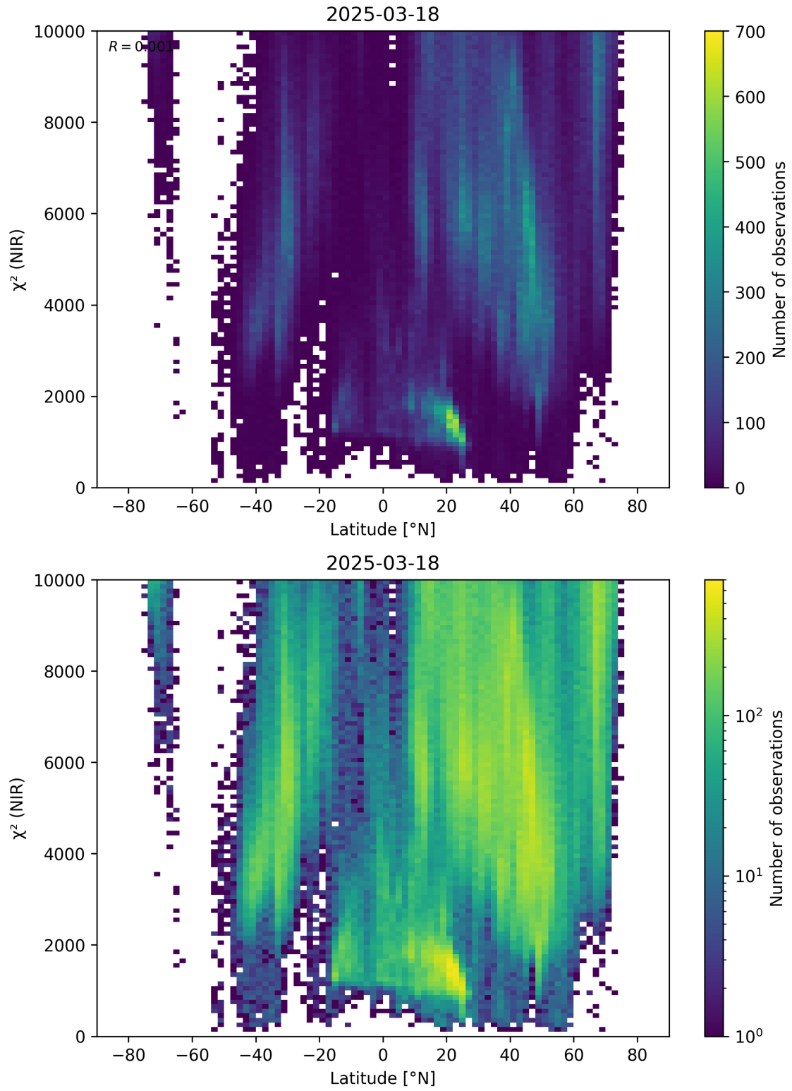
Figure 53: Scatter density plot of “Latitude” against “ \chi^2 (NIR)” for 2025-03-17 to 2025-03-19.
