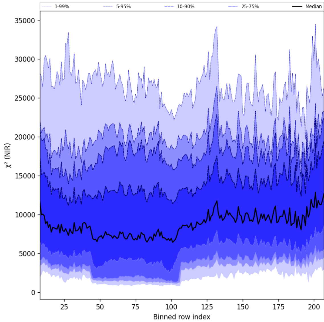
Figure 40: Along track statistics of “ \chi^2 (NIR)” for 2025-03-17 to 2025-03-19
