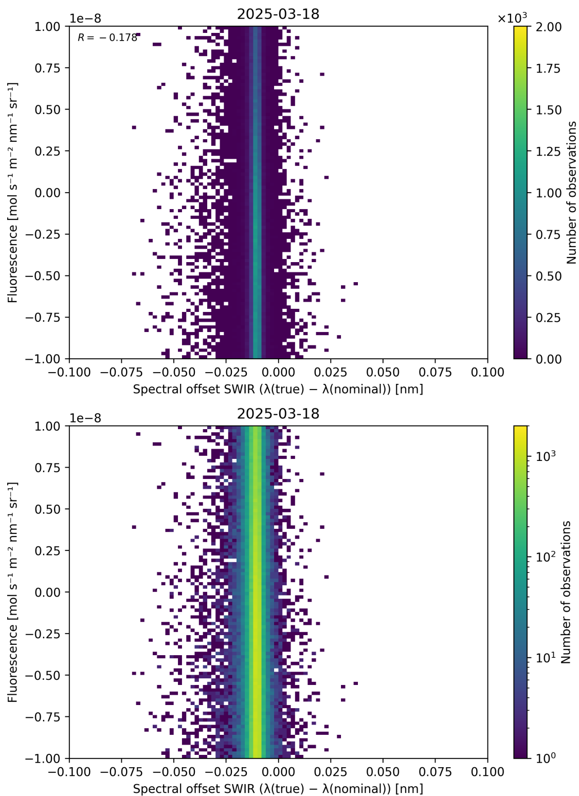
Figure 120: Scatter density plot of “Spectral offset SWIR ( \lambda_{\text{true}} - \lambda_{\text{nominal}} )” against “Fluorescence” for 2025-03-17 to 2025-03-19.
