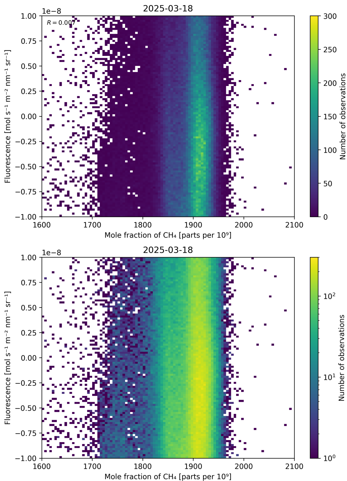
Figure 73: Scatter density plot of “Mole fraction of CH 4 ” against “Fluorescence” for 2025-03-17 to 2025-03-19.
