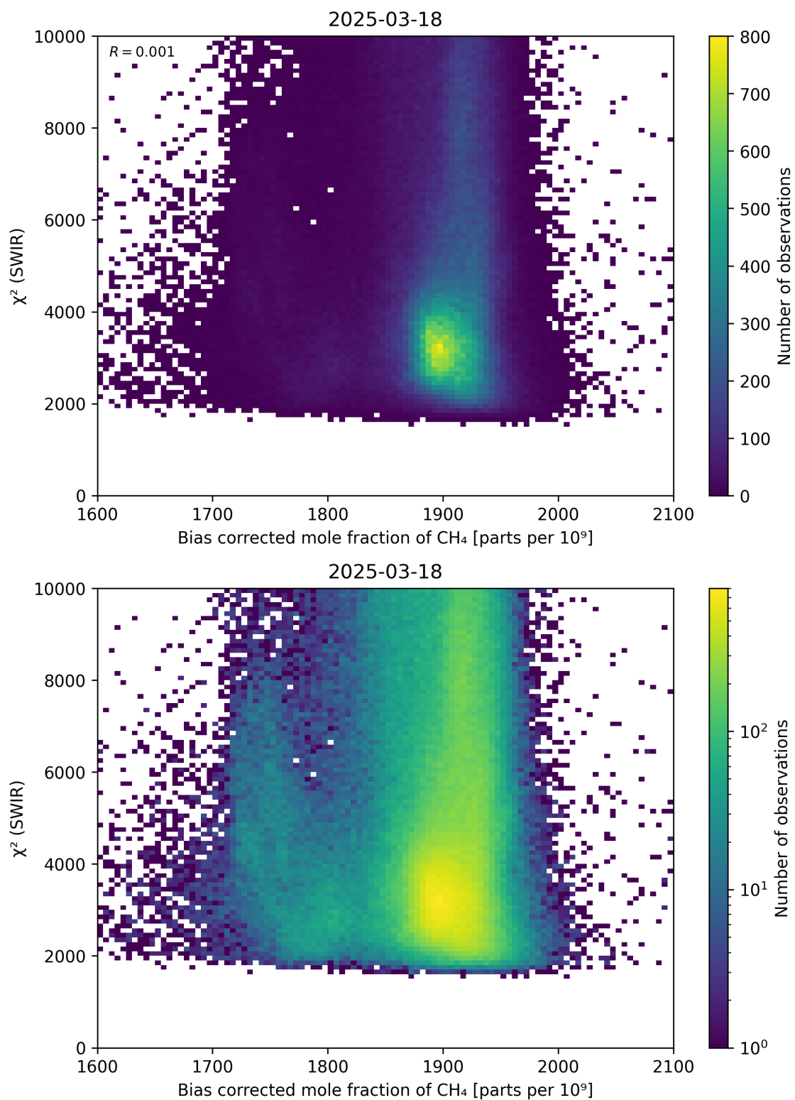
Figure 64: Scatter density plot of “Bias corrected mole fraction of CH 4 ” against “ \chi^2 (SWIR)” for 2025-03-17 to 2025-03-19.
