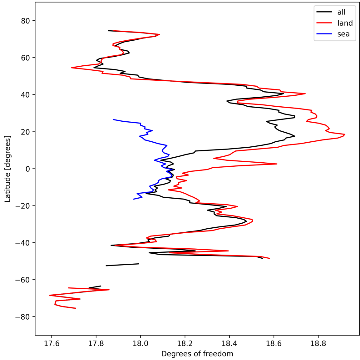
Figure 19: Zonal average of “Degrees of freedom” for 2025-03-17 to 2025-03-19.
