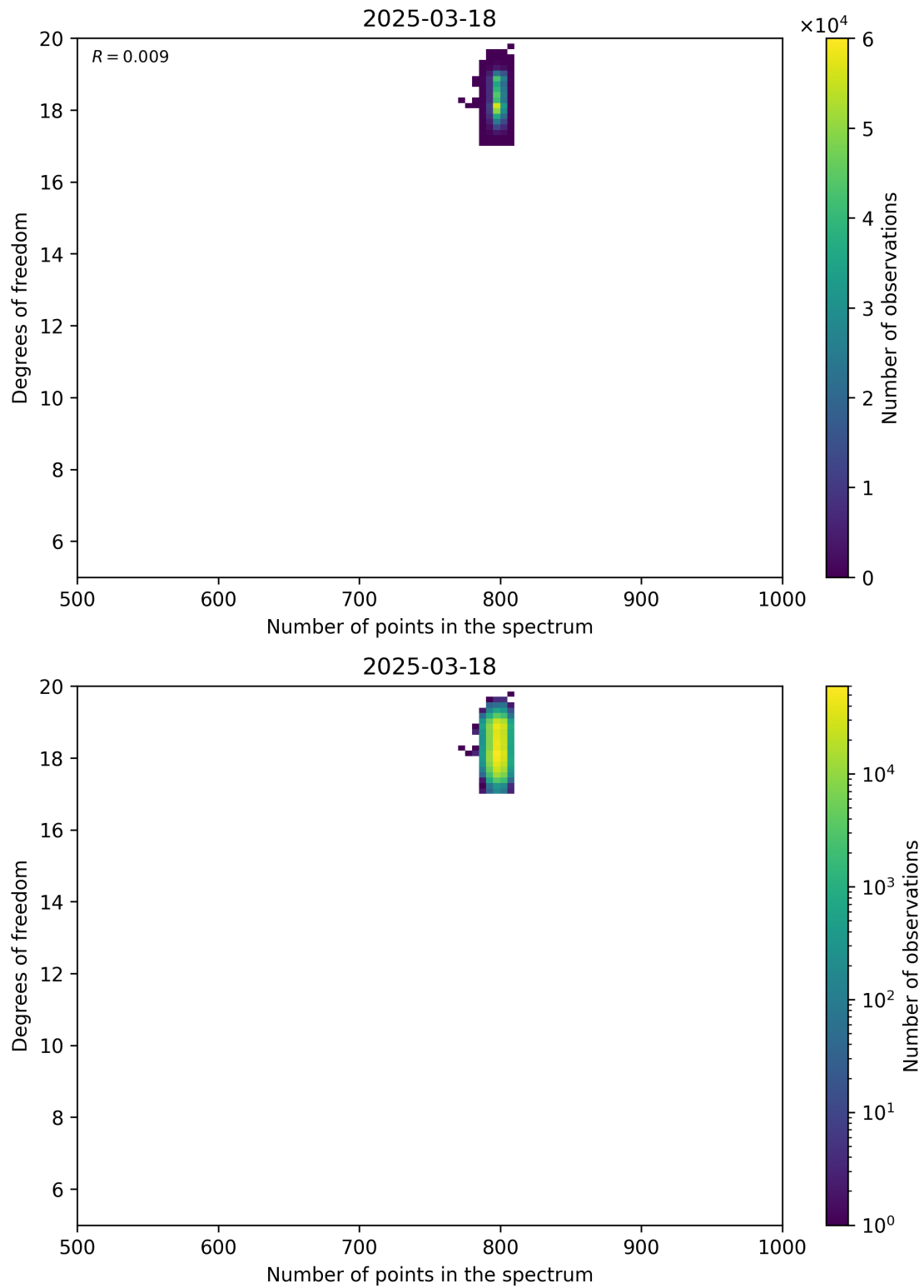
Figure 90: Scatter density plot of “Number of points in the spectrum” against “Degrees of freedom” for 2025-03-17 to 2025-03-19.
