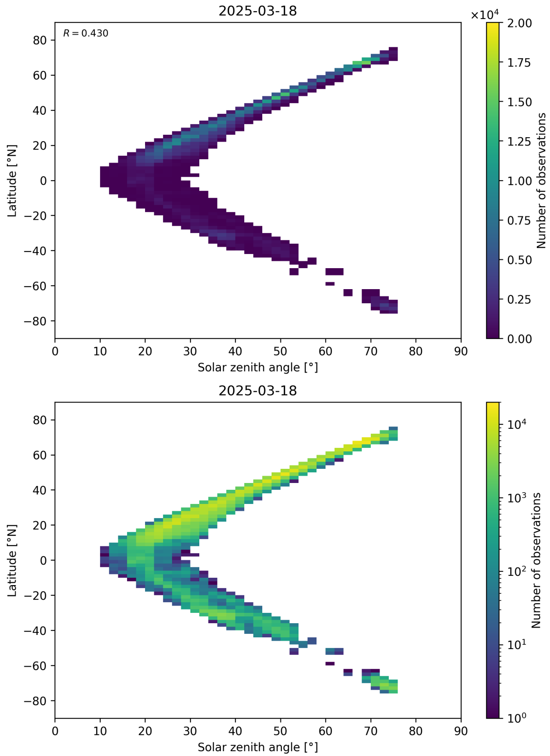
Figure 98: Scatter density plot of “Solar zenith angle” against “Latitude” for 2025-03-17 to 2025-03-19.
