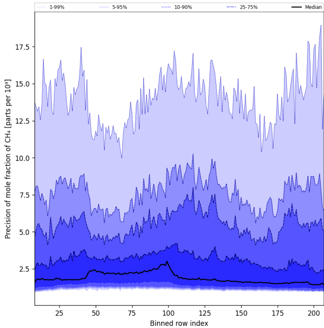
Figure 35: Along track statistics of “Precision of mole fraction of CH 4 ” for 2025-03-17 to 2025-03-19
