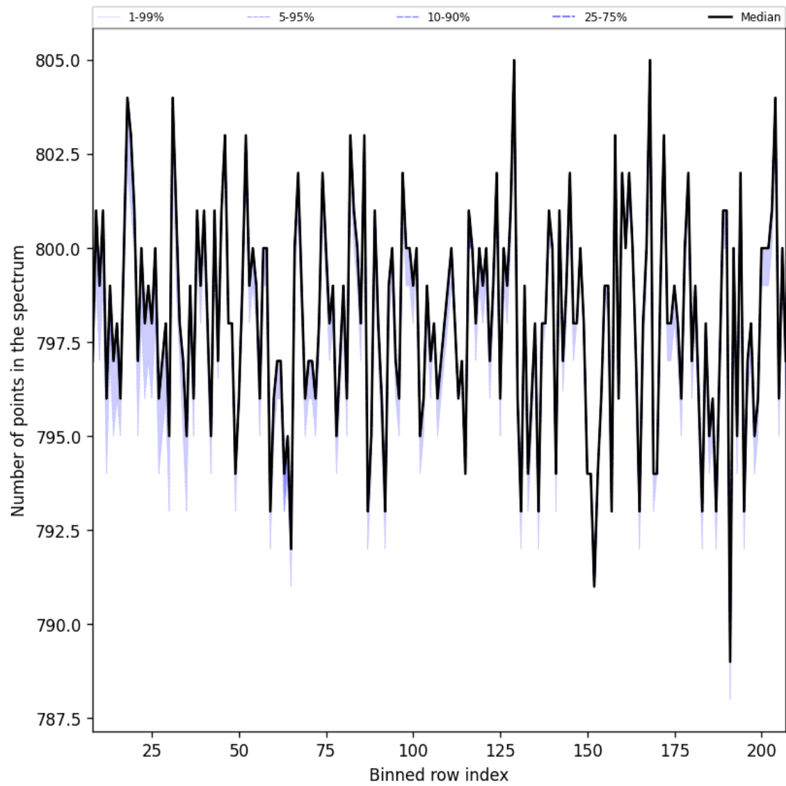
Figure 37: Along track statistics of “Number of points in the spectrum” for 2025-03-17 to 2025-03-19
