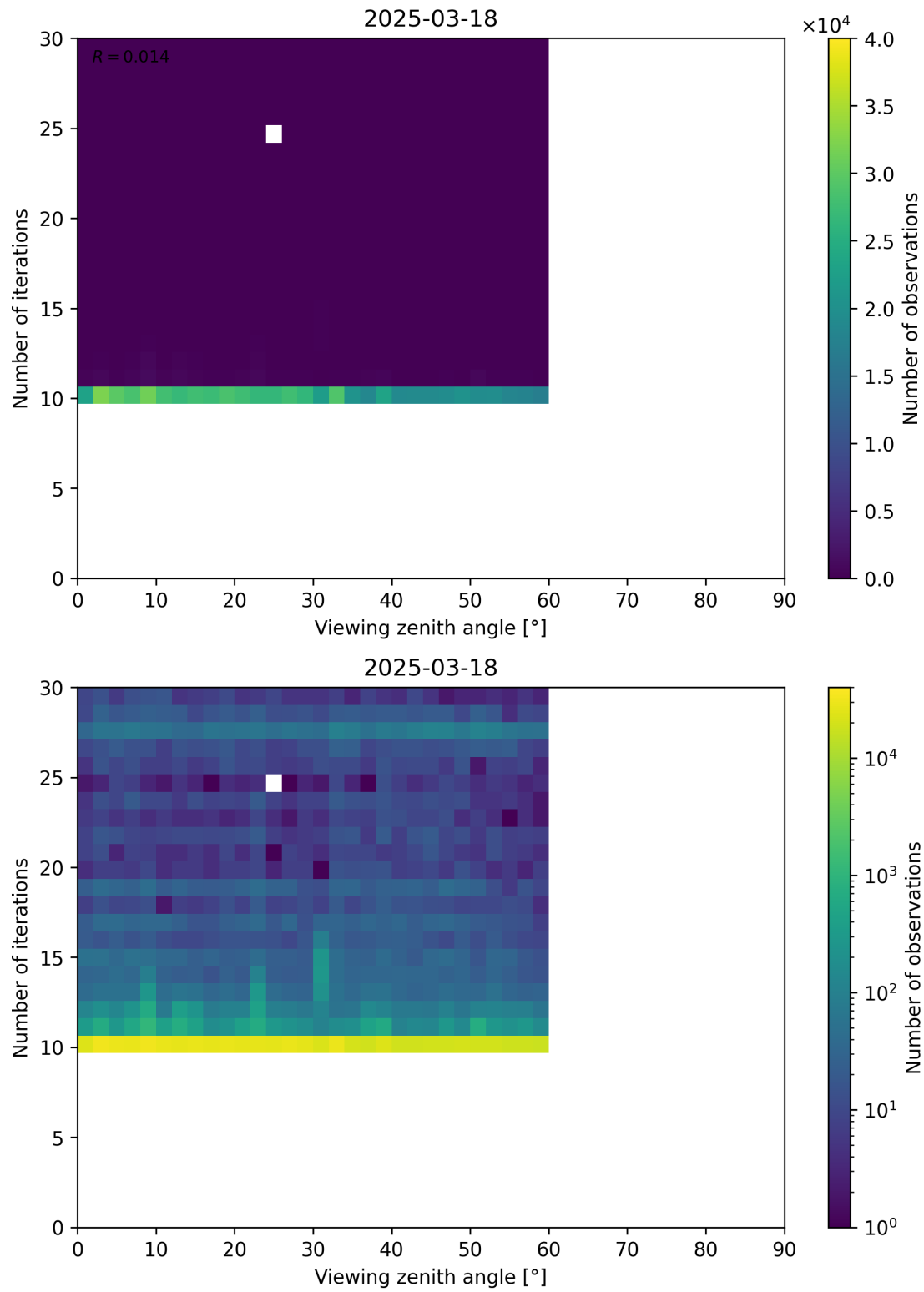
Figure 113: Scatter density plot of “Viewing zenith angle” against “Number of iterations” for 2025-03-17 to 2025-03-19.
