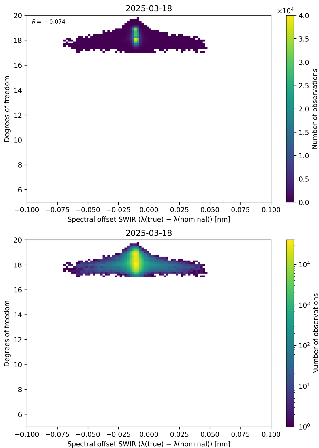
Figure 119: Scatter density plot of “Spectral offset SWIR ( \lambda_{\text{true}} - \lambda_{\text{nominal}} )” against “Degrees of freedom” for 2025-03-17 to 2025-03-19.
