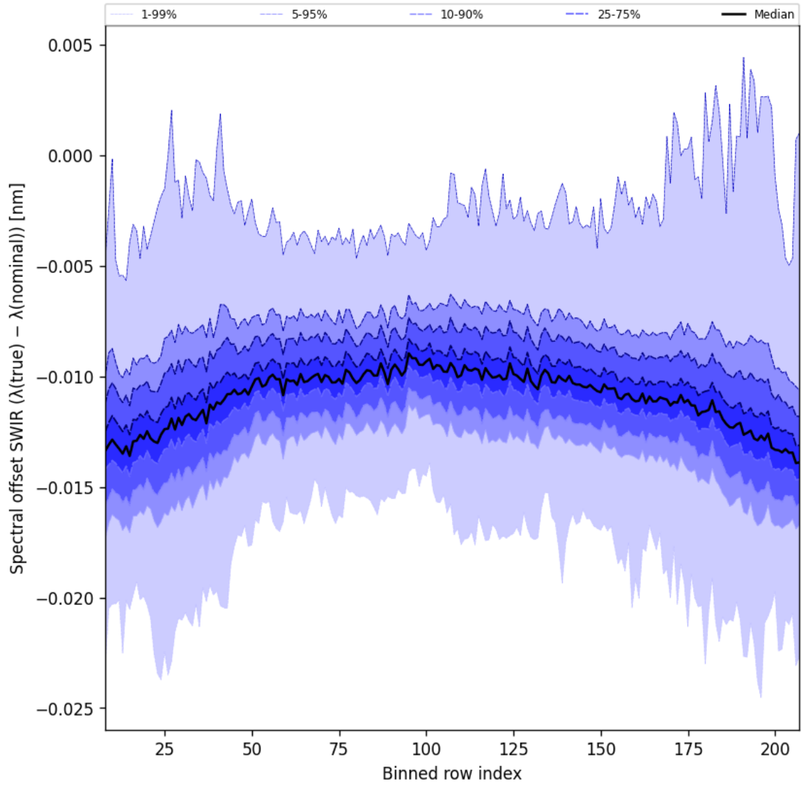
Figure 38: Along track statistics of “Spectral offset SWIR ( \lambda_{\text{true}} - \lambda_{\text{nominal}} )” for 2025-03-17 to 2025-03-19
