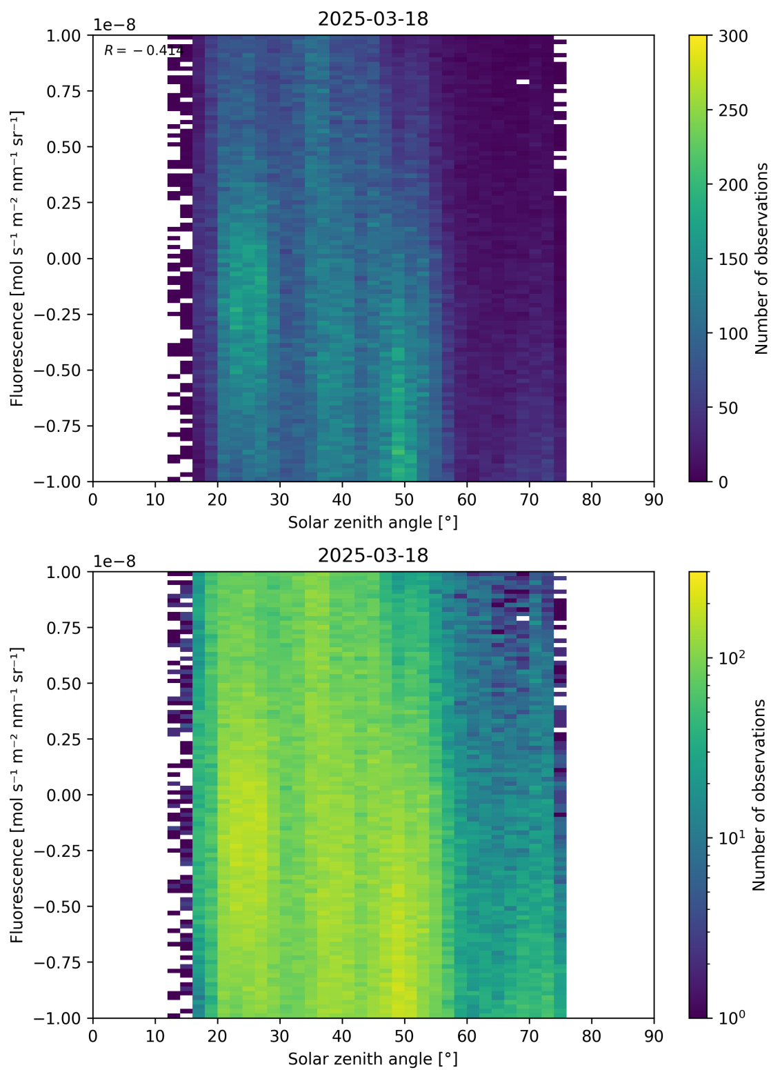
Figure 97: Scatter density plot of “Solar zenith angle” against “Fluorescence” for 2025-03-17 to 2025-03-19.
