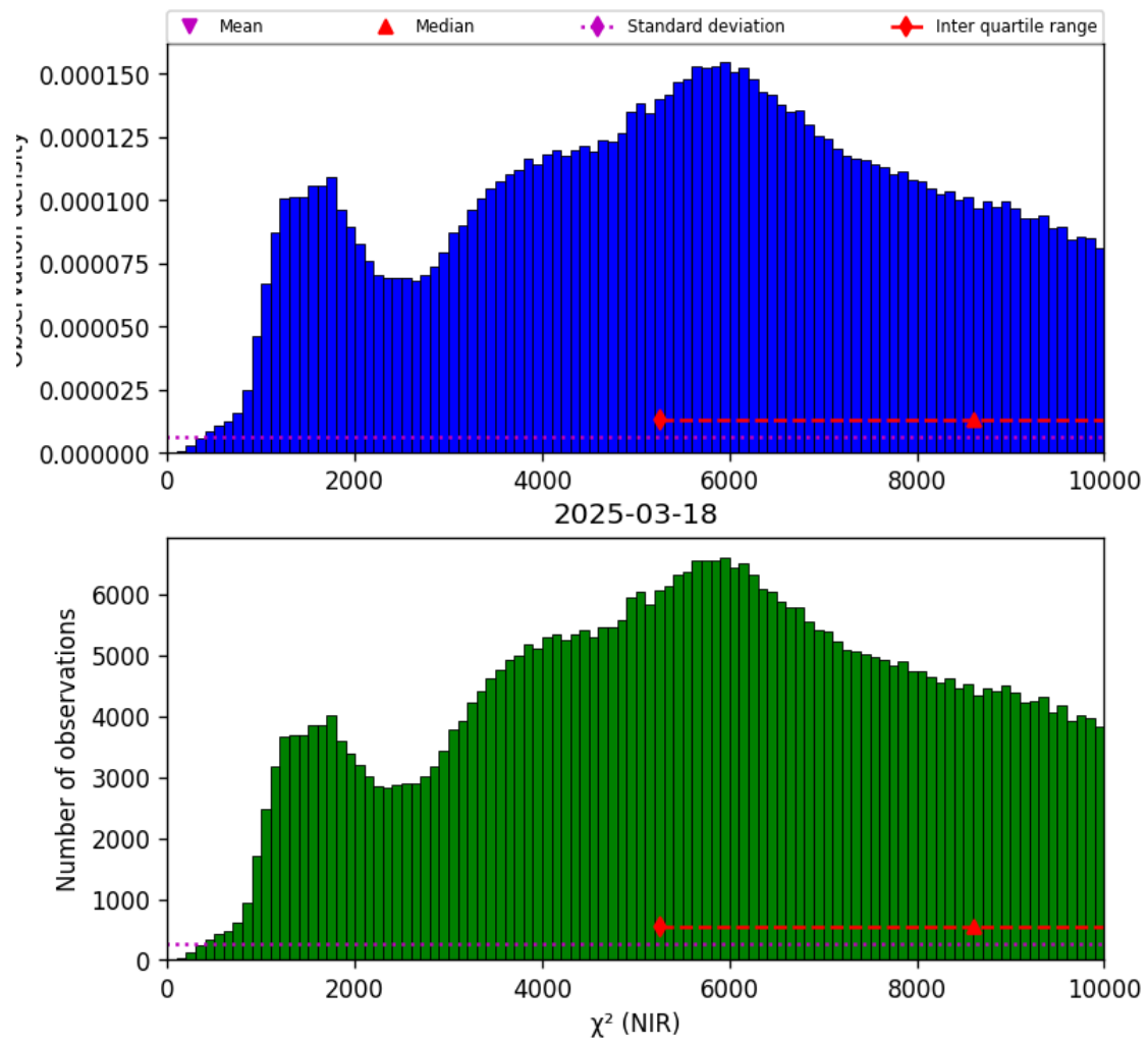
Figure 29: Histogram of “ \chi^2 (NIR)” for 2025-03-17 to 2025-03-19
