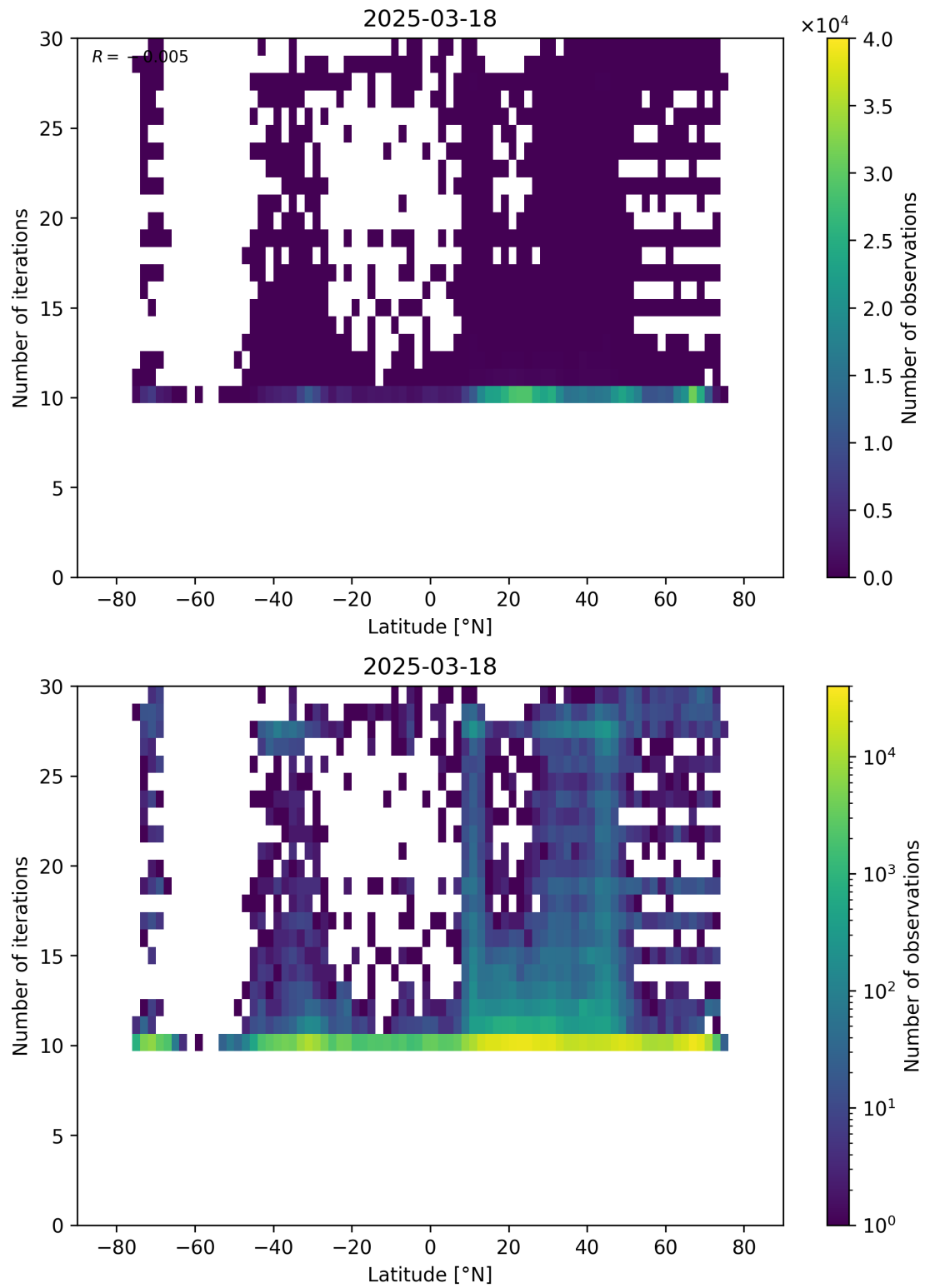
Figure 60: Scatter density plot of “Latitude” against “Number of iterations” for 2025-03-17 to 2025-03-19.
