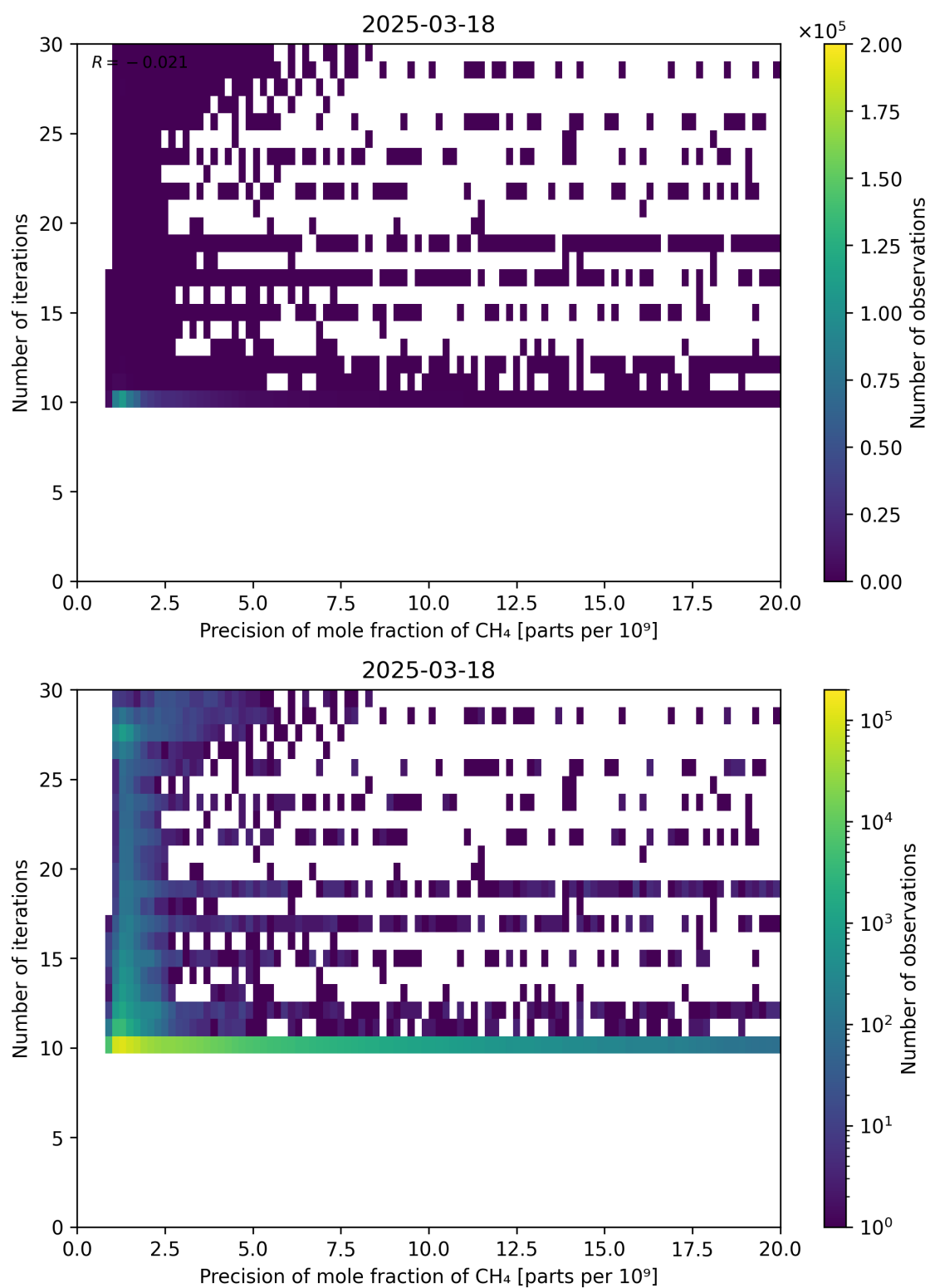
Figure 83: Scatter density plot of “Precision of mole fraction of CH 4 ” against “Number of iterations” for 2025-03-17 to 2025-03-19.
