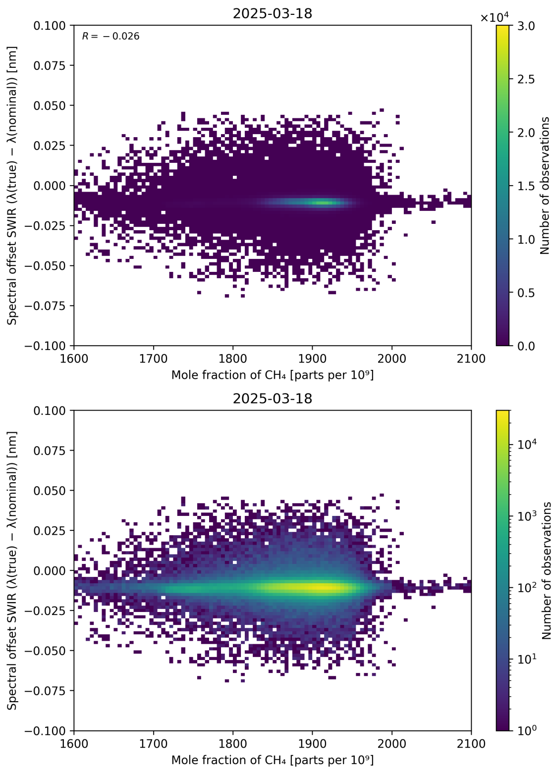
Figure 86: Scatter density plot of “Mole fraction of CH 4 ” against “Spectral offset SWIR ( \lambda_{\text{true}} - \lambda_{\text{nominal}} )” for 2025-03-17 to 2025-03-19.
