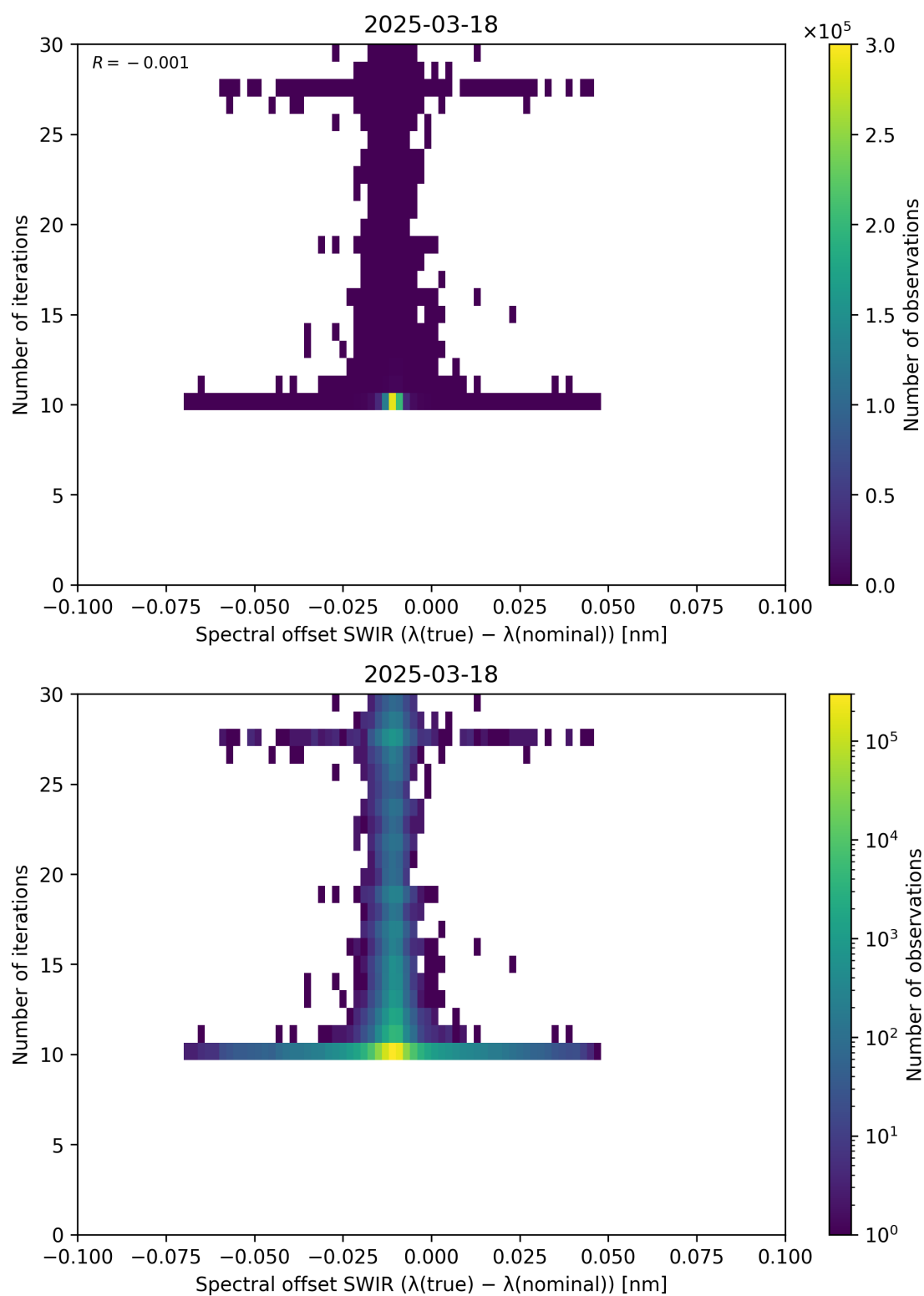
Figure 121: Scatter density plot of “Spectral offset SWIR ( \lambda_{\text{true}} - \lambda_{\text{nominal}} )” against “Number of iterations” for 2025-03-17 to 2025-03-19.
