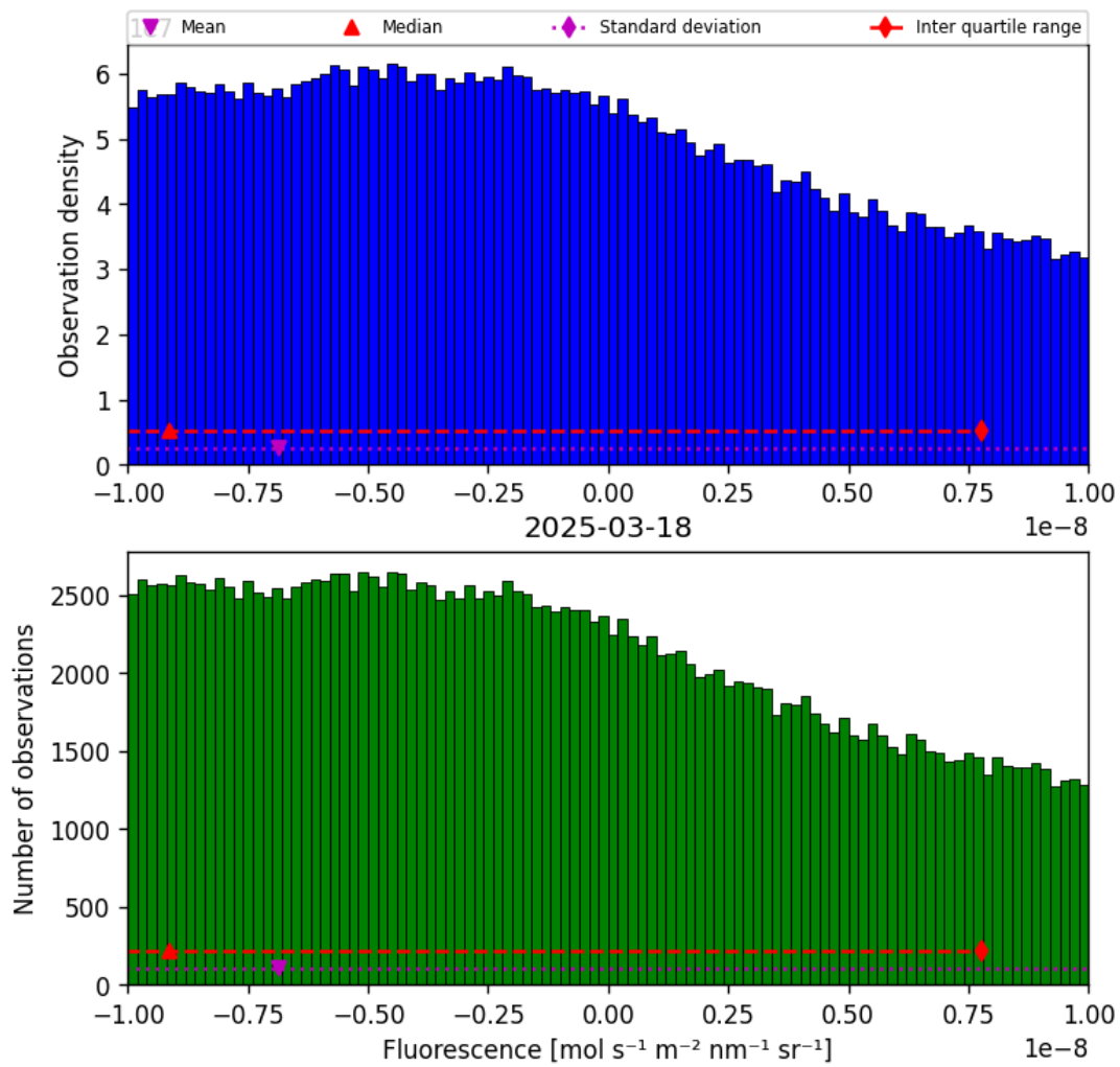
Figure 32: Histogram of “Fluorescence” for 2025-03-17 to 2025-03-19
