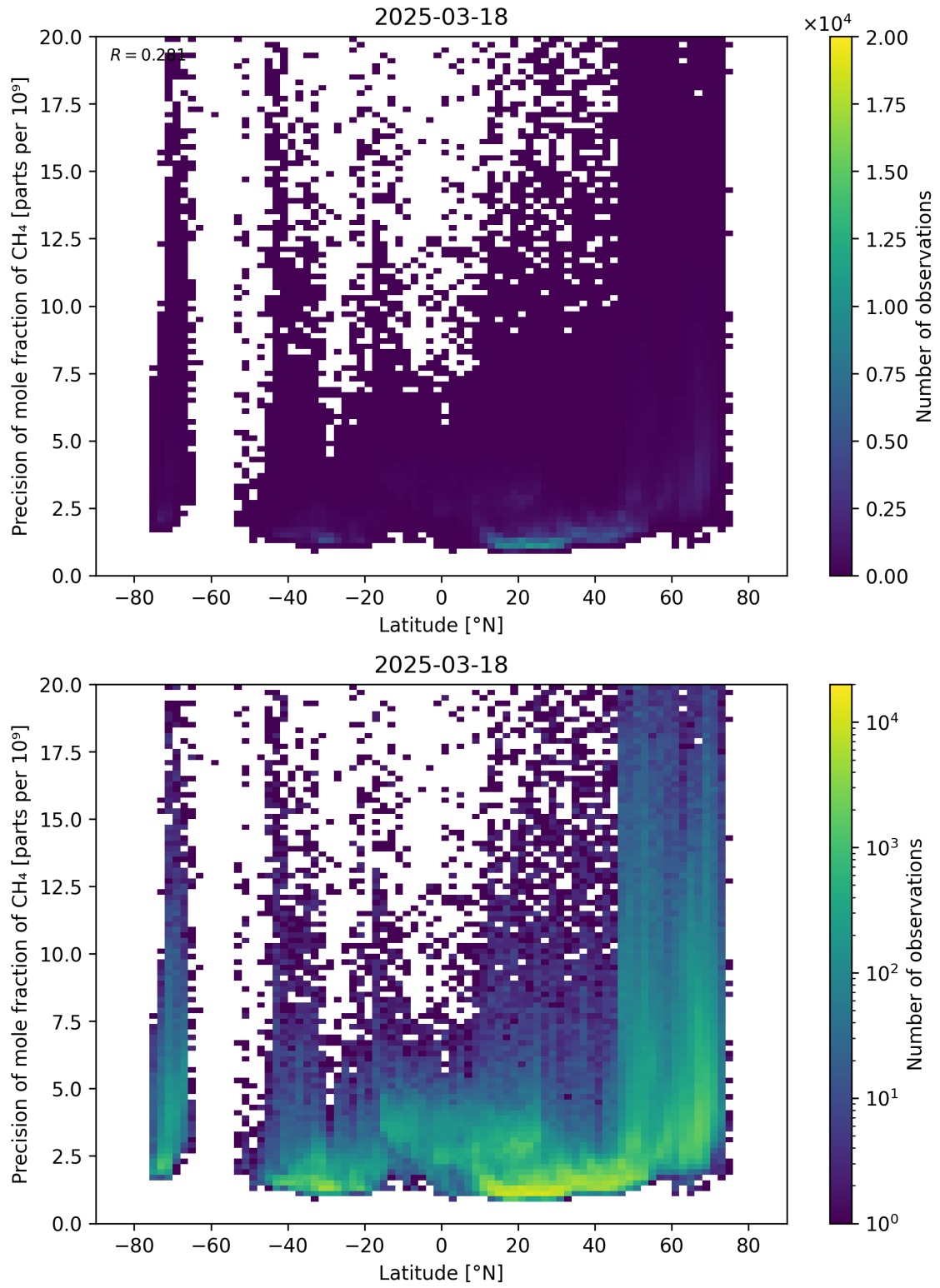
Figure 59: Scatter density plot of “Latitude” against “Precision of mole fraction of \text{CH}_4 ” for 2025-03-17 to 2025-03-19.
