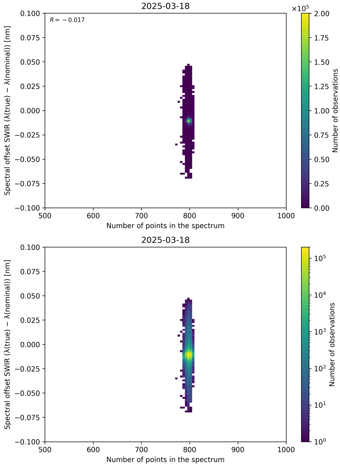
Figure 93: Scatter density plot of “Number of points in the spectrum” against “Spectral offset SWIR ( \lambda_{\text{true}} - \lambda_{\text{nominal}} )” for 2025-03-17 to 2025-03-19.
