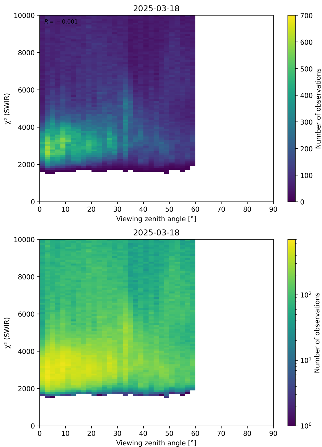
Figure 106: Scatter density plot of “Viewing zenith angle” against “ \chi^2 (SWIR)” for 2025-03-17 to 2025-03-19.
