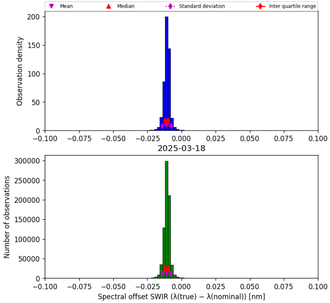
Figure 27: Histogram of “Spectral offset SWIR ( \lambda_{\text{true}} - \lambda_{\text{nominal}} )” for 2025-03-17 to 2025-03-19
