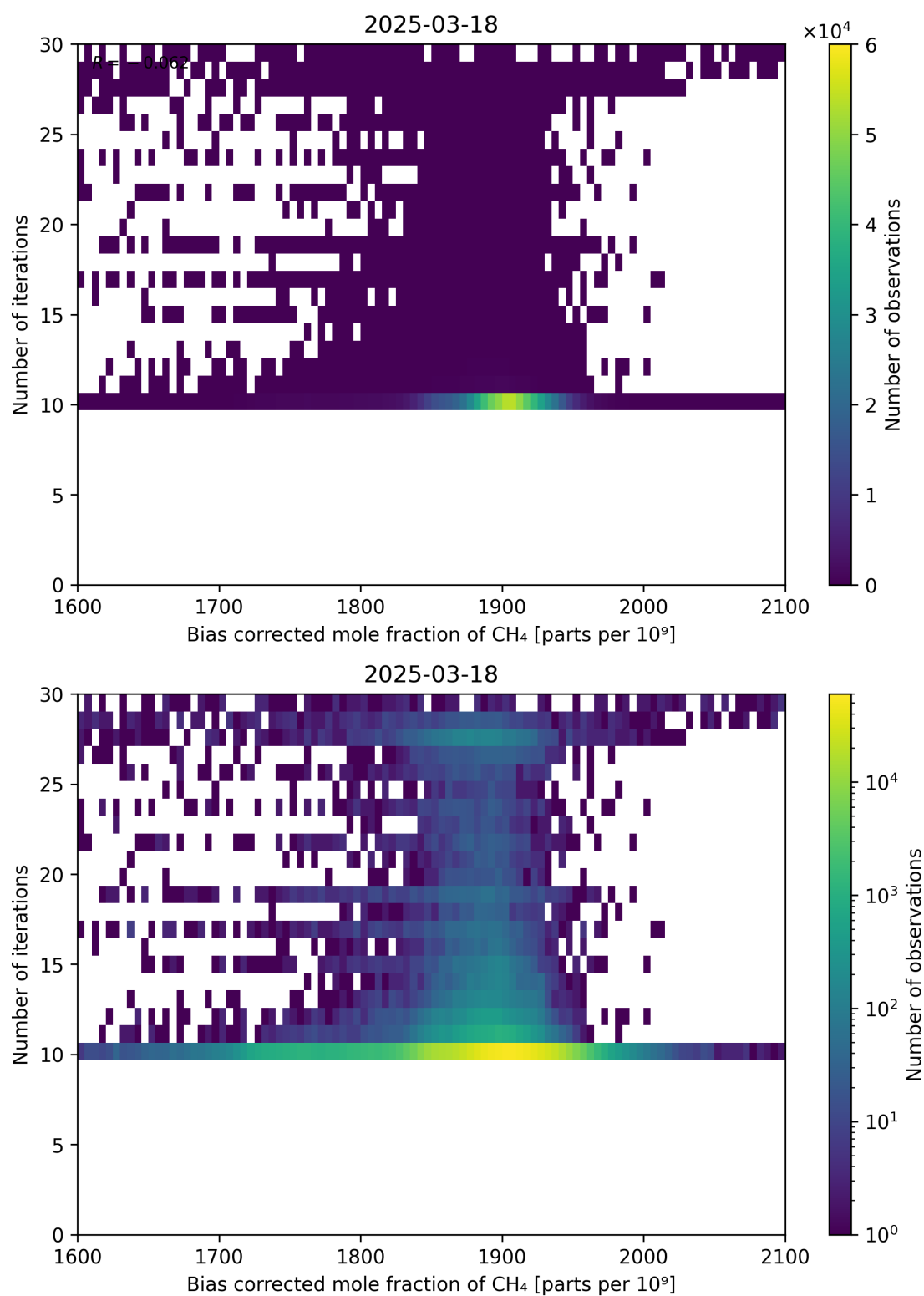
Figure 67: Scatter density plot of “Bias corrected mole fraction of \text{CH}_4 ” against “Number of iterations” for 2025-03-17 to 2025-03-19.
