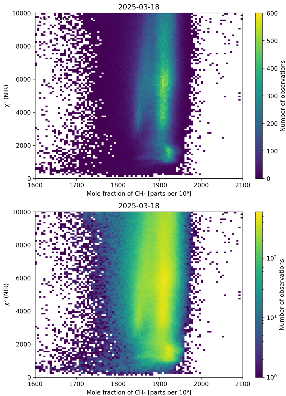
Figure 70: Scatter density plot of “Mole fraction of \text{CH}_4 ” against “ \chi^2 (NIR)” for 2025-03-17 to 2025-03-19.
