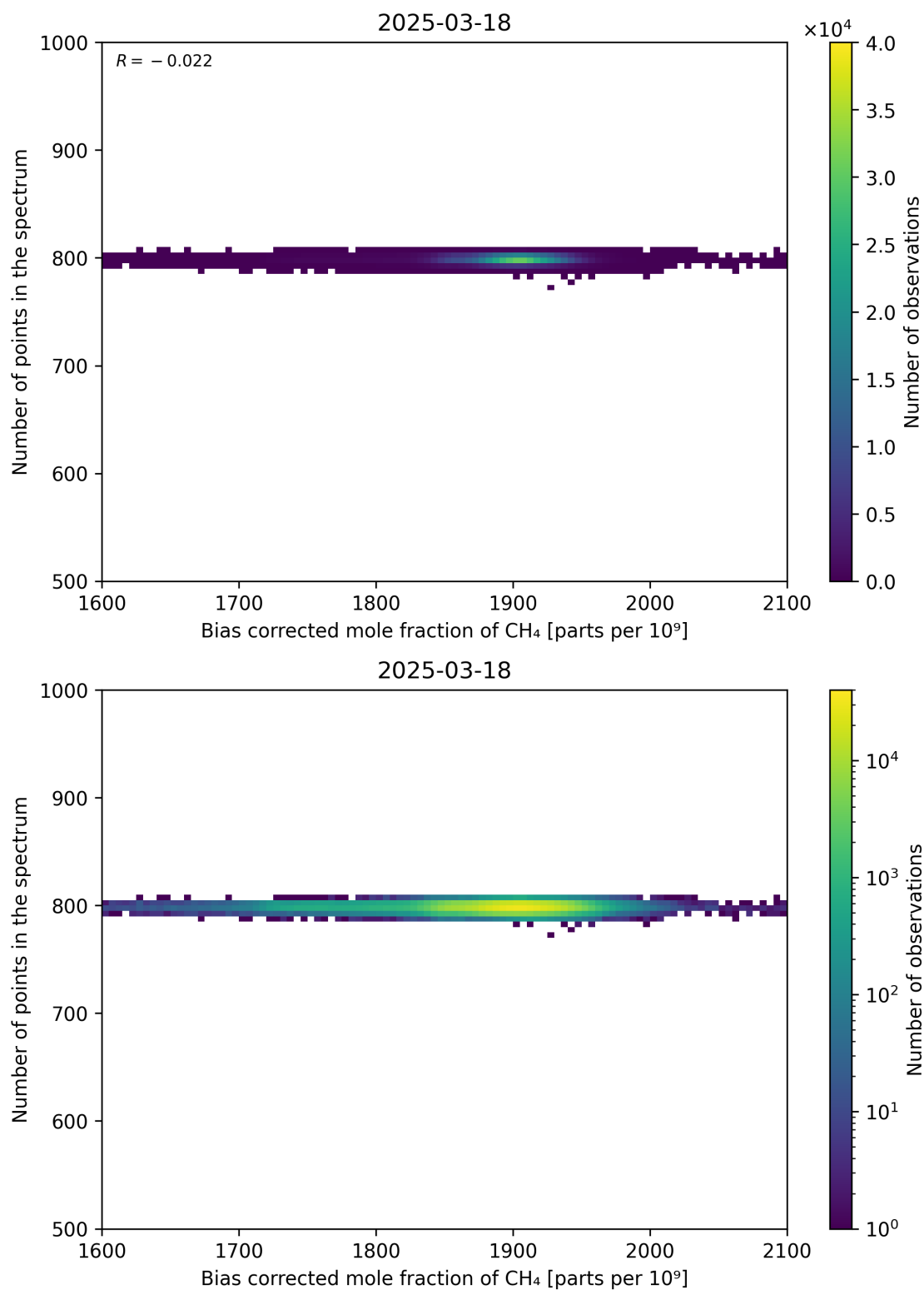
Figure 68: Scatter density plot of “Bias corrected mole fraction of CH 4 ” against “Number of points in the spectrum” for 2025-03-17 to 2025-03-19.
