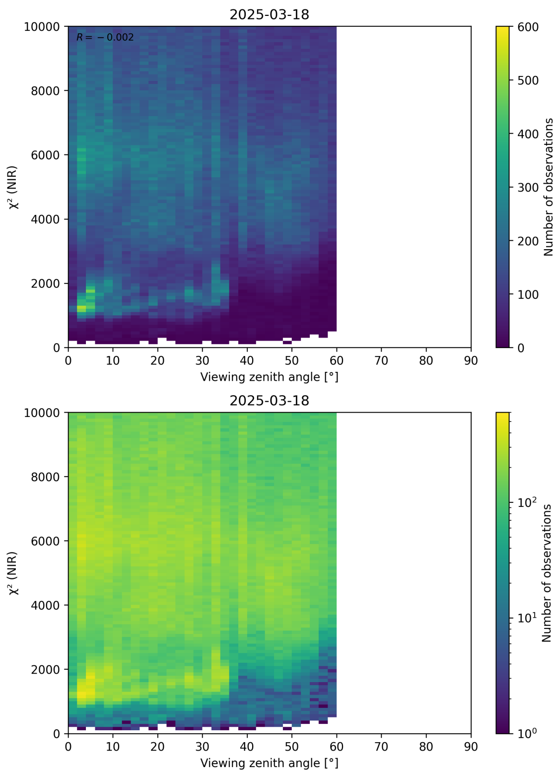
Figure 105: Scatter density plot of “Viewing zenith angle” against “ \chi^2 (NIR)” for 2025-03-17 to 2025-03-19.
