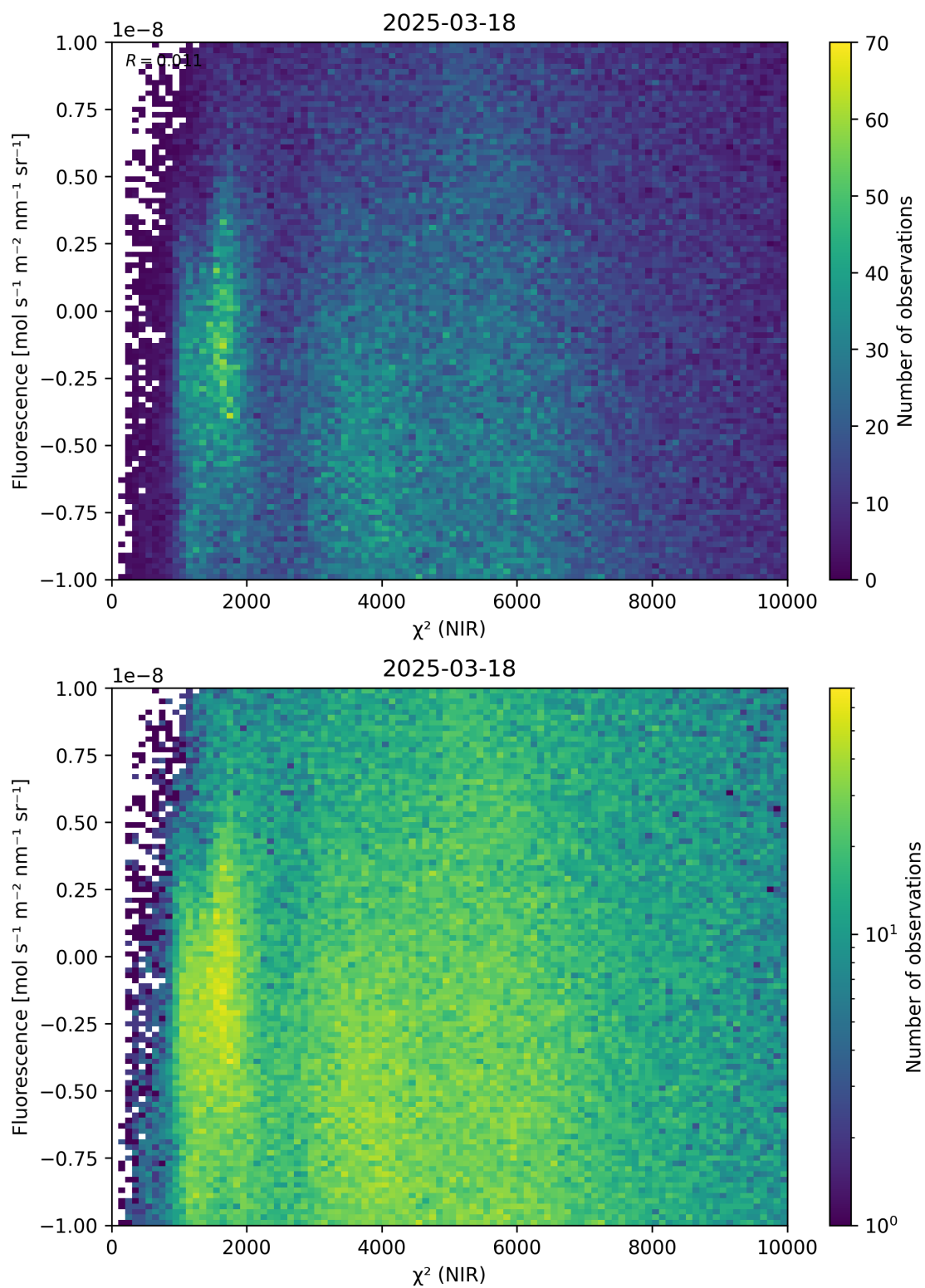
Figure 45: Scatter density plot of “ \chi^2 (NIR)” against “Fluorescence” for 2025-03-17 to 2025-03-19.
