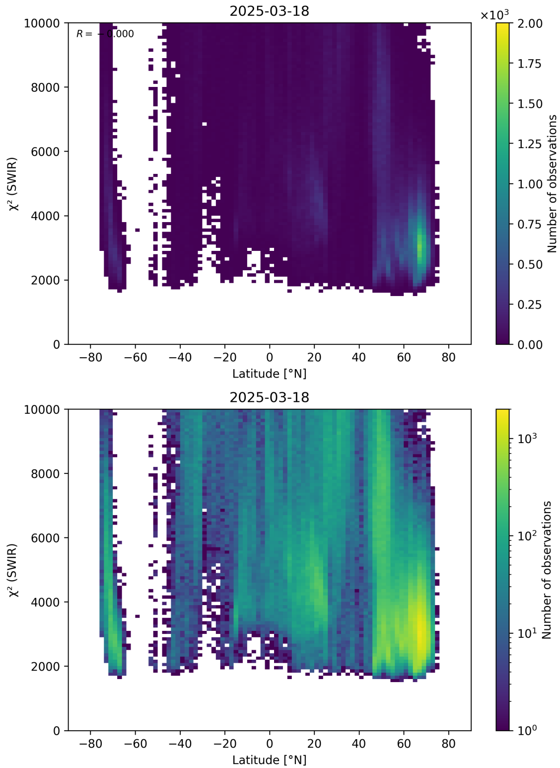
Figure 54: Scatter density plot of “Latitude” against “ \chi^2 (SWIR)” for 2025-03-17 to 2025-03-19.
