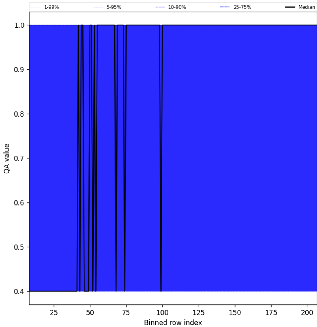
Figure 33: Along track statistics of “QA value” for 2025-03-17 to 2025-03-19
