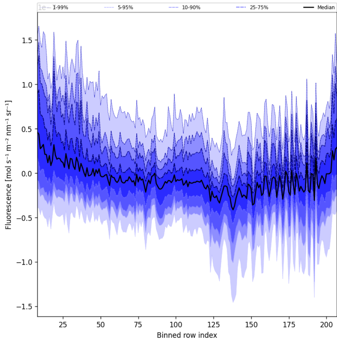
Figure 43: Along track statistics of “Fluorescence” for 2025-03-17 to 2025-03-19
