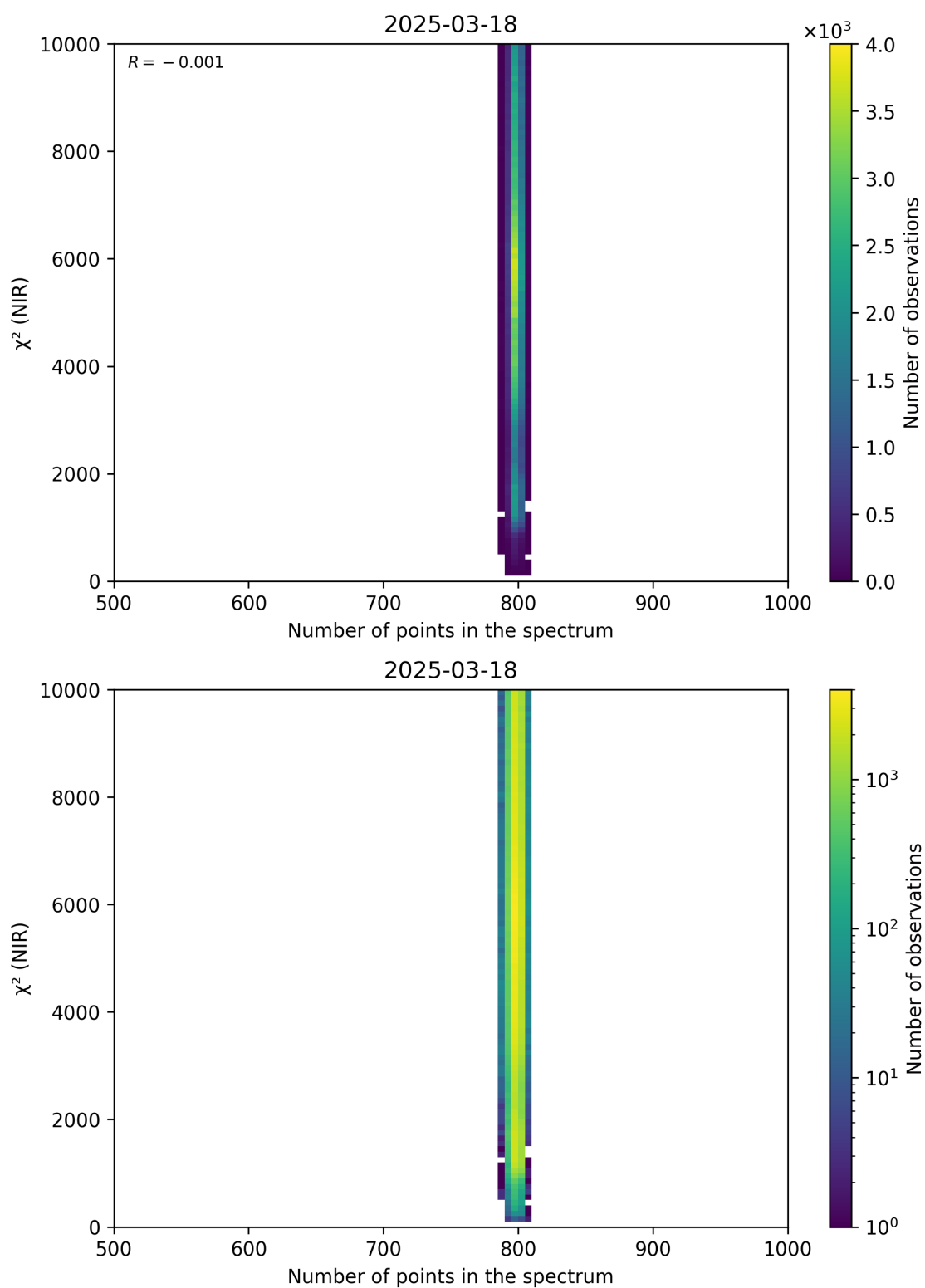
Figure 88: Scatter density plot of “Number of points in the spectrum” against “ \chi^2 (NIR)” for 2025-03-17 to 2025-03-19.
