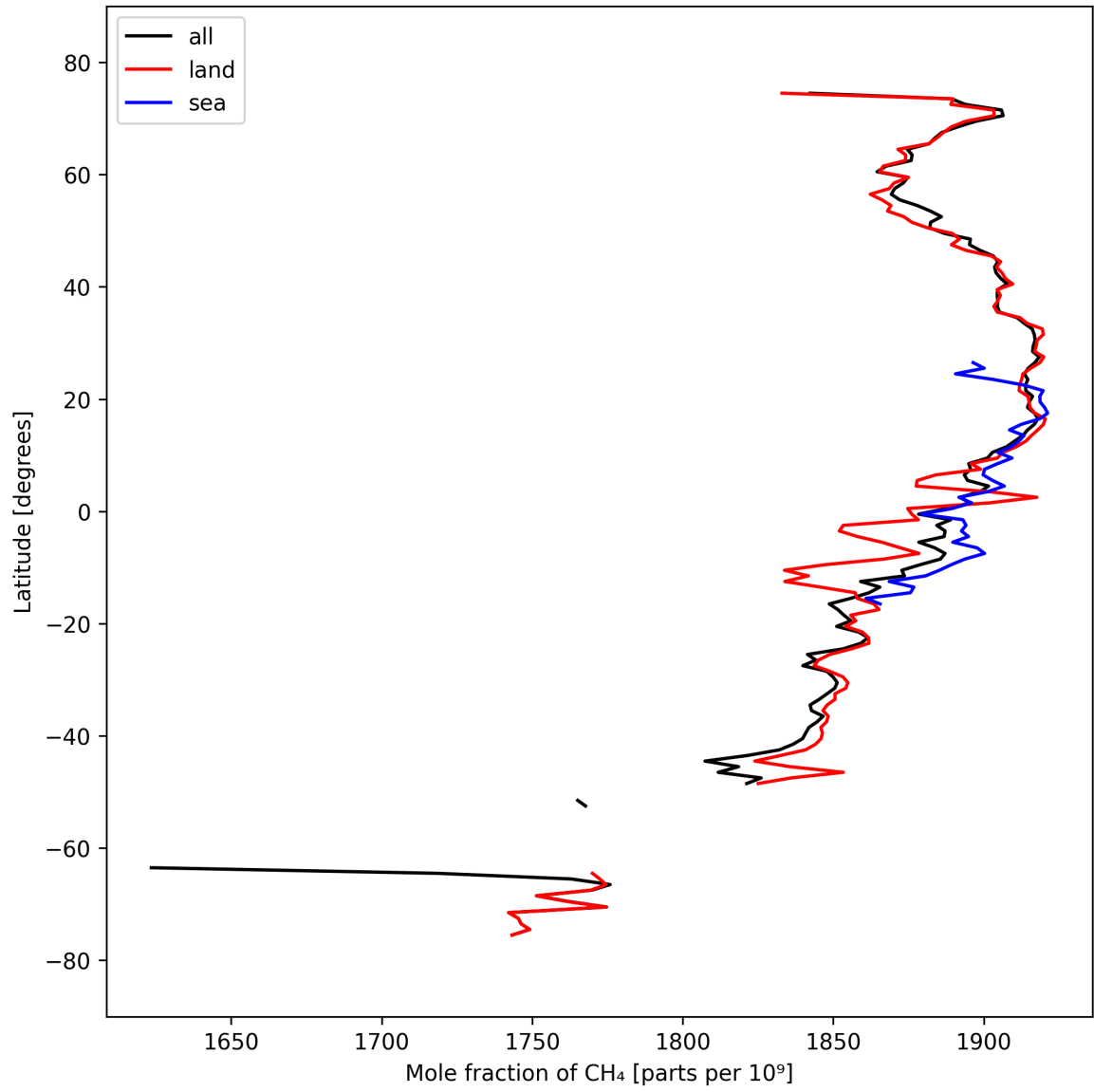
Figure 12: Zonal average of “Mole fraction of \text{CH}_4 ” for 2025-03-17 to 2025-03-19.
