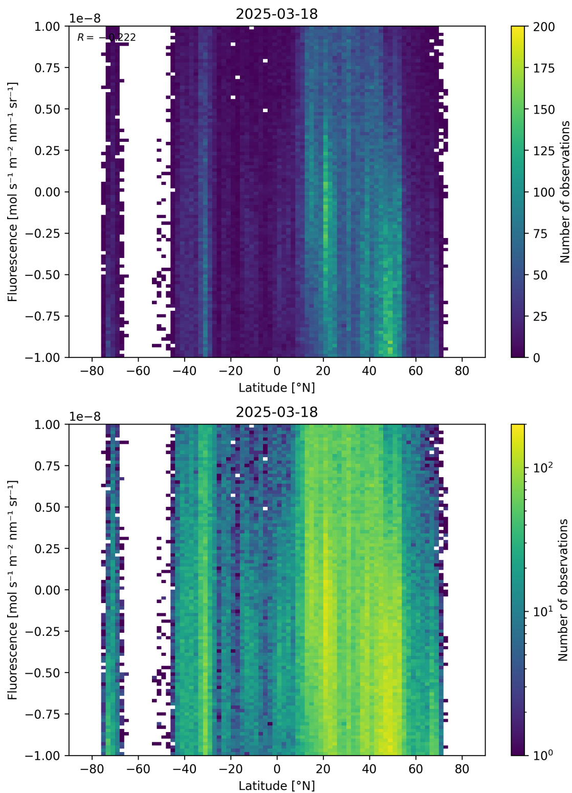
Figure 56: Scatter density plot of “Latitude” against “Fluorescence” for 2025-03-17 to 2025-03-19.
