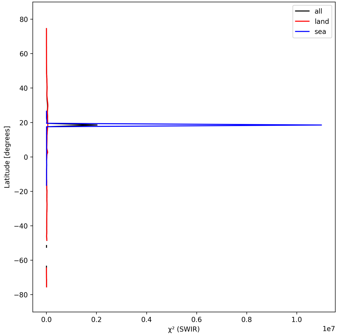
Figure 17: Zonal average of “ \chi^2 (SWIR)” for 2025-03-17 to 2025-03-19.
