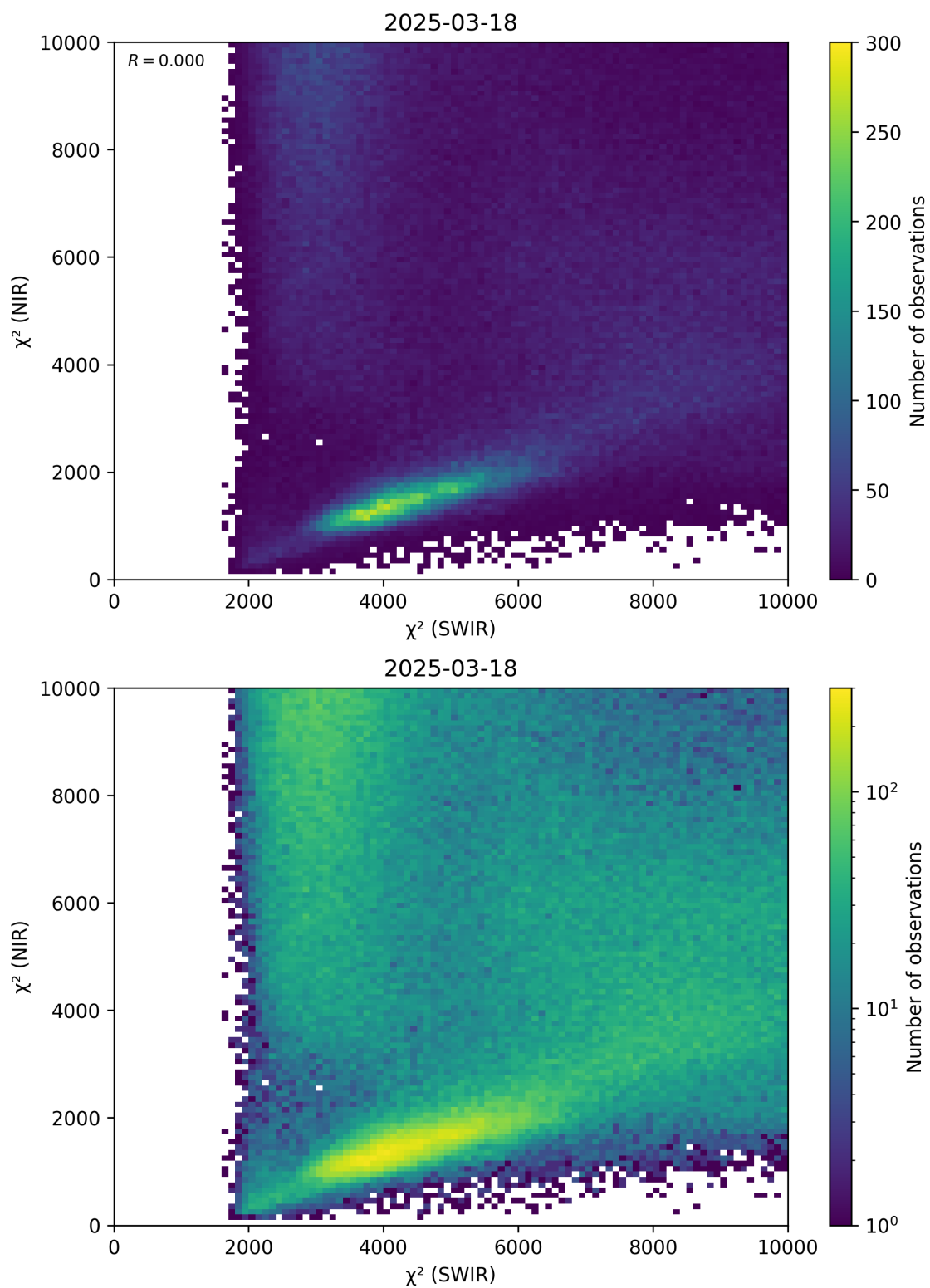
Figure 47: Scatter density plot of “ \chi^2 (SWIR)” against “ \chi^2 (NIR)” for 2025-03-17 to 2025-03-19.
