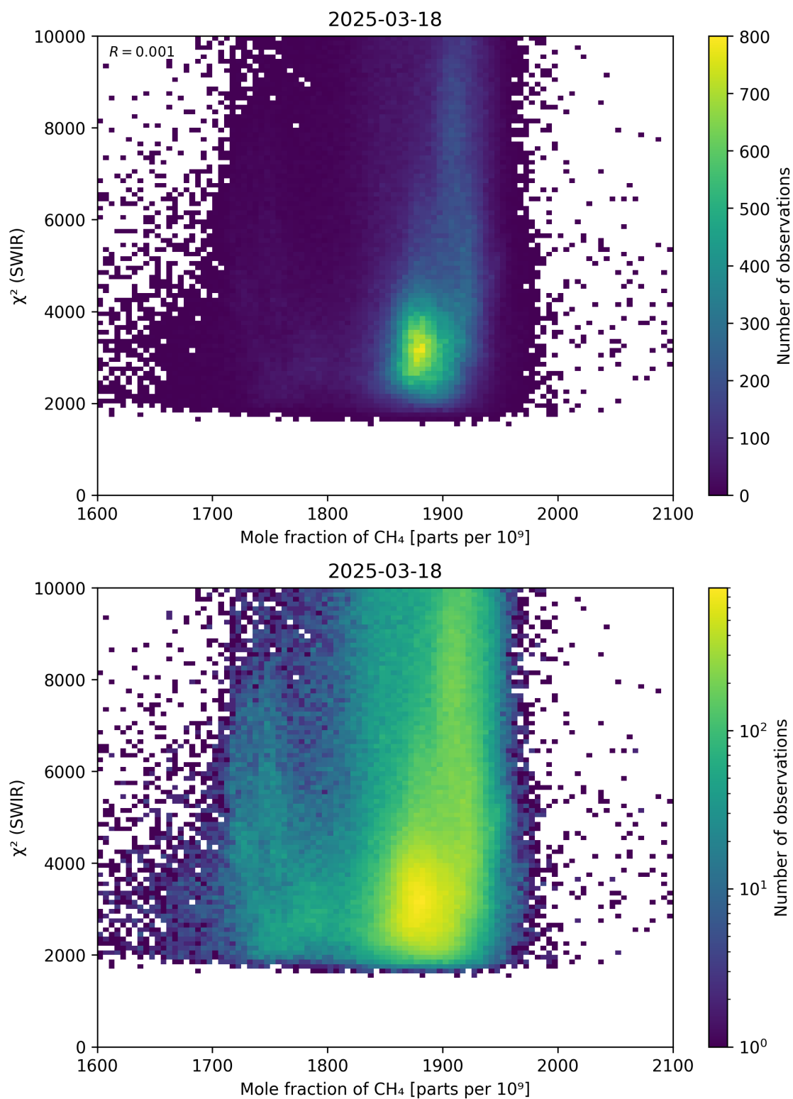
Figure 71: Scatter density plot of “Mole fraction of CH 4 ” against “ \chi^2 (SWIR)” for 2025-03-17 to 2025-03-19.
