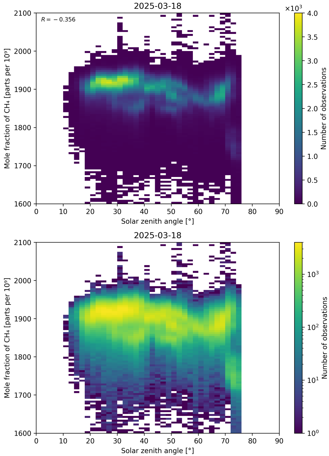
Figure 99: Scatter density plot of “Solar zenith angle” against “Mole fraction of CH 4 ” for 2025-03-17 to 2025-03-19.
