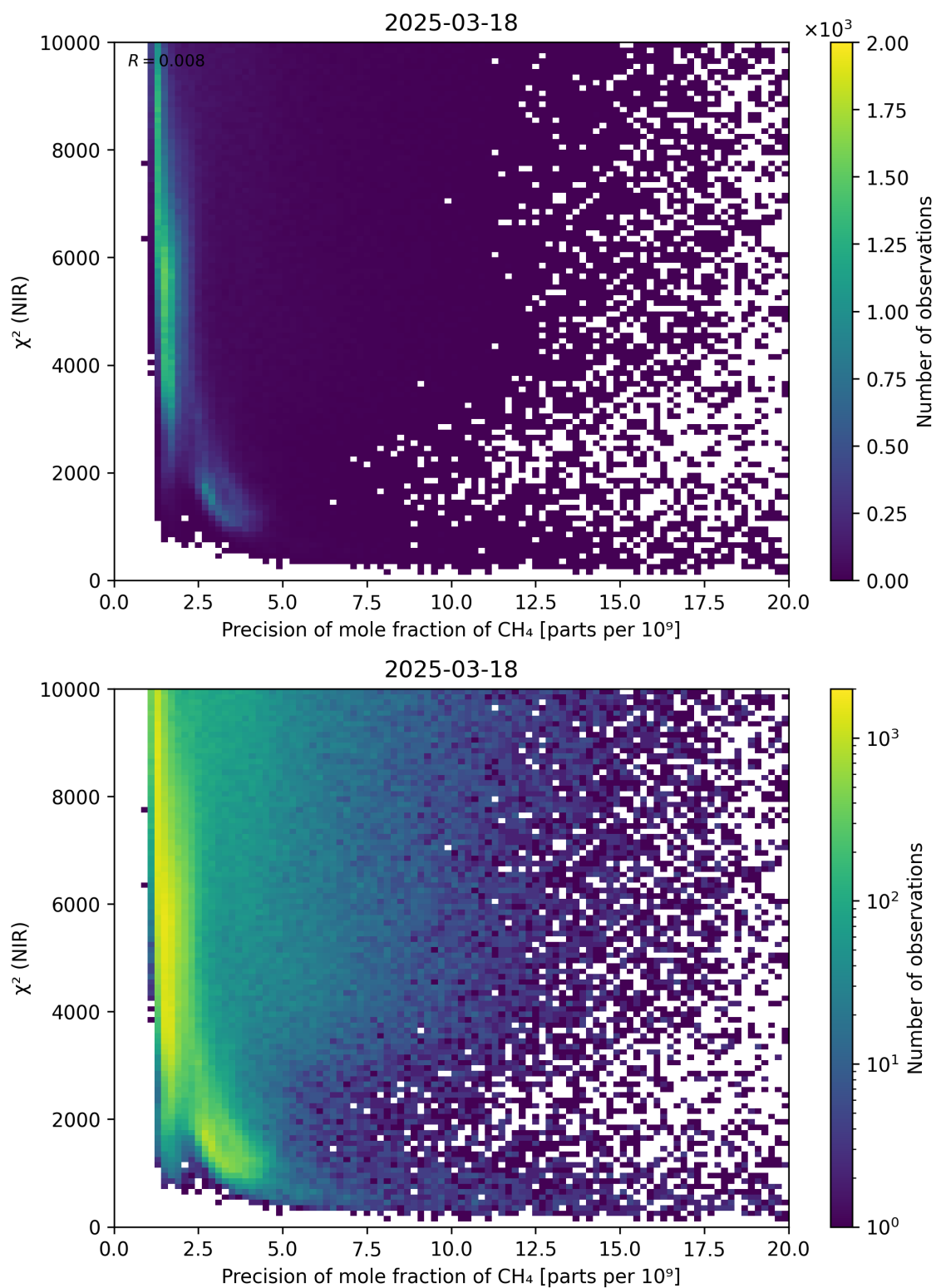
Figure 78: Scatter density plot of “Precision of mole fraction of \text{CH}_4 ” against “ \chi^2 (NIR)” for 2025-03-17 to 2025-03-19.
