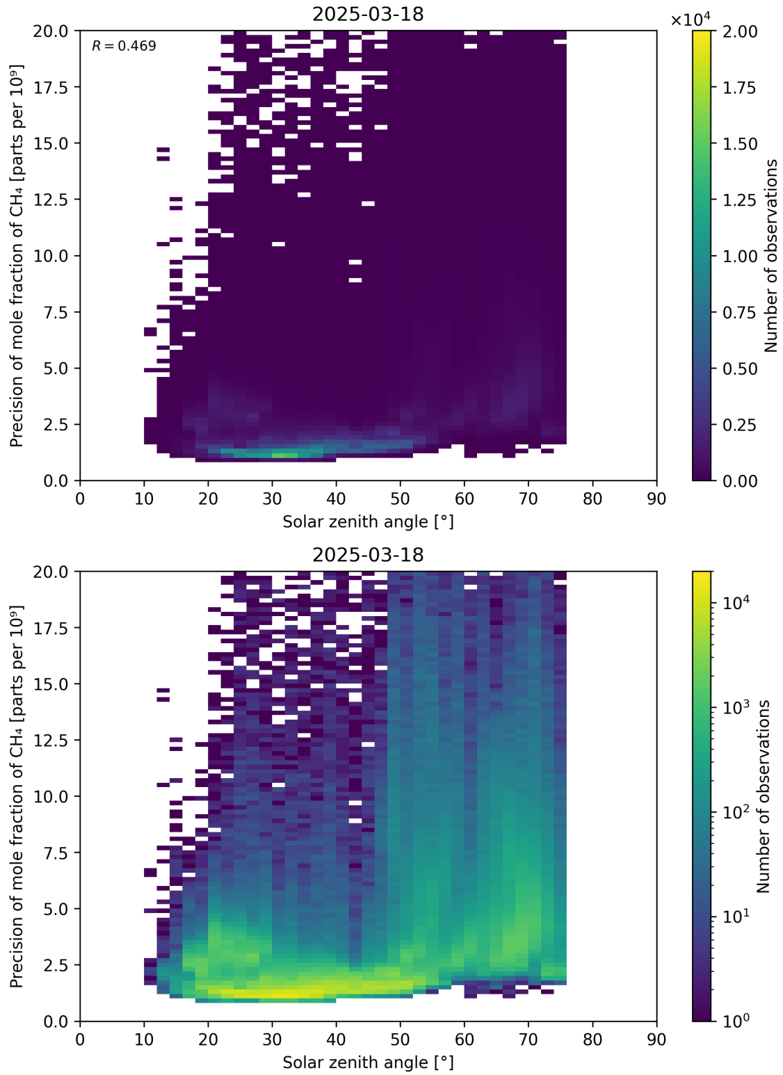
Figure 101: Scatter density plot of “Solar zenith angle” against “Precision of mole fraction of CH 4 ” for 2025-03-17 to 2025-03-19.
