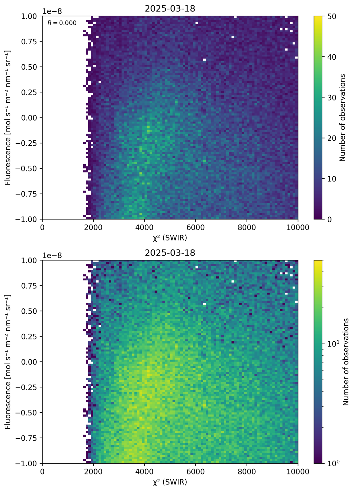
Figure 49: Scatter density plot of “ \chi^2 (SWIR)” against “Fluorescence” for 2025-03-17 to 2025-03-19.
