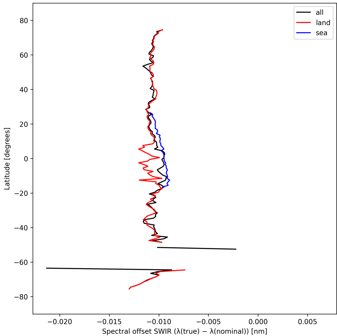
Figure 16: Zonal average of “Spectral offset SWIR ( \lambda_{\text{true}} - \lambda_{\text{nominal}} )” for 2025-03-17 to 2025-03-19.
