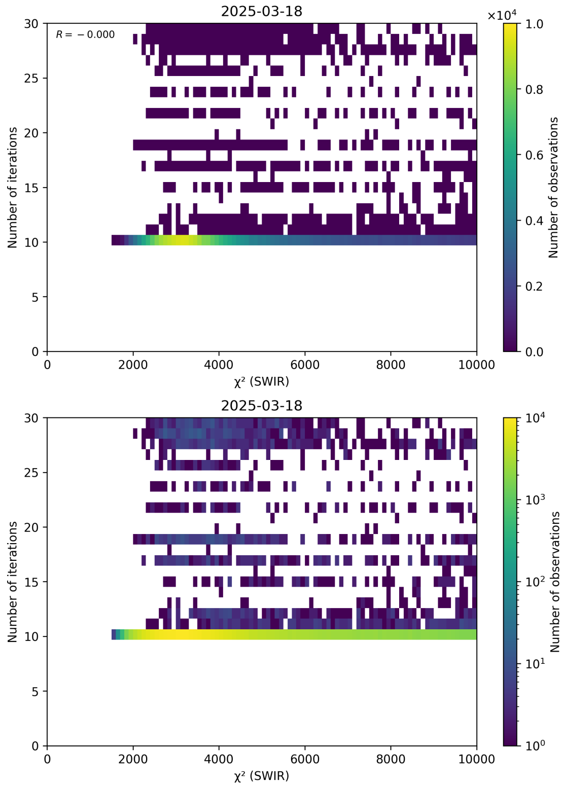
Figure 50: Scatter density plot of “ \chi^2 (SWIR)” against “Number of iterations” for 2025-03-17 to 2025-03-19.
