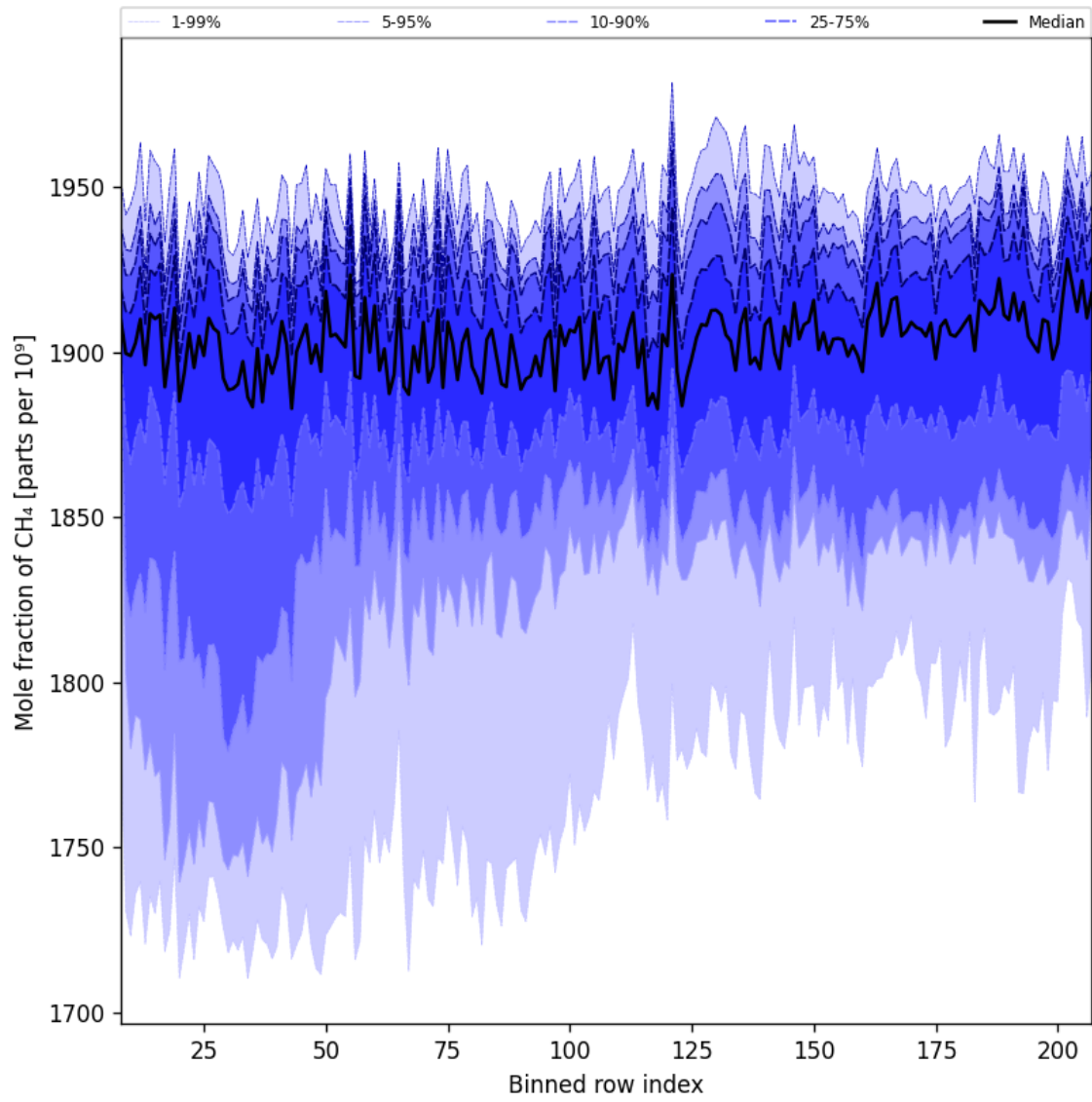
Figure 34: Along track statistics of “Mole fraction of CH 4 ” for 2025-03-17 to 2025-03-19
