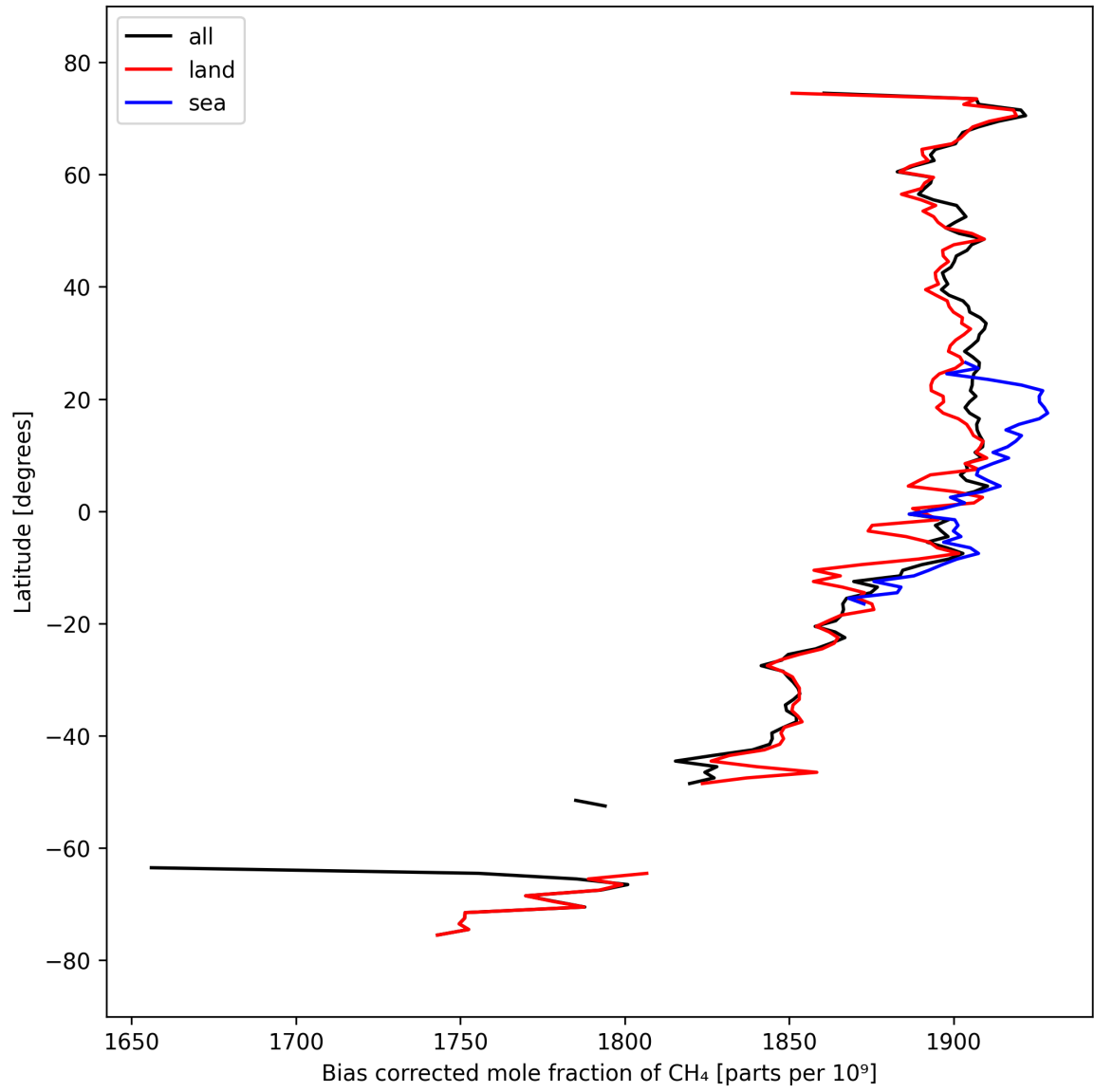
Figure 14: Zonal average of “Bias corrected mole fraction of \text{CH}_4 ” for 2025-03-17 to 2025-03-19.
