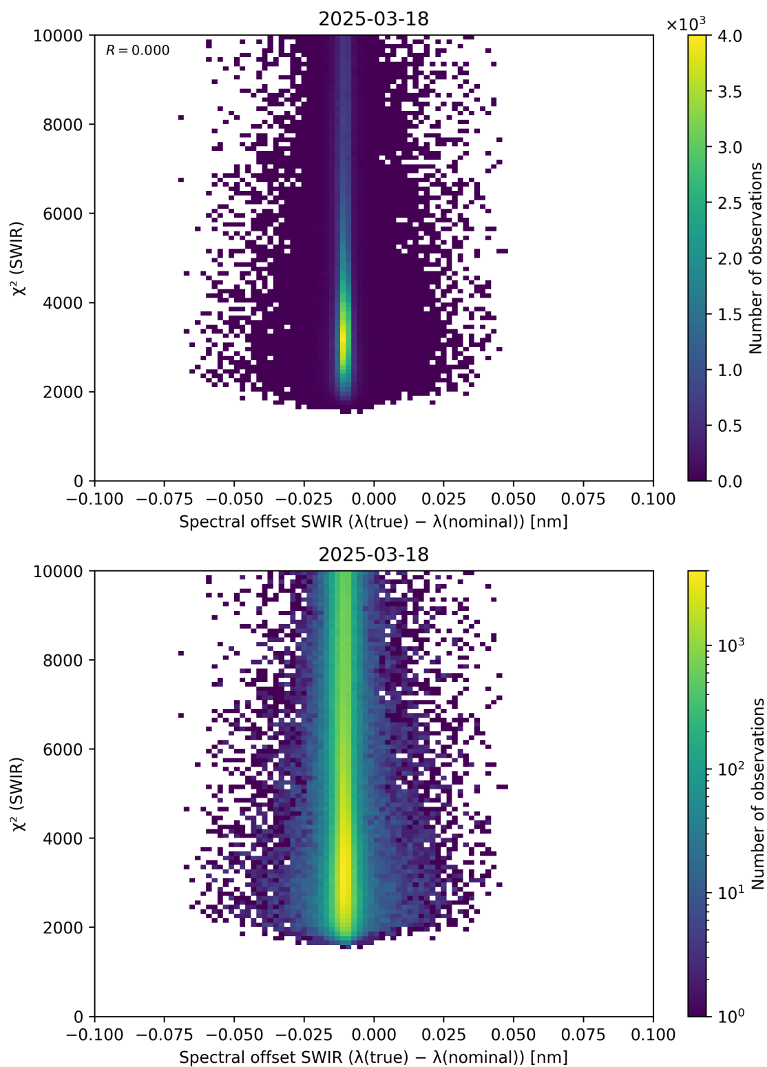
Figure 118: Scatter density plot of “Spectral offset SWIR ( \lambda_{\text{true}} - \lambda_{\text{nominal}} )” against “ \chi^2 (SWIR)” for 2025-03-17 to 2025-03-19.
