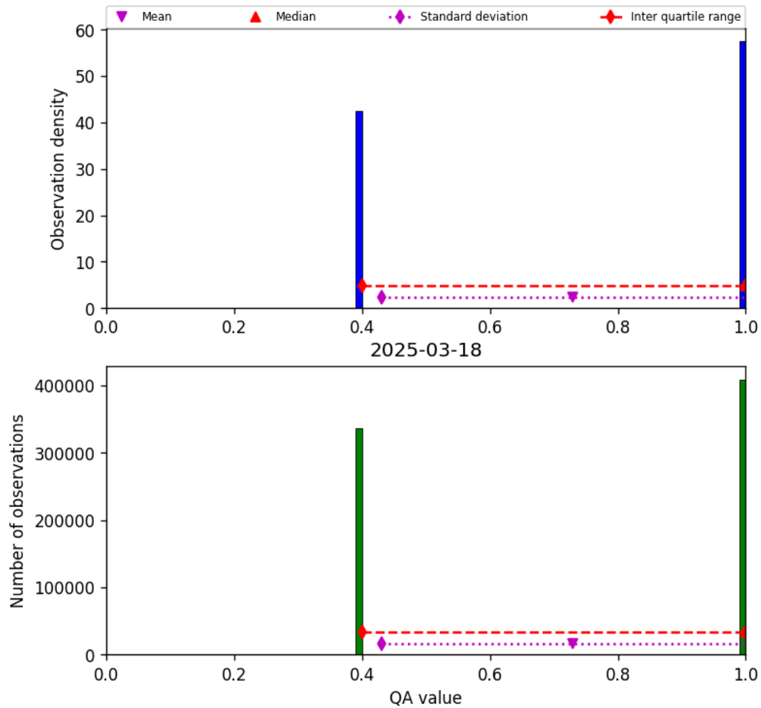
Figure 22: Histogram of “QA value” for 2025-03-17 to 2025-03-19
