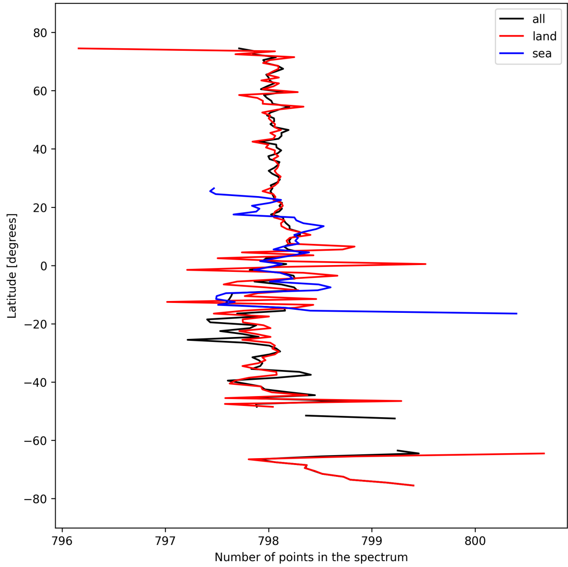
Figure 15: Zonal average of “Number of points in the spectrum” for 2025-03-17 to 2025-03-19.
