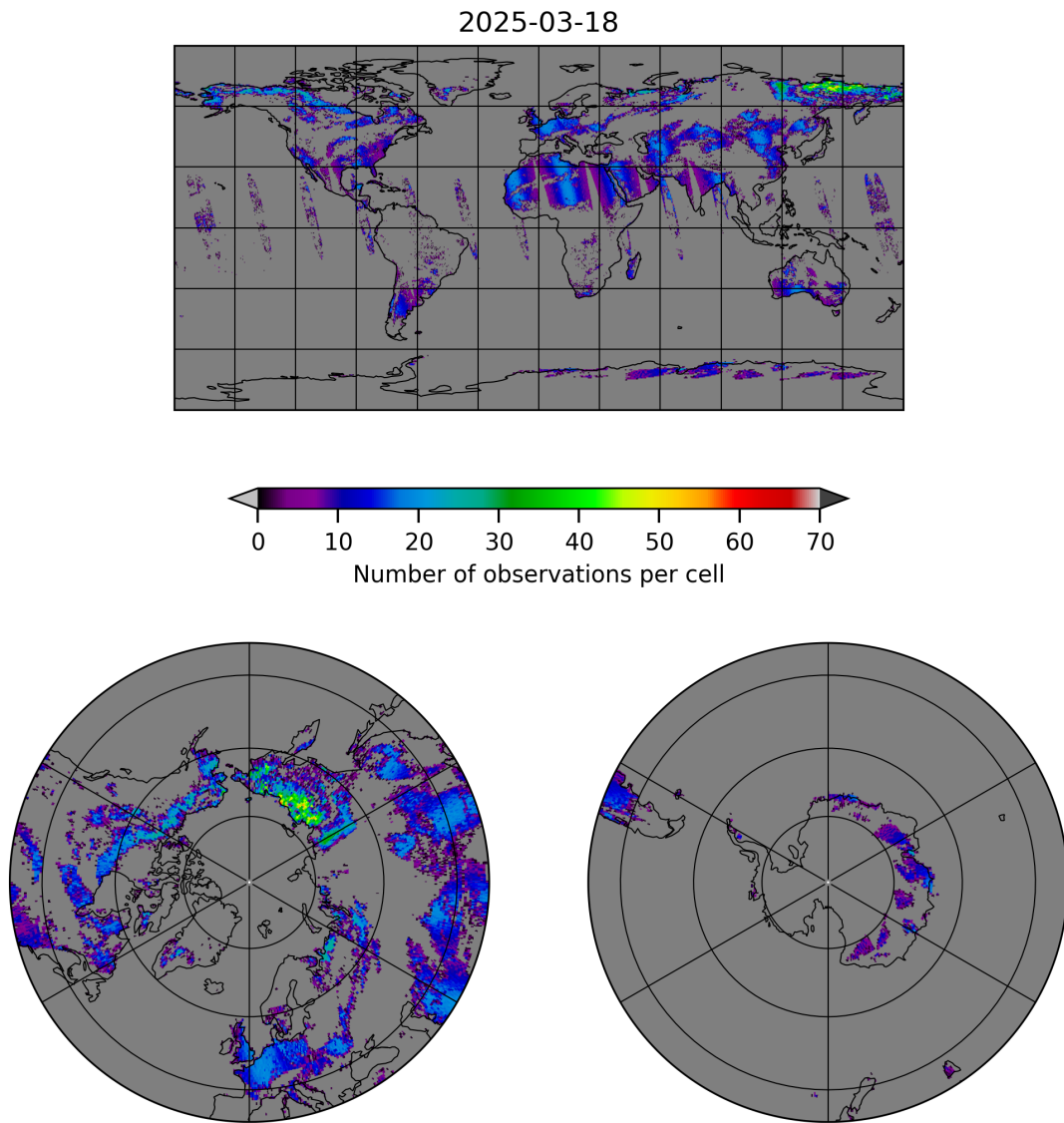
Figure 10: Map of the number of observations for 2025-03-17 to 2025-03-19
