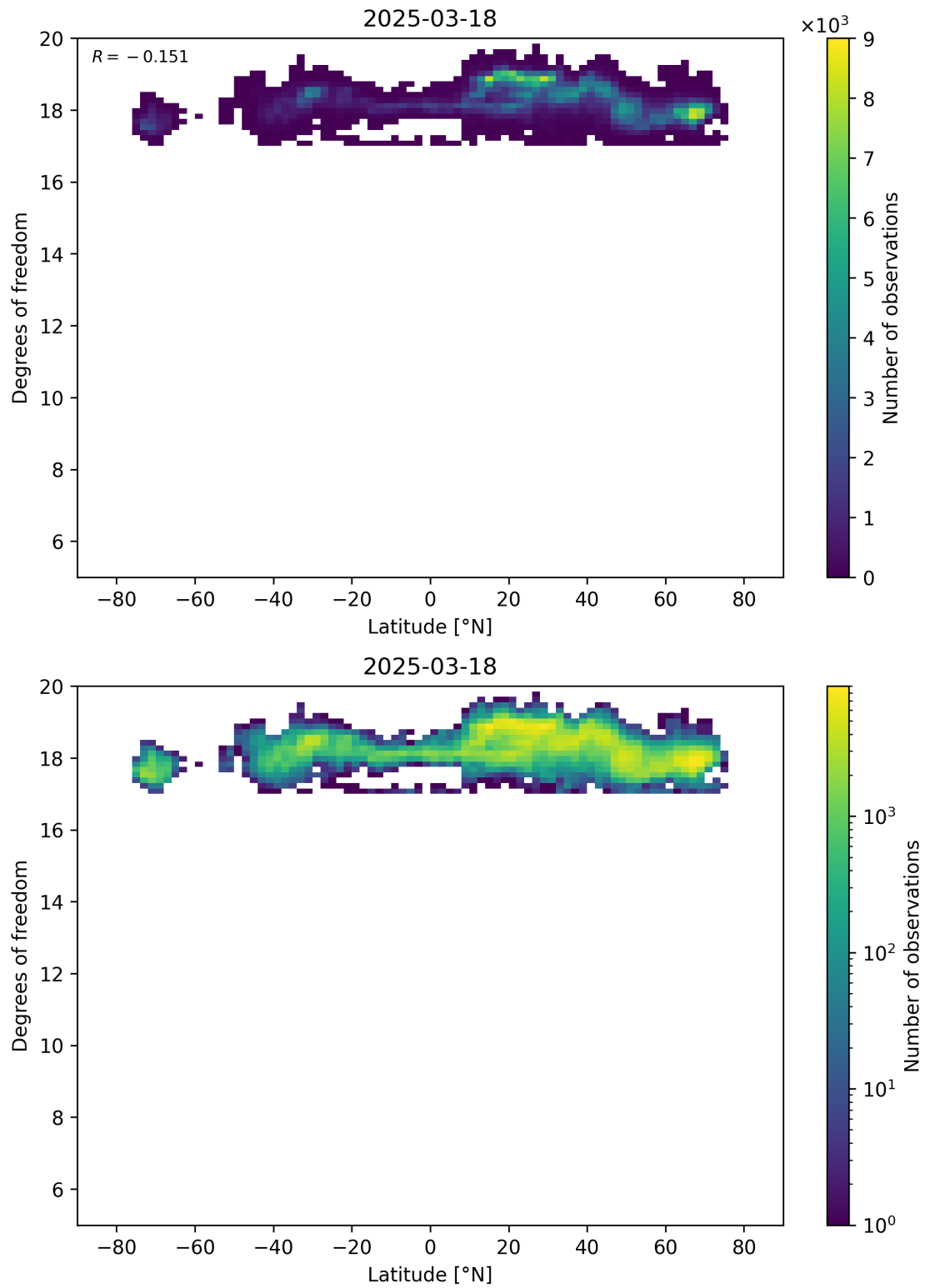
Figure 55: Scatter density plot of “Latitude” against “Degrees of freedom” for 2025-03-17 to 2025-03-19.
