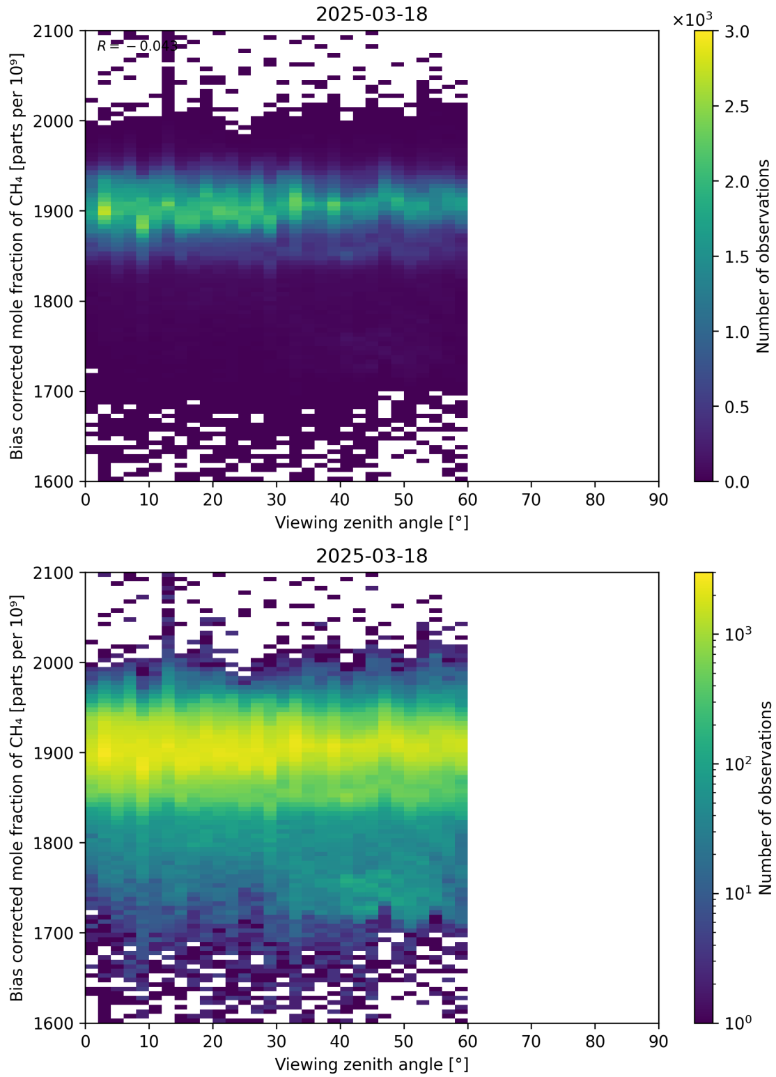
Figure 111: Scatter density plot of “Viewing zenith angle” against “Bias corrected mole fraction of CH 4 ” for 2025-03-17 to 2025-03-19.
