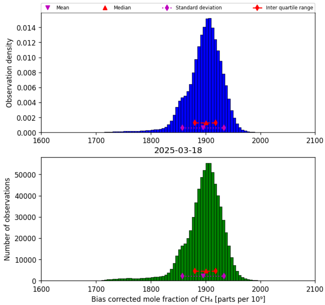
Figure 25: Histogram of “Bias corrected mole fraction of CH 4 ” for 2025-03-17 to 2025-03-19
