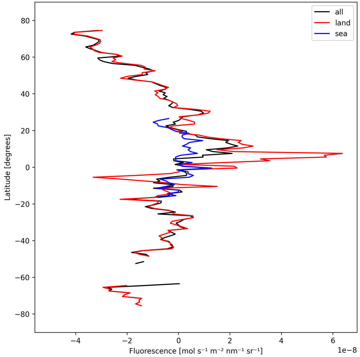
Figure 21: Zonal average of “Fluorescence” for 2025-03-17 to 2025-03-19.
