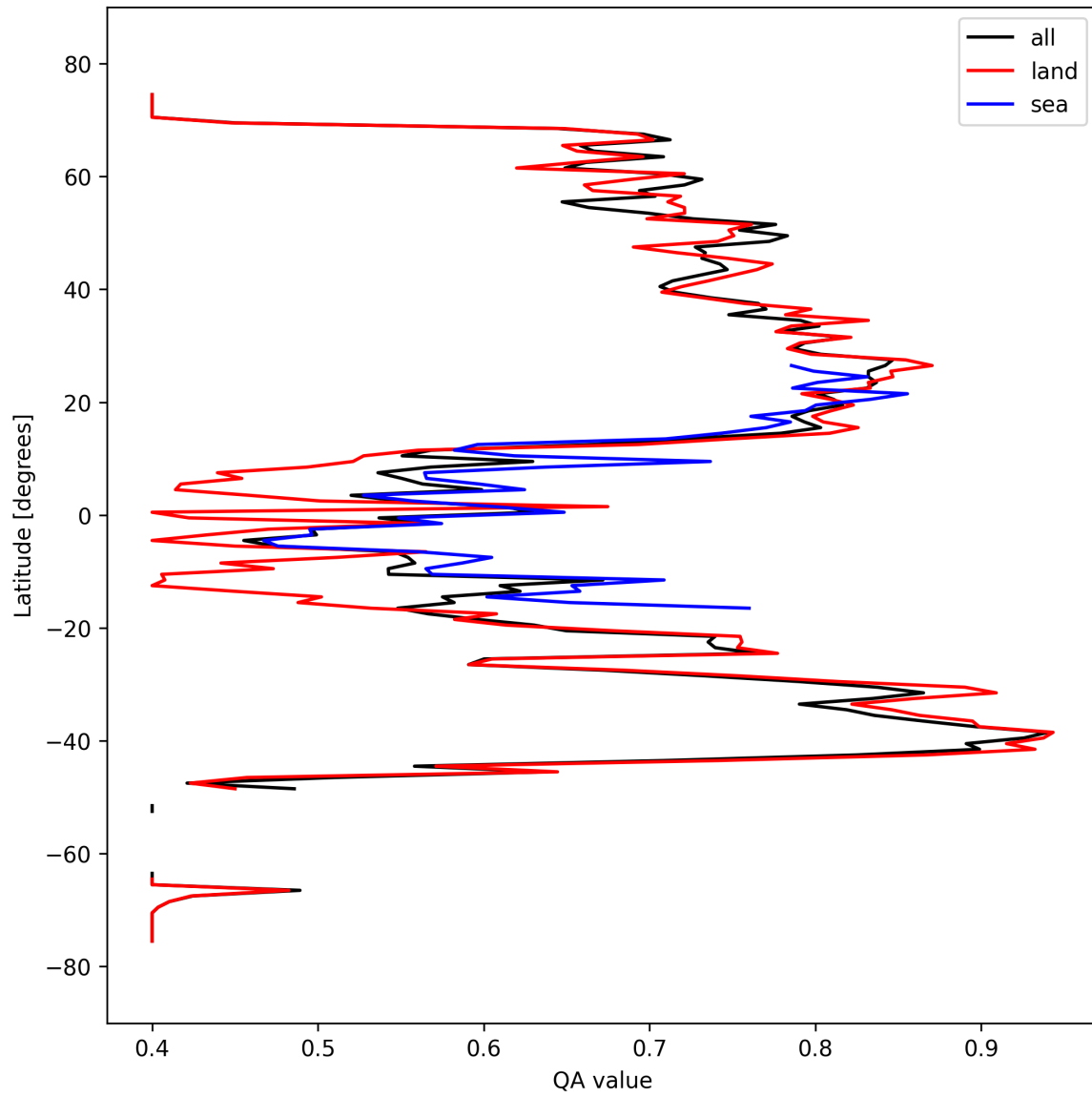
Figure 11: Zonal average of “QA value” for 2025-03-17 to 2025-03-19.
