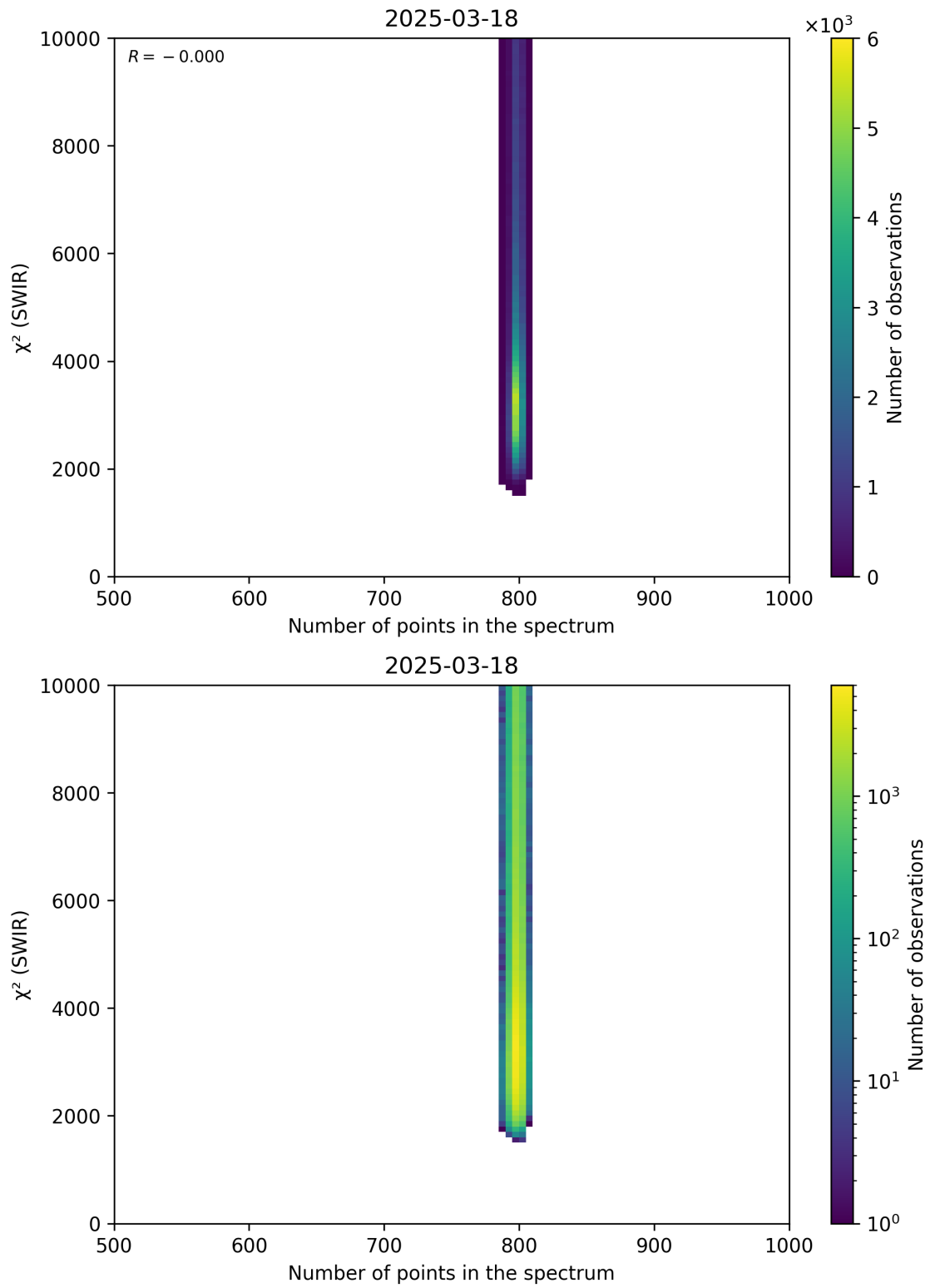
Figure 89: Scatter density plot of “Number of points in the spectrum” against “ \chi^2 (SWIR)” for 2025-03-17 to 2025-03-19.
