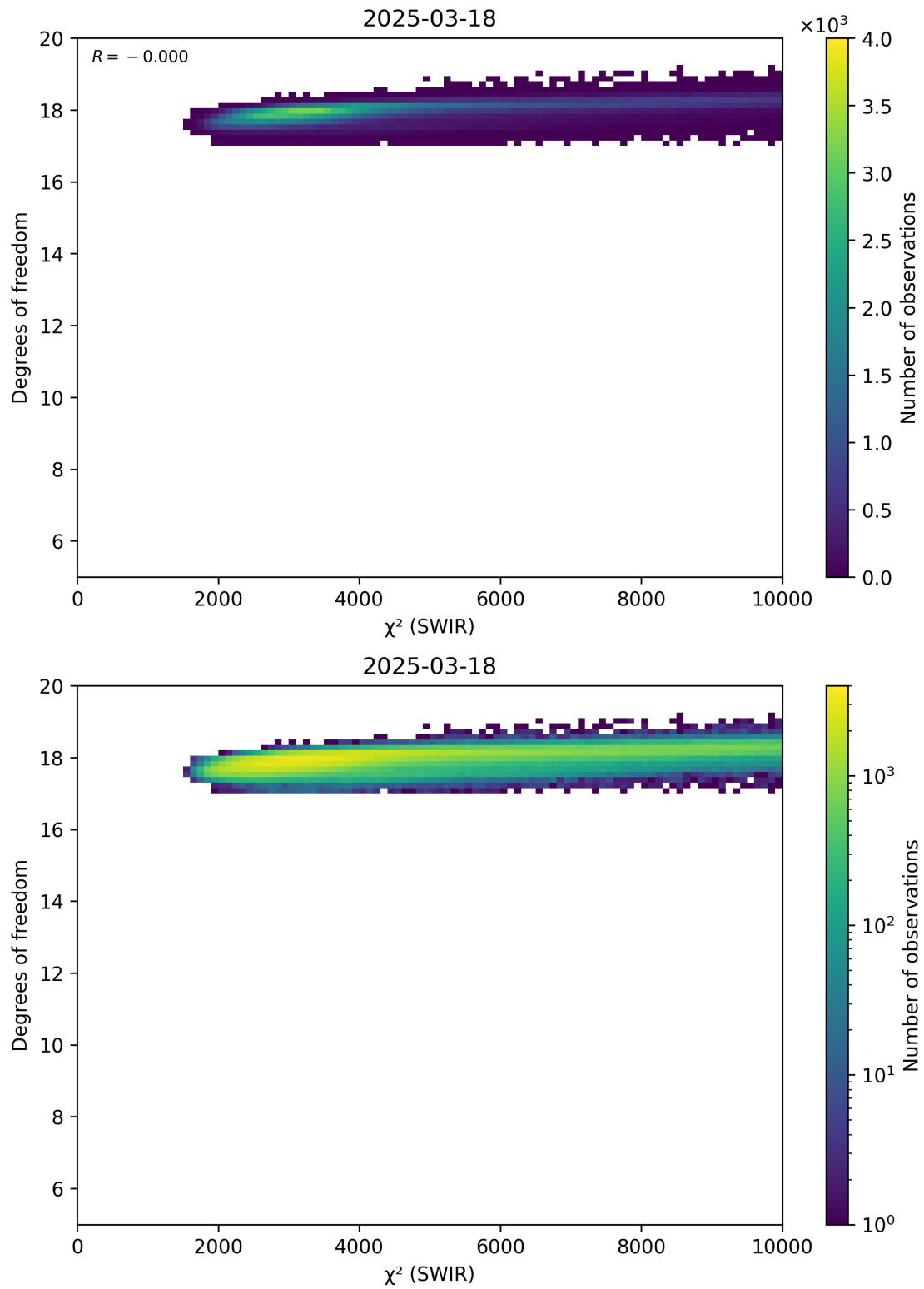
Figure 48: Scatter density plot of “ \chi^2 (SWIR)” against “Degrees of freedom” for 2025-03-17 to 2025-03-19.
