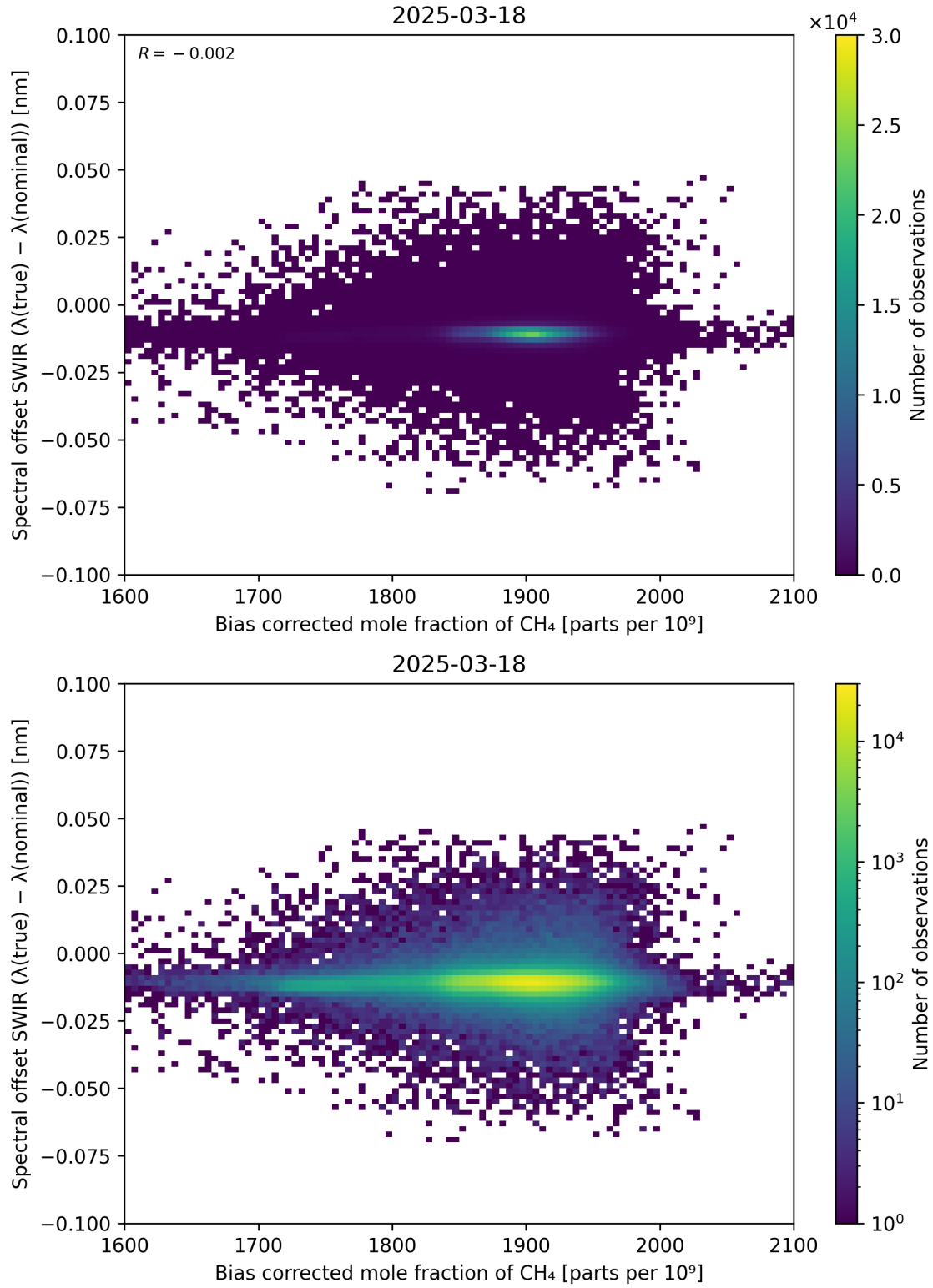
Figure 69: Scatter density plot of “Bias corrected mole fraction of \text{CH}_4 ” against “Spectral offset SWIR ( \lambda_{\text{true}} - \lambda_{\text{nominal}} )” for 2025-03-17 to 2025-03-19.
