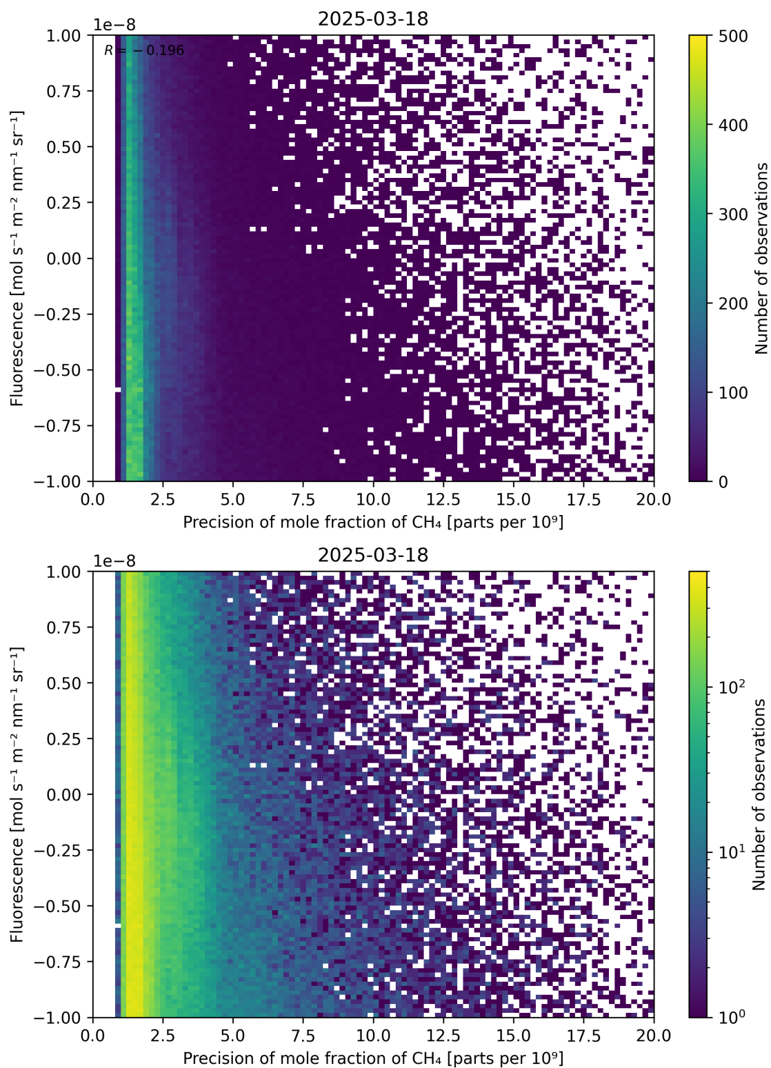
Figure 81: Scatter density plot of “Precision of mole fraction of \text{CH}_4 ” against “Fluorescence” for 2025-03-17 to 2025-03-19.
