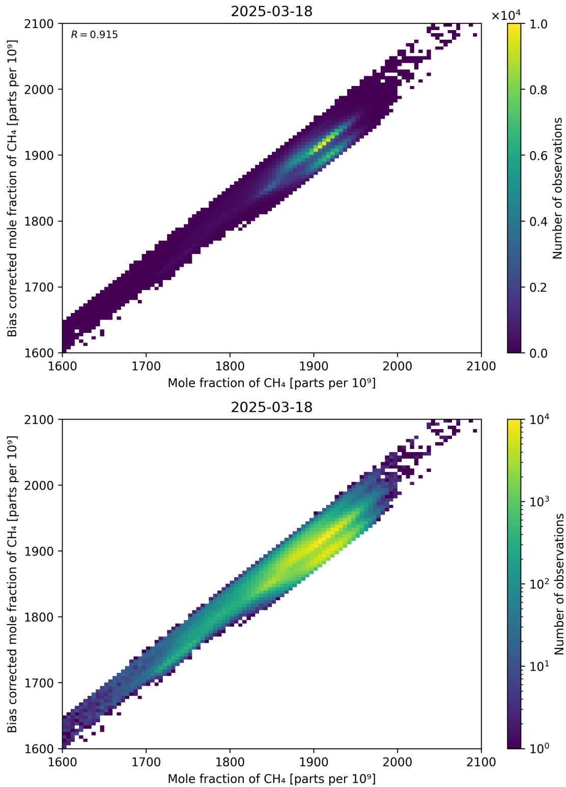
Figure 74: Scatter density plot of “Mole fraction of CH 4 ” against “Bias corrected mole fraction of CH 4 ” for 2025-03-17 to 2025-03-19.
