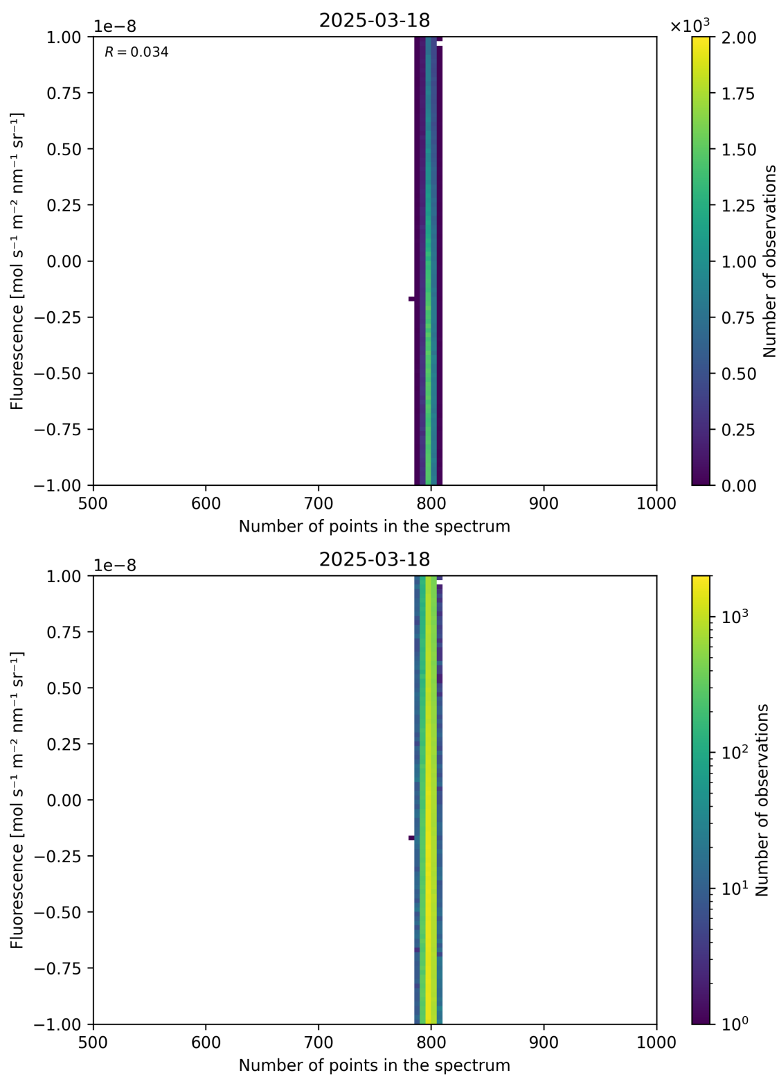
Figure 91: Scatter density plot of “Number of points in the spectrum” against “Fluorescence” for 2025-03-17 to 2025-03-19.
