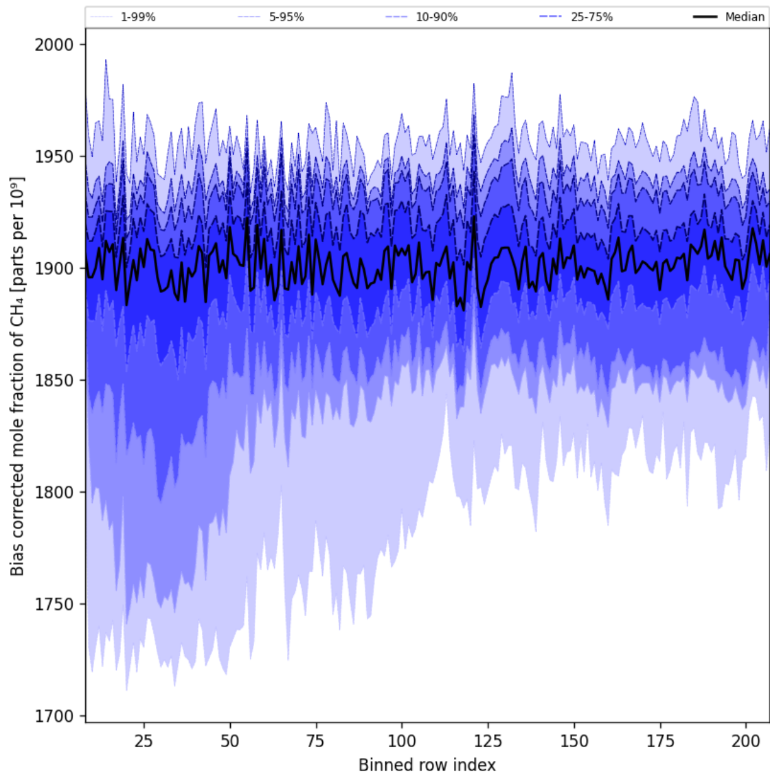
Figure 36: Along track statistics of “Bias corrected mole fraction of CH 4 ” for 2025-03-17 to 2025-03-19
