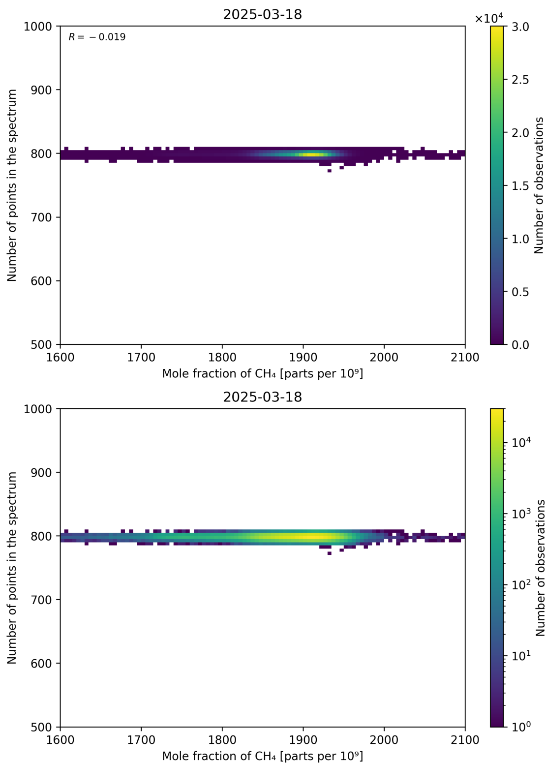
Figure 77: Scatter density plot of “Mole fraction of CH 4 ” against “Number of points in the spectrum” for 2025-03-17 to 2025-03-19.
