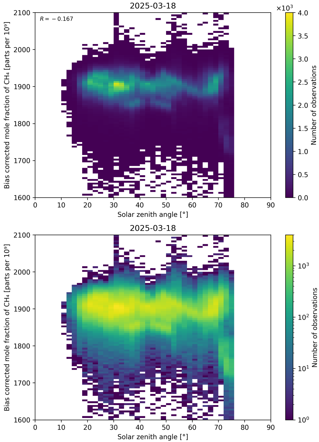
Figure 100: Scatter density plot of “Solar zenith angle” against “Bias corrected mole fraction of CH 4 ” for 2025-03-17 to 2025-03-19.
