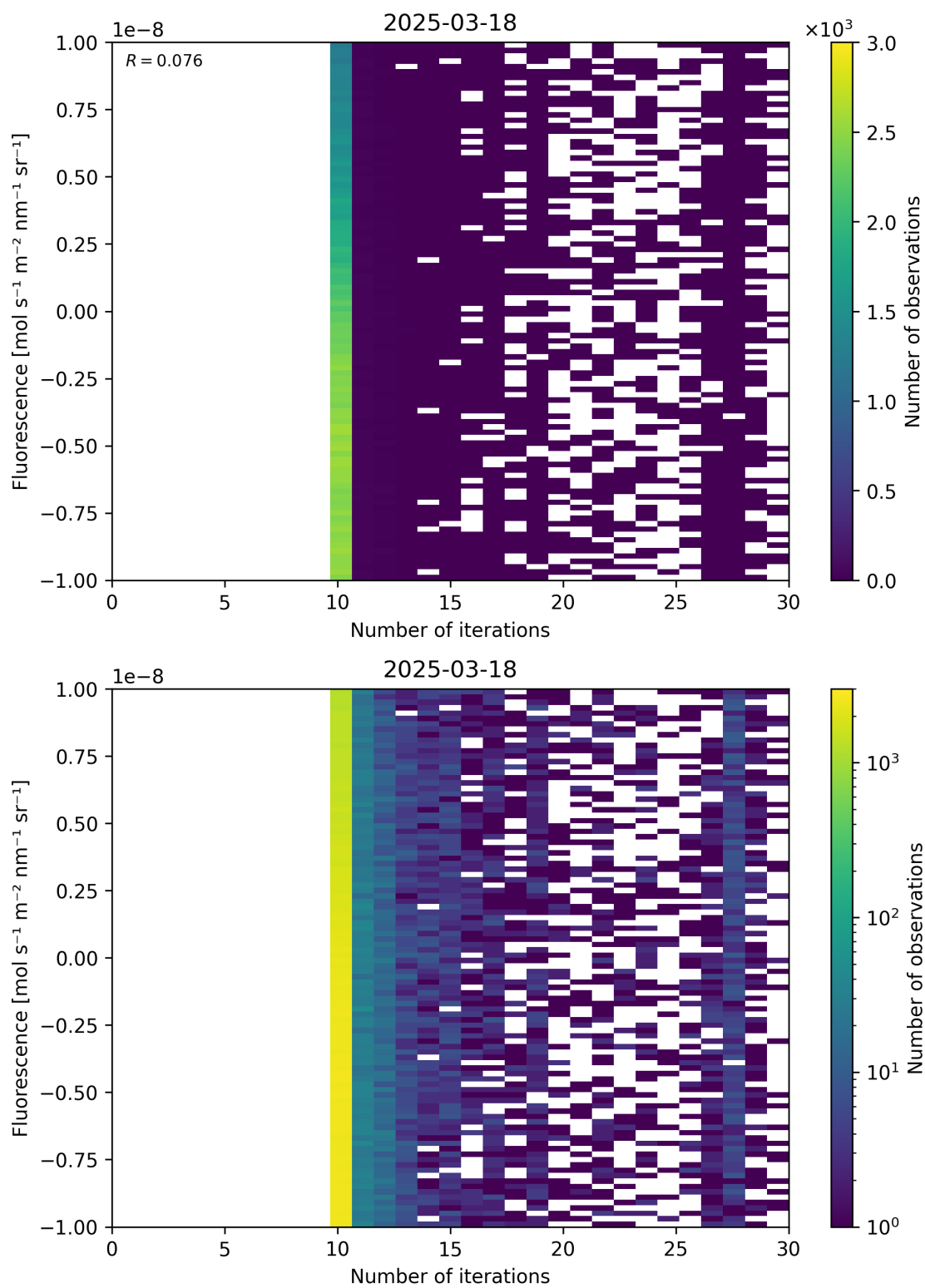
Figure 87: Scatter density plot of “Number of iterations” against “Fluorescence” for 2025-03-17 to 2025-03-19.
