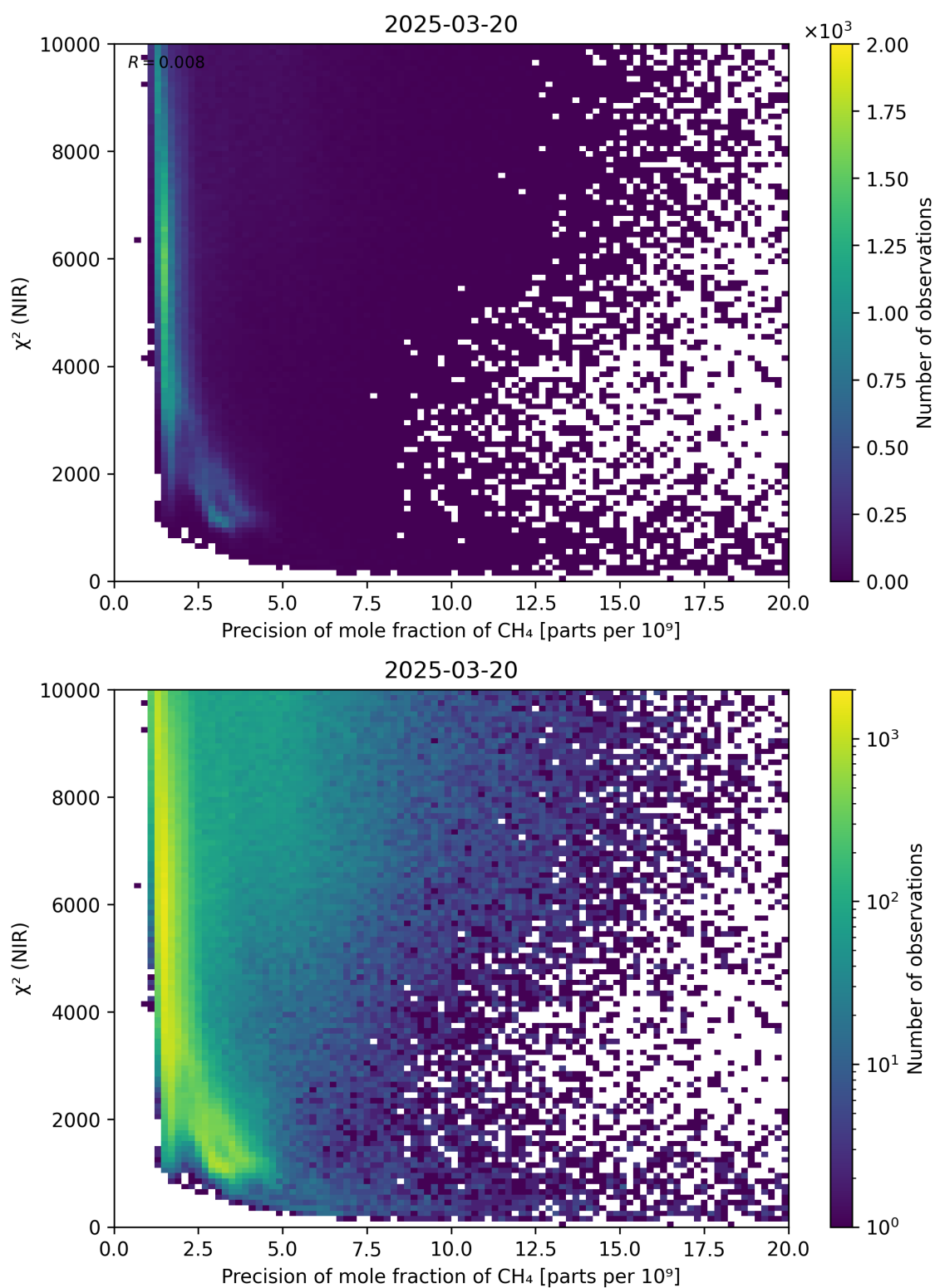
Figure 78: Scatter density plot of “Precision of mole fraction of \text{CH}_4 ” against “ \chi^2 (NIR)” for 2025-03-19 to 2025-03-21.
