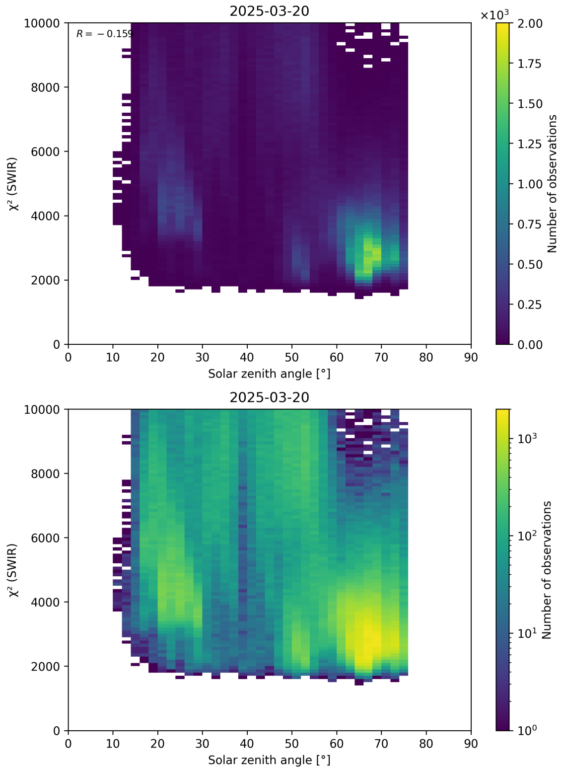
Figure 95: Scatter density plot of “Solar zenith angle” against “ \chi^2 (SWIR)” for 2025-03-19 to 2025-03-21.
