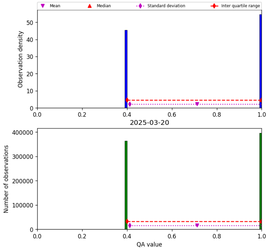
Figure 22: Histogram of “QA value” for 2025-03-19 to 2025-03-21
