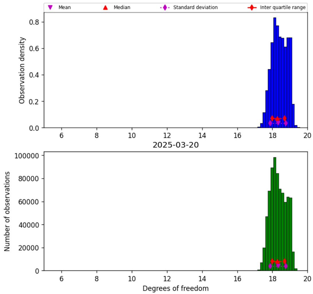
Figure 30: Histogram of “Degrees of freedom” for 2025-03-19 to 2025-03-21
