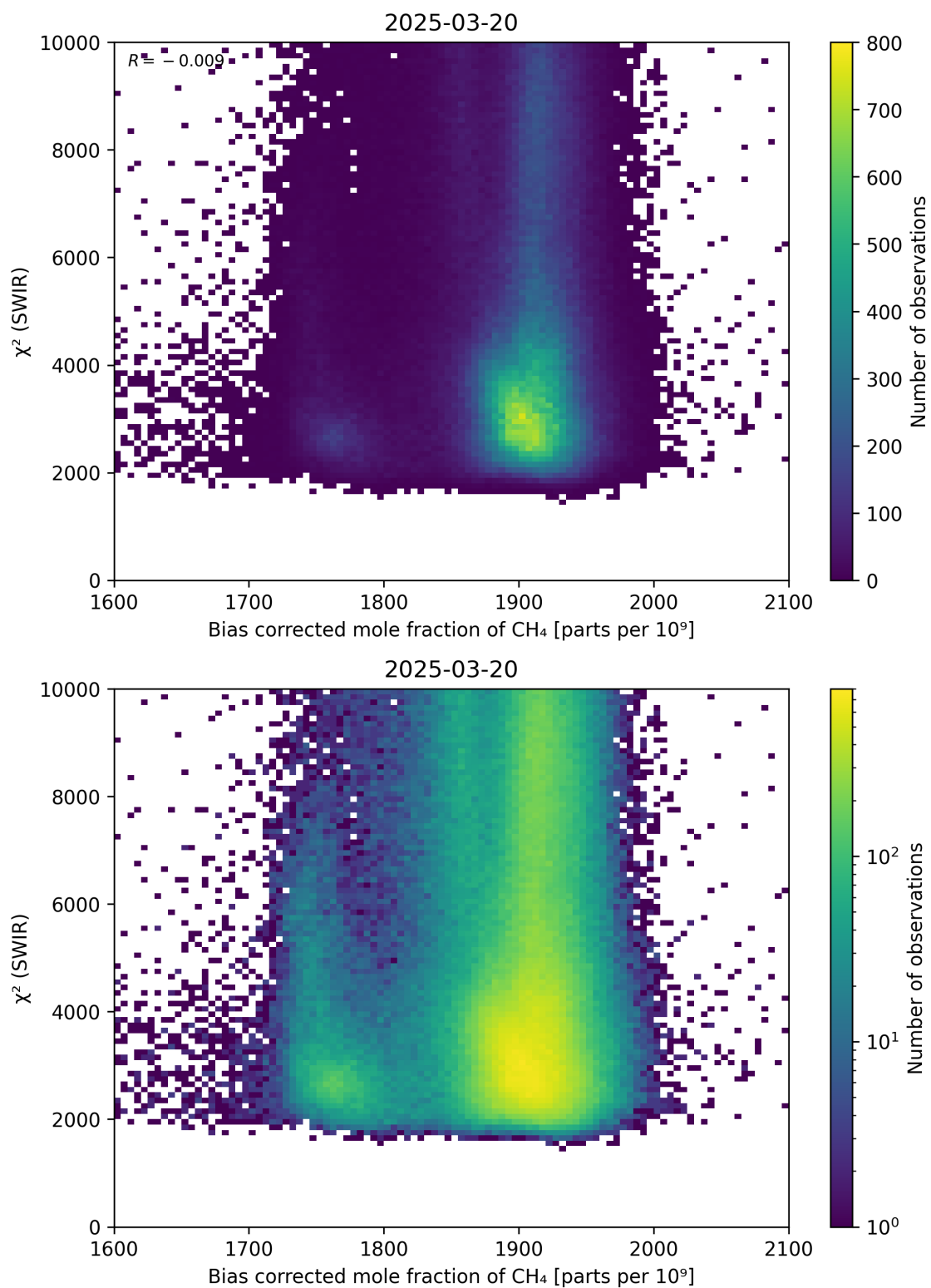
Figure 64: Scatter density plot of “Bias corrected mole fraction of CH 4 ” against “ \chi^2 (SWIR)” for 2025-03-19 to 2025-03-21.
