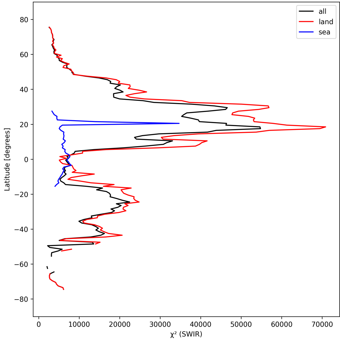
Figure 17: Zonal average of “ \chi^2 (SWIR)” for 2025-03-19 to 2025-03-21.
