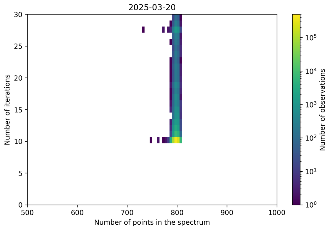
Figure 92: Scatter density plot of “Number of points in the spectrum” against “Number of iterations” for 2025-03-19 to 2025-03-21.
