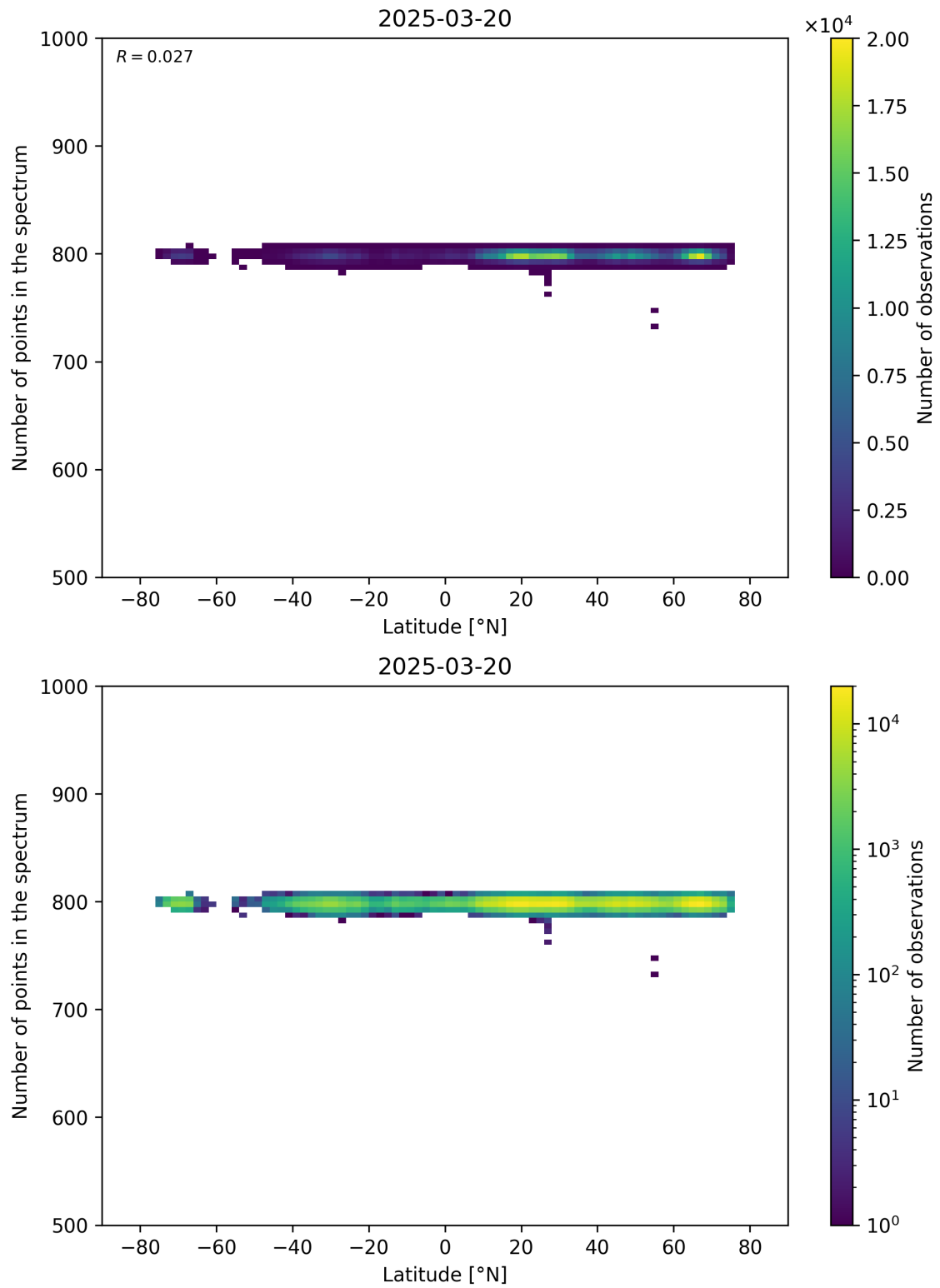
Figure 61: Scatter density plot of “Latitude” against “Number of points in the spectrum” for 2025-03-19 to 2025-03-21.
