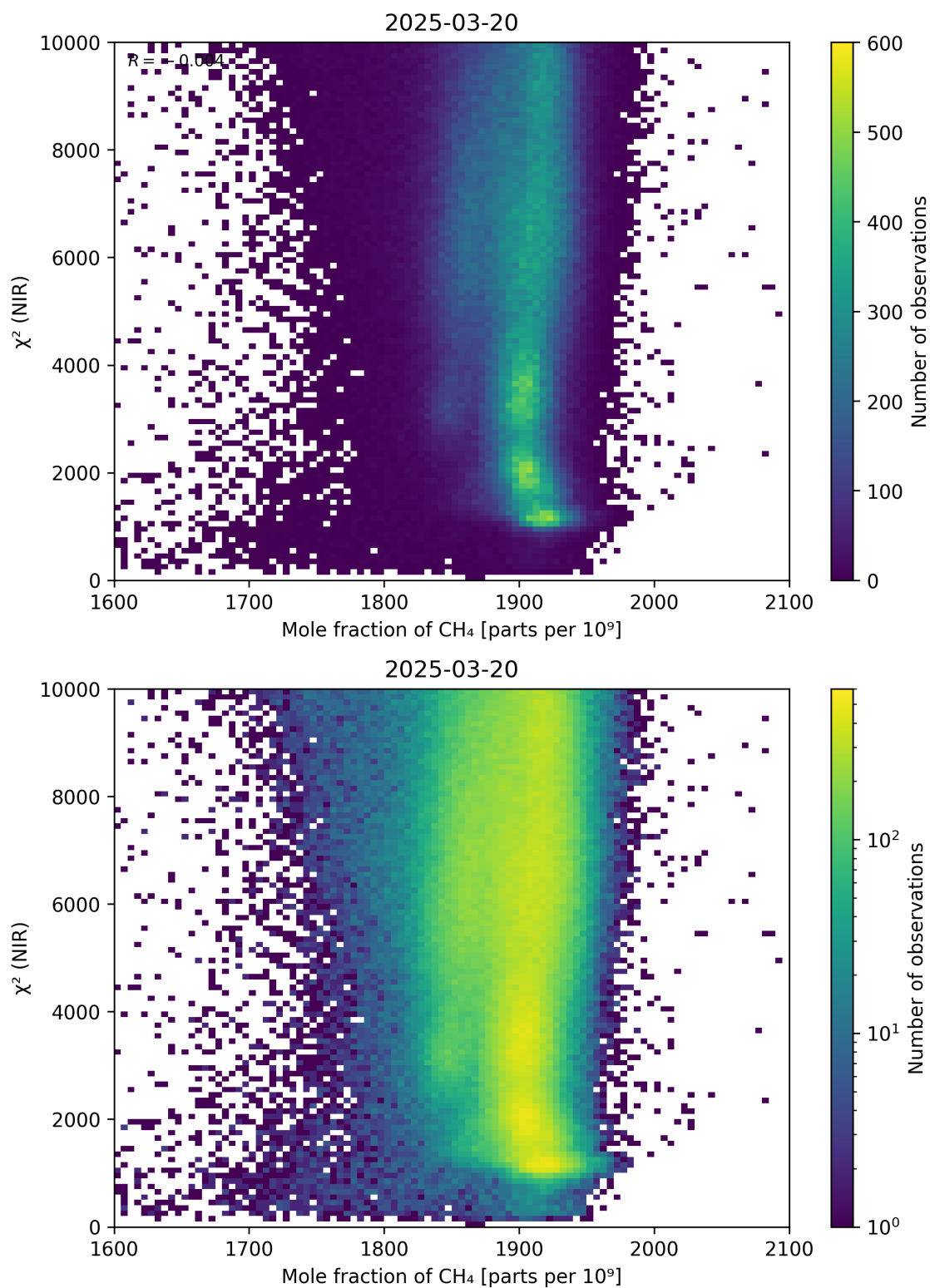
Figure 70: Scatter density plot of “Mole fraction of \text{CH}_4 ” against “ \chi^2 (NIR)” for 2025-03-19 to 2025-03-21.
