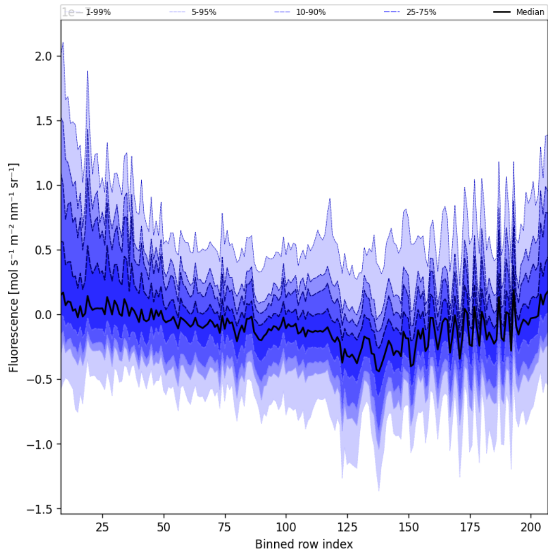
Figure 43: Along track statistics of “Fluorescence” for 2025-03-19 to 2025-03-21
