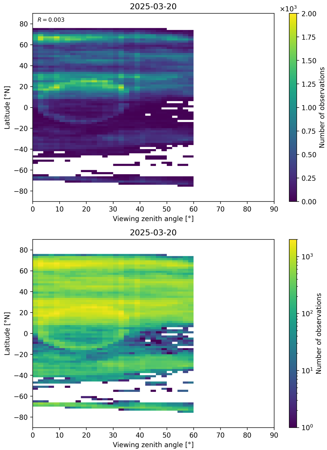
Figure 109: Scatter density plot of “Viewing zenith angle” against “Latitude” for 2025-03-19 to 2025-03-21.
