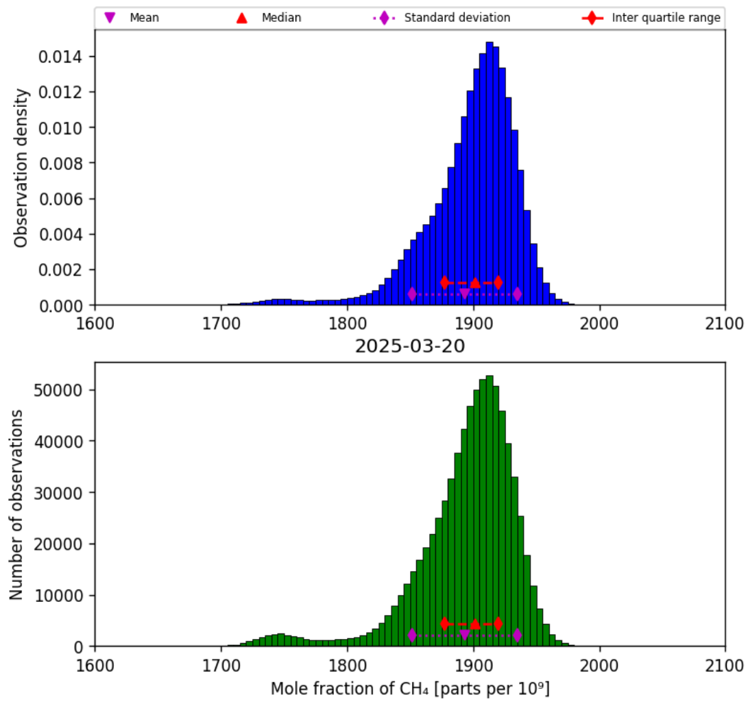
Figure 23: Histogram of “Mole fraction of CH 4 ” for 2025-03-19 to 2025-03-21
