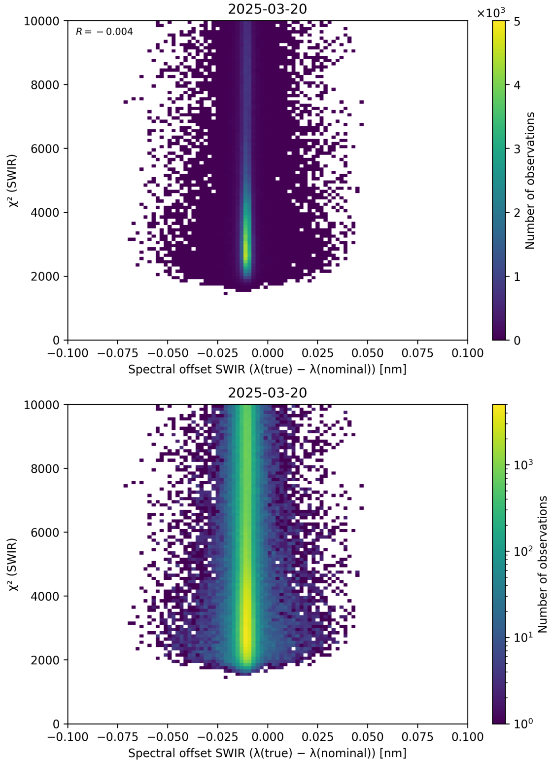
Figure 118: Scatter density plot of “Spectral offset SWIR ( \lambda_{\text{true}} - \lambda_{\text{nominal}} )” against “ \chi^2 (SWIR)” for 2025-03-19 to 2025-03-21.
