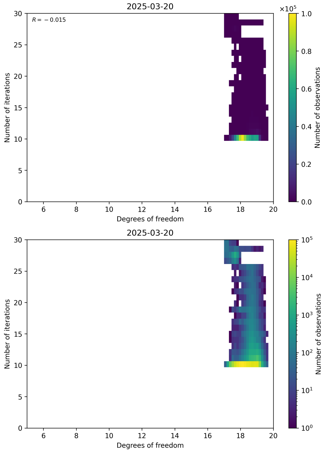
Figure 52: Scatter density plot of “Degrees of freedom” against “Number of iterations” for 2025-03-19 to 2025-03-21.
