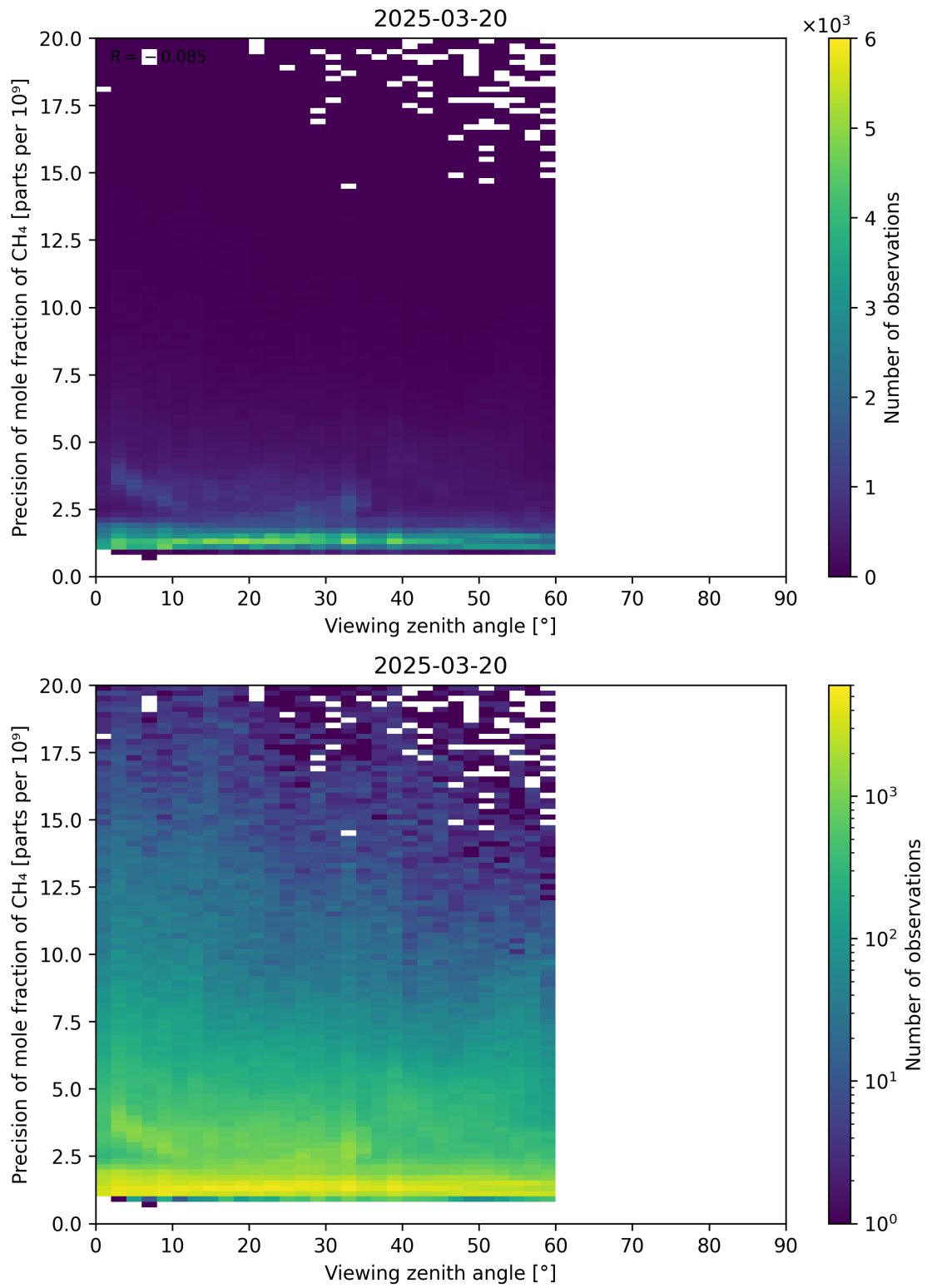
Figure 112: Scatter density plot of “Viewing zenith angle” against “Precision of mole fraction of CH 4 ” for 2025-03-19 to 2025-03-21.
