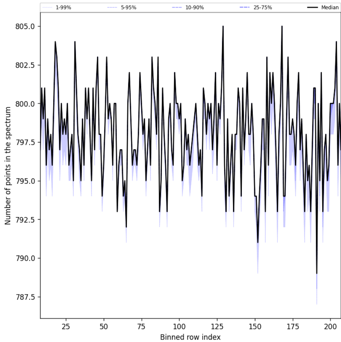
Figure 37: Along track statistics of “Number of points in the spectrum” for 2025-03-19 to 2025-03-21
