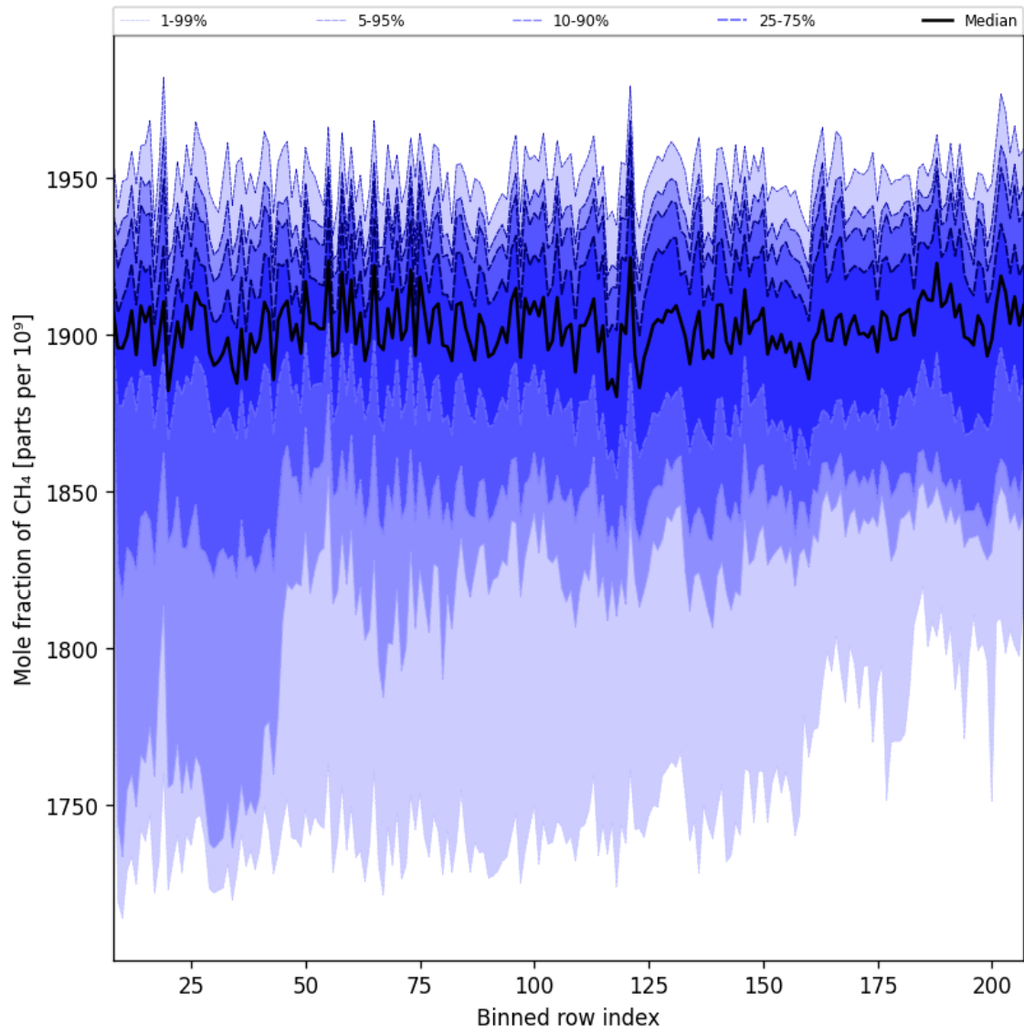
Figure 34: Along track statistics of “Mole fraction of CH 4 ” for 2025-03-19 to 2025-03-21
