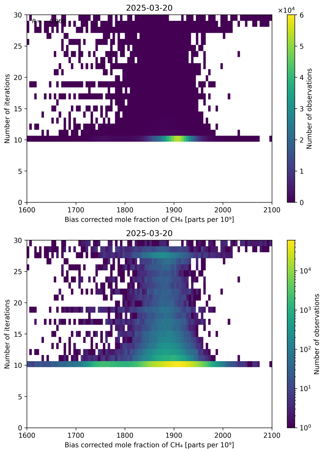
Figure 67: Scatter density plot of “Bias corrected mole fraction of CH 4 ” against “Number of iterations” for 2025-03-19 to 2025-03-21.
