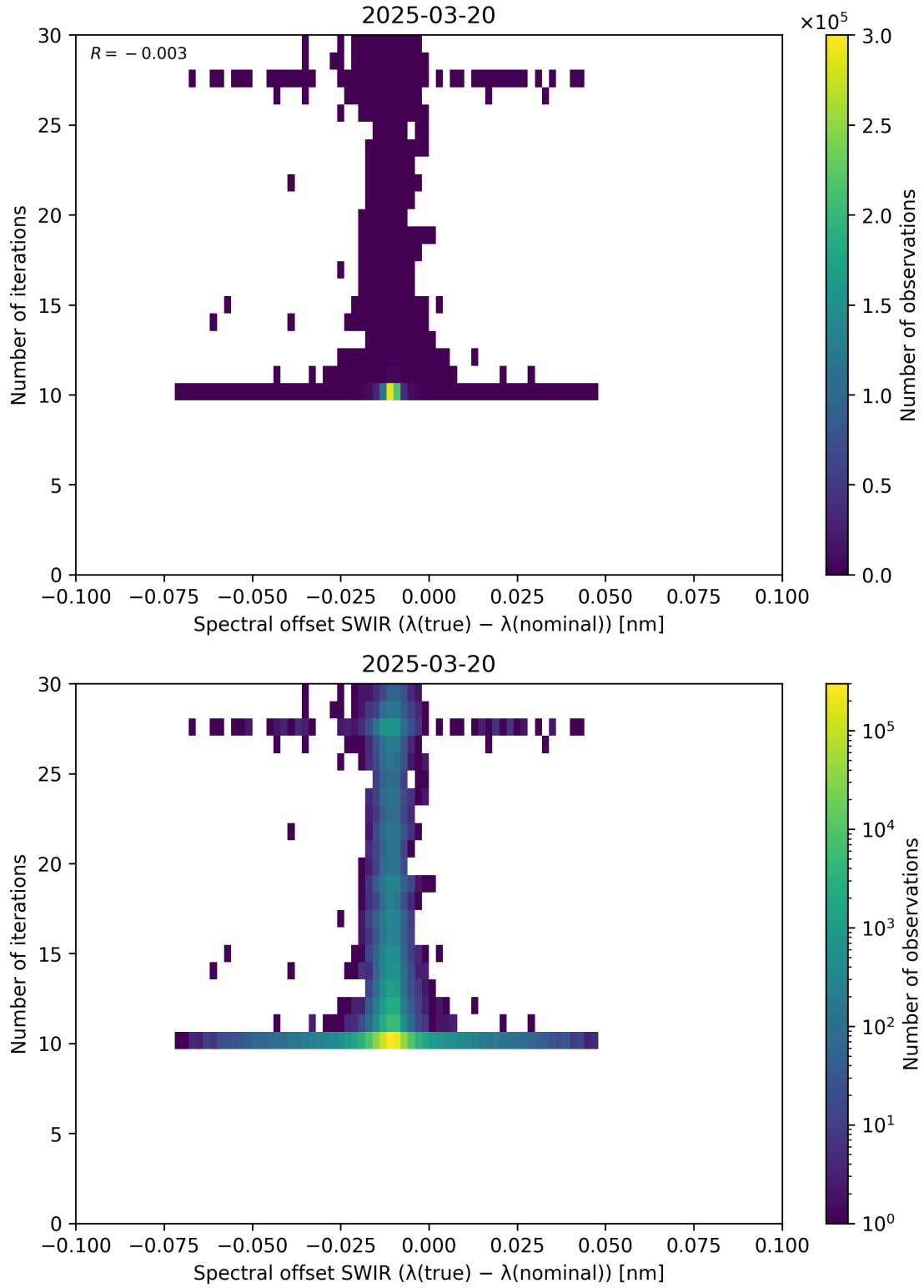
Figure 121: Scatter density plot of “Spectral offset SWIR ( \lambda_{\text{true}} - \lambda_{\text{nominal}} )” against “Number of iterations” for 2025-03-19 to 2025-03-21.
