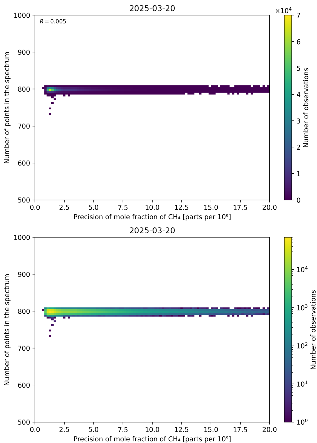
Figure 84: Scatter density plot of “Precision of mole fraction of CH 4 ” against “Number of points in the spectrum” for 2025-03-19 to 2025-03-21.
