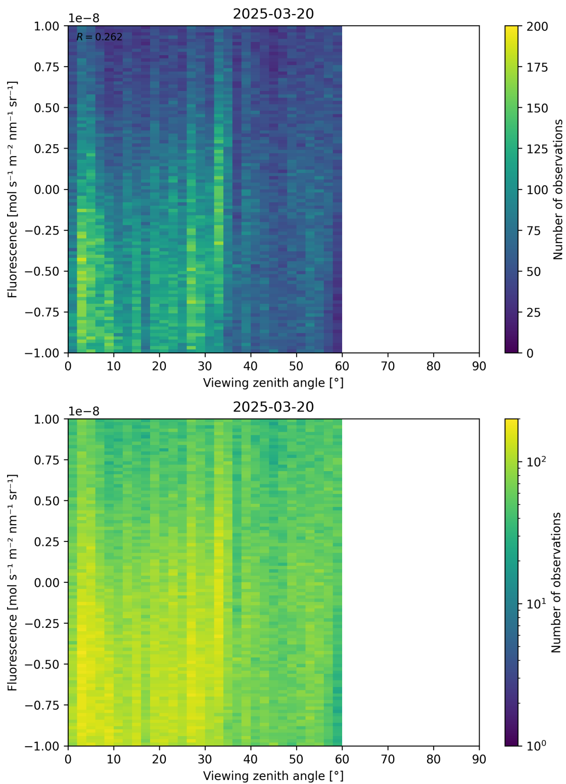
Figure 108: Scatter density plot of “Viewing zenith angle” against “Fluorescence” for 2025-03-19 to 2025-03-21.
