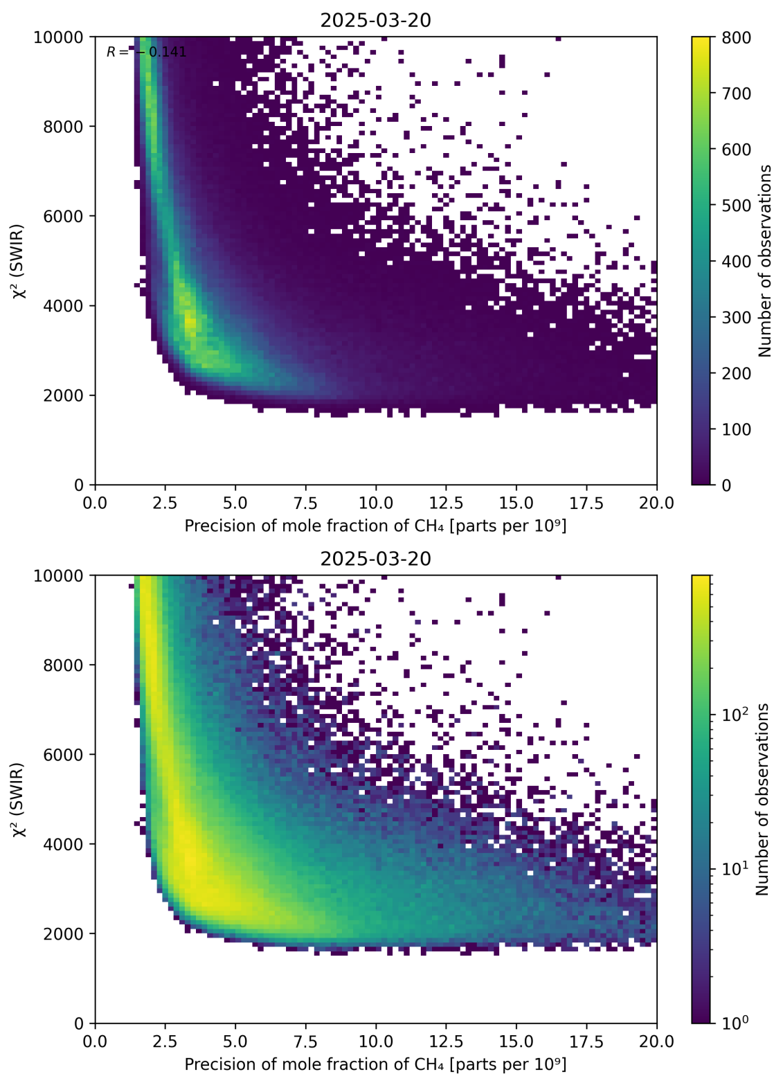
Figure 79: Scatter density plot of “Precision of mole fraction of \text{CH}_4 ” against “ \chi^2 (SWIR)” for 2025-03-19 to 2025-03-21.
