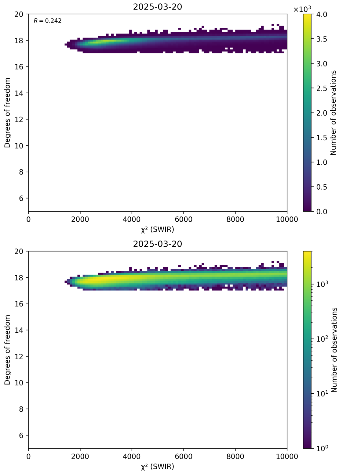
Figure 48: Scatter density plot of “ \chi^2 (SWIR)” against “Degrees of freedom” for 2025-03-19 to 2025-03-21.
