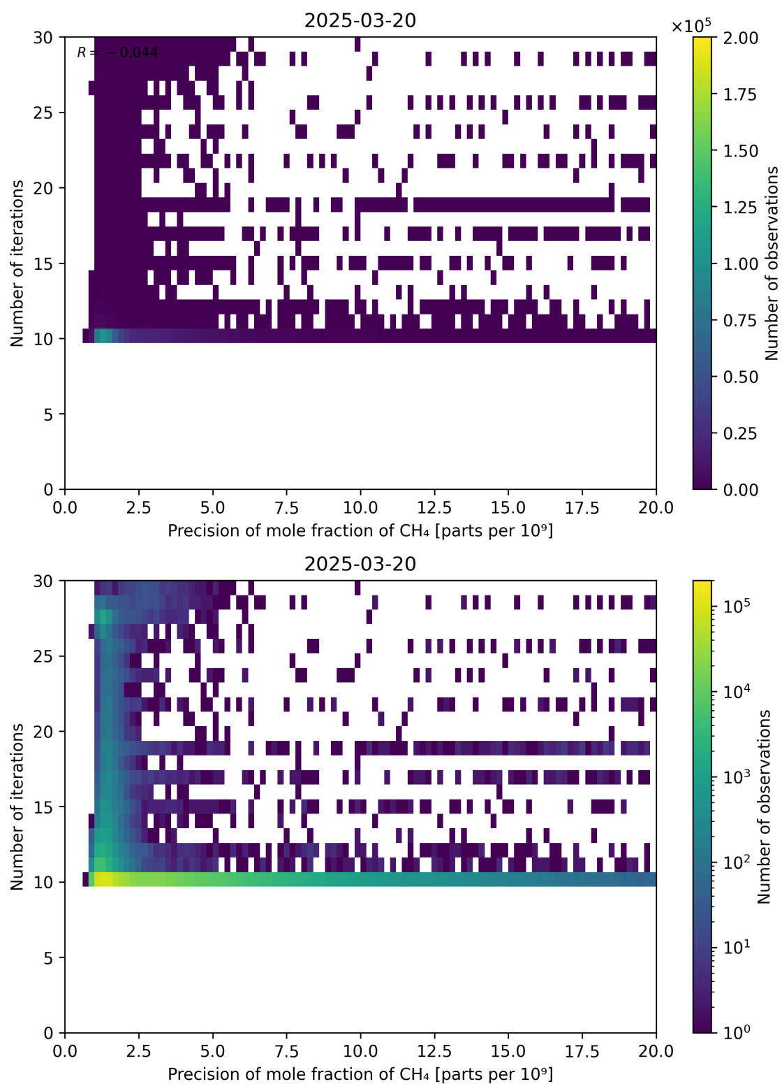
Figure 83: Scatter density plot of “Precision of mole fraction of CH 4 ” against “Number of iterations” for 2025-03-19 to 2025-03-21.
