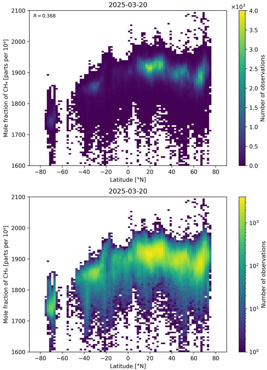
Figure 57: Scatter density plot of “Latitude” against “Mole fraction of CH 4 ” for 2025-03-19 to 2025-03-21.
