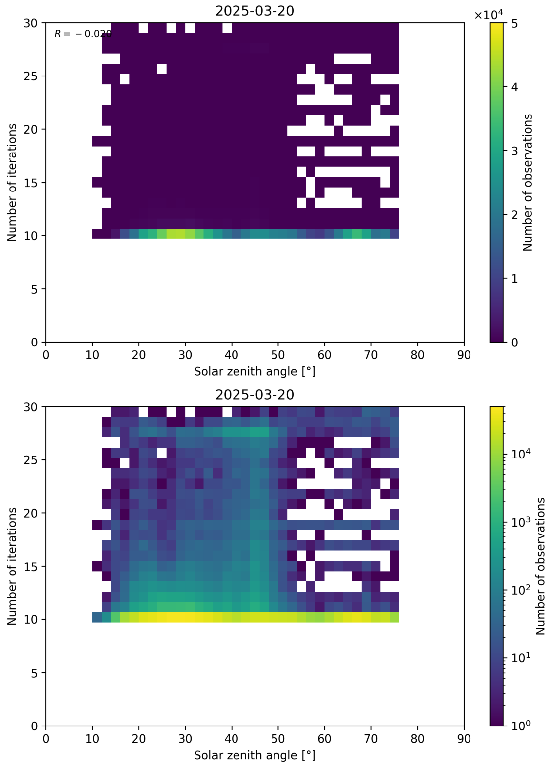
Figure 102: Scatter density plot of “Solar zenith angle” against “Number of iterations” for 2025-03-19 to 2025-03-21.
