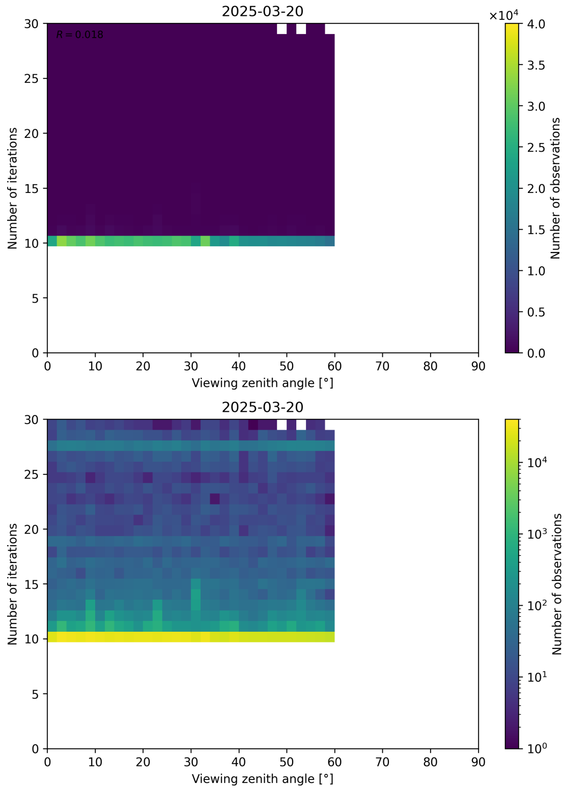
Figure 113: Scatter density plot of “Viewing zenith angle” against “Number of iterations” for 2025-03-19 to 2025-03-21.
