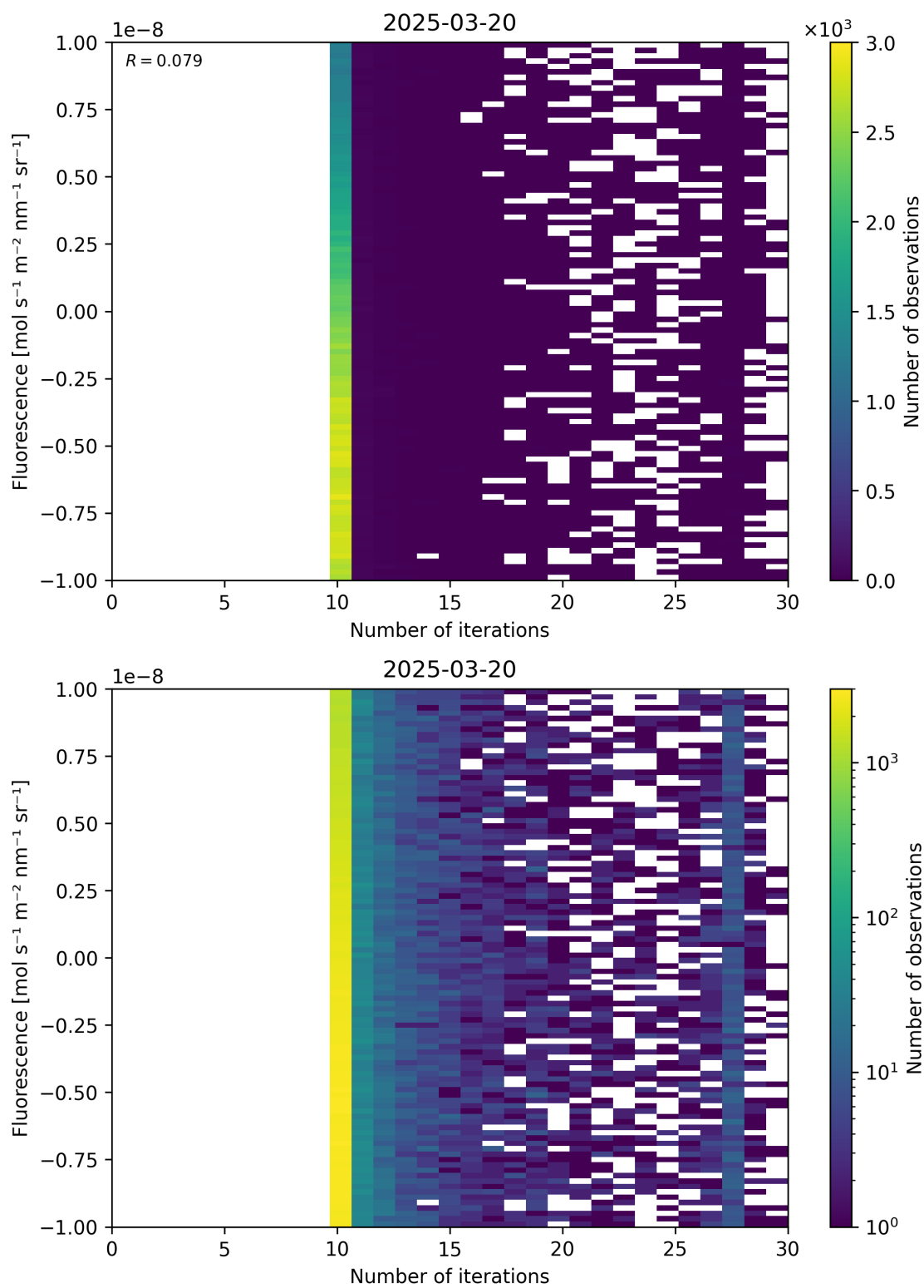
Figure 87: Scatter density plot of “Number of iterations” against “Fluorescence” for 2025-03-19 to 2025-03-21.
