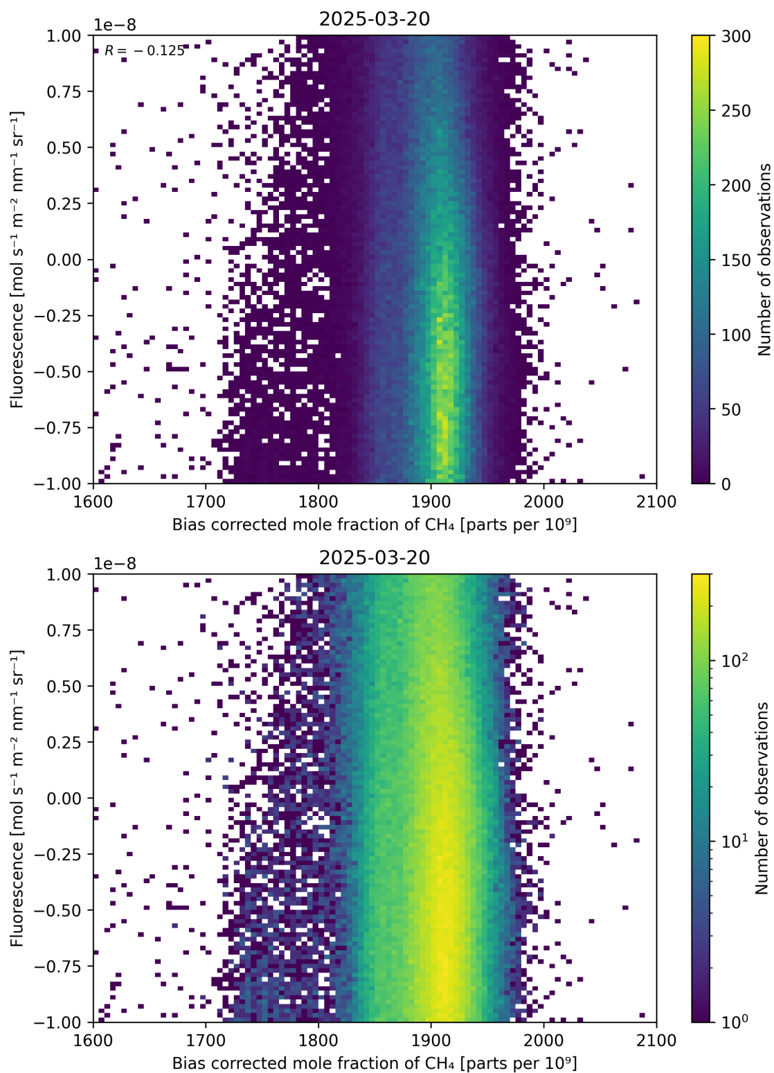
Figure 66: Scatter density plot of “Bias corrected mole fraction of \text{CH}_4 ” against “Fluorescence” for 2025-03-19 to 2025-03-21.
