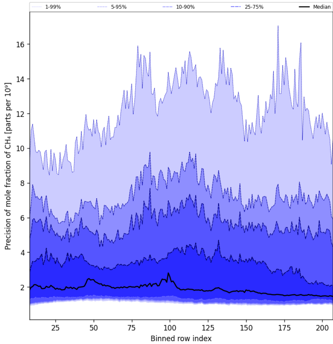
Figure 35: Along track statistics of “Precision of mole fraction of CH 4 ” for 2025-03-19 to 2025-03-21
