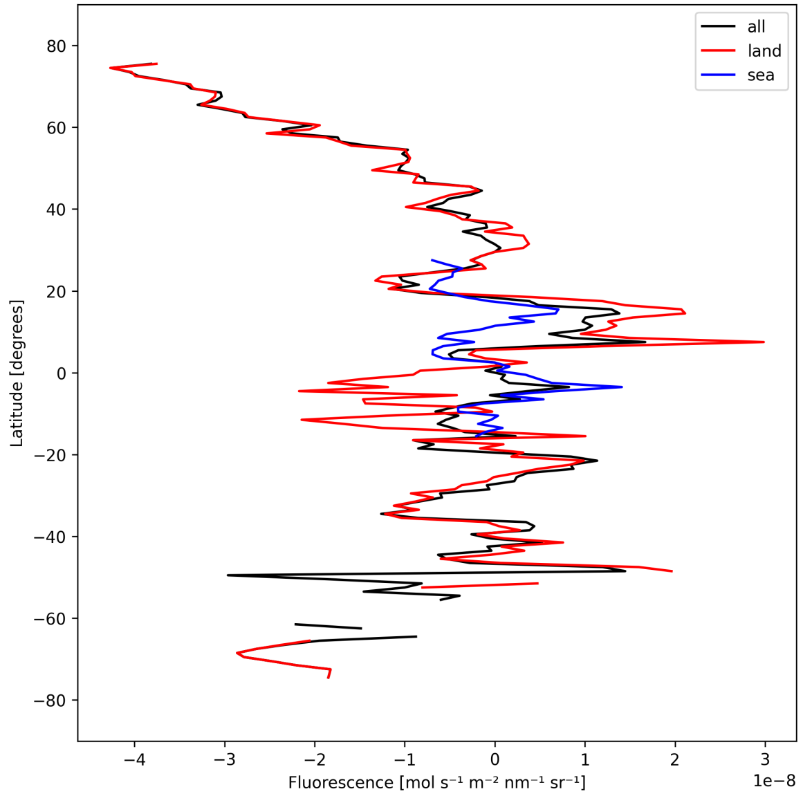
Figure 21: Zonal average of “Fluorescence” for 2025-03-19 to 2025-03-21.
