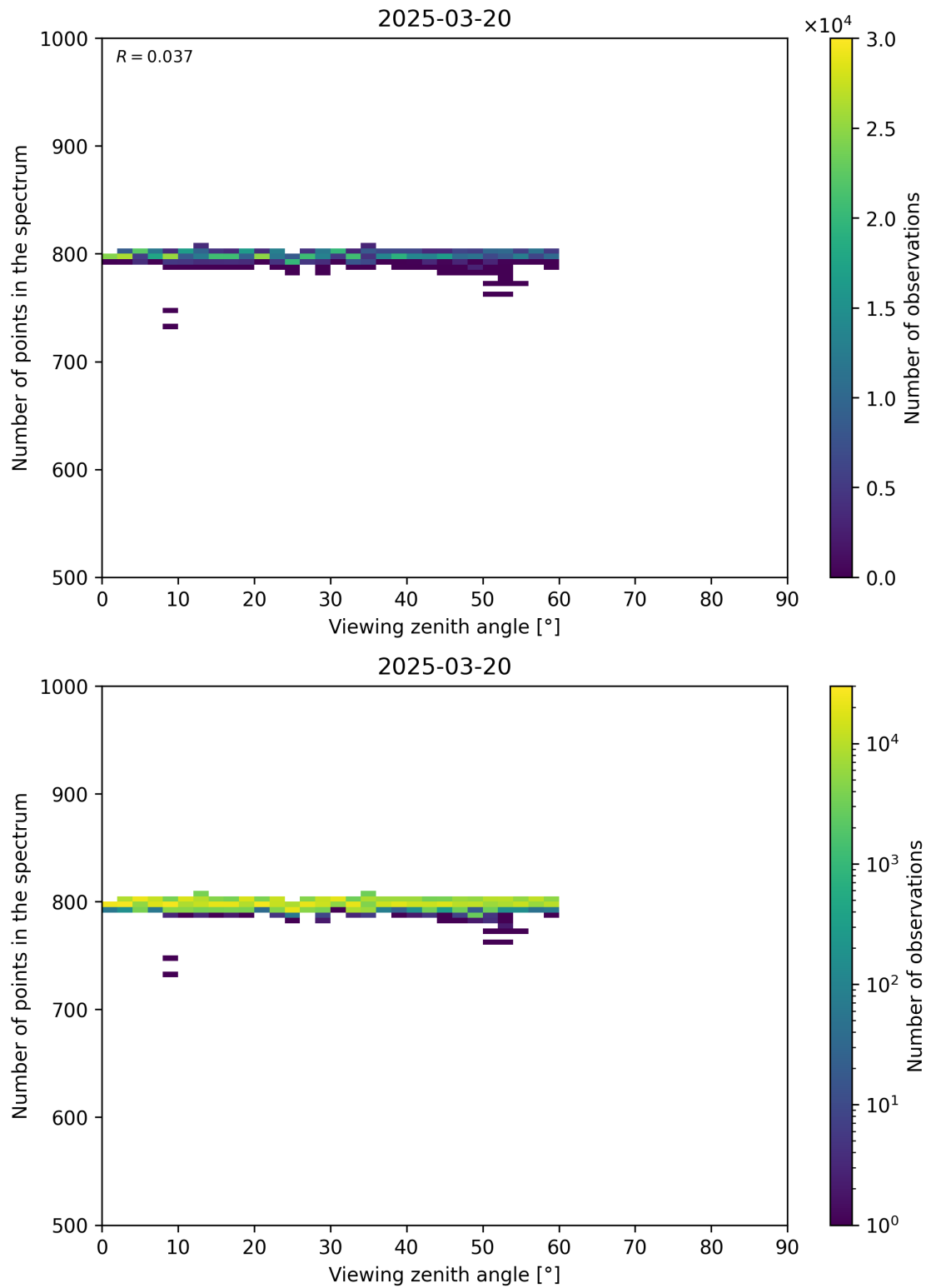
Figure 114: Scatter density plot of “Viewing zenith angle” against “Number of points in the spectrum” for 2025-03-19 to 2025-03-21.
