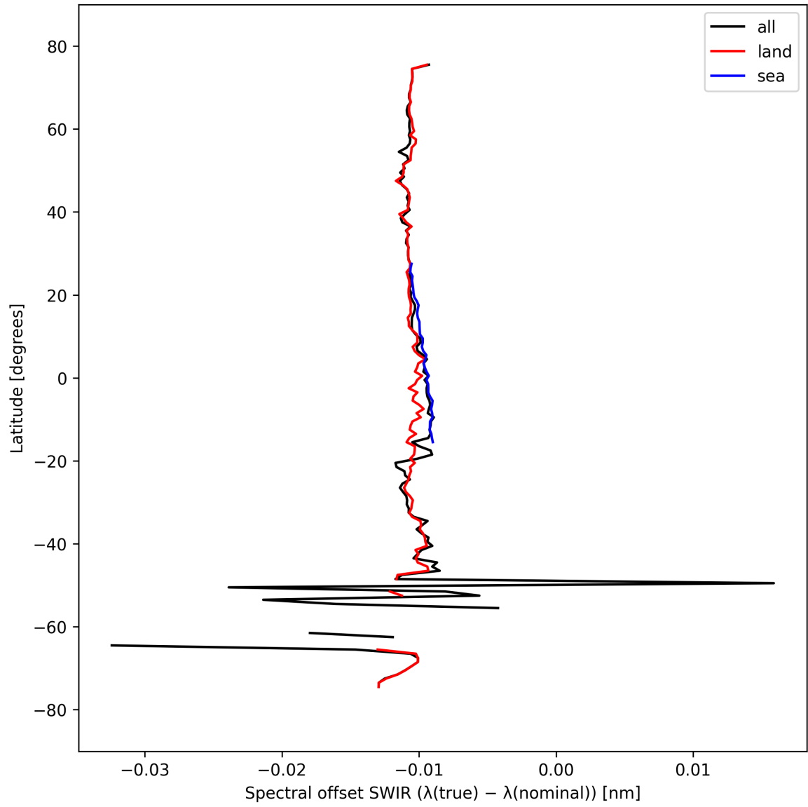
Figure 16: Zonal average of “Spectral offset SWIR ( \lambda_{\text{true}} - \lambda_{\text{nominal}} )” for 2025-03-19 to 2025-03-21.
