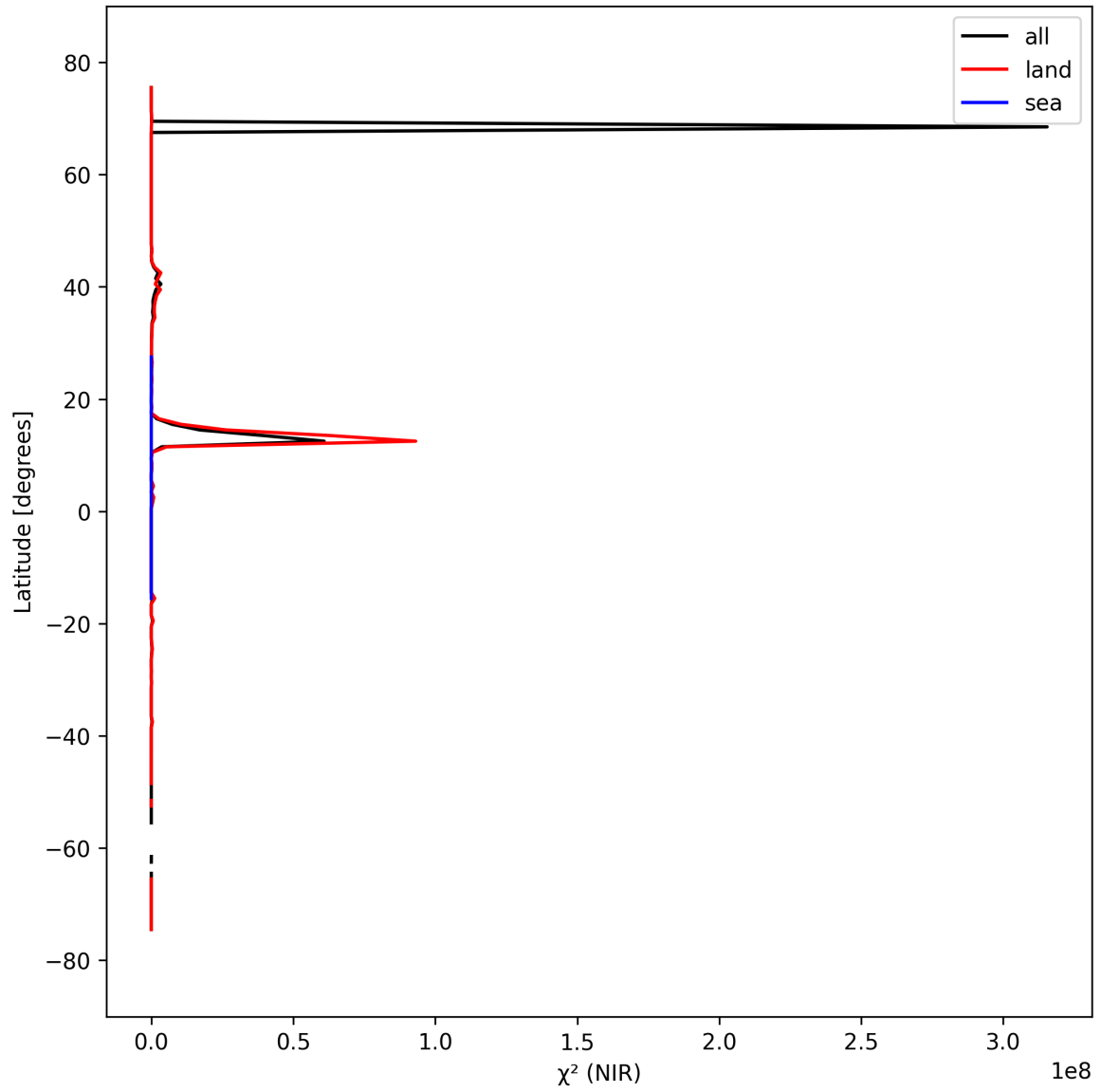
Figure 18: Zonal average of “ \chi^2 (NIR)” for 2025-03-19 to 2025-03-21.
