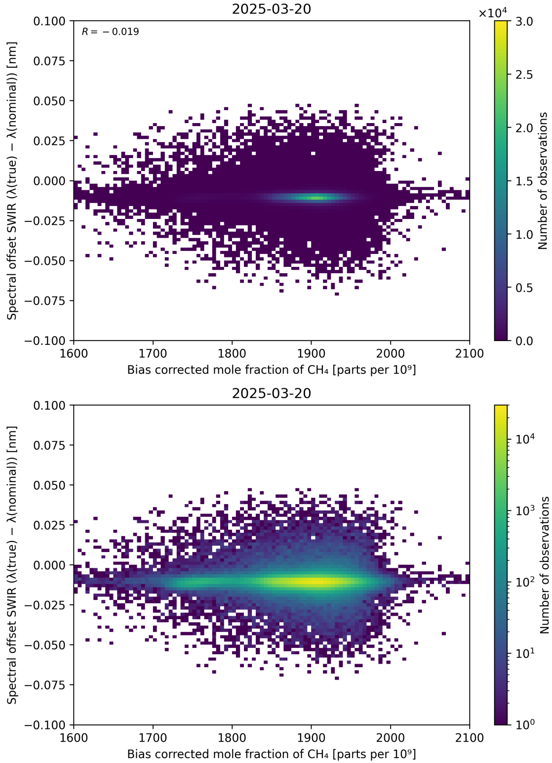
Figure 69: Scatter density plot of “Bias corrected mole fraction of \text{CH}_4 ” against “Spectral offset SWIR ( \lambda_{\text{true}} - \lambda_{\text{nominal}} )” for 2025-03-19 to 2025-03-21.
