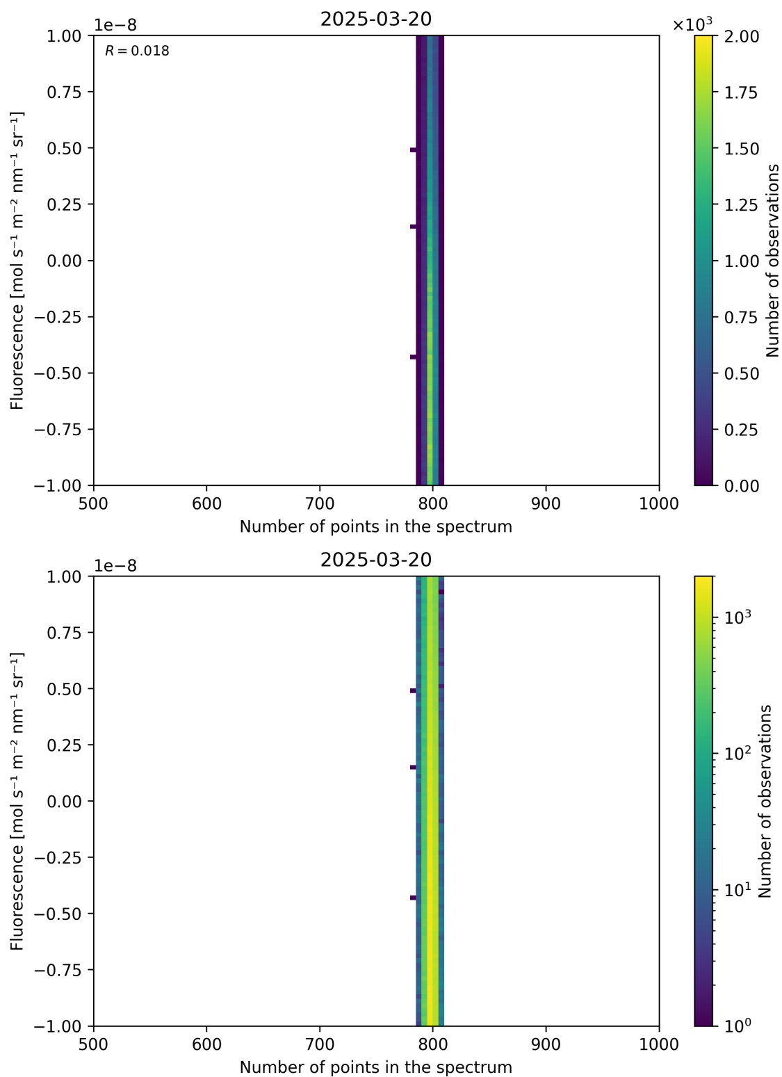
Figure 91: Scatter density plot of “Number of points in the spectrum” against “Fluorescence” for 2025-03-19 to 2025-03-21.
