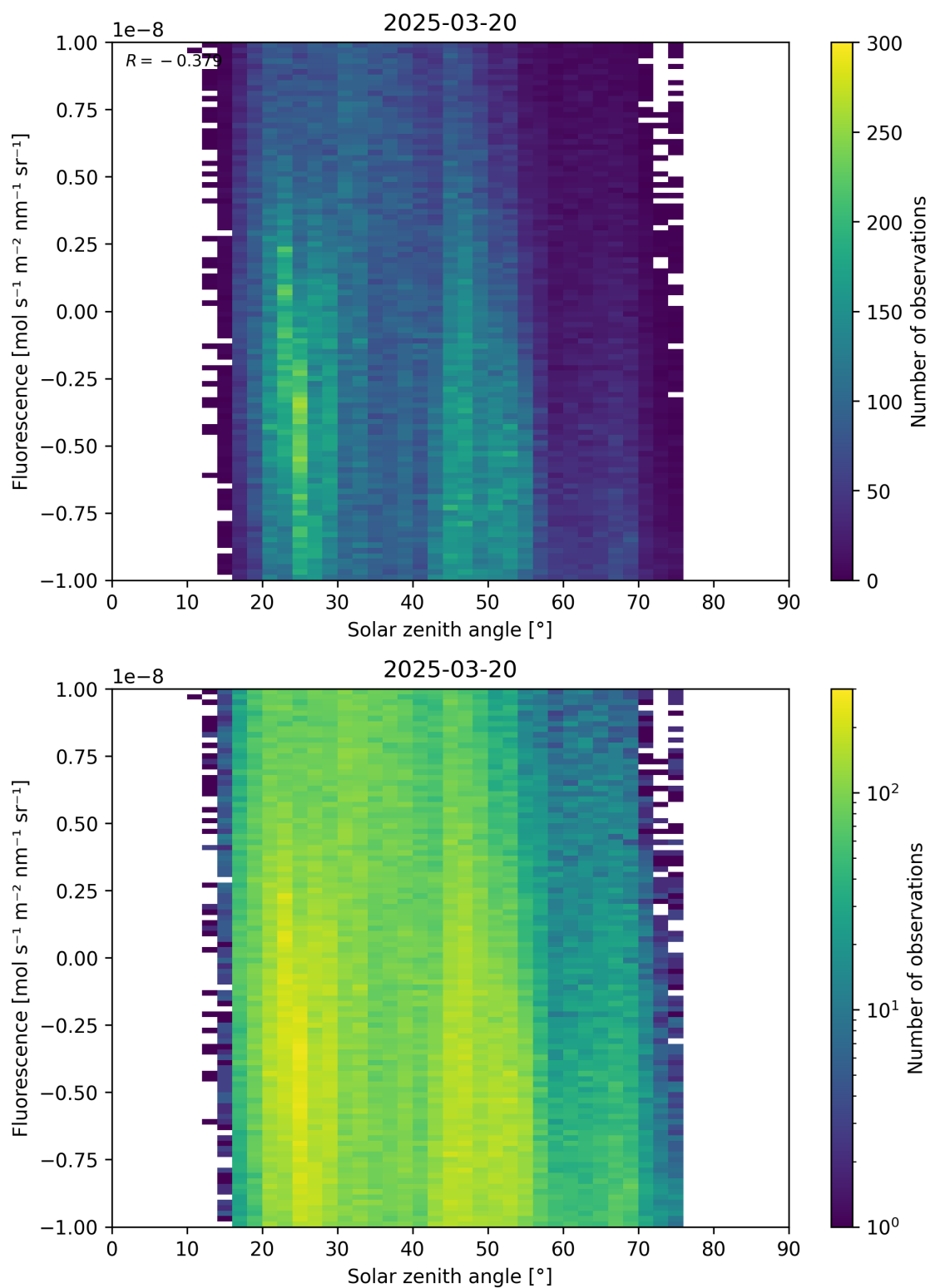
Figure 97: Scatter density plot of “Solar zenith angle” against “Fluorescence” for 2025-03-19 to 2025-03-21.
