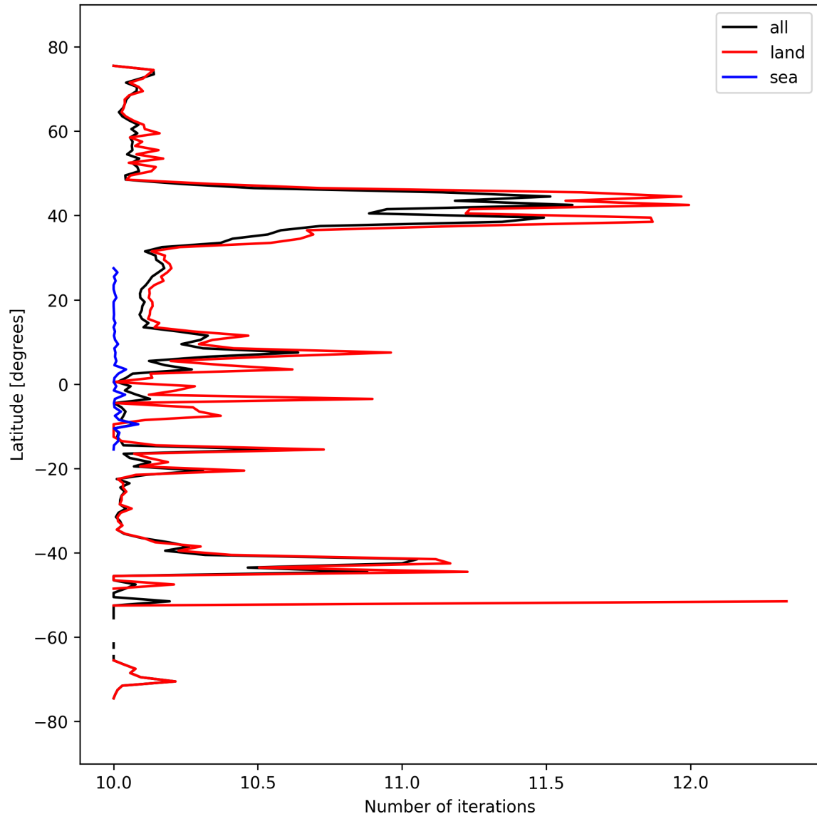
Figure 20: Zonal average of “Number of iterations” for 2025-03-19 to 2025-03-21.
