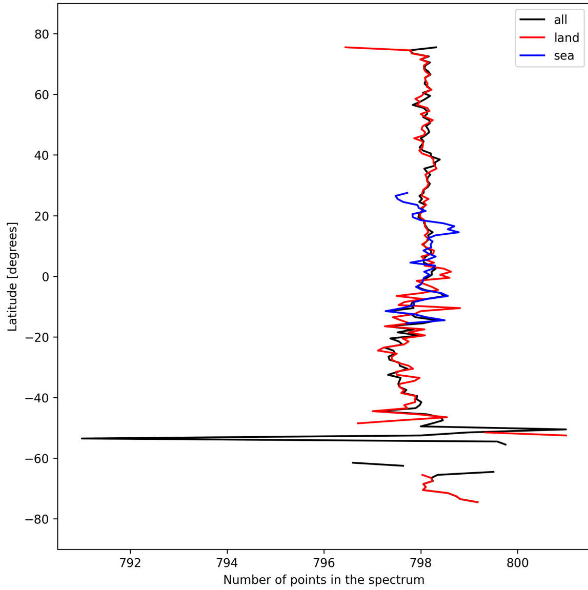
Figure 15: Zonal average of “Number of points in the spectrum” for 2025-03-19 to 2025-03-21.
