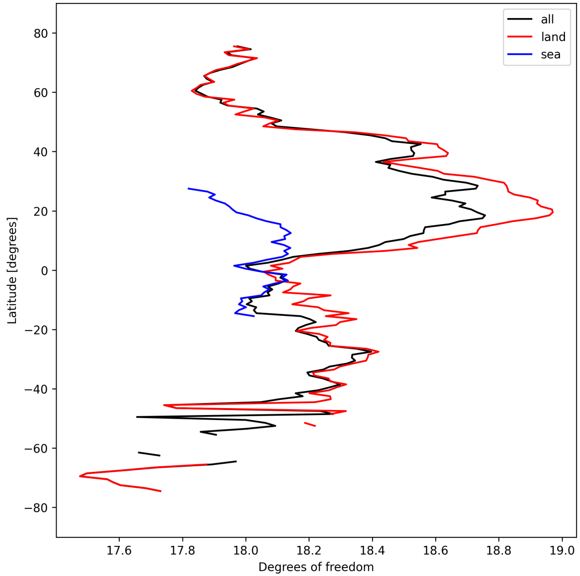
Figure 19: Zonal average of “Degrees of freedom” for 2025-03-19 to 2025-03-21.
