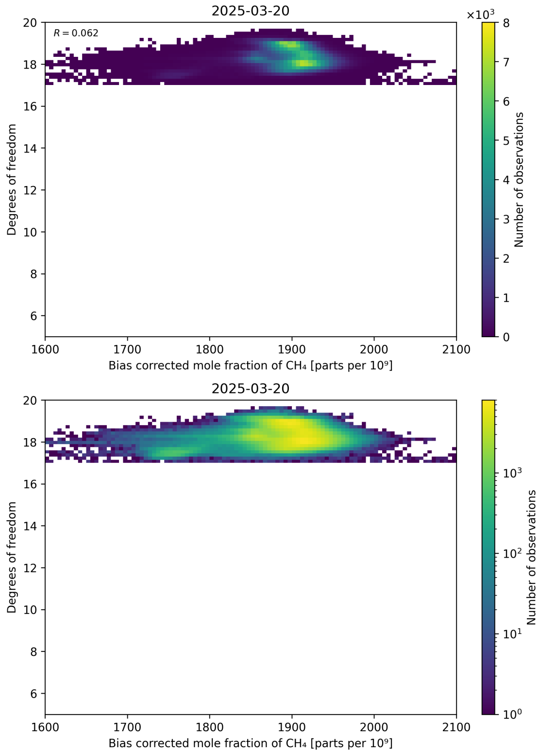
Figure 65: Scatter density plot of “Bias corrected mole fraction of \text{CH}_4 ” against “Degrees of freedom” for 2025-03-19 to 2025-03-21.
