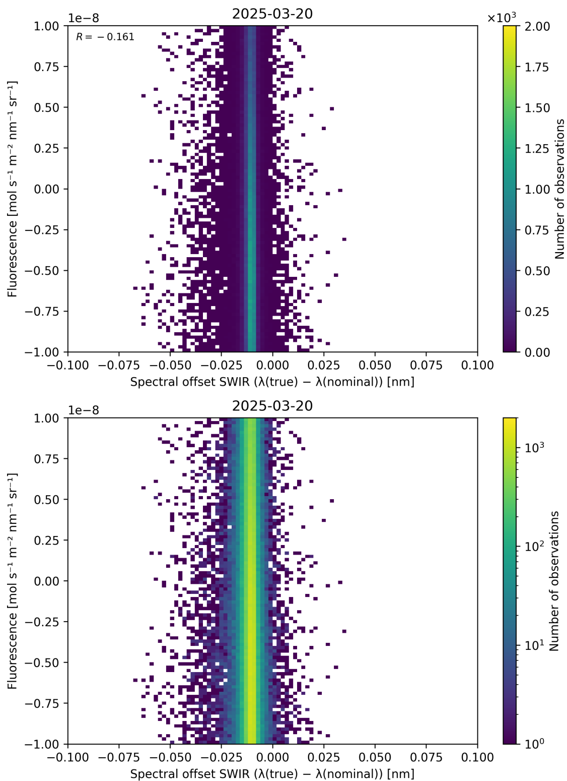
Figure 120: Scatter density plot of “Spectral offset SWIR ( \lambda_{\text{true}} - \lambda_{\text{nominal}} )” against “Fluorescence” for 2025-03-19 to 2025-03-21.
