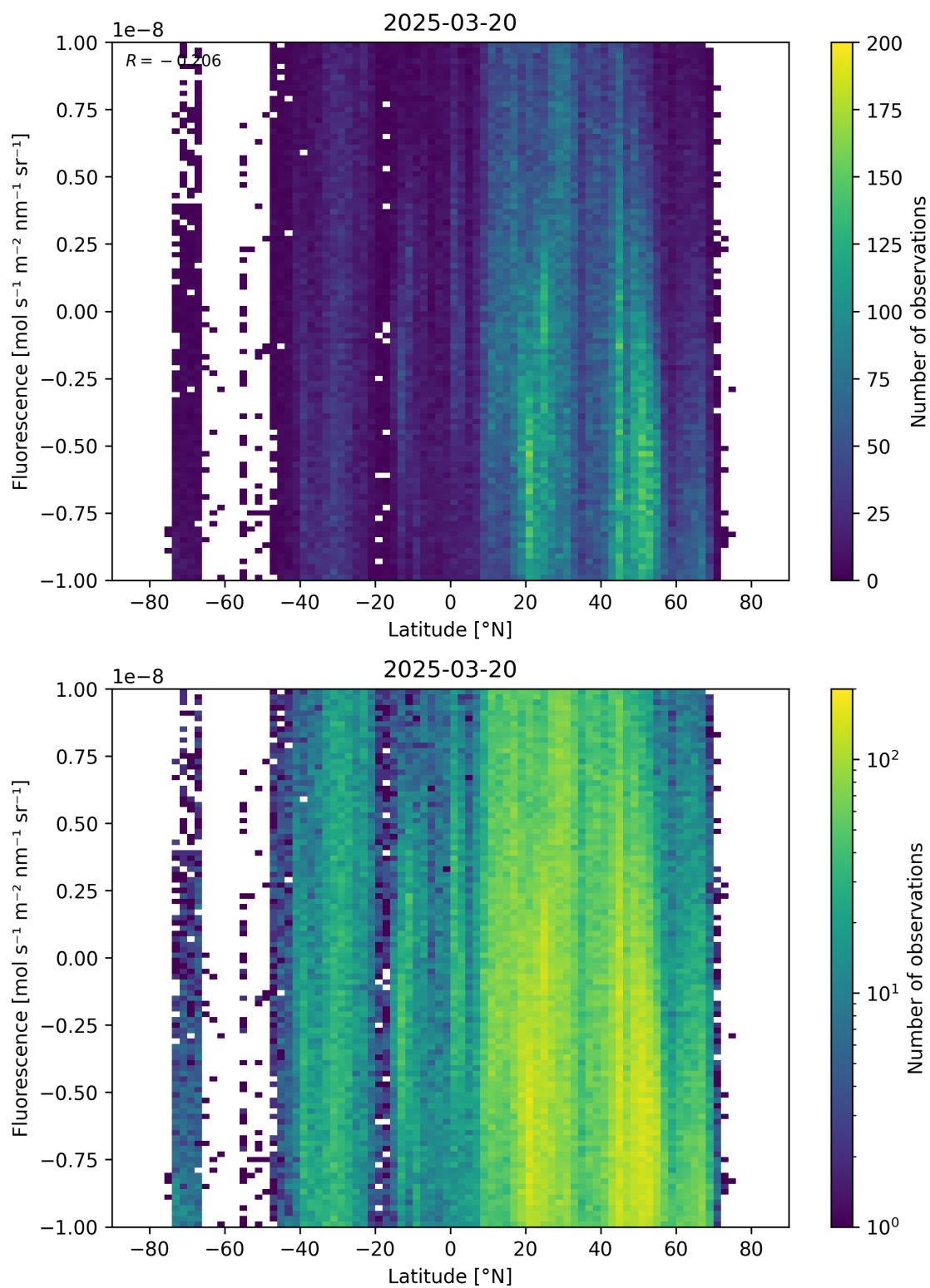
Figure 56: Scatter density plot of “Latitude” against “Fluorescence” for 2025-03-19 to 2025-03-21.
