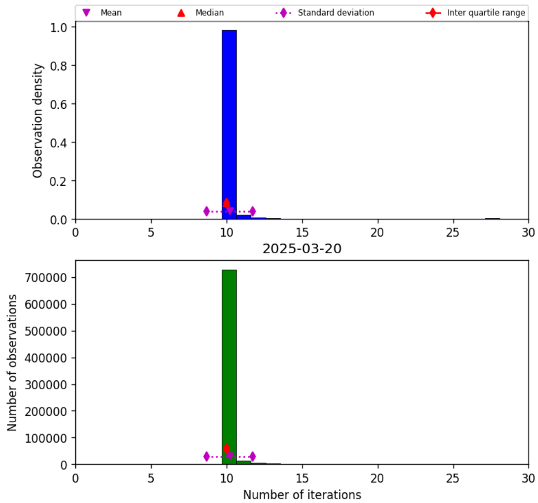
Figure 31: Histogram of "Number of iterations" for 2025-03-19 to 2025-03-21
