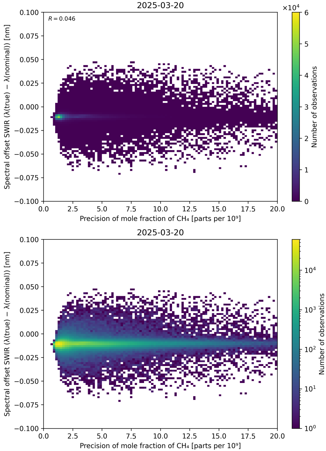
Figure 85: Scatter density plot of “Precision of mole fraction of CH 4 ” against “Spectral offset SWIR ( \lambda_{\text{true}} - \lambda_{\text{nominal}} )” for 2025-03-19 to 2025-03-21.
