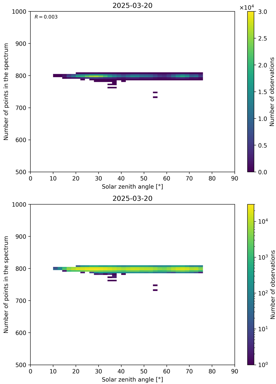
Figure 103: Scatter density plot of “Solar zenith angle” against “Number of points in the spectrum” for 2025-03-19 to 2025-03-21.
