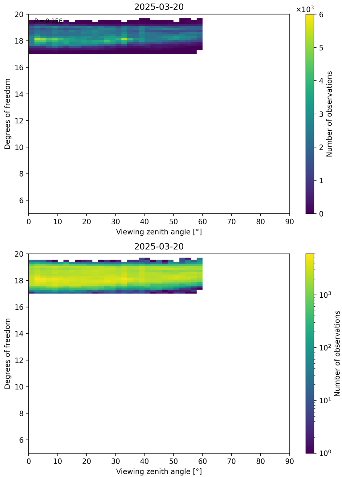
Figure 107: Scatter density plot of “Viewing zenith angle” against “Degrees of freedom” for 2025-03-19 to 2025-03-21.
