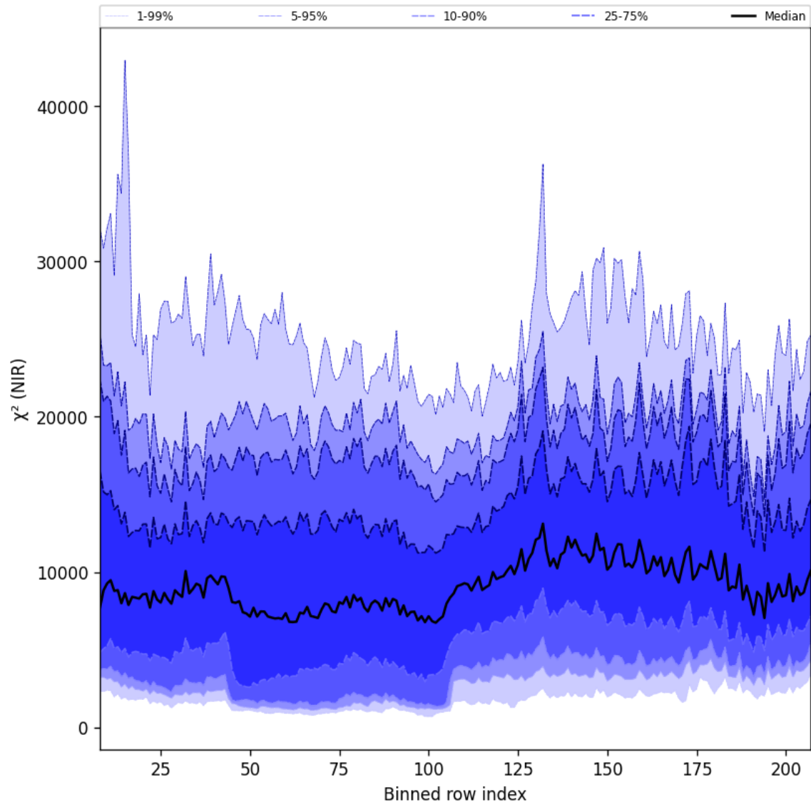
Figure 40: Along track statistics of " \chi^2 (NIR)" for 2025-03-19 to 2025-03-21
