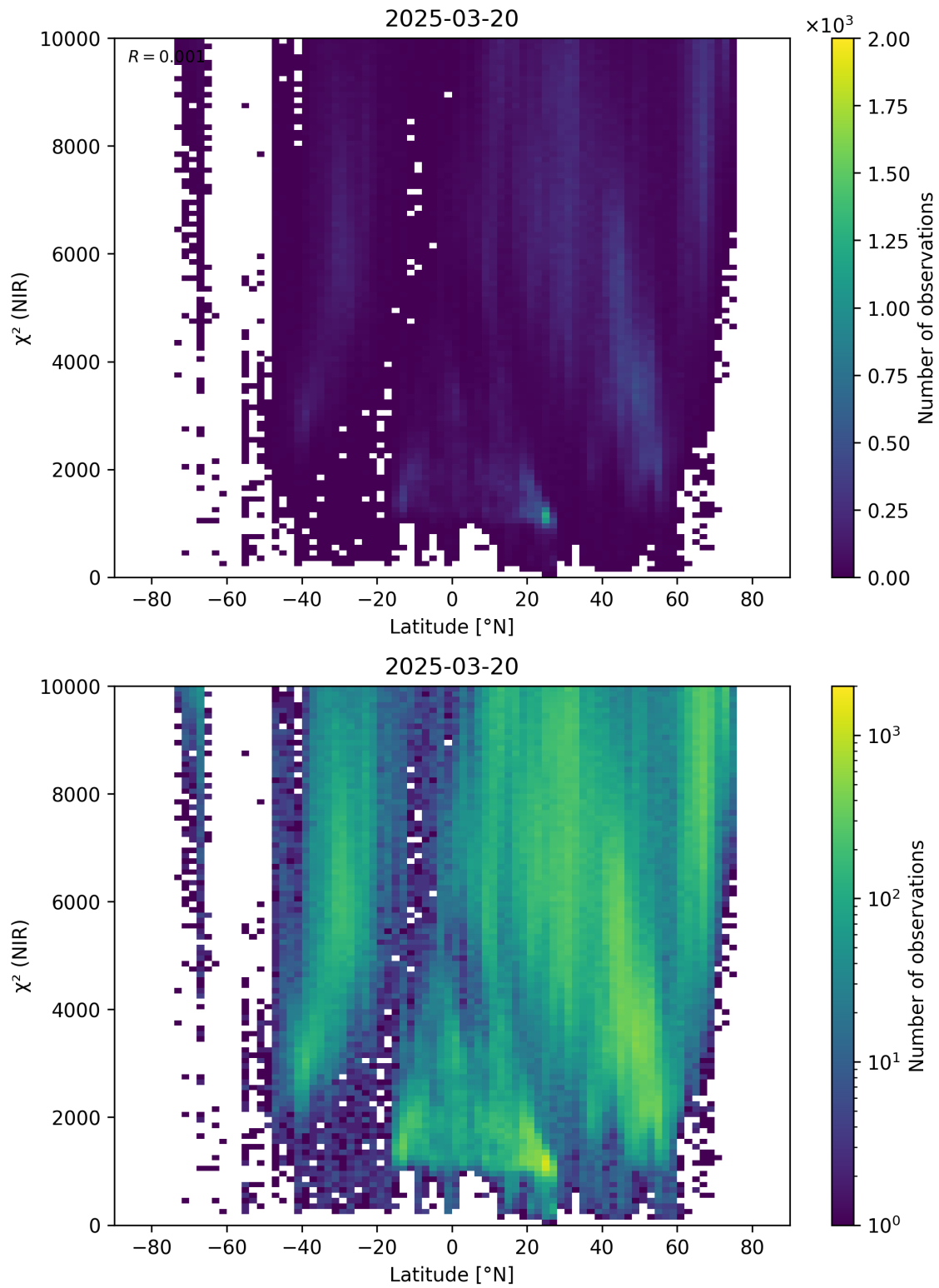
Figure 53: Scatter density plot of “Latitude” against “ \chi^2 (NIR)” for 2025-03-19 to 2025-03-21.
