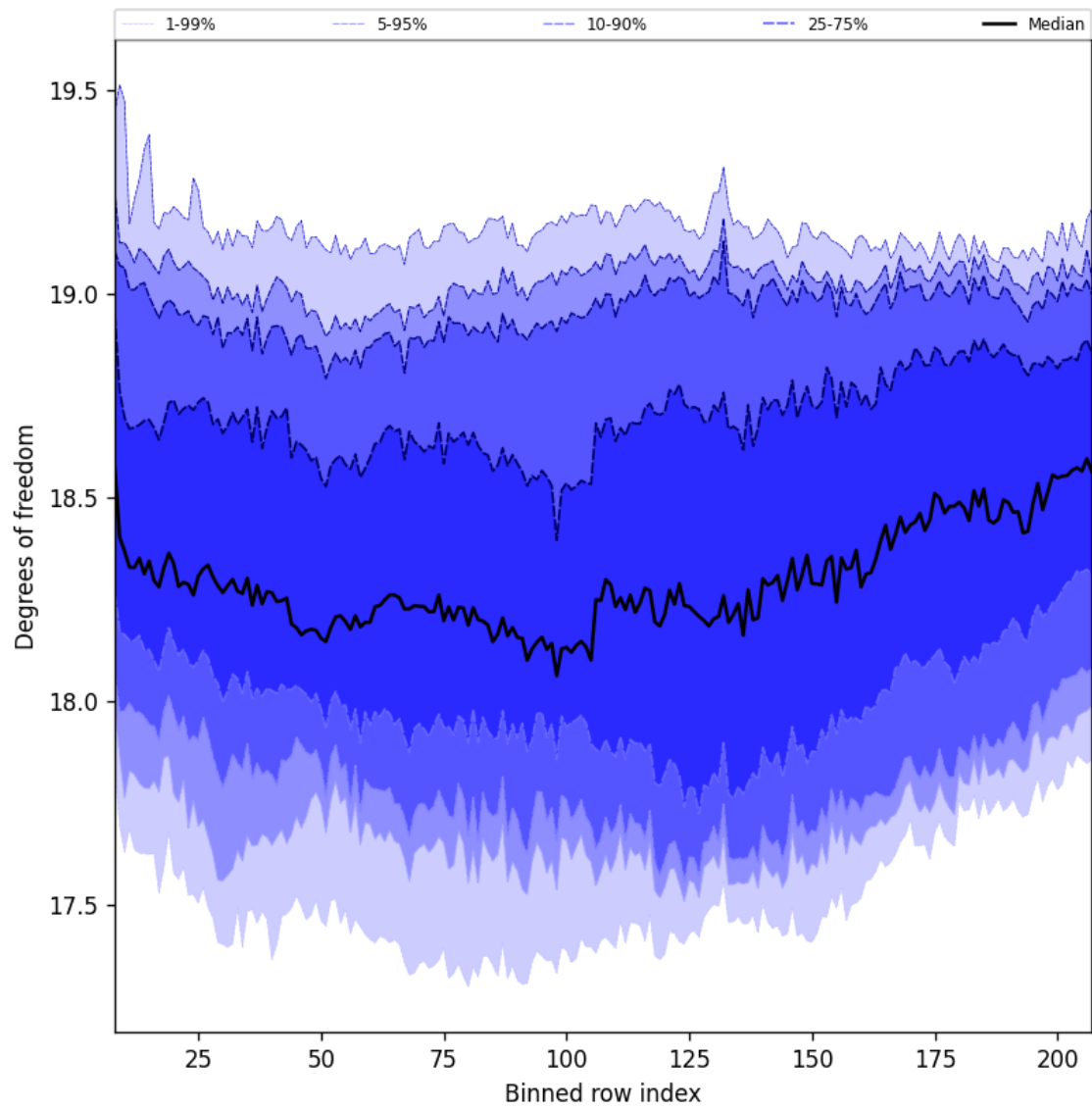
Figure 41: Along track statistics of “Degrees of freedom” for 2025-03-19 to 2025-03-21
