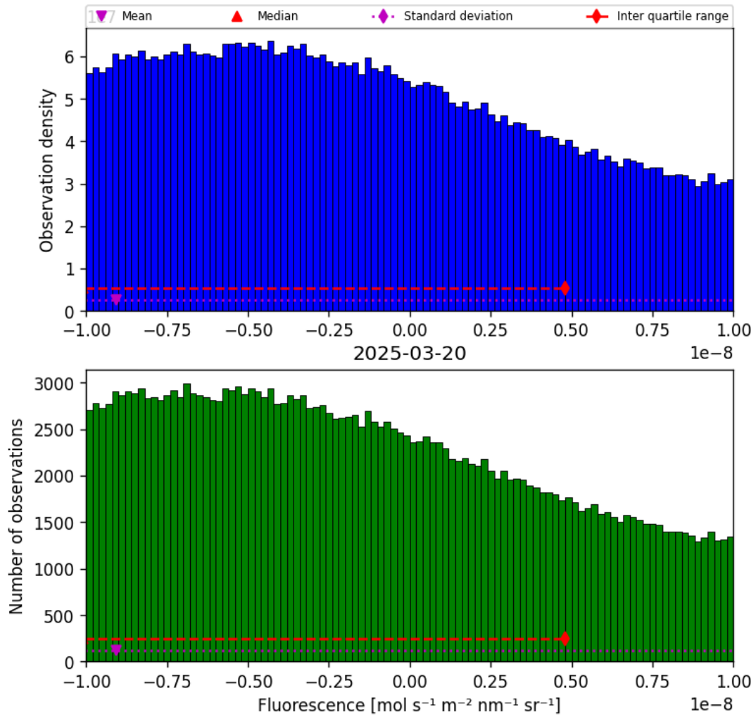
Figure 32: Histogram of “Fluorescence” for 2025-03-19 to 2025-03-21
