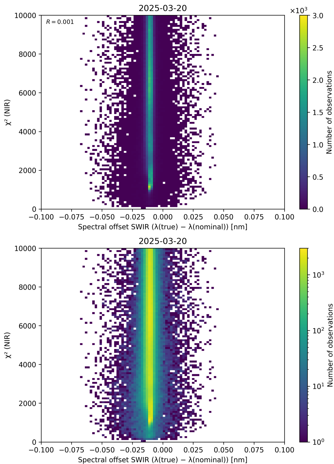
Figure 117: Scatter density plot of “Spectral offset SWIR ( \lambda_{\text{true}} - \lambda_{\text{nominal}} )” against “ \chi^2 (NIR)” for 2025-03-19 to 2025-03-21.
