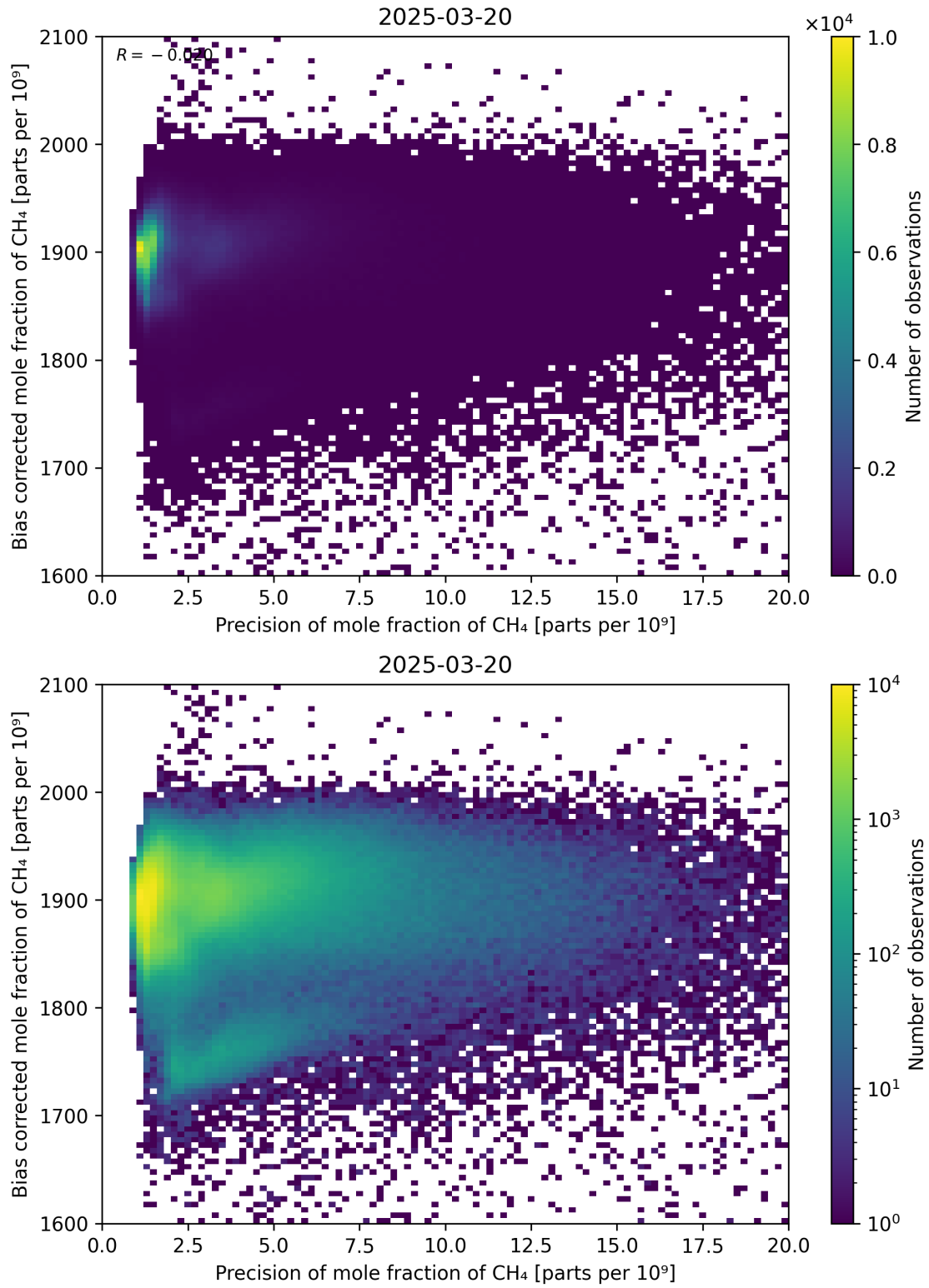
Figure 82: Scatter density plot of “Precision of mole fraction of CH 4 ” against “Bias corrected mole fraction of CH 4 ” for 2025-03-19 to 2025-03-21.
