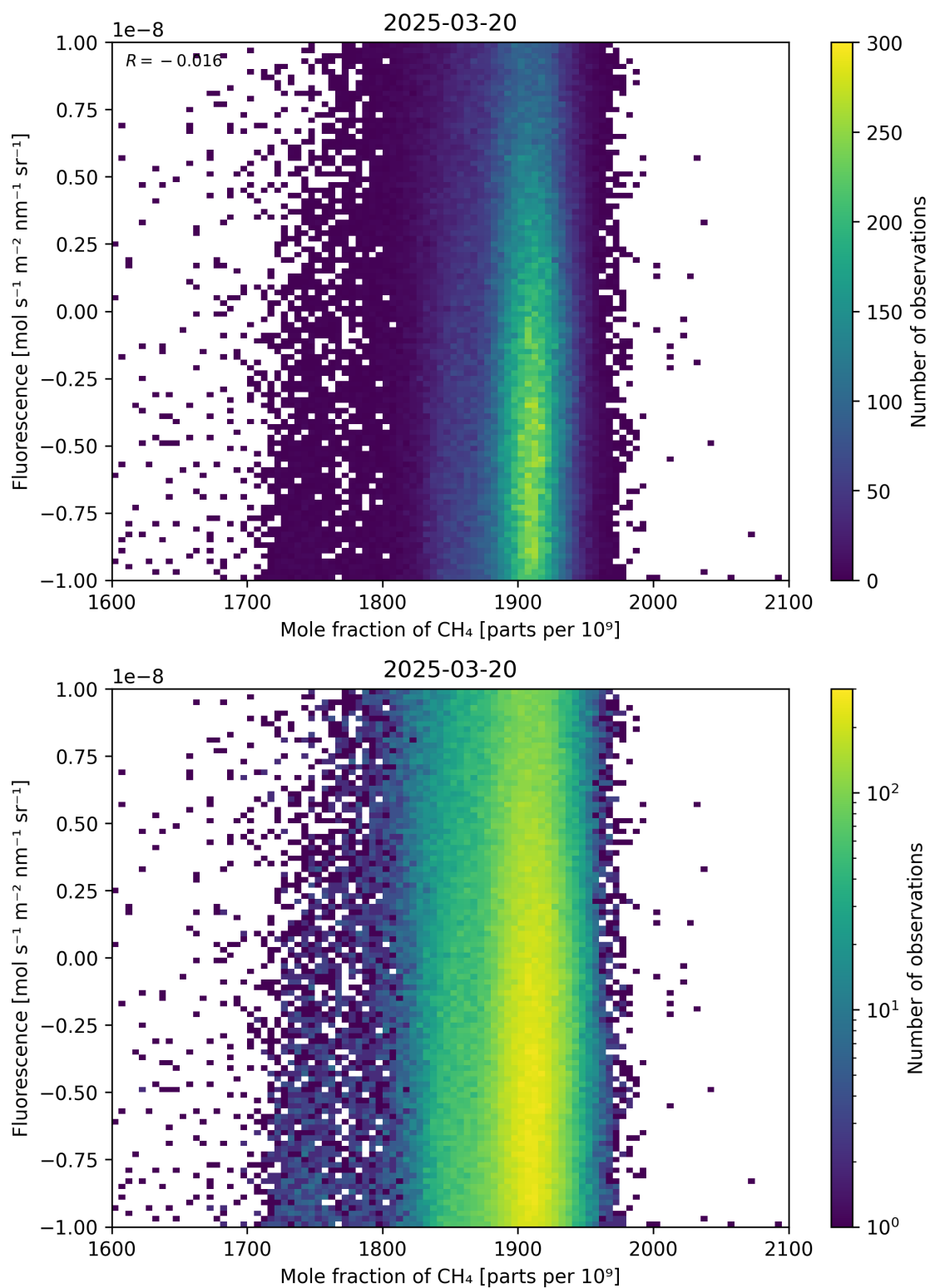
Figure 73: Scatter density plot of “Mole fraction of \text{CH}_4 ” against “Fluorescence” for 2025-03-19 to 2025-03-21.
