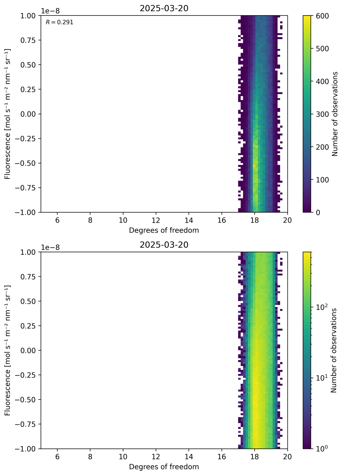
Figure 51: Scatter density plot of “Degrees of freedom” against “Fluorescence” for 2025-03-19 to 2025-03-21.
