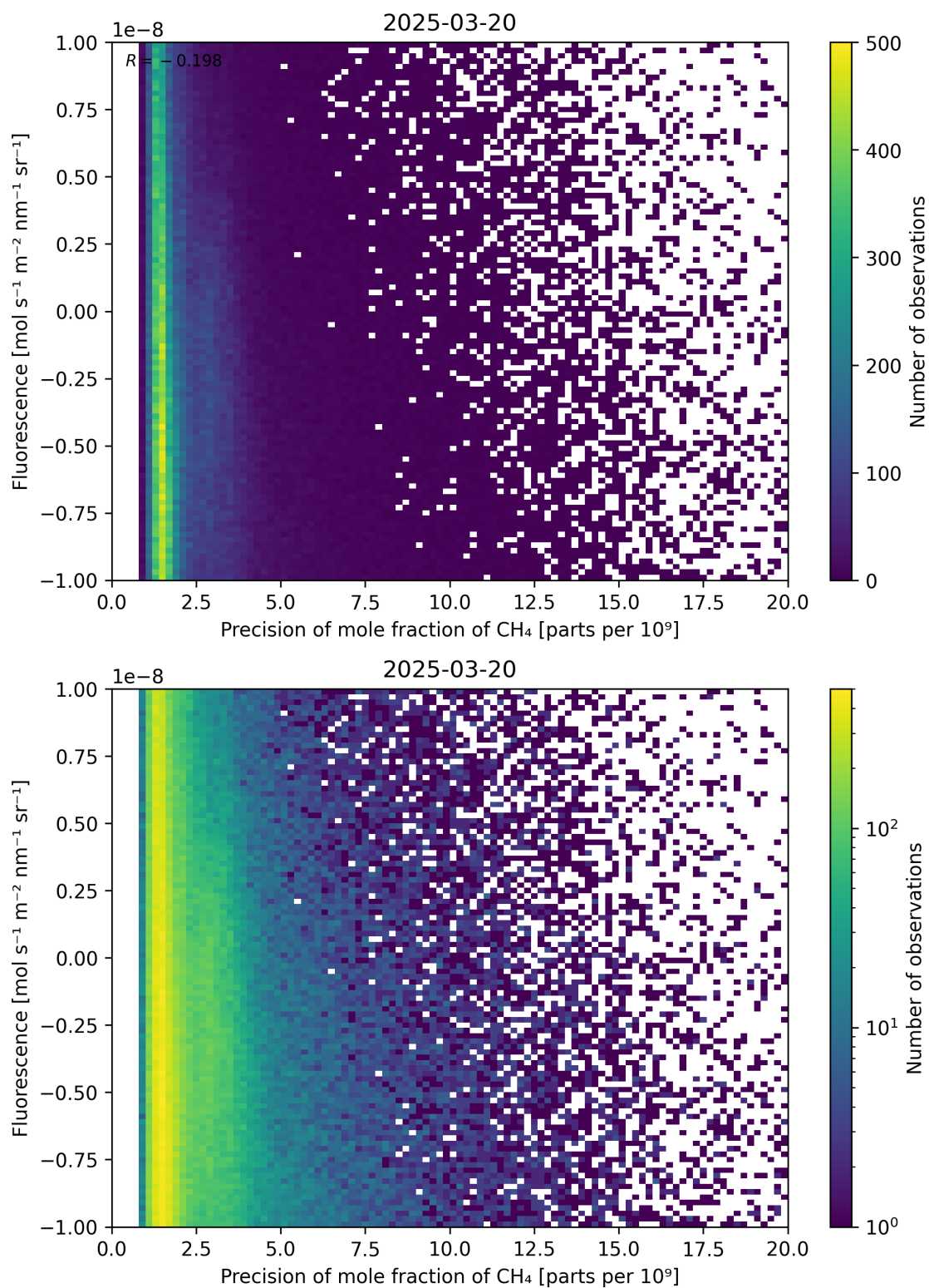
Figure 81: Scatter density plot of “Precision of mole fraction of \text{CH}_4 ” against “Fluorescence” for 2025-03-19 to 2025-03-21.
