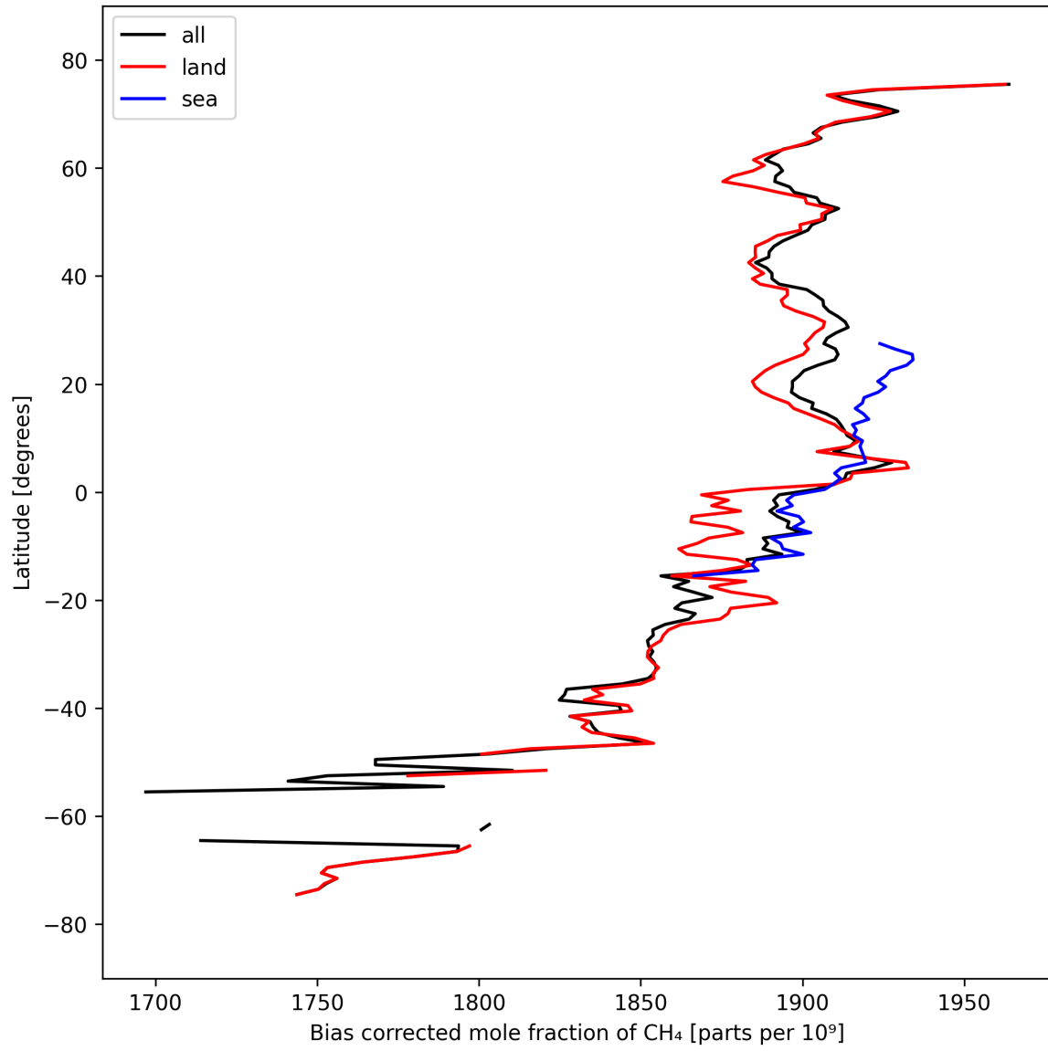
Figure 14: Zonal average of “Bias corrected mole fraction of CH 4 ” for 2025-03-19 to 2025-03-21.
