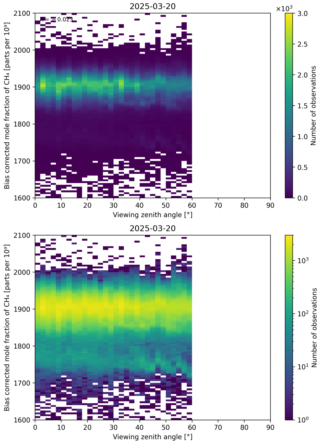
Figure 111: Scatter density plot of “Viewing zenith angle” against “Bias corrected mole fraction of CH 4 ” for 2025-03-19 to 2025-03-21.
