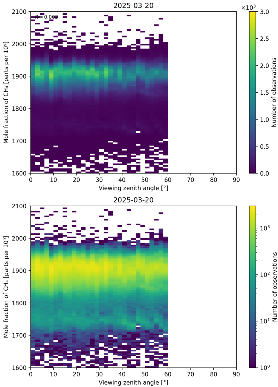
Figure 110: Scatter density plot of “Viewing zenith angle” against “Mole fraction of CH 4 ” for 2025-03-19 to 2025-03-21.
