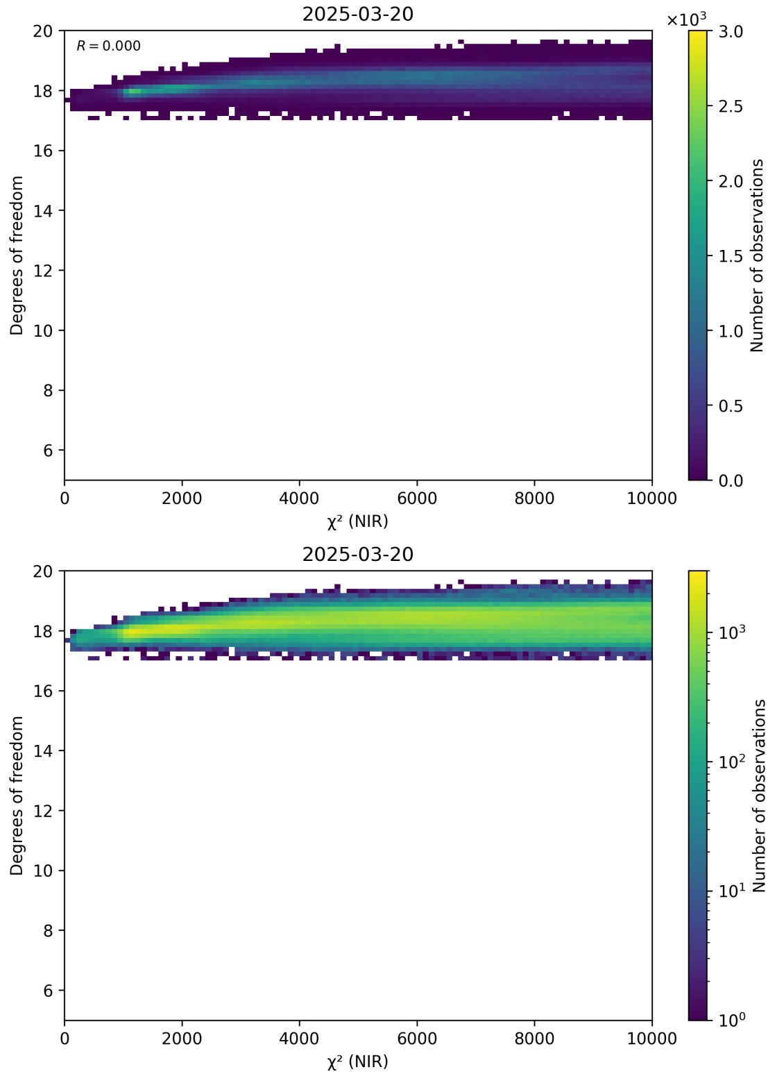
Figure 44: Scatter density plot of “ \chi^2 (NIR)” against “Degrees of freedom” for 2025-03-19 to 2025-03-21.
