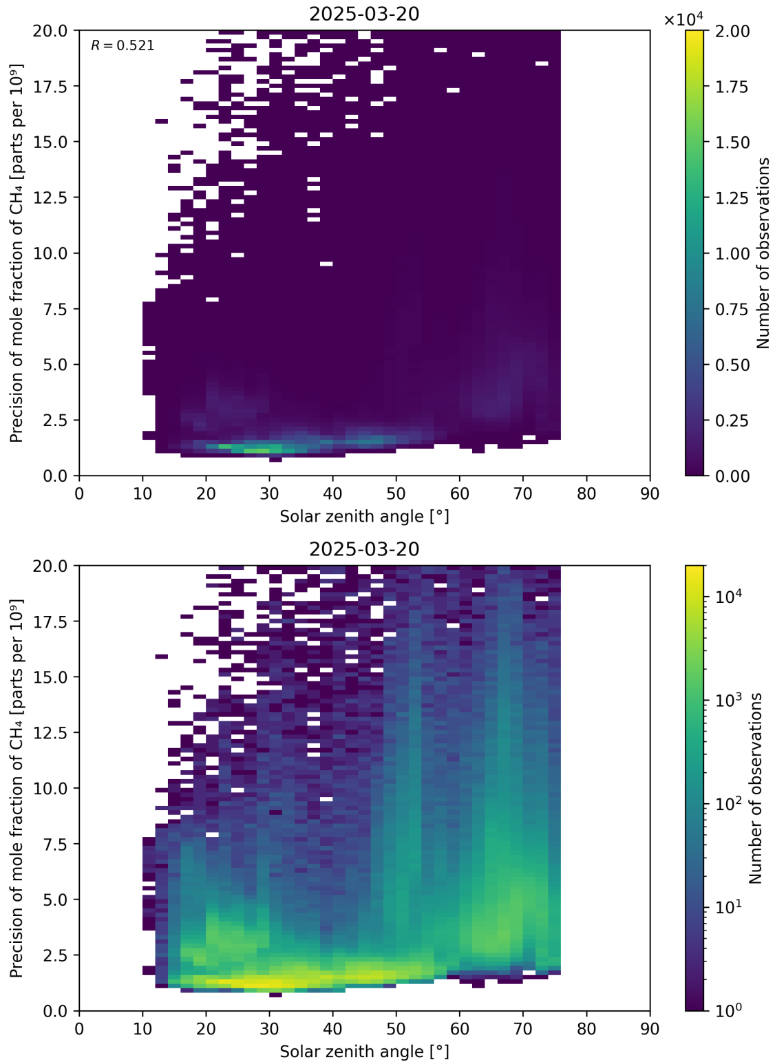
Figure 101: Scatter density plot of “Solar zenith angle” against “Precision of mole fraction of CH 4 ” for 2025-03-19 to 2025-03-21.
