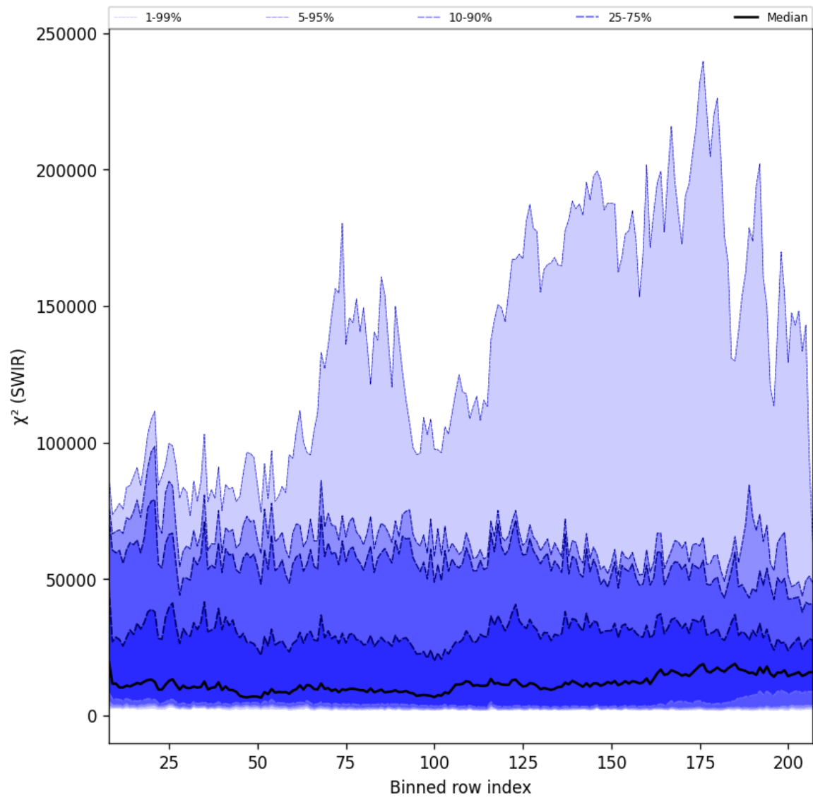
Figure 39: Along track statistics of “ \chi^2 (SWIR)” for 2025-03-19 to 2025-03-21
