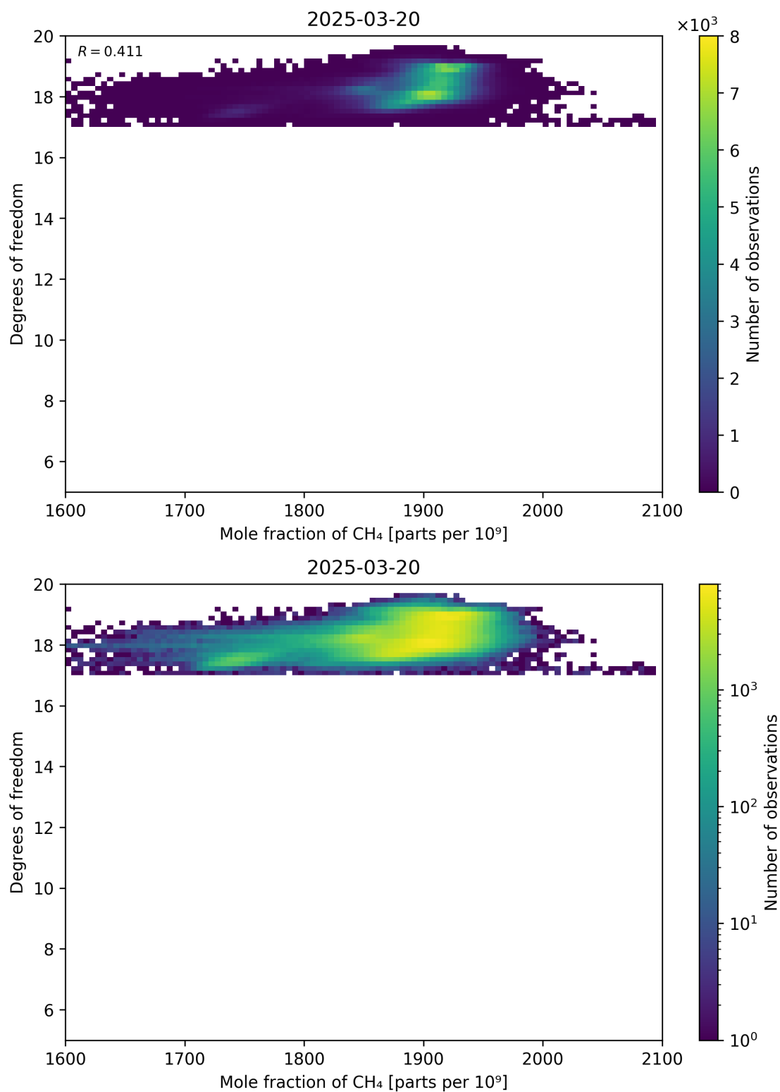
Figure 72: Scatter density plot of “Mole fraction of CH 4 ” against “Degrees of freedom” for 2025-03-19 to 2025-03-21.
