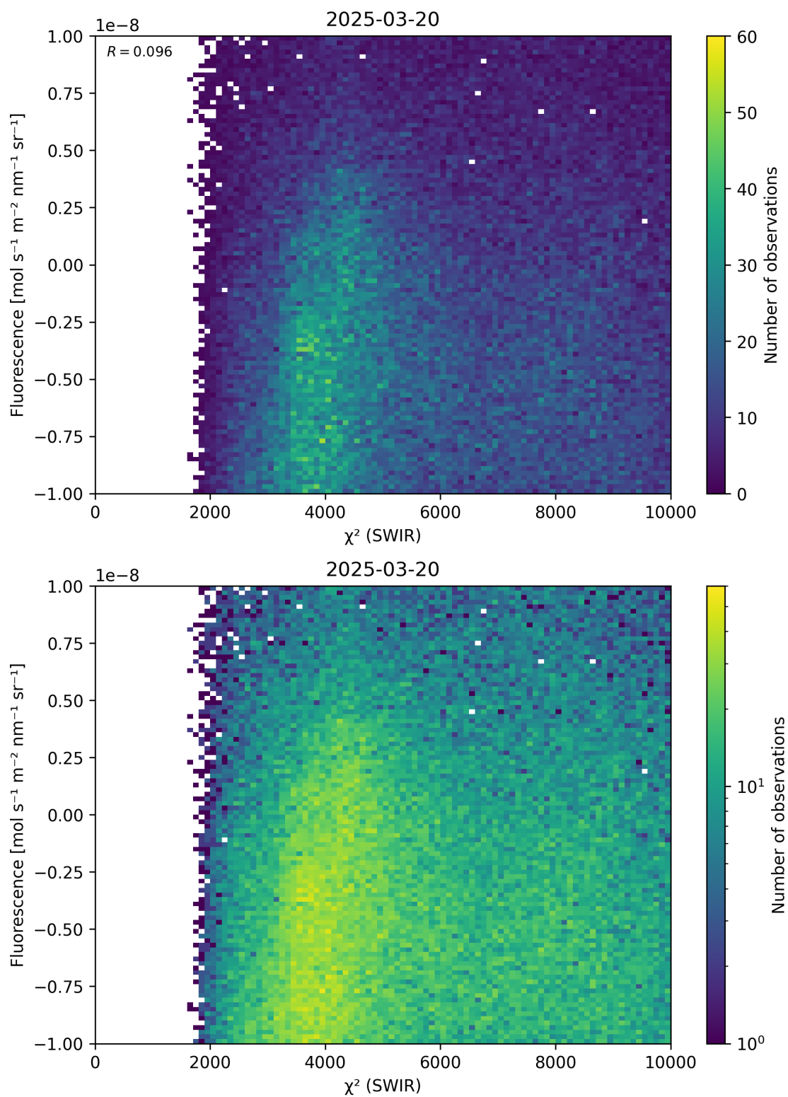
Figure 49: Scatter density plot of “ \chi^2 (SWIR)” against “Fluorescence” for 2025-03-19 to 2025-03-21.
