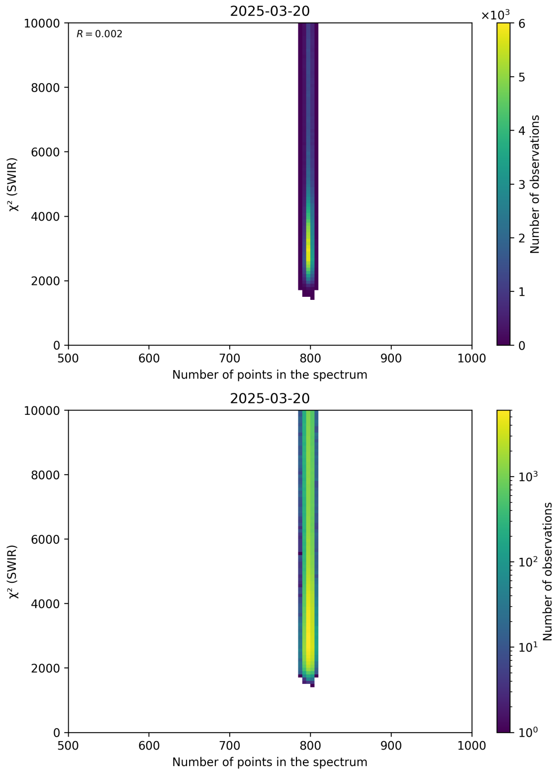
Figure 89: Scatter density plot of “Number of points in the spectrum” against “ \chi^2 (SWIR)” for 2025-03-19 to 2025-03-21.
