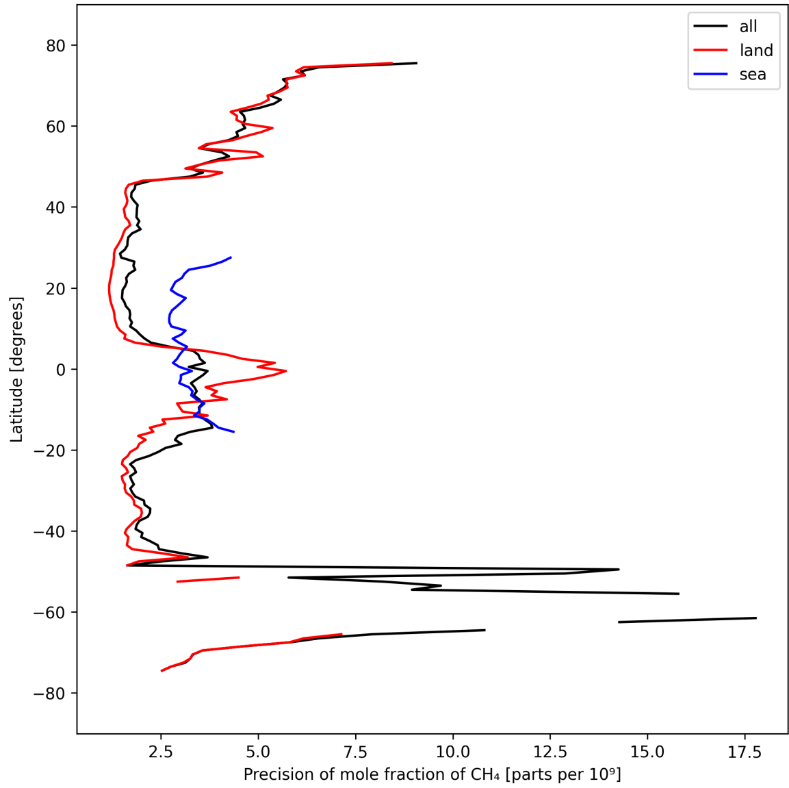
Figure 13: Zonal average of “Precision of mole fraction of CH 4 ” for 2025-03-19 to 2025-03-21.
