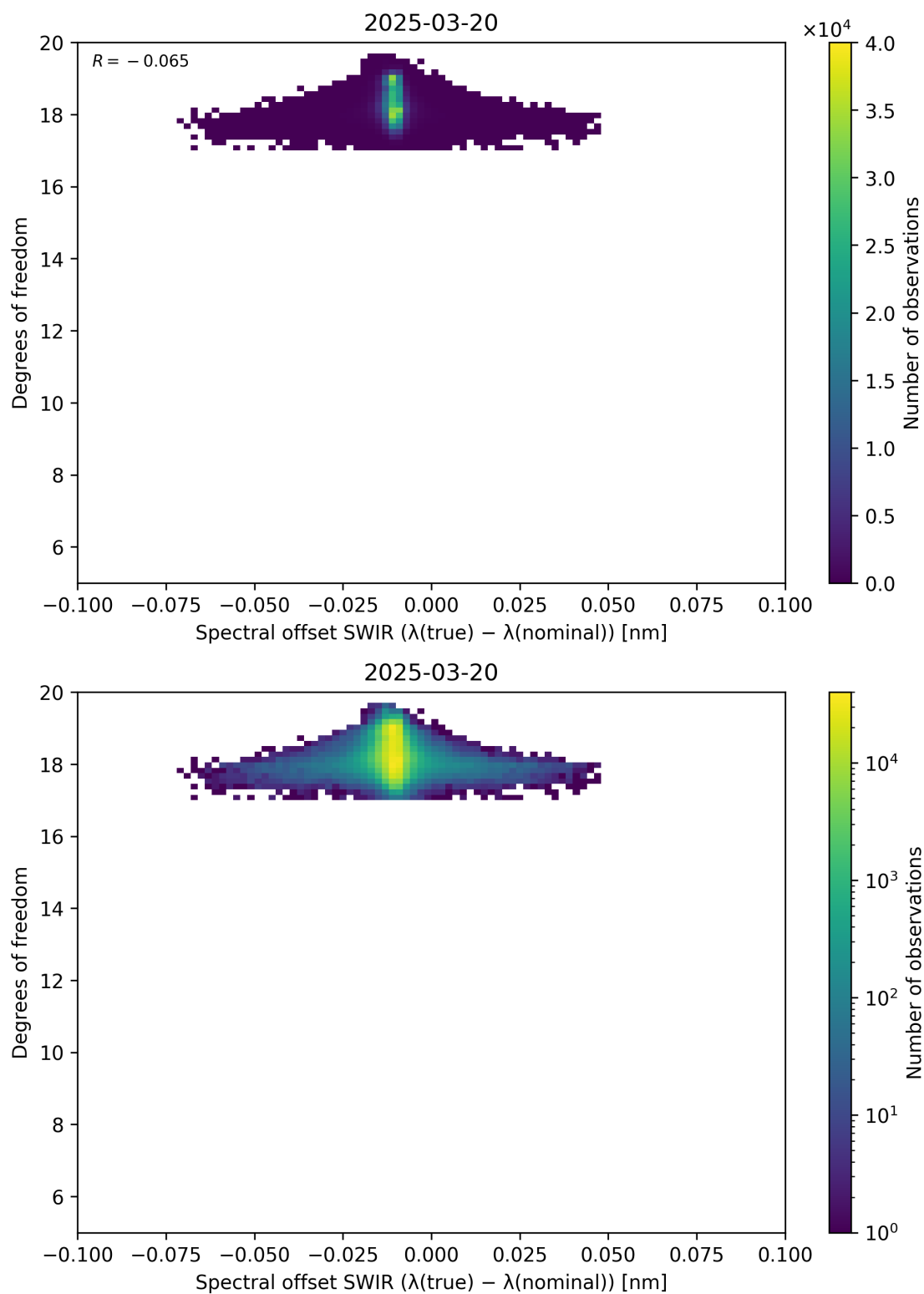
Figure 119: Scatter density plot of “Spectral offset SWIR ( \lambda_{\text{true}} - \lambda_{\text{nominal}} )” against “Degrees of freedom” for 2025-03-19 to 2025-03-21.
