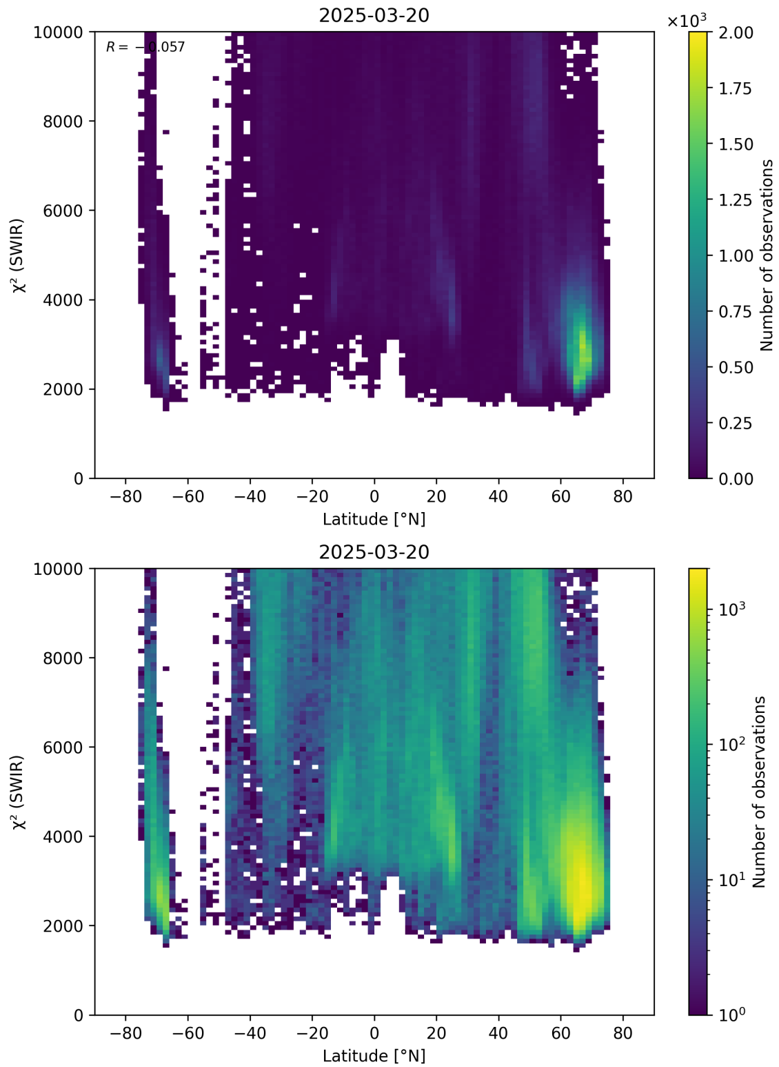
Figure 54: Scatter density plot of “Latitude” against “ \chi^2 (SWIR)” for 2025-03-19 to 2025-03-21.
