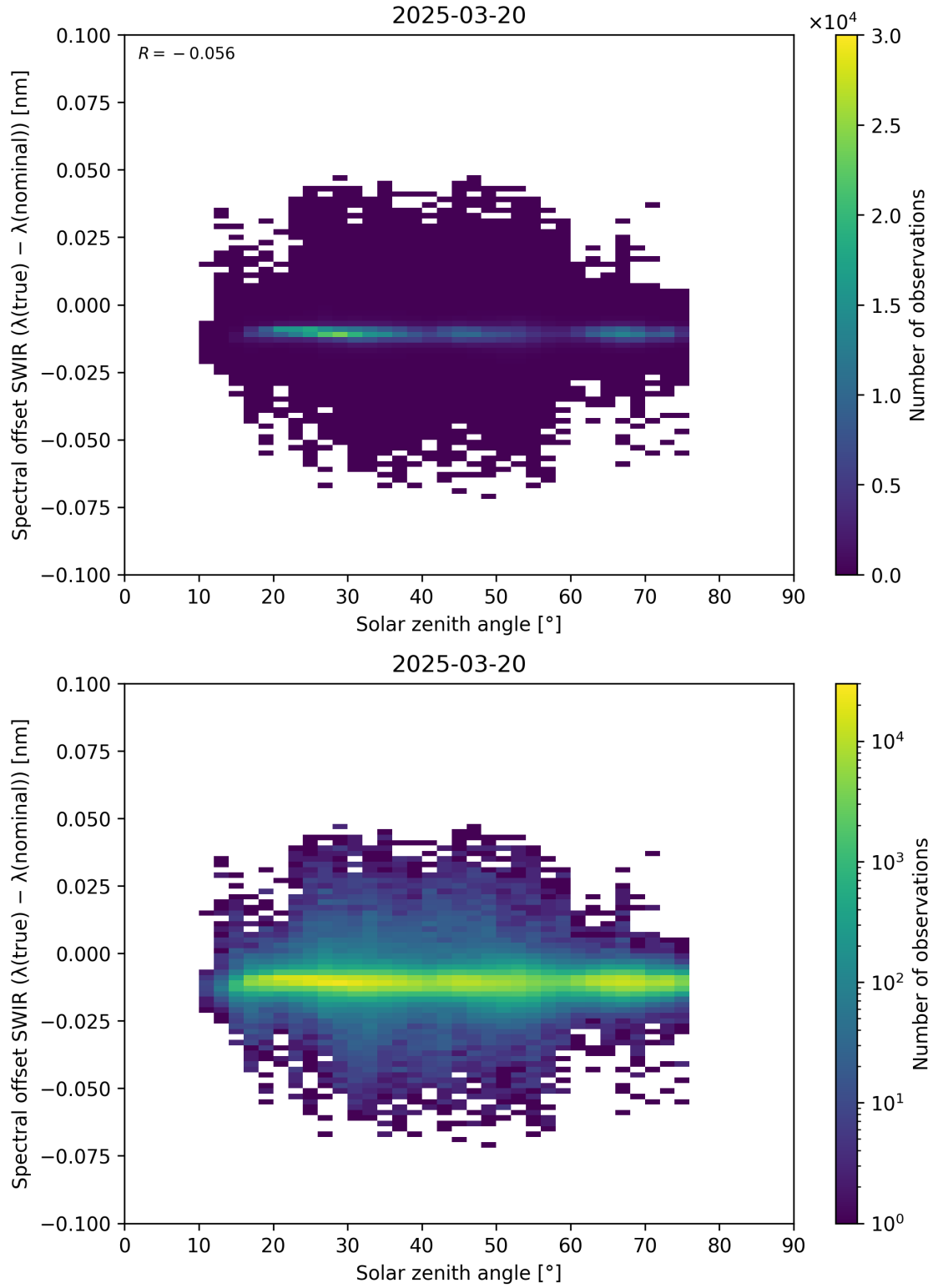
Figure 104: Scatter density plot of “Solar zenith angle” against “Spectral offset SWIR ( \lambda_{\text{true}} - \lambda_{\text{nominal}} )” for 2025-03-19 to 2025-03-21.
