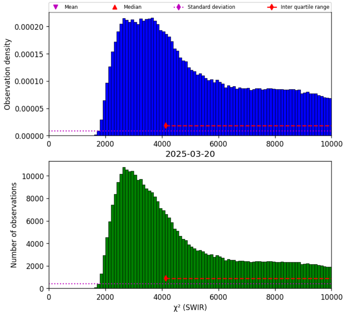
Figure 28: Histogram of “ \chi^2 (SWIR)” for 2025-03-19 to 2025-03-21
