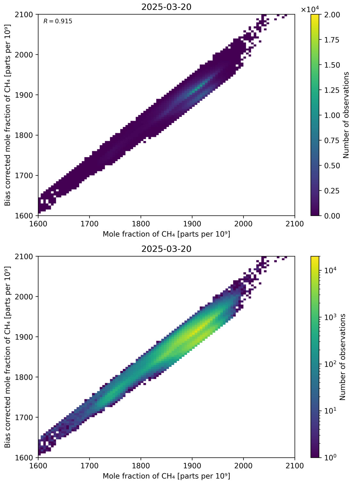
Figure 74: Scatter density plot of “Mole fraction of CH 4 ” against “Bias corrected mole fraction of CH 4 ” for 2025-03-19 to 2025-03-21.
