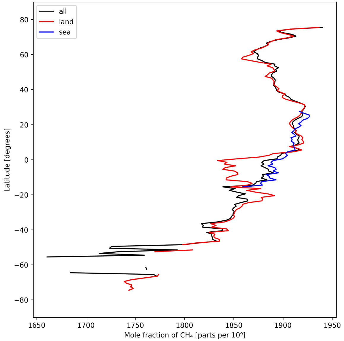
Figure 12: Zonal average of “Mole fraction of \text{CH}_4 ” for 2025-03-19 to 2025-03-21.
