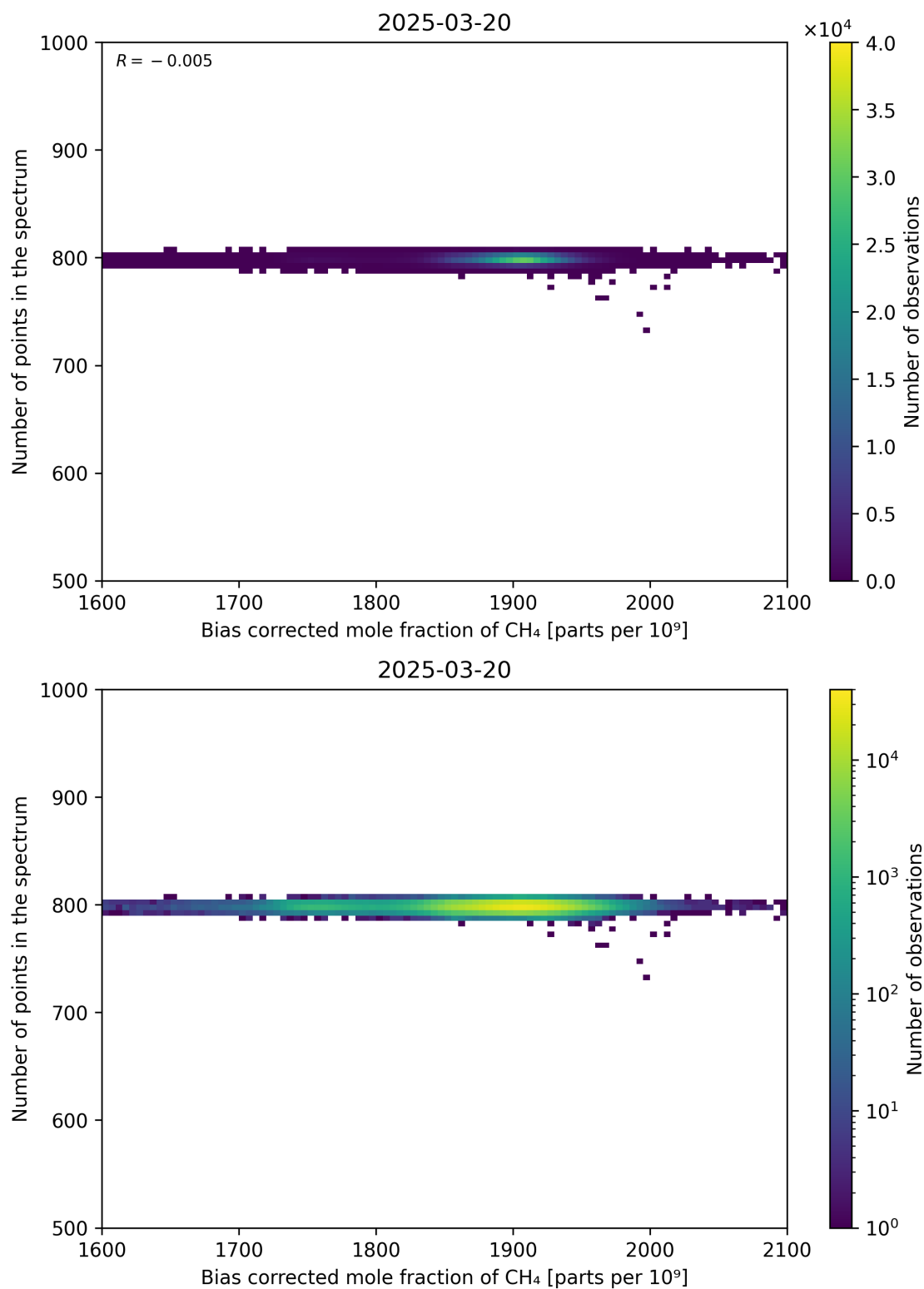
Figure 68: Scatter density plot of “Bias corrected mole fraction of CH 4 ” against “Number of points in the spectrum” for 2025-03-19 to 2025-03-21.
