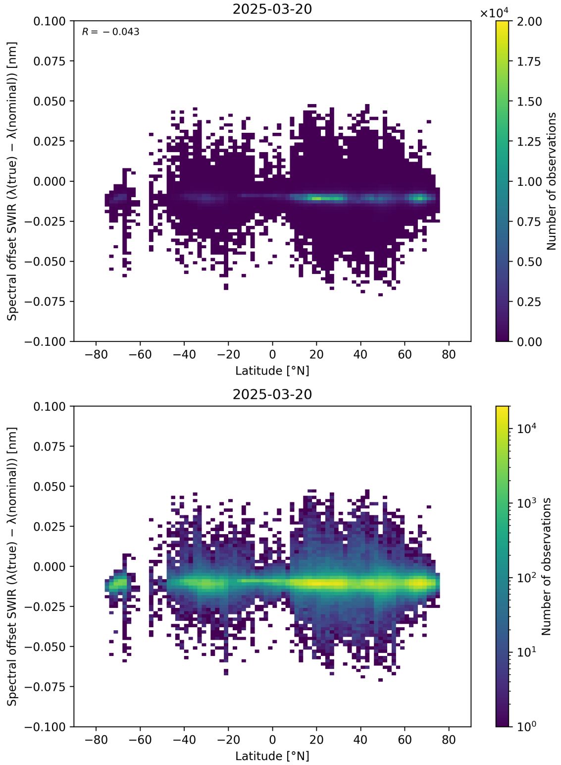
Figure 62: Scatter density plot of “Latitude” against “Spectral offset SWIR ( \lambda_{\text{true}} - \lambda_{\text{nominal}} )” for 2025-03-19 to 2025-03-21.
