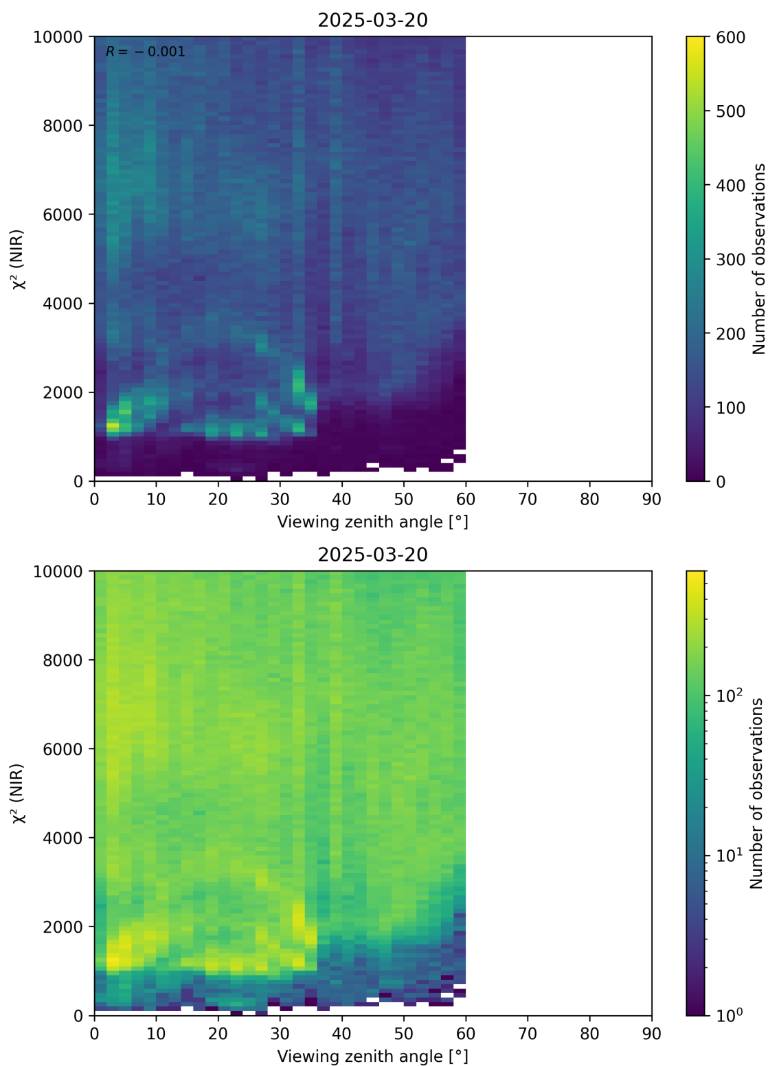
Figure 105: Scatter density plot of “Viewing zenith angle” against “ \chi^2 (NIR)” for 2025-03-19 to 2025-03-21.
