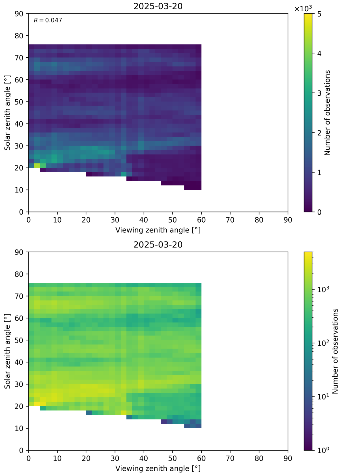
Figure 115: Scatter density plot of “Viewing zenith angle” against “Solar zenith angle” for 2025-03-19 to 2025-03-21.
