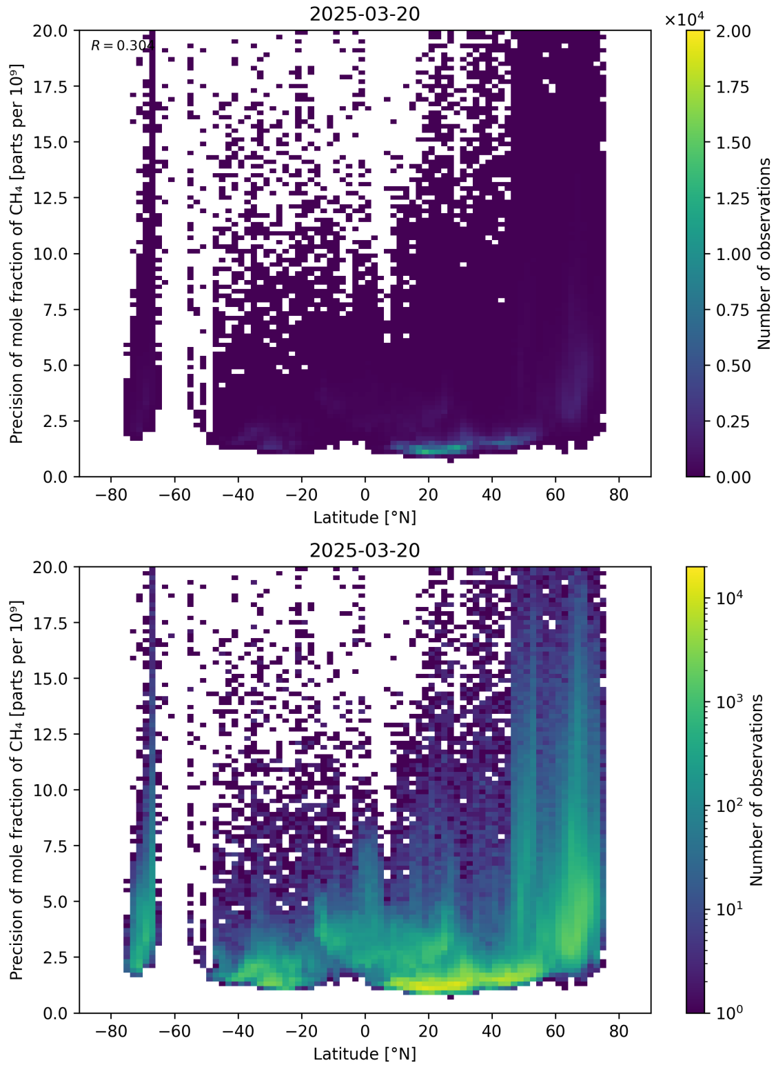
Figure 59: Scatter density plot of “Latitude” against “Precision of mole fraction of \text{CH}_4 ” for 2025-03-19 to 2025-03-21.
