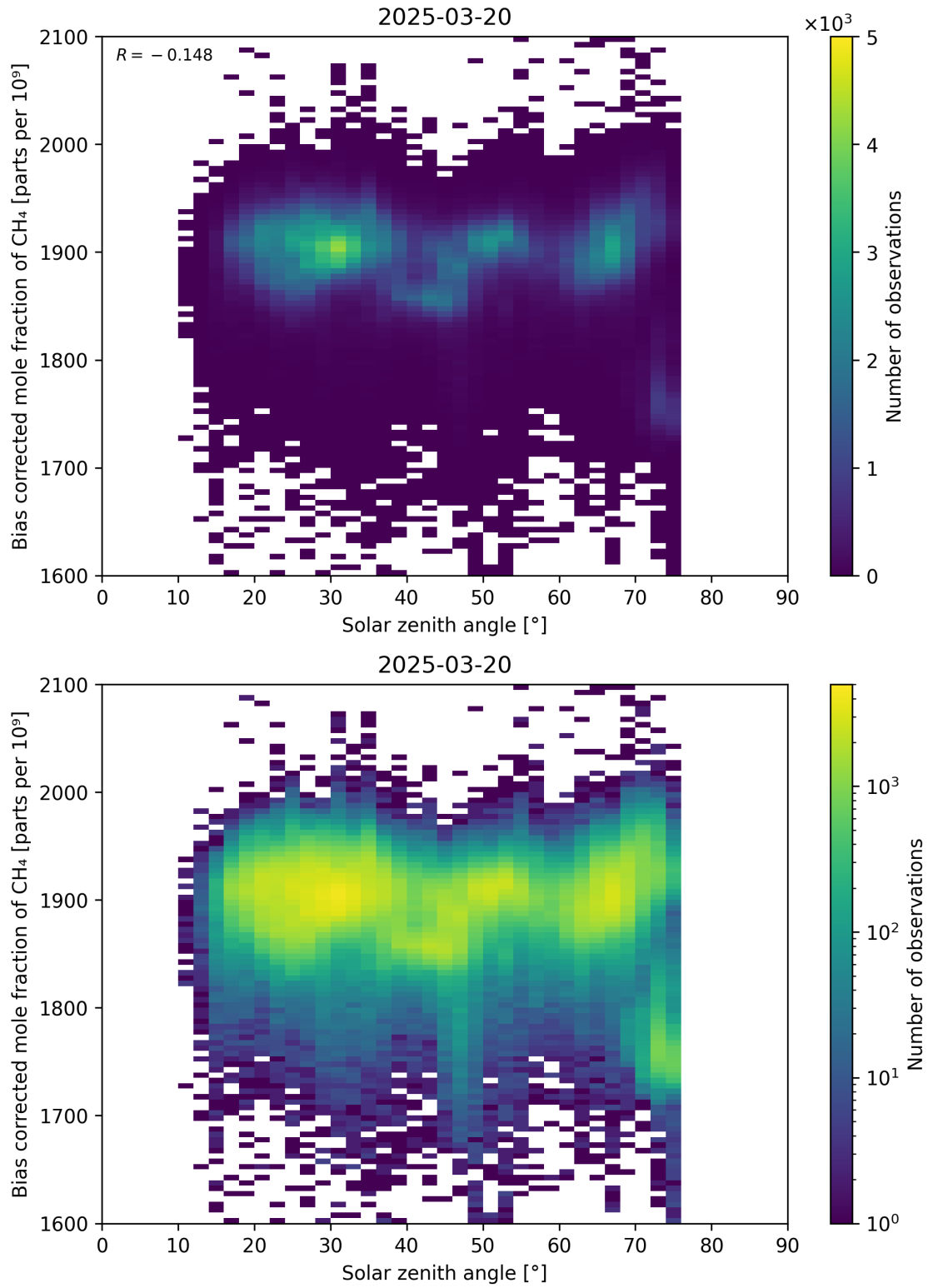
Figure 100: Scatter density plot of “Solar zenith angle” against “Bias corrected mole fraction of CH 4 ” for 2025-03-19 to 2025-03-21.
