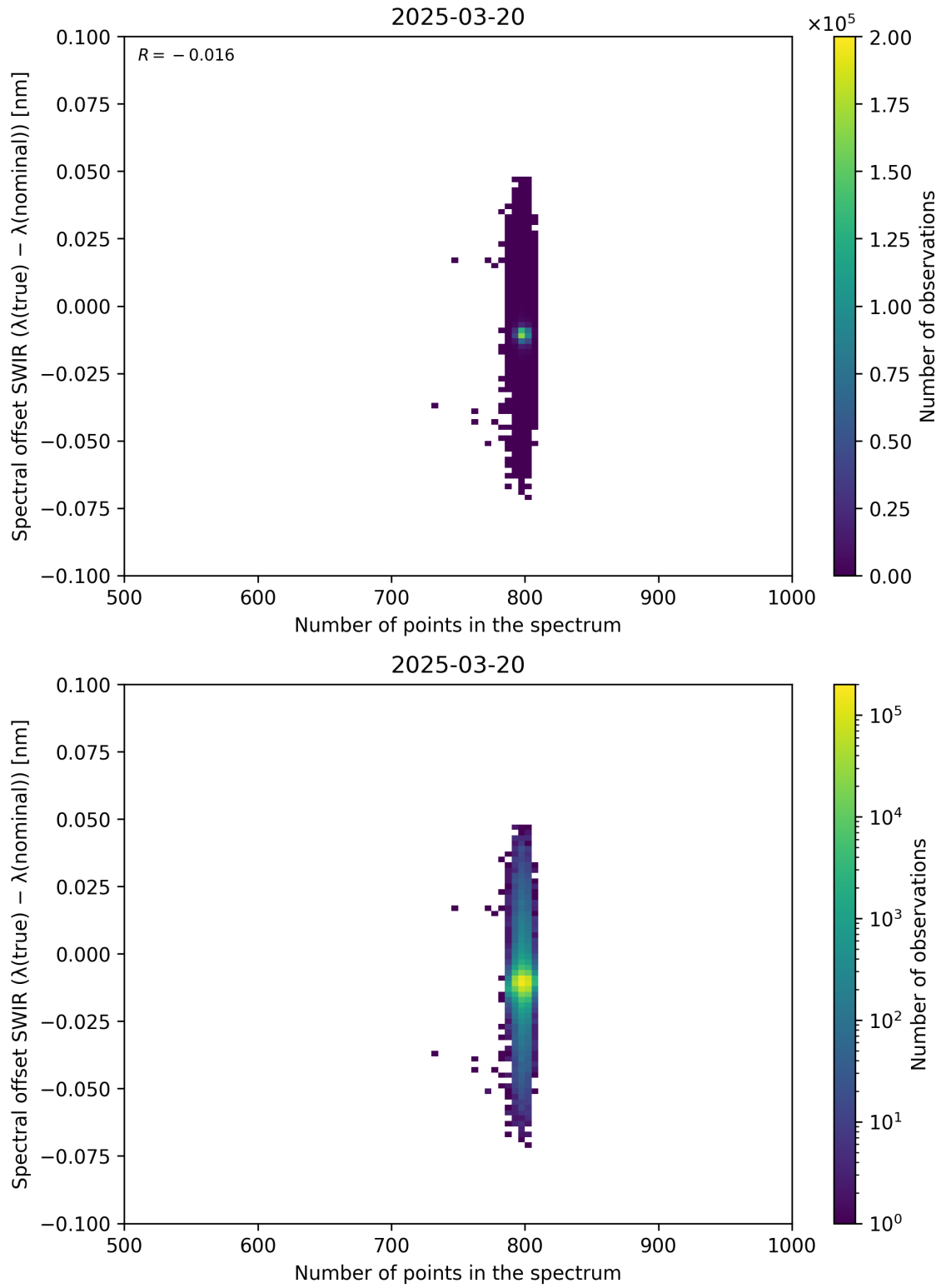
Figure 93: Scatter density plot of “Number of points in the spectrum” against “Spectral offset SWIR ( \lambda_{\text{true}} - \lambda_{\text{nominal}} )” for 2025-03-19 to 2025-03-21.
