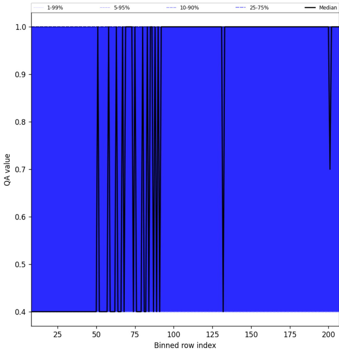
Figure 33: Along track statistics of “QA value” for 2025-03-19 to 2025-03-21
