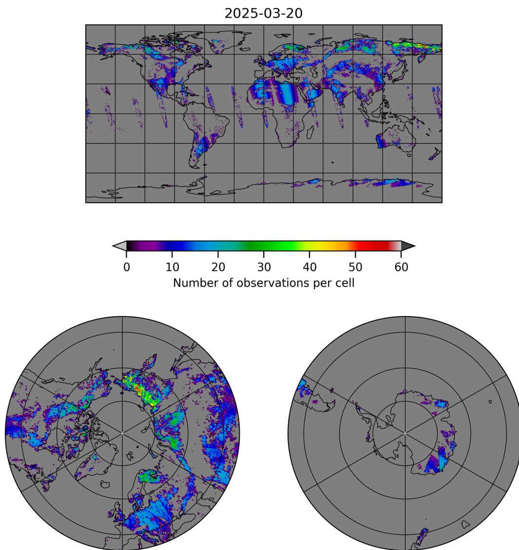
Figure 10: Map of the number of observations for 2025-03-19 to 2025-03-21
