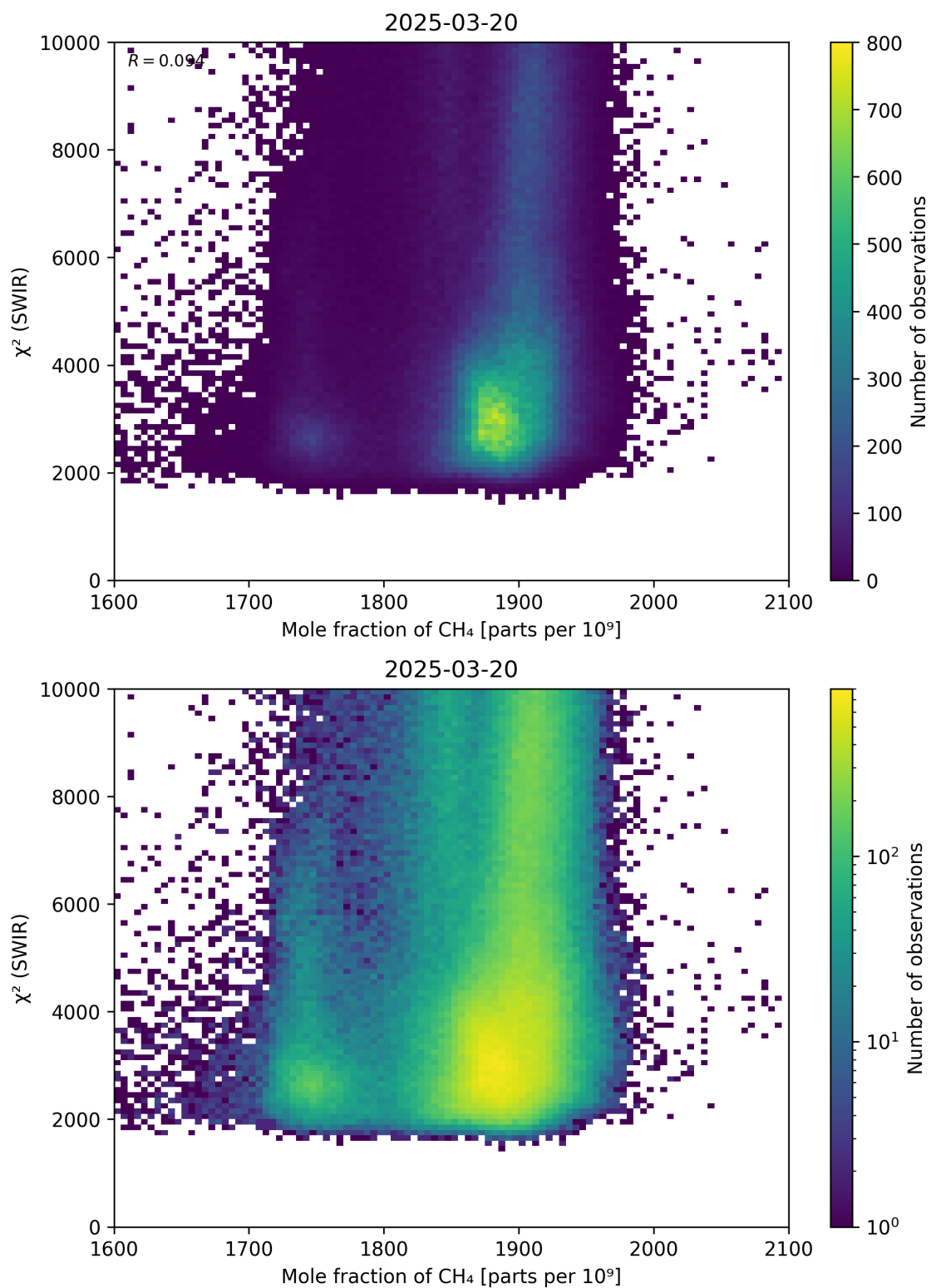
Figure 71: Scatter density plot of “Mole fraction of \text{CH}_4 ” against “ \chi^2 (SWIR)” for 2025-03-19 to 2025-03-21.
