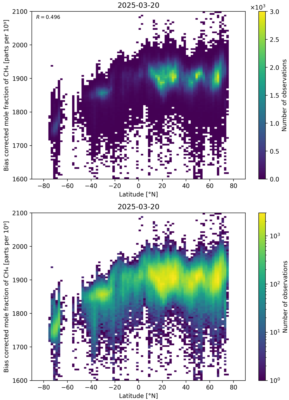
Figure 58: Scatter density plot of “Latitude” against “Bias corrected mole fraction of \text{CH}_4 ” for 2025-03-19 to 2025-03-21.
