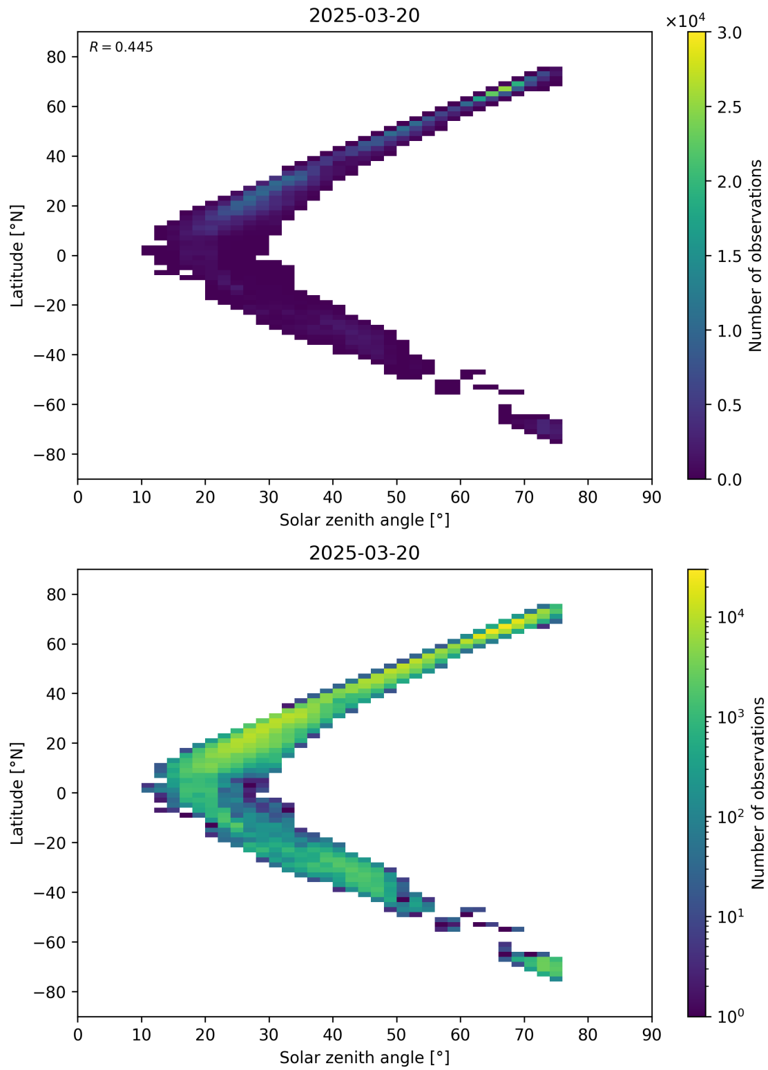
Figure 98: Scatter density plot of “Solar zenith angle” against “Latitude” for 2025-03-19 to 2025-03-21.
