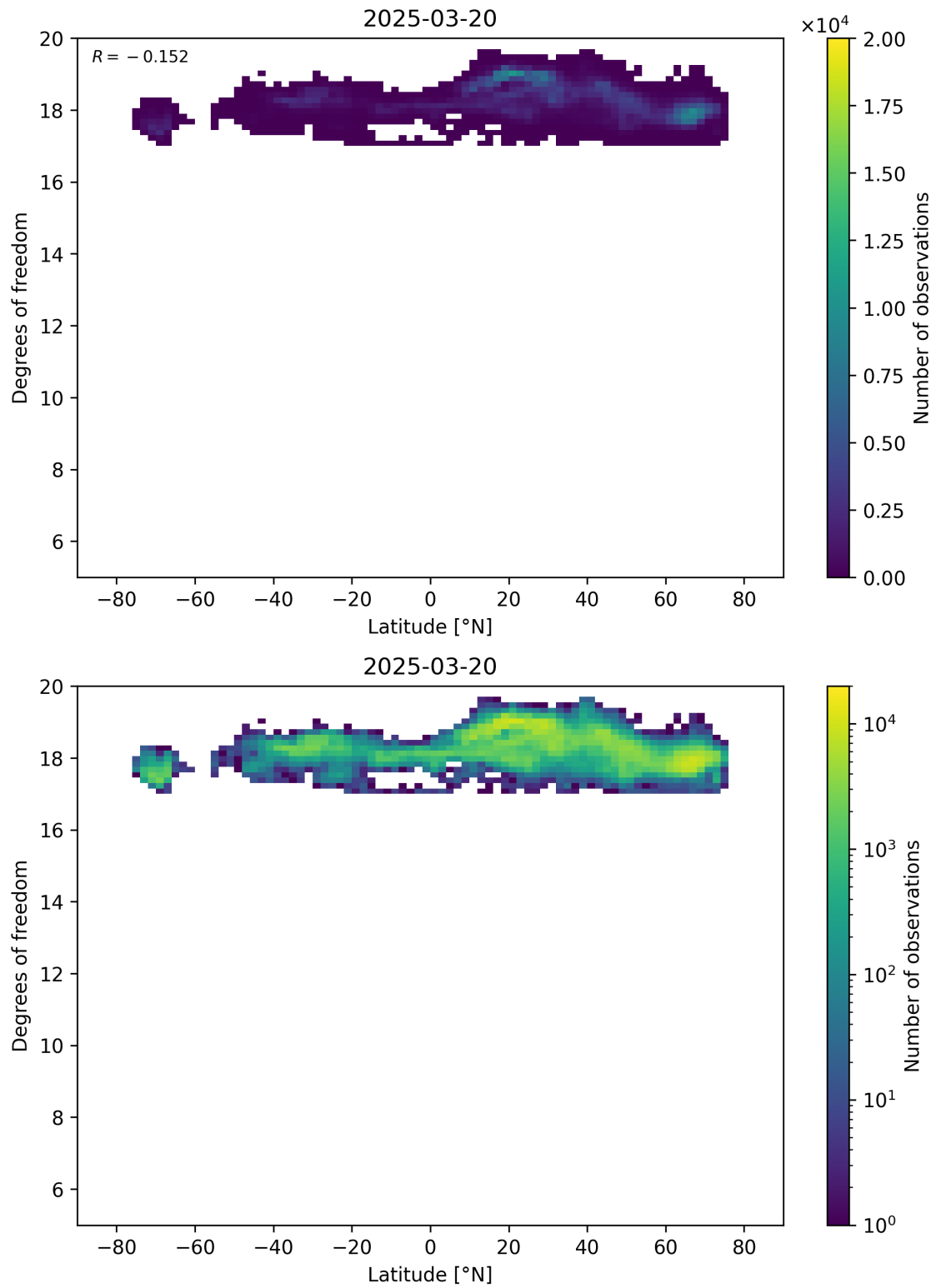
Figure 55: Scatter density plot of “Latitude” against “Degrees of freedom” for 2025-03-19 to 2025-03-21.
