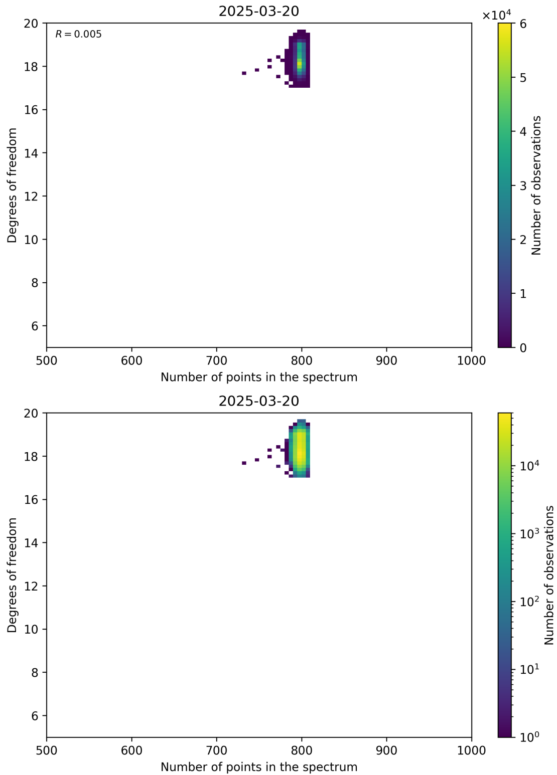
Figure 90: Scatter density plot of “Number of points in the spectrum” against “Degrees of freedom” for 2025-03-19 to 2025-03-21.
