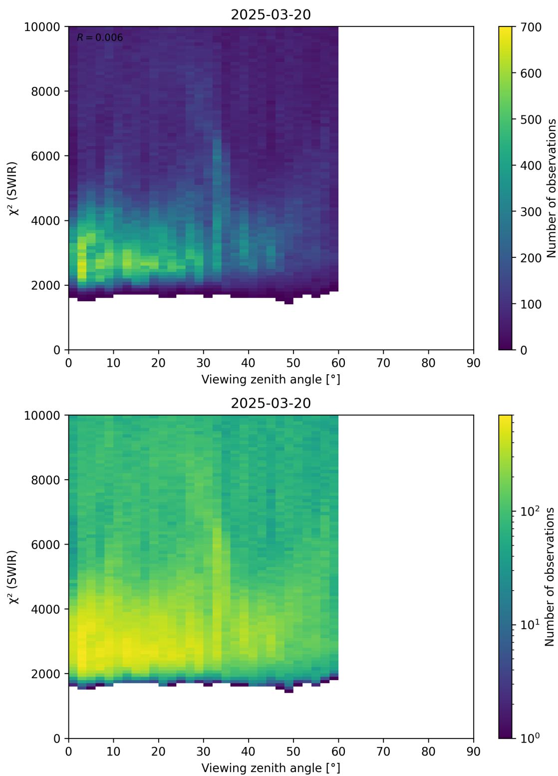
Figure 106: Scatter density plot of “Viewing zenith angle” against “ \chi^2 (SWIR)” for 2025-03-19 to 2025-03-21.
