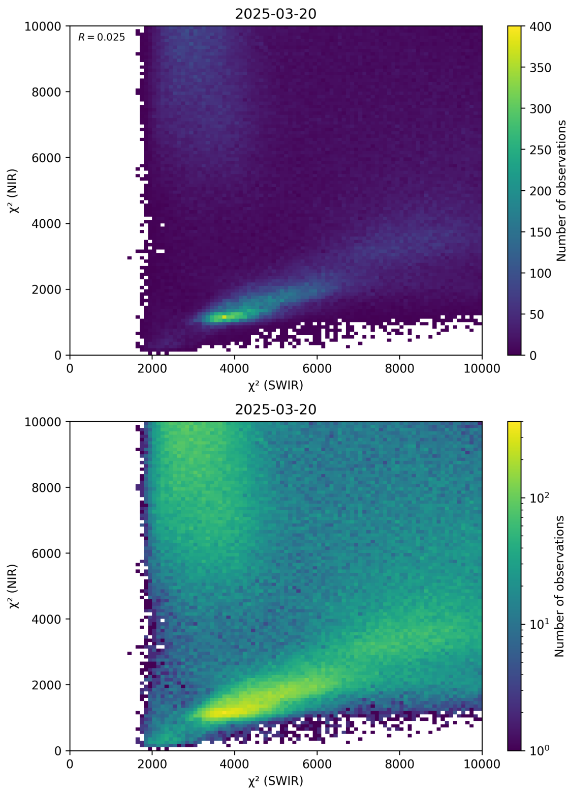
Figure 47: Scatter density plot of “ \chi^2 (SWIR)” against “ \chi^2 (NIR)” for 2025-03-19 to 2025-03-21.
