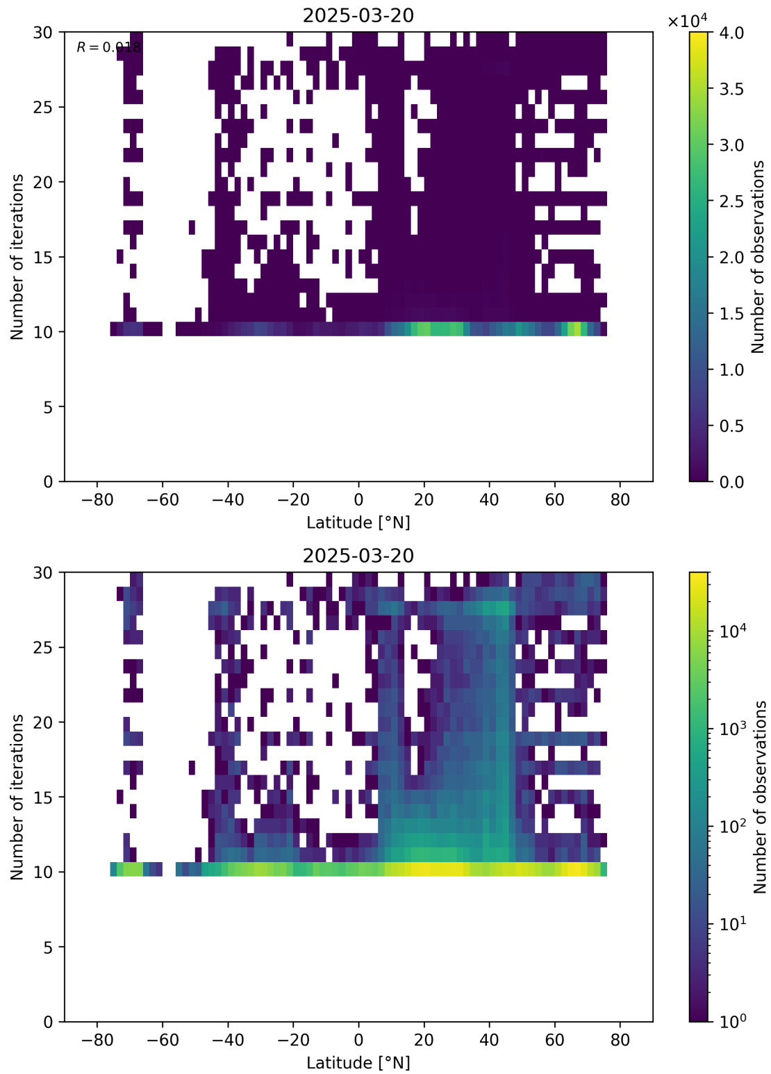
Figure 60: Scatter density plot of “Latitude” against “Number of iterations” for 2025-03-19 to 2025-03-21.
