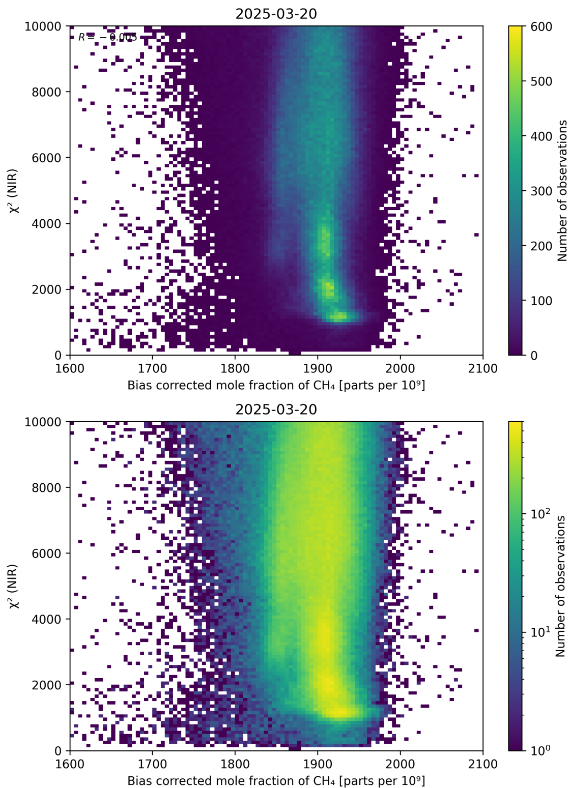
Figure 63: Scatter density plot of “Bias corrected mole fraction of \text{CH}_4 ” against “ \chi^2 (NIR)” for 2025-03-19 to 2025-03-21.
