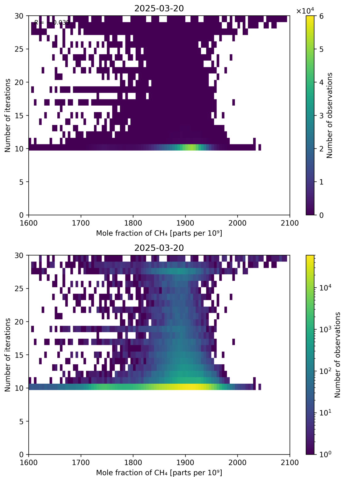
Figure 76: Scatter density plot of “Mole fraction of CH 4 ” against “Number of iterations” for 2025-03-19 to 2025-03-21.
