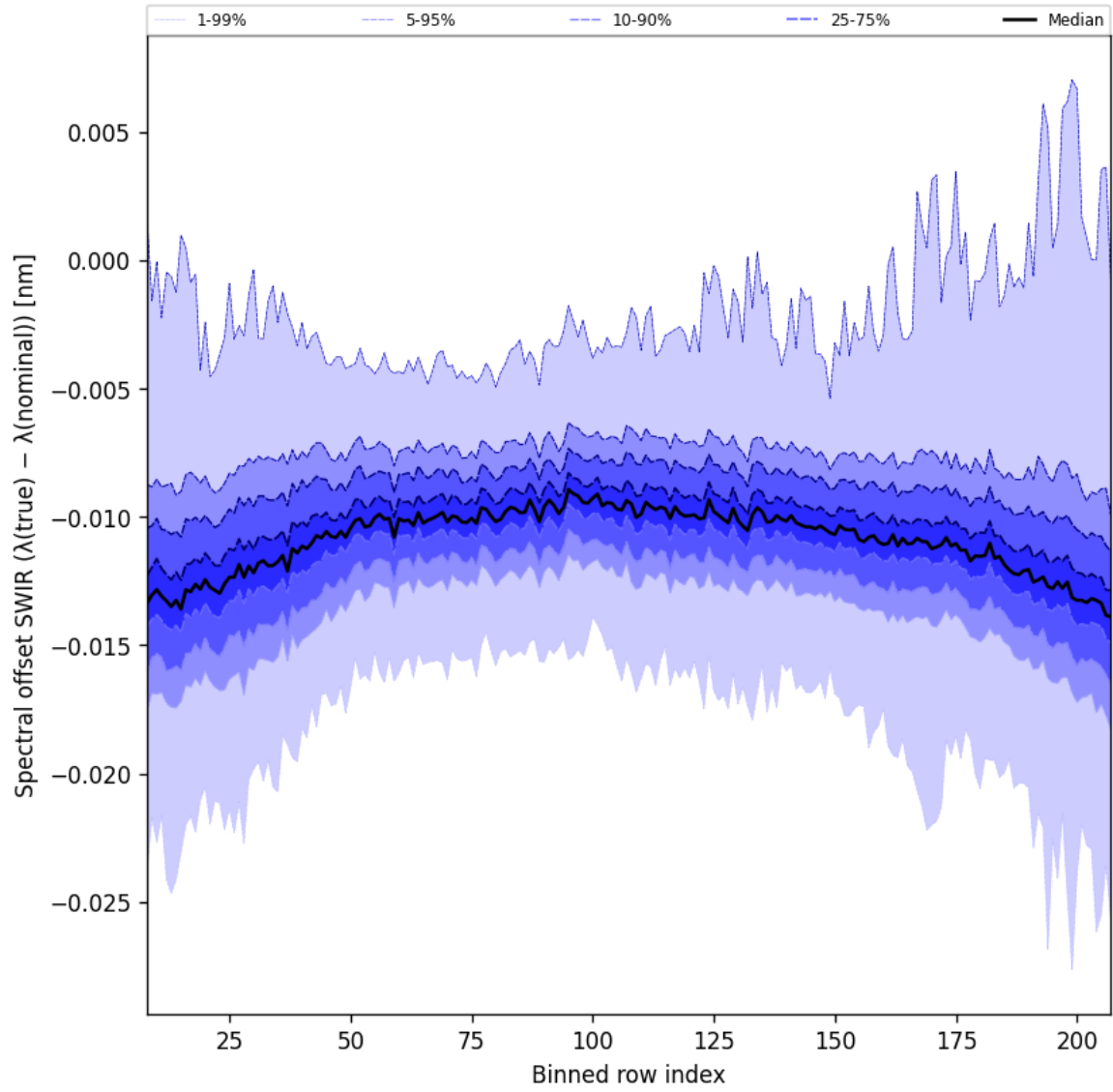
Figure 38: Along track statistics of “Spectral offset SWIR ( \lambda_{\text{true}} - \lambda_{\text{nominal}} )” for 2025-03-19 to 2025-03-21
