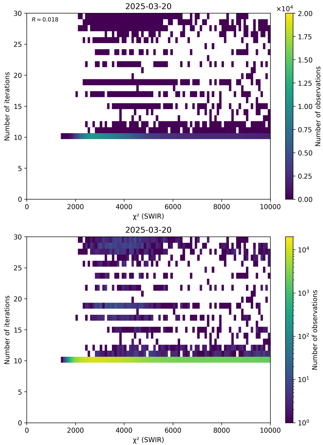
Figure 50: Scatter density plot of “ \chi^2 (SWIR)” against “Number of iterations” for 2025-03-19 to 2025-03-21.
