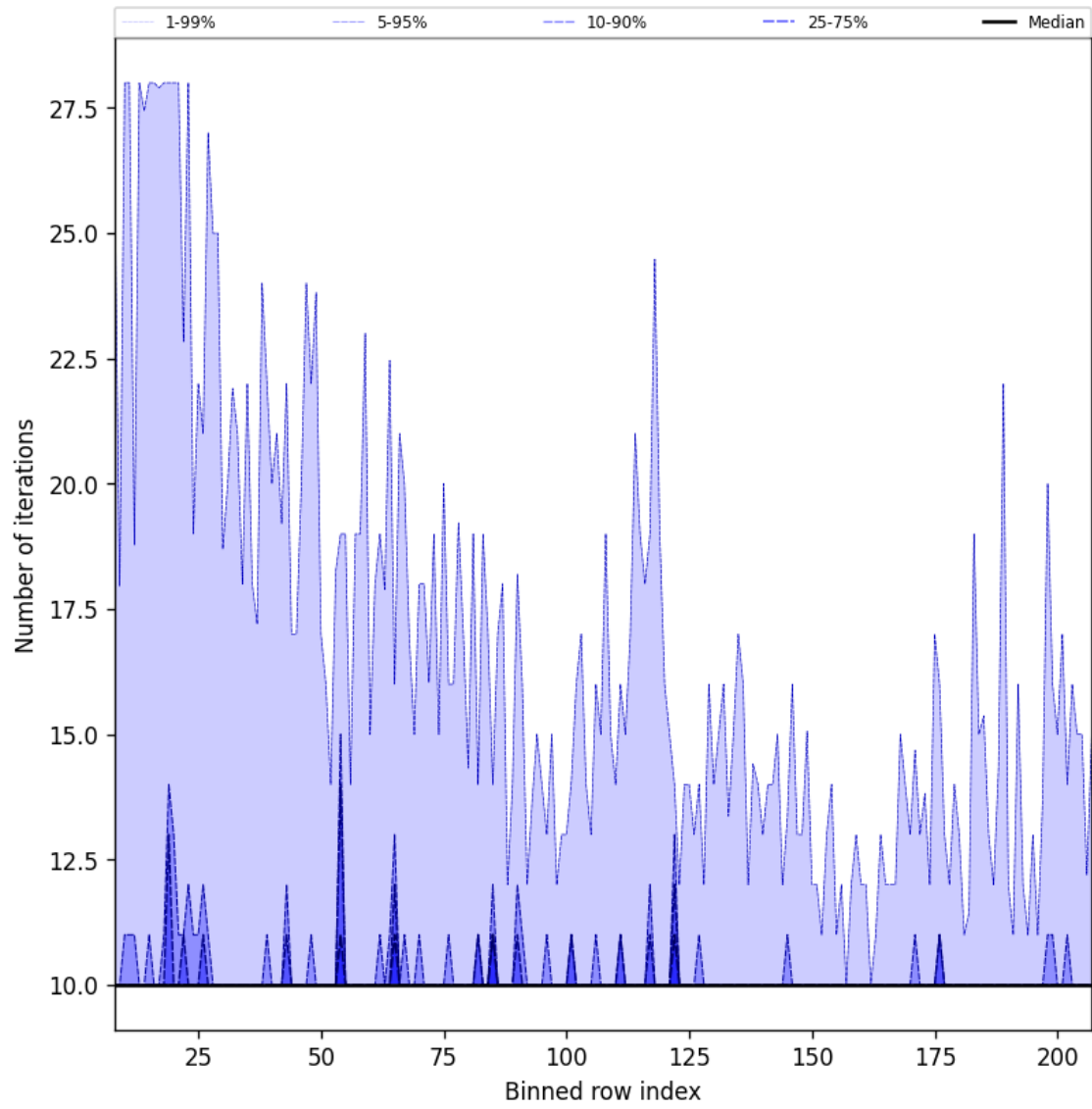
Figure 42: Along track statistics of “Number of iterations” for 2025-03-19 to 2025-03-21
