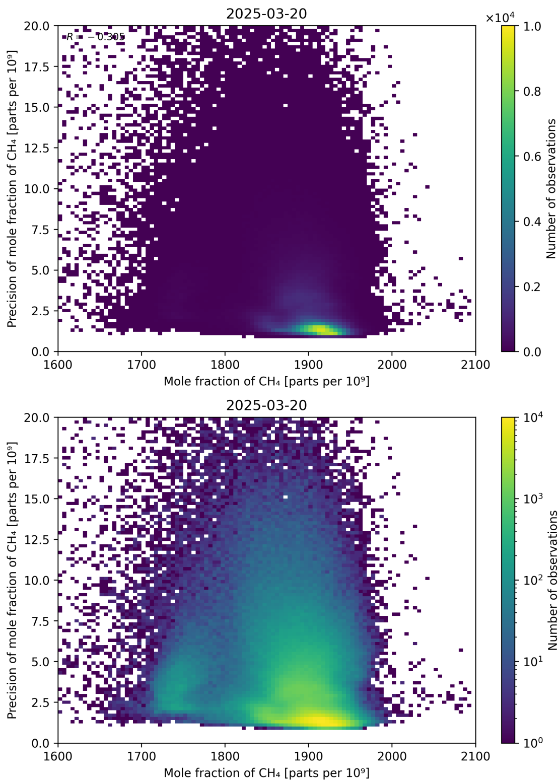
Figure 75: Scatter density plot of “Mole fraction of CH 4 ” against “Precision of mole fraction of CH 4 ” for 2025-03-19 to 2025-03-21.
