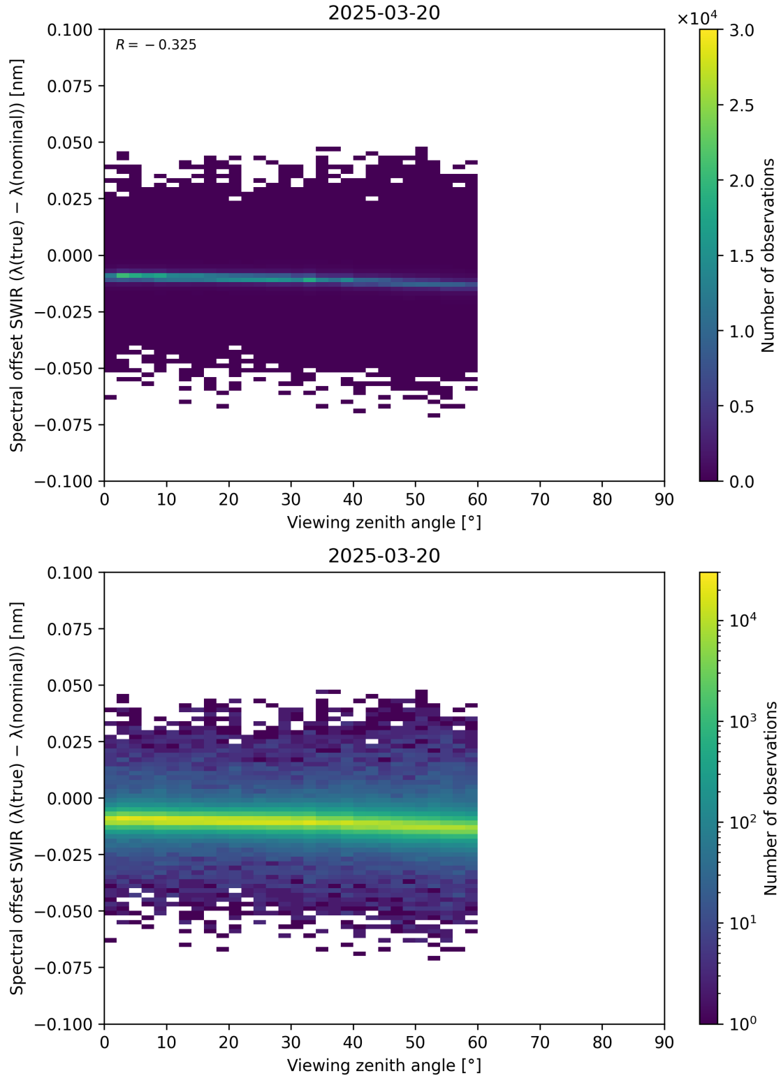
Figure 116: Scatter density plot of “Viewing zenith angle” against “Spectral offset SWIR ( \lambda_{\text{true}} - \lambda_{\text{nominal}} )” for 2025-03-19 to 2025-03-21.
