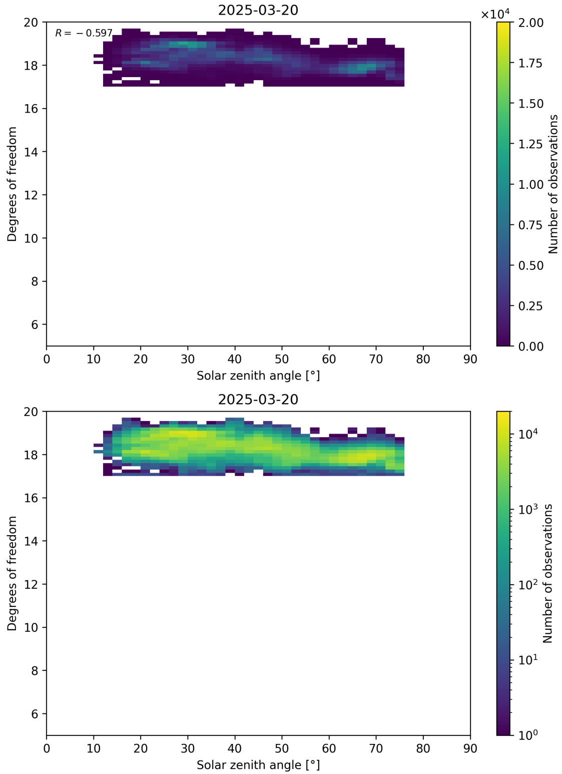
Figure 96: Scatter density plot of “Solar zenith angle” against “Degrees of freedom” for 2025-03-19 to 2025-03-21.
