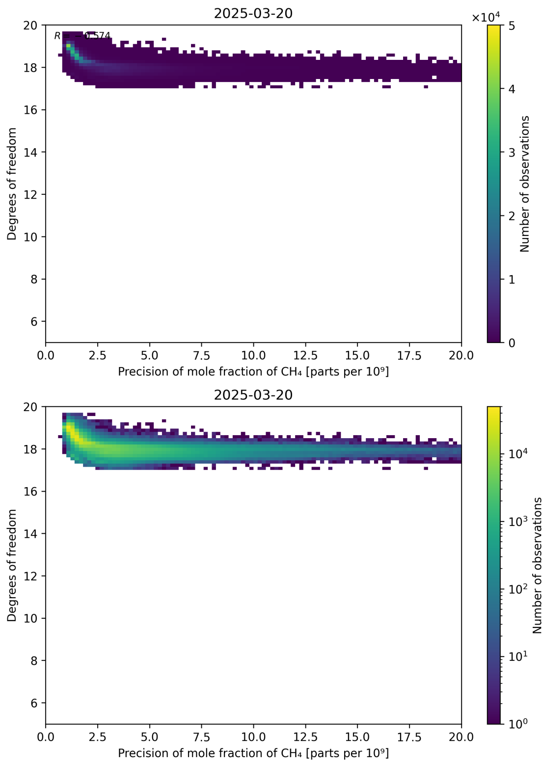
Figure 80: Scatter density plot of “Precision of mole fraction of CH 4 ” against “Degrees of freedom” for 2025-03-19 to 2025-03-21.
