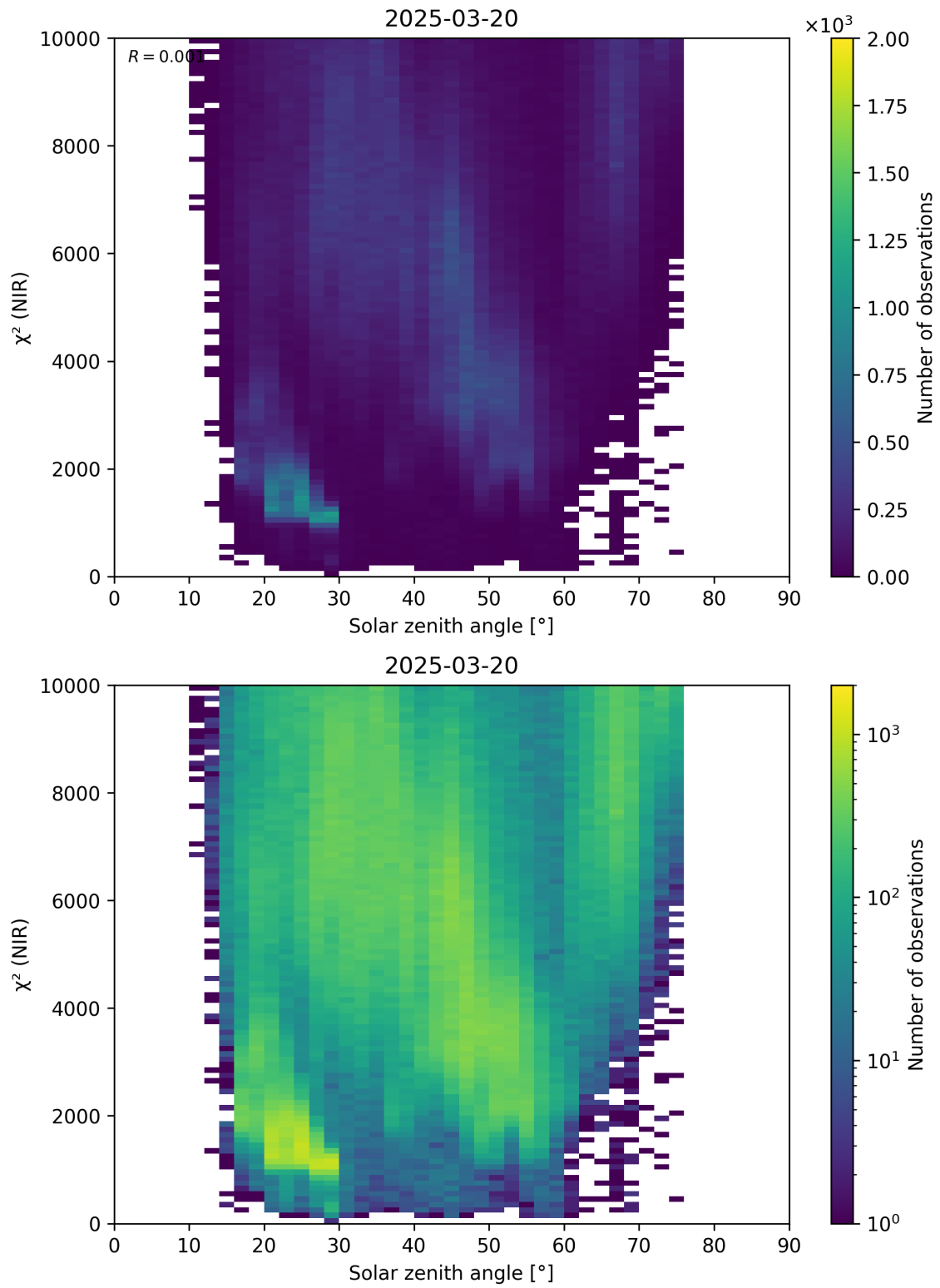
Figure 94: Scatter density plot of “Solar zenith angle” against “ \chi^2 (NIR)” for 2025-03-19 to 2025-03-21.
