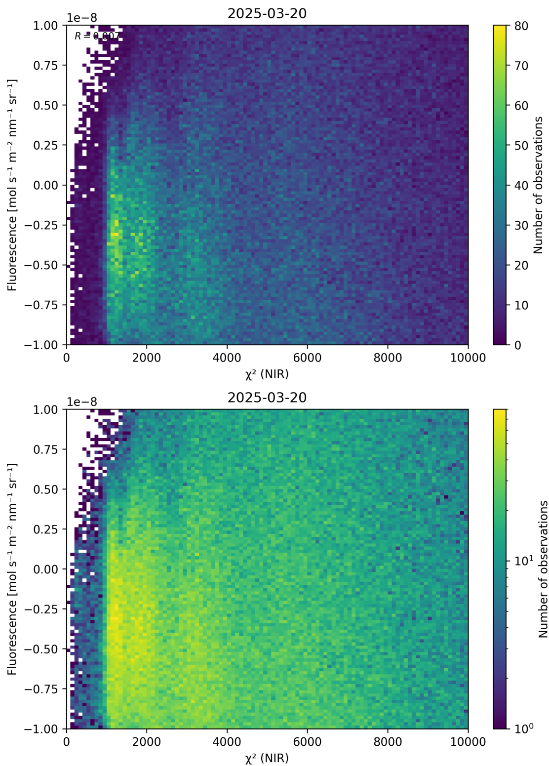
Figure 45: Scatter density plot of “ \chi^2 (NIR)” against “Fluorescence” for 2025-03-19 to 2025-03-21.
