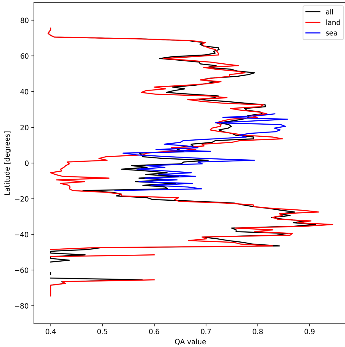
Figure 11: Zonal average of “QA value” for 2025-03-19 to 2025-03-21.
