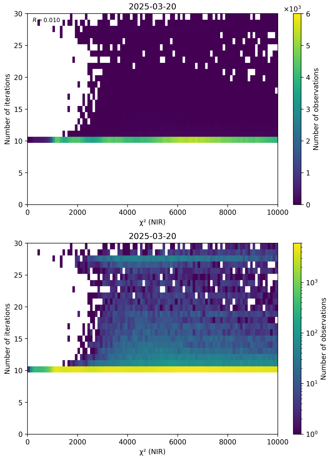
Figure 46: Scatter density plot of “ \chi^2 (NIR)” against “Number of iterations” for 2025-03-19 to 2025-03-21.
