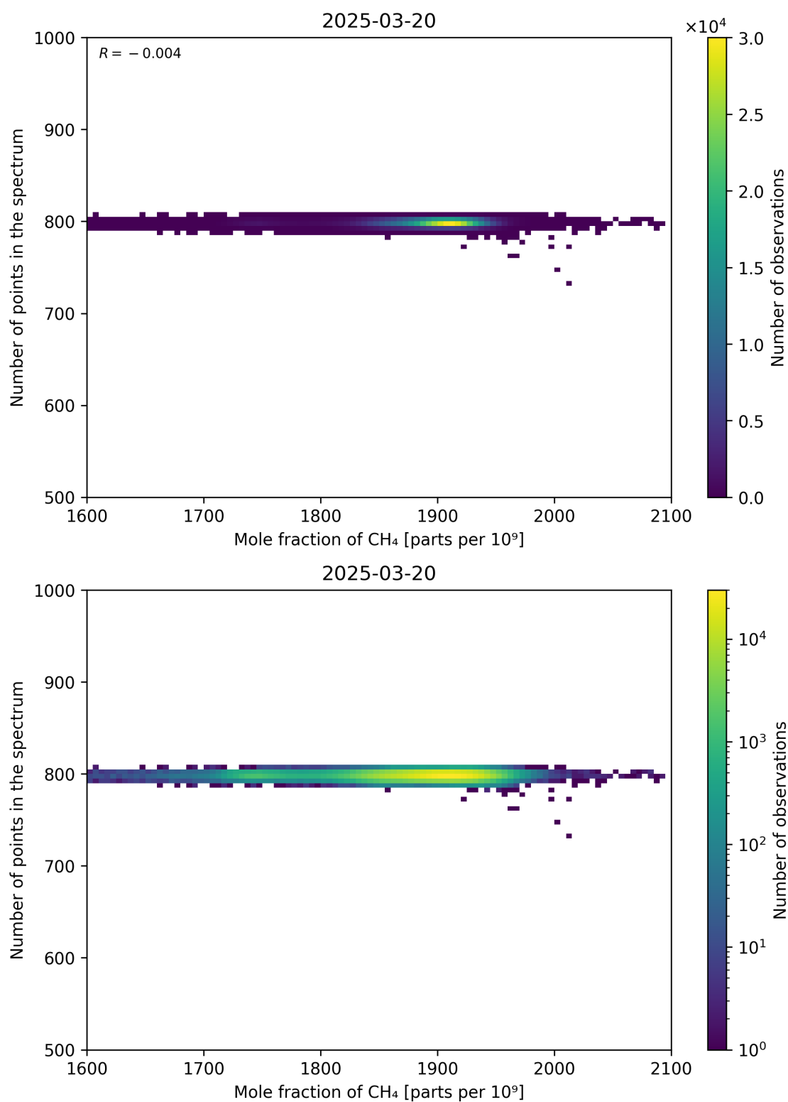
Figure 77: Scatter density plot of “Mole fraction of CH 4 ” against “Number of points in the spectrum” for 2025-03-19 to 2025-03-21.
