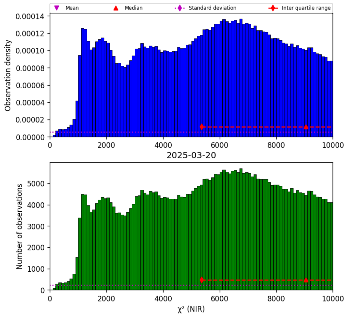
Figure 29: Histogram of “ \chi^2 (NIR)” for 2025-03-19 to 2025-03-21
