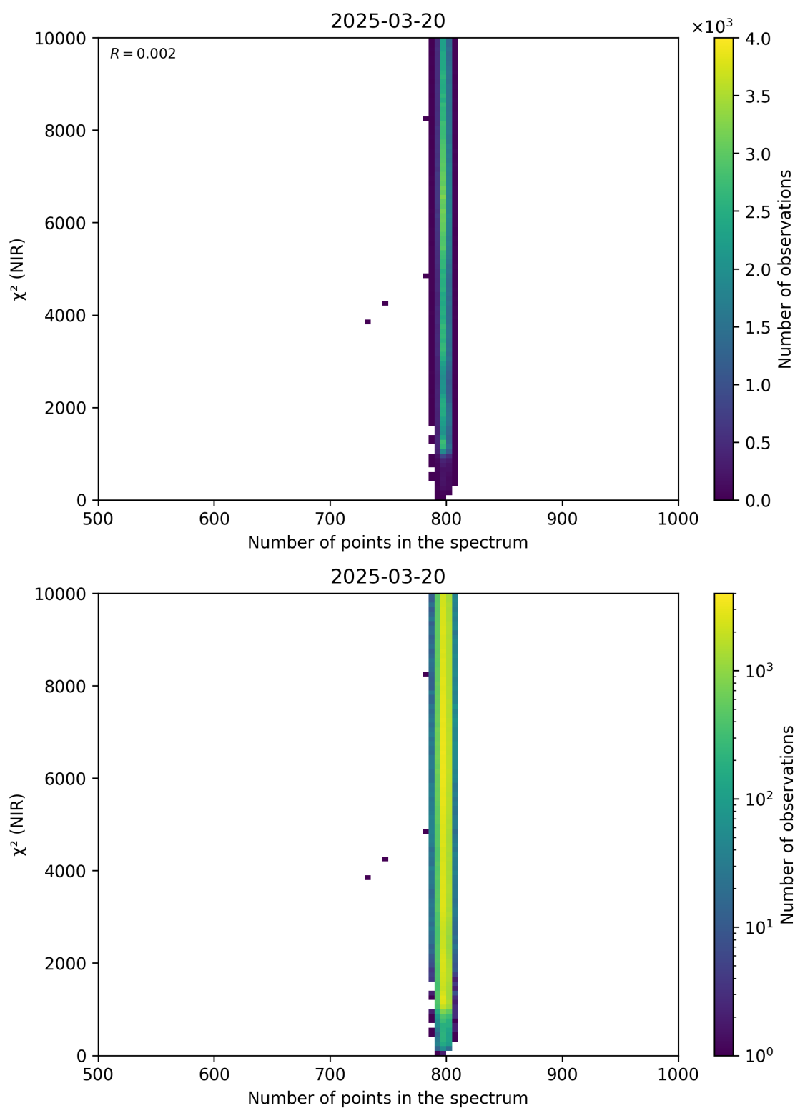
Figure 88: Scatter density plot of “Number of points in the spectrum” against “ \chi^2 (NIR)” for 2025-03-19 to 2025-03-21.
