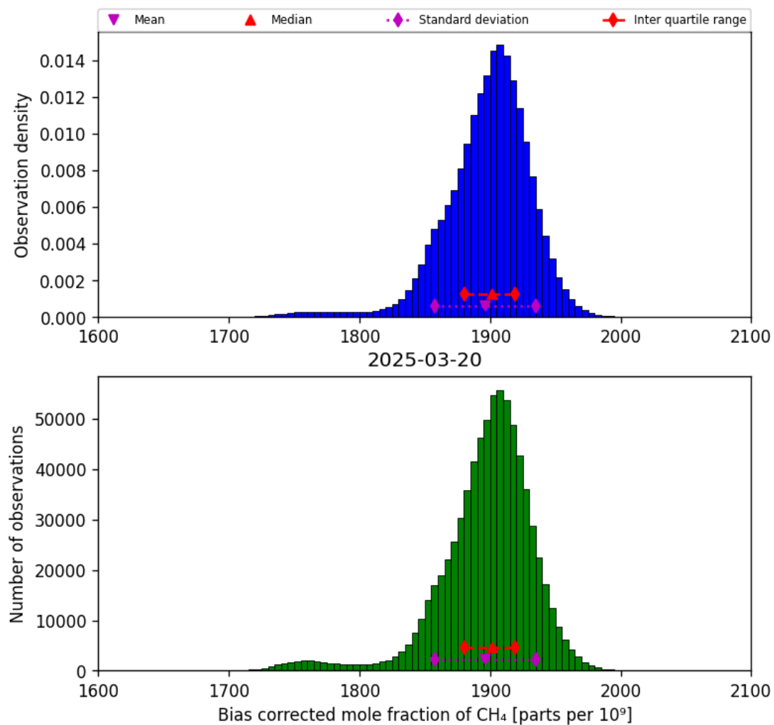
Figure 25: Histogram of “Bias corrected mole fraction of CH 4 ” for 2025-03-19 to 2025-03-21
