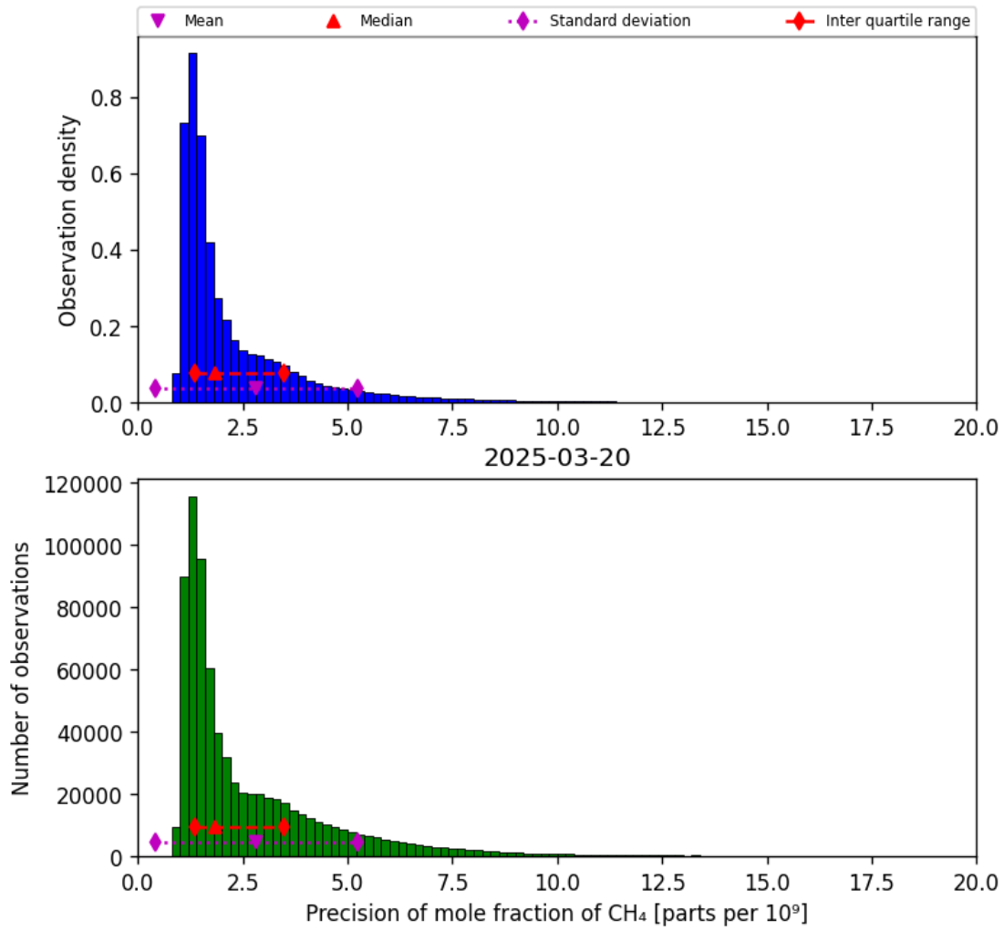
Figure 24: Histogram of “Precision of mole fraction of CH 4 ” for 2025-03-19 to 2025-03-21
