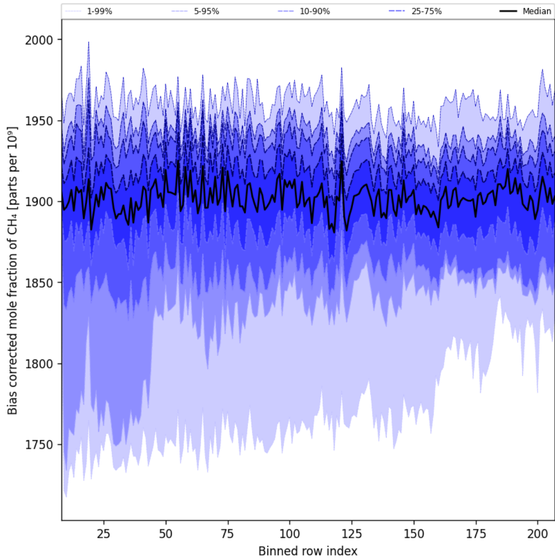
Figure 36: Along track statistics of “Bias corrected mole fraction of CH 4 ” for 2025-03-19 to 2025-03-21
