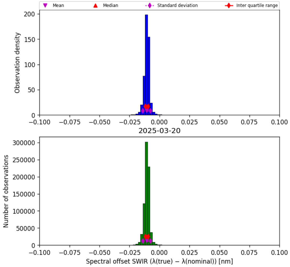
Figure 27: Histogram of “Spectral offset SWIR ( \lambda_{\text{true}} - \lambda_{\text{nominal}} )” for 2025-03-19 to 2025-03-21
