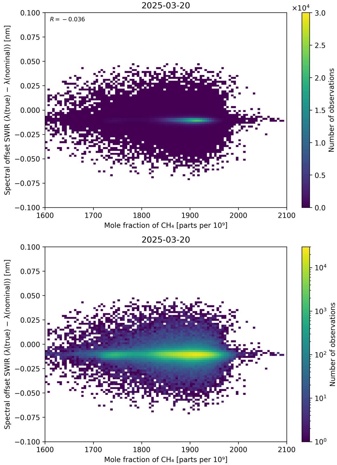
Figure 86: Scatter density plot of “Mole fraction of CH 4 ” against “Spectral offset SWIR ( \lambda_{\text{true}} - \lambda_{\text{nominal}} )” for 2025-03-19 to 2025-03-21.
