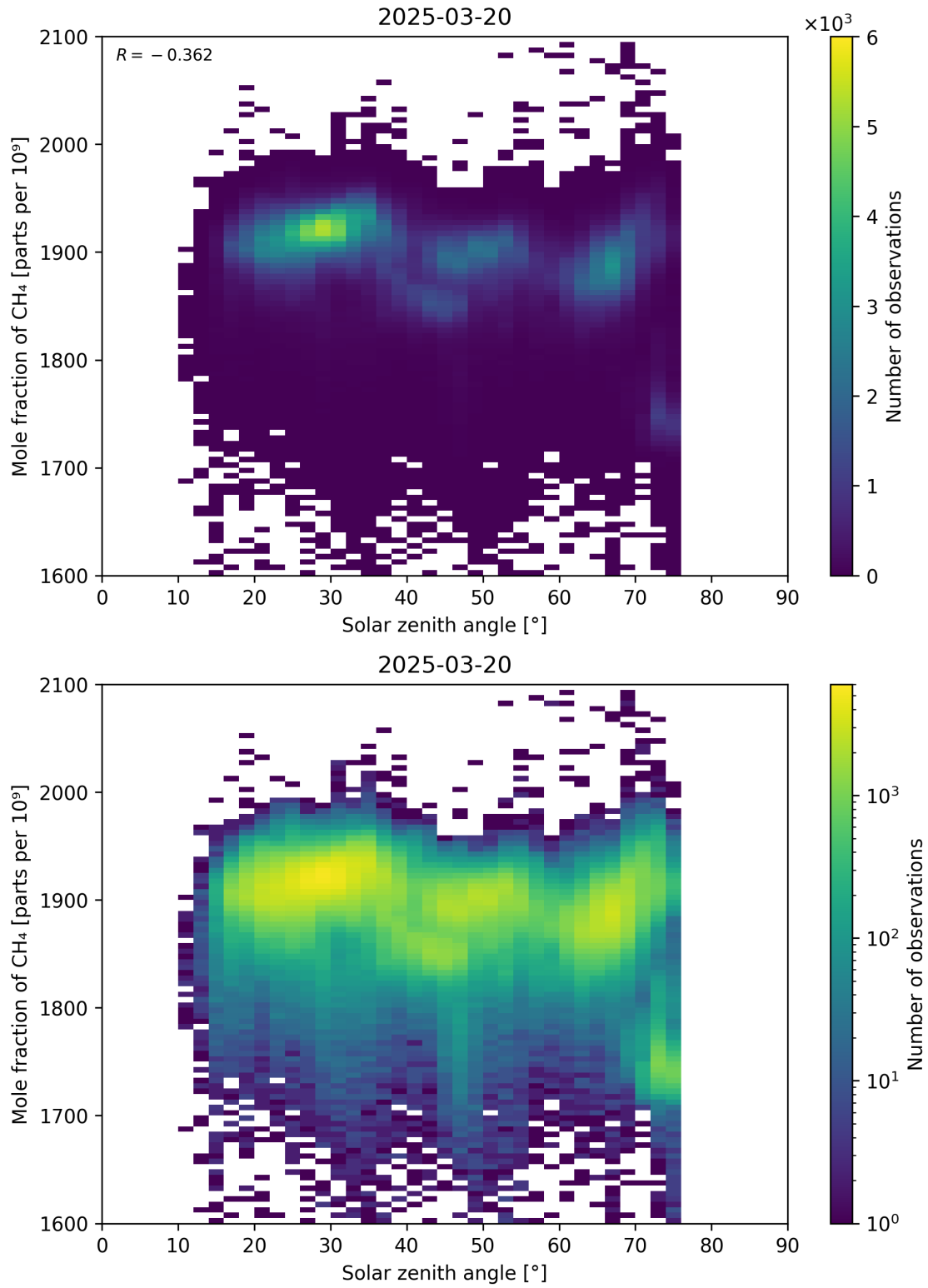
Figure 99: Scatter density plot of “Solar zenith angle” against “Mole fraction of CH 4 ” for 2025-03-19 to 2025-03-21.
