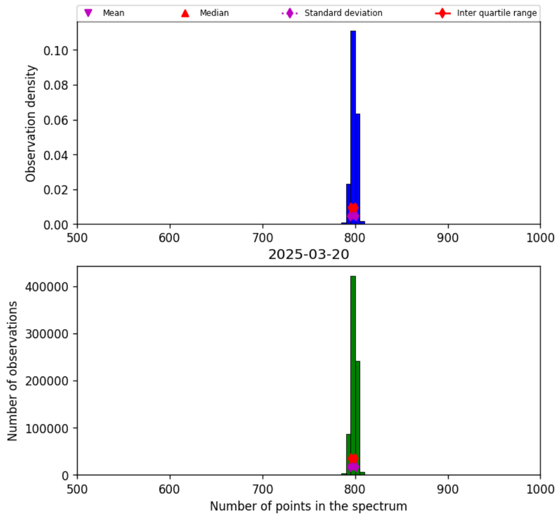
Figure 26: Histogram of “Number of points in the spectrum” for 2025-03-19 to 2025-03-21
