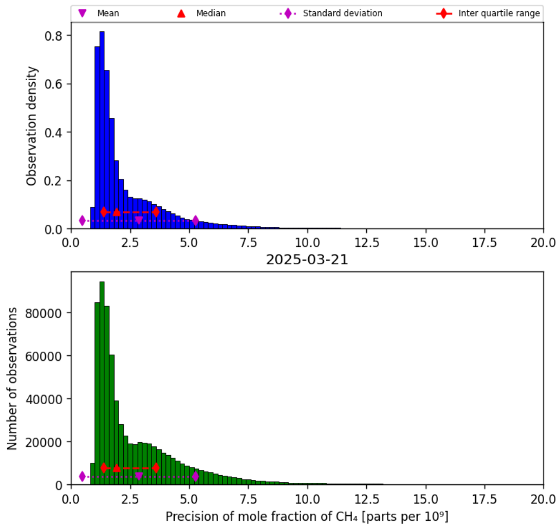
Figure 24: Histogram of “Precision of mole fraction of CH 4 ” for 2025-03-20 to 2025-03-22
