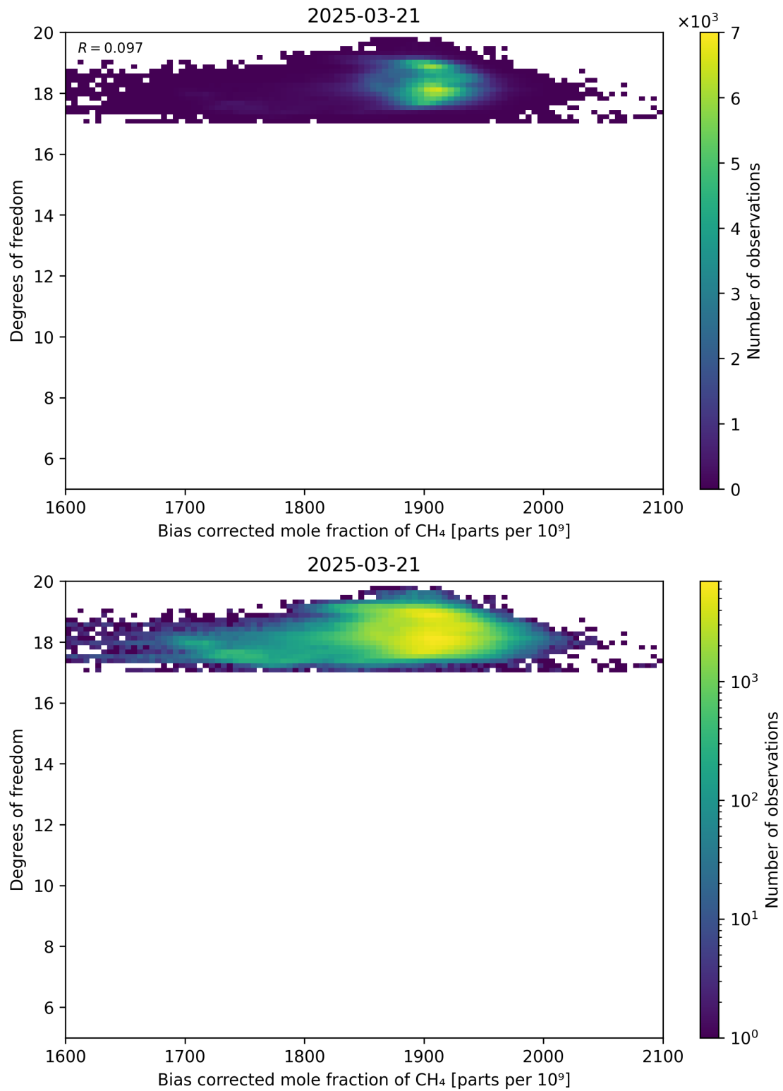
Figure 65: Scatter density plot of “Bias corrected mole fraction of CH 4 ” against “Degrees of freedom” for 2025-03-20 to 2025-03-22.
