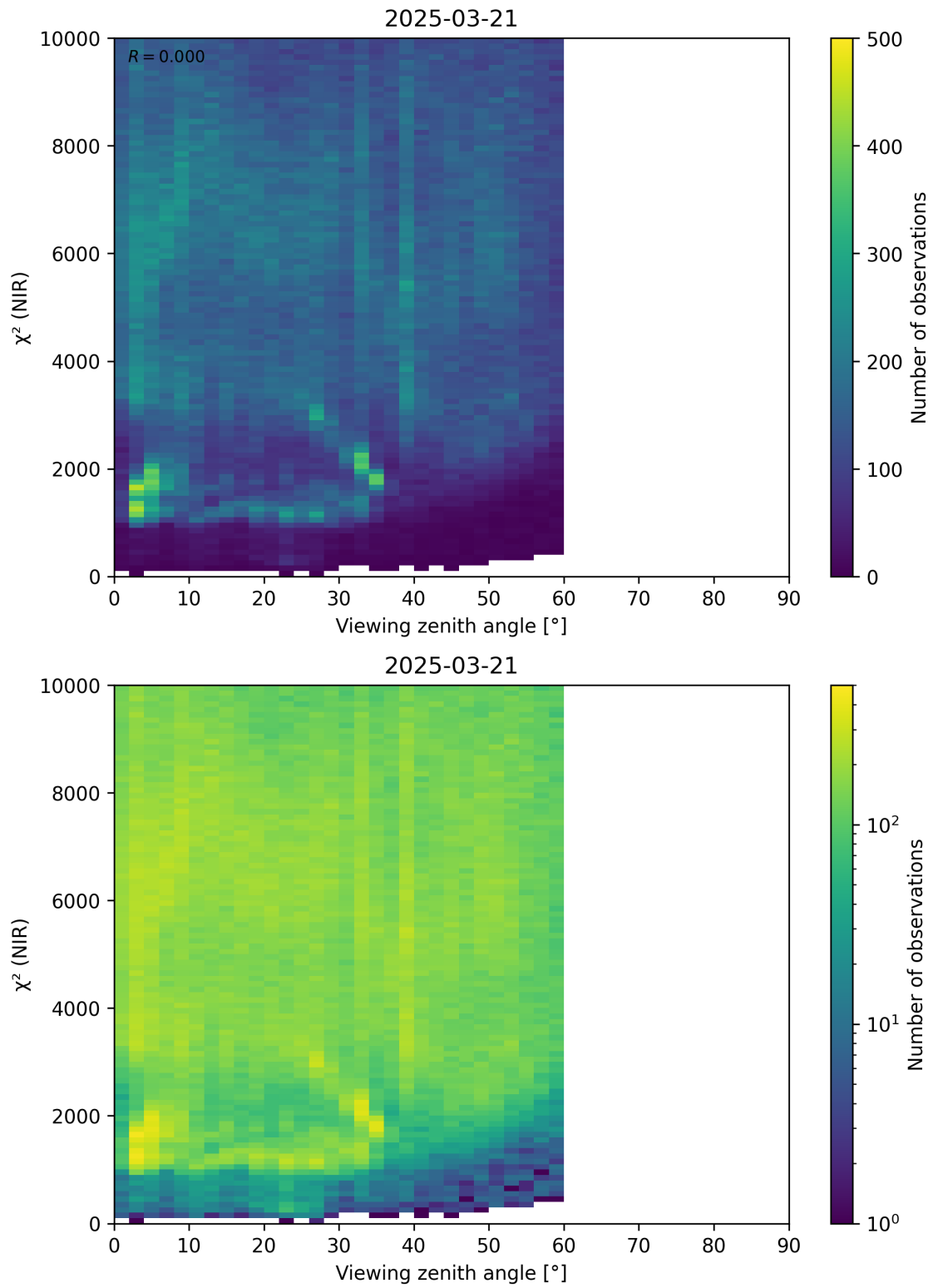
Figure 105: Scatter density plot of “Viewing zenith angle” against “ \chi^2 (NIR)” for 2025-03-20 to 2025-03-22.
