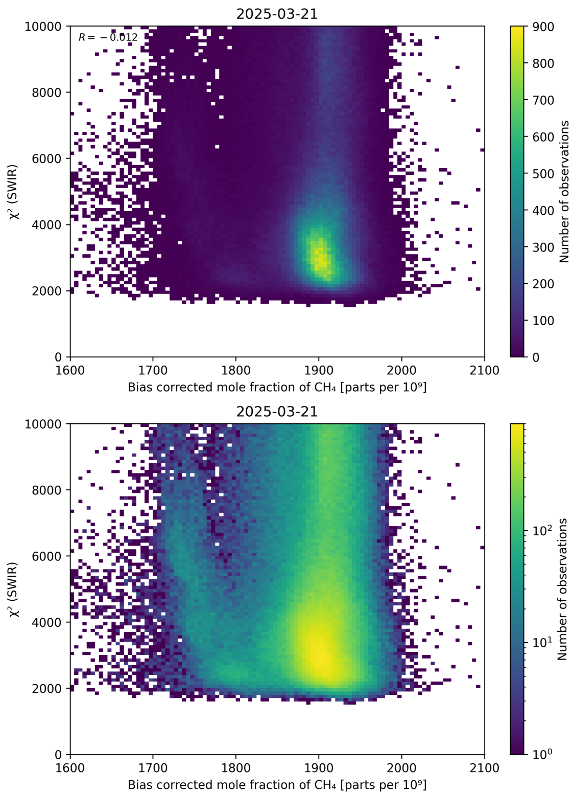
Figure 64: Scatter density plot of “Bias corrected mole fraction of \text{CH}_4 ” against “ \chi^2 (SWIR)” for 2025-03-20 to 2025-03-22.
