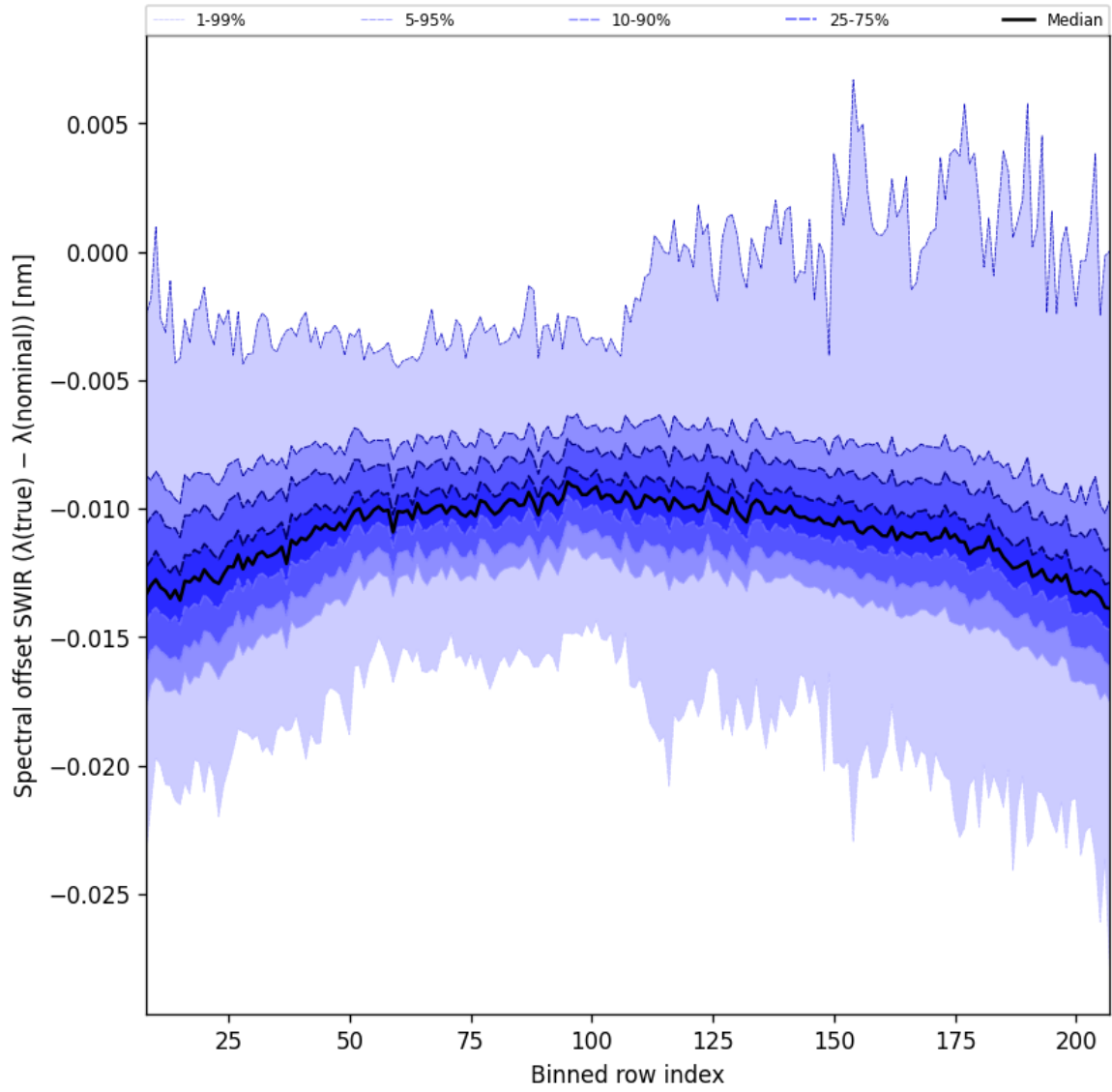
Figure 38: Along track statistics of “Spectral offset SWIR ( \lambda_{\text{true}} - \lambda_{\text{nominal}} )” for 2025-03-20 to 2025-03-22
