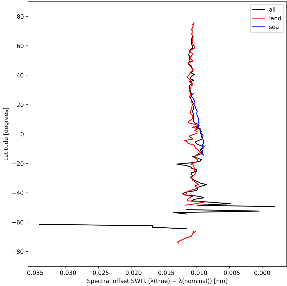
Figure 16: Zonal average of “Spectral offset SWIR ( \lambda_{\text{true}} - \lambda_{\text{nominal}} )” for 2025-03-20 to 2025-03-22.
