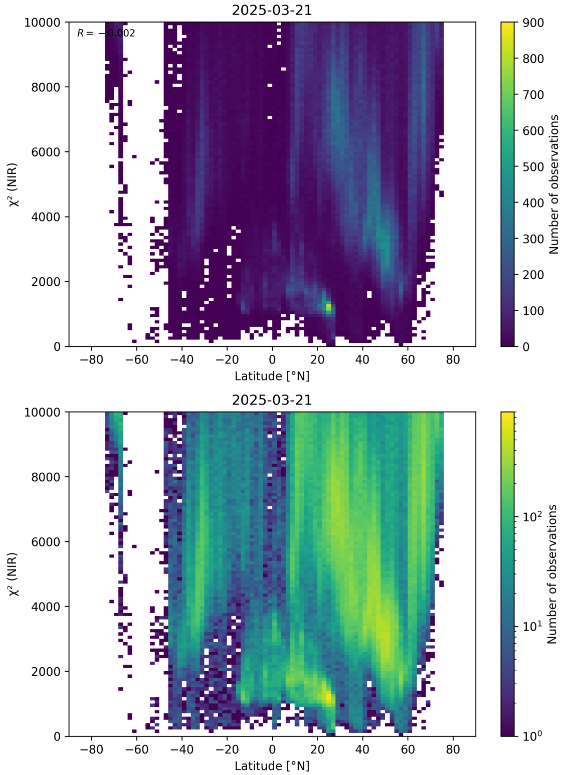
Figure 53: Scatter density plot of “Latitude” against “ \chi^2 (NIR)” for 2025-03-20 to 2025-03-22.
