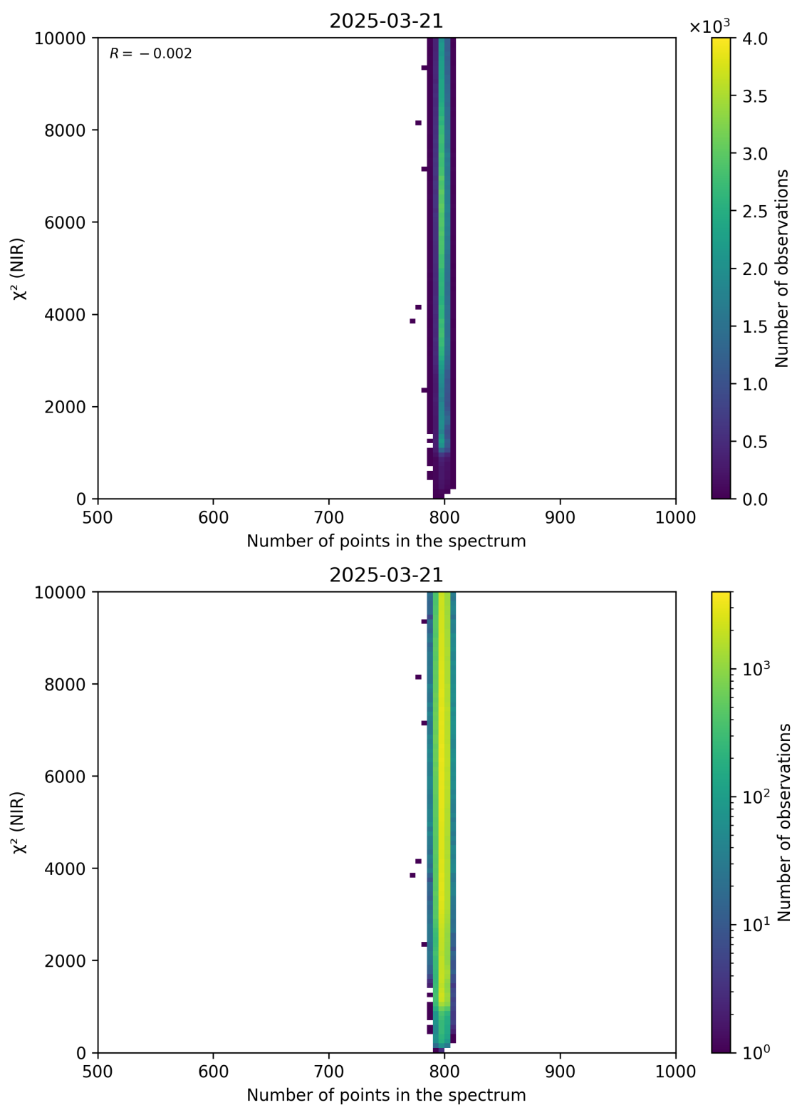
Figure 88: Scatter density plot of “Number of points in the spectrum” against “ \chi^2 (NIR)” for 2025-03-20 to 2025-03-22.
