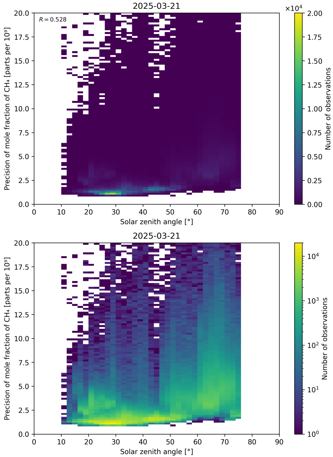
Figure 101: Scatter density plot of “Solar zenith angle” against “Precision of mole fraction of \text{CH}_4 ” for 2025-03-20 to 2025-03-22.
