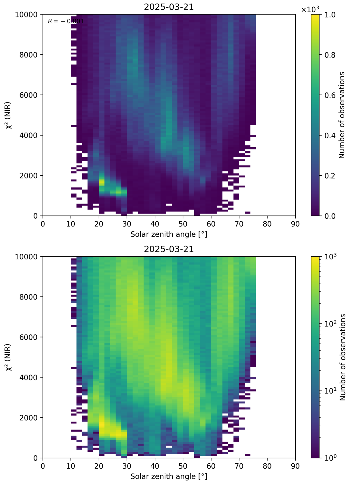
Figure 94: Scatter density plot of “Solar zenith angle” against “ \chi^2 (NIR)” for 2025-03-20 to 2025-03-22.
