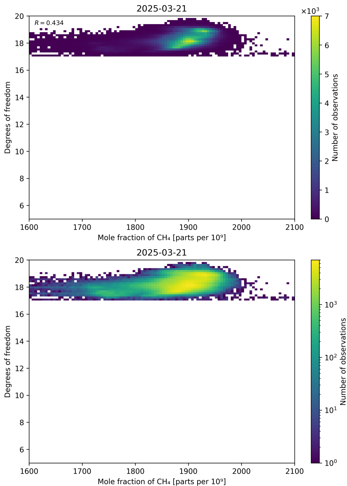
Figure 72: Scatter density plot of “Mole fraction of CH 4 ” against “Degrees of freedom” for 2025-03-20 to 2025-03-22.
