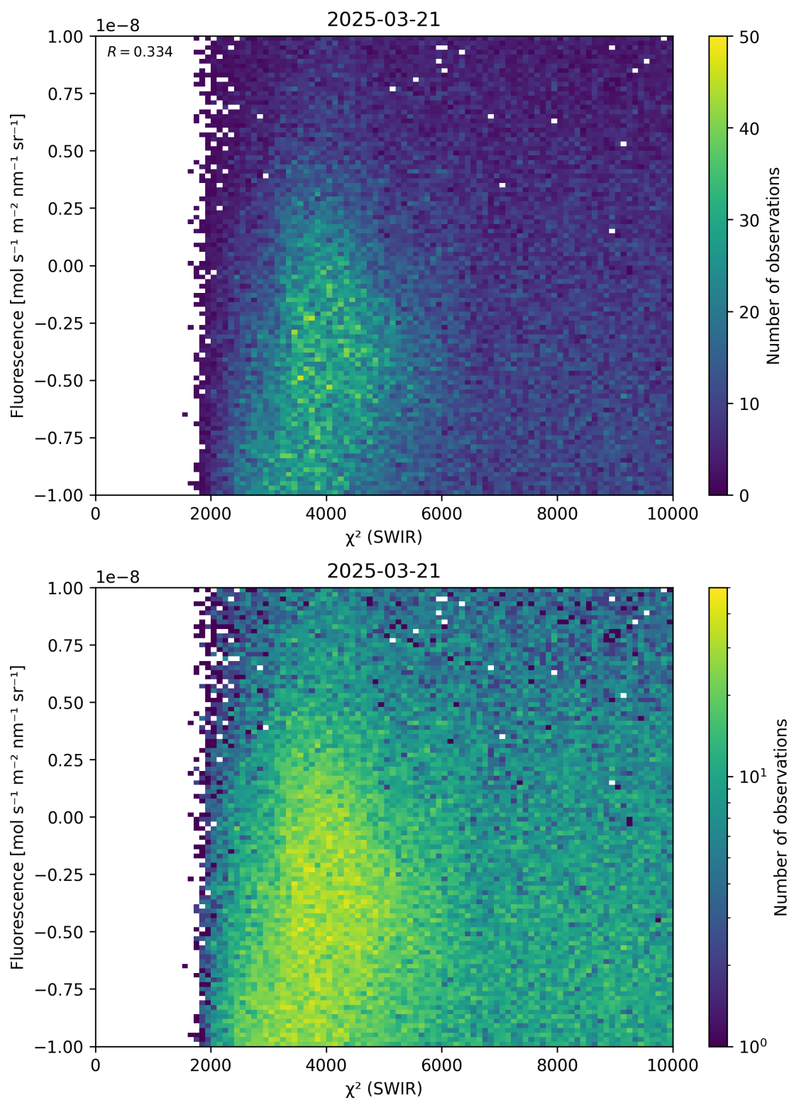
Figure 49: Scatter density plot of “ \chi^2 (SWIR)” against “Fluorescence” for 2025-03-20 to 2025-03-22.
