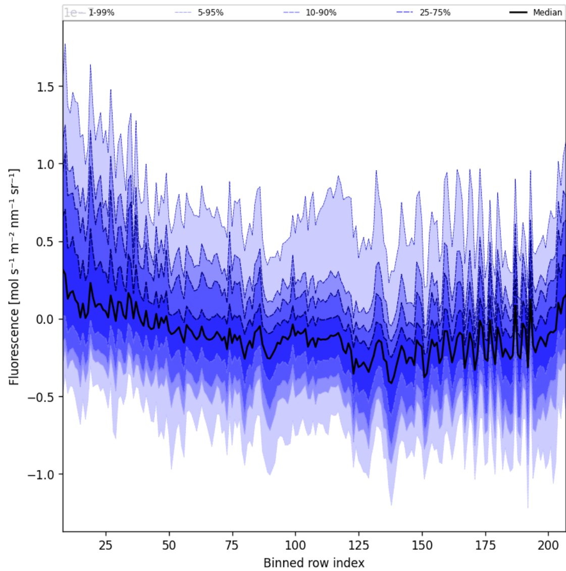
Figure 43: Along track statistics of “Fluorescence” for 2025-03-20 to 2025-03-22
