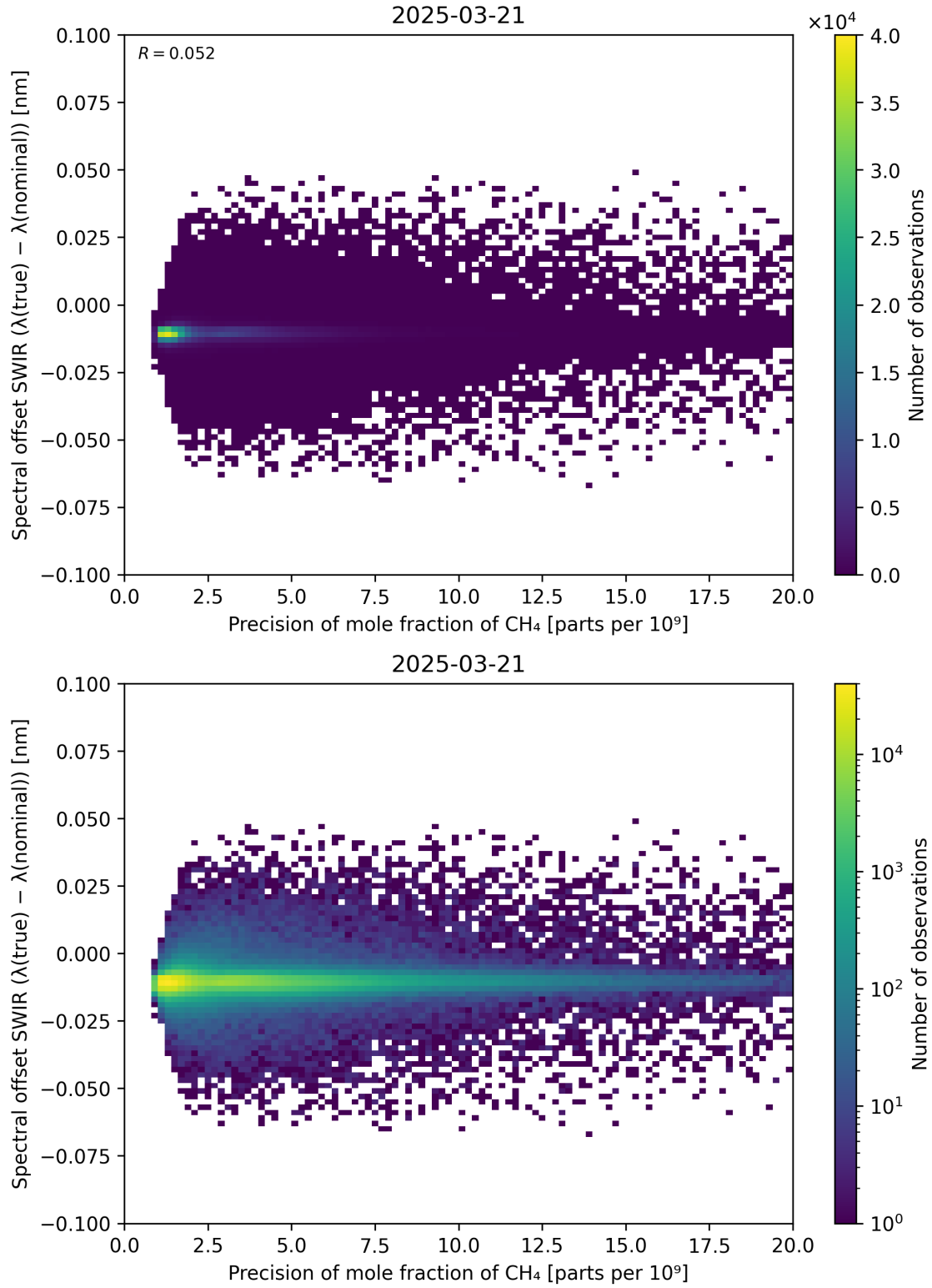
Figure 85: Scatter density plot of “Precision of mole fraction of \text{CH}_4 ” against “Spectral offset SWIR ( \lambda_{\text{true}} - \lambda_{\text{nominal}} )” for 2025-03-20 to 2025-03-22.
