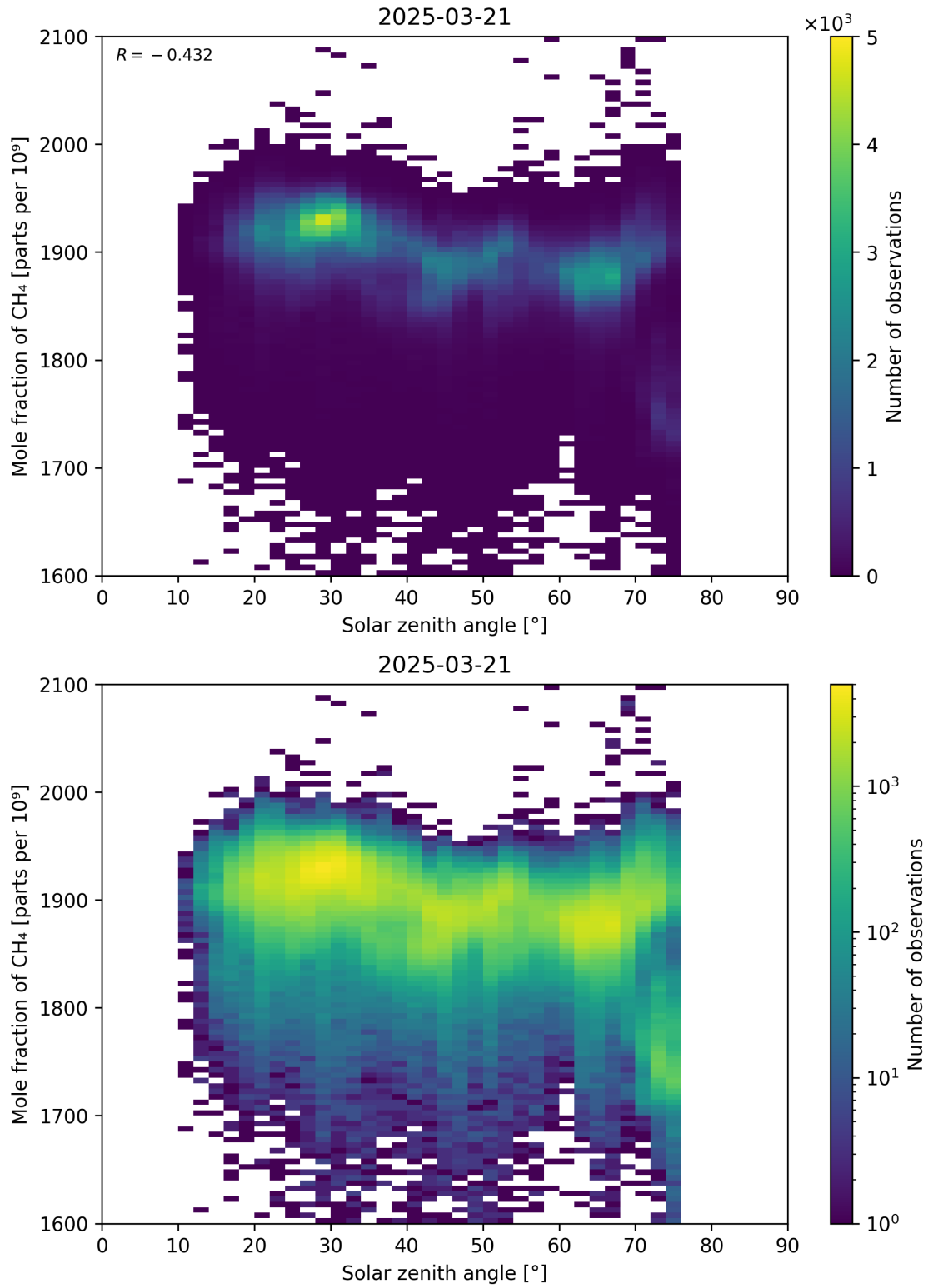
Figure 99: Scatter density plot of “Solar zenith angle” against “Mole fraction of CH 4 ” for 2025-03-20 to 2025-03-22.
