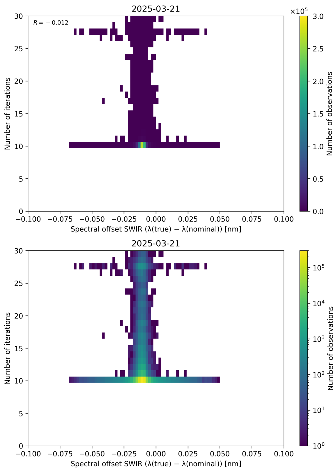
Figure 121: Scatter density plot of “Spectral offset SWIR ( \lambda_{\text{true}} - \lambda_{\text{nominal}} )” against “Number of iterations” for 2025-03-20 to 2025-03-22.
