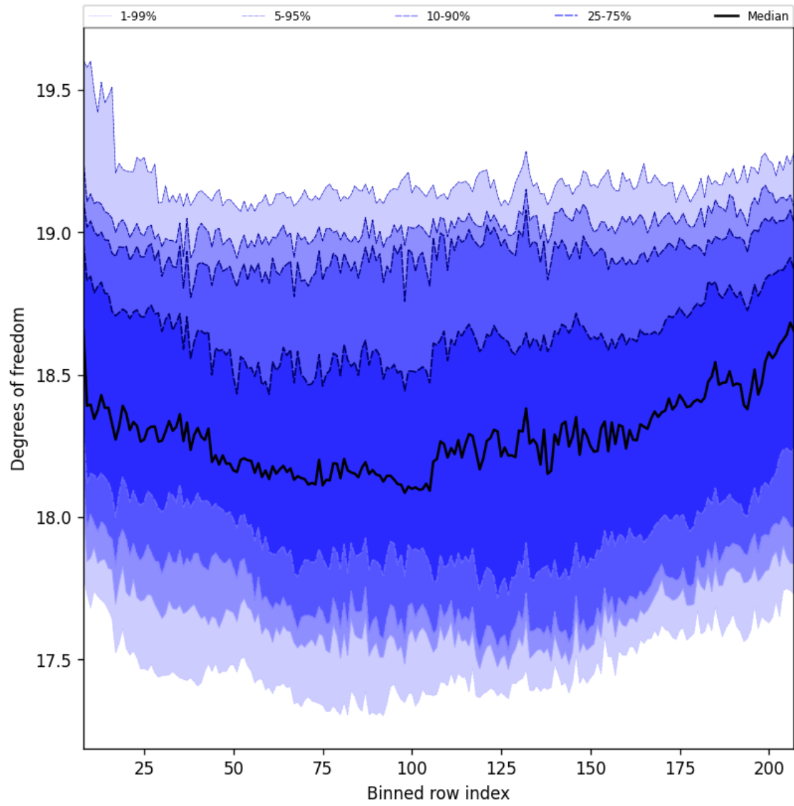
Figure 41: Along track statistics of “Degrees of freedom” for 2025-03-20 to 2025-03-22
