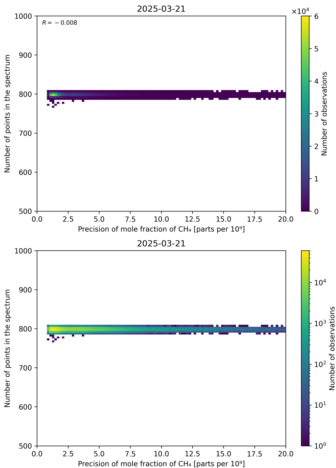
Figure 84: Scatter density plot of “Precision of mole fraction of CH 4 ” against “Number of points in the spectrum” for 2025-03-20 to 2025-03-22.
