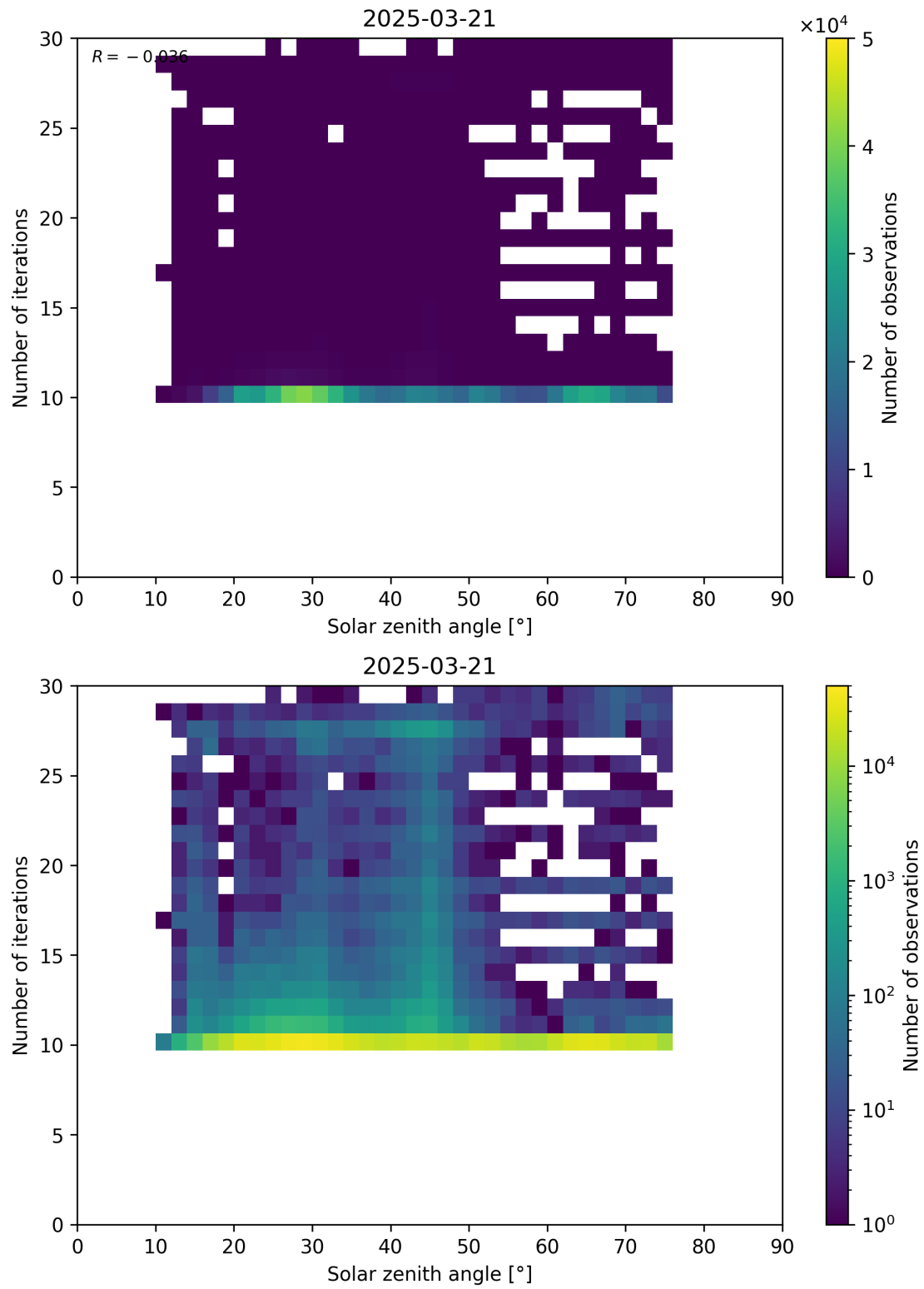
Figure 102: Scatter density plot of “Solar zenith angle” against “Number of iterations” for 2025-03-20 to 2025-03-22.
