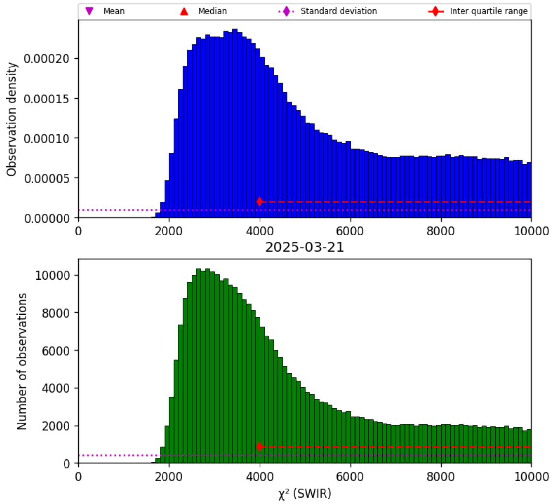
Figure 28: Histogram of “ \chi^2 (SWIR)” for 2025-03-20 to 2025-03-22
