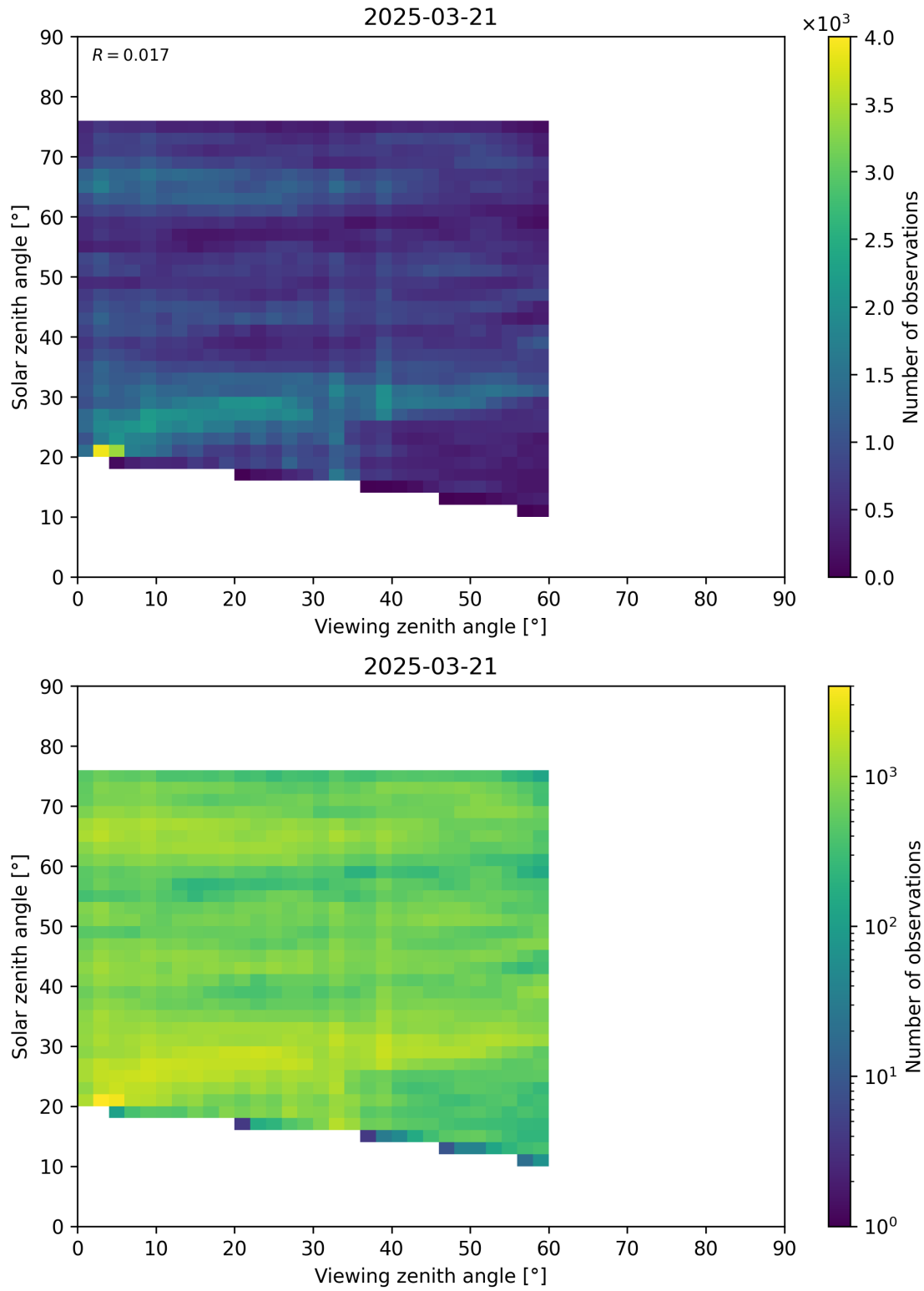
Figure 115: Scatter density plot of “Viewing zenith angle” against “Solar zenith angle” for 2025-03-20 to 2025-03-22.
