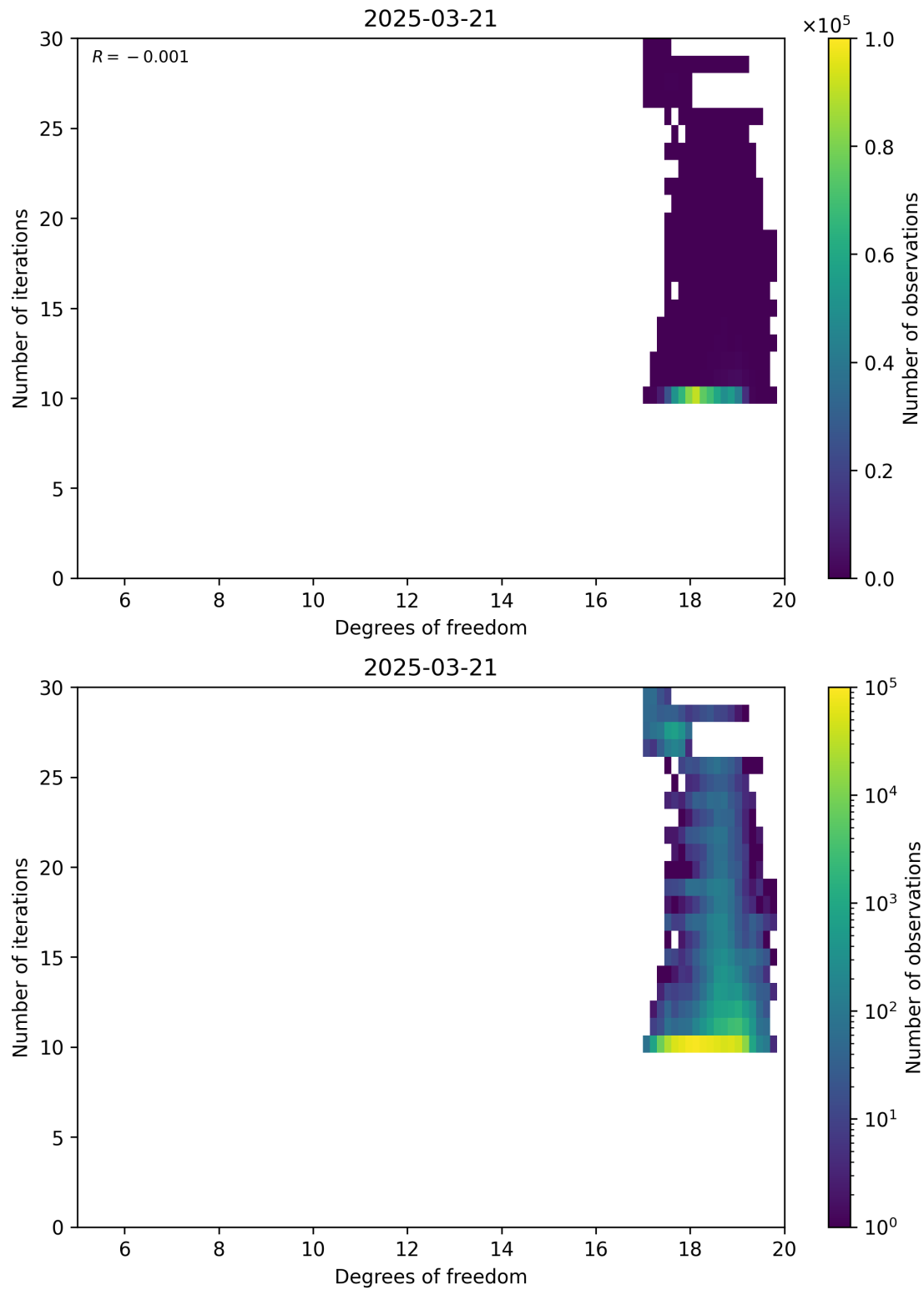
Figure 52: Scatter density plot of “Degrees of freedom” against “Number of iterations” for 2025-03-20 to 2025-03-22.
