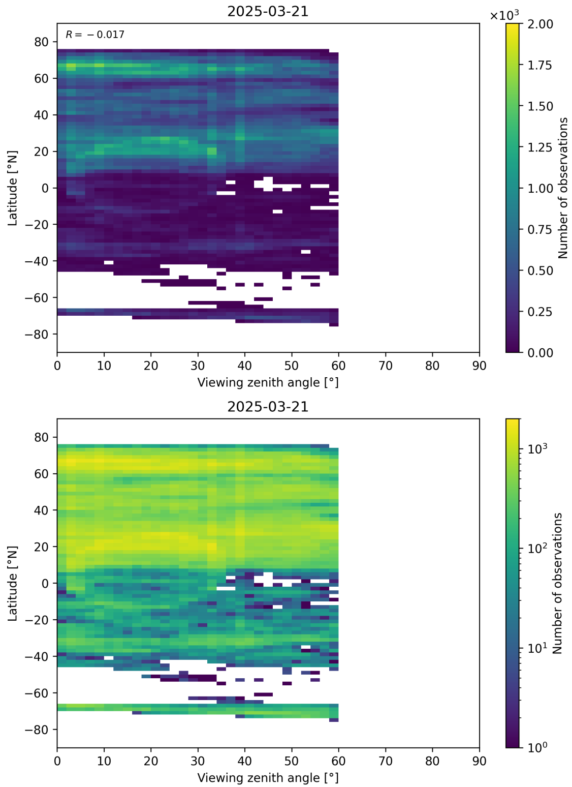
Figure 109: Scatter density plot of “Viewing zenith angle” against “Latitude” for 2025-03-20 to 2025-03-22.
