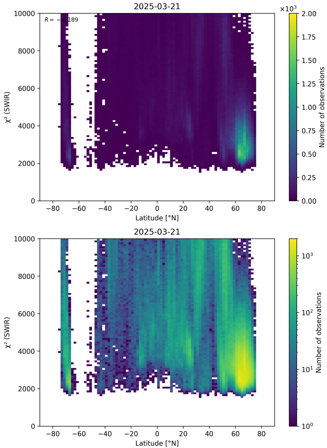
Figure 54: Scatter density plot of “Latitude” against “ \chi^2 (SWIR)” for 2025-03-20 to 2025-03-22.
