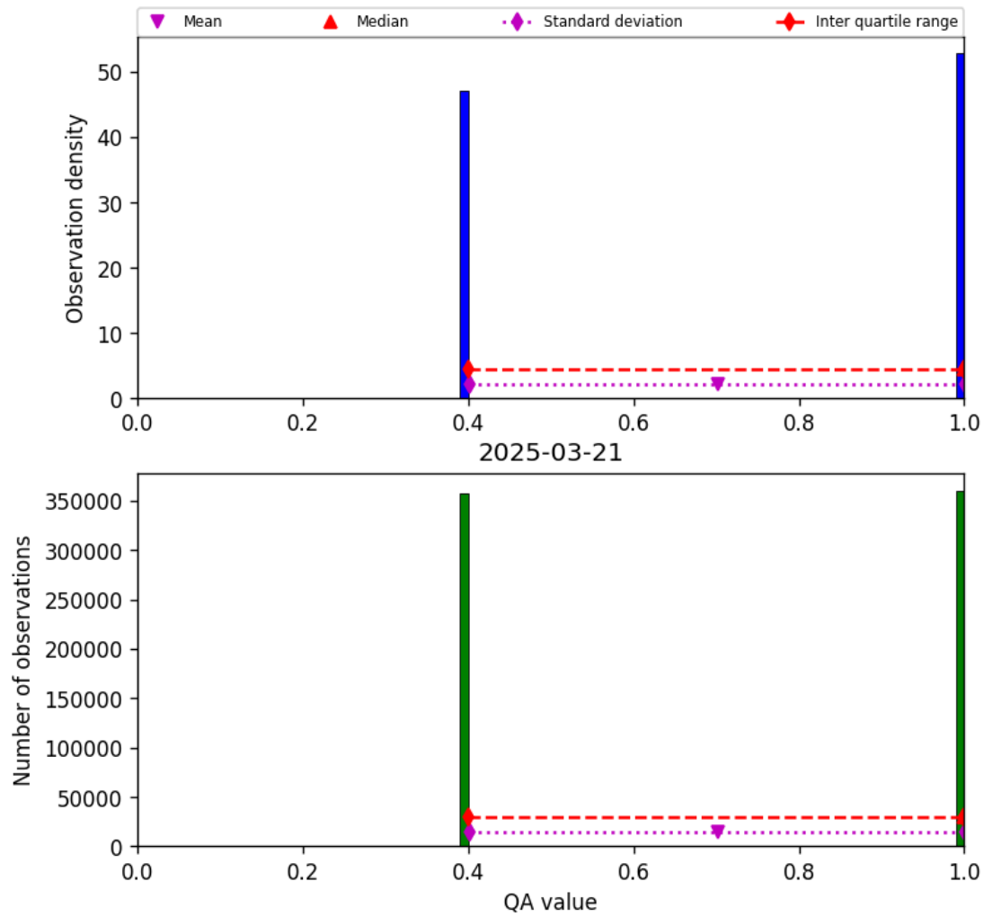
Figure 22: Histogram of “QA value” for 2025-03-20 to 2025-03-22
