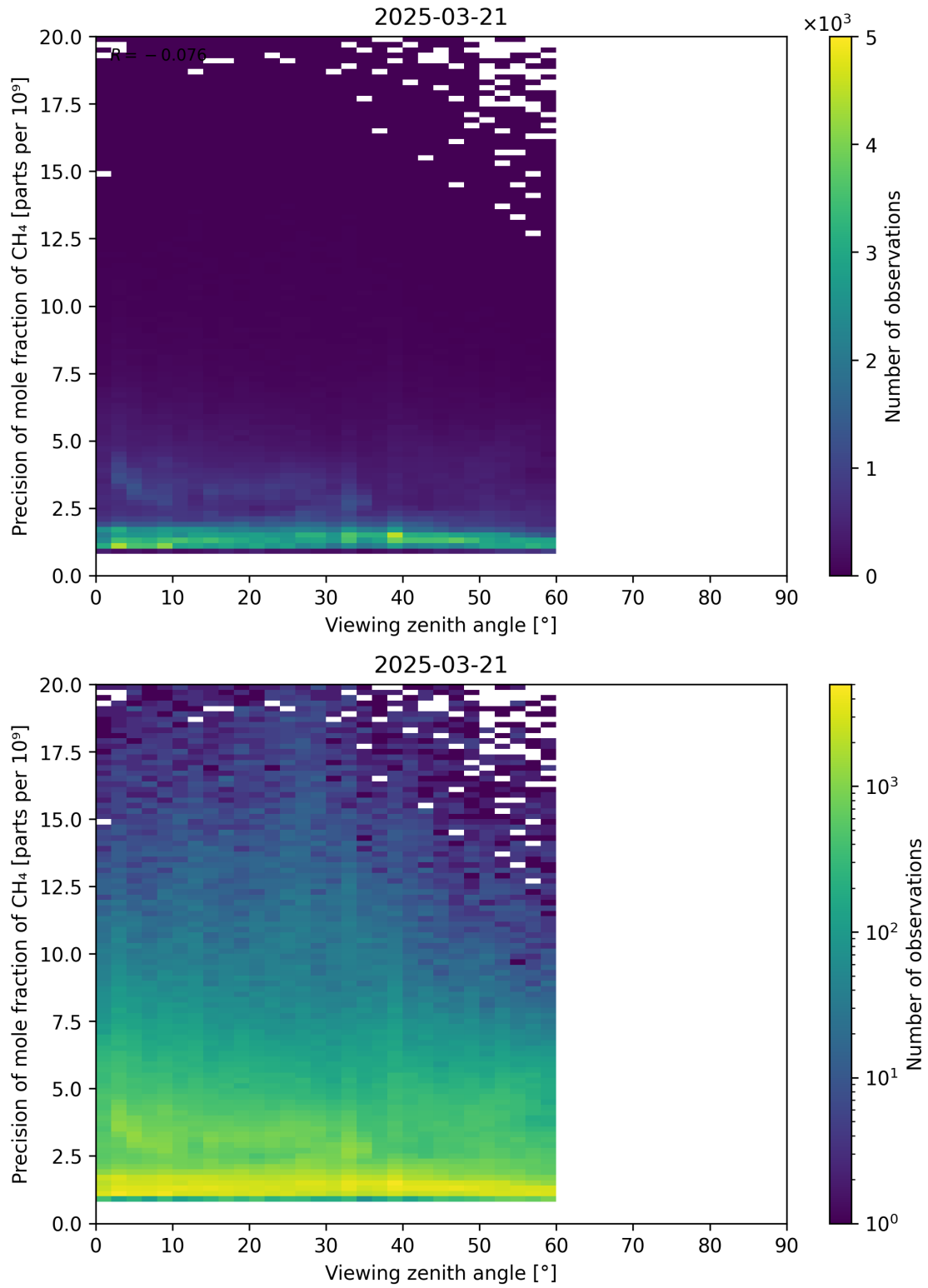
Figure 112: Scatter density plot of “Viewing zenith angle” against “Precision of mole fraction of CH 4 ” for 2025-03-20 to 2025-03-22.
