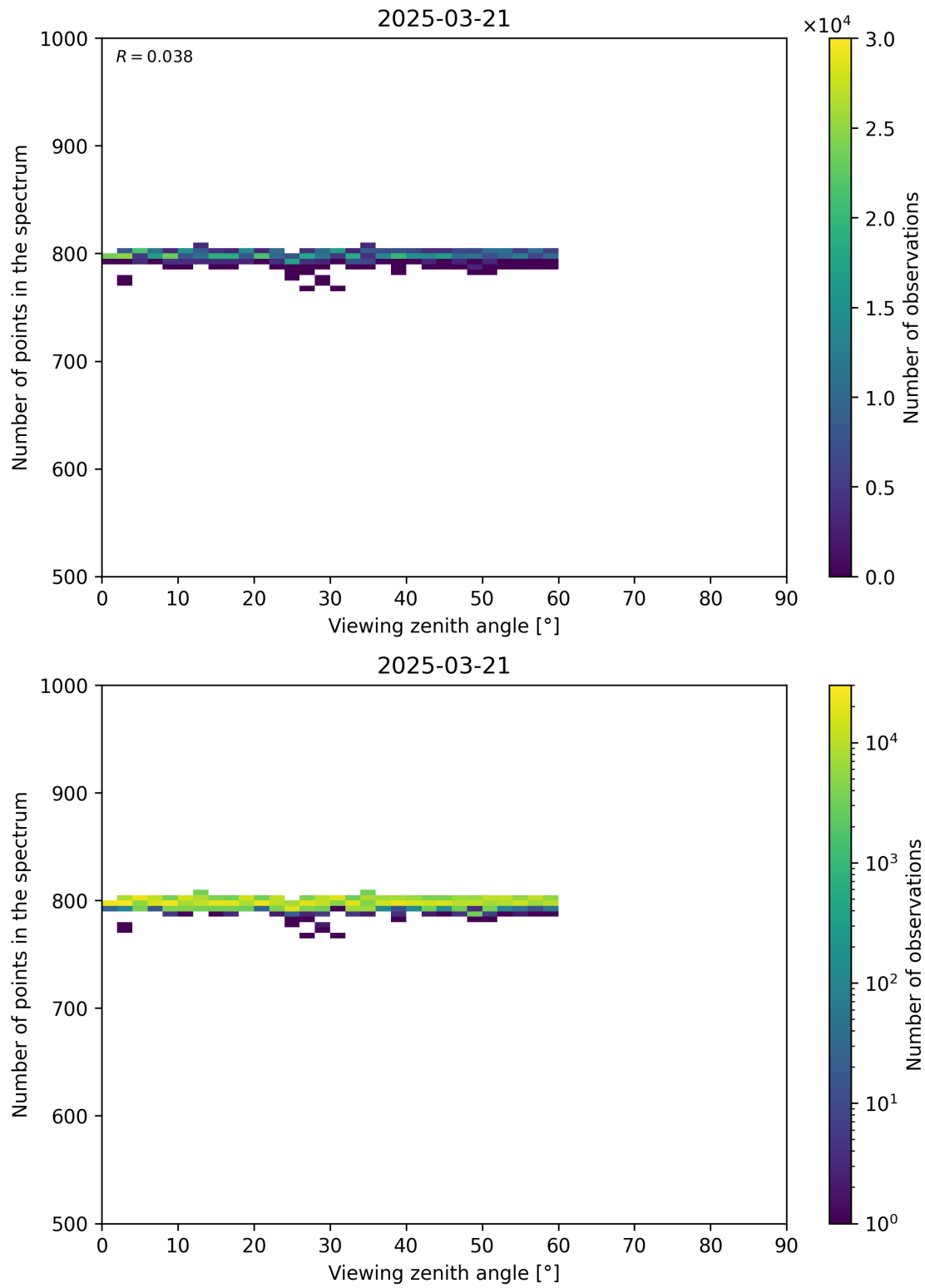
Figure 114: Scatter density plot of “Viewing zenith angle” against “Number of points in the spectrum” for 2025-03-20 to 2025-03-22.
