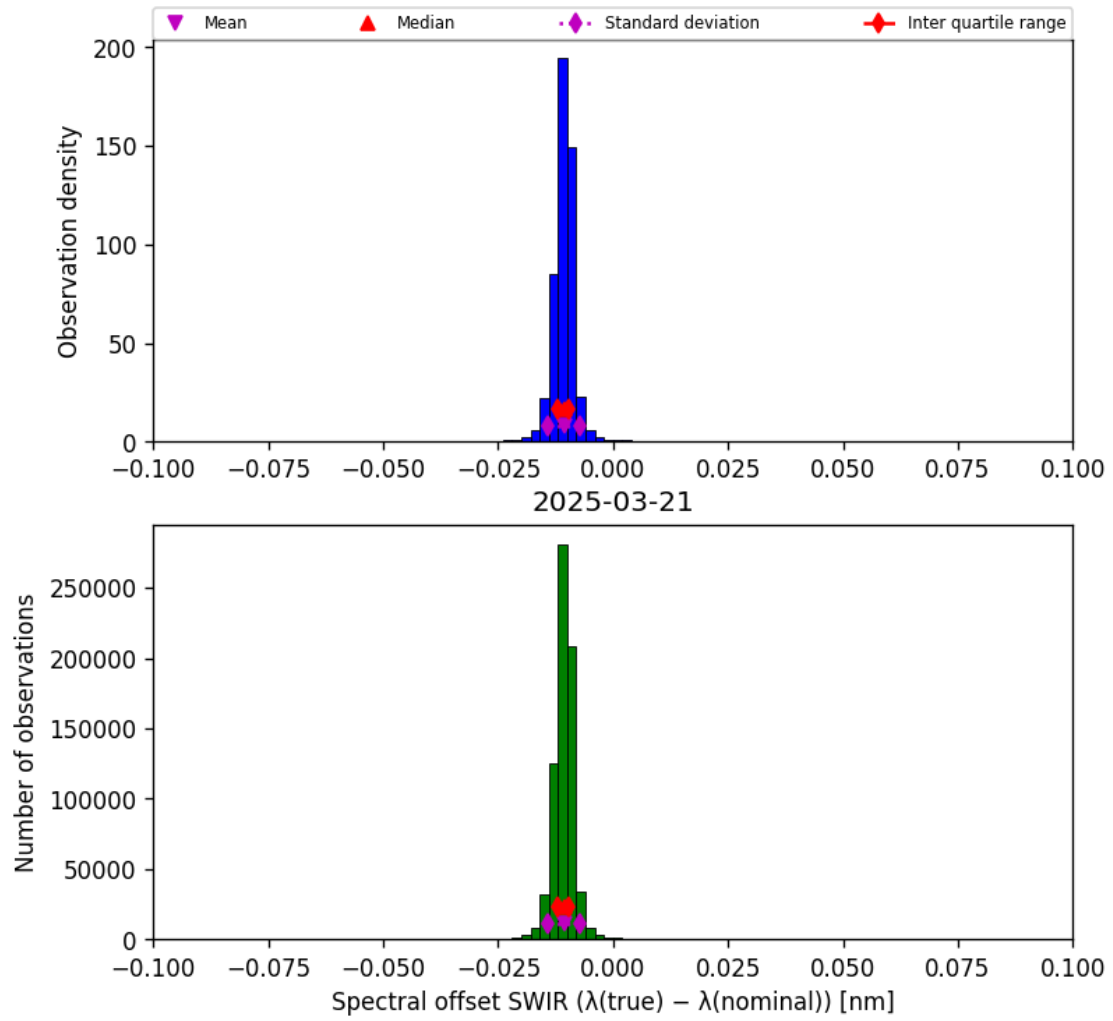
Figure 27: Histogram of “Spectral offset SWIR ( \lambda_{\text{true}} - \lambda_{\text{nominal}} )” for 2025-03-20 to 2025-03-22
