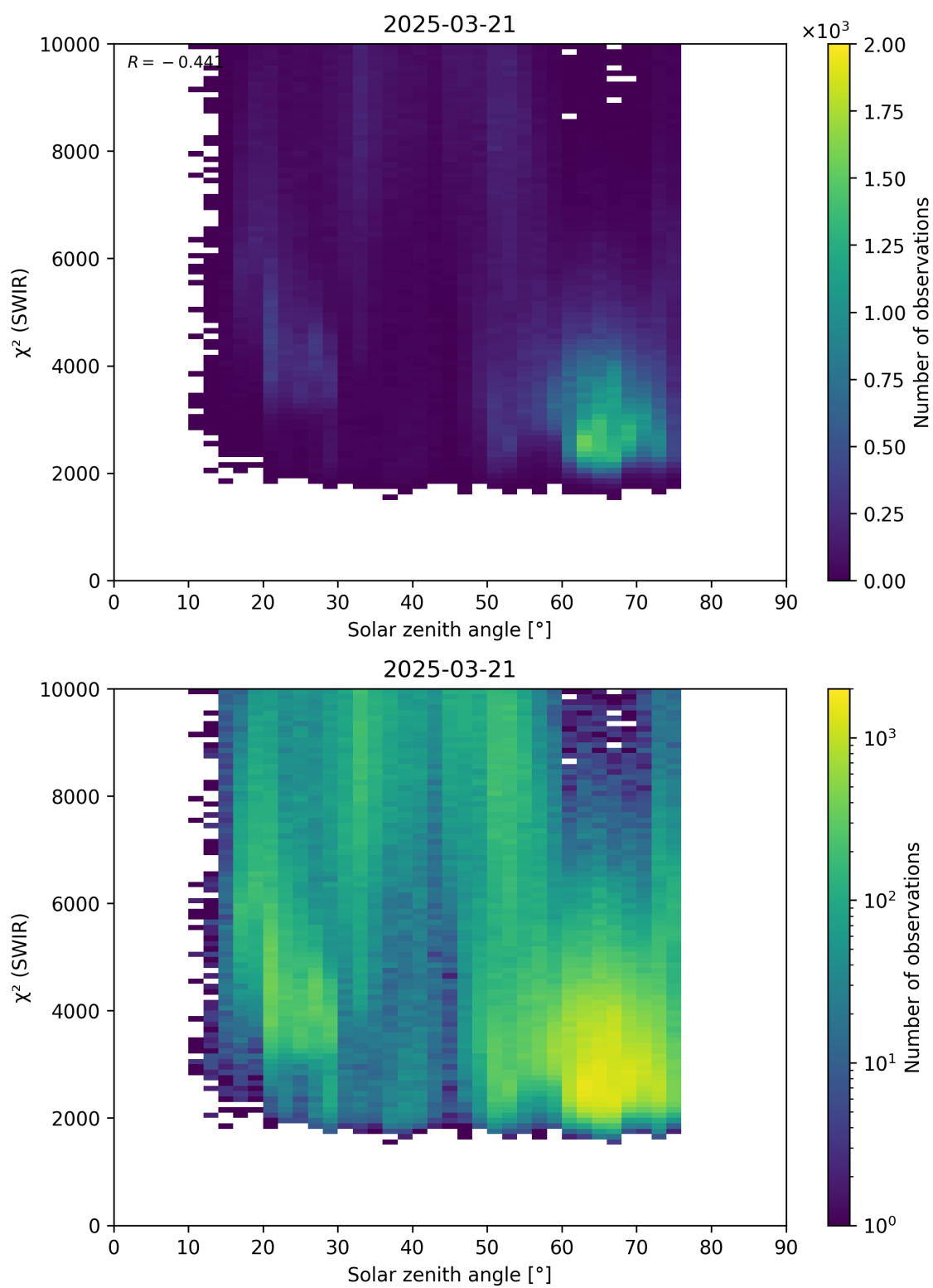
Figure 95: Scatter density plot of “Solar zenith angle” against “ \chi^2 (SWIR)” for 2025-03-20 to 2025-03-22.
