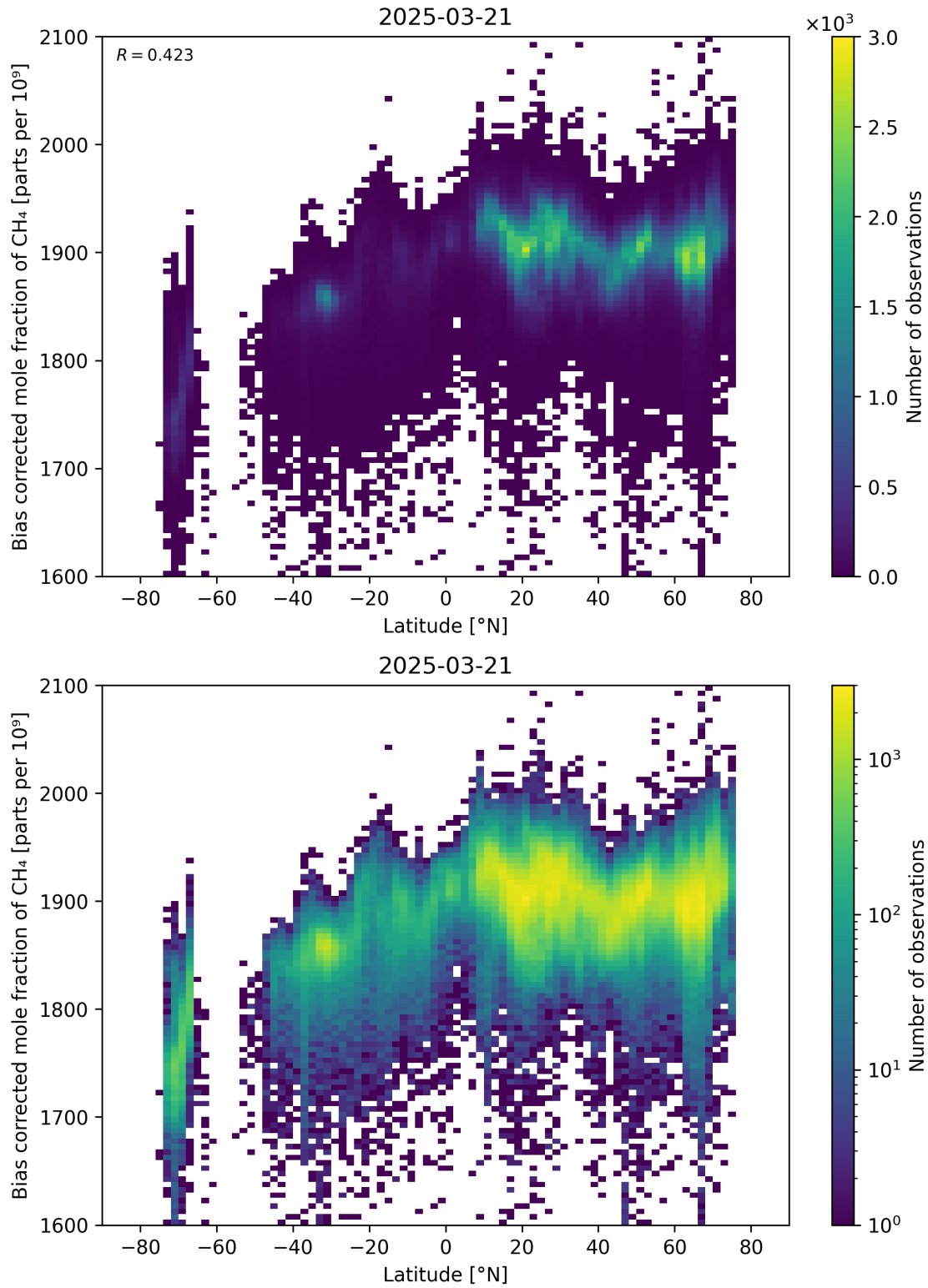
Figure 58: Scatter density plot of “Latitude” against “Bias corrected mole fraction of \text{CH}_4 ” for 2025-03-20 to 2025-03-22.
