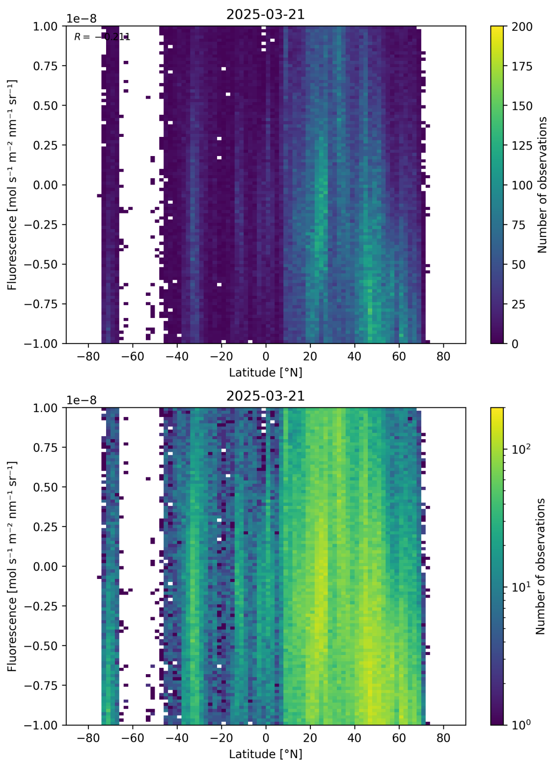
Figure 56: Scatter density plot of “Latitude” against “Fluorescence” for 2025-03-20 to 2025-03-22.
