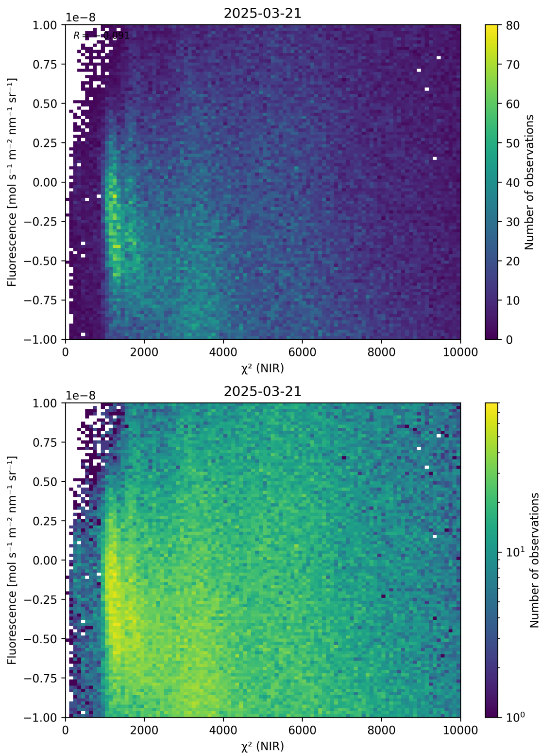
Figure 45: Scatter density plot of “ \chi^2 (NIR)” against “Fluorescence” for 2025-03-20 to 2025-03-22.
