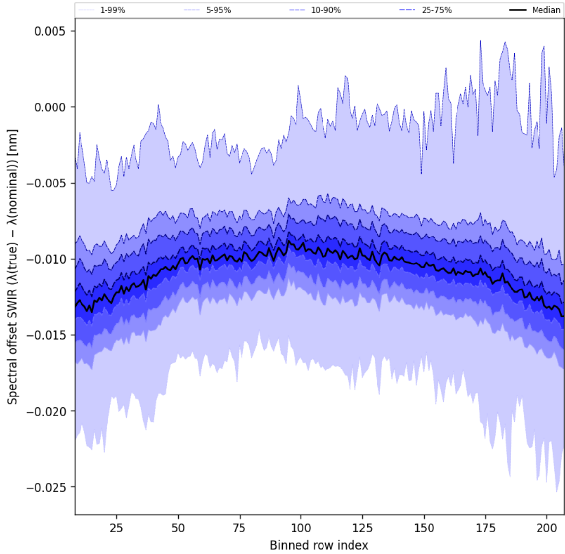
Figure 38: Along track statistics of “Spectral offset SWIR ( \lambda_{\text{true}} - \lambda_{\text{nominal}} )” for 2025-03-21 to 2025-03-23
