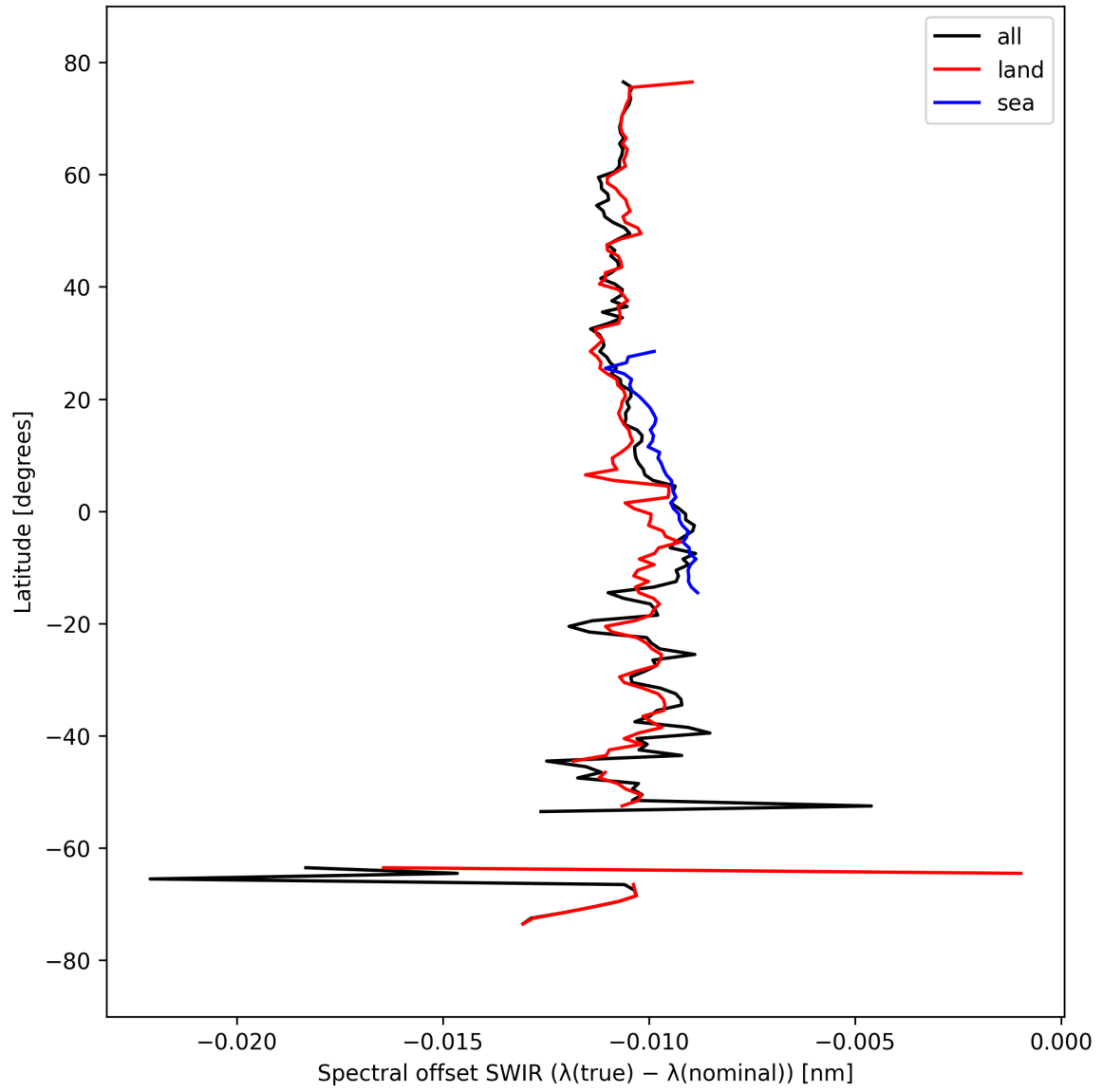
Figure 16: Zonal average of “Spectral offset SWIR ( \lambda_{\text{true}} - \lambda_{\text{nominal}} )” for 2025-03-21 to 2025-03-23.
