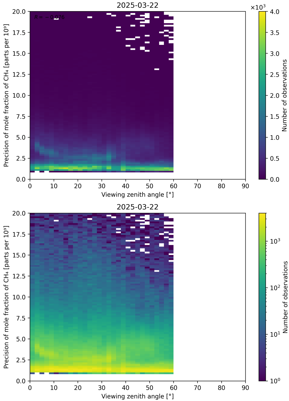
Figure 112: Scatter density plot of “Viewing zenith angle” against “Precision of mole fraction of CH 4 ” for 2025-03-21 to 2025-03-23.
