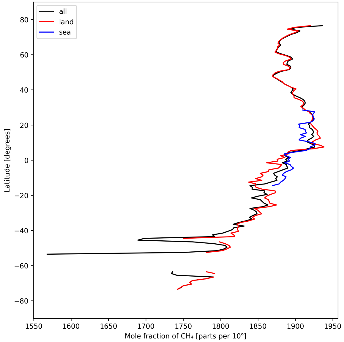
Figure 12: Zonal average of “Mole fraction of \text{CH}_4 ” for 2025-03-21 to 2025-03-23.
