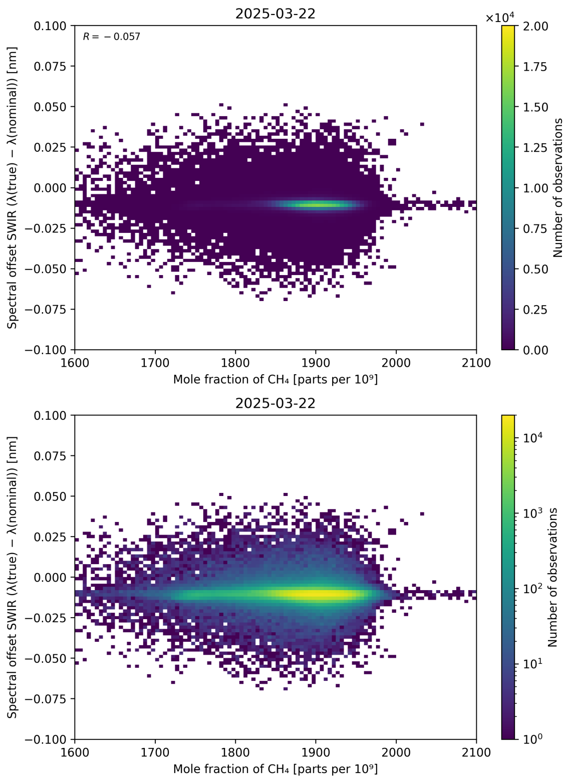
Figure 86: Scatter density plot of “Mole fraction of CH 4 ” against “Spectral offset SWIR ( \lambda_{\text{true}} - \lambda_{\text{nominal}} )” for 2025-03-21 to 2025-03-23.
