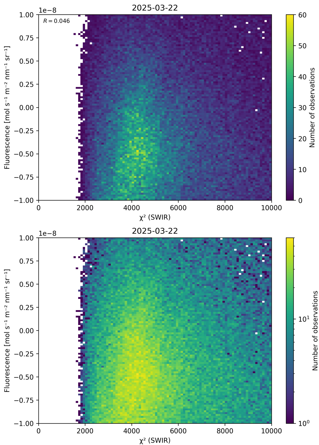
Figure 49: Scatter density plot of “ \chi^2 (SWIR)” against “Fluorescence” for 2025-03-21 to 2025-03-23.
