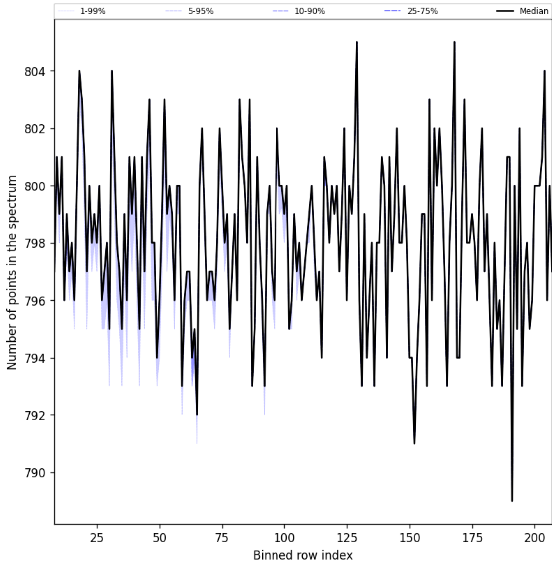
Figure 37: Along track statistics of “Number of points in the spectrum” for 2025-03-21 to 2025-03-23
