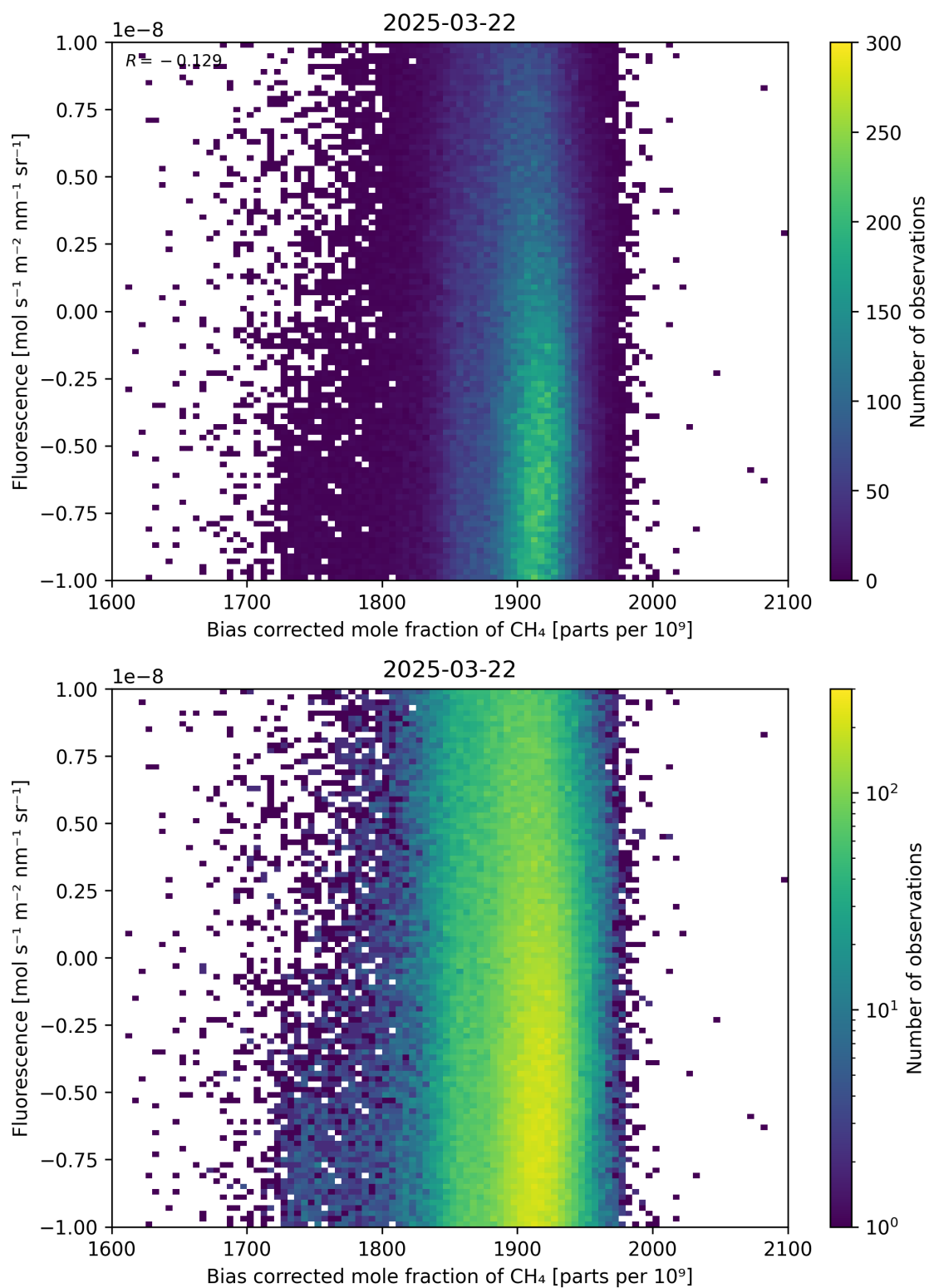
Figure 66: Scatter density plot of “Bias corrected mole fraction of CH 4 ” against “Fluorescence” for 2025-03-21 to 2025-03-23.
