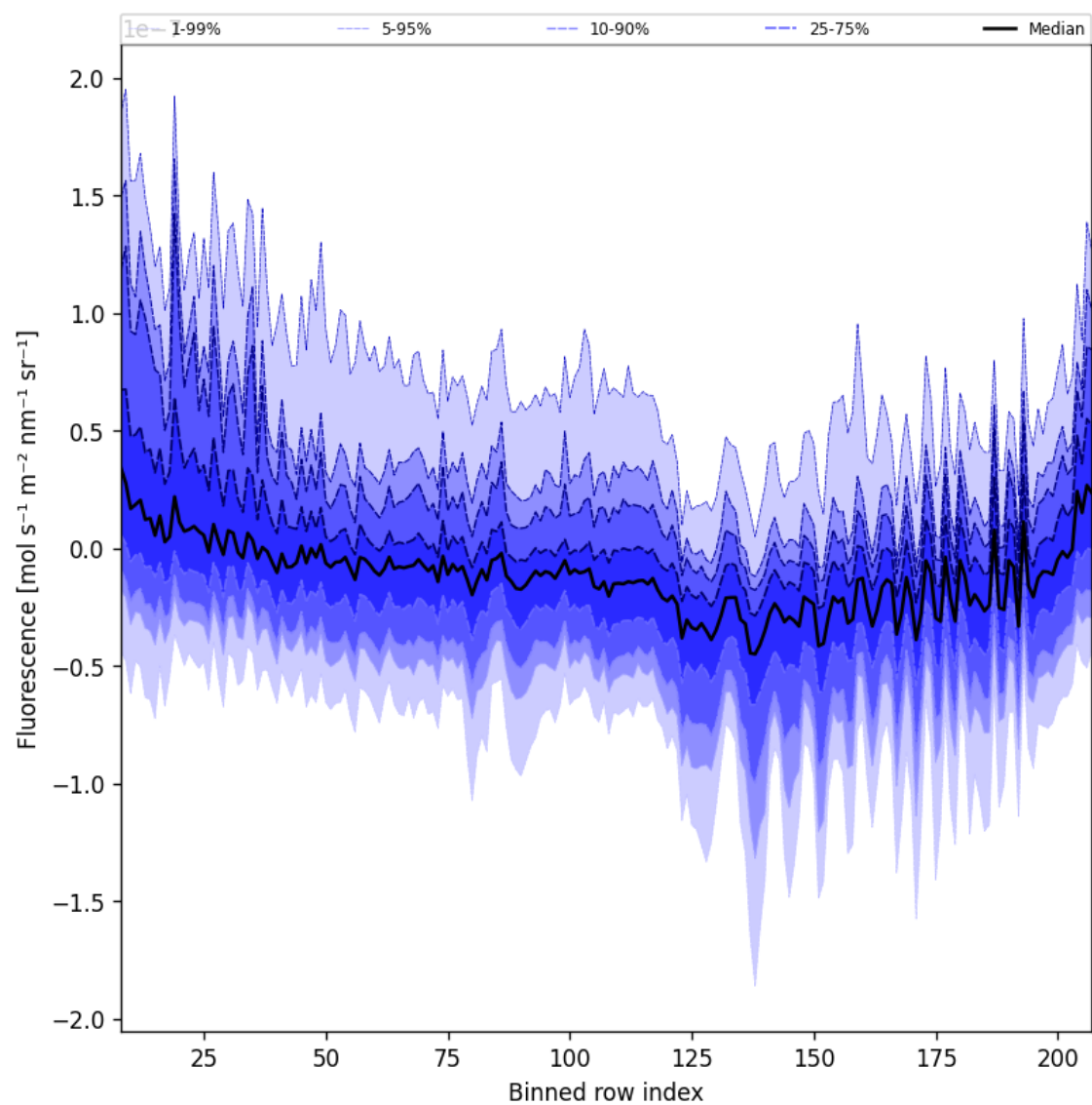
Figure 43: Along track statistics of “Fluorescence” for 2025-03-21 to 2025-03-23
