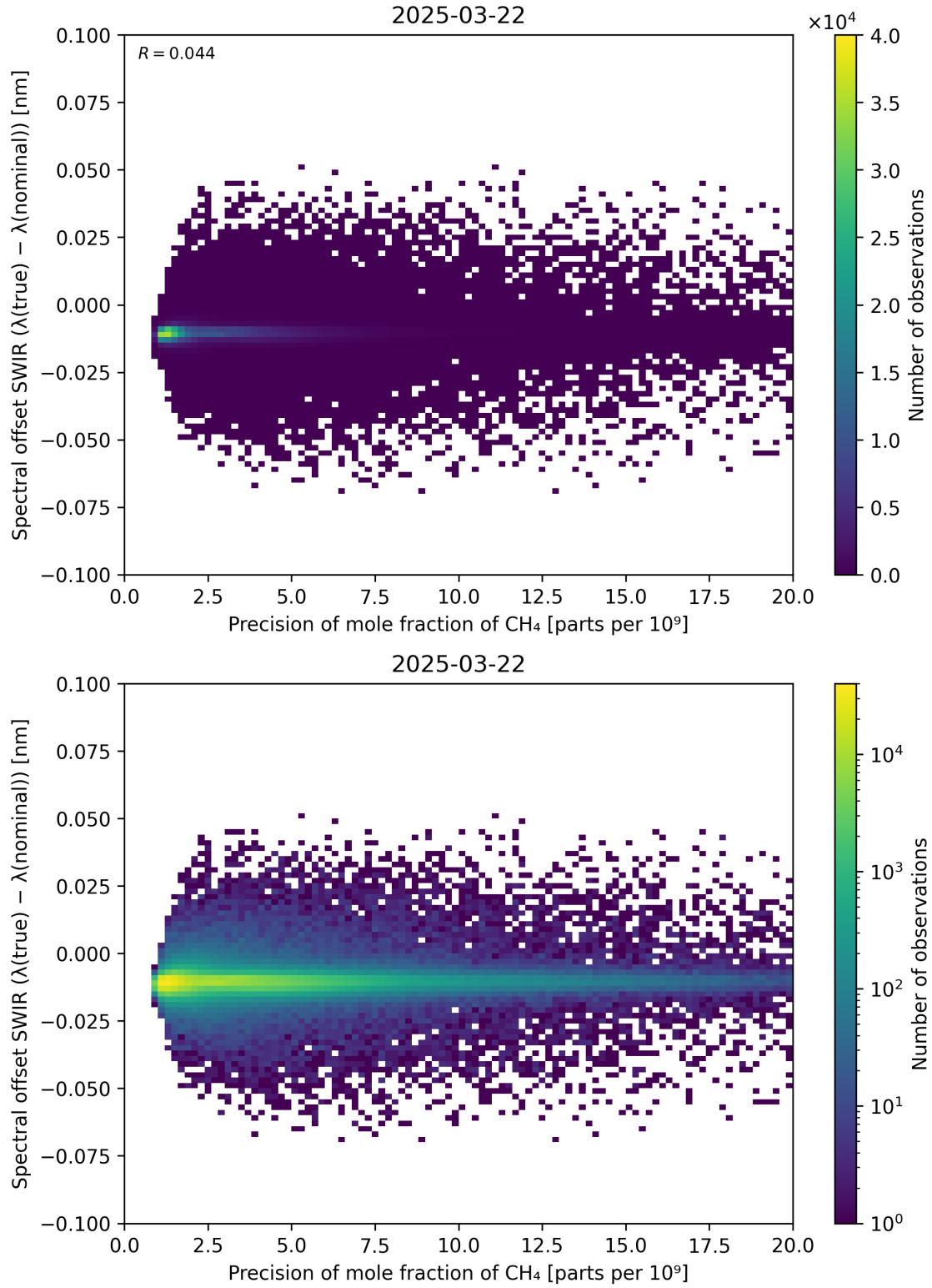
Figure 85: Scatter density plot of “Precision of mole fraction of CH 4 ” against “Spectral offset SWIR ( \lambda_{\text{true}} - \lambda_{\text{nominal}} )” for 2025-03-21 to 2025-03-23.
