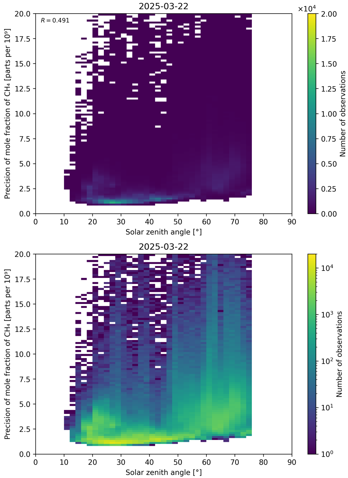
Figure 101: Scatter density plot of “Solar zenith angle” against “Precision of mole fraction of \text{CH}_4 ” for 2025-03-21 to 2025-03-23.
