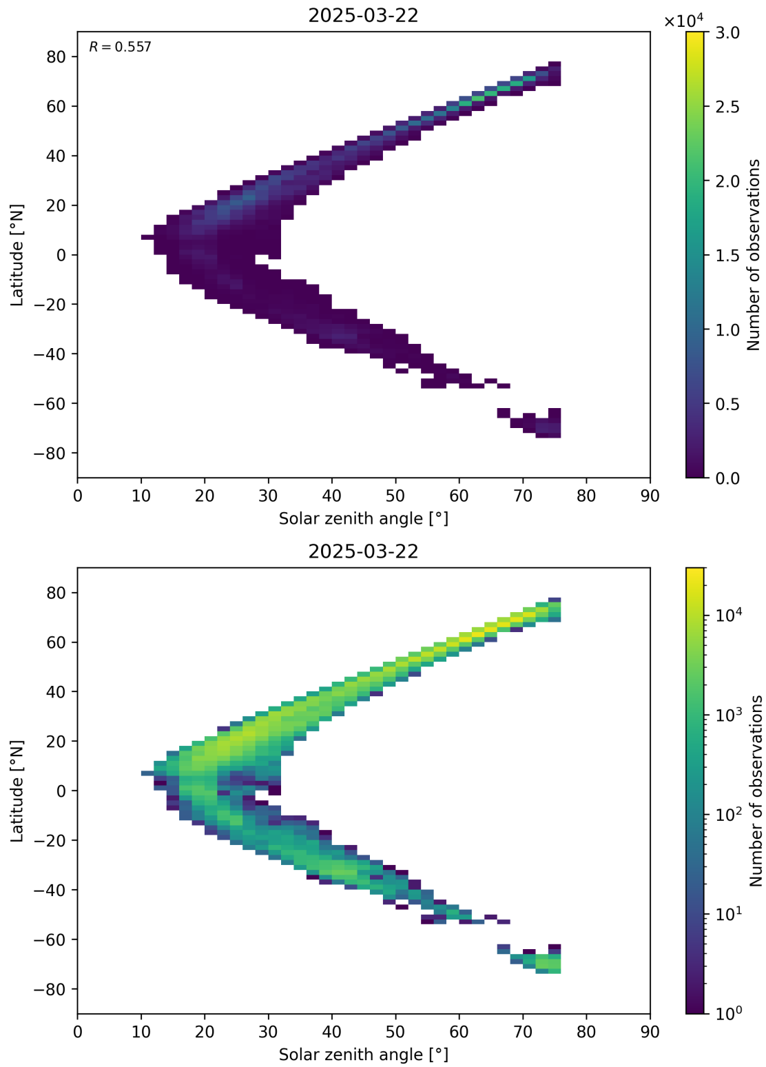
Figure 98: Scatter density plot of “Solar zenith angle” against “Latitude” for 2025-03-21 to 2025-03-23.
