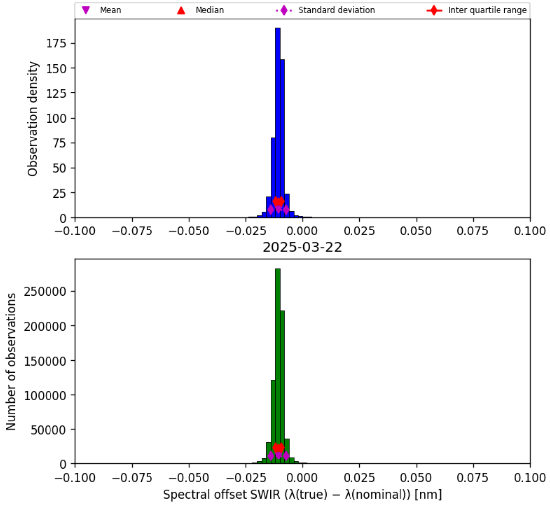
Figure 27: Histogram of “Spectral offset SWIR ( \lambda_{\text{true}} - \lambda_{\text{nominal}} )” for 2025-03-21 to 2025-03-23
