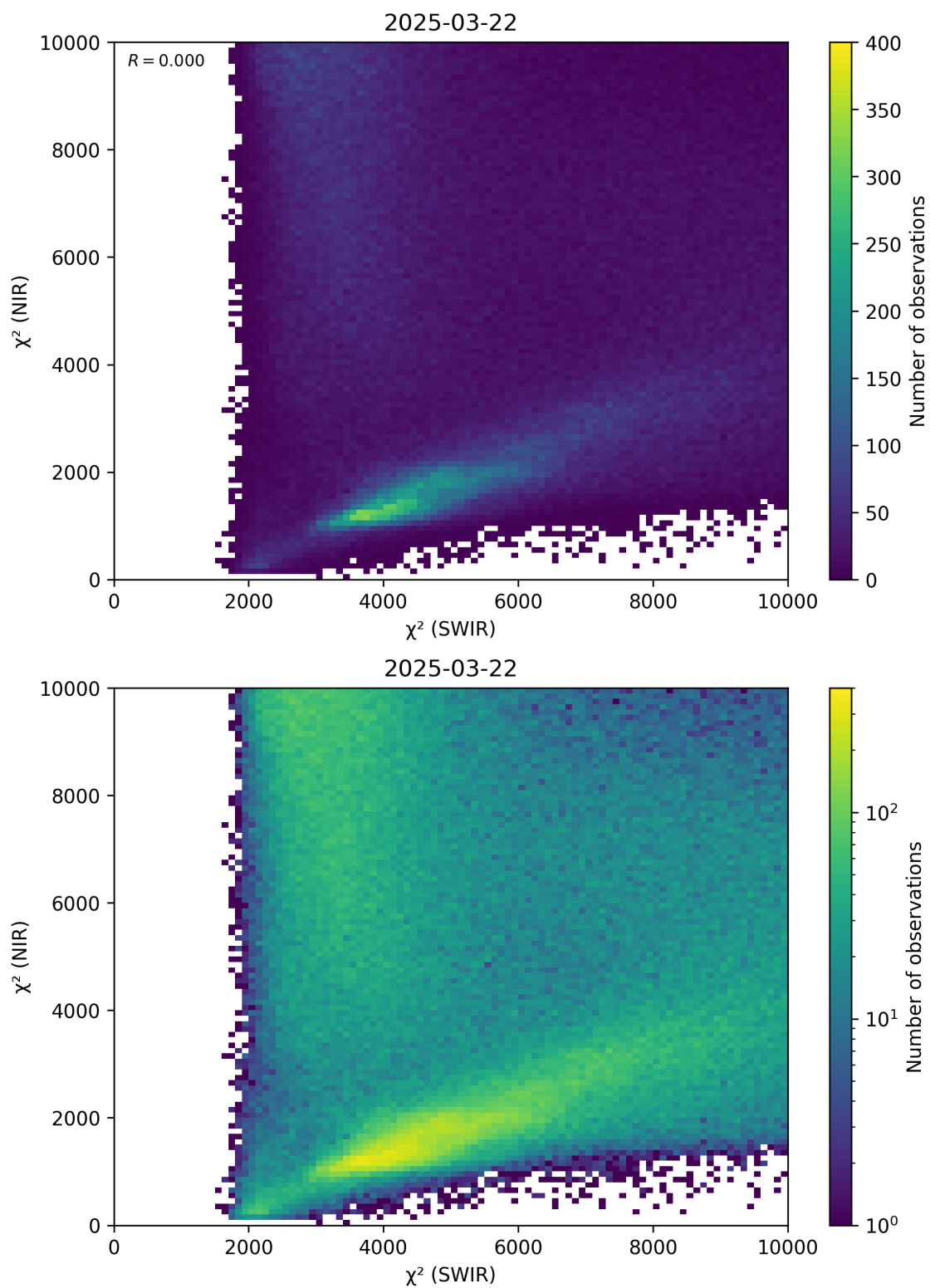
Figure 47: Scatter density plot of “ \chi^2 (SWIR)” against “ \chi^2 (NIR)” for 2025-03-21 to 2025-03-23.
