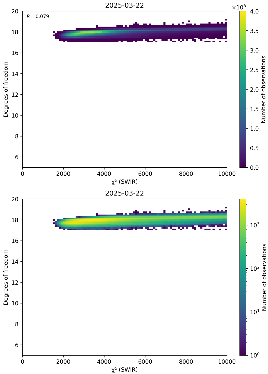
Figure 48: Scatter density plot of “ \chi^2 (SWIR)” against “Degrees of freedom” for 2025-03-21 to 2025-03-23.
