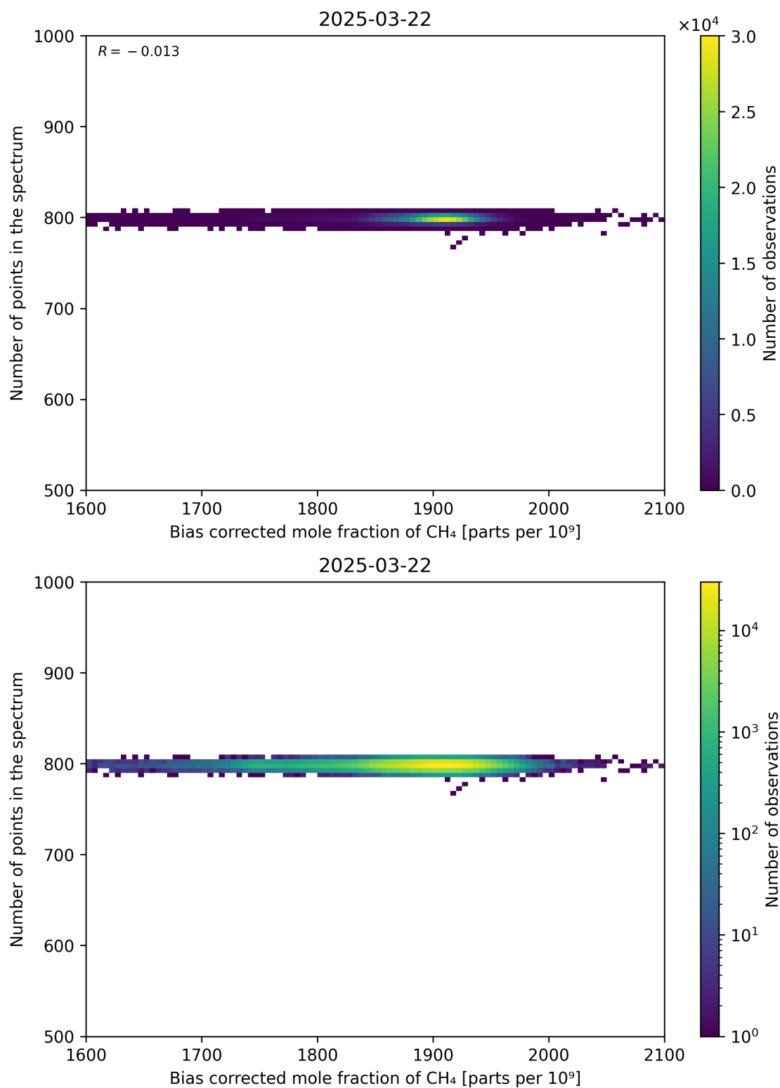
Figure 68: Scatter density plot of “Bias corrected mole fraction of CH 4 ” against “Number of points in the spectrum” for 2025-03-21 to 2025-03-23.
