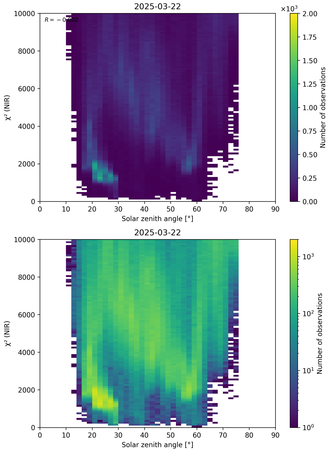
Figure 94: Scatter density plot of “Solar zenith angle” against “ \chi^2 (NIR)” for 2025-03-21 to 2025-03-23.
