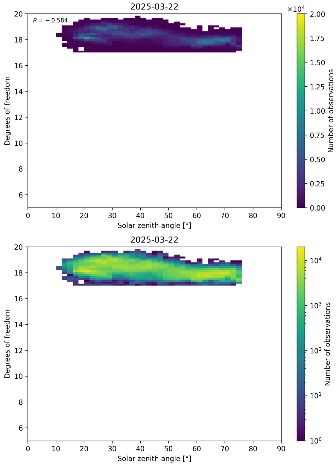
Figure 96: Scatter density plot of “Solar zenith angle” against “Degrees of freedom” for 2025-03-21 to 2025-03-23.
