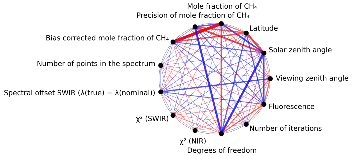
Figure 1: Map of correlation graph for 2025-03-21 to 2025-03-23.
