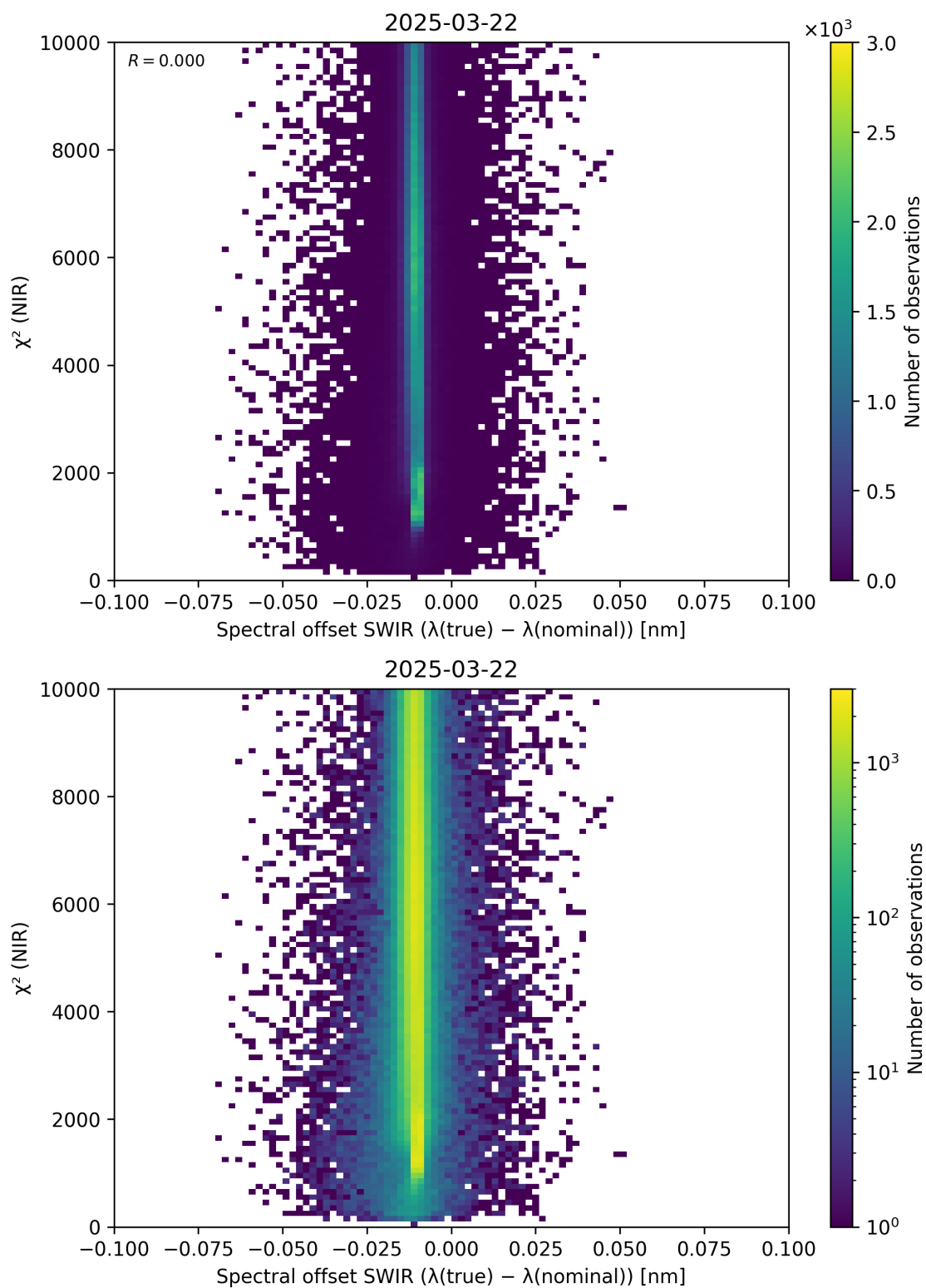
Figure 117: Scatter density plot of “Spectral offset SWIR ( \lambda_{\text{true}} - \lambda_{\text{nominal}} )” against “ \chi^2 (NIR)” for 2025-03-21 to 2025-03-23.
