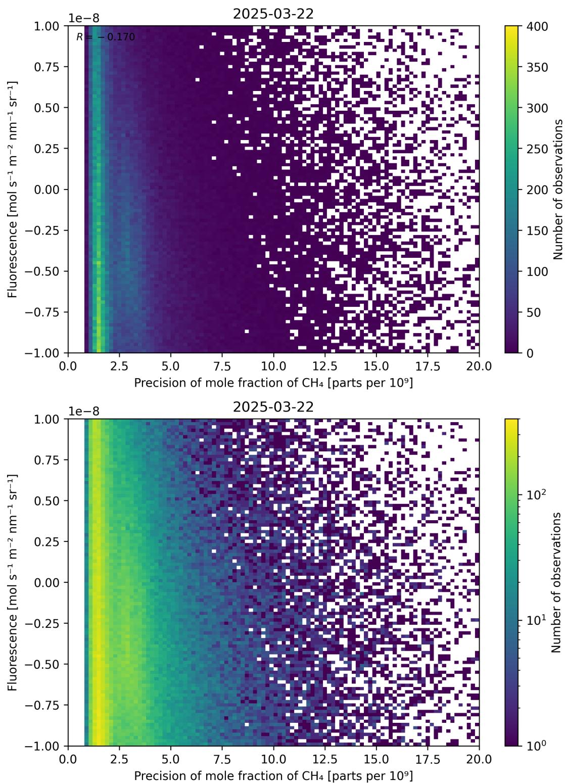
Figure 81: Scatter density plot of “Precision of mole fraction of \text{CH}_4 ” against “Fluorescence” for 2025-03-21 to 2025-03-23.
