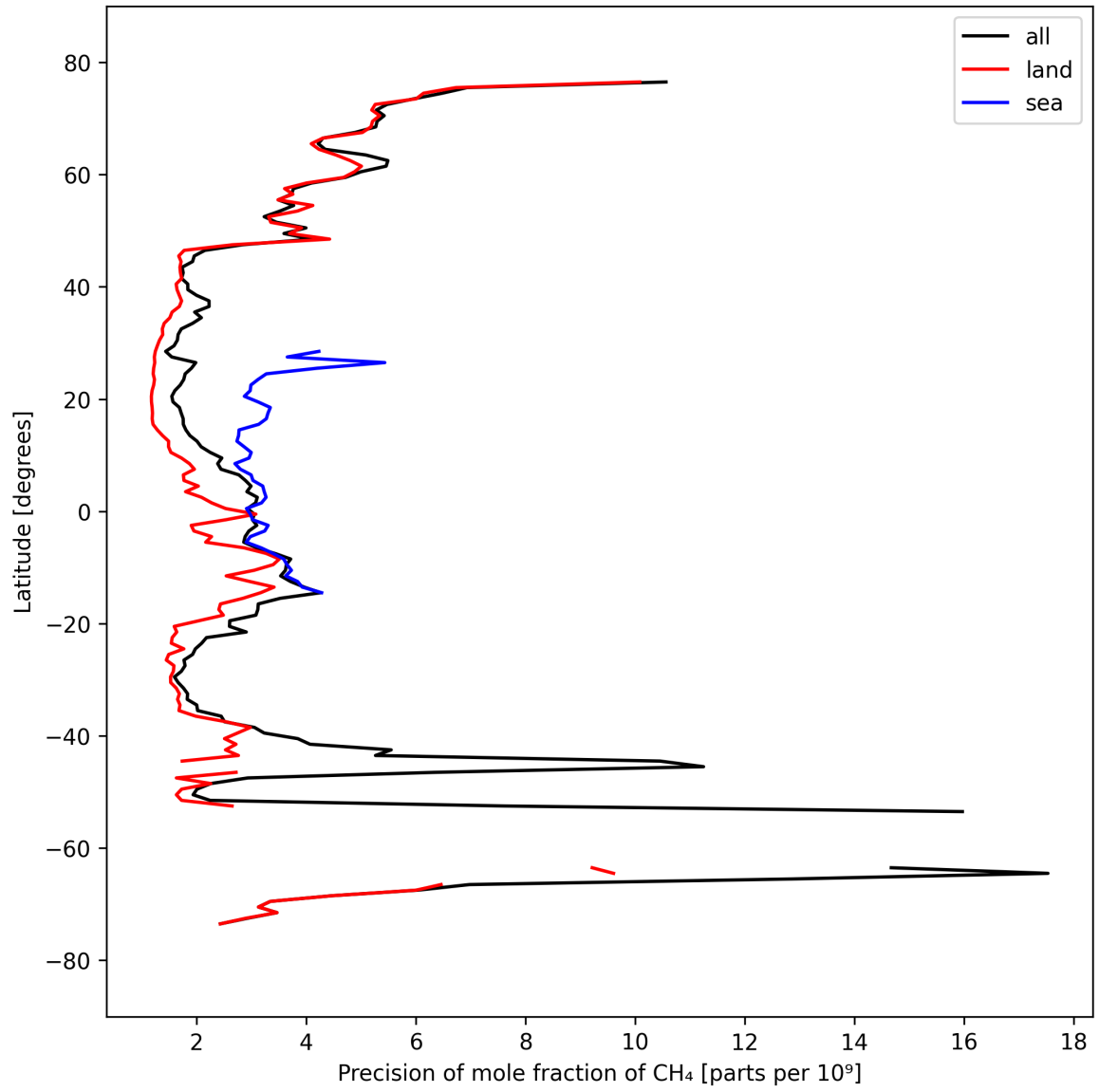
Figure 13: Zonal average of “Precision of mole fraction of CH 4 ” for 2025-03-21 to 2025-03-23.
