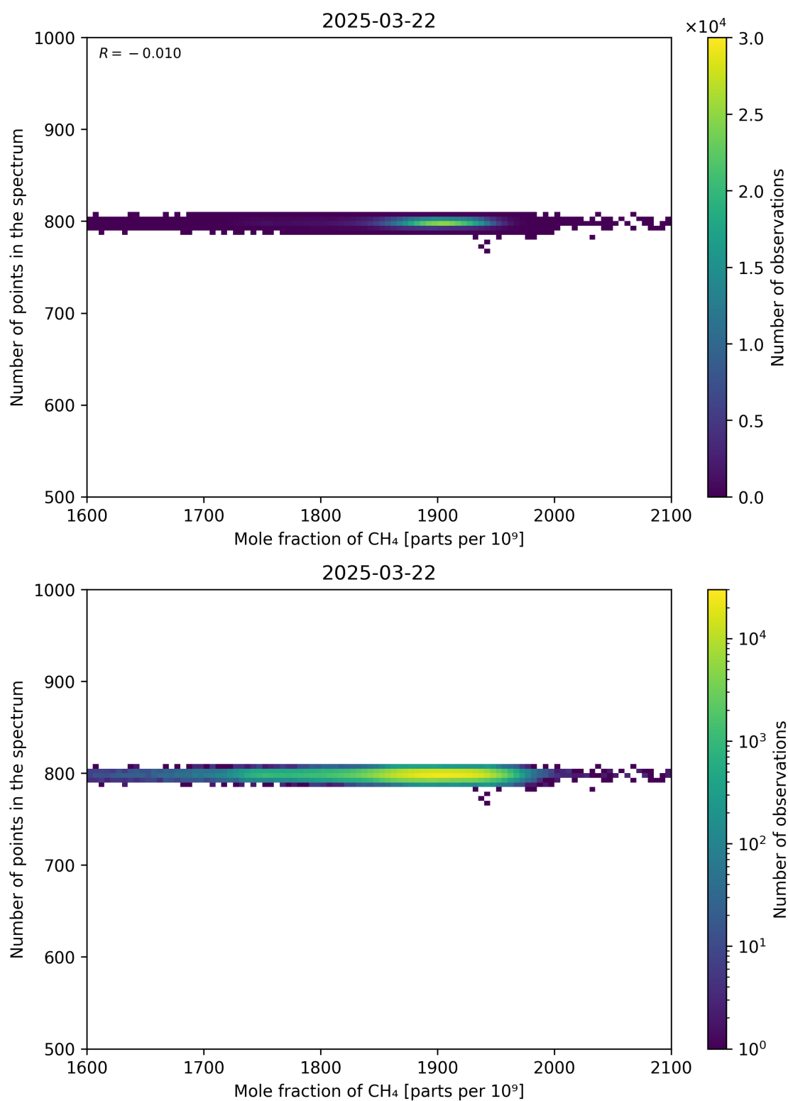
Figure 77: Scatter density plot of “Mole fraction of CH 4 ” against “Number of points in the spectrum” for 2025-03-21 to 2025-03-23.
