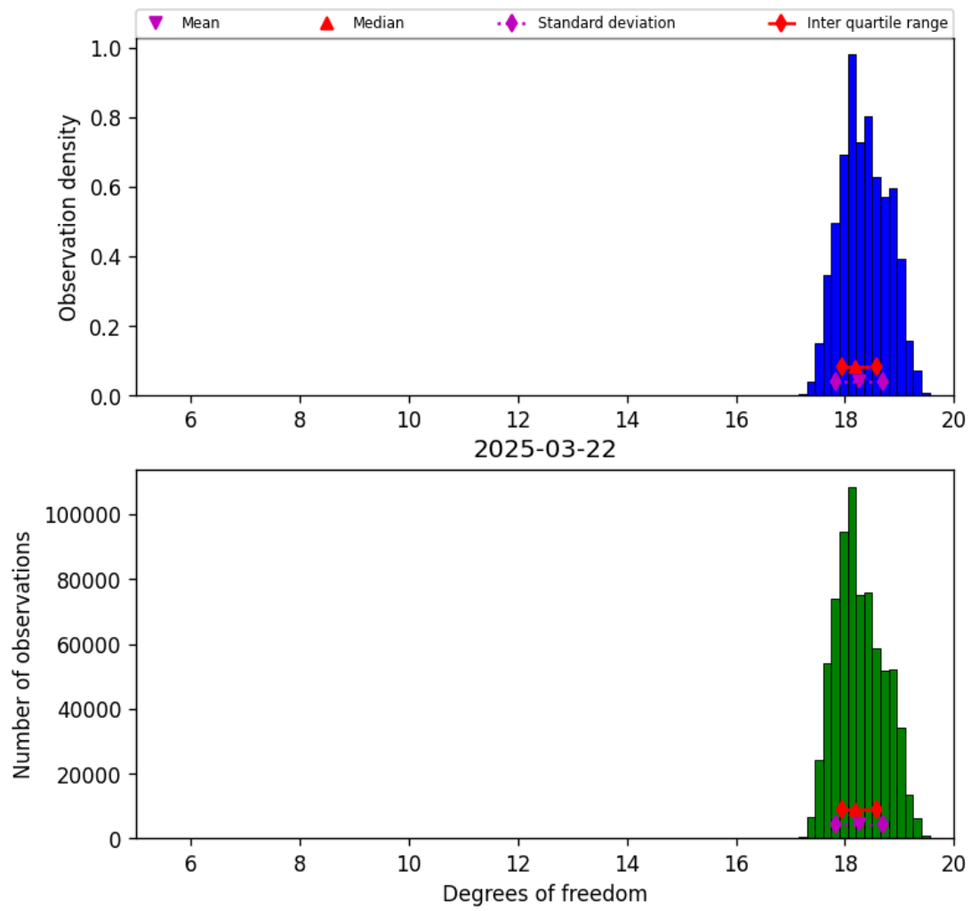
Figure 30: Histogram of “Degrees of freedom” for 2025-03-21 to 2025-03-23
