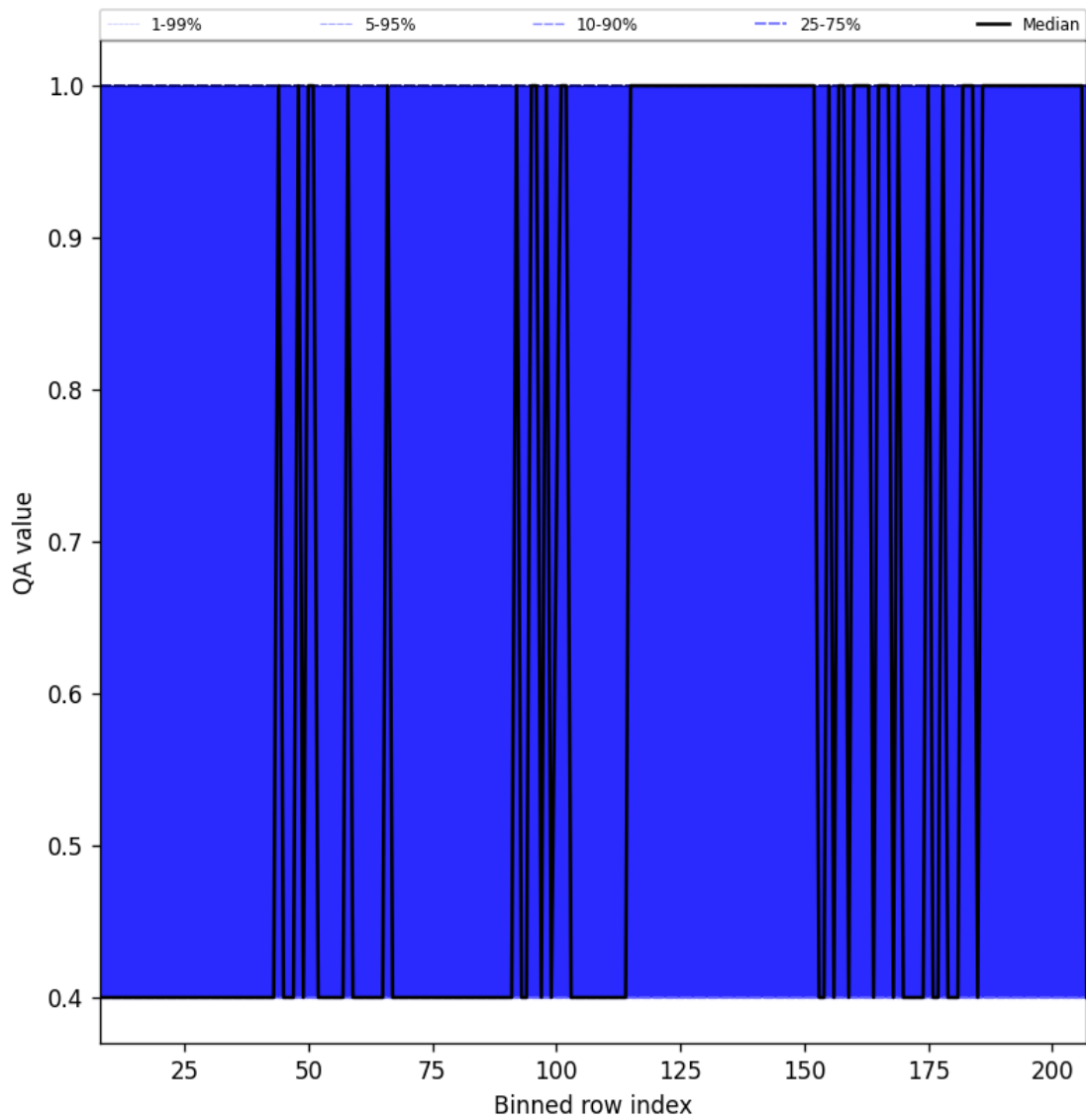
Figure 33: Along track statistics of “QA value” for 2025-03-21 to 2025-03-23
