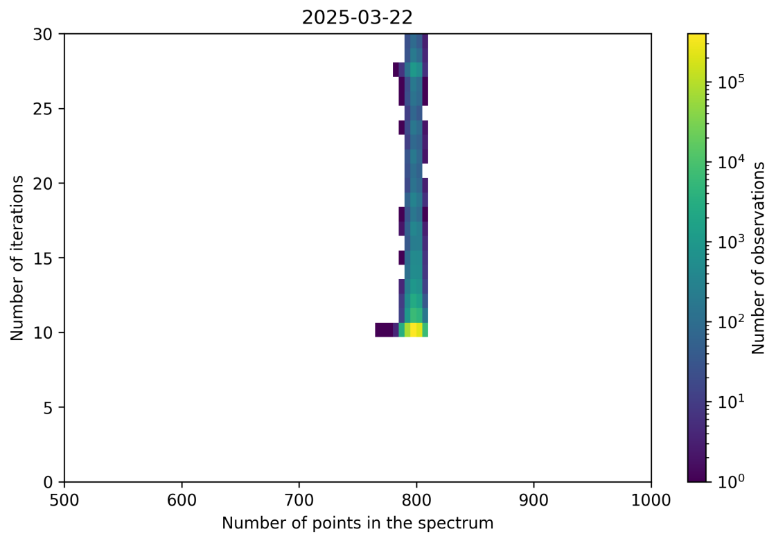
Figure 92: Scatter density plot of “Number of points in the spectrum” against “Number of iterations” for 2025-03-21 to 2025-03-23.
