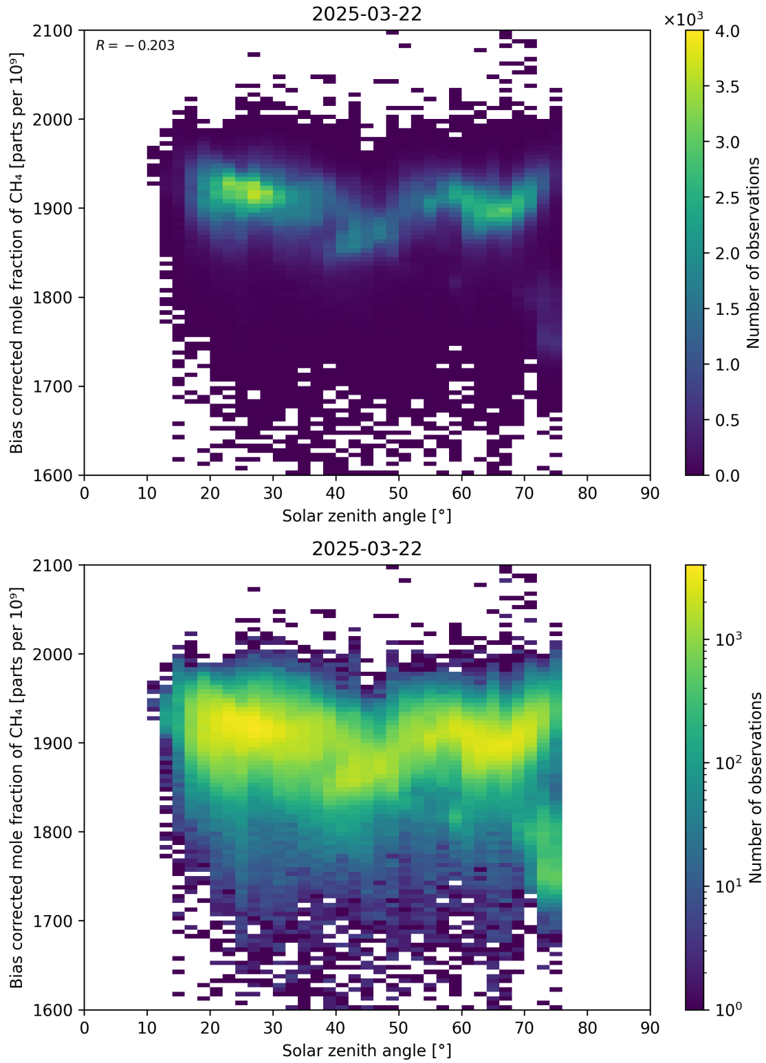
Figure 100: Scatter density plot of “Solar zenith angle” against “Bias corrected mole fraction of CH 4 ” for 2025-03-21 to 2025-03-23.
