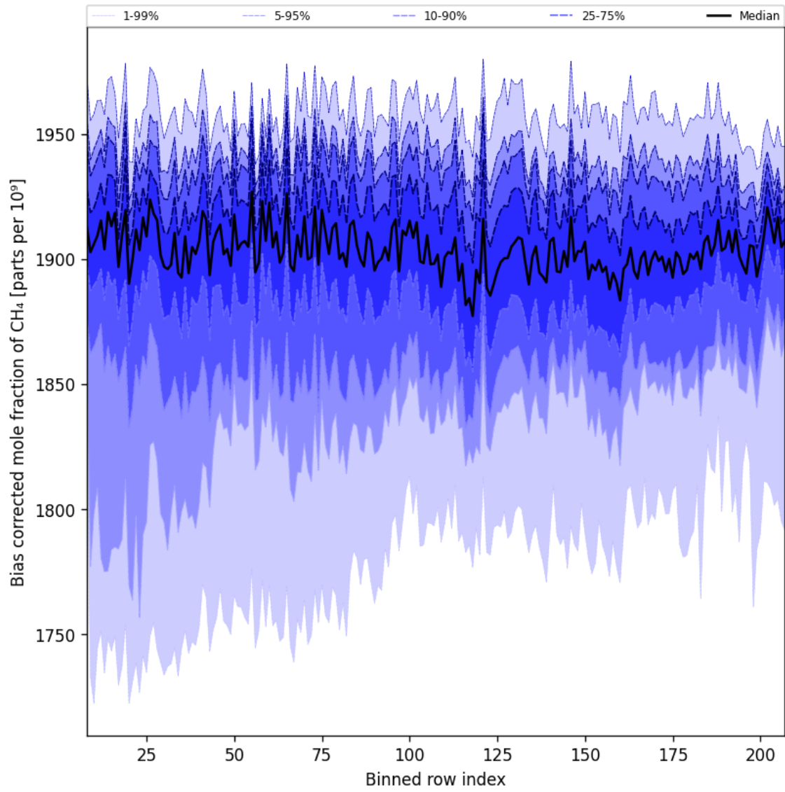
Figure 36: Along track statistics of “Bias corrected mole fraction of CH 4 ” for 2025-03-21 to 2025-03-23
