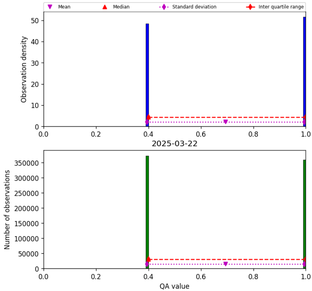
Figure 22: Histogram of “QA value” for 2025-03-21 to 2025-03-23
