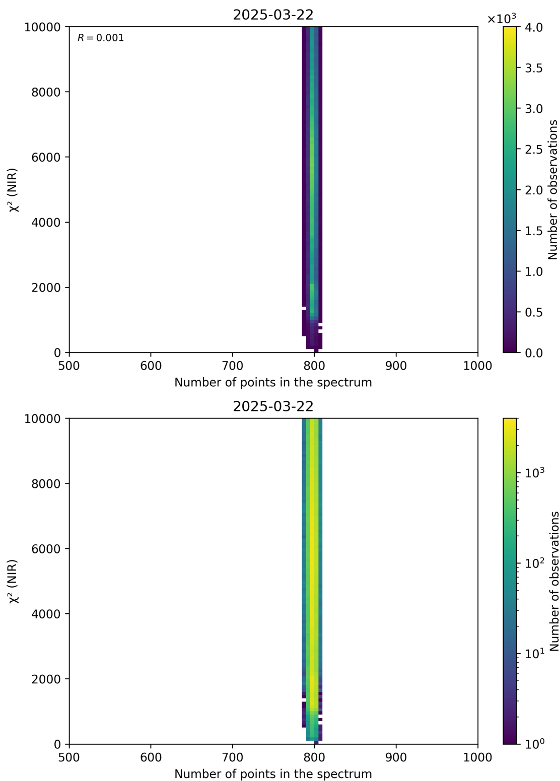
Figure 88: Scatter density plot of “Number of points in the spectrum” against “ \chi^2 (NIR)” for 2025-03-21 to 2025-03-23.
