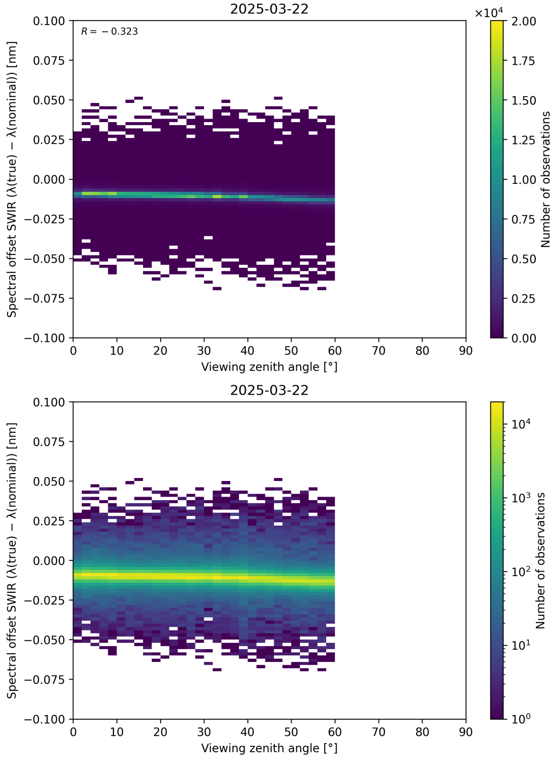
Figure 116: Scatter density plot of “Viewing zenith angle” against “Spectral offset SWIR ( \lambda_{\text{true}} - \lambda_{\text{nominal}} )” for 2025-03-21 to 2025-03-23.
