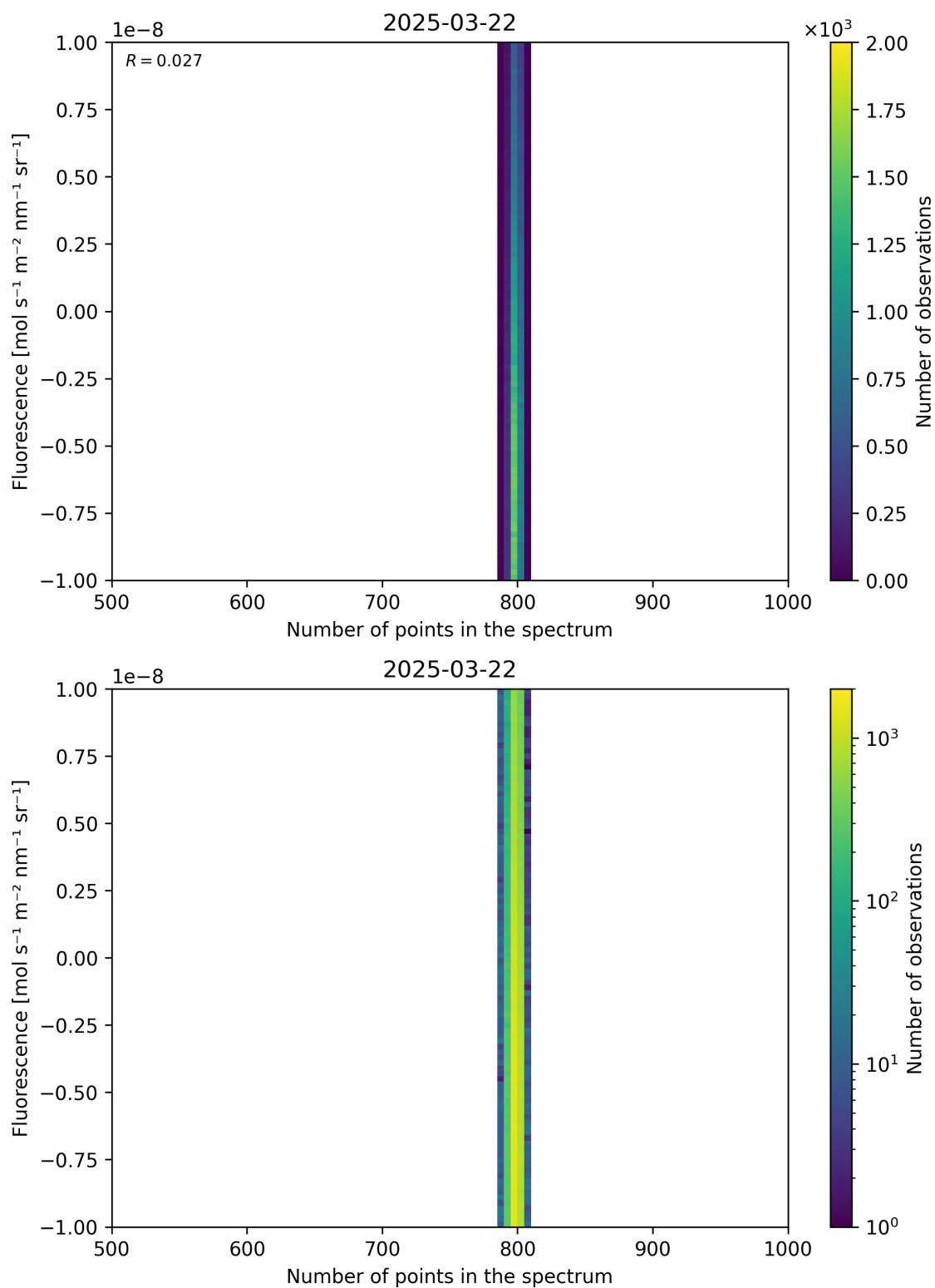
Figure 91: Scatter density plot of “Number of points in the spectrum” against “Fluorescence” for 2025-03-21 to 2025-03-23.
