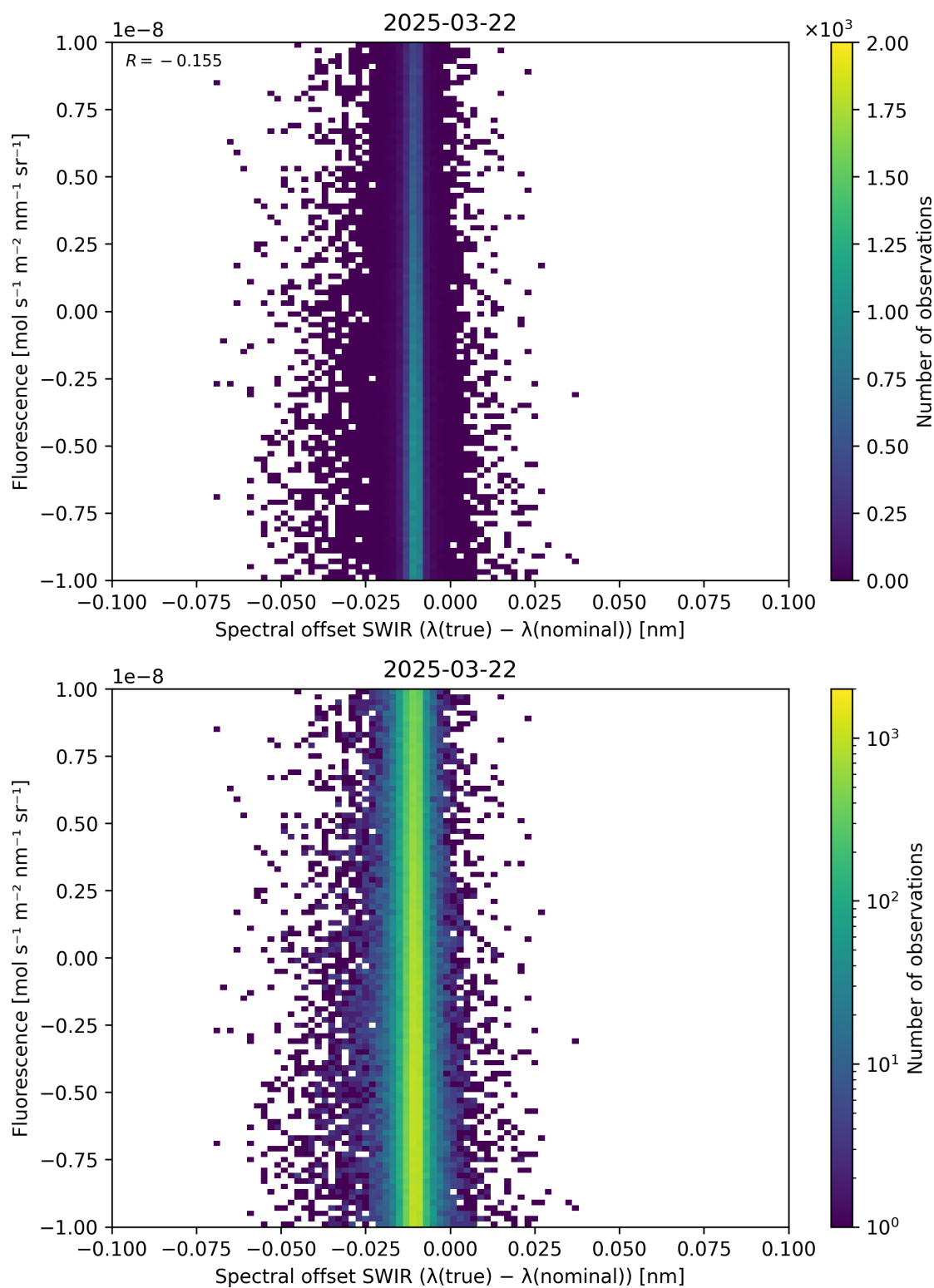
Figure 120: Scatter density plot of “Spectral offset SWIR ( \lambda_{\text{true}} - \lambda_{\text{nominal}} )” against “Fluorescence” for 2025-03-21 to 2025-03-23.
