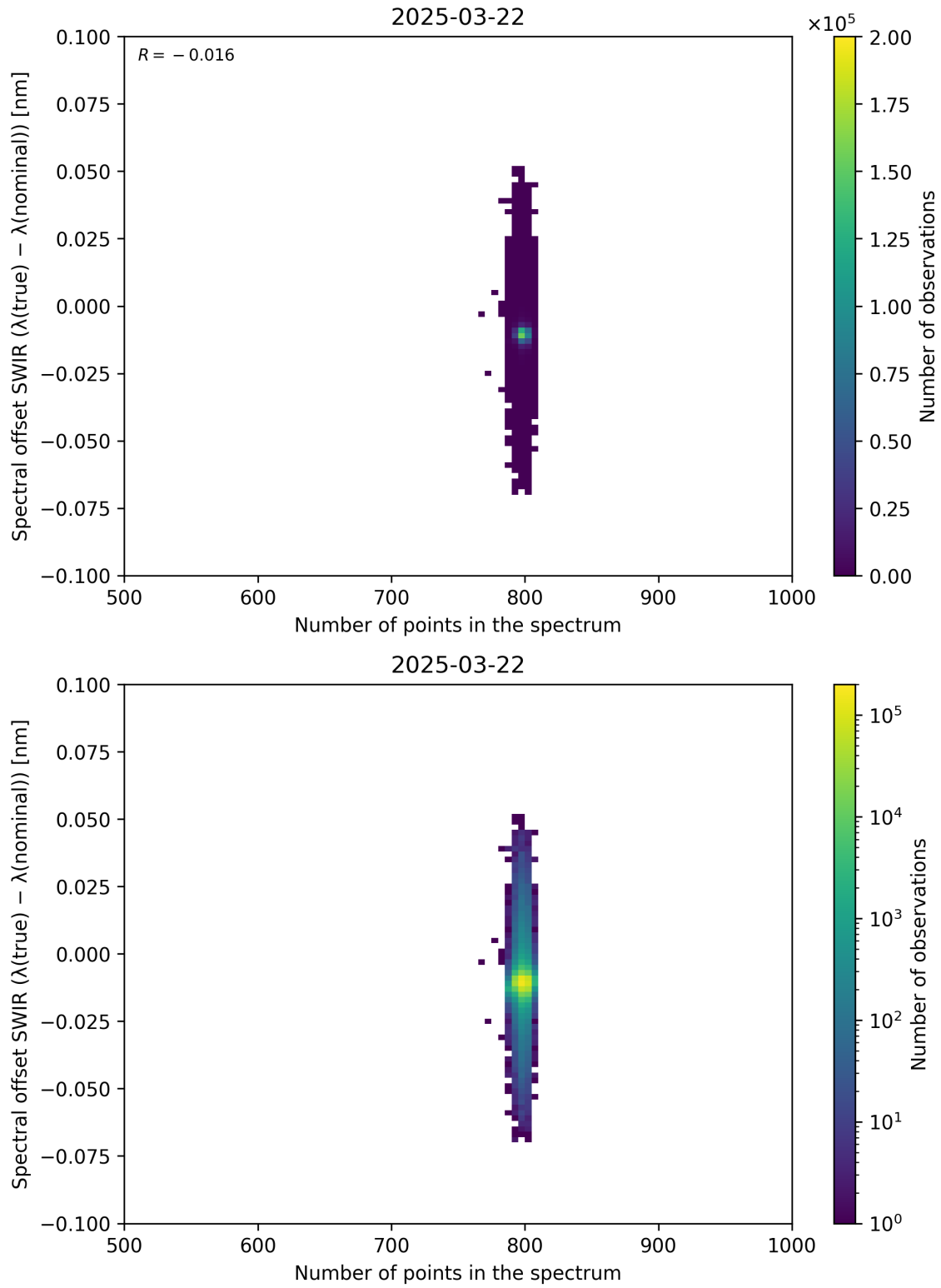
Figure 93: Scatter density plot of “Number of points in the spectrum” against “Spectral offset SWIR ( \lambda_{\text{true}} - \lambda_{\text{nominal}} )” for 2025-03-21 to 2025-03-23.
