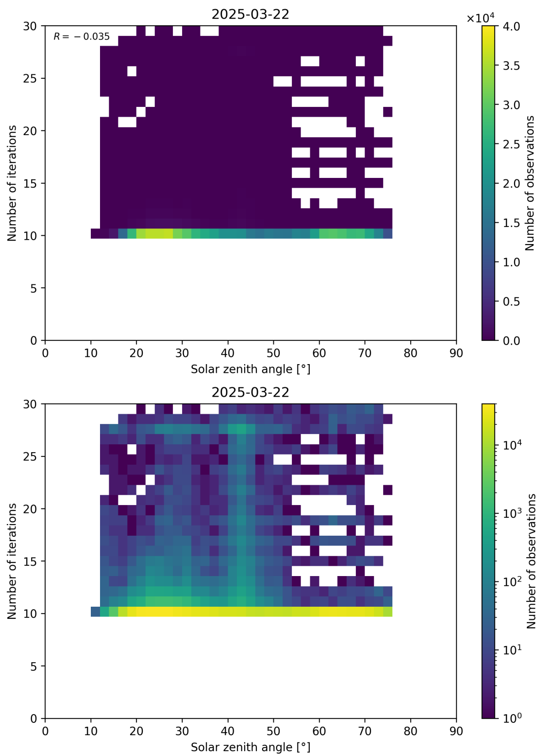
Figure 102: Scatter density plot of “Solar zenith angle” against “Number of iterations” for 2025-03-21 to 2025-03-23.
