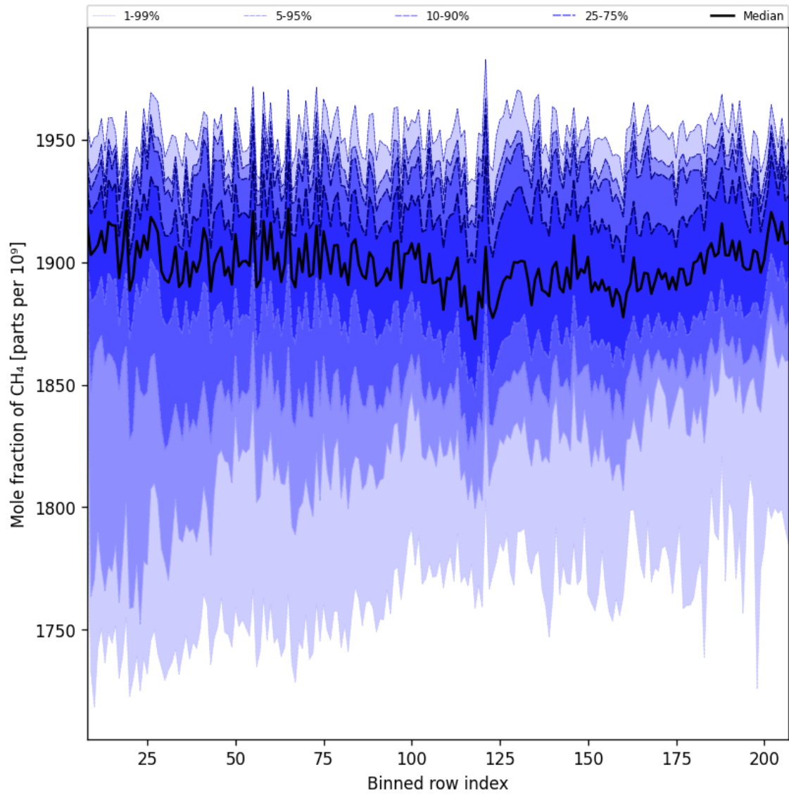
Figure 34: Along track statistics of “Mole fraction of CH 4 ” for 2025-03-21 to 2025-03-23
