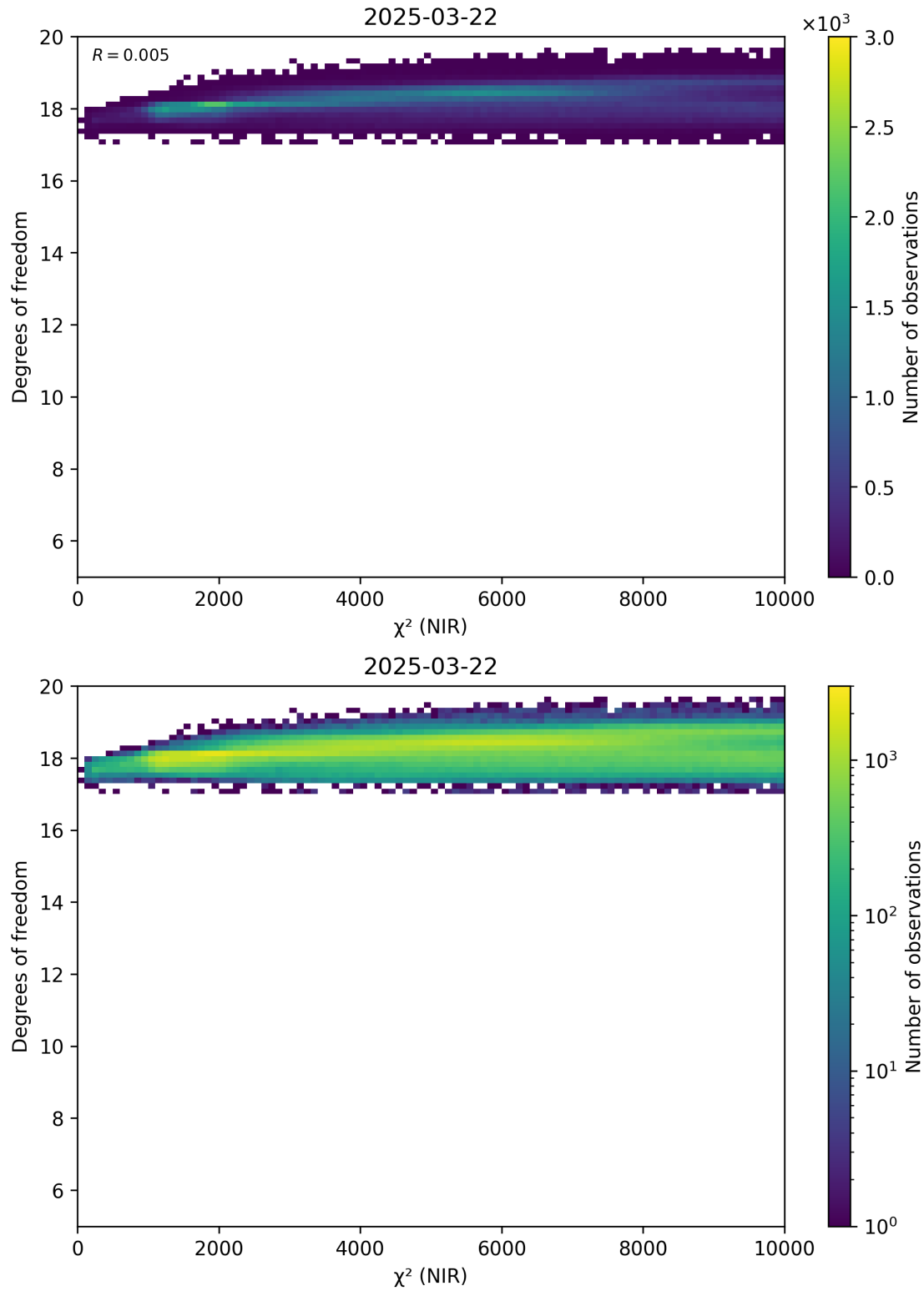
Figure 44: Scatter density plot of “ \chi^2 (NIR)” against “Degrees of freedom” for 2025-03-21 to 2025-03-23.
