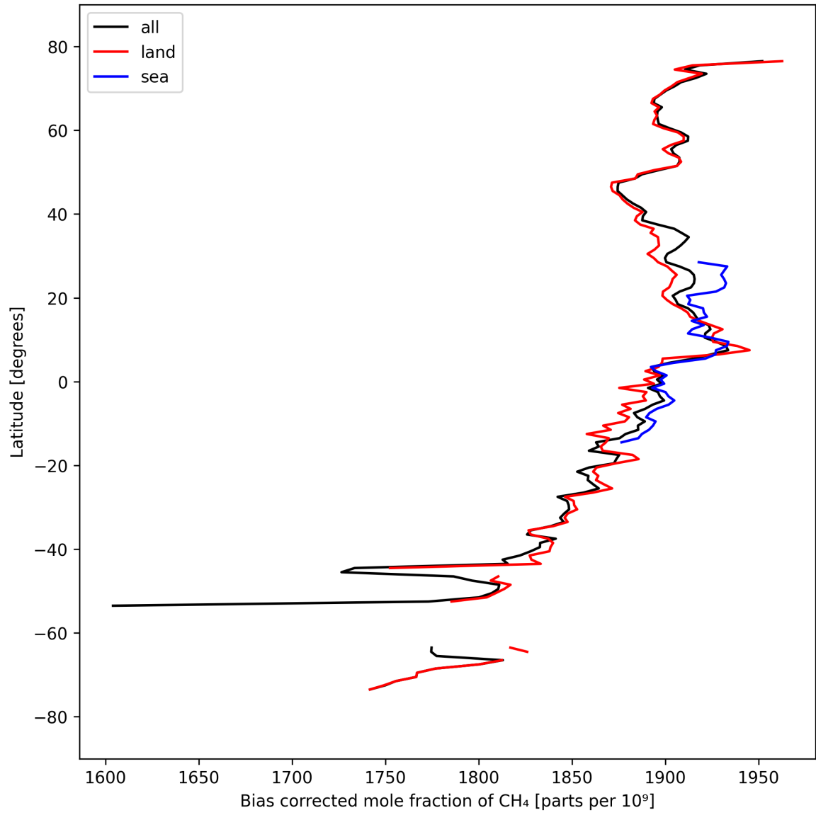
Figure 14: Zonal average of “Bias corrected mole fraction of CH 4 ” for 2025-03-21 to 2025-03-23.
