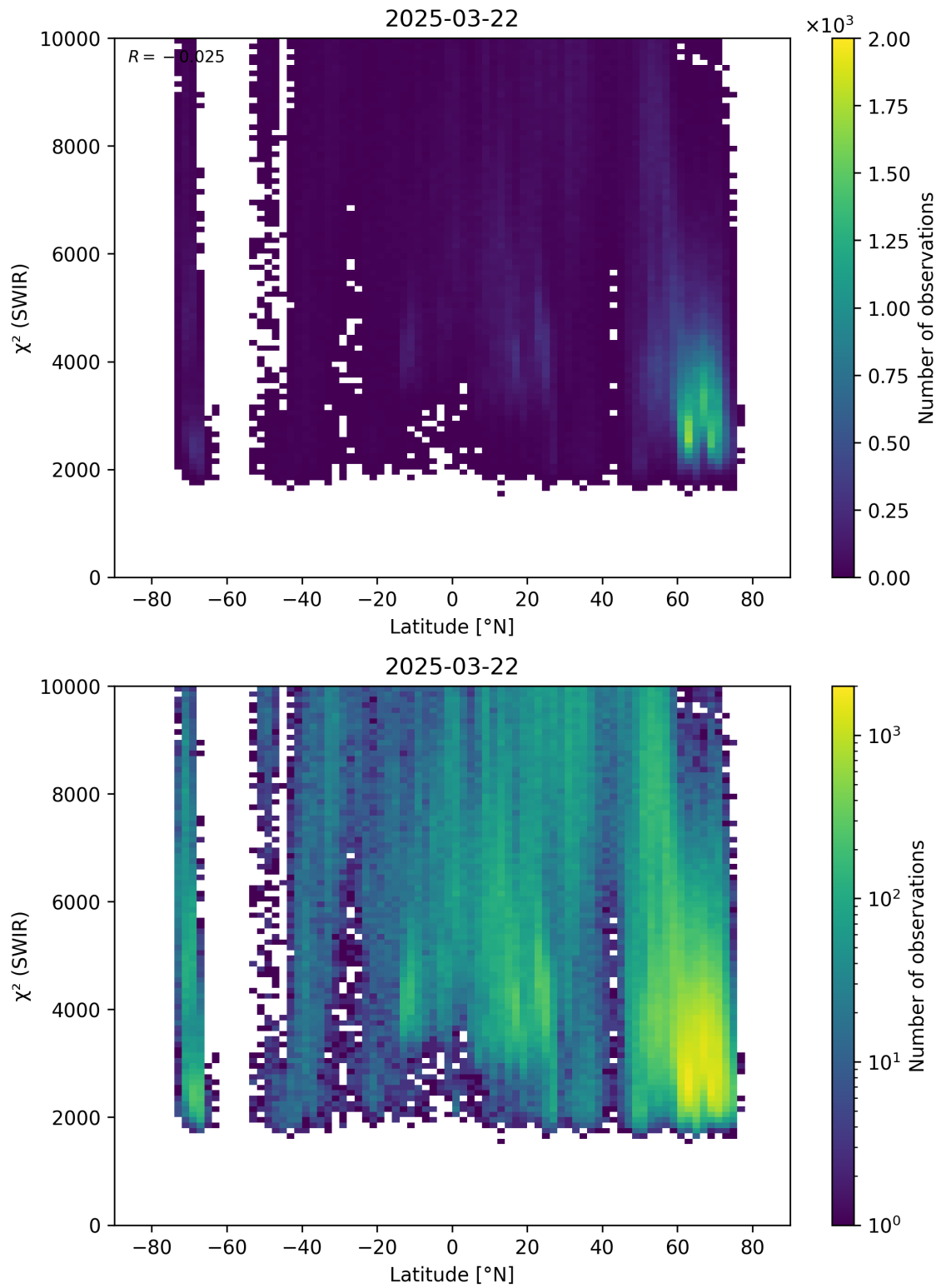
Figure 54: Scatter density plot of “Latitude” against “ \chi^2 (SWIR)” for 2025-03-21 to 2025-03-23.
