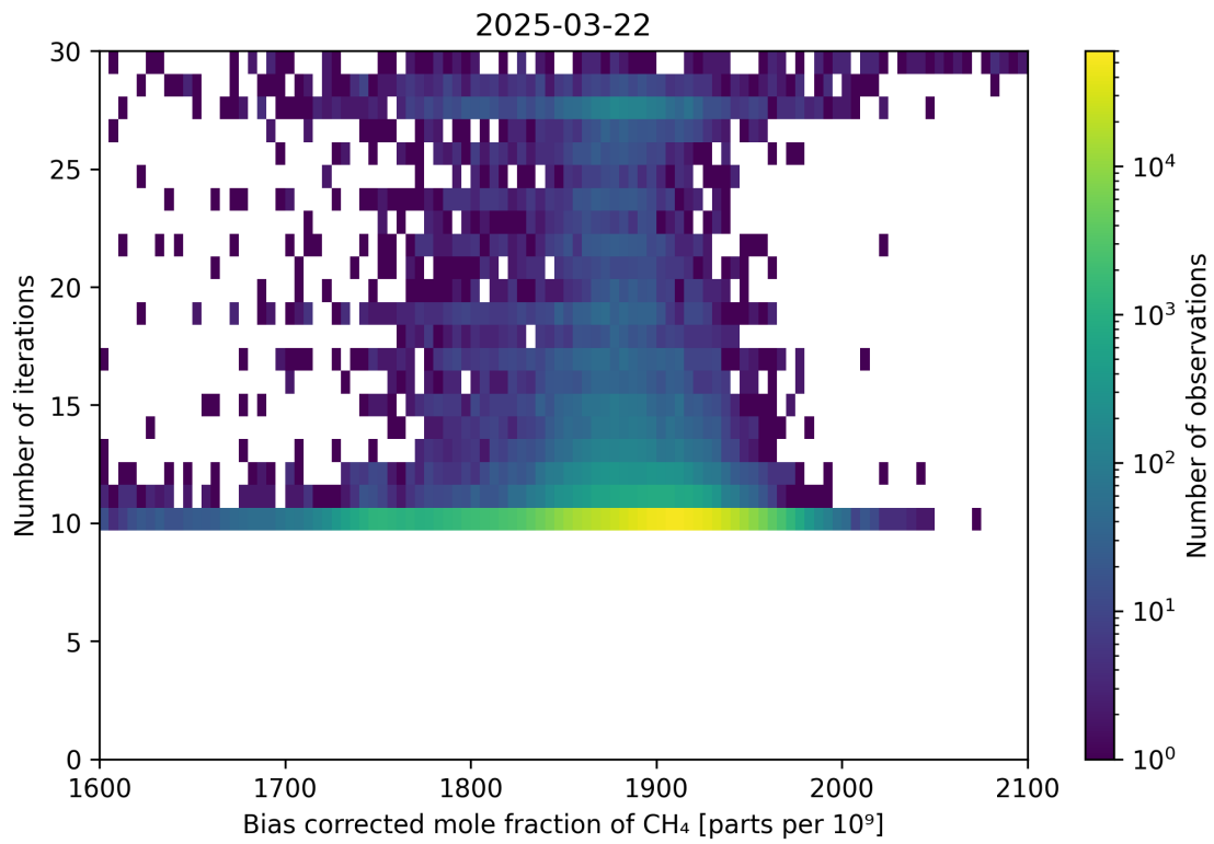
Figure 67: Scatter density plot of “Bias corrected mole fraction of CH 4 ” against “Number of iterations” for 2025-03-21 to 2025-03-23.
