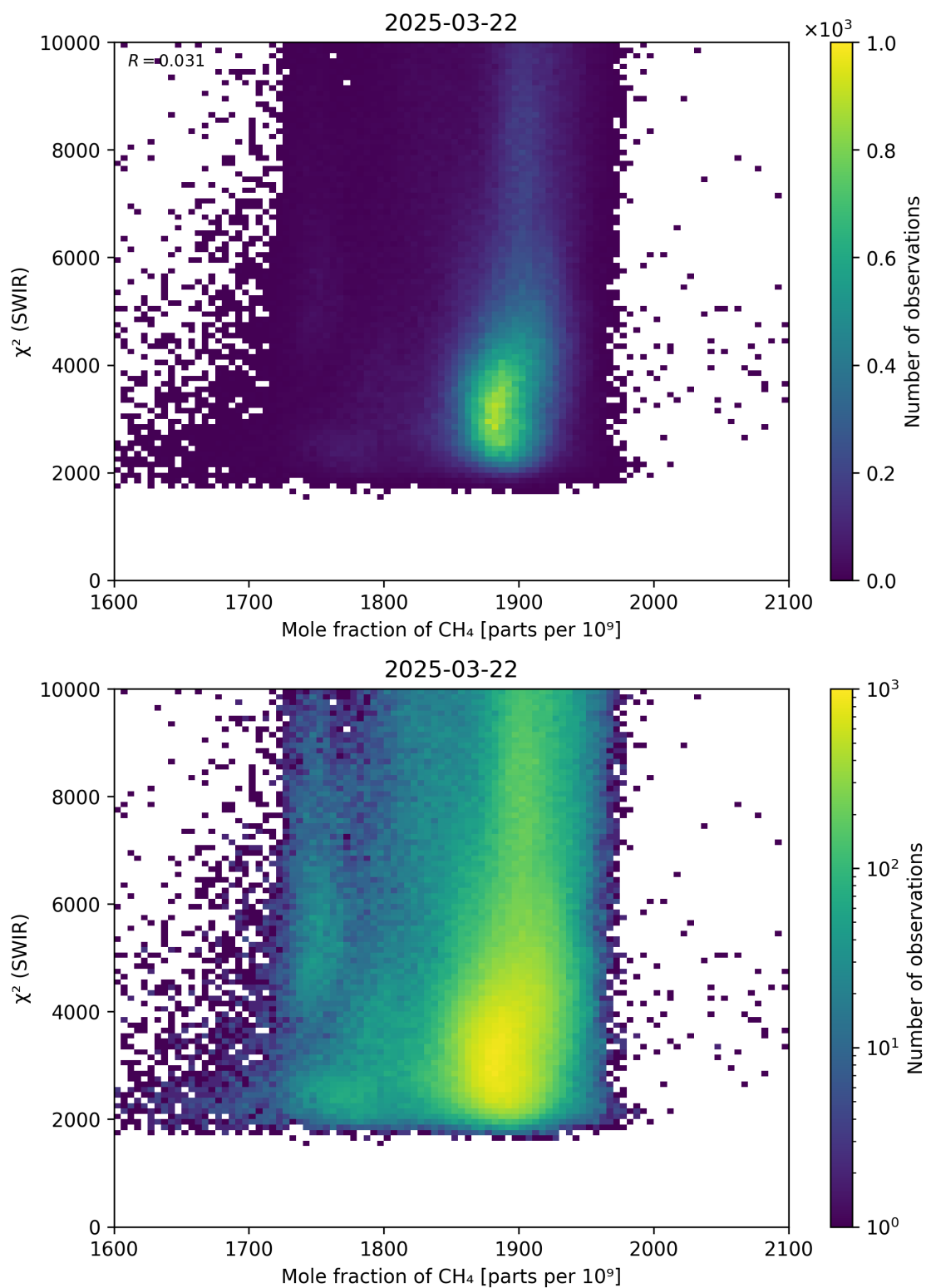
Figure 71: Scatter density plot of “Mole fraction of \text{CH}_4 ” against “ \chi^2 (SWIR)” for 2025-03-21 to 2025-03-23.
