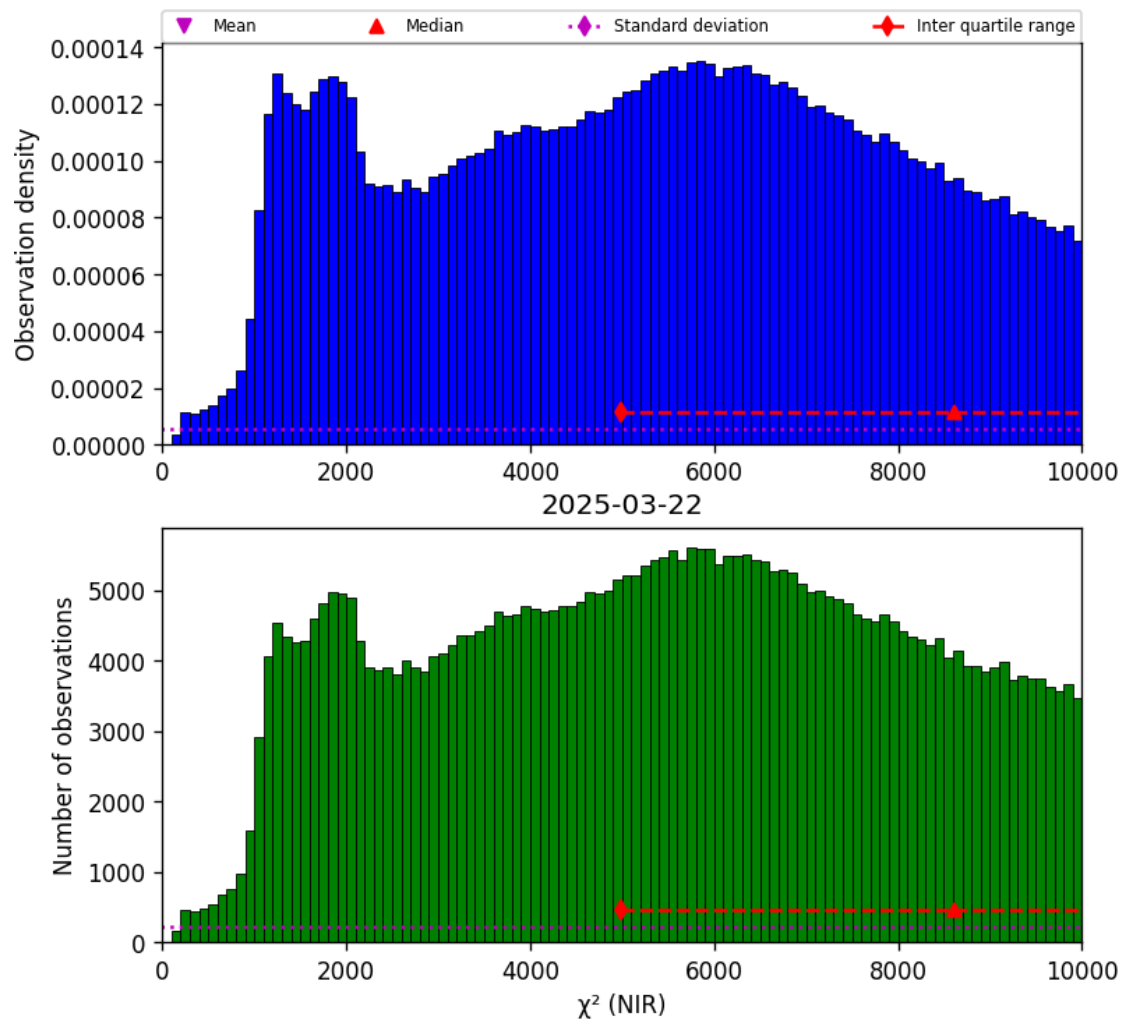
Figure 29: Histogram of “ \chi^2 (NIR)” for 2025-03-21 to 2025-03-23
