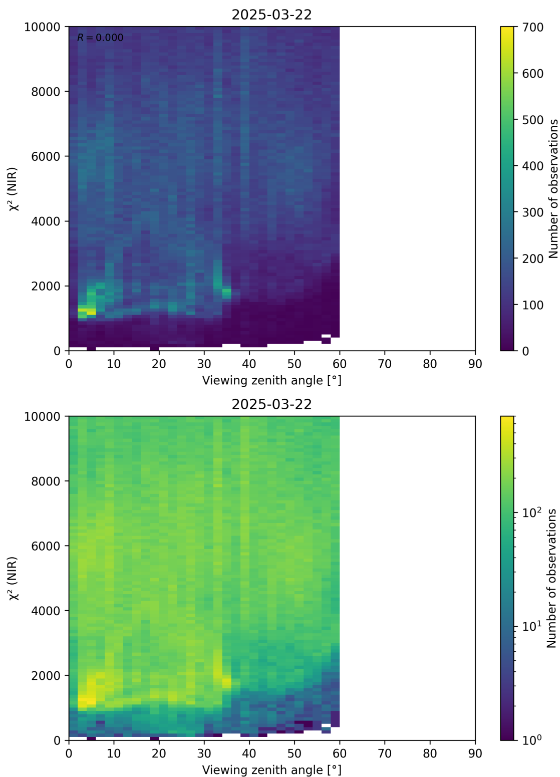
Figure 105: Scatter density plot of “Viewing zenith angle” against “ \chi^2 (NIR)” for 2025-03-21 to 2025-03-23.
