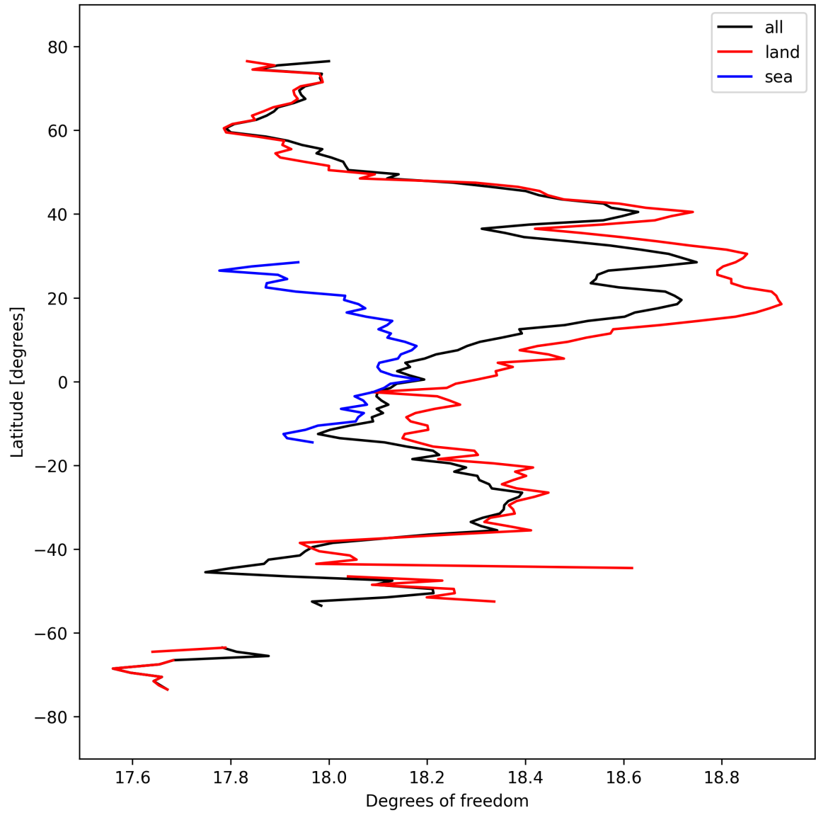
Figure 19: Zonal average of “Degrees of freedom” for 2025-03-21 to 2025-03-23.
