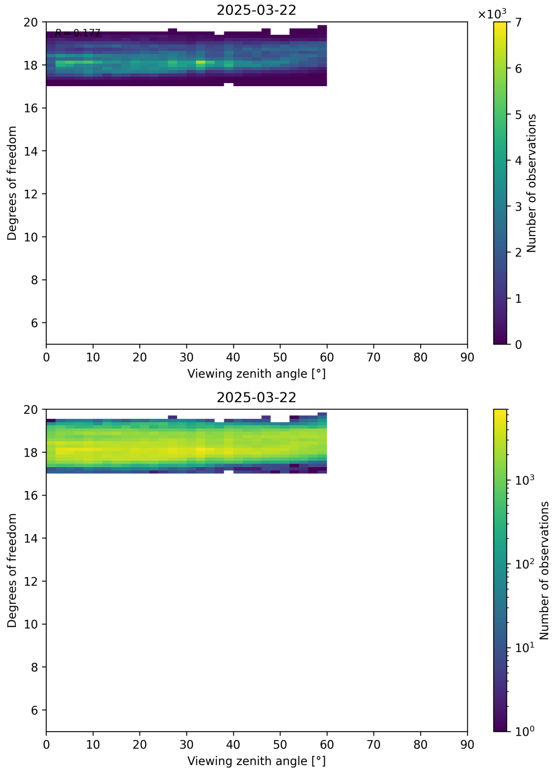
Figure 107: Scatter density plot of “Viewing zenith angle” against “Degrees of freedom” for 2025-03-21 to 2025-03-23.
