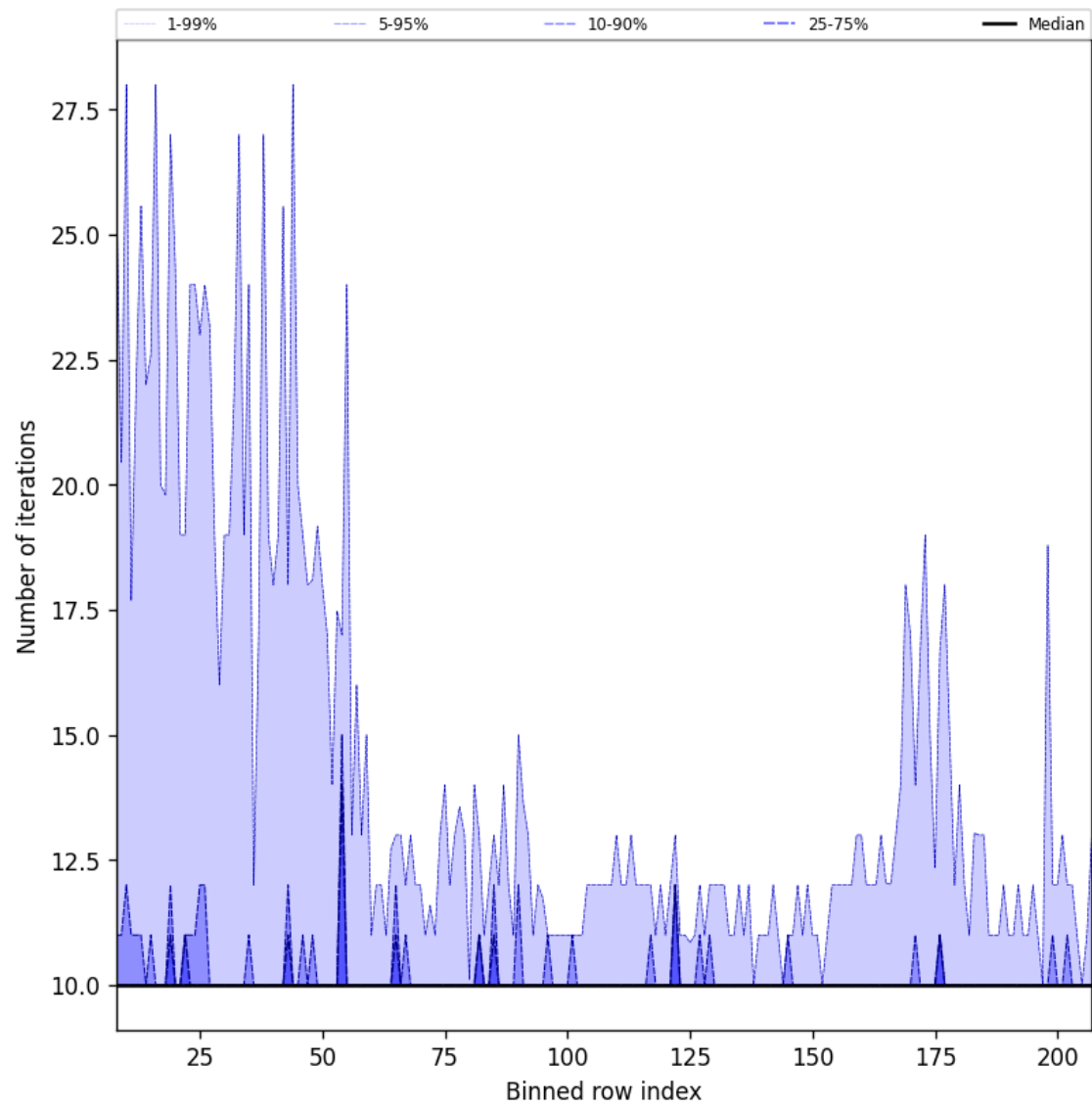
Figure 42: Along track statistics of “Number of iterations” for 2025-03-21 to 2025-03-23
