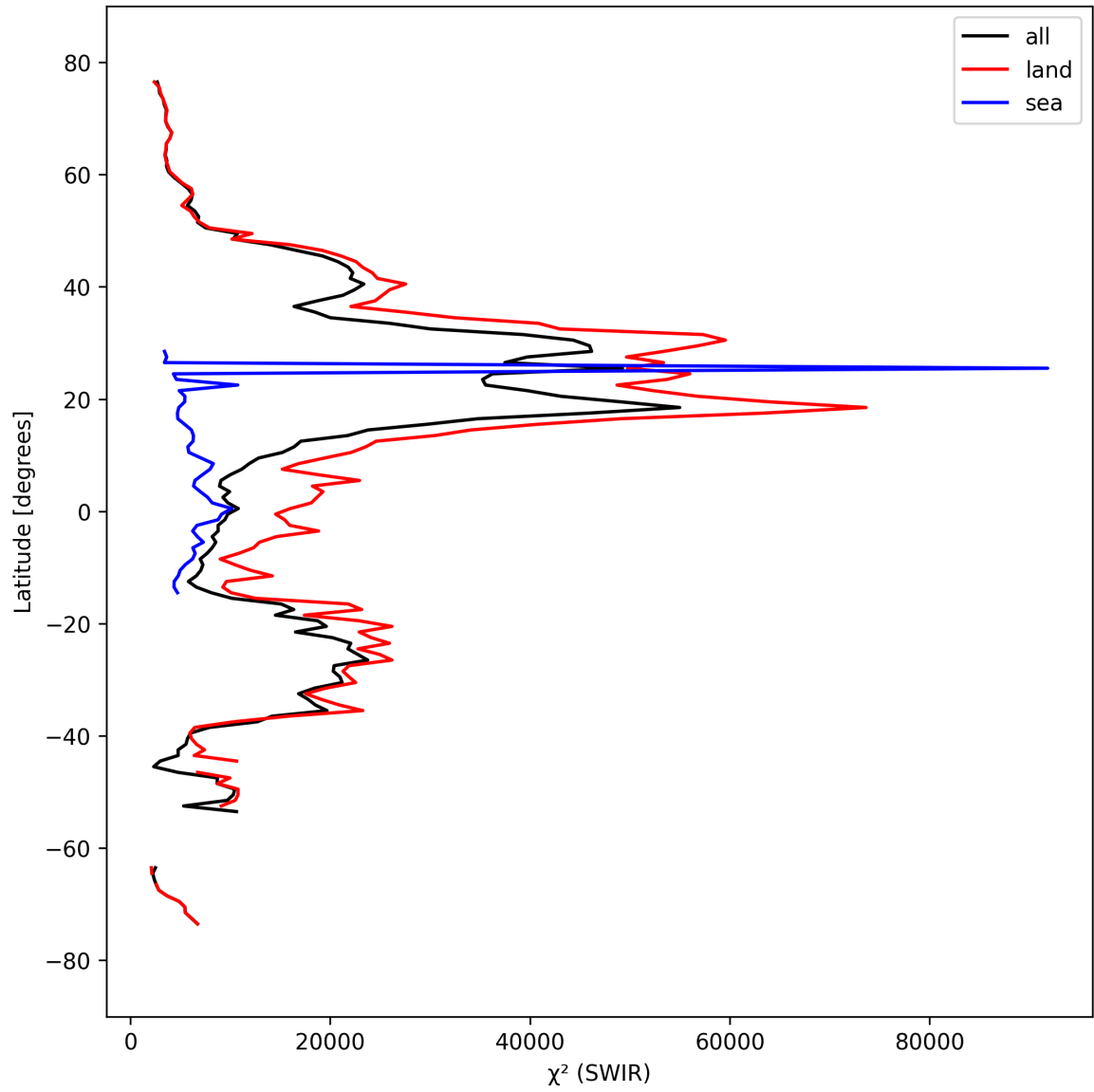
Figure 17: Zonal average of “ \chi^2 (SWIR)” for 2025-03-21 to 2025-03-23.
