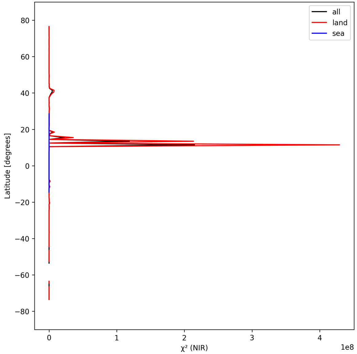
Figure 18: Zonal average of “ \chi^2 (NIR)” for 2025-03-21 to 2025-03-23.
