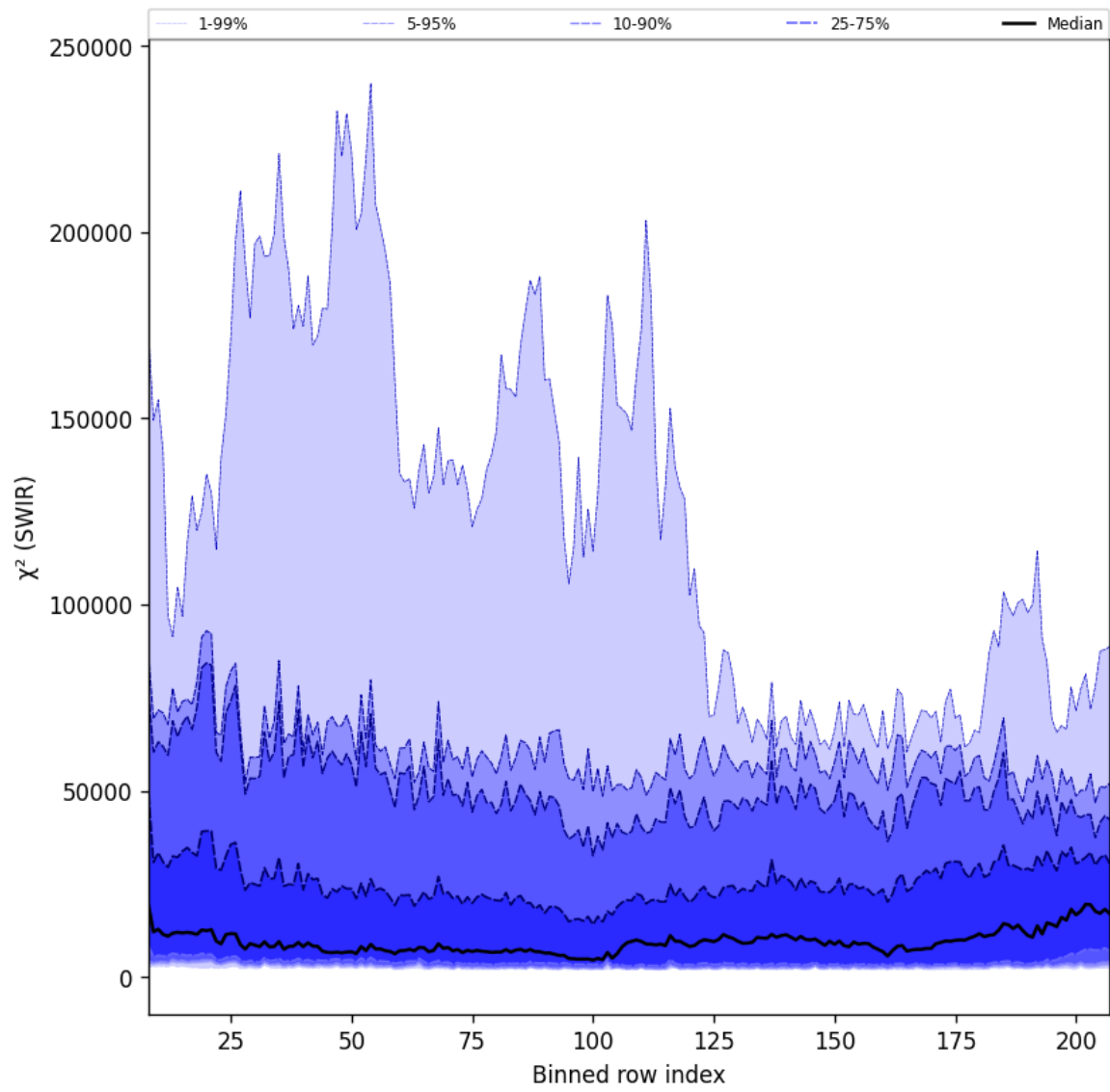
Figure 39: Along track statistics of “ \chi^2 (SWIR)” for 2025-03-21 to 2025-03-23
