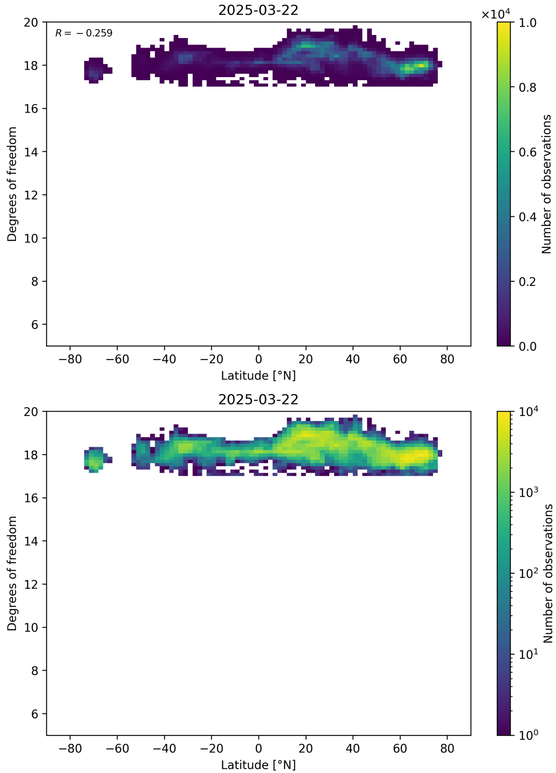
Figure 55: Scatter density plot of “Latitude” against “Degrees of freedom” for 2025-03-21 to 2025-03-23.
