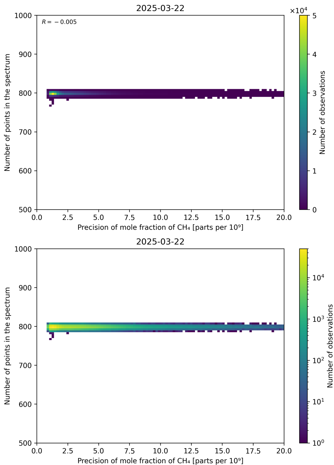
Figure 84: Scatter density plot of “Precision of mole fraction of CH 4 ” against “Number of points in the spectrum” for 2025-03-21 to 2025-03-23.
