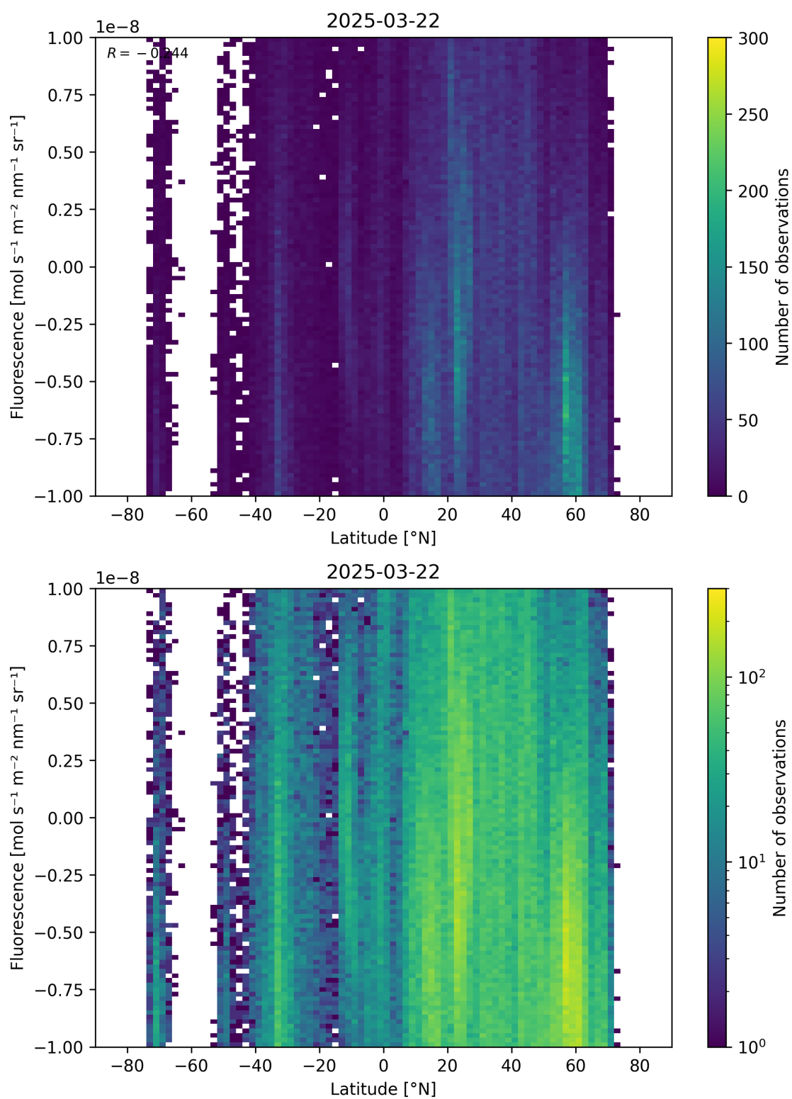
Figure 56: Scatter density plot of “Latitude” against “Fluorescence” for 2025-03-21 to 2025-03-23.
