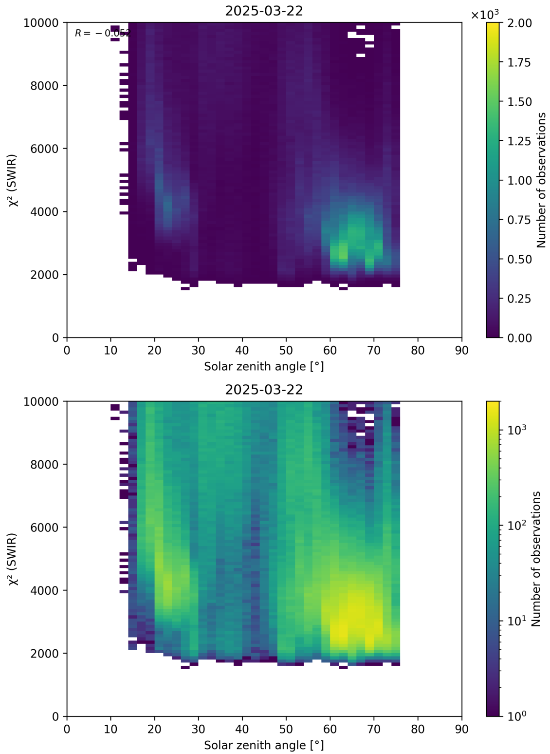
Figure 95: Scatter density plot of “Solar zenith angle” against “ \chi^2 (SWIR)” for 2025-03-21 to 2025-03-23.
