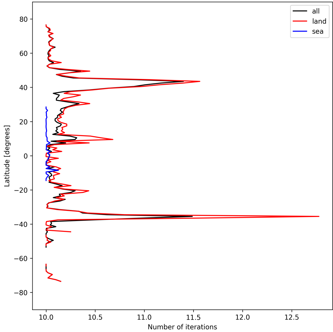
Figure 20: Zonal average of “Number of iterations” for 2025-03-21 to 2025-03-23.
