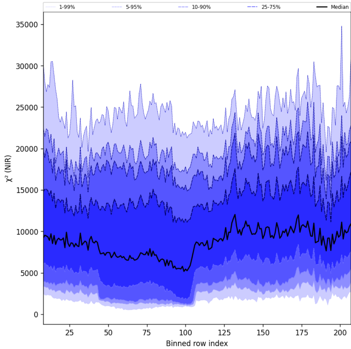
Figure 40: Along track statistics of " \chi^2 (NIR)" for 2025-03-21 to 2025-03-23
