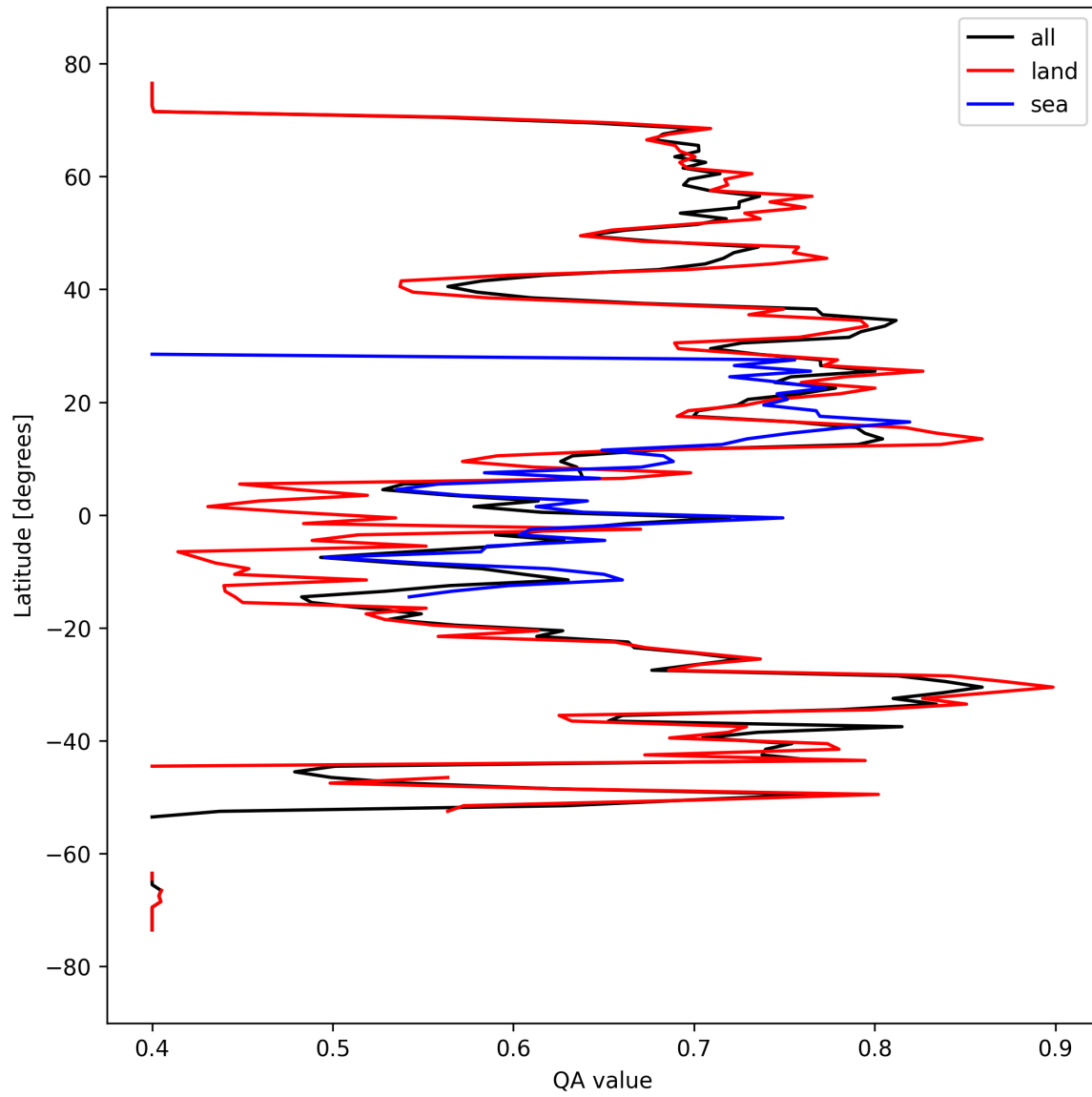
Figure 11: Zonal average of “QA value” for 2025-03-21 to 2025-03-23.
