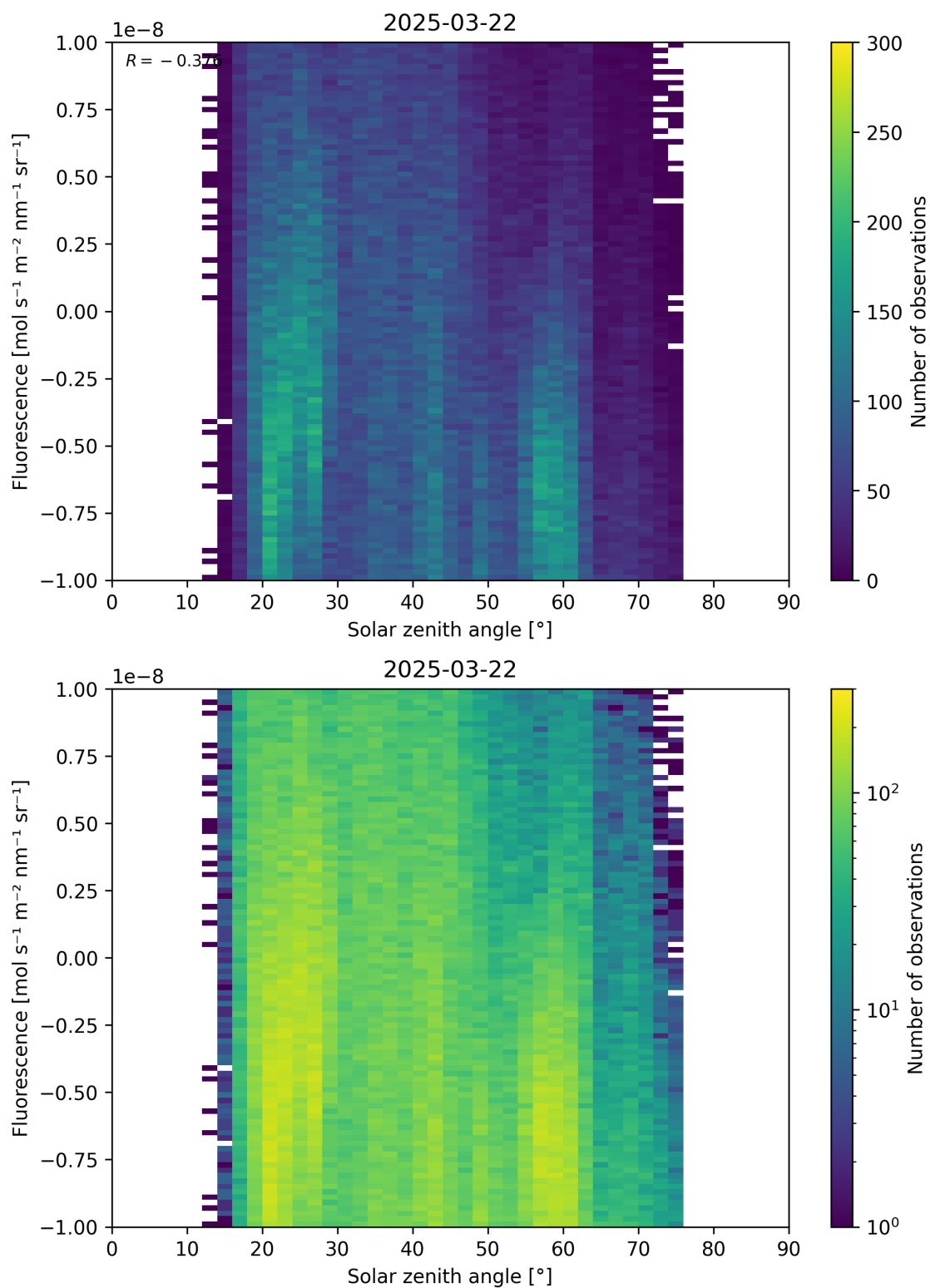
Figure 97: Scatter density plot of “Solar zenith angle” against “Fluorescence” for 2025-03-21 to 2025-03-23.
