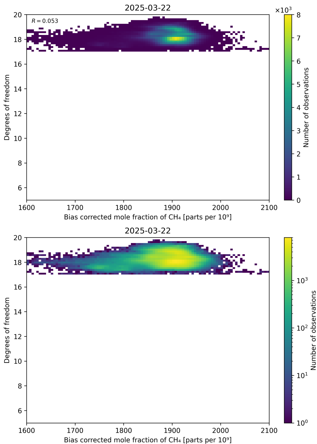
Figure 65: Scatter density plot of “Bias corrected mole fraction of CH 4 ” against “Degrees of freedom” for 2025-03-21 to 2025-03-23.
