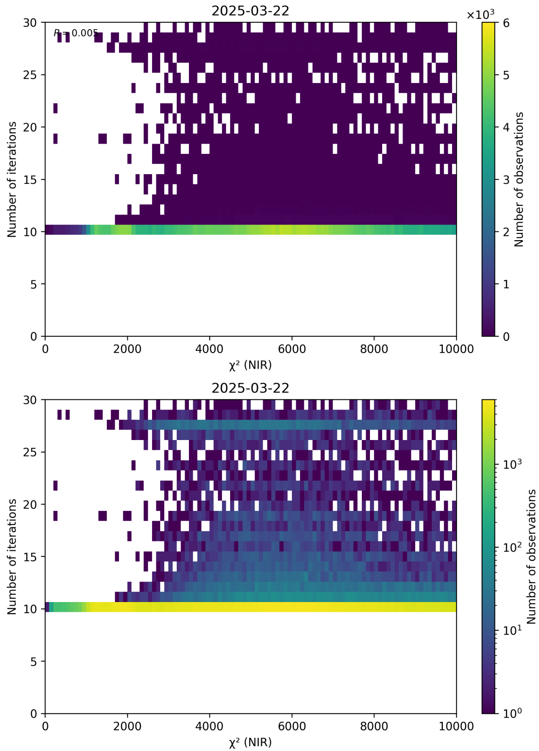
Figure 46: Scatter density plot of “ \chi^2 (NIR)” against “Number of iterations” for 2025-03-21 to 2025-03-23.
