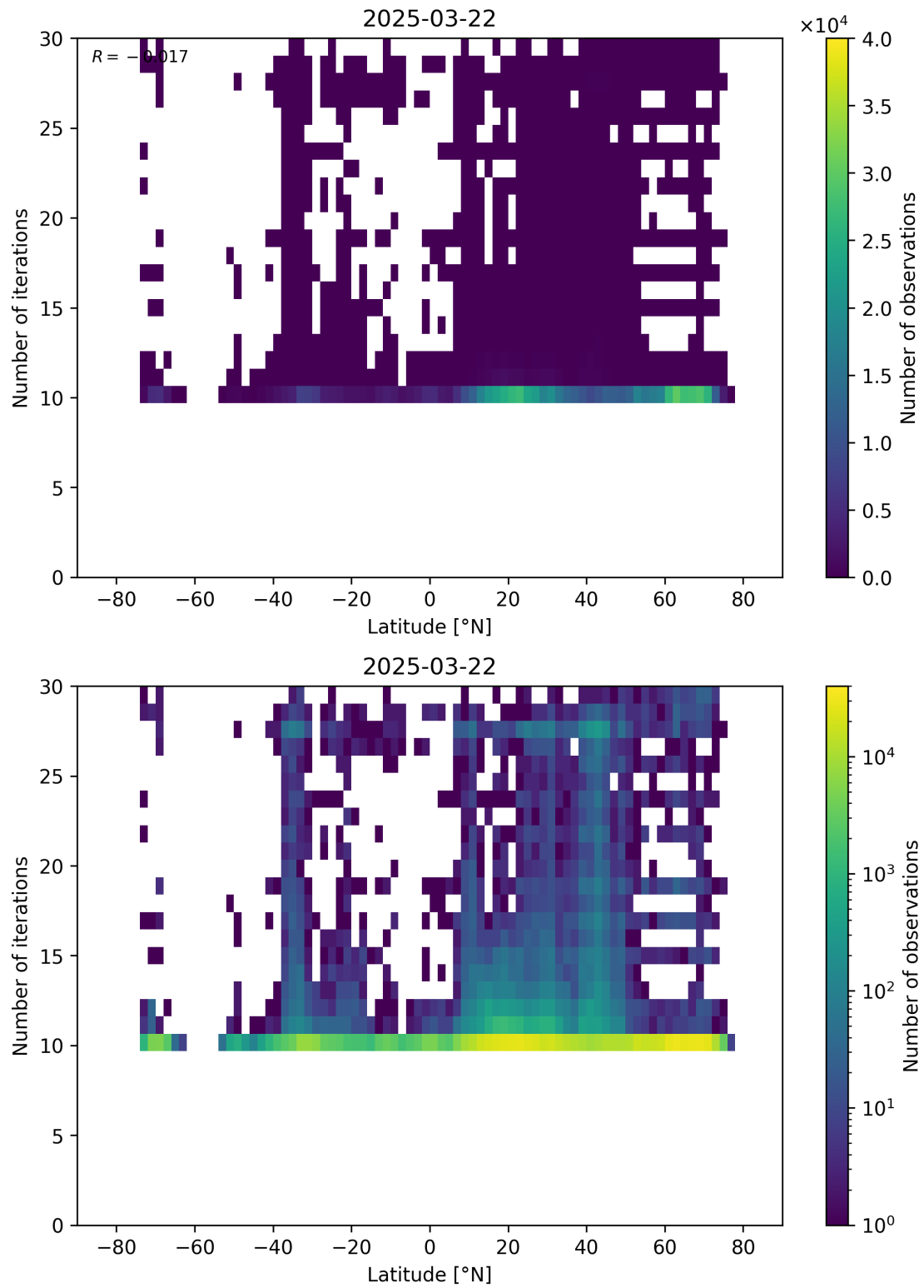
Figure 60: Scatter density plot of “Latitude” against “Number of iterations” for 2025-03-21 to 2025-03-23.
