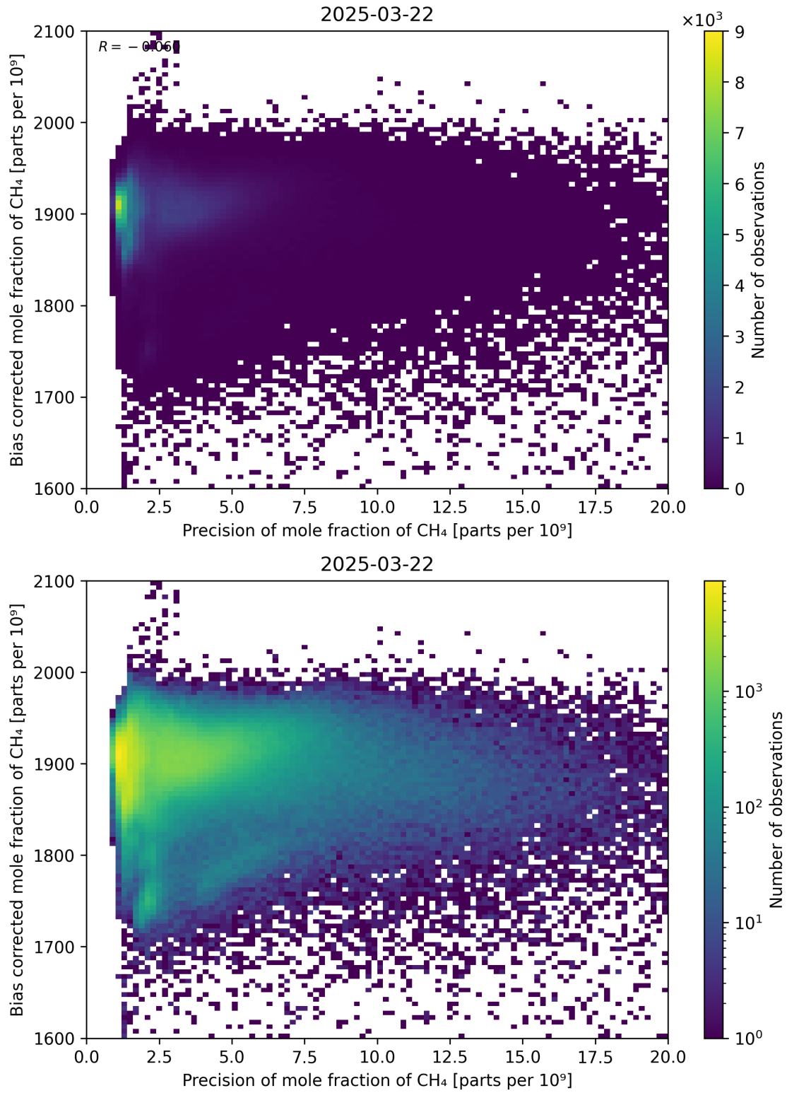
Figure 82: Scatter density plot of “Precision of mole fraction of CH 4 ” against “Bias corrected mole fraction of CH 4 ” for 2025-03-21 to 2025-03-23.
