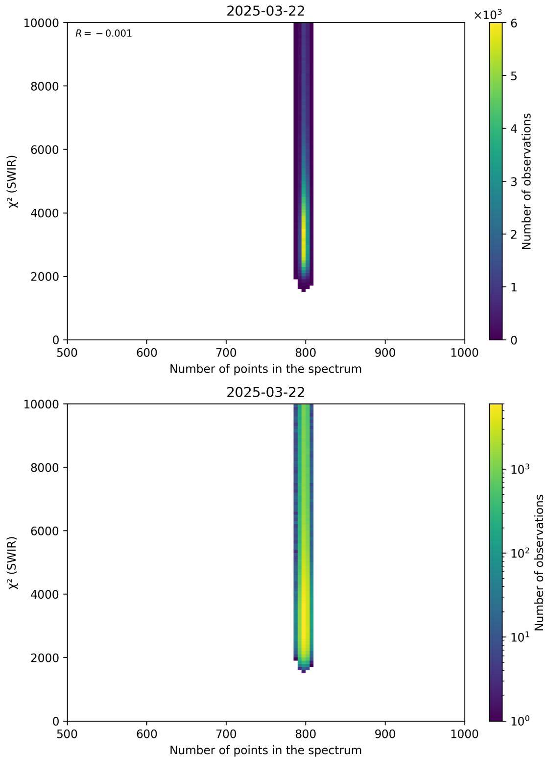
Figure 89: Scatter density plot of “Number of points in the spectrum” against “ \chi^2 (SWIR)” for 2025-03-21 to 2025-03-23.
