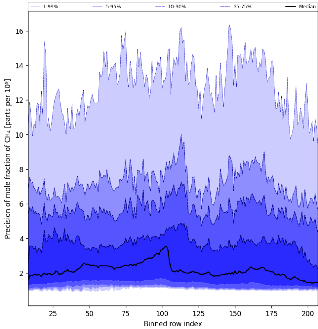
Figure 35: Along track statistics of “Precision of mole fraction of CH 4 ” for 2025-03-21 to 2025-03-23
