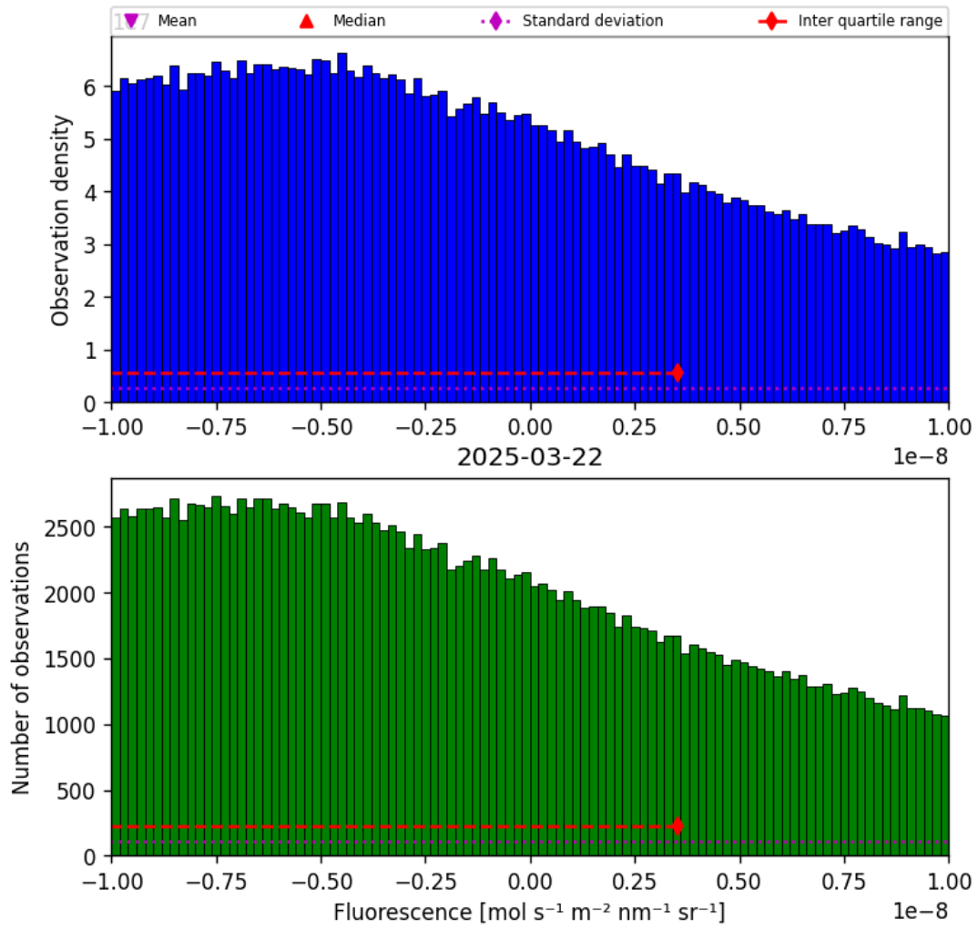
Figure 32: Histogram of “Fluorescence” for 2025-03-21 to 2025-03-23
