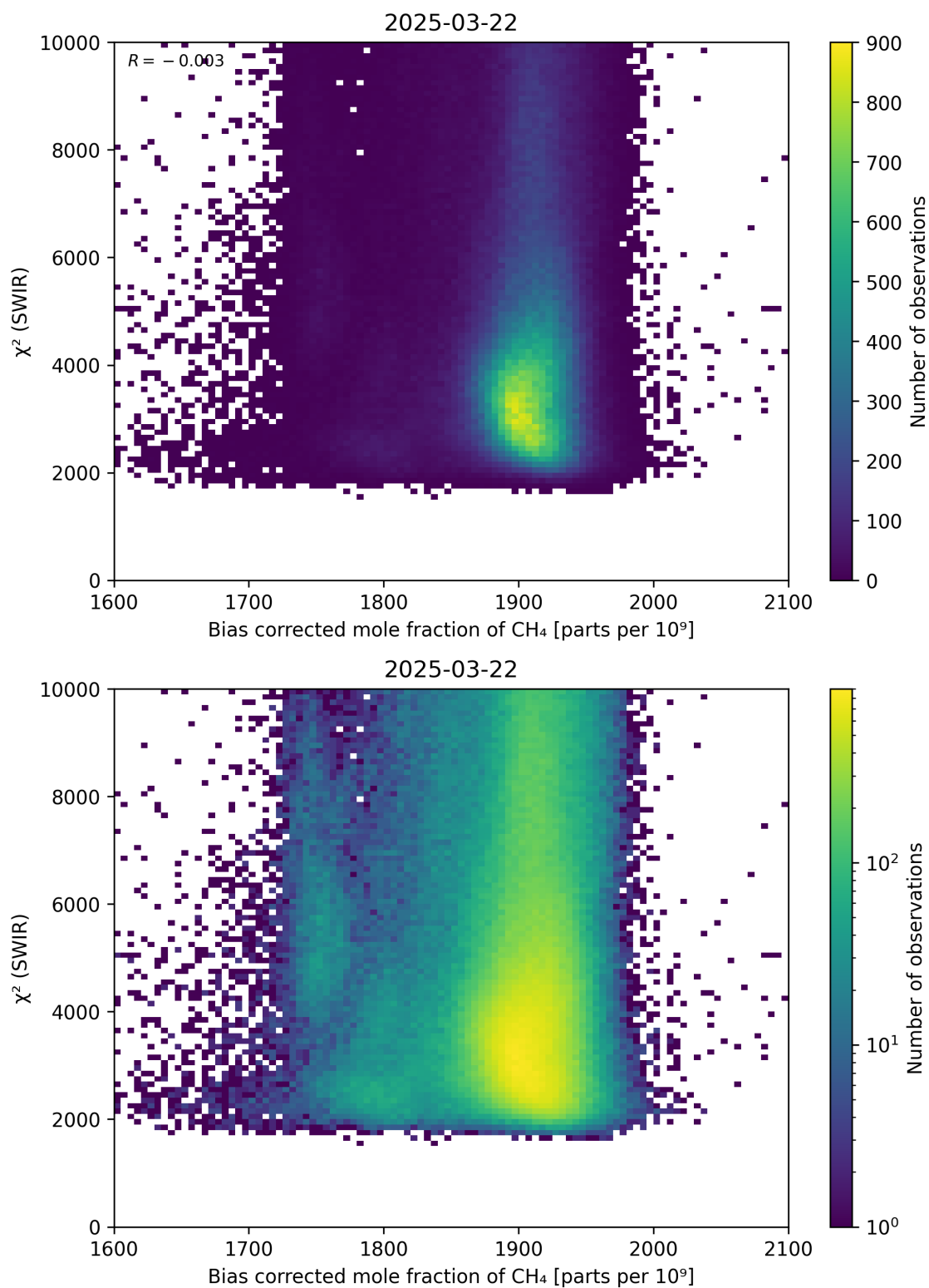
Figure 64: Scatter density plot of “Bias corrected mole fraction of CH 4 ” against “ \chi^2 (SWIR)” for 2025-03-21 to 2025-03-23.
