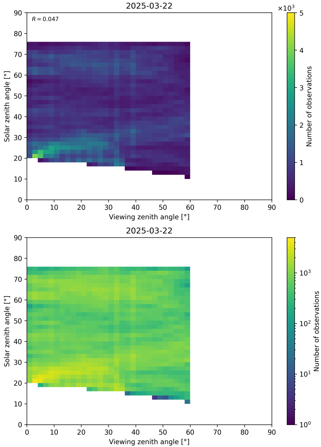
Figure 115: Scatter density plot of “Viewing zenith angle” against “Solar zenith angle” for 2025-03-21 to 2025-03-23.
