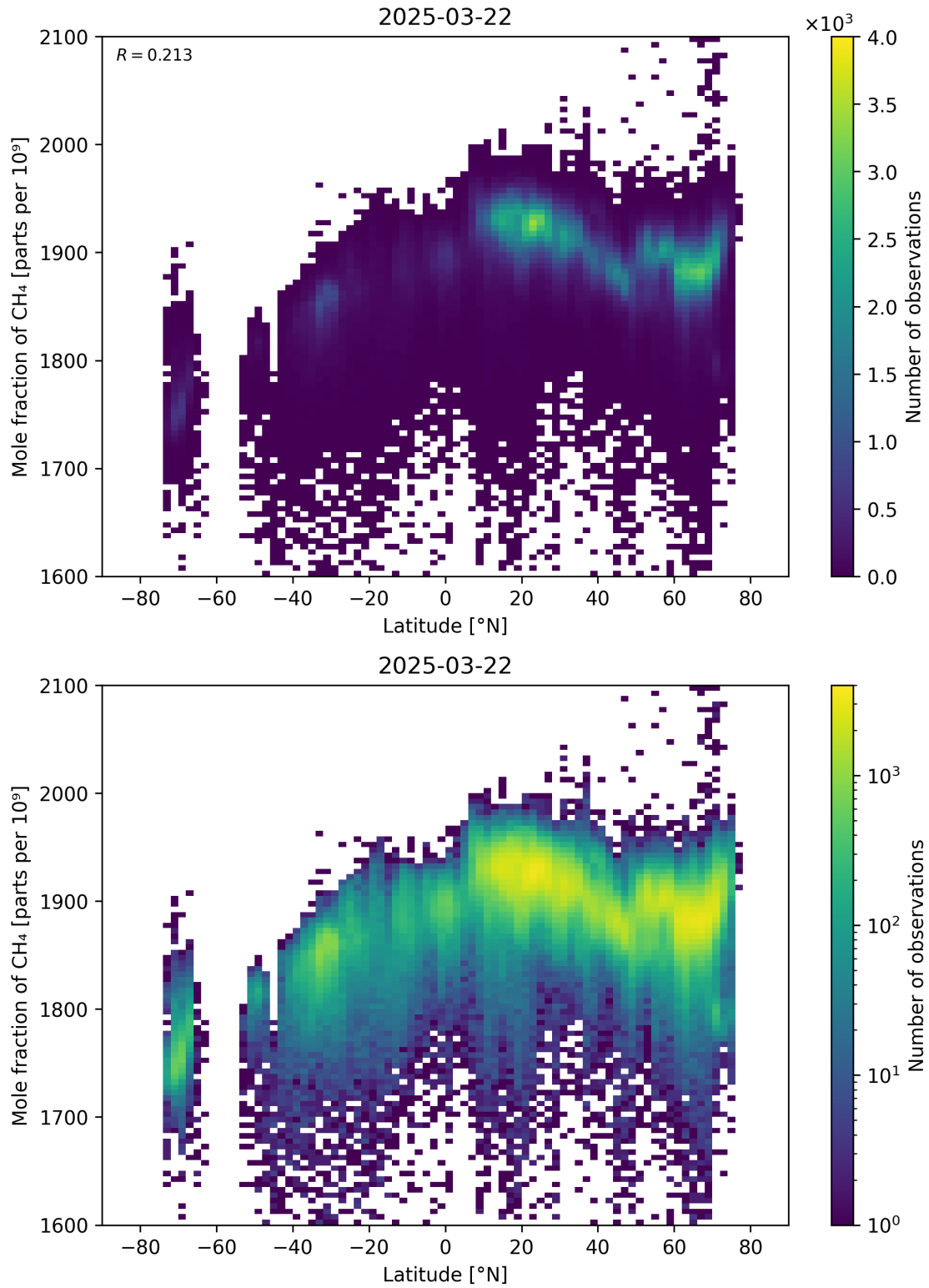
Figure 57: Scatter density plot of “Latitude” against “Mole fraction of CH 4 ” for 2025-03-21 to 2025-03-23.
