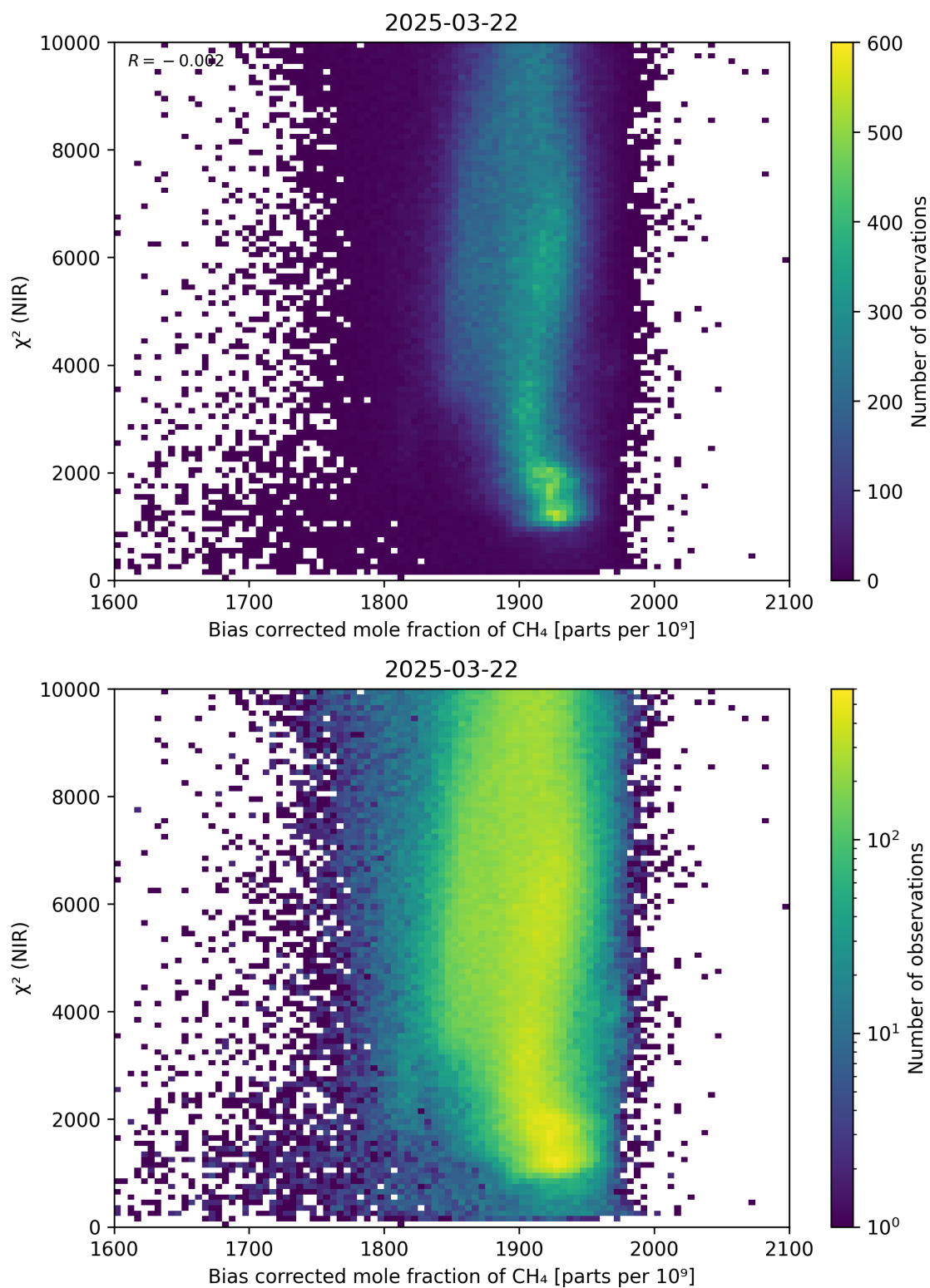
Figure 63: Scatter density plot of “Bias corrected mole fraction of CH 4 ” against “ \chi^2 (NIR)” for 2025-03-21 to 2025-03-23.
