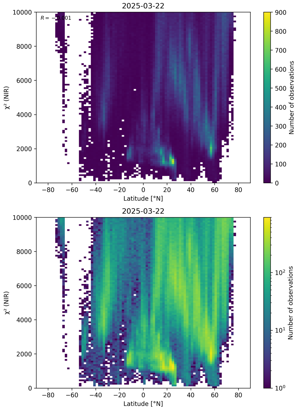
Figure 53: Scatter density plot of “Latitude” against “ \chi^2 (NIR)” for 2025-03-21 to 2025-03-23.
