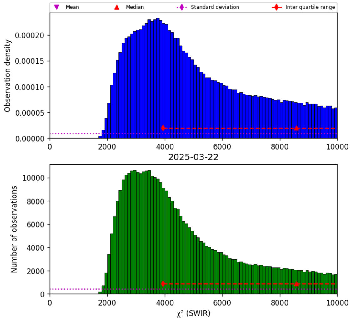
Figure 28: Histogram of “ \chi^2 (SWIR)” for 2025-03-21 to 2025-03-23
