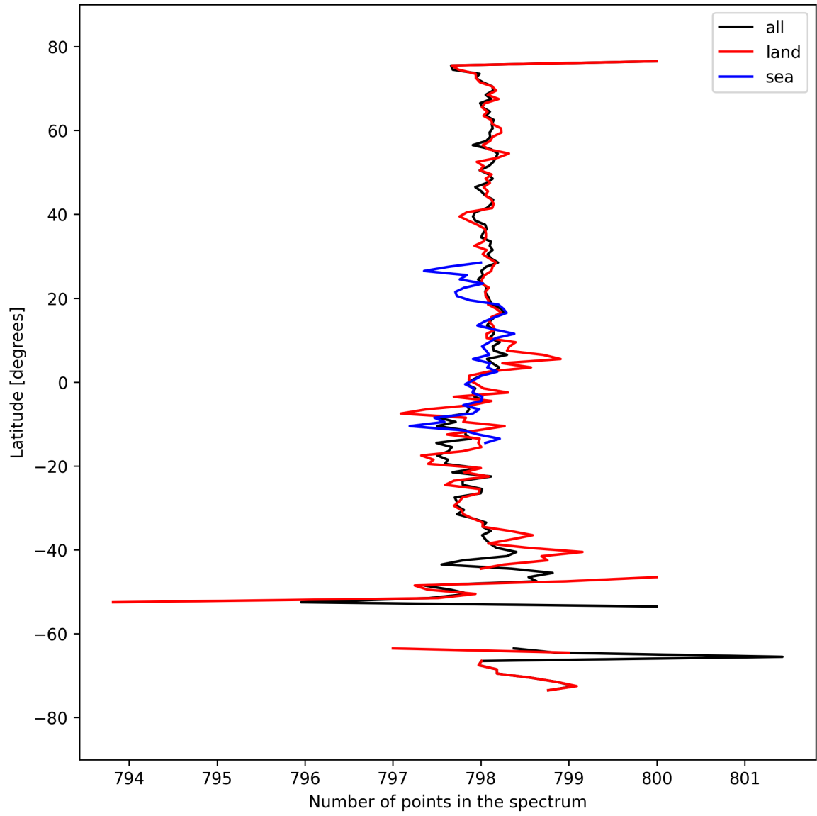
Figure 15: Zonal average of “Number of points in the spectrum” for 2025-03-21 to 2025-03-23.
