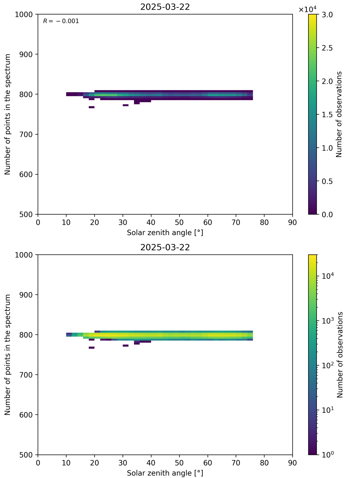
Figure 103: Scatter density plot of “Solar zenith angle” against “Number of points in the spectrum” for 2025-03-21 to 2025-03-23.
