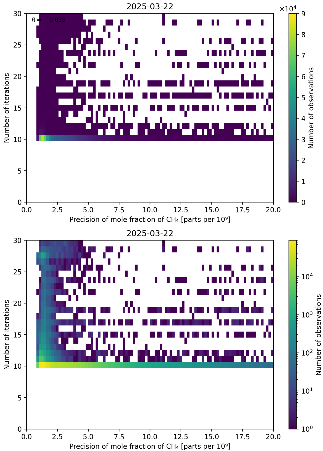
Figure 83: Scatter density plot of “Precision of mole fraction of CH 4 ” against “Number of iterations” for 2025-03-21 to 2025-03-23.
