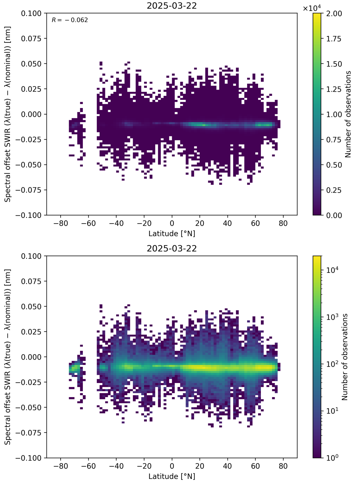
Figure 62: Scatter density plot of “Latitude” against “Spectral offset SWIR ( \lambda_{\text{true}} - \lambda_{\text{nominal}} )” for 2025-03-21 to 2025-03-23.
