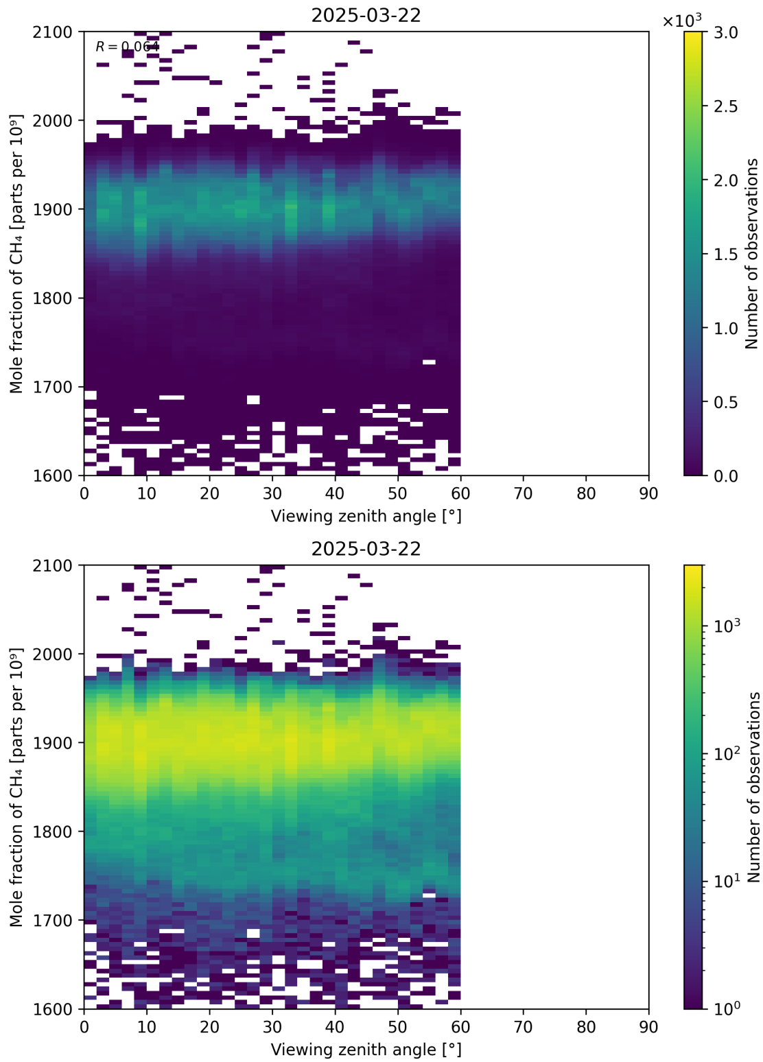
Figure 110: Scatter density plot of “Viewing zenith angle” against “Mole fraction of CH 4 ” for 2025-03-21 to 2025-03-23.
