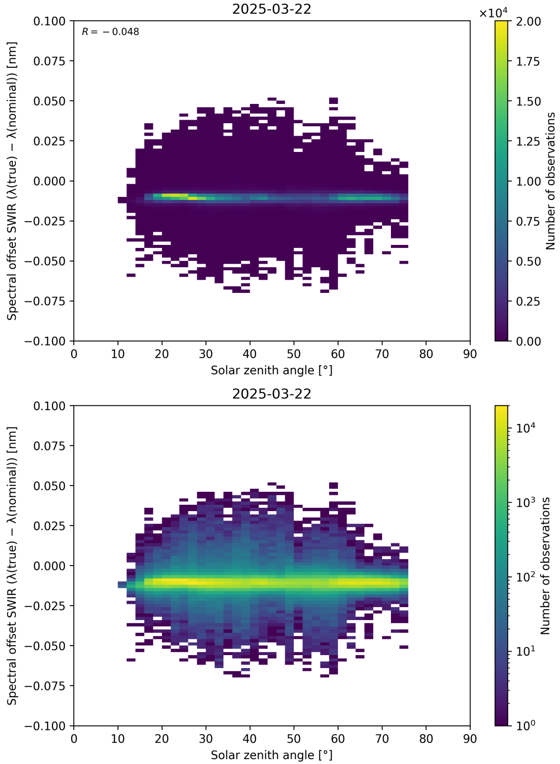
Figure 104: Scatter density plot of “Solar zenith angle” against “Spectral offset SWIR ( \lambda_{\text{true}} - \lambda_{\text{nominal}} )” for 2025-03-21 to 2025-03-23.
