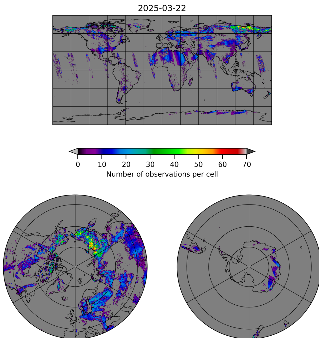
Figure 10: Map of the number of observations for 2025-03-21 to 2025-03-23
