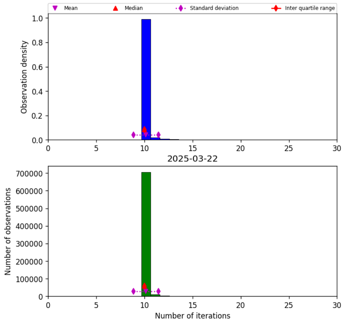
Figure 31: Histogram of “Number of iterations” for 2025-03-21 to 2025-03-23
