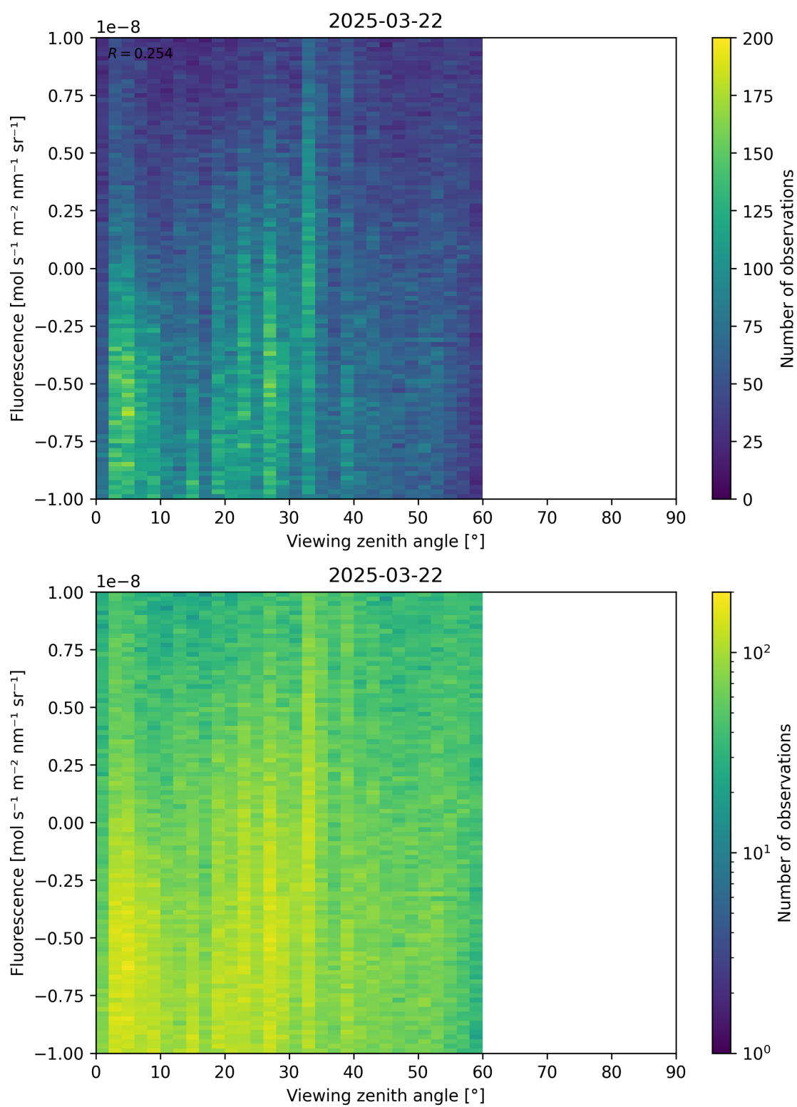
Figure 108: Scatter density plot of “Viewing zenith angle” against “Fluorescence” for 2025-03-21 to 2025-03-23.
