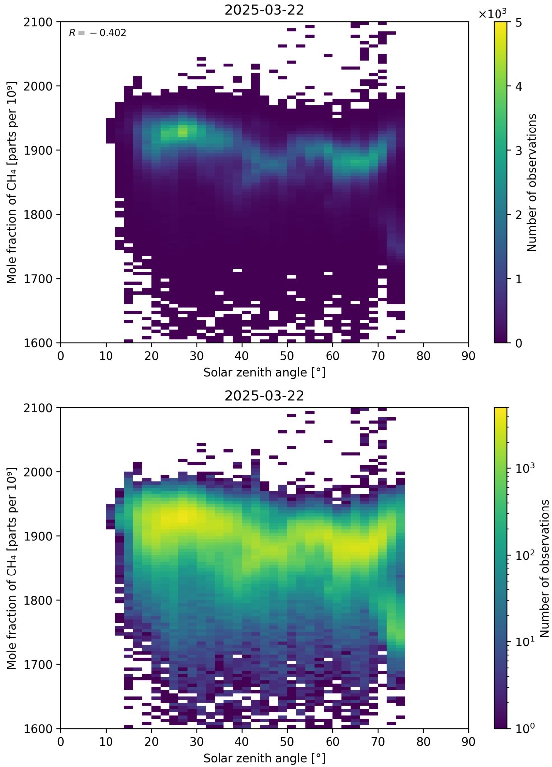
Figure 99: Scatter density plot of “Solar zenith angle” against “Mole fraction of CH 4 ” for 2025-03-21 to 2025-03-23.
