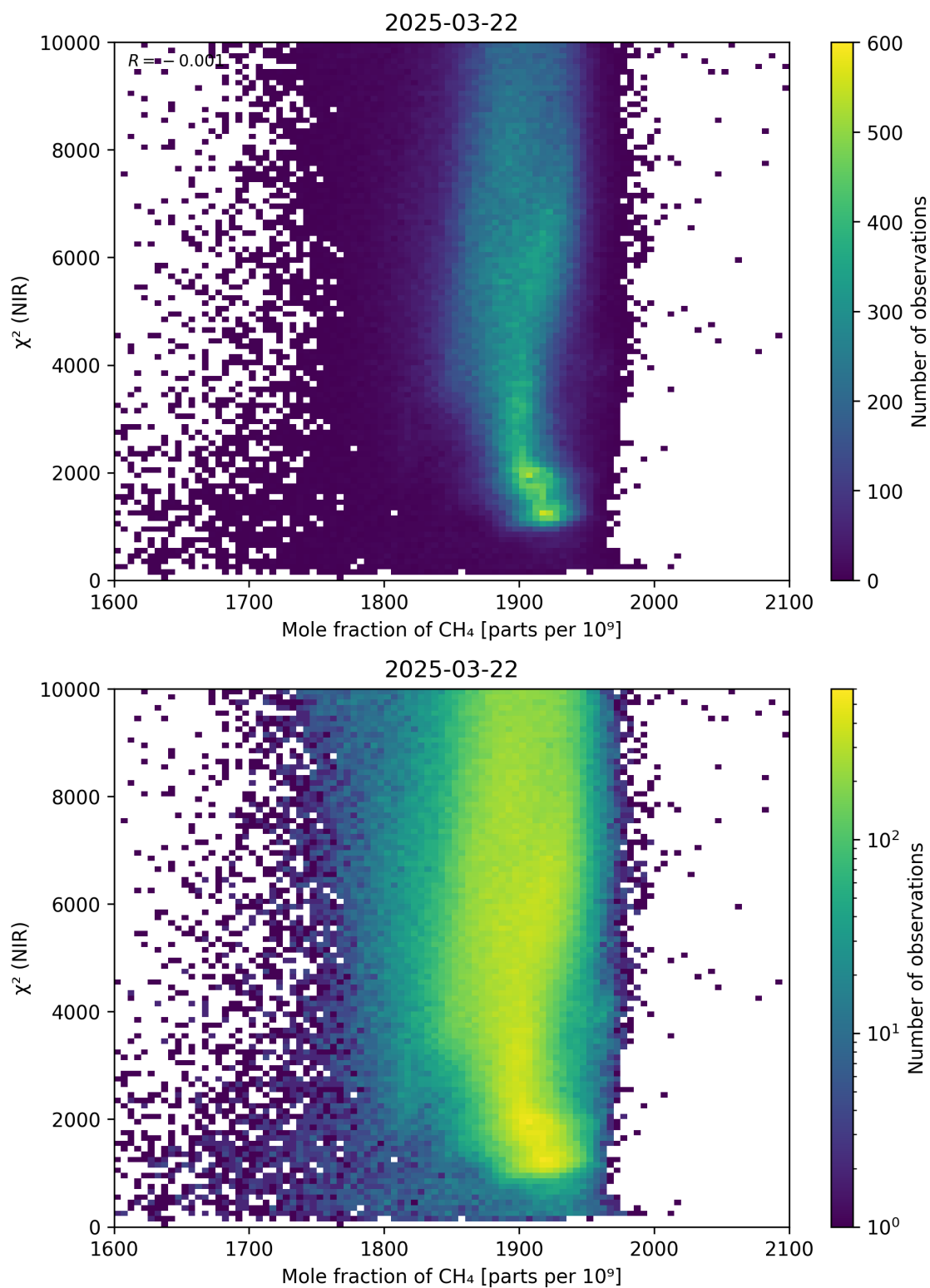
Figure 70: Scatter density plot of “Mole fraction of \text{CH}_4 ” against “ \chi^2 (NIR)” for 2025-03-21 to 2025-03-23.
