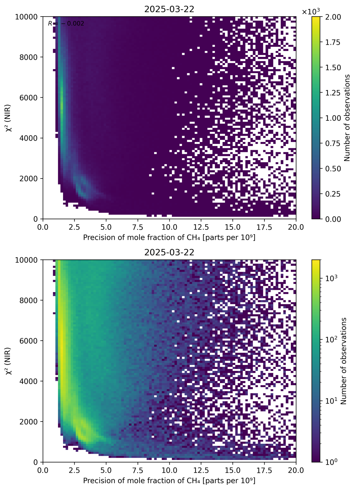
Figure 78: Scatter density plot of “Precision of mole fraction of CH 4 ” against “ \chi^2 (NIR)” for 2025-03-21 to 2025-03-23.
