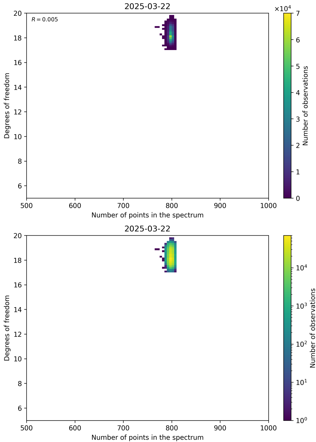
Figure 90: Scatter density plot of “Number of points in the spectrum” against “Degrees of freedom” for 2025-03-21 to 2025-03-23.
