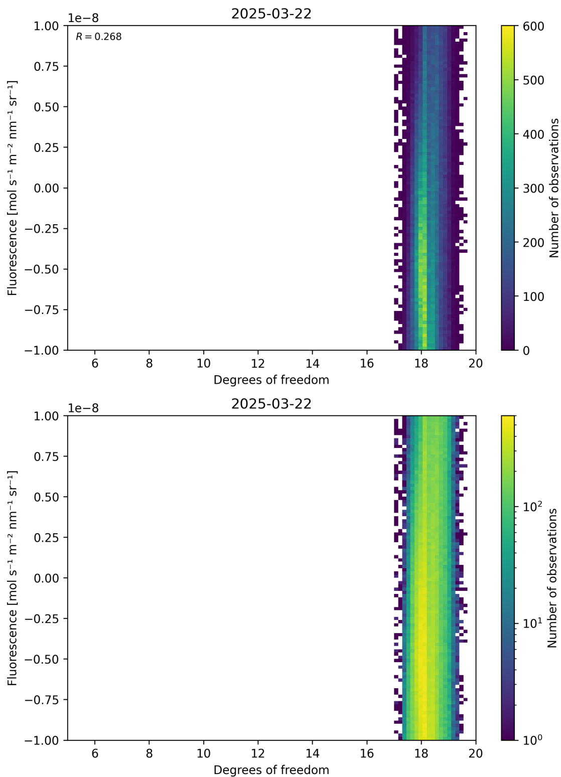
Figure 51: Scatter density plot of “Degrees of freedom” against “Fluorescence” for 2025-03-21 to 2025-03-23.
