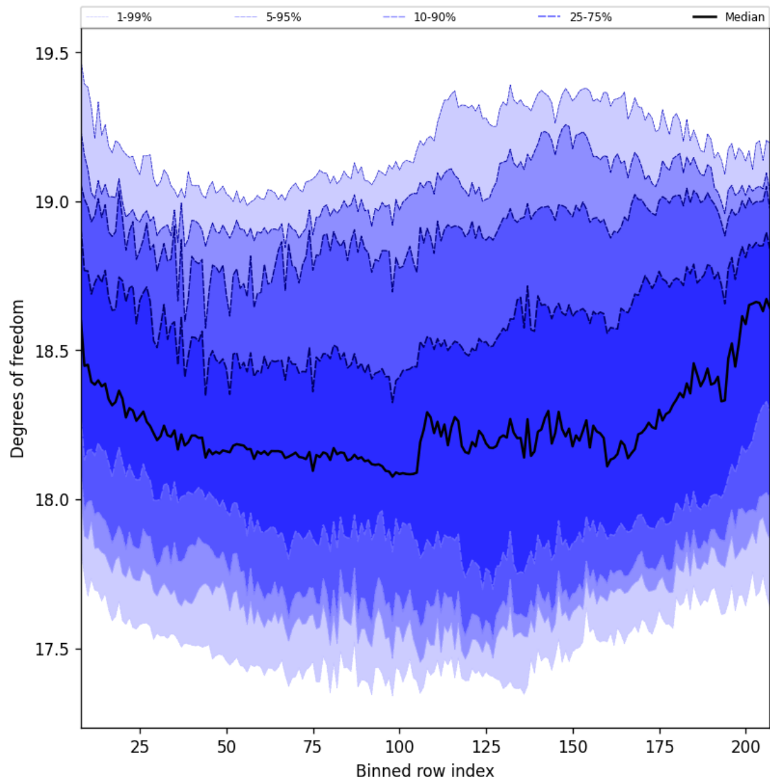
Figure 41: Along track statistics of “Degrees of freedom” for 2025-03-21 to 2025-03-23
