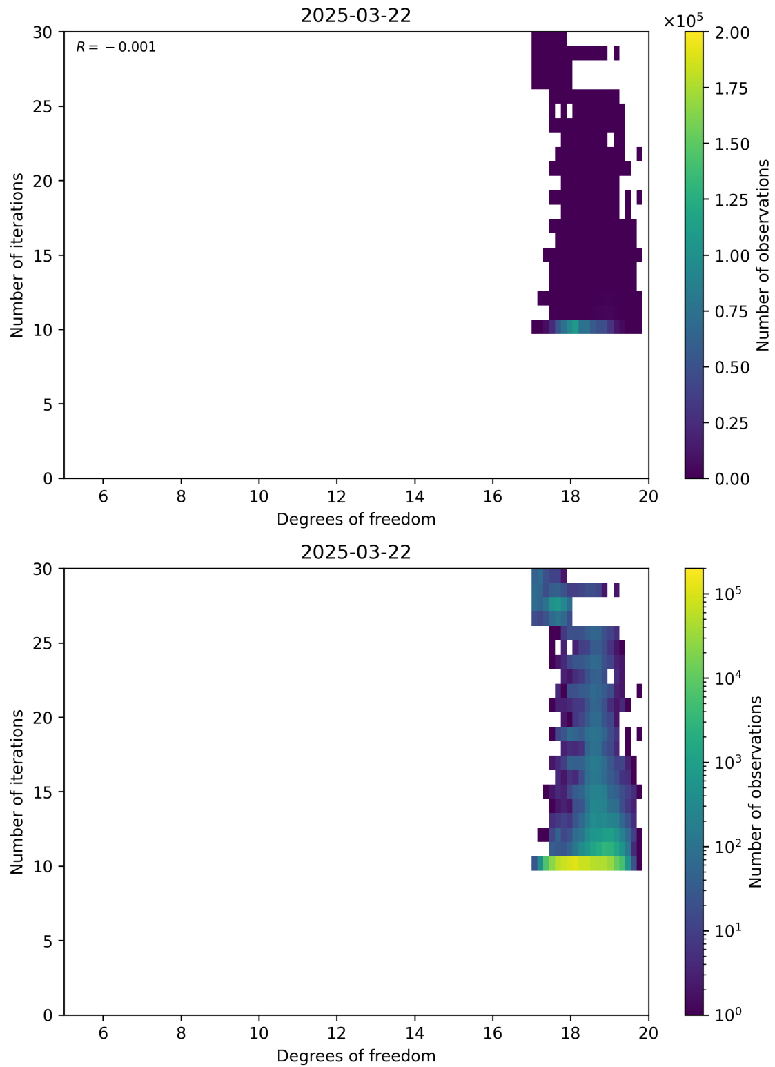
Figure 52: Scatter density plot of “Degrees of freedom” against “Number of iterations” for 2025-03-21 to 2025-03-23.
