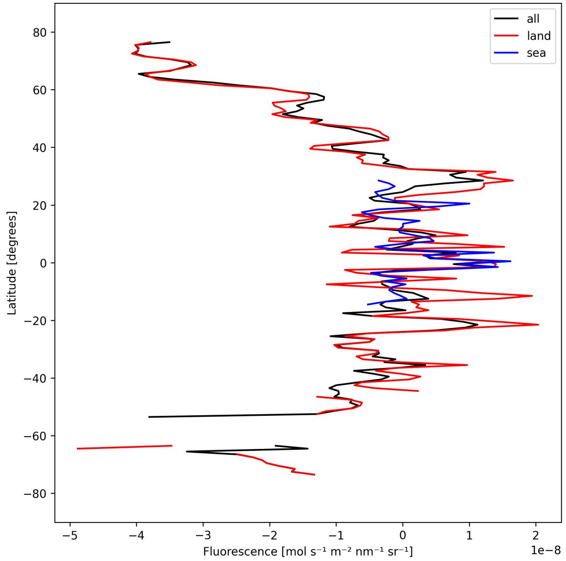
Figure 21: Zonal average of “Fluorescence” for 2025-03-21 to 2025-03-23.
