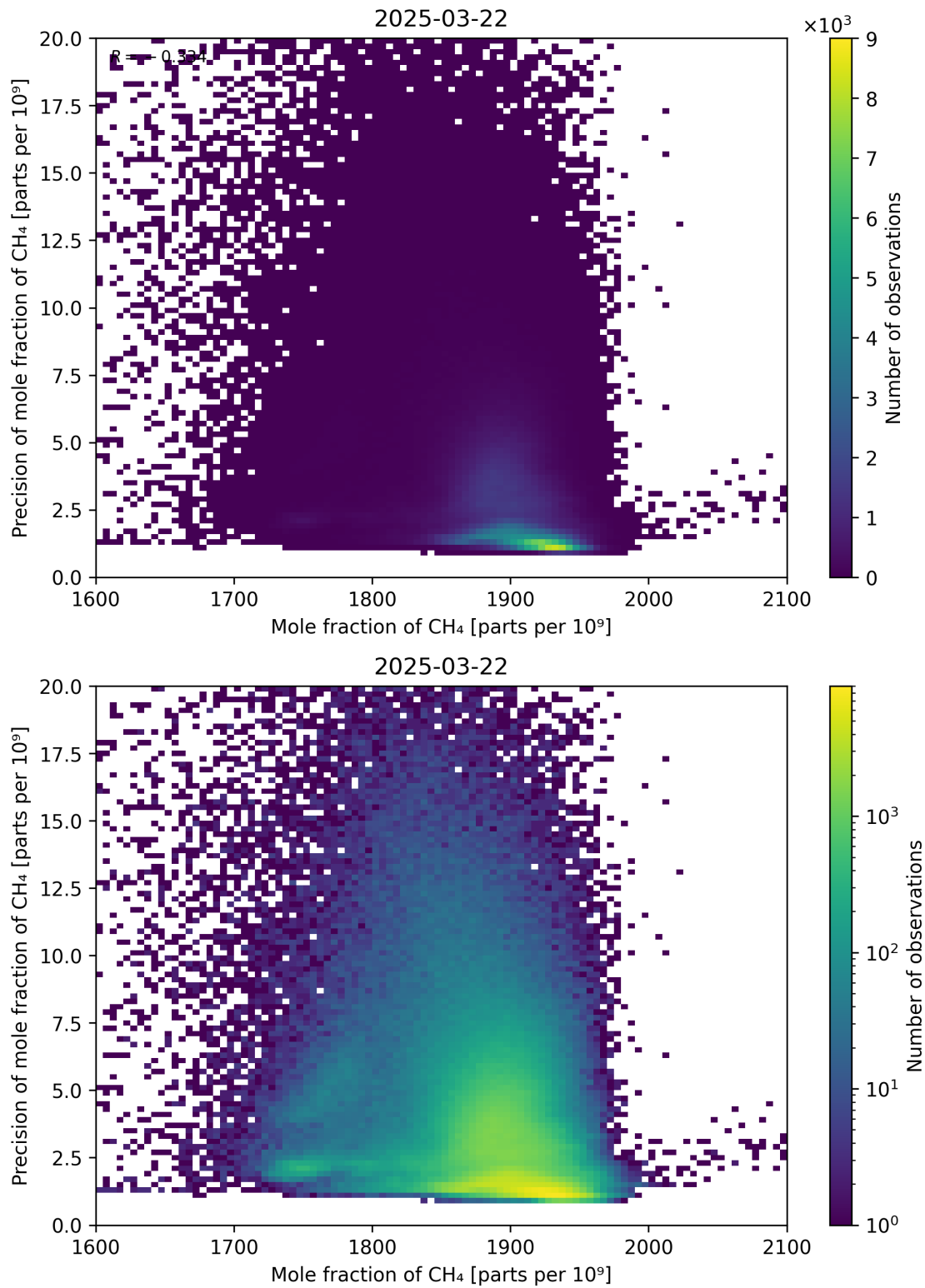
Figure 75: Scatter density plot of “Mole fraction of CH 4 ” against “Precision of mole fraction of CH 4 ” for 2025-03-21 to 2025-03-23.
