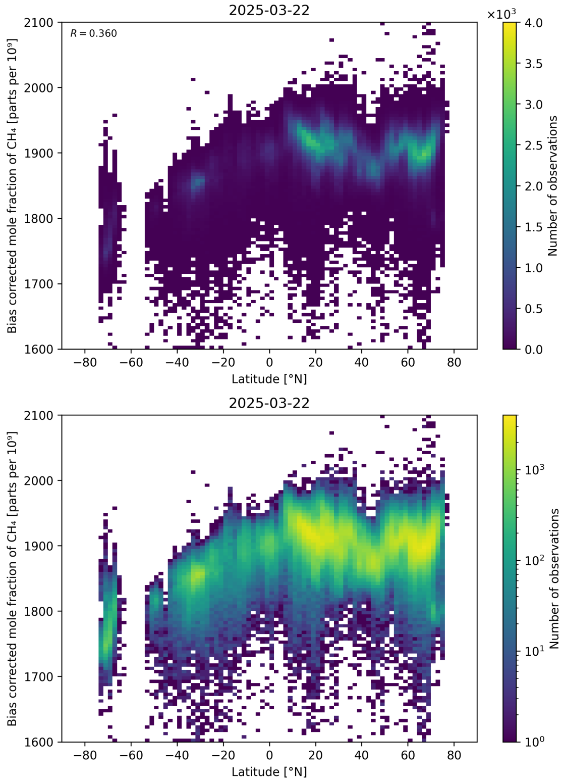
Figure 58: Scatter density plot of “Latitude” against “Bias corrected mole fraction of CH 4 ” for 2025-03-21 to 2025-03-23.
