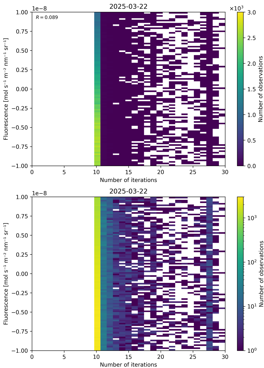
Figure 87: Scatter density plot of “Number of iterations” against “Fluorescence” for 2025-03-21 to 2025-03-23.
