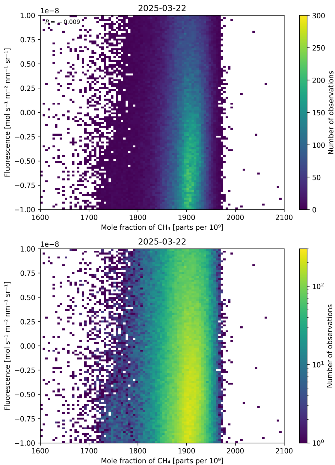
Figure 73: Scatter density plot of “Mole fraction of \text{CH}_4 ” against “Fluorescence” for 2025-03-21 to 2025-03-23.
