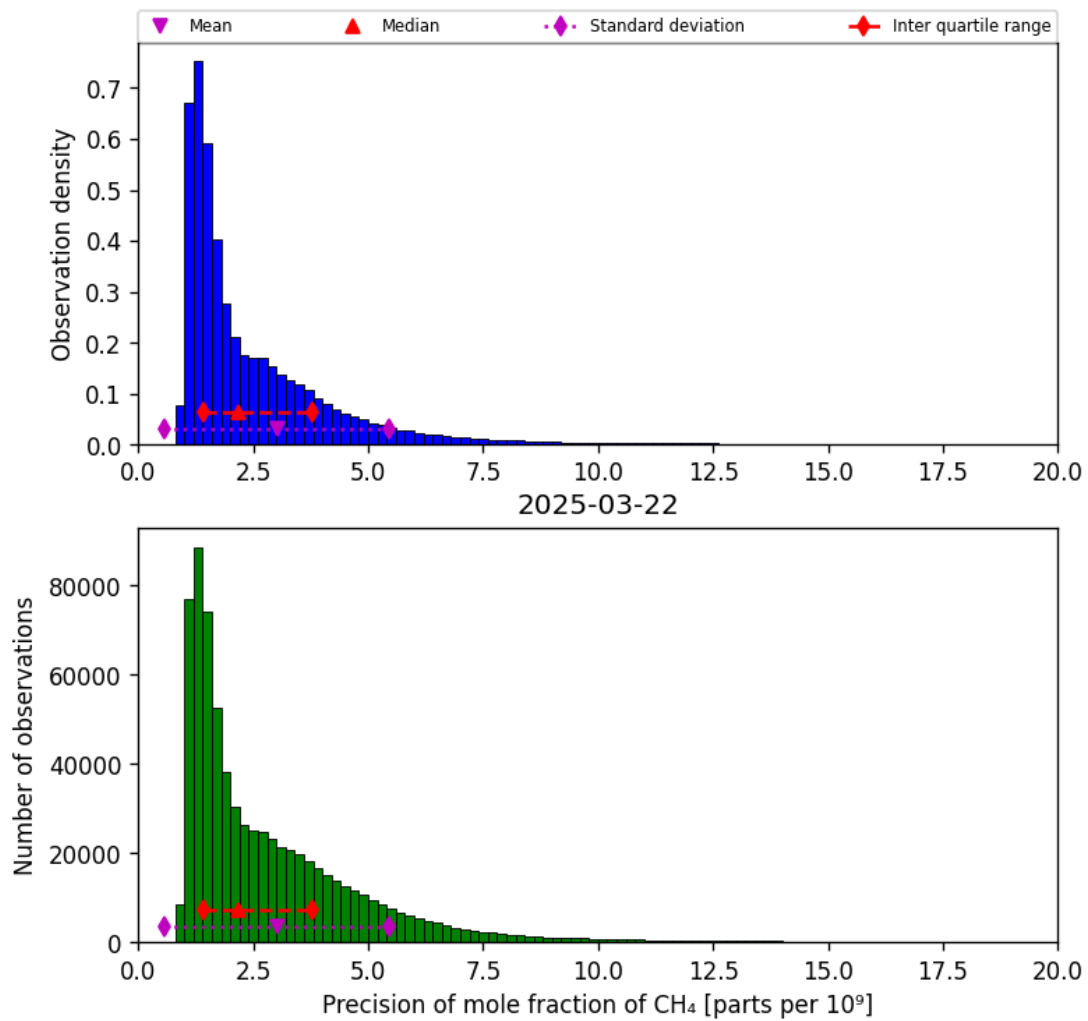
Figure 24: Histogram of “Precision of mole fraction of CH 4 ” for 2025-03-21 to 2025-03-23
