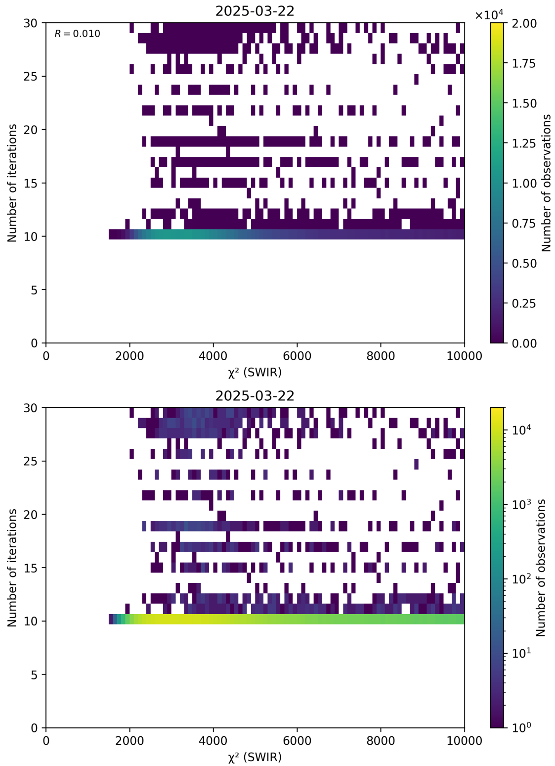
Figure 50: Scatter density plot of “ \chi^2 (SWIR)” against “Number of iterations” for 2025-03-21 to 2025-03-23.
