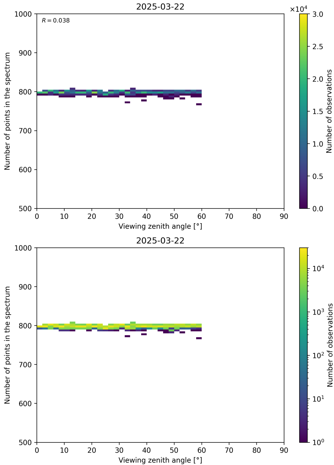
Figure 114: Scatter density plot of “Viewing zenith angle” against “Number of points in the spectrum” for 2025-03-21 to 2025-03-23.
