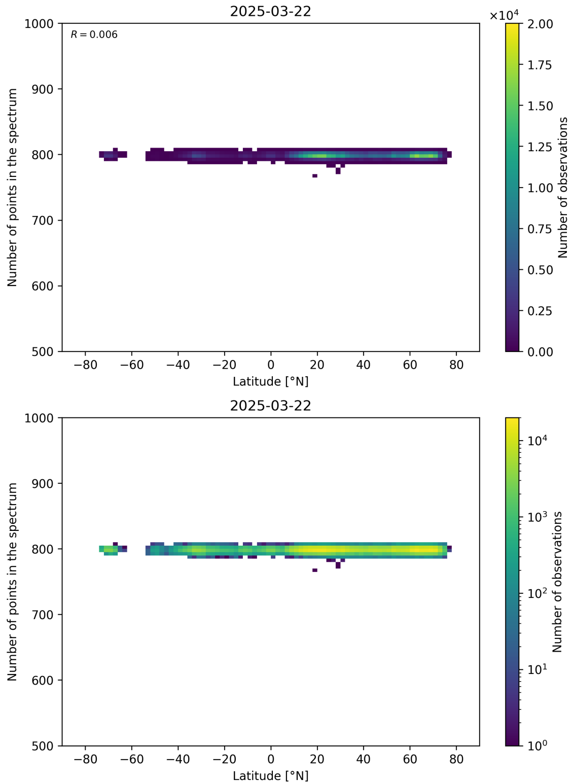
Figure 61: Scatter density plot of “Latitude” against “Number of points in the spectrum” for 2025-03-21 to 2025-03-23.
