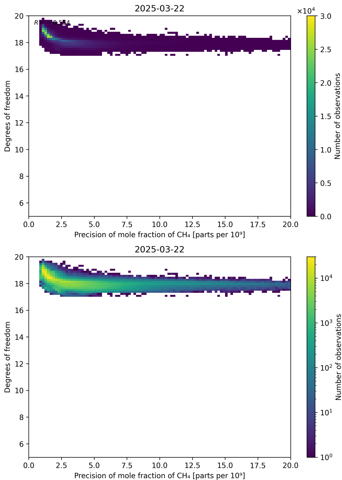
Figure 80: Scatter density plot of “Precision of mole fraction of CH 4 ” against “Degrees of freedom” for 2025-03-21 to 2025-03-23.
