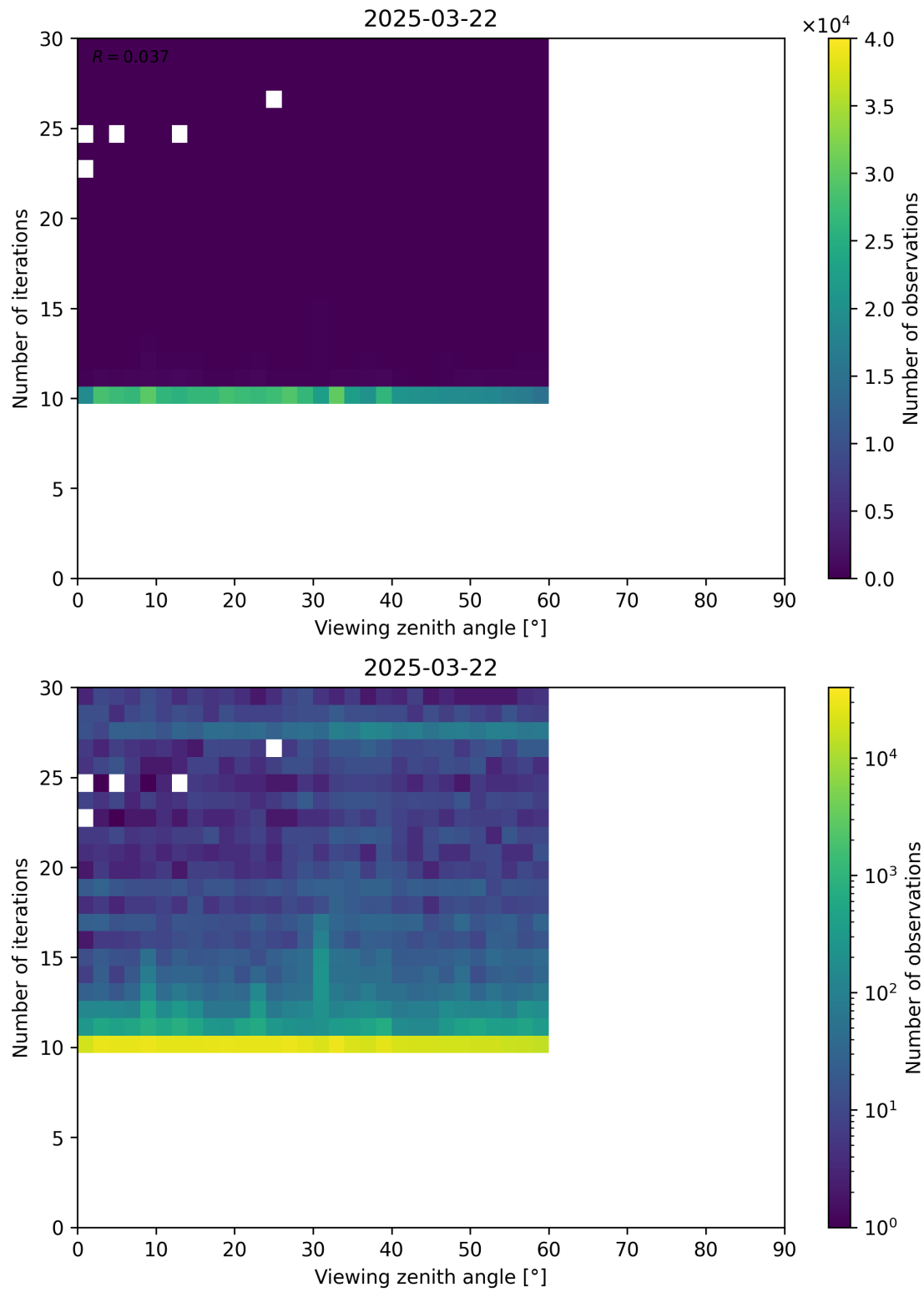
Figure 113: Scatter density plot of “Viewing zenith angle” against “Number of iterations” for 2025-03-21 to 2025-03-23.
