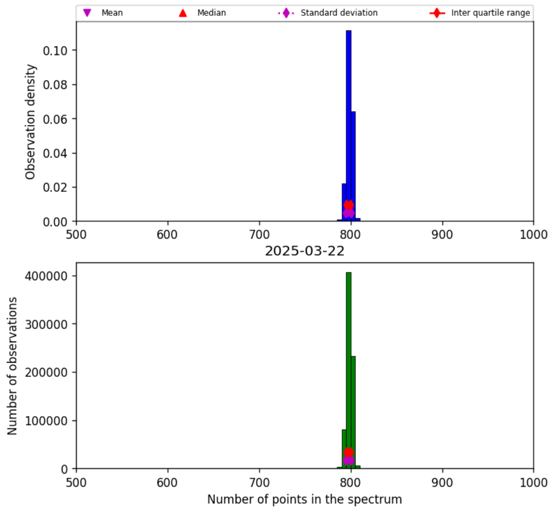
Figure 26: Histogram of “Number of points in the spectrum” for 2025-03-21 to 2025-03-23
