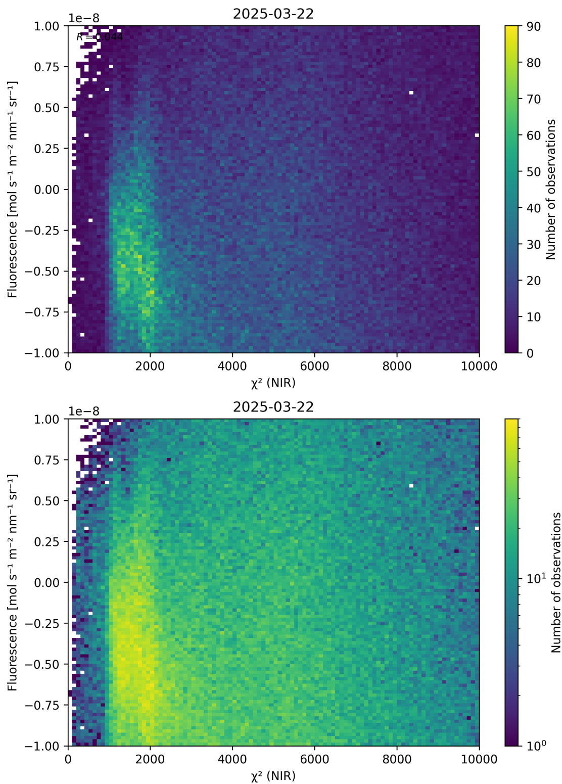
Figure 45: Scatter density plot of “ \chi^2 (NIR)” against “Fluorescence” for 2025-03-21 to 2025-03-23.
