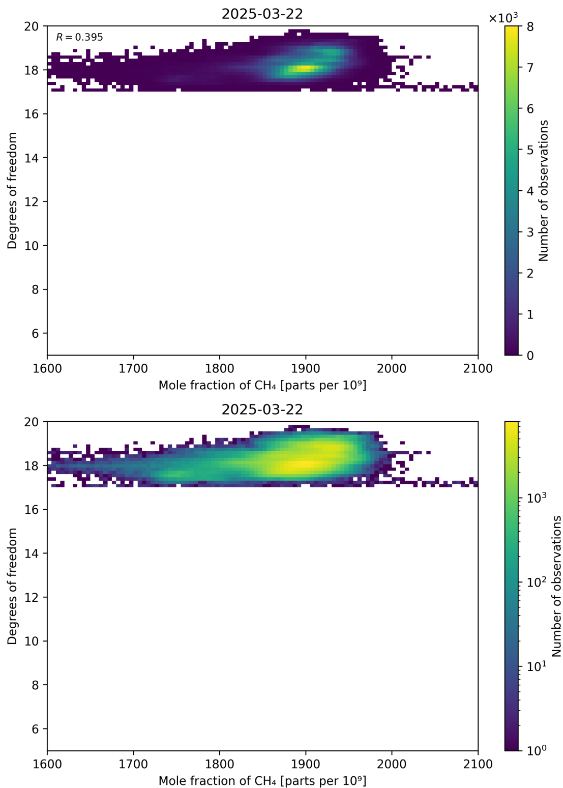
Figure 72: Scatter density plot of “Mole fraction of CH 4 ” against “Degrees of freedom” for 2025-03-21 to 2025-03-23.
