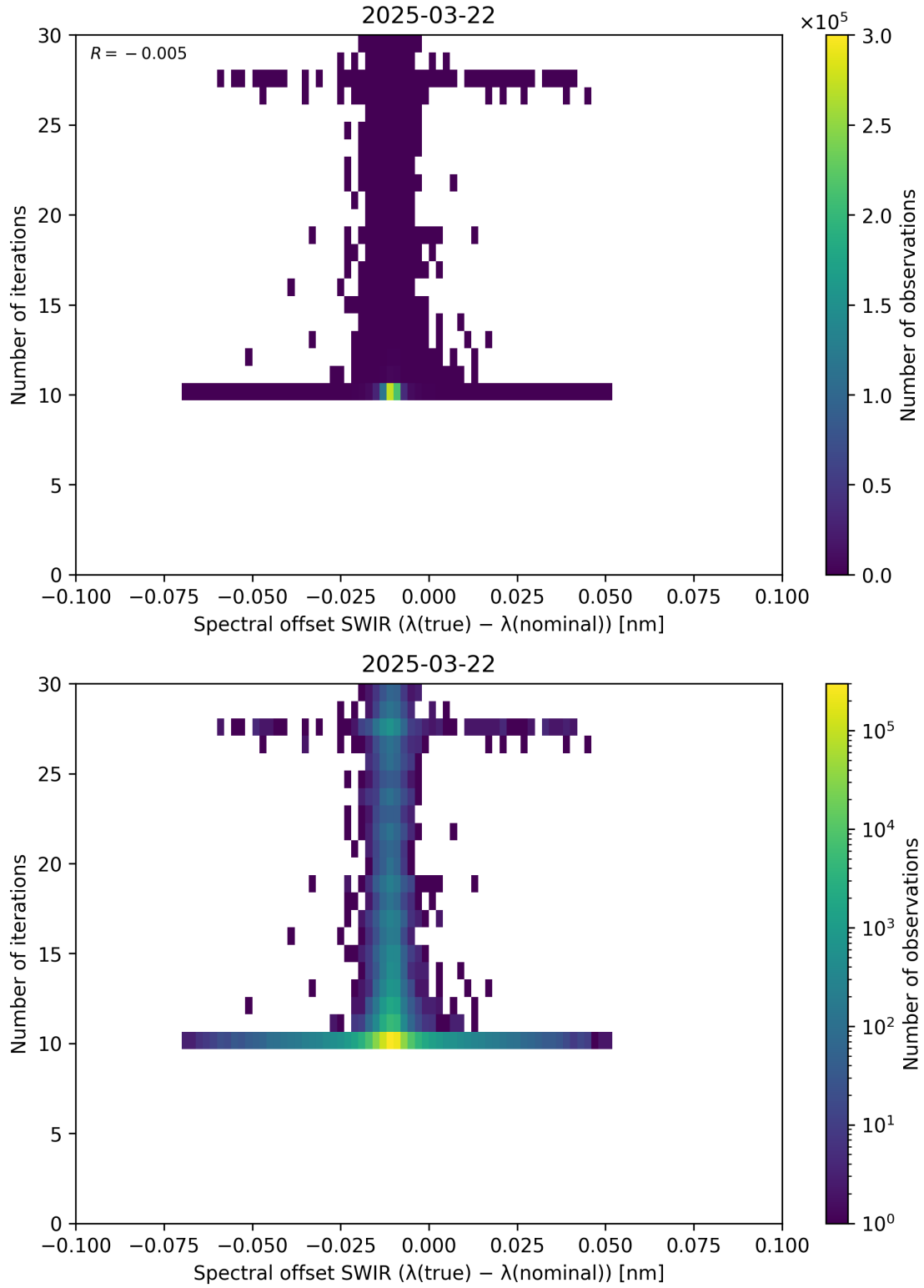
Figure 121: Scatter density plot of “Spectral offset SWIR ( \lambda_{\text{true}} - \lambda_{\text{nominal}} )” against “Number of iterations” for 2025-03-21 to 2025-03-23.
