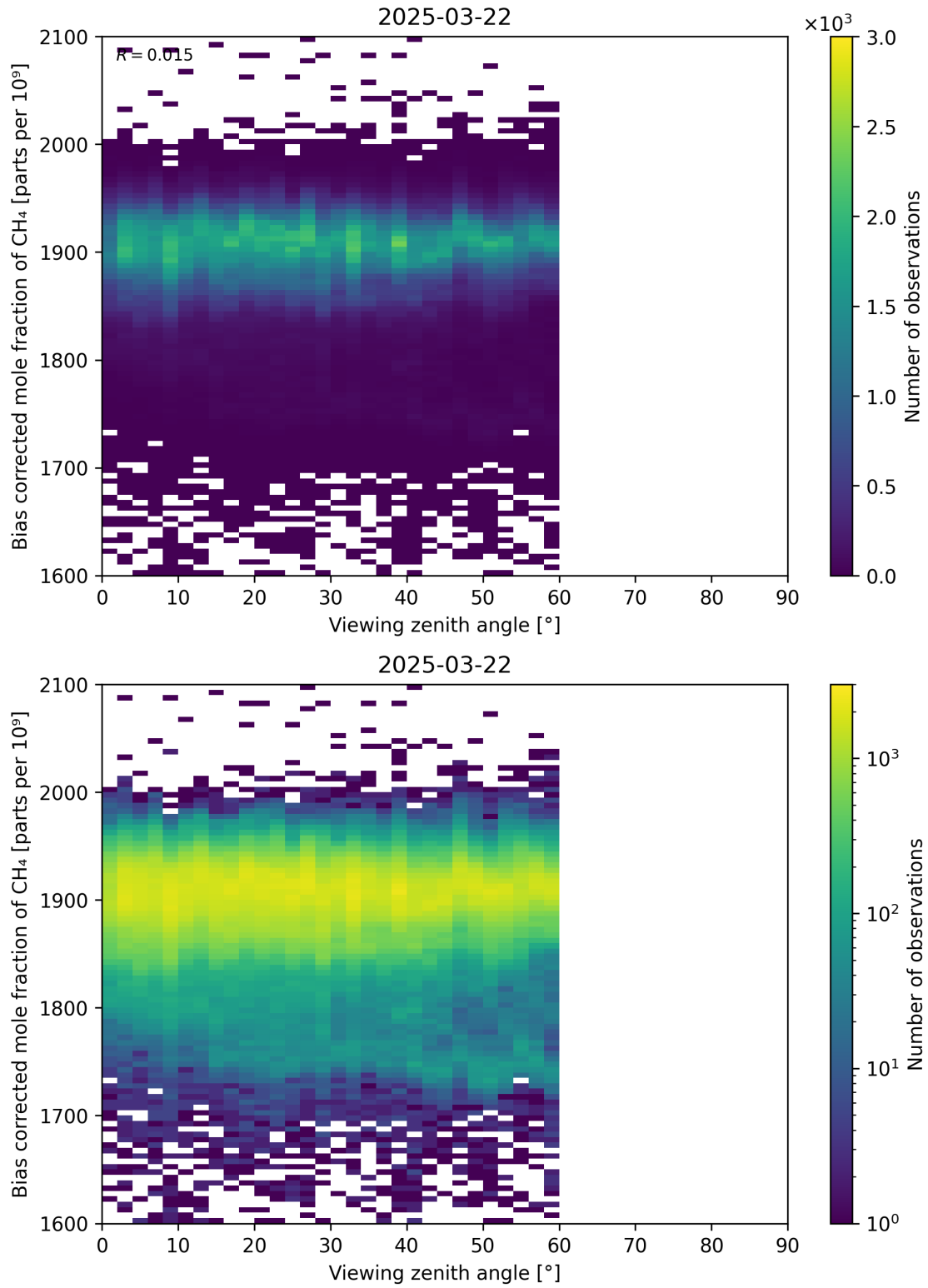
Figure 111: Scatter density plot of “Viewing zenith angle” against “Bias corrected mole fraction of CH 4 ” for 2025-03-21 to 2025-03-23.
