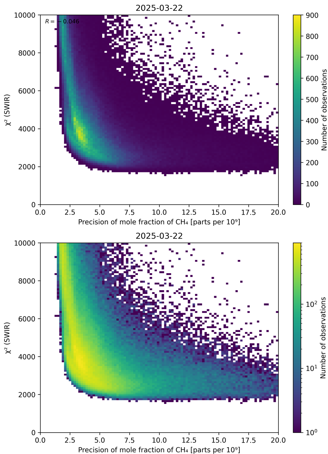
Figure 79: Scatter density plot of “Precision of mole fraction of \text{CH}_4 ” against “ \chi^2 (SWIR)” for 2025-03-21 to 2025-03-23.
