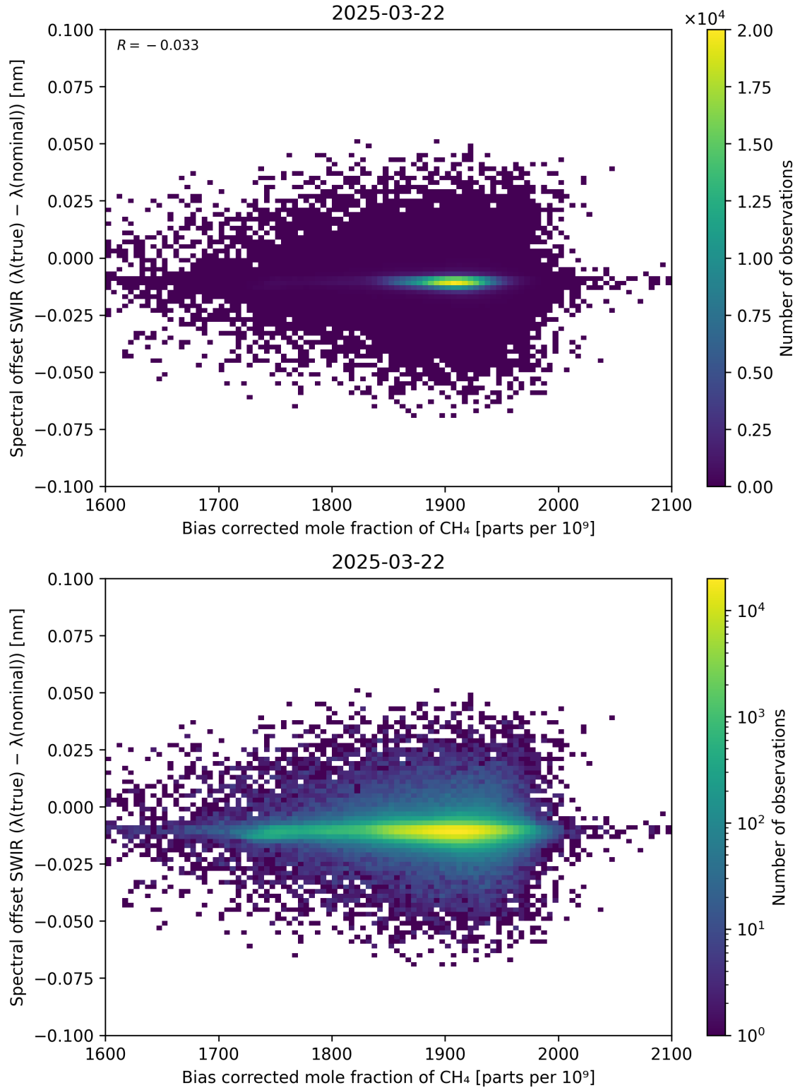
Figure 69: Scatter density plot of “Bias corrected mole fraction of CH 4 ” against “Spectral offset SWIR ( \lambda_{\text{true}} - \lambda_{\text{nominal}} )” for 2025-03-21 to 2025-03-23.
