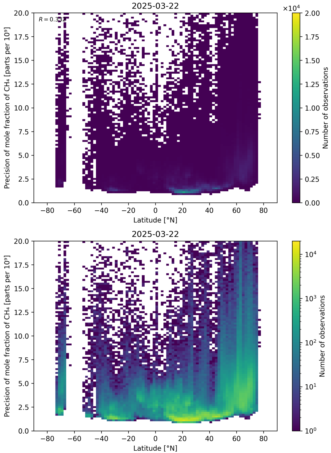
Figure 59: Scatter density plot of “Latitude” against “Precision of mole fraction of \text{CH}_4 ” for 2025-03-21 to 2025-03-23.
