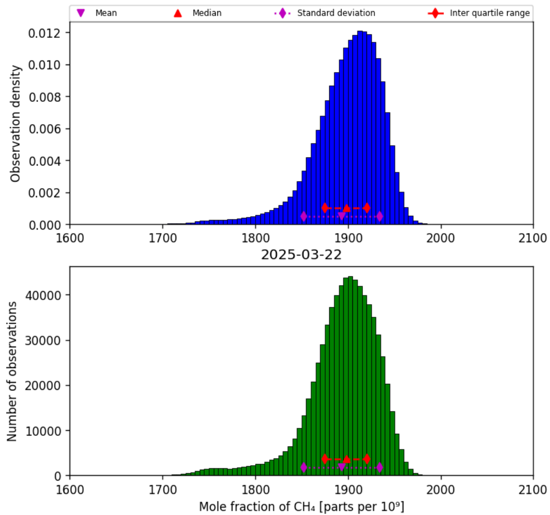
Figure 23: Histogram of “Mole fraction of CH 4 ” for 2025-03-21 to 2025-03-23
