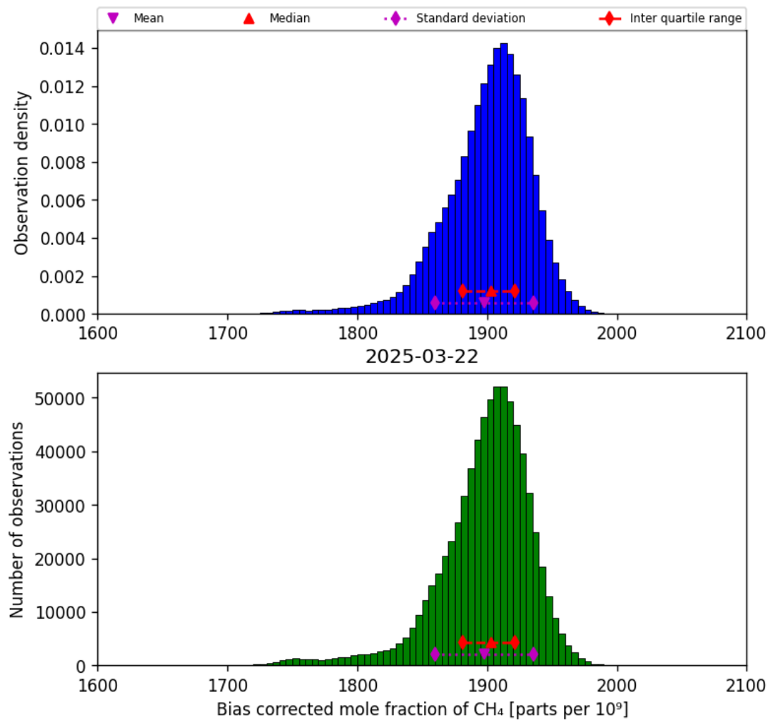
Figure 25: Histogram of “Bias corrected mole fraction of CH 4 ” for 2025-03-21 to 2025-03-23
