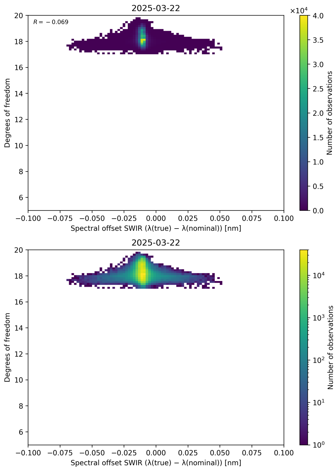
Figure 119: Scatter density plot of “Spectral offset SWIR ( \lambda_{\text{true}} - \lambda_{\text{nominal}} )” against “Degrees of freedom” for 2025-03-21 to 2025-03-23.
