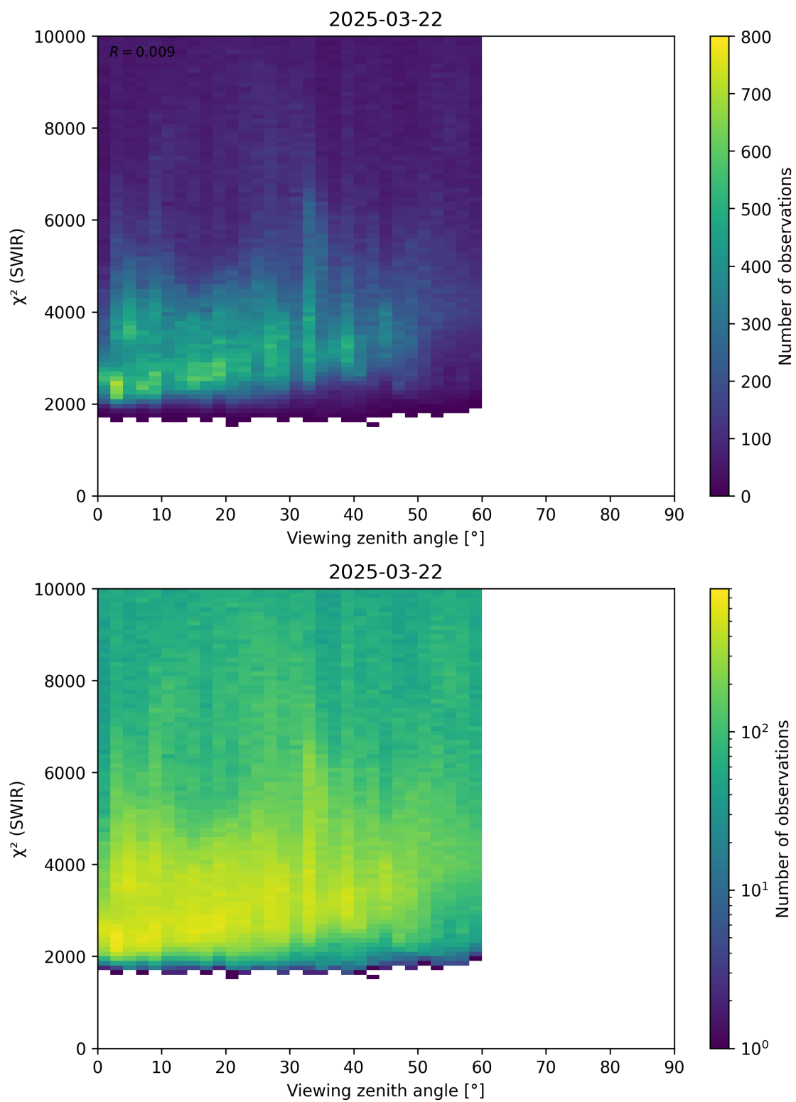
Figure 106: Scatter density plot of “Viewing zenith angle” against “ \chi^2 (SWIR)” for 2025-03-21 to 2025-03-23.
