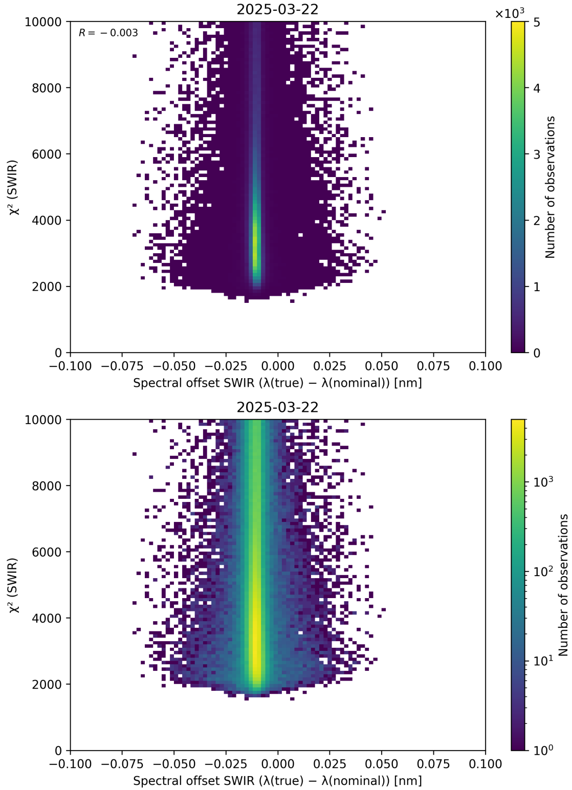
Figure 118: Scatter density plot of “Spectral offset SWIR ( \lambda_{\text{true}} - \lambda_{\text{nominal}} )” against “ \chi^2 (SWIR)” for 2025-03-21 to 2025-03-23.
