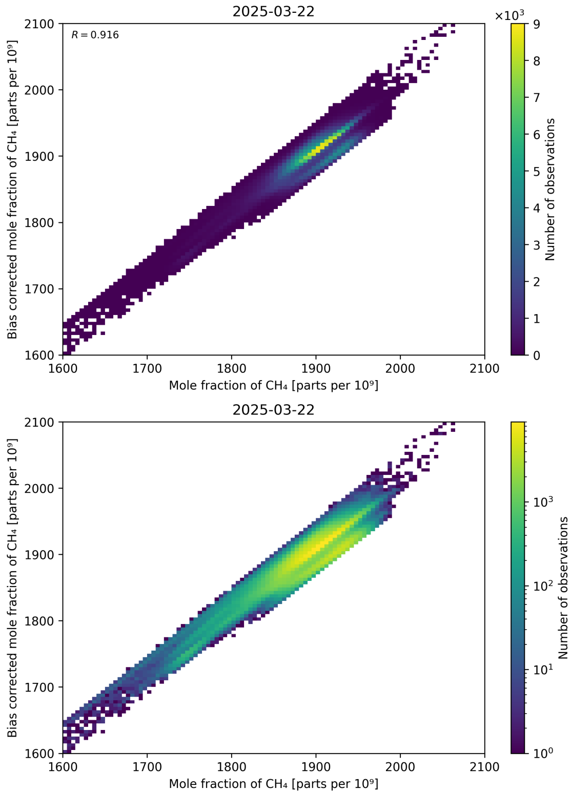
Figure 74: Scatter density plot of “Mole fraction of CH 4 ” against “Bias corrected mole fraction of CH 4 ” for 2025-03-21 to 2025-03-23.
