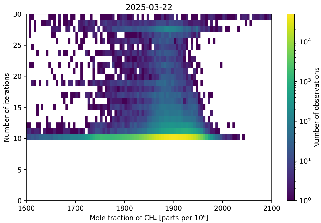
Figure 76: Scatter density plot of “Mole fraction of CH 4 ” against “Number of iterations” for 2025-03-21 to 2025-03-23.
