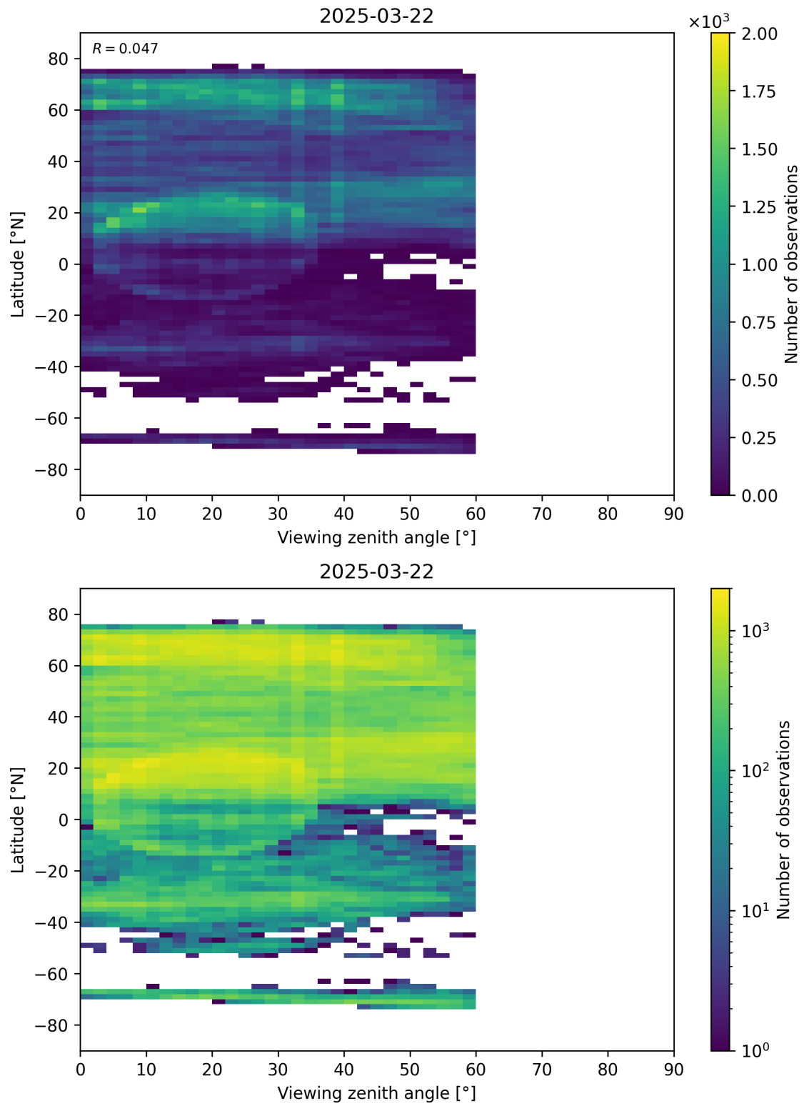
Figure 109: Scatter density plot of “Viewing zenith angle” against “Latitude” for 2025-03-21 to 2025-03-23.
