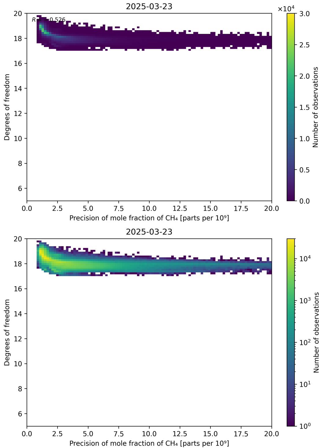
Figure 80: Scatter density plot of “Precision of mole fraction of CH 4 ” against “Degrees of freedom” for 2025-03-23 to 2025-03-24.
