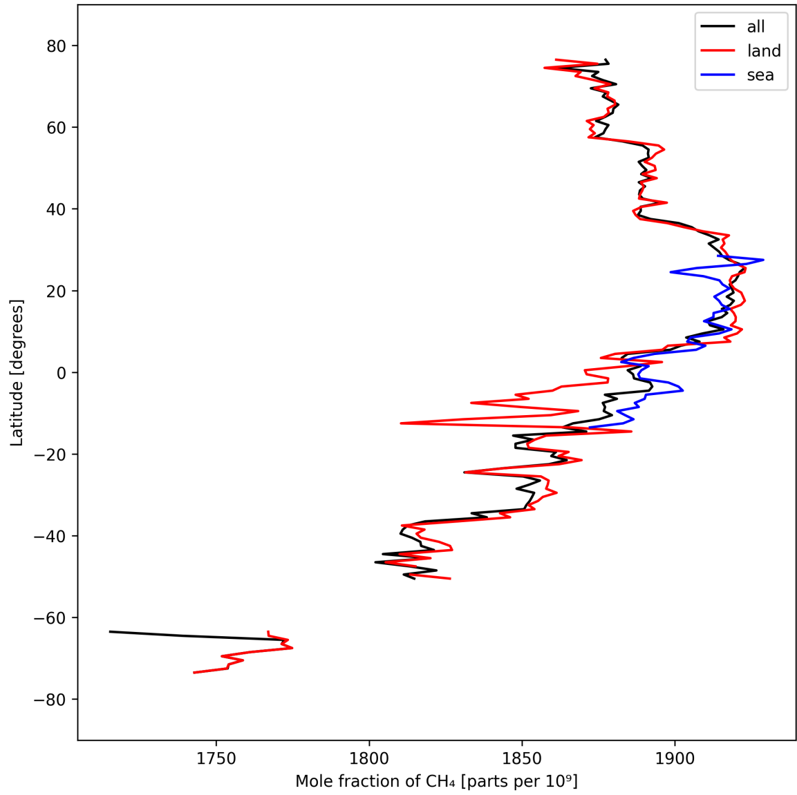
Figure 12: Zonal average of “Mole fraction of CH 4 ” for 2025-03-23 to 2025-03-24.
