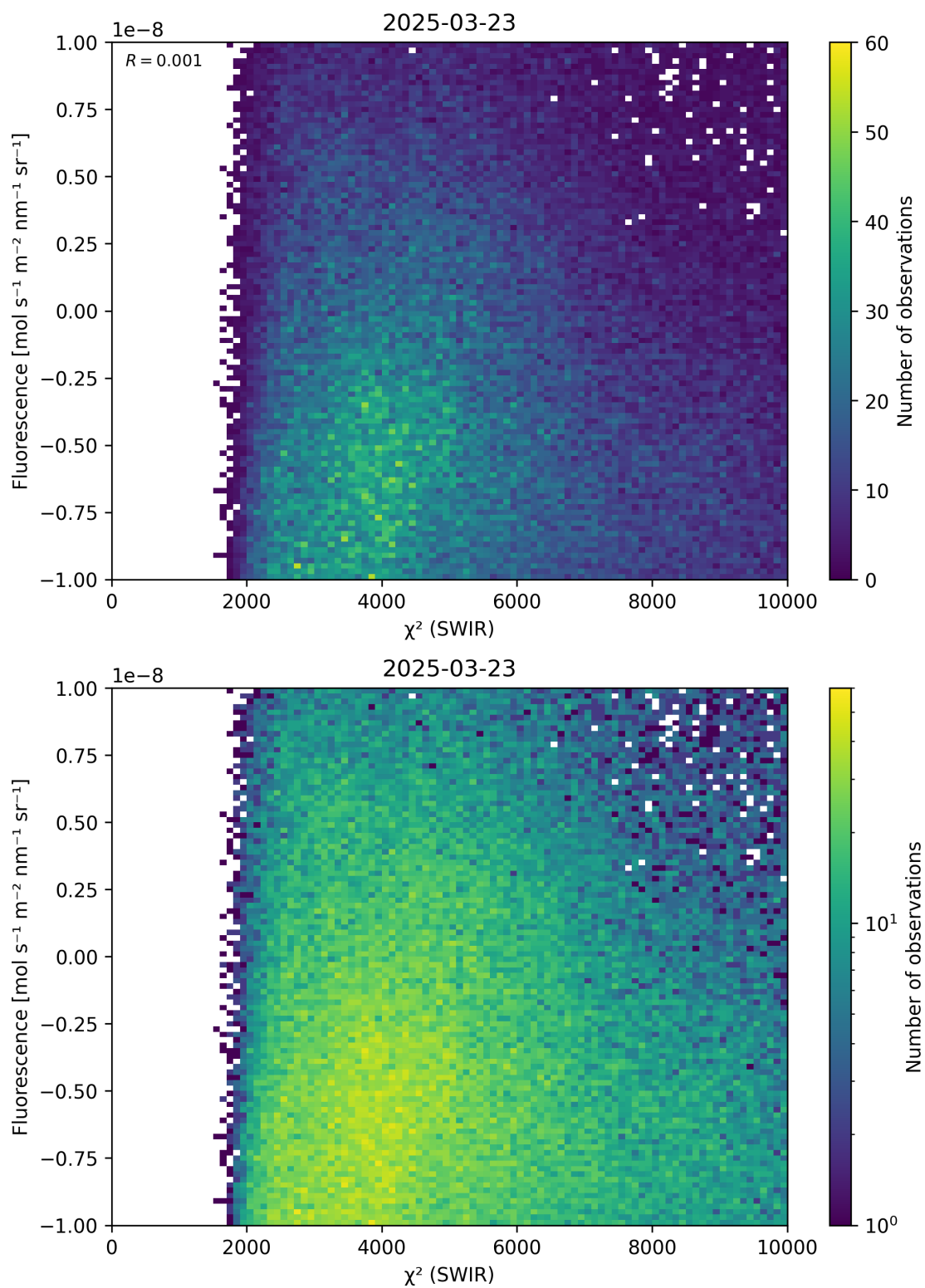
Figure 49: Scatter density plot of “ \chi^2 (SWIR)” against “Fluorescence” for 2025-03-23 to 2025-03-24.
