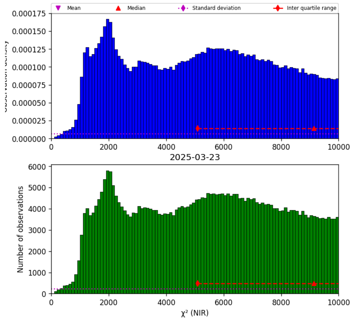
Figure 29: Histogram of “ \chi^2 (NIR)” for 2025-03-23 to 2025-03-24
