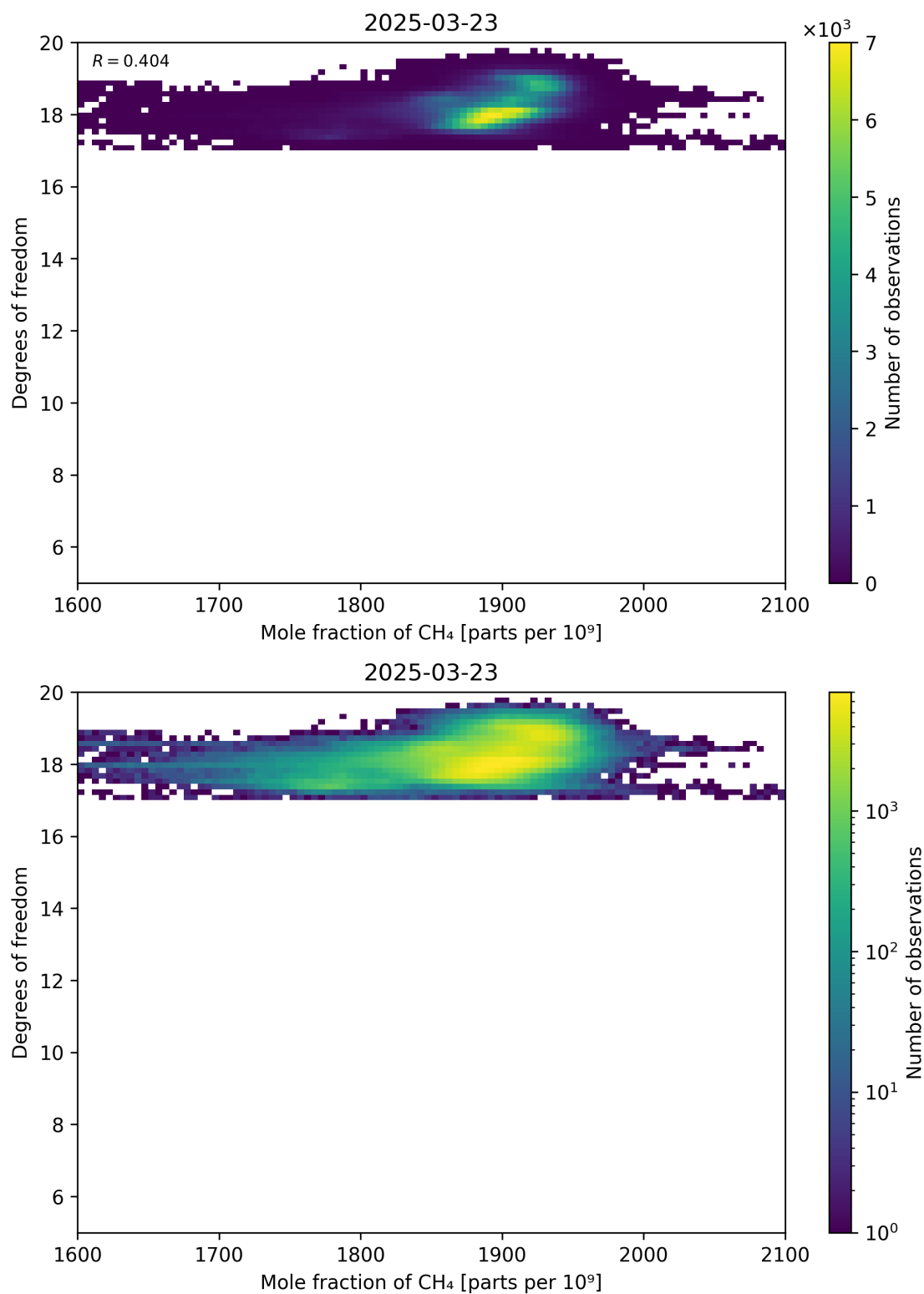
Figure 72: Scatter density plot of “Mole fraction of CH 4 ” against “Degrees of freedom” for 2025-03-23 to 2025-03-24.
