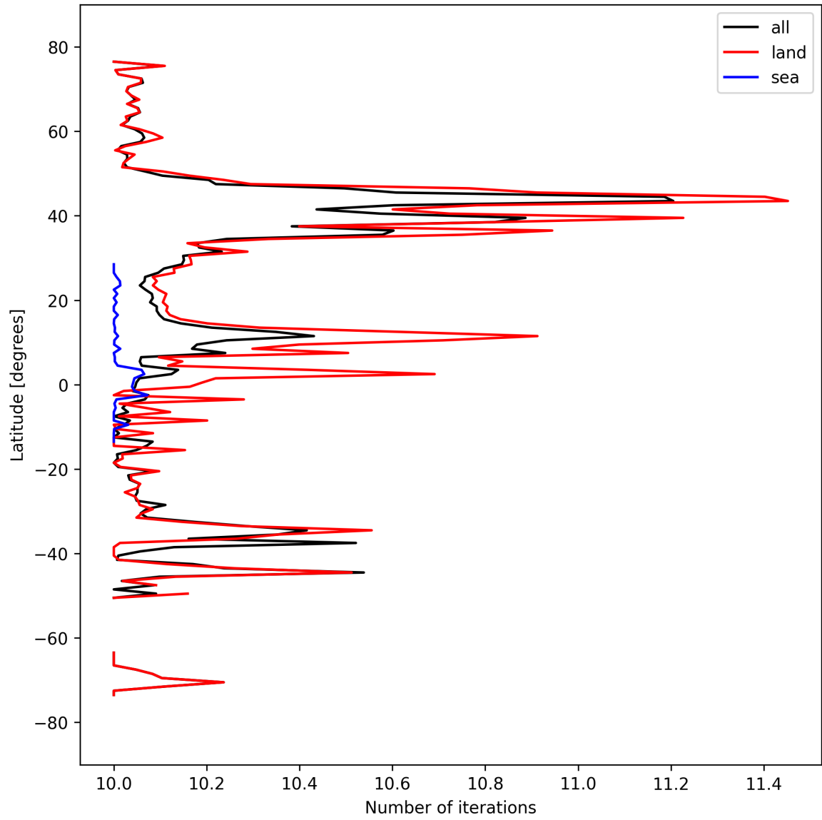
Figure 20: Zonal average of “Number of iterations” for 2025-03-23 to 2025-03-24.
