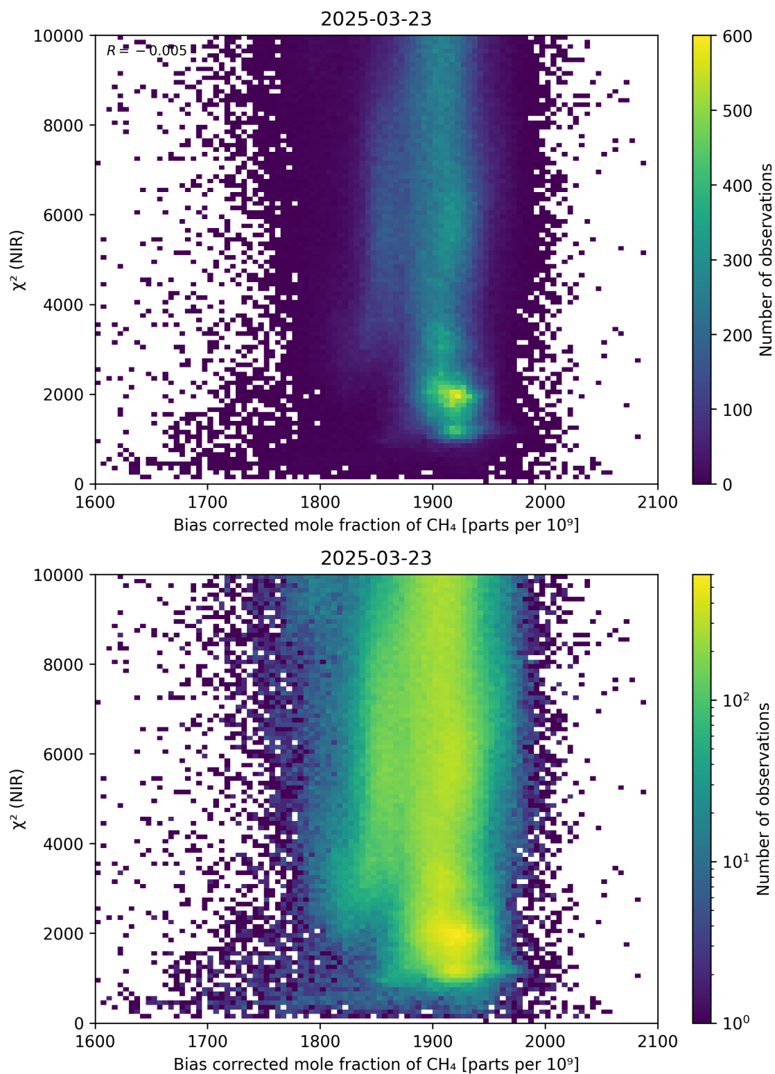
Figure 63: Scatter density plot of “Bias corrected mole fraction of \text{CH}_4 ” against “ \chi^2 (NIR)” for 2025-03-23 to 2025-03-24.
