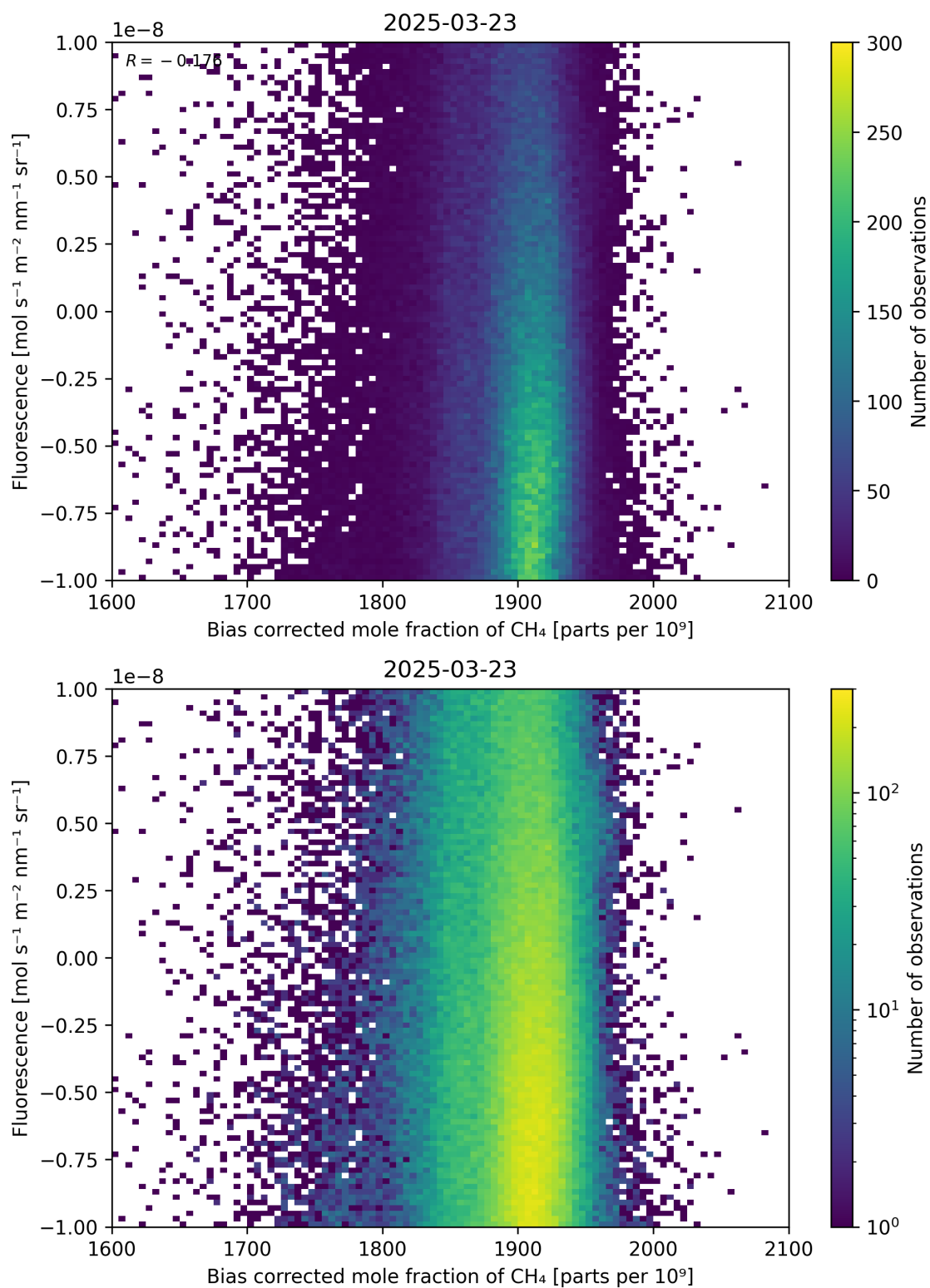
Figure 66: Scatter density plot of “Bias corrected mole fraction of \text{CH}_4 ” against “Fluorescence” for 2025-03-23 to 2025-03-24.
