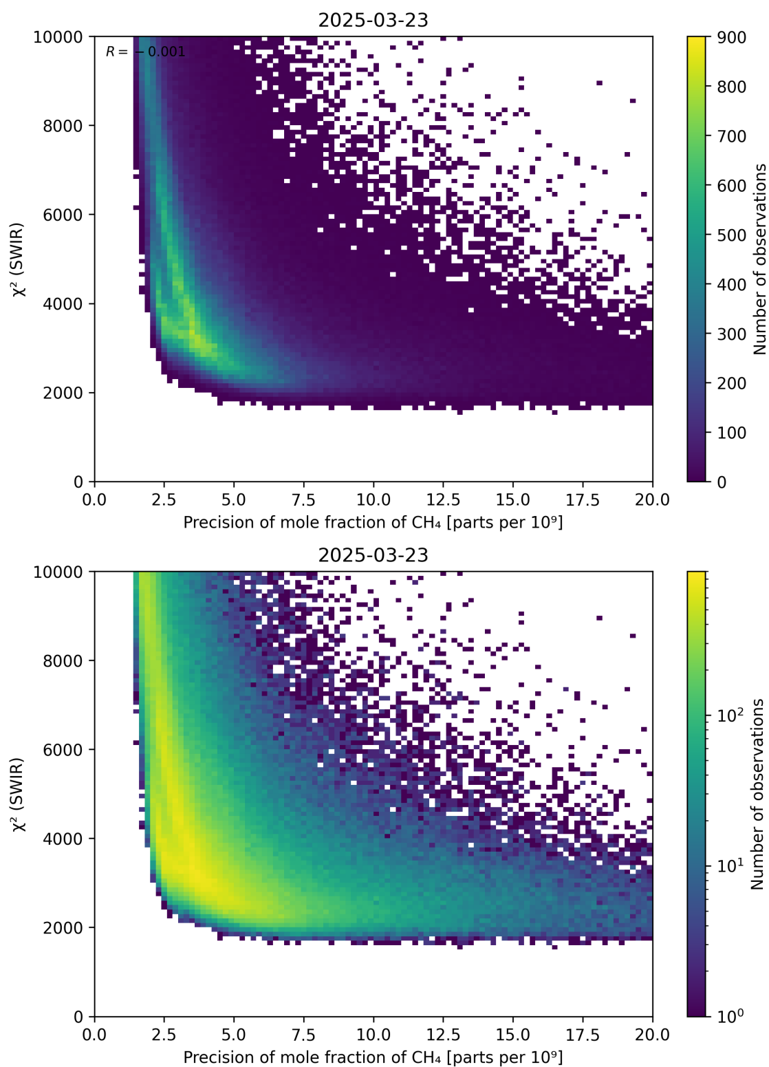
Figure 79: Scatter density plot of “Precision of mole fraction of \text{CH}_4 ” against “ \chi^2 (SWIR)” for 2025-03-23 to 2025-03-24.
