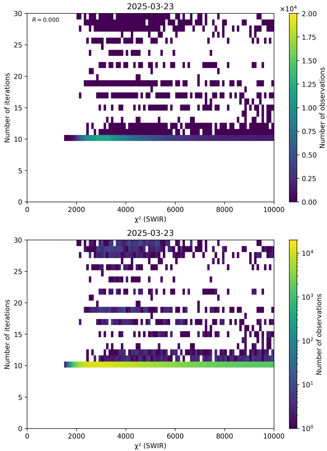
Figure 50: Scatter density plot of “ \chi^2 (SWIR)” against “Number of iterations” for 2025-03-23 to 2025-03-24.
