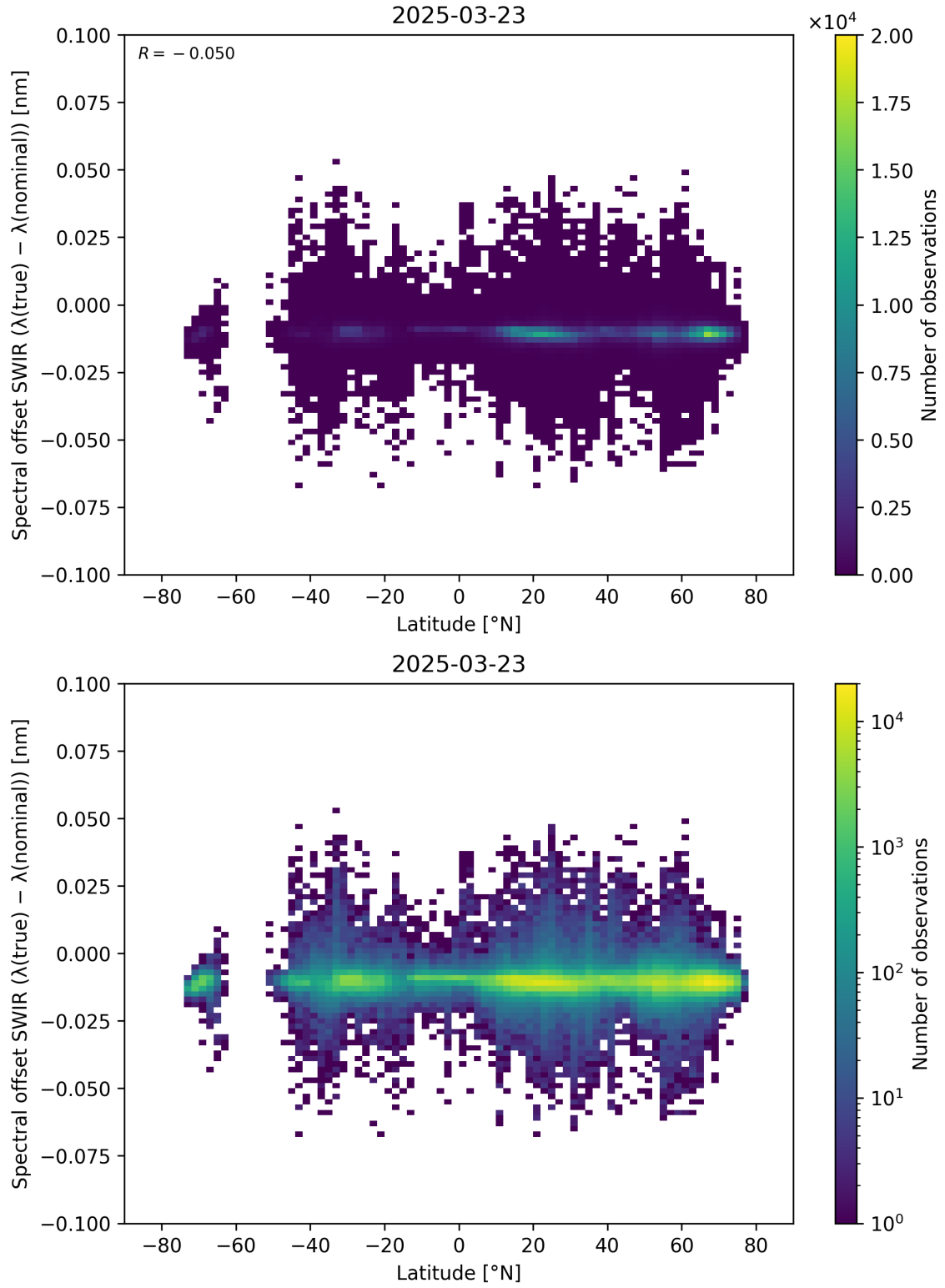
Figure 62: Scatter density plot of “Latitude” against “Spectral offset SWIR ( \lambda_{\text{true}} - \lambda_{\text{nominal}} )” for 2025-03-23 to 2025-03-24.
