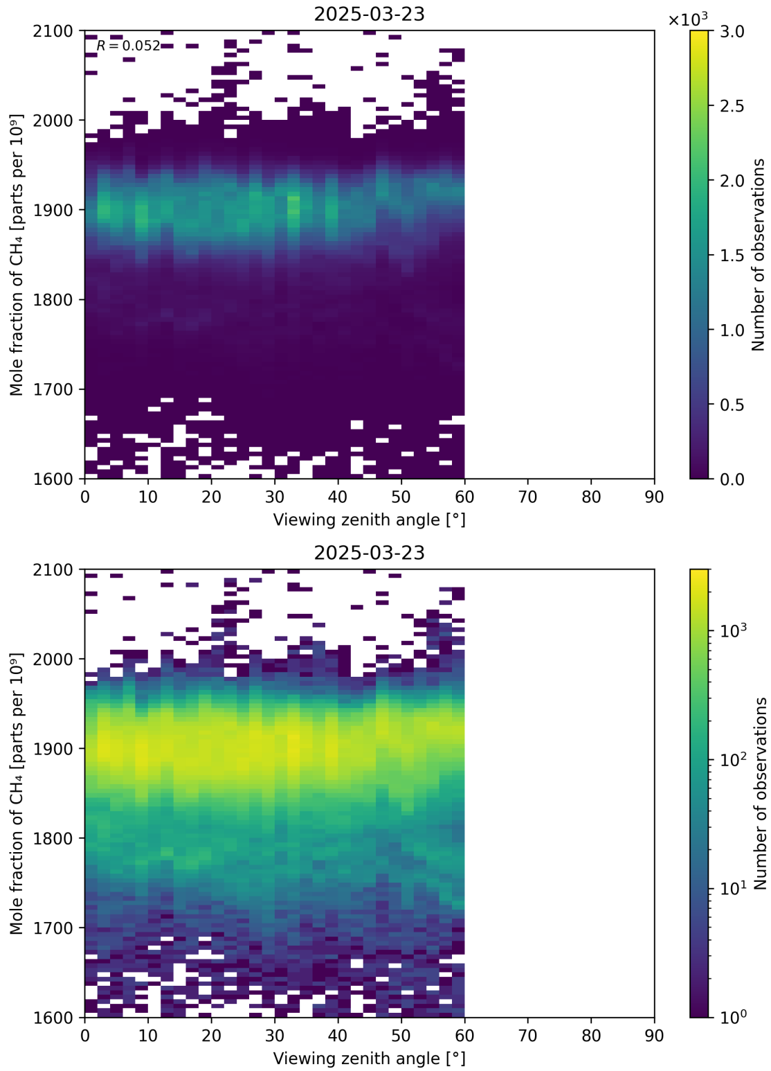
Figure 110: Scatter density plot of “Viewing zenith angle” against “Mole fraction of CH 4 ” for 2025-03-23 to 2025-03-24.
