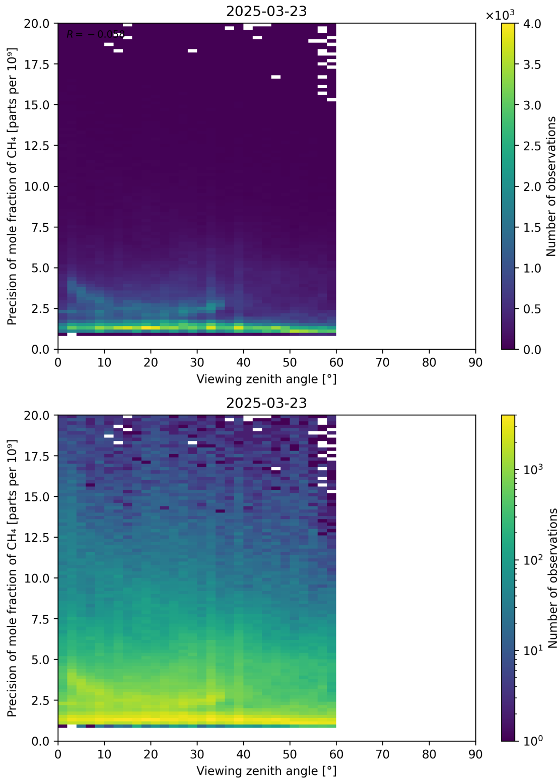
Figure 112: Scatter density plot of “Viewing zenith angle” against “Precision of mole fraction of \text{CH}_4 ” for 2025-03-23 to 2025-03-24.
