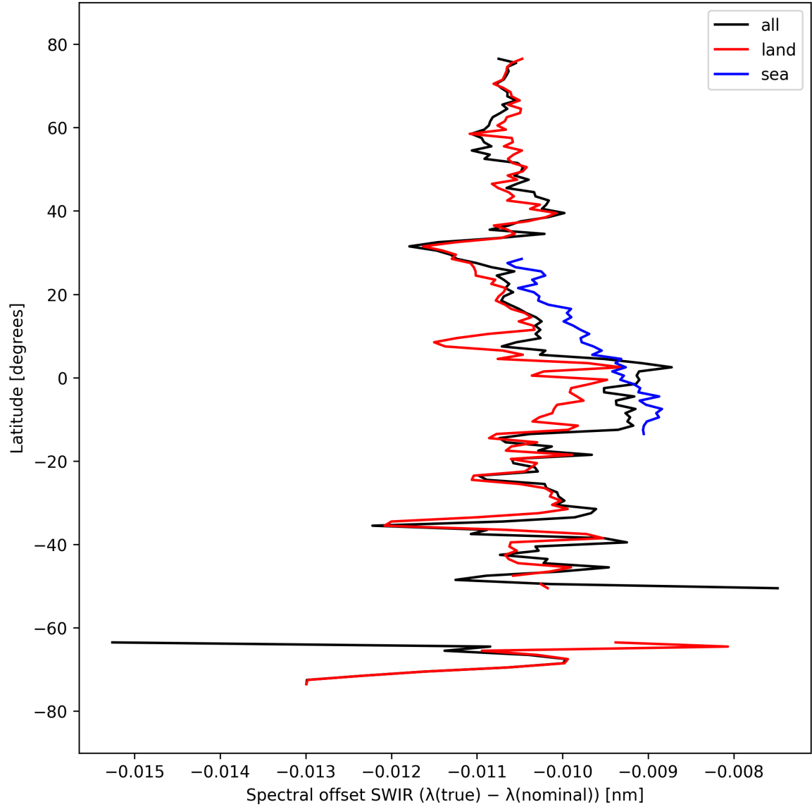
Figure 16: Zonal average of “Spectral offset SWIR ( \lambda_{\text{true}} - \lambda_{\text{nominal}} )” for 2025-03-23 to 2025-03-24.
