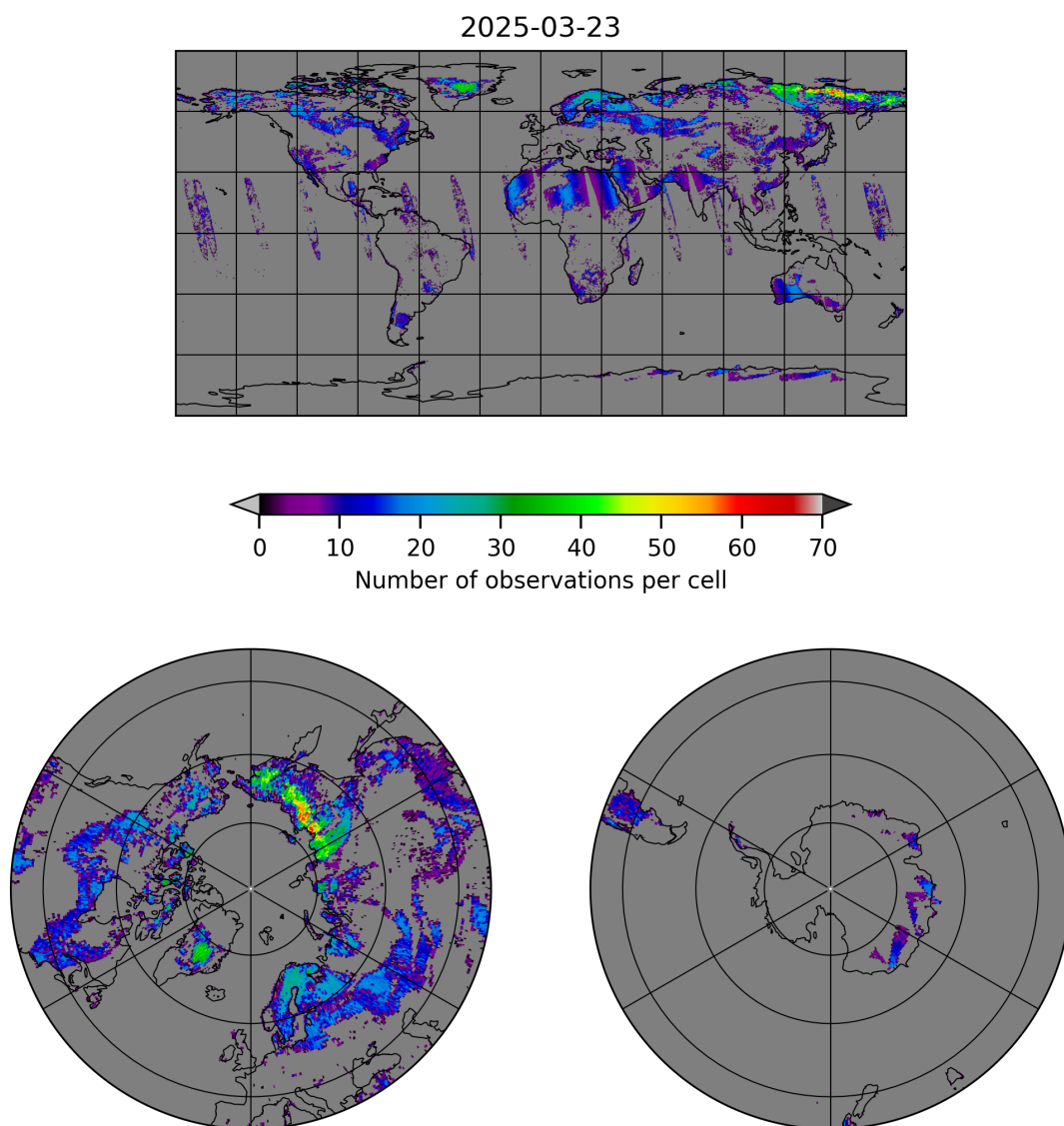
Figure 10: Map of the number of observations for 2025-03-23 to 2025-03-24
