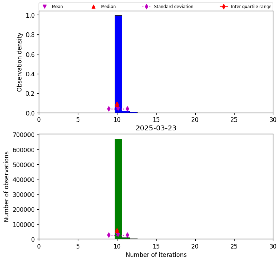
Figure 31: Histogram of “Number of iterations” for 2025-03-23 to 2025-03-24
