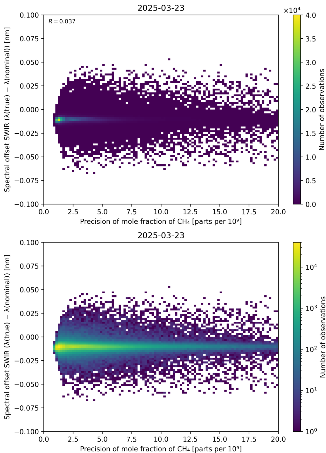
Figure 85: Scatter density plot of “Precision of mole fraction of \text{CH}_4 ” against “Spectral offset SWIR ( \lambda_{\text{true}} - \lambda_{\text{nominal}} )” for 2025-03-23 to 2025-03-24.
