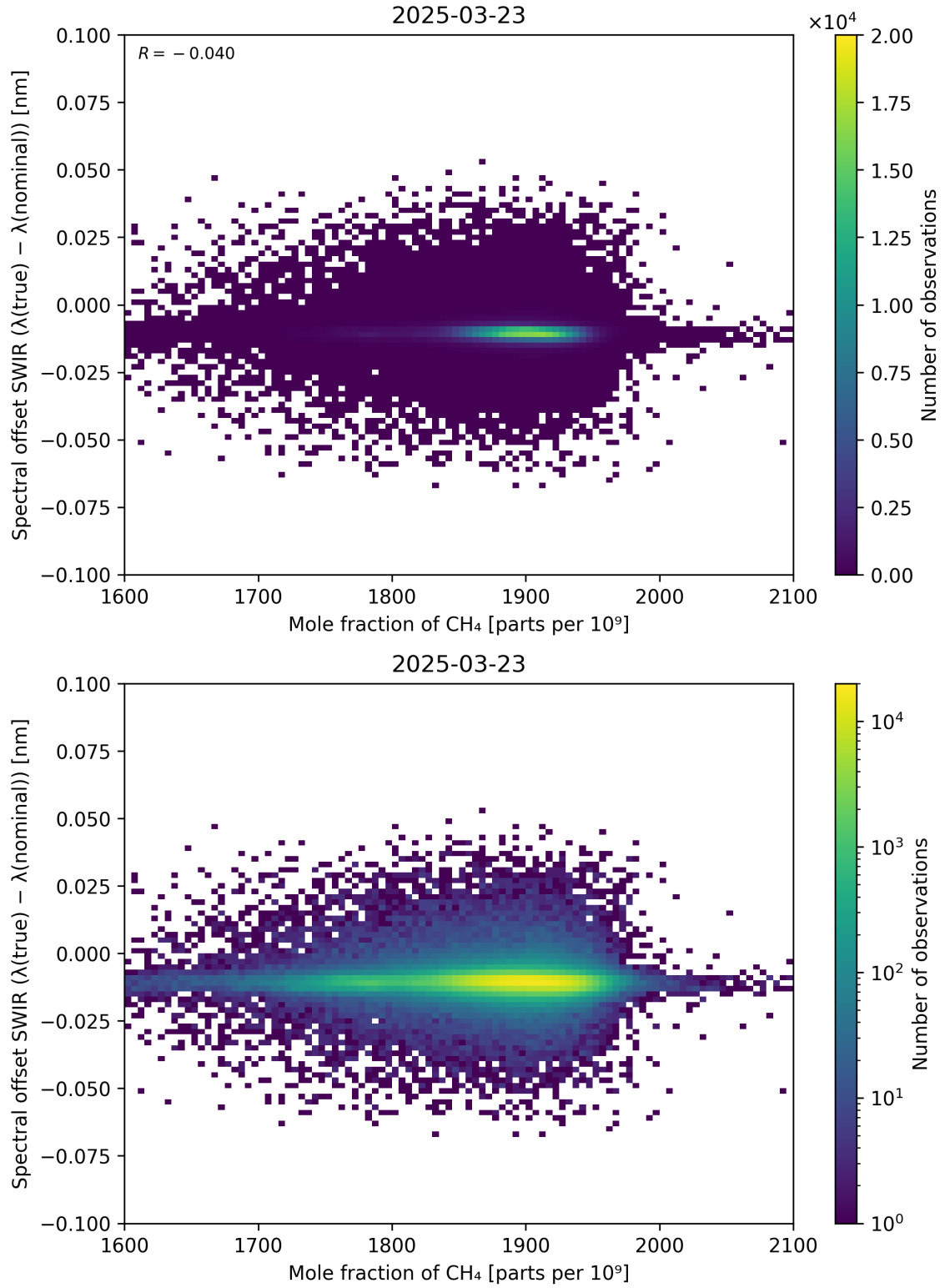
Figure 86: Scatter density plot of “Mole fraction of \text{CH}_4 ” against “Spectral offset SWIR ( \lambda_{\text{true}} - \lambda_{\text{nominal}} )” for 2025-03-23 to 2025-03-24.
