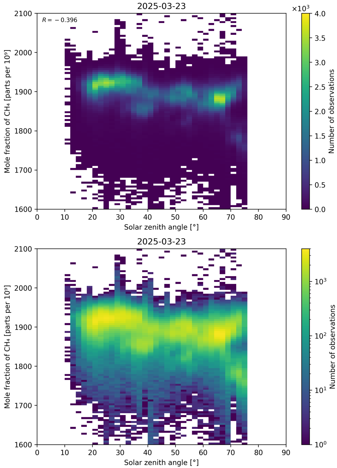
Figure 99: Scatter density plot of “Solar zenith angle” against “Mole fraction of CH 4 ” for 2025-03-23 to 2025-03-24.
