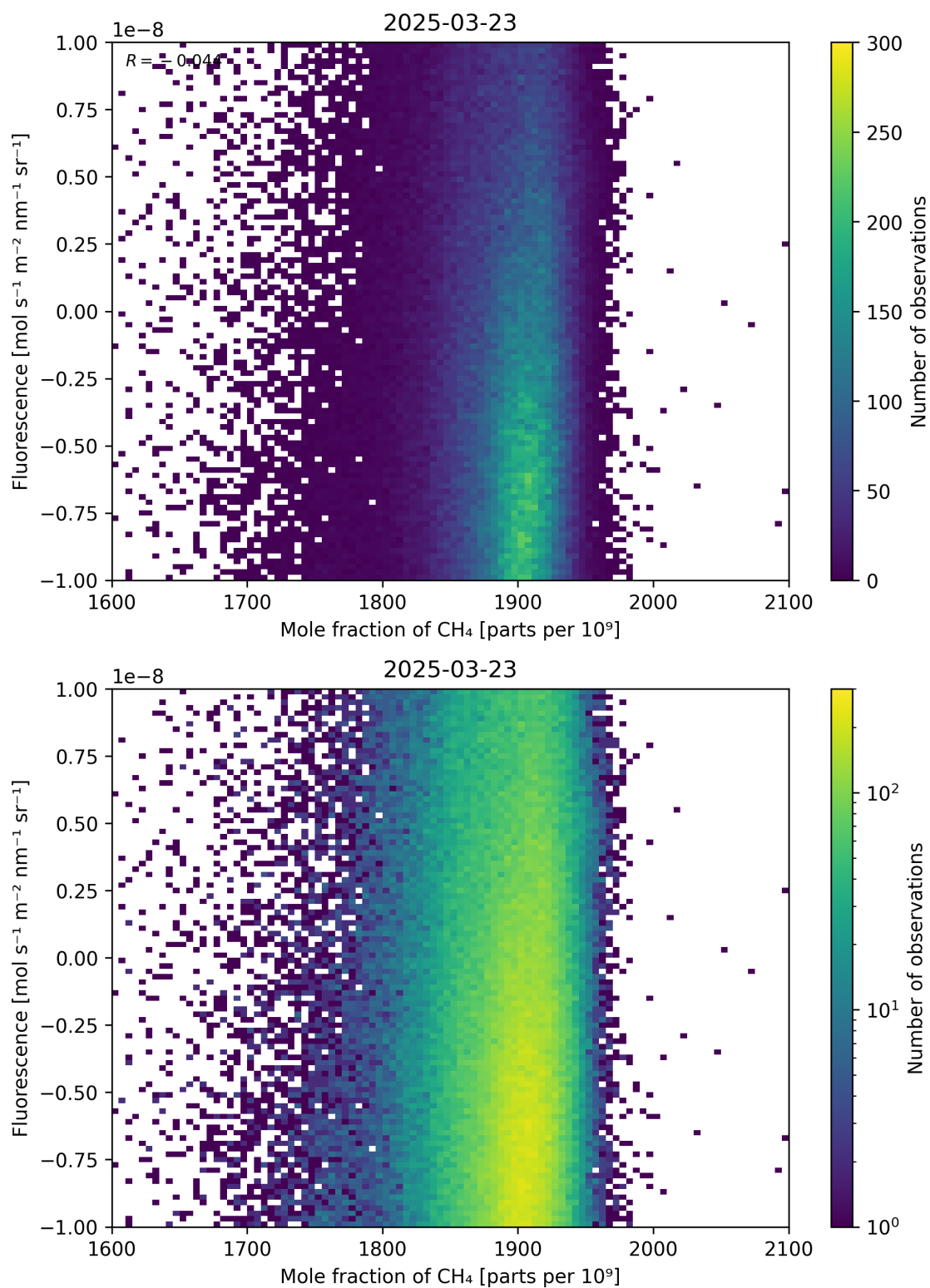
Figure 73: Scatter density plot of “Mole fraction of \text{CH}_4 ” against “Fluorescence” for 2025-03-23 to 2025-03-24.
