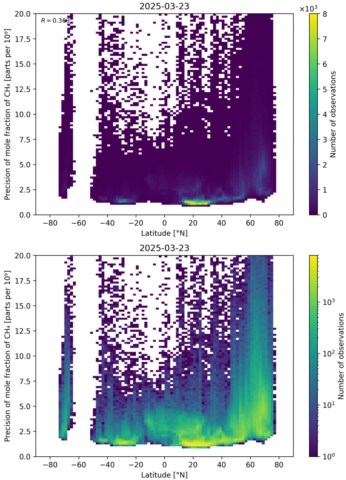
Figure 59: Scatter density plot of “Latitude” against “Precision of mole fraction of CH 4 ” for 2025-03-23 to 2025-03-24.
