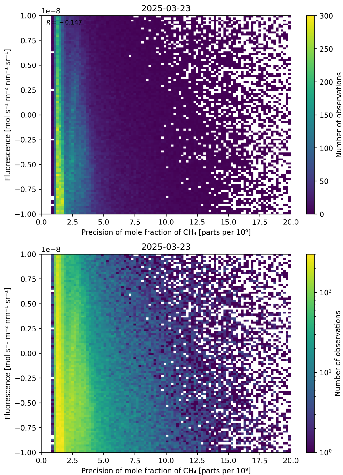
Figure 81: Scatter density plot of “Precision of mole fraction of \text{CH}_4 ” against “Fluorescence” for 2025-03-23 to 2025-03-24.
