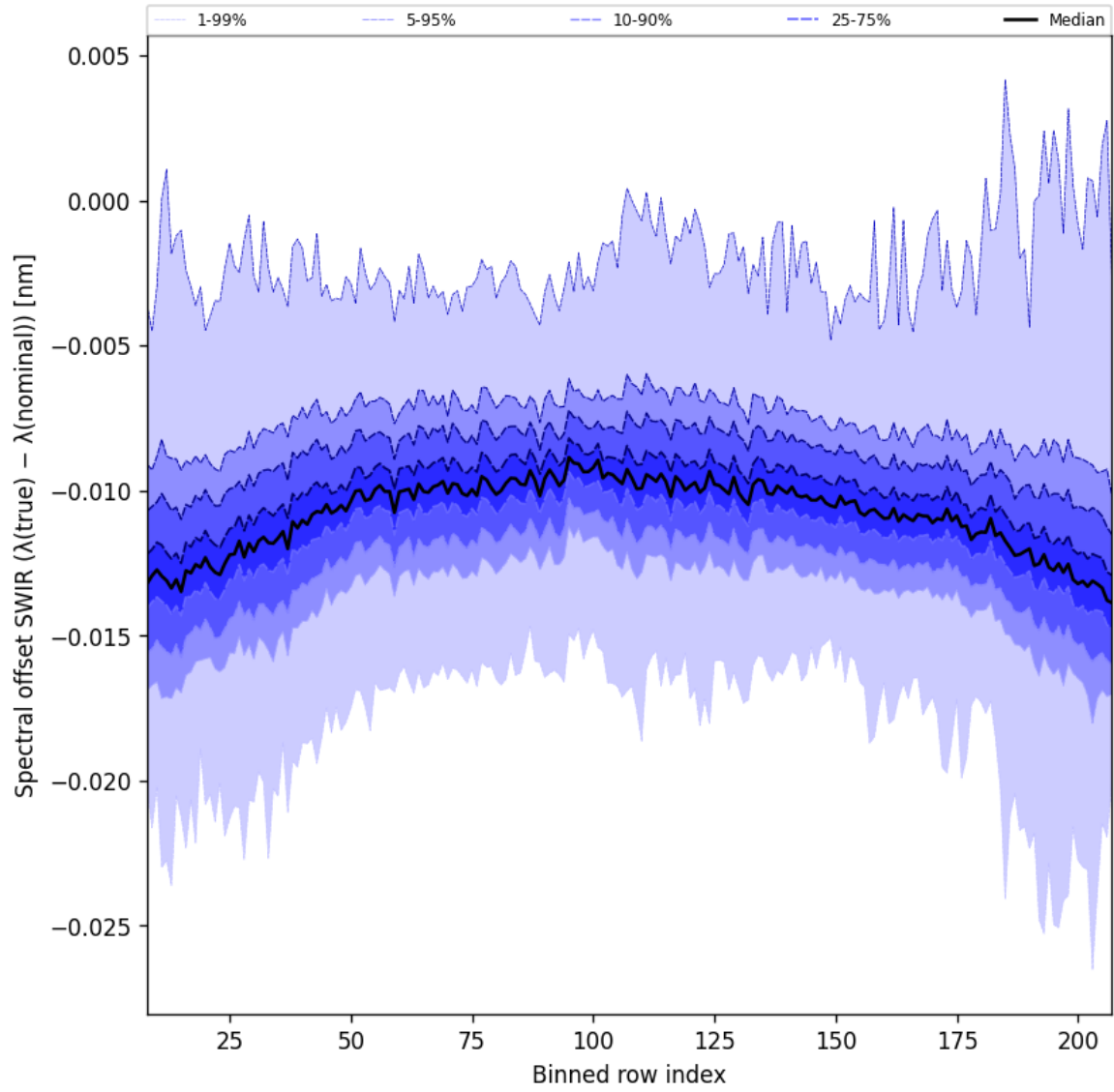
Figure 38: Along track statistics of “Spectral offset SWIR ( \lambda_{\text{true}} - \lambda_{\text{nominal}} )” for 2025-03-23 to 2025-03-24
