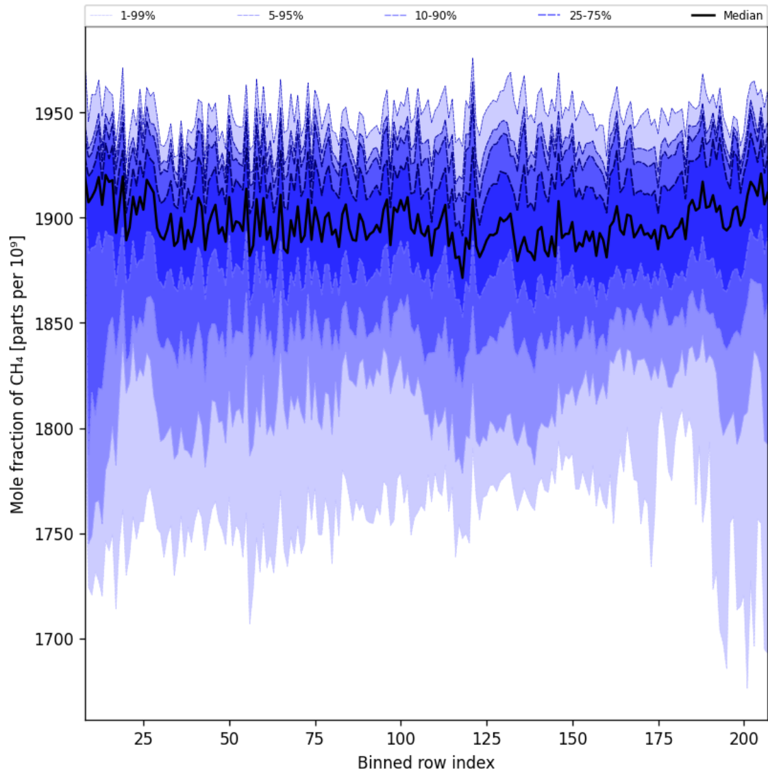
Figure 34: Along track statistics of “Mole fraction of CH 4 ” for 2025-03-23 to 2025-03-24
