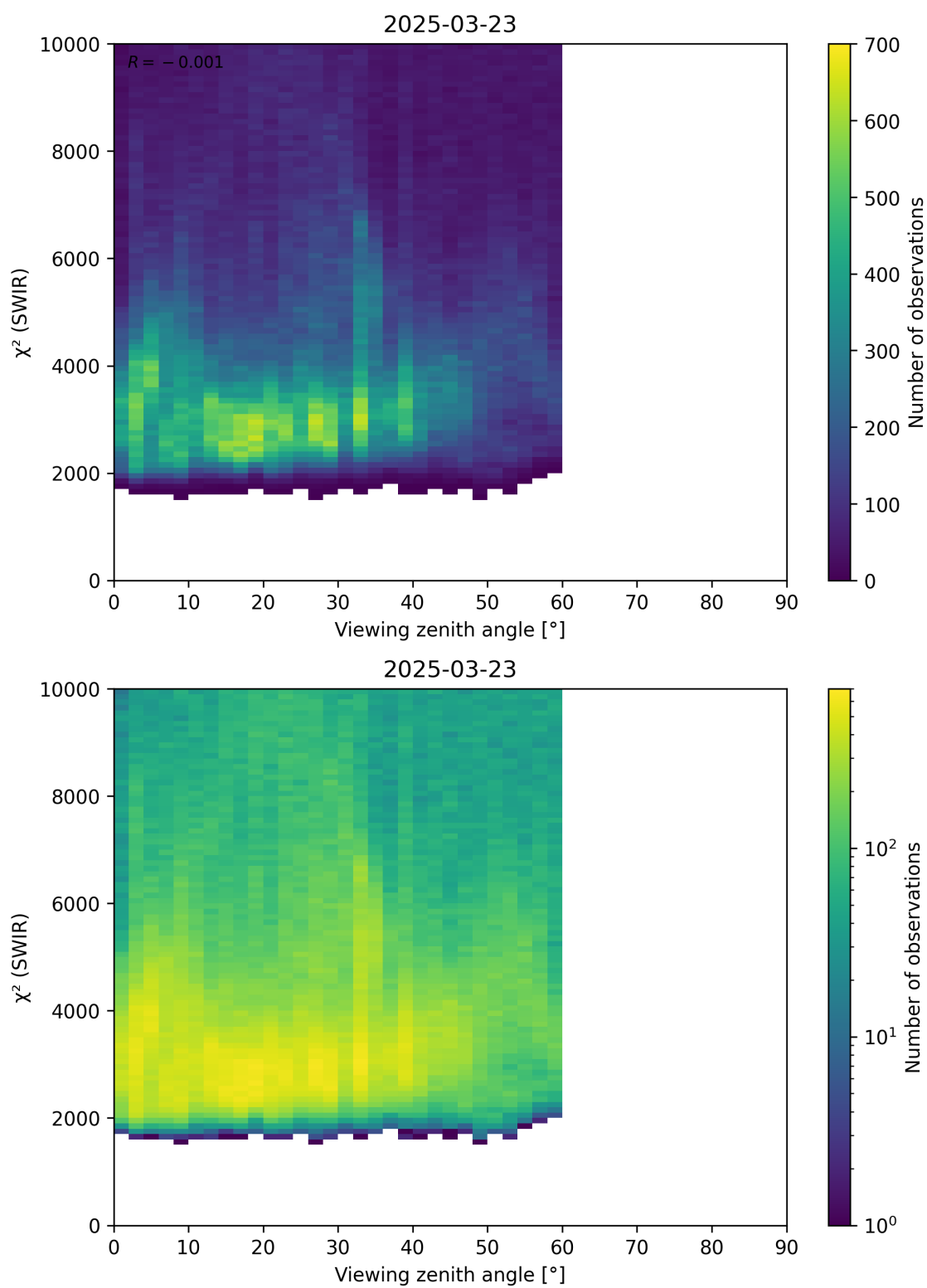
Figure 106: Scatter density plot of “Viewing zenith angle” against “ \chi^2 (SWIR)” for 2025-03-23 to 2025-03-24.
