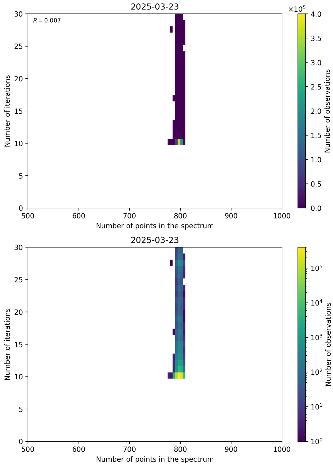
Figure 92: Scatter density plot of “Number of points in the spectrum” against “Number of iterations” for 2025-03-23 to 2025-03-24.
