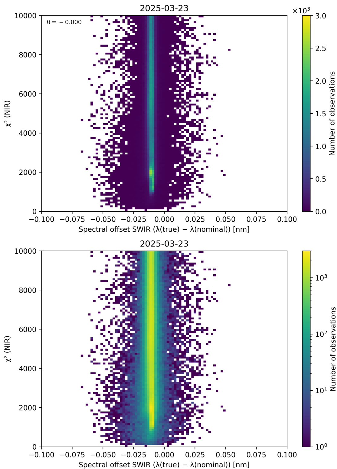
Figure 117: Scatter density plot of “Spectral offset SWIR ( \lambda_{\text{true}} - \lambda_{\text{nominal}} )” against “ \chi^2 (NIR)” for 2025-03-23 to 2025-03-24.
