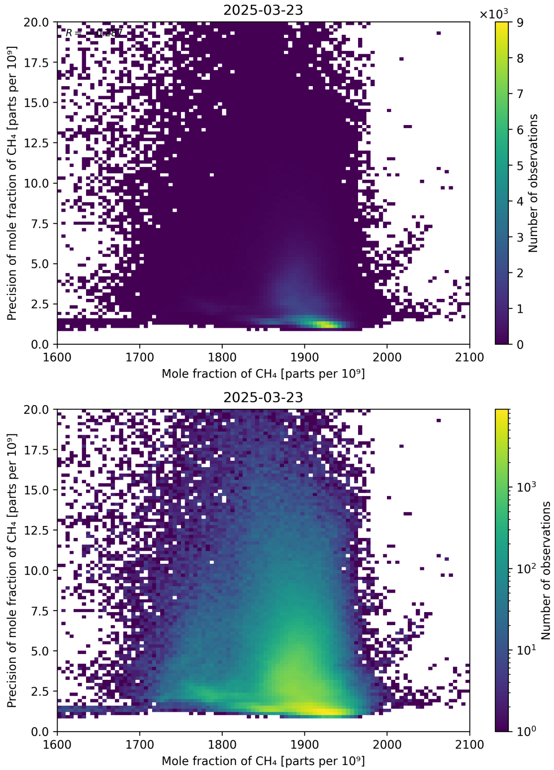
Figure 75: Scatter density plot of “Mole fraction of CH 4 ” against “Precision of mole fraction of CH 4 ” for 2025-03-23 to 2025-03-24.
