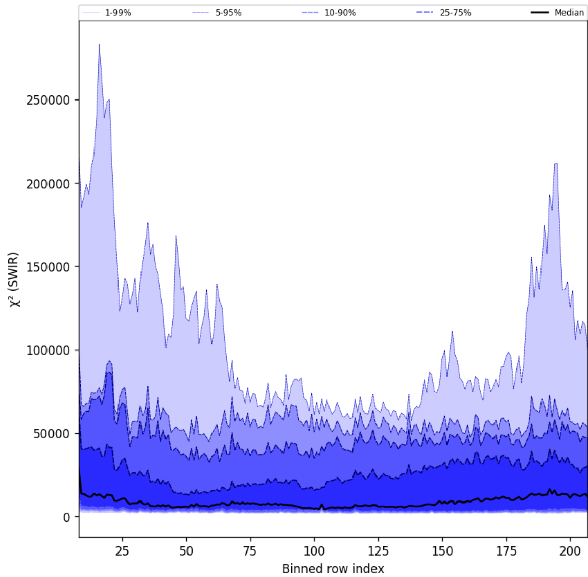
Figure 39: Along track statistics of “ \chi^2 (SWIR)” for 2025-03-23 to 2025-03-24
