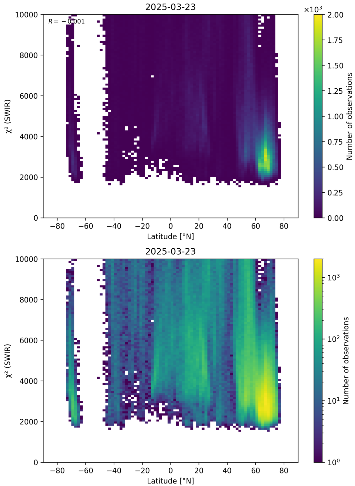
Figure 54: Scatter density plot of “Latitude” against “ \chi^2 (SWIR)” for 2025-03-23 to 2025-03-24.
