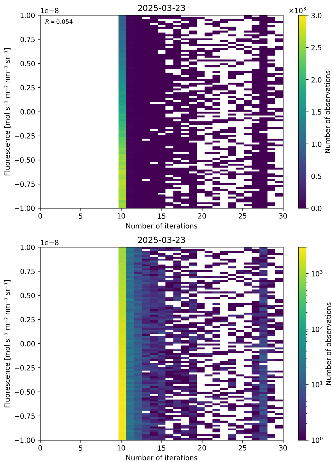
Figure 87: Scatter density plot of “Number of iterations” against “Fluorescence” for 2025-03-23 to 2025-03-24.
