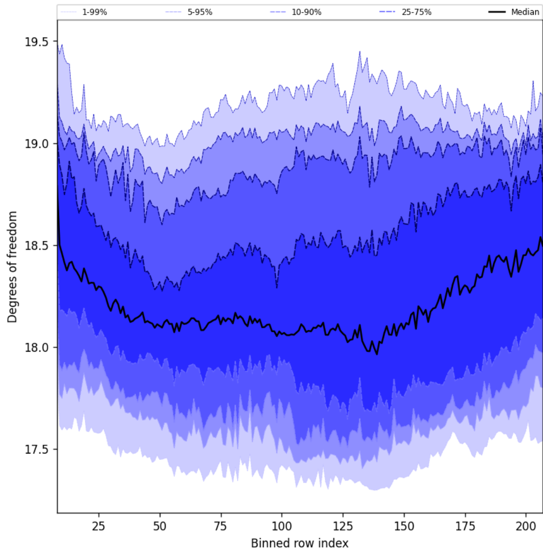
Figure 41: Along track statistics of “Degrees of freedom” for 2025-03-23 to 2025-03-24
