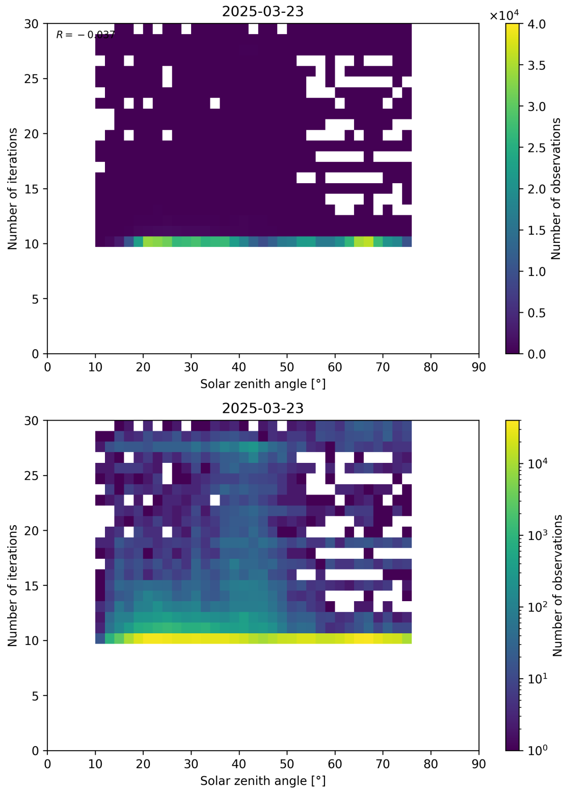
Figure 102: Scatter density plot of “Solar zenith angle” against “Number of iterations” for 2025-03-23 to 2025-03-24.
