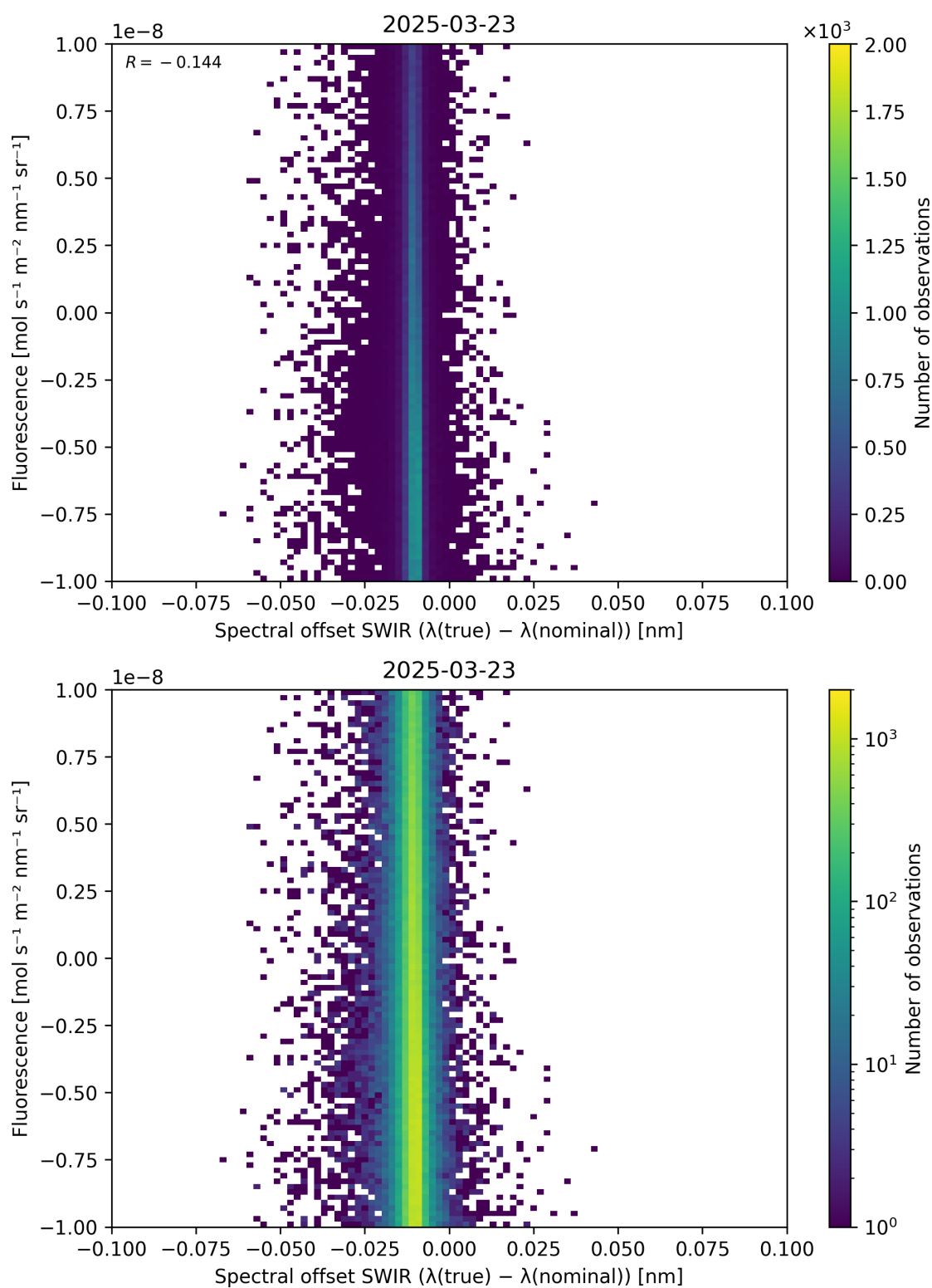
Figure 120: Scatter density plot of “Spectral offset SWIR ( \lambda_{\text{true}} - \lambda_{\text{nominal}} )” against “Fluorescence” for 2025-03-23 to 2025-03-24.
