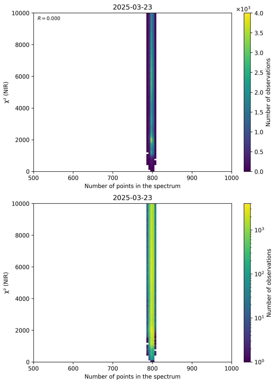
Figure 88: Scatter density plot of “Number of points in the spectrum” against “ \chi^2 (NIR)” for 2025-03-23 to 2025-03-24.
