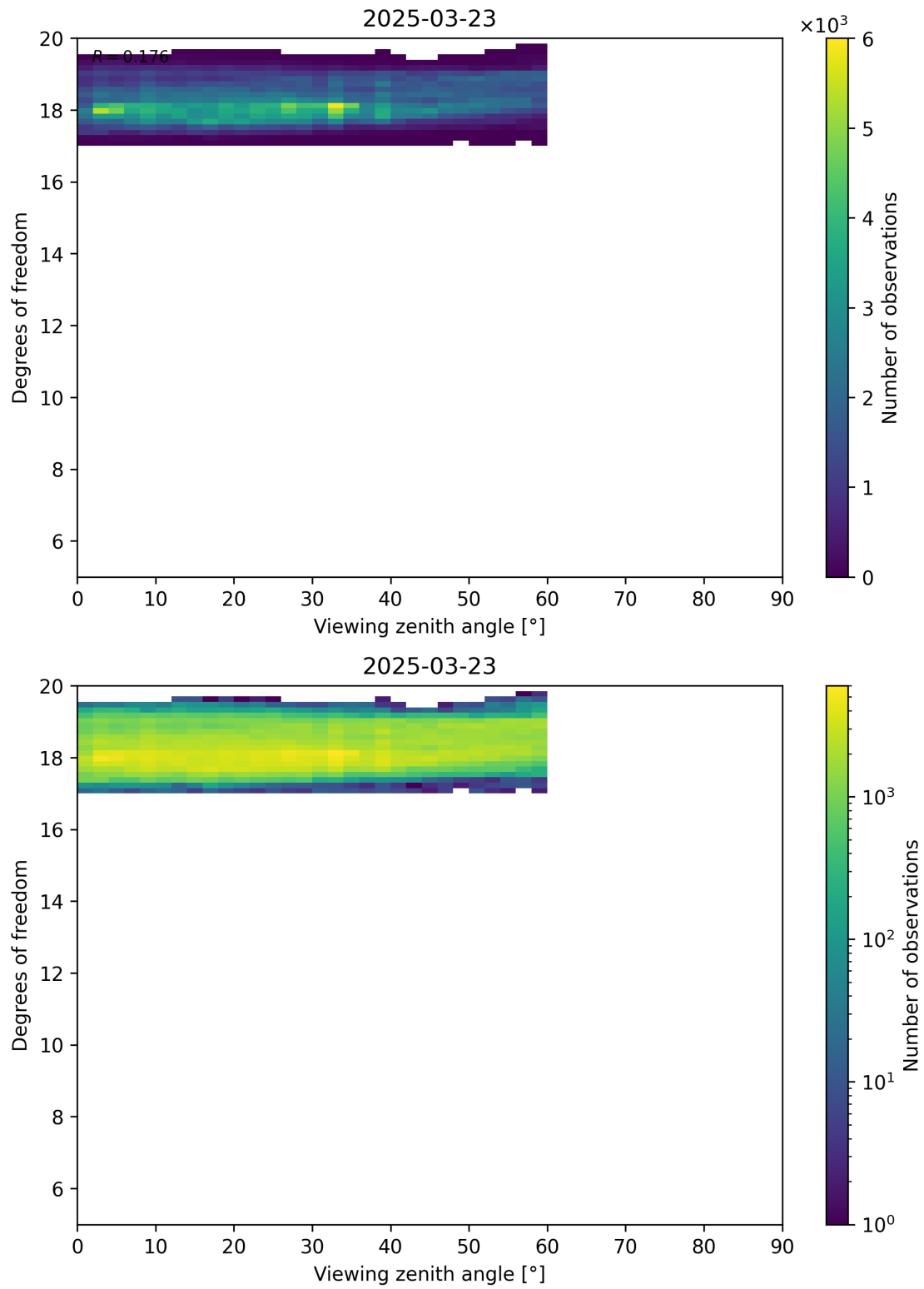
Figure 107: Scatter density plot of “Viewing zenith angle” against “Degrees of freedom” for 2025-03-23 to 2025-03-24.
