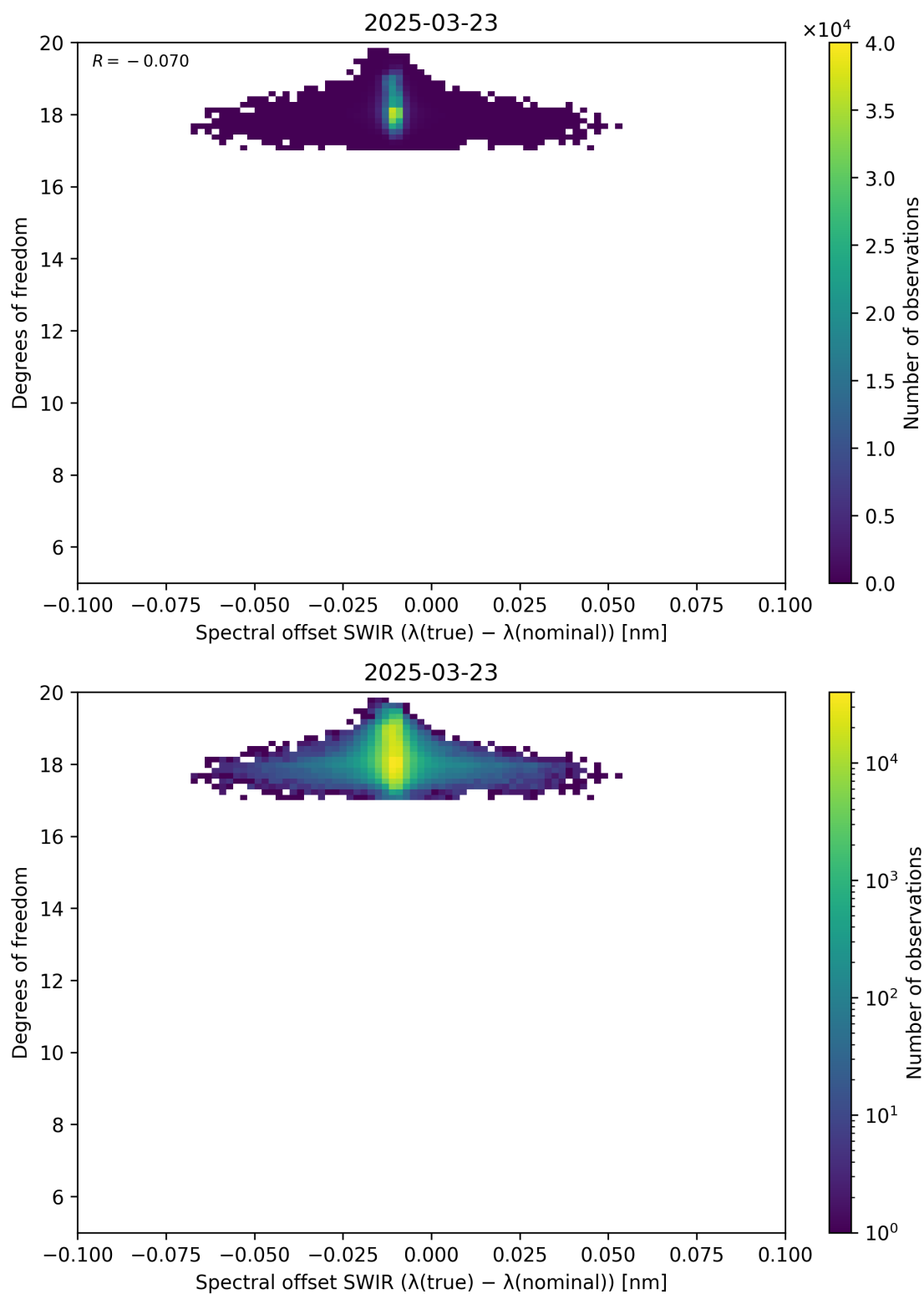
Figure 119: Scatter density plot of “Spectral offset SWIR ( \lambda_{\text{true}} - \lambda_{\text{nominal}} )” against “Degrees of freedom” for 2025-03-23 to 2025-03-24.
