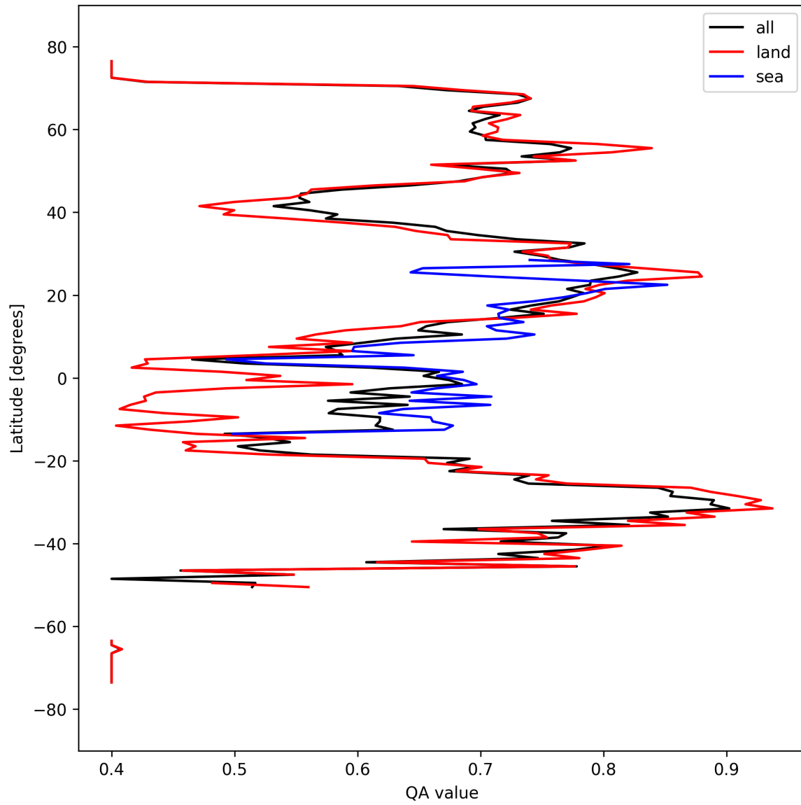
Figure 11: Zonal average of “QA value” for 2025-03-23 to 2025-03-24.
