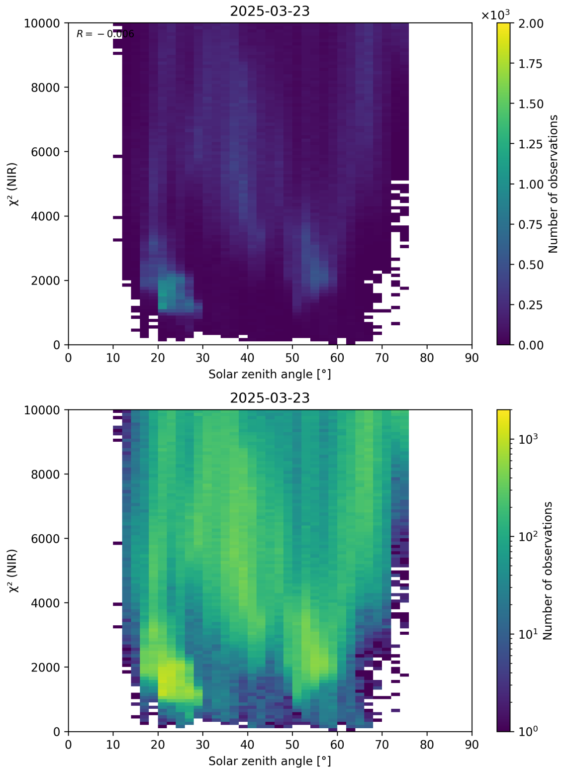
Figure 94: Scatter density plot of “Solar zenith angle” against “ \chi^2 (NIR)” for 2025-03-23 to 2025-03-24.
