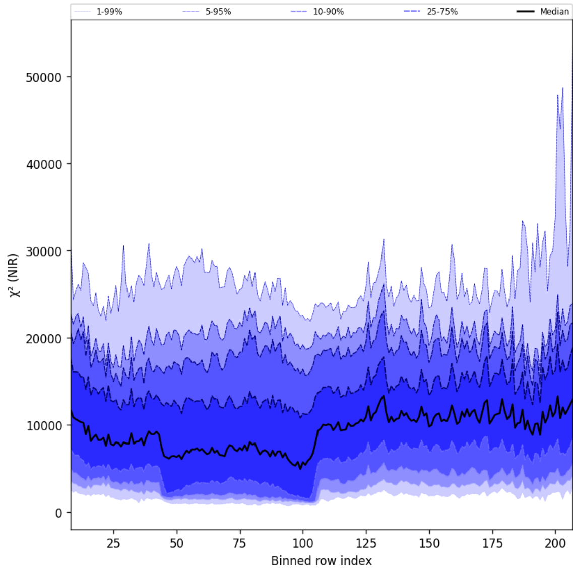
Figure 40: Along track statistics of “ \chi^2 (NIR)” for 2025-03-23 to 2025-03-24
