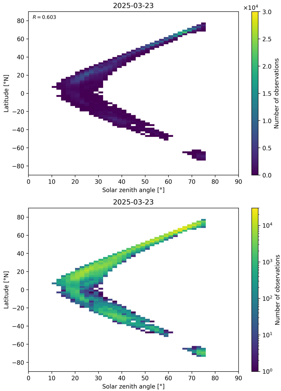
Figure 98: Scatter density plot of “Solar zenith angle” against “Latitude” for 2025-03-23 to 2025-03-24.
