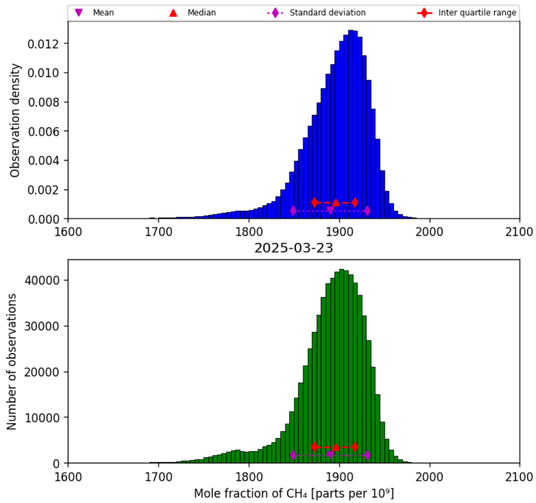
Figure 23: Histogram of “Mole fraction of CH 4 ” for 2025-03-23 to 2025-03-24
