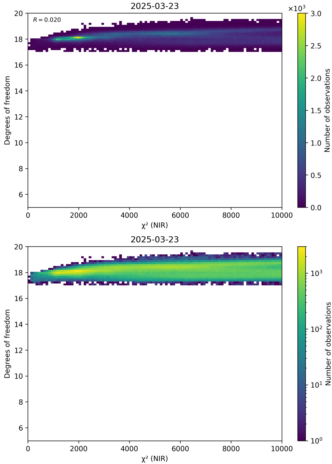
Figure 44: Scatter density plot of “ \chi^2 (NIR)” against “Degrees of freedom” for 2025-03-23 to 2025-03-24.
