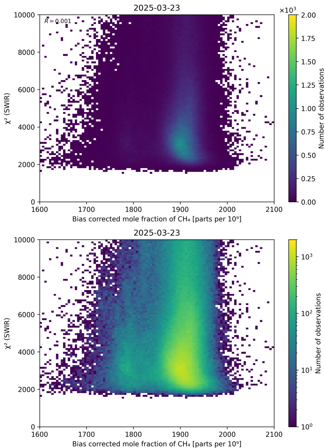
Figure 64: Scatter density plot of “Bias corrected mole fraction of \text{CH}_4 ” against “ \chi^2 (SWIR)” for 2025-03-23 to 2025-03-24.
