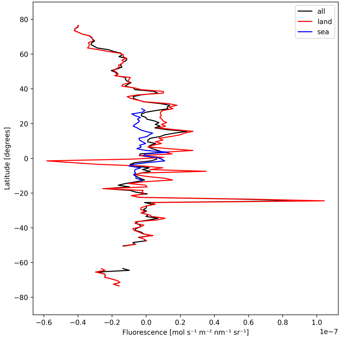
Figure 21: Zonal average of “Fluorescence” for 2025-03-23 to 2025-03-24.
