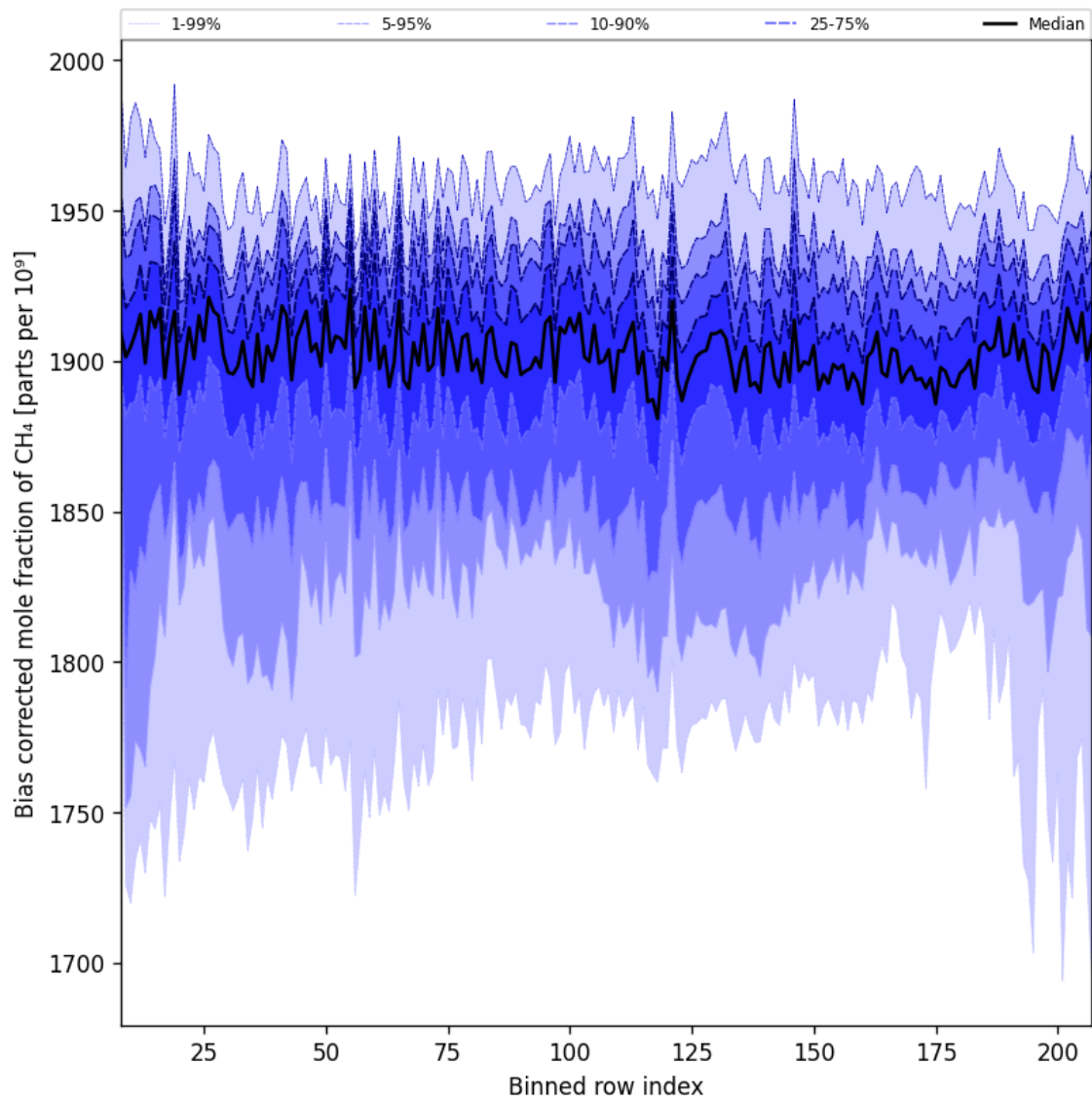
Figure 36: Along track statistics of “Bias corrected mole fraction of CH 4 ” for 2025-03-23 to 2025-03-24
