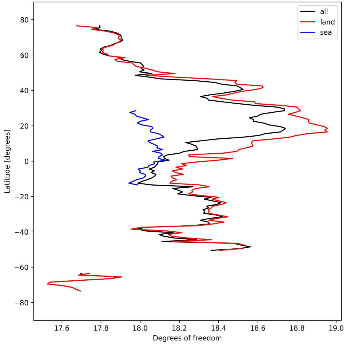
Figure 19: Zonal average of “Degrees of freedom” for 2025-03-23 to 2025-03-24.
