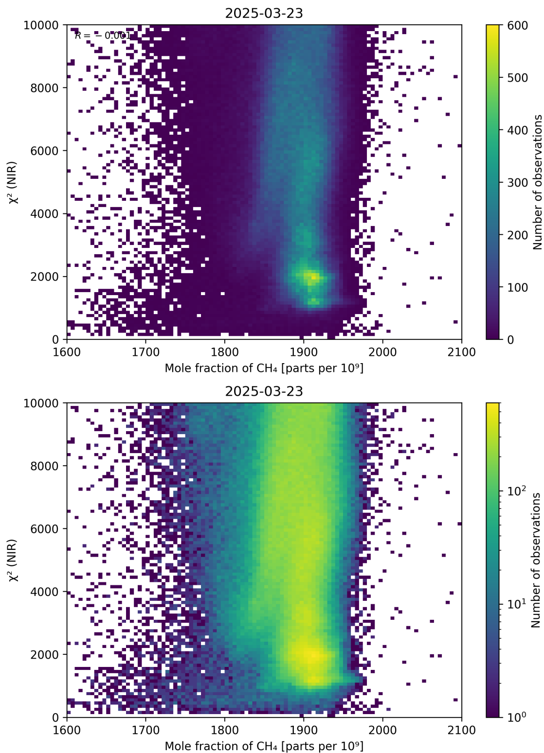
Figure 70: Scatter density plot of “Mole fraction of CH 4 ” against “ \chi^2 (NIR)” for 2025-03-23 to 2025-03-24.
