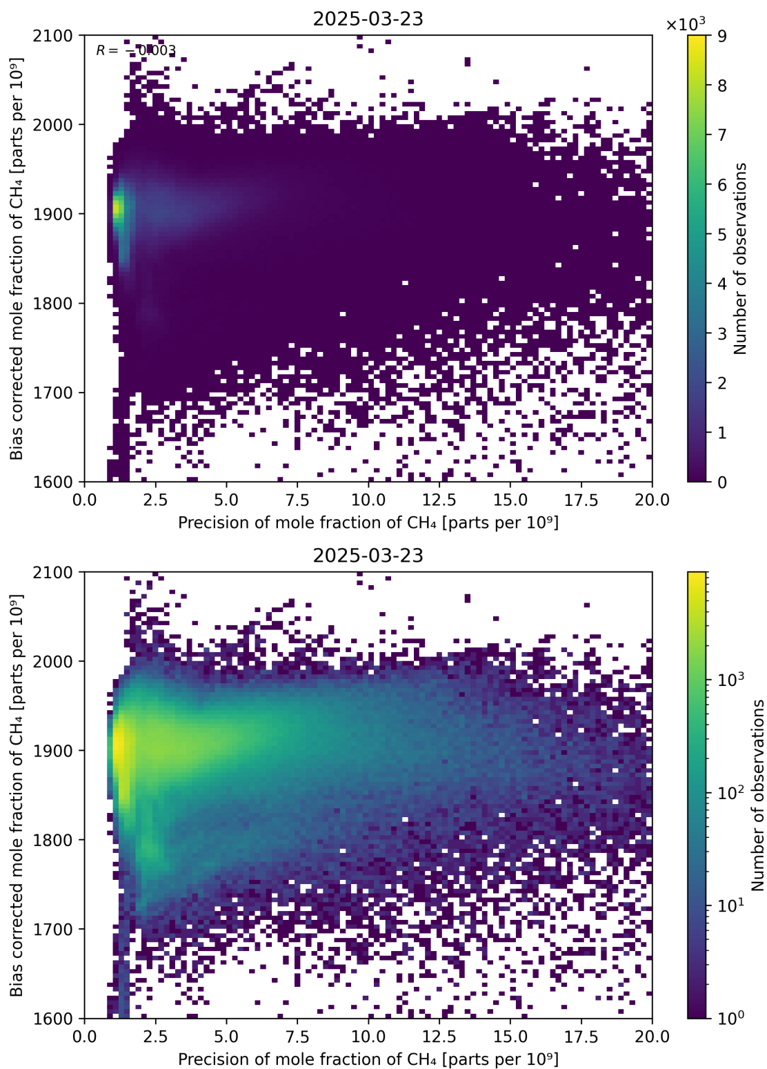
Figure 82: Scatter density plot of “Precision of mole fraction of \text{CH}_4 ” against “Bias corrected mole fraction of \text{CH}_4 ” for 2025-03-23 to 2025-03-24.
