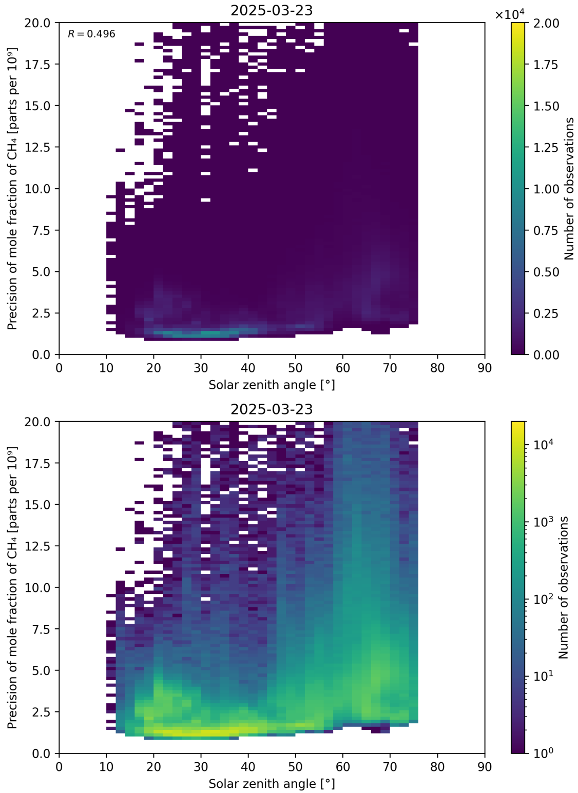
Figure 101: Scatter density plot of “Solar zenith angle” against “Precision of mole fraction of \text{CH}_4 ” for 2025-03-23 to 2025-03-24.
