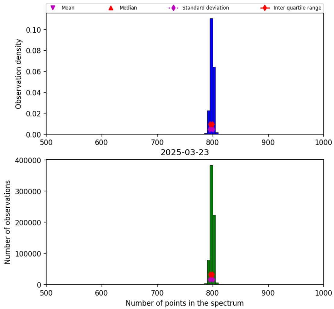
Figure 26: Histogram of “Number of points in the spectrum” for 2025-03-23 to 2025-03-24
