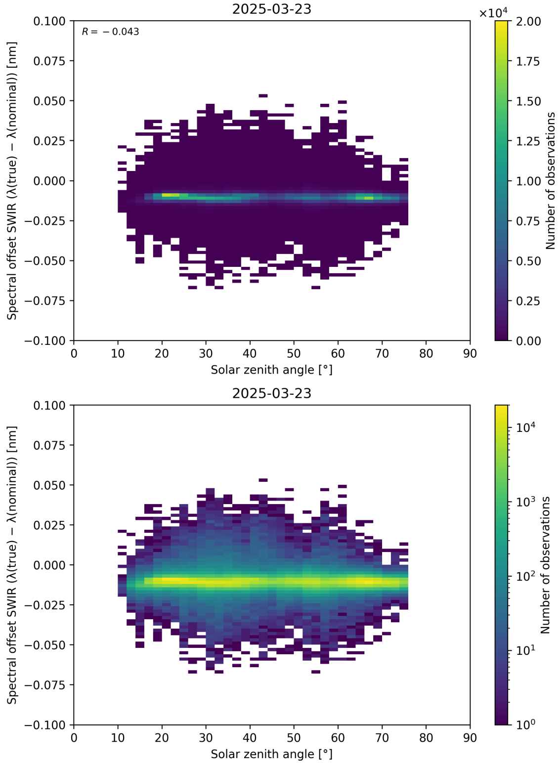
Figure 104: Scatter density plot of “Solar zenith angle” against “Spectral offset SWIR ( \lambda_{\text{true}} - \lambda_{\text{nominal}} )” for 2025-03-23 to 2025-03-24.
