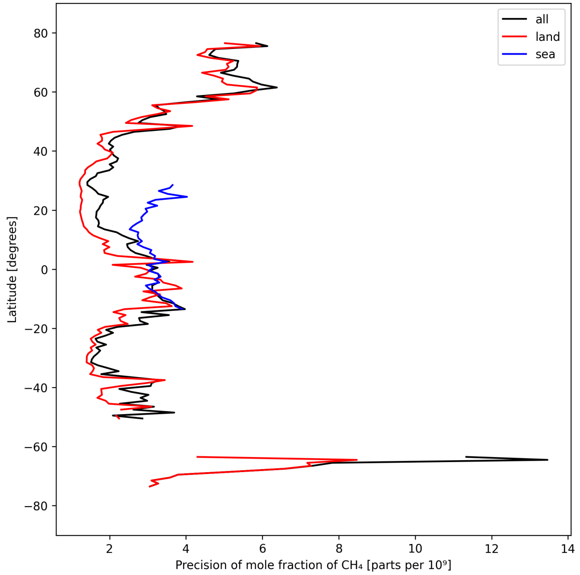
Figure 13: Zonal average of “Precision of mole fraction of CH 4 ” for 2025-03-23 to 2025-03-24.
