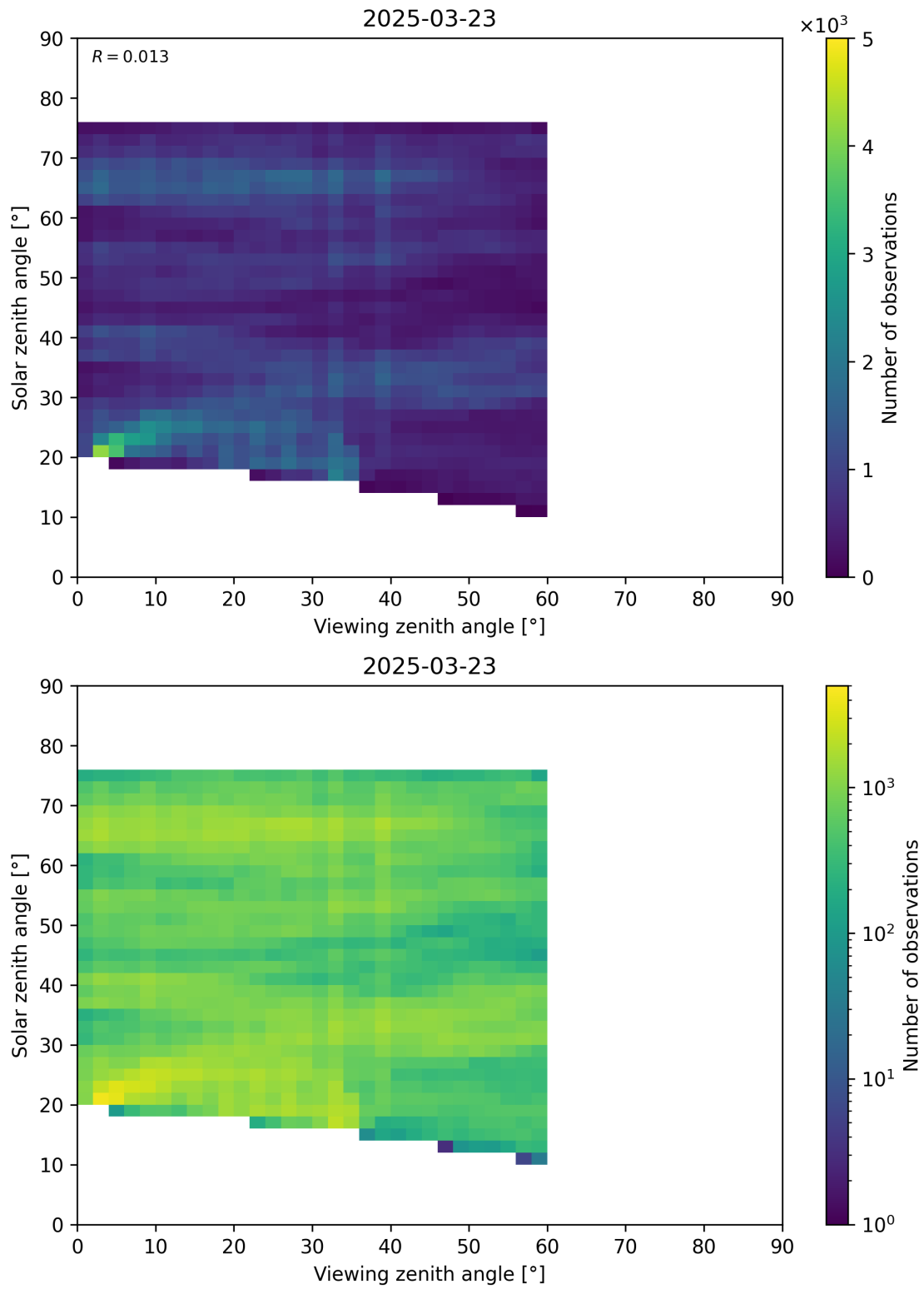
Figure 115: Scatter density plot of “Viewing zenith angle” against “Solar zenith angle” for 2025-03-23 to 2025-03-24.
