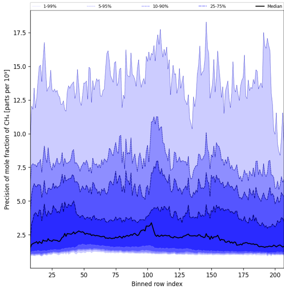
Figure 35: Along track statistics of “Precision of mole fraction of CH 4 ” for 2025-03-23 to 2025-03-24
