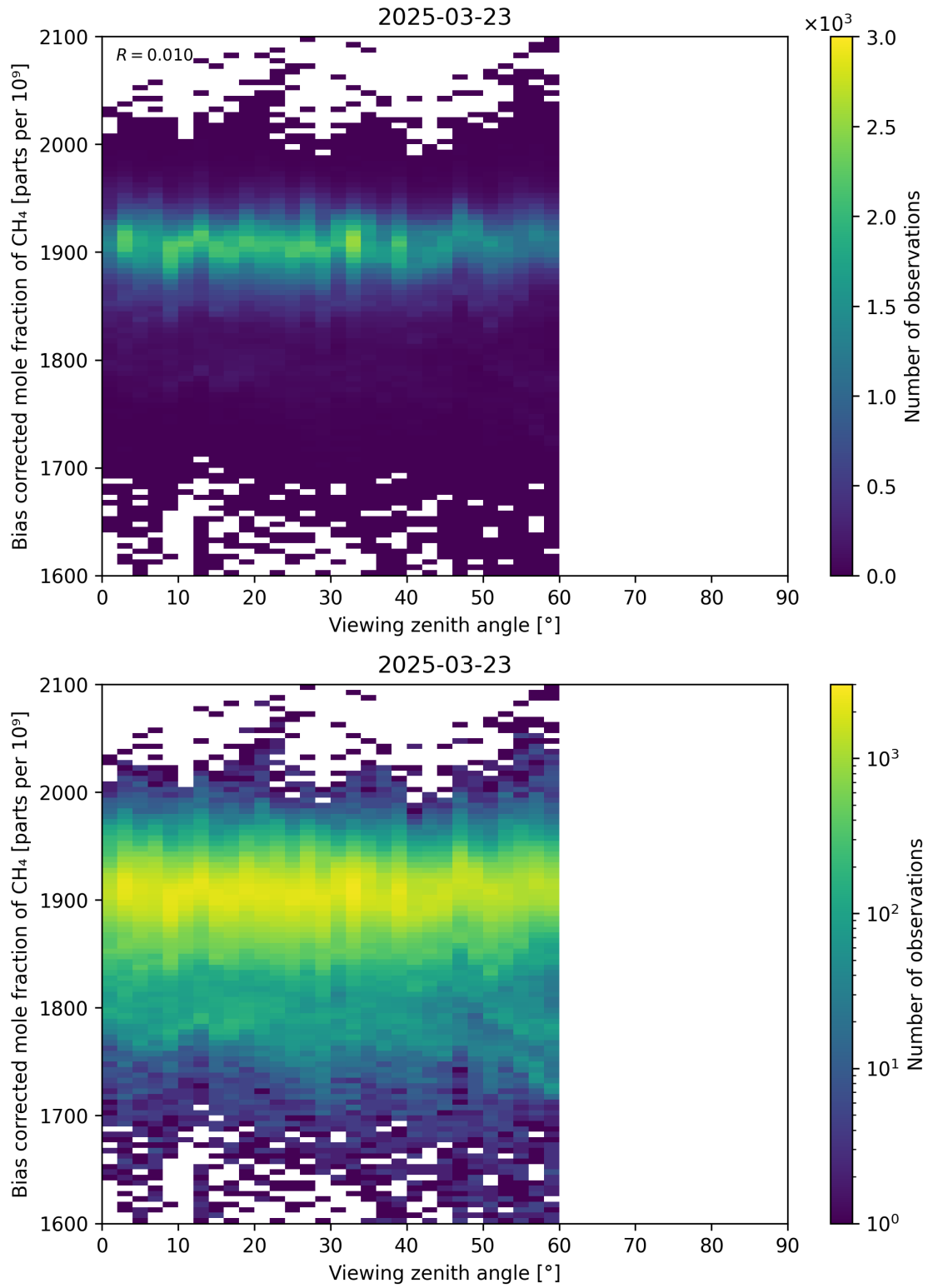
Figure 111: Scatter density plot of “Viewing zenith angle” against “Bias corrected mole fraction of CH 4 ” for 2025-03-23 to 2025-03-24.
