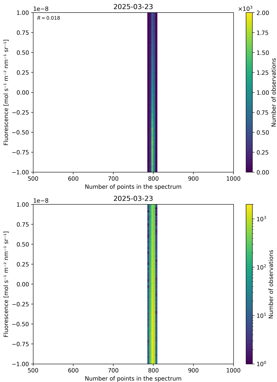
Figure 91: Scatter density plot of “Number of points in the spectrum” against “Fluorescence” for 2025-03-23 to 2025-03-24.
