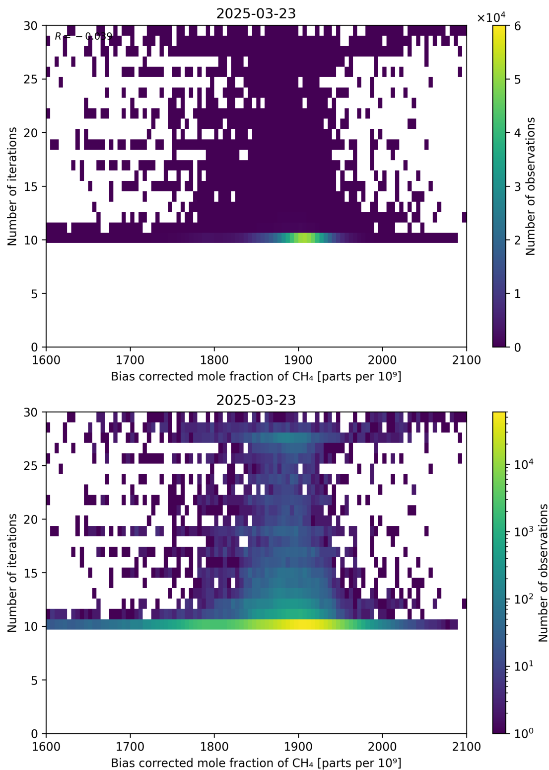
Figure 67: Scatter density plot of “Bias corrected mole fraction of CH 4 ” against “Number of iterations” for 2025-03-23 to 2025-03-24.
