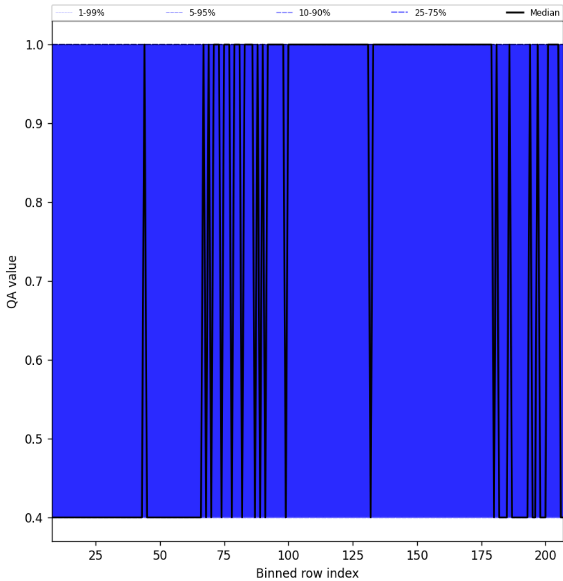
Figure 33: Along track statistics of “QA value” for 2025-03-23 to 2025-03-24
