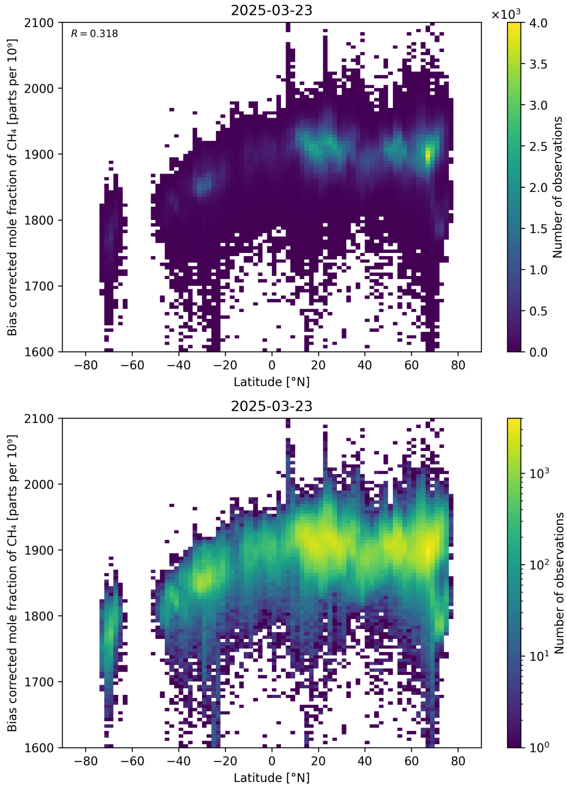
Figure 58: Scatter density plot of “Latitude” against “Bias corrected mole fraction of \text{CH}_4 ” for 2025-03-23 to 2025-03-24.
