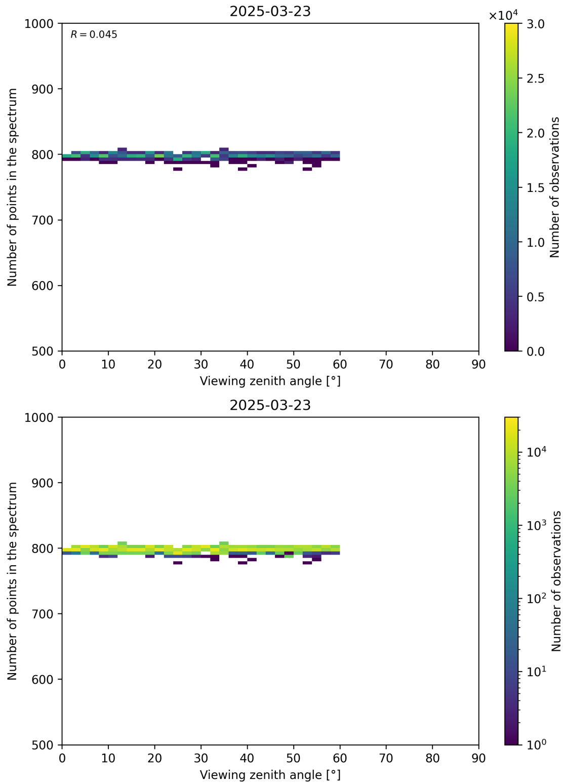
Figure 114: Scatter density plot of “Viewing zenith angle” against “Number of points in the spectrum” for 2025-03-23 to 2025-03-24.
