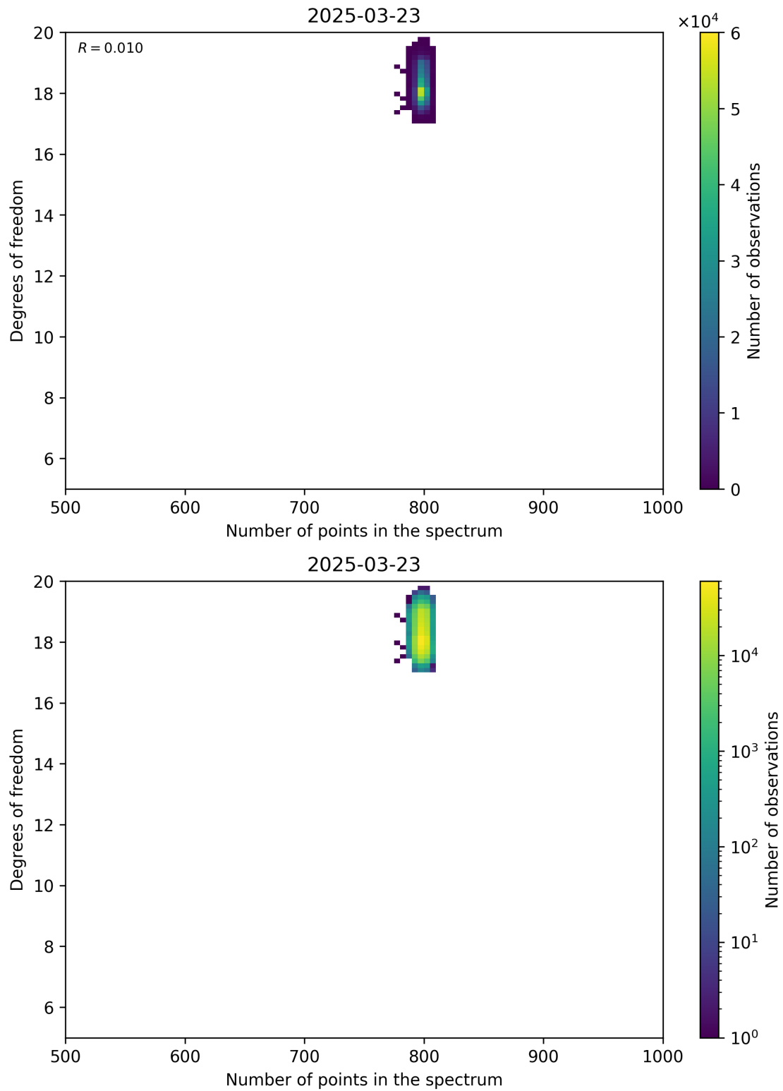
Figure 90: Scatter density plot of “Number of points in the spectrum” against “Degrees of freedom” for 2025-03-23 to 2025-03-24.
