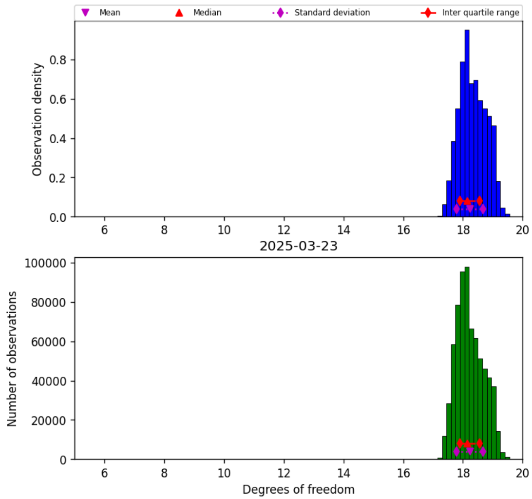
Figure 30: Histogram of “Degrees of freedom” for 2025-03-23 to 2025-03-24
