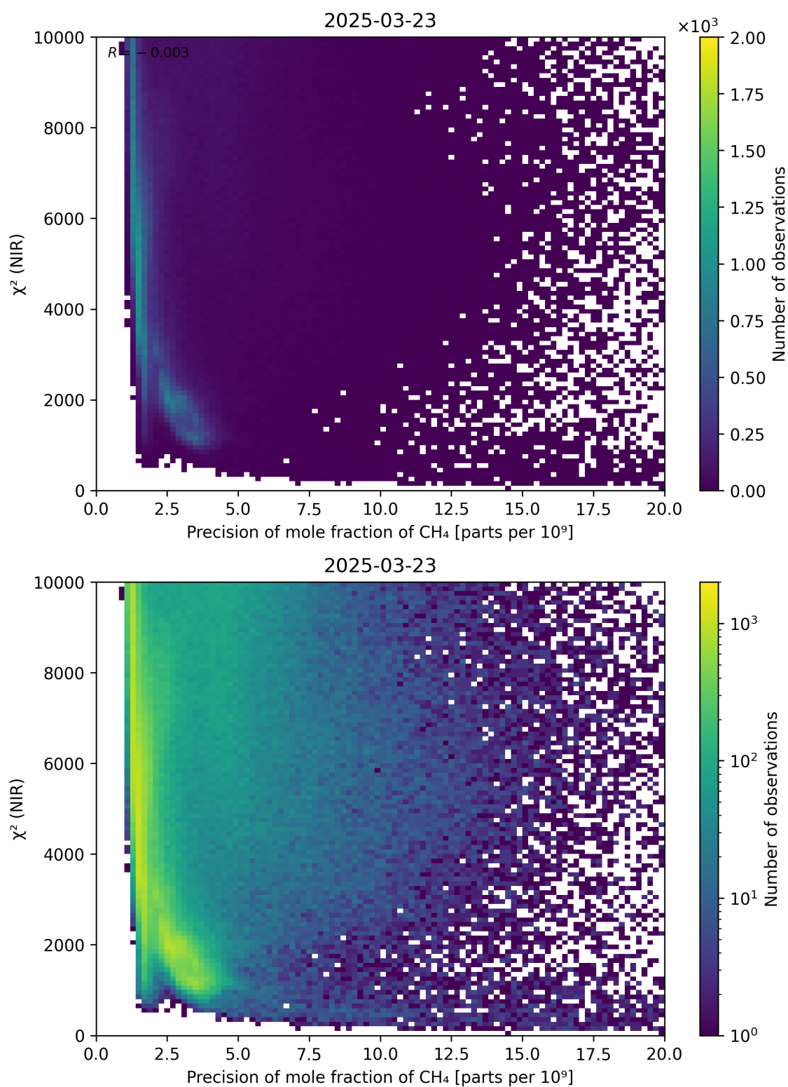
Figure 78: Scatter density plot of “Precision of mole fraction of CH 4 ” against “ \chi^2 (NIR)” for 2025-03-23 to 2025-03-24.
