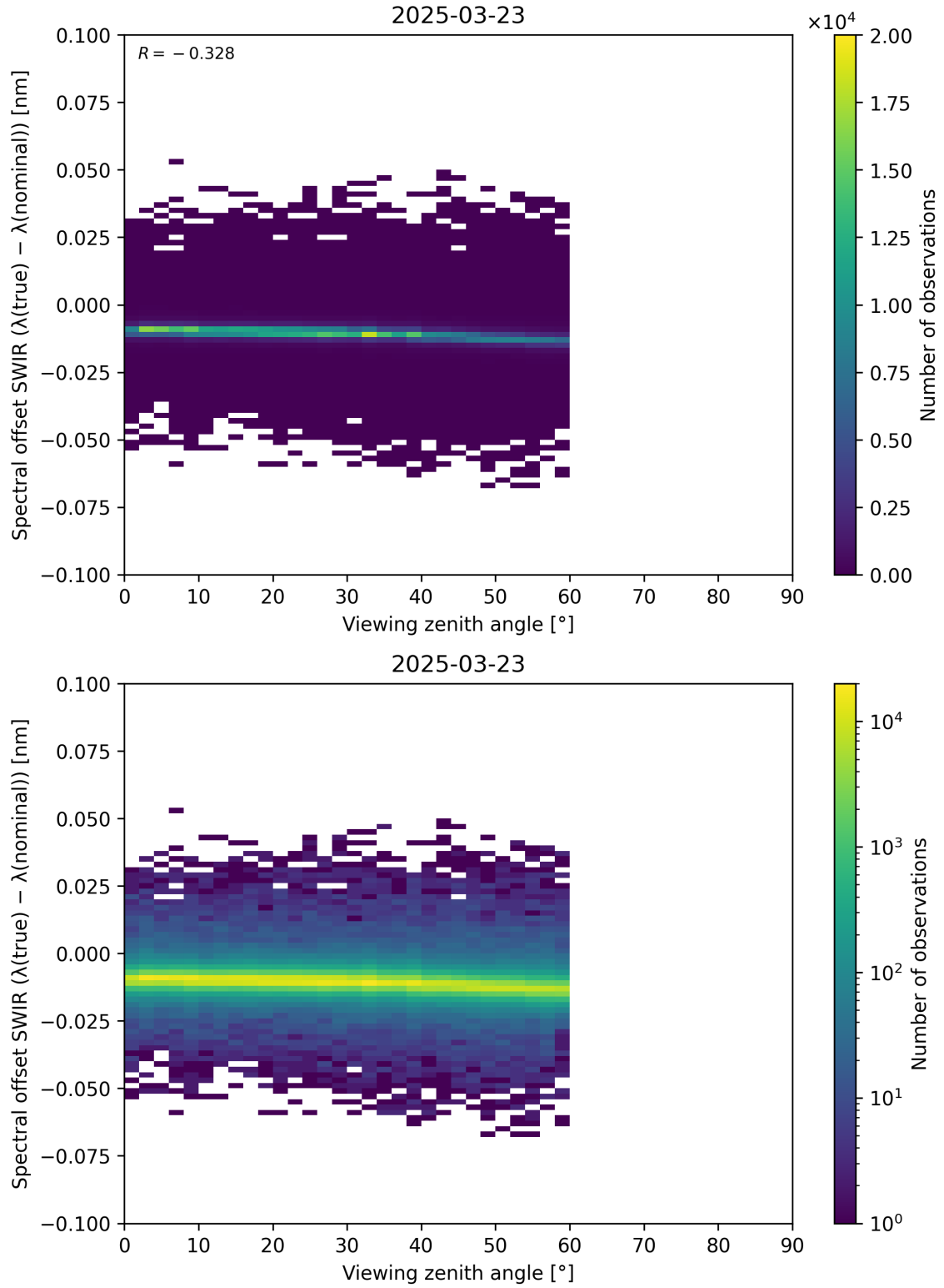
Figure 116: Scatter density plot of “Viewing zenith angle” against “Spectral offset SWIR ( \lambda_{\text{true}} - \lambda_{\text{nominal}} )” for 2025-03-23 to 2025-03-24.
