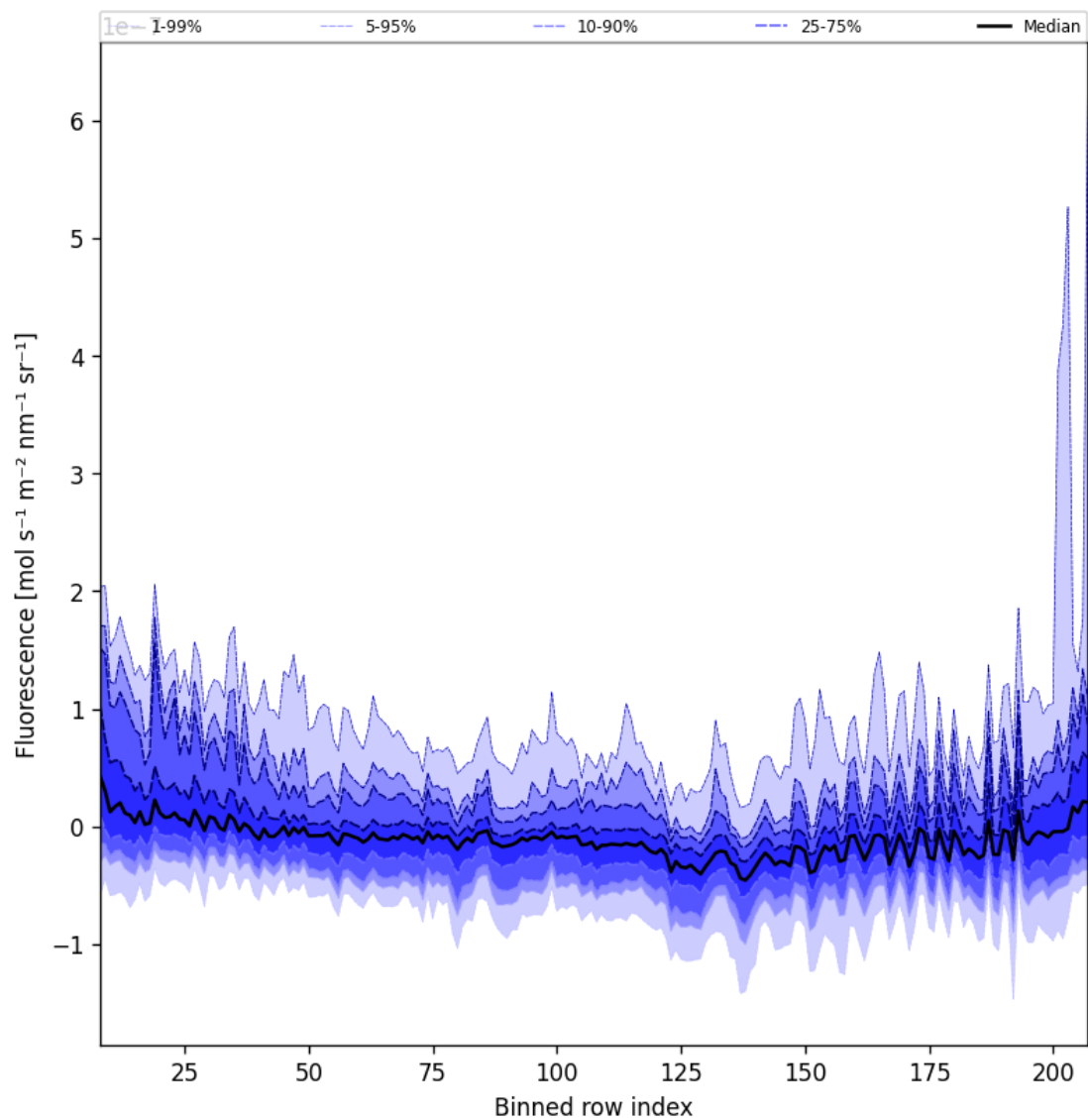
Figure 43: Along track statistics of “Fluorescence” for 2025-03-23 to 2025-03-24
