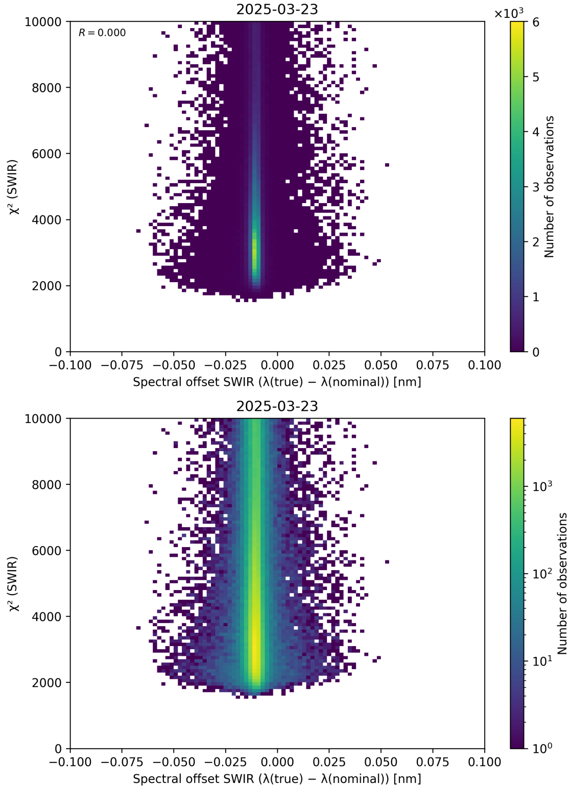
Figure 118: Scatter density plot of “Spectral offset SWIR ( \lambda_{\text{true}} - \lambda_{\text{nominal}} )” against “ \chi^2 (SWIR)” for 2025-03-23 to 2025-03-24.
