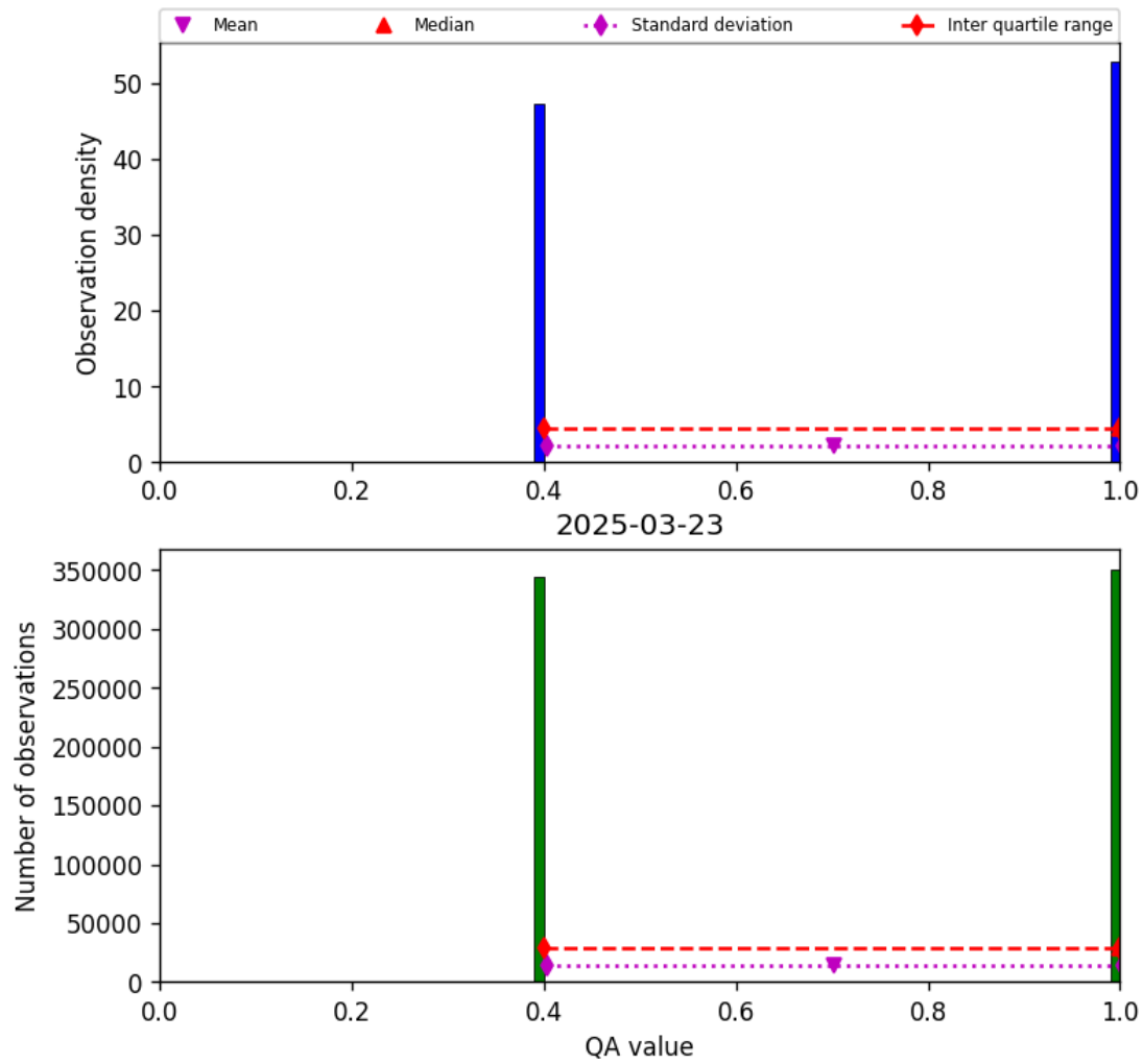
Figure 22: Histogram of “QA value” for 2025-03-23 to 2025-03-24
