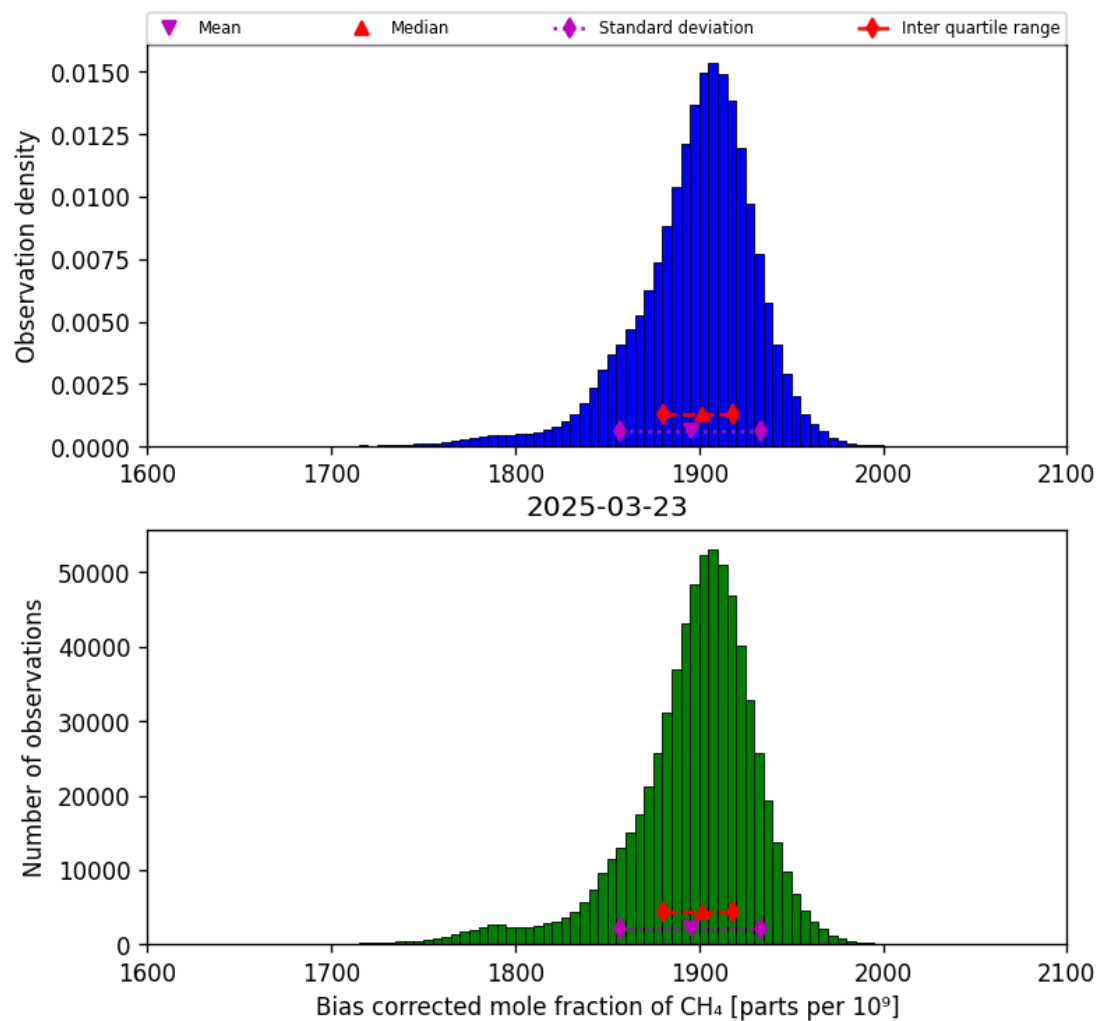
Figure 25: Histogram of “Bias corrected mole fraction of CH 4 ” for 2025-03-23 to 2025-03-24
