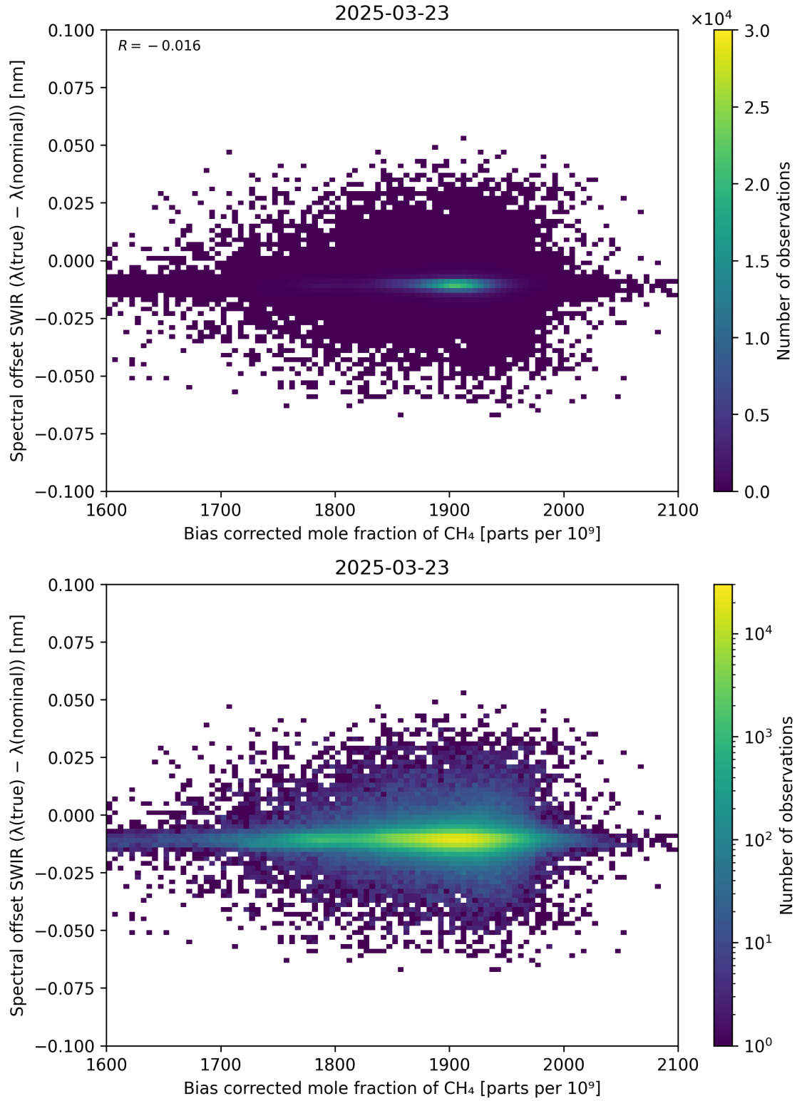
Figure 69: Scatter density plot of “Bias corrected mole fraction of \text{CH}_4 ” against “Spectral offset SWIR ( \lambda_{\text{true}} - \lambda_{\text{nominal}} )” for 2025-03-23 to 2025-03-24.
