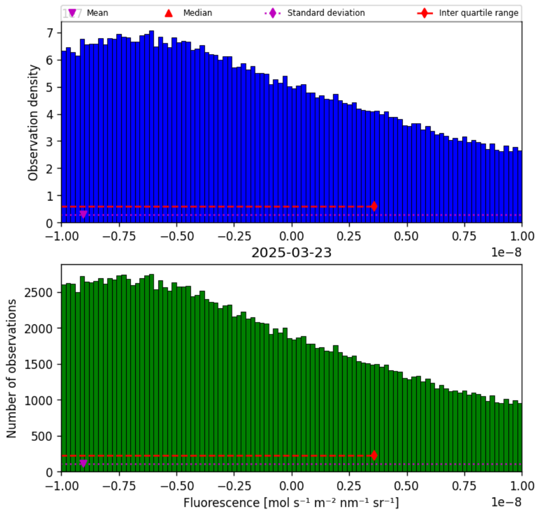
Figure 32: Histogram of “Fluorescence” for 2025-03-23 to 2025-03-24
