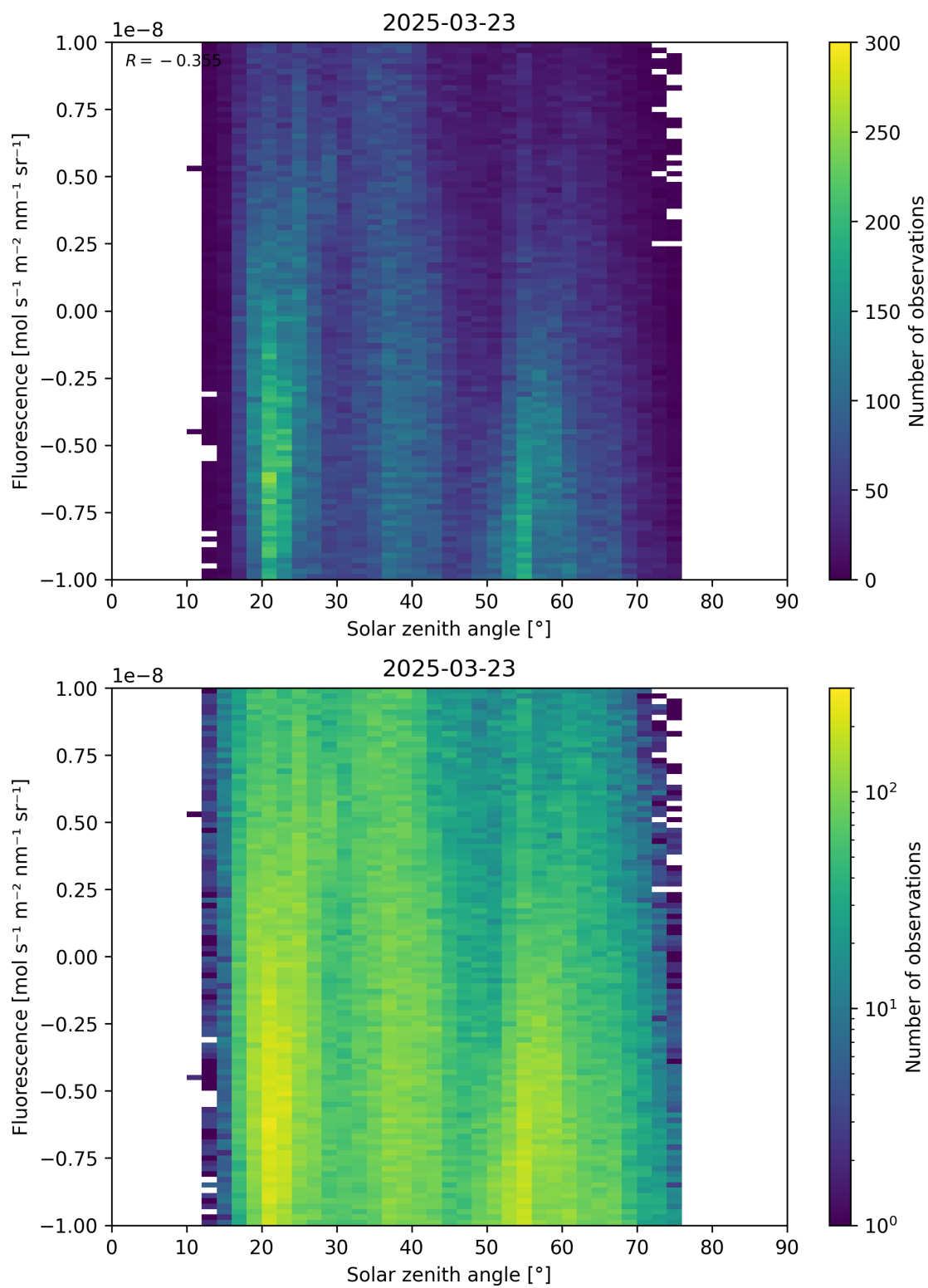
Figure 97: Scatter density plot of “Solar zenith angle” against “Fluorescence” for 2025-03-23 to 2025-03-24.
