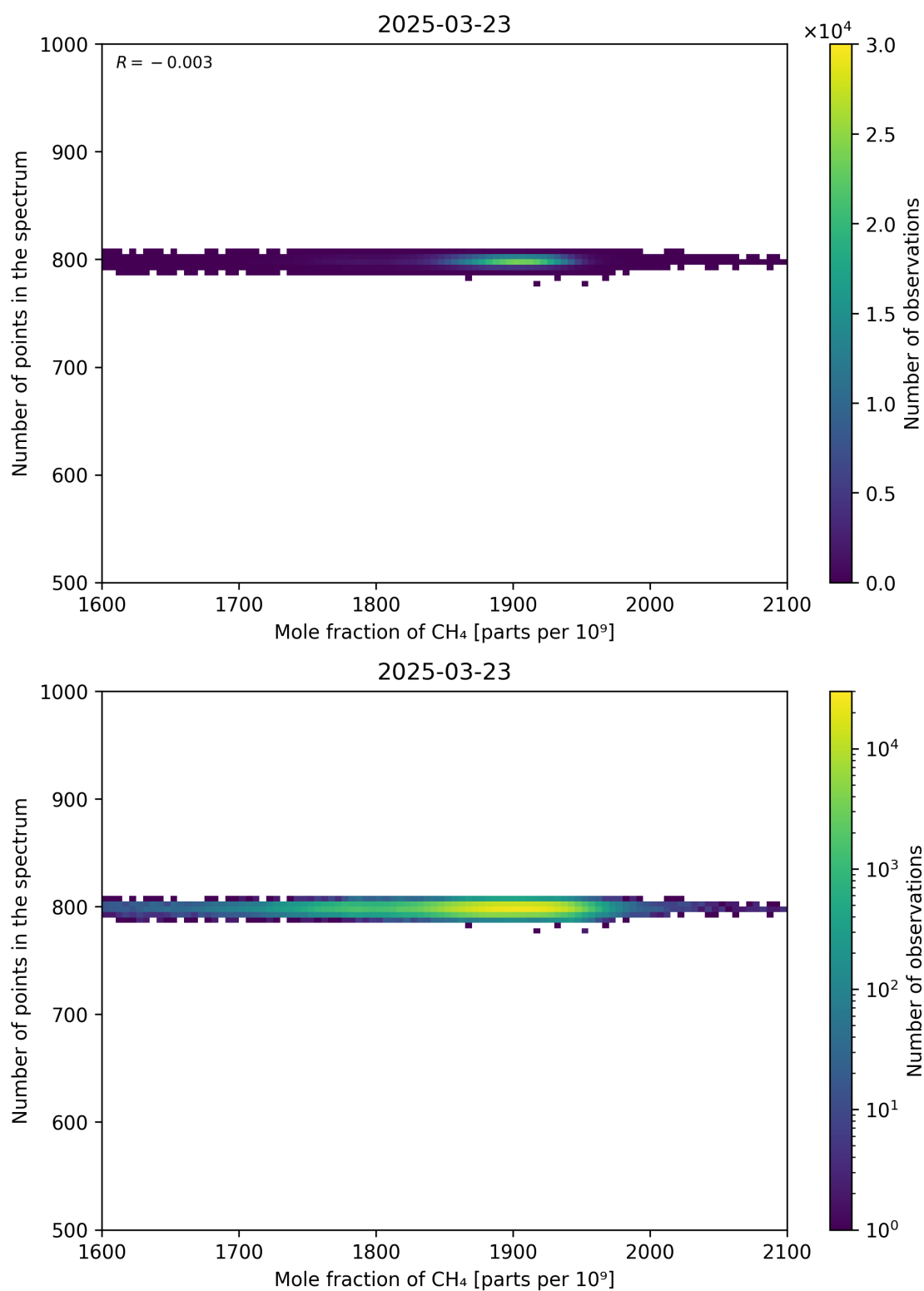
Figure 77: Scatter density plot of “Mole fraction of CH 4 ” against “Number of points in the spectrum” for 2025-03-23 to 2025-03-24.
