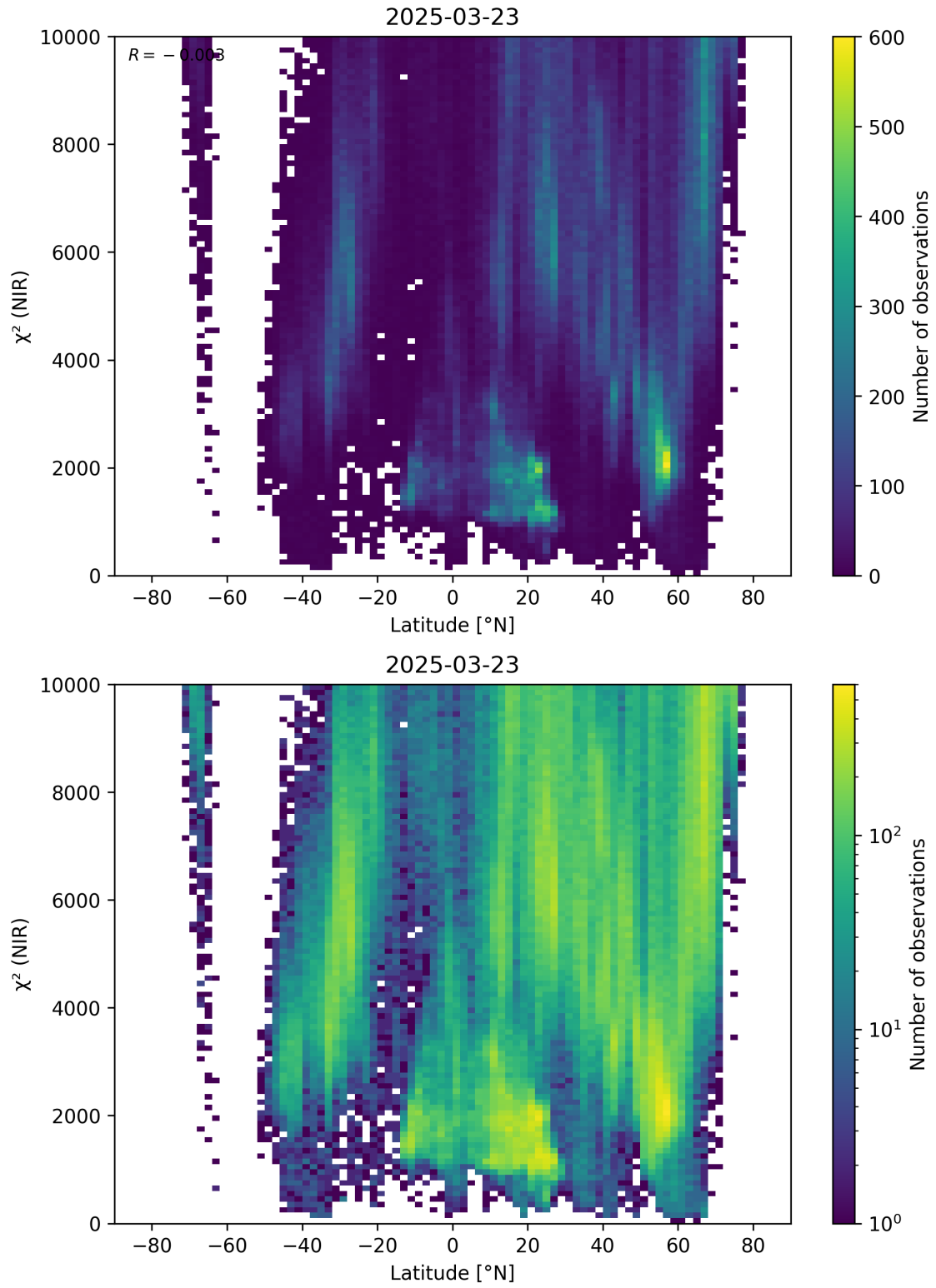
Figure 53: Scatter density plot of “Latitude” against “ \chi^2 (NIR)” for 2025-03-23 to 2025-03-24.
