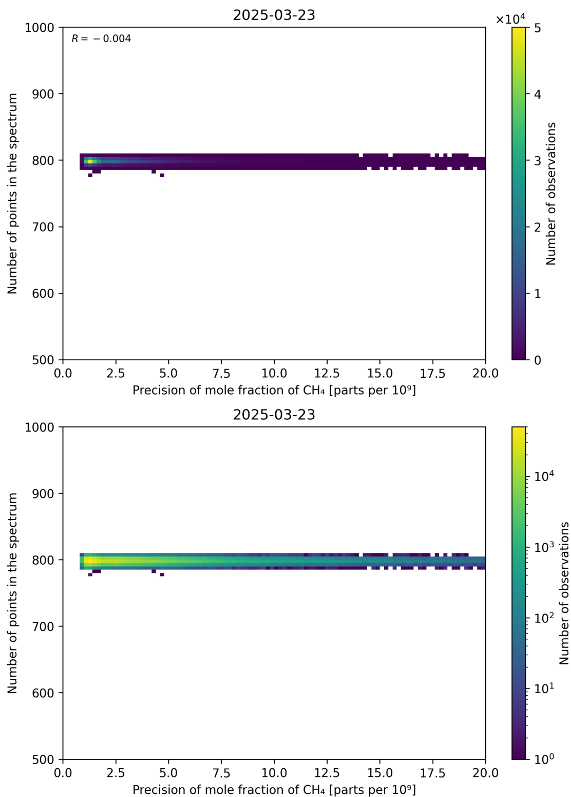
Figure 84: Scatter density plot of “Precision of mole fraction of CH 4 ” against “Number of points in the spectrum” for 2025-03-23 to 2025-03-24.
