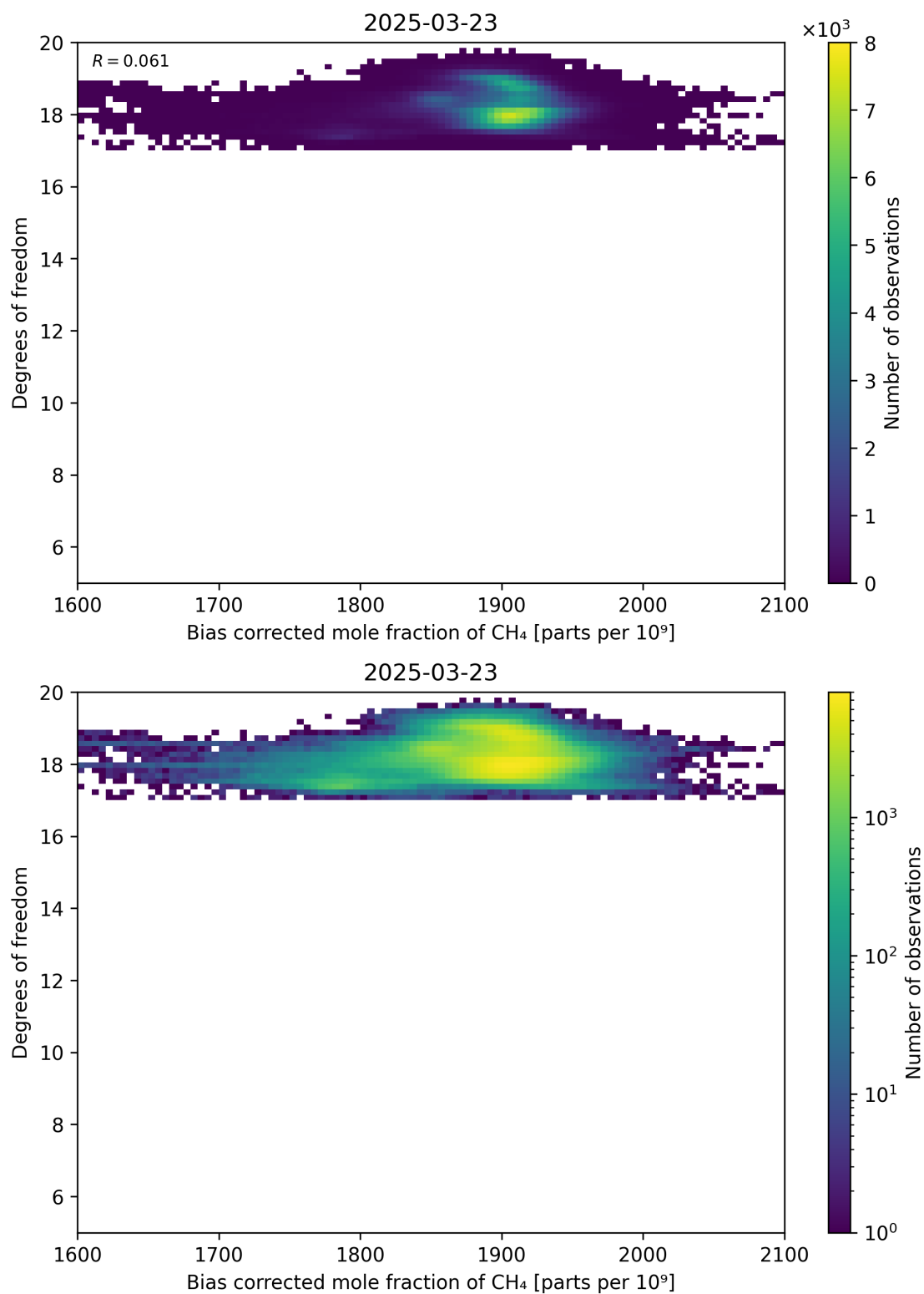
Figure 65: Scatter density plot of “Bias corrected mole fraction of CH 4 ” against “Degrees of freedom” for 2025-03-23 to 2025-03-24.
