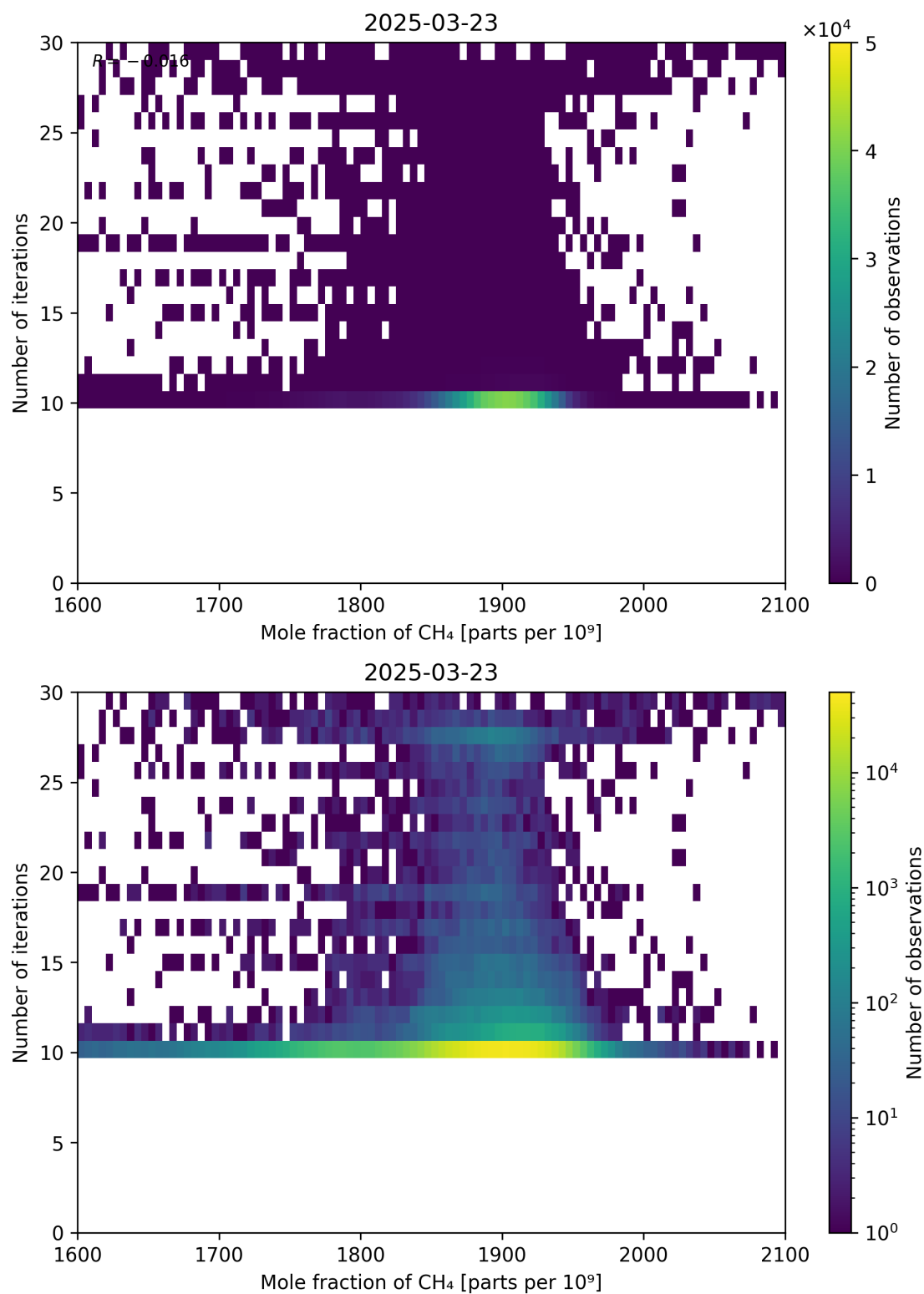
Figure 76: Scatter density plot of “Mole fraction of CH 4 ” against “Number of iterations” for 2025-03-23 to 2025-03-24.
