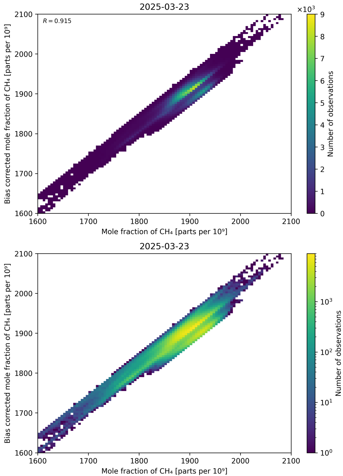
Figure 74: Scatter density plot of “Mole fraction of CH 4 ” against “Bias corrected mole fraction of CH 4 ” for 2025-03-23 to 2025-03-24.
