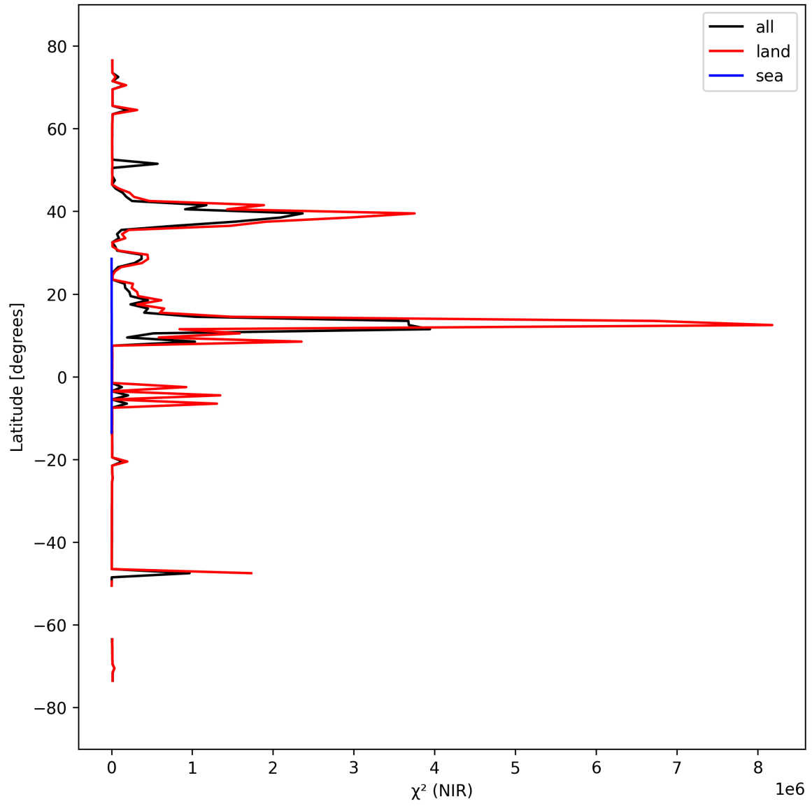
Figure 18: Zonal average of “ \chi^2 (NIR)” for 2025-03-23 to 2025-03-24.
