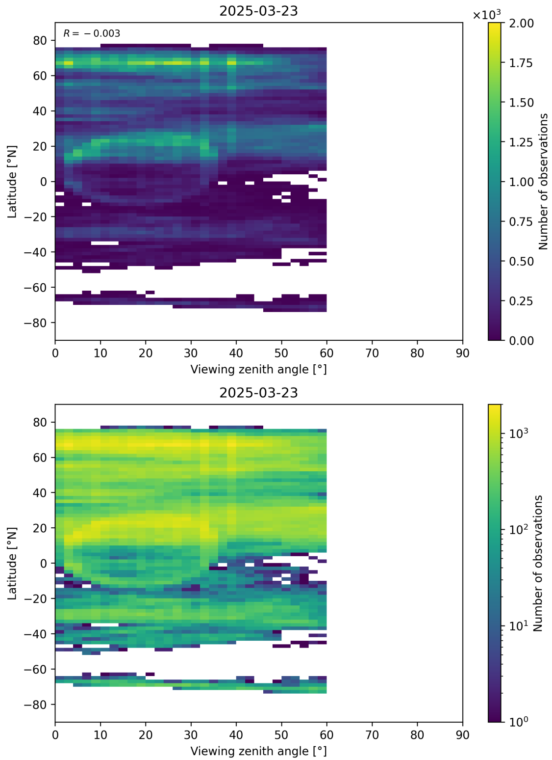
Figure 109: Scatter density plot of “Viewing zenith angle” against “Latitude” for 2025-03-23 to 2025-03-24.
