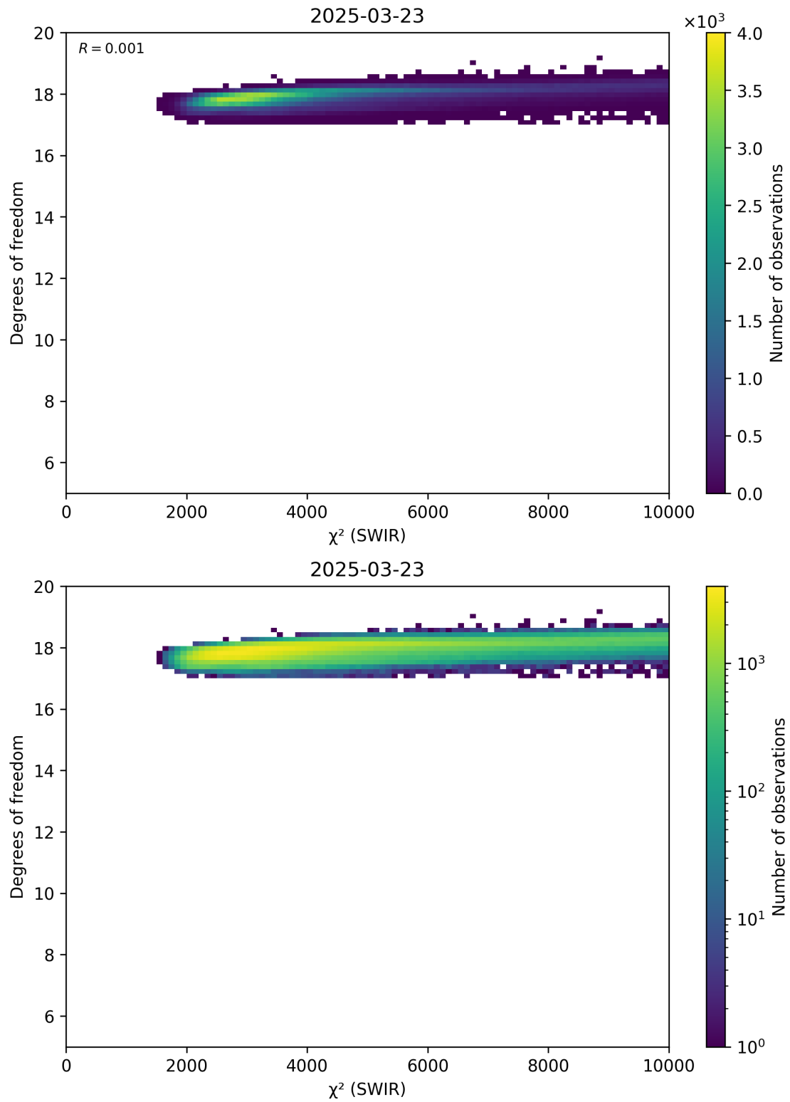
Figure 48: Scatter density plot of “ \chi^2 (SWIR)” against “Degrees of freedom” for 2025-03-23 to 2025-03-24.
