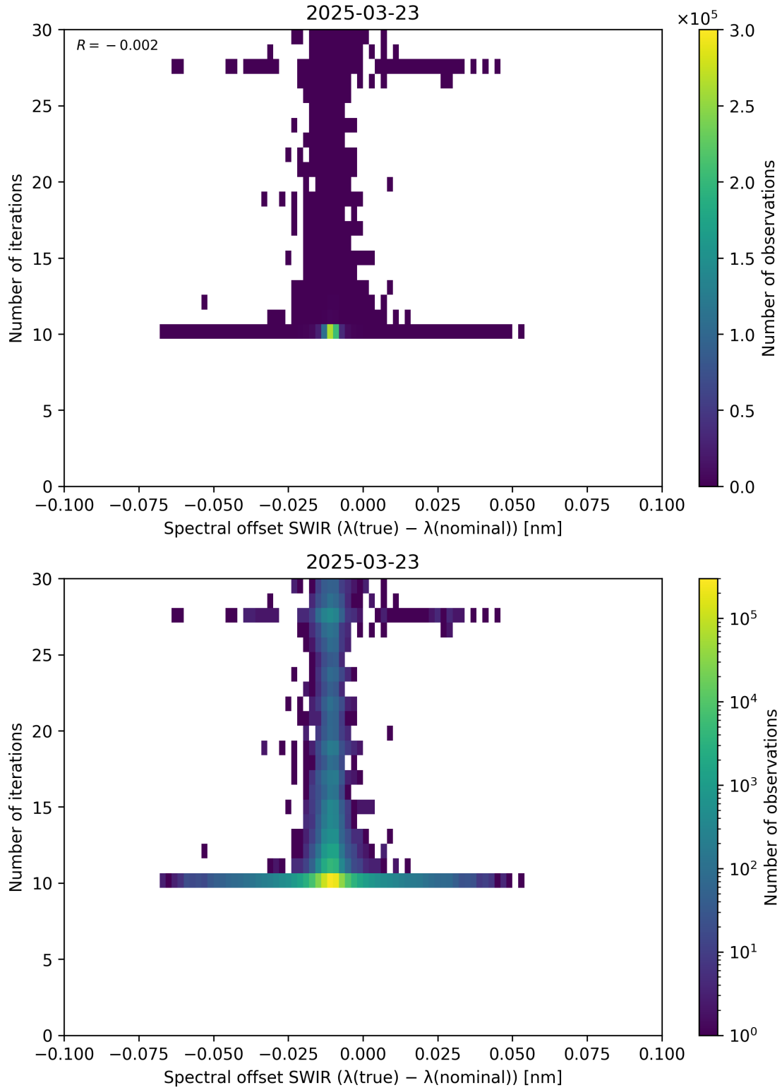
Figure 121: Scatter density plot of “Spectral offset SWIR ( \lambda_{\text{true}} - \lambda_{\text{nominal}} )” against “Number of iterations” for 2025-03-23 to 2025-03-24.
