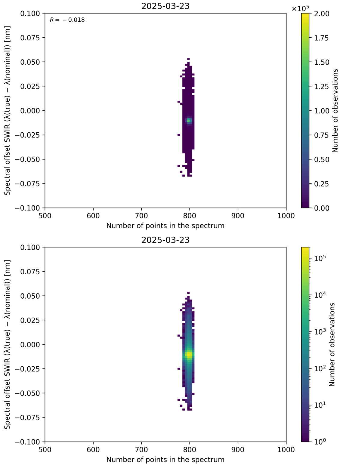
Figure 93: Scatter density plot of “Number of points in the spectrum” against “Spectral offset SWIR ( \lambda_{\text{true}} - \lambda_{\text{nominal}} )” for 2025-03-23 to 2025-03-24.
