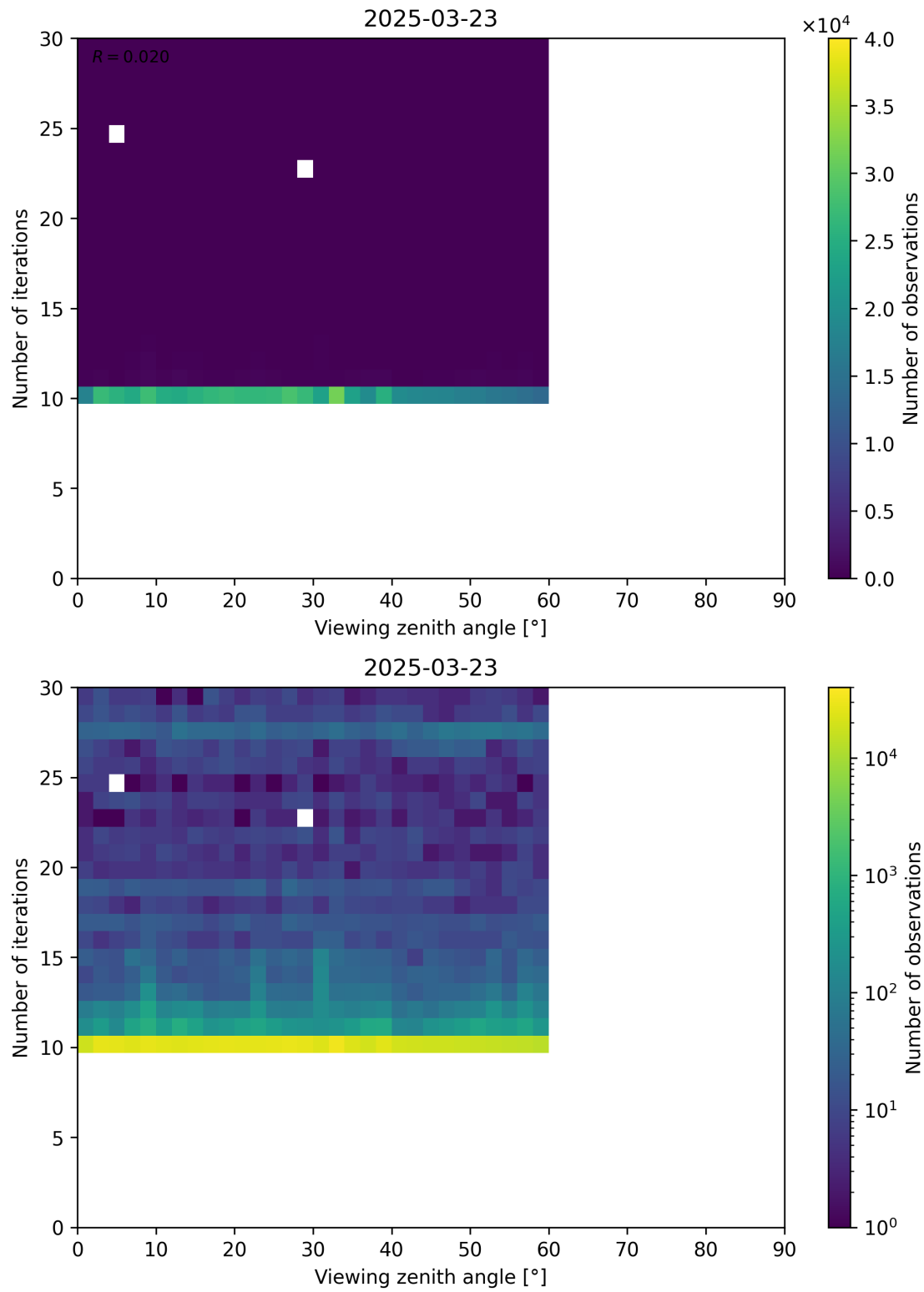
Figure 113: Scatter density plot of “Viewing zenith angle” against “Number of iterations” for 2025-03-23 to 2025-03-24.
