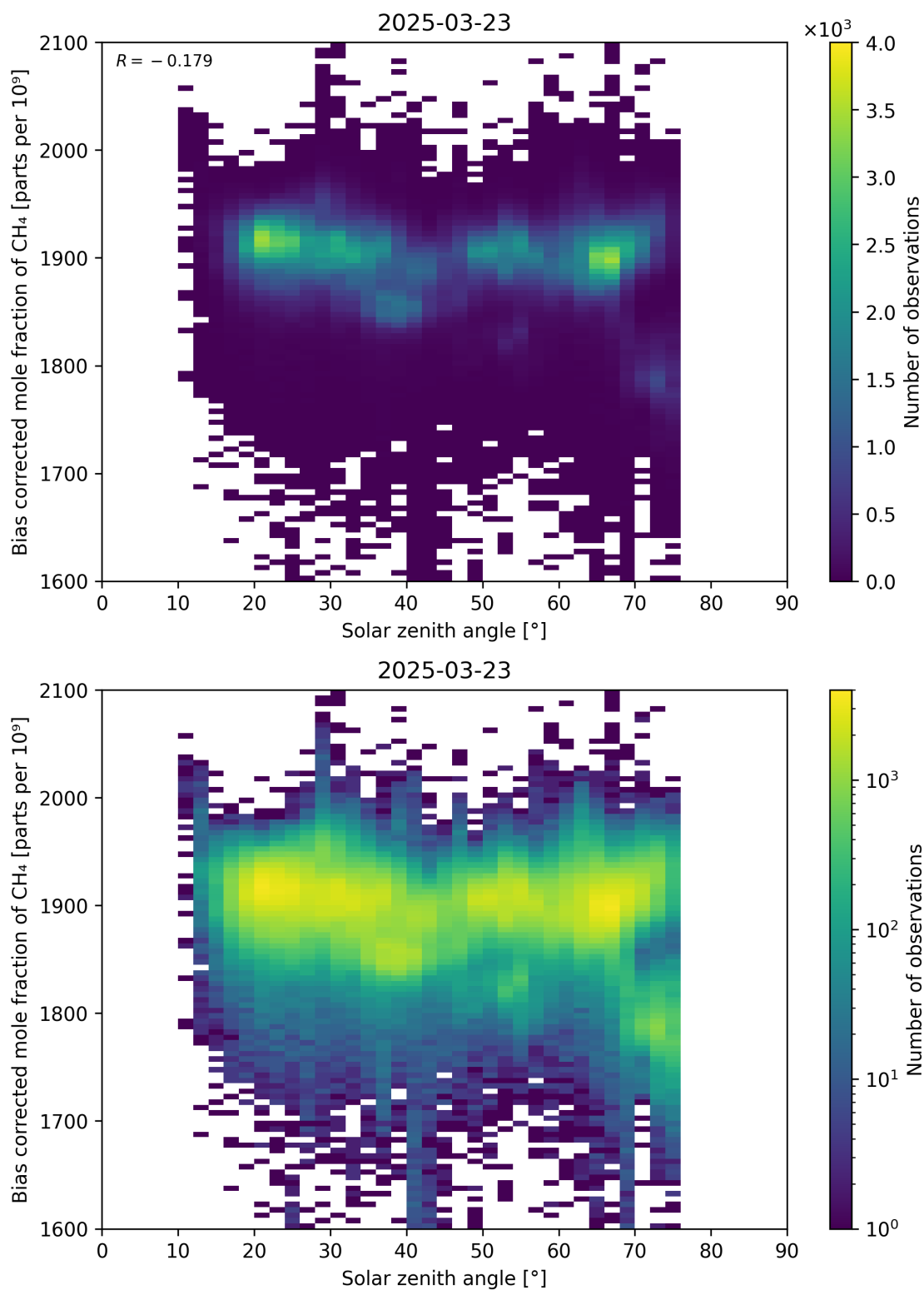
Figure 100: Scatter density plot of “Solar zenith angle” against “Bias corrected mole fraction of CH 4 ” for 2025-03-23 to 2025-03-24.
