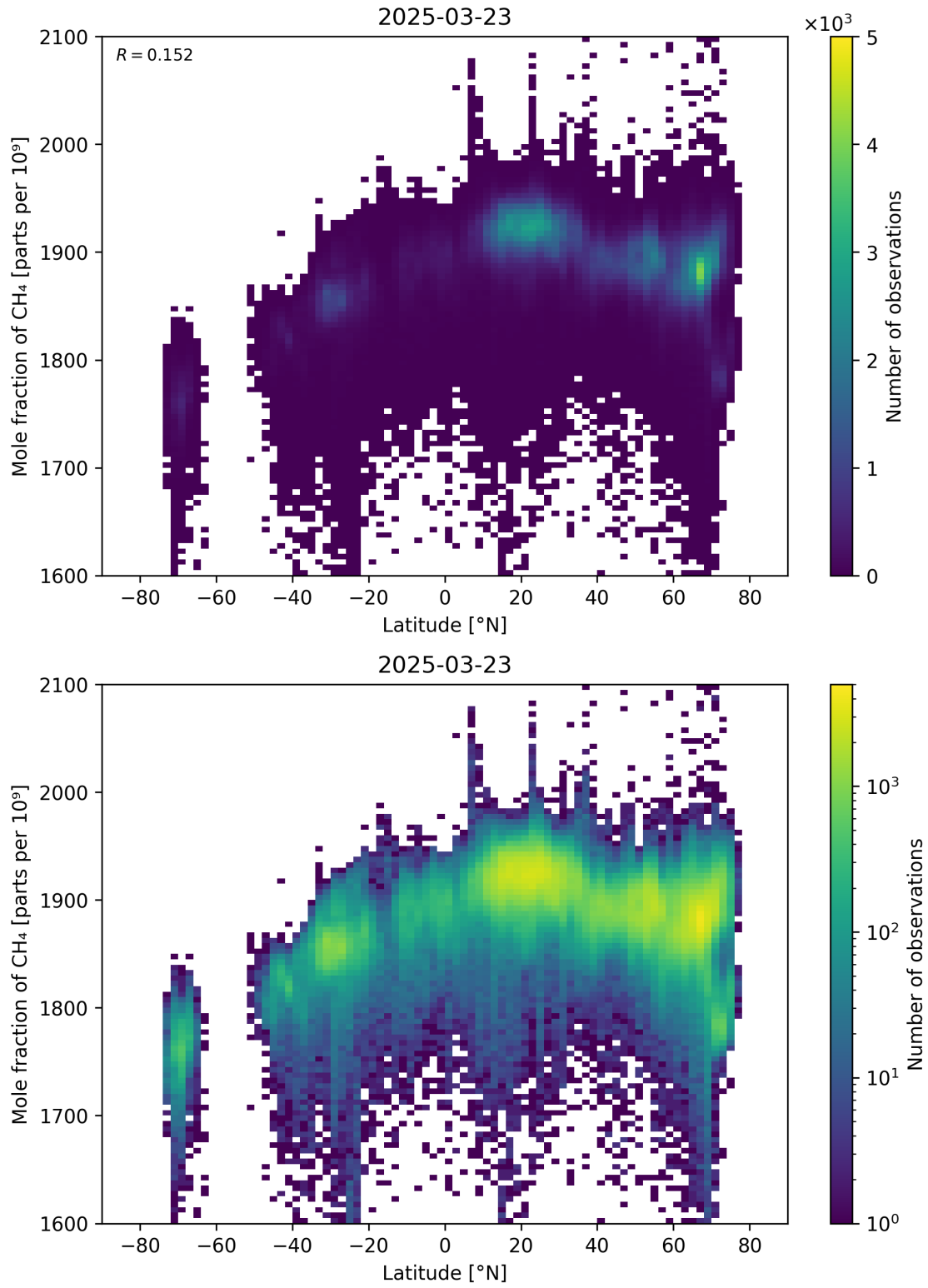
Figure 57: Scatter density plot of “Latitude” against “Mole fraction of \text{CH}_4 ” for 2025-03-23 to 2025-03-24.
