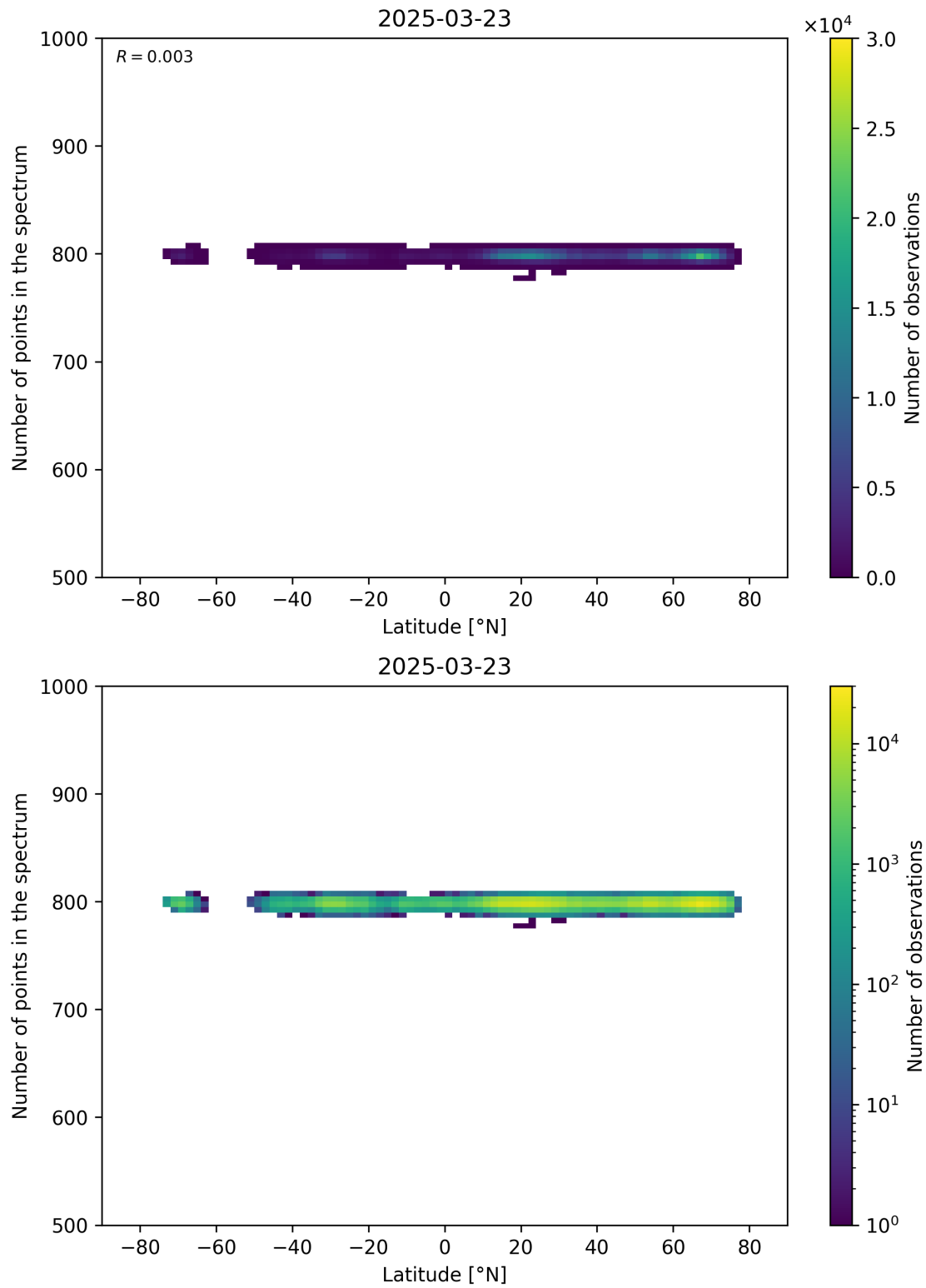
Figure 61: Scatter density plot of “Latitude” against “Number of points in the spectrum” for 2025-03-23 to 2025-03-24.
