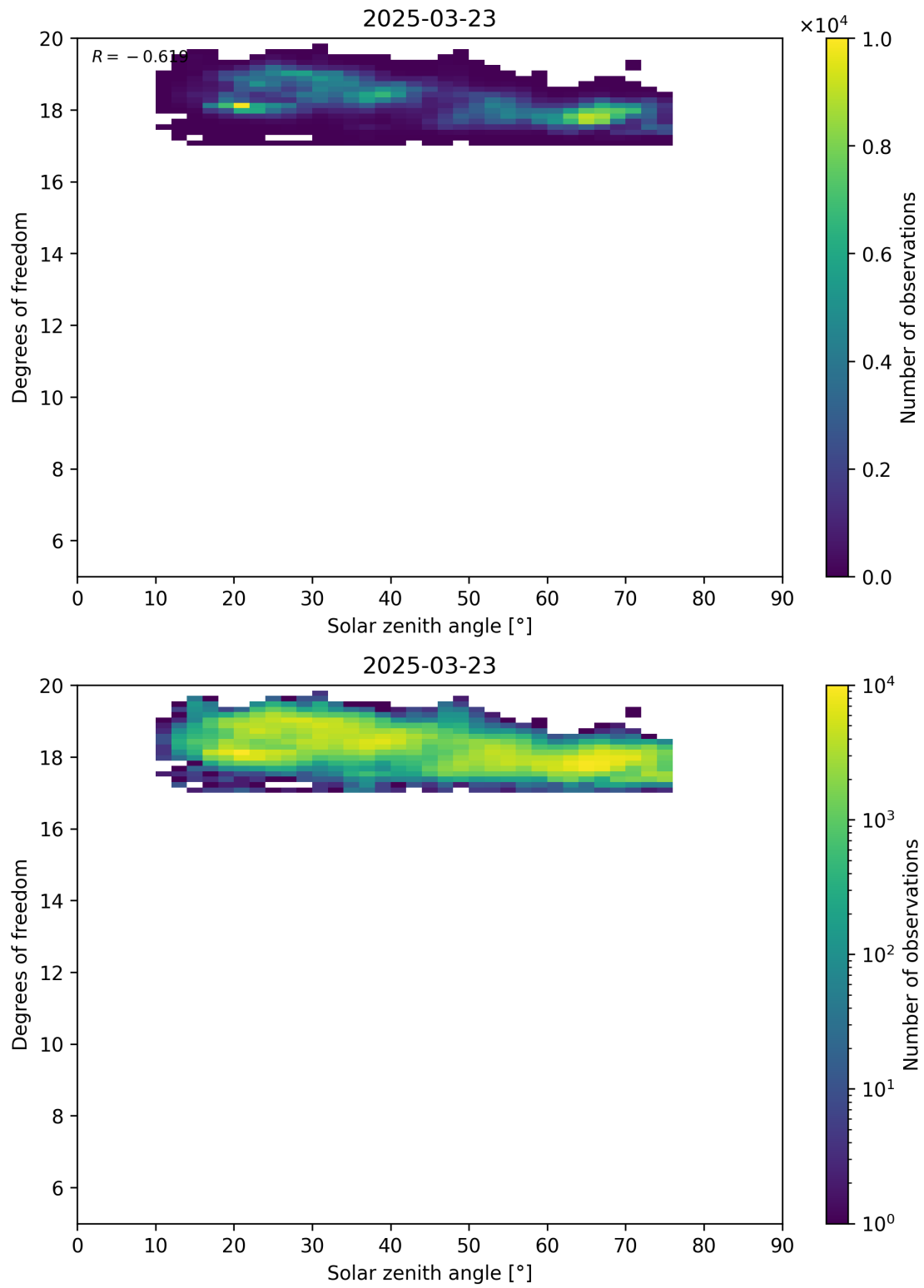
Figure 96: Scatter density plot of “Solar zenith angle” against “Degrees of freedom” for 2025-03-23 to 2025-03-24.
