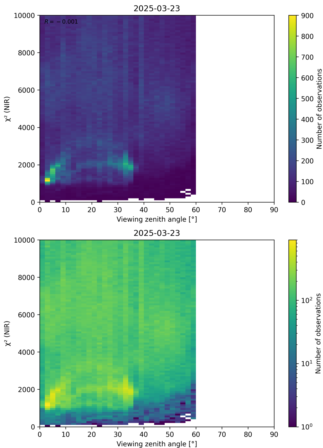
Figure 105: Scatter density plot of “Viewing zenith angle” against “ \chi^2 (NIR)” for 2025-03-23 to 2025-03-24.
