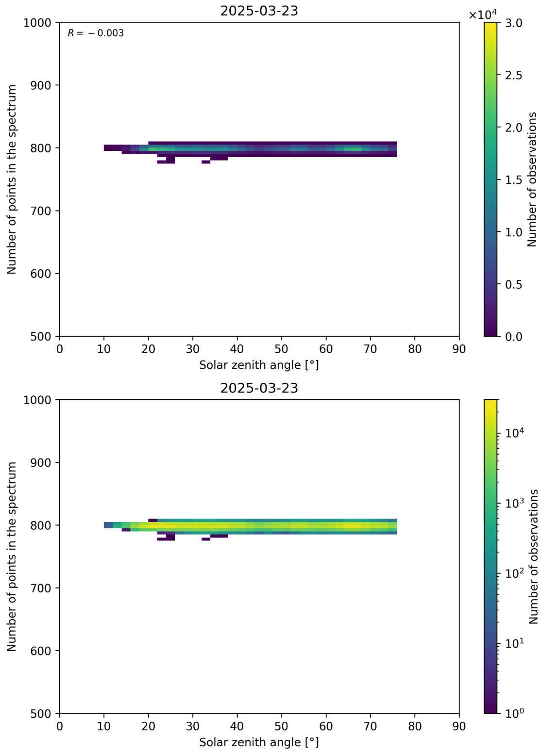
Figure 103: Scatter density plot of “Solar zenith angle” against “Number of points in the spectrum” for 2025-03-23 to 2025-03-24.
