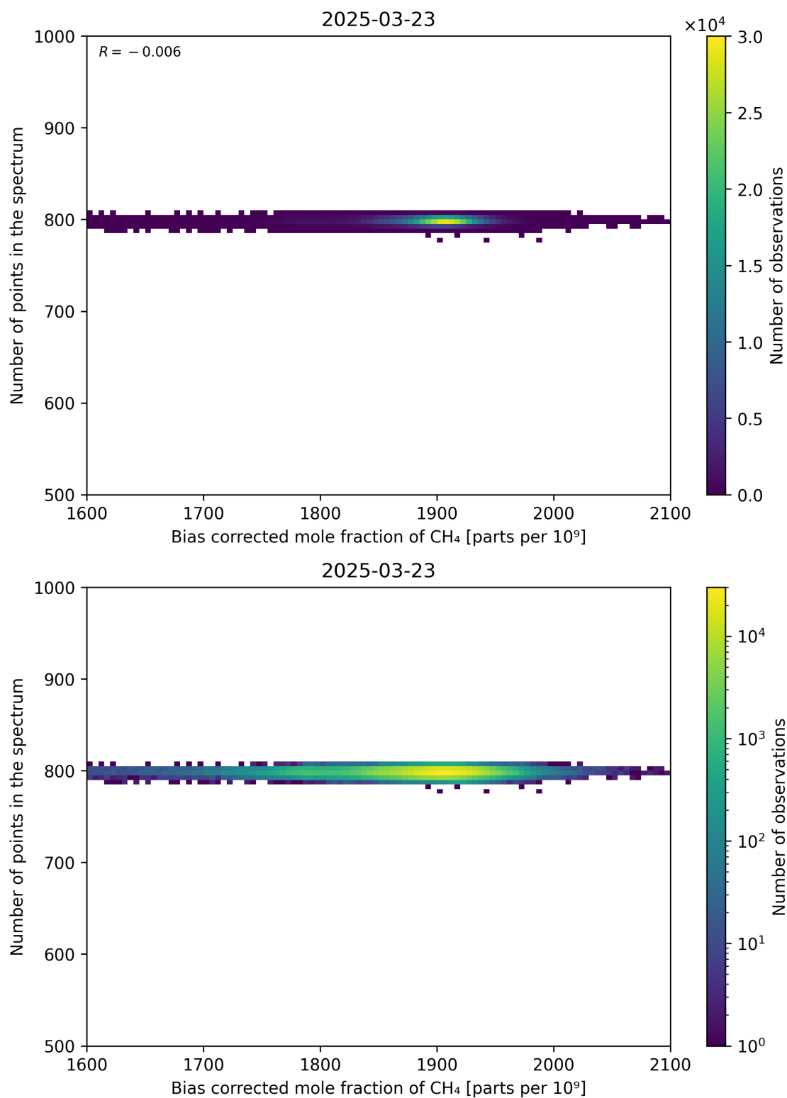
Figure 68: Scatter density plot of “Bias corrected mole fraction of CH 4 ” against “Number of points in the spectrum” for 2025-03-23 to 2025-03-24.
