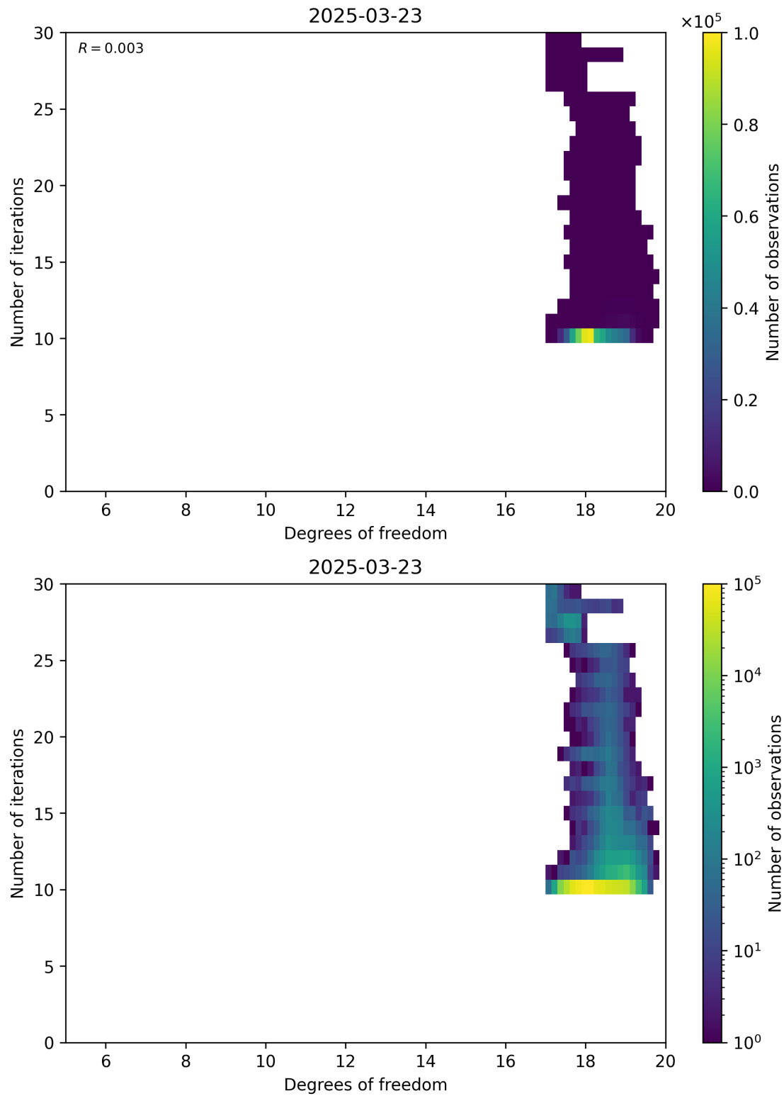
Figure 52: Scatter density plot of “Degrees of freedom” against “Number of iterations” for 2025-03-23 to 2025-03-24.
