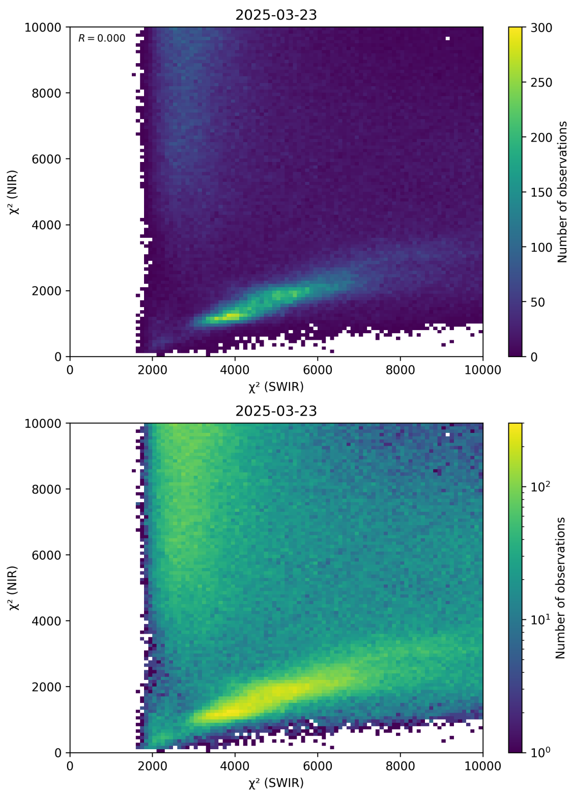
Figure 47: Scatter density plot of “ \chi^2 (SWIR)” against “ \chi^2 (NIR)” for 2025-03-23 to 2025-03-24.
