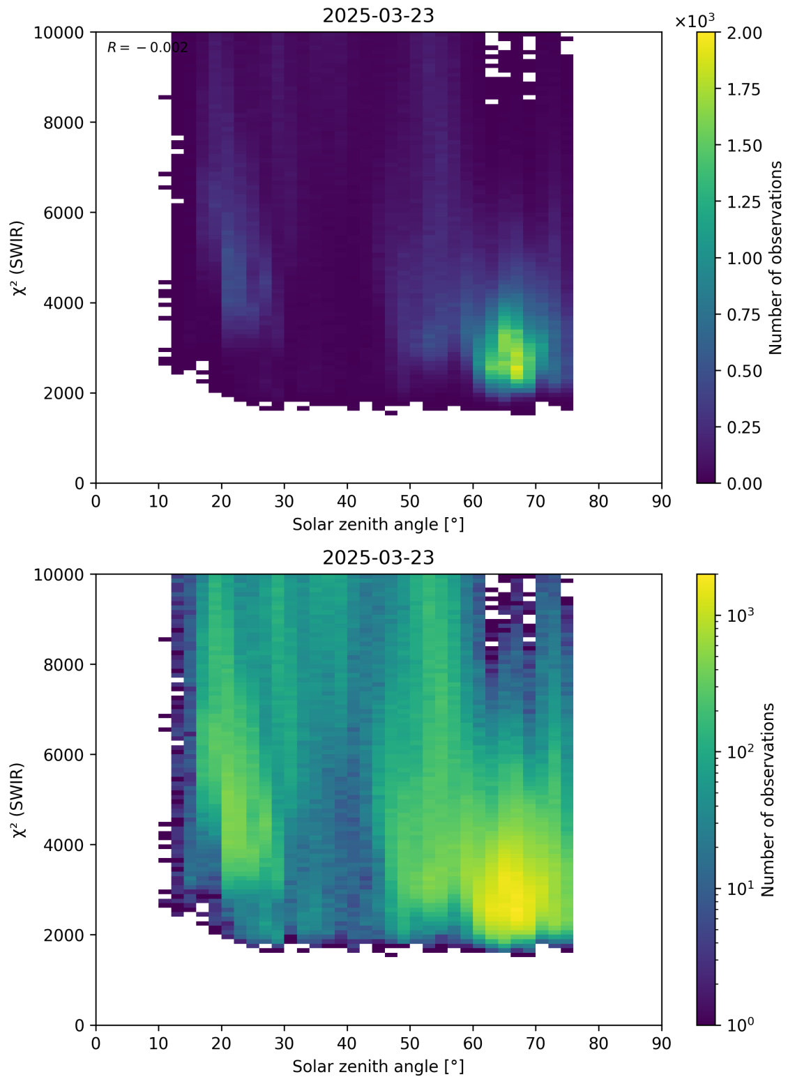
Figure 95: Scatter density plot of “Solar zenith angle” against “ \chi^2 (SWIR)” for 2025-03-23 to 2025-03-24.
