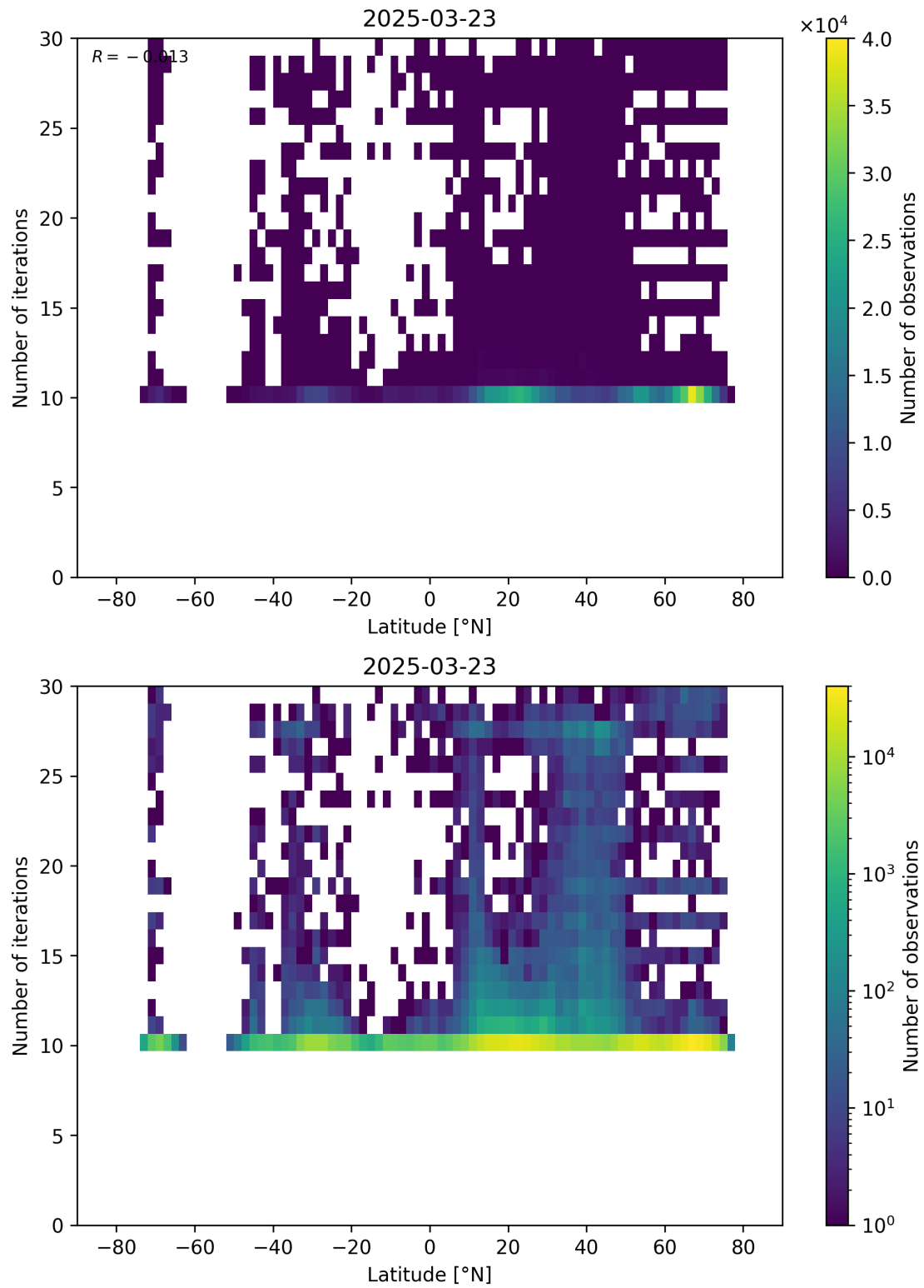
Figure 60: Scatter density plot of “Latitude” against “Number of iterations” for 2025-03-23 to 2025-03-24.
