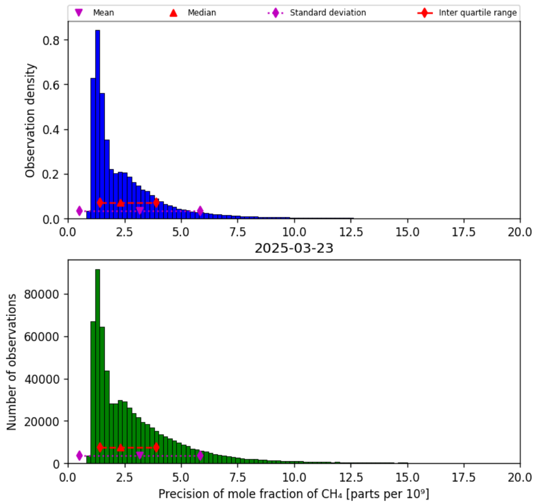
Figure 24: Histogram of “Precision of mole fraction of CH 4 ” for 2025-03-23 to 2025-03-24
