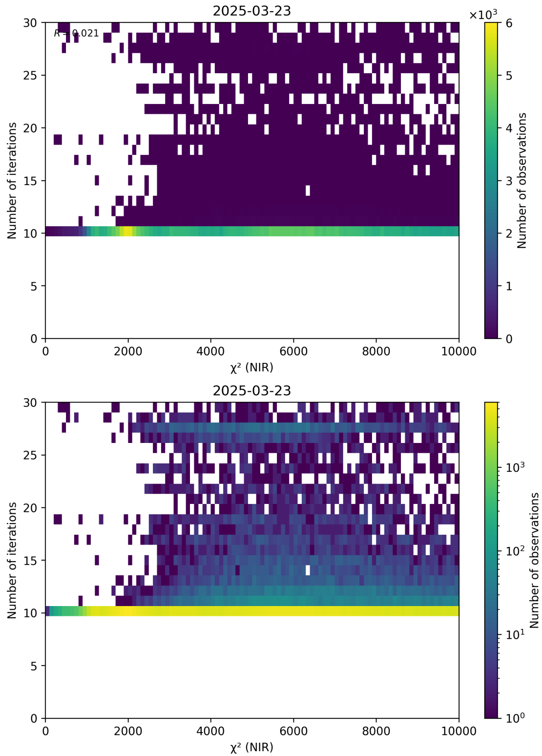
Figure 46: Scatter density plot of “ \chi^2 (NIR)” against “Number of iterations” for 2025-03-23 to 2025-03-24.
