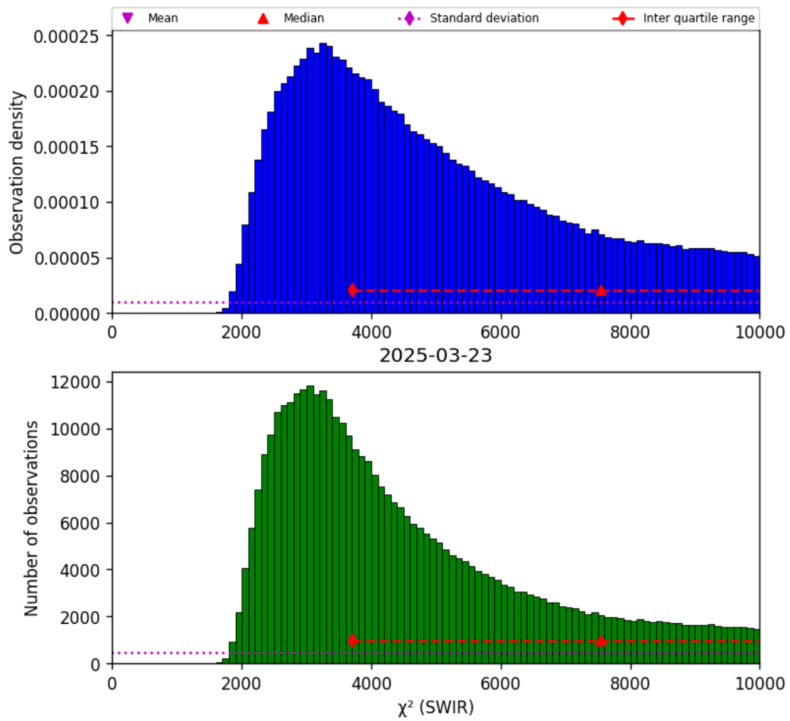
Figure 28: Histogram of “ \chi^2 (SWIR)” for 2025-03-23 to 2025-03-24
