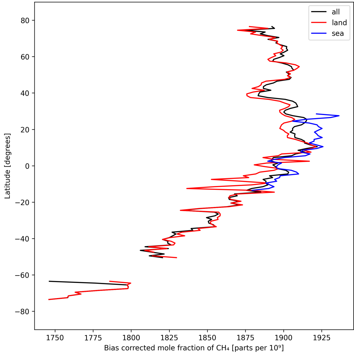
Figure 14: Zonal average of “Bias corrected mole fraction of CH 4 ” for 2025-03-23 to 2025-03-24.
