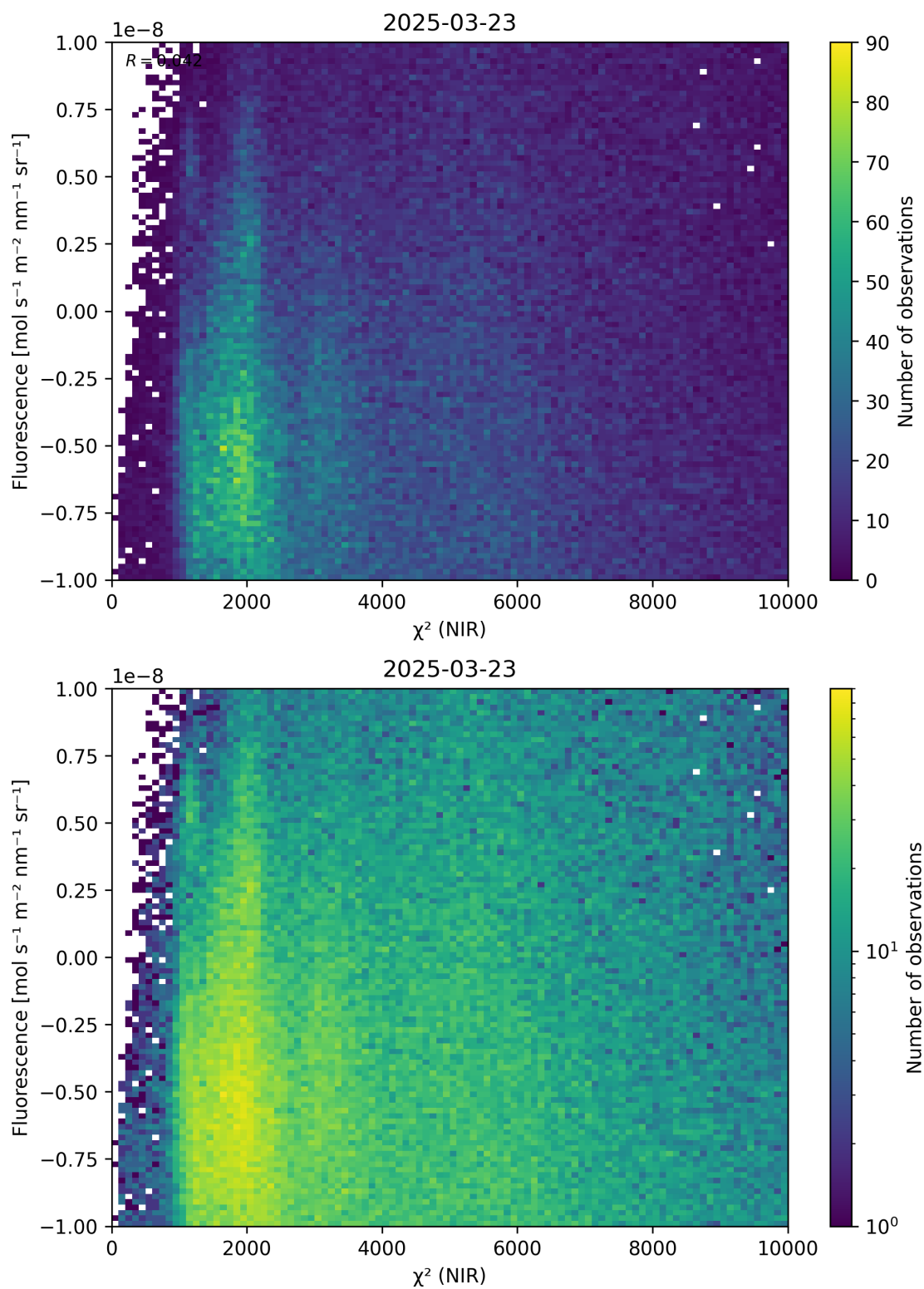
Figure 45: Scatter density plot of “ \chi^2 (NIR)” against “Fluorescence” for 2025-03-23 to 2025-03-24.
