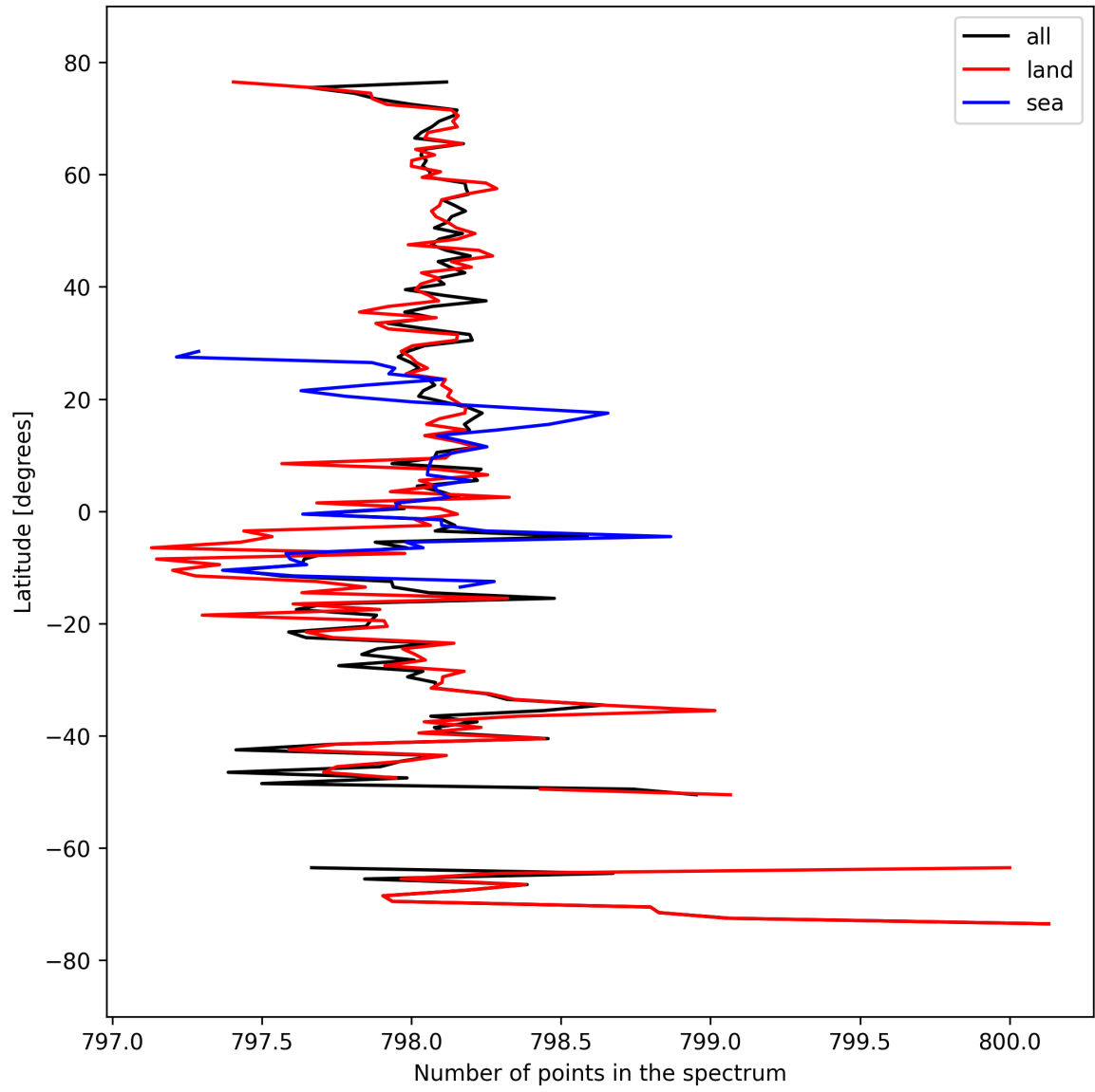
Figure 15: Zonal average of “Number of points in the spectrum” for 2025-03-23 to 2025-03-24.
