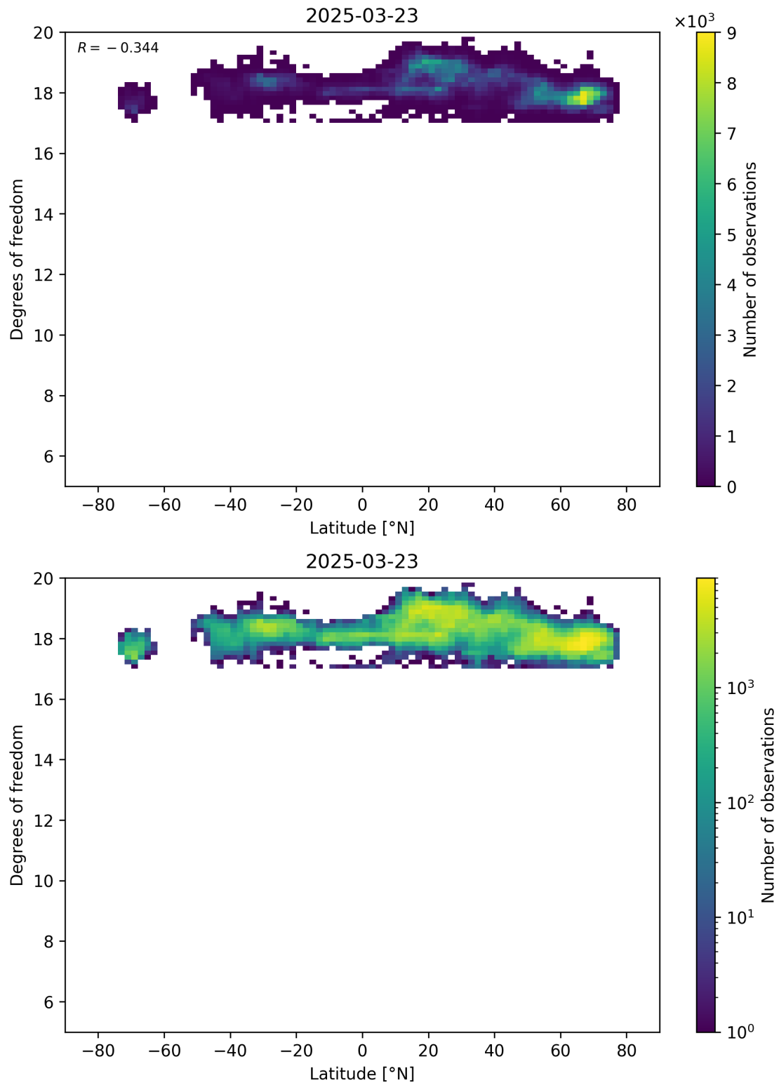
Figure 55: Scatter density plot of “Latitude” against “Degrees of freedom” for 2025-03-23 to 2025-03-24.
