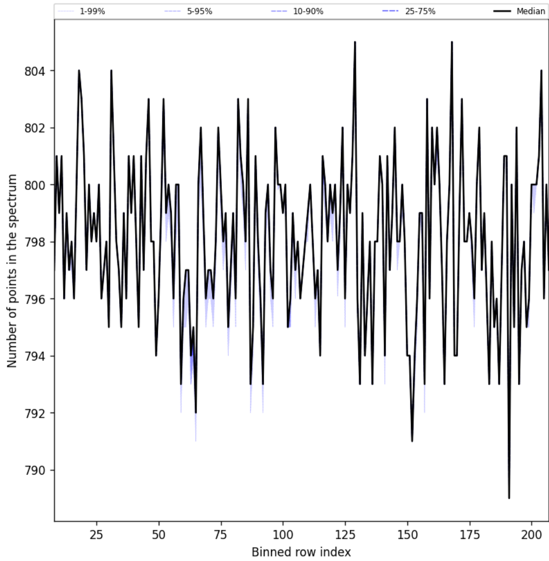
Figure 37: Along track statistics of “Number of points in the spectrum” for 2025-03-23 to 2025-03-24
