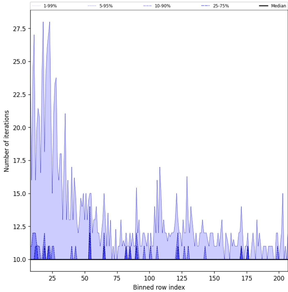
Figure 42: Along track statistics of “Number of iterations” for 2025-03-23 to 2025-03-24
