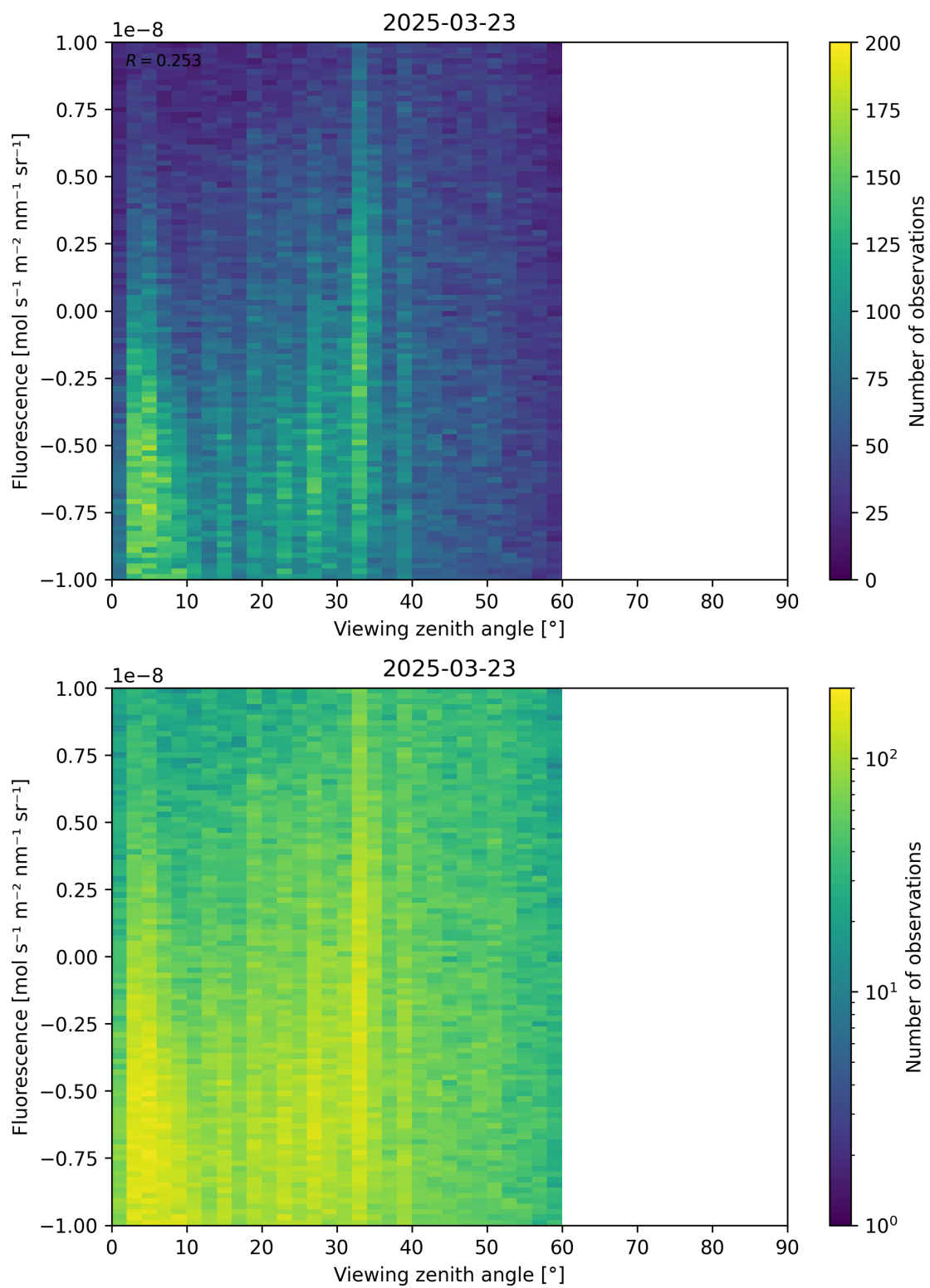
Figure 108: Scatter density plot of “Viewing zenith angle” against “Fluorescence” for 2025-03-23 to 2025-03-24.
