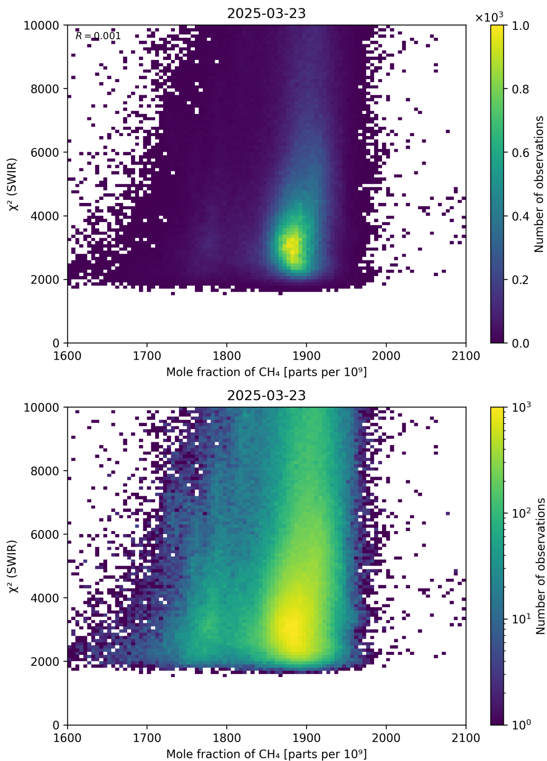
Figure 71: Scatter density plot of “Mole fraction of \text{CH}_4 ” against “ \chi^2 (SWIR)” for 2025-03-23 to 2025-03-24.
