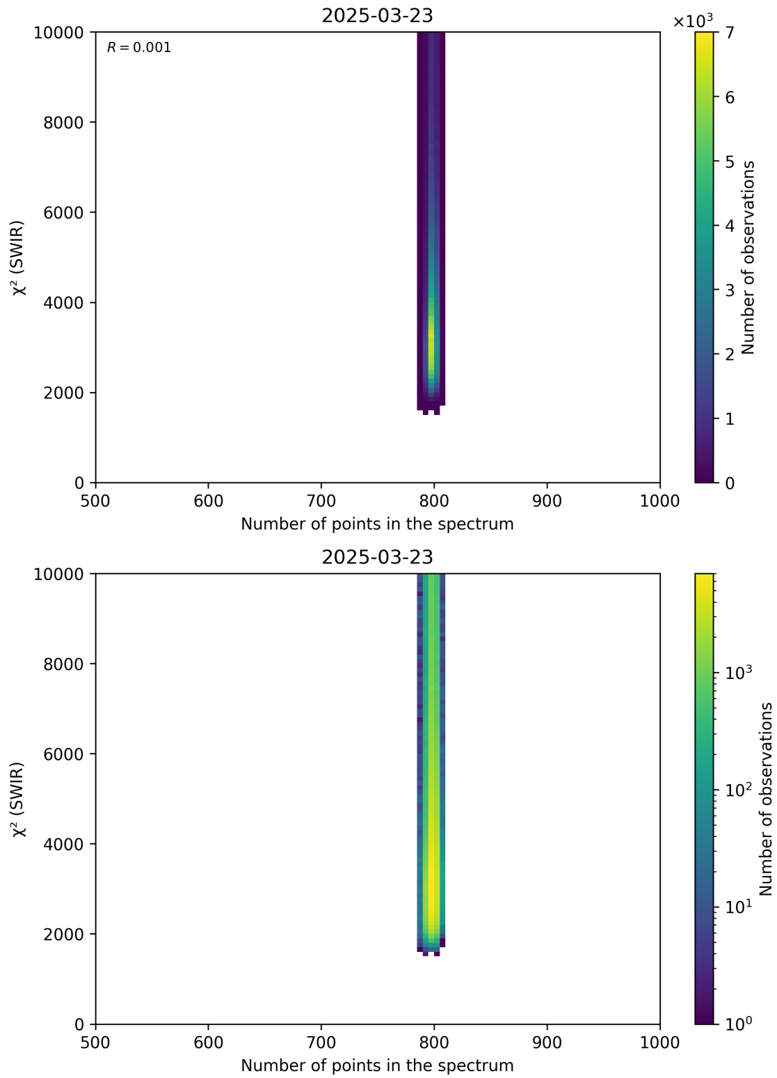
Figure 89: Scatter density plot of “Number of points in the spectrum” against “ \chi^2 (SWIR)” for 2025-03-23 to 2025-03-24.
