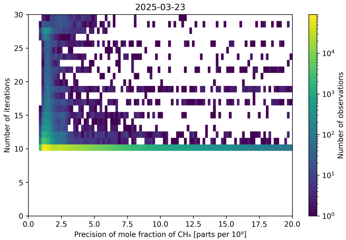
Figure 83: Scatter density plot of “Precision of mole fraction of CH 4 ” against “Number of iterations” for 2025-03-23 to 2025-03-24.
