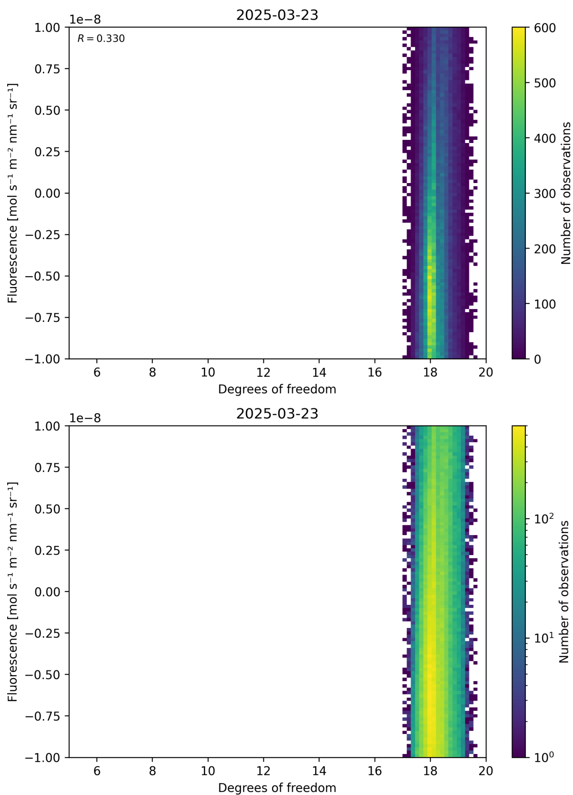
Figure 51: Scatter density plot of “Degrees of freedom” against “Fluorescence” for 2025-03-23 to 2025-03-24.
