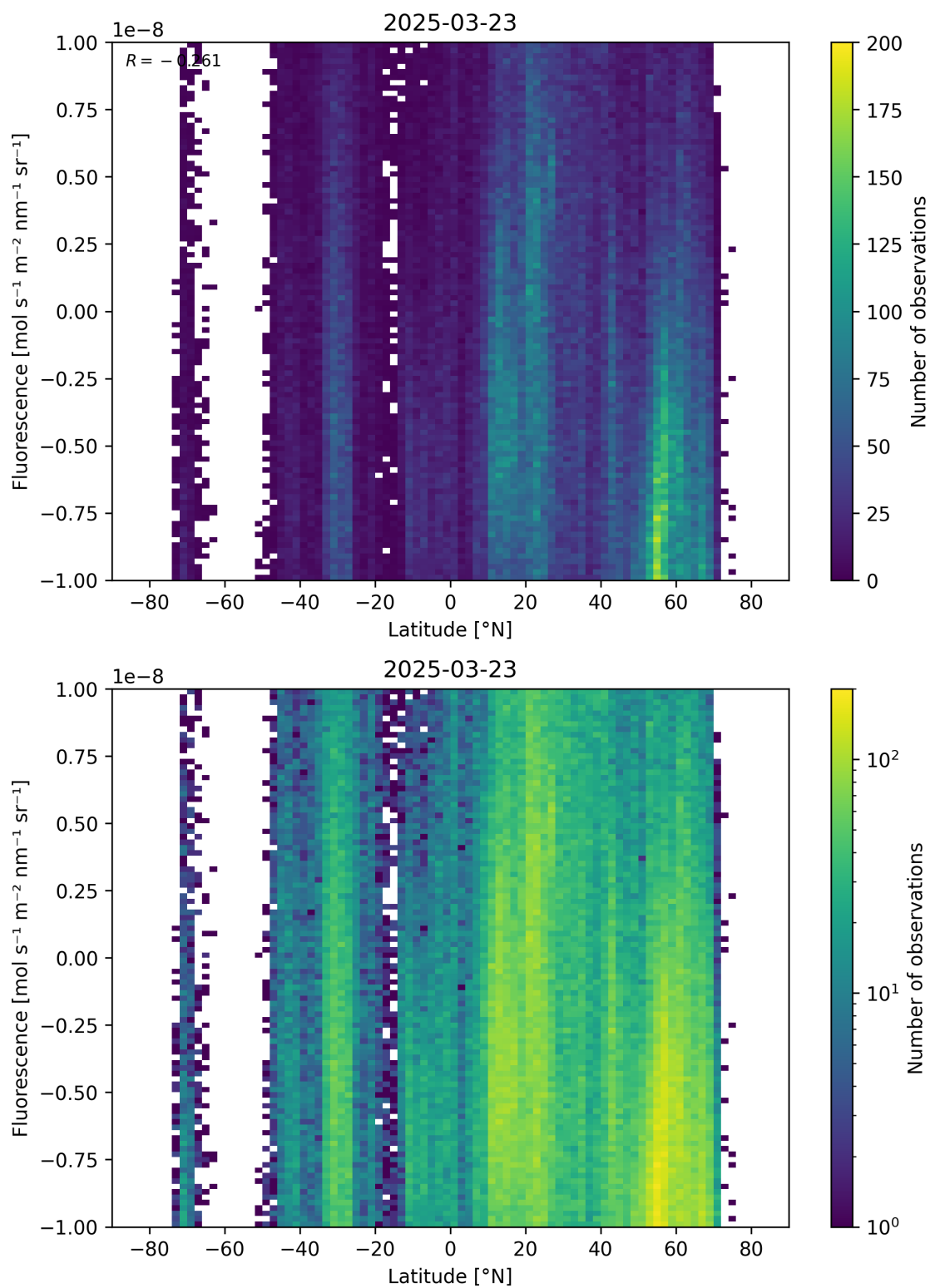
Figure 56: Scatter density plot of “Latitude” against “Fluorescence” for 2025-03-23 to 2025-03-24.
