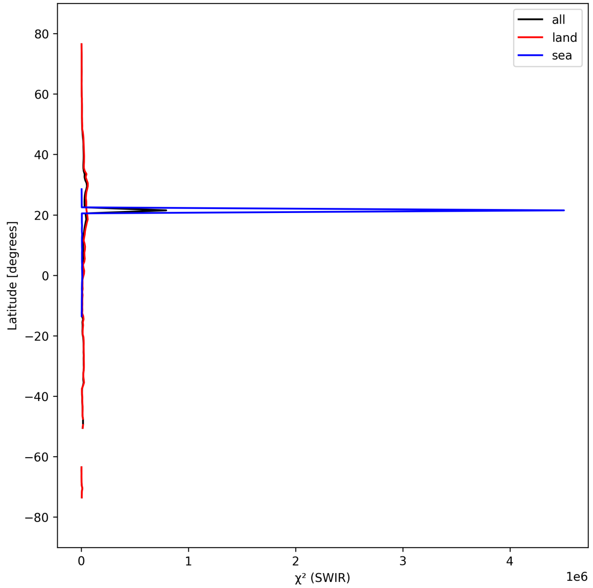
Figure 17: Zonal average of “ \chi^2 (SWIR)” for 2025-03-23 to 2025-03-24.
