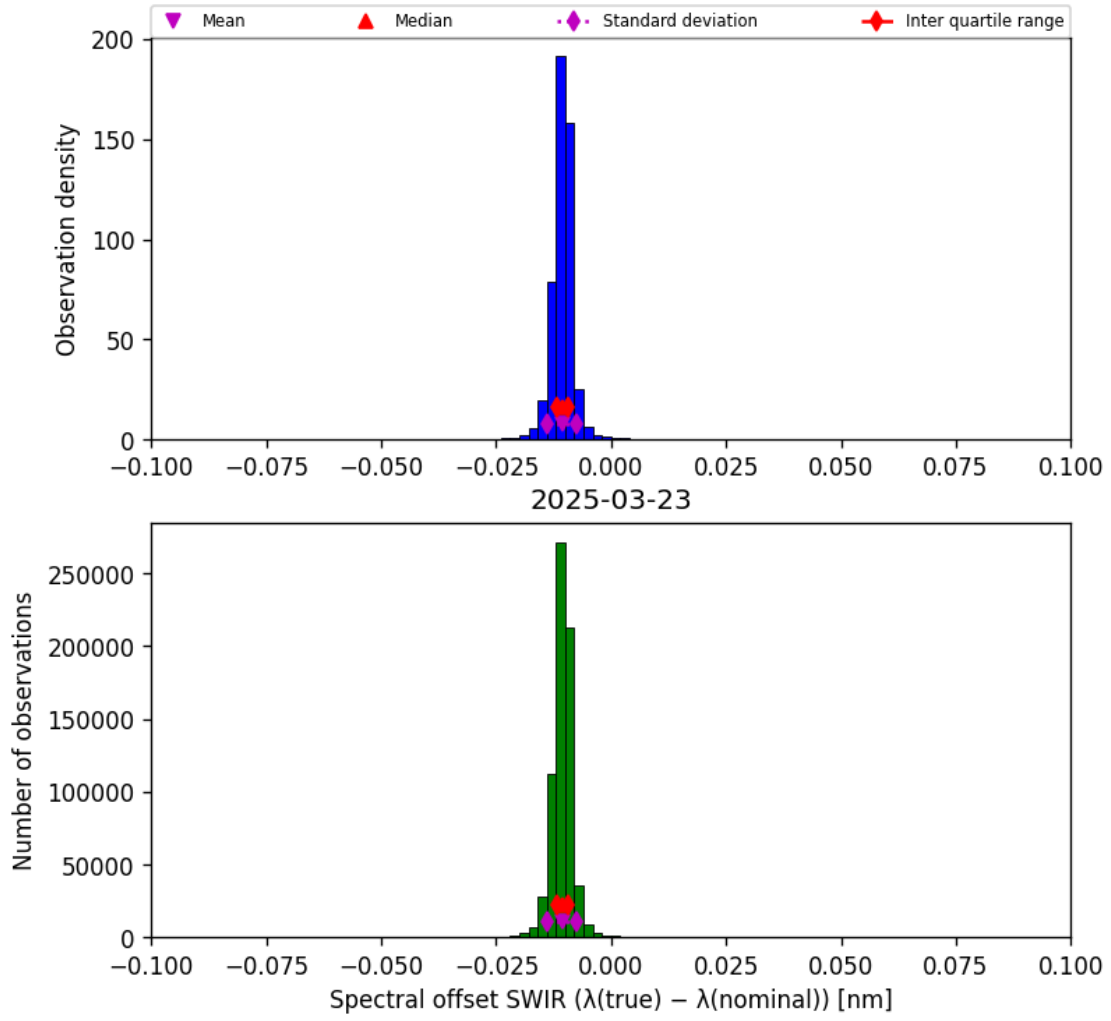
Figure 27: Histogram of “Spectral offset SWIR ( \lambda_{\text{true}} - \lambda_{\text{nominal}} )” for 2025-03-23 to 2025-03-24
