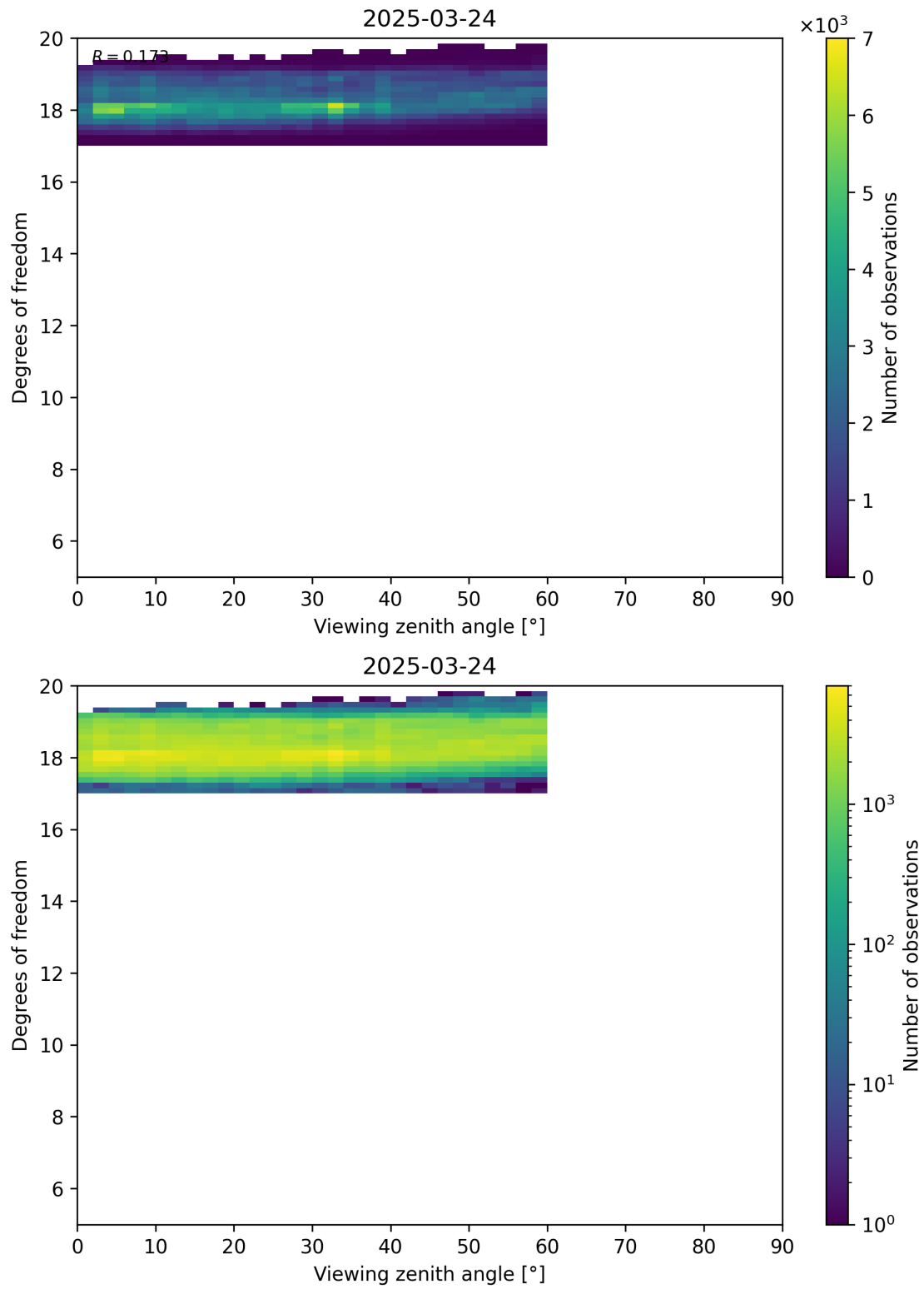
Figure 107: Scatter density plot of “Viewing zenith angle” against “Degrees of freedom” for 2025-03-23 to 2025-03-25.
