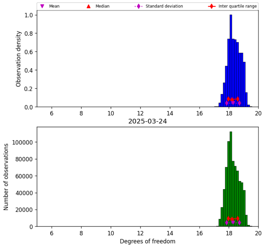
Figure 30: Histogram of “Degrees of freedom” for 2025-03-23 to 2025-03-25
