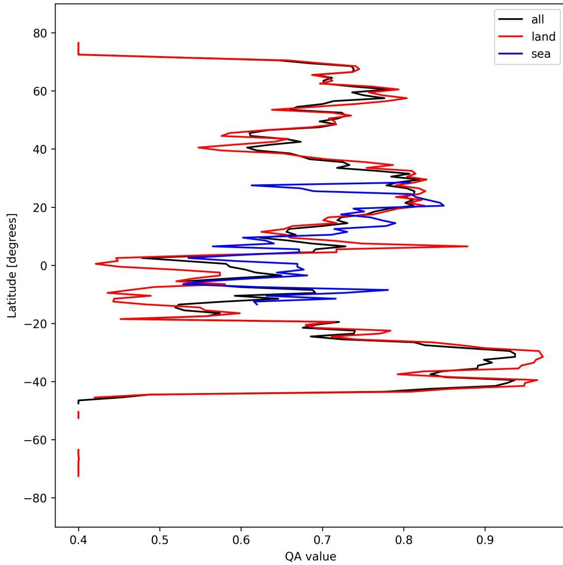
Figure 11: Zonal average of “QA value” for 2025-03-23 to 2025-03-25.
