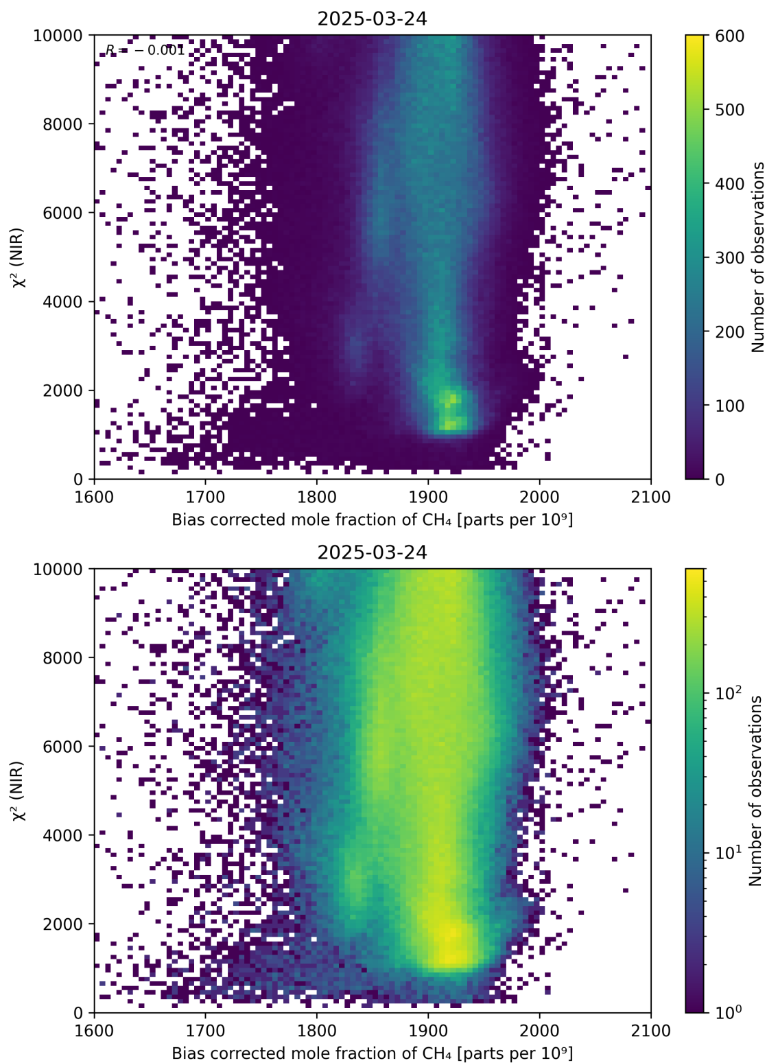
Figure 63: Scatter density plot of “Bias corrected mole fraction of \text{CH}_4 ” against “ \chi^2 (NIR)” for 2025-03-23 to 2025-03-25.
