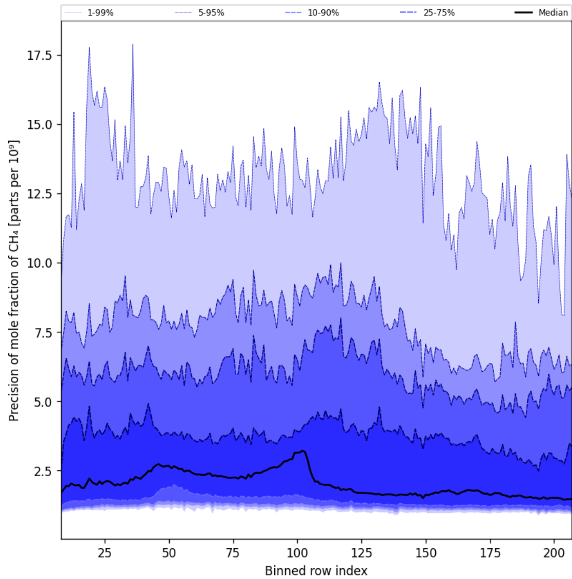
Figure 35: Along track statistics of “Precision of mole fraction of CH 4 ” for 2025-03-23 to 2025-03-25
