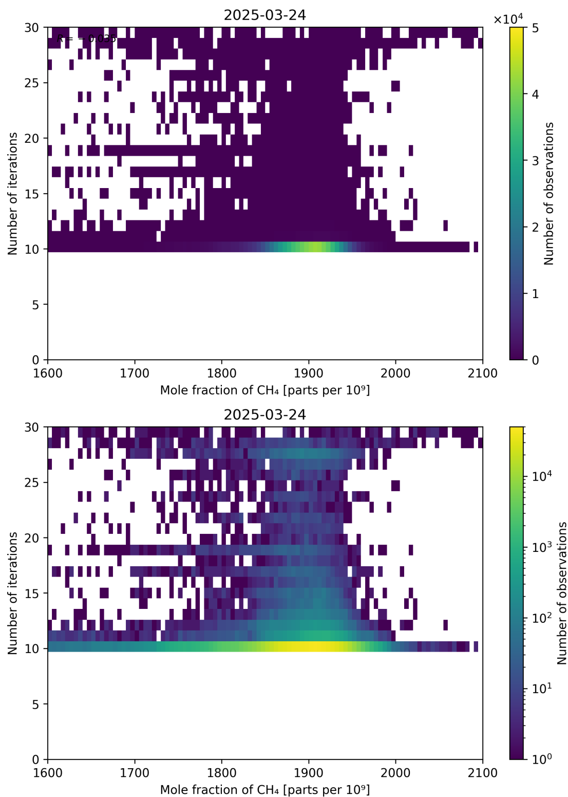
Figure 76: Scatter density plot of “Mole fraction of CH 4 ” against “Number of iterations” for 2025-03-23 to 2025-03-25.
