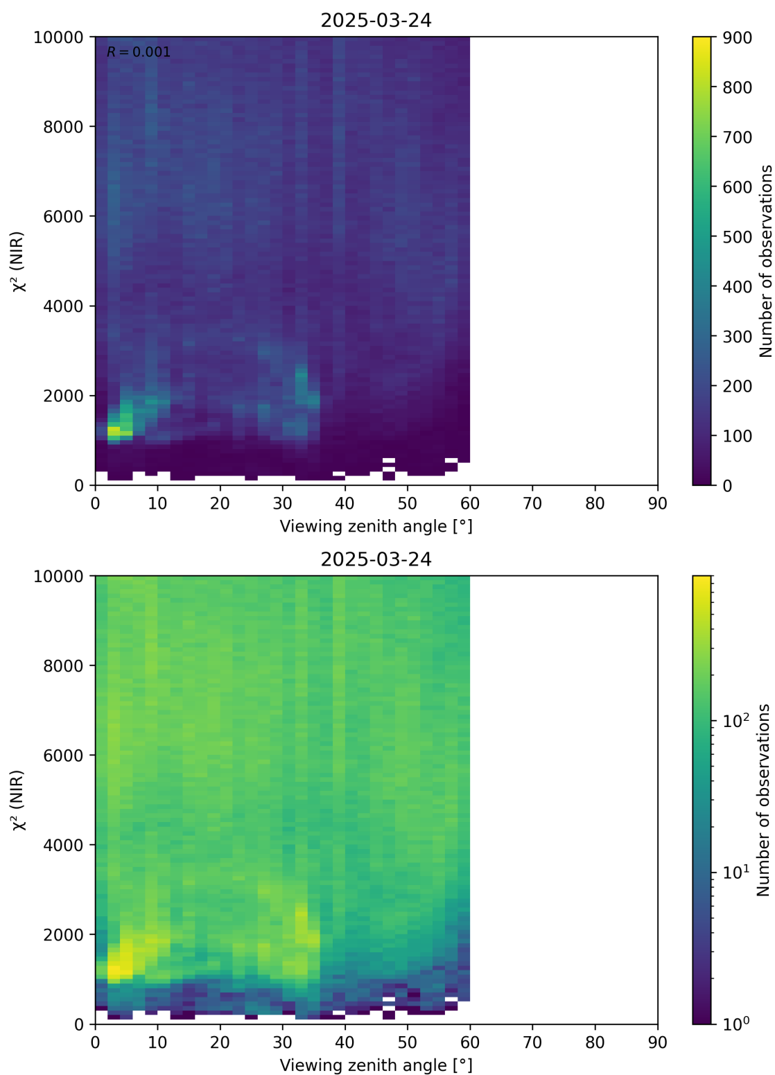
Figure 105: Scatter density plot of “Viewing zenith angle” against “ \chi^2 (NIR)” for 2025-03-23 to 2025-03-25.
