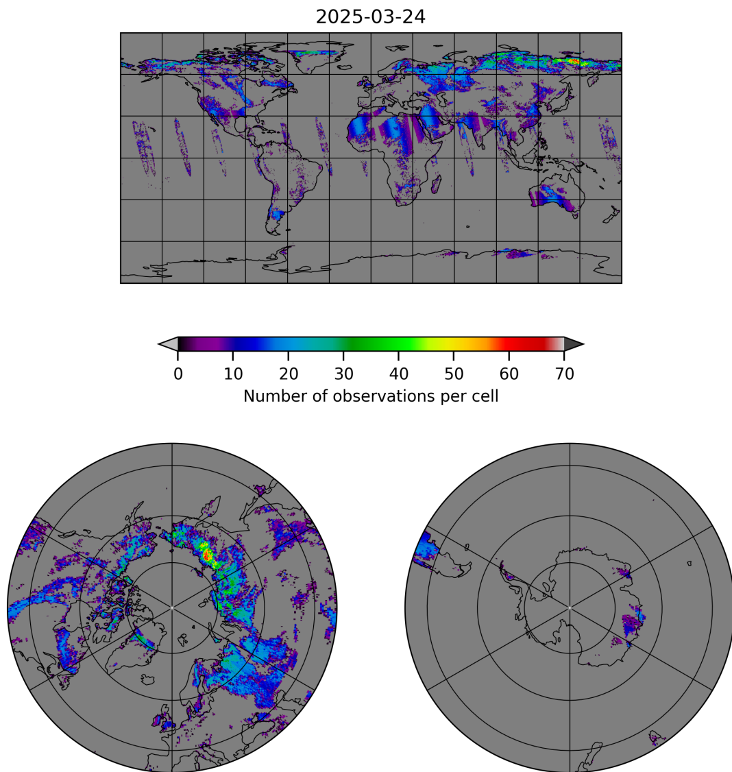
Figure 10: Map of the number of observations for 2025-03-23 to 2025-03-25
