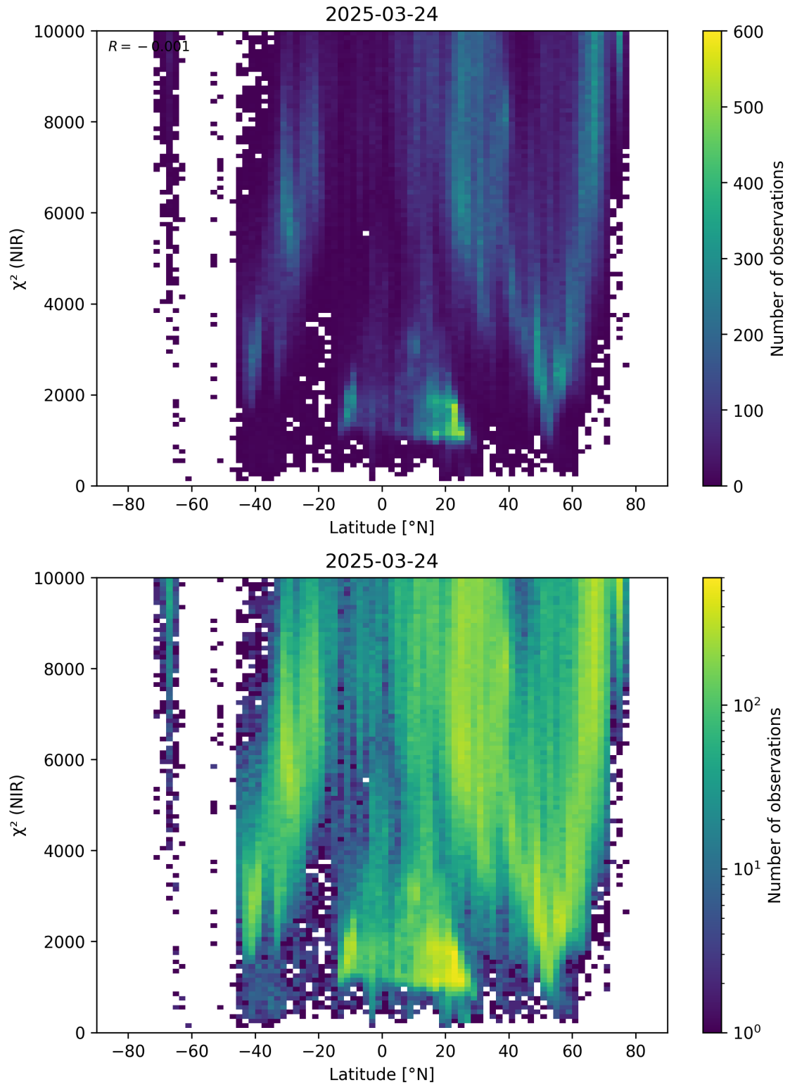
Figure 53: Scatter density plot of “Latitude” against “ \chi^2 (NIR)” for 2025-03-23 to 2025-03-25.
