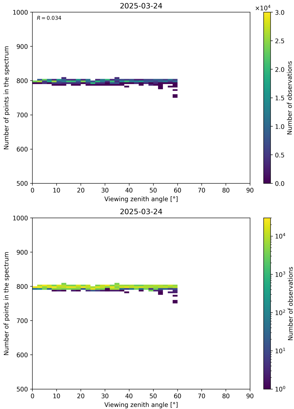
Figure 114: Scatter density plot of “Viewing zenith angle” against “Number of points in the spectrum” for 2025-03-23 to 2025-03-25.
