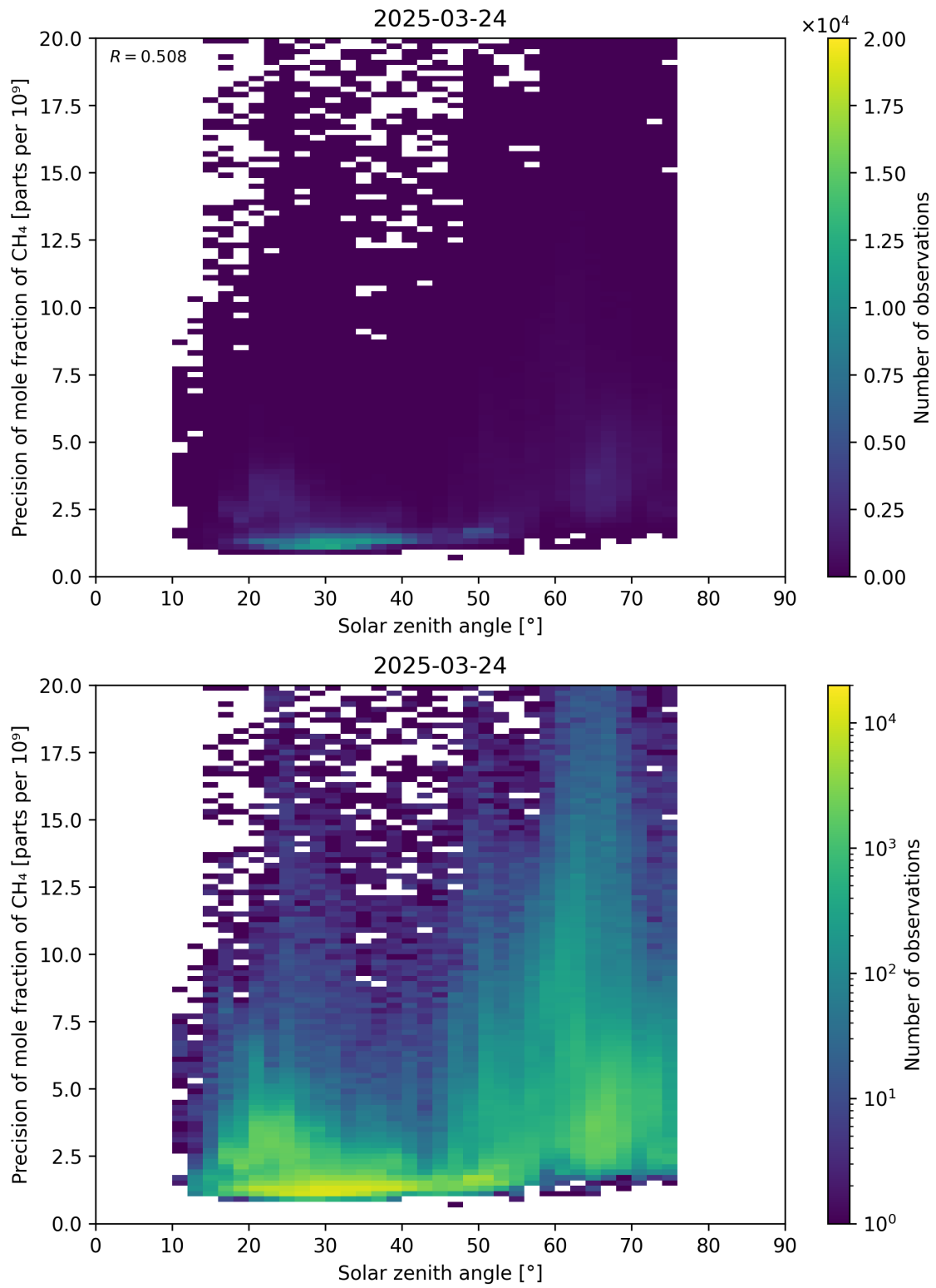
Figure 101: Scatter density plot of “Solar zenith angle” against “Precision of mole fraction of CH 4 ” for 2025-03-23 to 2025-03-25.
