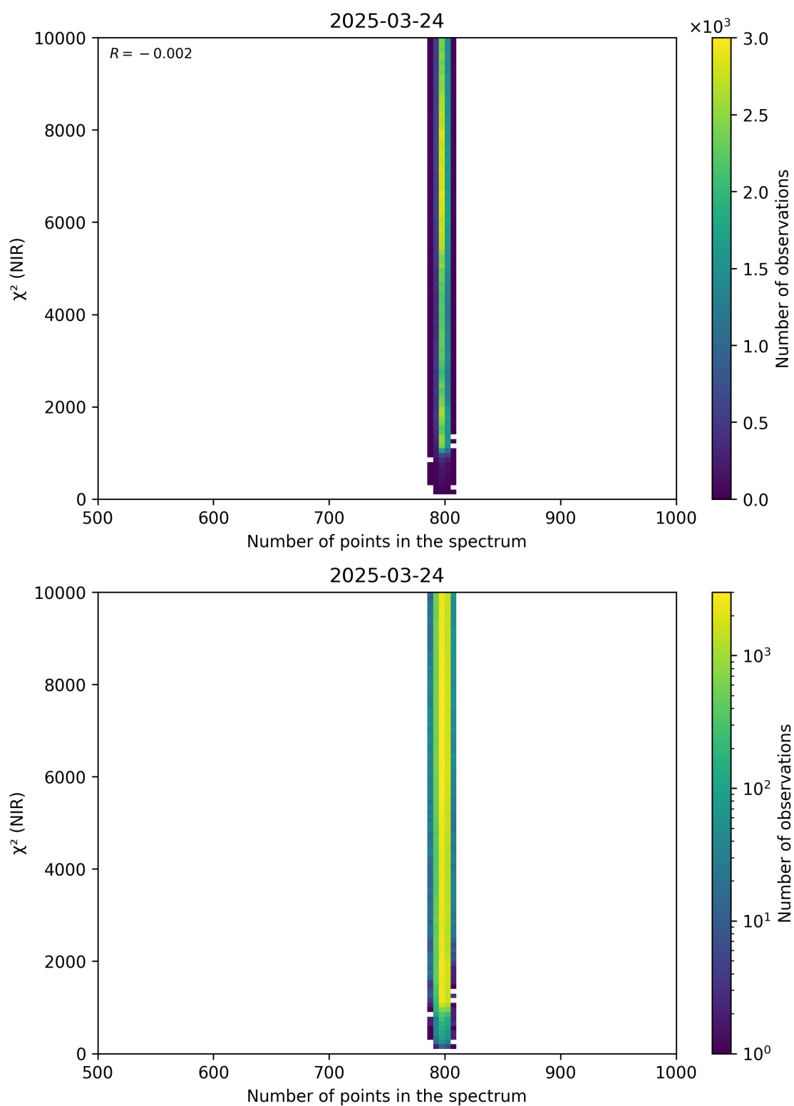
Figure 88: Scatter density plot of “Number of points in the spectrum” against “ \chi^2 (NIR)” for 2025-03-23 to 2025-03-25.
