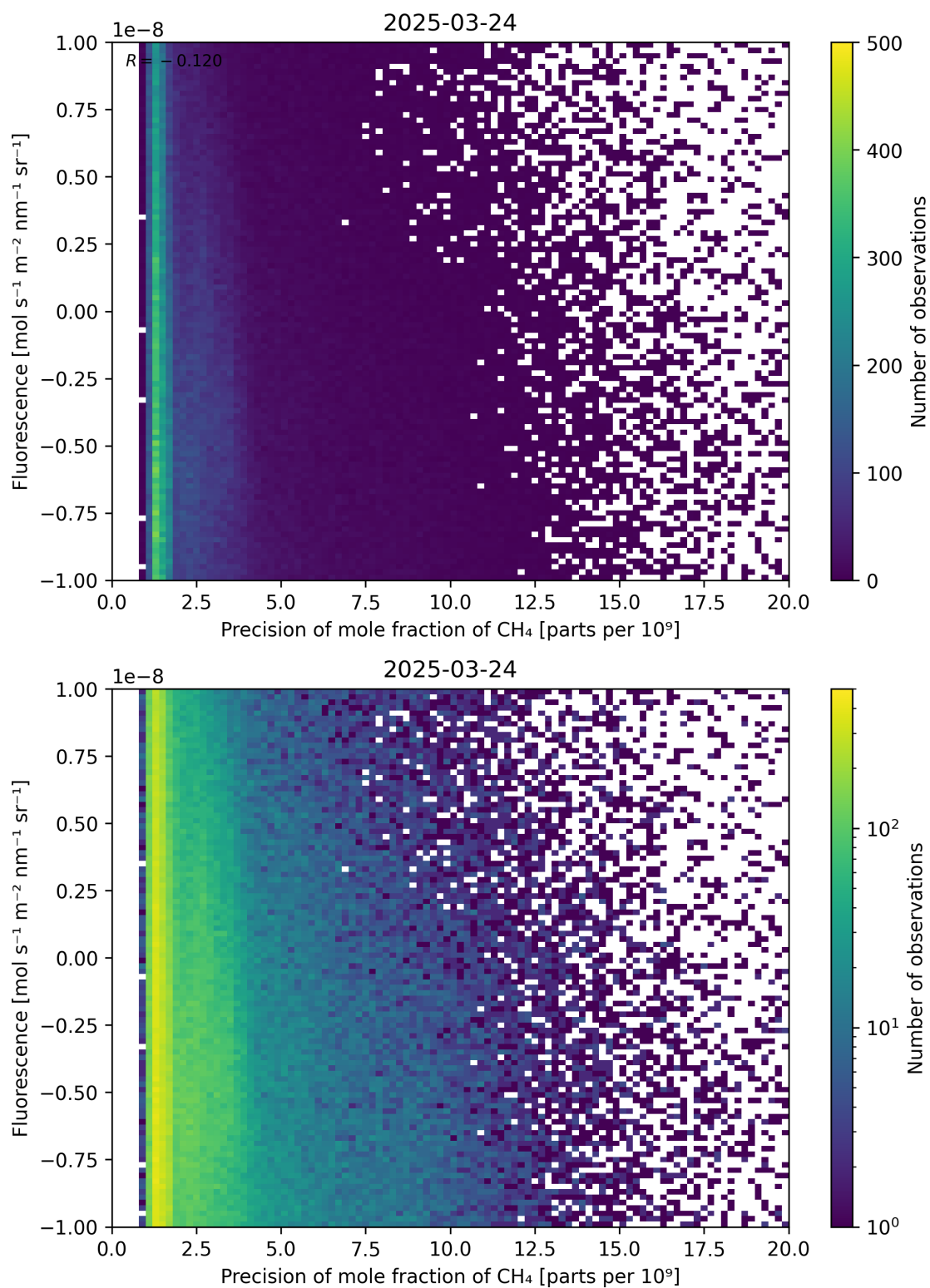
Figure 81: Scatter density plot of “Precision of mole fraction of CH 4 ” against “Fluorescence” for 2025-03-23 to 2025-03-25.
