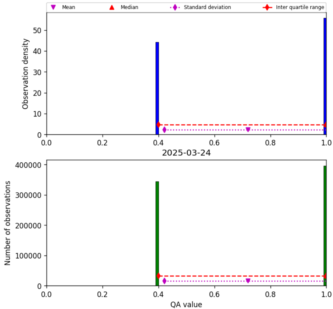
Figure 22: Histogram of “QA value” for 2025-03-23 to 2025-03-25
