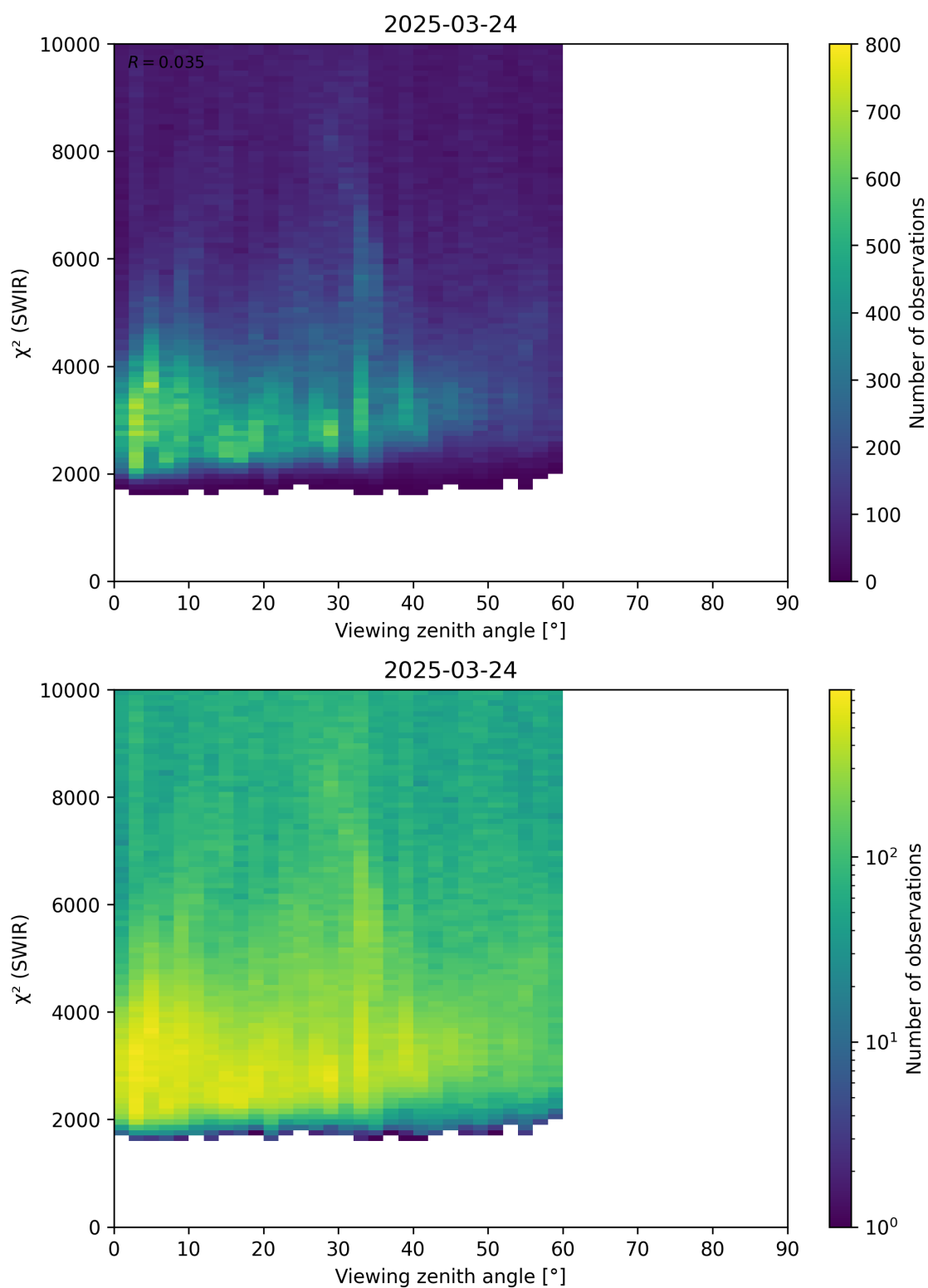
Figure 106: Scatter density plot of “Viewing zenith angle” against “ \chi^2 (SWIR)” for 2025-03-23 to 2025-03-25.
