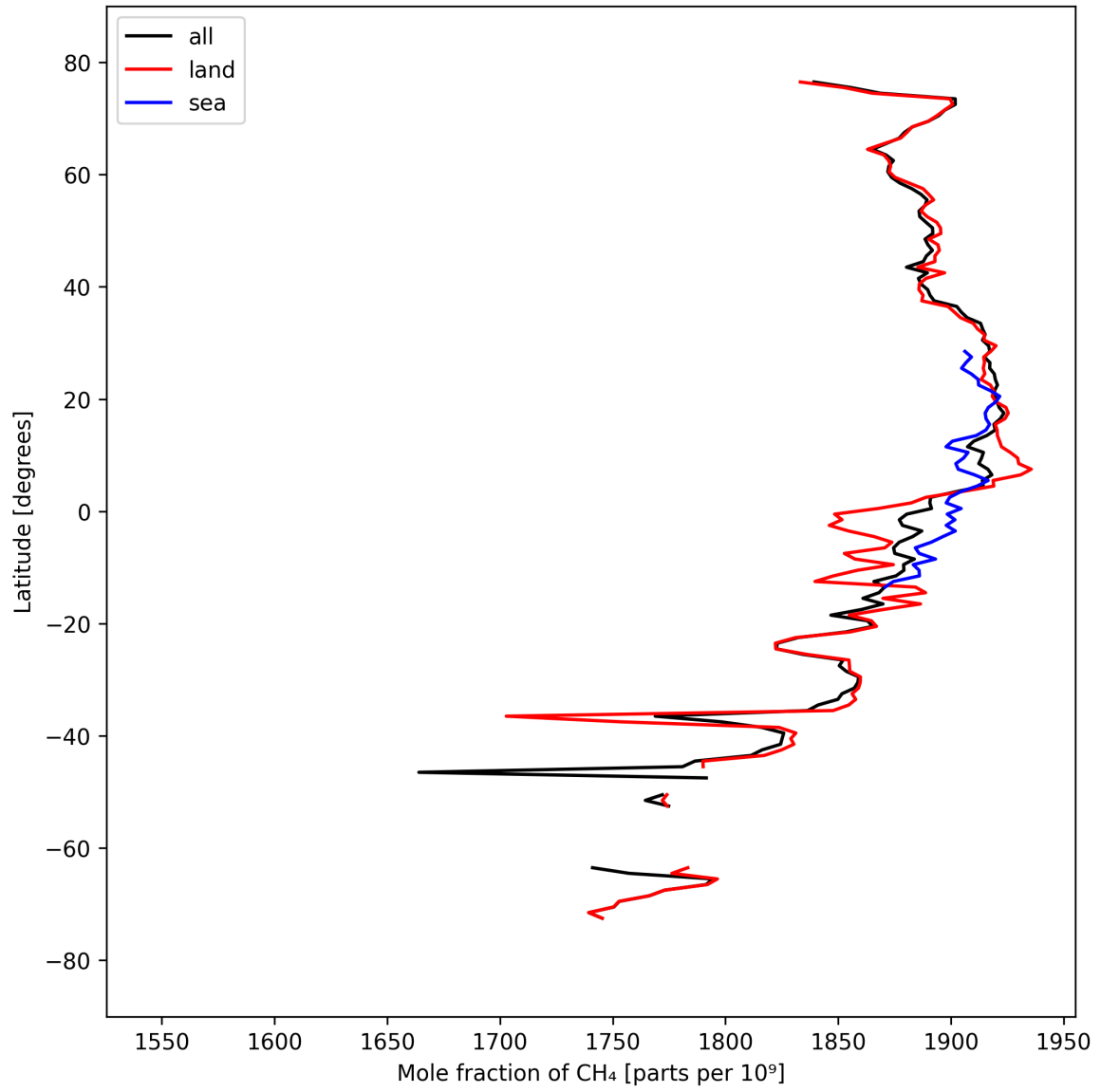
Figure 12: Zonal average of “Mole fraction of CH 4 ” for 2025-03-23 to 2025-03-25.
