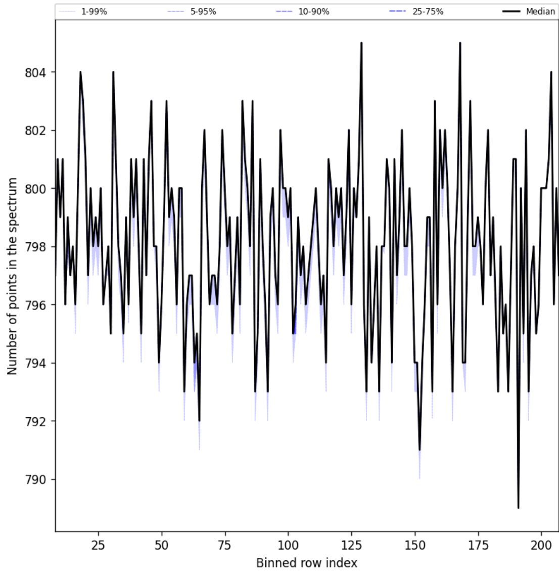
Figure 37: Along track statistics of “Number of points in the spectrum” for 2025-03-23 to 2025-03-25
