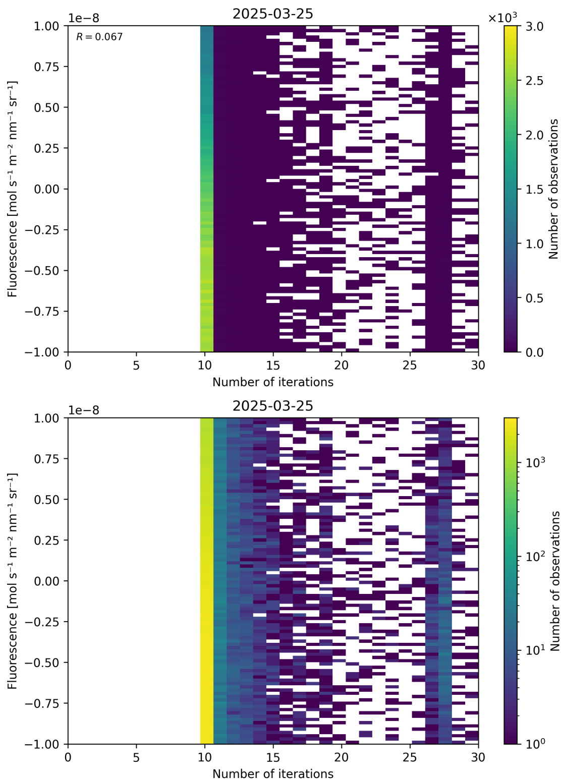
Figure 87: Scatter density plot of “Number of iterations” against “Fluorescence” for 2025-03-24 to 2025-03-26.
