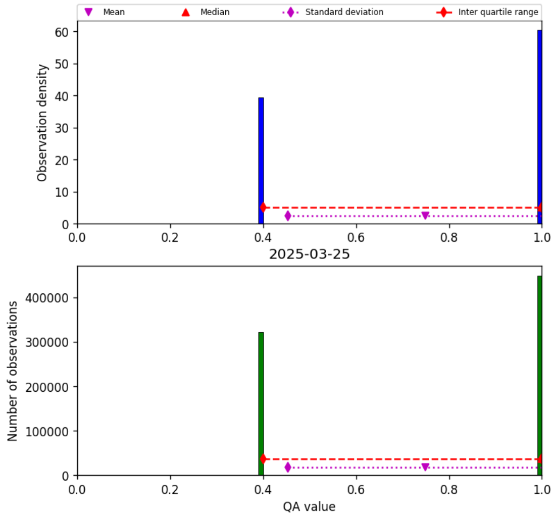
Figure 22: Histogram of “QA value” for 2025-03-24 to 2025-03-26
