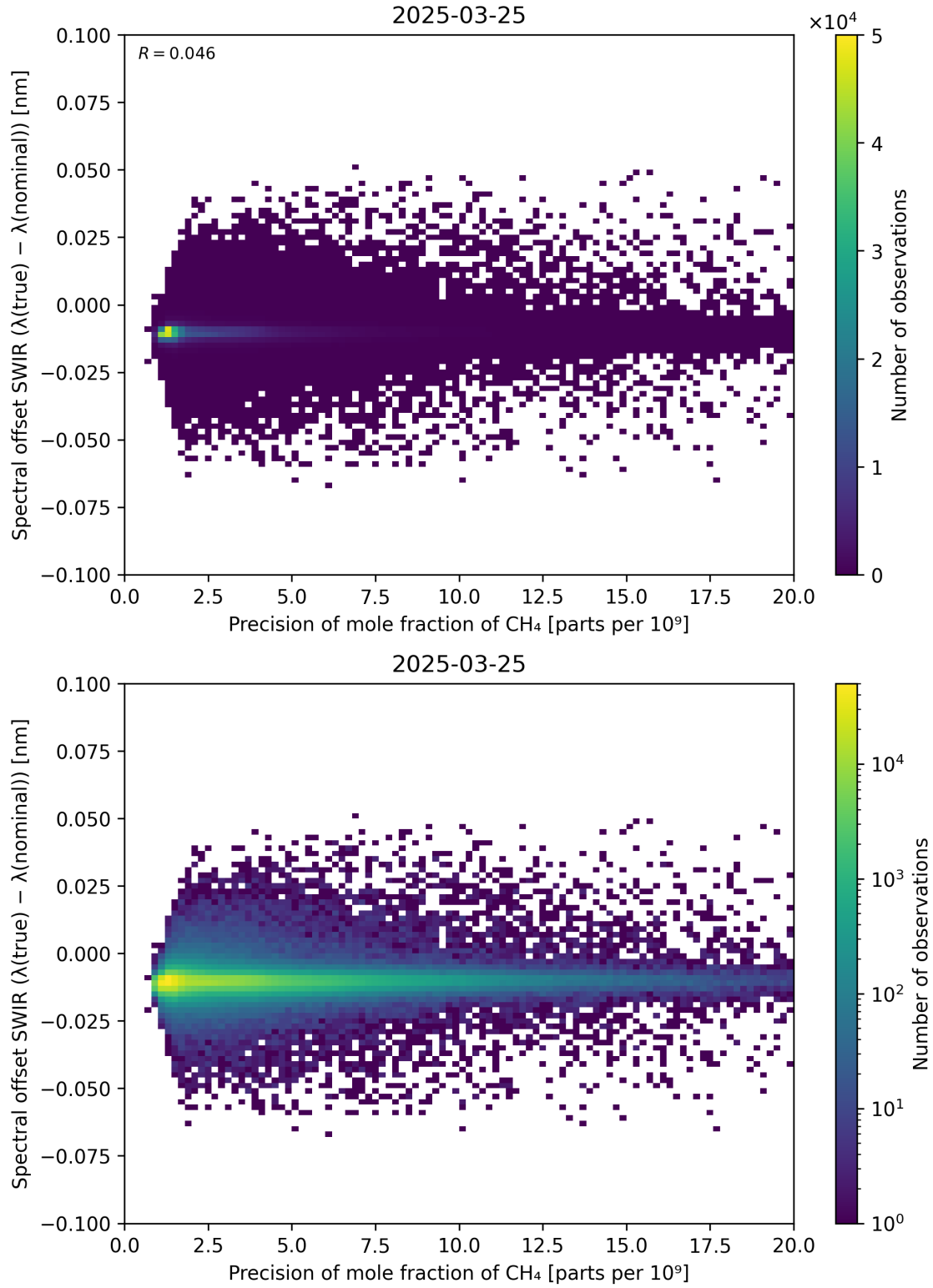
Figure 85: Scatter density plot of “Precision of mole fraction of CH 4 ” against “Spectral offset SWIR ( \lambda_{\text{true}} - \lambda_{\text{nominal}} )” for 2025-03-24 to 2025-03-26.
