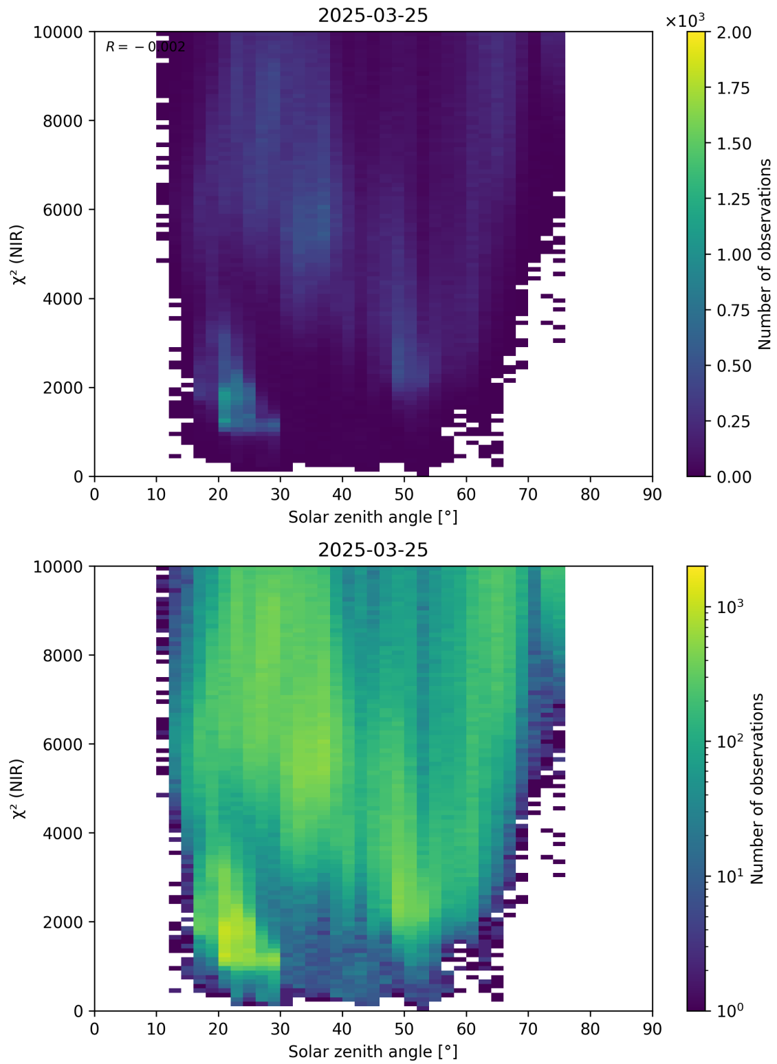
Figure 94: Scatter density plot of “Solar zenith angle” against “ \chi^2 (NIR)” for 2025-03-24 to 2025-03-26.
