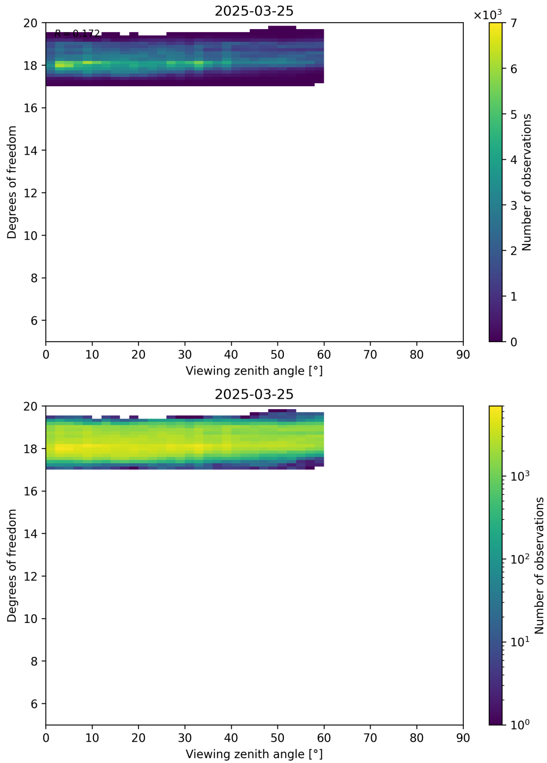
Figure 107: Scatter density plot of “Viewing zenith angle” against “Degrees of freedom” for 2025-03-24 to 2025-03-26.
