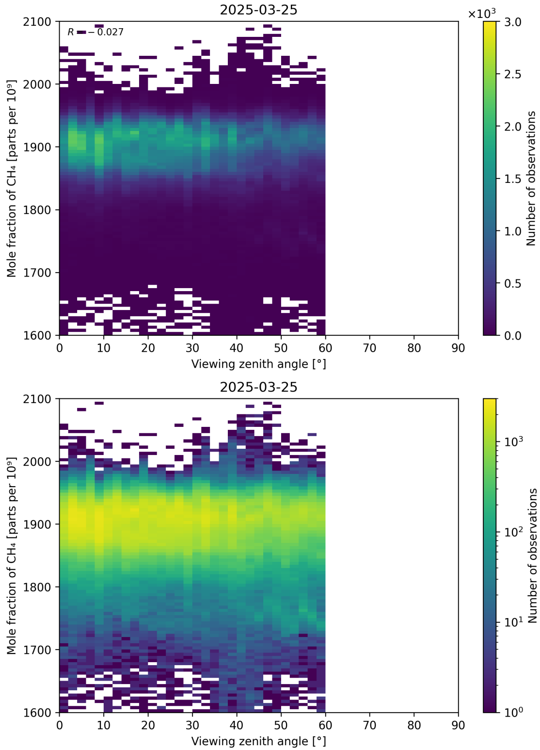
Figure 110: Scatter density plot of “Viewing zenith angle” against “Mole fraction of CH 4 ” for 2025-03-24 to 2025-03-26.
