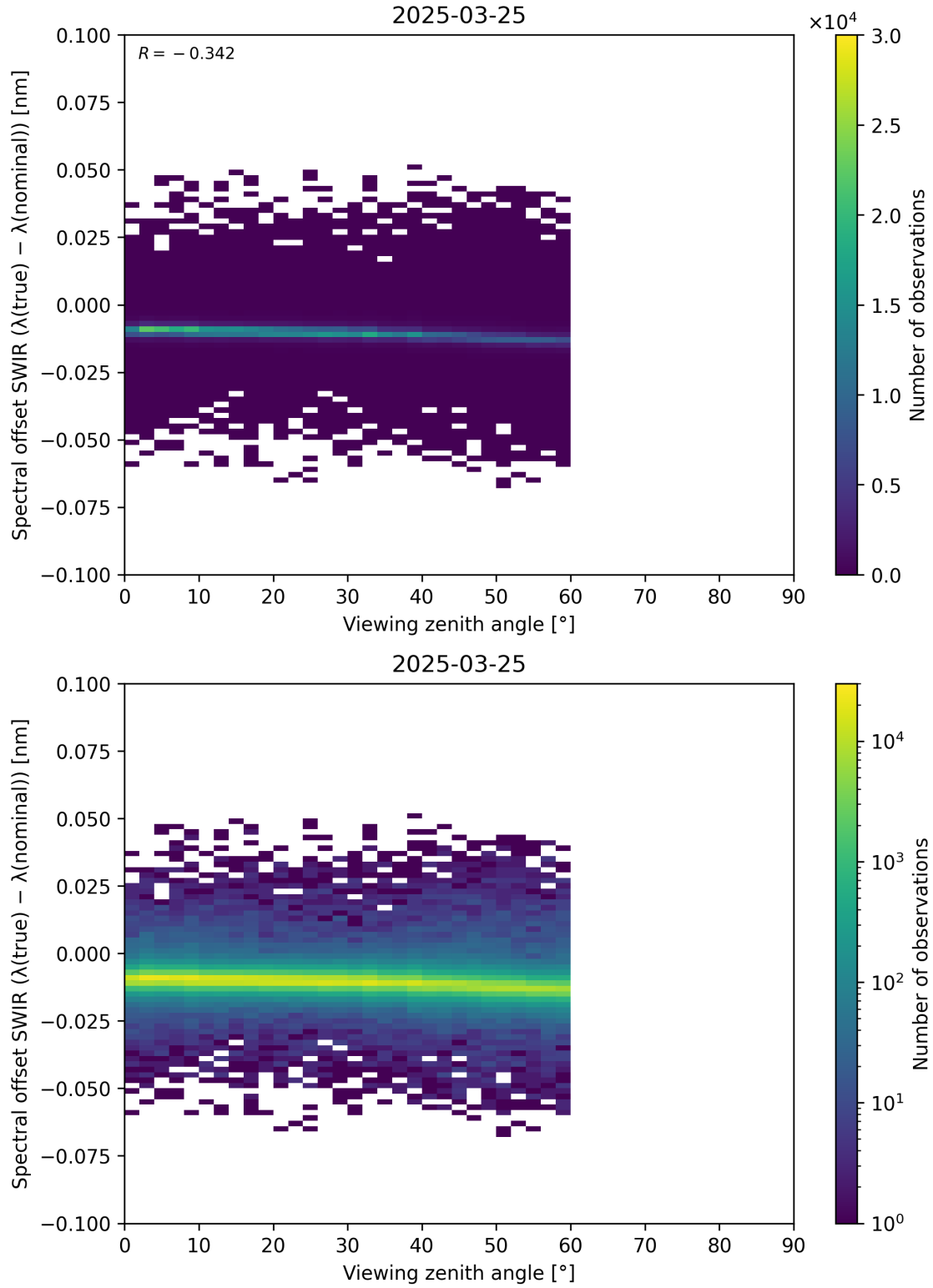
Figure 116: Scatter density plot of “Viewing zenith angle” against “Spectral offset SWIR ( \lambda_{\text{true}} - \lambda_{\text{nominal}} )” for 2025-03-24 to 2025-03-26.
