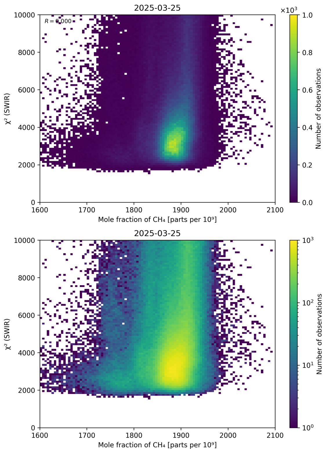
Figure 71: Scatter density plot of “Mole fraction of \text{CH}_4 ” against “ \chi^2 (SWIR)” for 2025-03-24 to 2025-03-26.
