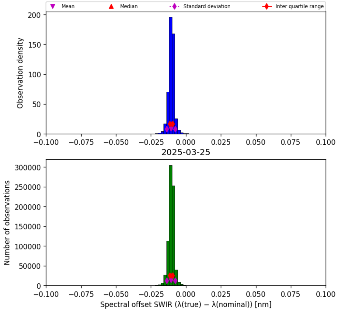
Figure 27: Histogram of “Spectral offset SWIR ( \lambda_{\text{true}} - \lambda_{\text{nominal}} )” for 2025-03-24 to 2025-03-26
