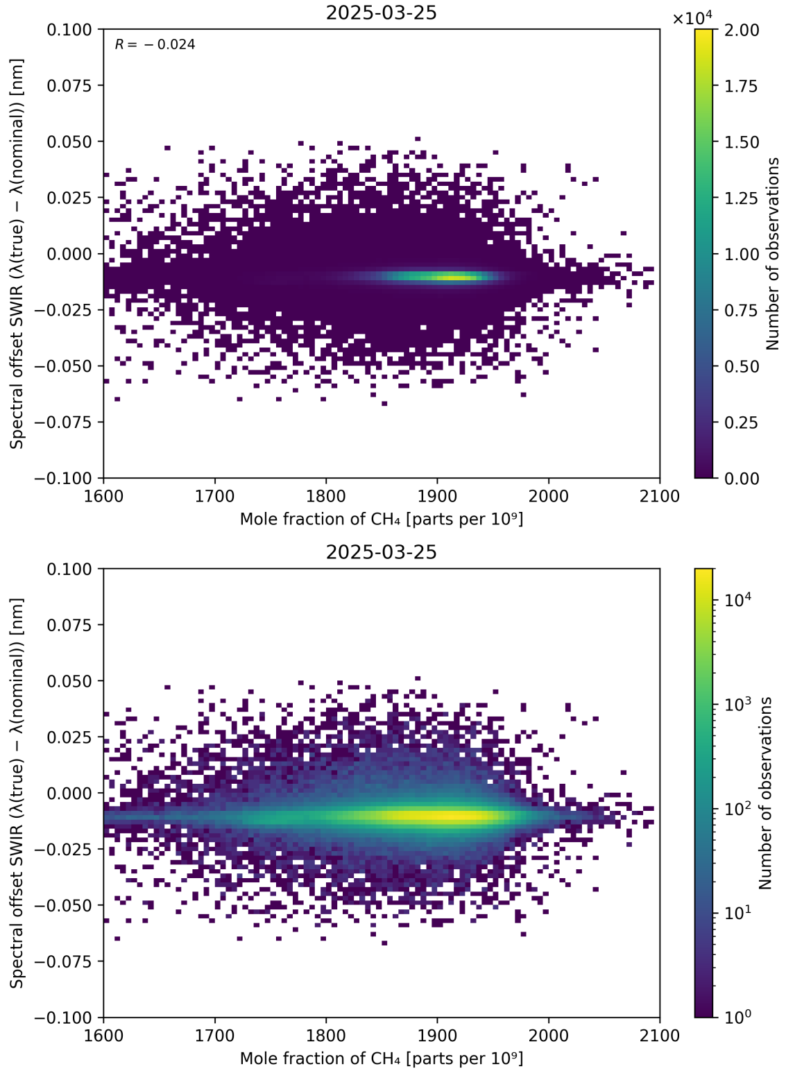
Figure 86: Scatter density plot of “Mole fraction of \text{CH}_4 ” against “Spectral offset SWIR ( \lambda_{\text{true}} - \lambda_{\text{nominal}} )” for 2025-03-24 to 2025-03-26.
