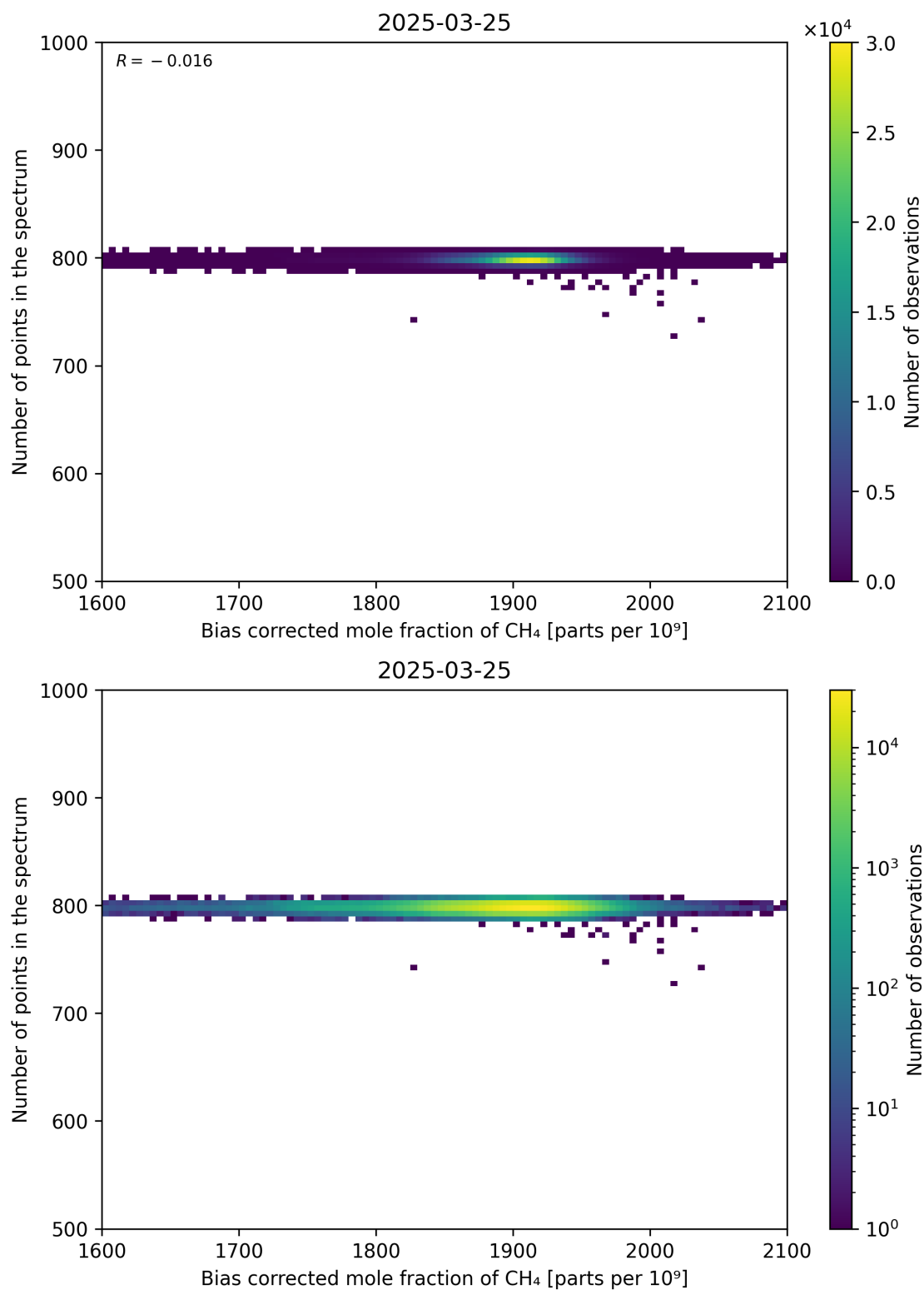
Figure 68: Scatter density plot of “Bias corrected mole fraction of CH 4 ” against “Number of points in the spectrum” for 2025-03-24 to 2025-03-26.
