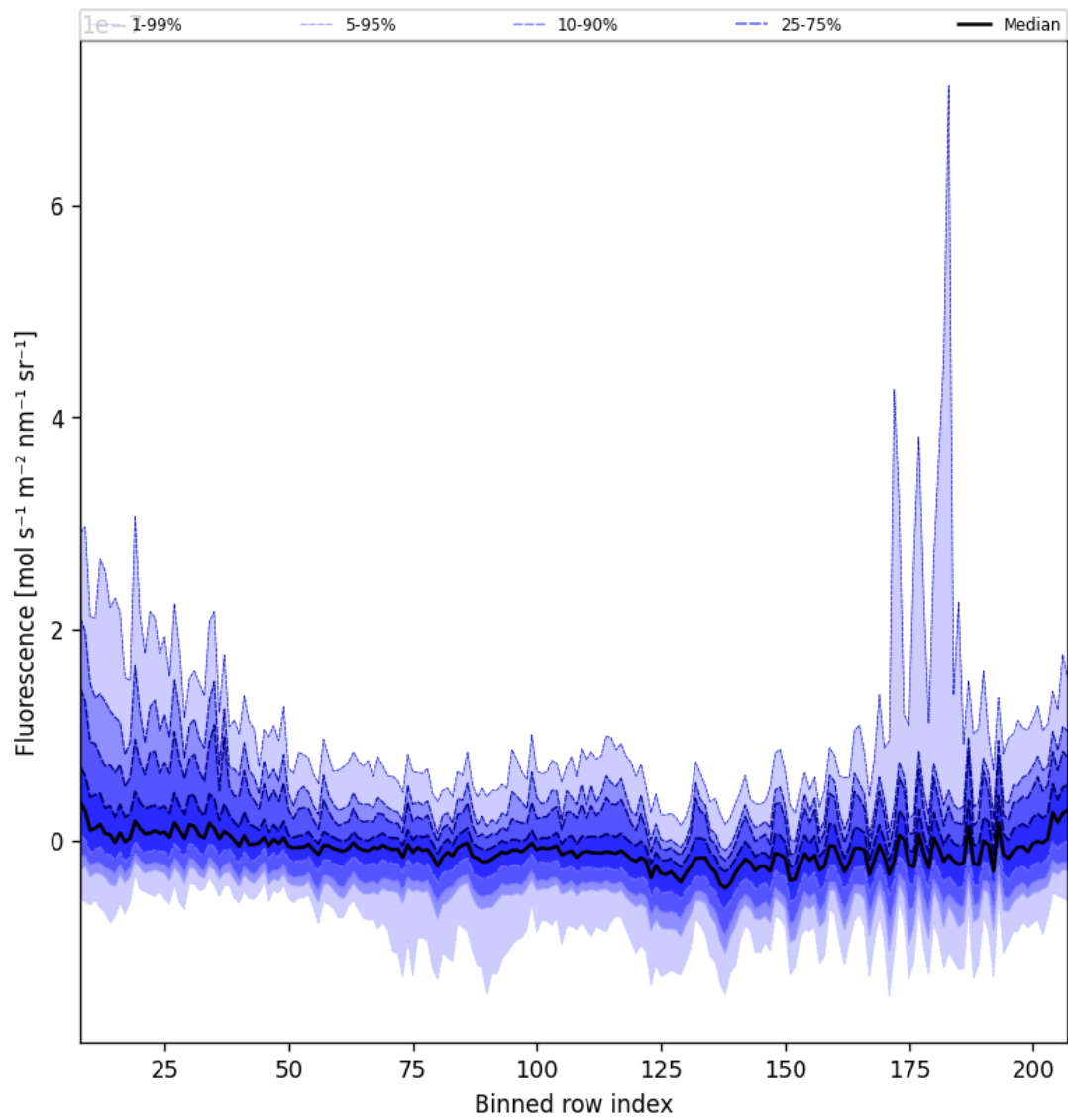
Figure 43: Along track statistics of “Fluorescence” for 2025-03-24 to 2025-03-26
