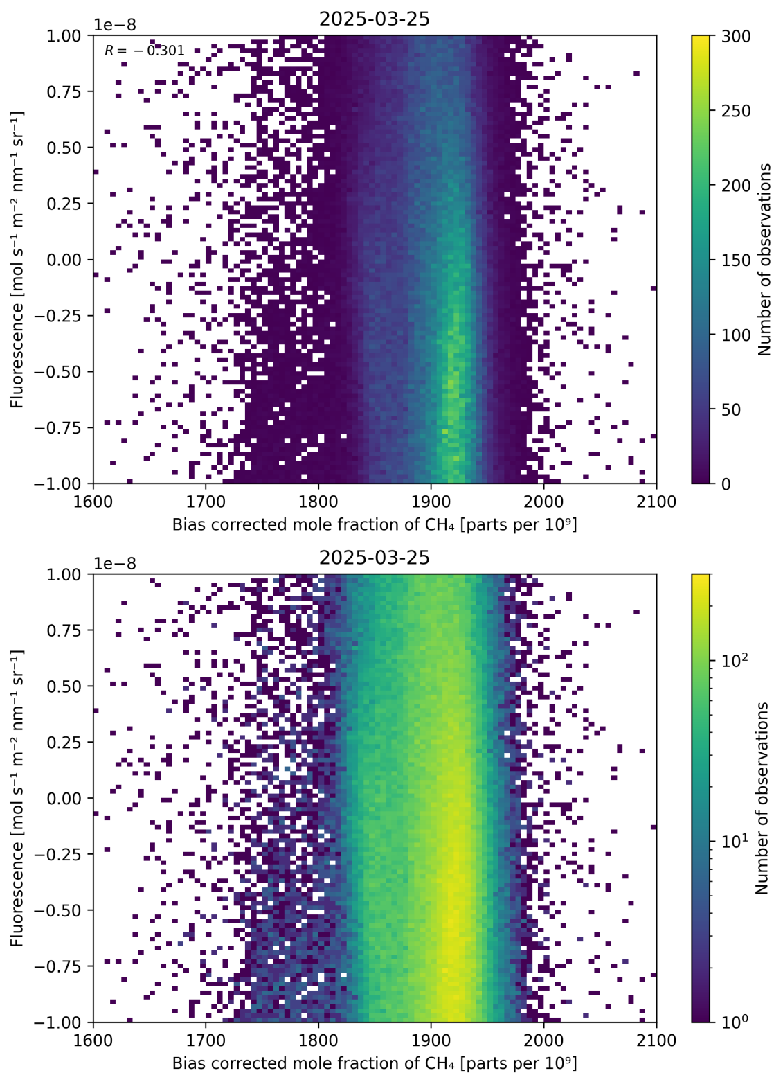
Figure 66: Scatter density plot of “Bias corrected mole fraction of \text{CH}_4 ” against “Fluorescence” for 2025-03-24 to 2025-03-26.
