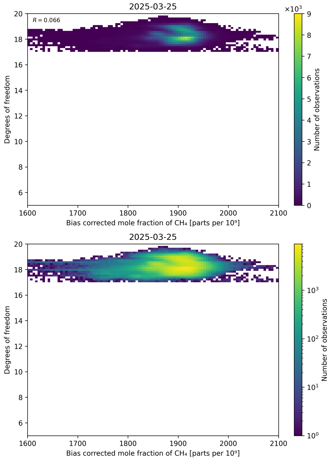
Figure 65: Scatter density plot of “Bias corrected mole fraction of CH 4 ” against “Degrees of freedom” for 2025-03-24 to 2025-03-26.
