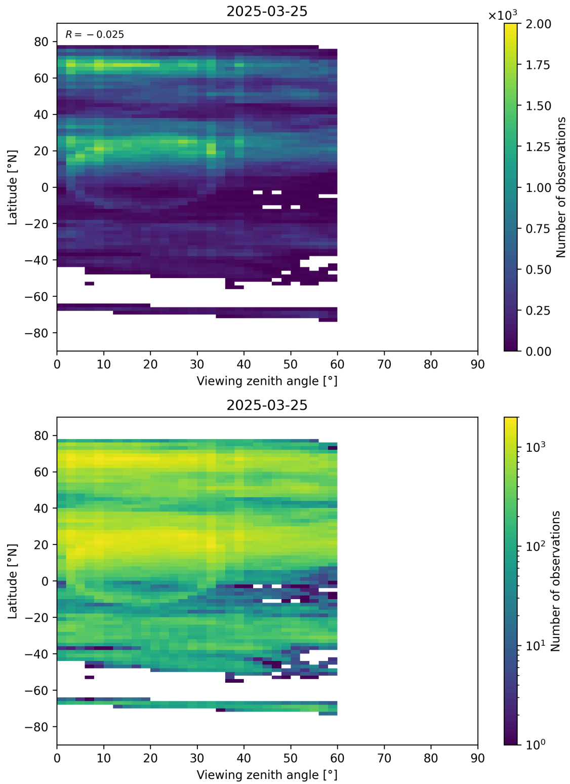
Figure 109: Scatter density plot of “Viewing zenith angle” against “Latitude” for 2025-03-24 to 2025-03-26.
