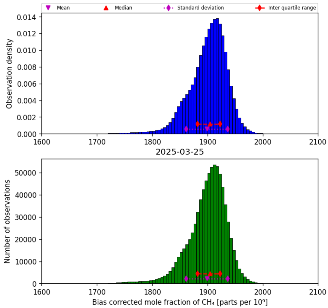
Figure 25: Histogram of “Bias corrected mole fraction of CH 4 ” for 2025-03-24 to 2025-03-26
