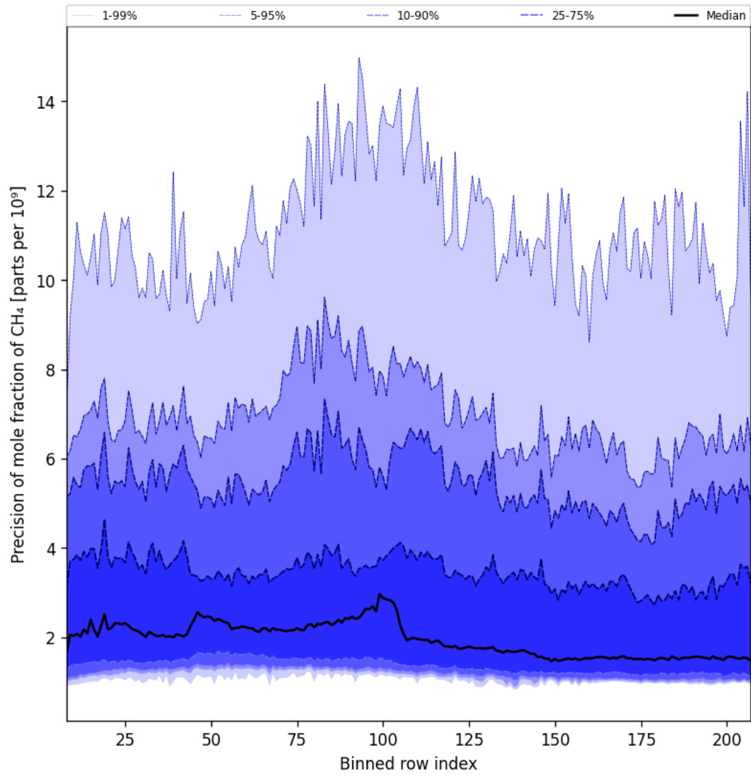
Figure 35: Along track statistics of “Precision of mole fraction of CH 4 ” for 2025-03-24 to 2025-03-26
