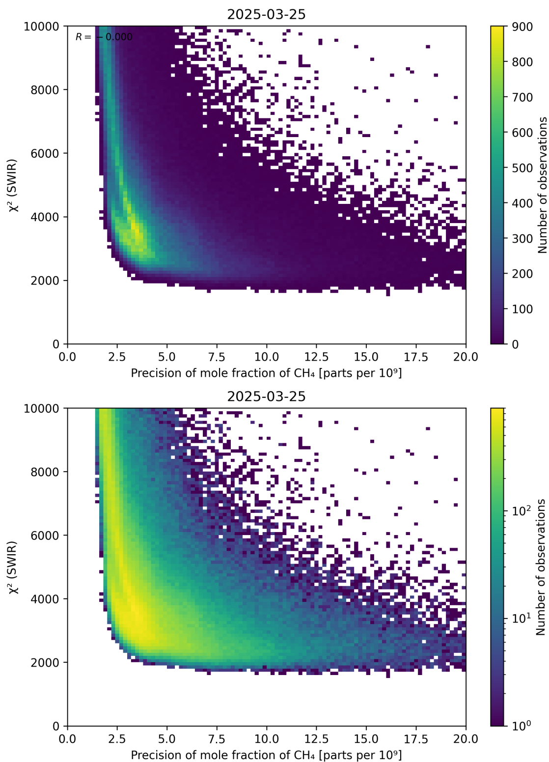
Figure 79: Scatter density plot of “Precision of mole fraction of \text{CH}_4 ” against “ \chi^2 (SWIR)” for 2025-03-24 to 2025-03-26.
