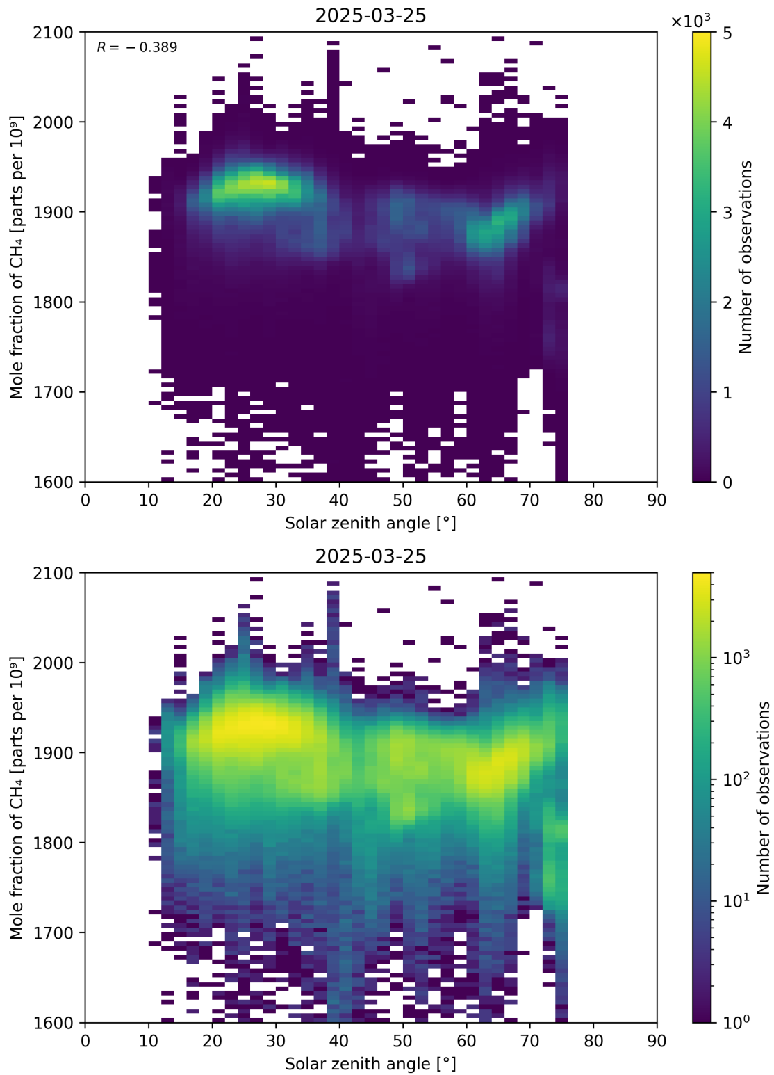
Figure 99: Scatter density plot of “Solar zenith angle” against “Mole fraction of CH 4 ” for 2025-03-24 to 2025-03-26.
