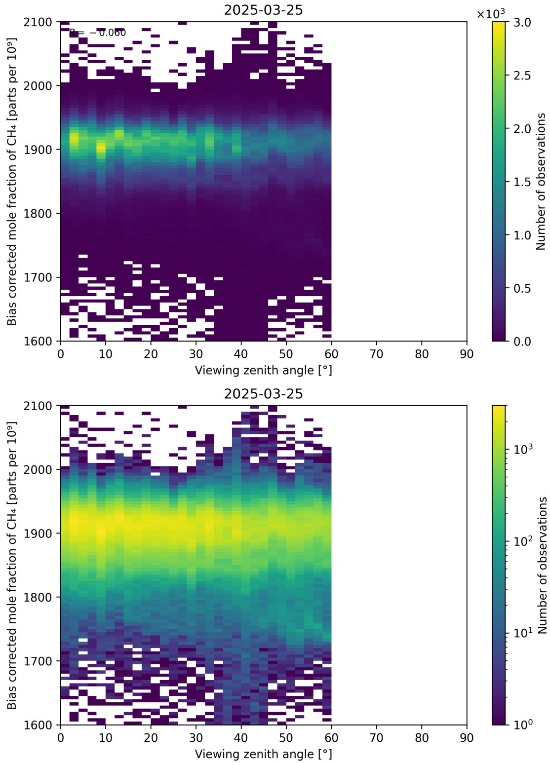
Figure 111: Scatter density plot of “Viewing zenith angle” against “Bias corrected mole fraction of CH 4 ” for 2025-03-24 to 2025-03-26.
