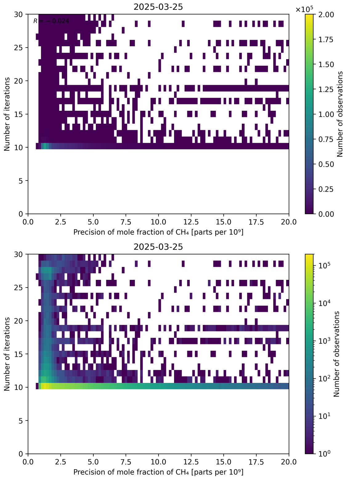
Figure 83: Scatter density plot of “Precision of mole fraction of CH 4 ” against “Number of iterations” for 2025-03-24 to 2025-03-26.
