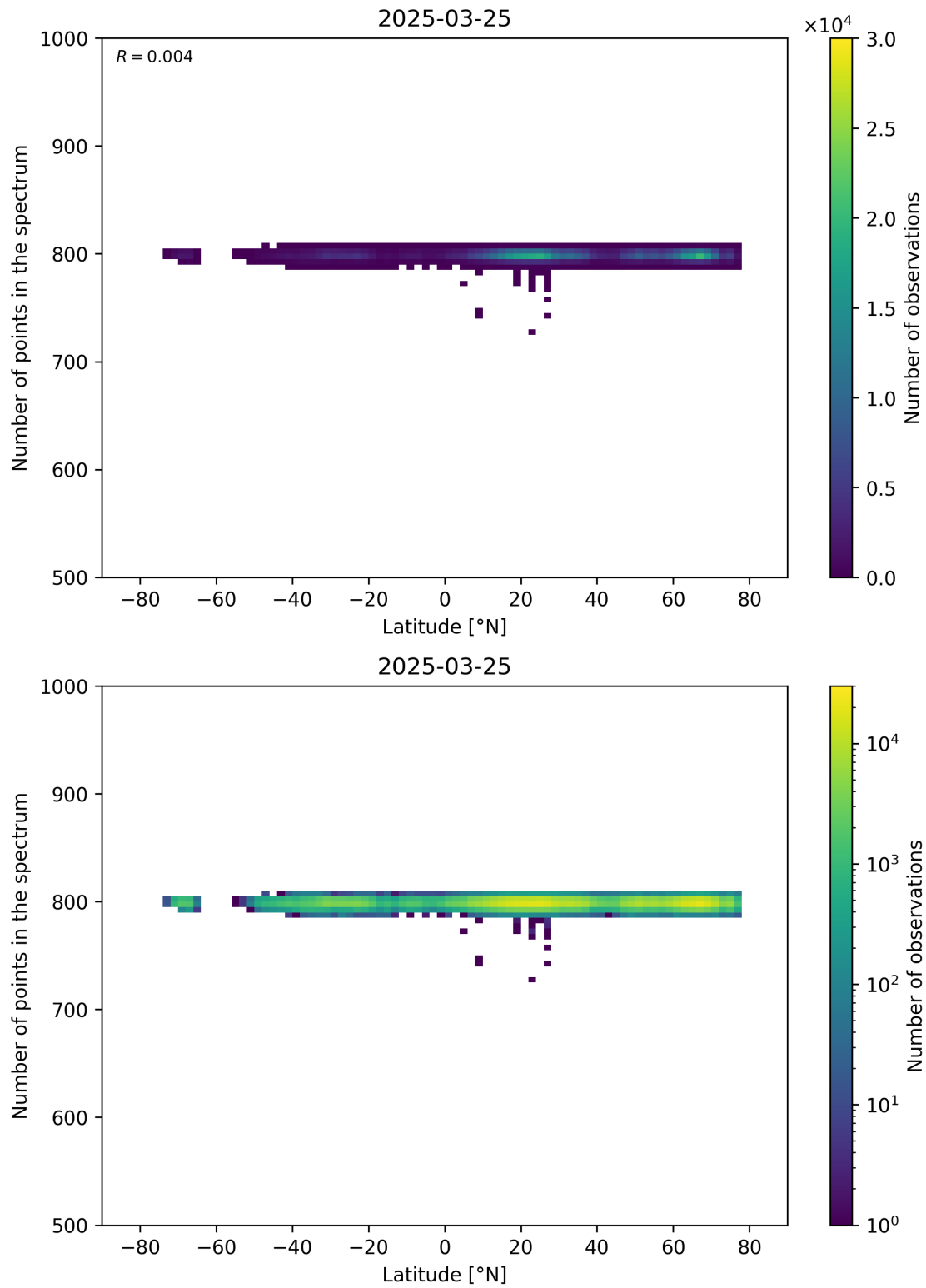
Figure 61: Scatter density plot of “Latitude” against “Number of points in the spectrum” for 2025-03-24 to 2025-03-26.
