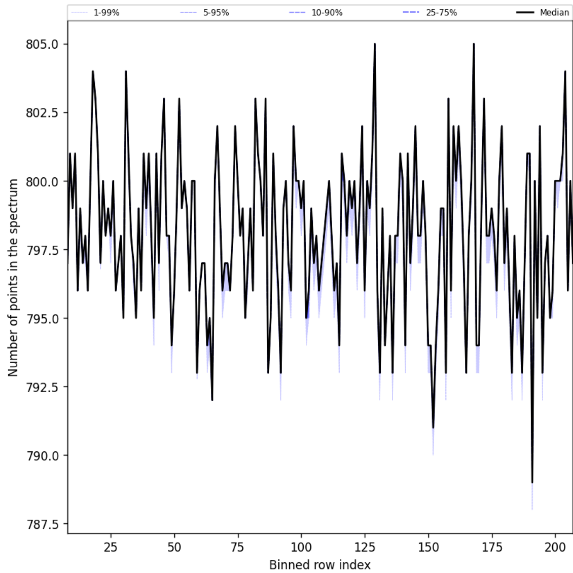
Figure 37: Along track statistics of “Number of points in the spectrum” for 2025-03-24 to 2025-03-26
