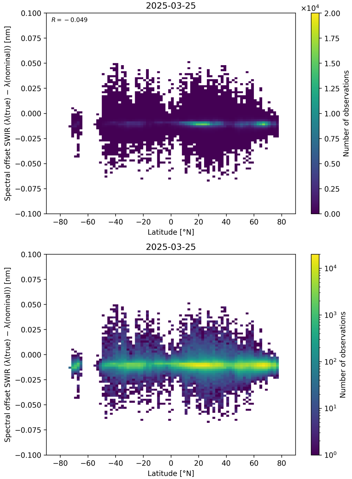
Figure 62: Scatter density plot of “Latitude” against “Spectral offset SWIR ( \lambda_{\text{true}} - \lambda_{\text{nominal}} )” for 2025-03-24 to 2025-03-26.
