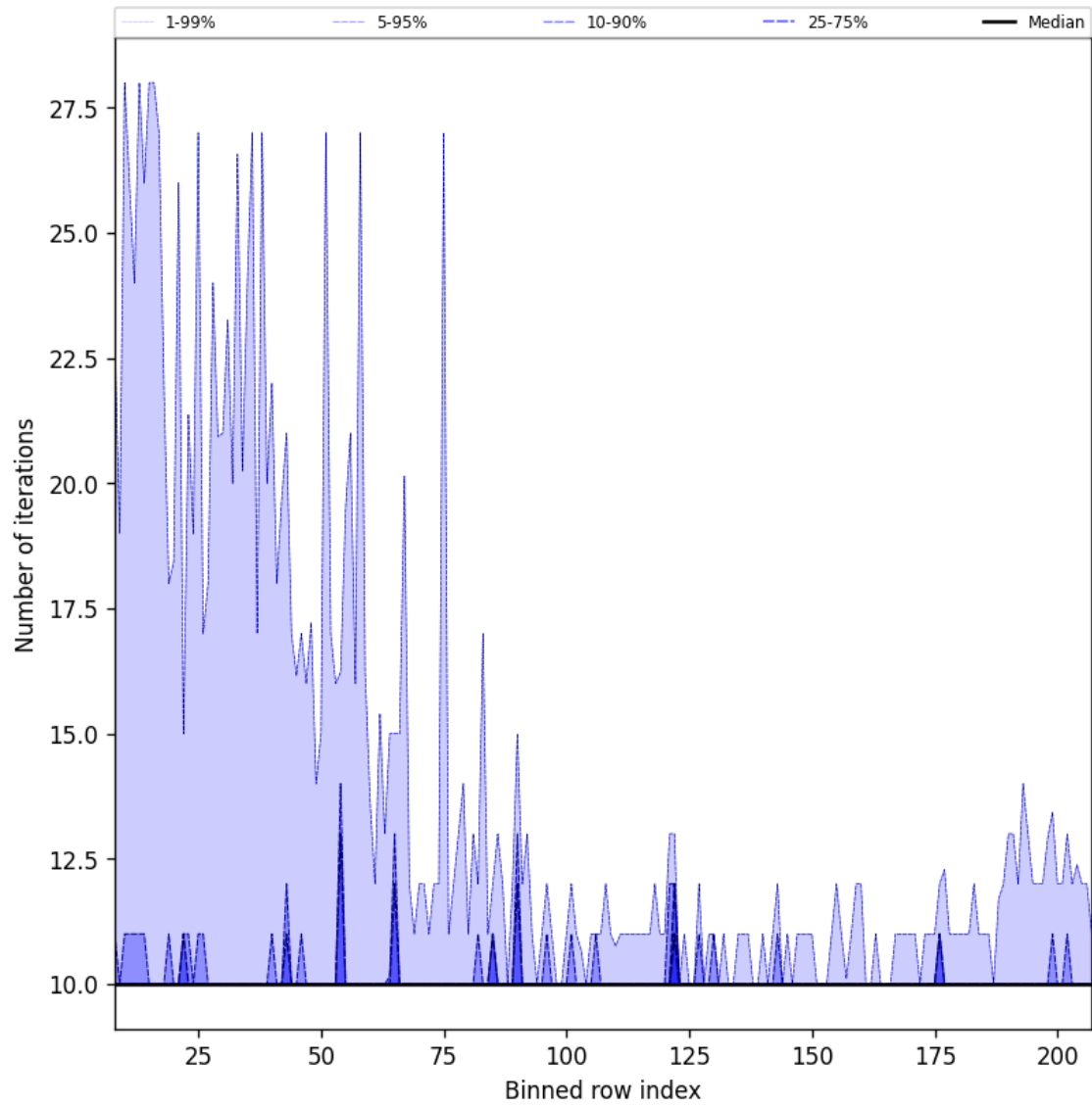
Figure 42: Along track statistics of “Number of iterations” for 2025-03-24 to 2025-03-26
