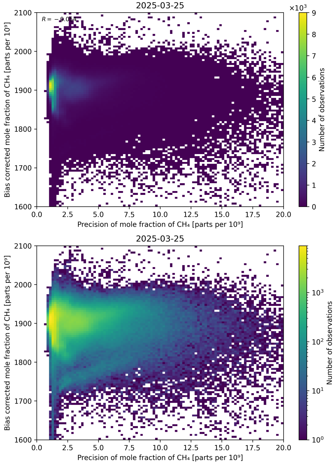
Figure 82: Scatter density plot of “Precision of mole fraction of CH 4 ” against “Bias corrected mole fraction of CH 4 ” for 2025-03-24 to 2025-03-26.
