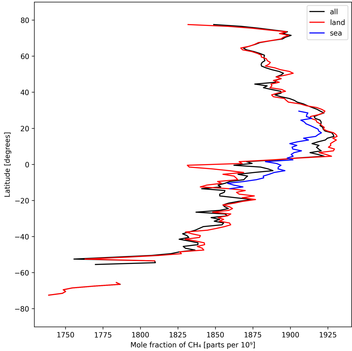
Figure 12: Zonal average of “Mole fraction of CH 4 ” for 2025-03-24 to 2025-03-26.
