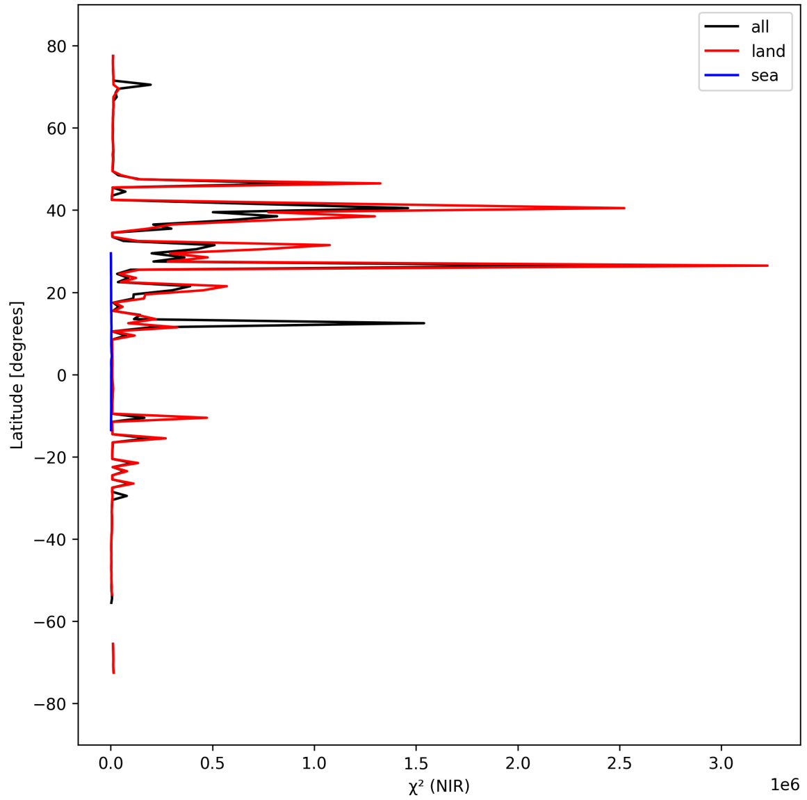
Figure 18: Zonal average of “ \chi^2 (NIR)” for 2025-03-24 to 2025-03-26.
