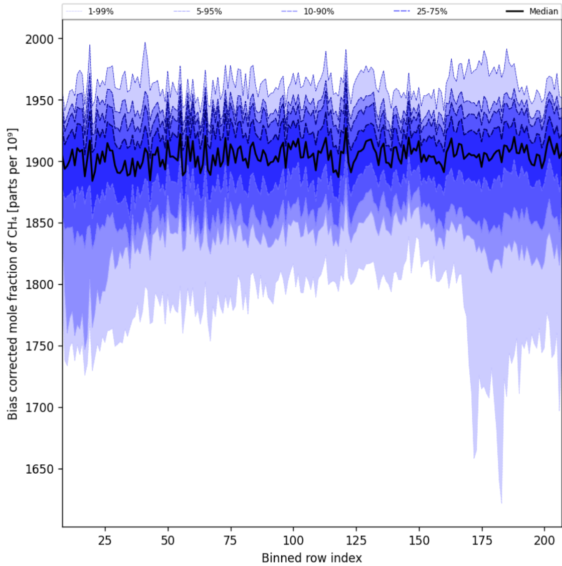
Figure 36: Along track statistics of “Bias corrected mole fraction of CH 4 ” for 2025-03-24 to 2025-03-26
