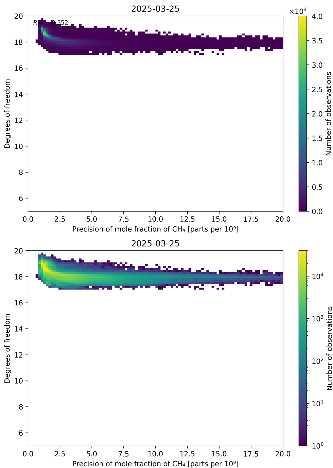
Figure 80: Scatter density plot of “Precision of mole fraction of CH 4 ” against “Degrees of freedom” for 2025-03-24 to 2025-03-26.
