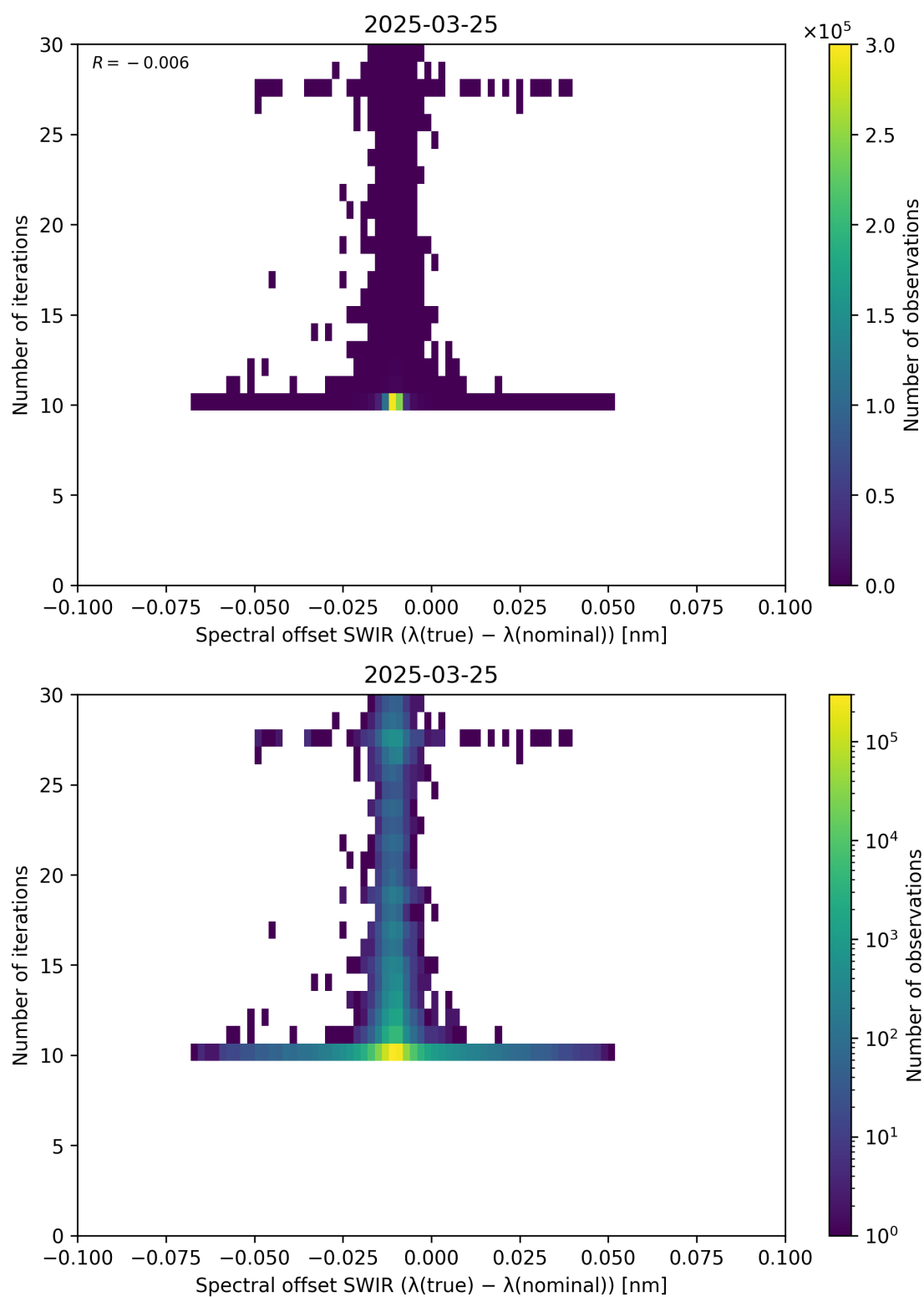
Figure 121: Scatter density plot of “Spectral offset SWIR ( \lambda_{\text{true}} - \lambda_{\text{nominal}} )” against “Number of iterations” for 2025-03-24 to 2025-03-26.
