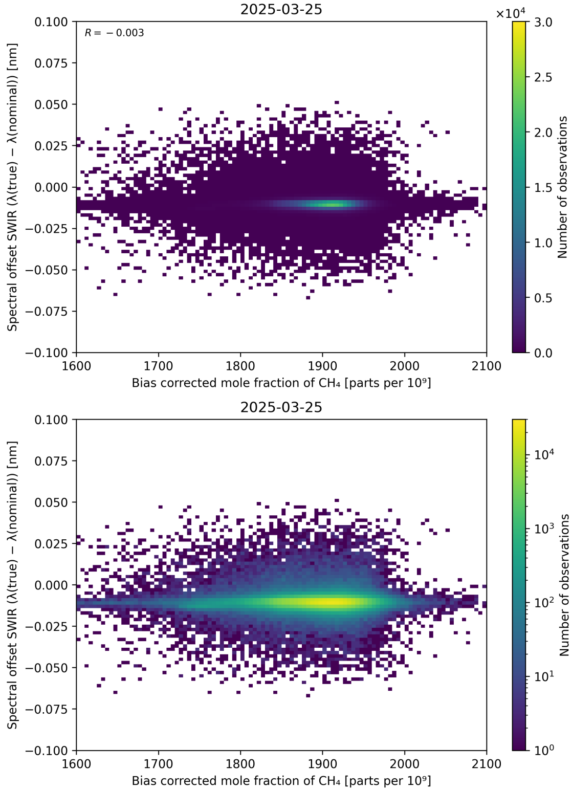
Figure 69: Scatter density plot of “Bias corrected mole fraction of \text{CH}_4 ” against “Spectral offset SWIR ( \lambda_{\text{true}} - \lambda_{\text{nominal}} )” for 2025-03-24 to 2025-03-26.
