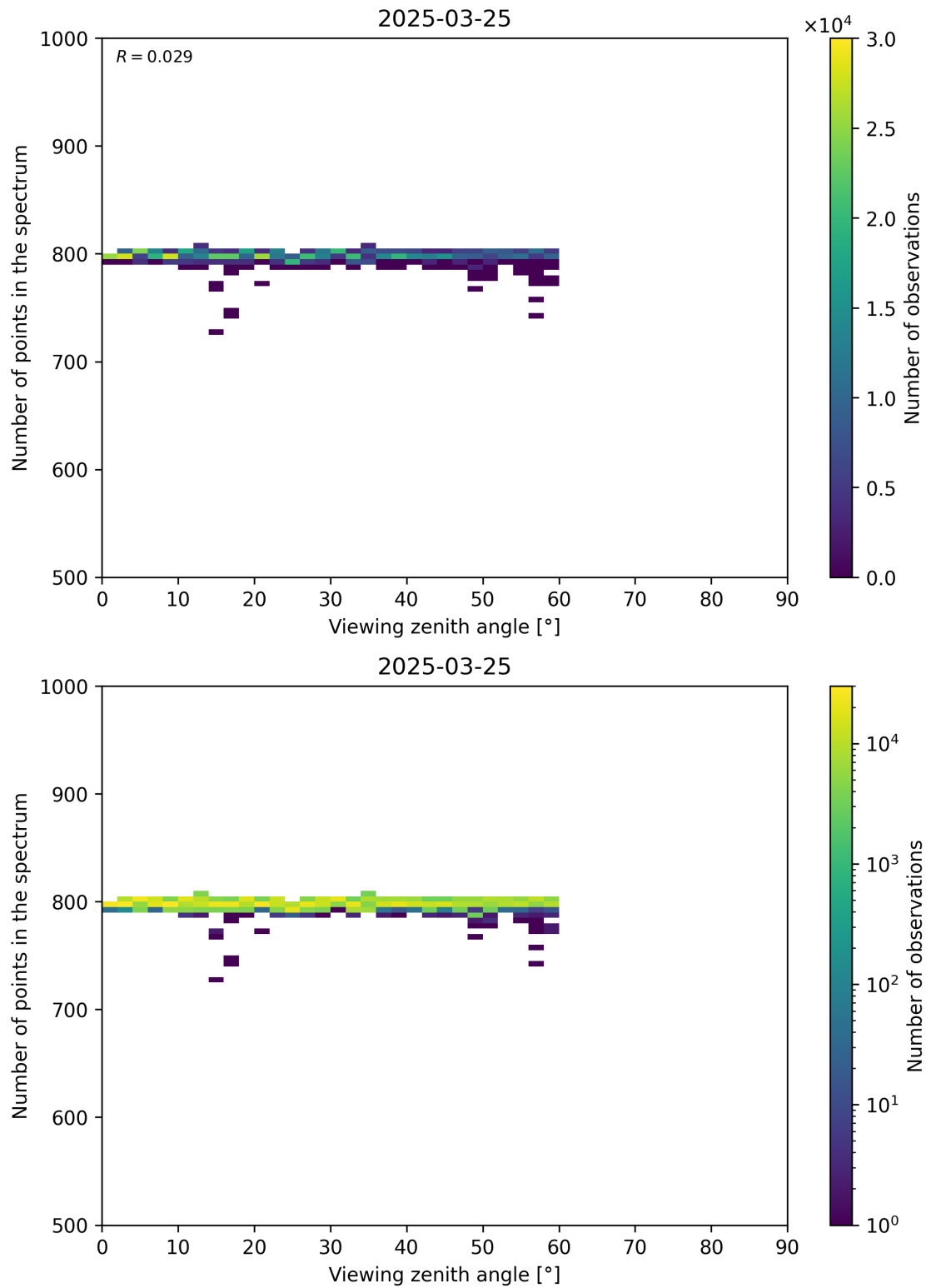
Figure 114: Scatter density plot of “Viewing zenith angle” against “Number of points in the spectrum” for 2025-03-24 to 2025-03-26.
