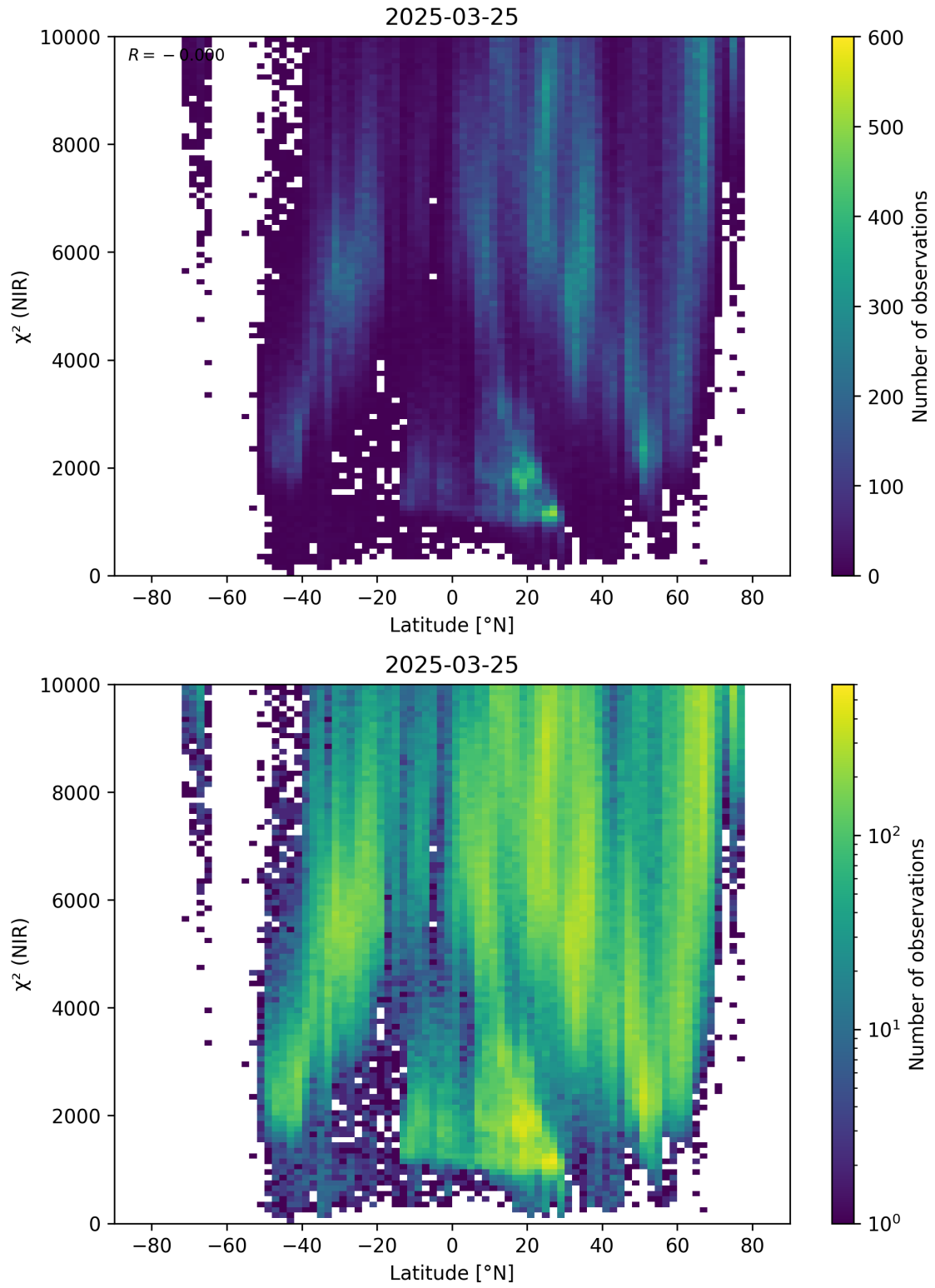
Figure 53: Scatter density plot of “Latitude” against “ \chi^2 (NIR)” for 2025-03-24 to 2025-03-26.
