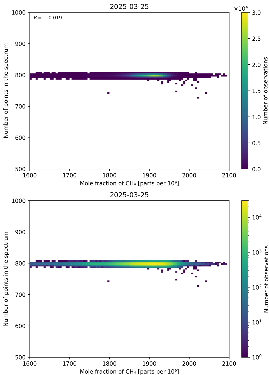
Figure 77: Scatter density plot of “Mole fraction of CH 4 ” against “Number of points in the spectrum” for 2025-03-24 to 2025-03-26.
