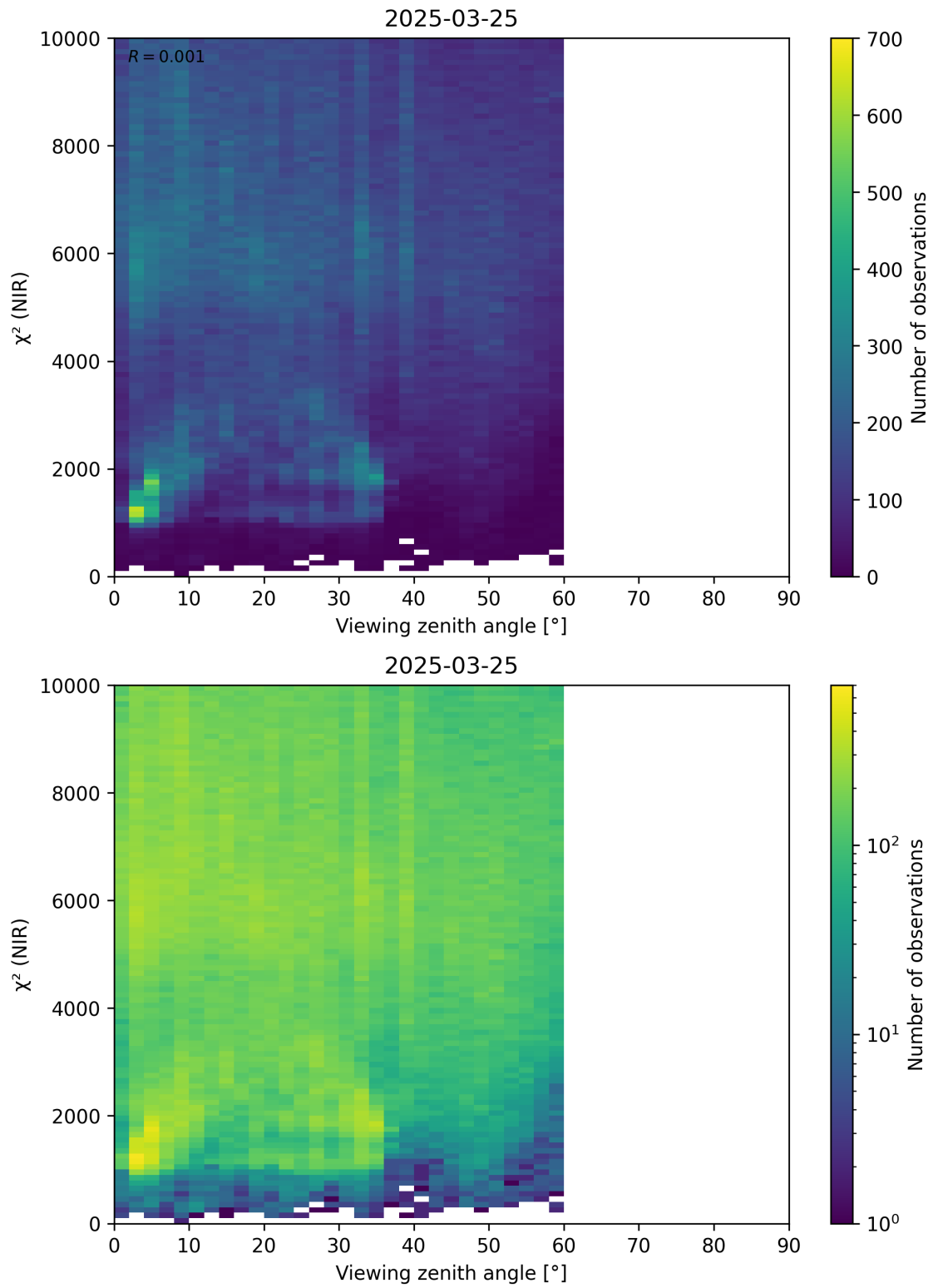
Figure 105: Scatter density plot of “Viewing zenith angle” against “ \chi^2 (NIR)” for 2025-03-24 to 2025-03-26.
