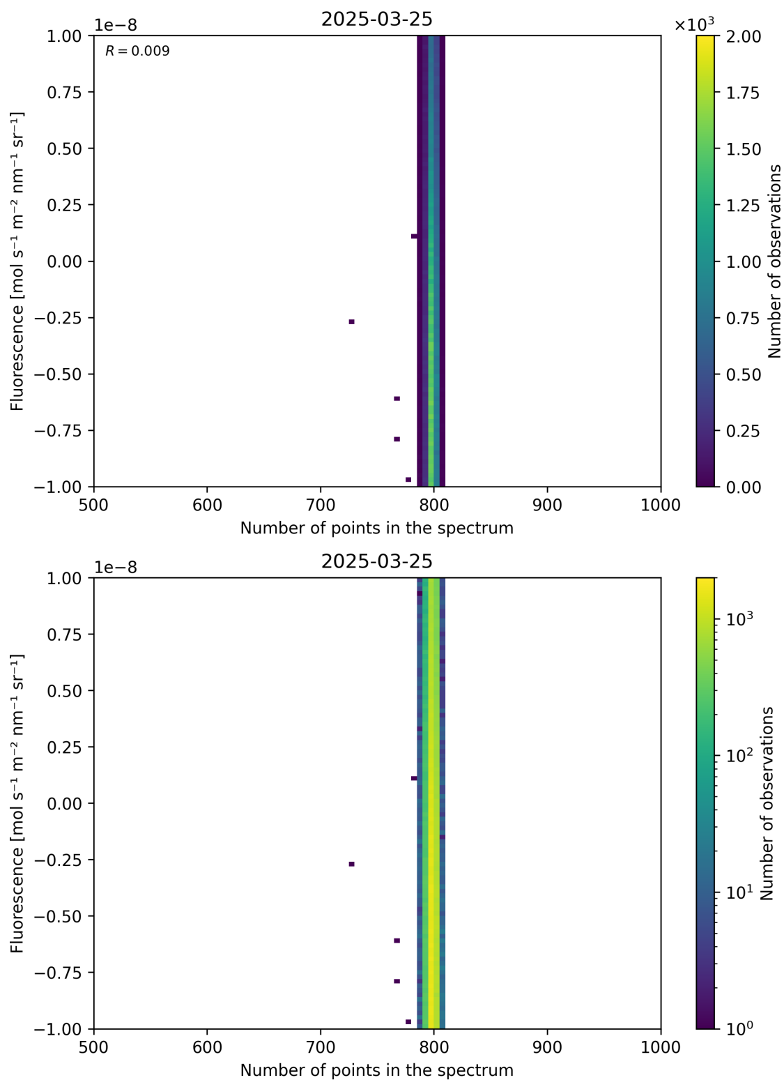
Figure 91: Scatter density plot of “Number of points in the spectrum” against “Fluorescence” for 2025-03-24 to 2025-03-26.
