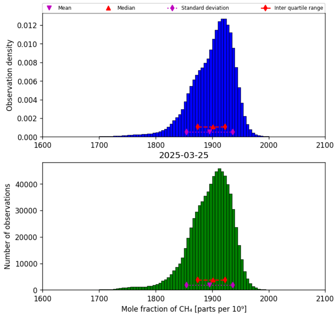
Figure 23: Histogram of “Mole fraction of CH 4 ” for 2025-03-24 to 2025-03-26
