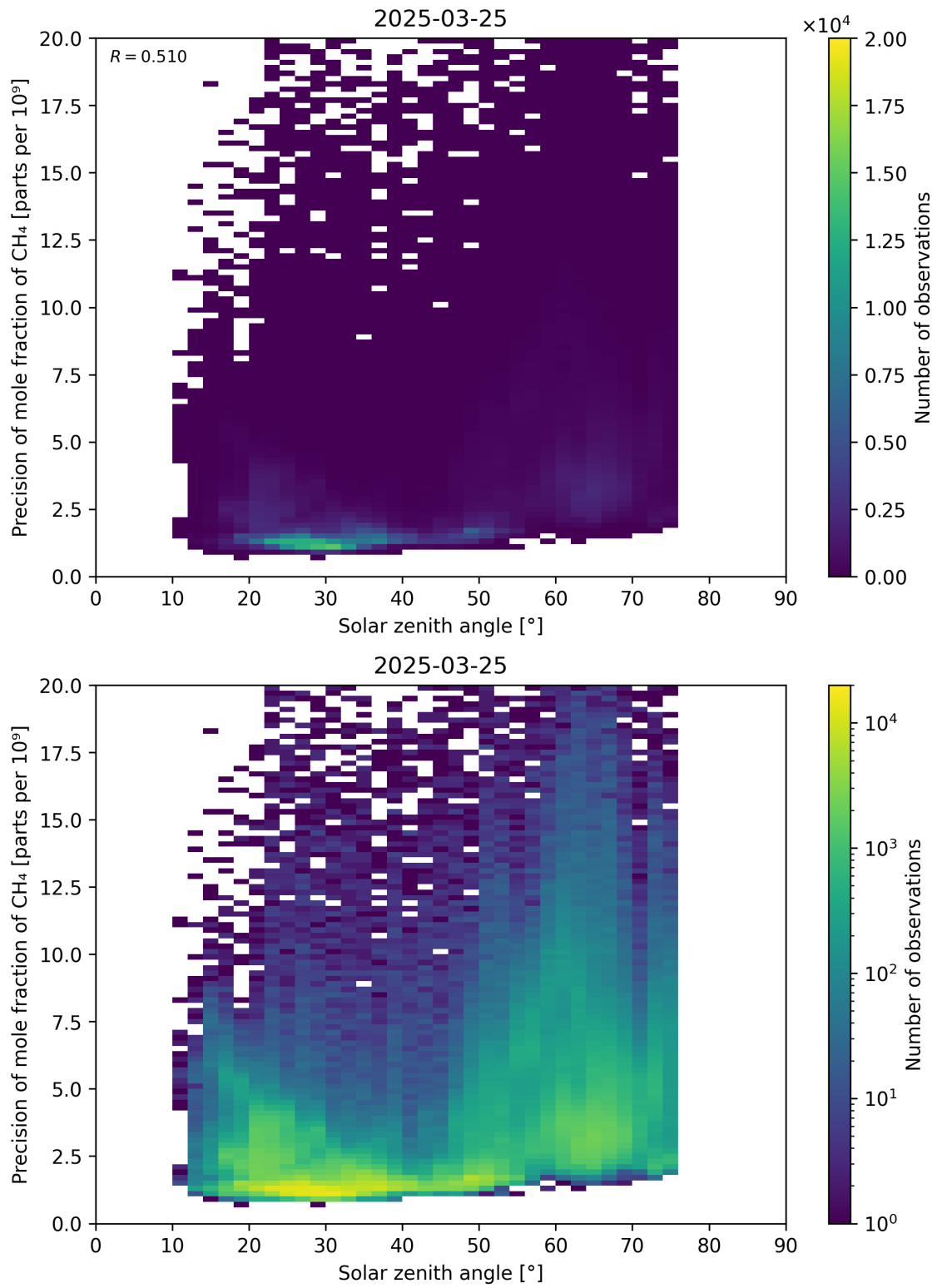
Figure 101: Scatter density plot of “Solar zenith angle” against “Precision of mole fraction of CH 4 ” for 2025-03-24 to 2025-03-26.
