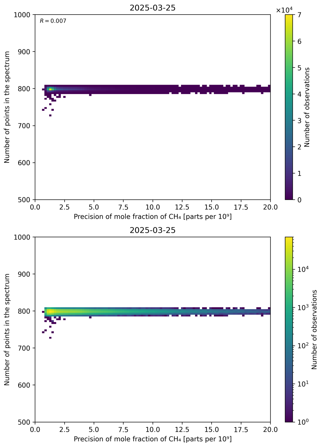
Figure 84: Scatter density plot of “Precision of mole fraction of CH 4 ” against “Number of points in the spectrum” for 2025-03-24 to 2025-03-26.
