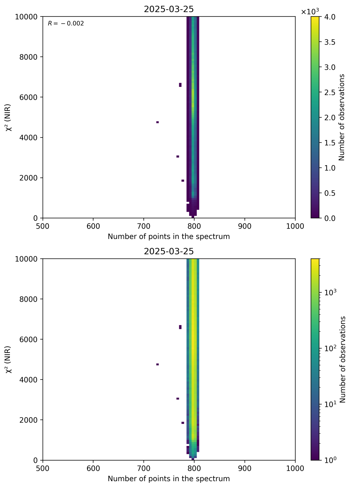
Figure 88: Scatter density plot of “Number of points in the spectrum” against “ \chi^2 (NIR)” for 2025-03-24 to 2025-03-26.
