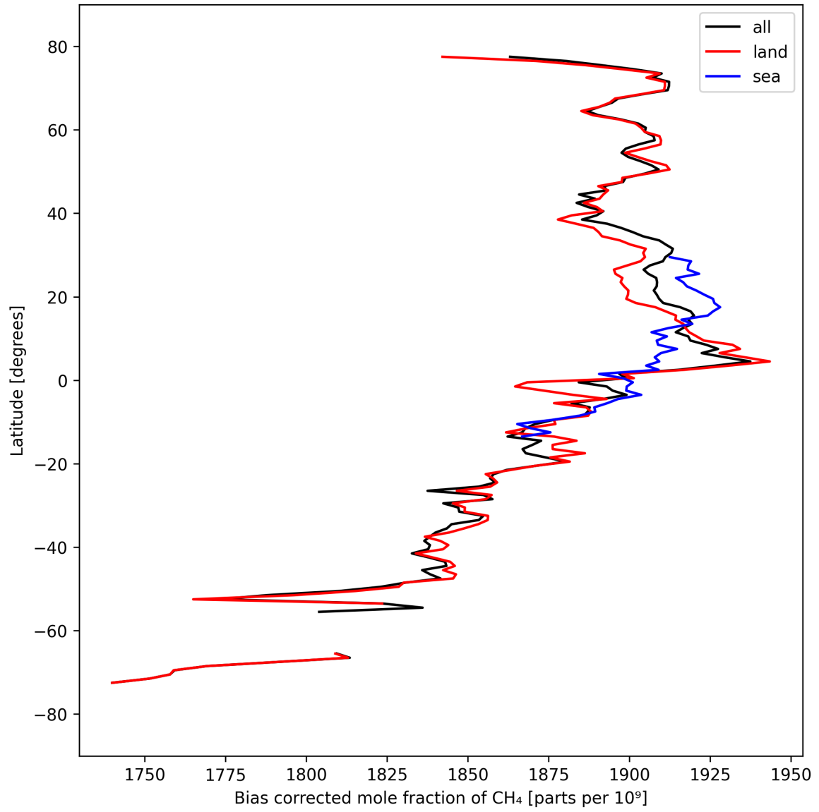
Figure 14: Zonal average of “Bias corrected mole fraction of CH 4 ” for 2025-03-24 to 2025-03-26.
