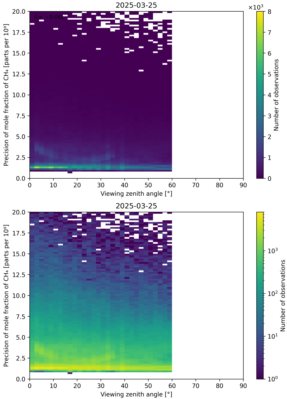
Figure 112: Scatter density plot of “Viewing zenith angle” against “Precision of mole fraction of CH 4 ” for 2025-03-24 to 2025-03-26.
