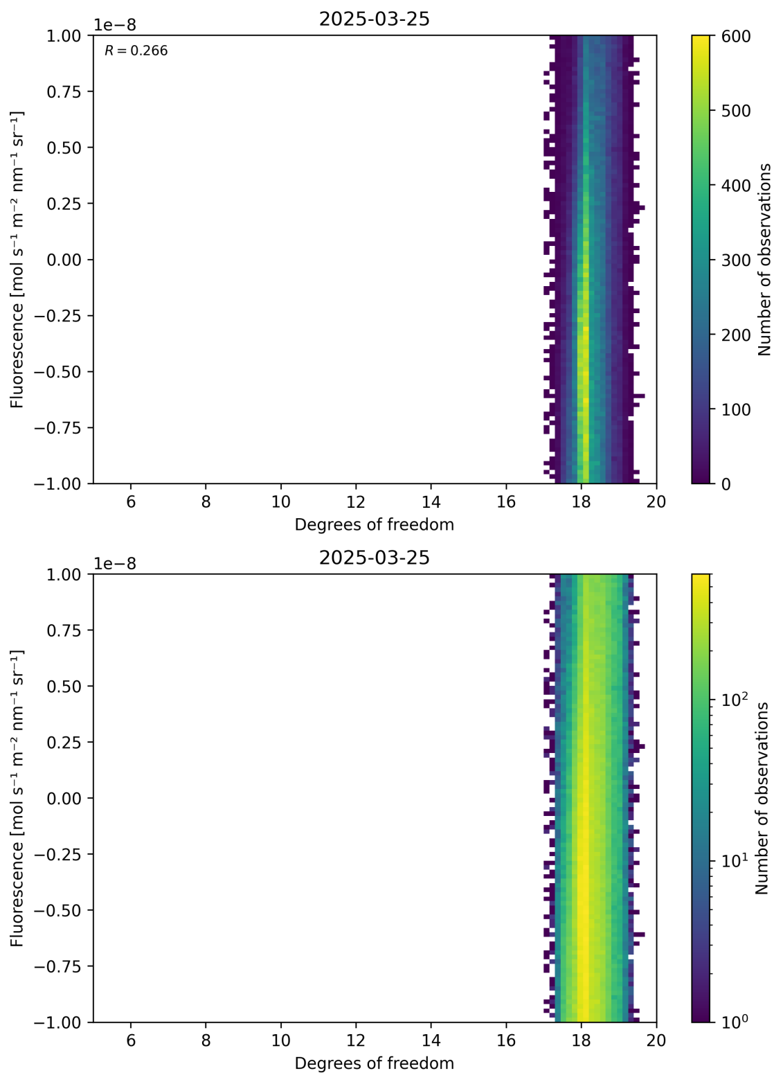
Figure 51: Scatter density plot of “Degrees of freedom” against “Fluorescence” for 2025-03-24 to 2025-03-26.
