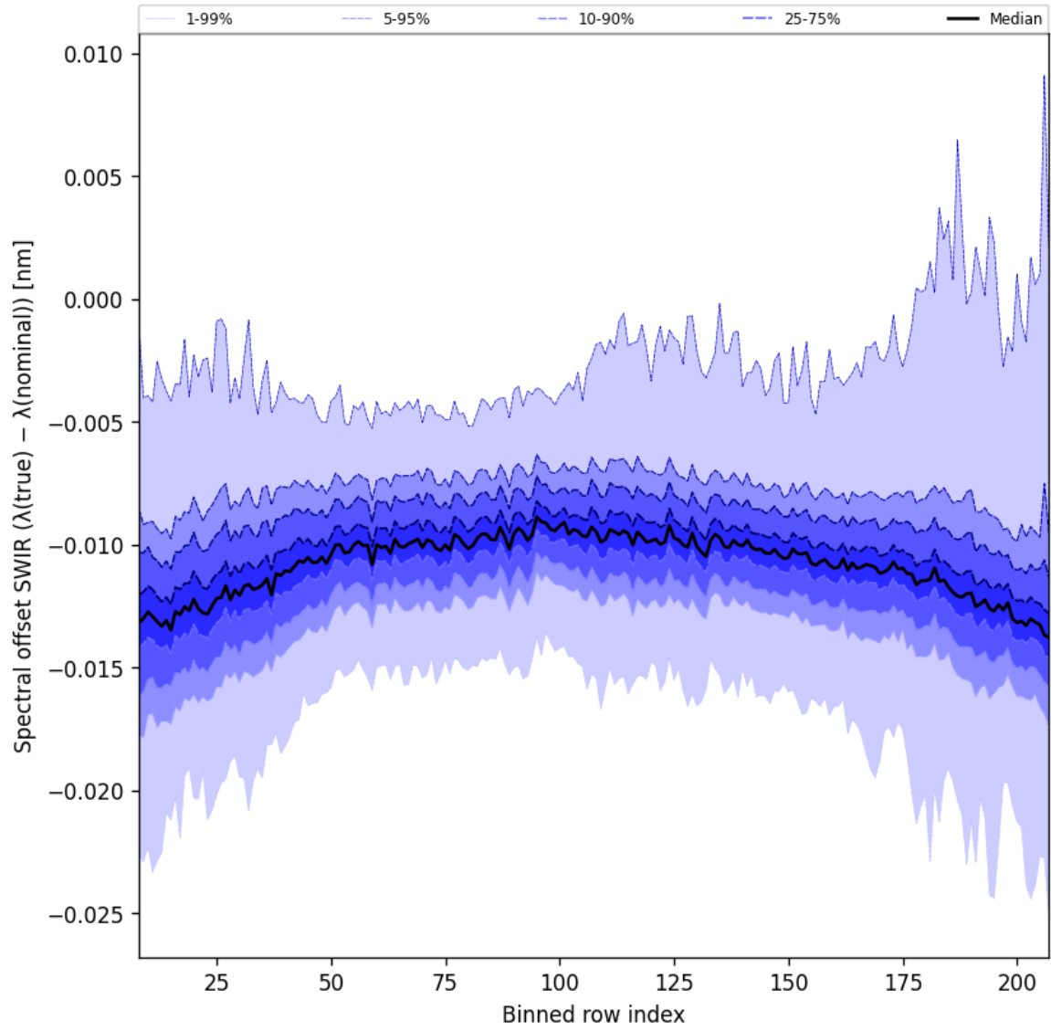
Figure 38: Along track statistics of “Spectral offset SWIR ( \lambda_{\text{true}} - \lambda_{\text{nominal}} )” for 2025-03-24 to 2025-03-26
