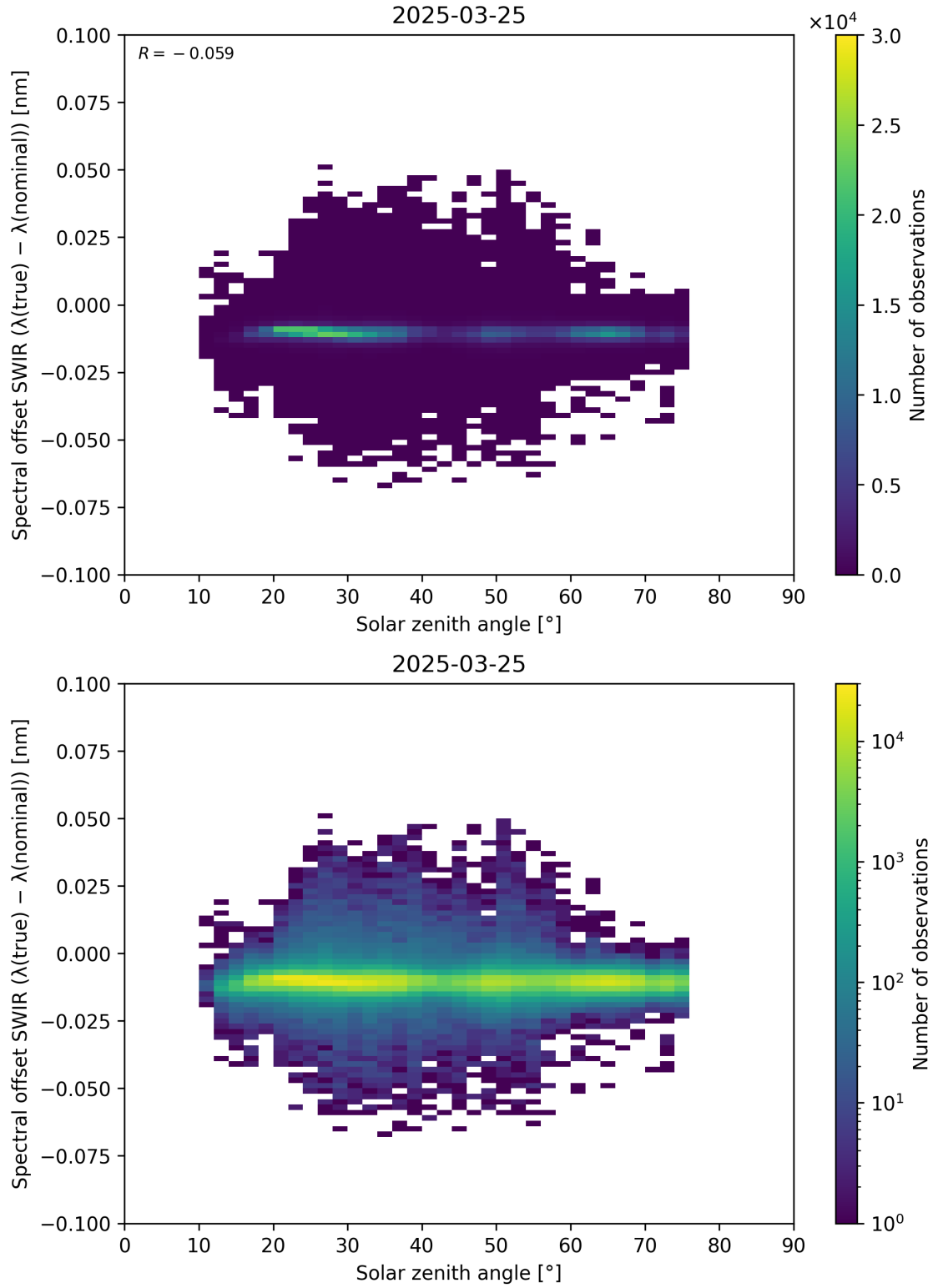
Figure 104: Scatter density plot of “Solar zenith angle” against “Spectral offset SWIR ( \lambda_{\text{true}} - \lambda_{\text{nominal}} )” for 2025-03-24 to 2025-03-26.
