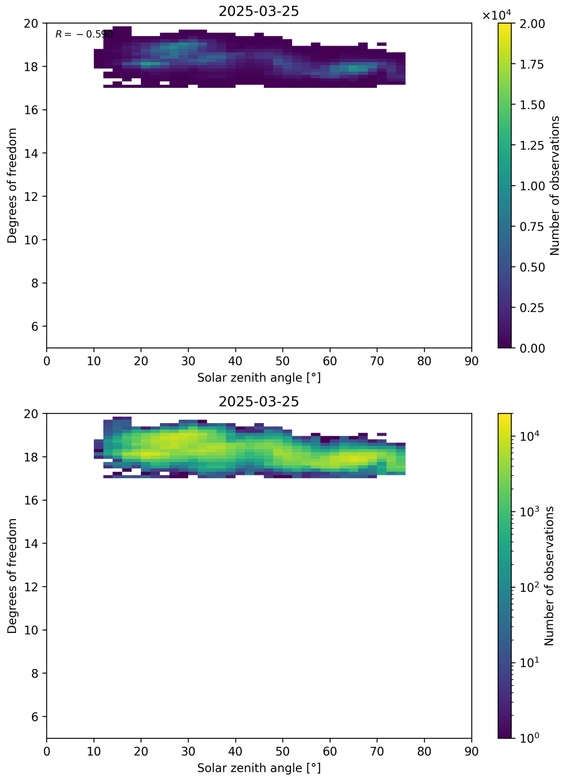
Figure 96: Scatter density plot of “Solar zenith angle” against “Degrees of freedom” for 2025-03-24 to 2025-03-26.
