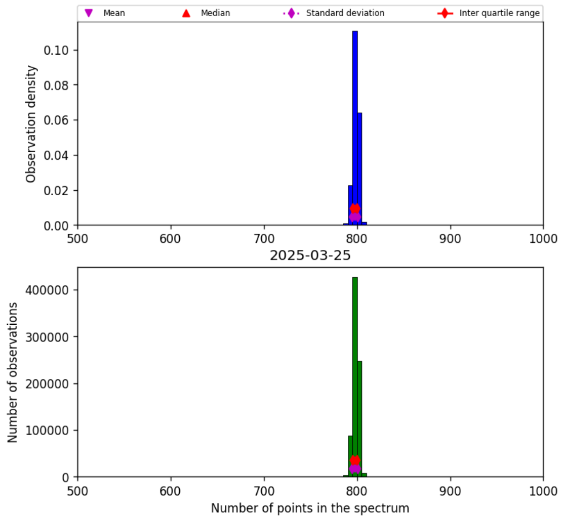
Figure 26: Histogram of “Number of points in the spectrum” for 2025-03-24 to 2025-03-26
