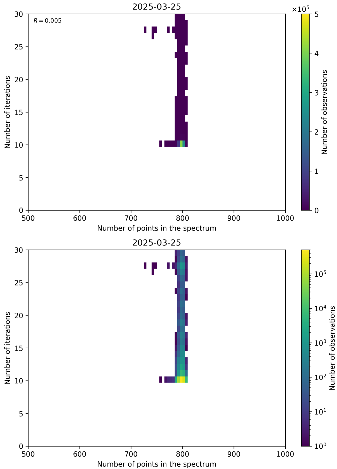
Figure 92: Scatter density plot of “Number of points in the spectrum” against “Number of iterations” for 2025-03-24 to 2025-03-26.
