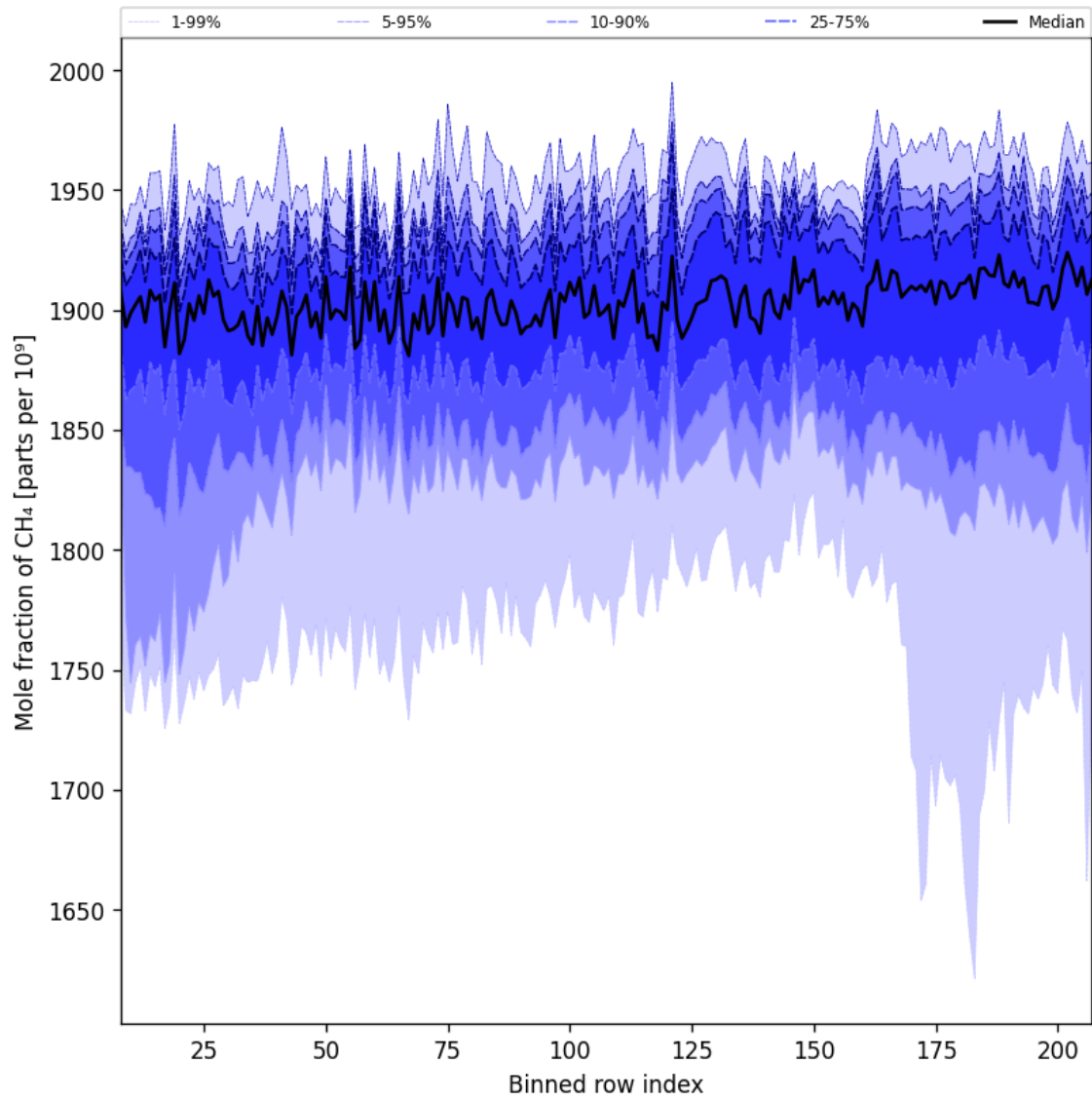
Figure 34: Along track statistics of “Mole fraction of \text{CH}_4 ” for 2025-03-24 to 2025-03-26
