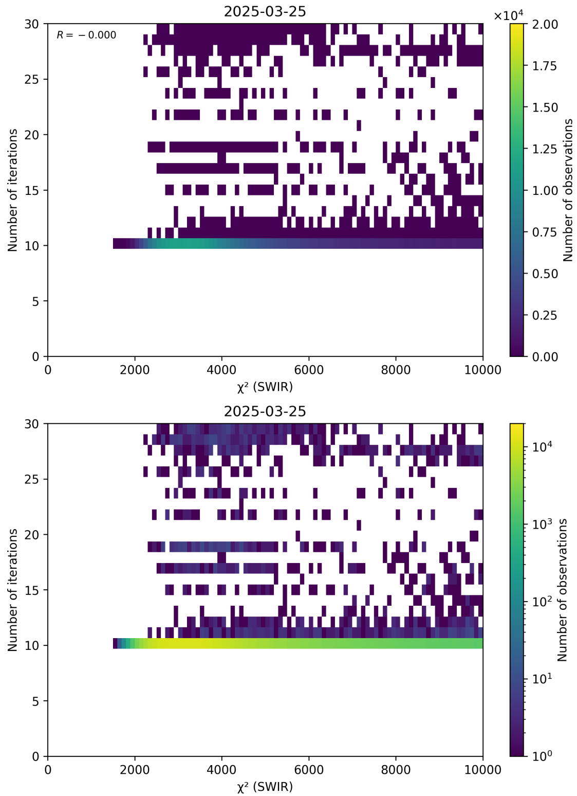
Figure 50: Scatter density plot of “ \chi^2 (SWIR)” against “Number of iterations” for 2025-03-24 to 2025-03-26.
