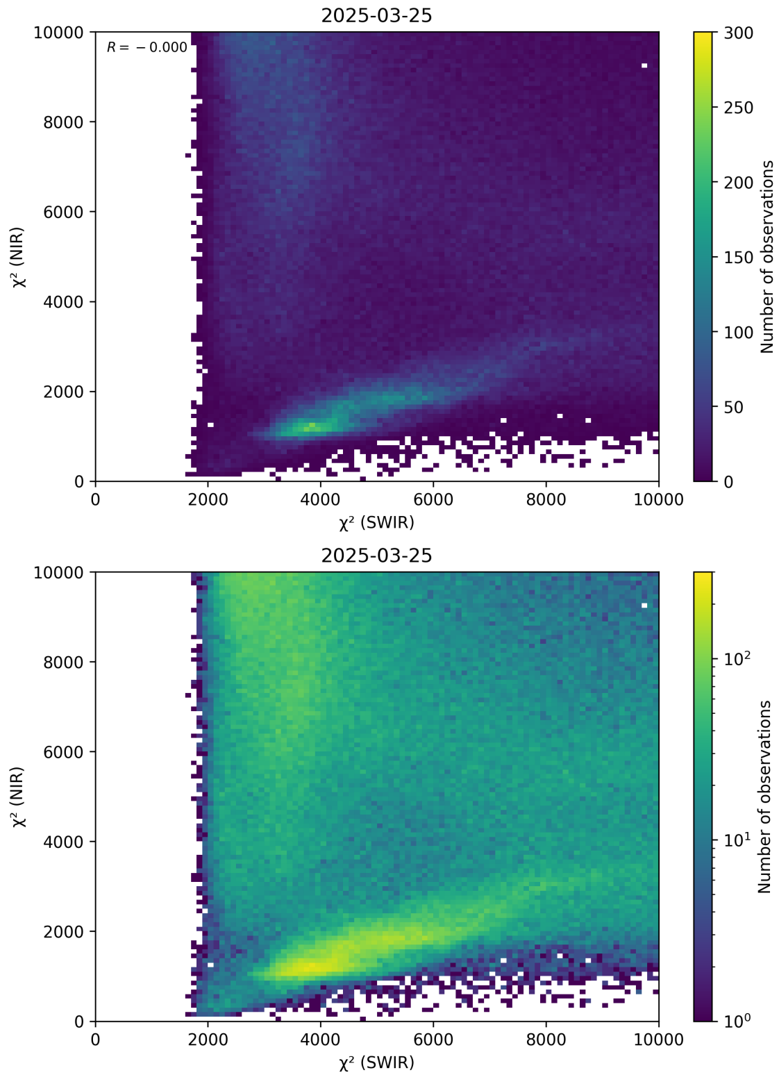
Figure 47: Scatter density plot of “ \chi^2 (SWIR)” against “ \chi^2 (NIR)” for 2025-03-24 to 2025-03-26.
