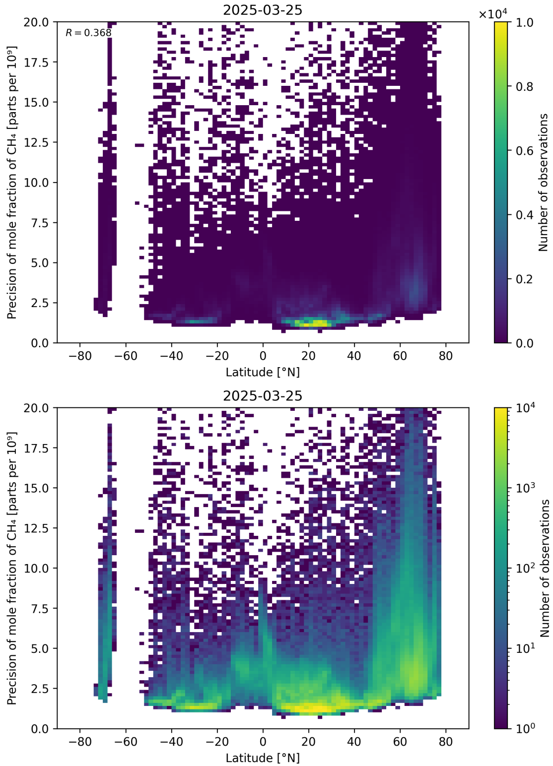
Figure 59: Scatter density plot of “Latitude” against “Precision of mole fraction of \text{CH}_4 ” for 2025-03-24 to 2025-03-26.
