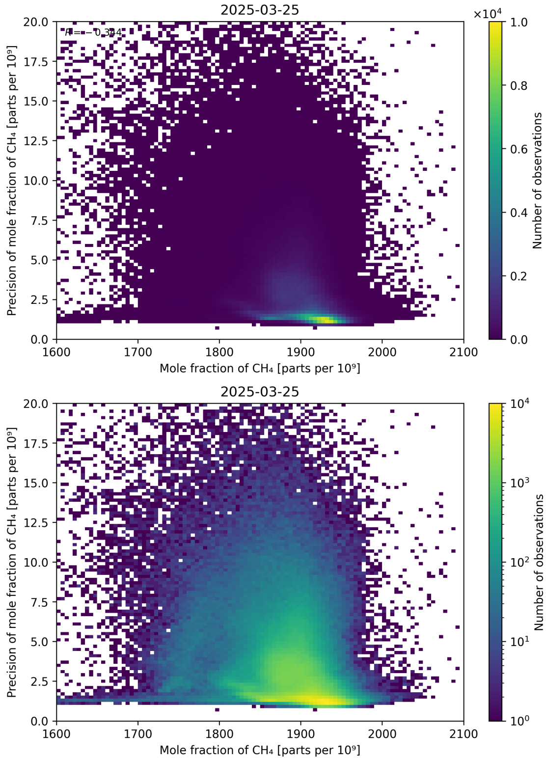
Figure 75: Scatter density plot of “Mole fraction of CH 4 ” against “Precision of mole fraction of CH 4 ” for 2025-03-24 to 2025-03-26.
