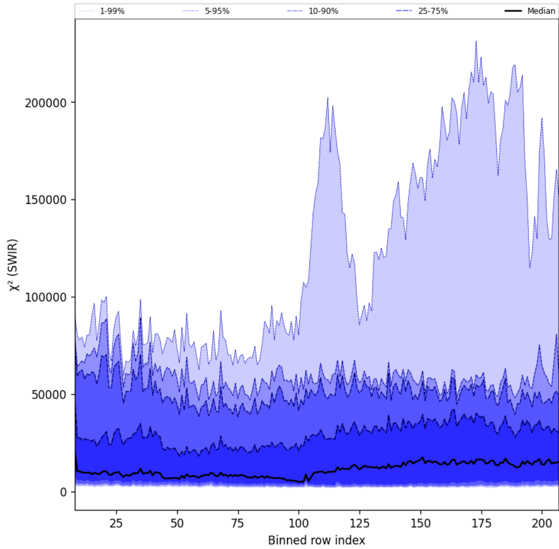
Figure 39: Along track statistics of “ \chi^2 (SWIR)” for 2025-03-24 to 2025-03-26
