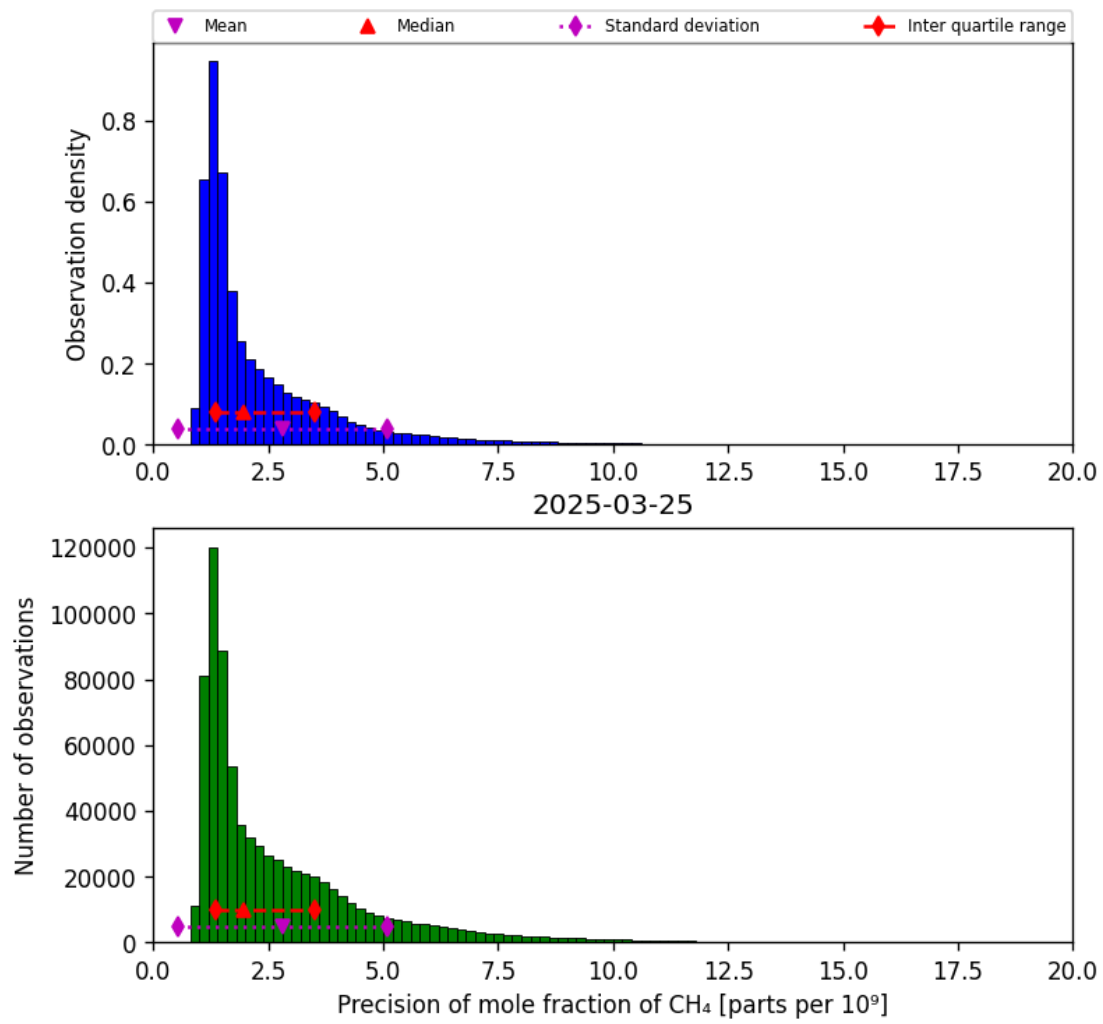
Figure 24: Histogram of “Precision of mole fraction of CH 4 ” for 2025-03-24 to 2025-03-26
