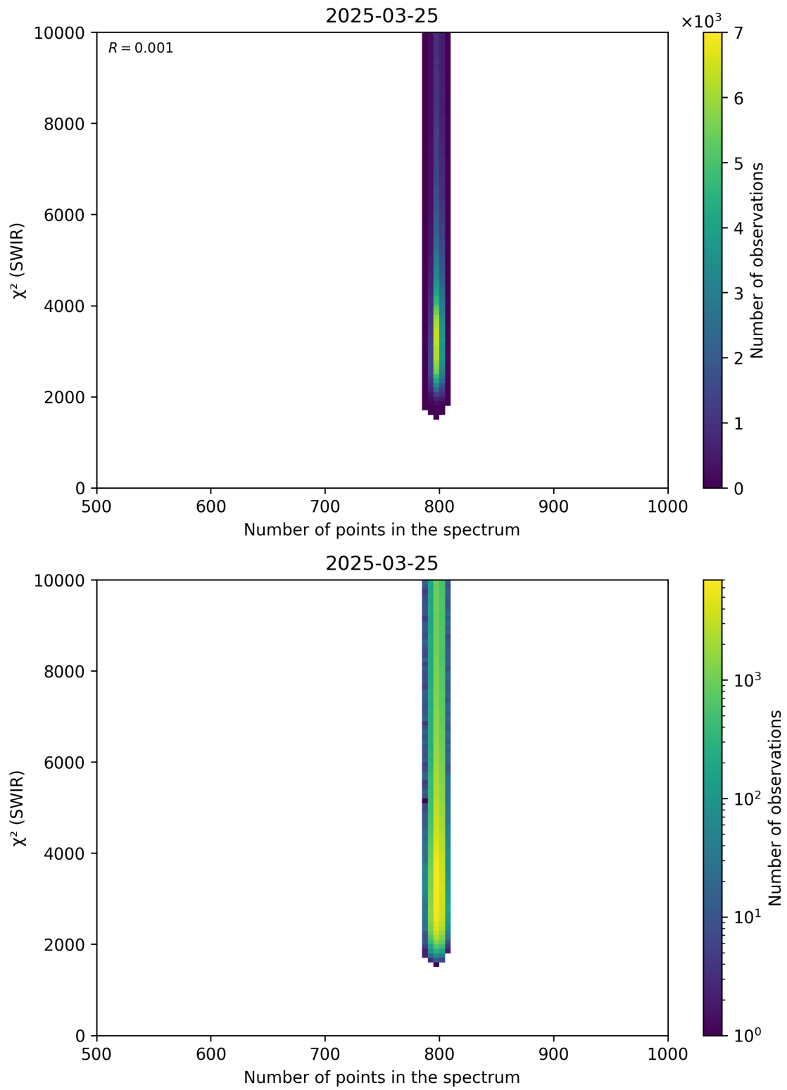
Figure 89: Scatter density plot of “Number of points in the spectrum” against “ \chi^2 (SWIR)” for 2025-03-24 to 2025-03-26.
