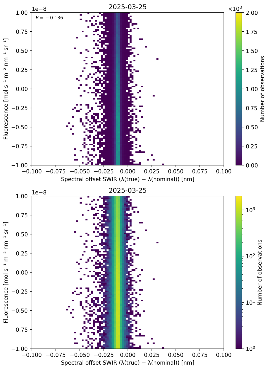
Figure 120: Scatter density plot of “Spectral offset SWIR ( \lambda_{\text{true}} - \lambda_{\text{nominal}} )” against “Fluorescence” for 2025-03-24 to 2025-03-26.
