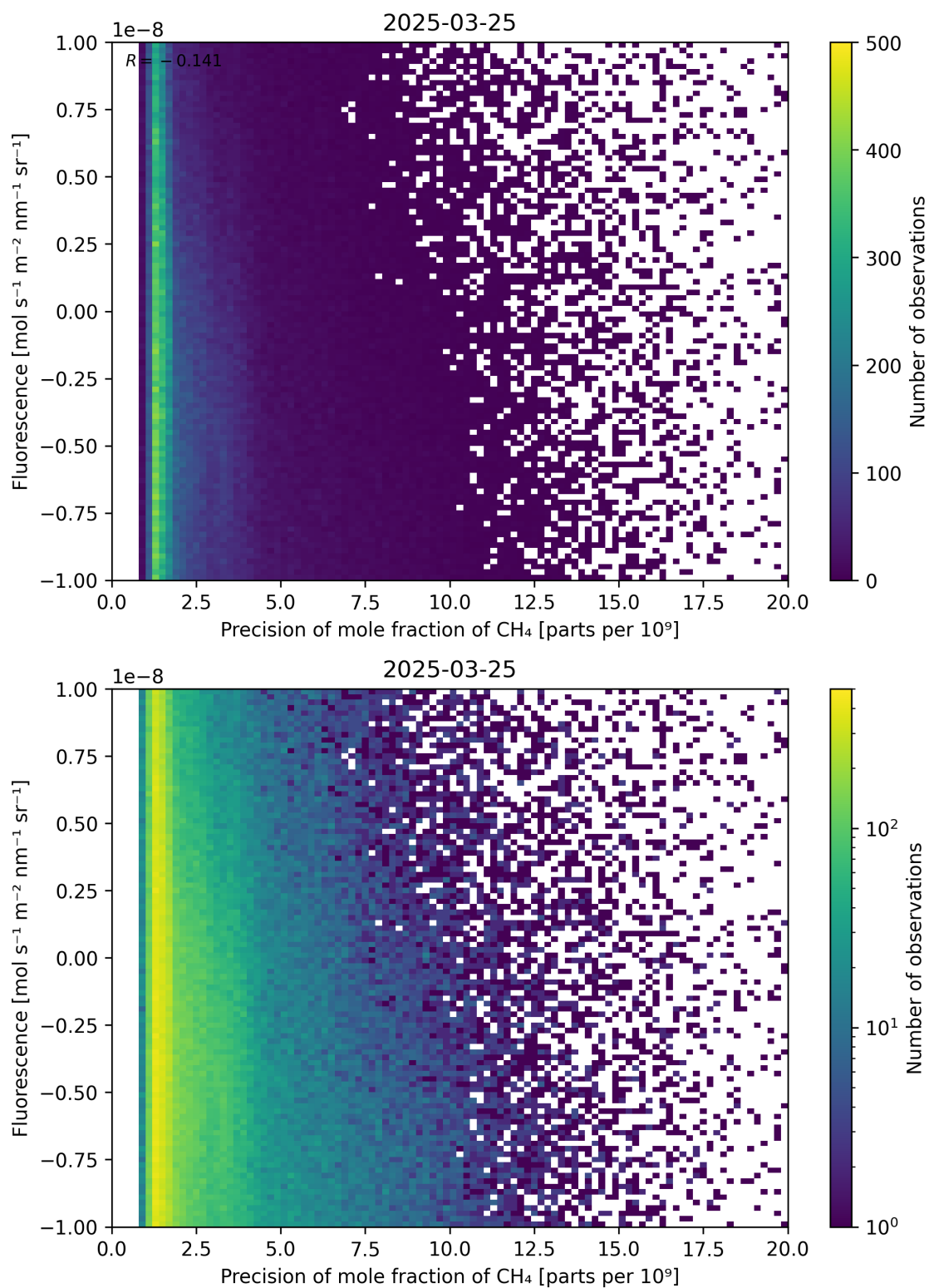
Figure 81: Scatter density plot of “Precision of mole fraction of CH 4 ” against “Fluorescence” for 2025-03-24 to 2025-03-26.
