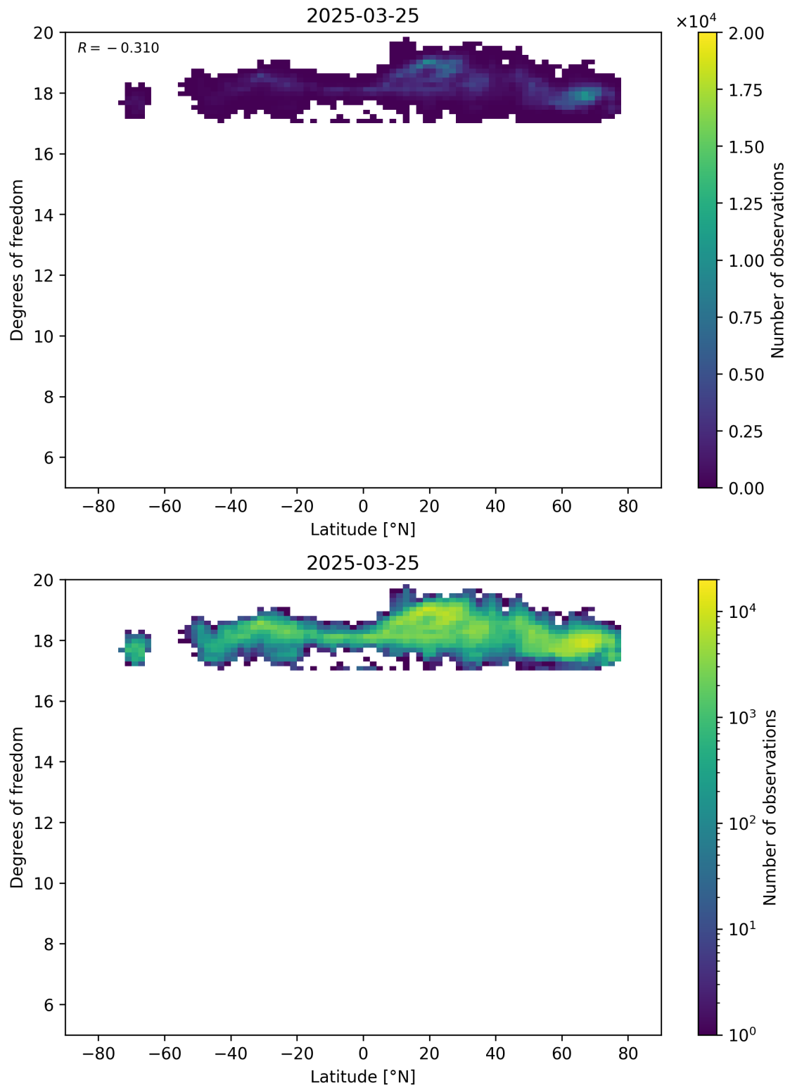
Figure 55: Scatter density plot of “Latitude” against “Degrees of freedom” for 2025-03-24 to 2025-03-26.
