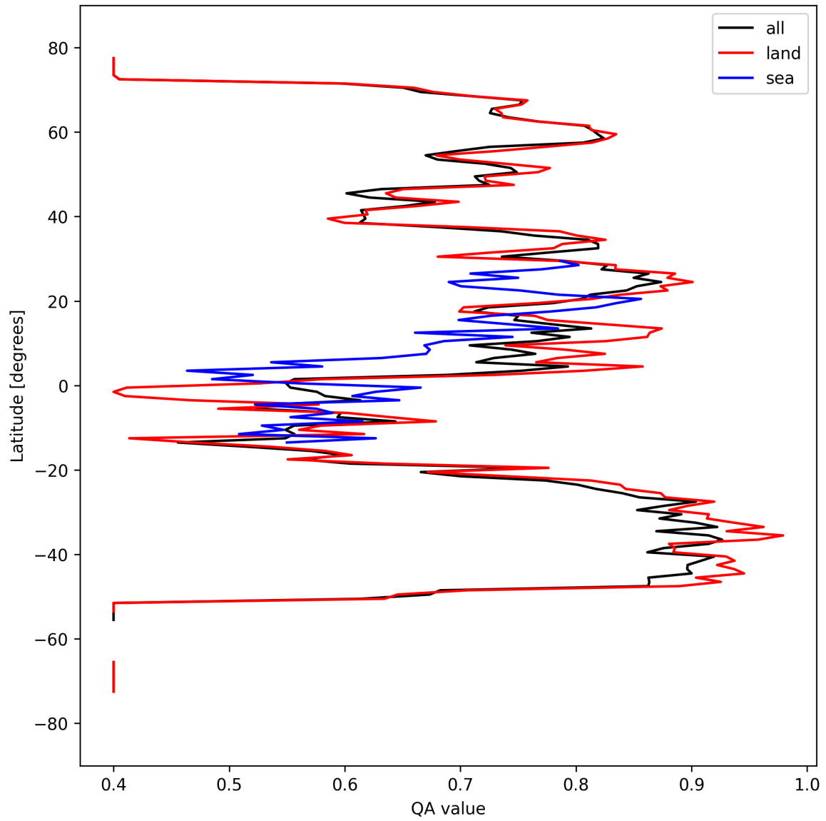
Figure 11: Zonal average of “QA value” for 2025-03-24 to 2025-03-26.
