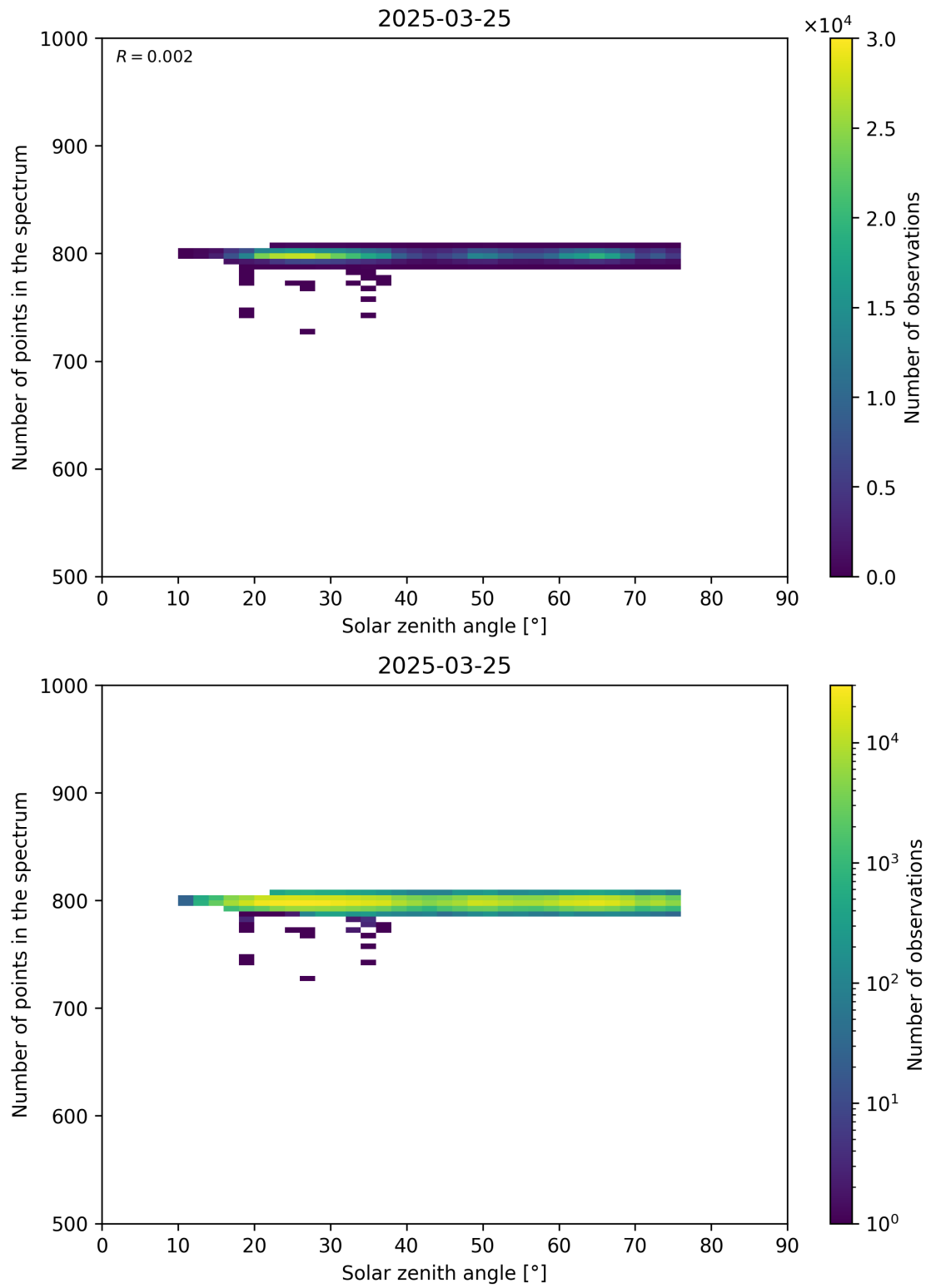
Figure 103: Scatter density plot of “Solar zenith angle” against “Number of points in the spectrum” for 2025-03-24 to 2025-03-26.
