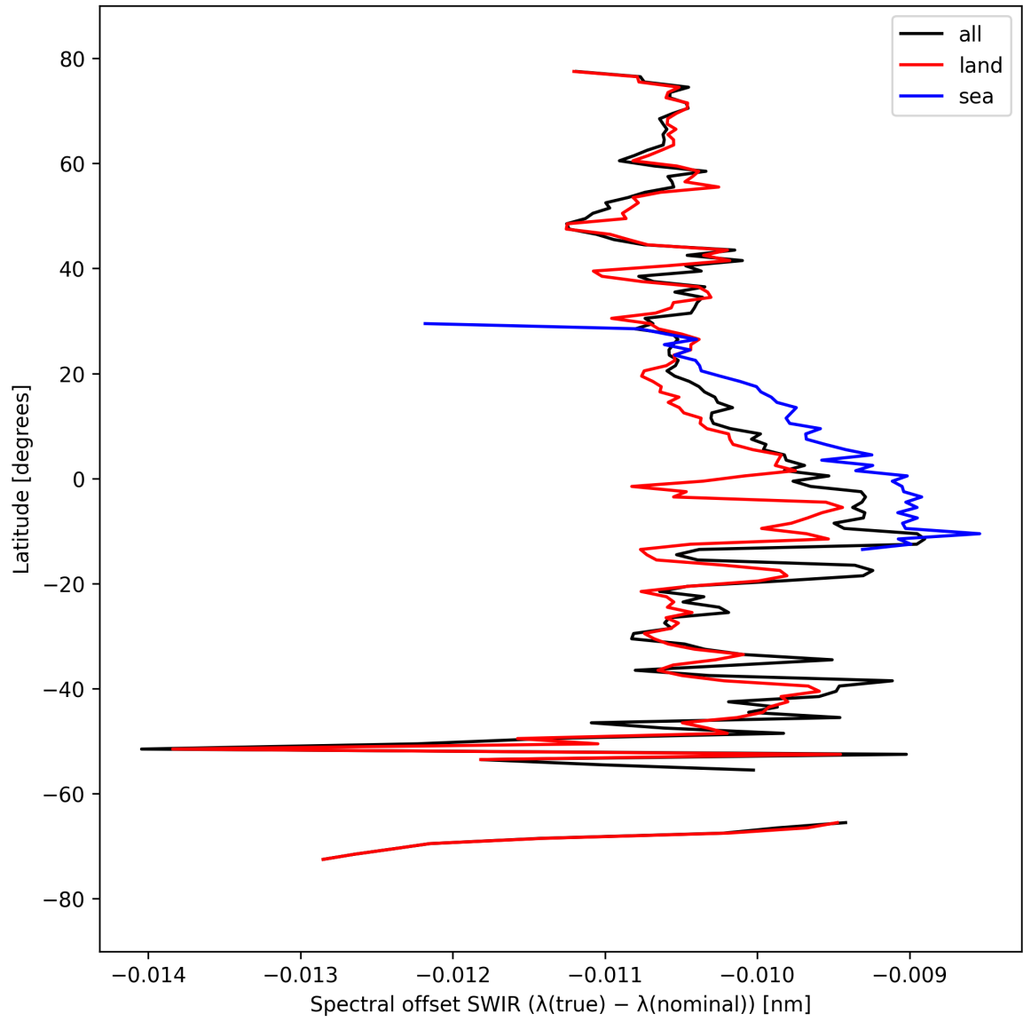
Figure 16: Zonal average of “Spectral offset SWIR ( \lambda_{\text{true}} - \lambda_{\text{nominal}} )” for 2025-03-24 to 2025-03-26.
