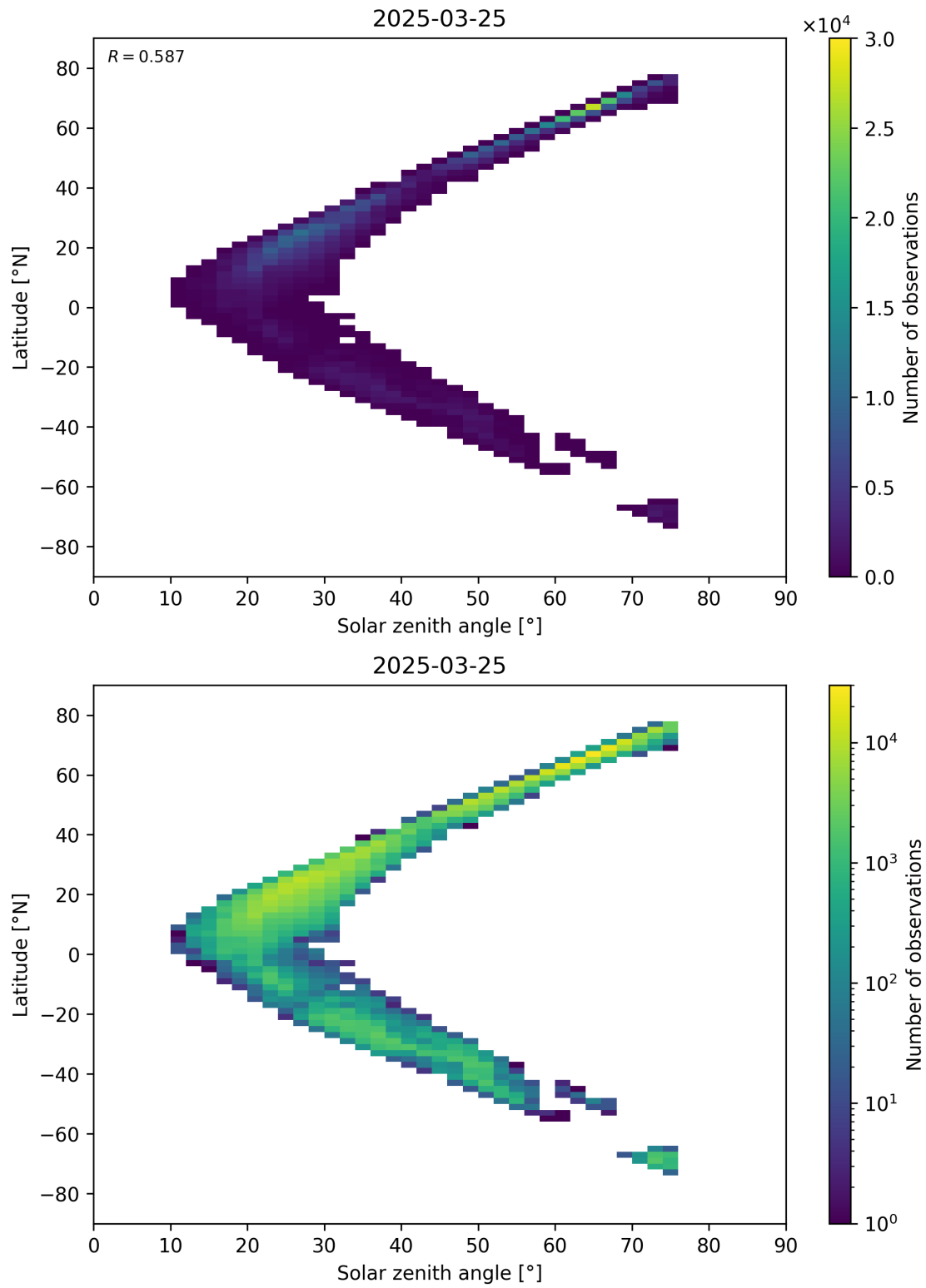
Figure 98: Scatter density plot of “Solar zenith angle” against “Latitude” for 2025-03-24 to 2025-03-26.
