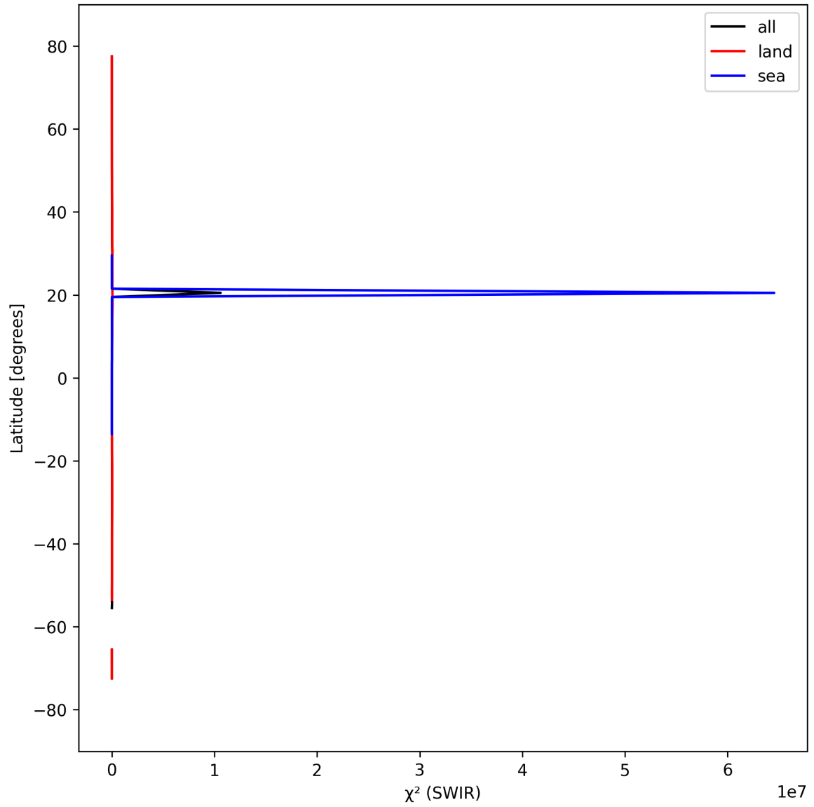
Figure 17: Zonal average of “ \chi^2 (SWIR)” for 2025-03-24 to 2025-03-26.
