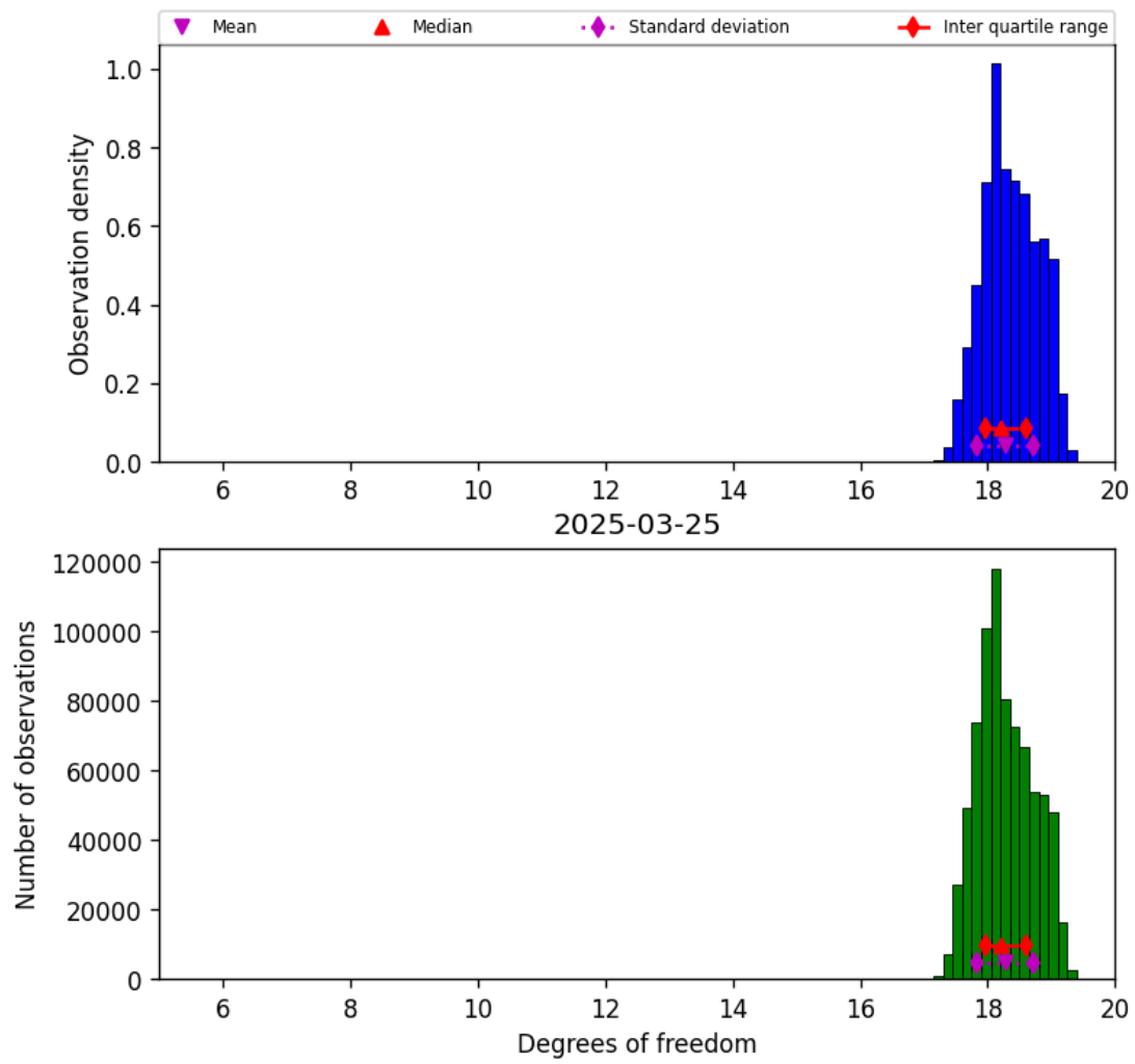
Figure 30: Histogram of “Degrees of freedom” for 2025-03-24 to 2025-03-26
