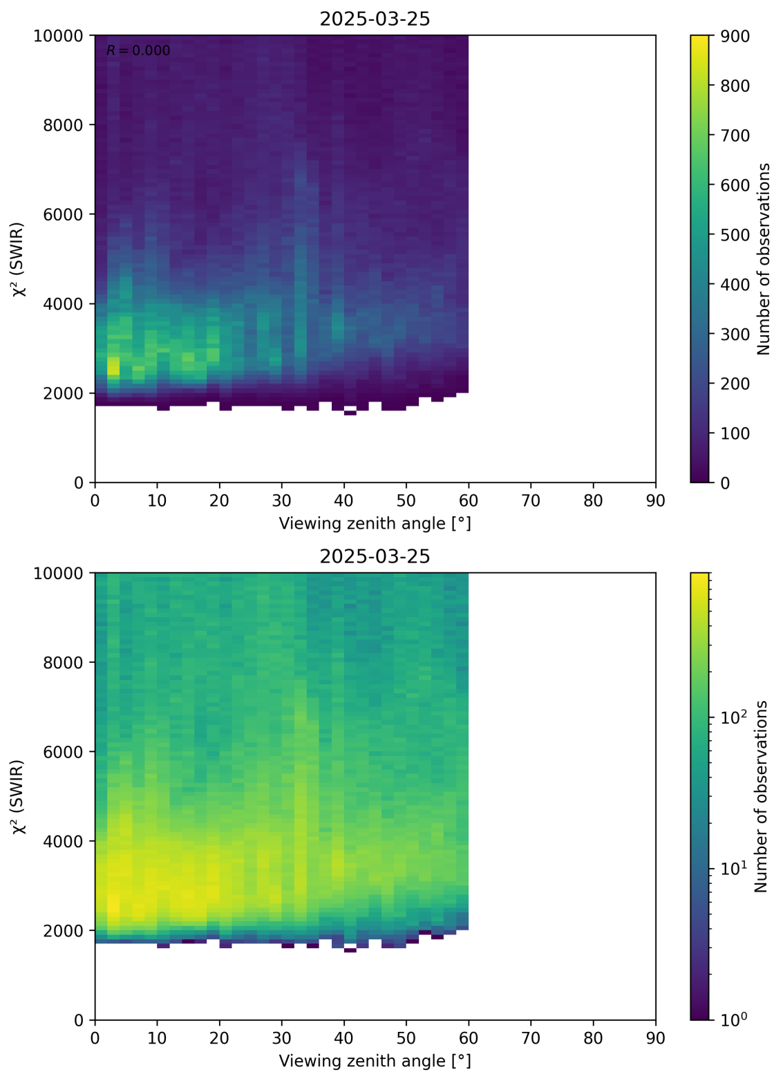
Figure 106: Scatter density plot of “Viewing zenith angle” against “ \chi^2 (SWIR)” for 2025-03-24 to 2025-03-26.
