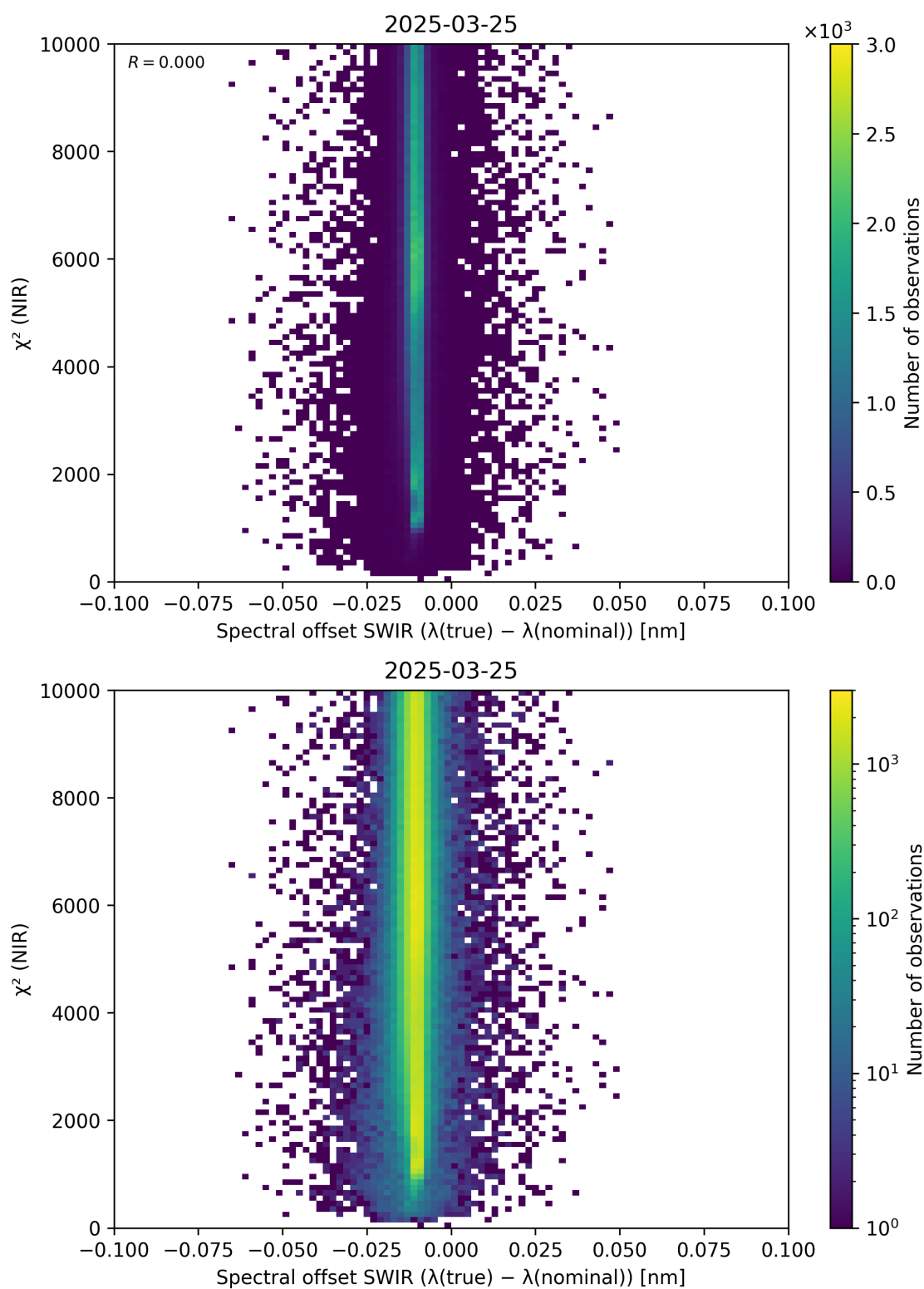
Figure 117: Scatter density plot of “Spectral offset SWIR ( \lambda_{\text{true}} - \lambda_{\text{nominal}} )” against “ \chi^2 (NIR)” for 2025-03-24 to 2025-03-26.
