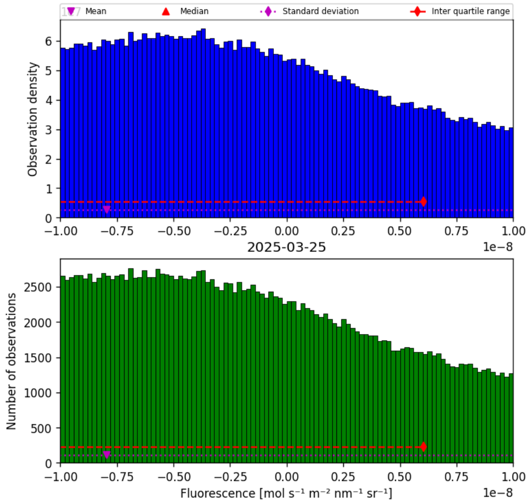
Figure 32: Histogram of “Fluorescence” for 2025-03-24 to 2025-03-26
