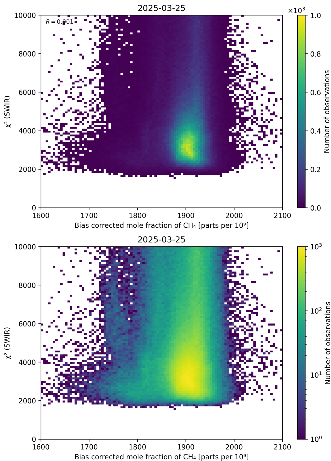
Figure 64: Scatter density plot of “Bias corrected mole fraction of \text{CH}_4 ” against “ \chi^2 (SWIR)” for 2025-03-24 to 2025-03-26.
