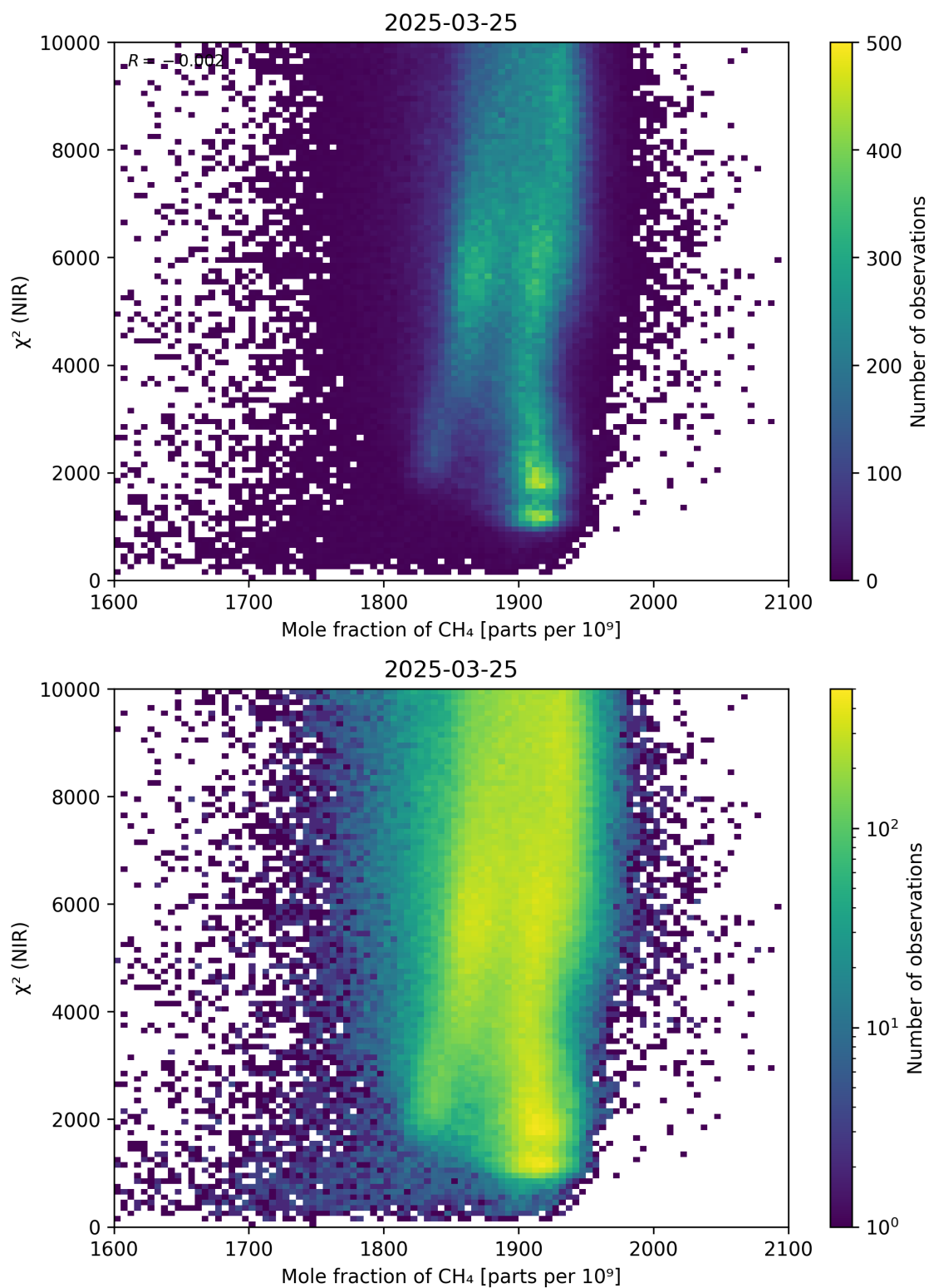
Figure 70: Scatter density plot of “Mole fraction of CH 4 ” against “ \chi^2 (NIR)” for 2025-03-24 to 2025-03-26.
