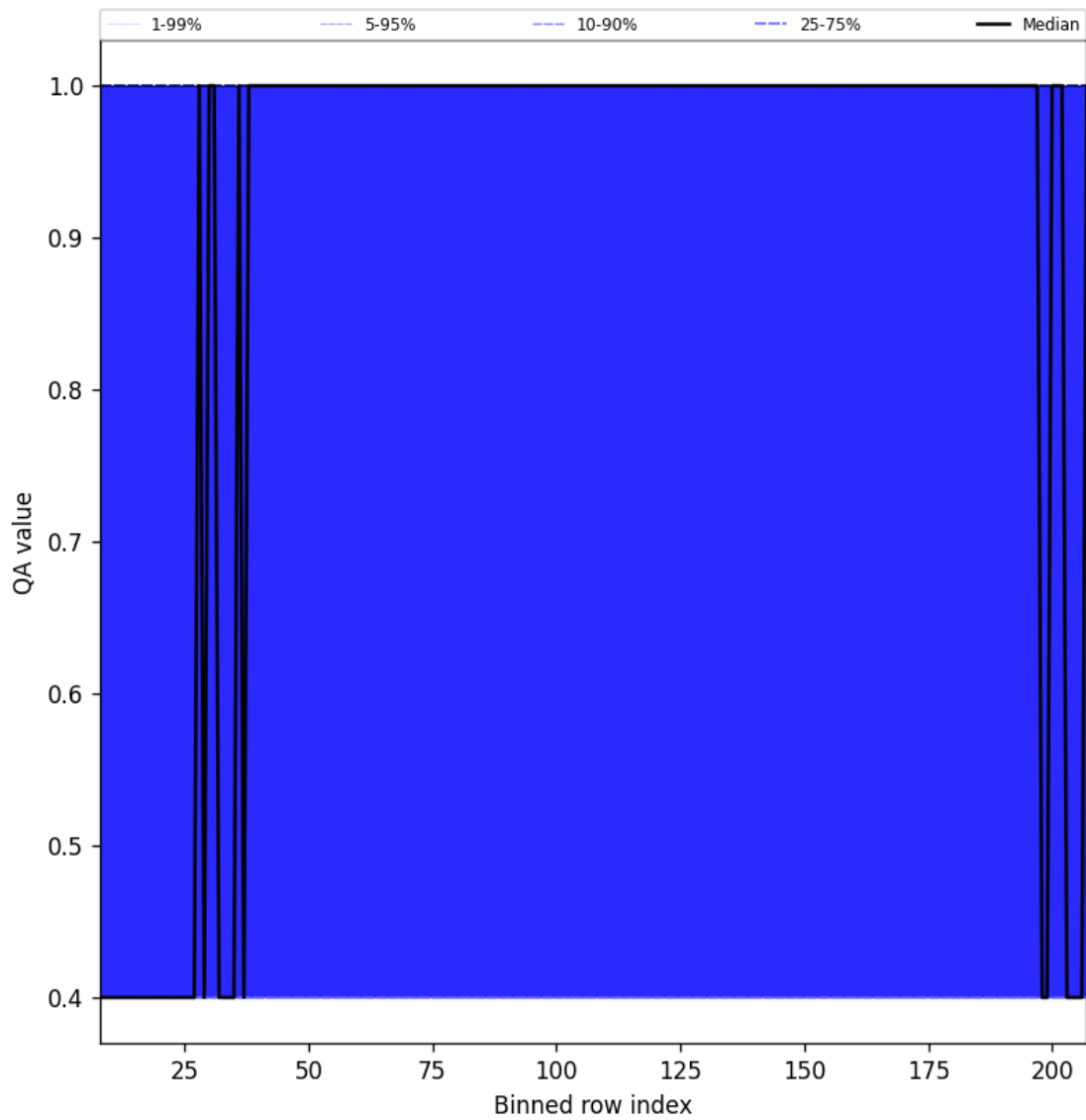
Figure 33: Along track statistics of “QA value” for 2025-03-24 to 2025-03-26
