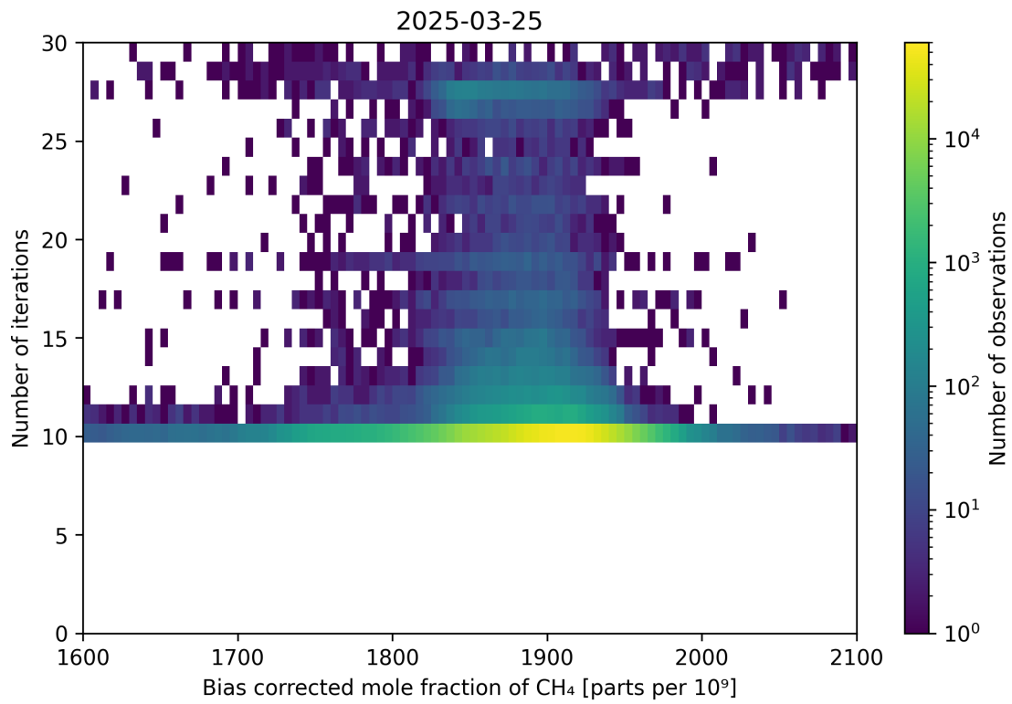
Figure 67: Scatter density plot of “Bias corrected mole fraction of CH 4 ” against “Number of iterations” for 2025-03-24 to 2025-03-26.
