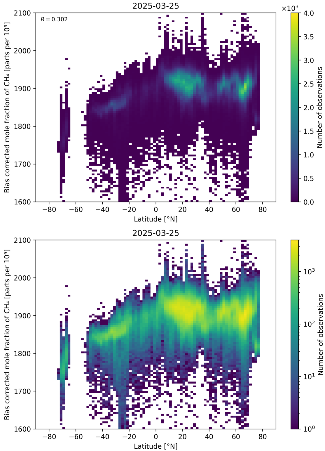
Figure 58: Scatter density plot of “Latitude” against “Bias corrected mole fraction of \text{CH}_4 ” for 2025-03-24 to 2025-03-26.
