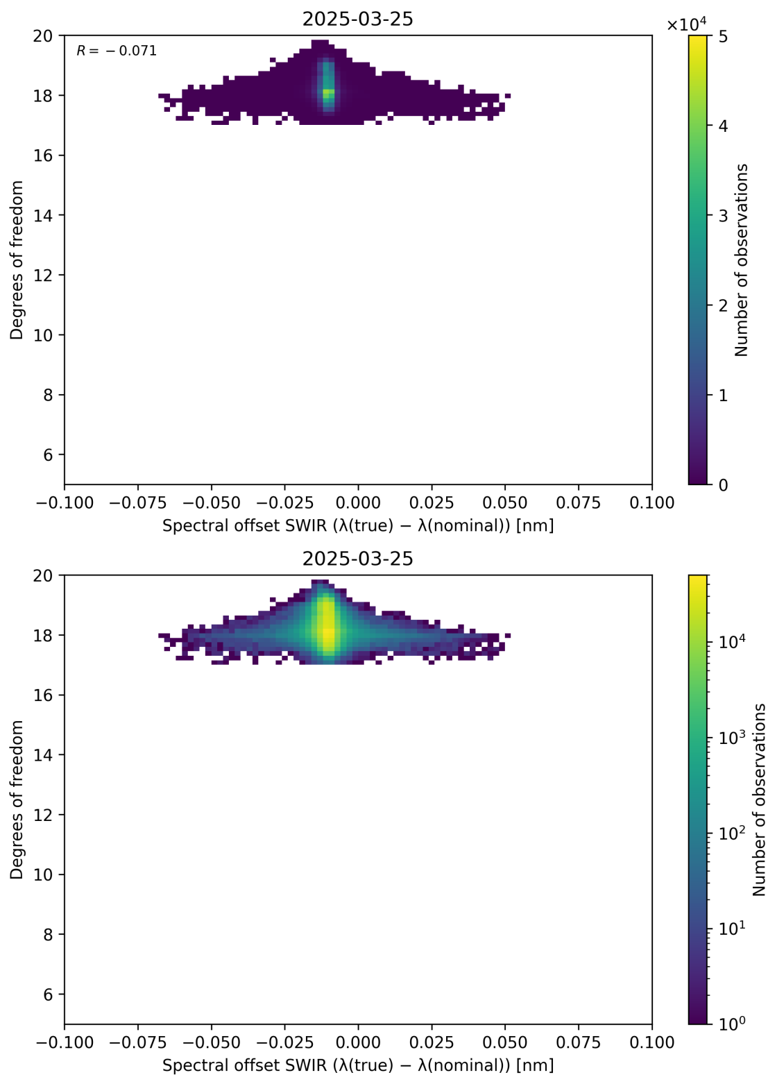
Figure 119: Scatter density plot of “Spectral offset SWIR ( \lambda_{\text{true}} - \lambda_{\text{nominal}} )” against “Degrees of freedom” for 2025-03-24 to 2025-03-26.
