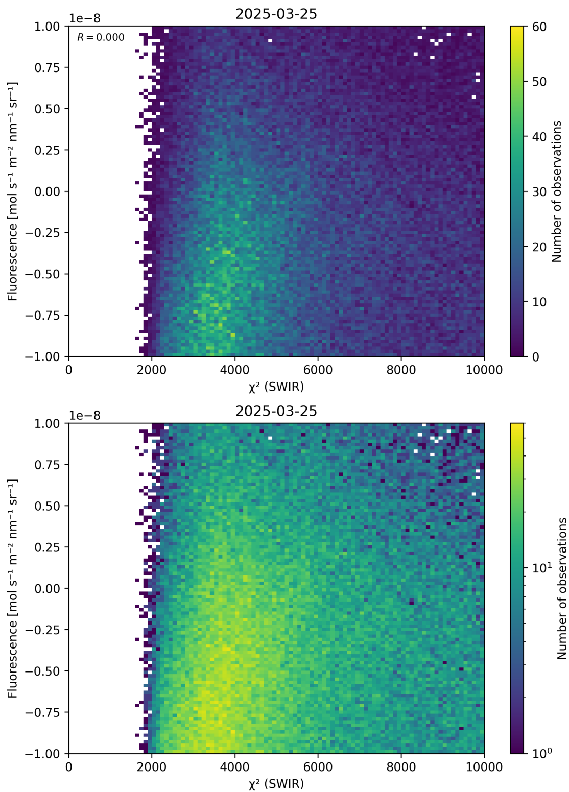
Figure 49: Scatter density plot of “ \chi^2 (SWIR)” against “Fluorescence” for 2025-03-24 to 2025-03-26.
