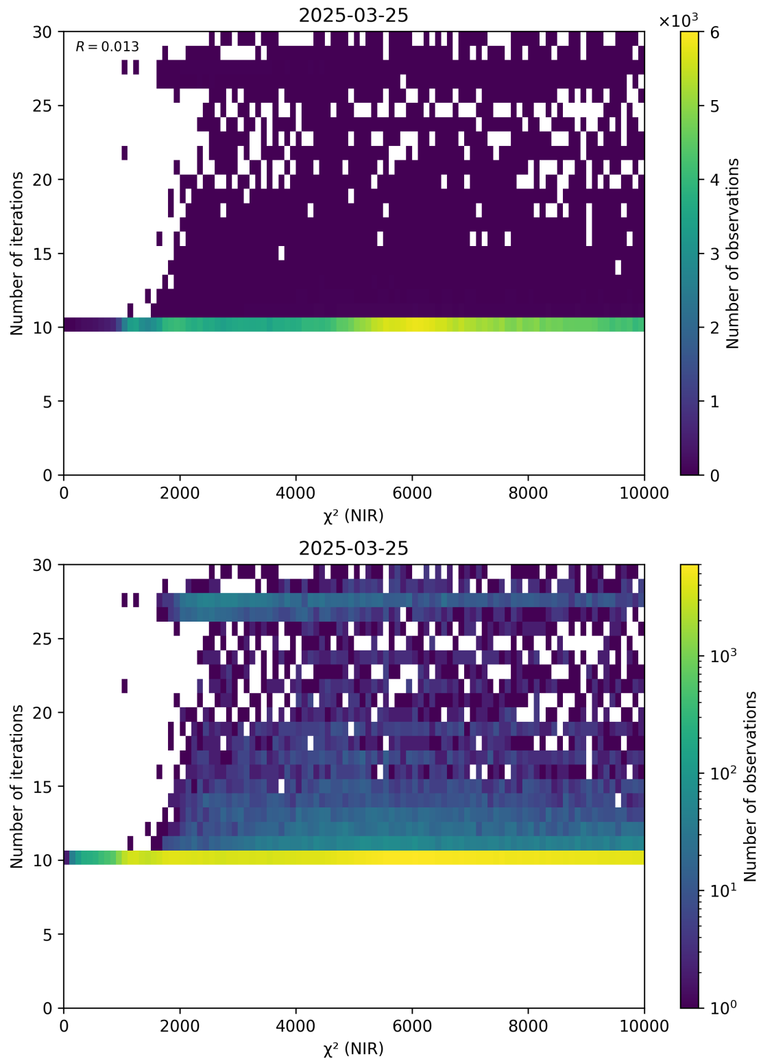
Figure 46: Scatter density plot of “ \chi^2 (NIR)” against “Number of iterations” for 2025-03-24 to 2025-03-26.
