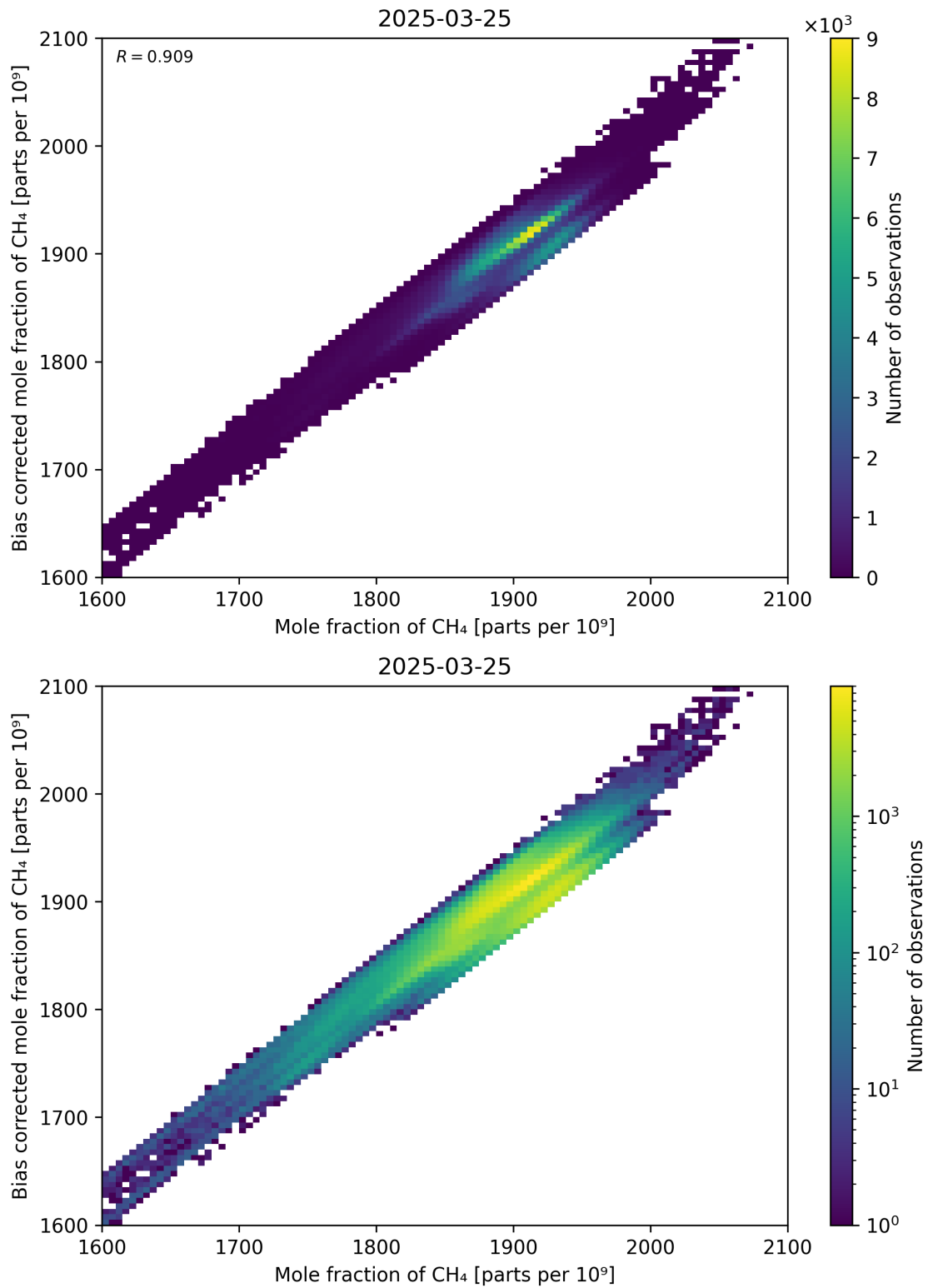
Figure 74: Scatter density plot of “Mole fraction of CH 4 ” against “Bias corrected mole fraction of CH 4 ” for 2025-03-24 to 2025-03-26.
