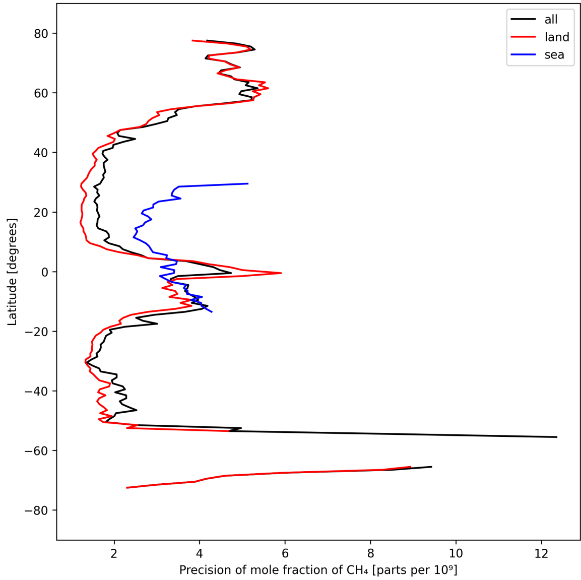
Figure 13: Zonal average of “Precision of mole fraction of CH 4 ” for 2025-03-24 to 2025-03-26.
