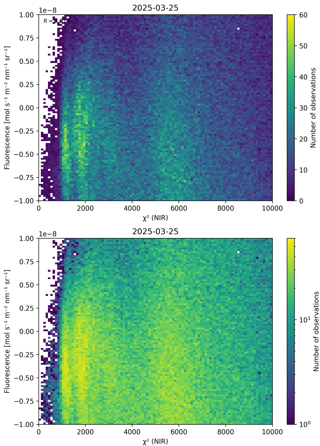
Figure 45: Scatter density plot of “ \chi^2 (NIR)” against “Fluorescence” for 2025-03-24 to 2025-03-26.
