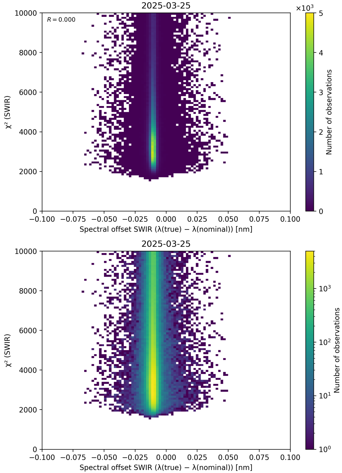
Figure 118: Scatter density plot of “Spectral offset SWIR ( \lambda_{\text{true}} - \lambda_{\text{nominal}} )” against “ \chi^2 (SWIR)” for 2025-03-24 to 2025-03-26.
