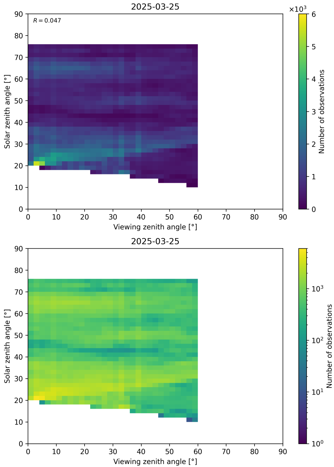
Figure 115: Scatter density plot of “Viewing zenith angle” against “Solar zenith angle” for 2025-03-24 to 2025-03-26.
