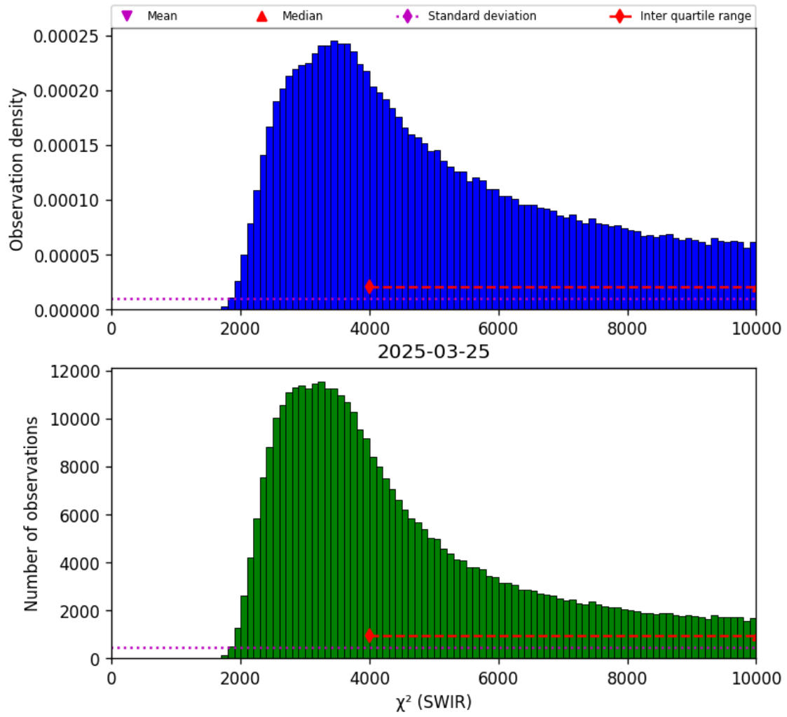
Figure 28: Histogram of “ \chi^2 (SWIR)” for 2025-03-24 to 2025-03-26
