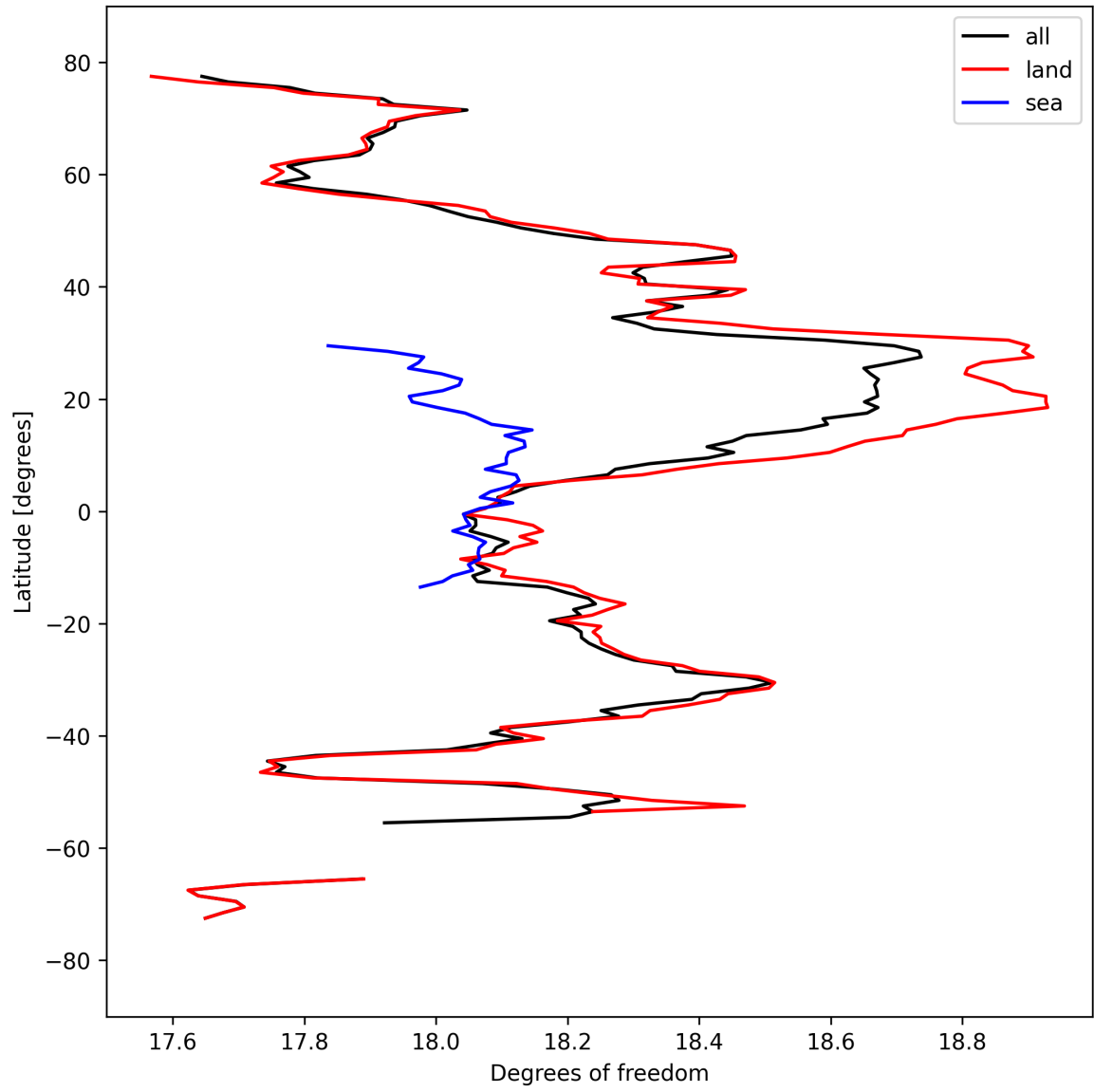
Figure 19: Zonal average of “Degrees of freedom” for 2025-03-24 to 2025-03-26.
