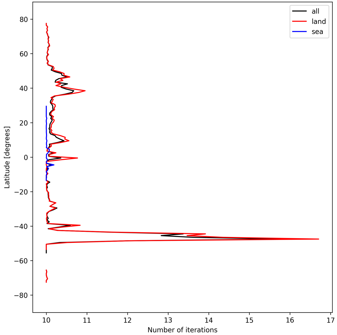
Figure 20: Zonal average of “Number of iterations” for 2025-03-24 to 2025-03-26.
