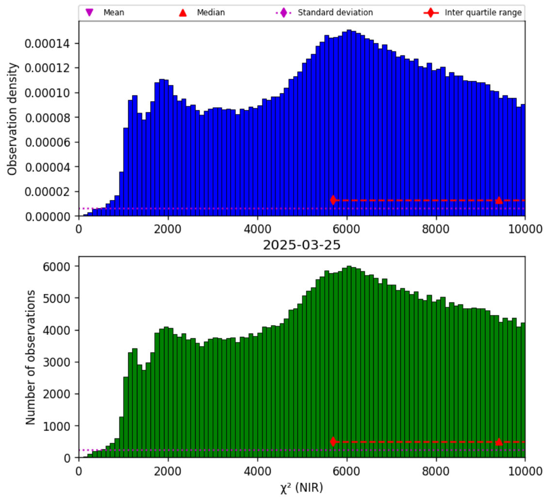
Figure 29: Histogram of “ \chi^2 (NIR)” for 2025-03-24 to 2025-03-26
