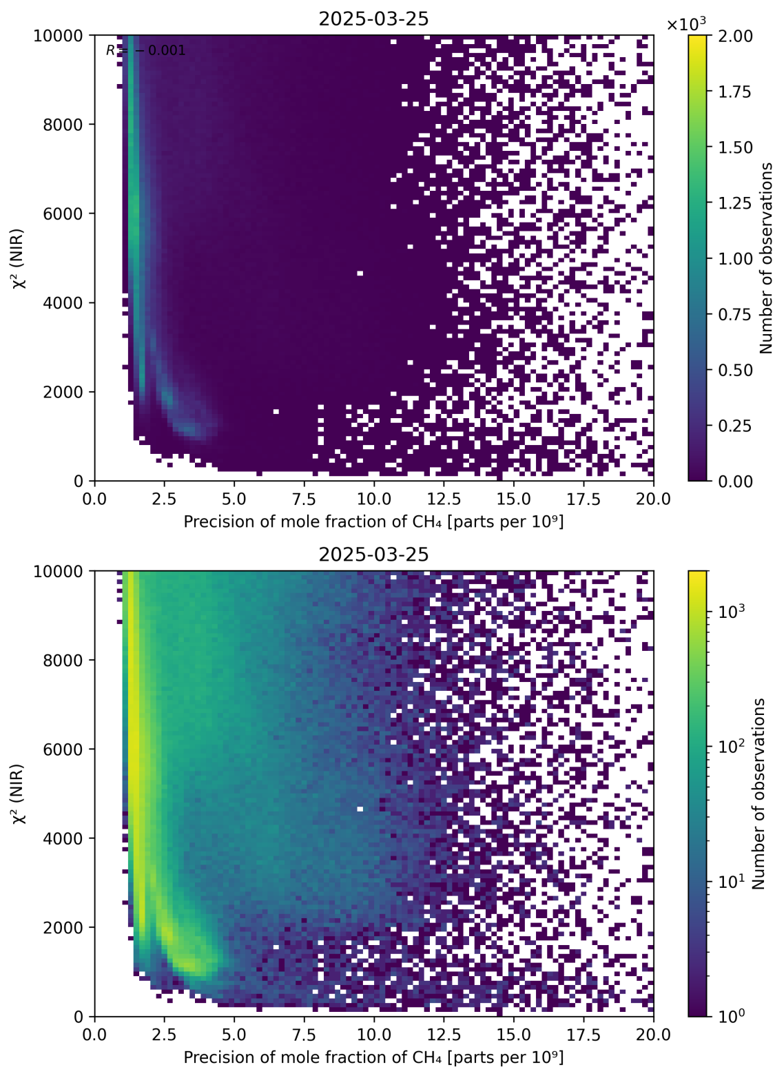
Figure 78: Scatter density plot of “Precision of mole fraction of CH 4 ” against “ \chi^2 (NIR)” for 2025-03-24 to 2025-03-26.
