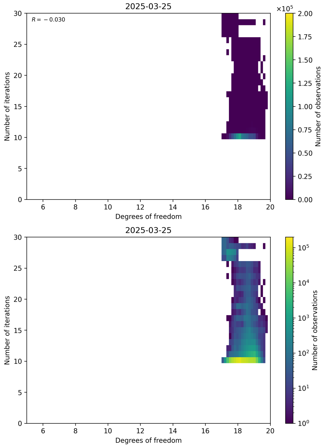
Figure 52: Scatter density plot of “Degrees of freedom” against “Number of iterations” for 2025-03-24 to 2025-03-26.
