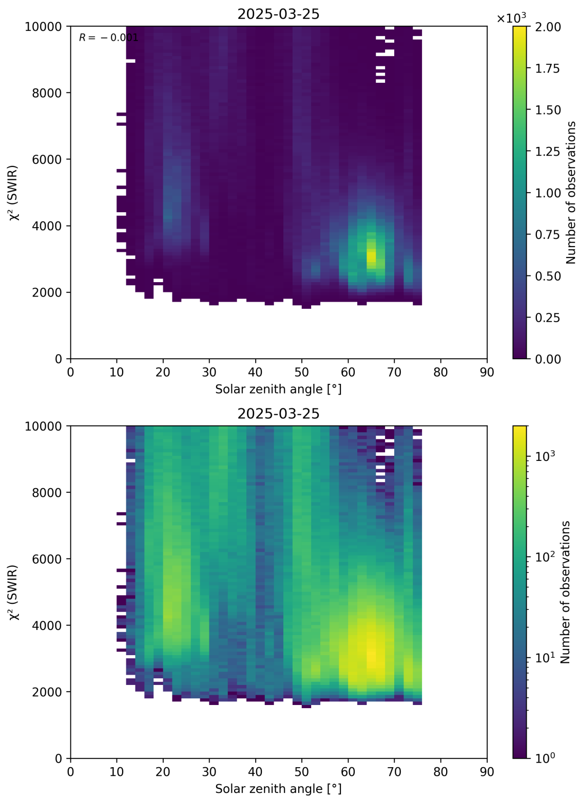
Figure 95: Scatter density plot of “Solar zenith angle” against “ \chi^2 (SWIR)” for 2025-03-24 to 2025-03-26.
