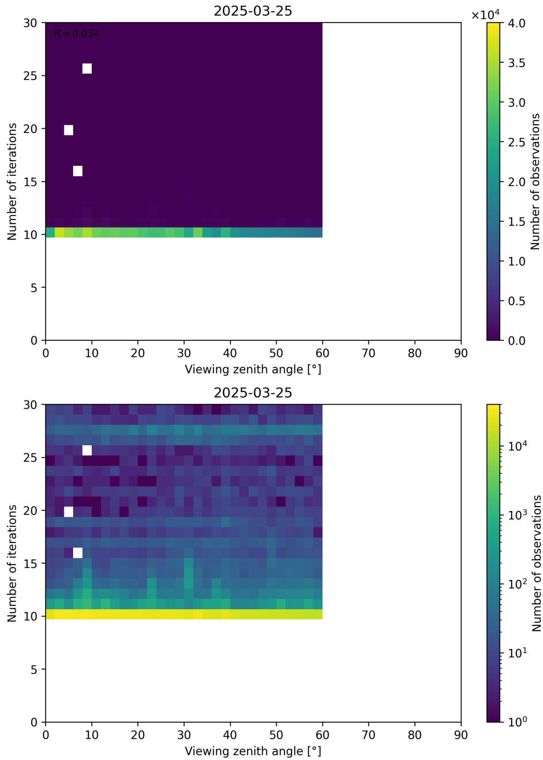
Figure 113: Scatter density plot of “Viewing zenith angle” against “Number of iterations” for 2025-03-24 to 2025-03-26.
