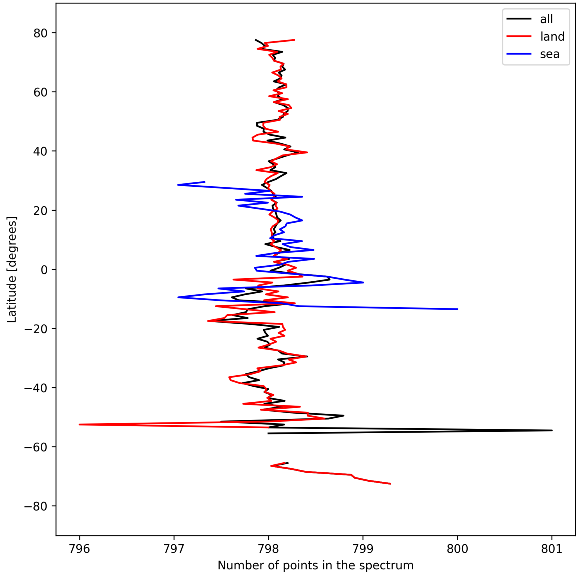
Figure 15: Zonal average of “Number of points in the spectrum” for 2025-03-24 to 2025-03-26.
