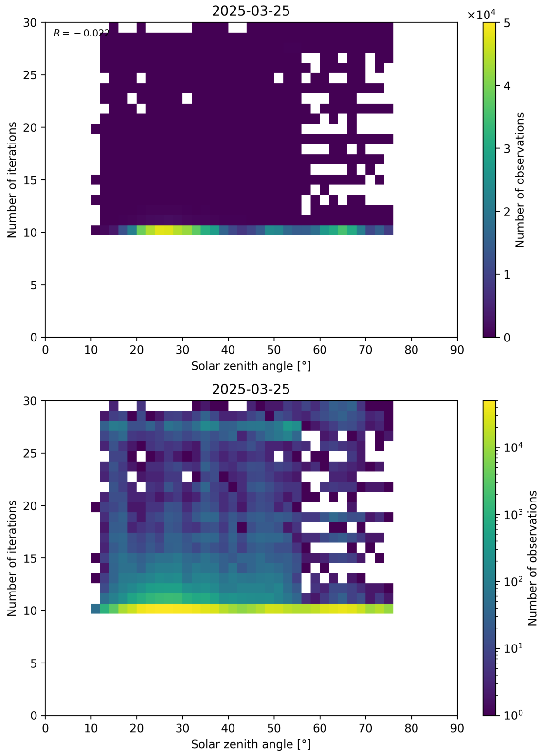
Figure 102: Scatter density plot of “Solar zenith angle” against “Number of iterations” for 2025-03-24 to 2025-03-26.
