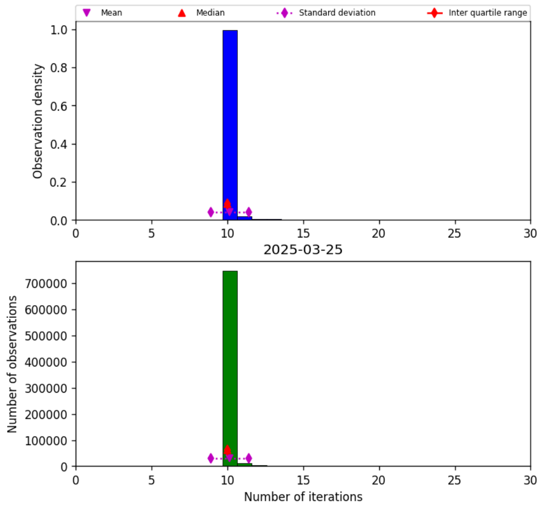
Figure 31: Histogram of “Number of iterations” for 2025-03-24 to 2025-03-26
