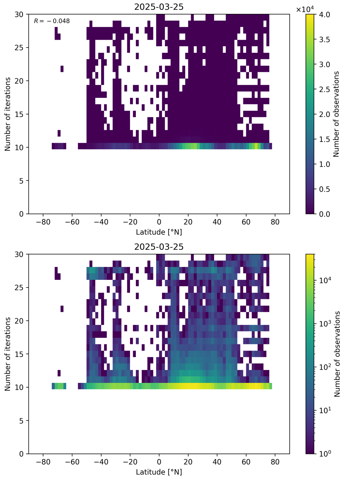
Figure 60: Scatter density plot of “Latitude” against “Number of iterations” for 2025-03-24 to 2025-03-26.
