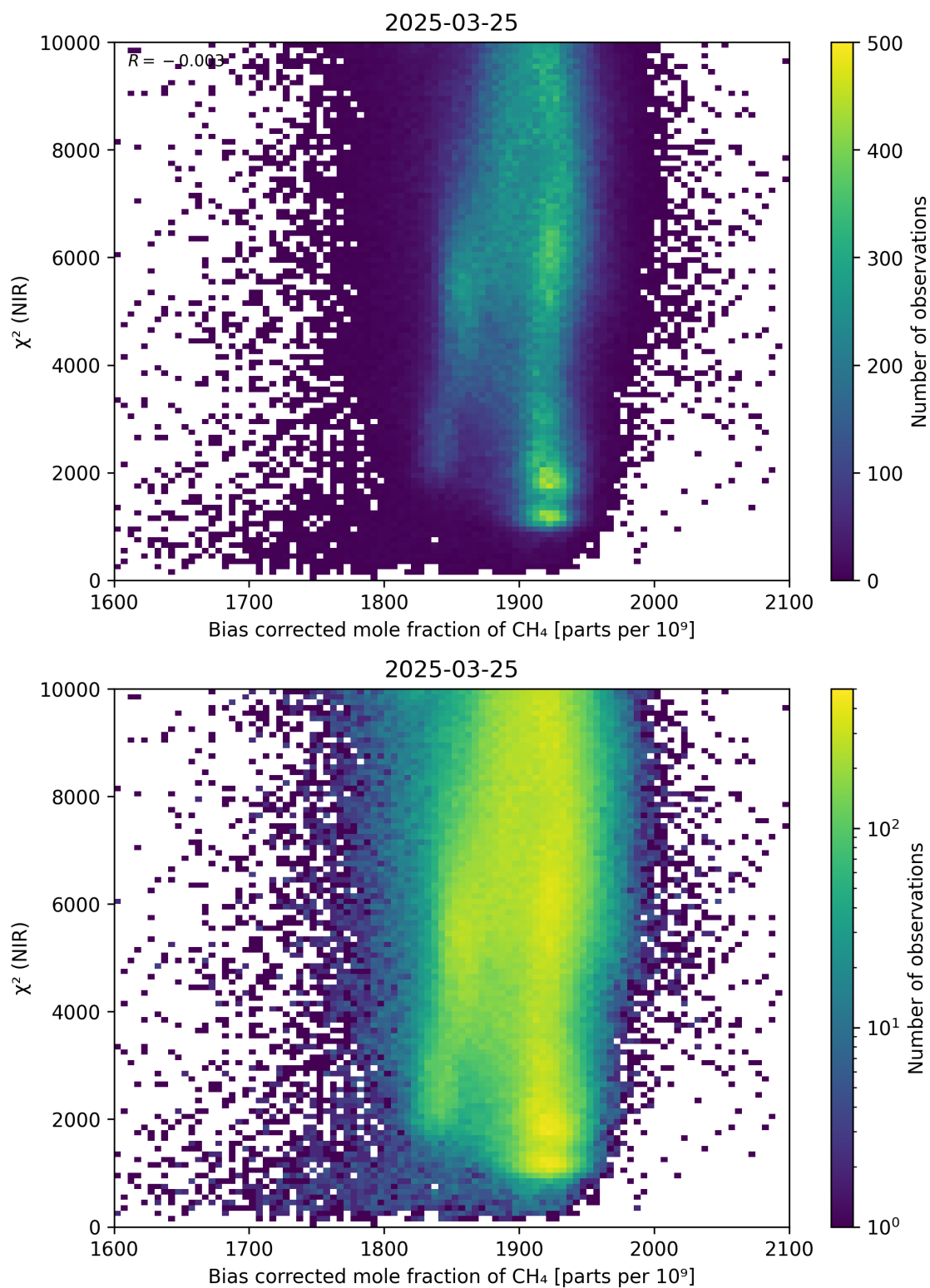
Figure 63: Scatter density plot of “Bias corrected mole fraction of CH 4 ” against “ \chi^2 (NIR)” for 2025-03-24 to 2025-03-26.
