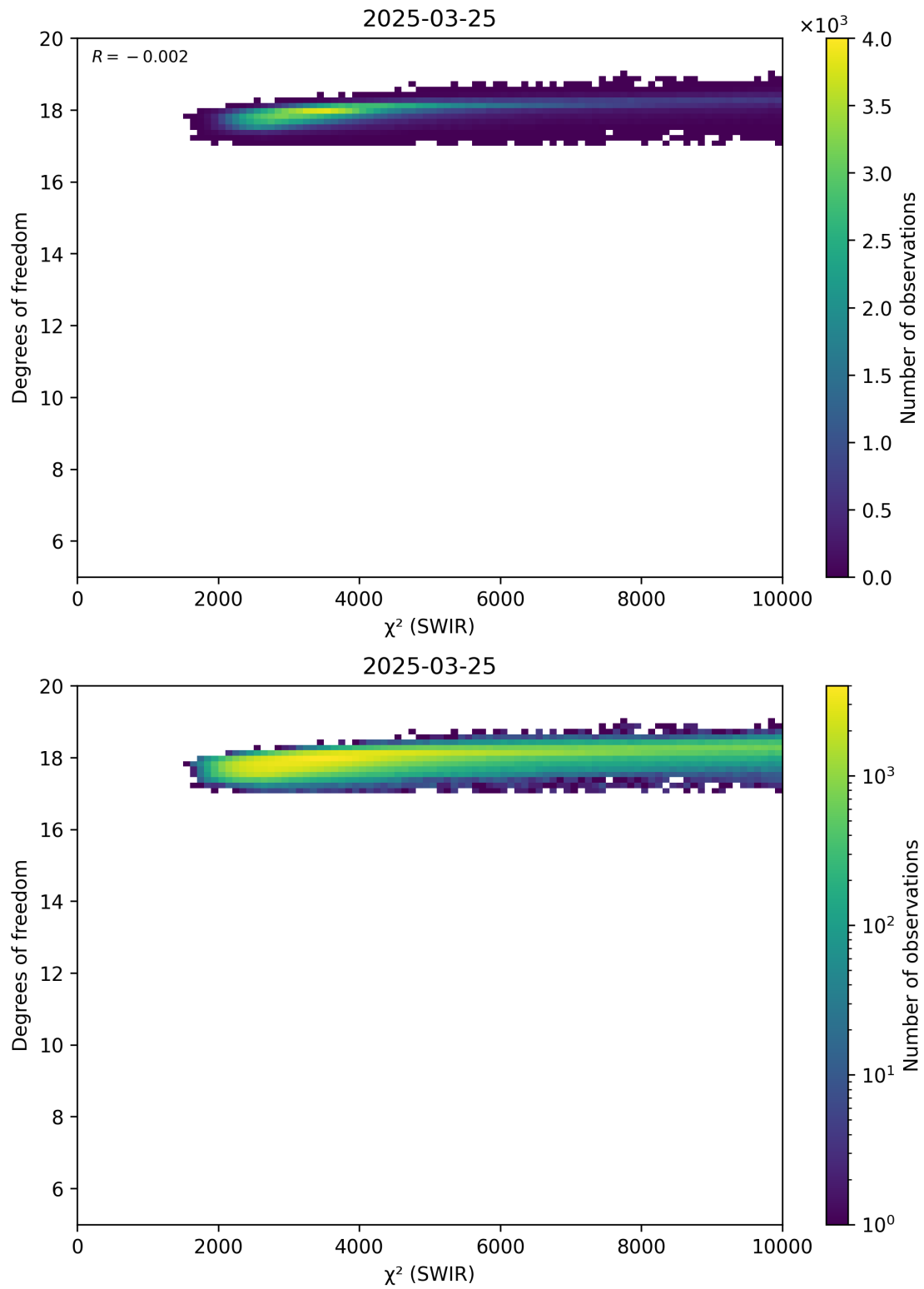
Figure 48: Scatter density plot of “ \chi^2 (SWIR)” against “Degrees of freedom” for 2025-03-24 to 2025-03-26.
