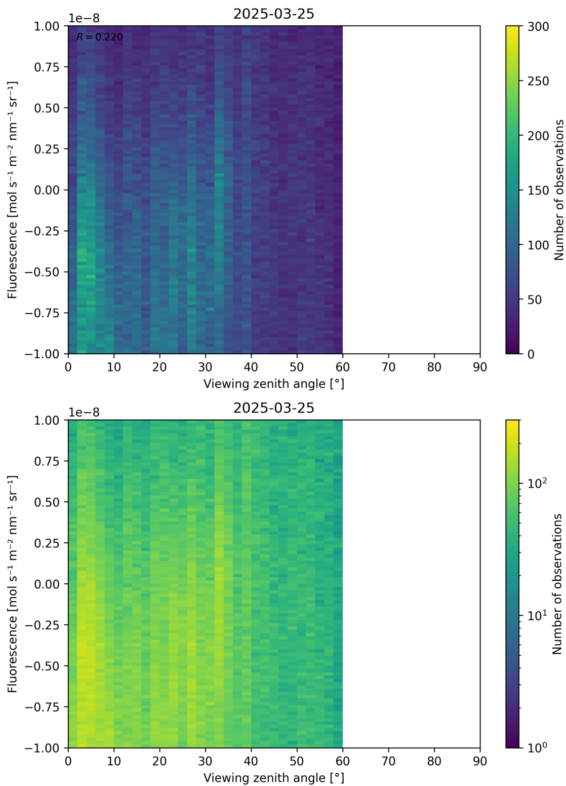
Figure 108: Scatter density plot of “Viewing zenith angle” against “Fluorescence” for 2025-03-24 to 2025-03-26.
