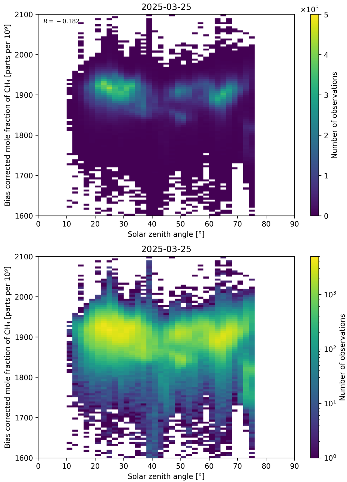
Figure 100: Scatter density plot of “Solar zenith angle” against “Bias corrected mole fraction of CH 4 ” for 2025-03-24 to 2025-03-26.
