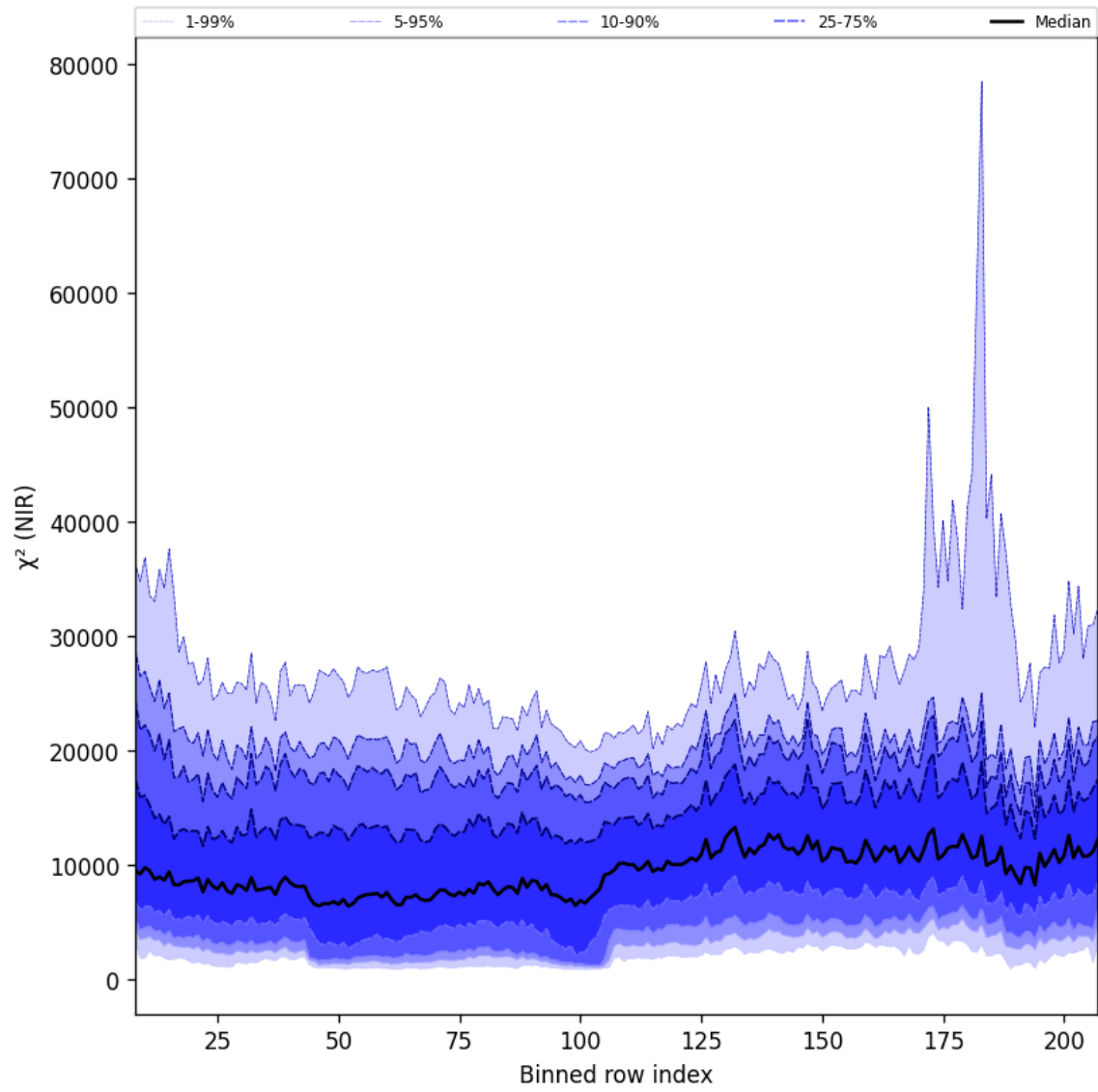
Figure 40: Along track statistics of “ \chi^2 (NIR)” for 2025-03-24 to 2025-03-26
