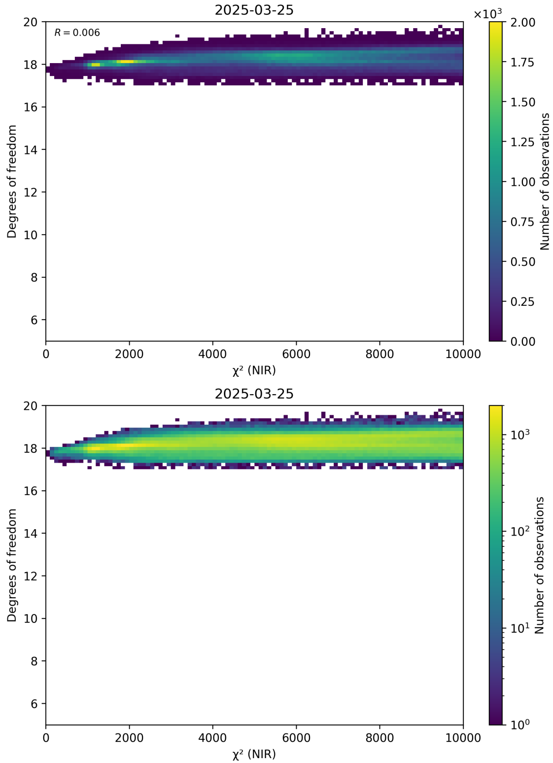
Figure 44: Scatter density plot of “ \chi^2 (NIR)” against “Degrees of freedom” for 2025-03-24 to 2025-03-26.
