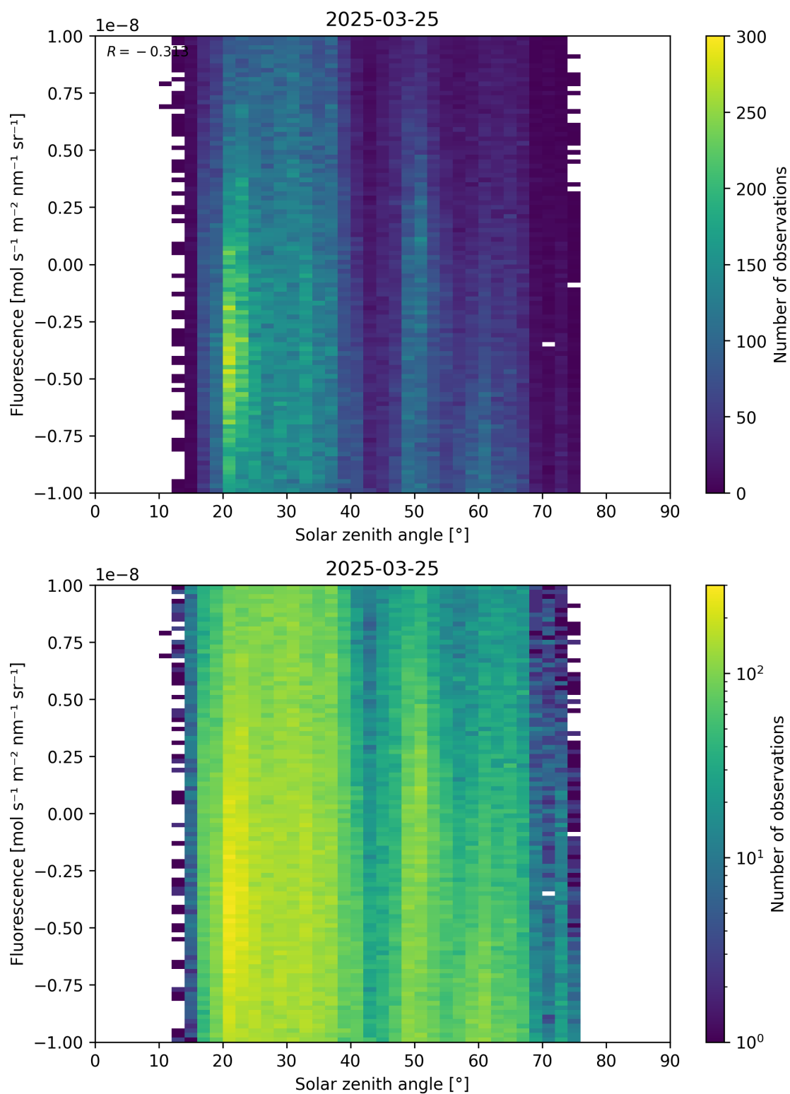
Figure 97: Scatter density plot of “Solar zenith angle” against “Fluorescence” for 2025-03-24 to 2025-03-26.
