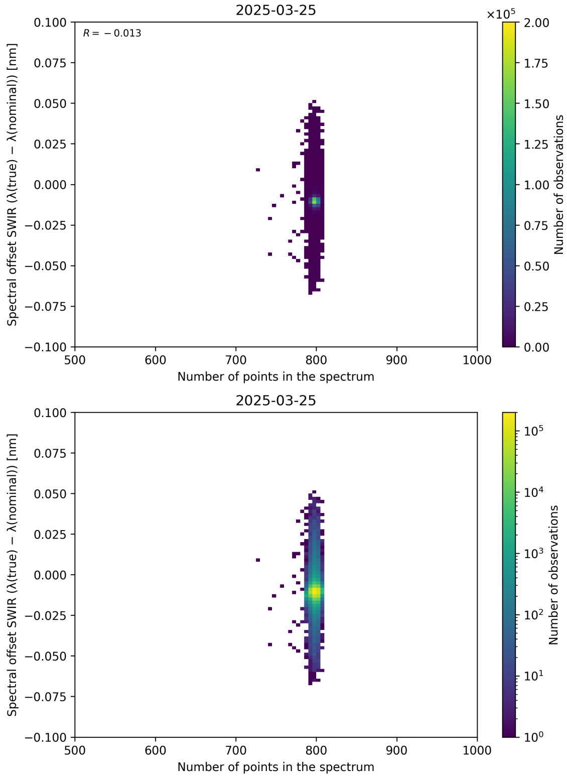
Figure 93: Scatter density plot of “Number of points in the spectrum” against “Spectral offset SWIR ( \lambda_{\text{true}} - \lambda_{\text{nominal}} )” for 2025-03-24 to 2025-03-26.
