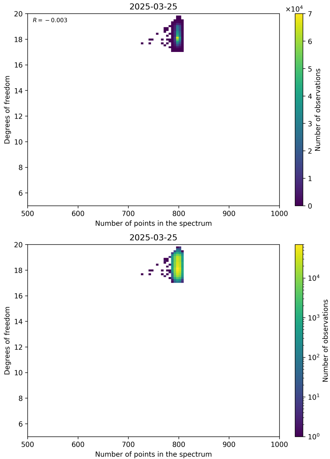
Figure 90: Scatter density plot of “Number of points in the spectrum” against “Degrees of freedom” for 2025-03-24 to 2025-03-26.
