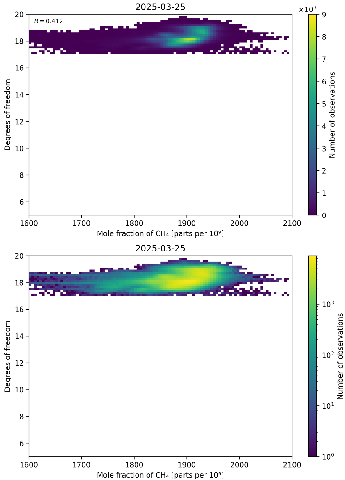
Figure 72: Scatter density plot of “Mole fraction of CH 4 ” against “Degrees of freedom” for 2025-03-24 to 2025-03-26.
