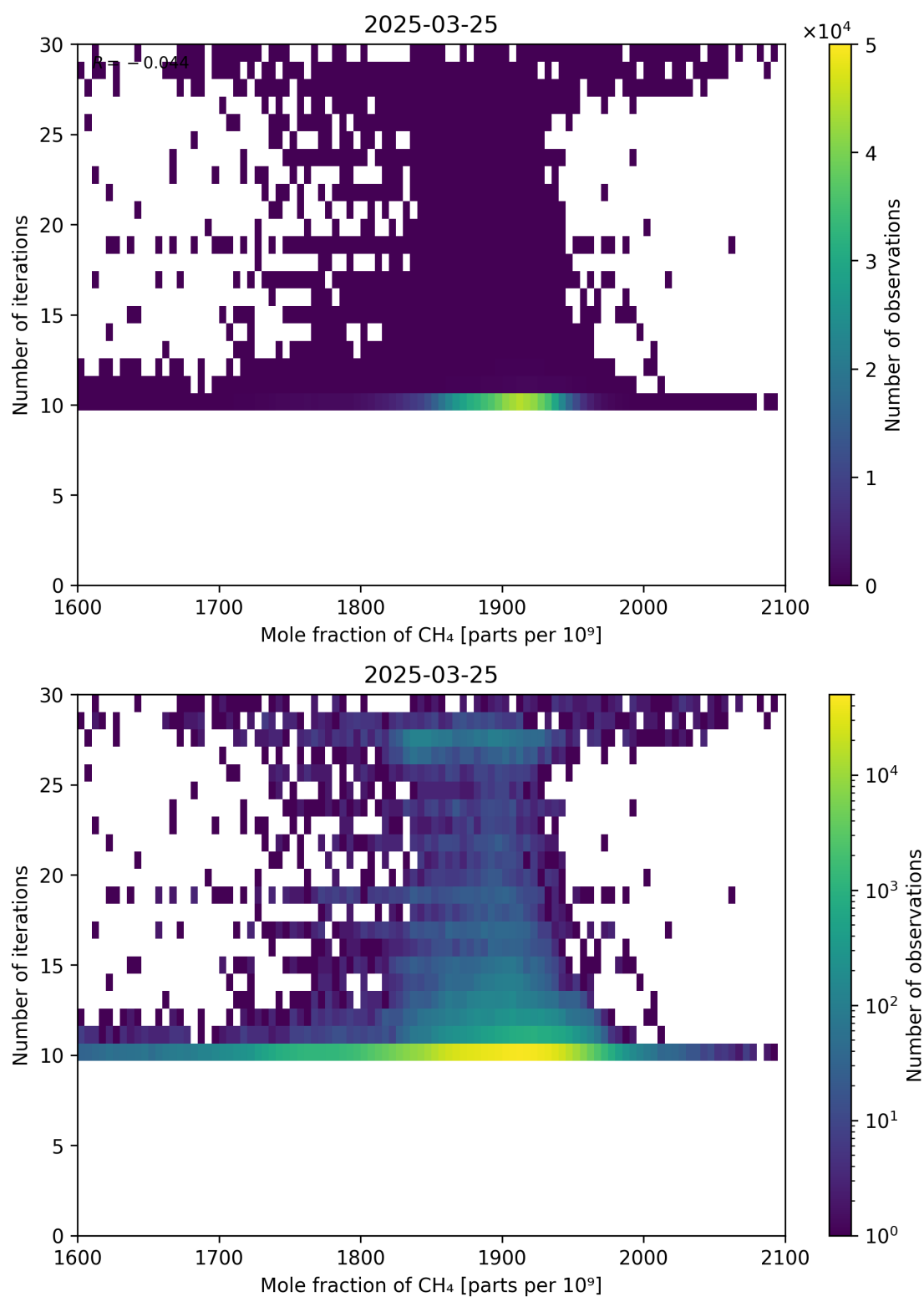
Figure 76: Scatter density plot of “Mole fraction of CH 4 ” against “Number of iterations” for 2025-03-24 to 2025-03-26.
