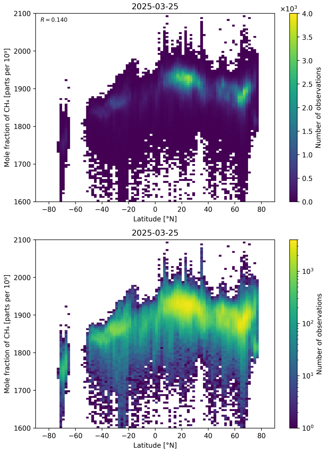
Figure 57: Scatter density plot of “Latitude” against “Mole fraction of CH 4 ” for 2025-03-24 to 2025-03-26.
