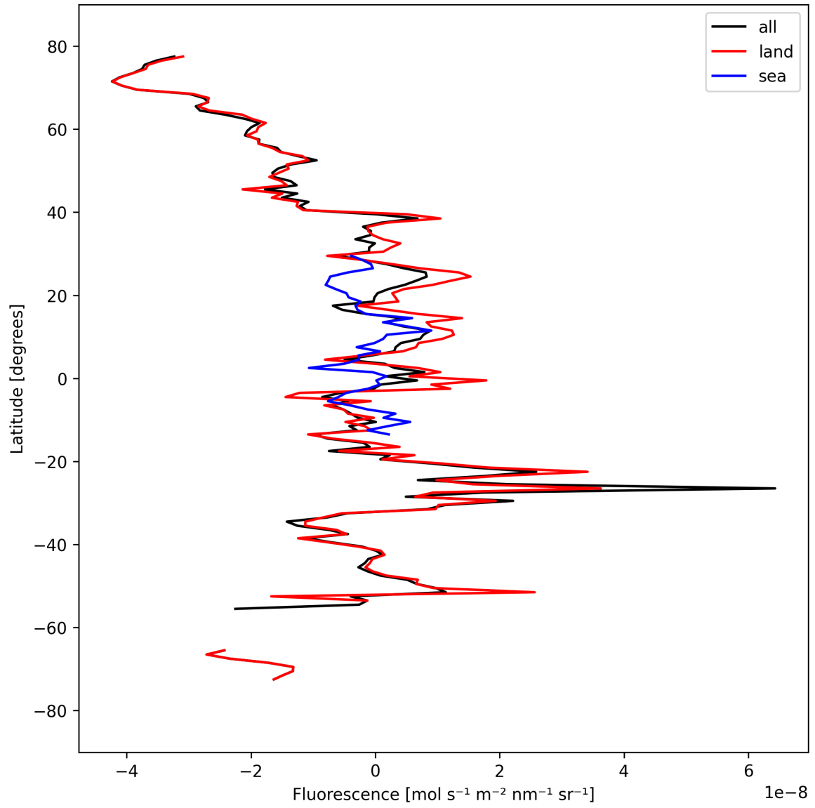
Figure 21: Zonal average of “Fluorescence” for 2025-03-24 to 2025-03-26.
