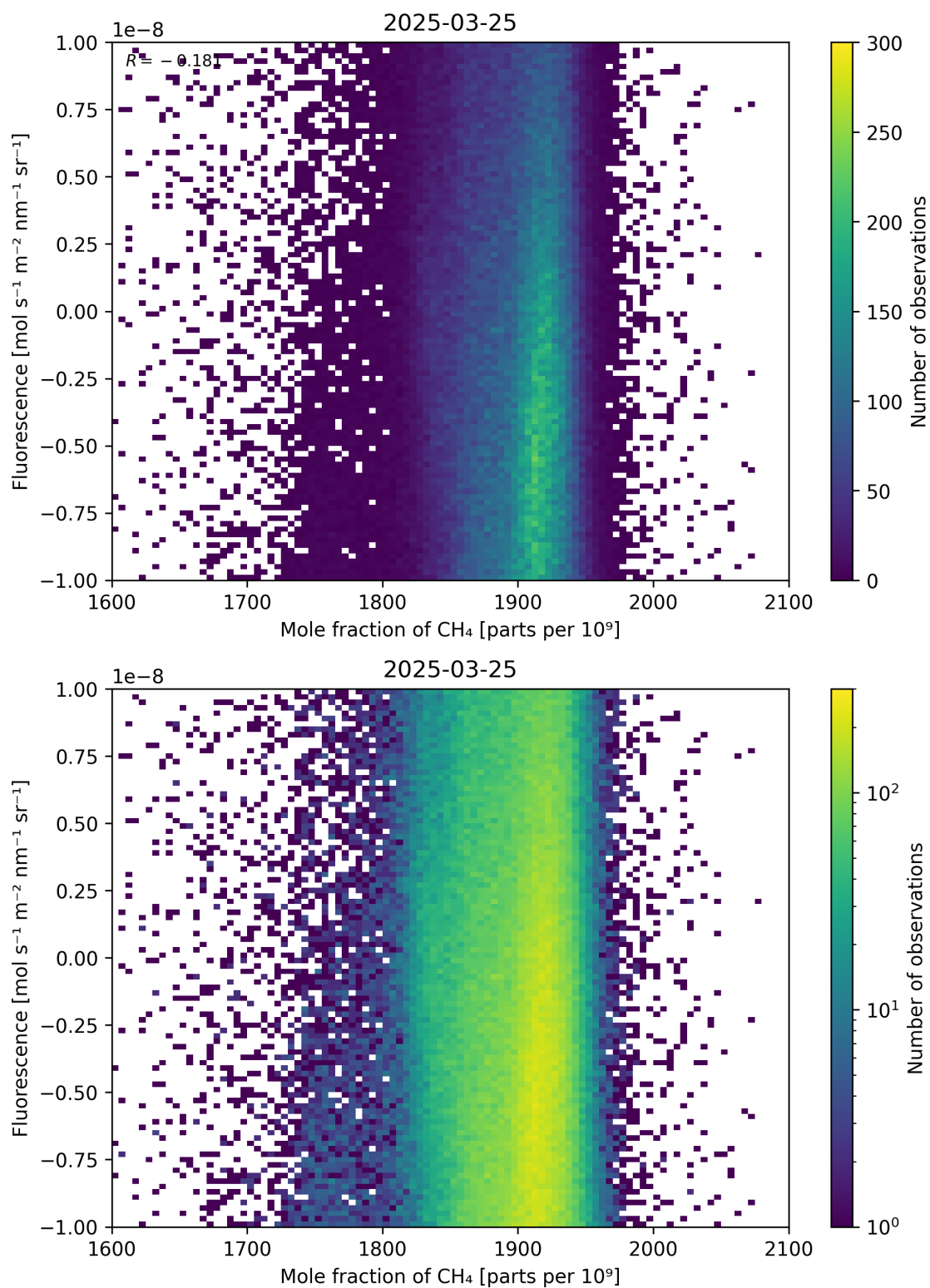
Figure 73: Scatter density plot of “Mole fraction of \text{CH}_4 ” against “Fluorescence” for 2025-03-24 to 2025-03-26.
