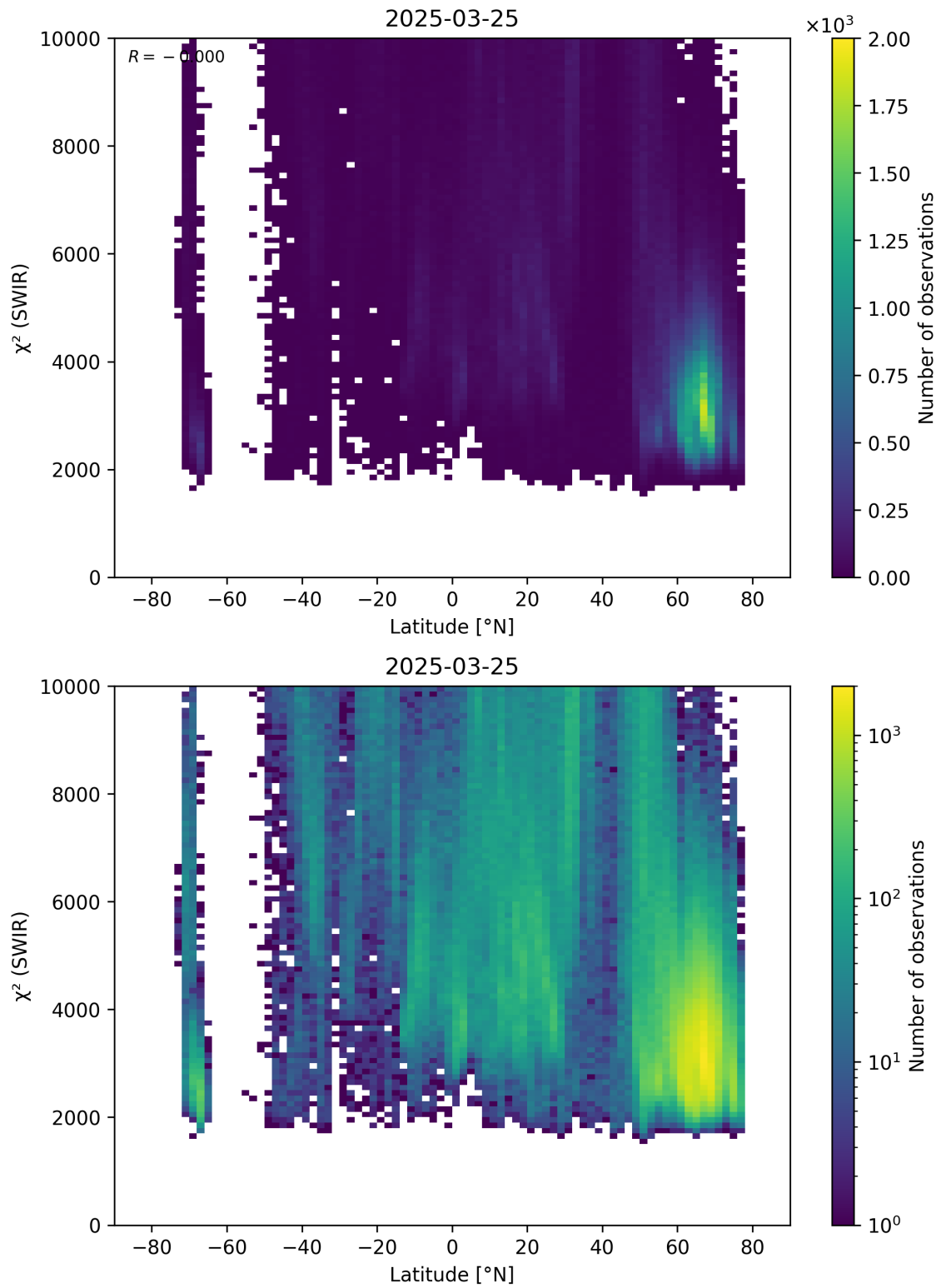
Figure 54: Scatter density plot of “Latitude” against “ \chi^2 (SWIR)” for 2025-03-24 to 2025-03-26.
