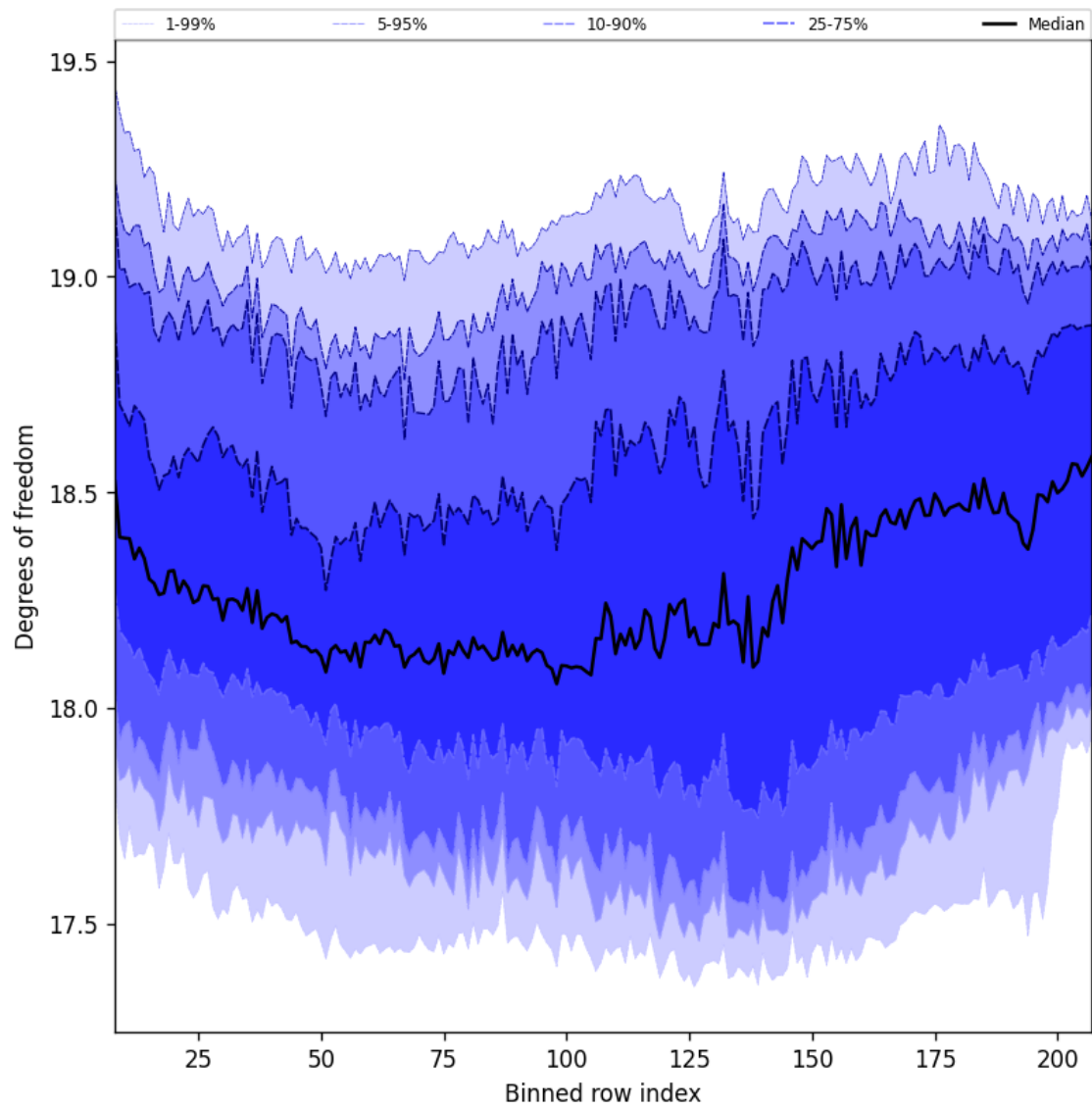
Figure 41: Along track statistics of “Degrees of freedom” for 2025-03-24 to 2025-03-26
