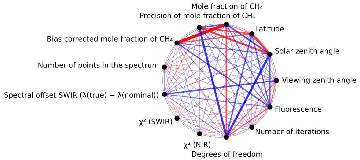
Figure 1: Map of correlation graph for 2025-03-24 to 2025-03-26.
