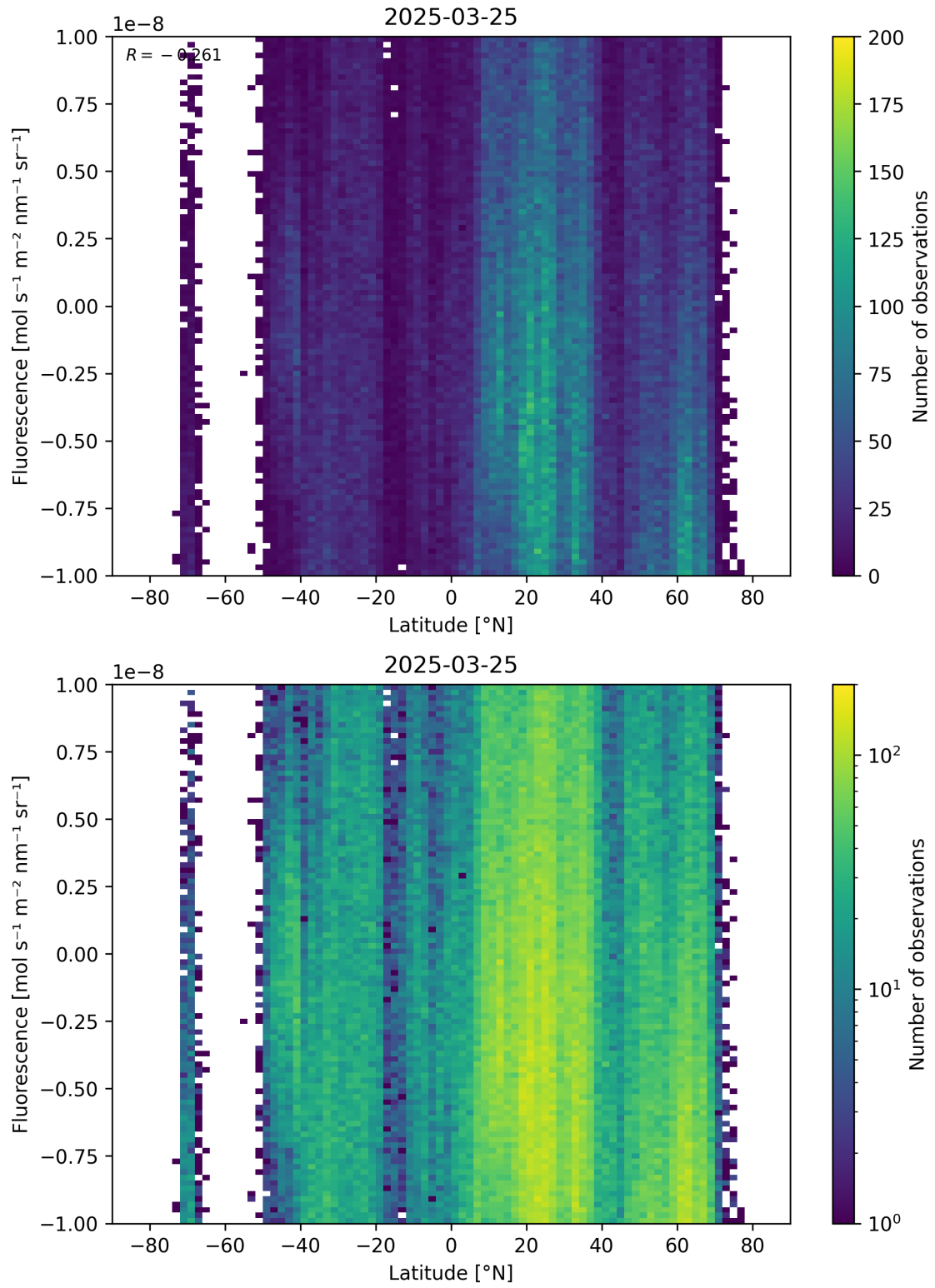
Figure 56: Scatter density plot of “Latitude” against “Fluorescence” for 2025-03-24 to 2025-03-26.
